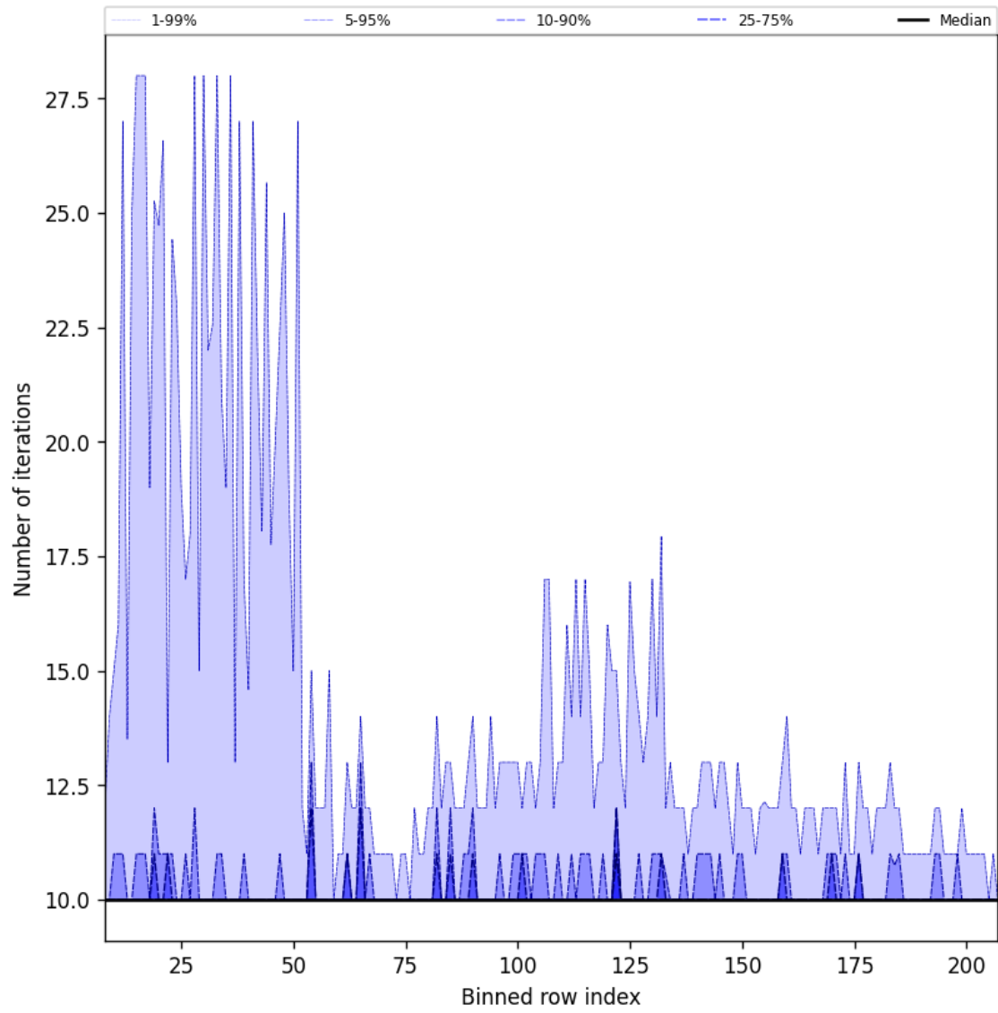
Figure 42: Along track statistics of “Number of iterations” for 2025-05-21 to 2025-05-23
