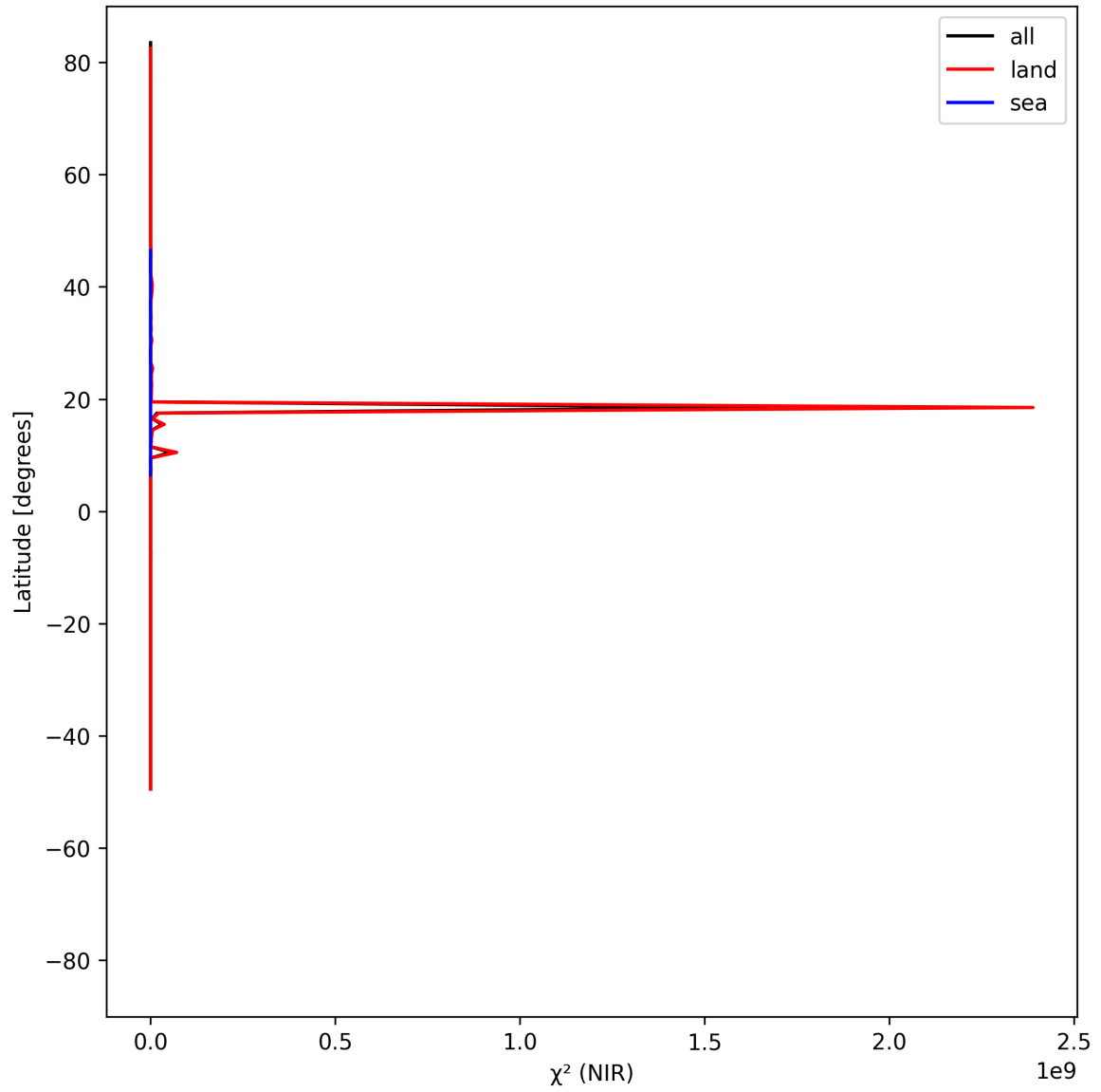
Figure 18: Zonal average of “ \chi^2 (NIR)” for 2025-05-21 to 2025-05-23.
