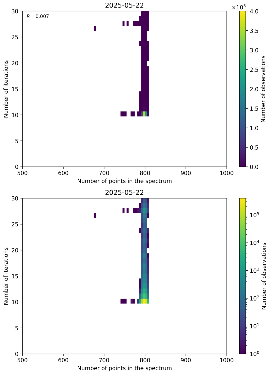
Figure 92: Scatter density plot of “Number of points in the spectrum” against “Number of iterations” for 2025-05-21 to 2025-05-23.
