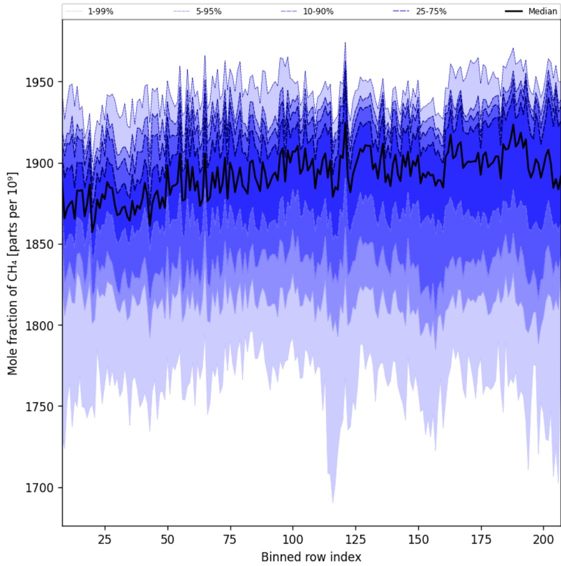
Figure 34: Along track statistics of “Mole fraction of CH 4 ” for 2025-05-21 to 2025-05-23
