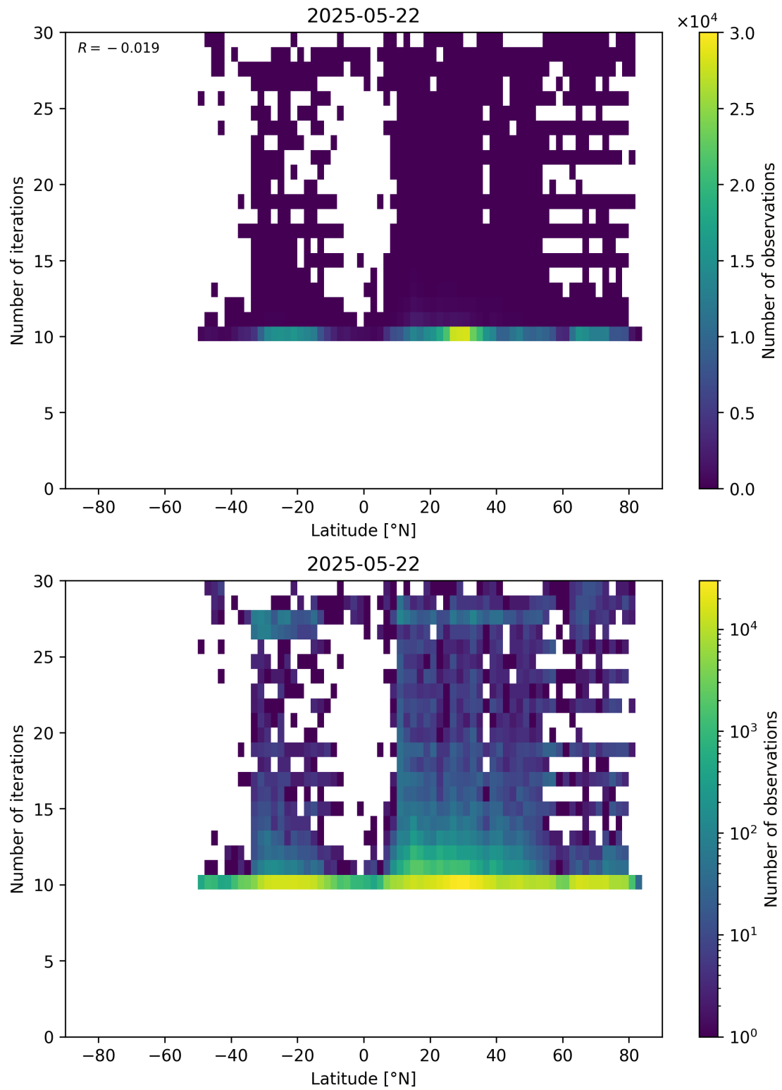
Figure 60: Scatter density plot of “Latitude” against “Number of iterations” for 2025-05-21 to 2025-05-23.
