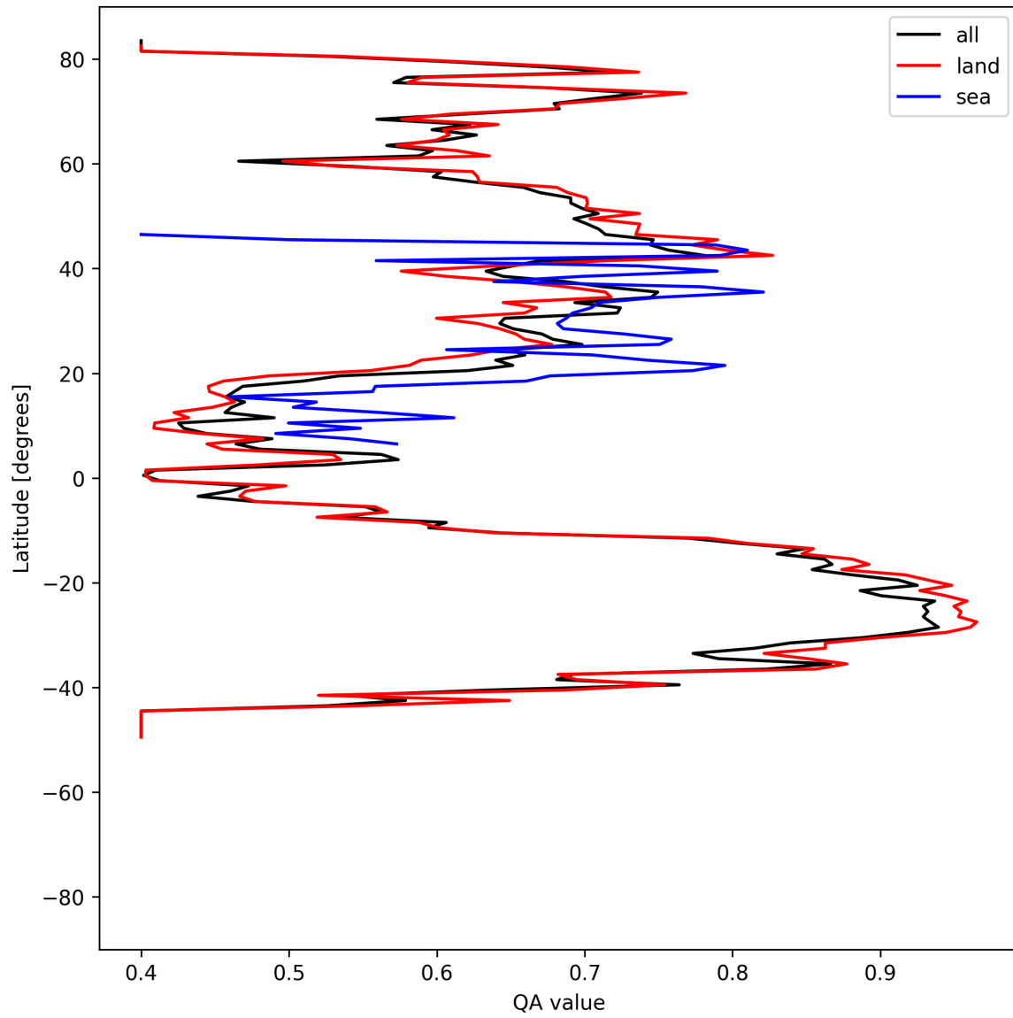
Figure 11: Zonal average of “QA value” for 2025-05-21 to 2025-05-23.
