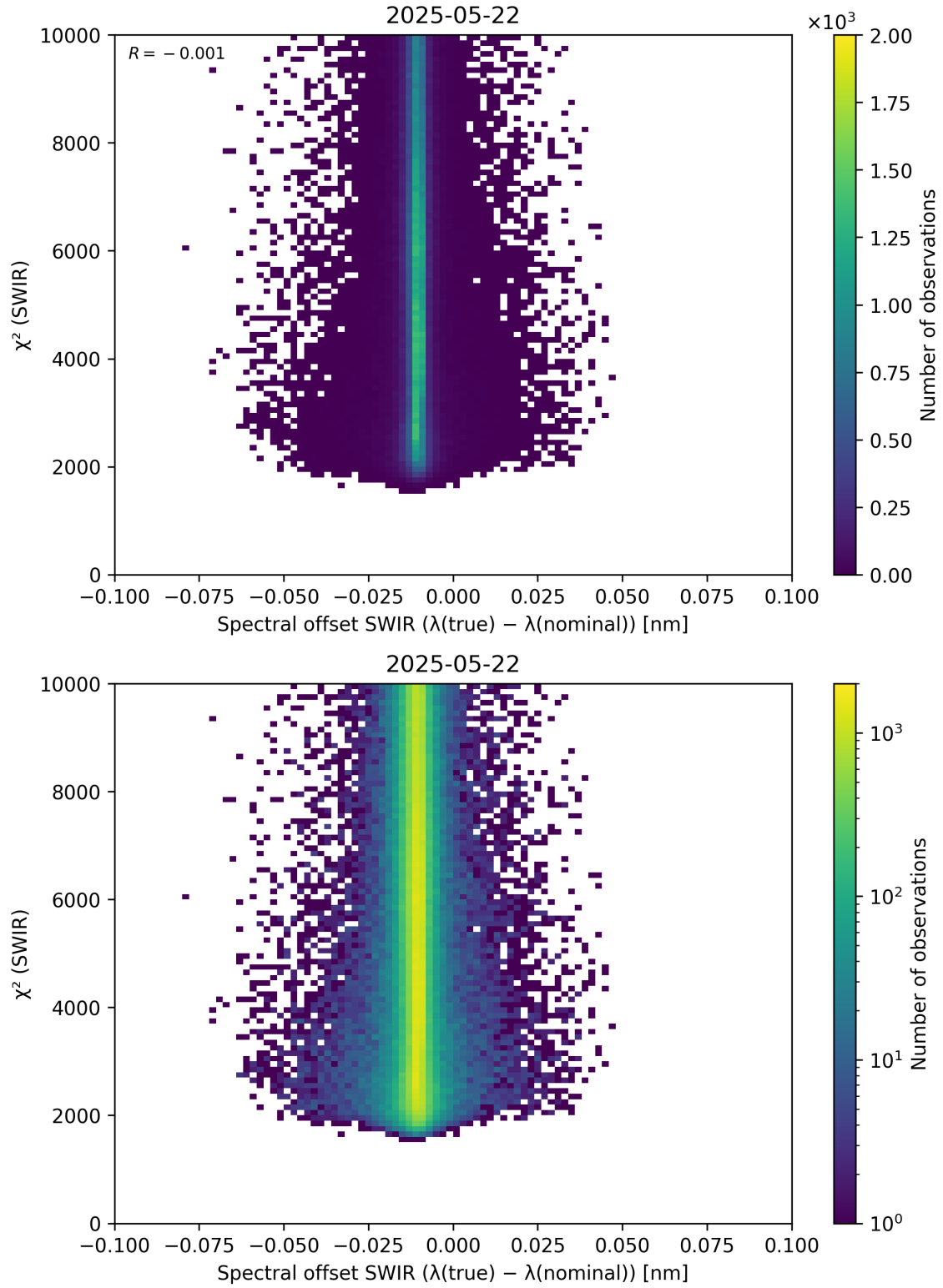
Figure 118: Scatter density plot of “Spectral offset SWIR ( \lambda_{\text{true}} - \lambda_{\text{nominal}} )” against “ \chi^2 (SWIR)” for 2025-05-21 to 2025-05-23.
