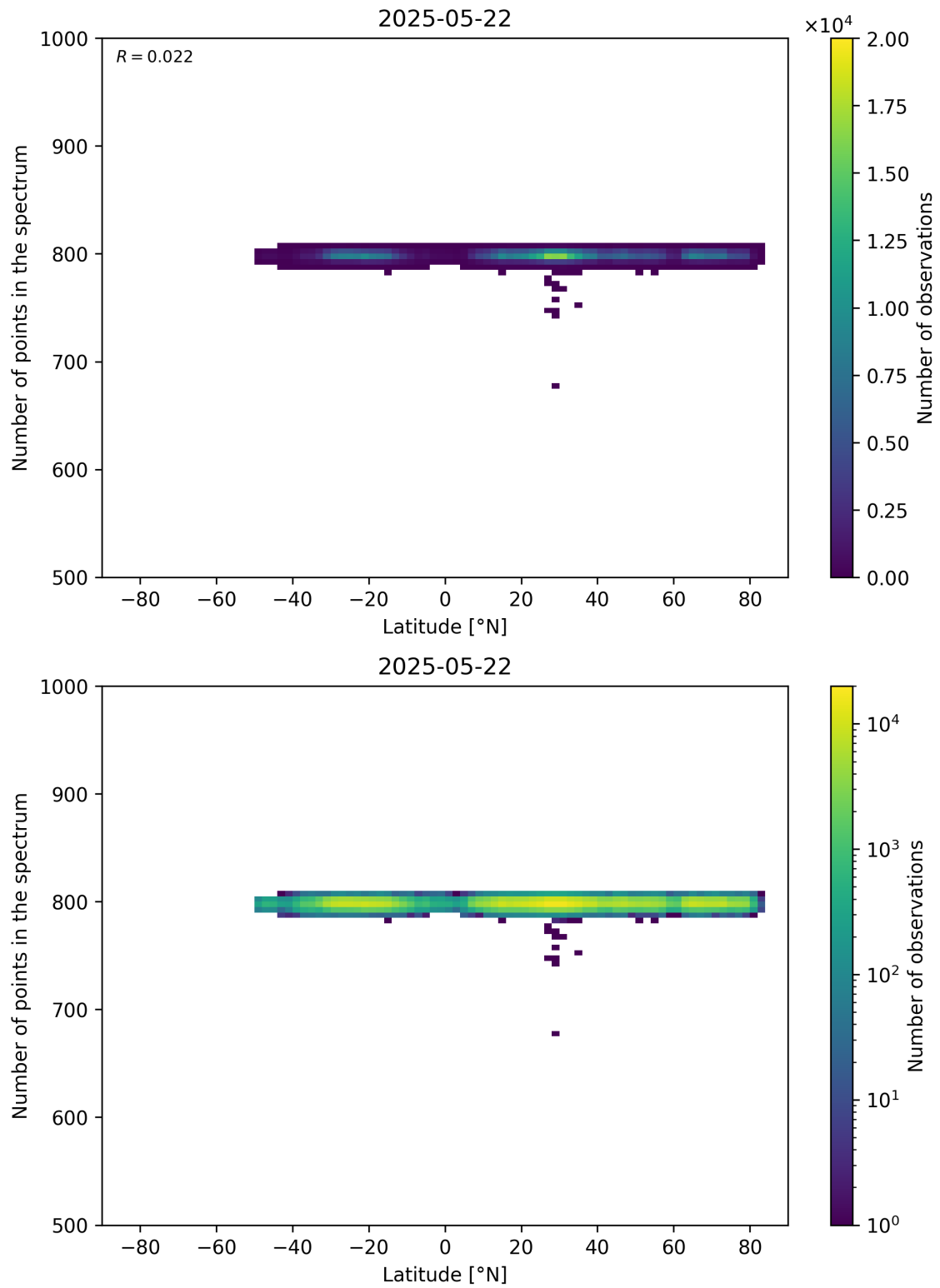
Figure 61: Scatter density plot of “Latitude” against “Number of points in the spectrum” for 2025-05-21 to 2025-05-23.
