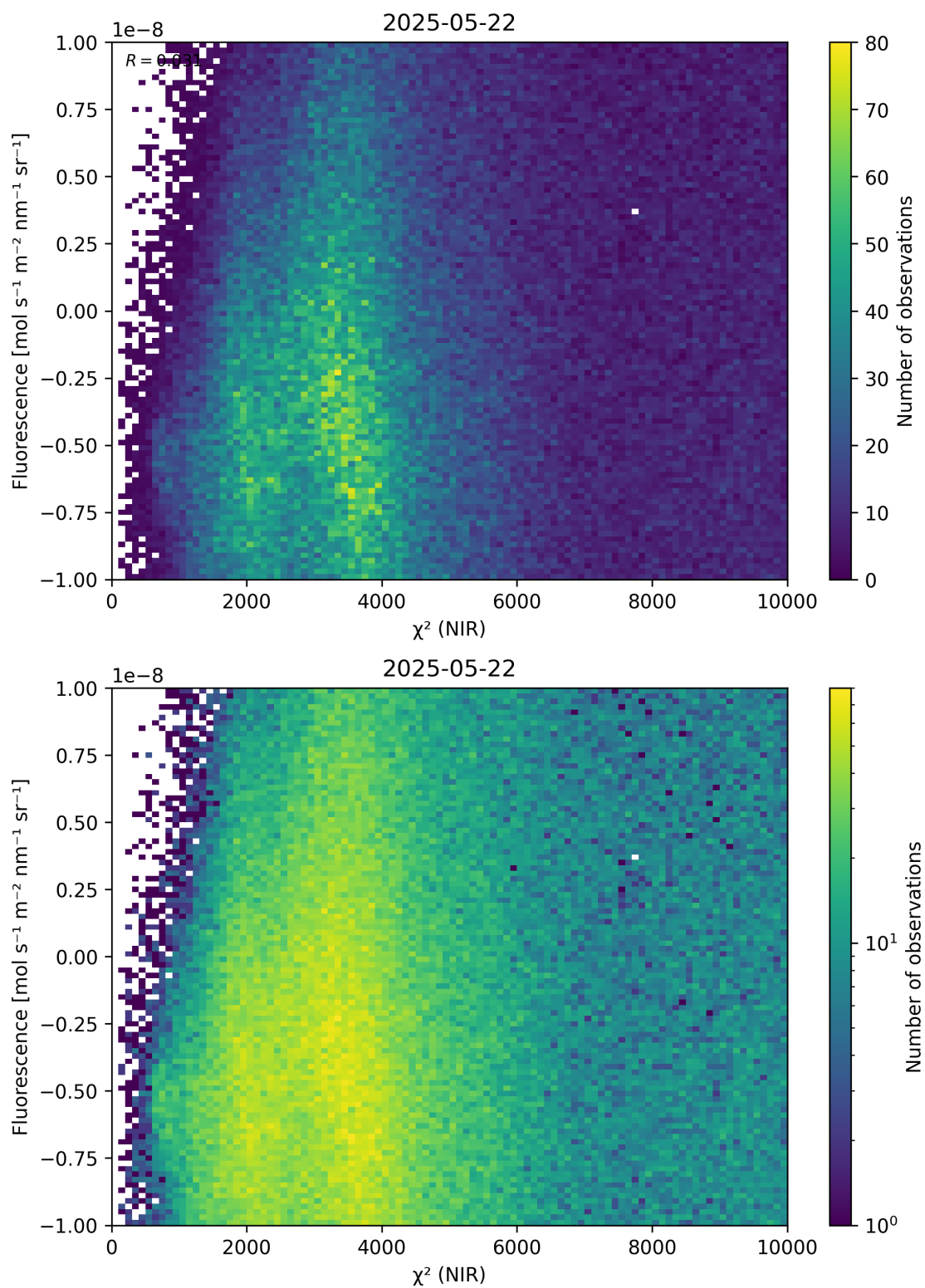
Figure 45: Scatter density plot of “ \chi^2 (NIR)” against “Fluorescence” for 2025-05-21 to 2025-05-23.
