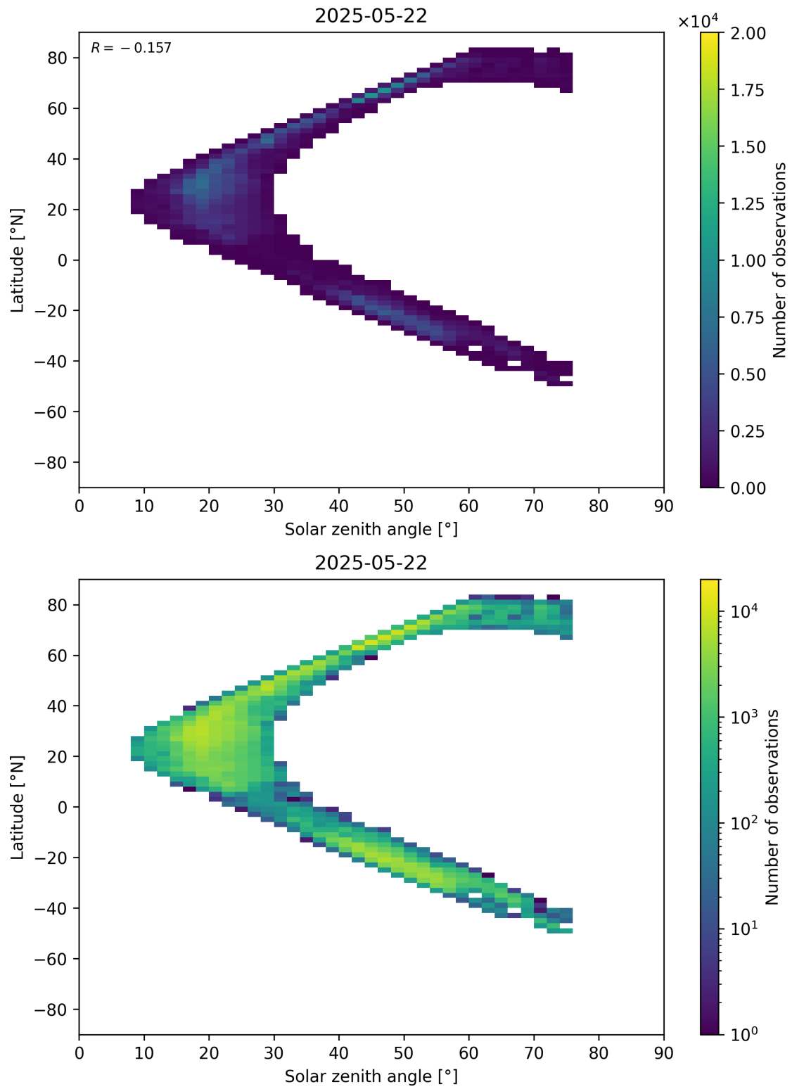
Figure 98: Scatter density plot of “Solar zenith angle” against “Latitude” for 2025-05-21 to 2025-05-23.
