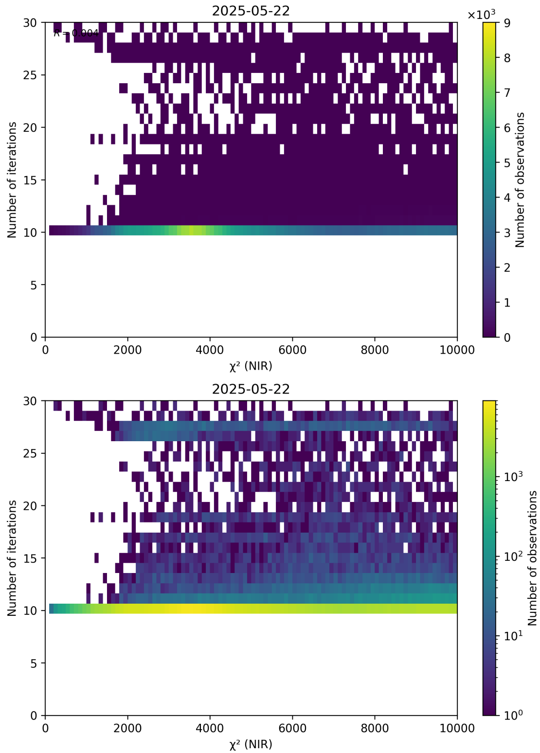
Figure 46: Scatter density plot of “ \chi^2 (NIR)” against “Number of iterations” for 2025-05-21 to 2025-05-23.
