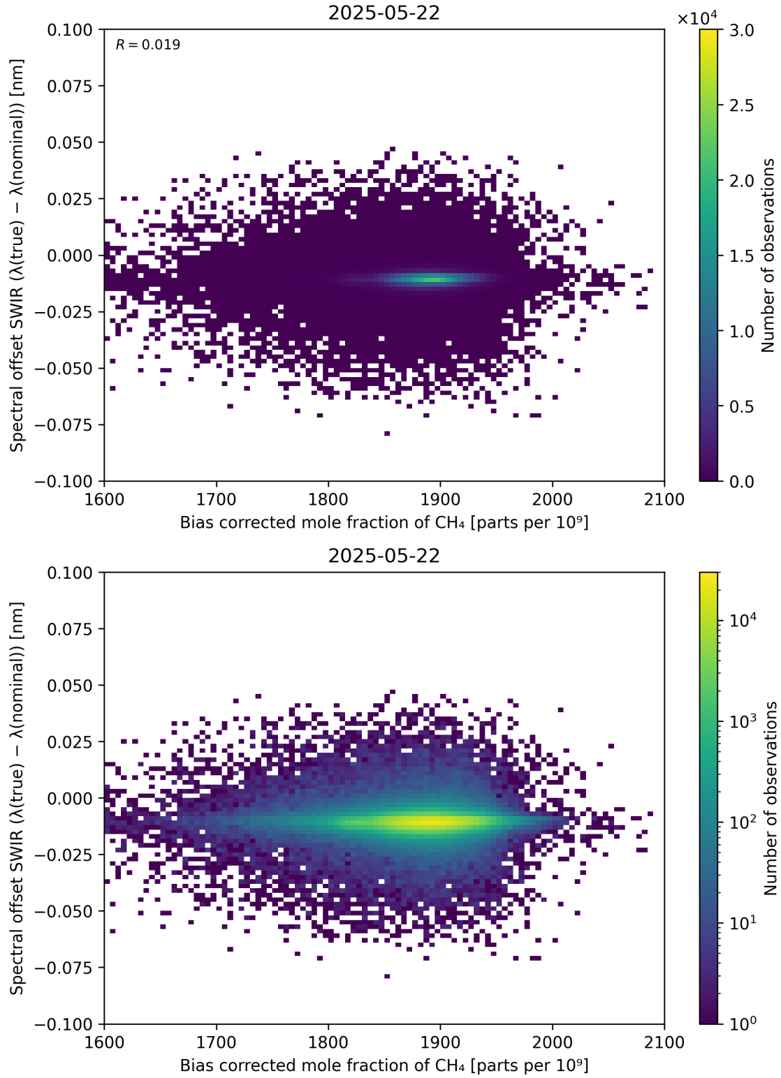
Figure 69: Scatter density plot of “Bias corrected mole fraction of \text{CH}_4 ” against “Spectral offset SWIR ( \lambda_{\text{true}} - \lambda_{\text{nominal}} )” for 2025-05-21 to 2025-05-23.
