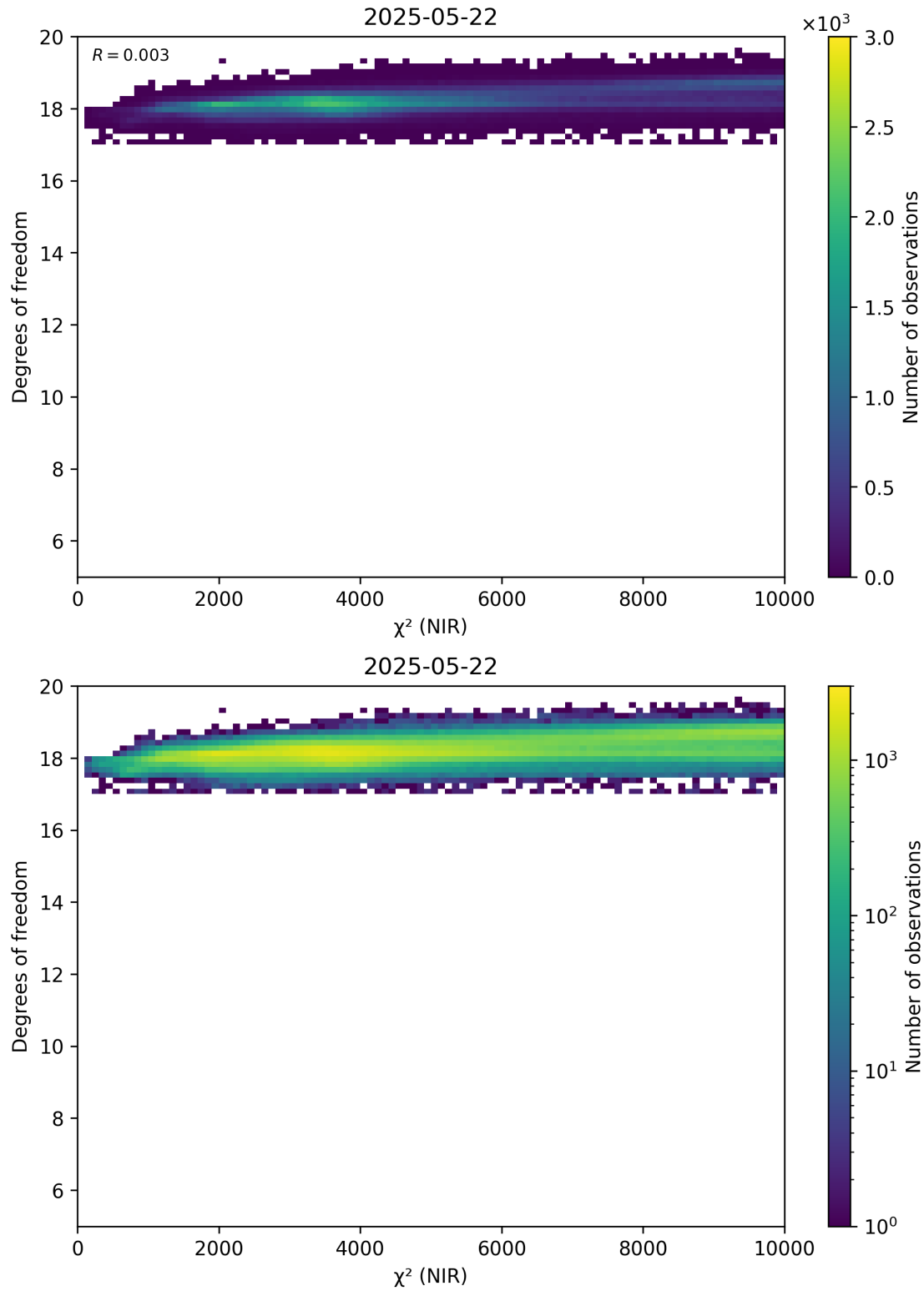
Figure 44: Scatter density plot of “ \chi^2 (NIR)” against “Degrees of freedom” for 2025-05-21 to 2025-05-23.
