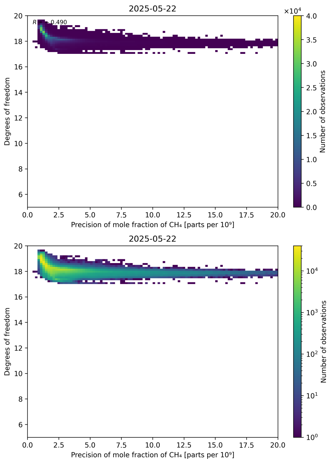
Figure 80: Scatter density plot of “Precision of mole fraction of CH 4 ” against “Degrees of freedom” for 2025-05-21 to 2025-05-23.
