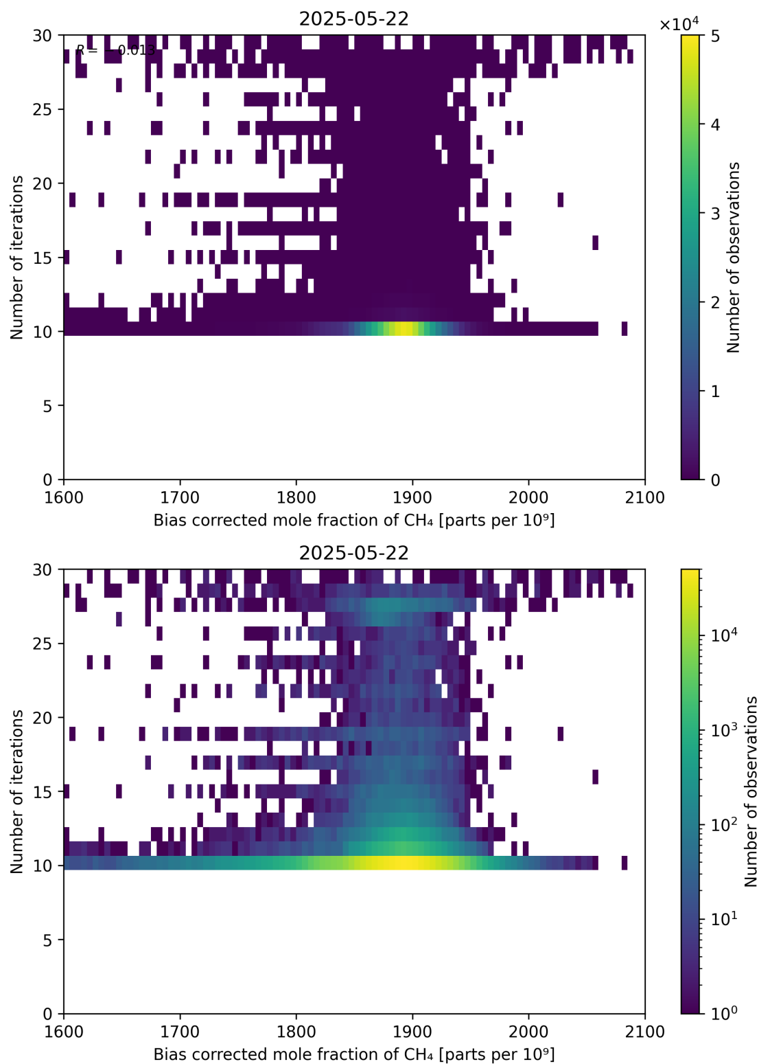
Figure 67: Scatter density plot of “Bias corrected mole fraction of \text{CH}_4 ” against “Number of iterations” for 2025-05-21 to 2025-05-23.
