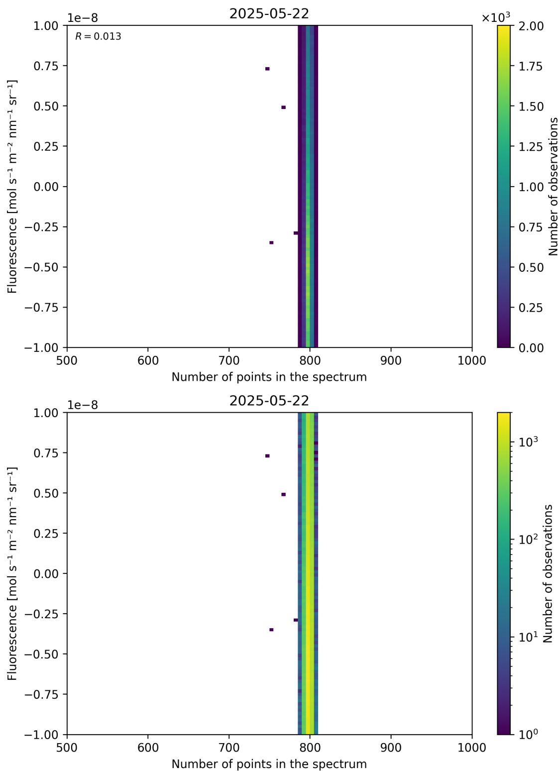
Figure 91: Scatter density plot of “Number of points in the spectrum” against “Fluorescence” for 2025-05-21 to 2025-05-23.
