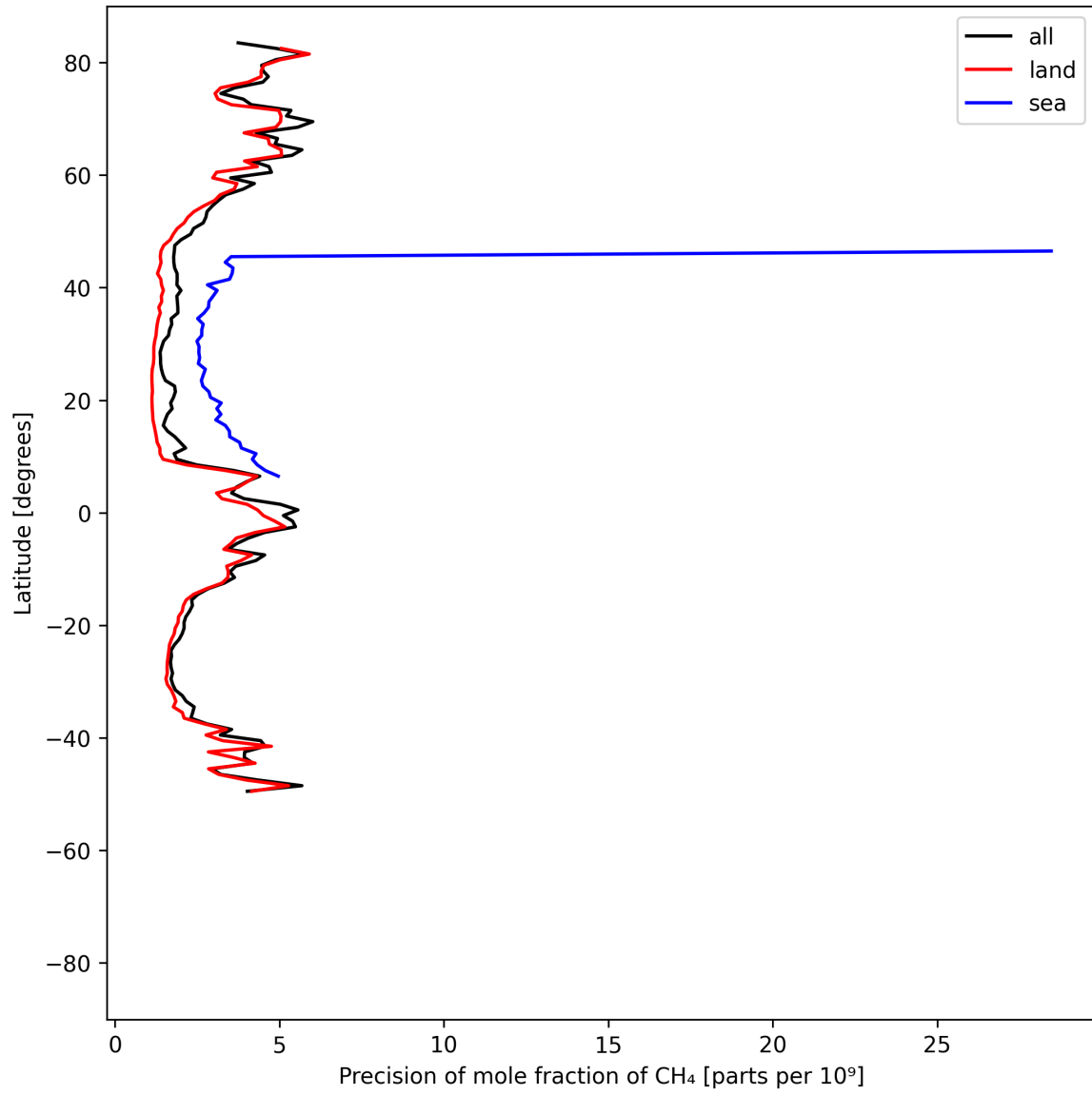
Figure 13: Zonal average of “Precision of mole fraction of CH 4 ” for 2025-05-21 to 2025-05-23.
