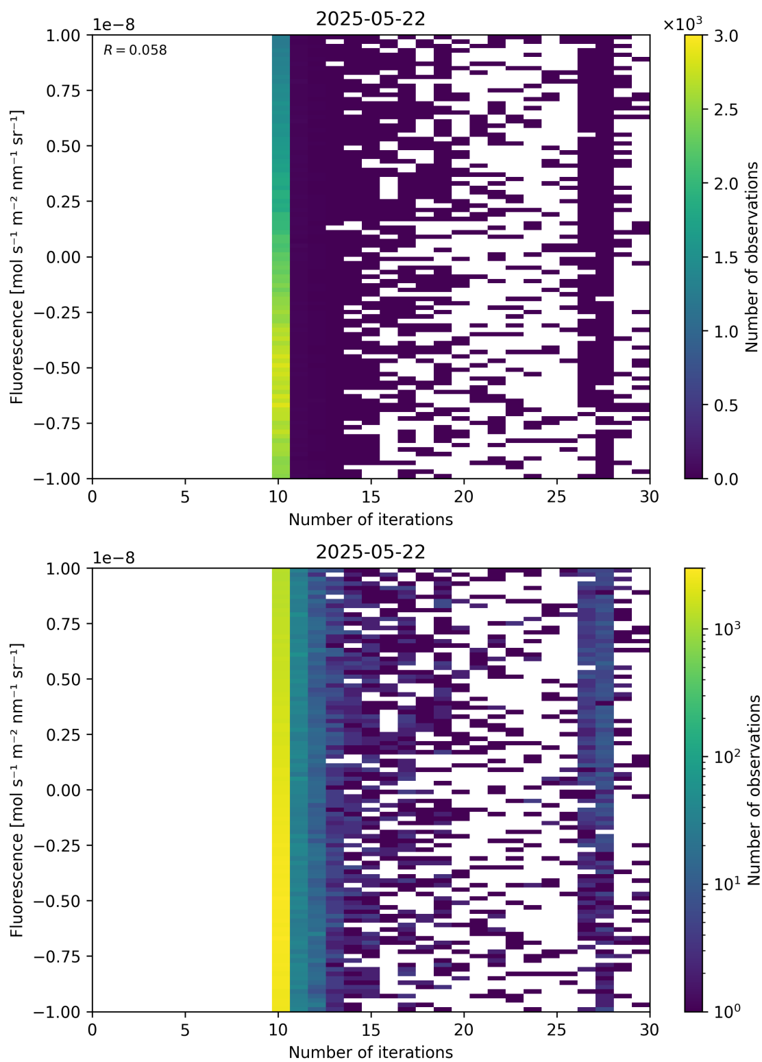
Figure 87: Scatter density plot of “Number of iterations” against “Fluorescence” for 2025-05-21 to 2025-05-23.
