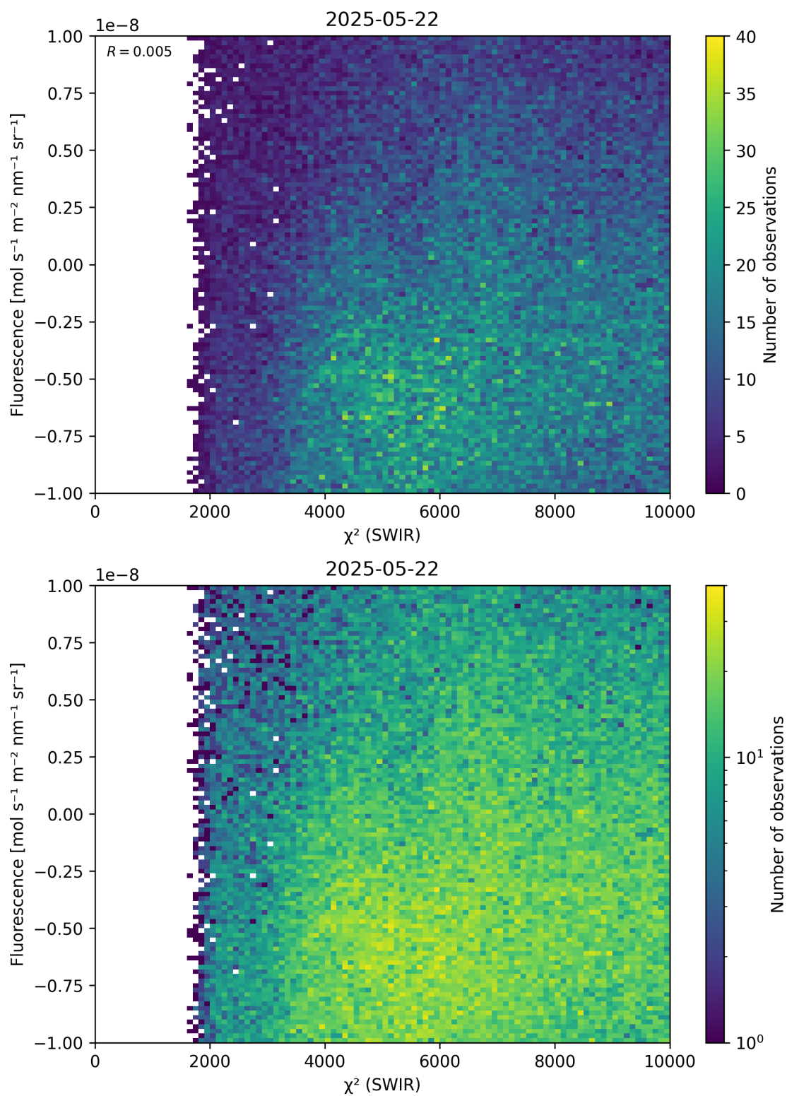
Figure 49: Scatter density plot of “ \chi^2 (SWIR)” against “Fluorescence” for 2025-05-21 to 2025-05-23.
