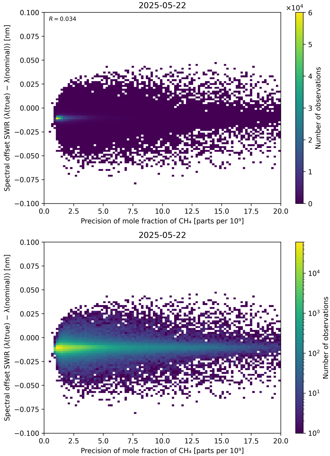
Figure 85: Scatter density plot of “Precision of mole fraction of CH 4 ” against “Spectral offset SWIR ( \lambda_{\text{true}} - \lambda_{\text{nominal}} )” for 2025-05-21 to 2025-05-23.
