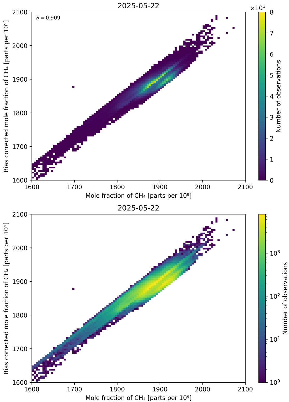
Figure 74: Scatter density plot of “Mole fraction of CH 4 ” against “Bias corrected mole fraction of CH 4 ” for 2025-05-21 to 2025-05-23.
