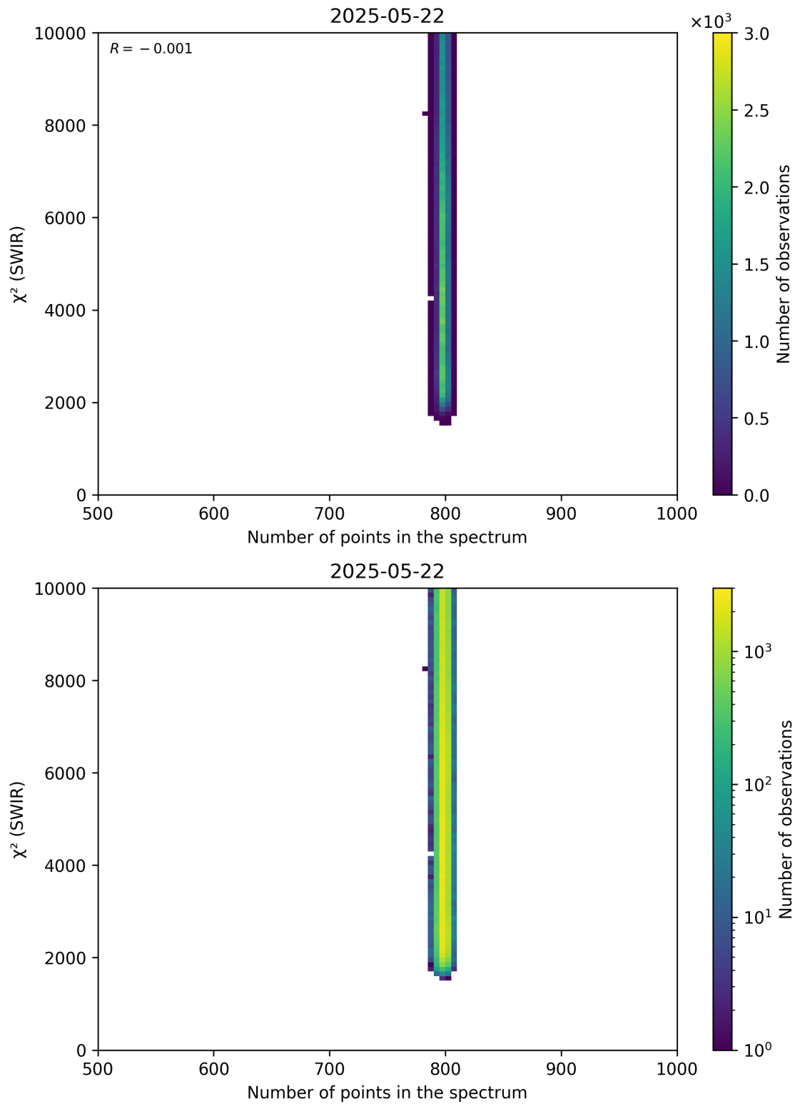
Figure 89: Scatter density plot of “Number of points in the spectrum” against “ \chi^2 (SWIR)” for 2025-05-21 to 2025-05-23.
