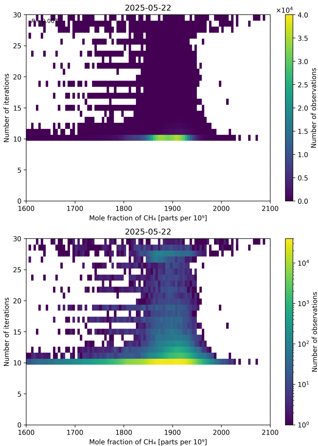
Figure 76: Scatter density plot of “Mole fraction of CH 4 ” against “Number of iterations” for 2025-05-21 to 2025-05-23.
