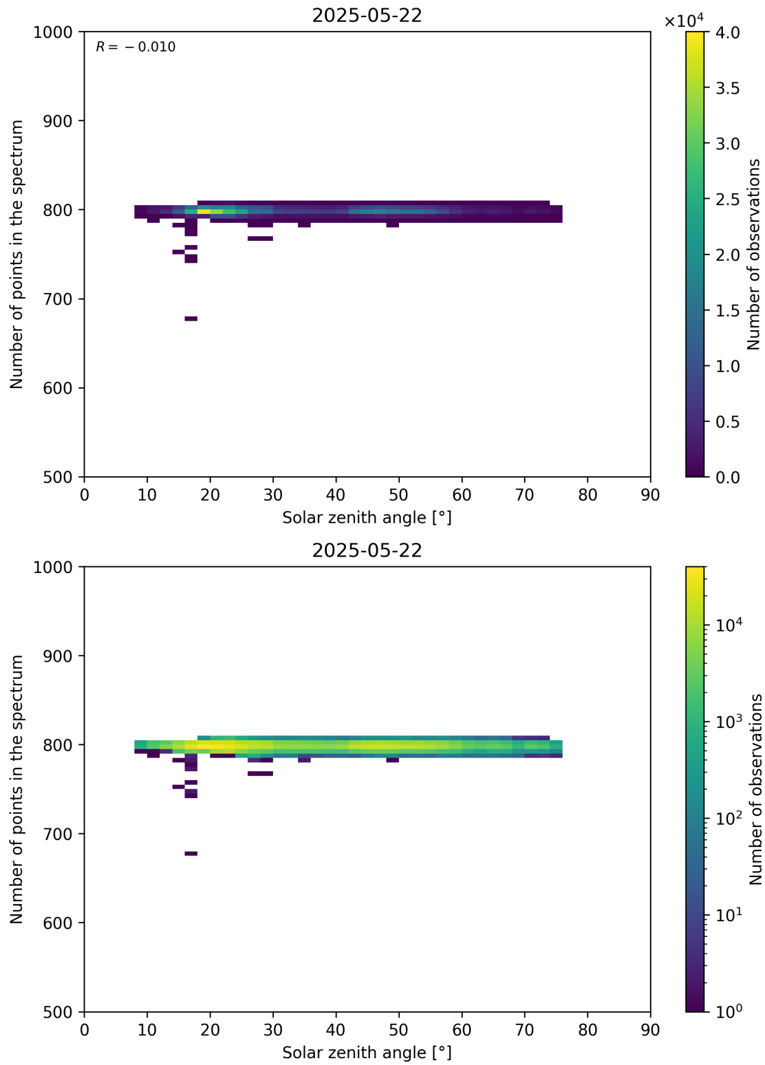
Figure 103: Scatter density plot of “Solar zenith angle” against “Number of points in the spectrum” for 2025-05-21 to 2025-05-23.
