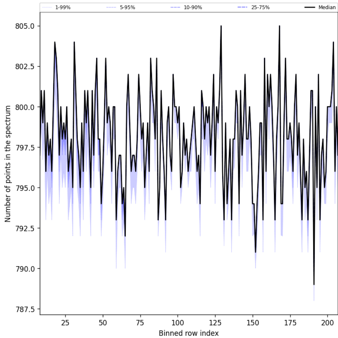
Figure 37: Along track statistics of “Number of points in the spectrum” for 2025-05-21 to 2025-05-23
