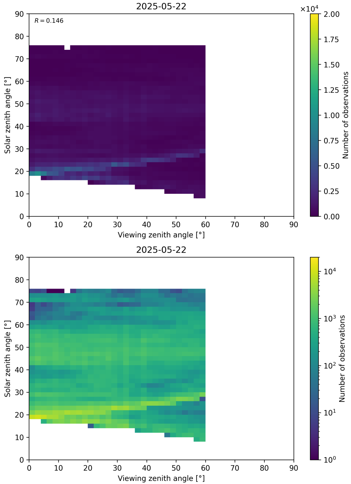
Figure 115: Scatter density plot of “Viewing zenith angle” against “Solar zenith angle” for 2025-05-21 to 2025-05-23.
