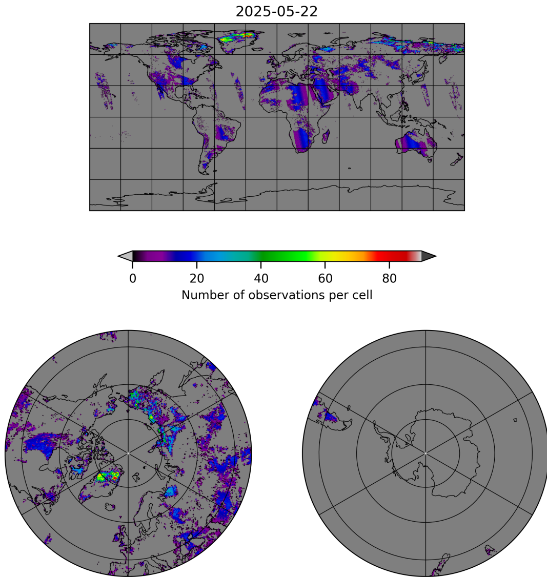
Figure 10: Map of the number of observations for 2025-05-21 to 2025-05-23
