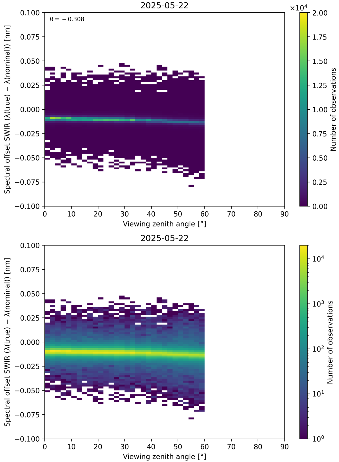
Figure 116: Scatter density plot of “Viewing zenith angle” against “Spectral offset SWIR ( \lambda_{\text{true}} - \lambda_{\text{nominal}} )” for 2025-05-21 to 2025-05-23.
