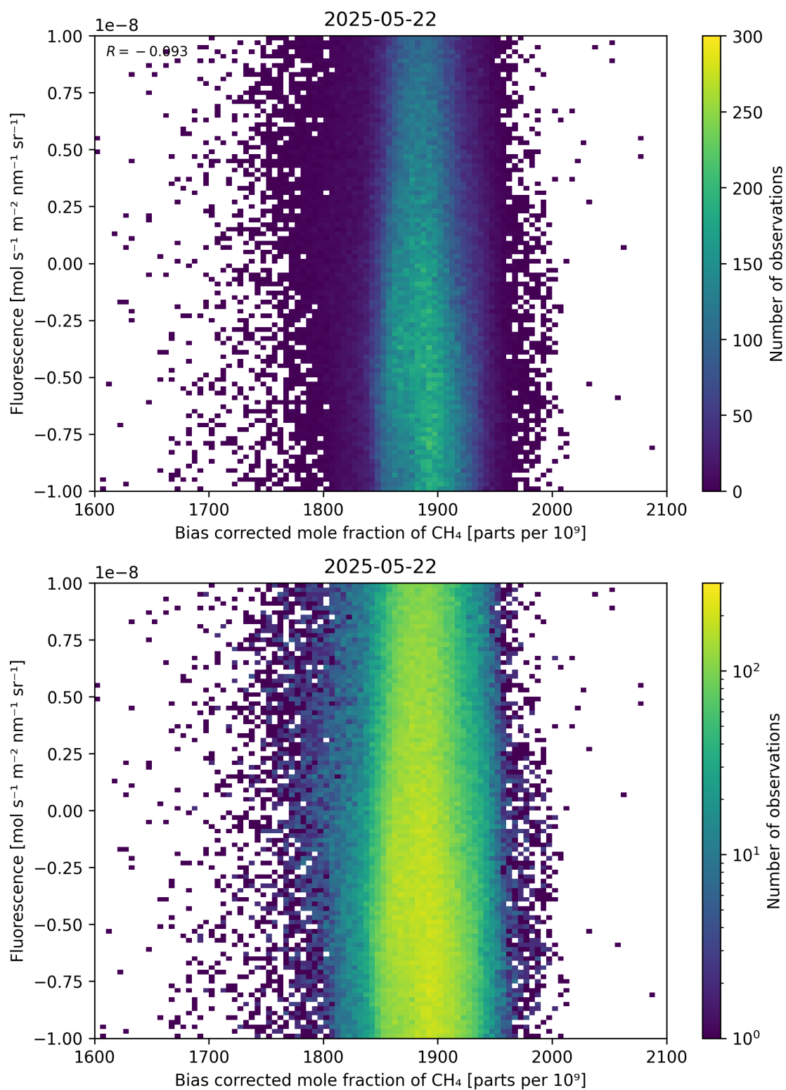
Figure 66: Scatter density plot of “Bias corrected mole fraction of CH 4 ” against “Fluorescence” for 2025-05-21 to 2025-05-23.
