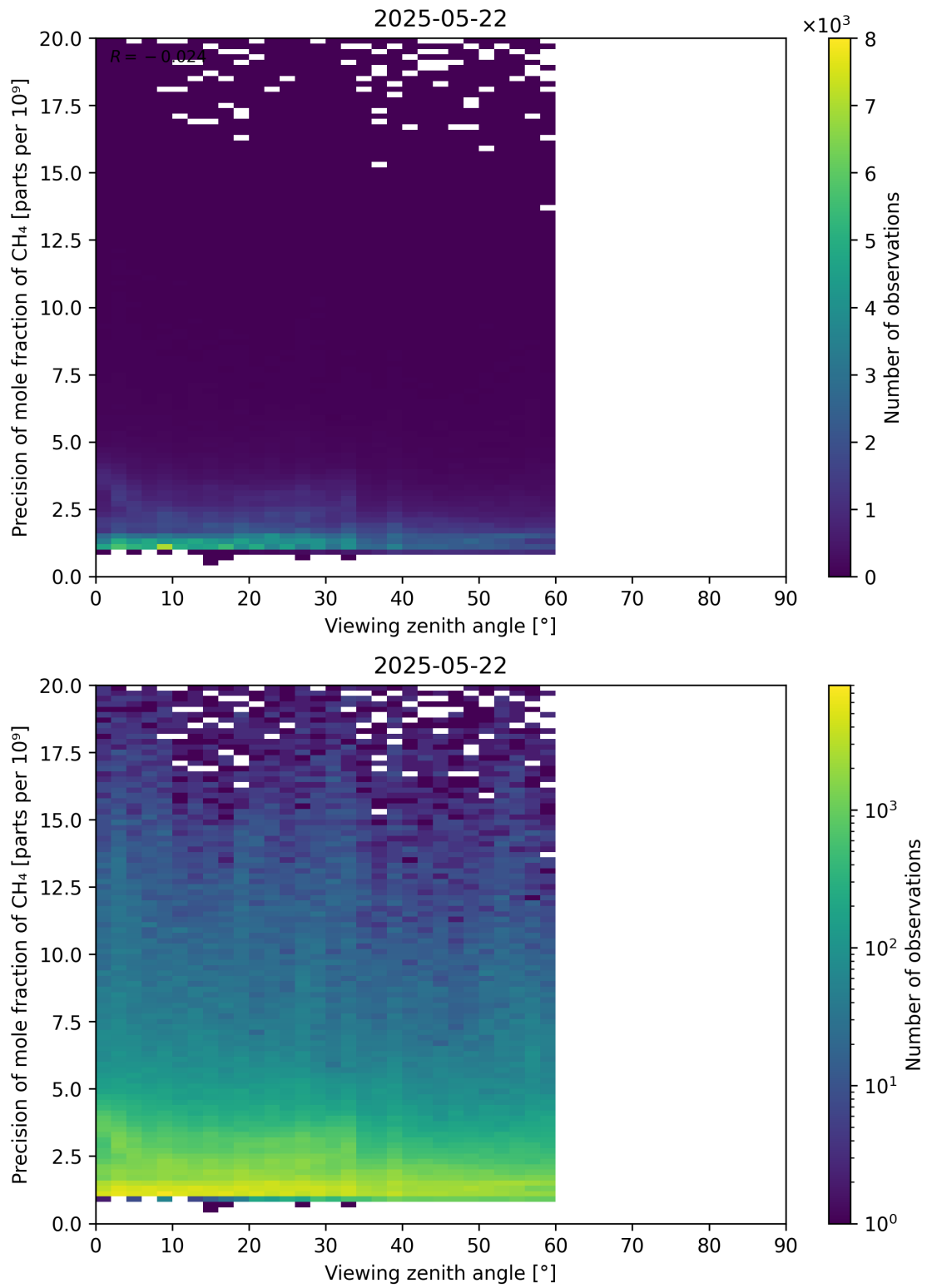
Figure 112: Scatter density plot of “Viewing zenith angle” against “Precision of mole fraction of CH 4 ” for 2025-05-21 to 2025-05-23.
