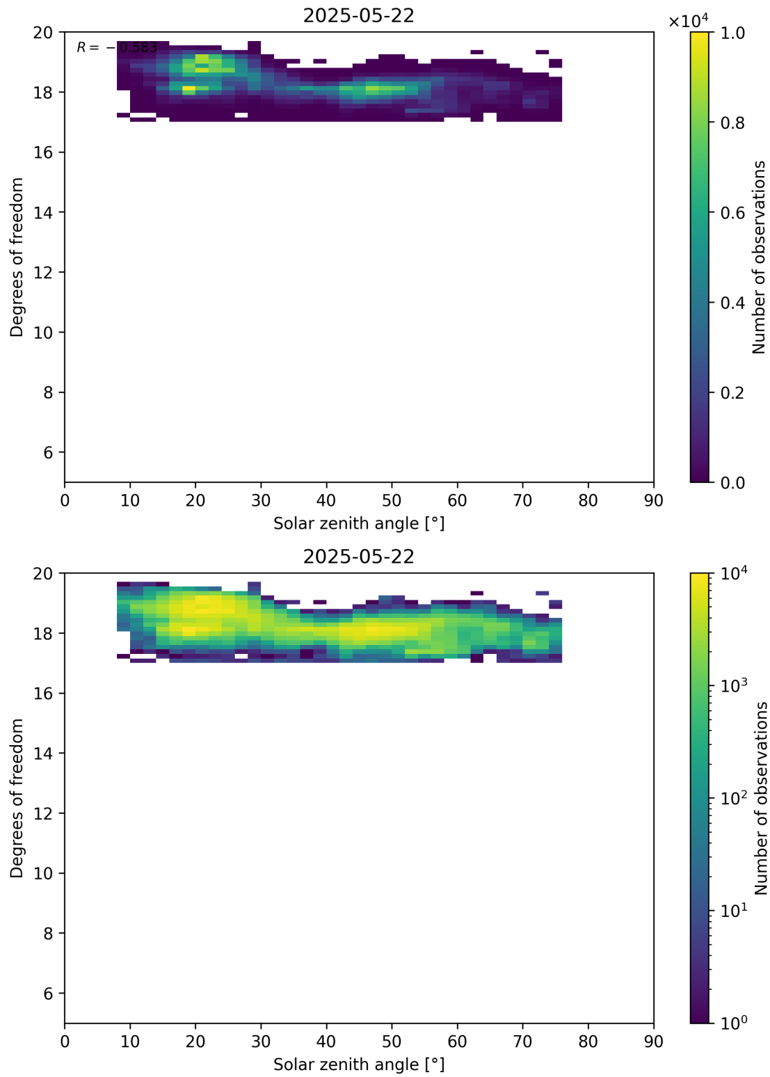
Figure 96: Scatter density plot of “Solar zenith angle” against “Degrees of freedom” for 2025-05-21 to 2025-05-23.
