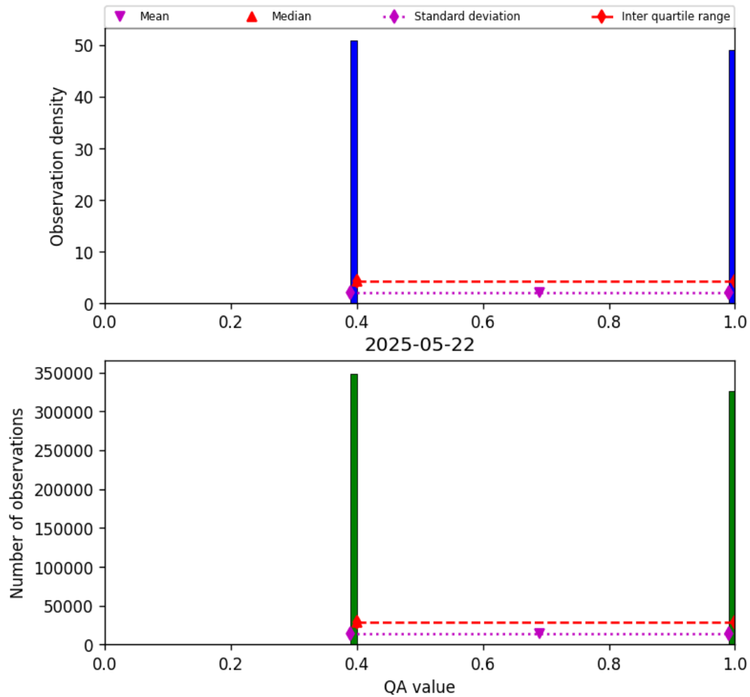
Figure 22: Histogram of “QA value” for 2025-05-21 to 2025-05-23
