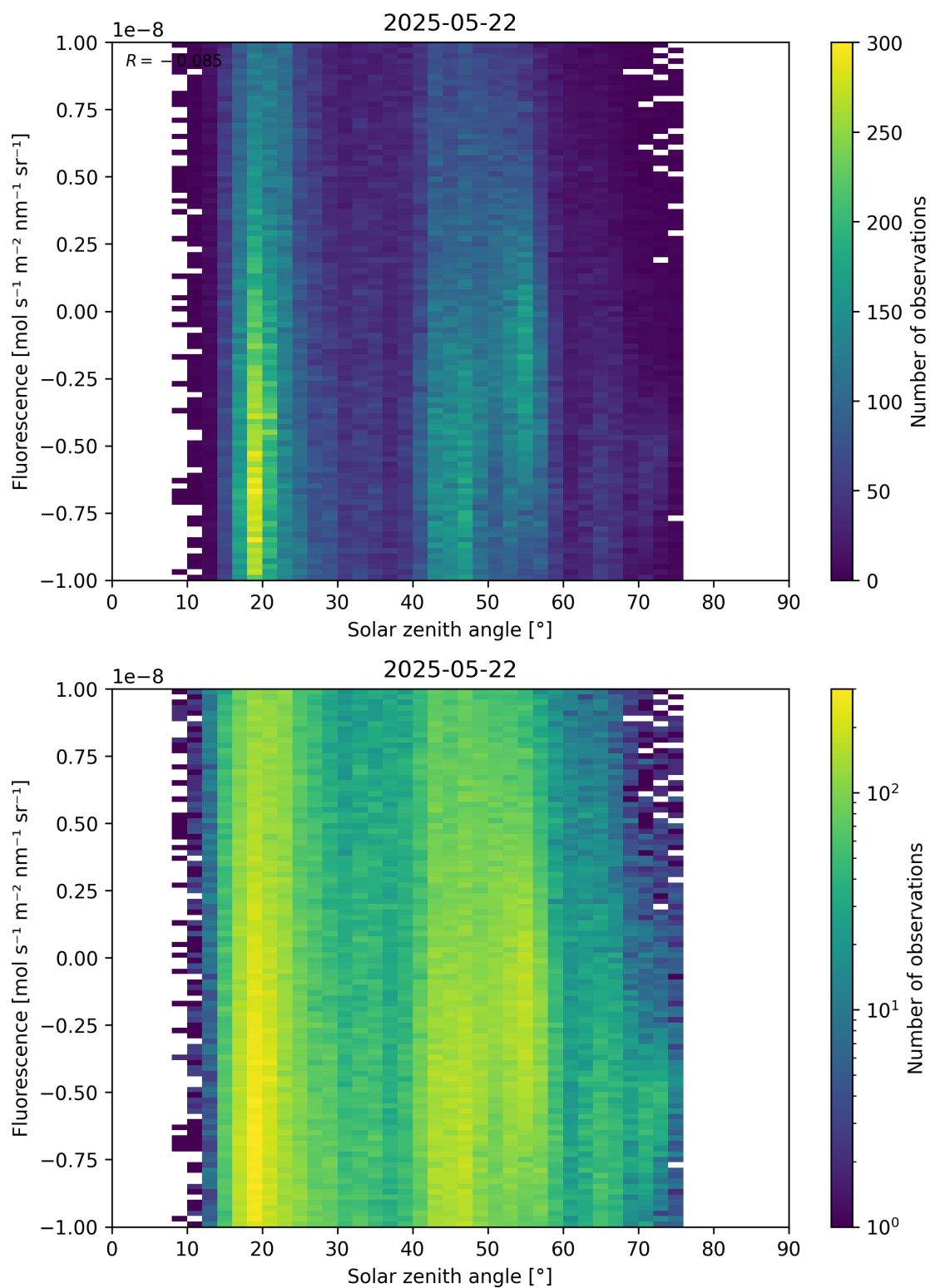
Figure 97: Scatter density plot of “Solar zenith angle” against “Fluorescence” for 2025-05-21 to 2025-05-23.
