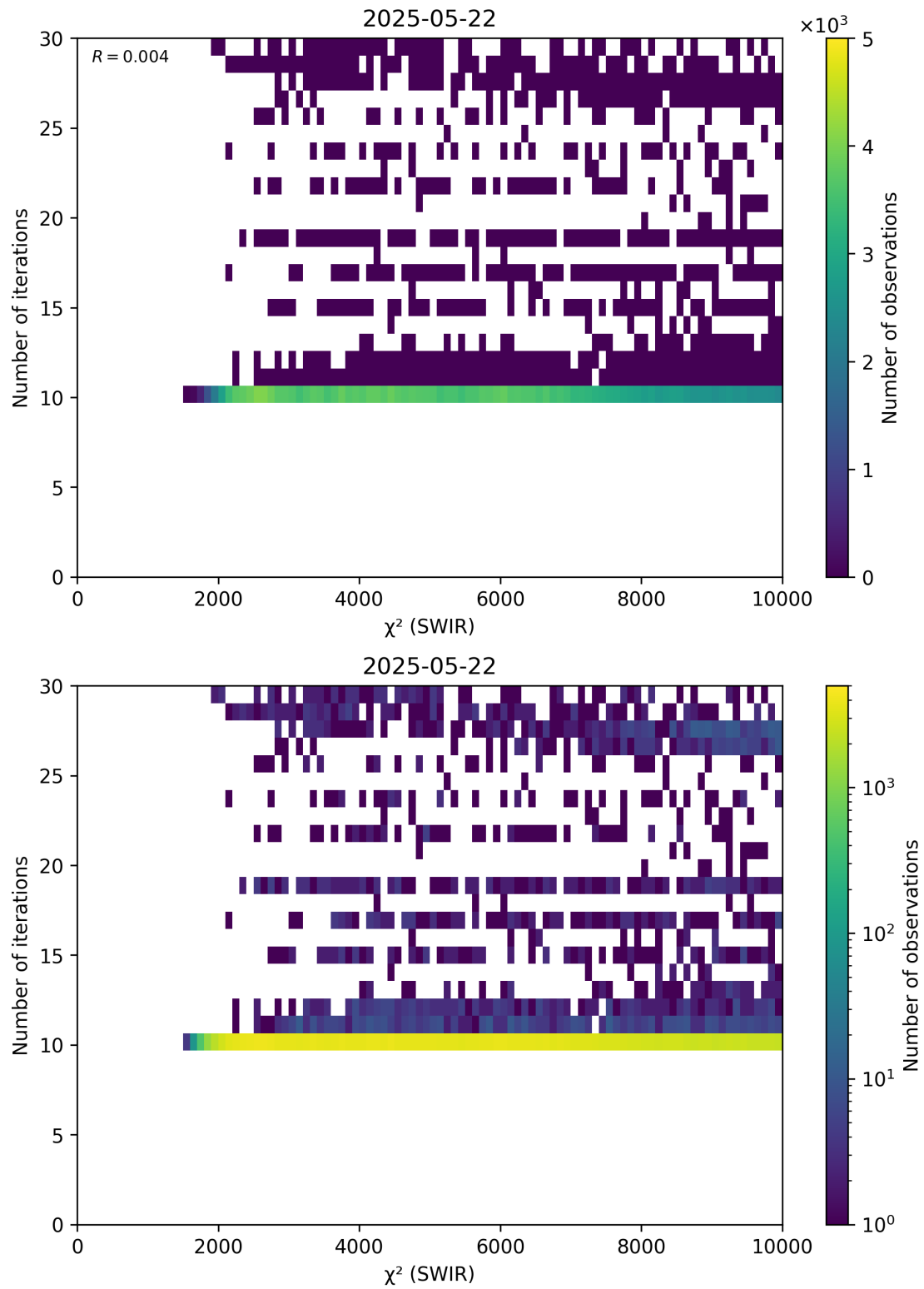
Figure 50: Scatter density plot of “ \chi^2 (SWIR)” against “Number of iterations” for 2025-05-21 to 2025-05-23.
