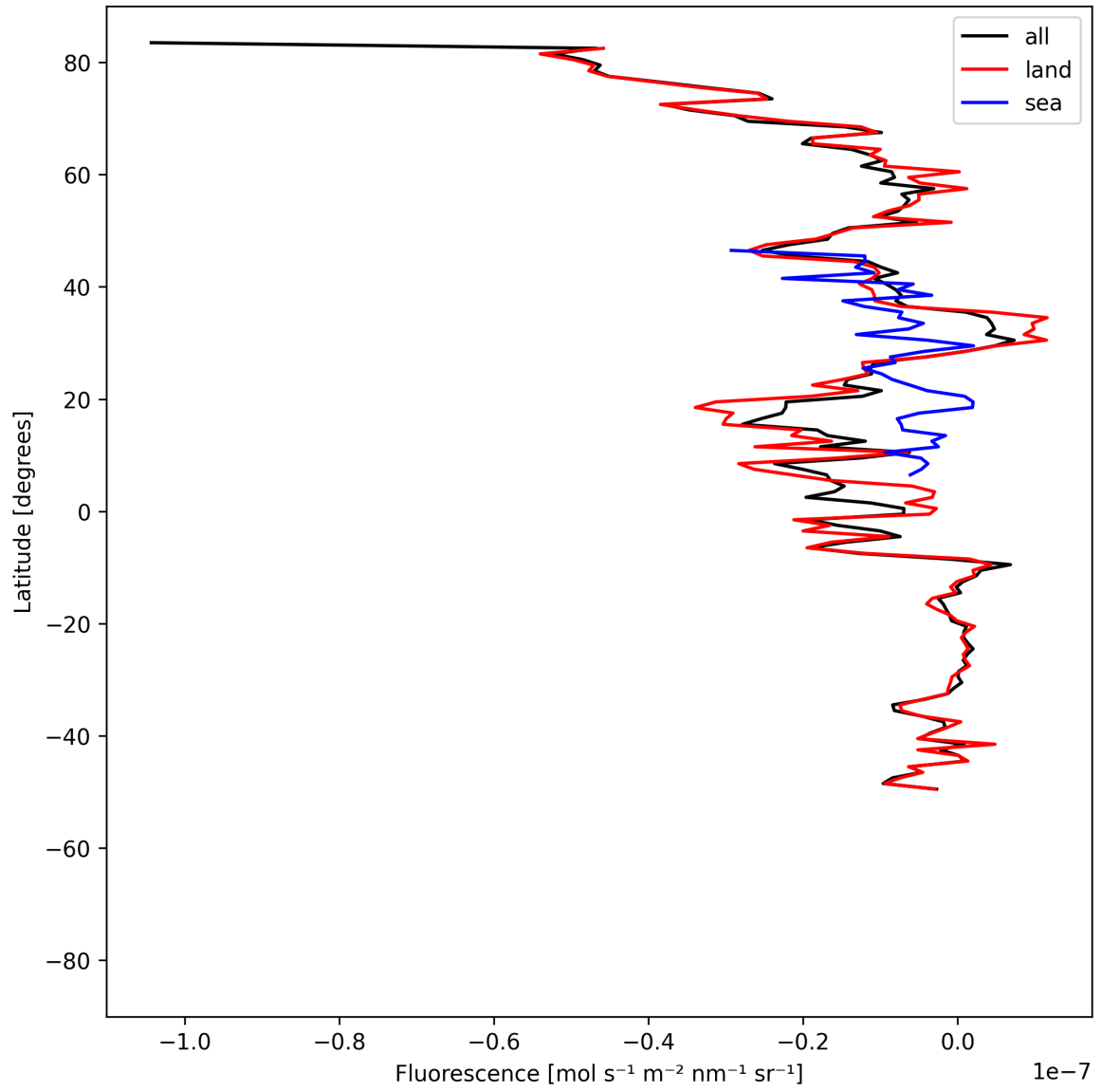
Figure 21: Zonal average of “Fluorescence” for 2025-05-21 to 2025-05-23.
