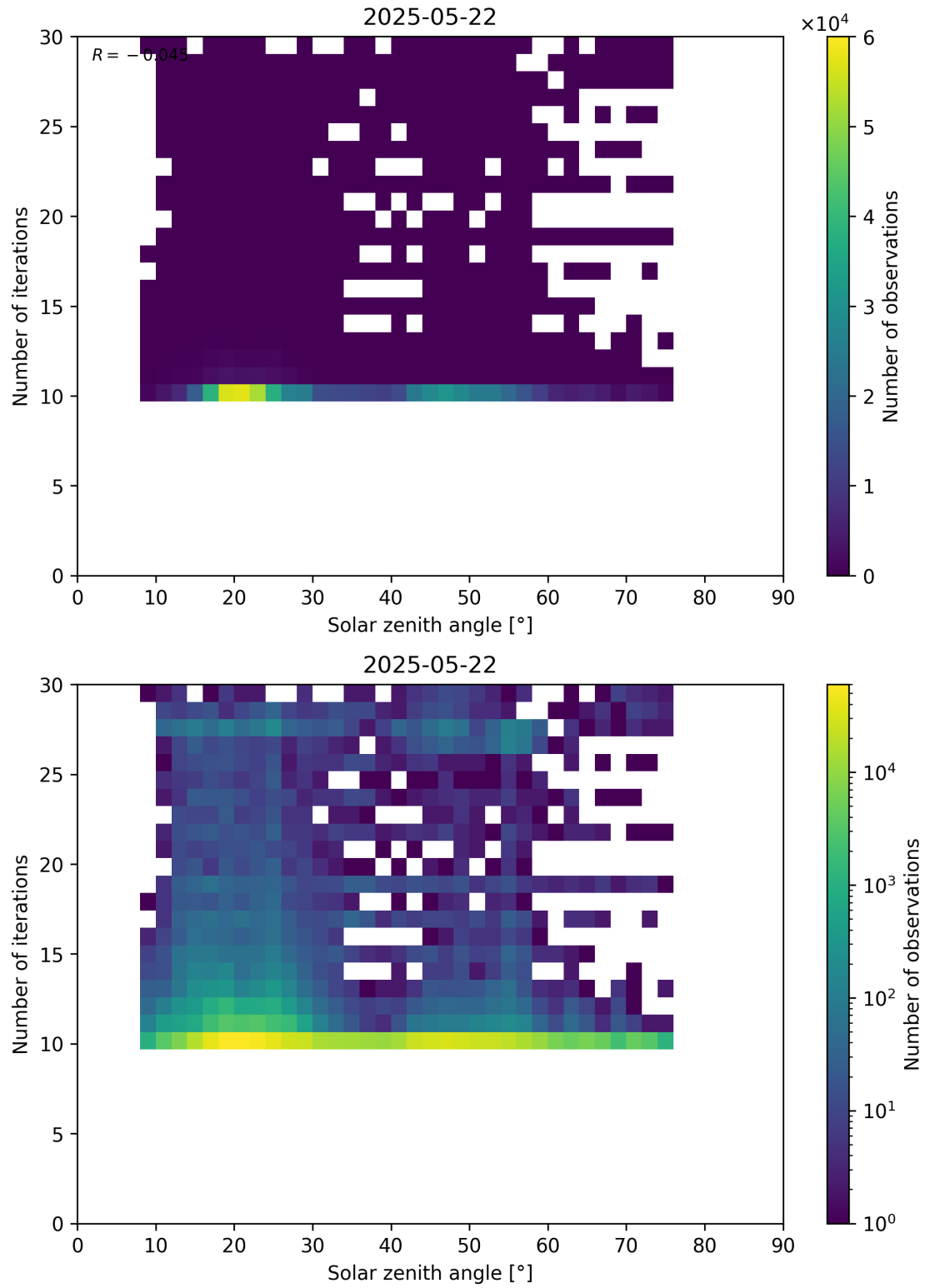
Figure 102: Scatter density plot of “Solar zenith angle” against “Number of iterations” for 2025-05-21 to 2025-05-23.
