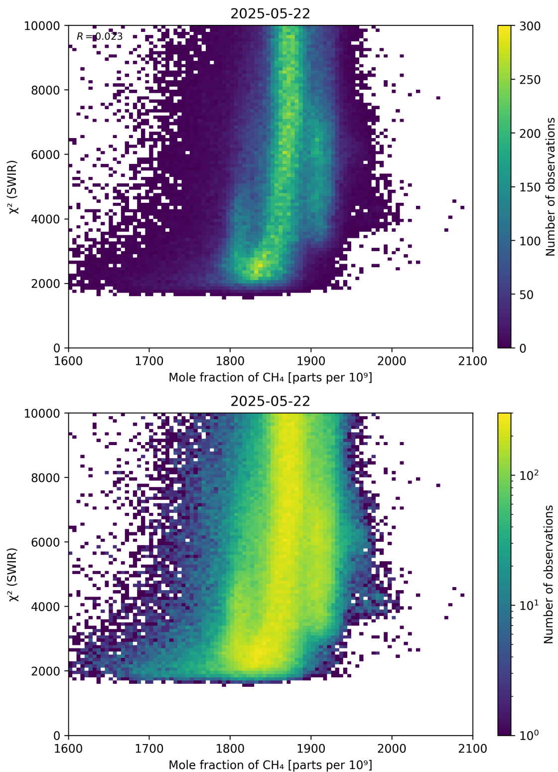
Figure 71: Scatter density plot of “Mole fraction of \text{CH}_4 ” against “ \chi^2 (SWIR)” for 2025-05-21 to 2025-05-23.
