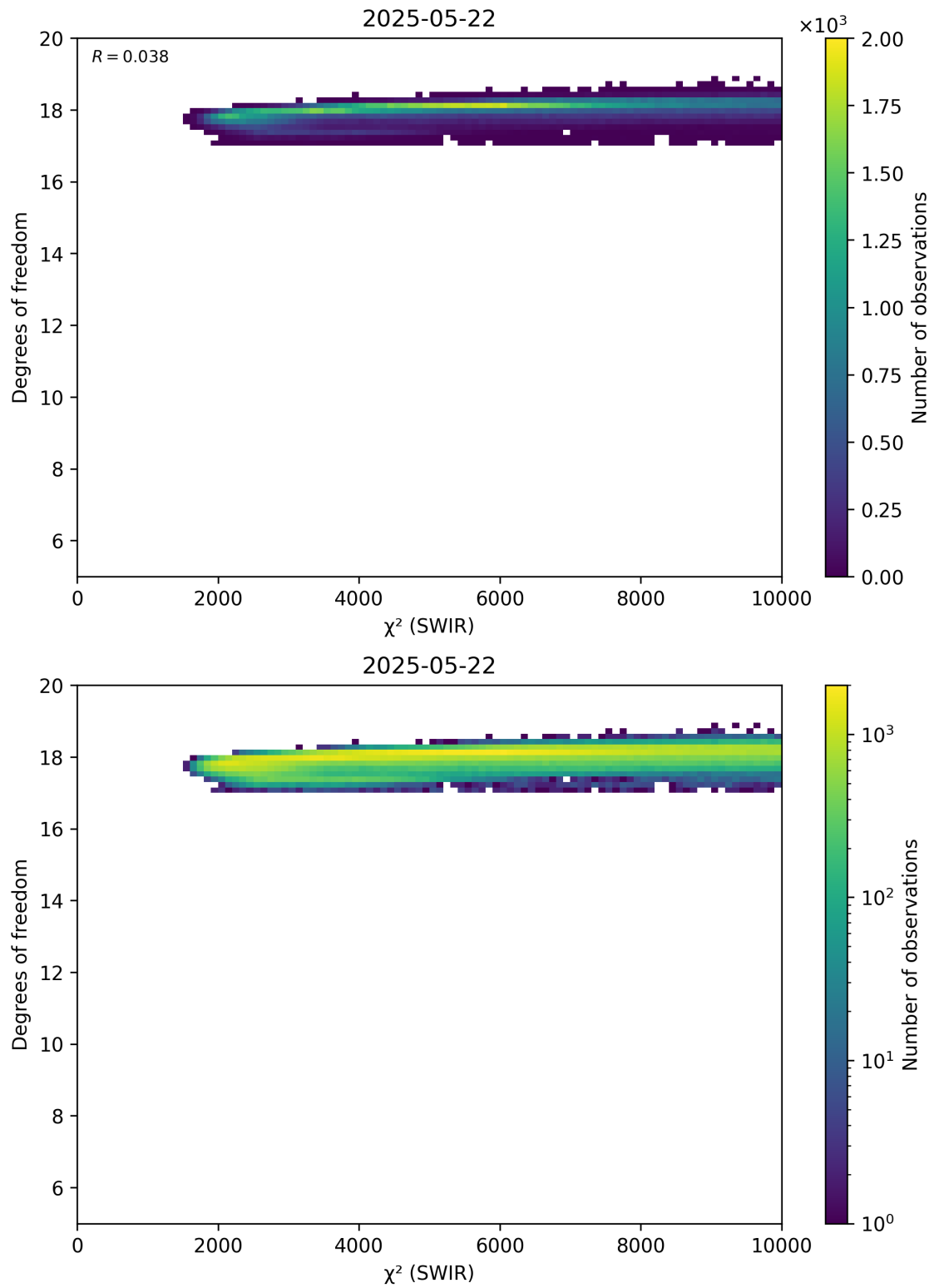
Figure 48: Scatter density plot of “ \chi^2 (SWIR)” against “Degrees of freedom” for 2025-05-21 to 2025-05-23.
