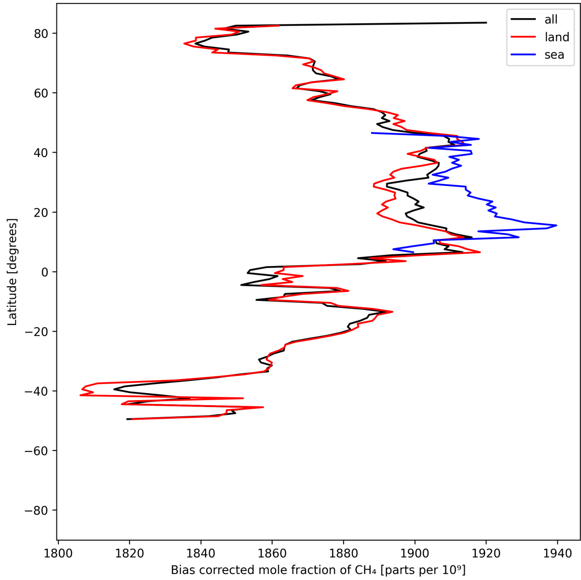
Figure 14: Zonal average of “Bias corrected mole fraction of CH 4 ” for 2025-05-21 to 2025-05-23.
