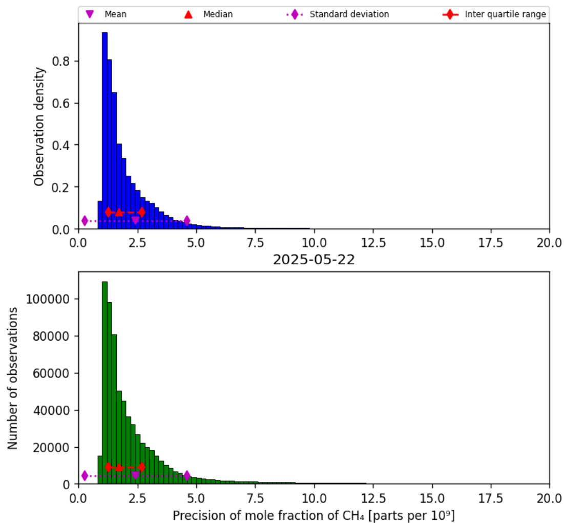
Figure 24: Histogram of “Precision of mole fraction of CH 4 ” for 2025-05-21 to 2025-05-23
