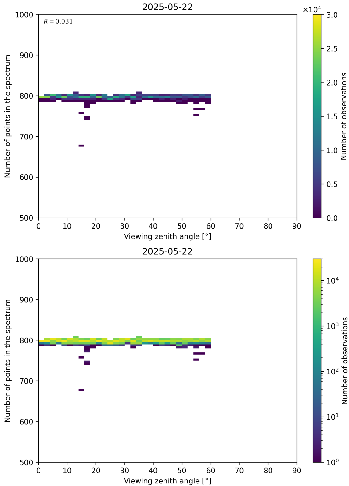
Figure 114: Scatter density plot of “Viewing zenith angle” against “Number of points in the spectrum” for 2025-05-21 to 2025-05-23.
