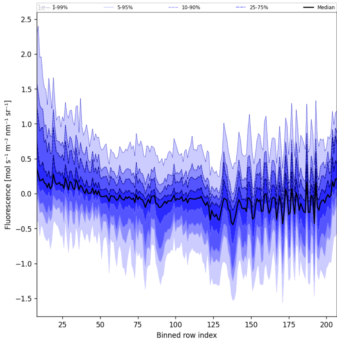
Figure 43: Along track statistics of “Fluorescence” for 2025-05-21 to 2025-05-23
