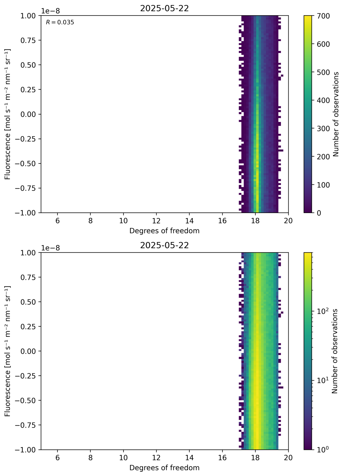
Figure 51: Scatter density plot of “Degrees of freedom” against “Fluorescence” for 2025-05-21 to 2025-05-23.
