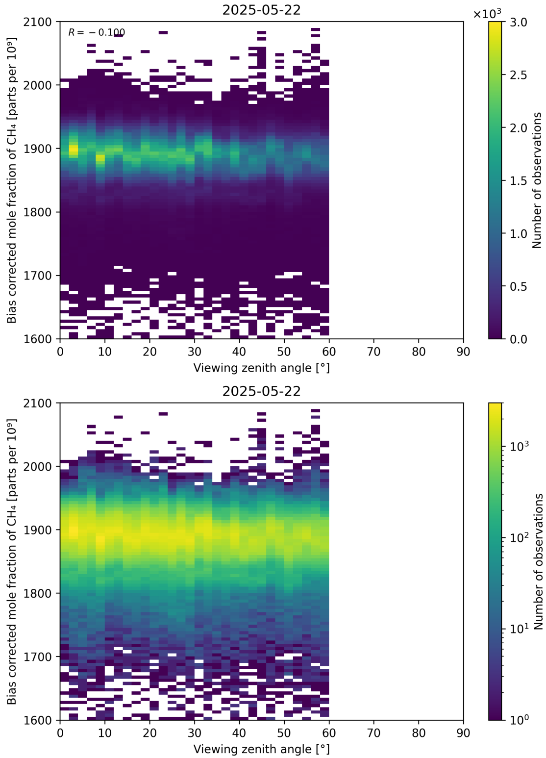
Figure 111: Scatter density plot of “Viewing zenith angle” against “Bias corrected mole fraction of CH 4 ” for 2025-05-21 to 2025-05-23.
