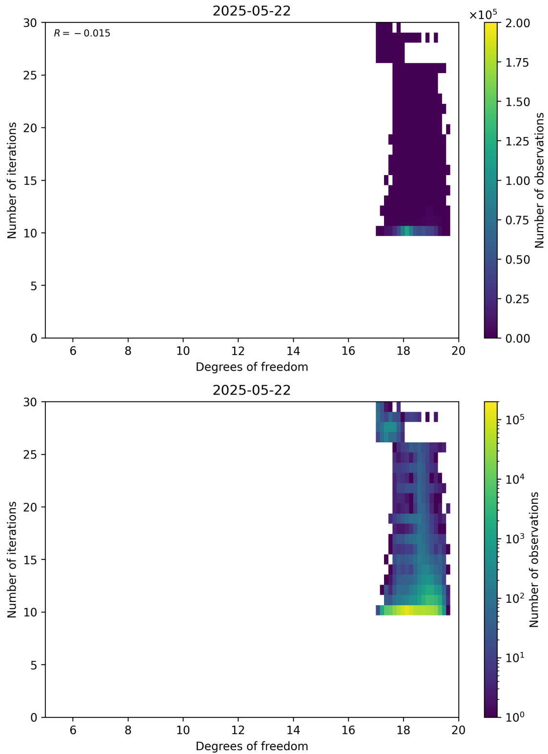
Figure 52: Scatter density plot of “Degrees of freedom” against “Number of iterations” for 2025-05-21 to 2025-05-23.
