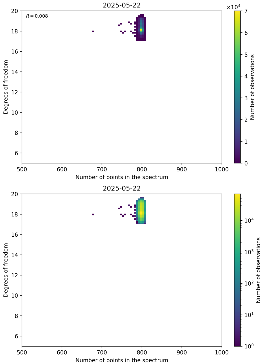
Figure 90: Scatter density plot of “Number of points in the spectrum” against “Degrees of freedom” for 2025-05-21 to 2025-05-23.
