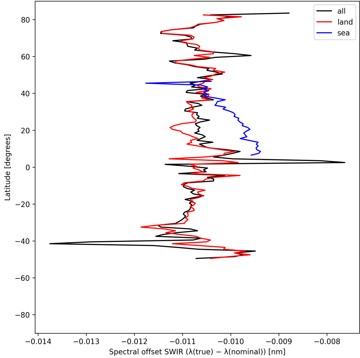
Figure 16: Zonal average of “Spectral offset SWIR ( \lambda_{\text{true}} - \lambda_{\text{nominal}} )” for 2025-05-21 to 2025-05-23.
