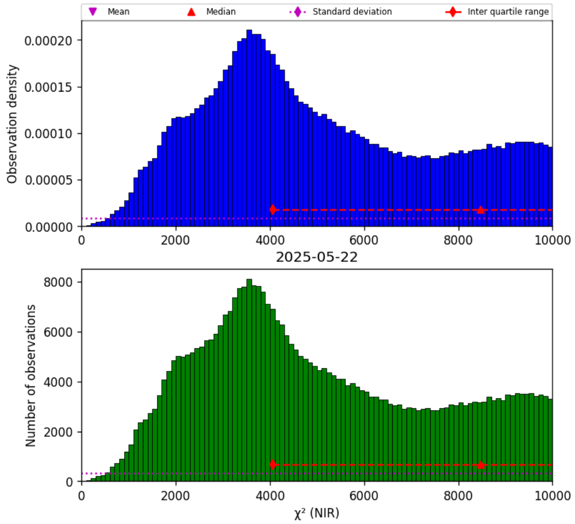
Figure 29: Histogram of “ \chi^2 (NIR)” for 2025-05-21 to 2025-05-23
