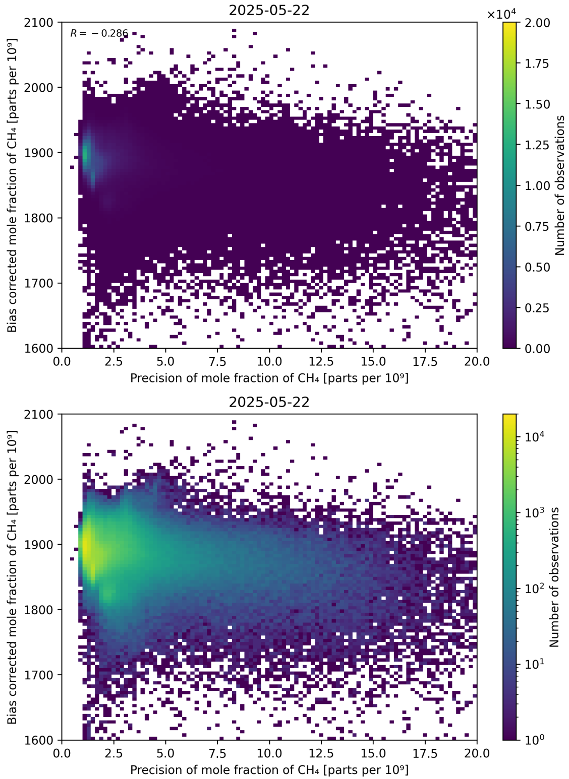
Figure 82: Scatter density plot of “Precision of mole fraction of CH 4 ” against “Bias corrected mole fraction of CH 4 ” for 2025-05-21 to 2025-05-23.
