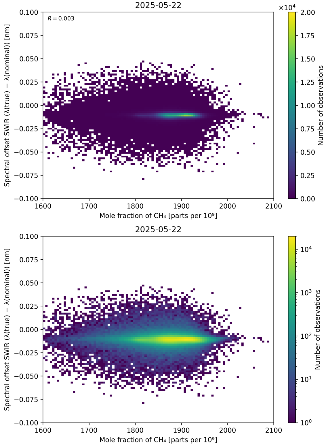
Figure 86: Scatter density plot of “Mole fraction of CH 4 ” against “Spectral offset SWIR ( \lambda_{\text{true}} - \lambda_{\text{nominal}} )” for 2025-05-21 to 2025-05-23.
