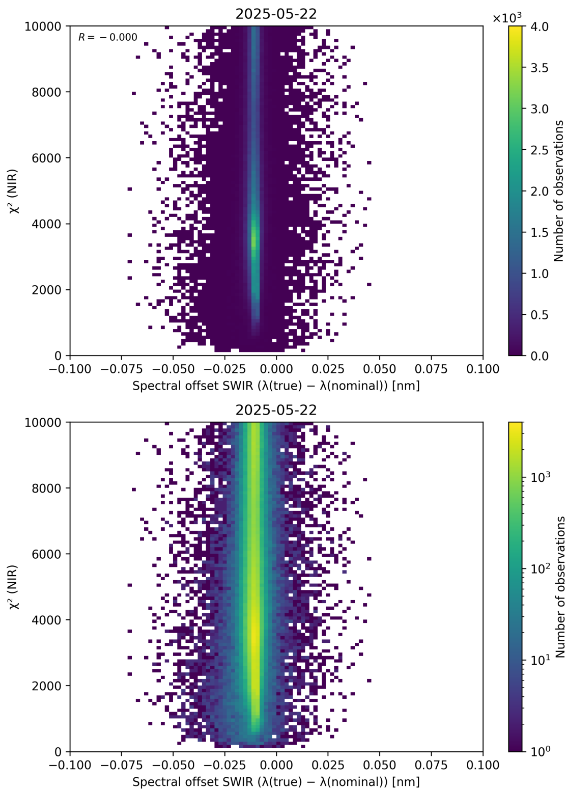
Figure 117: Scatter density plot of “Spectral offset SWIR ( \lambda_{\text{true}} - \lambda_{\text{nominal}} )” against “ \chi^2 (NIR)” for 2025-05-21 to 2025-05-23.
