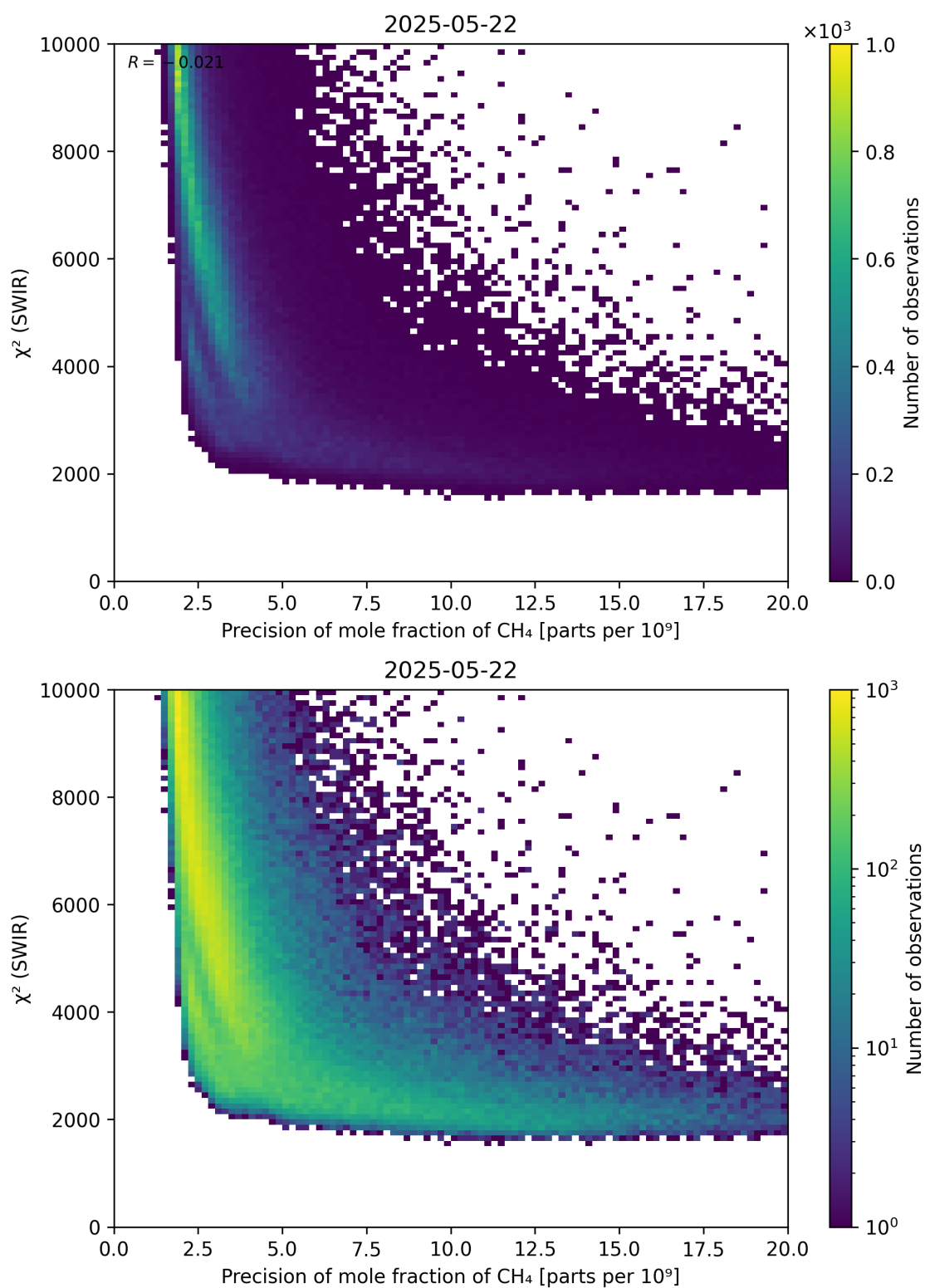
Figure 79: Scatter density plot of “Precision of mole fraction of \text{CH}_4 ” against “ \chi^2 (SWIR)” for 2025-05-21 to 2025-05-23.
