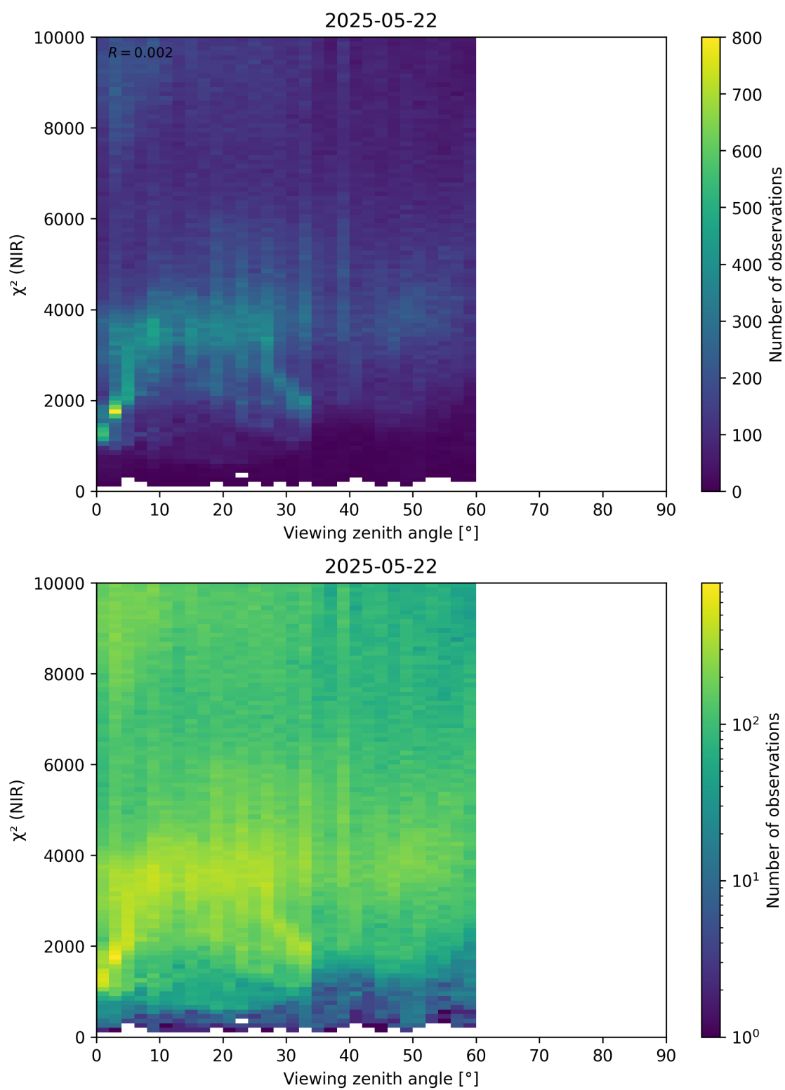
Figure 105: Scatter density plot of “Viewing zenith angle” against “ \chi^2 (NIR)” for 2025-05-21 to 2025-05-23.
