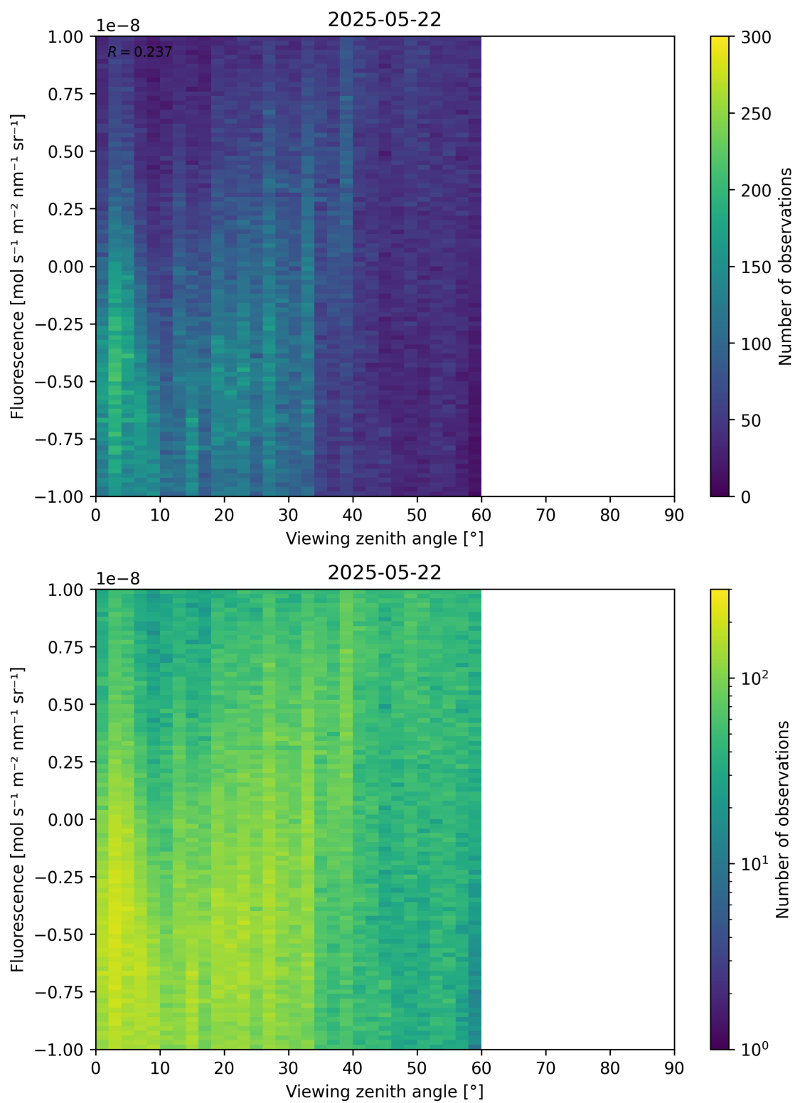
Figure 108: Scatter density plot of “Viewing zenith angle” against “Fluorescence” for 2025-05-21 to 2025-05-23.
