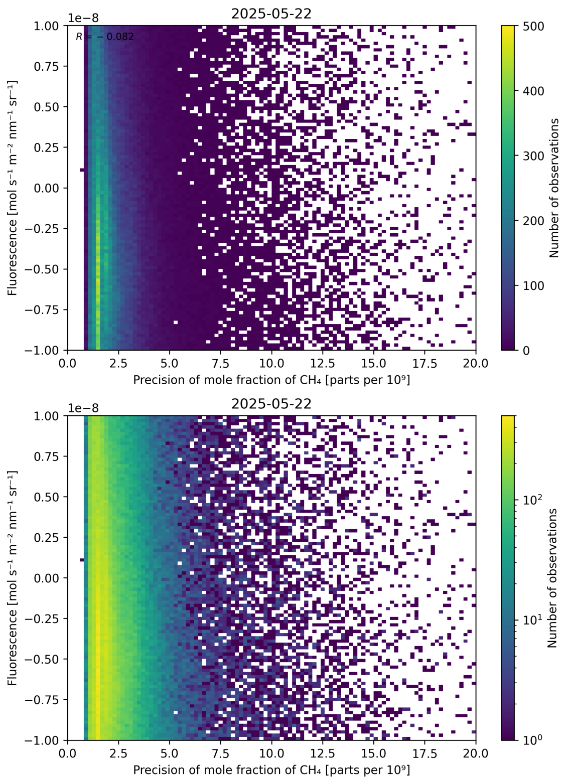
Figure 81: Scatter density plot of “Precision of mole fraction of \text{CH}_4 ” against “Fluorescence” for 2025-05-21 to 2025-05-23.
