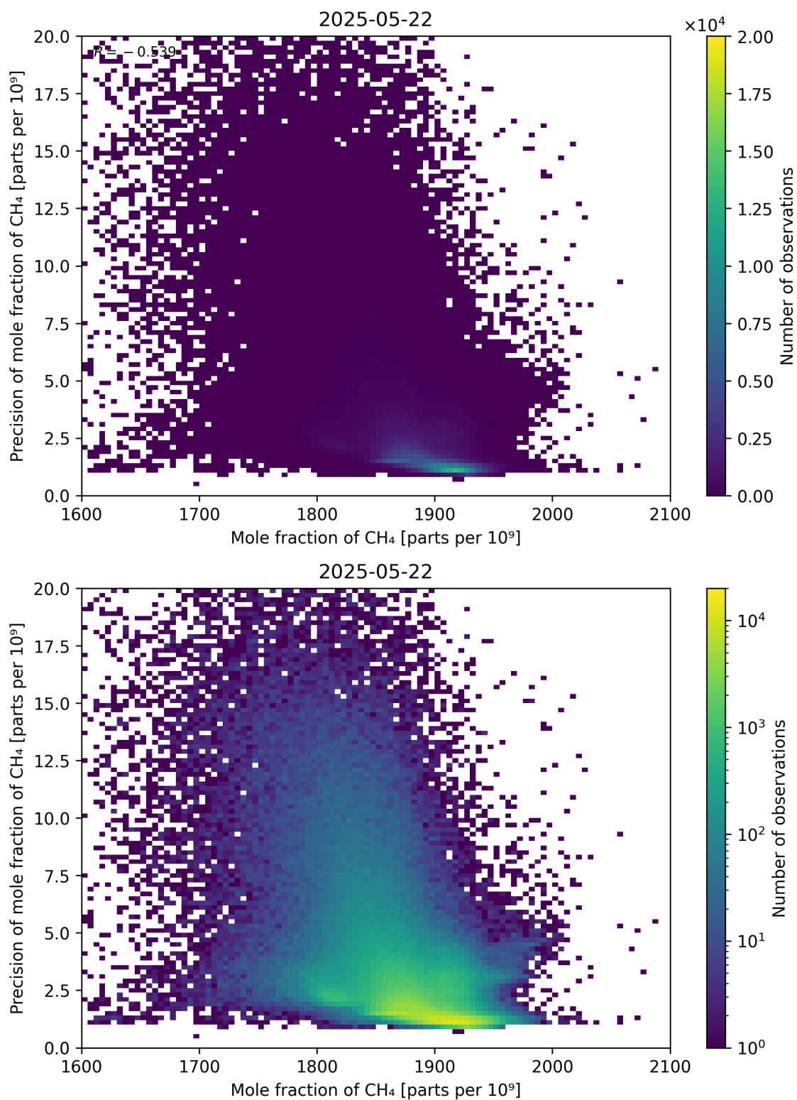
Figure 75: Scatter density plot of “Mole fraction of CH 4 ” against “Precision of mole fraction of CH 4 ” for 2025-05-21 to 2025-05-23.
