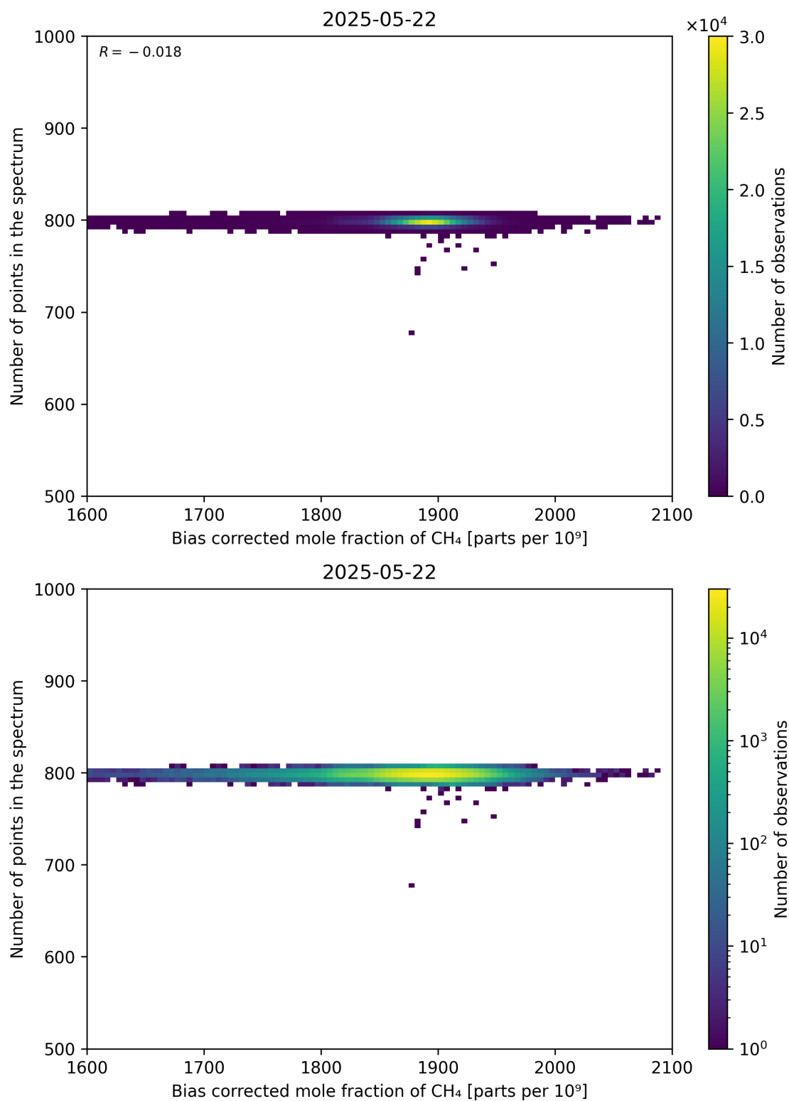
Figure 68: Scatter density plot of “Bias corrected mole fraction of CH 4 ” against “Number of points in the spectrum” for 2025-05-21 to 2025-05-23.
