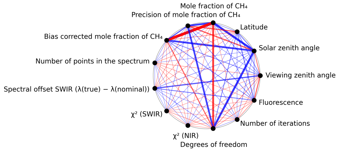
Figure 1: Map of correlation graph for 2025-05-21 to 2025-05-23.
