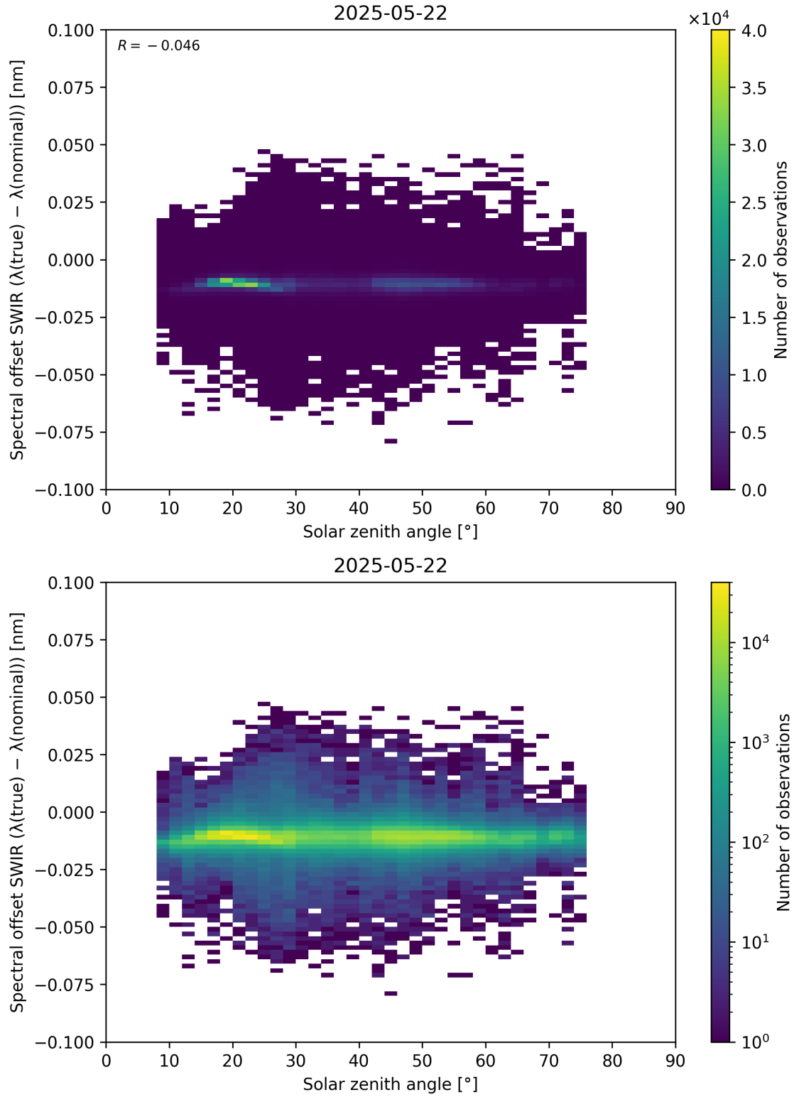
Figure 104: Scatter density plot of “Solar zenith angle” against “Spectral offset SWIR ( \lambda_{\text{true}} - \lambda_{\text{nominal}} )” for 2025-05-21 to 2025-05-23.
