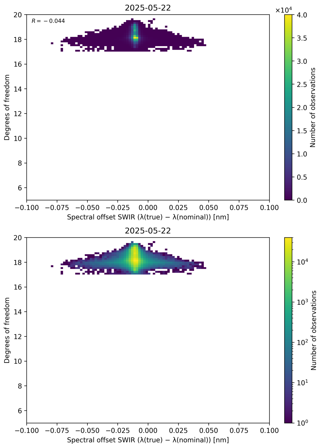
Figure 119: Scatter density plot of “Spectral offset SWIR ( \lambda_{\text{true}} - \lambda_{\text{nominal}} )” against “Degrees of freedom” for 2025-05-21 to 2025-05-23.
