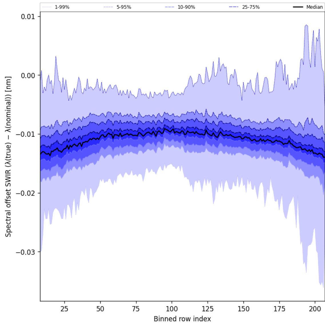
Figure 38: Along track statistics of “Spectral offset SWIR ( \lambda_{\text{true}} - \lambda_{\text{nominal}} )” for 2025-05-21 to 2025-05-23
