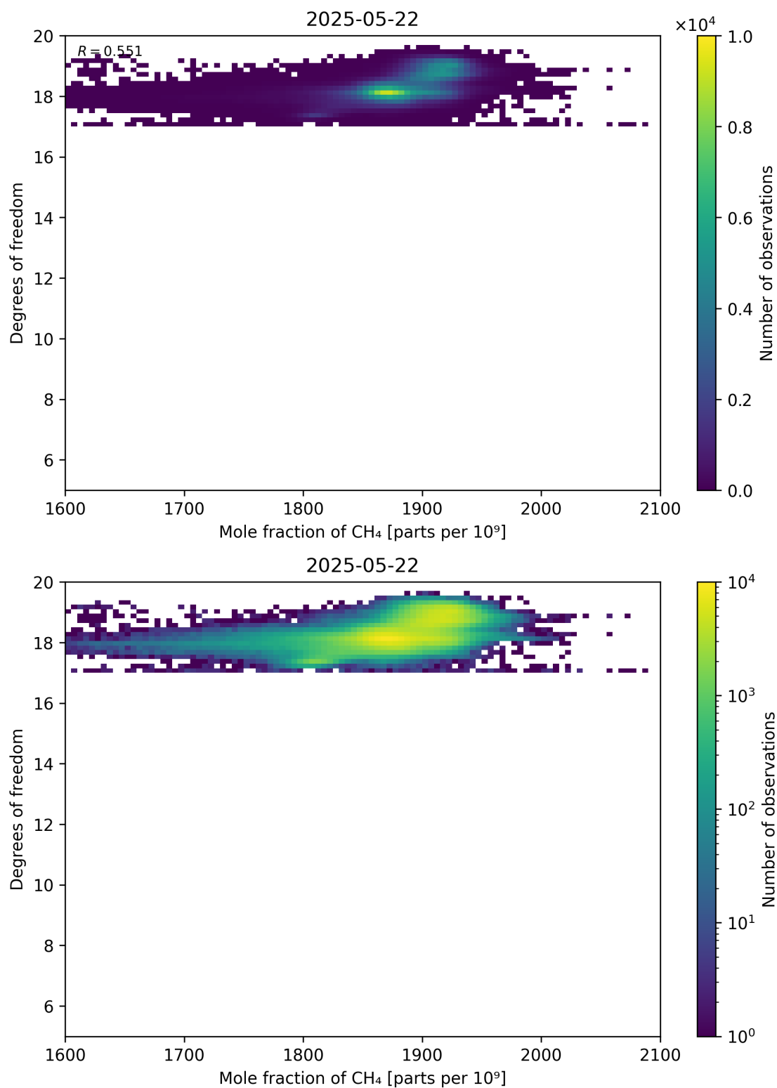
Figure 72: Scatter density plot of “Mole fraction of CH 4 ” against “Degrees of freedom” for 2025-05-21 to 2025-05-23.
