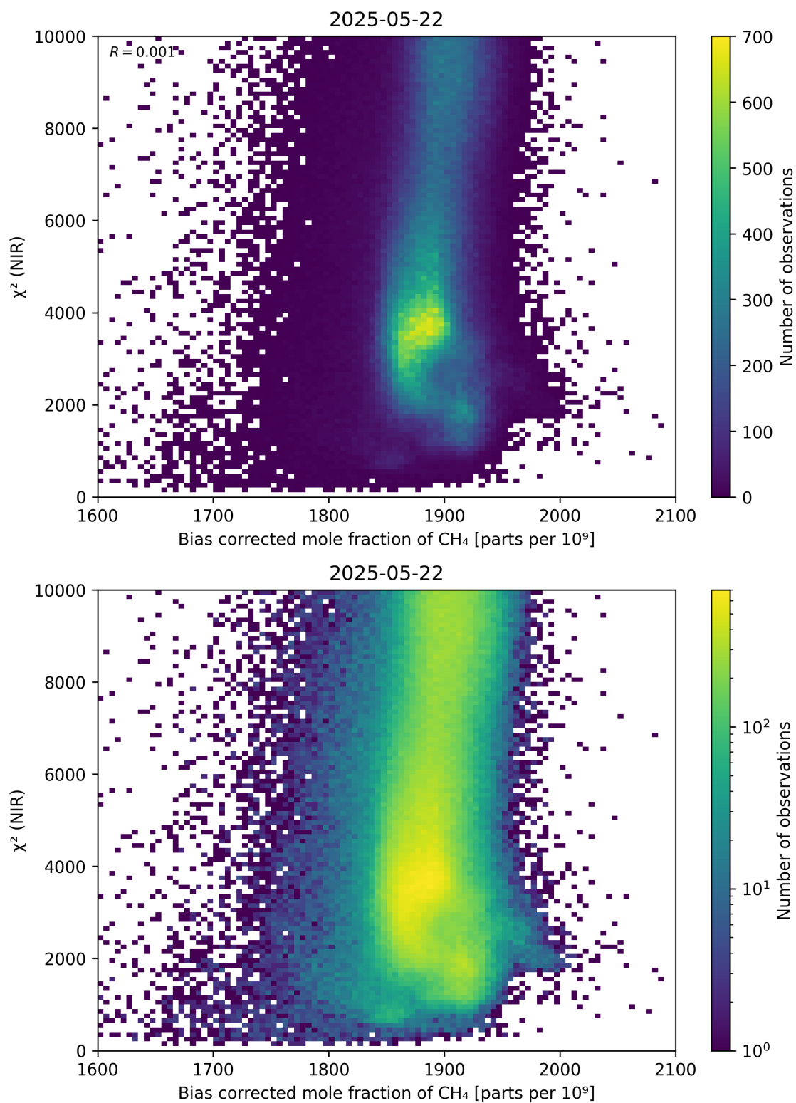
Figure 63: Scatter density plot of “Bias corrected mole fraction of CH 4 ” against “ \chi^2 (NIR)” for 2025-05-21 to 2025-05-23.
