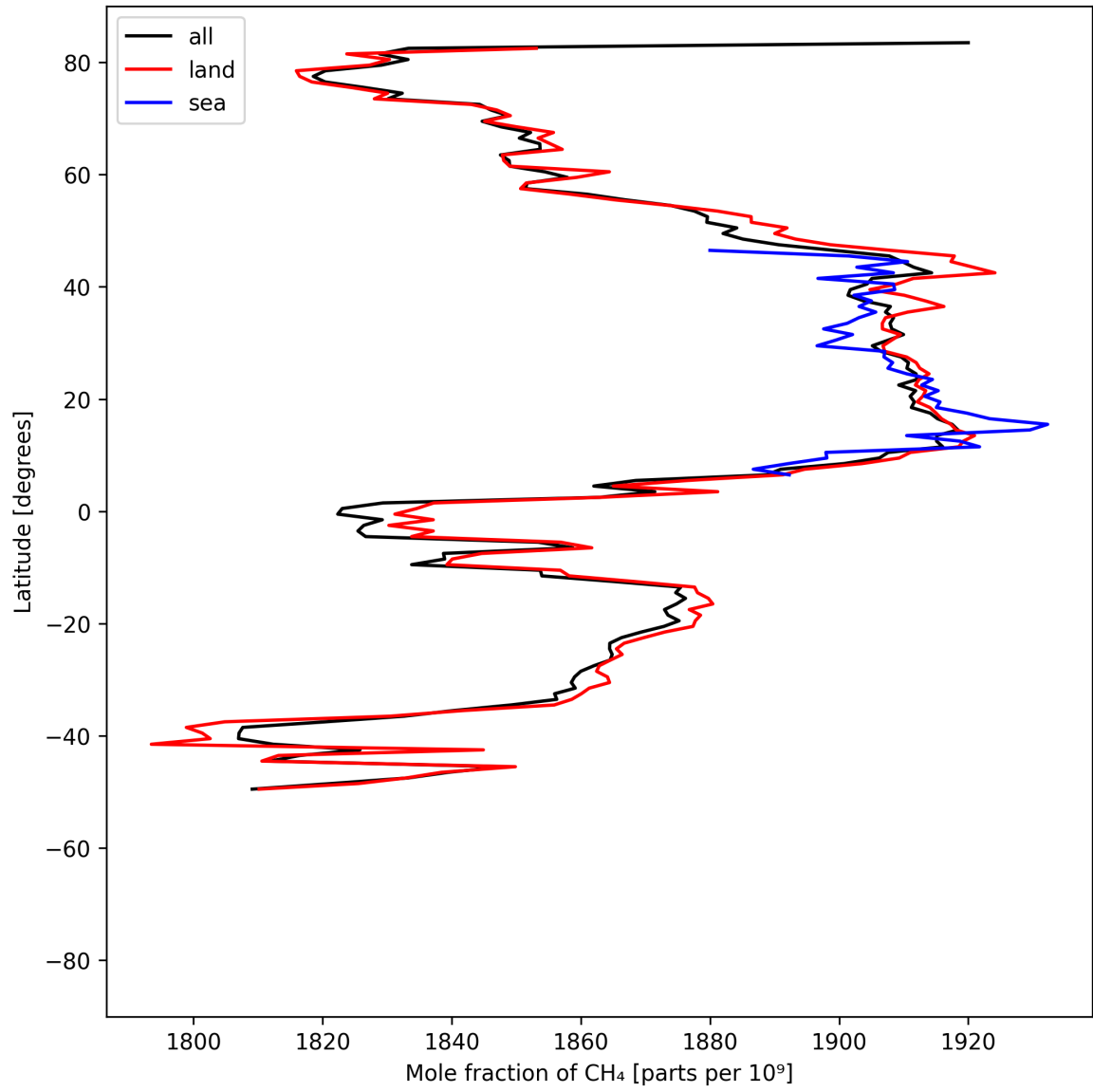
Figure 12: Zonal average of “Mole fraction of \text{CH}_4 ” for 2025-05-21 to 2025-05-23.
