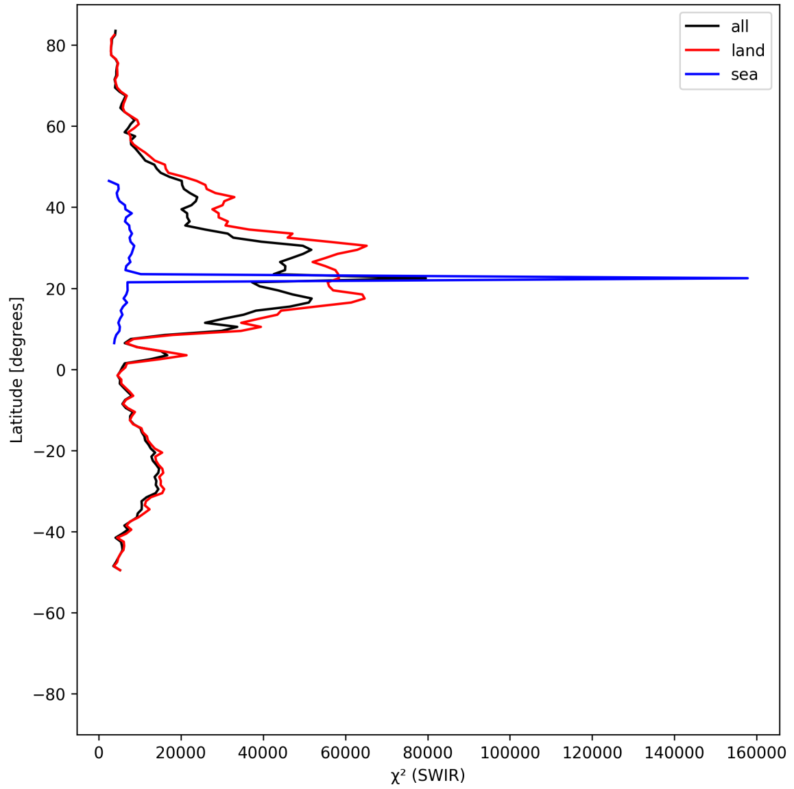
Figure 17: Zonal average of “ \chi^2 (SWIR)” for 2025-05-21 to 2025-05-23.
