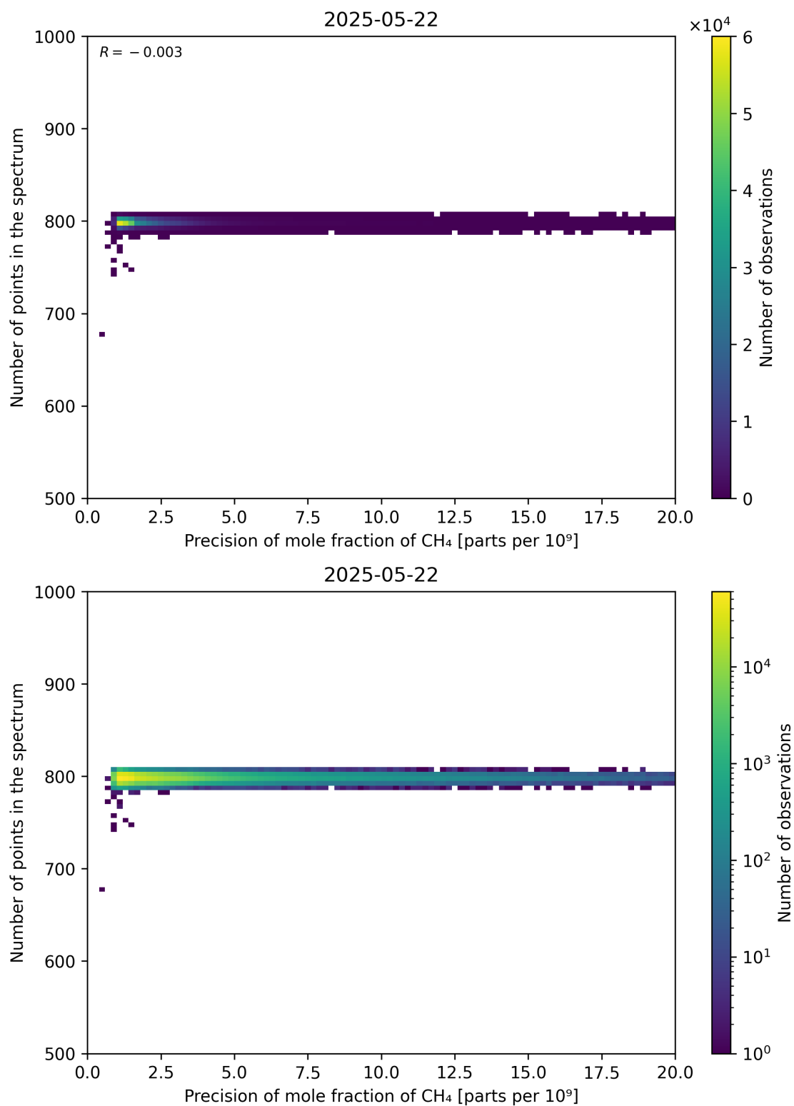
Figure 84: Scatter density plot of “Precision of mole fraction of CH 4 ” against “Number of points in the spectrum” for 2025-05-21 to 2025-05-23.
