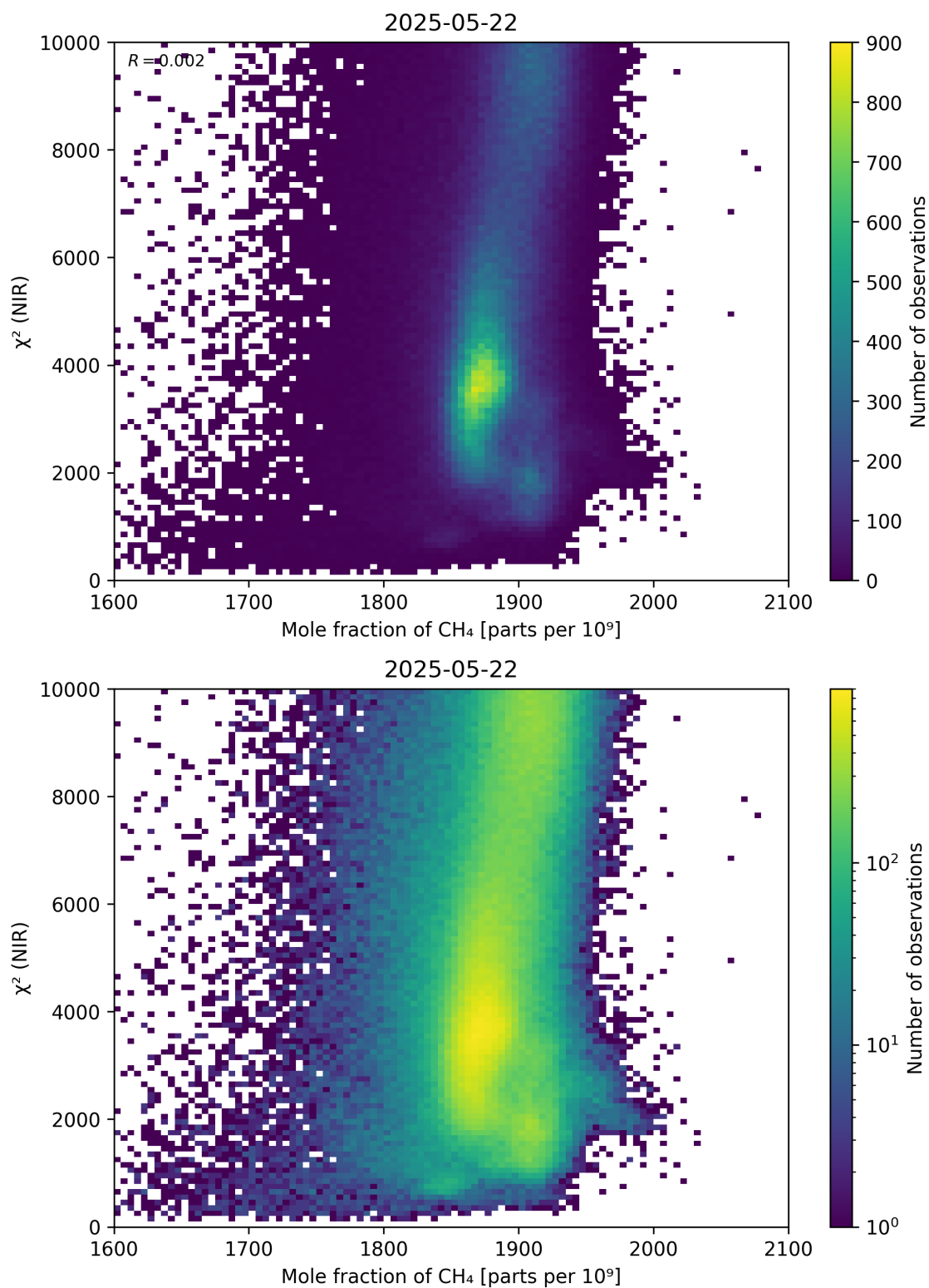
Figure 70: Scatter density plot of “Mole fraction of CH 4 ” against “ \chi^2 (NIR)” for 2025-05-21 to 2025-05-23.
