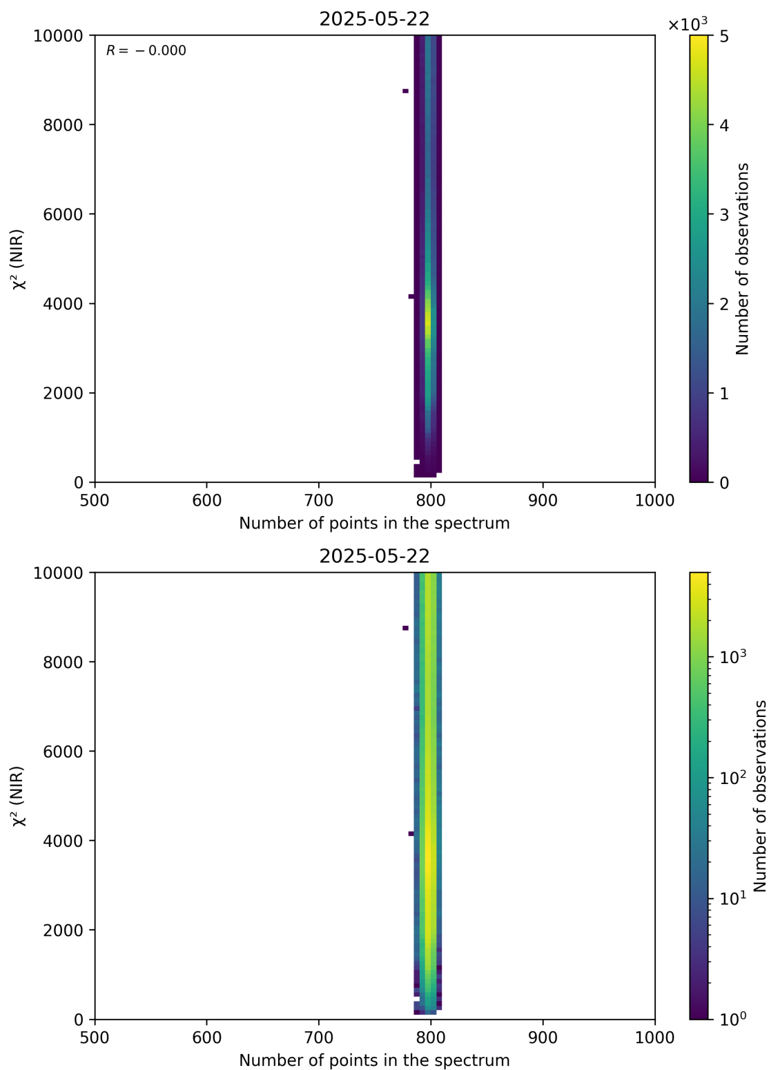
Figure 88: Scatter density plot of “Number of points in the spectrum” against “ \chi^2 (NIR)” for 2025-05-21 to 2025-05-23.
