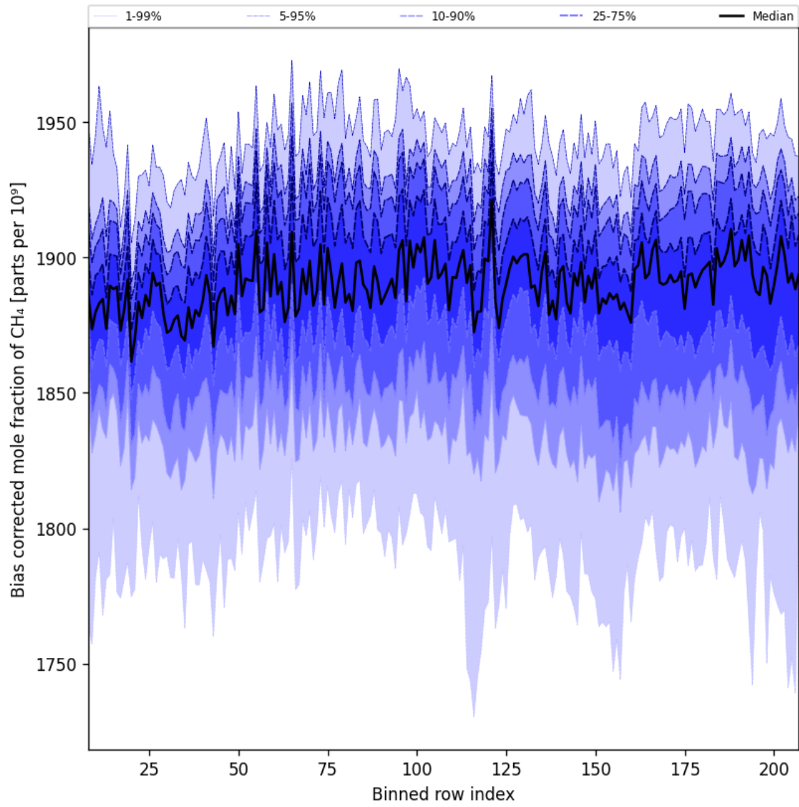
Figure 36: Along track statistics of “Bias corrected mole fraction of CH 4 ” for 2025-05-21 to 2025-05-23
