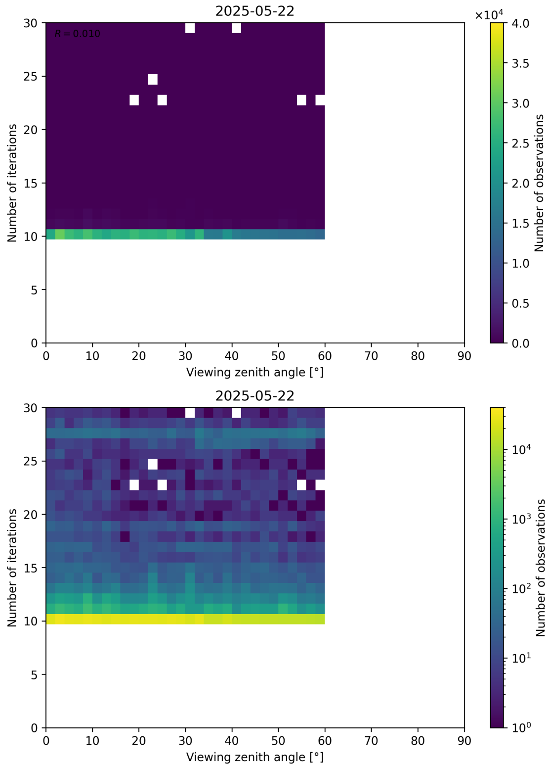
Figure 113: Scatter density plot of “Viewing zenith angle” against “Number of iterations” for 2025-05-21 to 2025-05-23.
