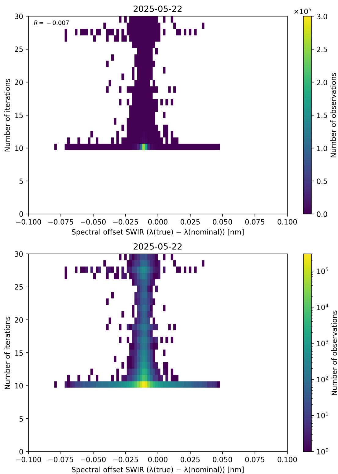
Figure 121: Scatter density plot of “Spectral offset SWIR ( \lambda_{\text{true}} - \lambda_{\text{nominal}} )” against “Number of iterations” for 2025-05-21 to 2025-05-23.
