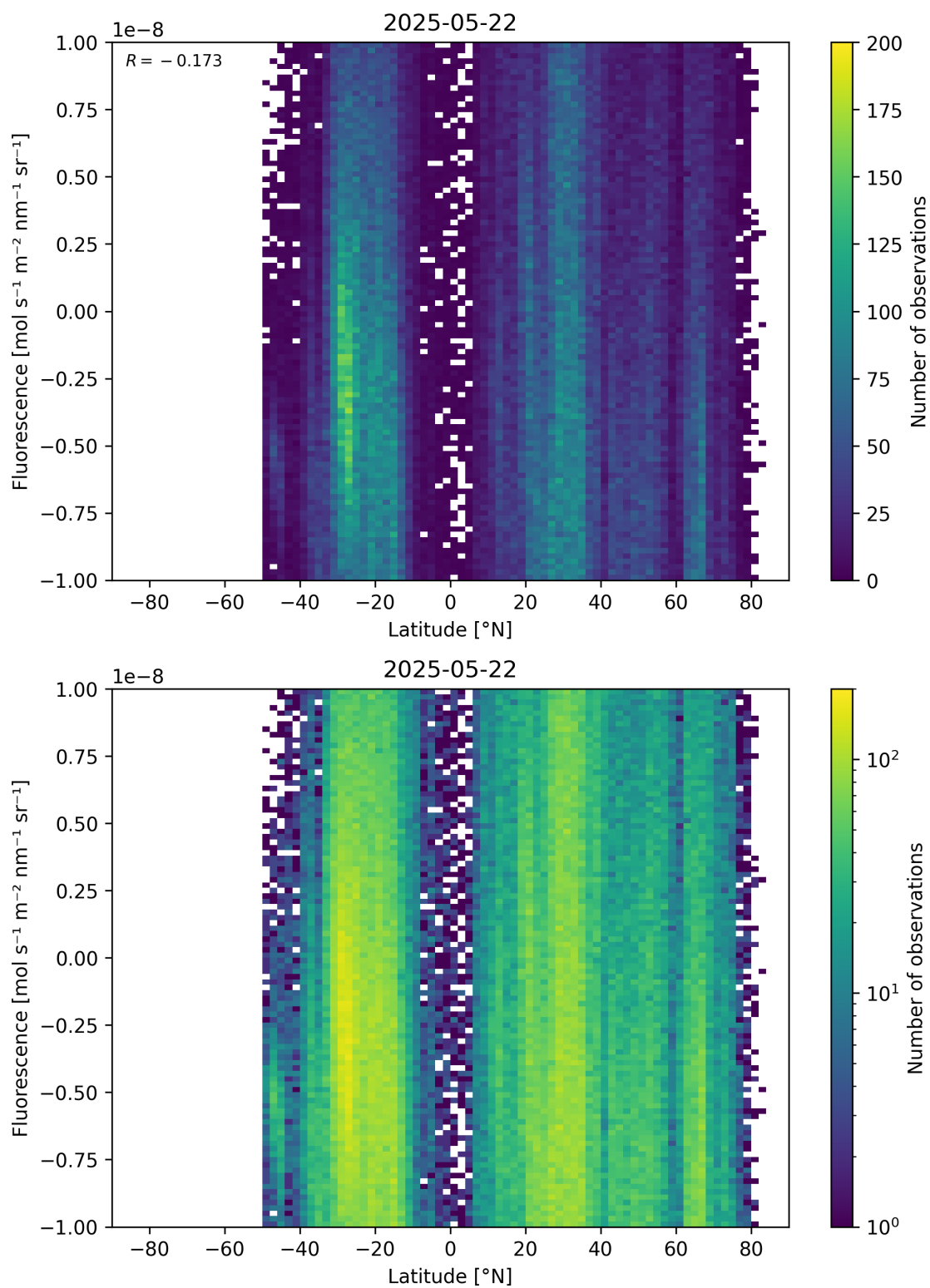
Figure 56: Scatter density plot of “Latitude” against “Fluorescence” for 2025-05-21 to 2025-05-23.
