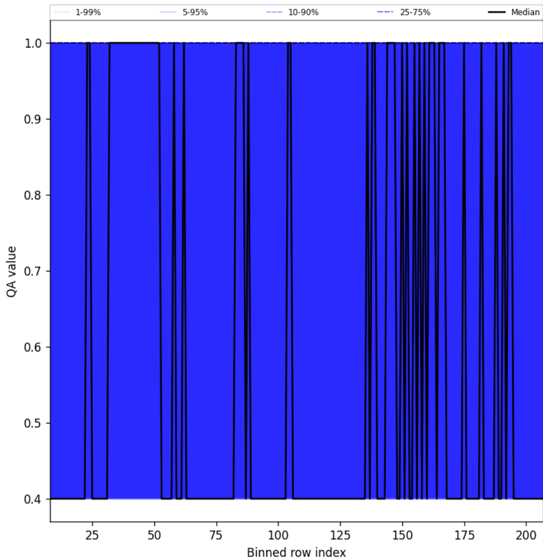
Figure 33: Along track statistics of “QA value” for 2025-05-21 to 2025-05-23
