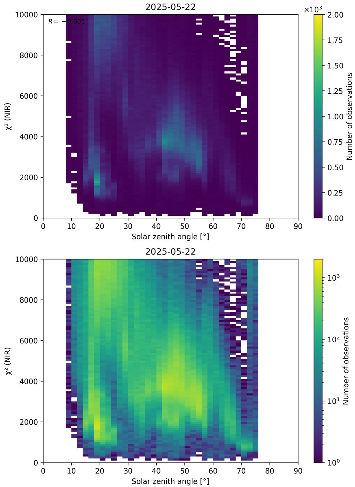
Figure 94: Scatter density plot of “Solar zenith angle” against “ \chi^2 (NIR)” for 2025-05-21 to 2025-05-23.
