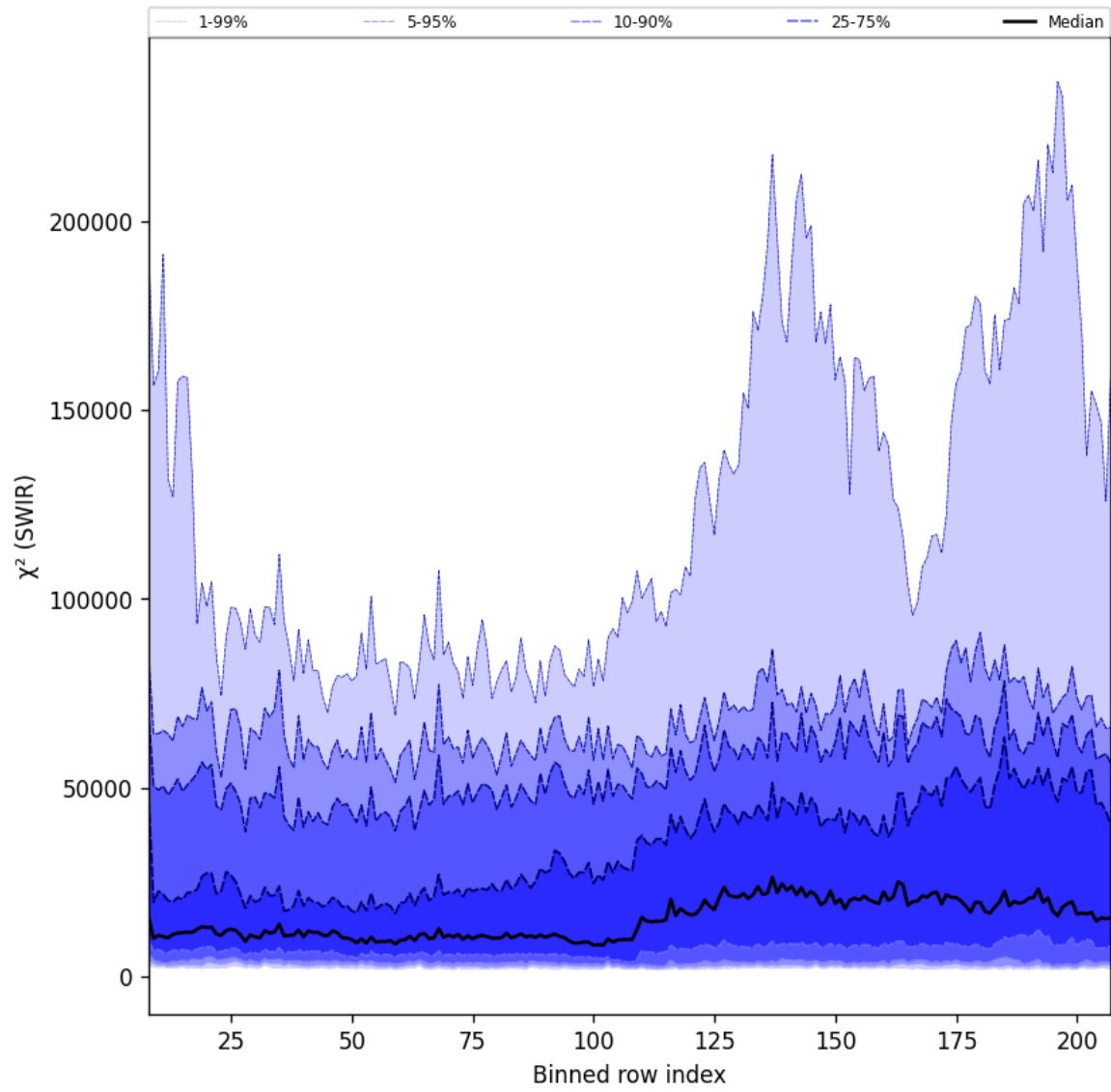
Figure 39: Along track statistics of “ \chi^2 (SWIR)” for 2025-05-21 to 2025-05-23
