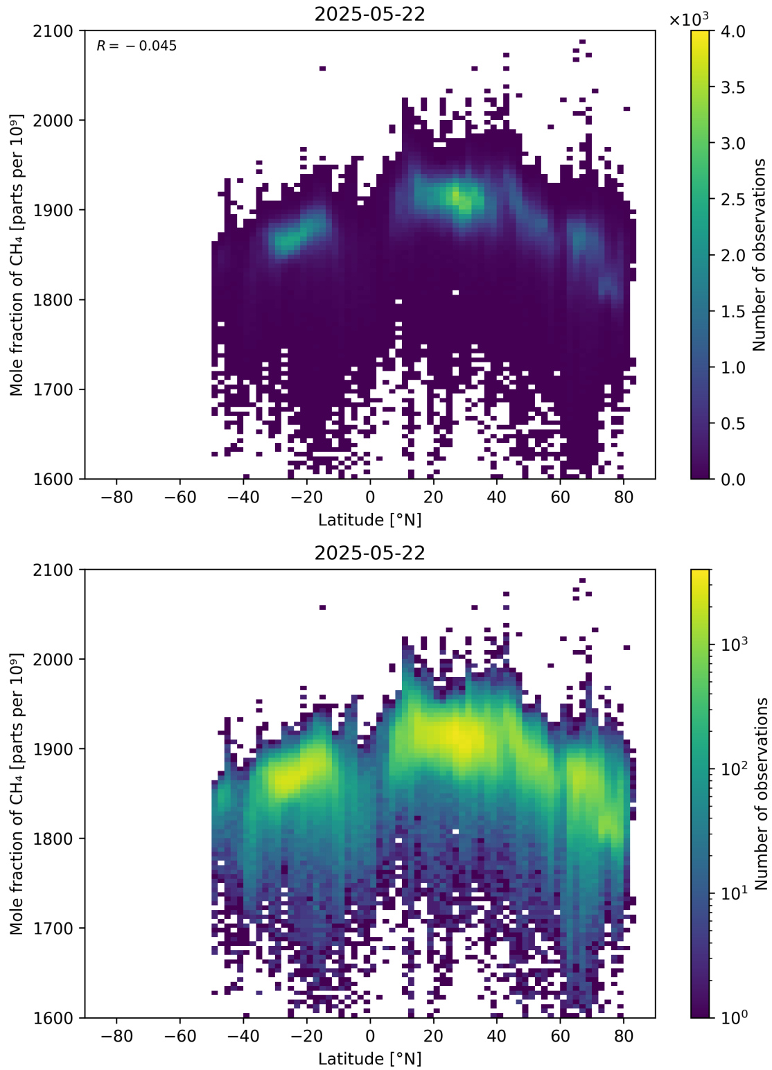
Figure 57: Scatter density plot of “Latitude” against “Mole fraction of CH 4 ” for 2025-05-21 to 2025-05-23.
