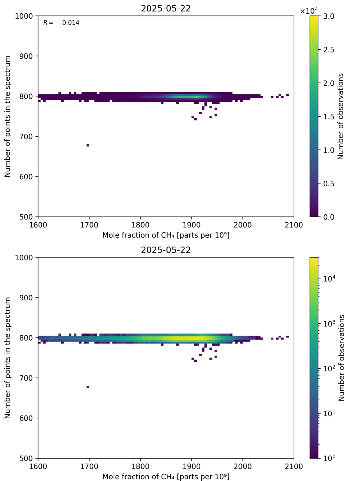
Figure 77: Scatter density plot of “Mole fraction of CH 4 ” against “Number of points in the spectrum” for 2025-05-21 to 2025-05-23.
