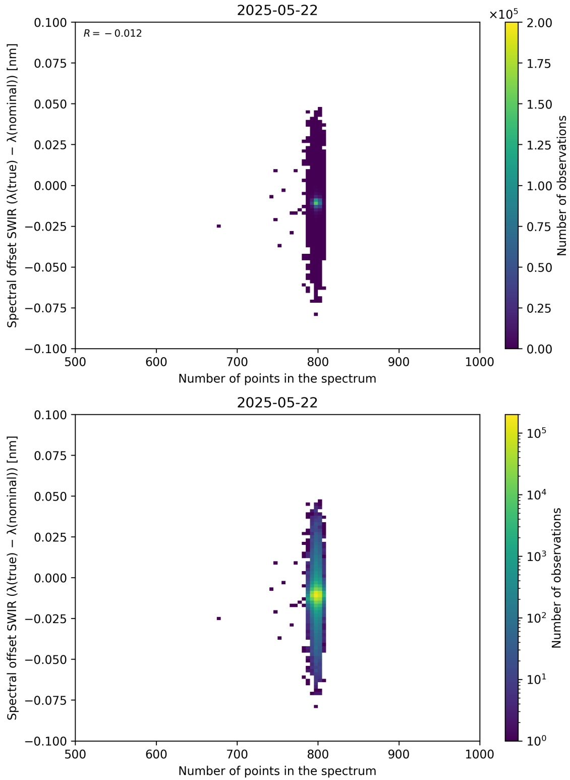
Figure 93: Scatter density plot of “Number of points in the spectrum” against “Spectral offset SWIR ( \lambda_{\text{true}} - \lambda_{\text{nominal}} )” for 2025-05-21 to 2025-05-23.
