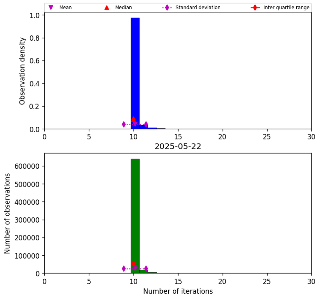
Figure 31: Histogram of “Number of iterations” for 2025-05-21 to 2025-05-23
