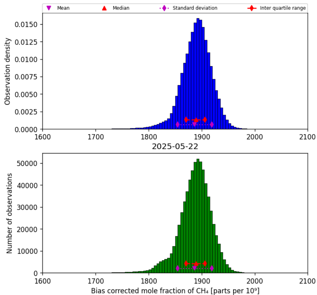
Figure 25: Histogram of “Bias corrected mole fraction of CH 4 ” for 2025-05-21 to 2025-05-23
