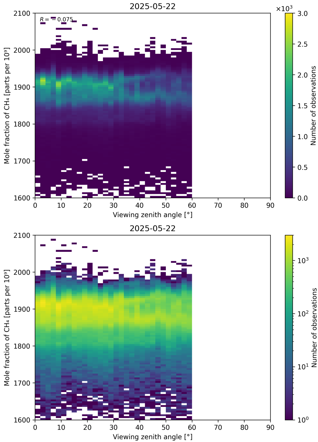
Figure 110: Scatter density plot of “Viewing zenith angle” against “Mole fraction of CH 4 ” for 2025-05-21 to 2025-05-23.
