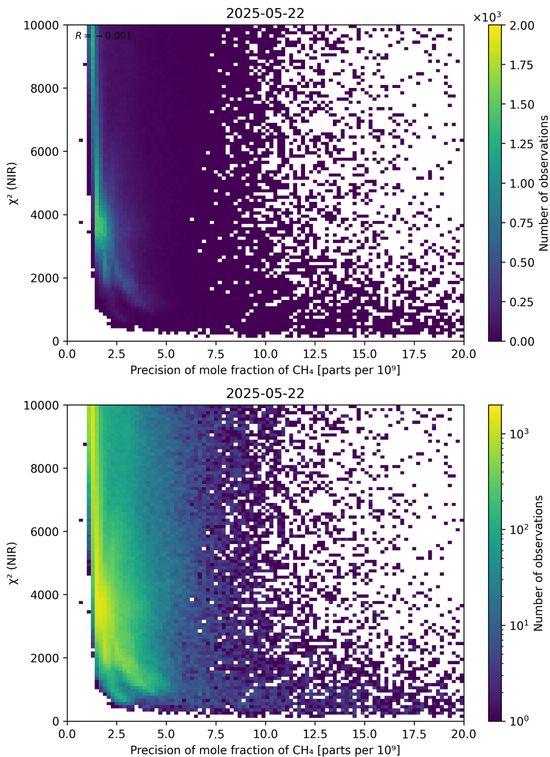
Figure 78: Scatter density plot of “Precision of mole fraction of CH 4 ” against “ \chi^2 (NIR)” for 2025-05-21 to 2025-05-23.
