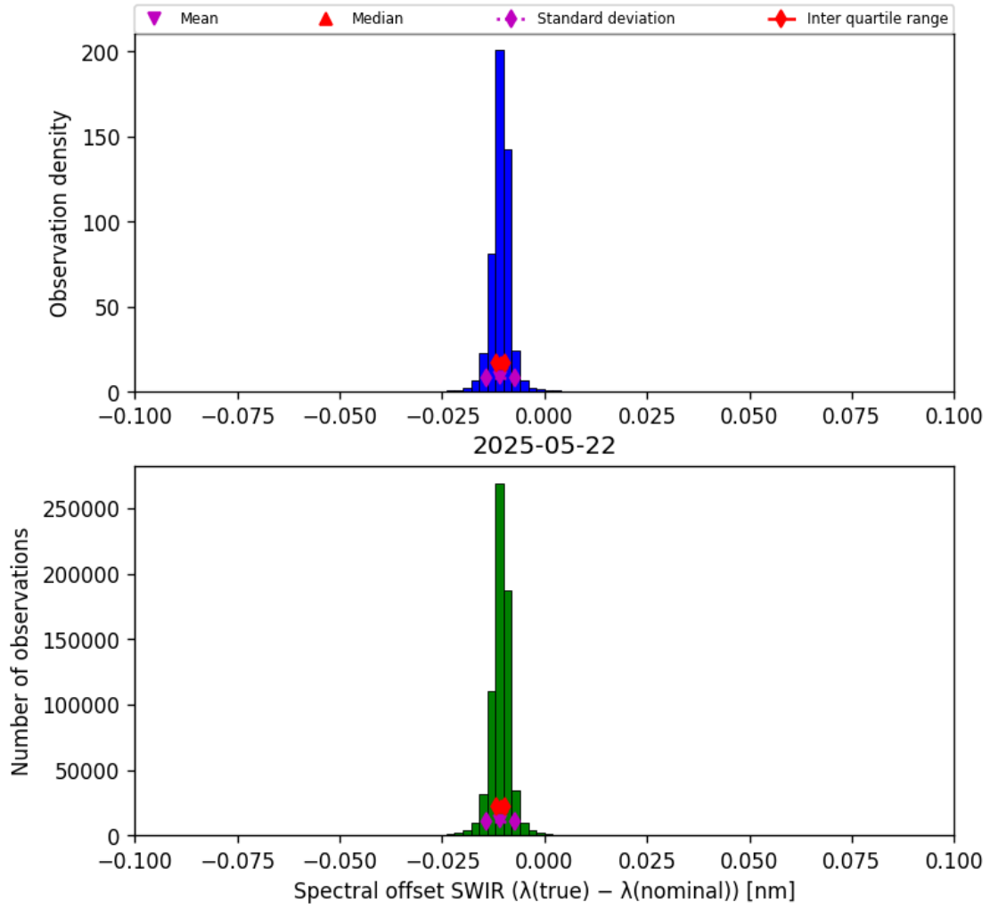
Figure 27: Histogram of “Spectral offset SWIR ( \lambda_{\text{true}} - \lambda_{\text{nominal}} )” for 2025-05-21 to 2025-05-23
