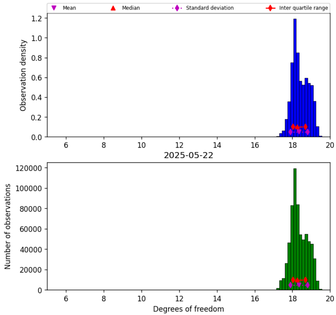
Figure 30: Histogram of “Degrees of freedom” for 2025-05-21 to 2025-05-23
