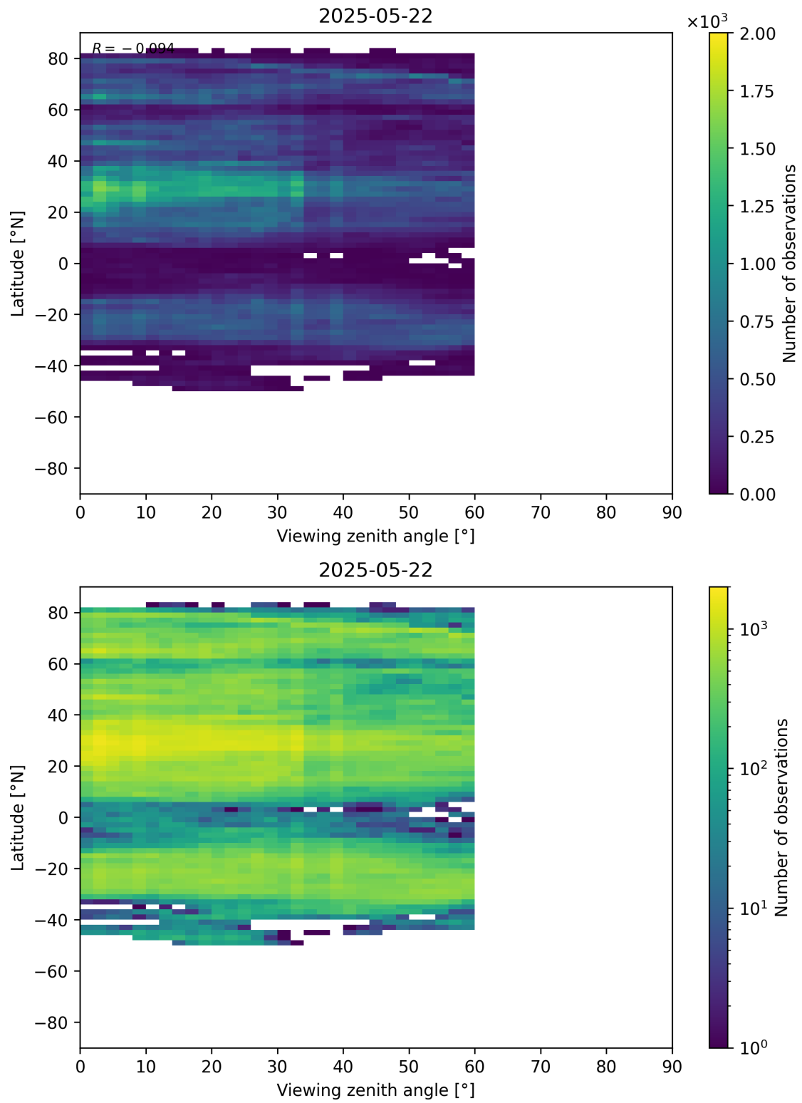
Figure 109: Scatter density plot of “Viewing zenith angle” against “Latitude” for 2025-05-21 to 2025-05-23.
