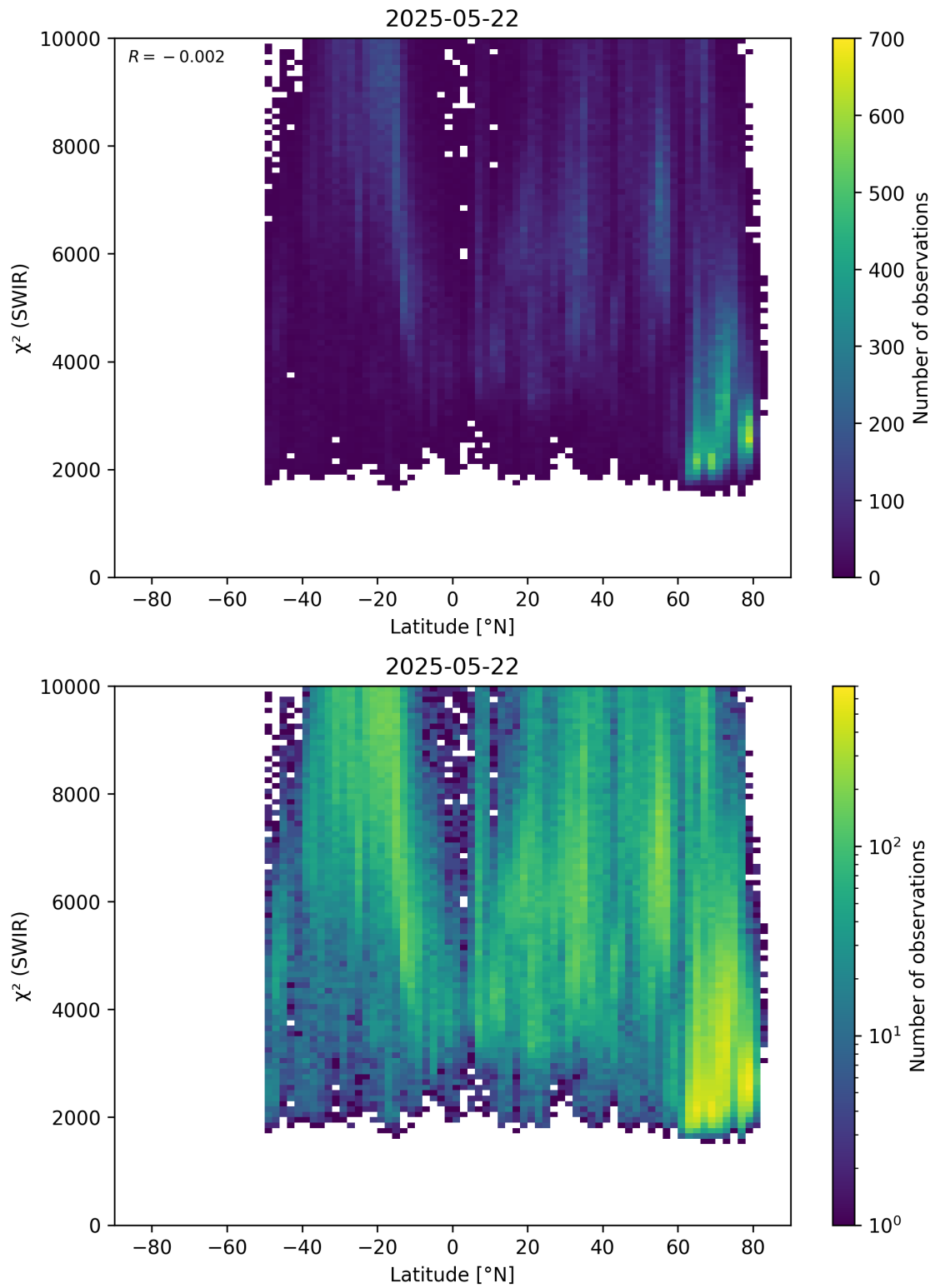
Figure 54: Scatter density plot of “Latitude” against “ \chi^2 (SWIR)” for 2025-05-21 to 2025-05-23.
