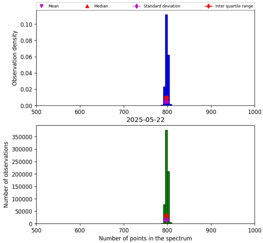
Figure 26: Histogram of “Number of points in the spectrum” for 2025-05-21 to 2025-05-23
