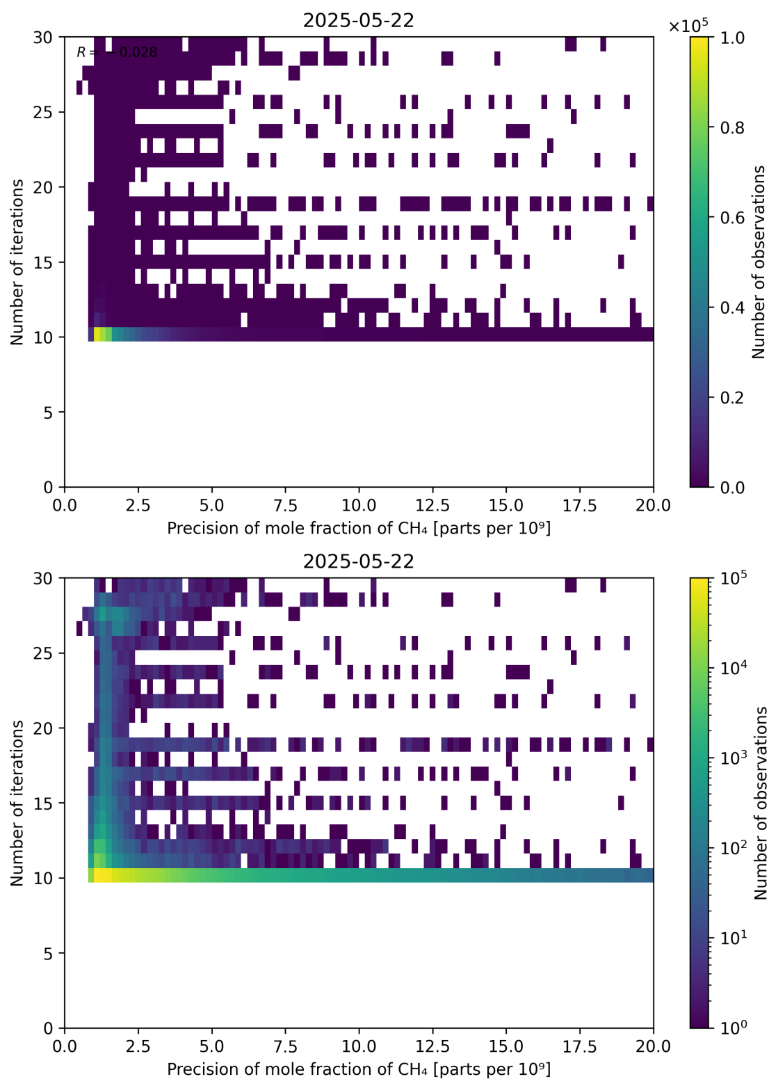
Figure 83: Scatter density plot of “Precision of mole fraction of CH 4 ” against “Number of iterations” for 2025-05-21 to 2025-05-23.
