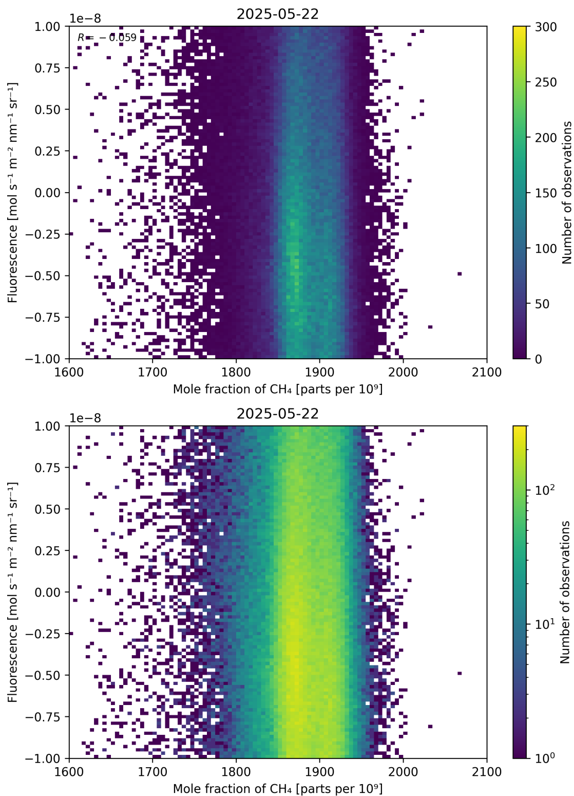
Figure 73: Scatter density plot of “Mole fraction of \text{CH}_4 ” against “Fluorescence” for 2025-05-21 to 2025-05-23.
