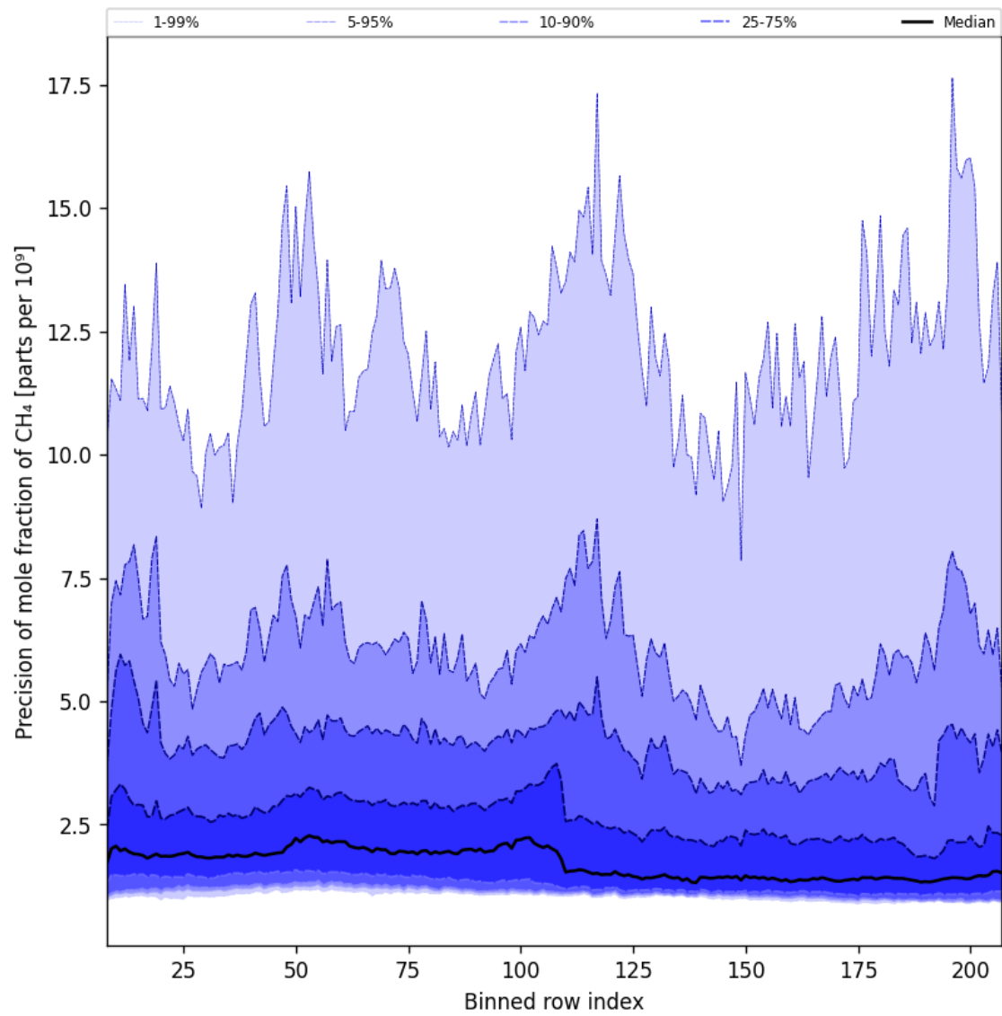
Figure 35: Along track statistics of “Precision of mole fraction of \text{CH}_4 ” for 2025-05-21 to 2025-05-23
