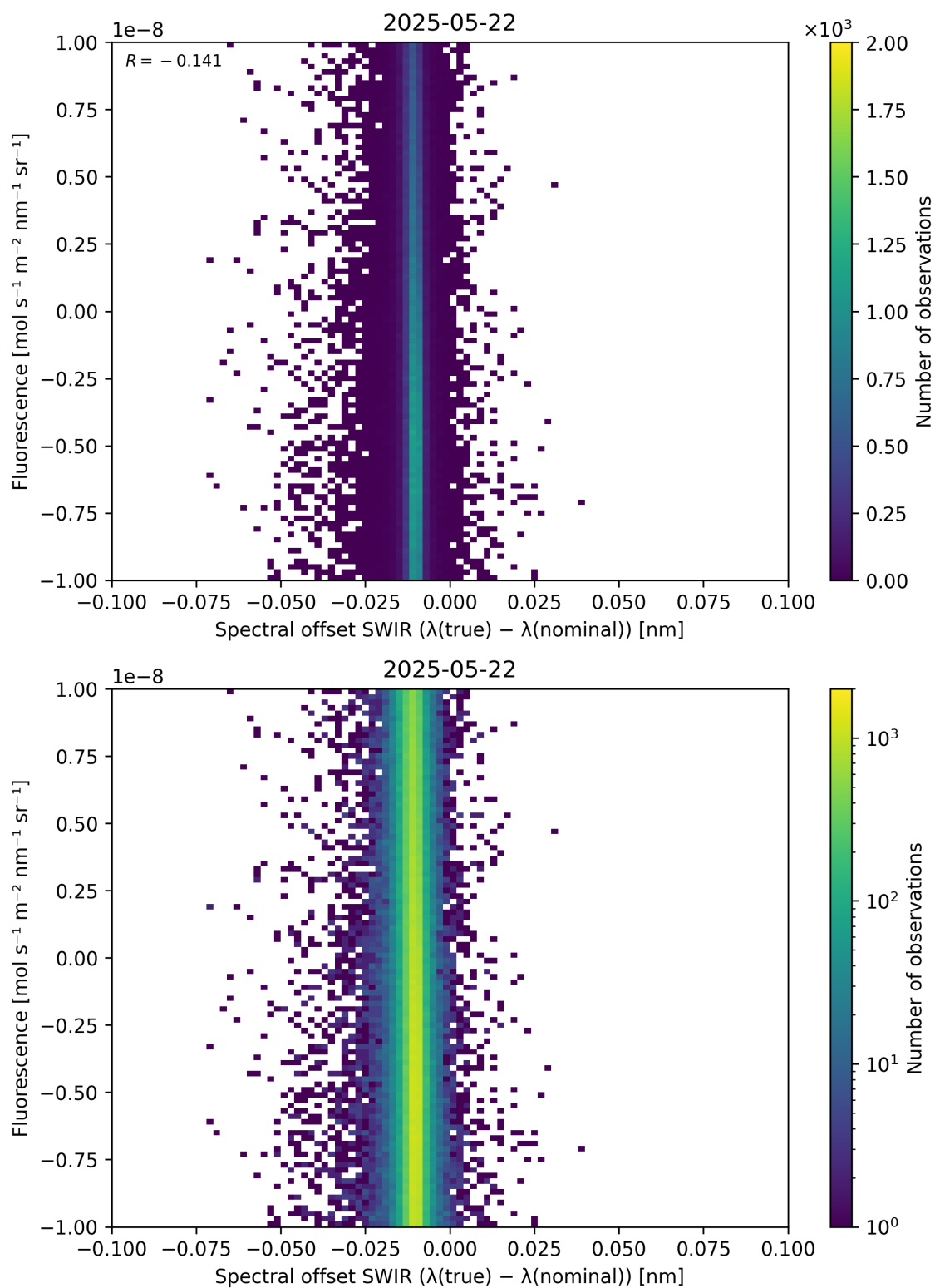
Figure 120: Scatter density plot of “Spectral offset SWIR ( \lambda_{\text{true}} - \lambda_{\text{nominal}} )” against “Fluorescence” for 2025-05-21 to 2025-05-23.
