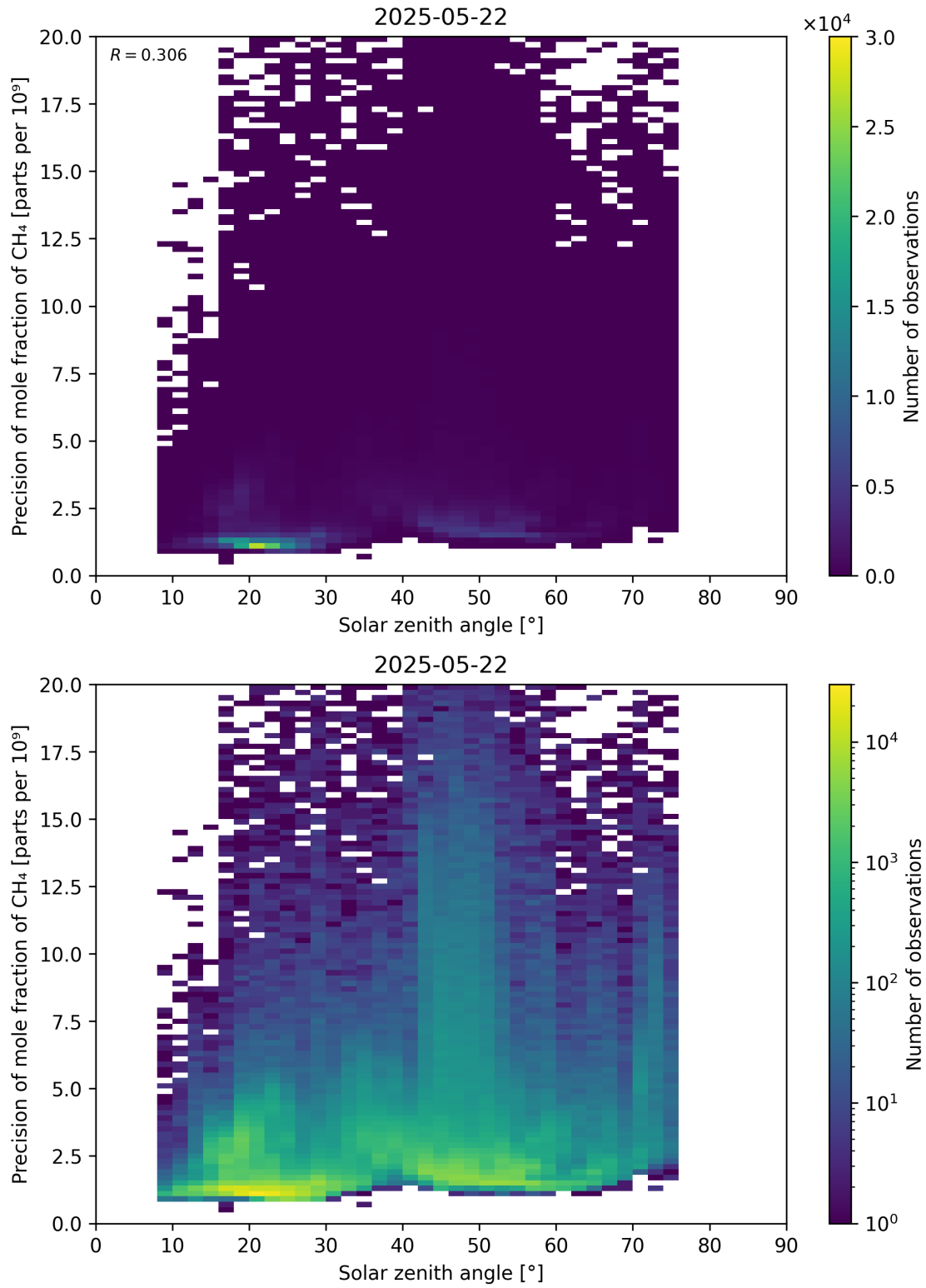
Figure 101: Scatter density plot of “Solar zenith angle” against “Precision of mole fraction of \text{CH}_4 ” for 2025-05-21 to 2025-05-23.
