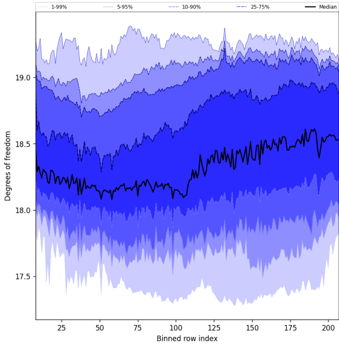
Figure 41: Along track statistics of “Degrees of freedom” for 2025-05-21 to 2025-05-23
