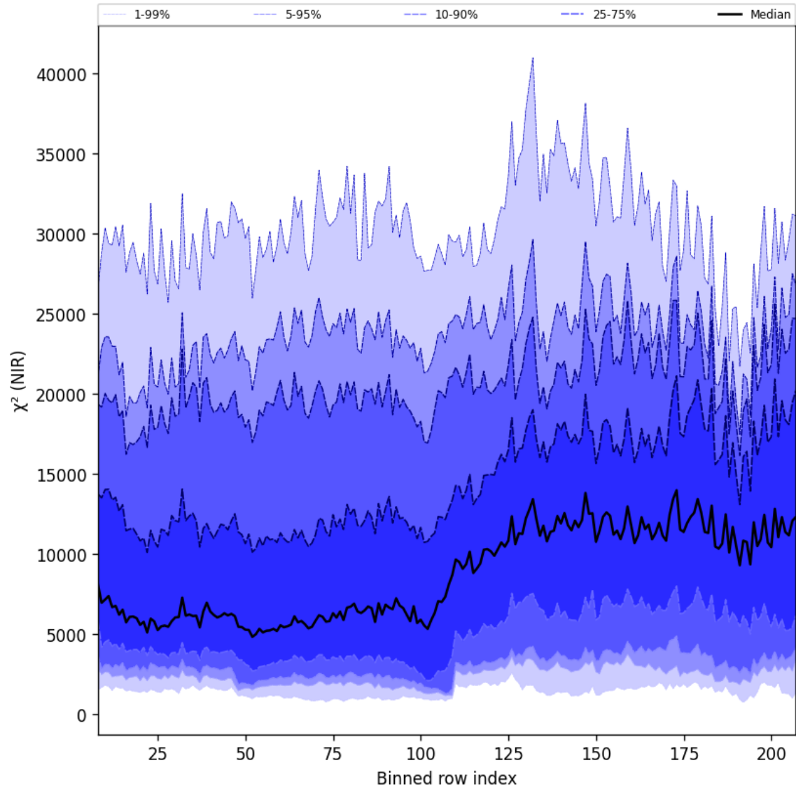
Figure 40: Along track statistics of “ \chi^2 (NIR)” for 2025-05-21 to 2025-05-23
