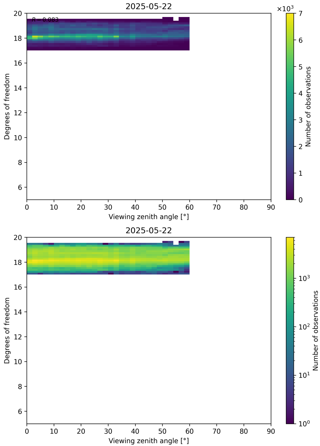
Figure 107: Scatter density plot of “Viewing zenith angle” against “Degrees of freedom” for 2025-05-21 to 2025-05-23.
