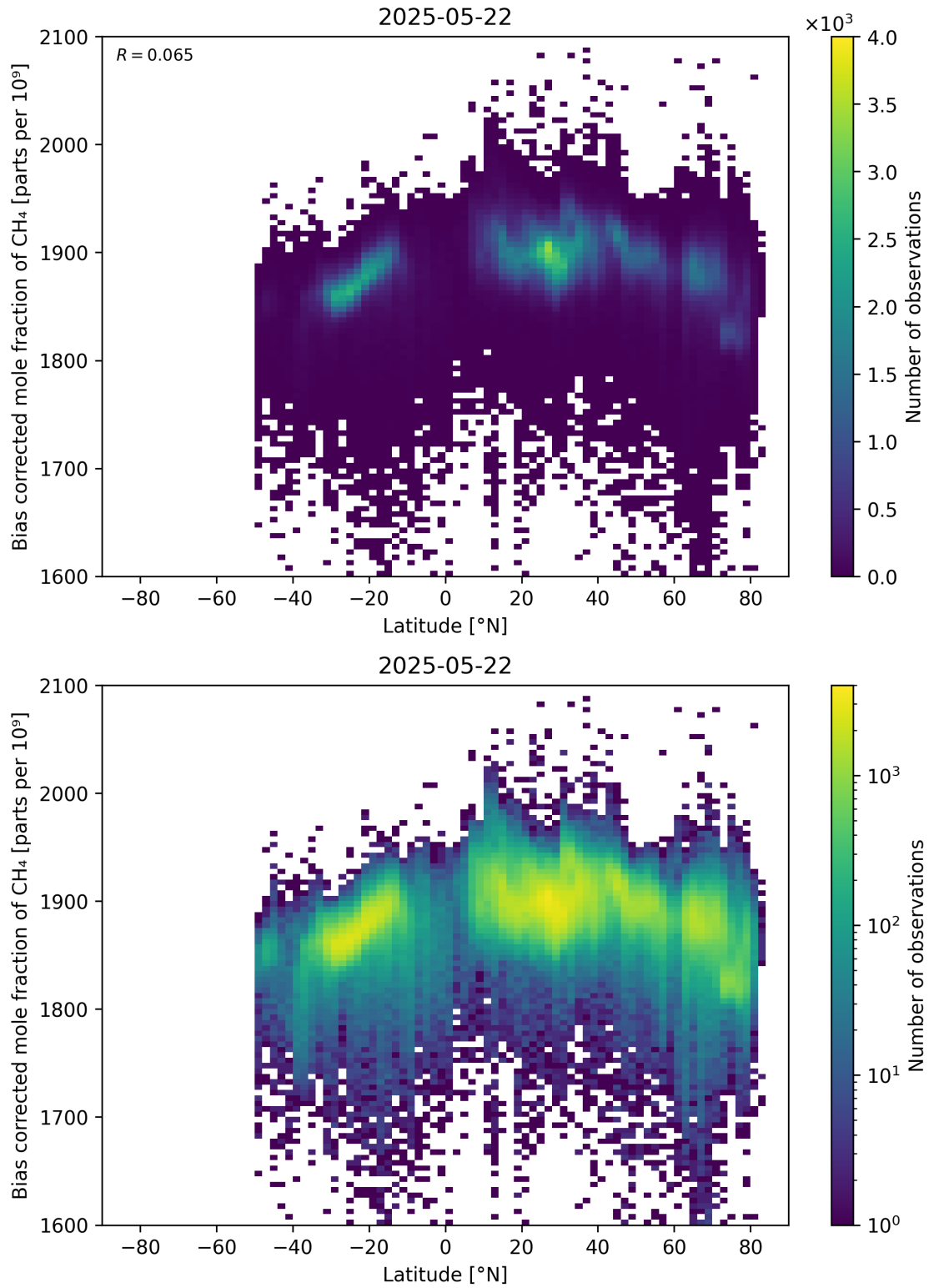
Figure 58: Scatter density plot of “Latitude” against “Bias corrected mole fraction of CH 4 ” for 2025-05-21 to 2025-05-23.
