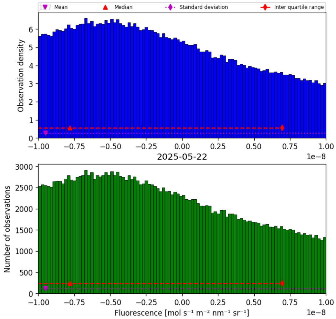
Figure 32: Histogram of “Fluorescence” for 2025-05-21 to 2025-05-23
