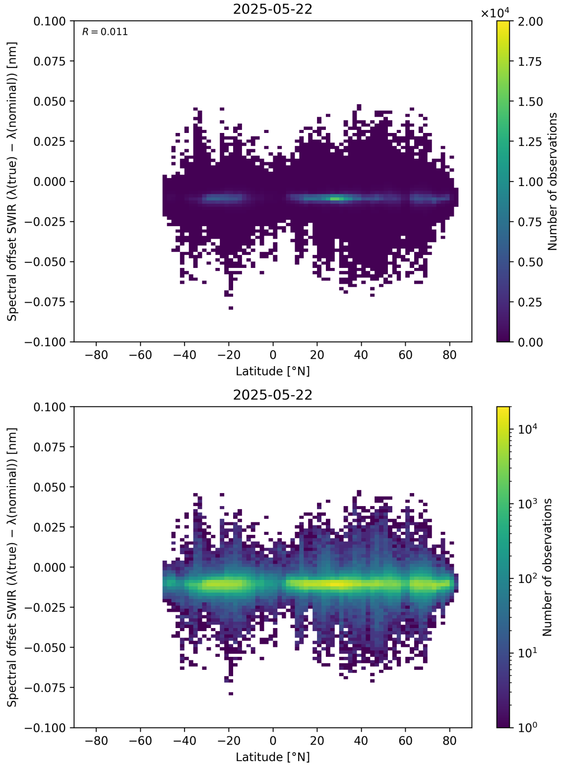
Figure 62: Scatter density plot of “Latitude” against “Spectral offset SWIR ( \lambda_{\text{true}} - \lambda_{\text{nominal}} )” for 2025-05-21 to 2025-05-23.
