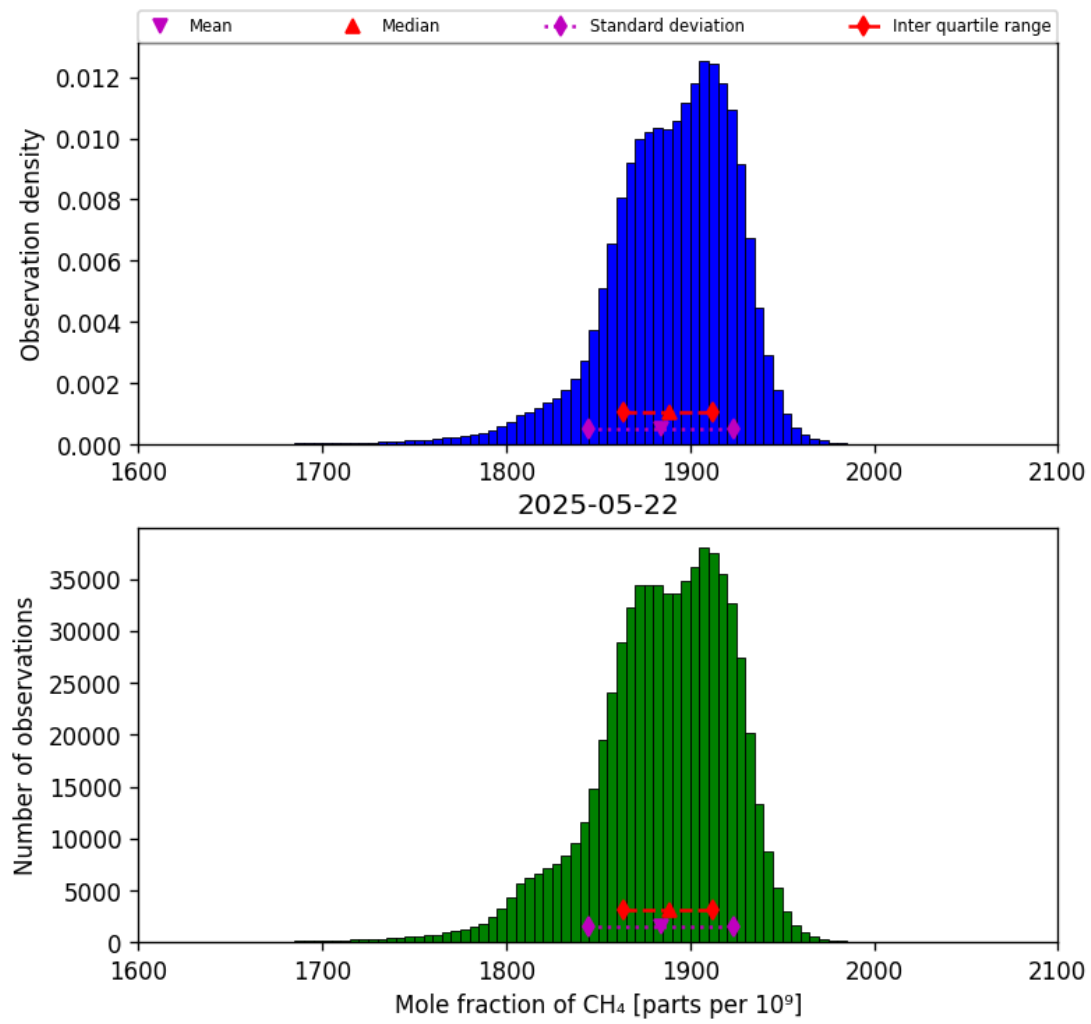
Figure 23: Histogram of “Mole fraction of CH 4 ” for 2025-05-21 to 2025-05-23
