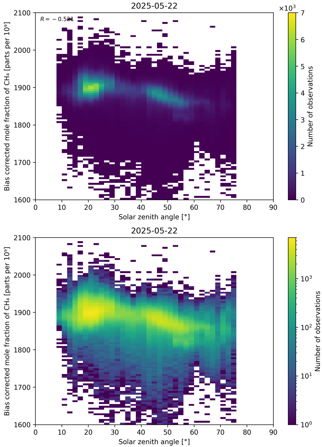
Figure 100: Scatter density plot of “Solar zenith angle” against “Bias corrected mole fraction of CH 4 ” for 2025-05-21 to 2025-05-23.
