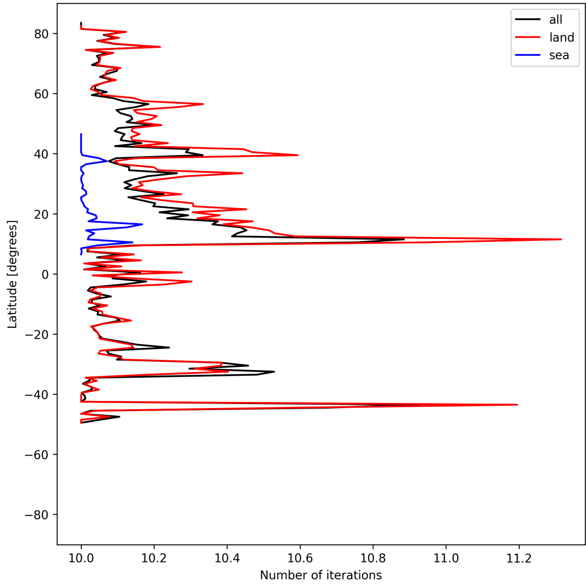
Figure 20: Zonal average of “Number of iterations” for 2025-05-21 to 2025-05-23.
