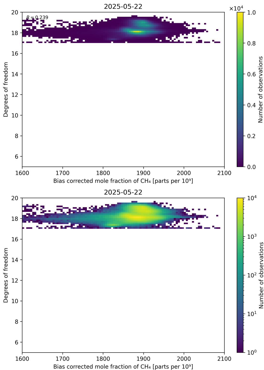
Figure 65: Scatter density plot of “Bias corrected mole fraction of CH 4 ” against “Degrees of freedom” for 2025-05-21 to 2025-05-23.
