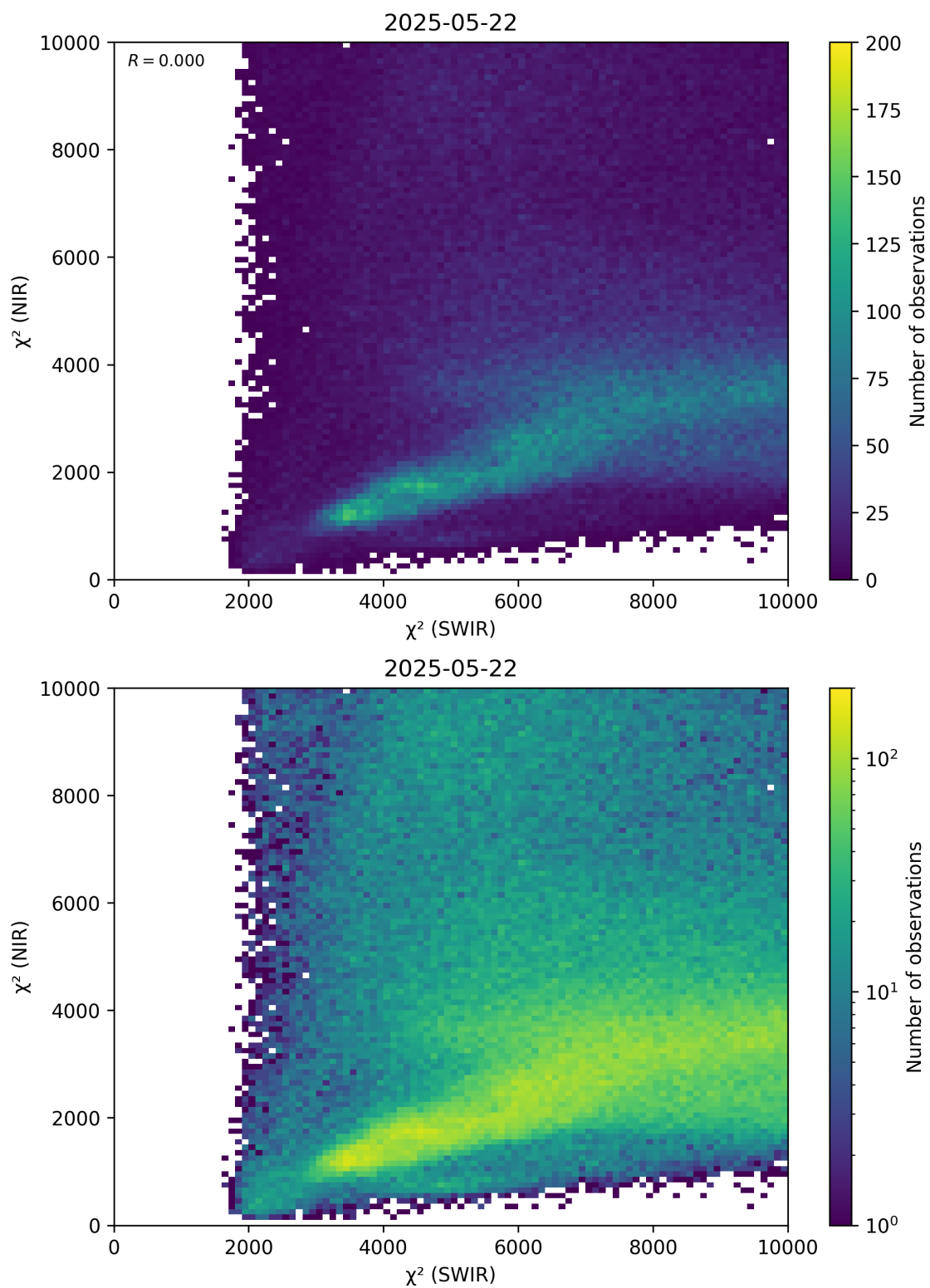
Figure 47: Scatter density plot of “ \chi^2 (SWIR)” against “ \chi^2 (NIR)” for 2025-05-21 to 2025-05-23.
