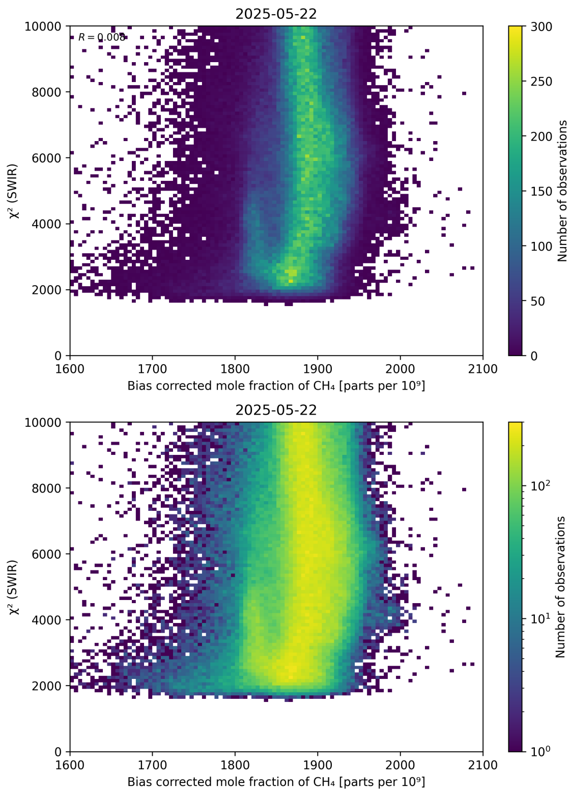
Figure 64: Scatter density plot of “Bias corrected mole fraction of \text{CH}_4 ” against “ \chi^2 (SWIR)” for 2025-05-21 to 2025-05-23.
