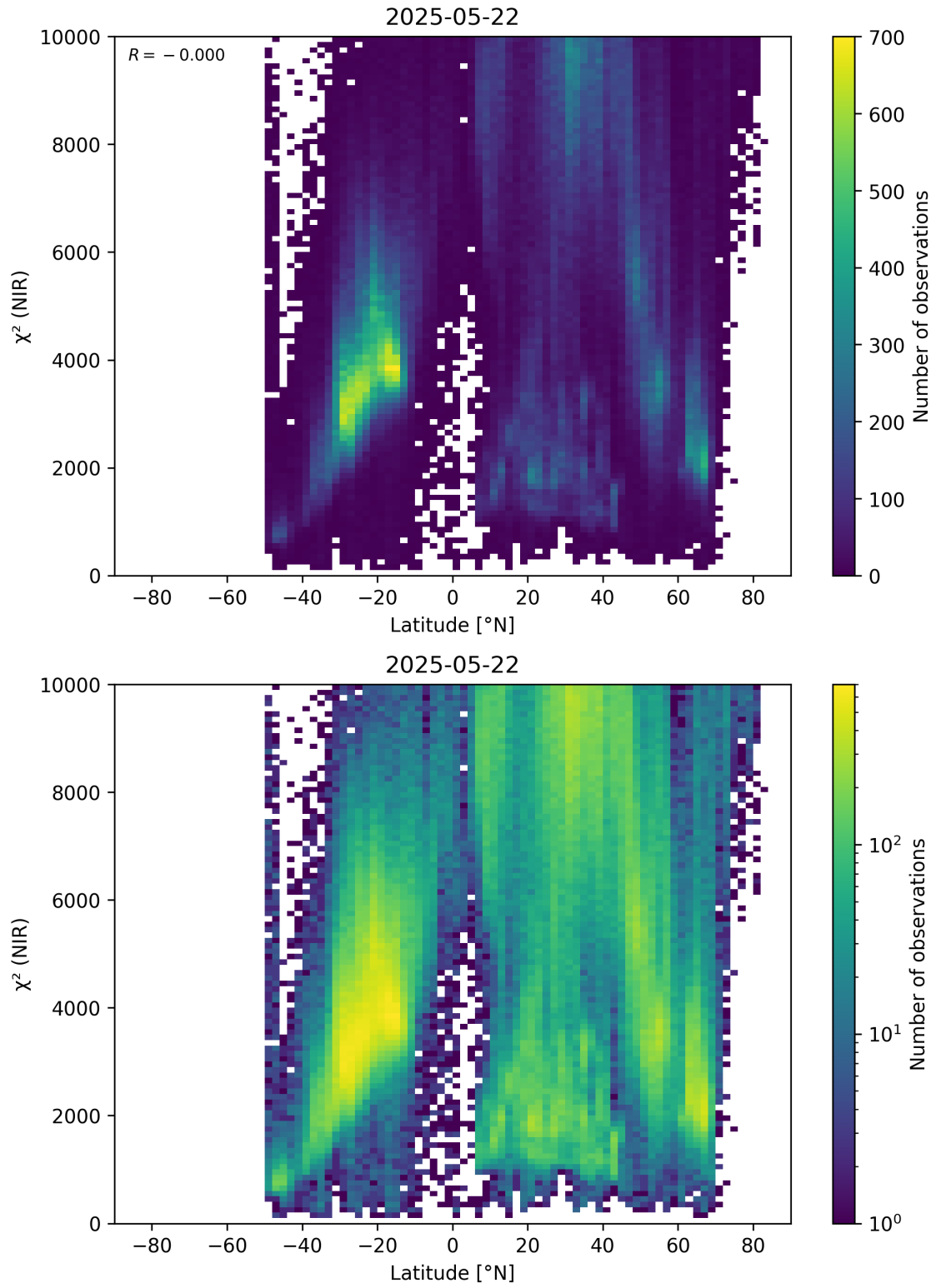
Figure 53: Scatter density plot of “Latitude” against “ \chi^2 (NIR)” for 2025-05-21 to 2025-05-23.
