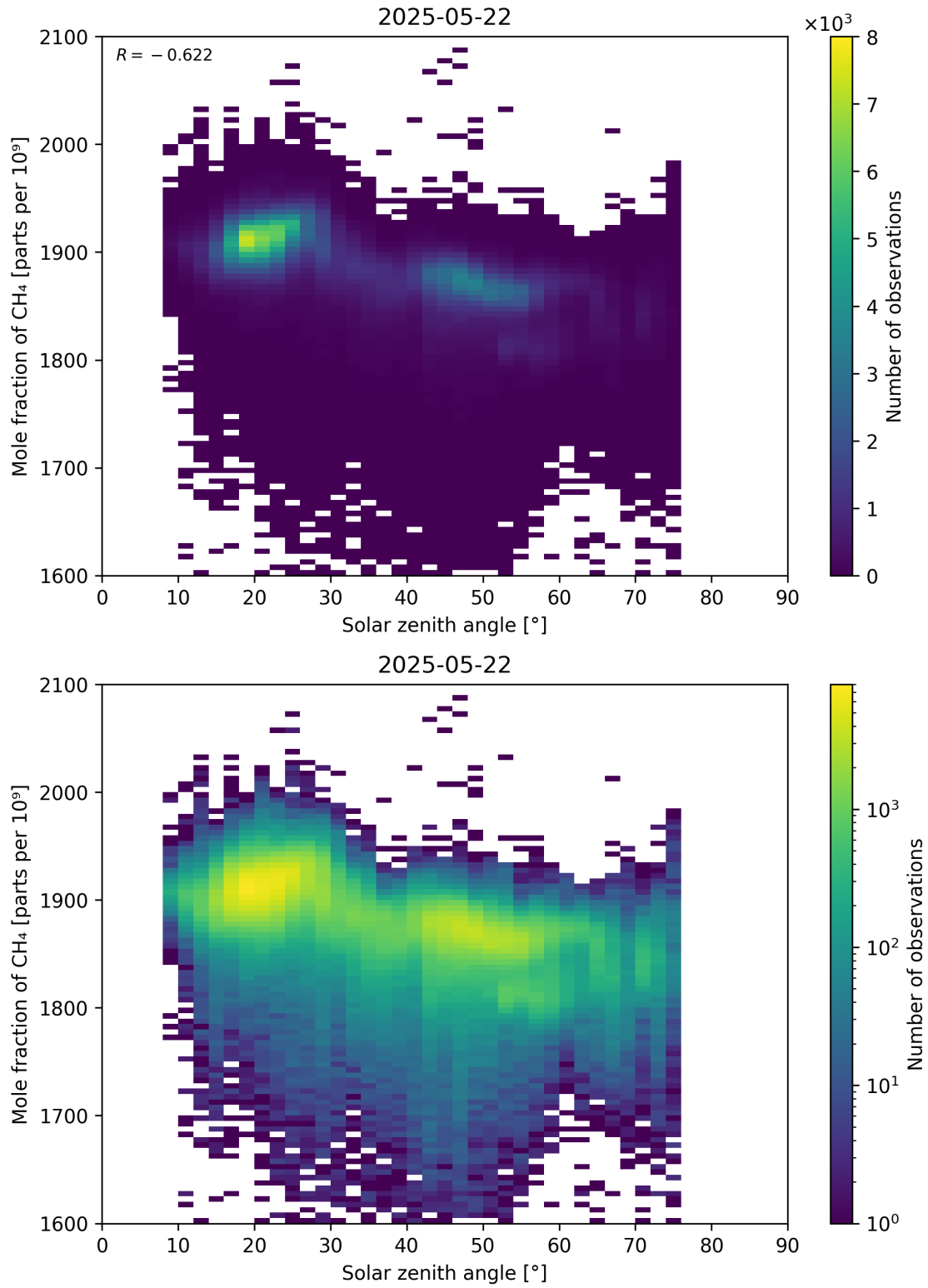
Figure 99: Scatter density plot of “Solar zenith angle” against “Mole fraction of \text{CH}_4 ” for 2025-05-21 to 2025-05-23.
