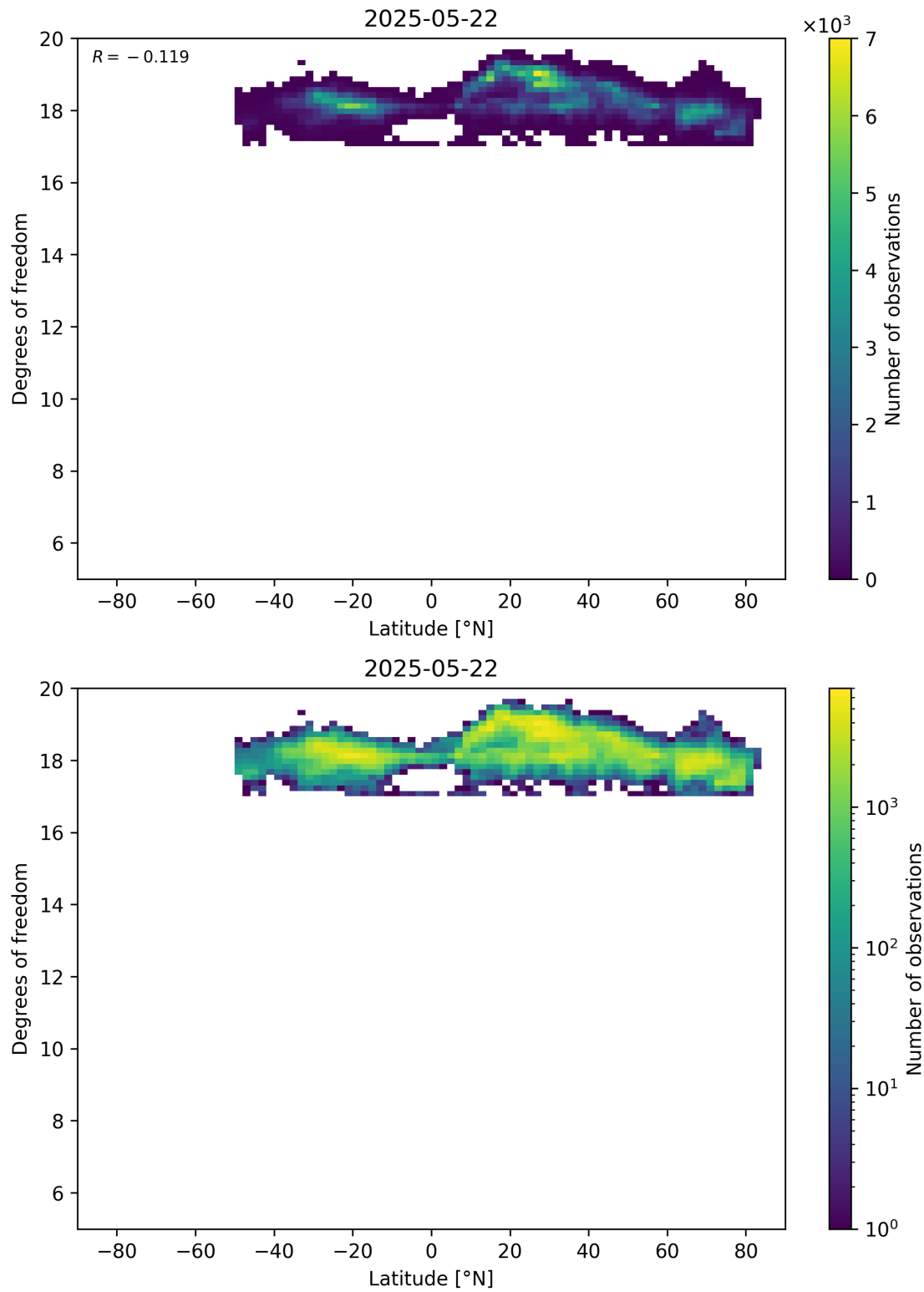
Figure 55: Scatter density plot of “Latitude” against “Degrees of freedom” for 2025-05-21 to 2025-05-23.
