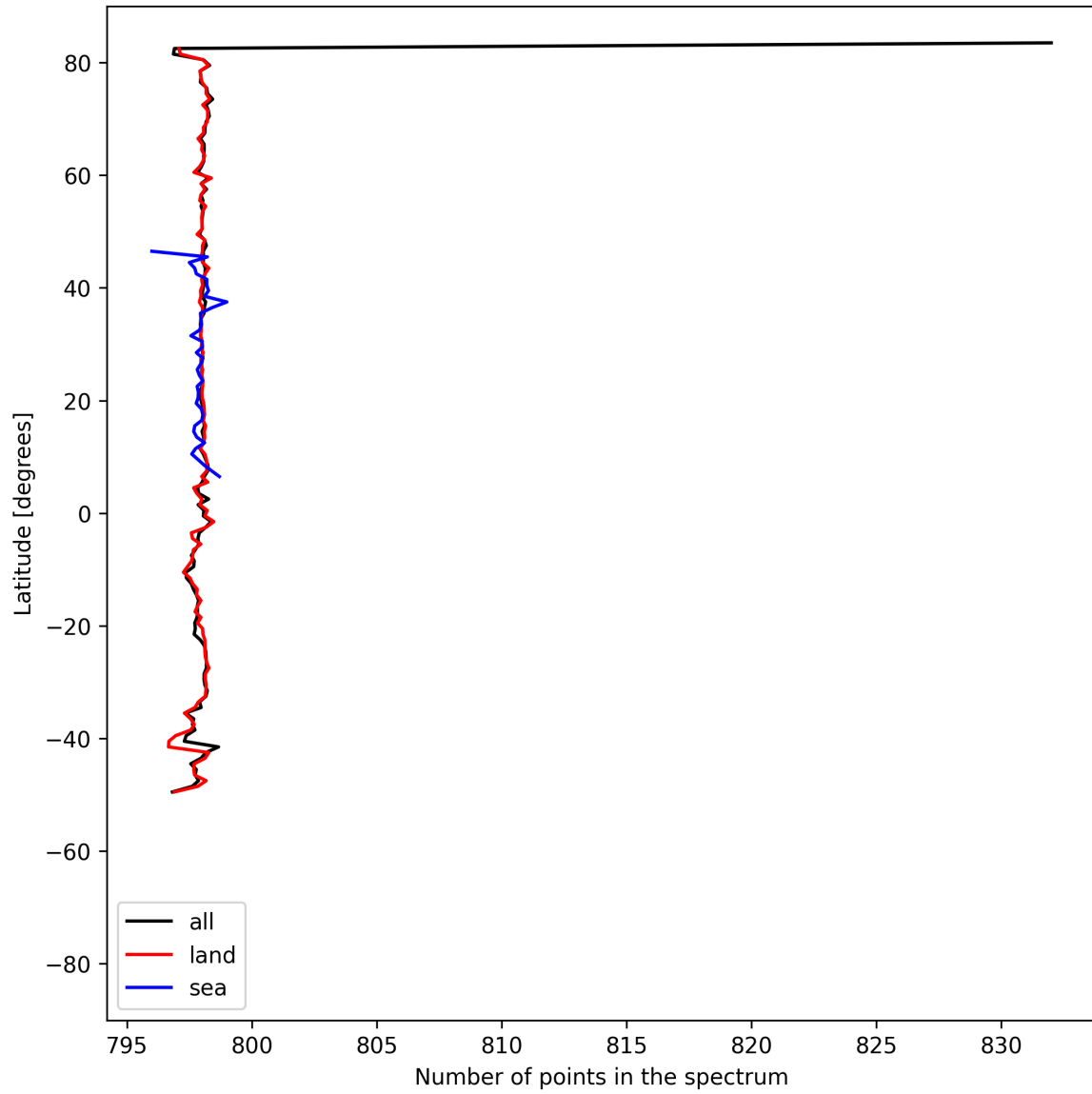
Figure 15: Zonal average of “Number of points in the spectrum” for 2025-05-21 to 2025-05-23.
