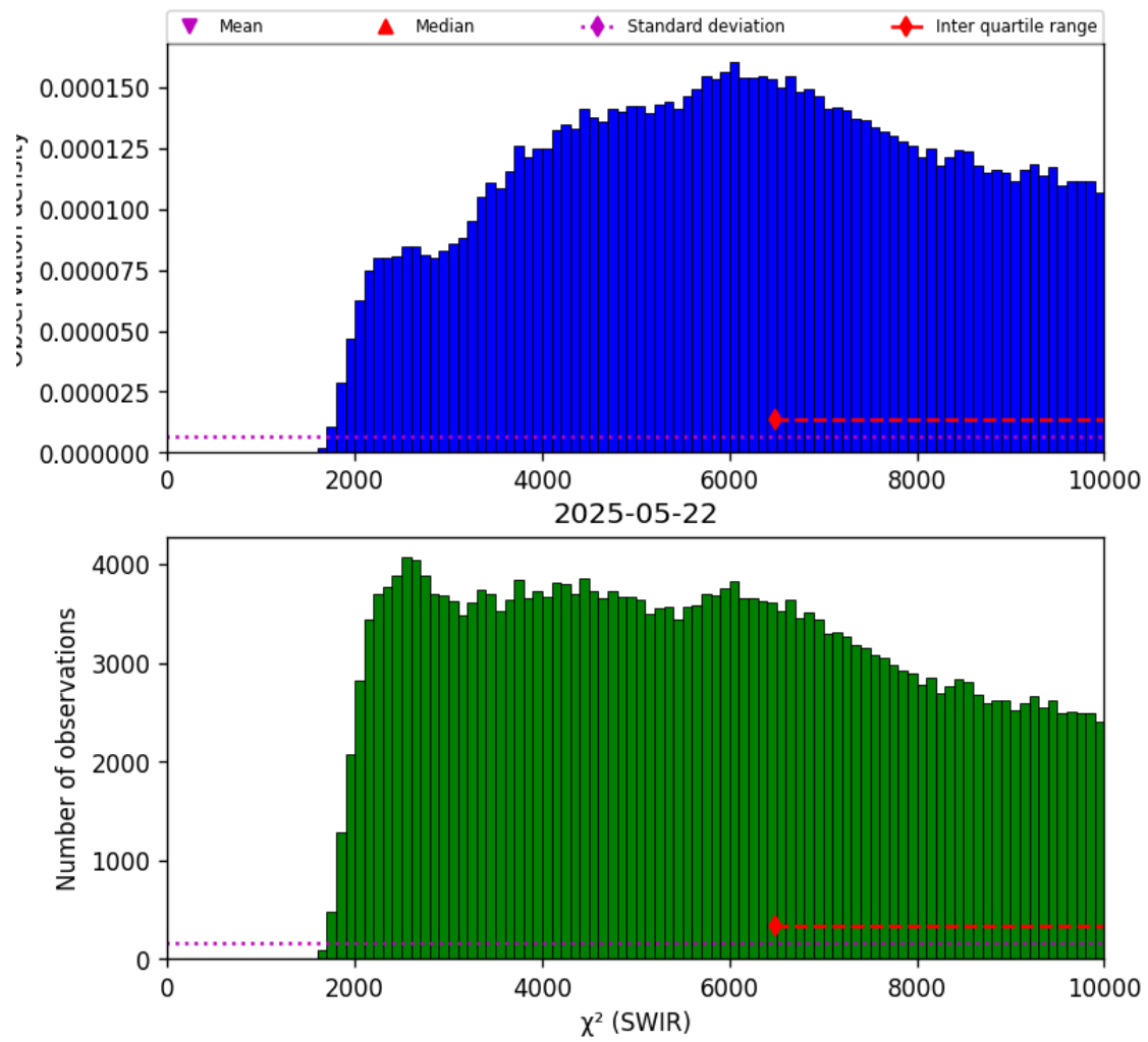
Figure 28: Histogram of “ \chi^2 (SWIR)” for 2025-05-21 to 2025-05-23
