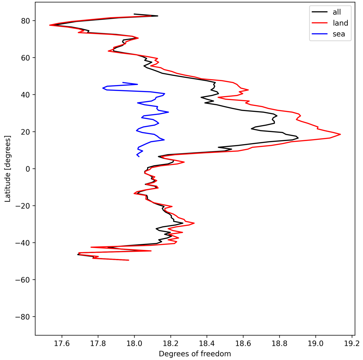
Figure 19: Zonal average of “Degrees of freedom” for 2025-05-21 to 2025-05-23.
