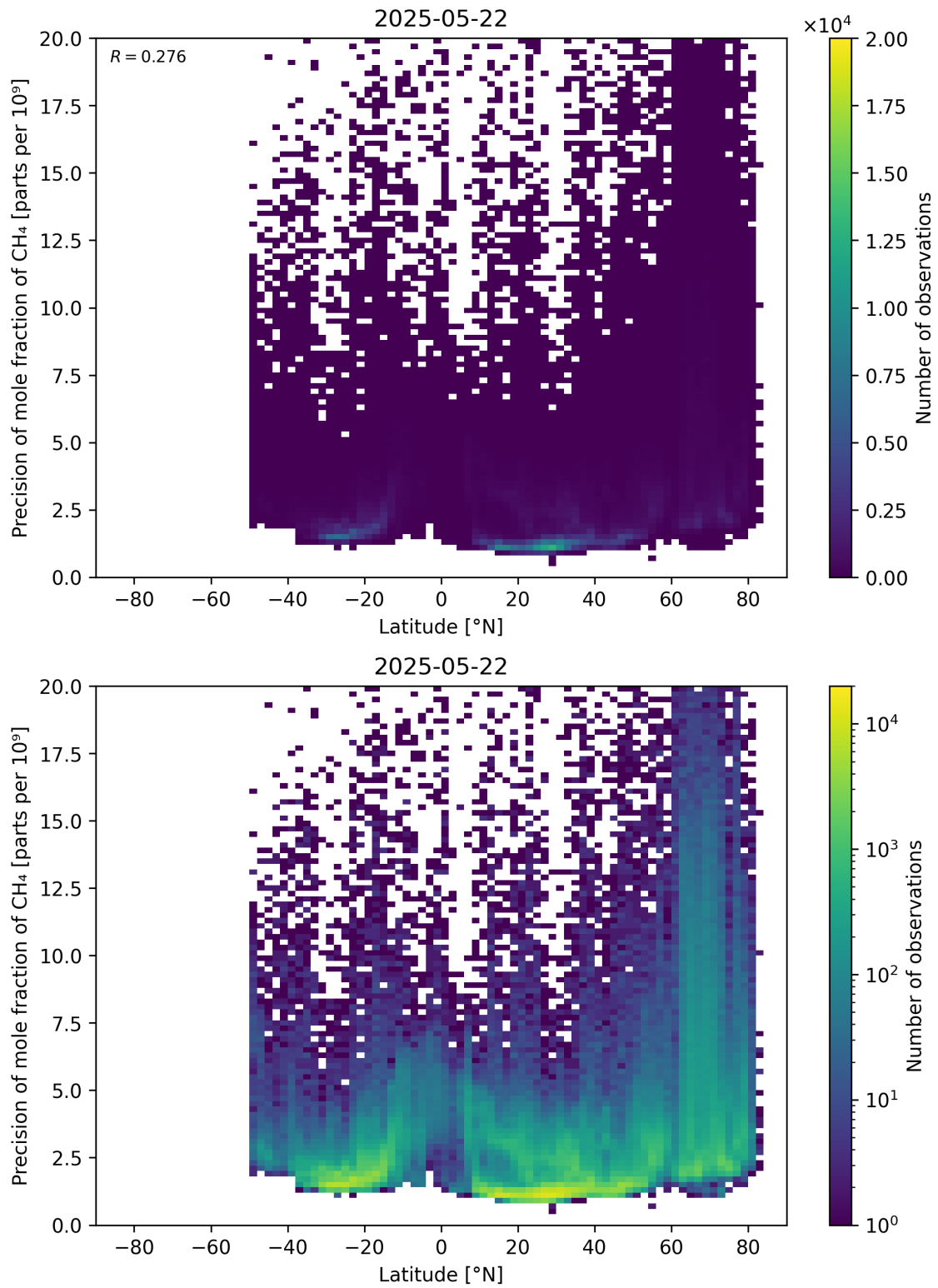
Figure 59: Scatter density plot of “Latitude” against “Precision of mole fraction of \text{CH}_4 ” for 2025-05-21 to 2025-05-23.
