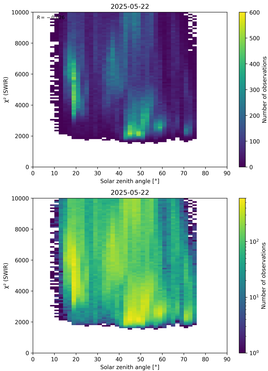
Figure 95: Scatter density plot of “Solar zenith angle” against “ \chi^2 (SWIR)” for 2025-05-21 to 2025-05-23.
