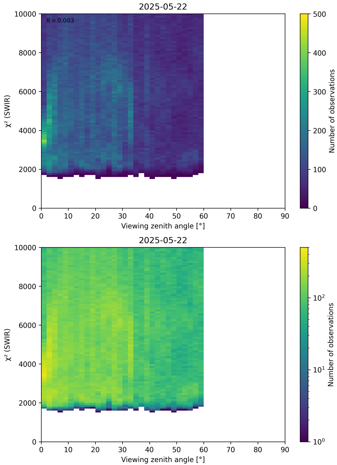
Figure 106: Scatter density plot of “Viewing zenith angle” against “ \chi^2 (SWIR)” for 2025-05-21 to 2025-05-23.
