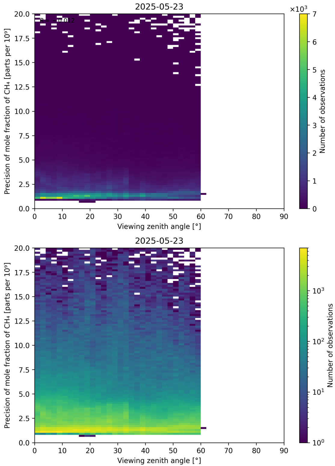
Figure 112: Scatter density plot of “Viewing zenith angle” against “Precision of mole fraction of CH 4 ” for 2025-05-22 to 2025-05-24.
