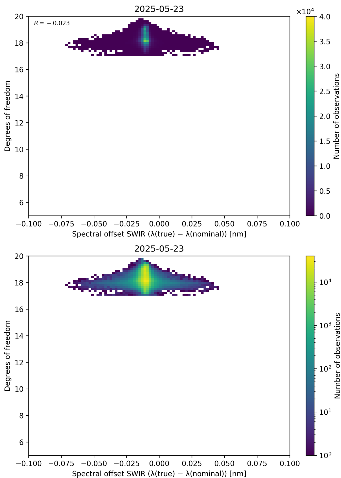
Figure 119: Scatter density plot of “Spectral offset SWIR ( \lambda_{\text{true}} - \lambda_{\text{nominal}} )” against “Degrees of freedom” for 2025-05-22 to 2025-05-24.
