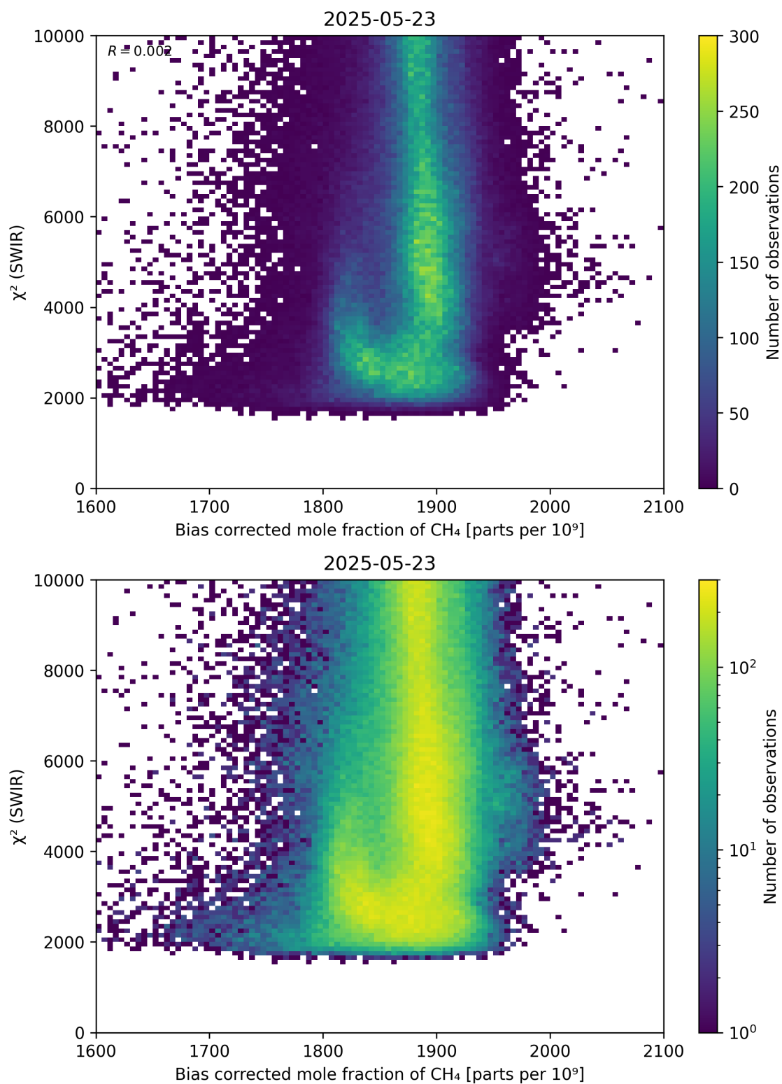
Figure 64: Scatter density plot of “Bias corrected mole fraction of CH 4 ” against “ \chi^2 (SWIR)” for 2025-05-22 to 2025-05-24.
