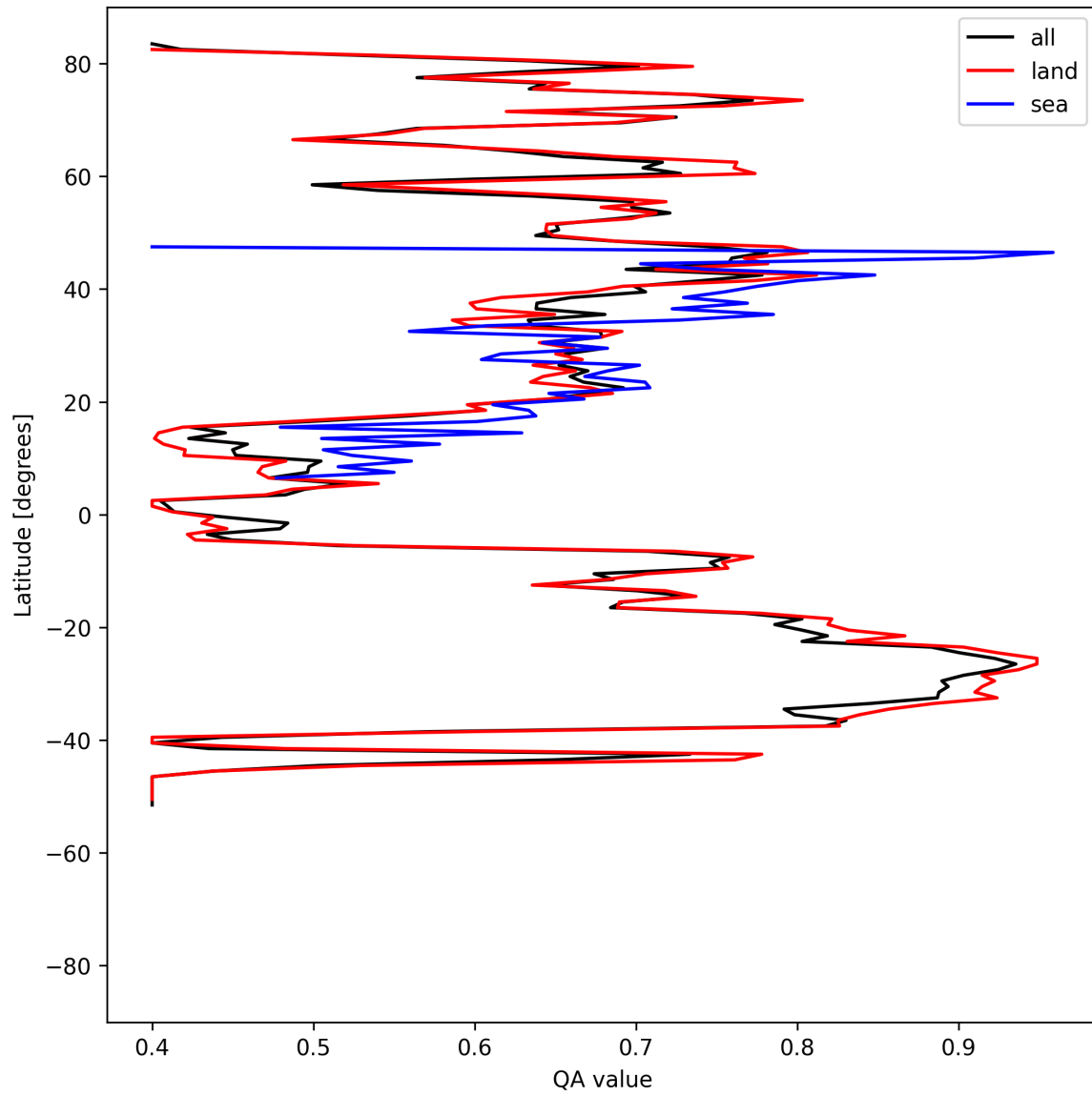
Figure 11: Zonal average of “QA value” for 2025-05-22 to 2025-05-24.
