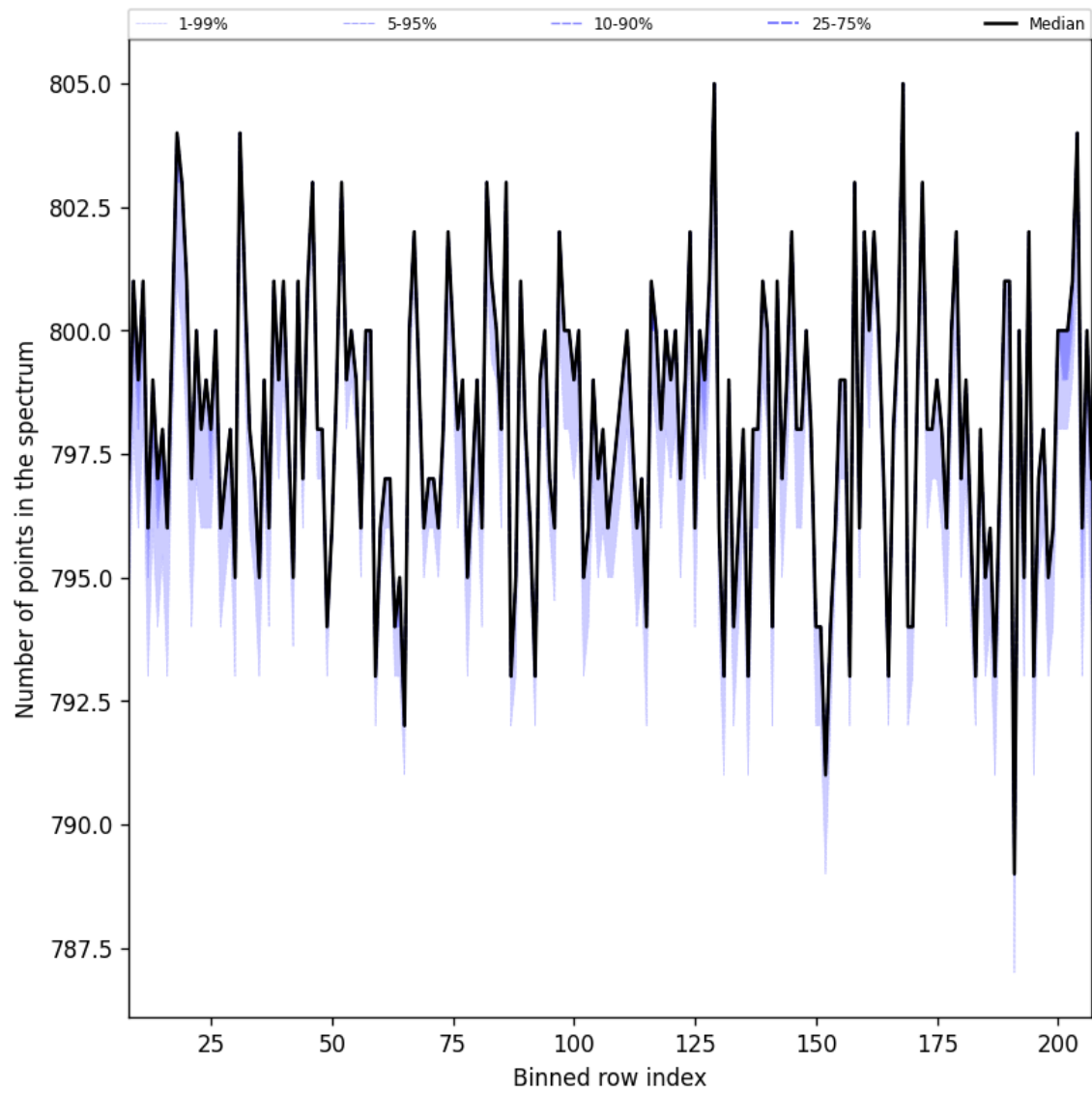
Figure 37: Along track statistics of “Number of points in the spectrum” for 2025-05-22 to 2025-05-24
