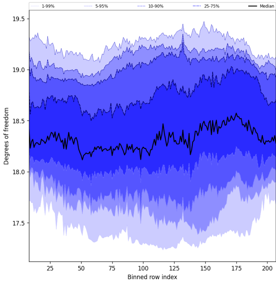
Figure 41: Along track statistics of “Degrees of freedom” for 2025-05-22 to 2025-05-24
