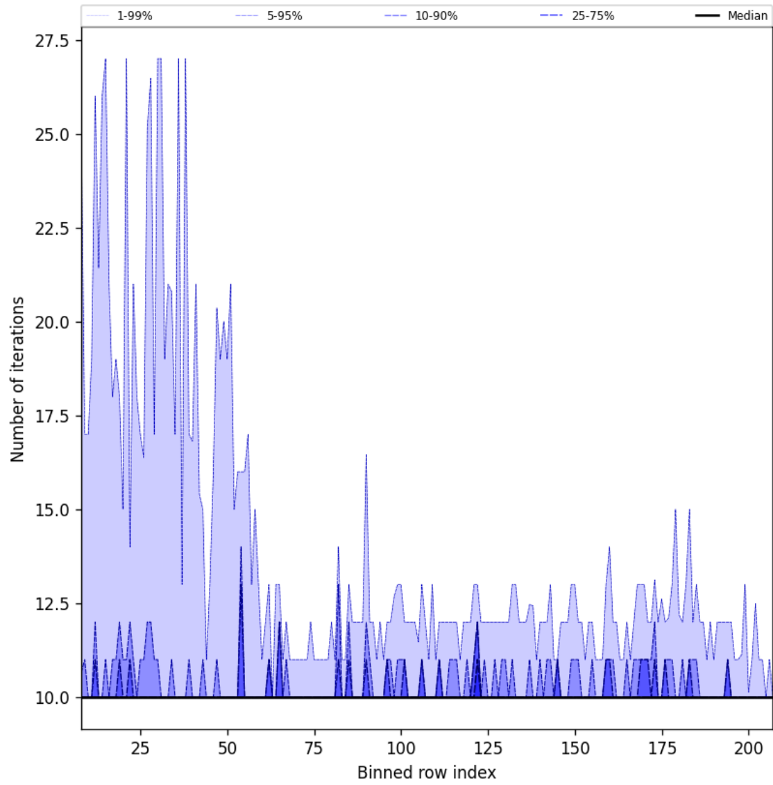
Figure 42: Along track statistics of “Number of iterations” for 2025-05-22 to 2025-05-24
