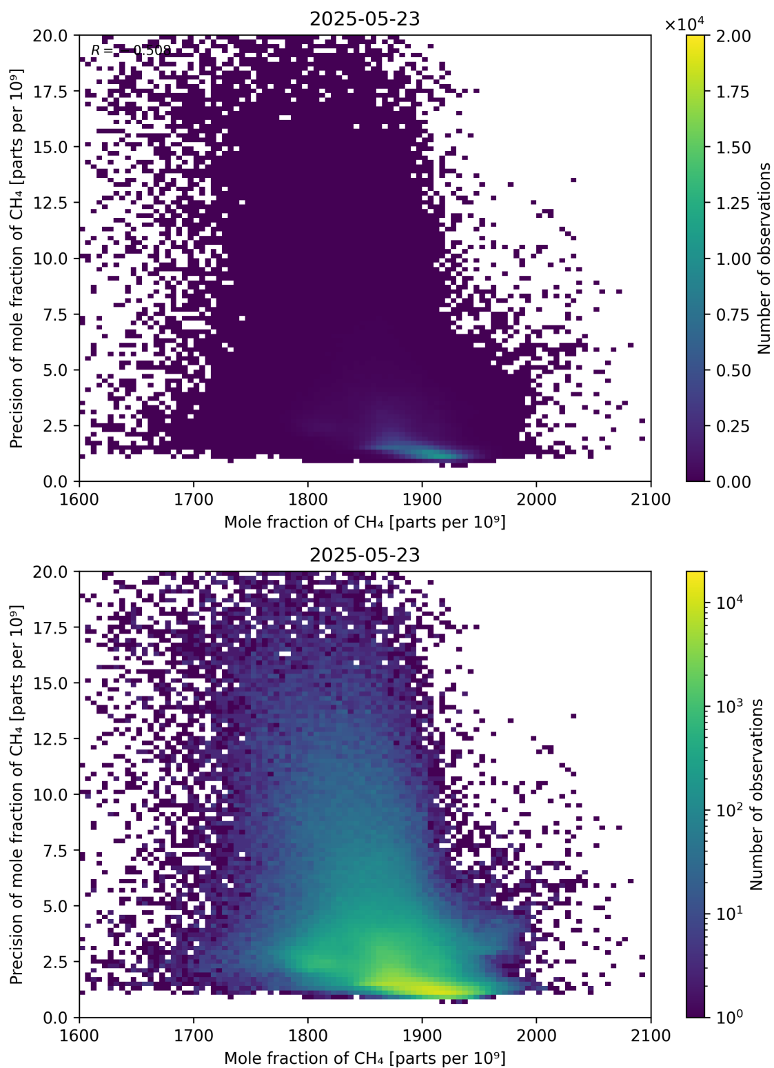
Figure 75: Scatter density plot of “Mole fraction of CH 4 ” against “Precision of mole fraction of CH 4 ” for 2025-05-22 to 2025-05-24.
