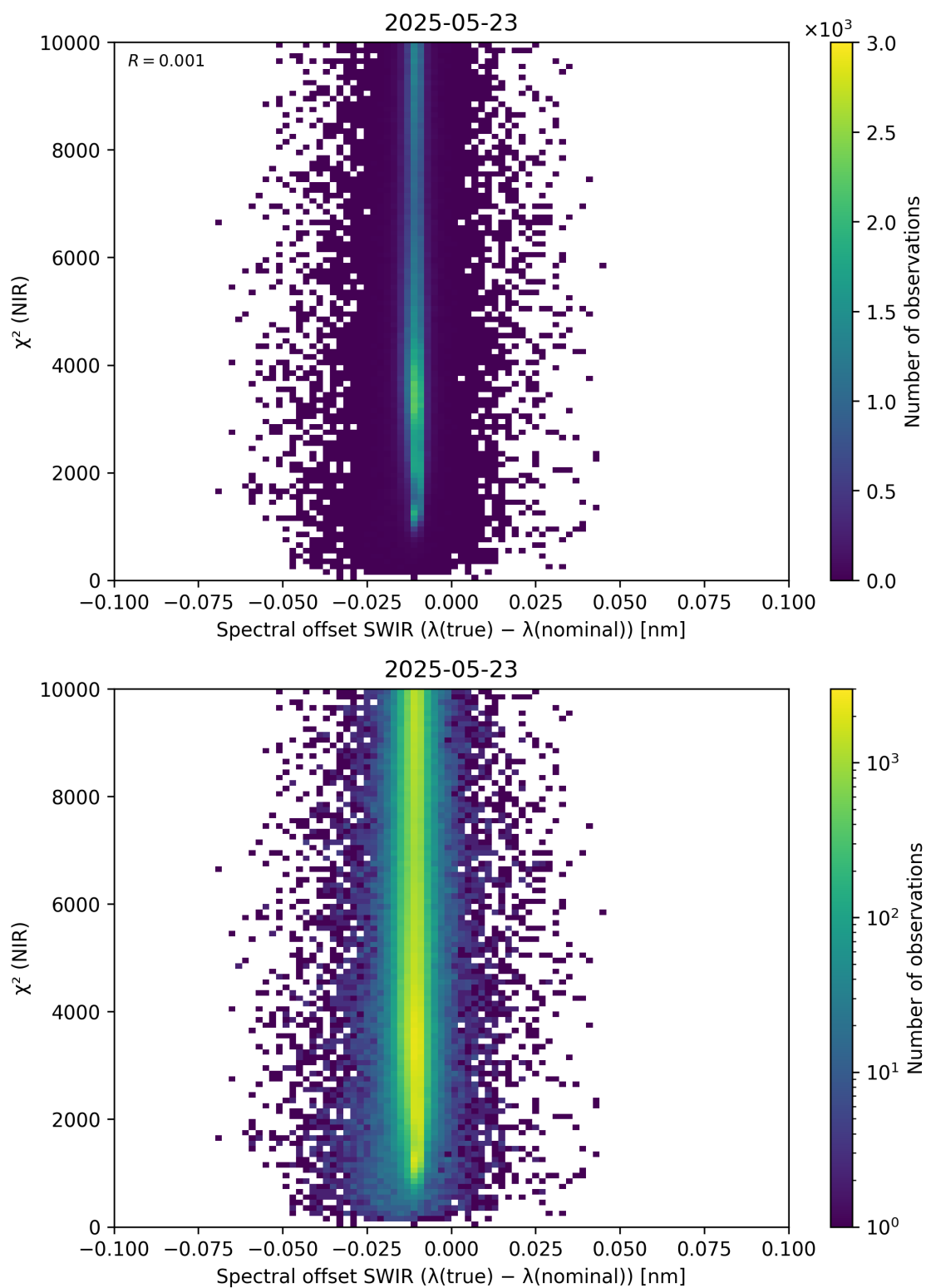
Figure 117: Scatter density plot of “Spectral offset SWIR ( \lambda_{\text{true}} - \lambda_{\text{nominal}} )” against “ \chi^2 (NIR)” for 2025-05-22 to 2025-05-24.
