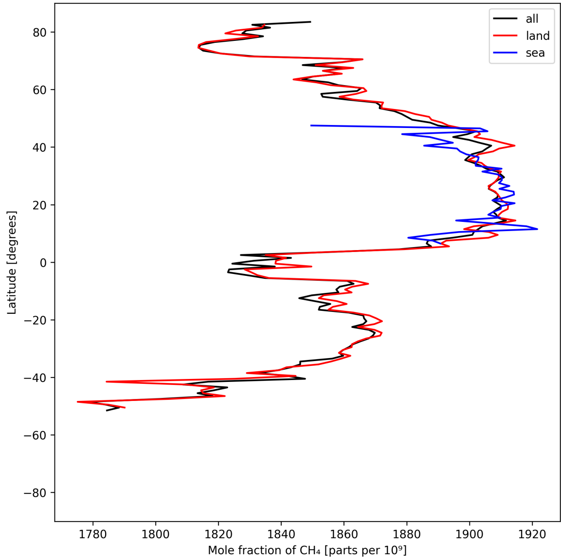
Figure 12: Zonal average of “Mole fraction of \text{CH}_4 ” for 2025-05-22 to 2025-05-24.
