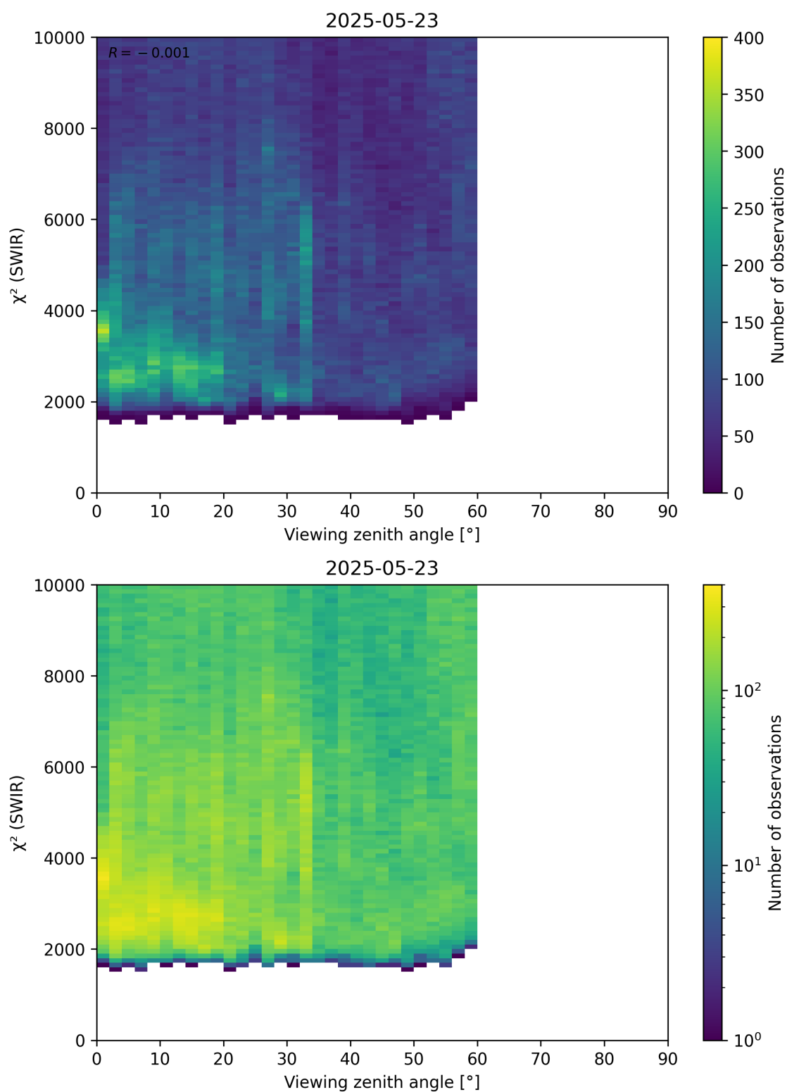
Figure 106: Scatter density plot of “Viewing zenith angle” against “ \chi^2 (SWIR)” for 2025-05-22 to 2025-05-24.
