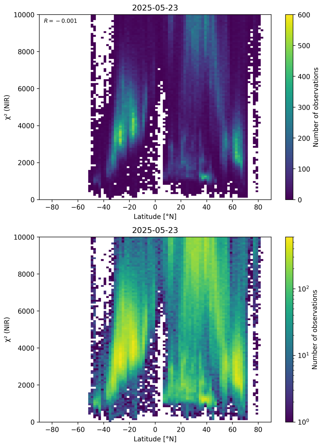
Figure 53: Scatter density plot of “Latitude” against “ \chi^2 (NIR)” for 2025-05-22 to 2025-05-24.
