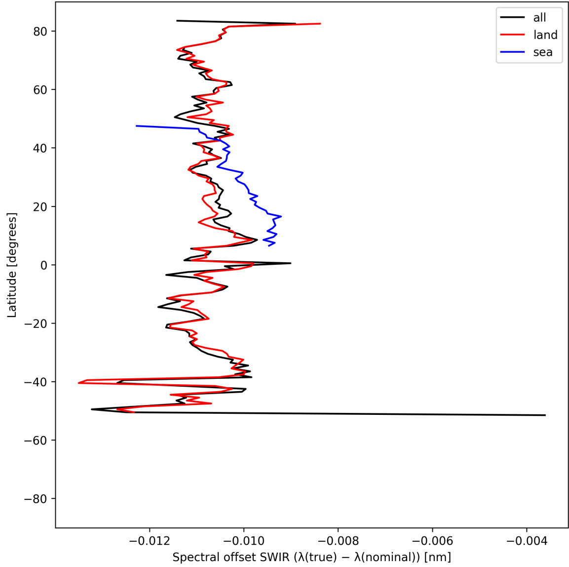
Figure 16: Zonal average of “Spectral offset SWIR ( \lambda_{\text{true}} - \lambda_{\text{nominal}} )” for 2025-05-22 to 2025-05-24.
