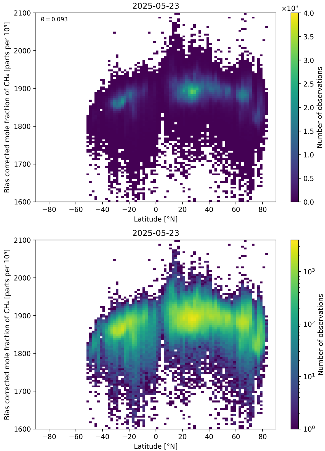
Figure 58: Scatter density plot of “Latitude” against “Bias corrected mole fraction of CH 4 ” for 2025-05-22 to 2025-05-24.
