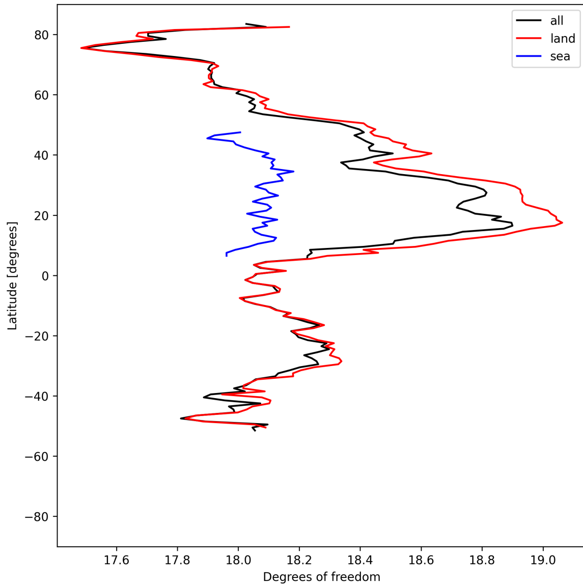
Figure 19: Zonal average of “Degrees of freedom” for 2025-05-22 to 2025-05-24.
