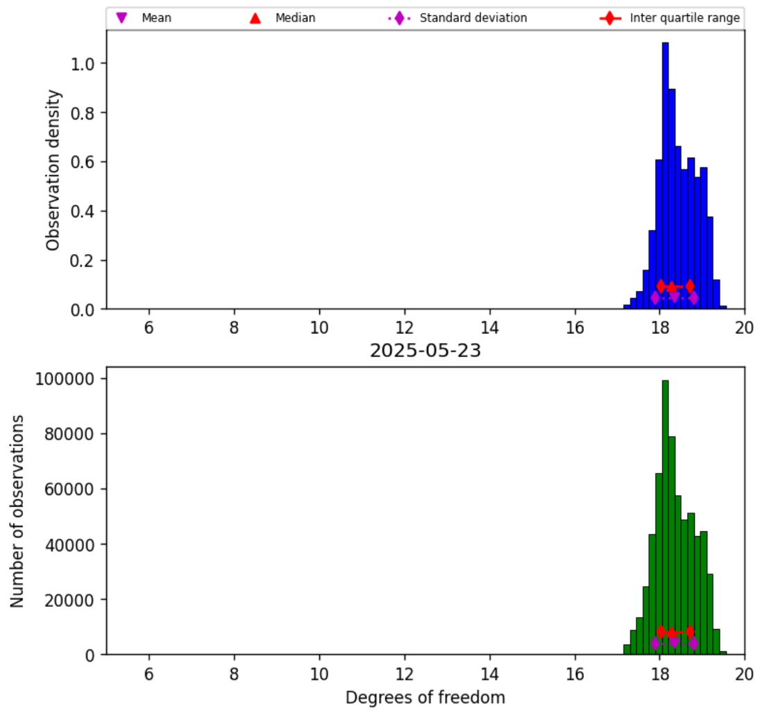
Figure 30: Histogram of “Degrees of freedom” for 2025-05-22 to 2025-05-24
