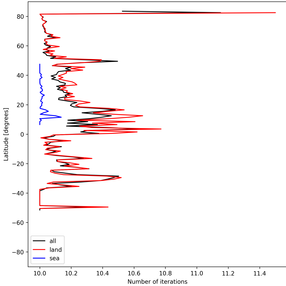
Figure 20: Zonal average of “Number of iterations” for 2025-05-22 to 2025-05-24.
