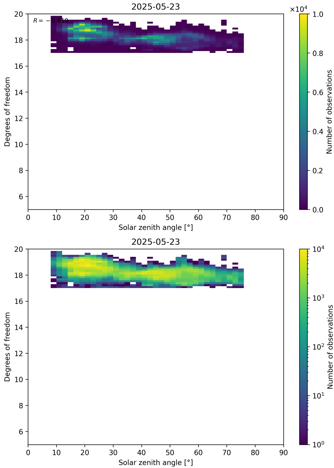
Figure 96: Scatter density plot of “Solar zenith angle” against “Degrees of freedom” for 2025-05-22 to 2025-05-24.
