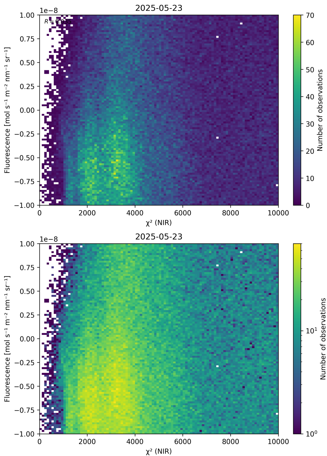
Figure 45: Scatter density plot of “ \chi^2 (NIR)” against “Fluorescence” for 2025-05-22 to 2025-05-24.
