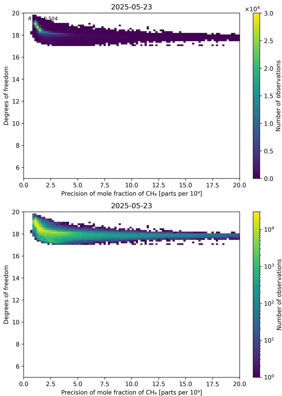
Figure 80: Scatter density plot of “Precision of mole fraction of CH 4 ” against “Degrees of freedom” for 2025-05-22 to 2025-05-24.
