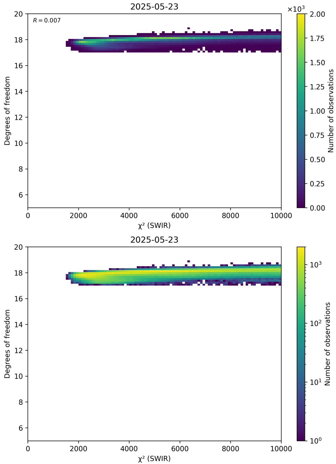
Figure 48: Scatter density plot of “ \chi^2 (SWIR)” against “Degrees of freedom” for 2025-05-22 to 2025-05-24.
