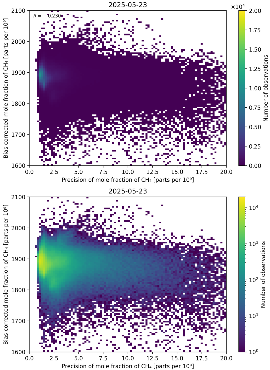
Figure 82: Scatter density plot of “Precision of mole fraction of CH 4 ” against “Bias corrected mole fraction of CH 4 ” for 2025-05-22 to 2025-05-24.
