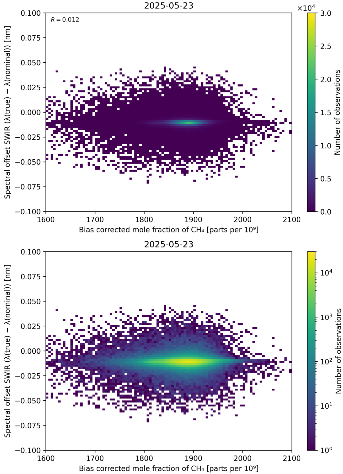
Figure 69: Scatter density plot of “Bias corrected mole fraction of \text{CH}_4 ” against “Spectral offset SWIR ( \lambda_{\text{true}} - \lambda_{\text{nominal}} )” for 2025-05-22 to 2025-05-24.
