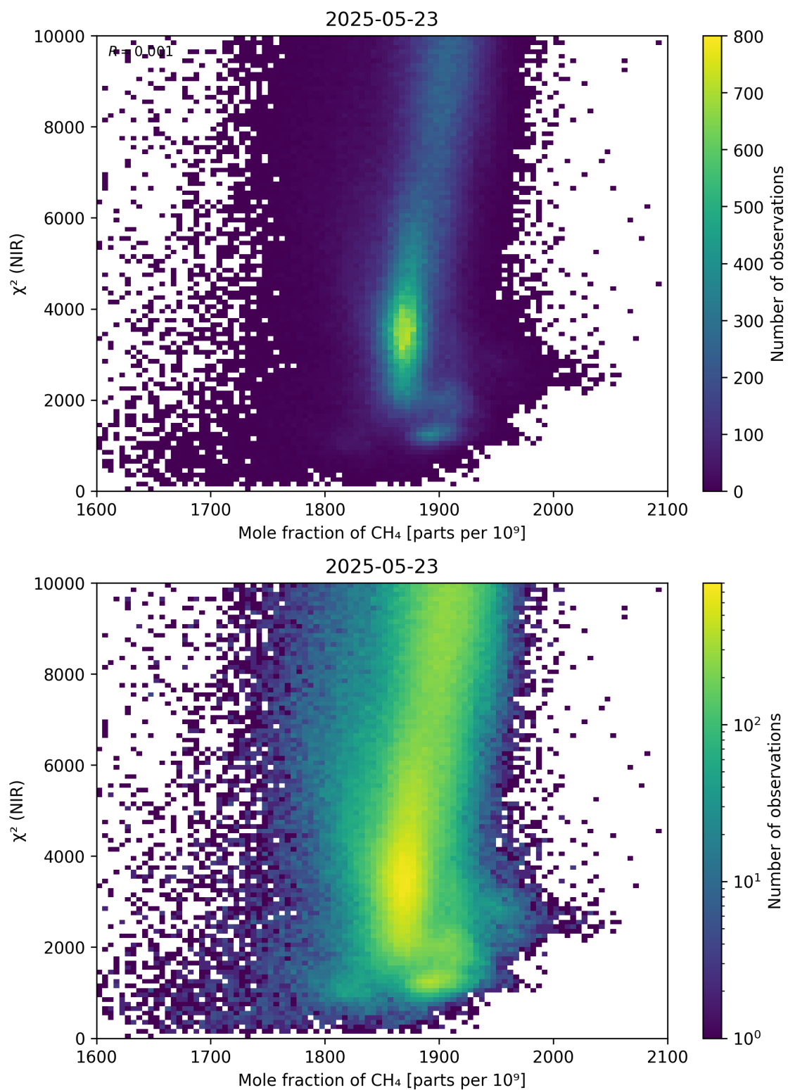
Figure 70: Scatter density plot of “Mole fraction of \text{CH}_4 ” against “ \chi^2 (NIR)” for 2025-05-22 to 2025-05-24.
