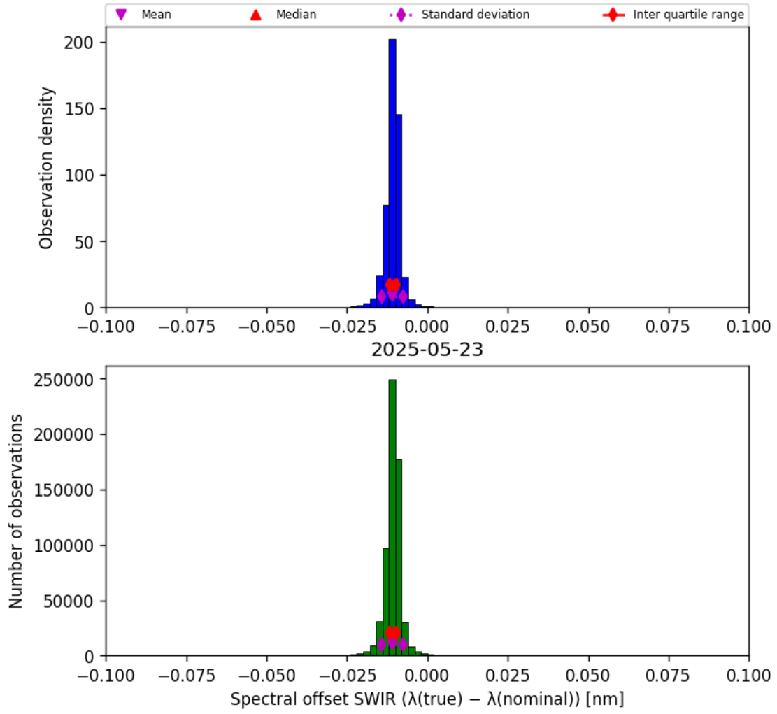
Figure 27: Histogram of “Spectral offset SWIR ( \lambda_{\text{true}} - \lambda_{\text{nominal}} )” for 2025-05-22 to 2025-05-24
