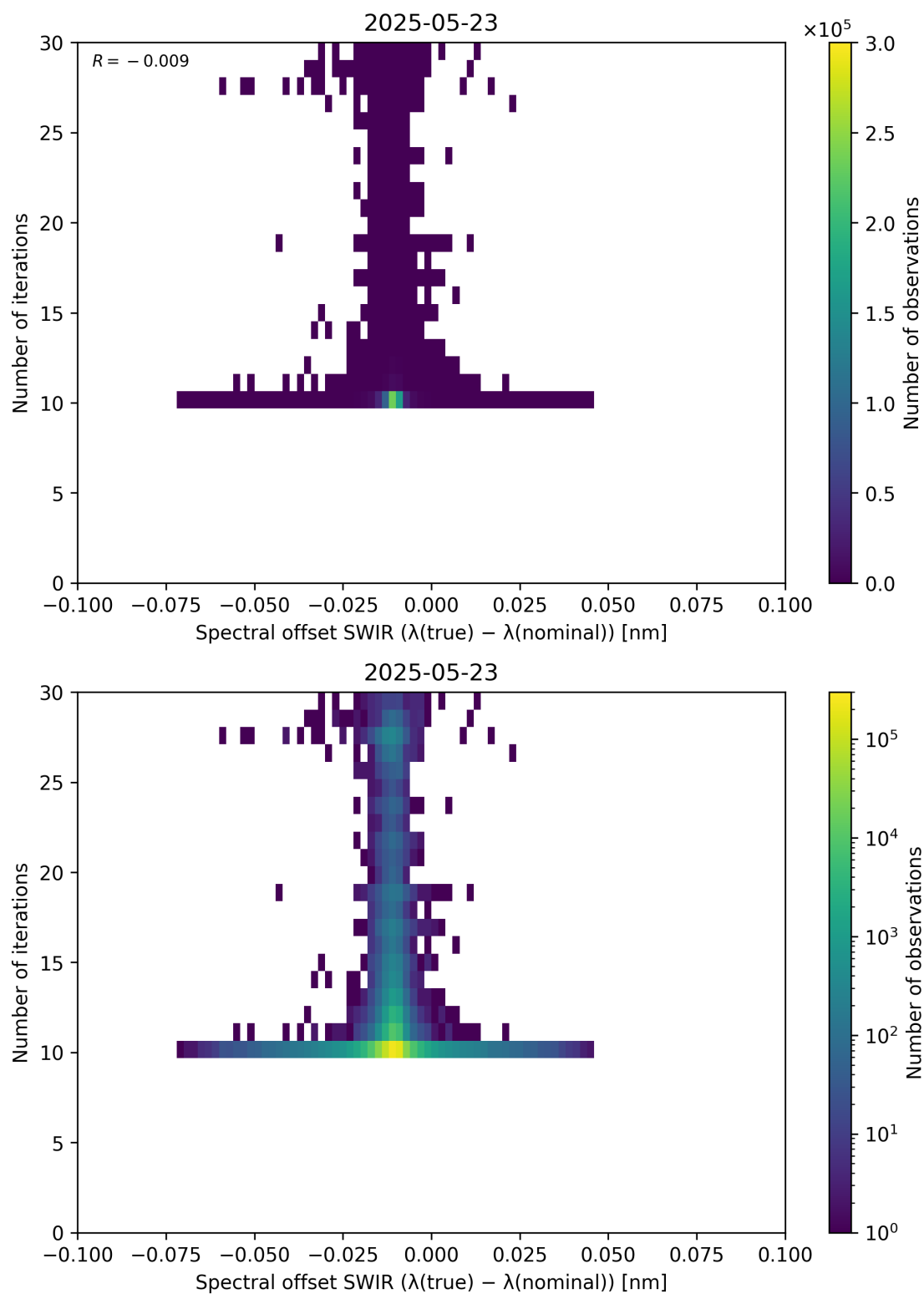
Figure 121: Scatter density plot of “Spectral offset SWIR ( \lambda_{\text{true}} - \lambda_{\text{nominal}} )” against “Number of iterations” for 2025-05-22 to 2025-05-24.
