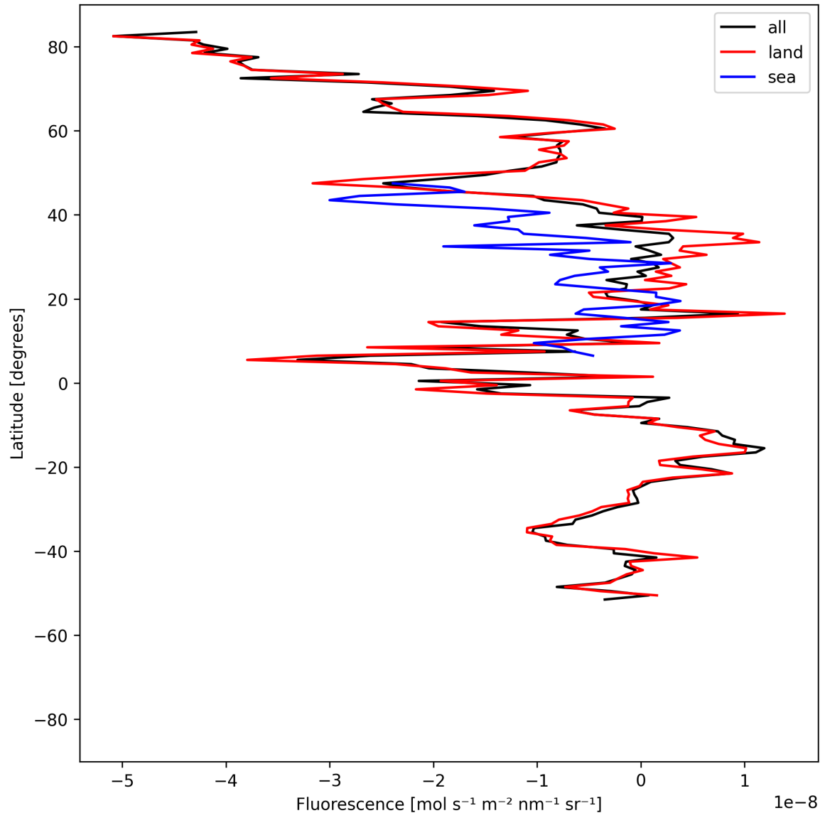
Figure 21: Zonal average of “Fluorescence” for 2025-05-22 to 2025-05-24.
