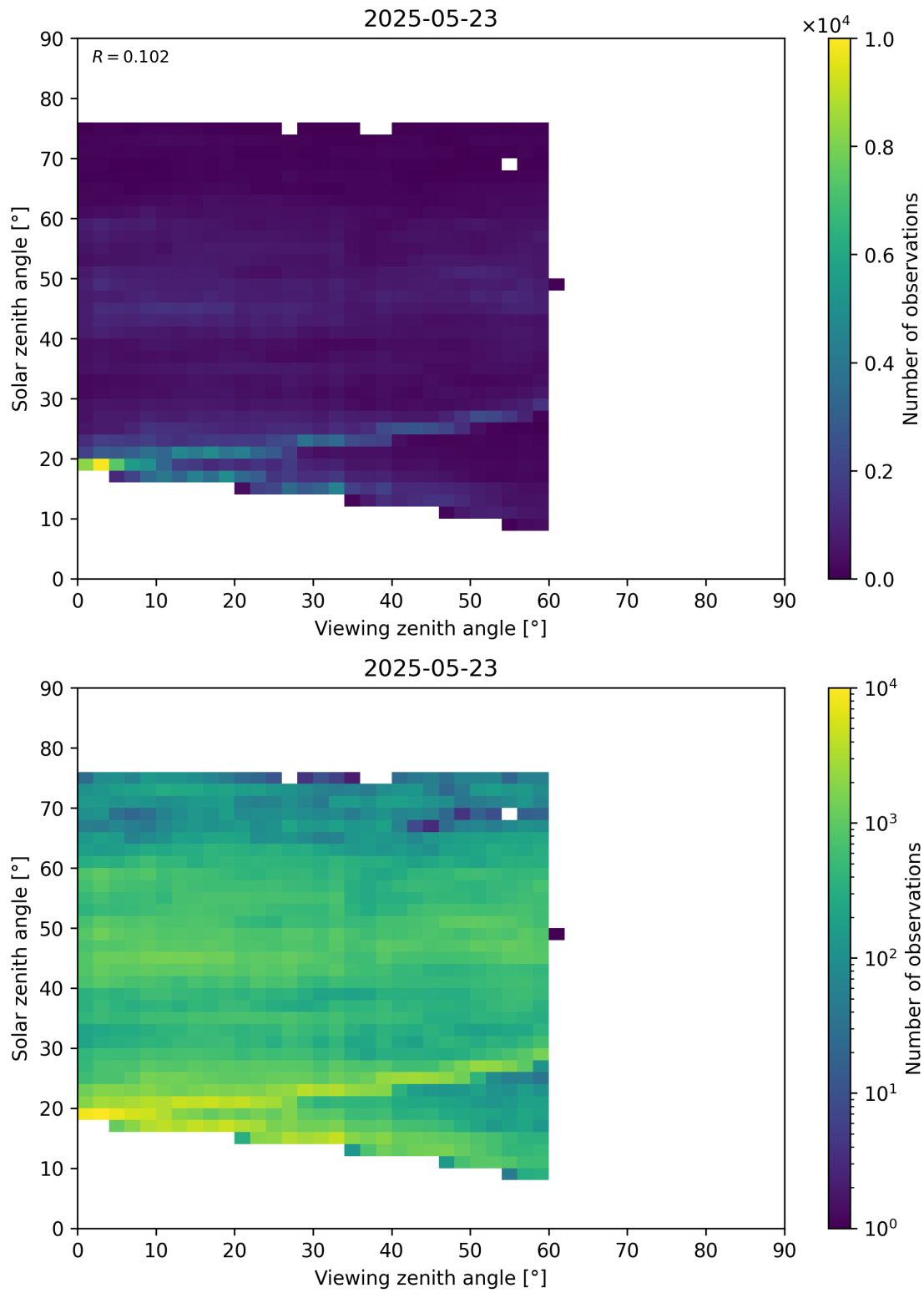
Figure 115: Scatter density plot of “Viewing zenith angle” against “Solar zenith angle” for 2025-05-22 to 2025-05-24.
