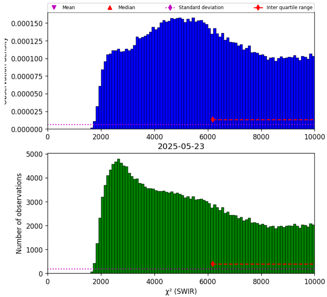
Figure 28: Histogram of “ \chi^2 (SWIR)” for 2025-05-22 to 2025-05-24
