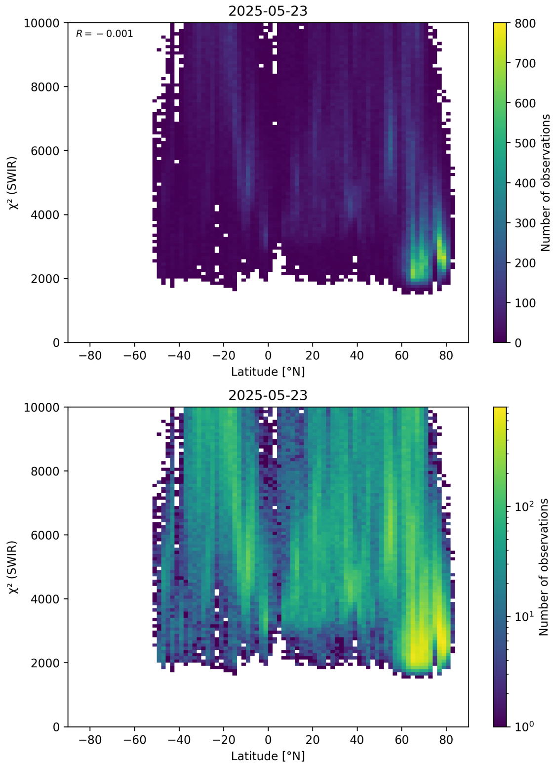
Figure 54: Scatter density plot of “Latitude” against “ \chi^2 (SWIR)” for 2025-05-22 to 2025-05-24.
