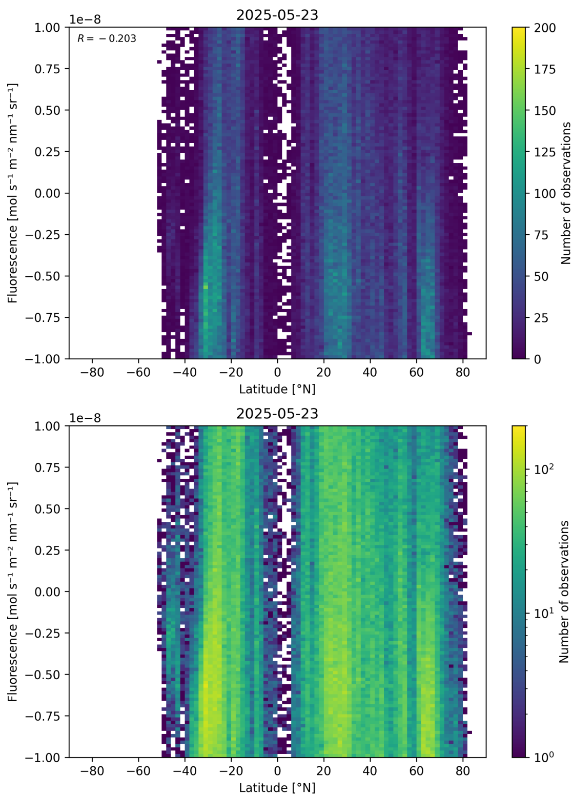
Figure 56: Scatter density plot of “Latitude” against “Fluorescence” for 2025-05-22 to 2025-05-24.
