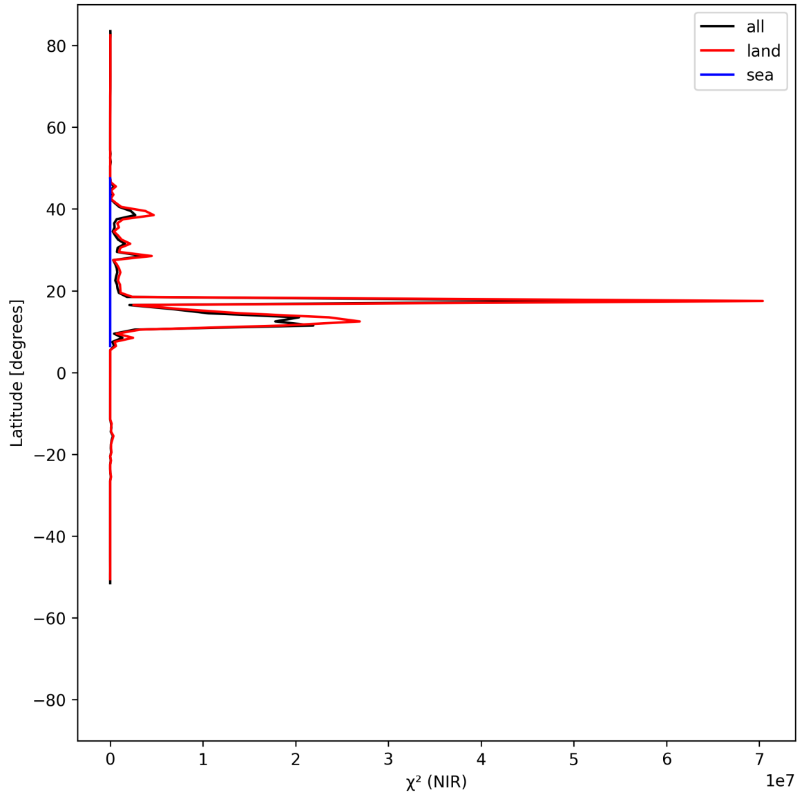
Figure 18: Zonal average of “ \chi^2 (NIR)” for 2025-05-22 to 2025-05-24.
