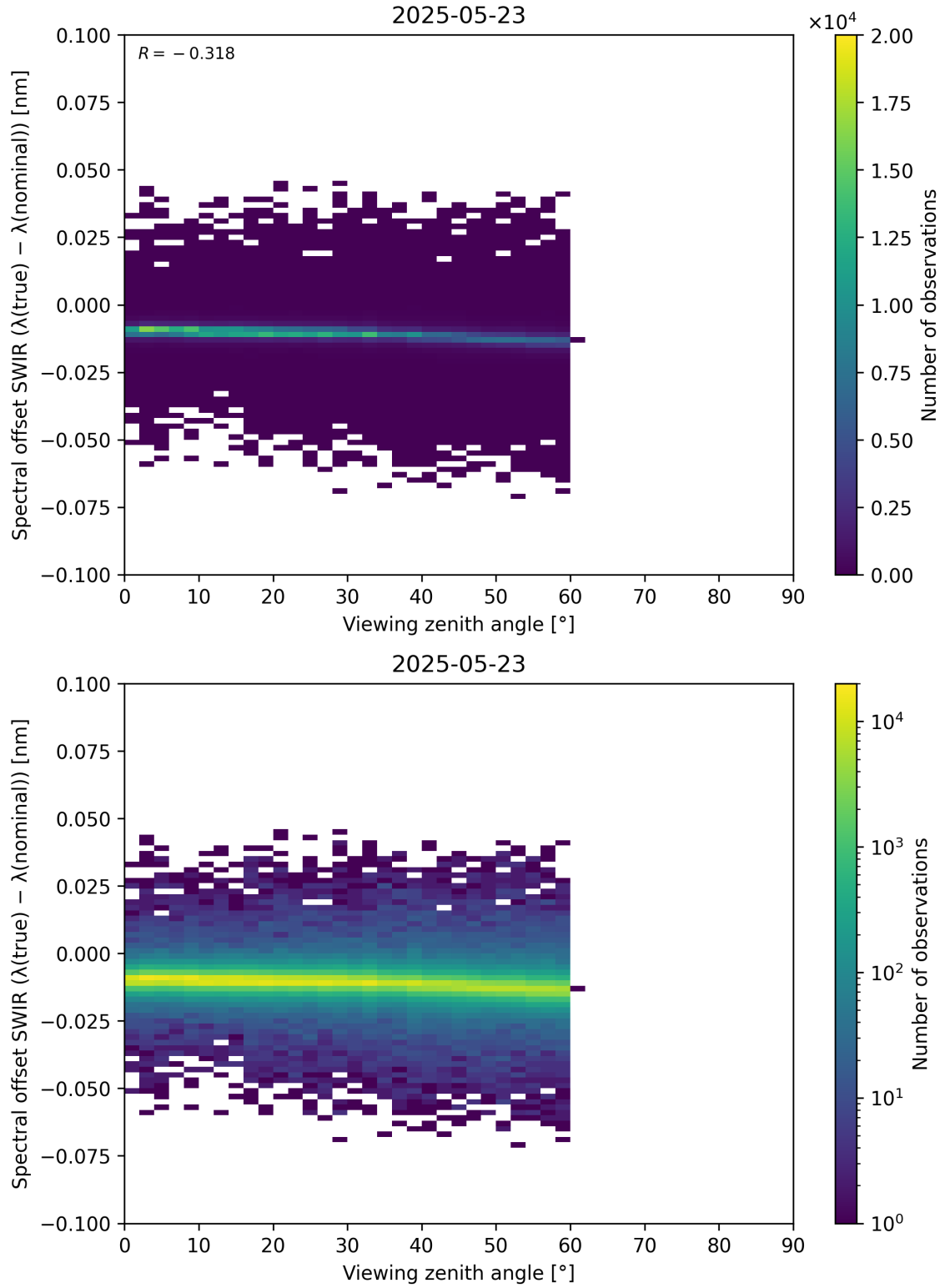
Figure 116: Scatter density plot of “Viewing zenith angle” against “Spectral offset SWIR ( \lambda_{\text{true}} - \lambda_{\text{nominal}} )” for 2025-05-22 to 2025-05-24.
