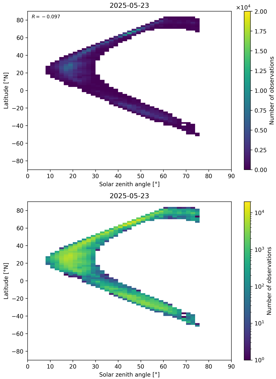
Figure 98: Scatter density plot of “Solar zenith angle” against “Latitude” for 2025-05-22 to 2025-05-24.
