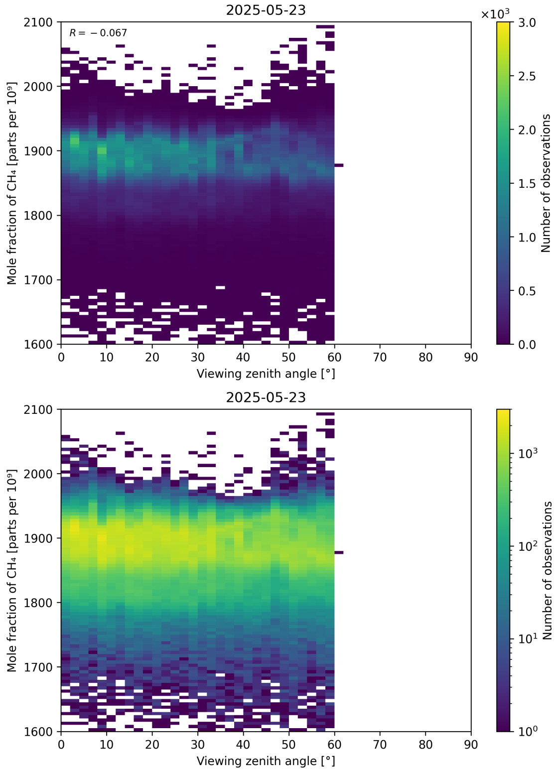
Figure 110: Scatter density plot of “Viewing zenith angle” against “Mole fraction of CH 4 ” for 2025-05-22 to 2025-05-24.
