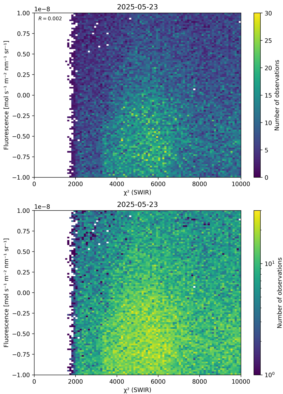
Figure 49: Scatter density plot of “ \chi^2 (SWIR)” against “Fluorescence” for 2025-05-22 to 2025-05-24.
