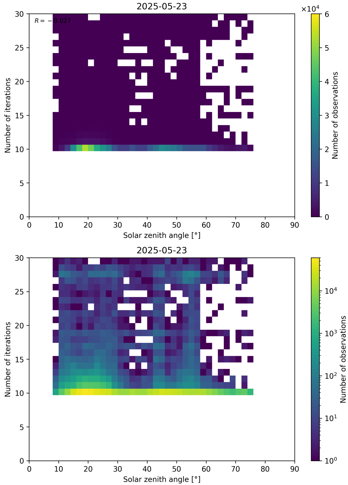
Figure 102: Scatter density plot of “Solar zenith angle” against “Number of iterations” for 2025-05-22 to 2025-05-24.
