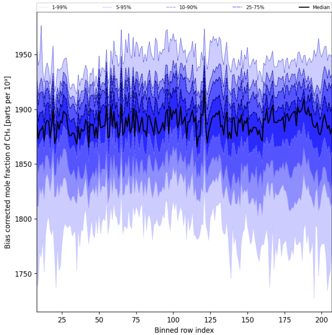
Figure 36: Along track statistics of “Bias corrected mole fraction of CH 4 ” for 2025-05-22 to 2025-05-24
