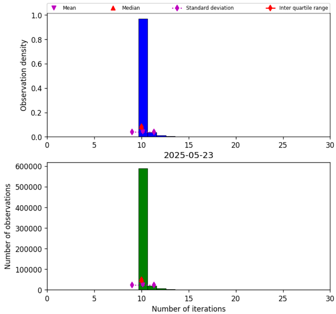
Figure 31: Histogram of “Number of iterations” for 2025-05-22 to 2025-05-24
