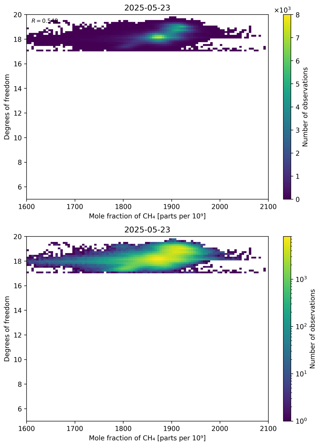
Figure 72: Scatter density plot of “Mole fraction of CH 4 ” against “Degrees of freedom” for 2025-05-22 to 2025-05-24.
