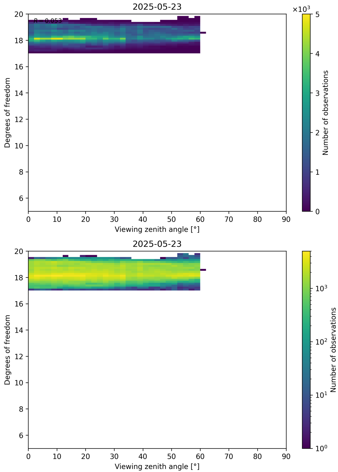
Figure 107: Scatter density plot of “Viewing zenith angle” against “Degrees of freedom” for 2025-05-22 to 2025-05-24.
