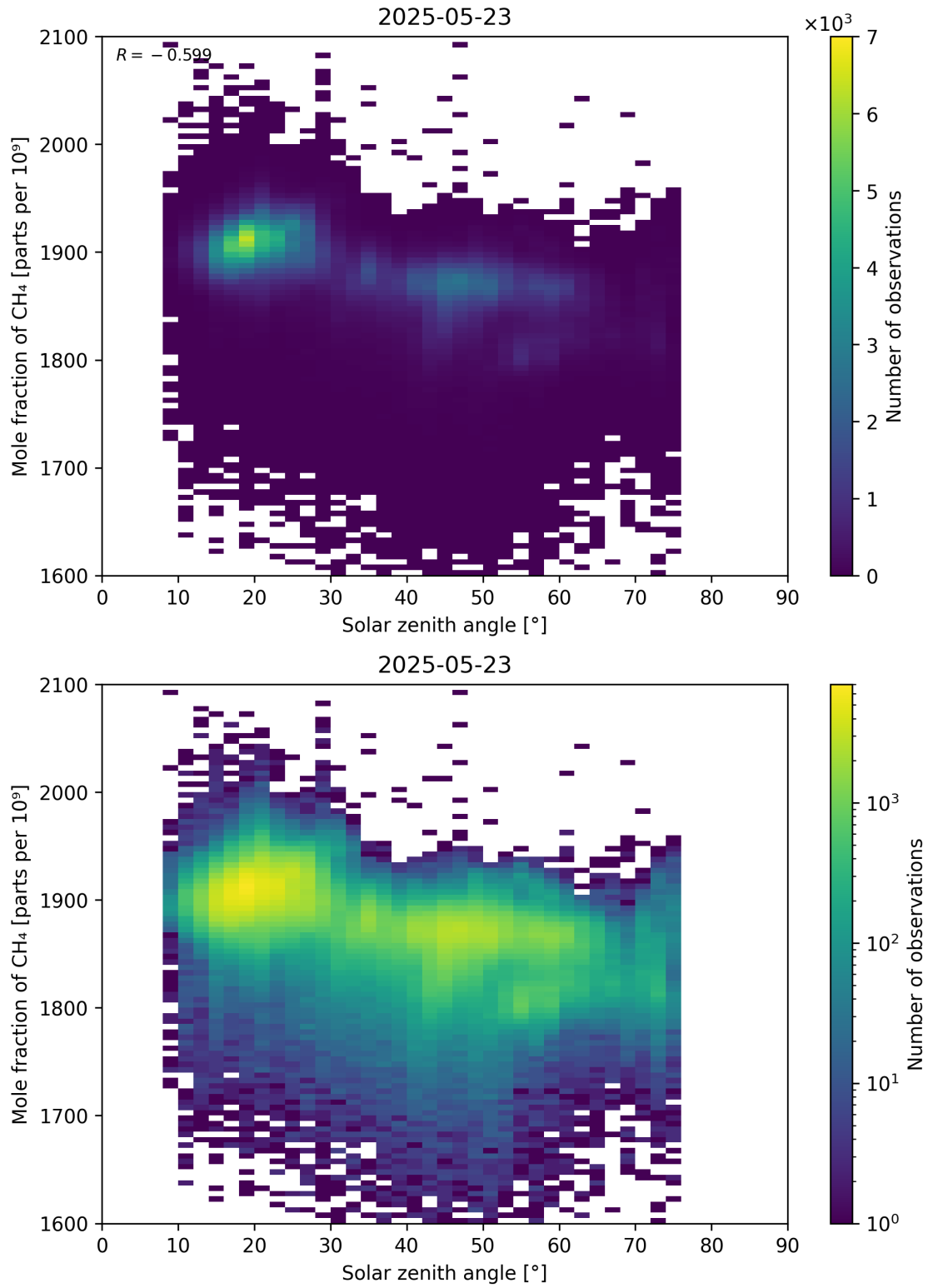
Figure 99: Scatter density plot of “Solar zenith angle” against “Mole fraction of CH 4 ” for 2025-05-22 to 2025-05-24.
