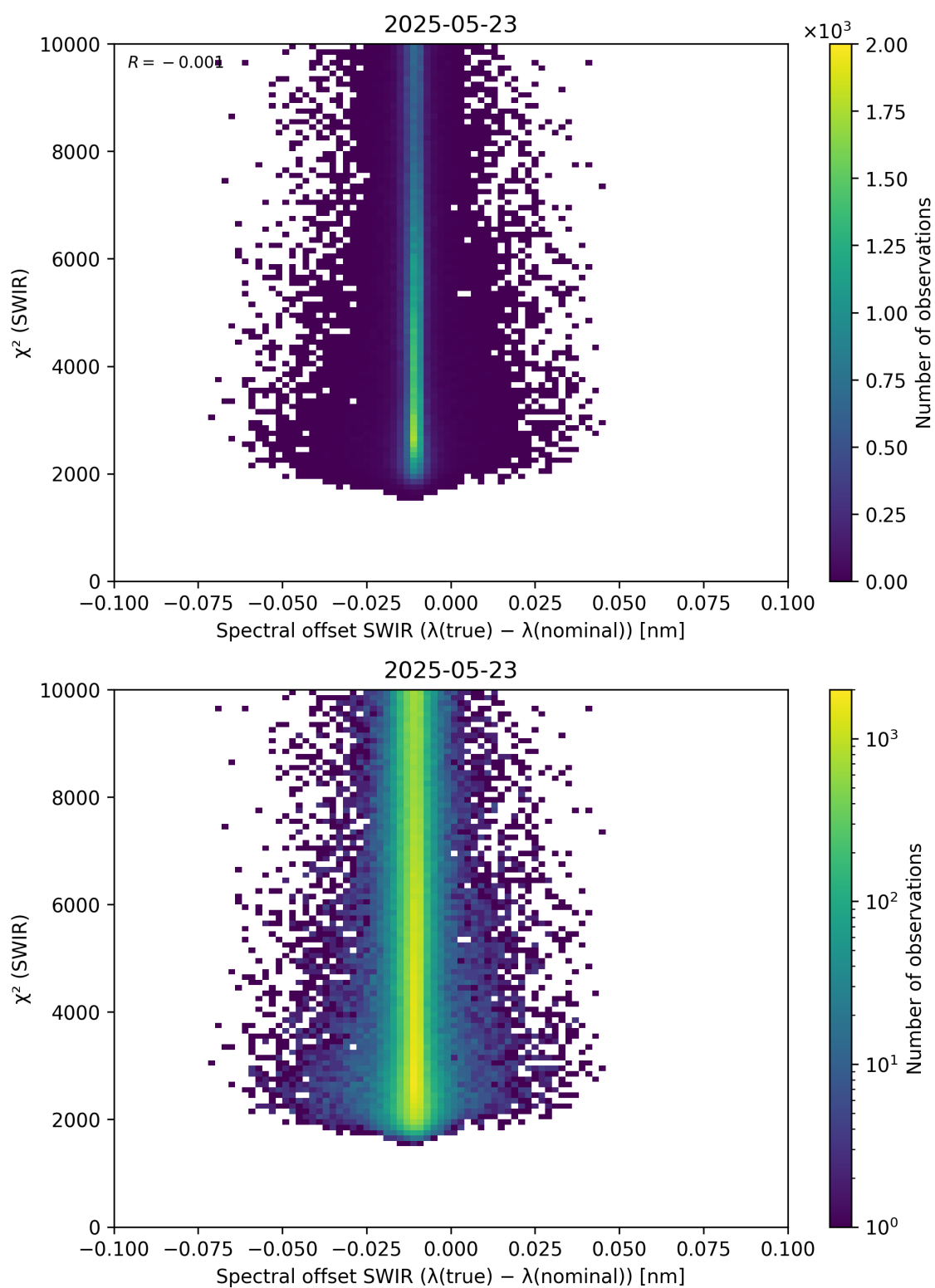
Figure 118: Scatter density plot of “Spectral offset SWIR ( \lambda_{\text{true}} - \lambda_{\text{nominal}} )” against “ \chi^2 (SWIR)” for 2025-05-22 to 2025-05-24.
