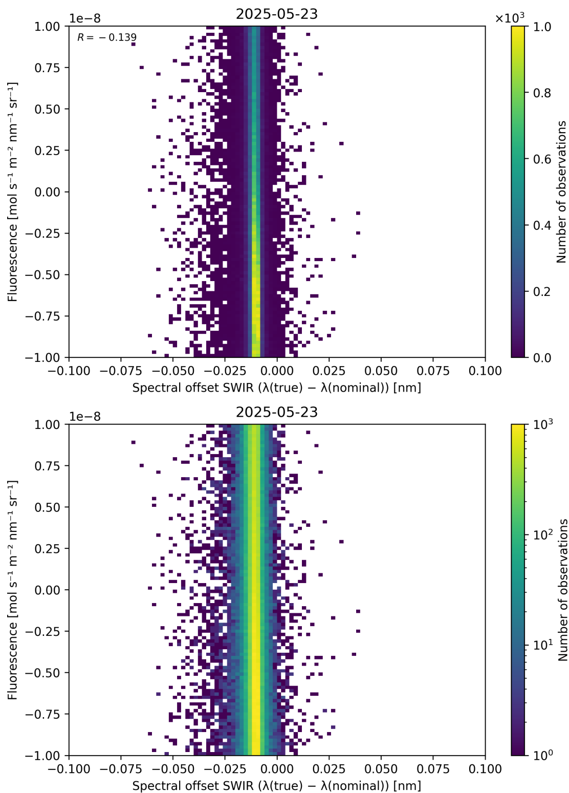
Figure 120: Scatter density plot of “Spectral offset SWIR ( \lambda_{\text{true}} - \lambda_{\text{nominal}} )” against “Fluorescence” for 2025-05-22 to 2025-05-24.
