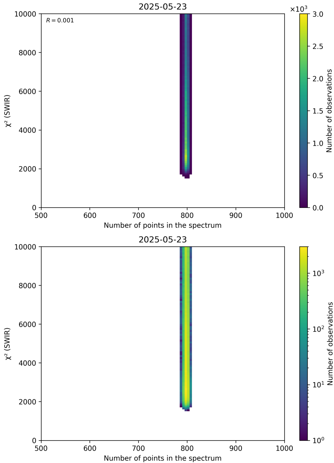
Figure 89: Scatter density plot of “Number of points in the spectrum” against “ \chi^2 (SWIR)” for 2025-05-22 to 2025-05-24.
