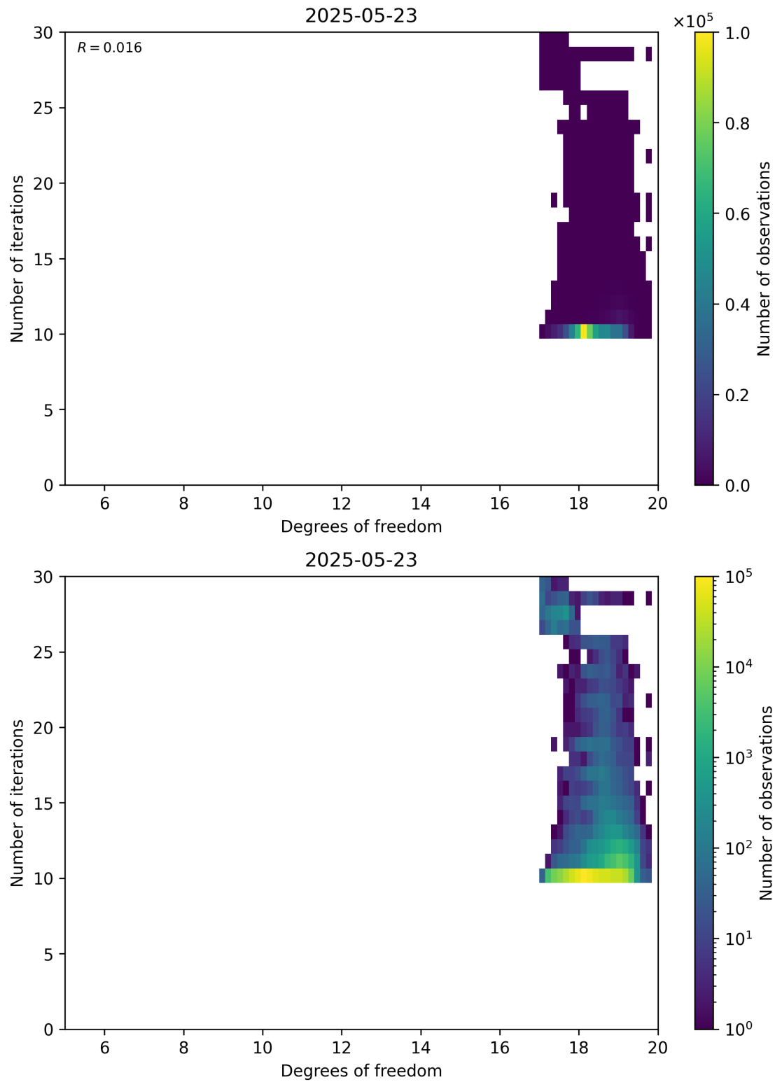
Figure 52: Scatter density plot of “Degrees of freedom” against “Number of iterations” for 2025-05-22 to 2025-05-24.
