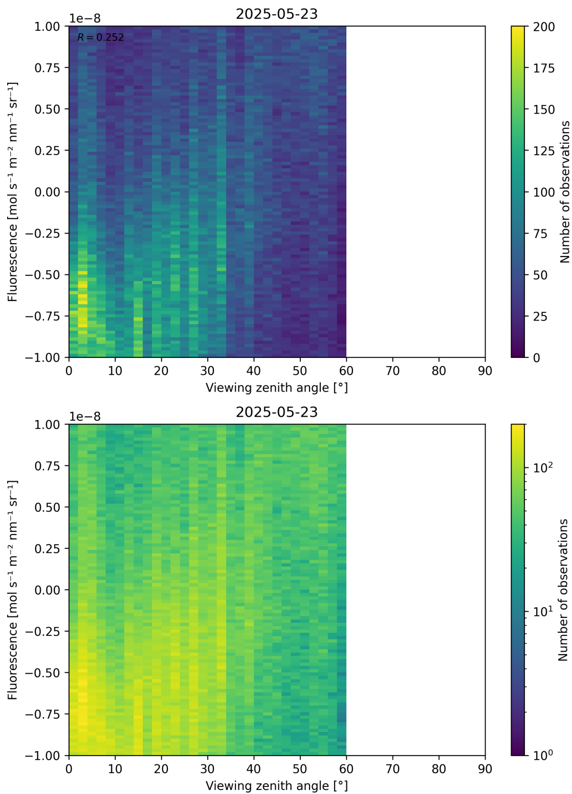
Figure 108: Scatter density plot of “Viewing zenith angle” against “Fluorescence” for 2025-05-22 to 2025-05-24.
