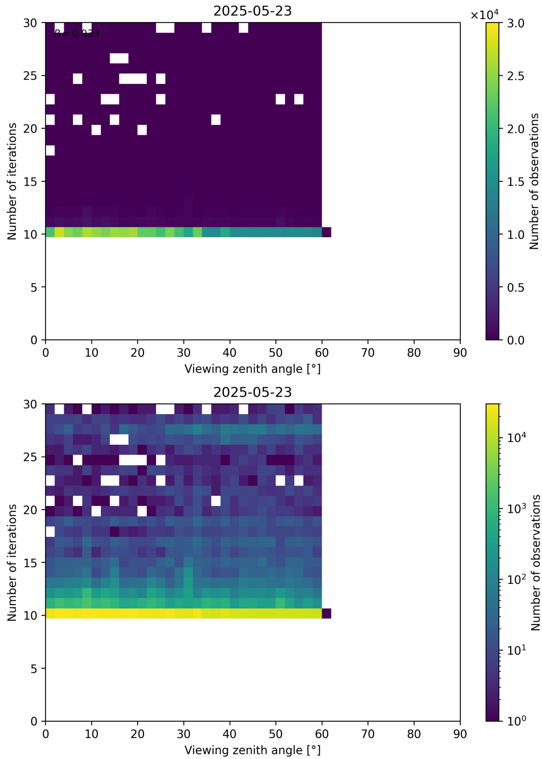
Figure 113: Scatter density plot of “Viewing zenith angle” against “Number of iterations” for 2025-05-22 to 2025-05-24.
