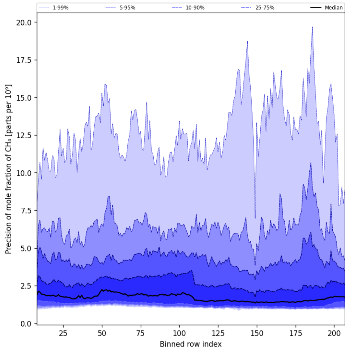
Figure 35: Along track statistics of “Precision of mole fraction of CH 4 ” for 2025-05-22 to 2025-05-24
