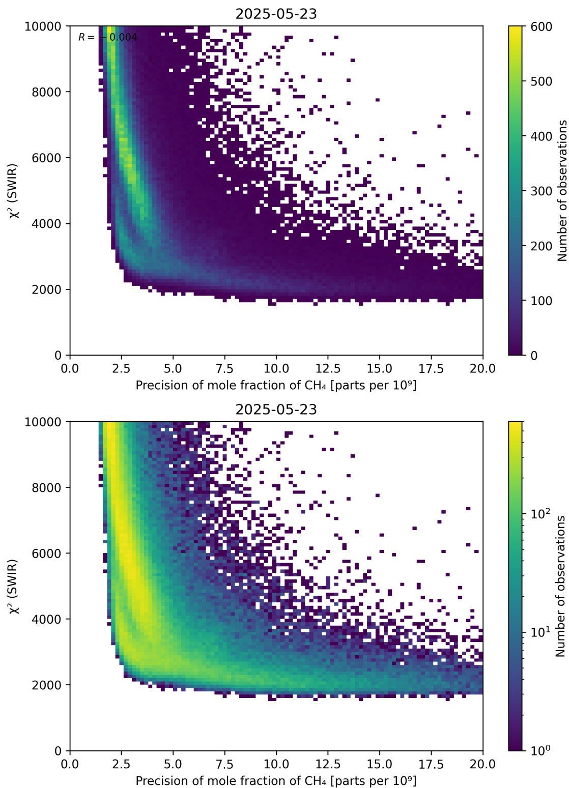
Figure 79: Scatter density plot of “Precision of mole fraction of \text{CH}_4 ” against “ \chi^2 (SWIR)” for 2025-05-22 to 2025-05-24.
