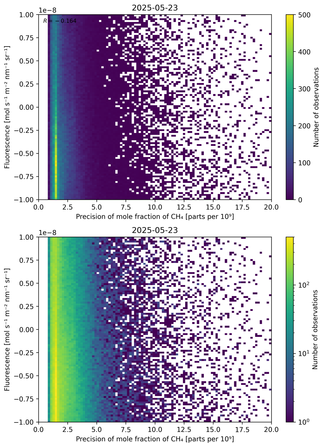
Figure 81: Scatter density plot of “Precision of mole fraction of \text{CH}_4 ” against “Fluorescence” for 2025-05-22 to 2025-05-24.
