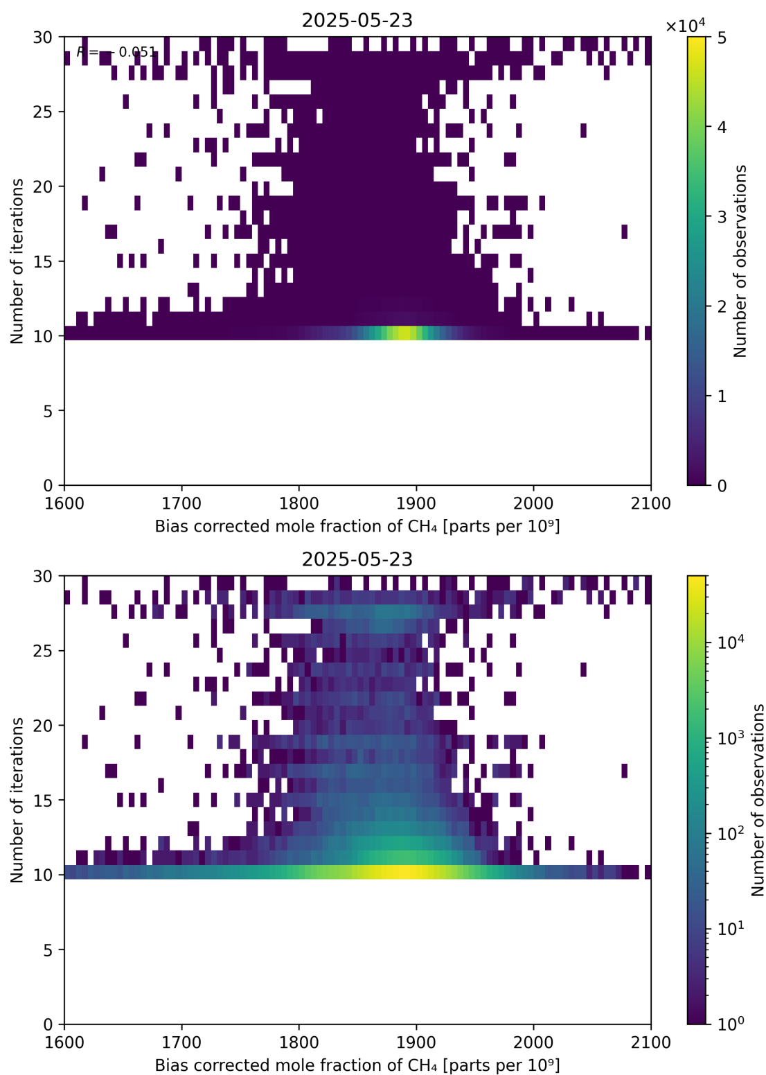
Figure 67: Scatter density plot of “Bias corrected mole fraction of CH 4 ” against “Number of iterations” for 2025-05-22 to 2025-05-24.
