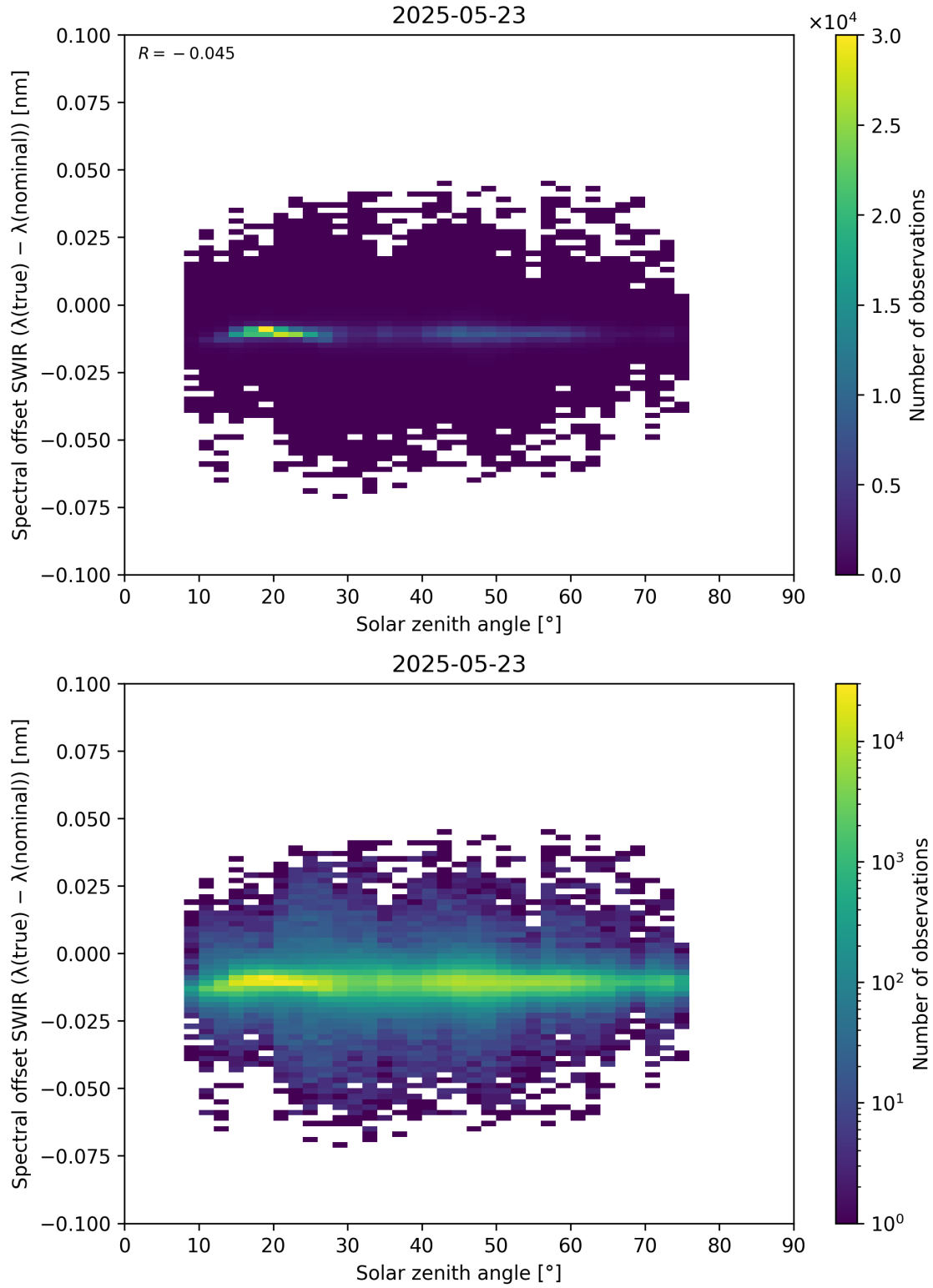
Figure 104: Scatter density plot of “Solar zenith angle” against “Spectral offset SWIR ( \lambda_{\text{true}} - \lambda_{\text{nominal}} )” for 2025-05-22 to 2025-05-24.
