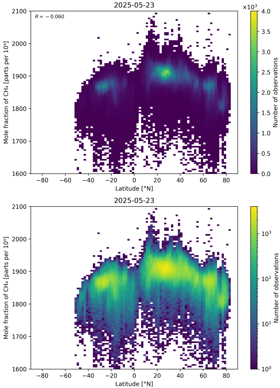
Figure 57: Scatter density plot of “Latitude” against “Mole fraction of CH 4 ” for 2025-05-22 to 2025-05-24.
