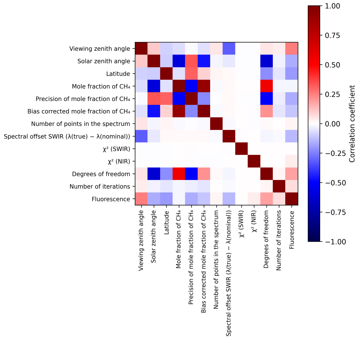
Figure 2: Map of correlation matrix for 2025-05-22 to 2025-05-24.
