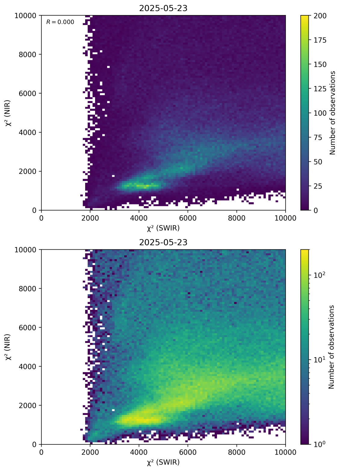
Figure 47: Scatter density plot of “ \chi^2 (SWIR)” against “ \chi^2 (NIR)” for 2025-05-22 to 2025-05-24.
