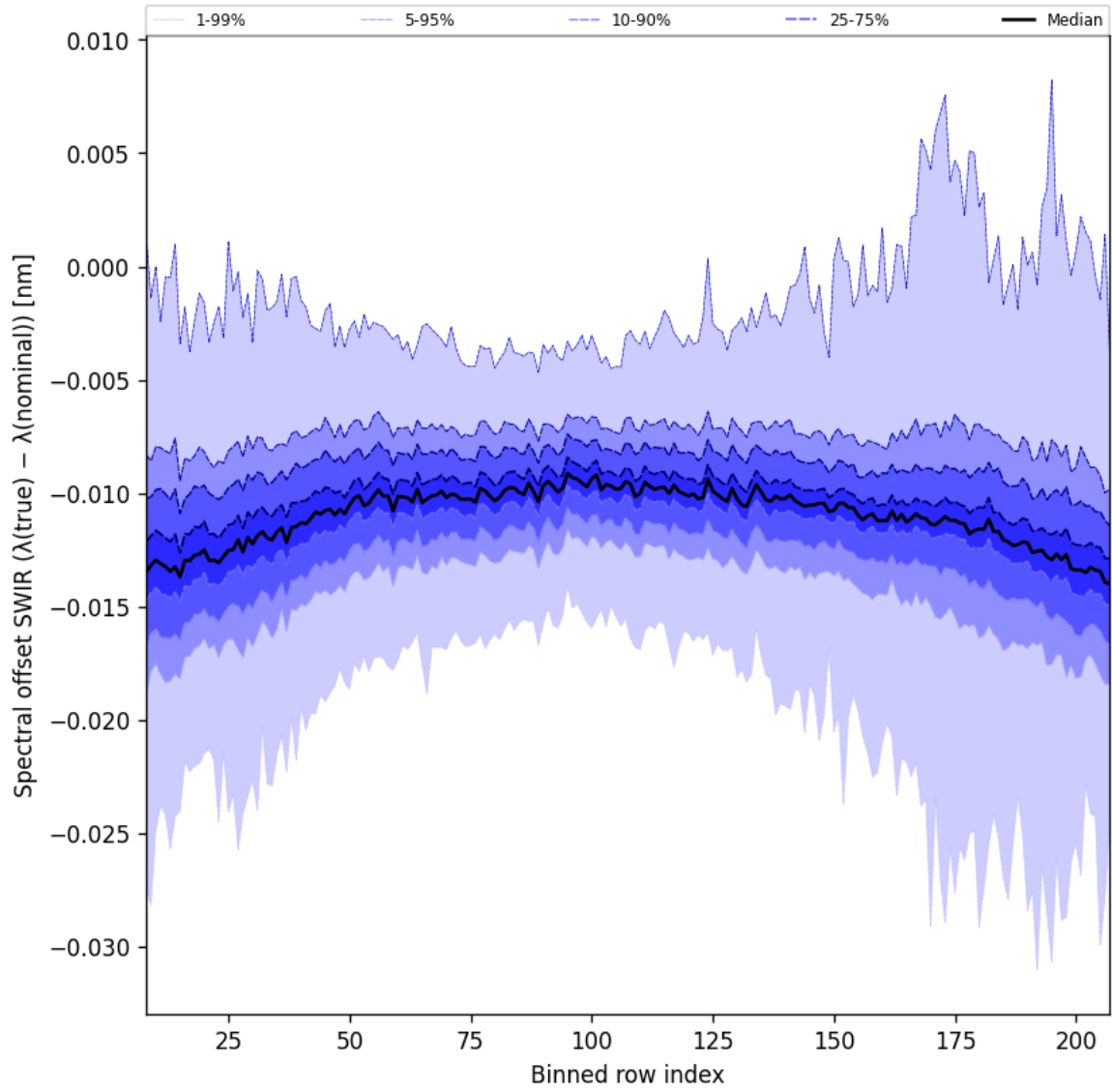
Figure 38: Along track statistics of “Spectral offset SWIR ( \lambda_{\text{true}} - \lambda_{\text{nominal}} )” for 2025-05-22 to 2025-05-24
