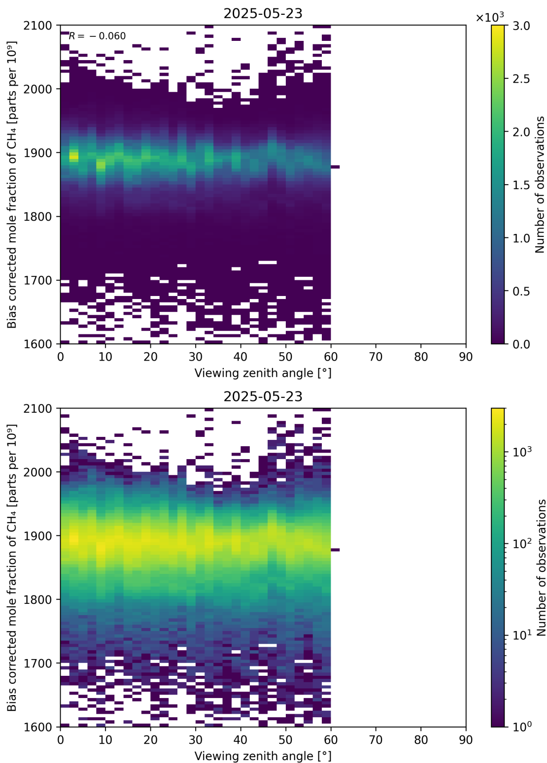
Figure 111: Scatter density plot of “Viewing zenith angle” against “Bias corrected mole fraction of CH 4 ” for 2025-05-22 to 2025-05-24.
