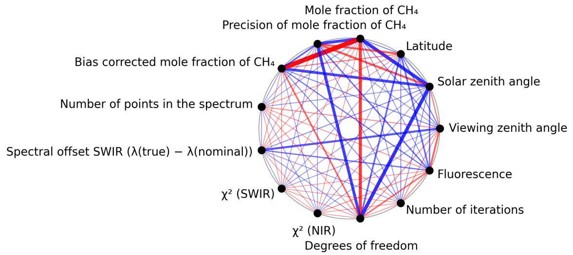
Figure 1: Map of correlation graph for 2025-05-22 to 2025-05-24.
