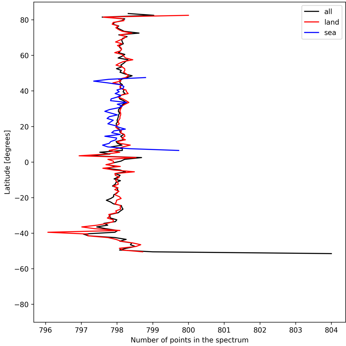
Figure 15: Zonal average of “Number of points in the spectrum” for 2025-05-22 to 2025-05-24.
