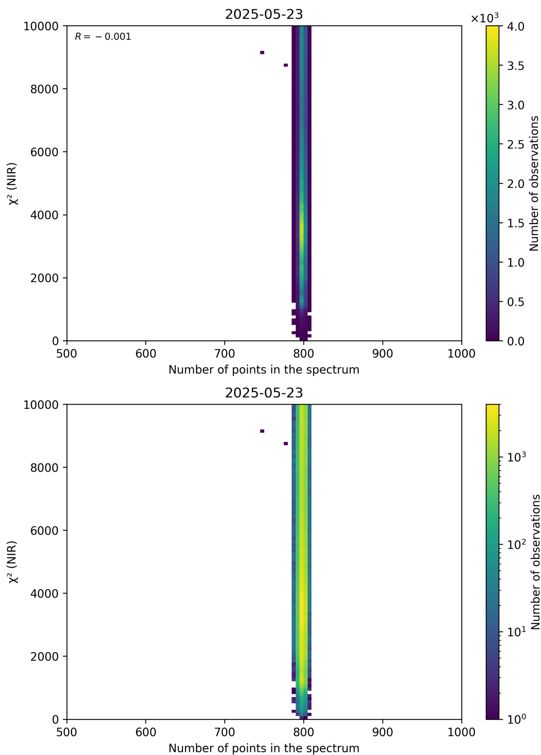
Figure 88: Scatter density plot of “Number of points in the spectrum” against “ \chi^2 (NIR)” for 2025-05-22 to 2025-05-24.
