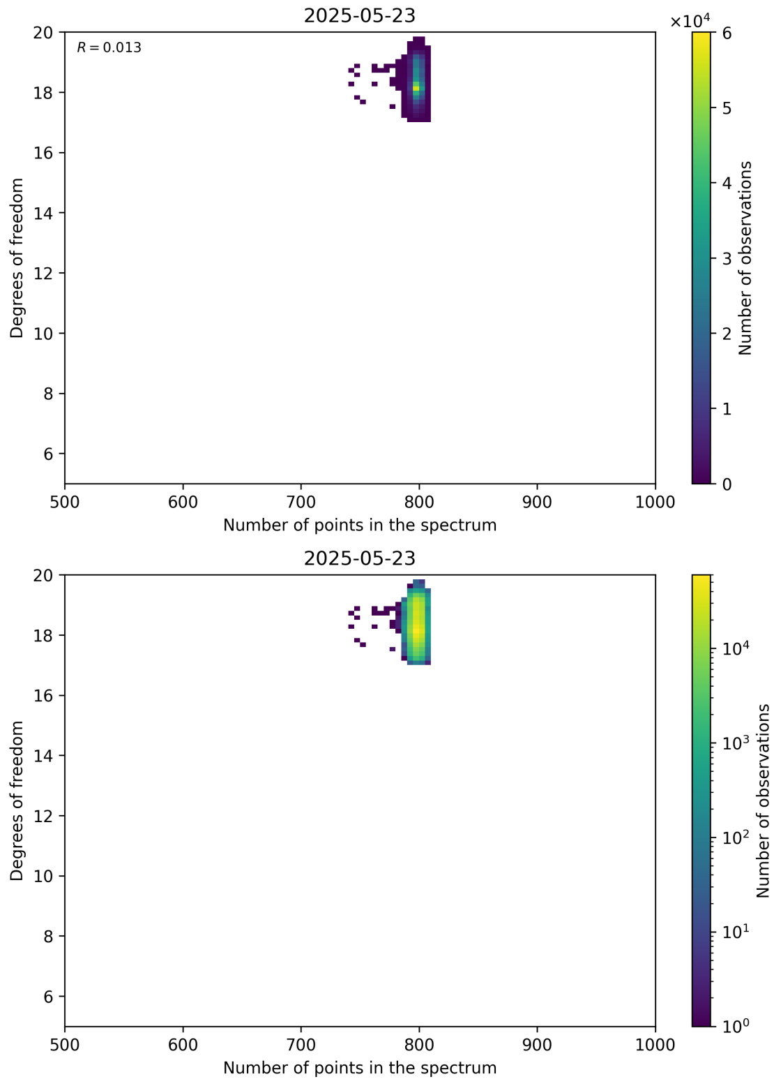
Figure 90: Scatter density plot of “Number of points in the spectrum” against “Degrees of freedom” for 2025-05-22 to 2025-05-24.
