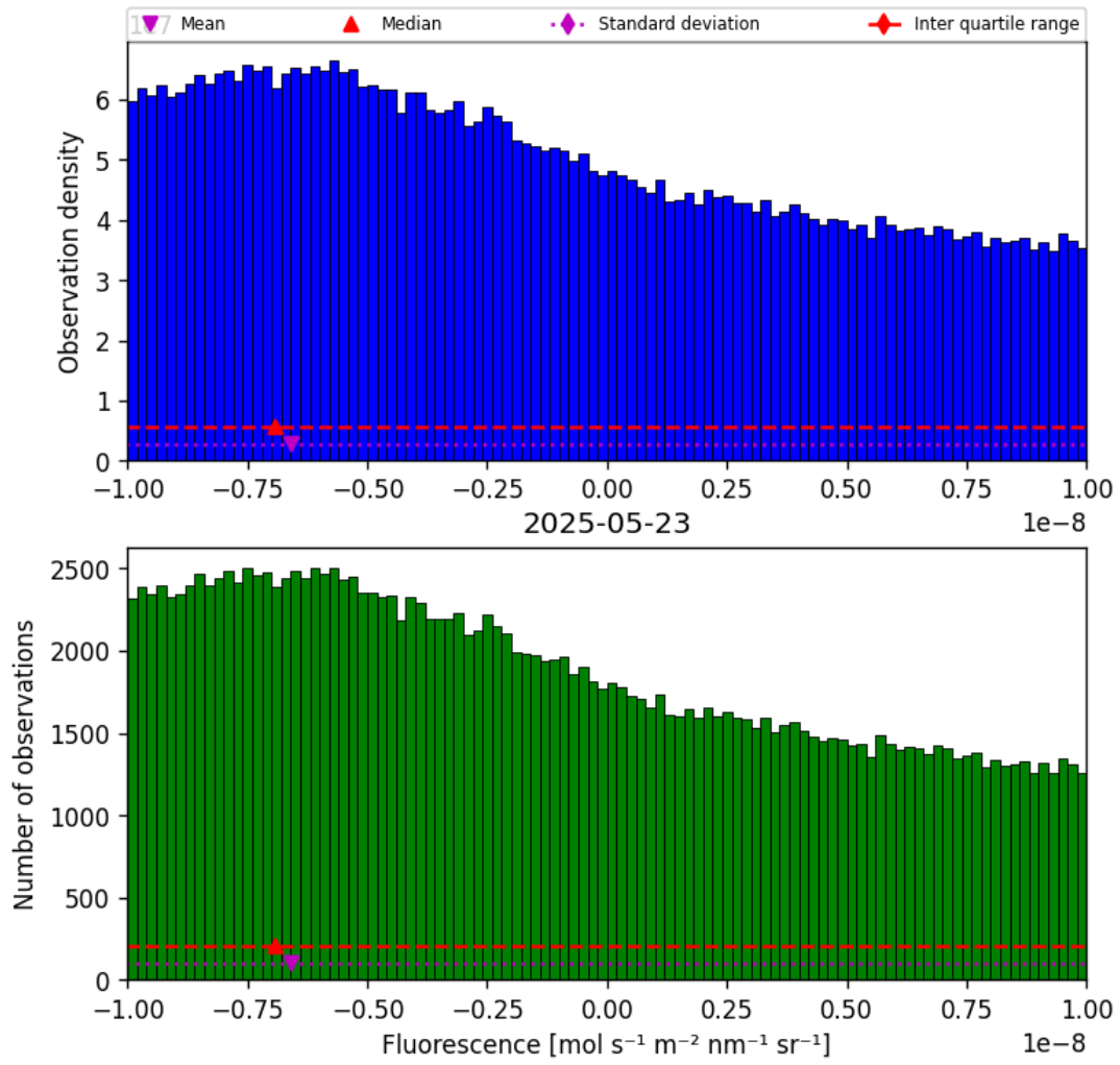
Figure 32: Histogram of “Fluorescence” for 2025-05-22 to 2025-05-24
