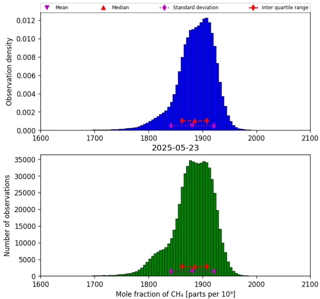
Figure 23: Histogram of “Mole fraction of CH 4 ” for 2025-05-22 to 2025-05-24
