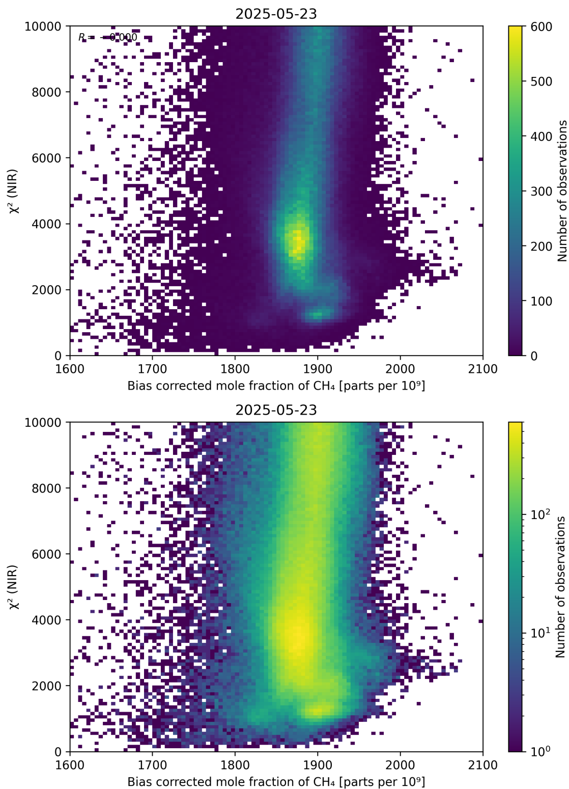
Figure 63: Scatter density plot of “Bias corrected mole fraction of \text{CH}_4 ” against “ \chi^2 (NIR)” for 2025-05-22 to 2025-05-24.
