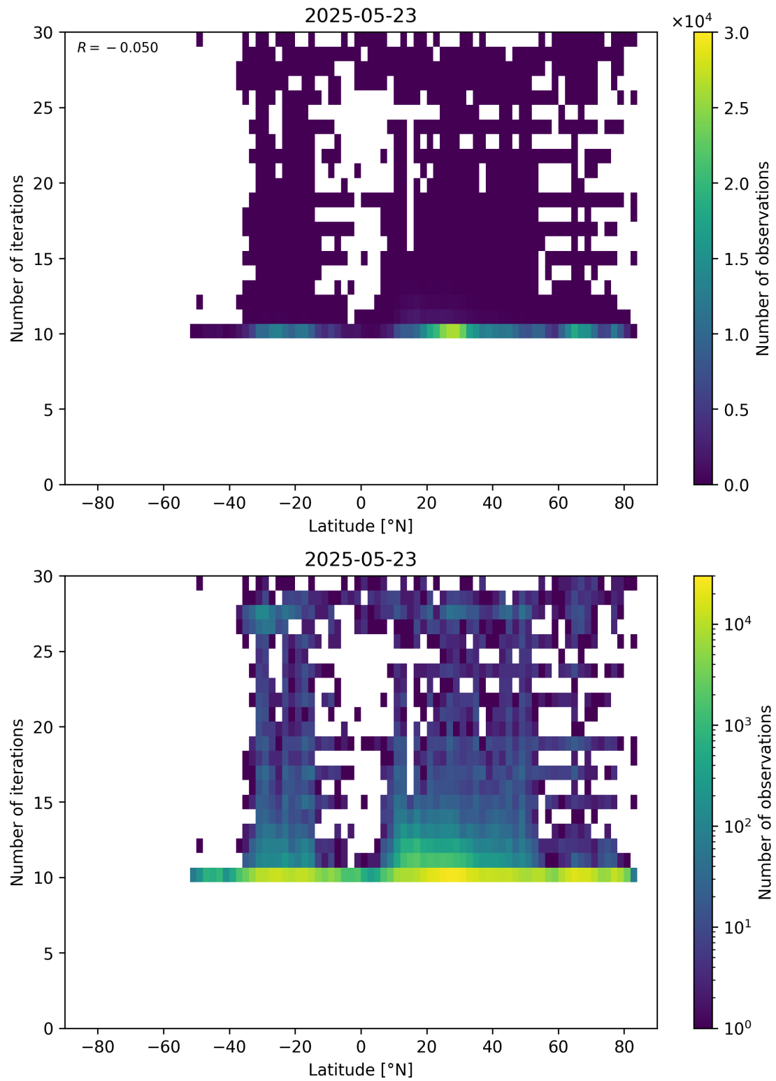
Figure 60: Scatter density plot of “Latitude” against “Number of iterations” for 2025-05-22 to 2025-05-24.
