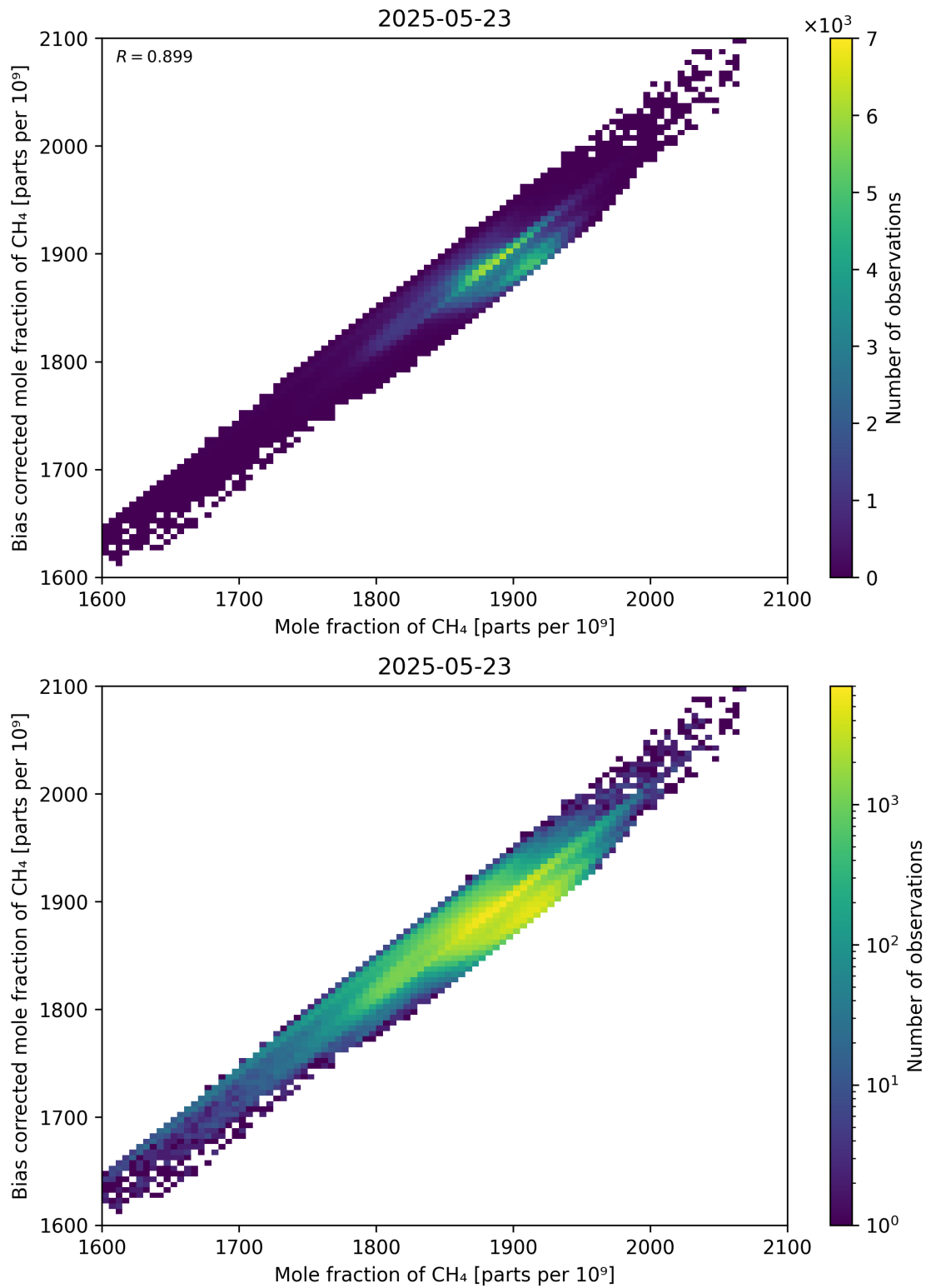
Figure 74: Scatter density plot of “Mole fraction of CH 4 ” against “Bias corrected mole fraction of CH 4 ” for 2025-05-22 to 2025-05-24.
