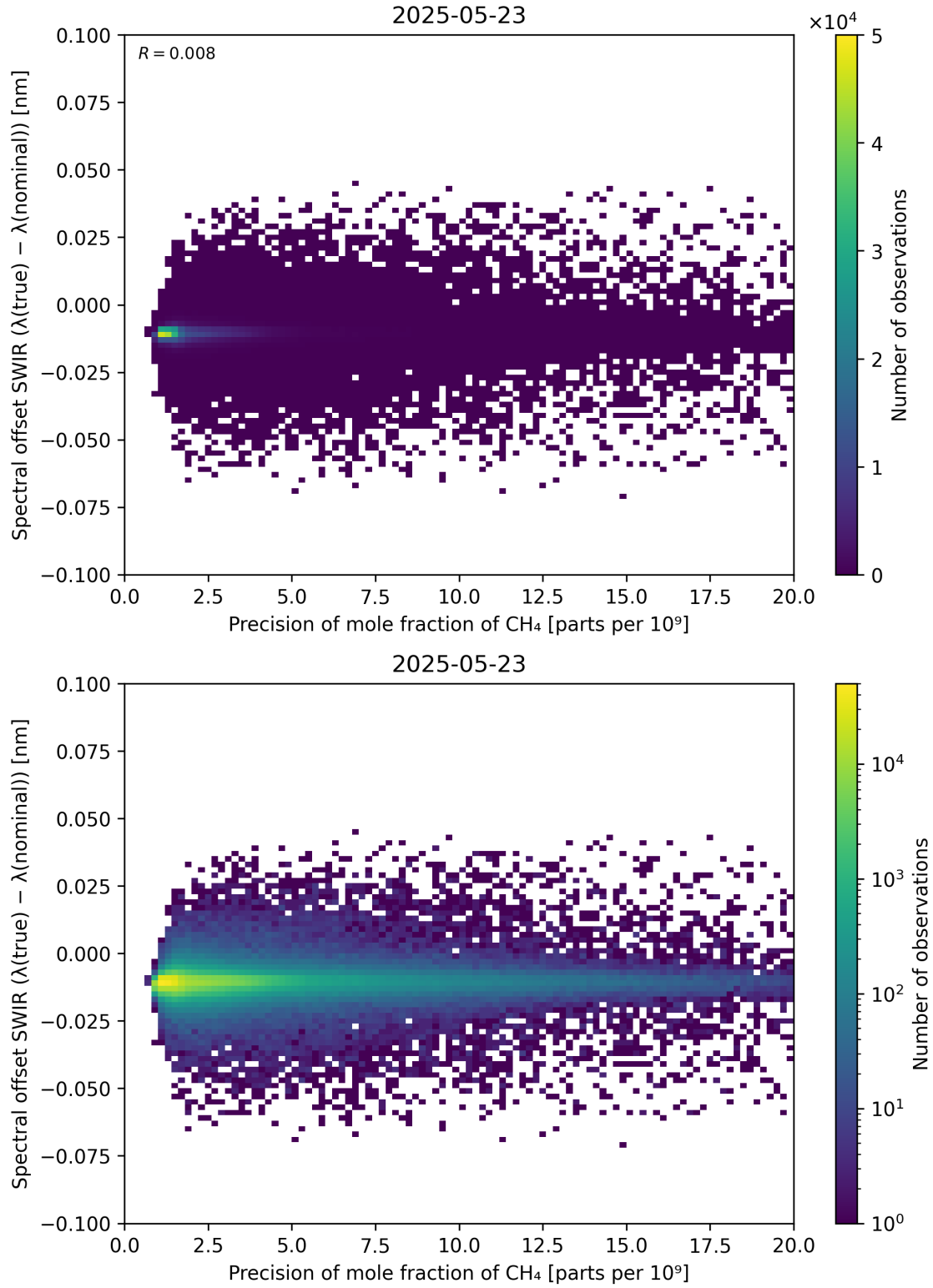
Figure 85: Scatter density plot of “Precision of mole fraction of CH 4 ” against “Spectral offset SWIR ( \lambda_{\text{true}} - \lambda_{\text{nominal}} )” for 2025-05-22 to 2025-05-24.
