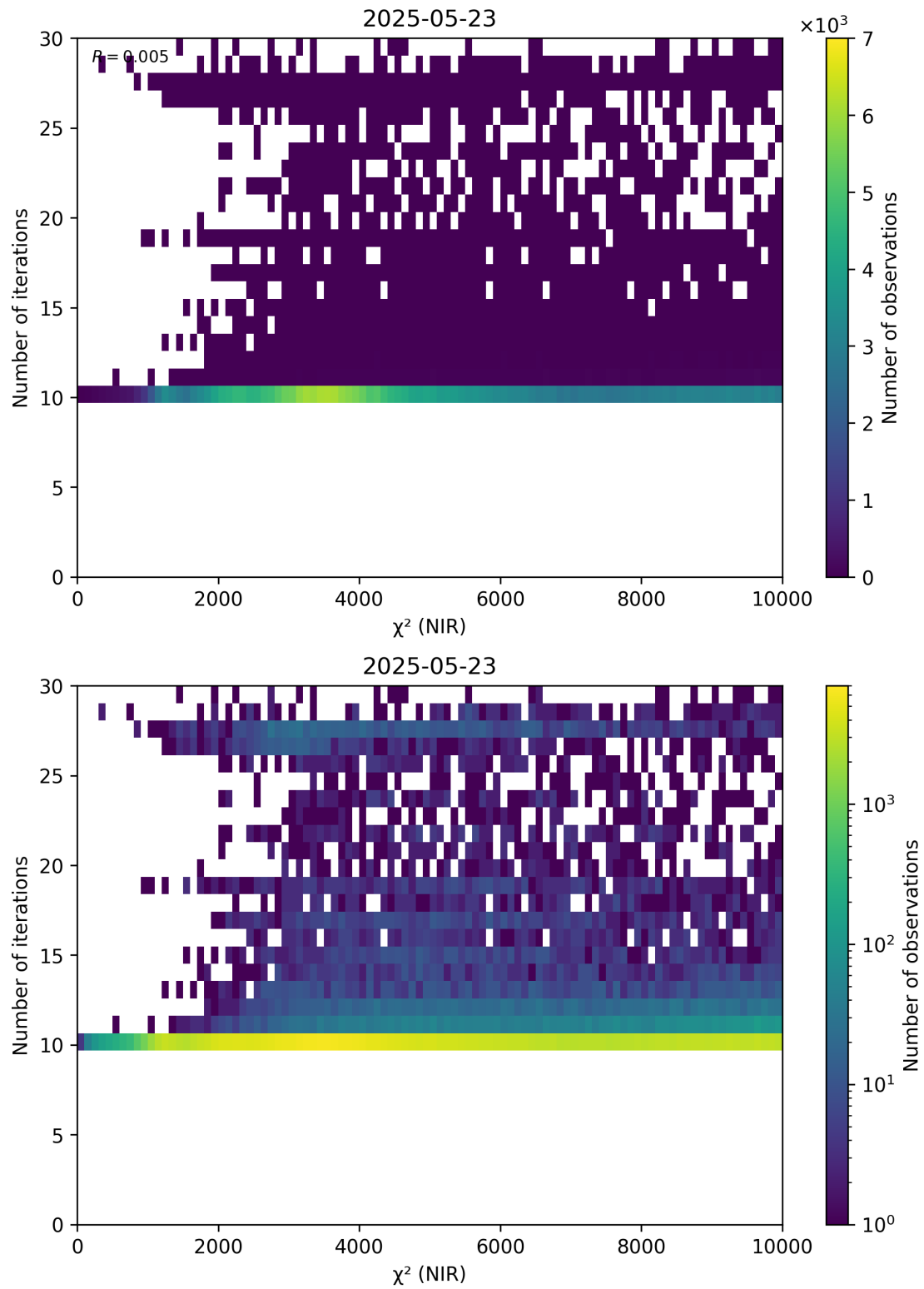
Figure 46: Scatter density plot of “ \chi^2 (NIR)” against “Number of iterations” for 2025-05-22 to 2025-05-24.
