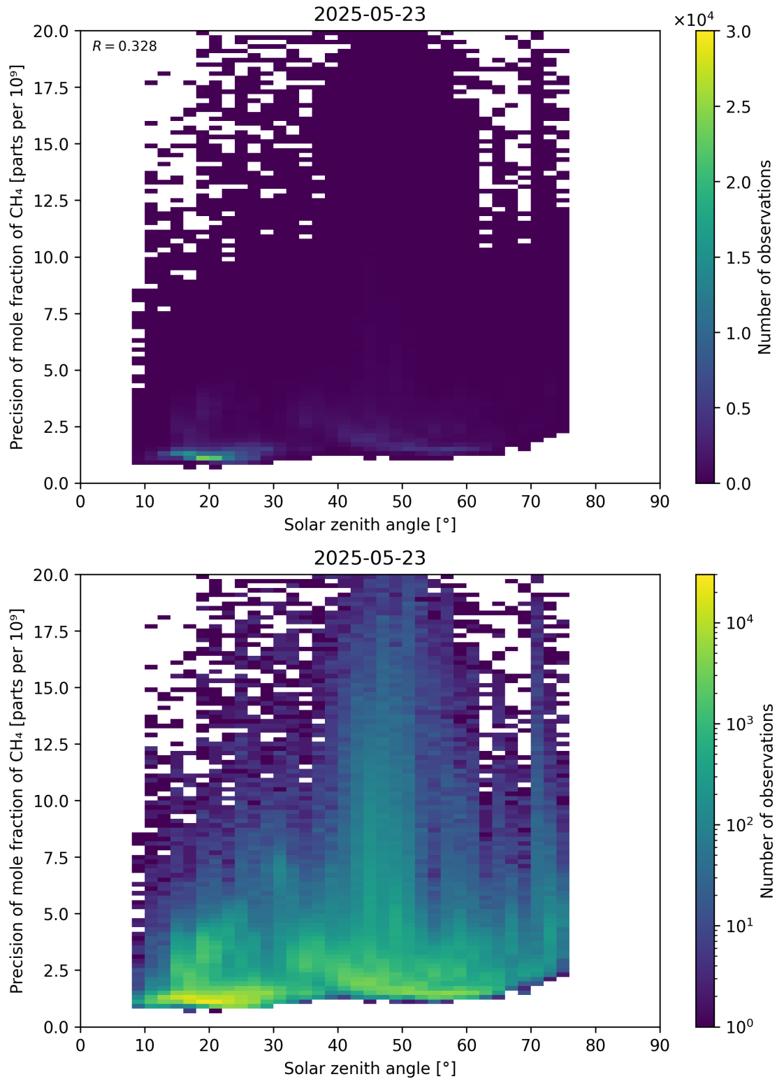
Figure 101: Scatter density plot of “Solar zenith angle” against “Precision of mole fraction of CH 4 ” for 2025-05-22 to 2025-05-24.
