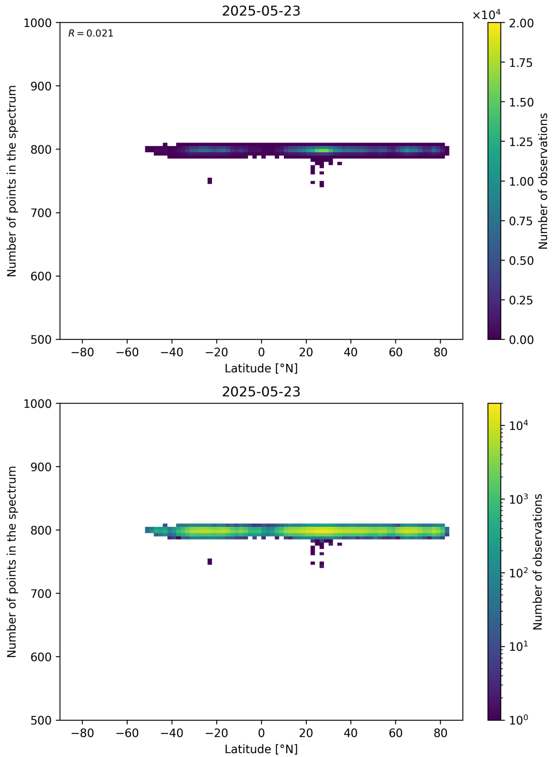
Figure 61: Scatter density plot of “Latitude” against “Number of points in the spectrum” for 2025-05-22 to 2025-05-24.
