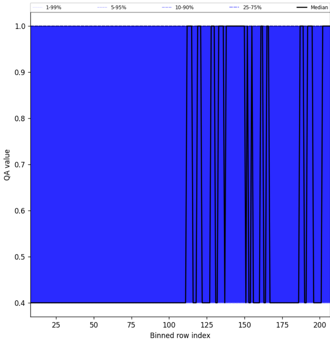
Figure 33: Along track statistics of “QA value” for 2025-05-22 to 2025-05-24
