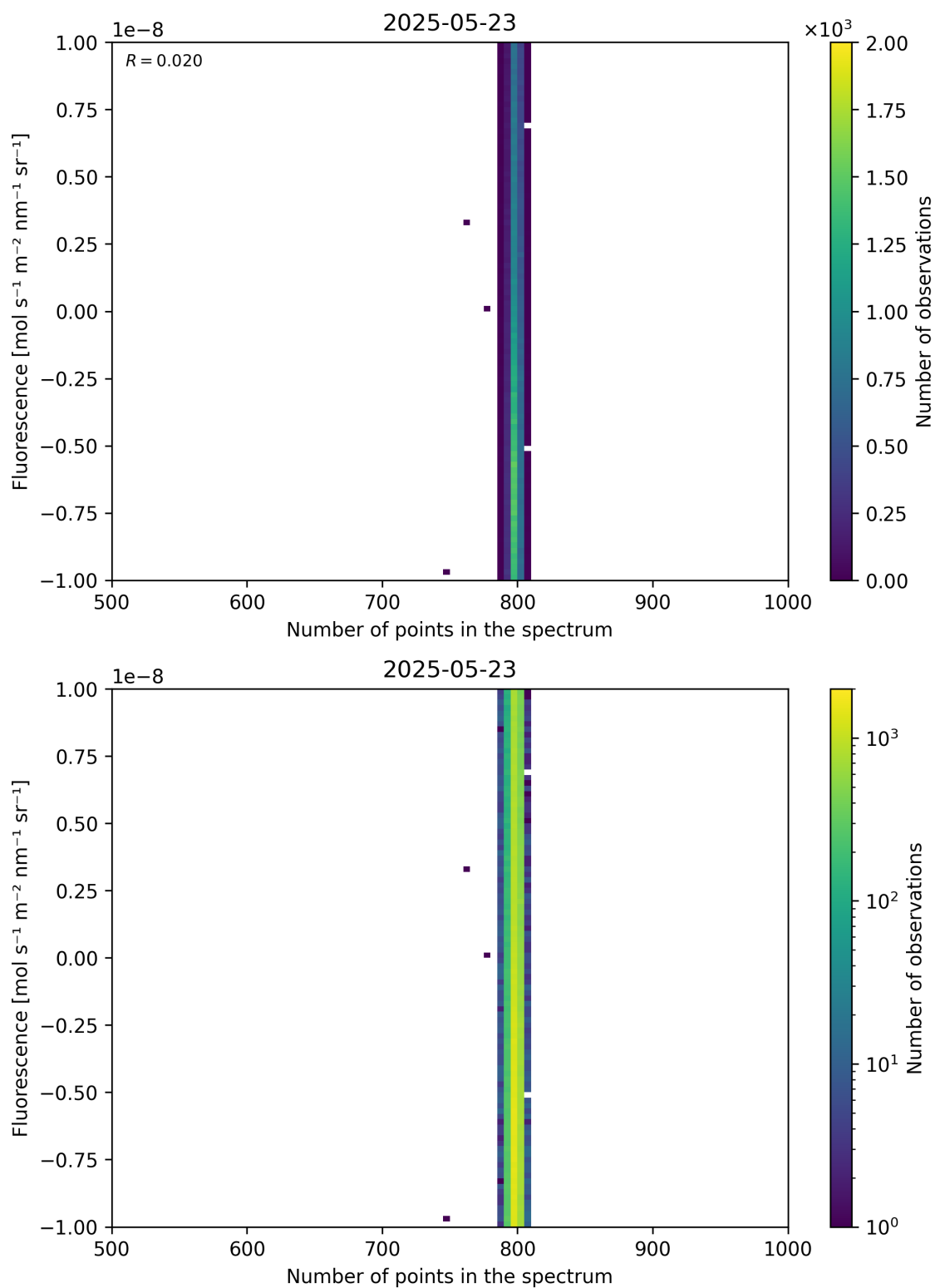
Figure 91: Scatter density plot of “Number of points in the spectrum” against “Fluorescence” for 2025-05-22 to 2025-05-24.
