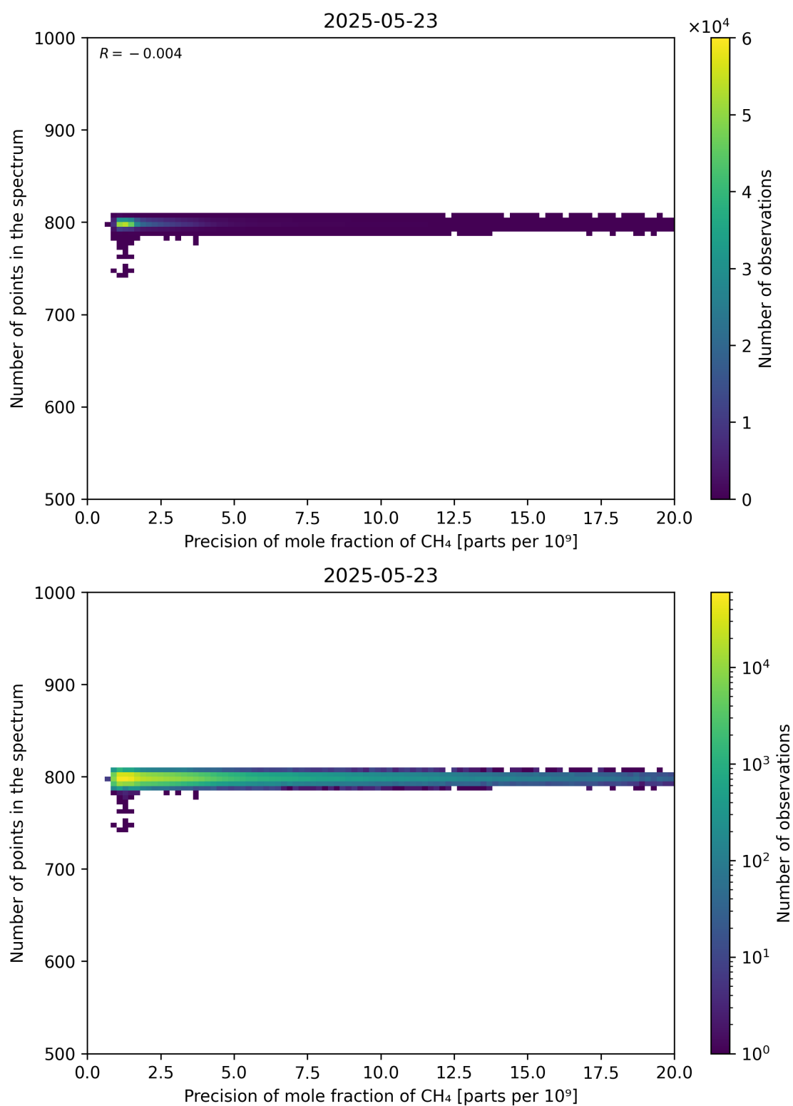
Figure 84: Scatter density plot of “Precision of mole fraction of CH 4 ” against “Number of points in the spectrum” for 2025-05-22 to 2025-05-24.
