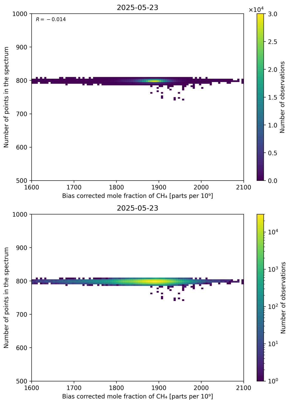
Figure 68: Scatter density plot of “Bias corrected mole fraction of CH 4 ” against “Number of points in the spectrum” for 2025-05-22 to 2025-05-24.
