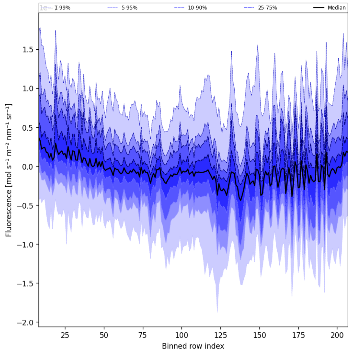
Figure 43: Along track statistics of “Fluorescence” for 2025-05-22 to 2025-05-24
