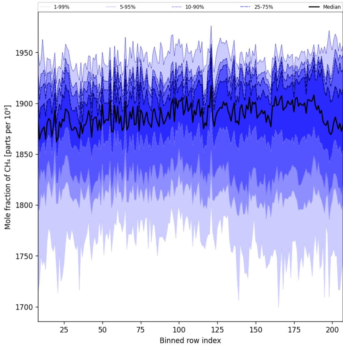
Figure 34: Along track statistics of “Mole fraction of CH 4 ” for 2025-05-22 to 2025-05-24
