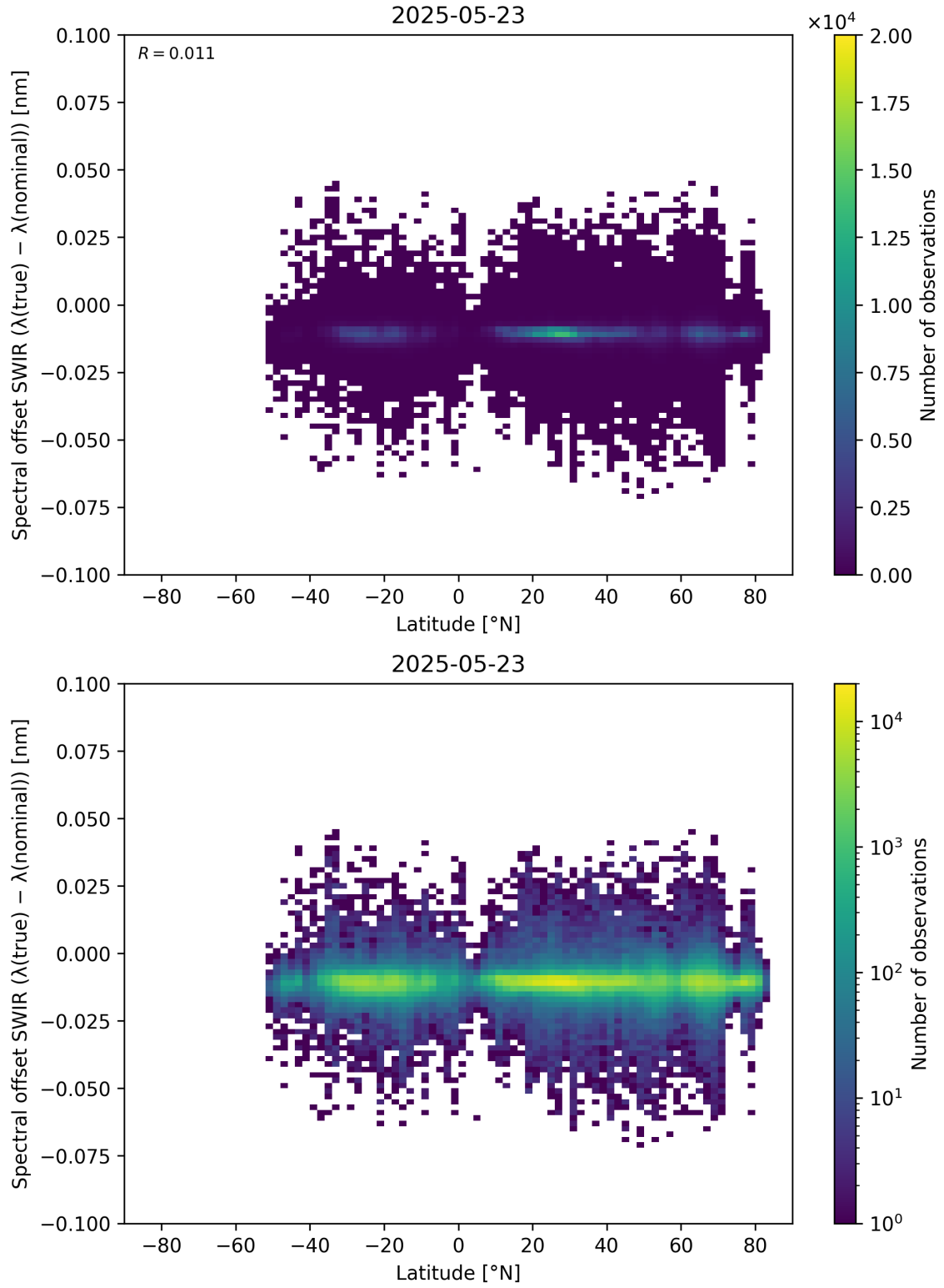
Figure 62: Scatter density plot of “Latitude” against “Spectral offset SWIR ( \lambda_{\text{true}} - \lambda_{\text{nominal}} )” for 2025-05-22 to 2025-05-24.
