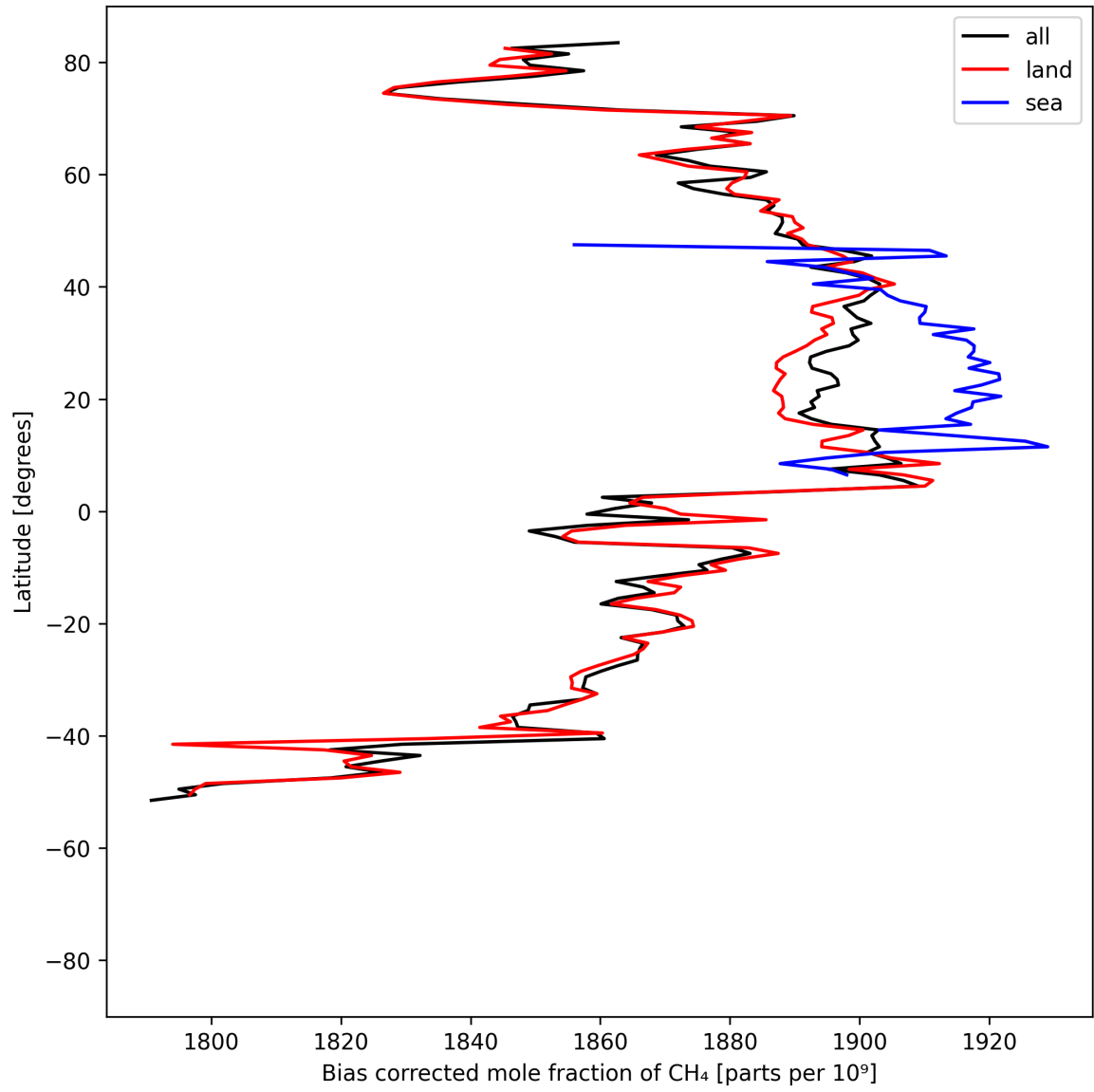
Figure 14: Zonal average of “Bias corrected mole fraction of CH 4 ” for 2025-05-22 to 2025-05-24.
