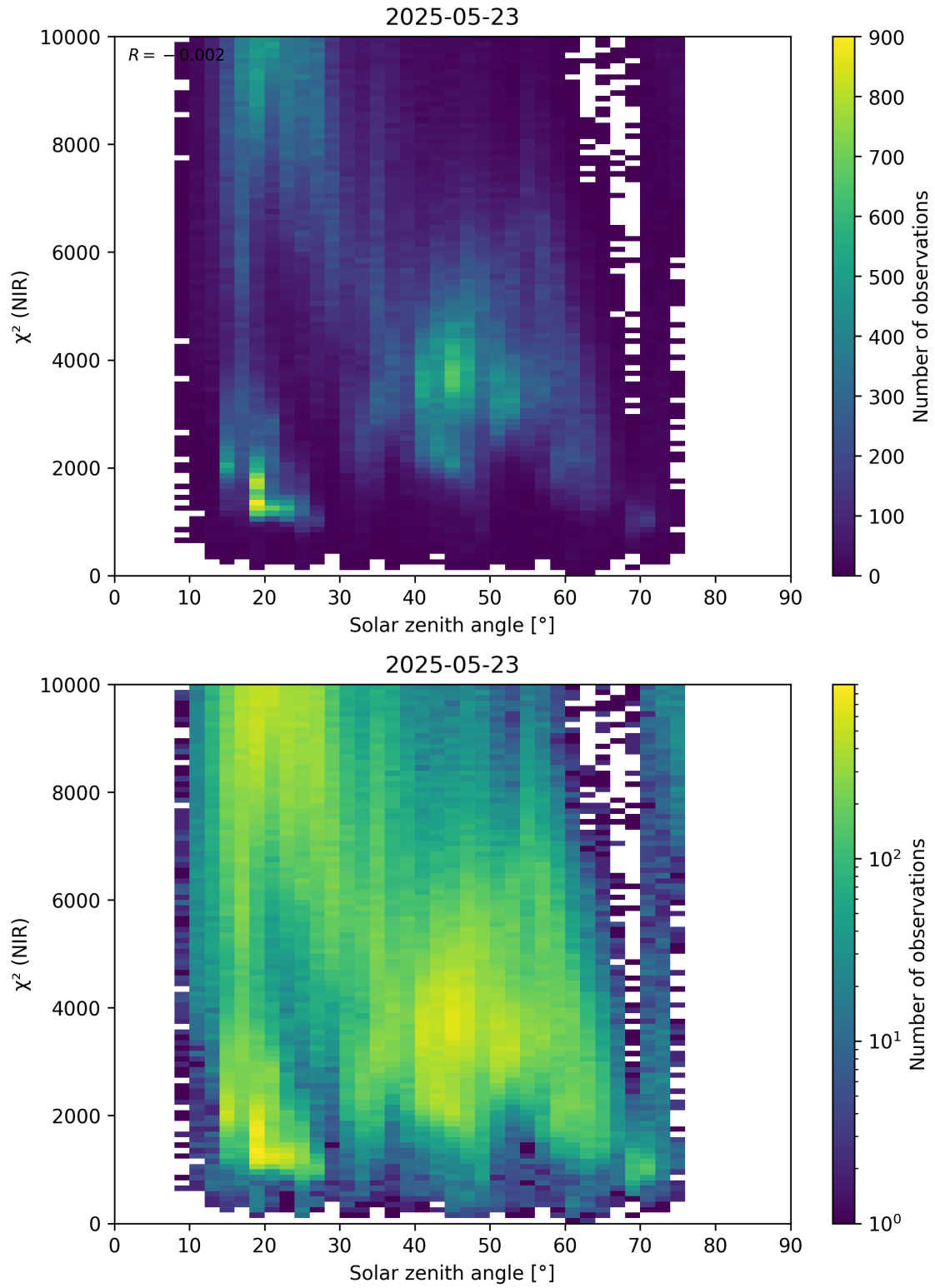
Figure 94: Scatter density plot of “Solar zenith angle” against “ \chi^2 (NIR)” for 2025-05-22 to 2025-05-24.
