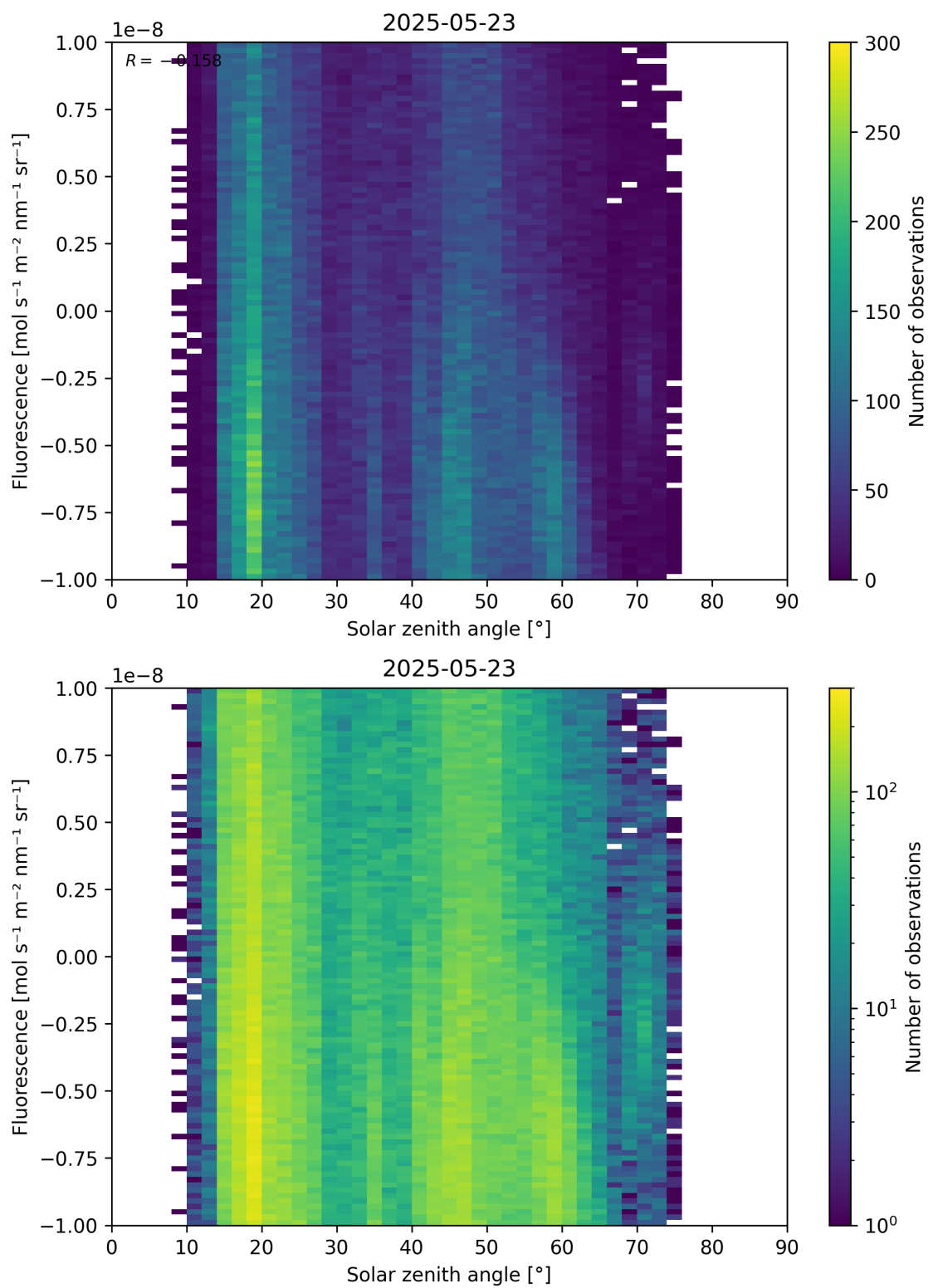
Figure 97: Scatter density plot of “Solar zenith angle” against “Fluorescence” for 2025-05-22 to 2025-05-24.
