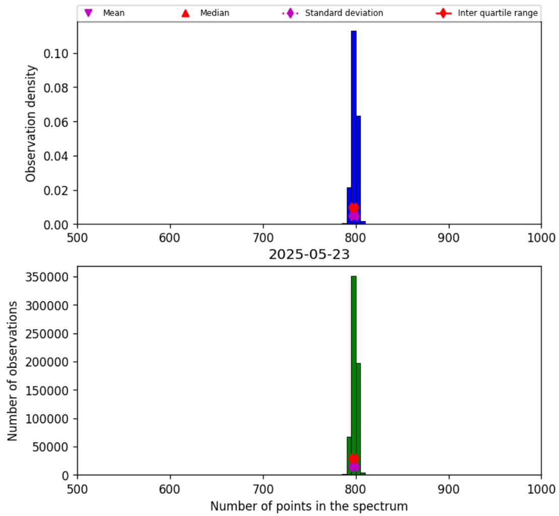
Figure 26: Histogram of “Number of points in the spectrum” for 2025-05-22 to 2025-05-24
