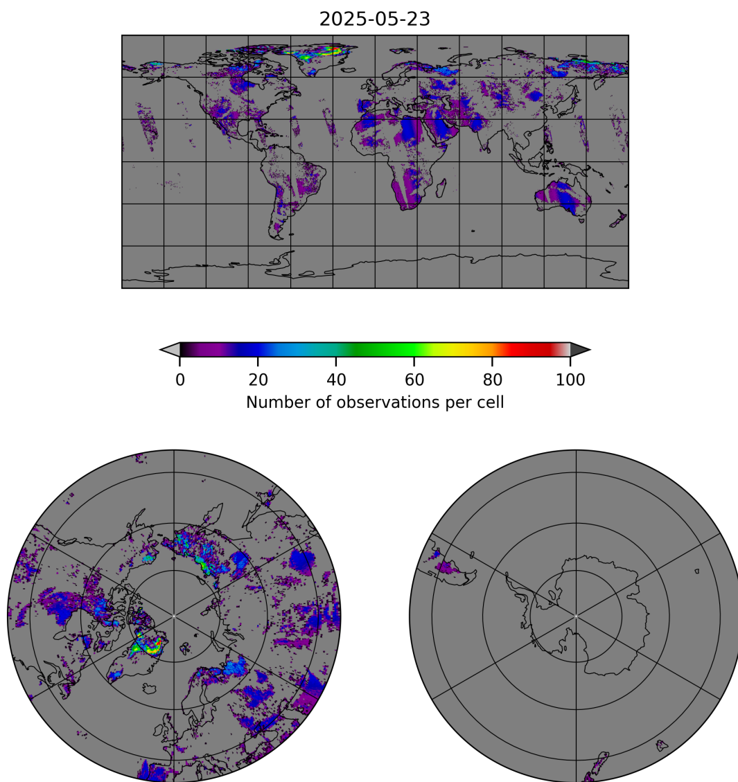
Figure 10: Map of the number of observations for 2025-05-22 to 2025-05-24
