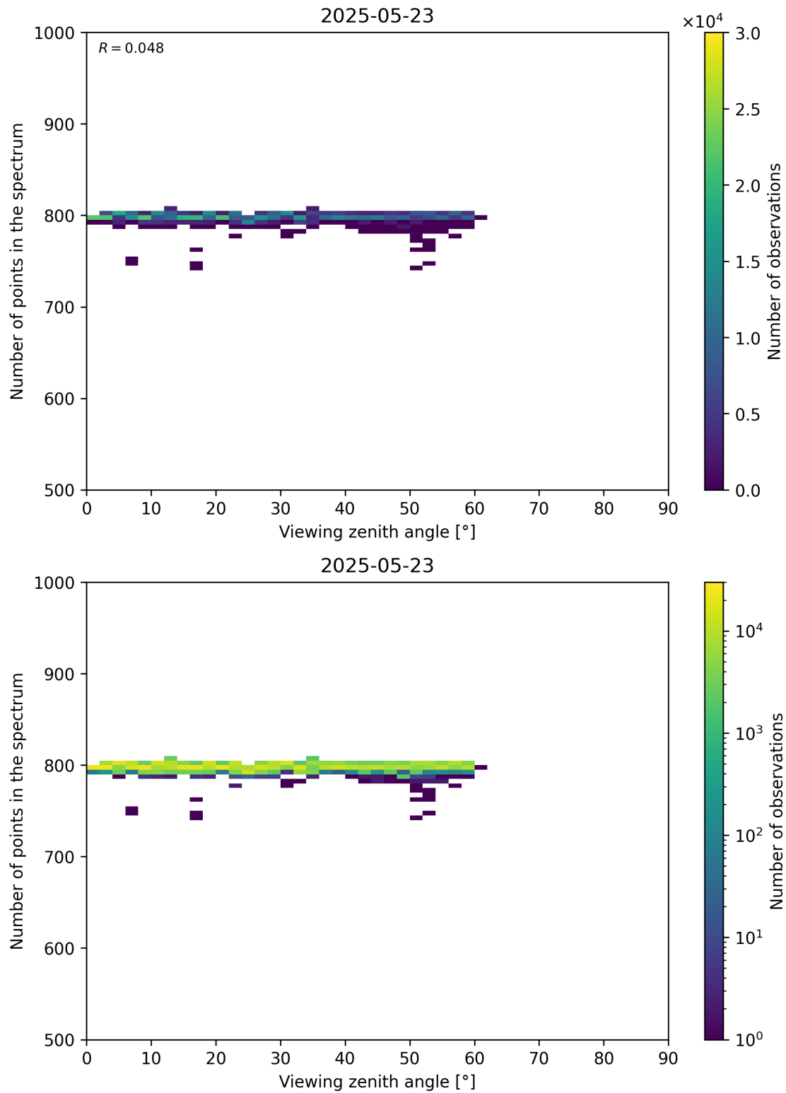
Figure 114: Scatter density plot of “Viewing zenith angle” against “Number of points in the spectrum” for 2025-05-22 to 2025-05-24.
