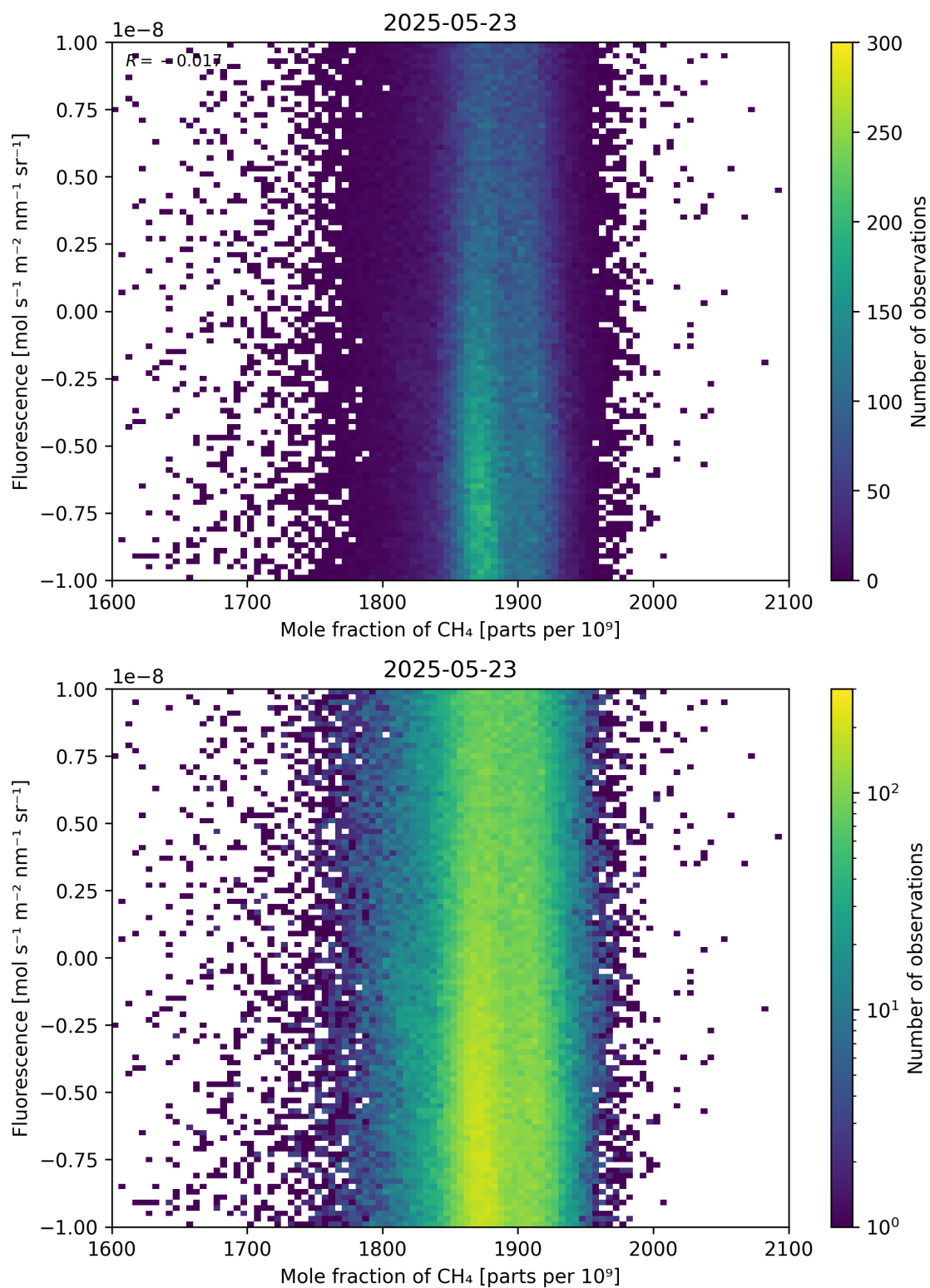
Figure 73: Scatter density plot of “Mole fraction of \text{CH}_4 ” against “Fluorescence” for 2025-05-22 to 2025-05-24.
