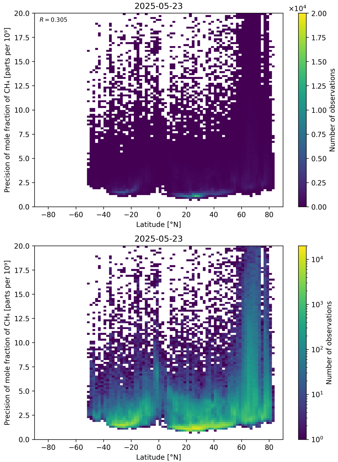
Figure 59: Scatter density plot of “Latitude” against “Precision of mole fraction of \text{CH}_4 ” for 2025-05-22 to 2025-05-24.
