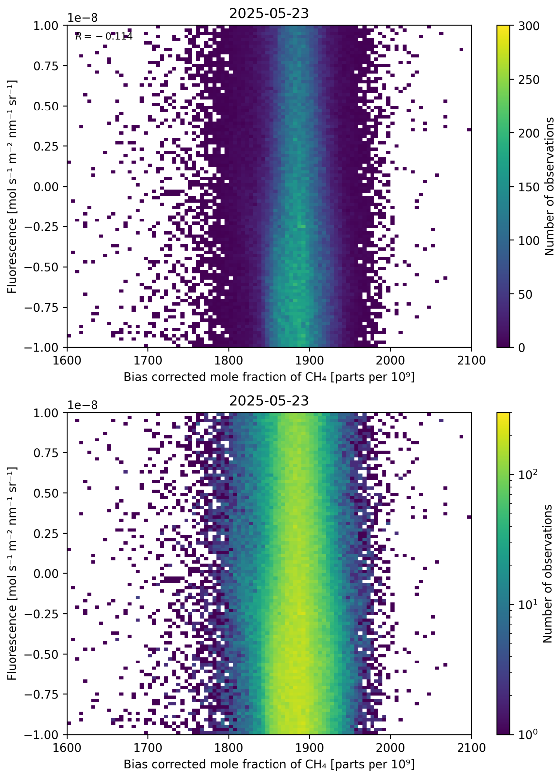
Figure 66: Scatter density plot of “Bias corrected mole fraction of \text{CH}_4 ” against “Fluorescence” for 2025-05-22 to 2025-05-24.
