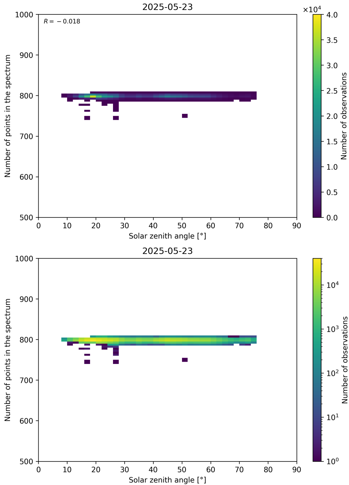
Figure 103: Scatter density plot of “Solar zenith angle” against “Number of points in the spectrum” for 2025-05-22 to 2025-05-24.
