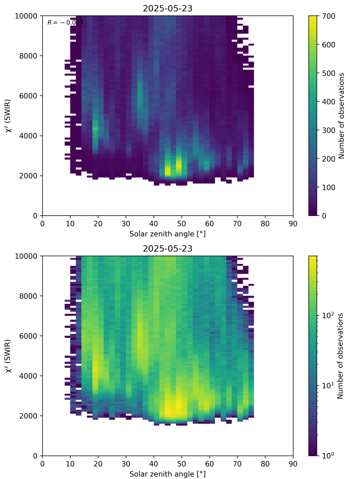
Figure 95: Scatter density plot of “Solar zenith angle” against “ \chi^2 (SWIR)” for 2025-05-22 to 2025-05-24.
