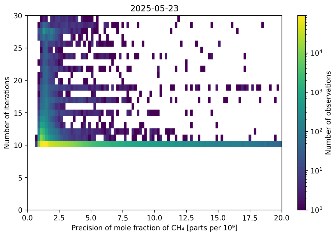
Figure 83: Scatter density plot of “Precision of mole fraction of CH 4 ” against “Number of iterations” for 2025-05-22 to 2025-05-24.
