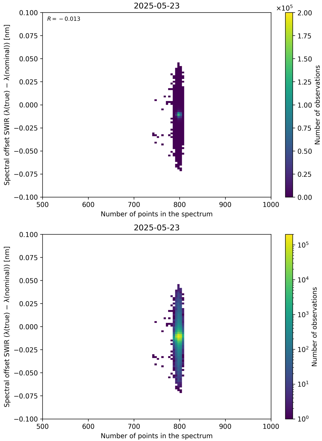
Figure 93: Scatter density plot of “Number of points in the spectrum” against “Spectral offset SWIR ( \lambda_{\text{true}} - \lambda_{\text{nominal}} )” for 2025-05-22 to 2025-05-24.
