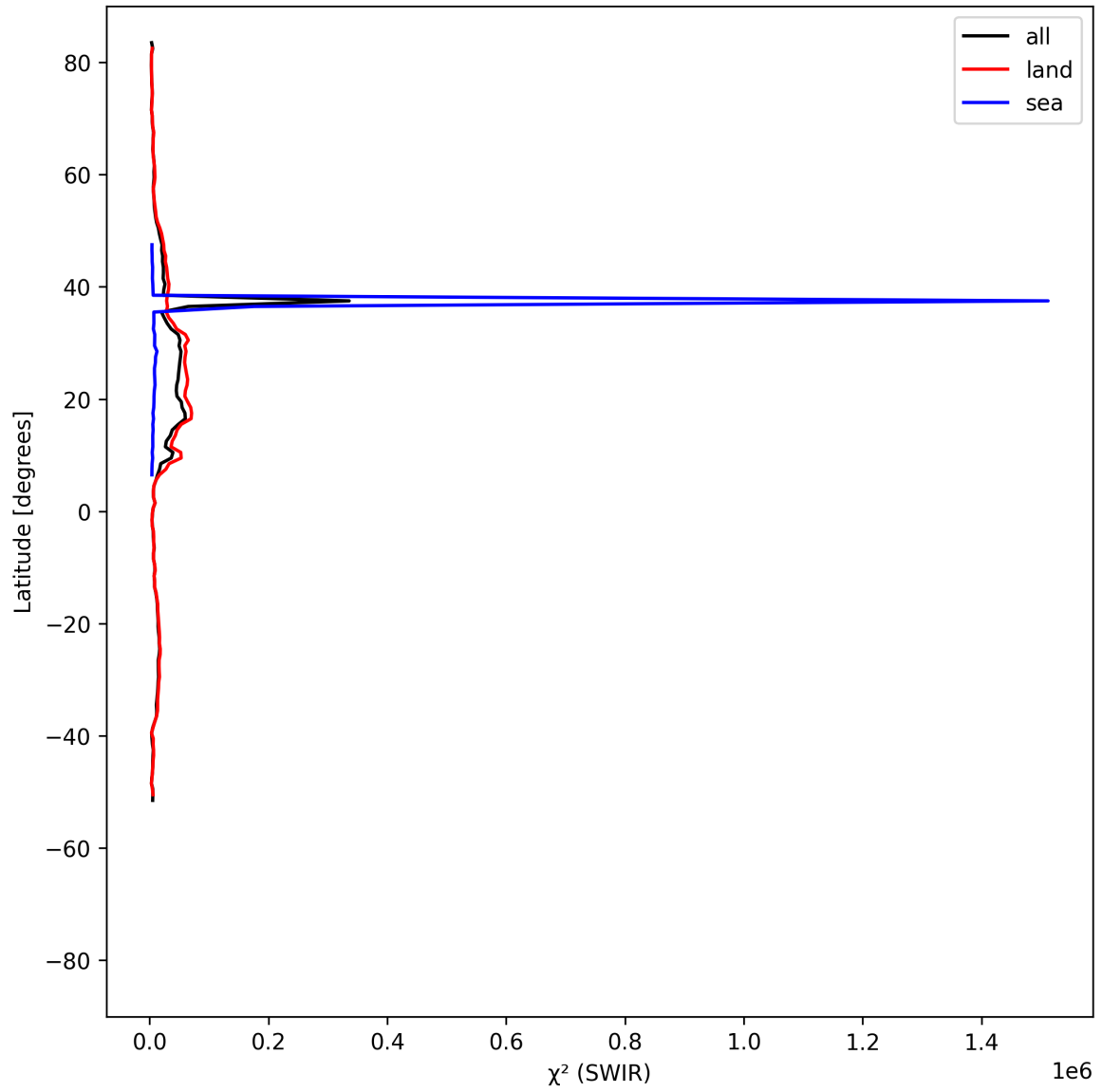
Figure 17: Zonal average of “ \chi^2 (SWIR)” for 2025-05-22 to 2025-05-24.
