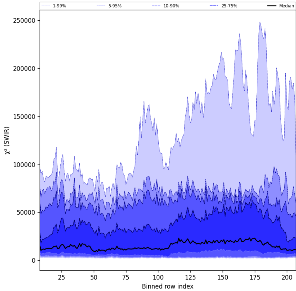
Figure 39: Along track statistics of “ \chi^2 (SWIR)” for 2025-05-22 to 2025-05-24
