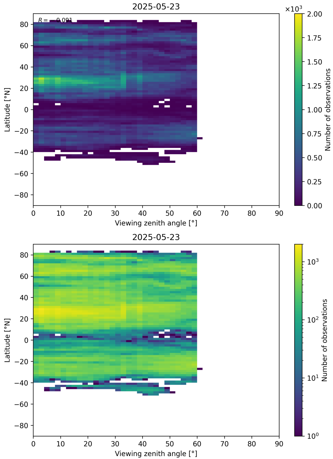
Figure 109: Scatter density plot of “Viewing zenith angle” against “Latitude” for 2025-05-22 to 2025-05-24.
