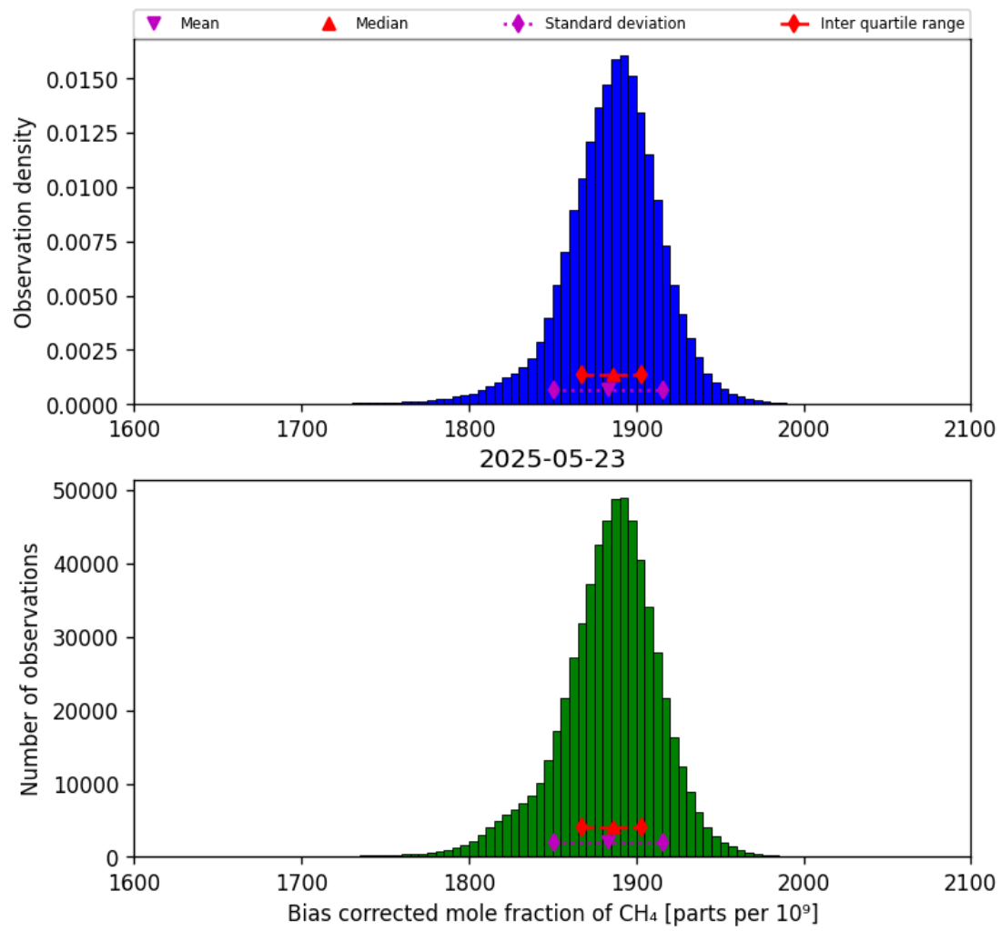
Figure 25: Histogram of “Bias corrected mole fraction of CH 4 ” for 2025-05-22 to 2025-05-24
