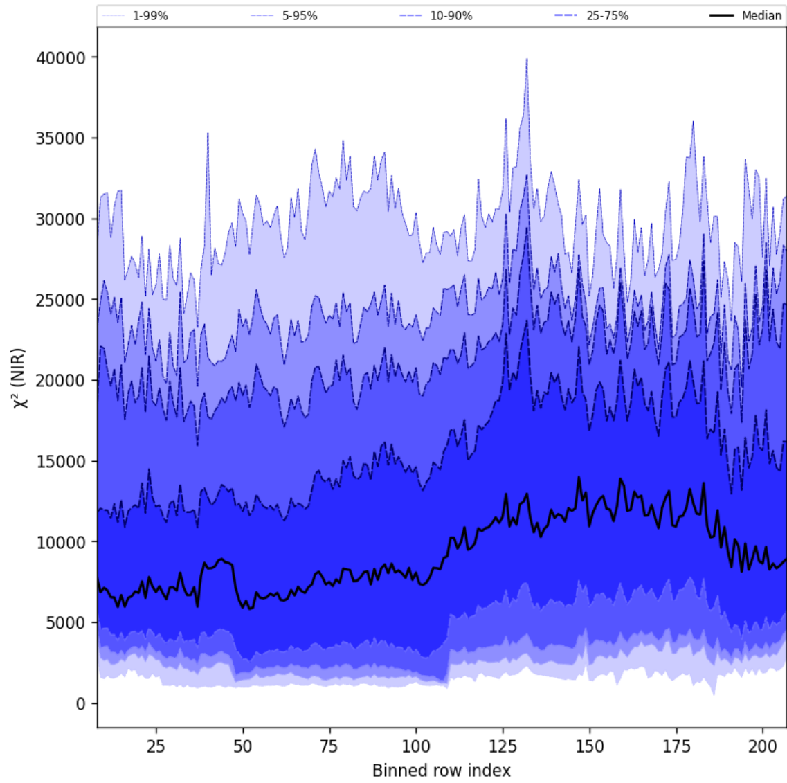
Figure 40: Along track statistics of " \chi^2 (NIR)" for 2025-05-22 to 2025-05-24
