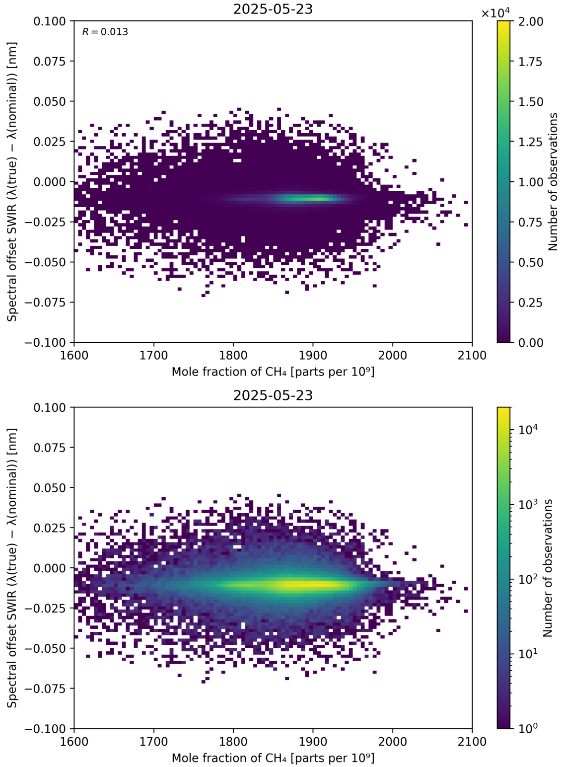
Figure 86: Scatter density plot of “Mole fraction of CH 4 ” against “Spectral offset SWIR ( \lambda_{\text{true}} - \lambda_{\text{nominal}} )” for 2025-05-22 to 2025-05-24.
