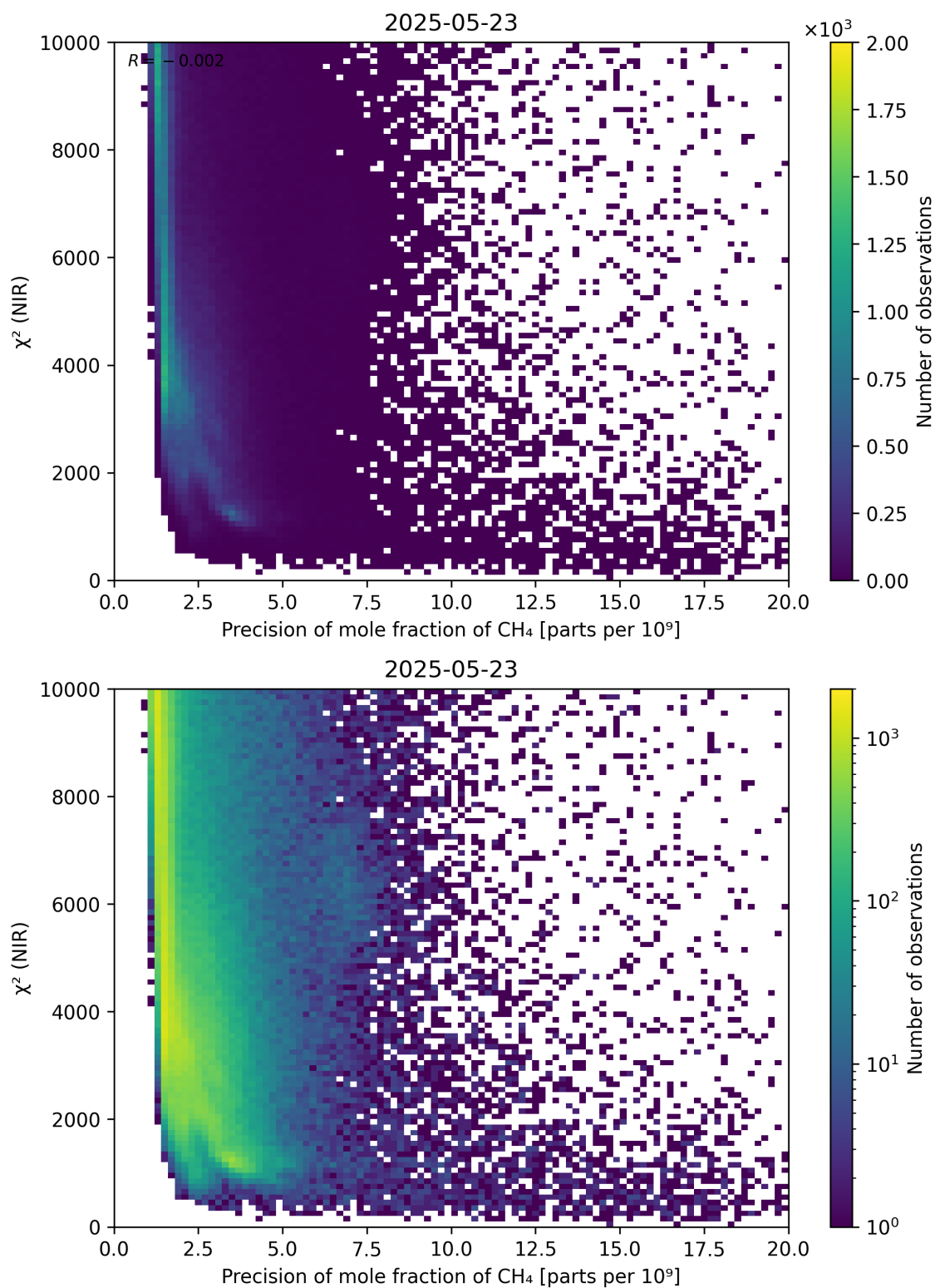
Figure 78: Scatter density plot of “Precision of mole fraction of CH 4 ” against “ \chi^2 (NIR)” for 2025-05-22 to 2025-05-24.
