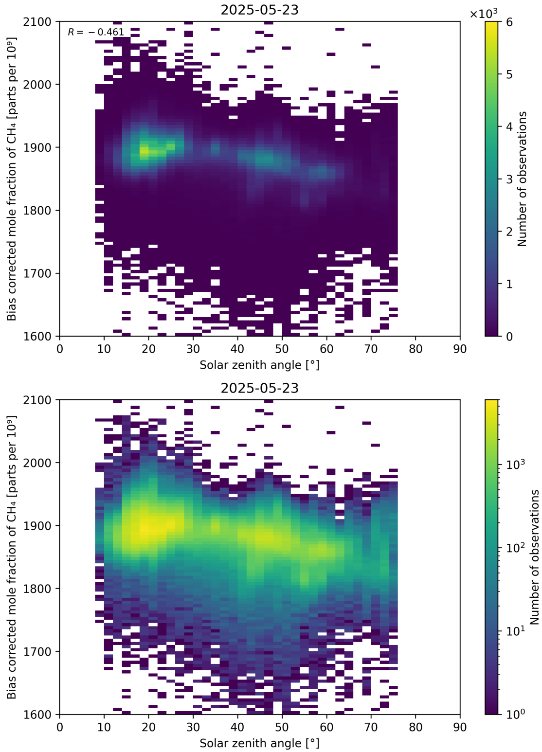
Figure 100: Scatter density plot of “Solar zenith angle” against “Bias corrected mole fraction of CH 4 ” for 2025-05-22 to 2025-05-24.
