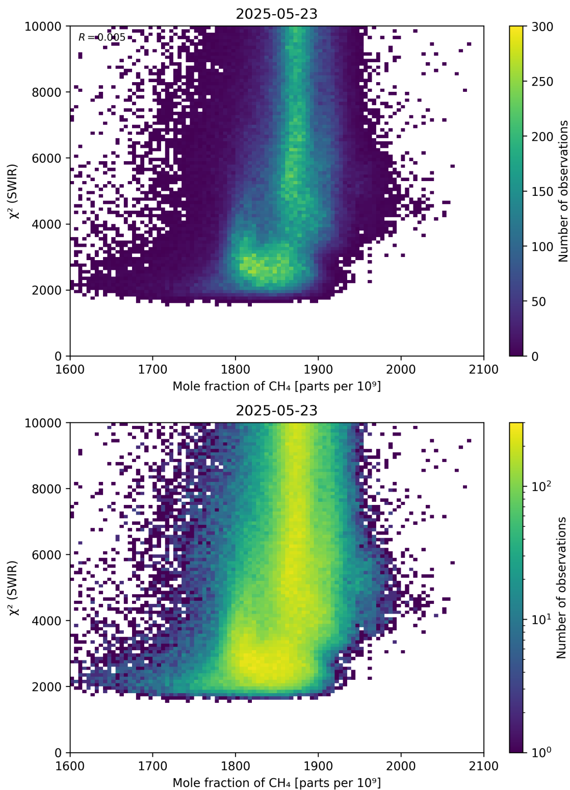
Figure 71: Scatter density plot of “Mole fraction of \text{CH}_4 ” against “ \chi^2 (SWIR)” for 2025-05-22 to 2025-05-24.
