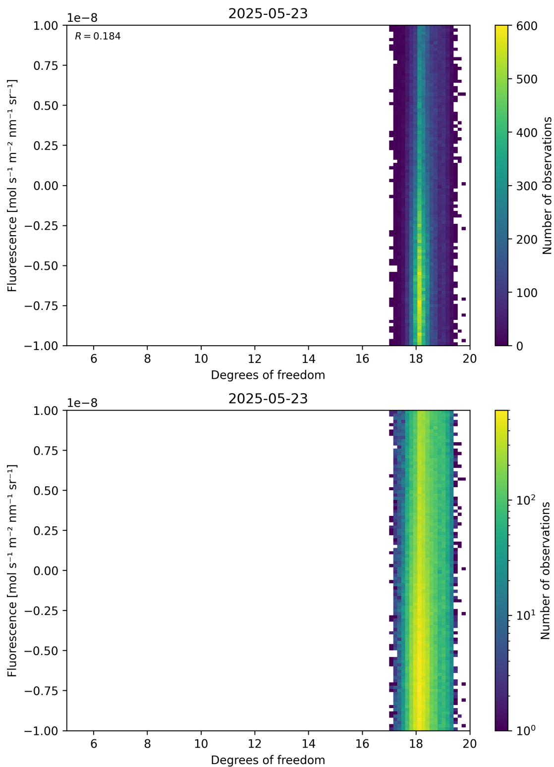
Figure 51: Scatter density plot of “Degrees of freedom” against “Fluorescence” for 2025-05-22 to 2025-05-24.
