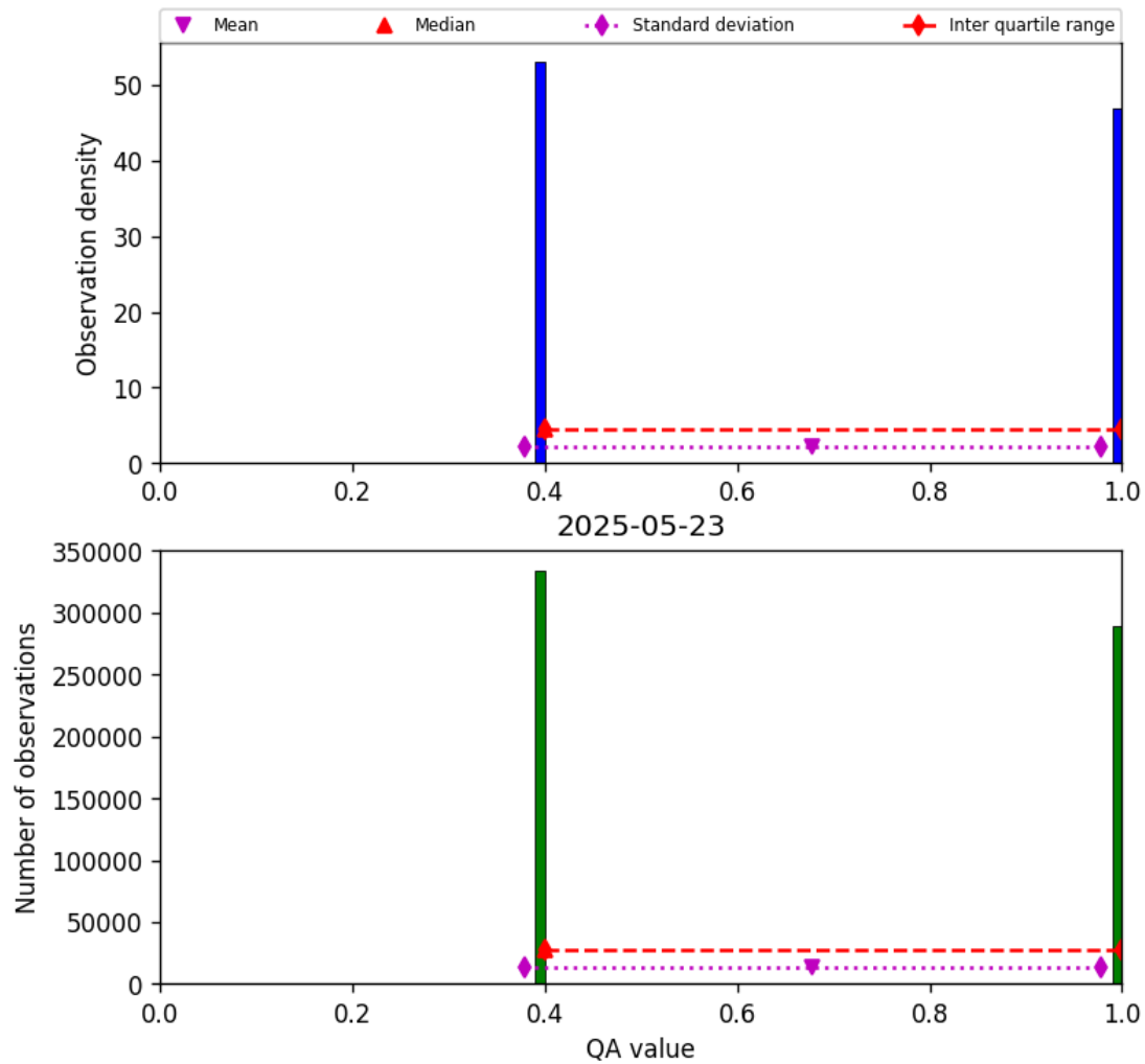
Figure 22: Histogram of “QA value” for 2025-05-22 to 2025-05-24
