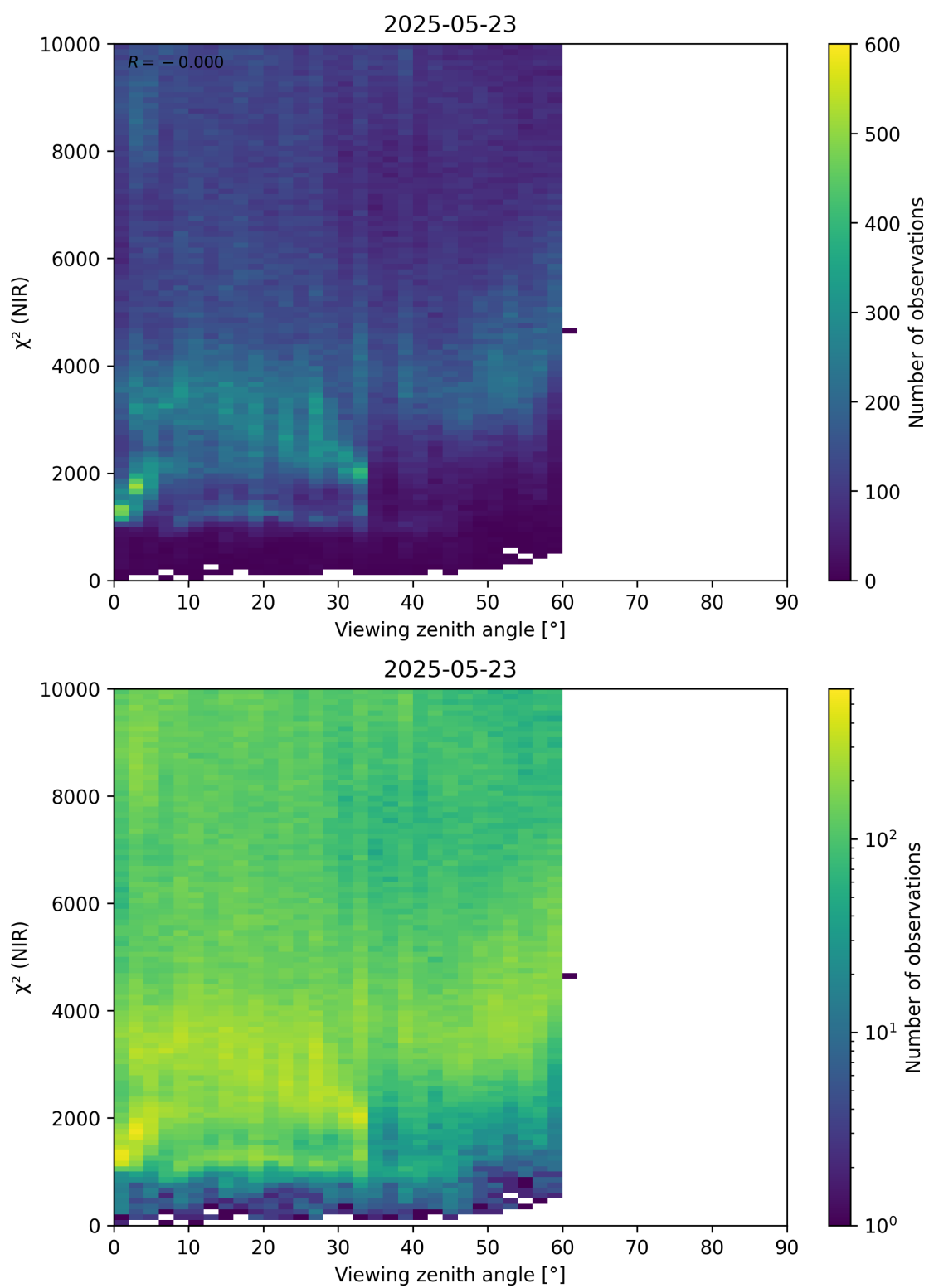
Figure 105: Scatter density plot of “Viewing zenith angle” against “ \chi^2 (NIR)” for 2025-05-22 to 2025-05-24.
