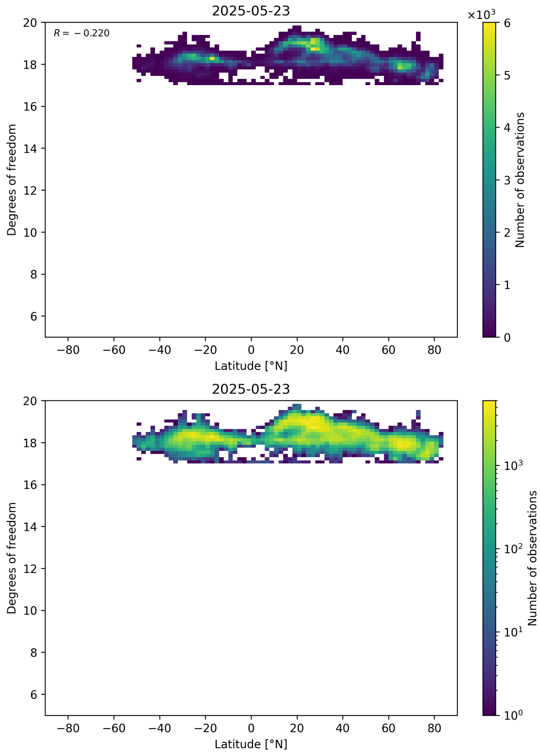
Figure 55: Scatter density plot of “Latitude” against “Degrees of freedom” for 2025-05-22 to 2025-05-24.
