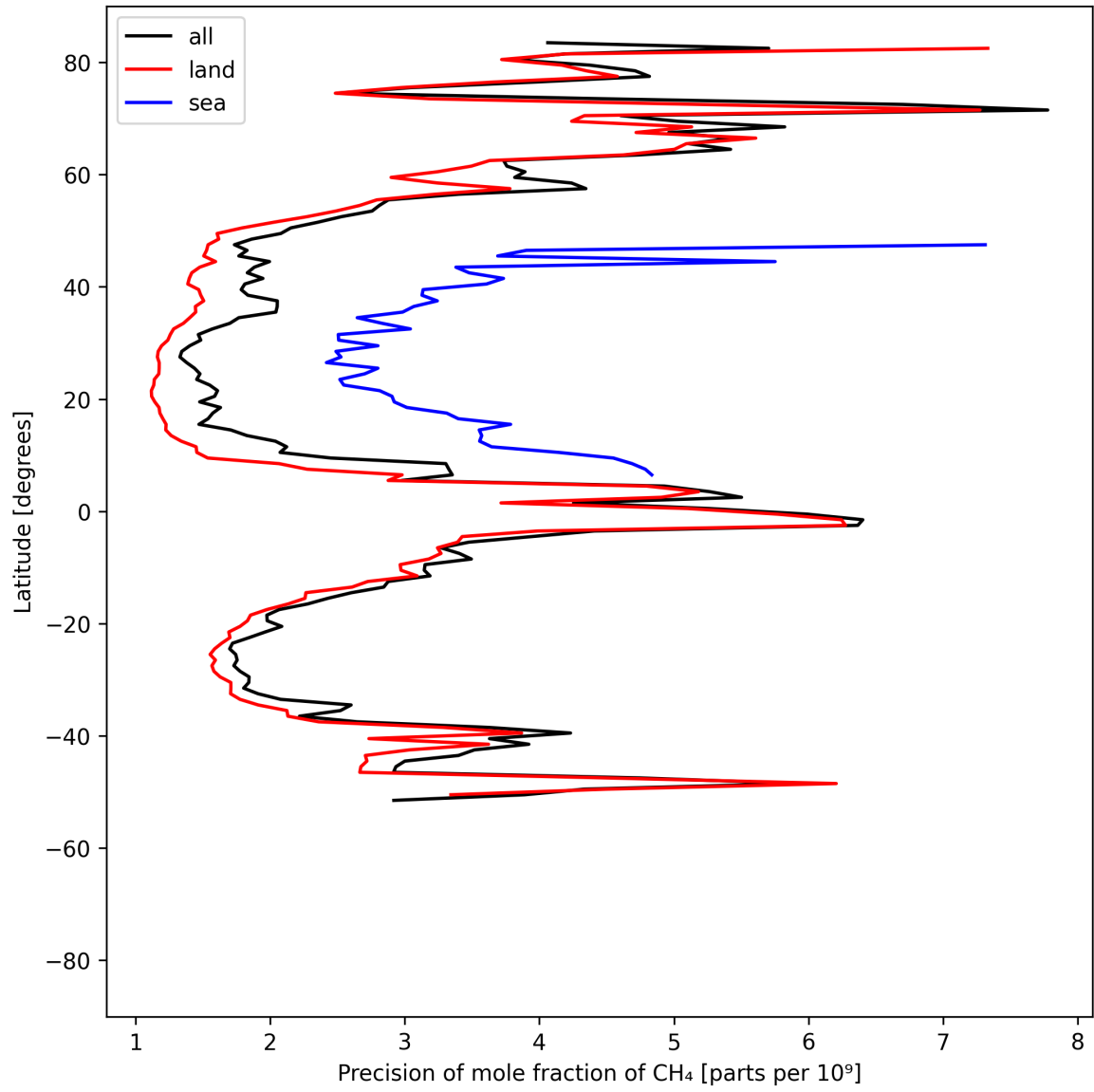
Figure 13: Zonal average of “Precision of mole fraction of CH 4 ” for 2025-05-22 to 2025-05-24.
