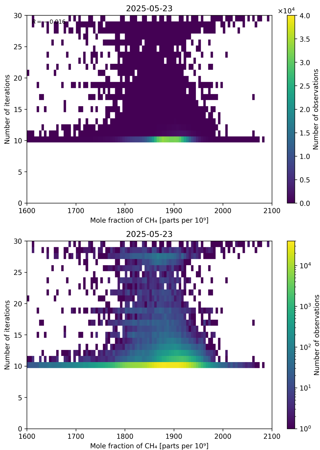
Figure 76: Scatter density plot of “Mole fraction of CH 4 ” against “Number of iterations” for 2025-05-22 to 2025-05-24.
