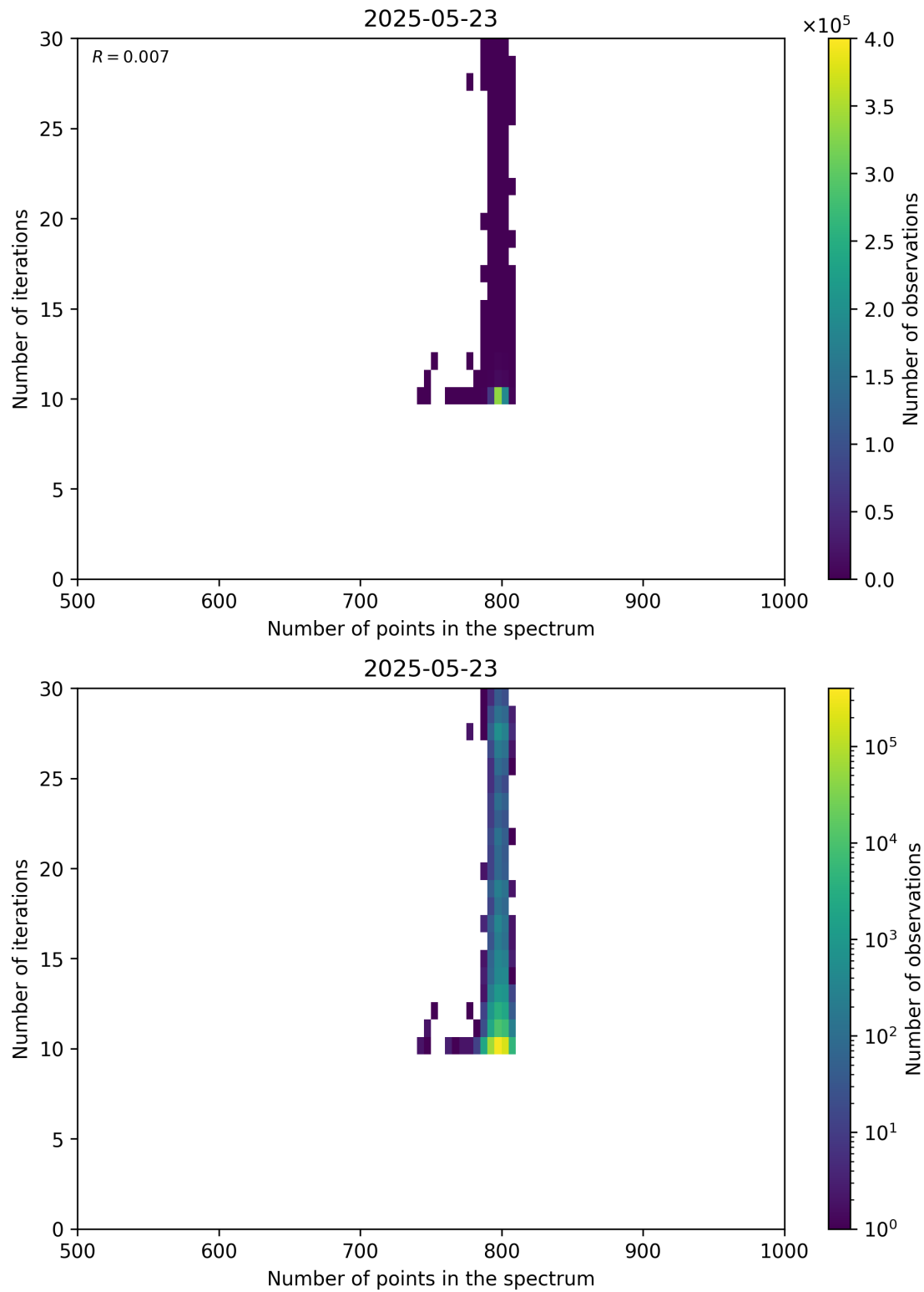
Figure 92: Scatter density plot of “Number of points in the spectrum” against “Number of iterations” for 2025-05-22 to 2025-05-24.
