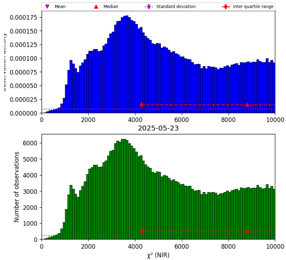
Figure 29: Histogram of “ \chi^2 (NIR)” for 2025-05-22 to 2025-05-24
