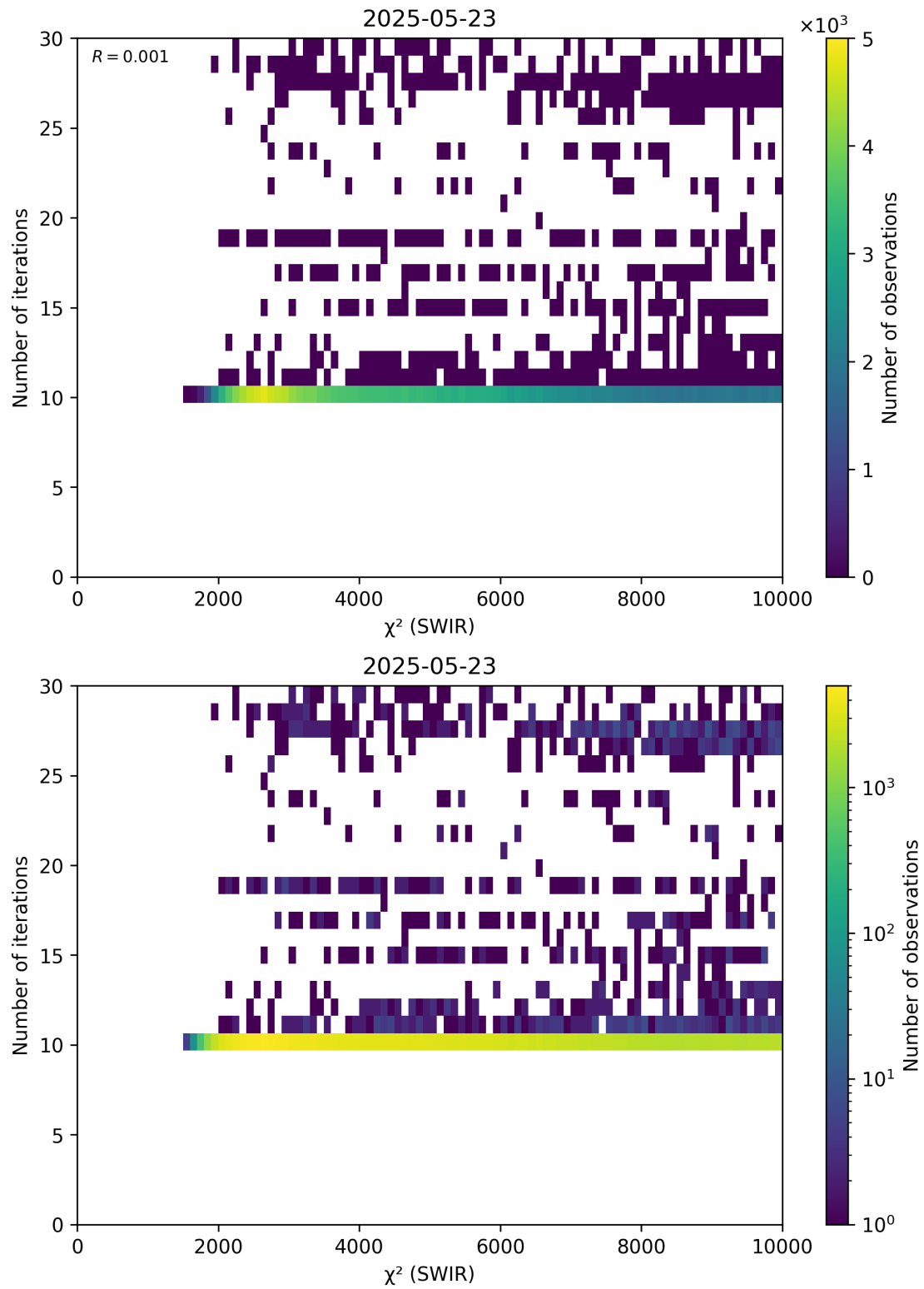
Figure 50: Scatter density plot of “ \chi^2 (SWIR)” against “Number of iterations” for 2025-05-22 to 2025-05-24.
