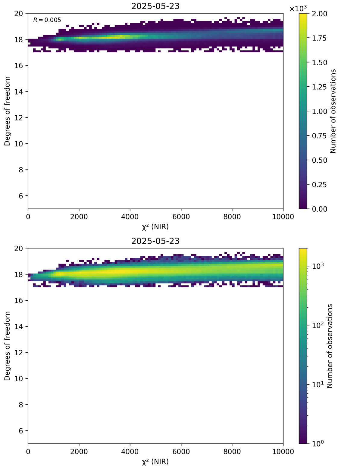
Figure 44: Scatter density plot of “ \chi^2 (NIR)” against “Degrees of freedom” for 2025-05-22 to 2025-05-24.
