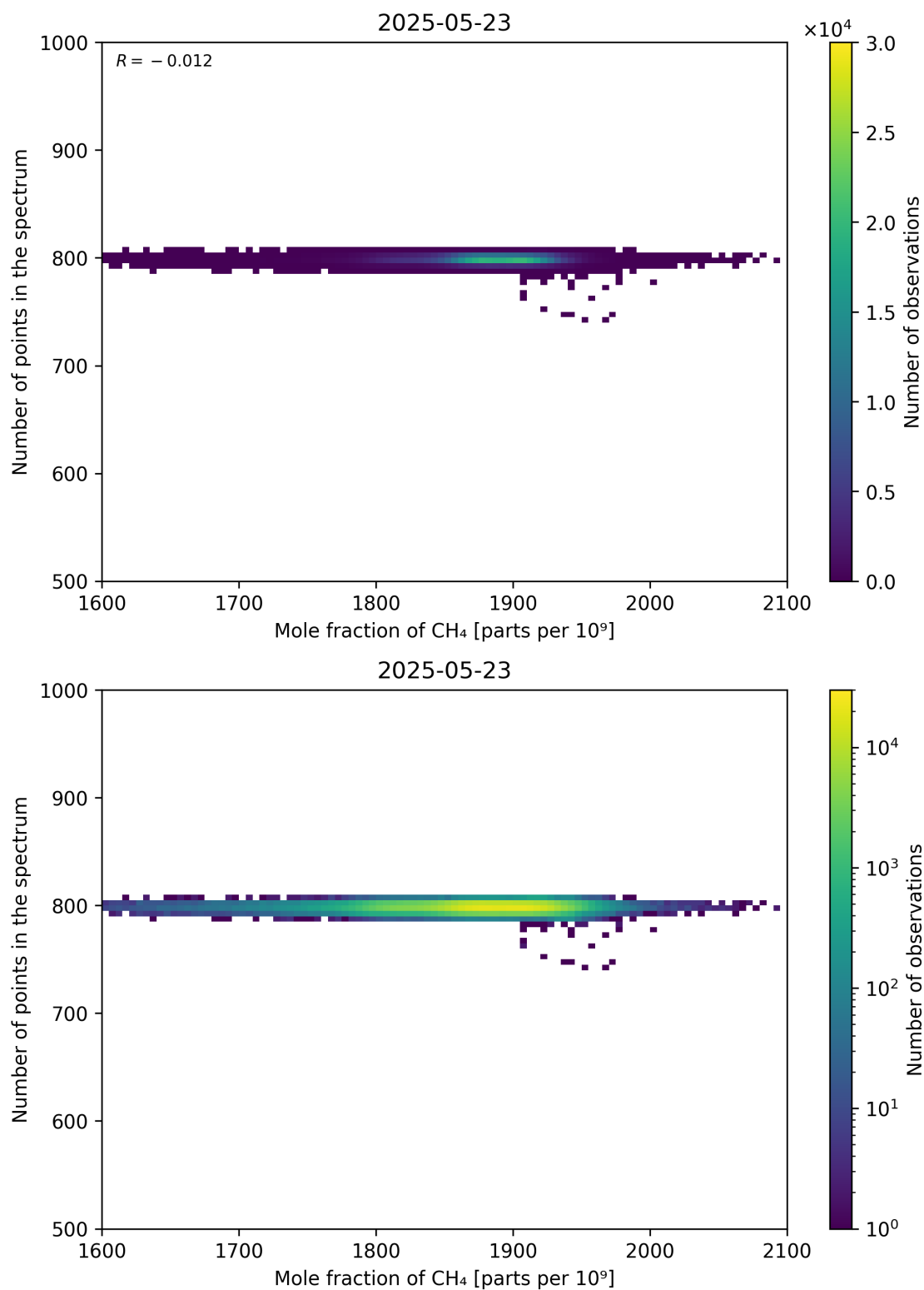
Figure 77: Scatter density plot of “Mole fraction of CH 4 ” against “Number of points in the spectrum” for 2025-05-22 to 2025-05-24.
