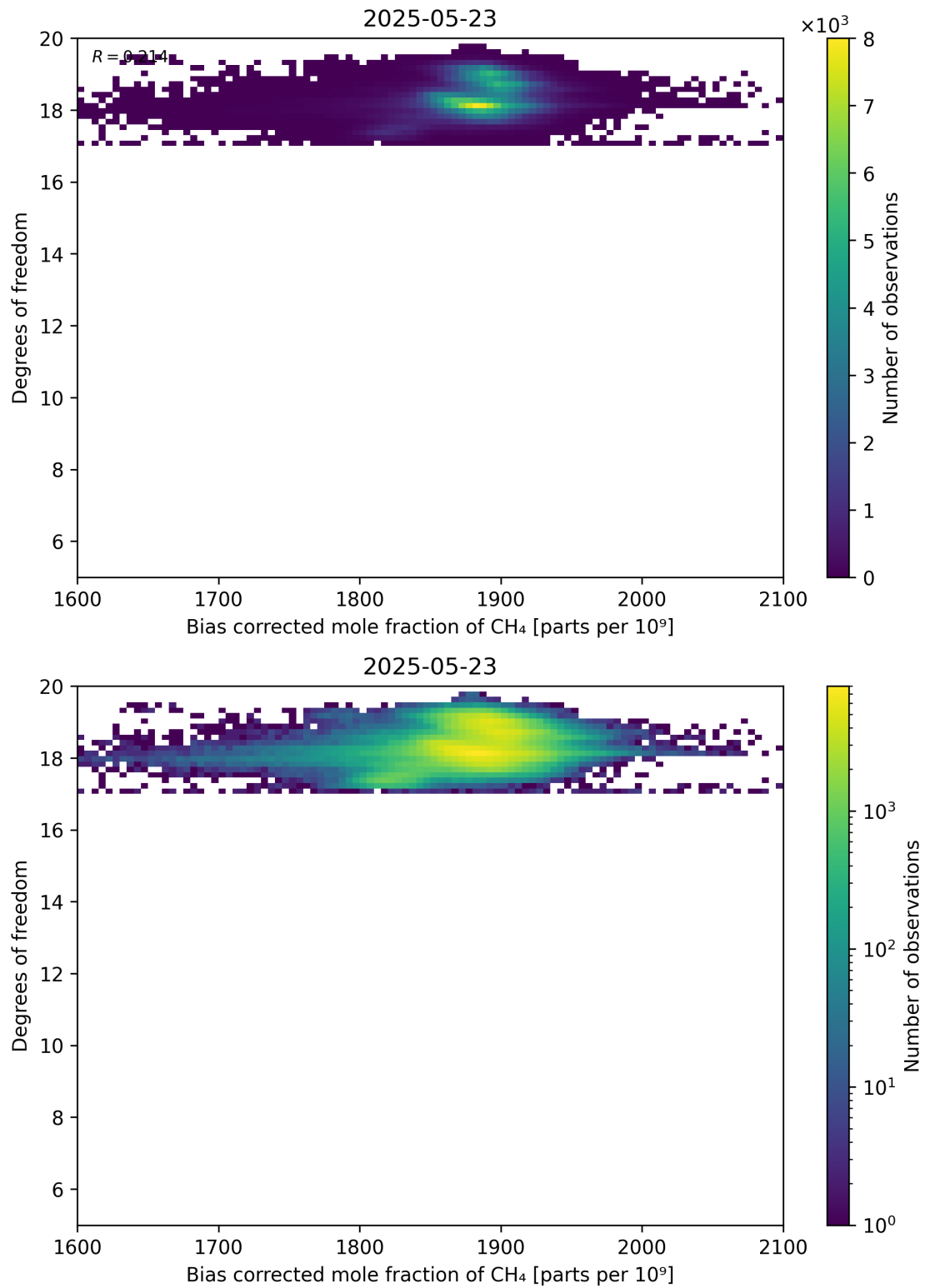
Figure 65: Scatter density plot of “Bias corrected mole fraction of CH 4 ” against “Degrees of freedom” for 2025-05-22 to 2025-05-24.
