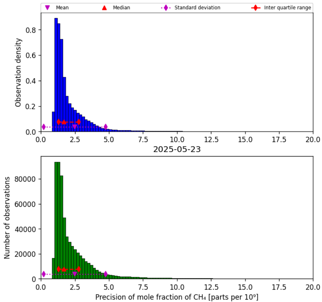
Figure 24: Histogram of “Precision of mole fraction of CH 4 ” for 2025-05-22 to 2025-05-24
