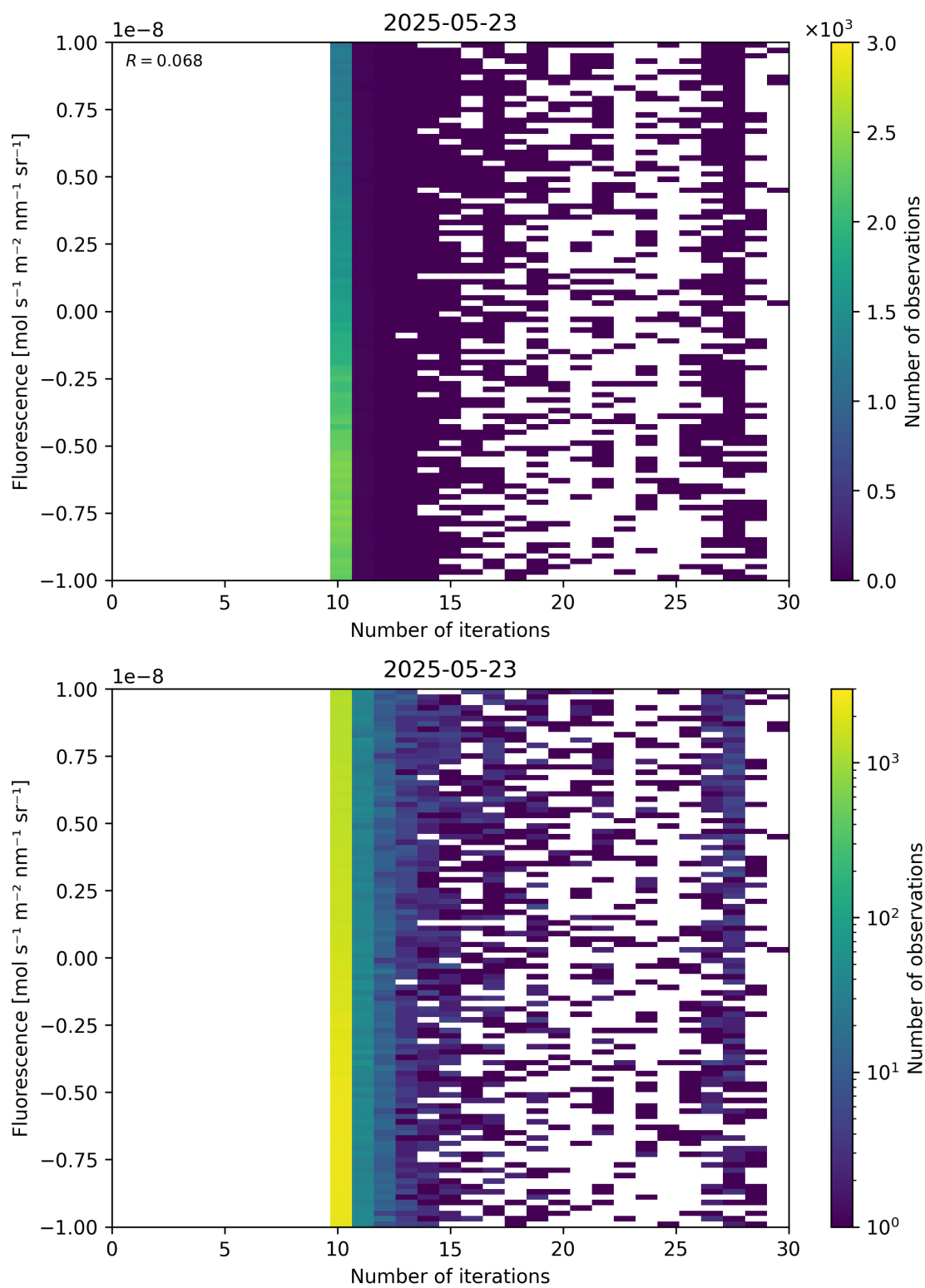
Figure 87: Scatter density plot of “Number of iterations” against “Fluorescence” for 2025-05-22 to 2025-05-24.
