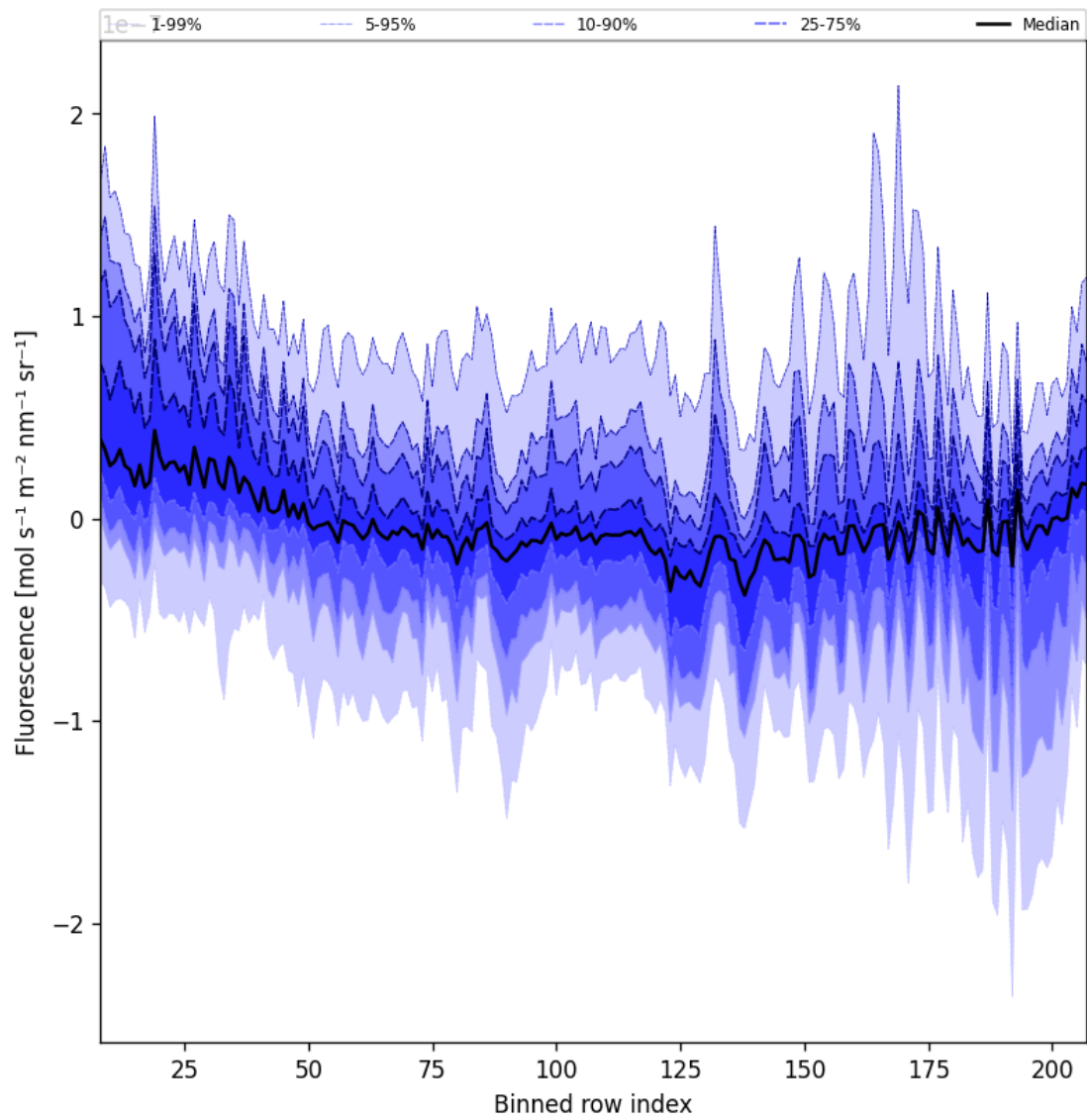
Figure 43: Along track statistics of “Fluorescence” for 2025-05-23 to 2025-05-25
