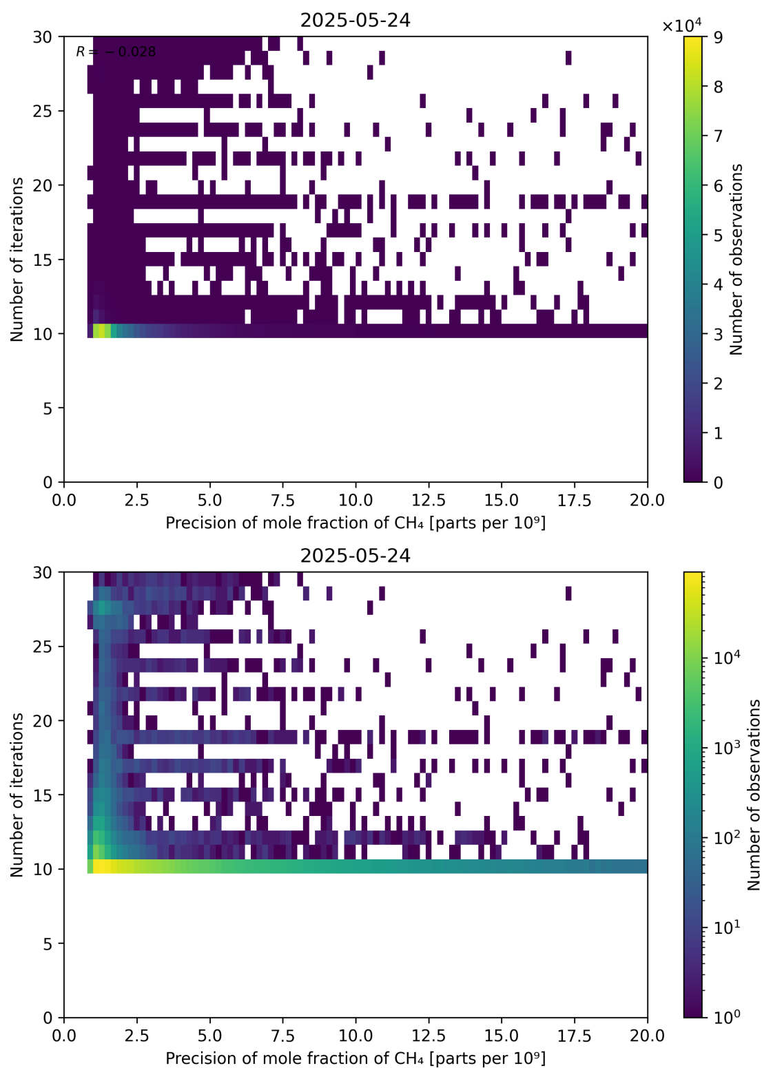
Figure 83: Scatter density plot of “Precision of mole fraction of CH 4 ” against “Number of iterations” for 2025-05-23 to 2025-05-25.
