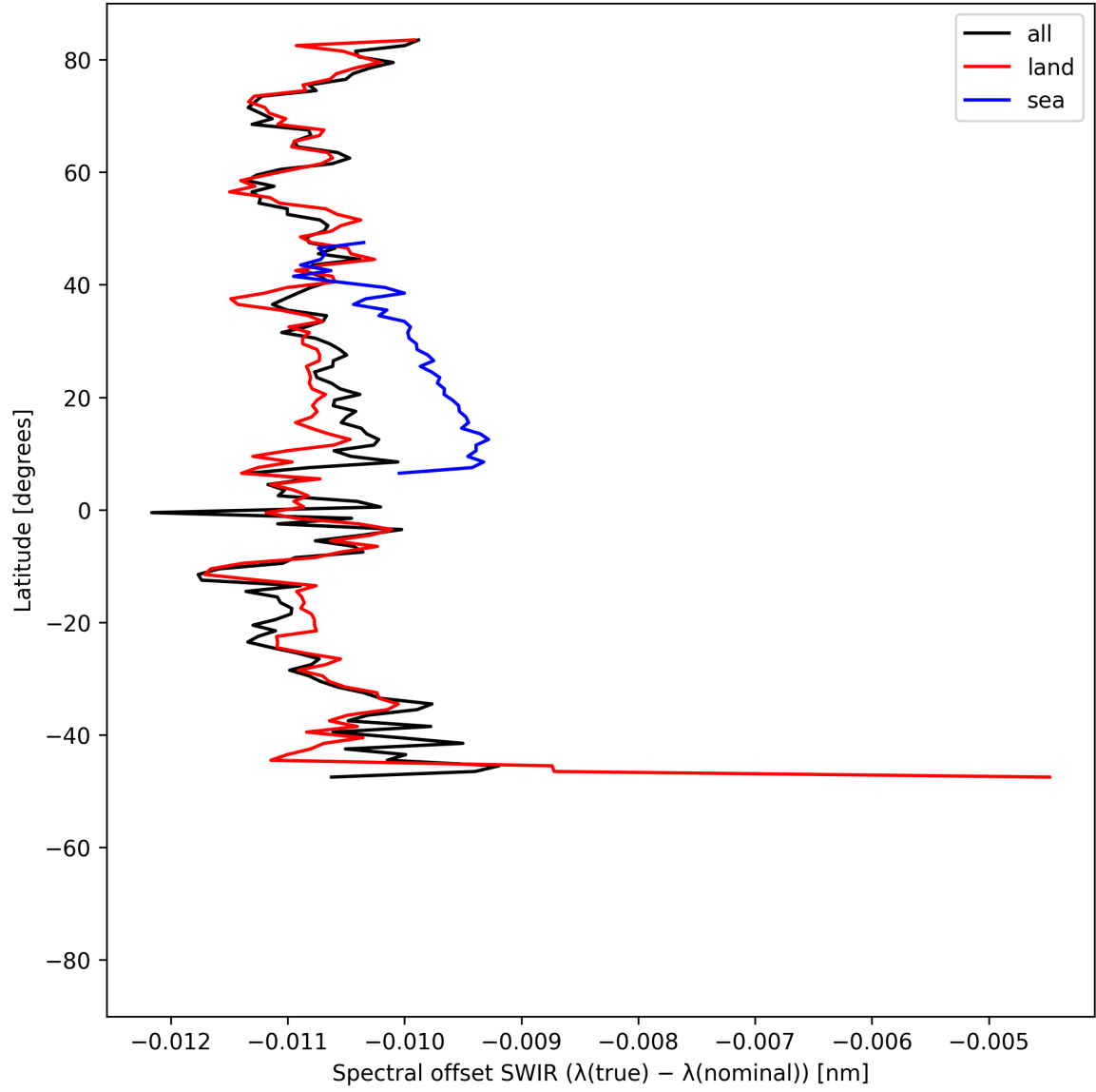
Figure 16: Zonal average of “Spectral offset SWIR ( \lambda_{\text{true}} - \lambda_{\text{nominal}} )” for 2025-05-23 to 2025-05-25.
