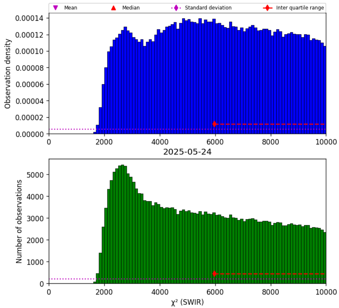
Figure 28: Histogram of “ \chi^2 (SWIR)” for 2025-05-23 to 2025-05-25
