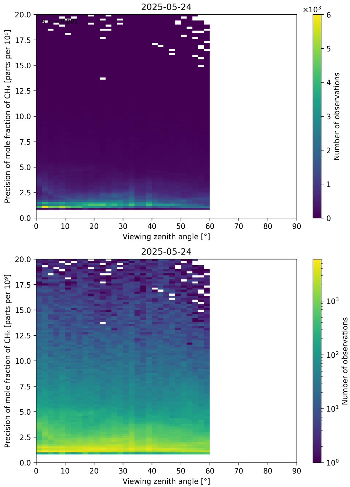
Figure 112: Scatter density plot of “Viewing zenith angle” against “Precision of mole fraction of CH 4 ” for 2025-05-23 to 2025-05-25.
