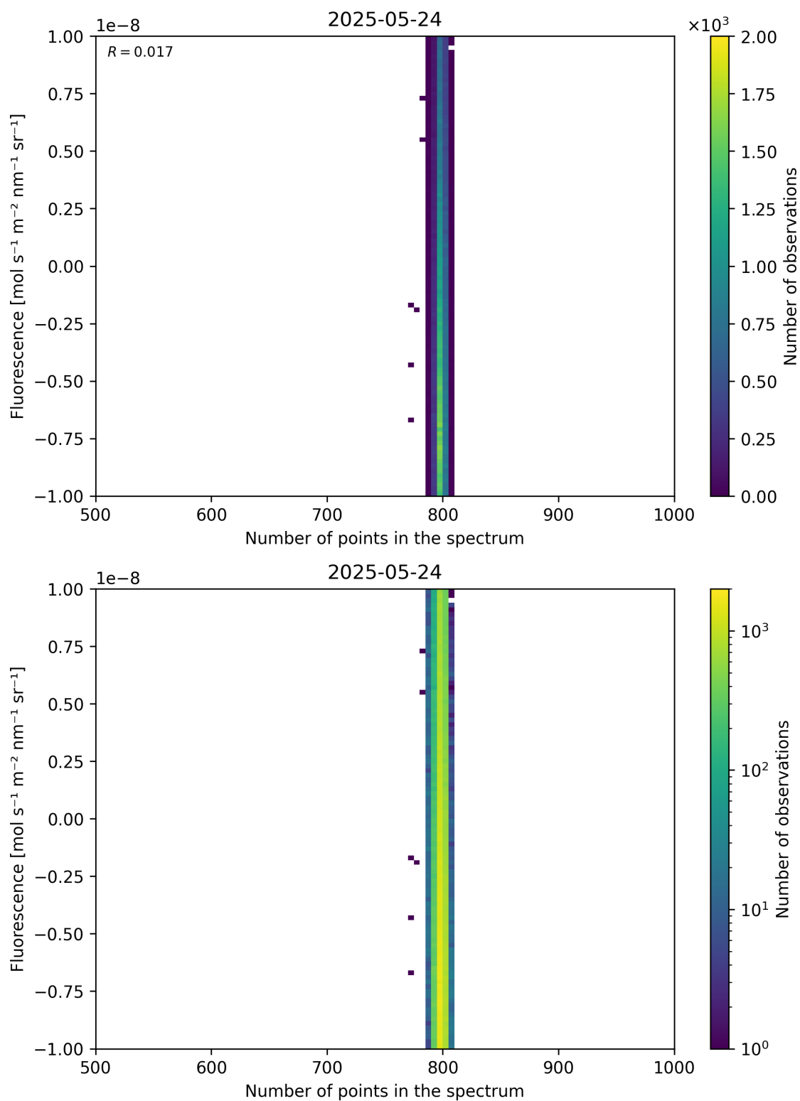
Figure 91: Scatter density plot of “Number of points in the spectrum” against “Fluorescence” for 2025-05-23 to 2025-05-25.
