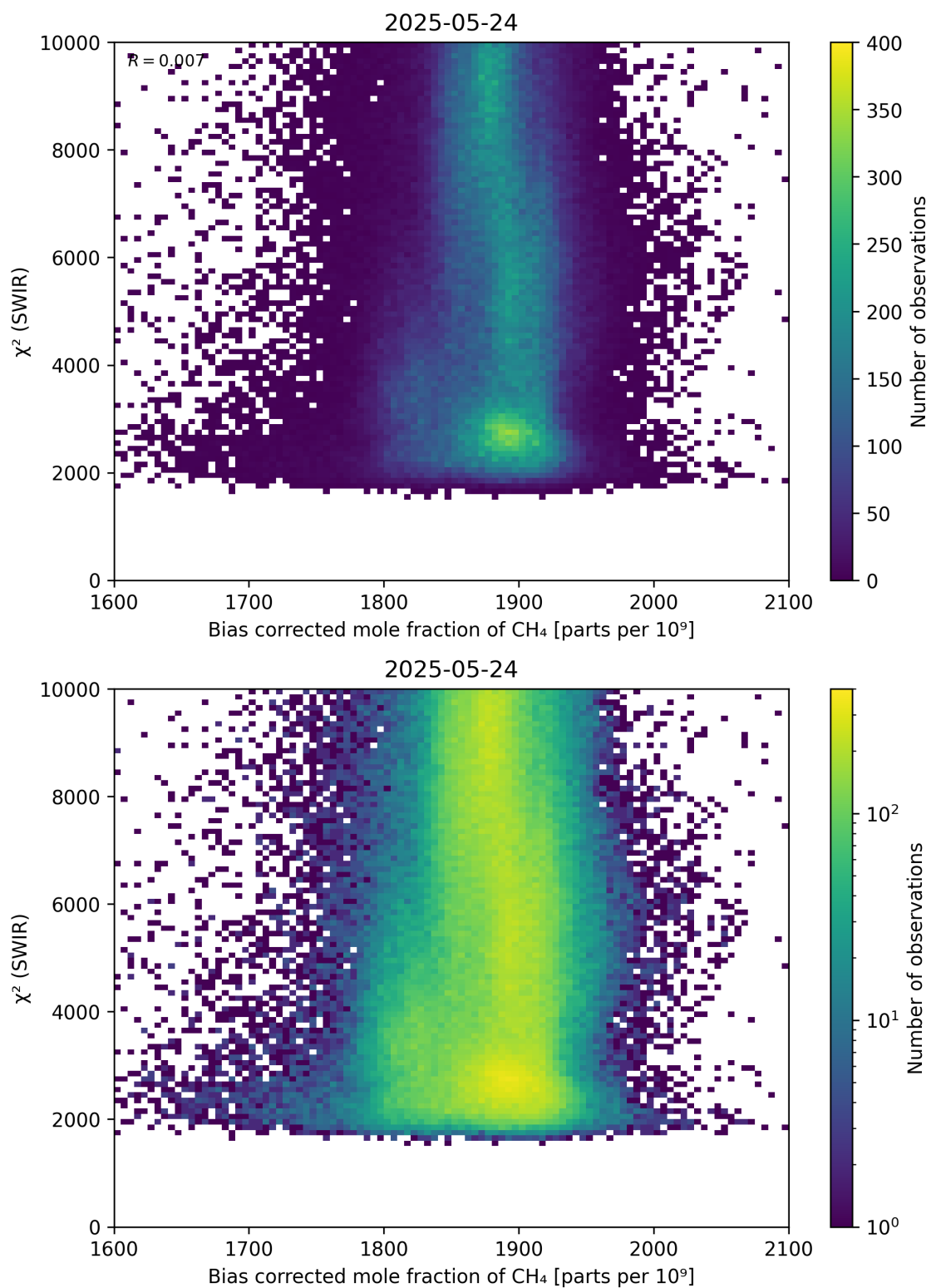
Figure 64: Scatter density plot of “Bias corrected mole fraction of \text{CH}_4 ” against “ \chi^2 (SWIR)” for 2025-05-23 to 2025-05-25.
