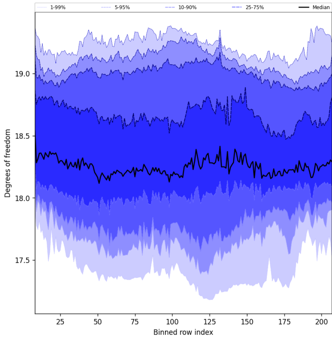
Figure 41: Along track statistics of “Degrees of freedom” for 2025-05-23 to 2025-05-25
