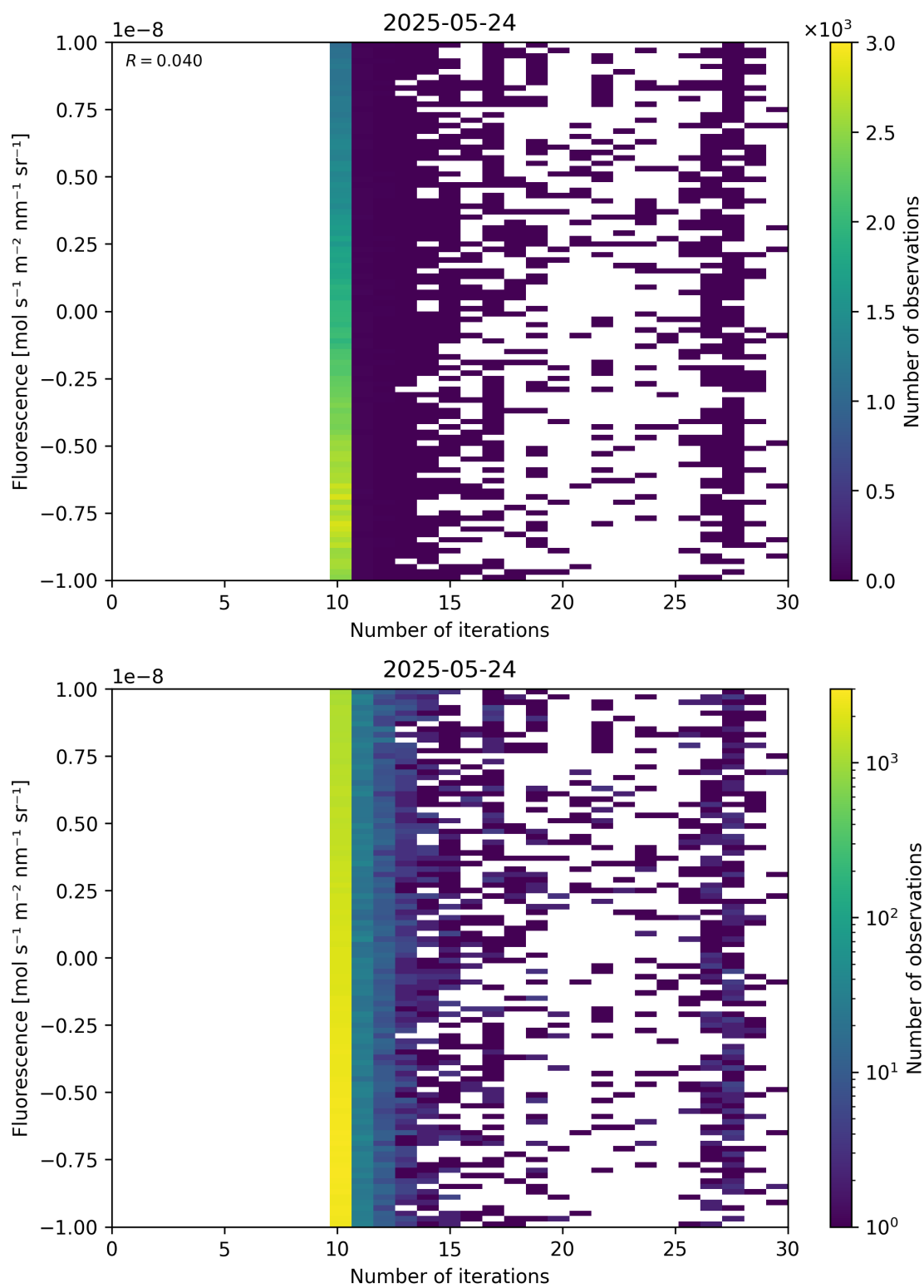
Figure 87: Scatter density plot of "Number of iterations" against "Fluorescence" for 2025-05-23 to 2025-05-25.
