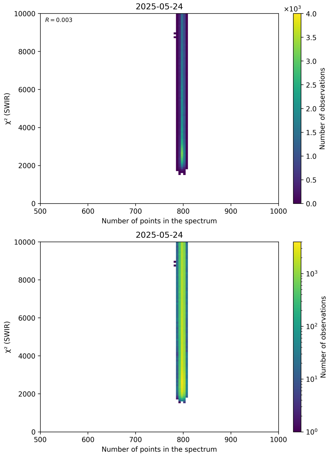
Figure 89: Scatter density plot of “Number of points in the spectrum” against “ \chi^2 (SWIR)” for 2025-05-23 to 2025-05-25.
