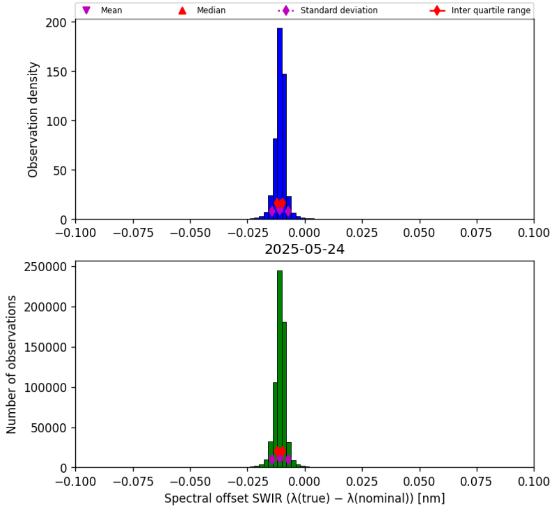
Figure 27: Histogram of “Spectral offset SWIR ( \lambda_{\text{true}} - \lambda_{\text{nominal}} )” for 2025-05-23 to 2025-05-25
