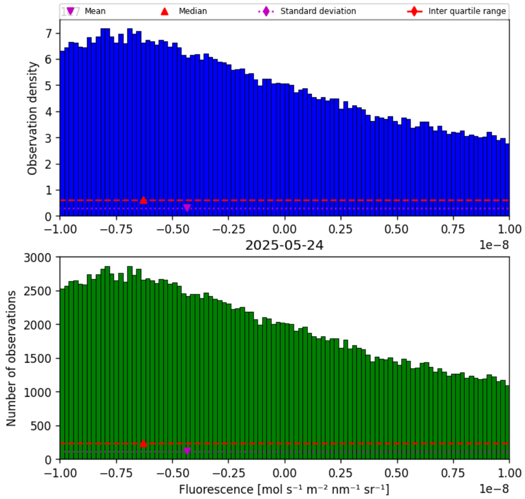
Figure 32: Histogram of “Fluorescence” for 2025-05-23 to 2025-05-25
