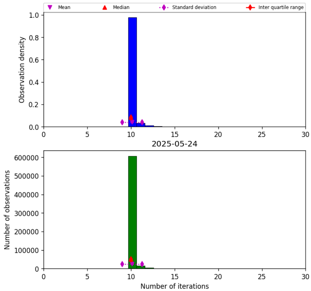
Figure 31: Histogram of “Number of iterations” for 2025-05-23 to 2025-05-25
