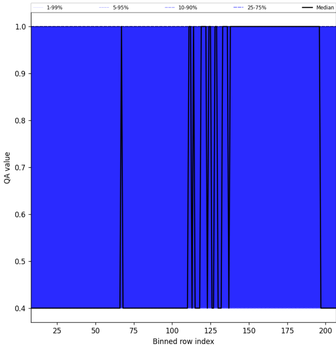
Figure 33: Along track statistics of “QA value” for 2025-05-23 to 2025-05-25
