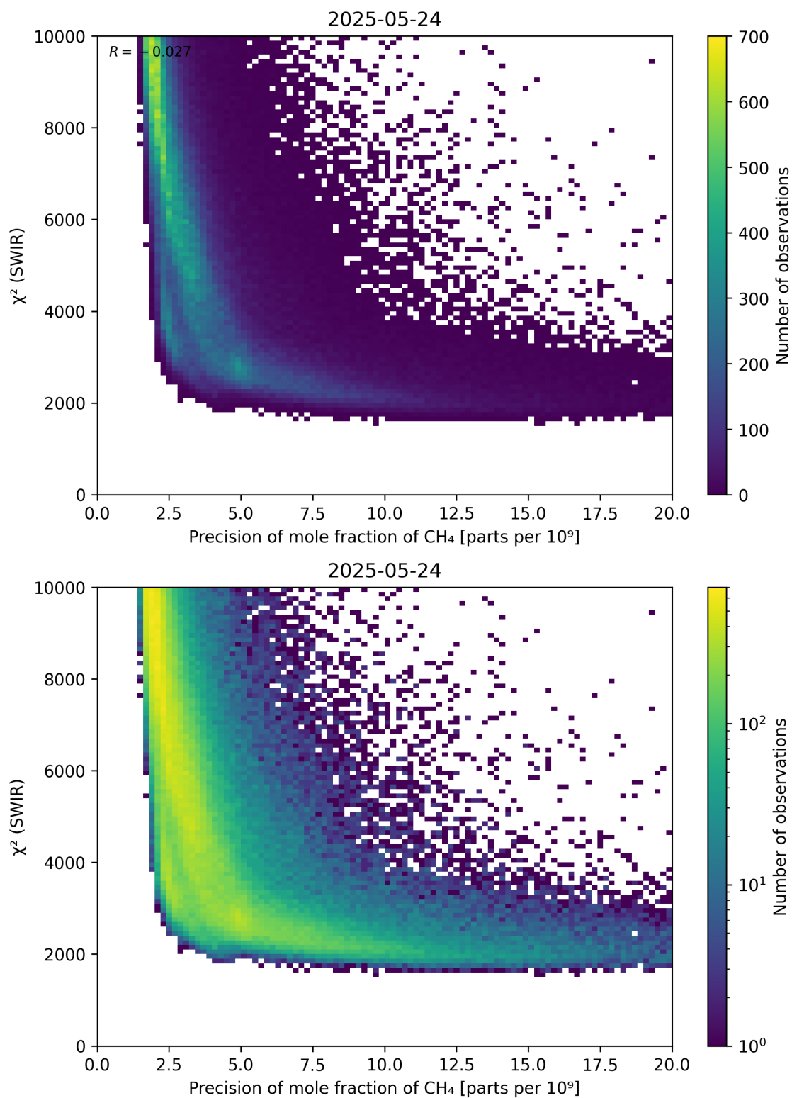
Figure 79: Scatter density plot of “Precision of mole fraction of \text{CH}_4 ” against “ \chi^2 (SWIR)” for 2025-05-23 to 2025-05-25.
