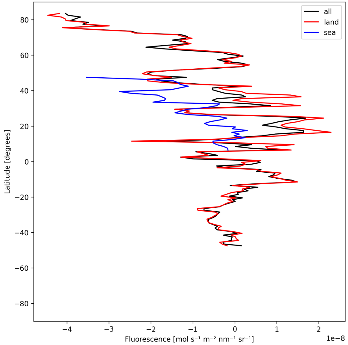
Figure 21: Zonal average of “Fluorescence” for 2025-05-23 to 2025-05-25.
