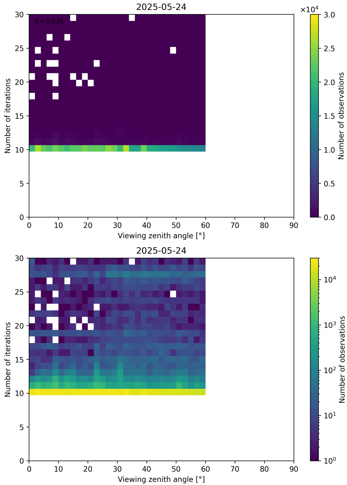
Figure 113: Scatter density plot of “Viewing zenith angle” against “Number of iterations” for 2025-05-23 to 2025-05-25.
