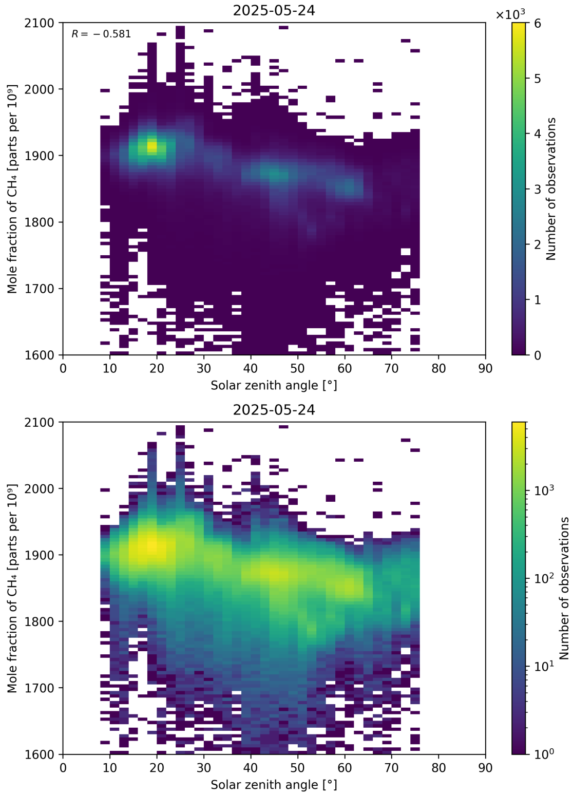
Figure 99: Scatter density plot of “Solar zenith angle” against “Mole fraction of \text{CH}_4 ” for 2025-05-23 to 2025-05-25.
