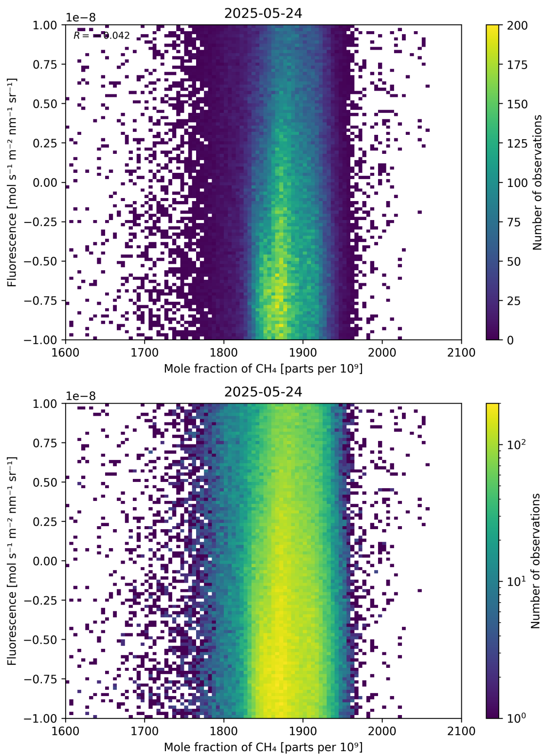
Figure 73: Scatter density plot of “Mole fraction of \text{CH}_4 ” against “Fluorescence” for 2025-05-23 to 2025-05-25.
