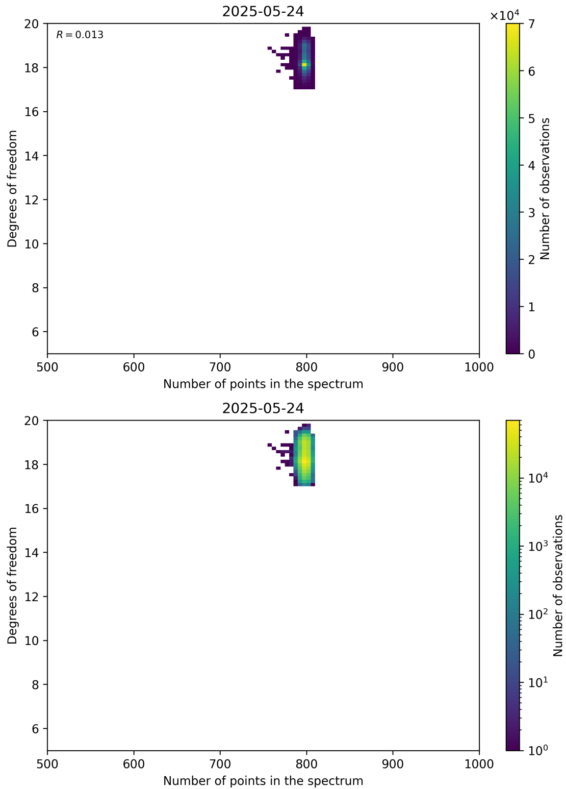
Figure 90: Scatter density plot of “Number of points in the spectrum” against “Degrees of freedom” for 2025-05-23 to 2025-05-25.
