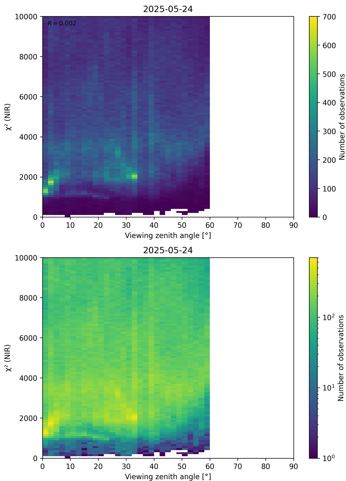
Figure 105: Scatter density plot of “Viewing zenith angle” against “ \chi^2 (NIR)” for 2025-05-23 to 2025-05-25.
