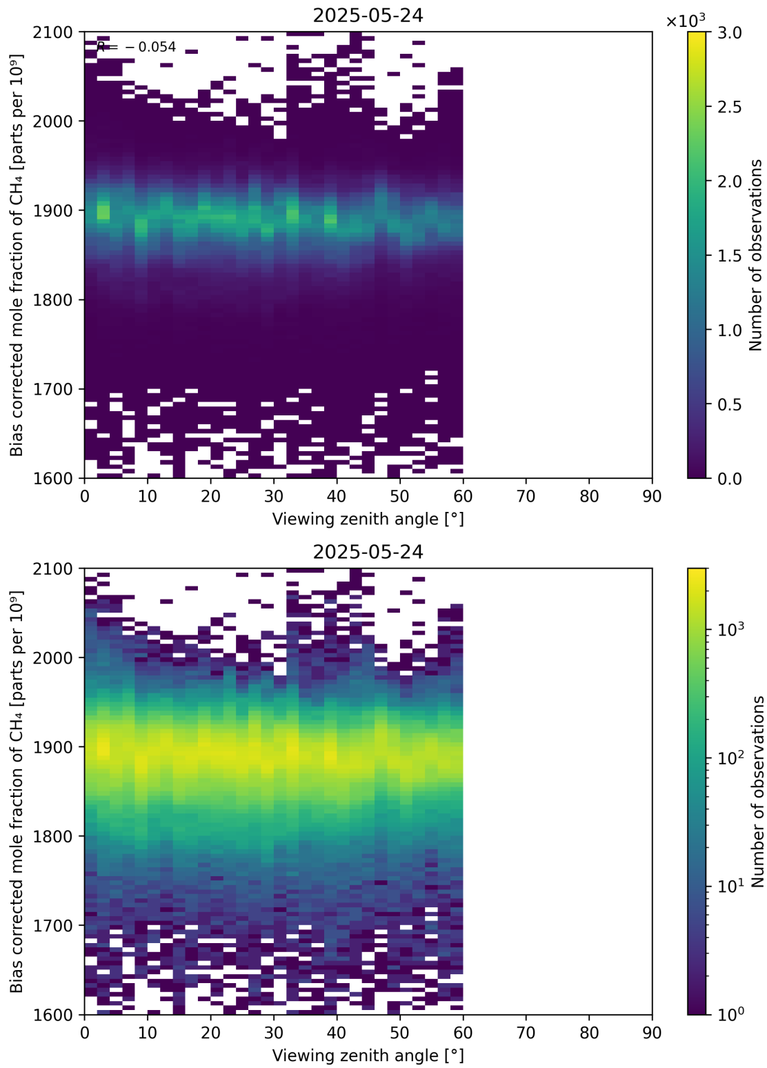
Figure 111: Scatter density plot of “Viewing zenith angle” against “Bias corrected mole fraction of CH 4 ” for 2025-05-23 to 2025-05-25.
