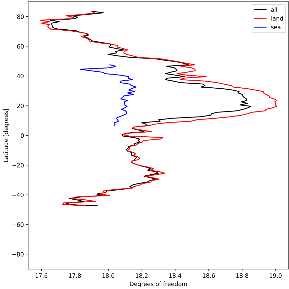
Figure 19: Zonal average of “Degrees of freedom” for 2025-05-23 to 2025-05-25.
