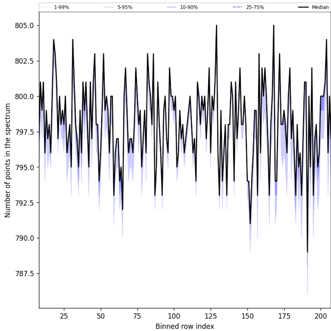
Figure 37: Along track statistics of “Number of points in the spectrum” for 2025-05-23 to 2025-05-25
