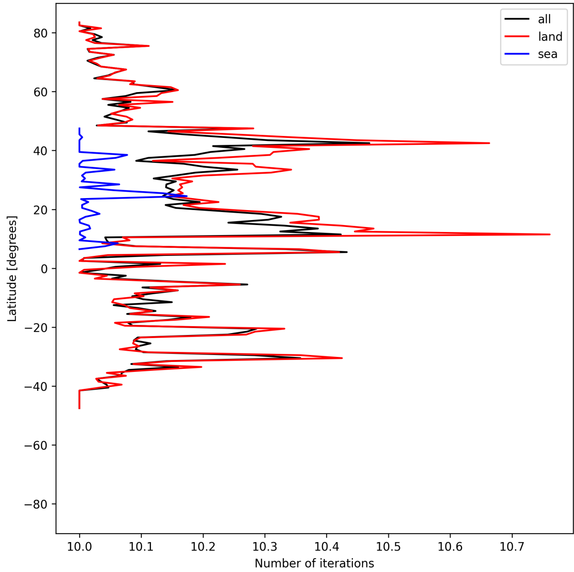
Figure 20: Zonal average of “Number of iterations” for 2025-05-23 to 2025-05-25.
