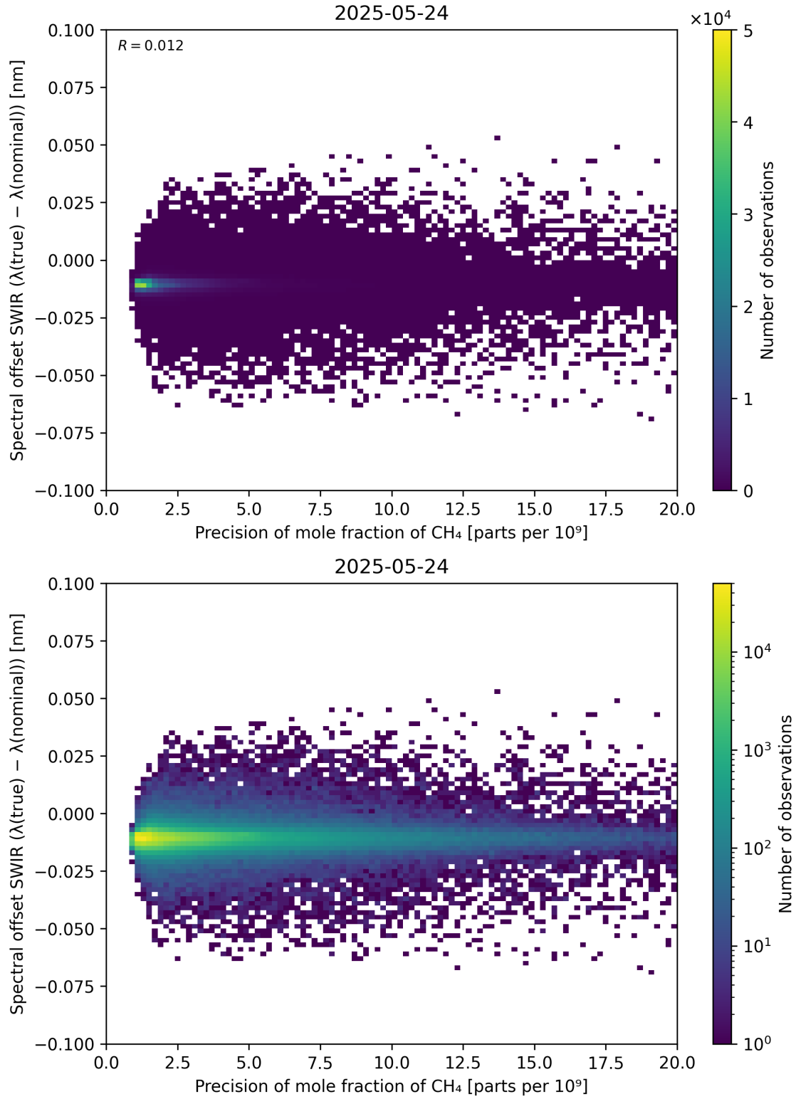
Figure 85: Scatter density plot of “Precision of mole fraction of \text{CH}_4 ” against “Spectral offset SWIR ( \lambda_{\text{true}} - \lambda_{\text{nominal}} )” for 2025-05-23 to 2025-05-25.
