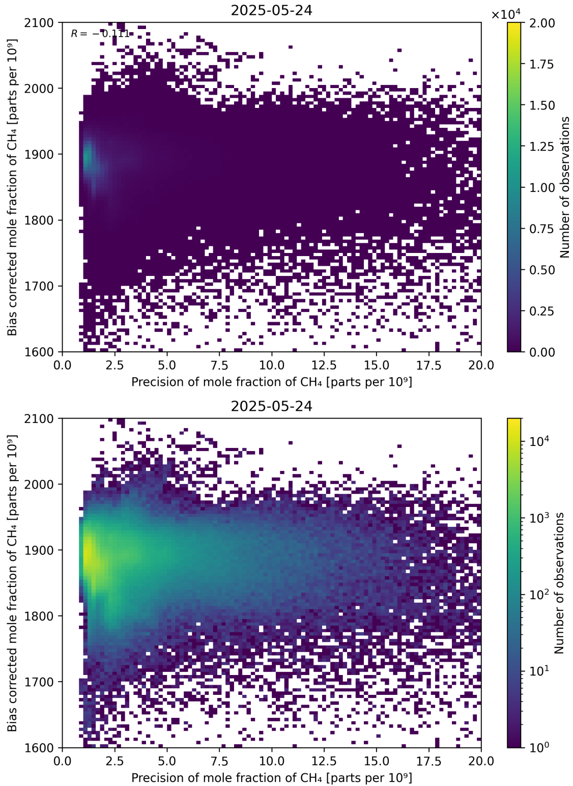
Figure 82: Scatter density plot of “Precision of mole fraction of CH 4 ” against “Bias corrected mole fraction of CH 4 ” for 2025-05-23 to 2025-05-25.
