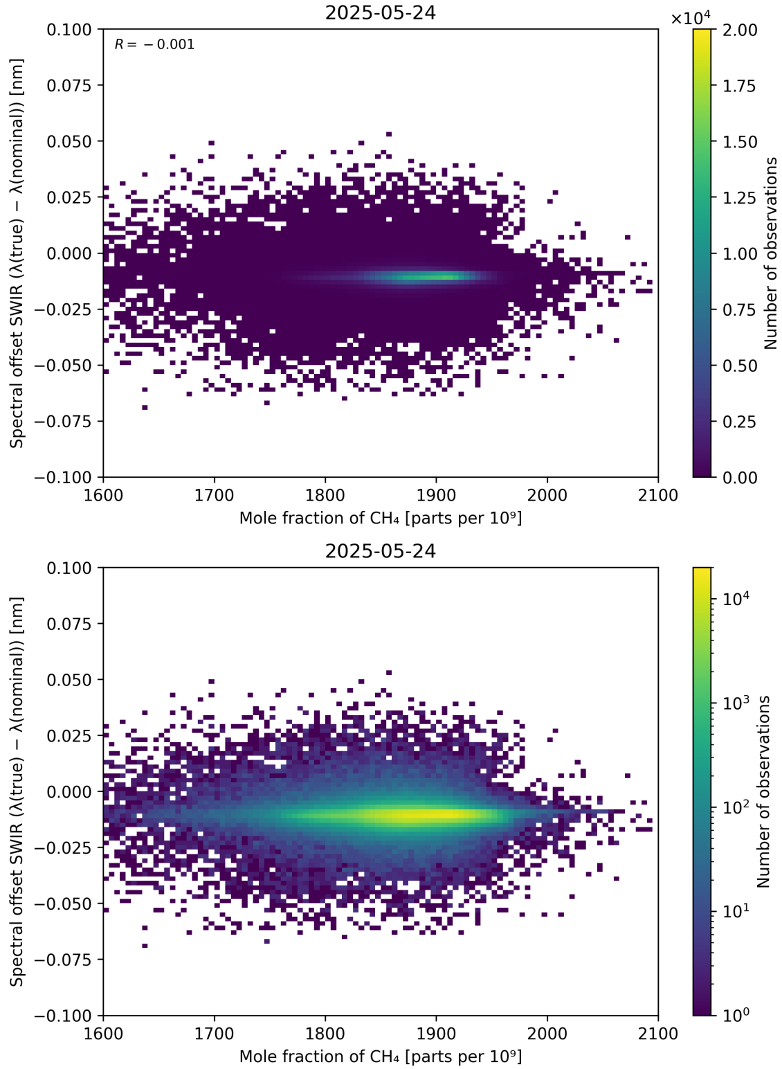
Figure 86: Scatter density plot of “Mole fraction of \text{CH}_4 ” against “Spectral offset SWIR ( \lambda_{\text{true}} - \lambda_{\text{nominal}} )” for 2025-05-23 to 2025-05-25.
