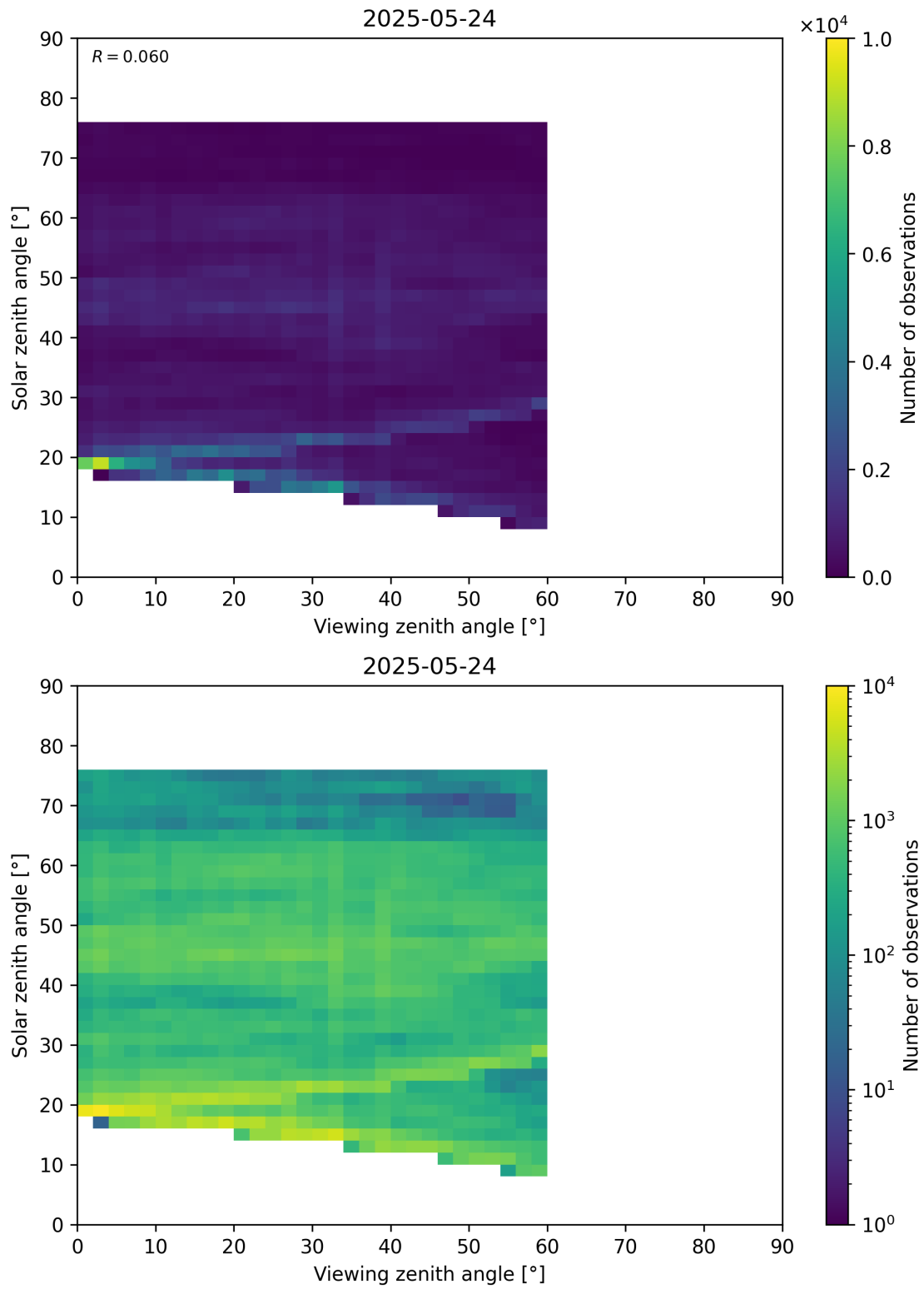
Figure 115: Scatter density plot of “Viewing zenith angle” against “Solar zenith angle” for 2025-05-23 to 2025-05-25.
