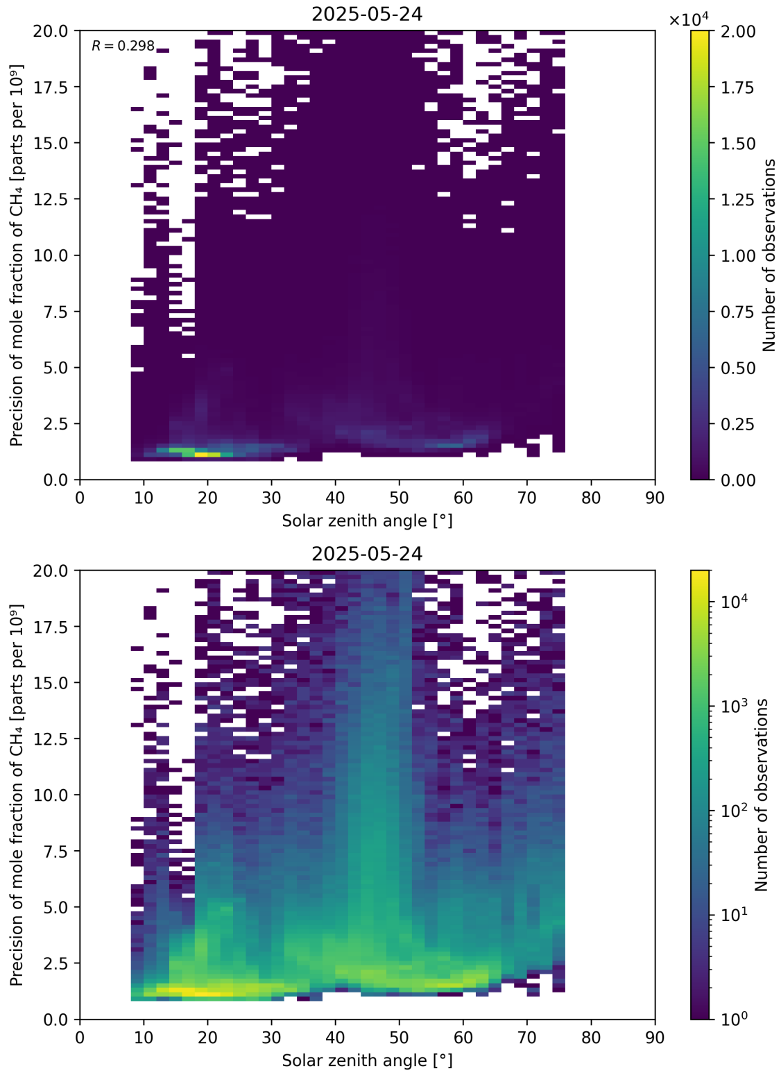
Figure 101: Scatter density plot of “Solar zenith angle” against “Precision of mole fraction of CH 4 ” for 2025-05-23 to 2025-05-25.
