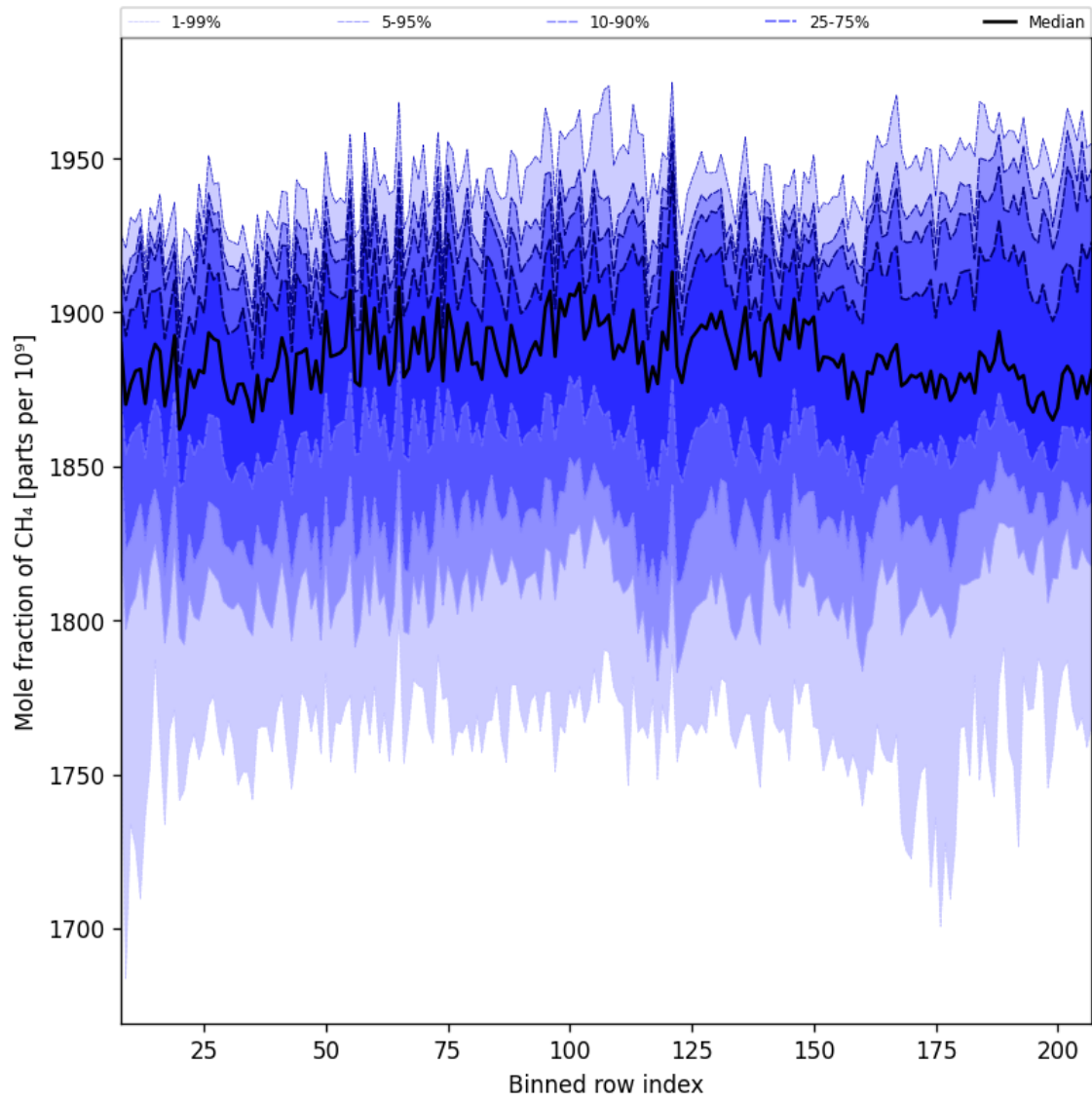
Figure 34: Along track statistics of “Mole fraction of CH 4 ” for 2025-05-23 to 2025-05-25
