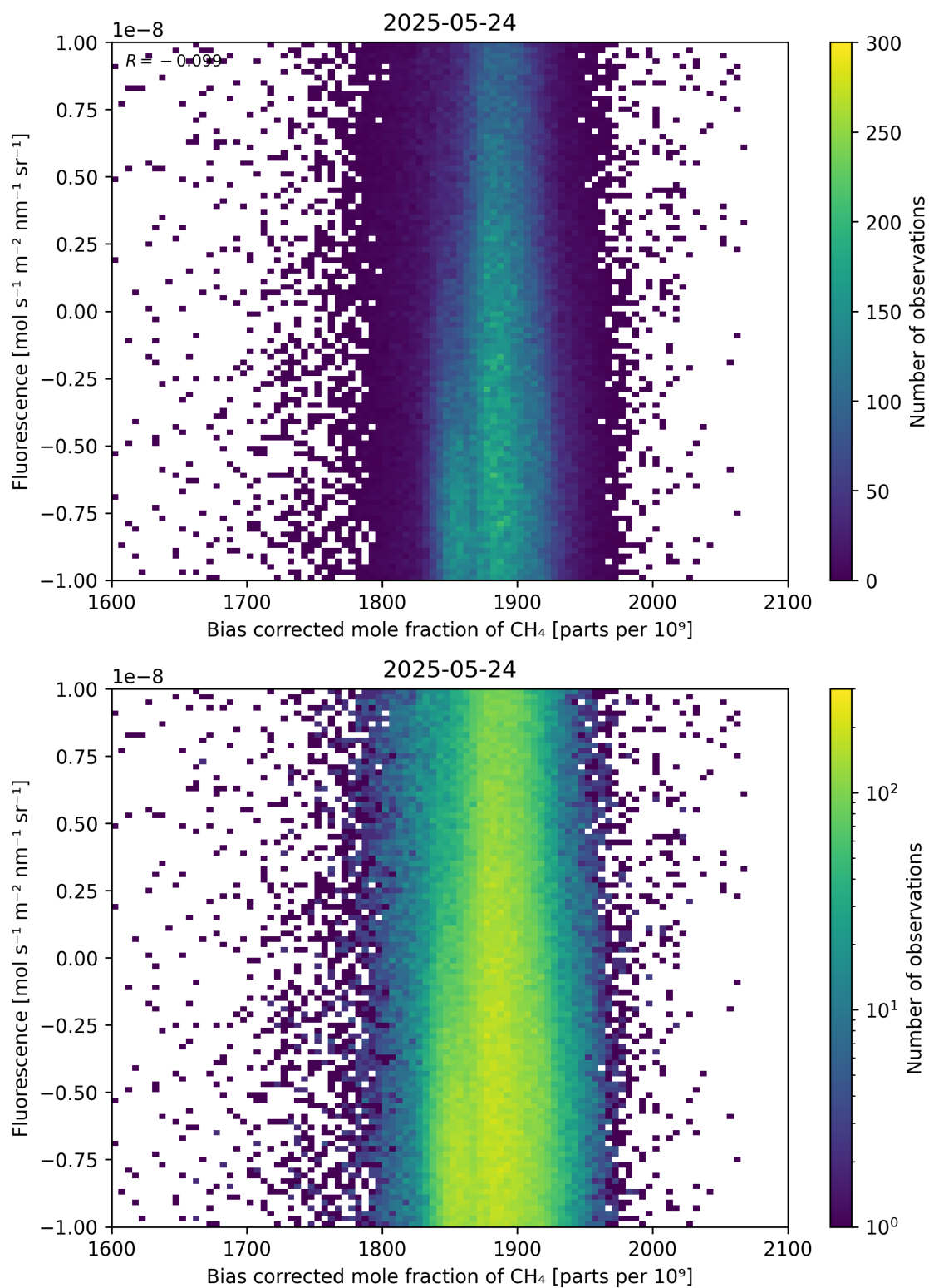
Figure 66: Scatter density plot of “Bias corrected mole fraction of \text{CH}_4 ” against “Fluorescence” for 2025-05-23 to 2025-05-25.
