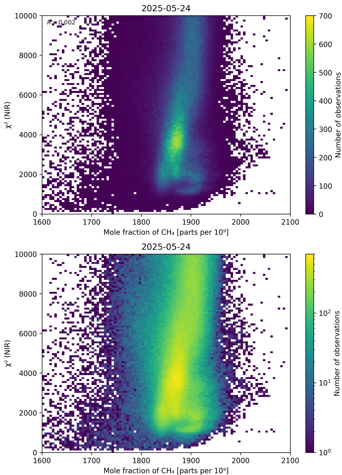
Figure 70: Scatter density plot of “Mole fraction of CH 4 ” against “ \chi^2 (NIR)” for 2025-05-23 to 2025-05-25.
