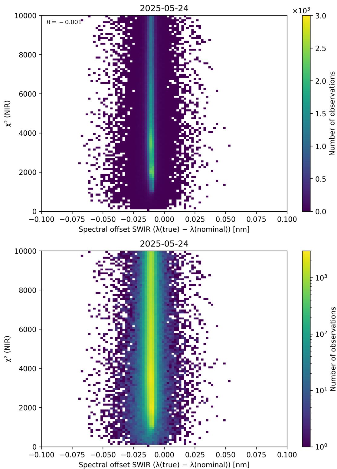
Figure 117: Scatter density plot of “Spectral offset SWIR ( \lambda_{\text{true}} - \lambda_{\text{nominal}} )” against “ \chi^2 (NIR)” for 2025-05-23 to 2025-05-25.
