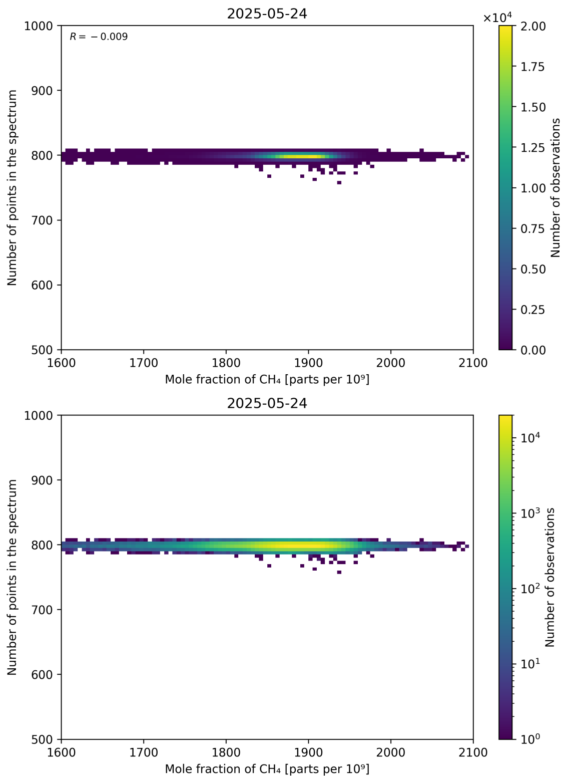
Figure 77: Scatter density plot of “Mole fraction of CH 4 ” against “Number of points in the spectrum” for 2025-05-23 to 2025-05-25.
