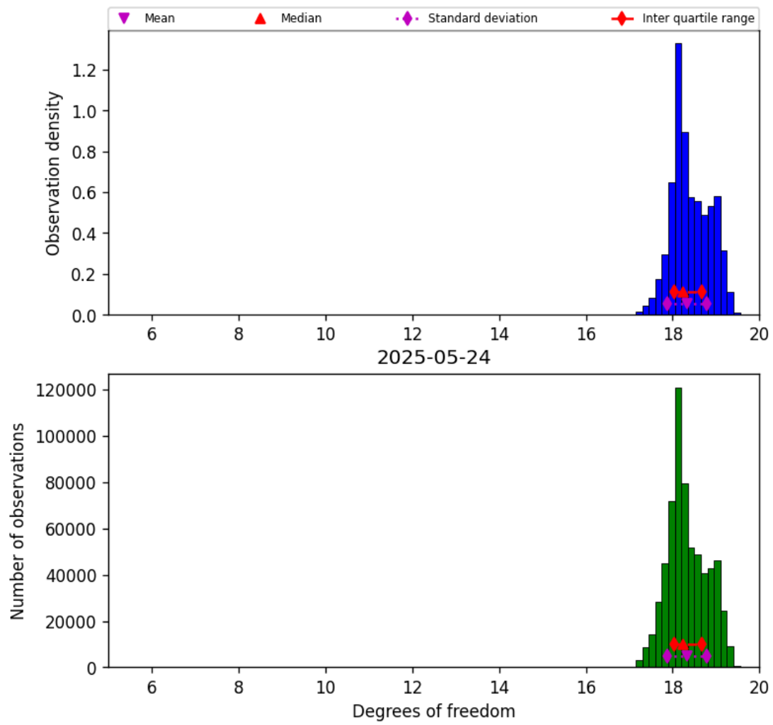
Figure 30: Histogram of “Degrees of freedom” for 2025-05-23 to 2025-05-25
