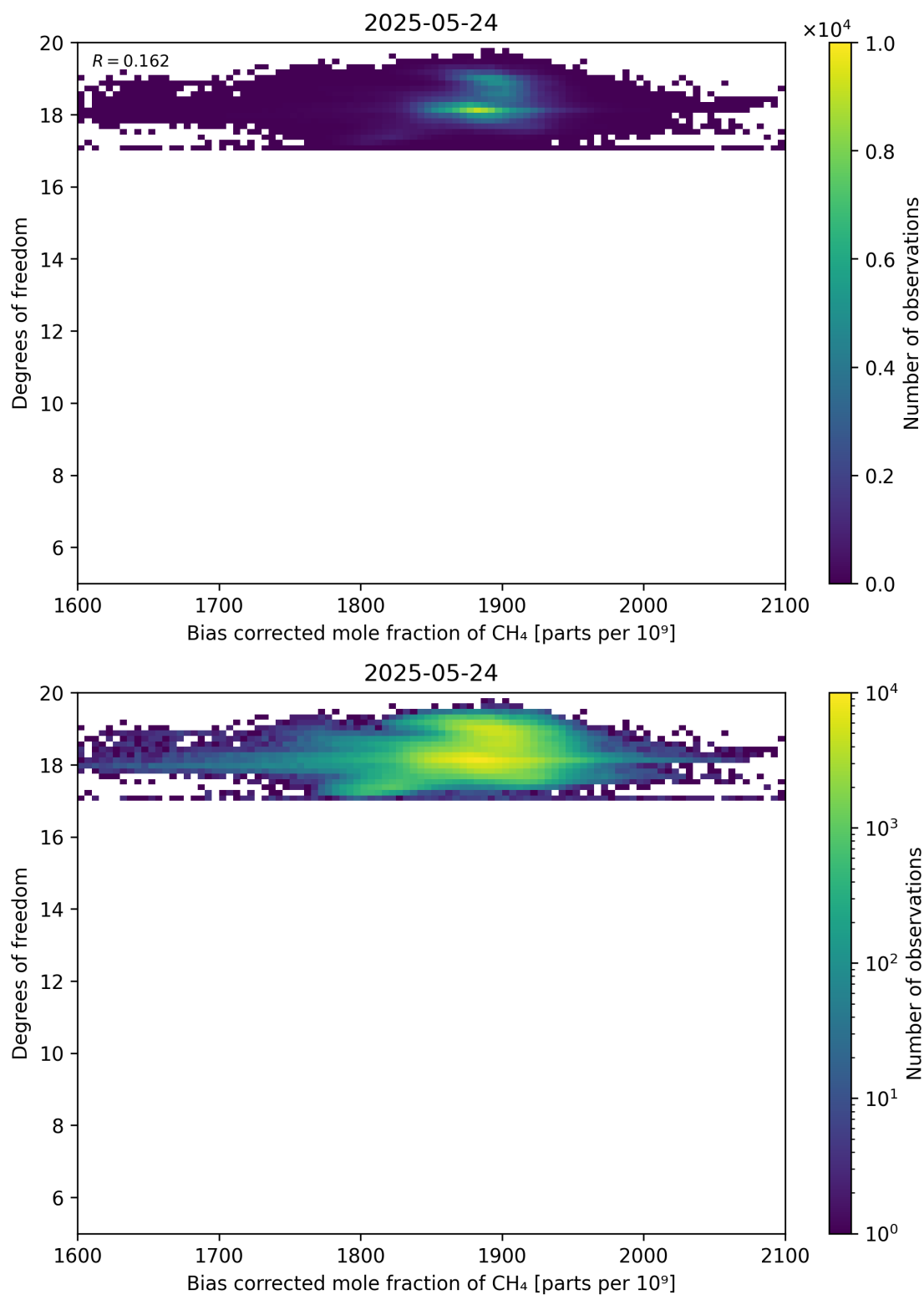
Figure 65: Scatter density plot of “Bias corrected mole fraction of CH 4 ” against “Degrees of freedom” for 2025-05-23 to 2025-05-25.
