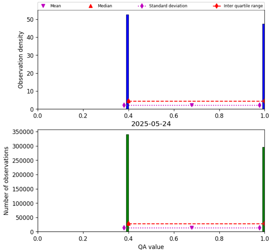
Figure 22: Histogram of “QA value” for 2025-05-23 to 2025-05-25
