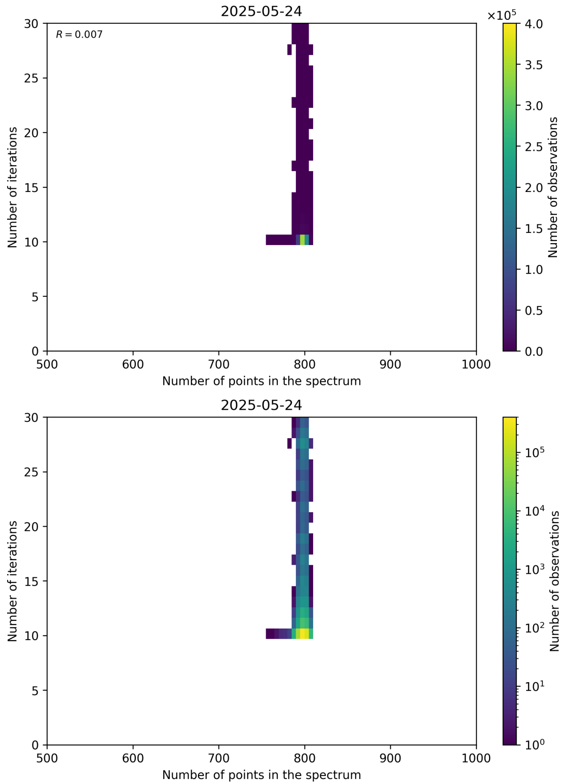
Figure 92: Scatter density plot of “Number of points in the spectrum” against “Number of iterations” for 2025-05-23 to 2025-05-25.
