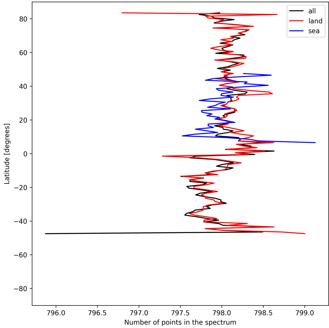
Figure 15: Zonal average of “Number of points in the spectrum” for 2025-05-23 to 2025-05-25.
