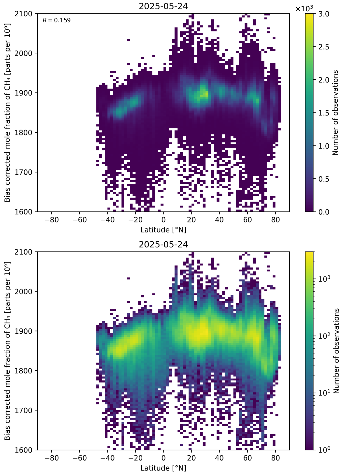
Figure 58: Scatter density plot of “Latitude” against “Bias corrected mole fraction of \text{CH}_4 ” for 2025-05-23 to 2025-05-25.
