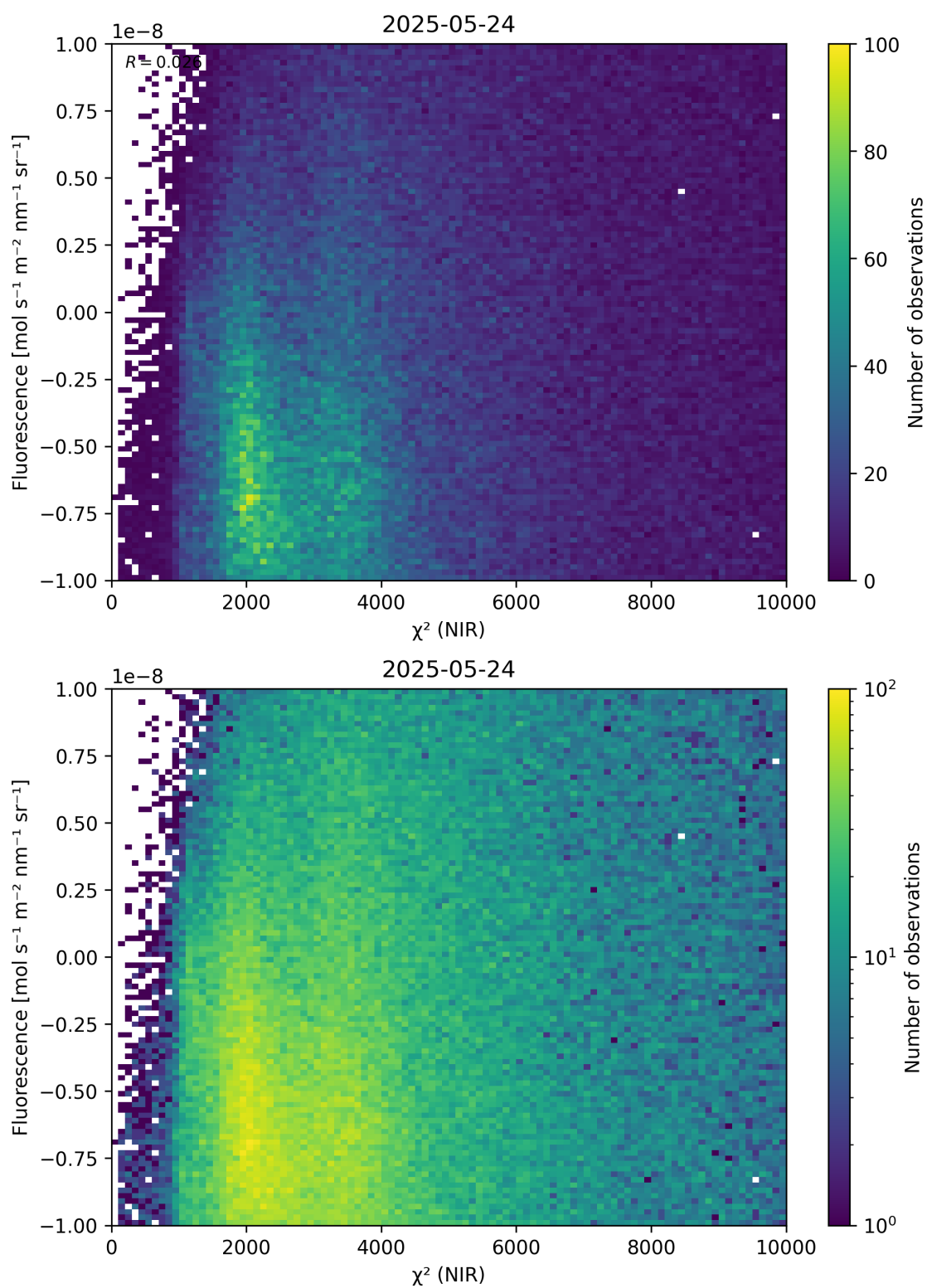
Figure 45: Scatter density plot of “ \chi^2 (NIR)” against “Fluorescence” for 2025-05-23 to 2025-05-25.
