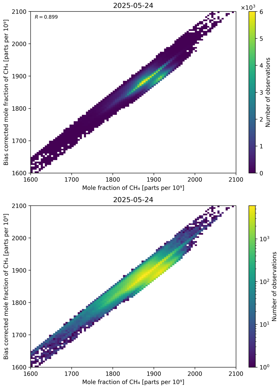
Figure 74: Scatter density plot of “Mole fraction of CH 4 ” against “Bias corrected mole fraction of CH 4 ” for 2025-05-23 to 2025-05-25.
