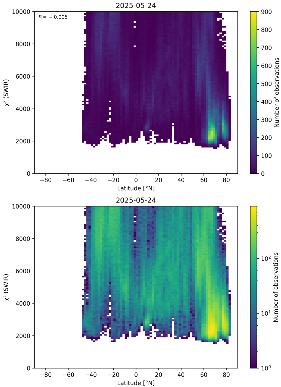
Figure 54: Scatter density plot of “Latitude” against “ \chi^2 (SWIR)” for 2025-05-23 to 2025-05-25.
