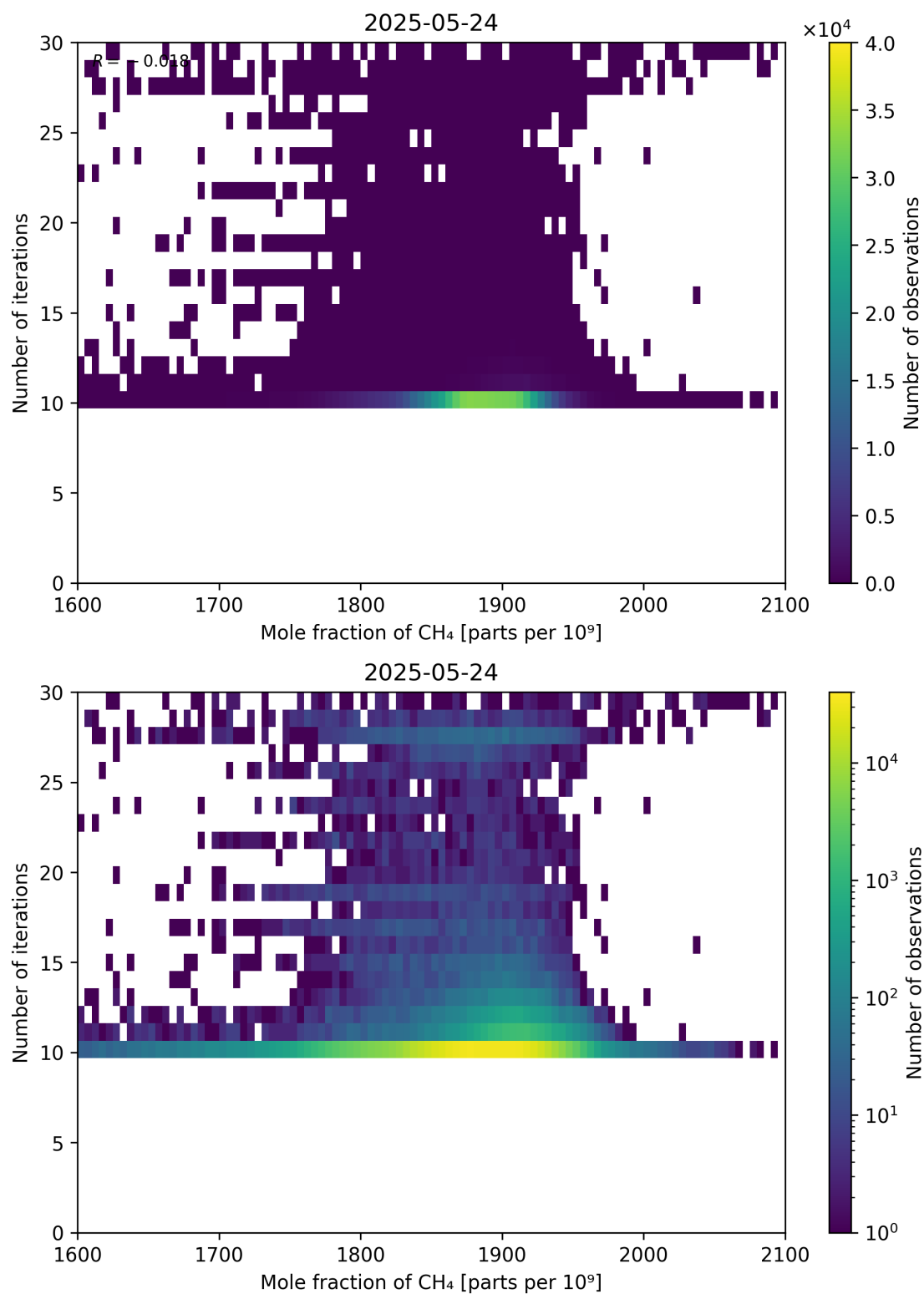
Figure 76: Scatter density plot of “Mole fraction of CH 4 ” against “Number of iterations” for 2025-05-23 to 2025-05-25.
