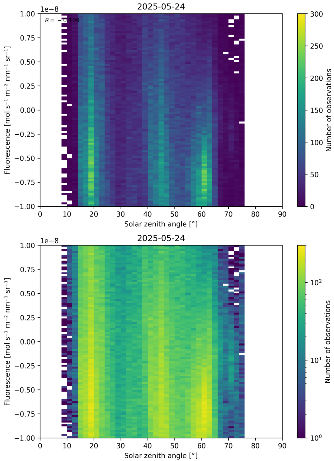
Figure 97: Scatter density plot of “Solar zenith angle” against “Fluorescence” for 2025-05-23 to 2025-05-25.
