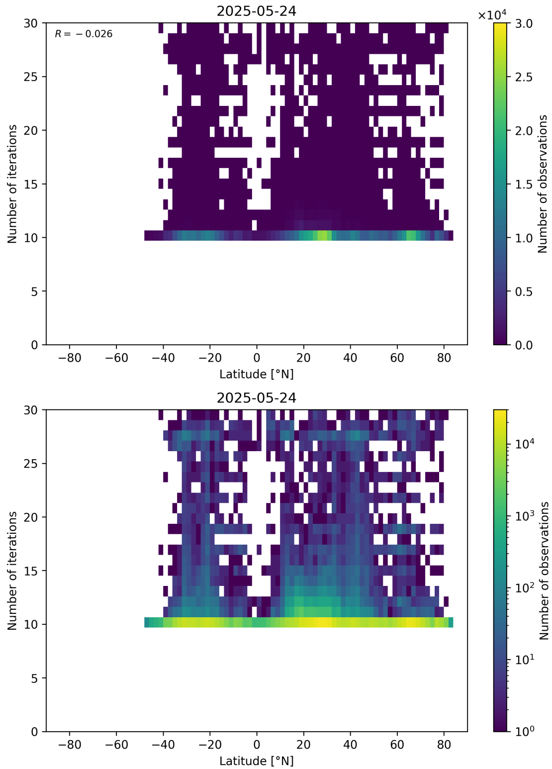
Figure 60: Scatter density plot of “Latitude” against “Number of iterations” for 2025-05-23 to 2025-05-25.
