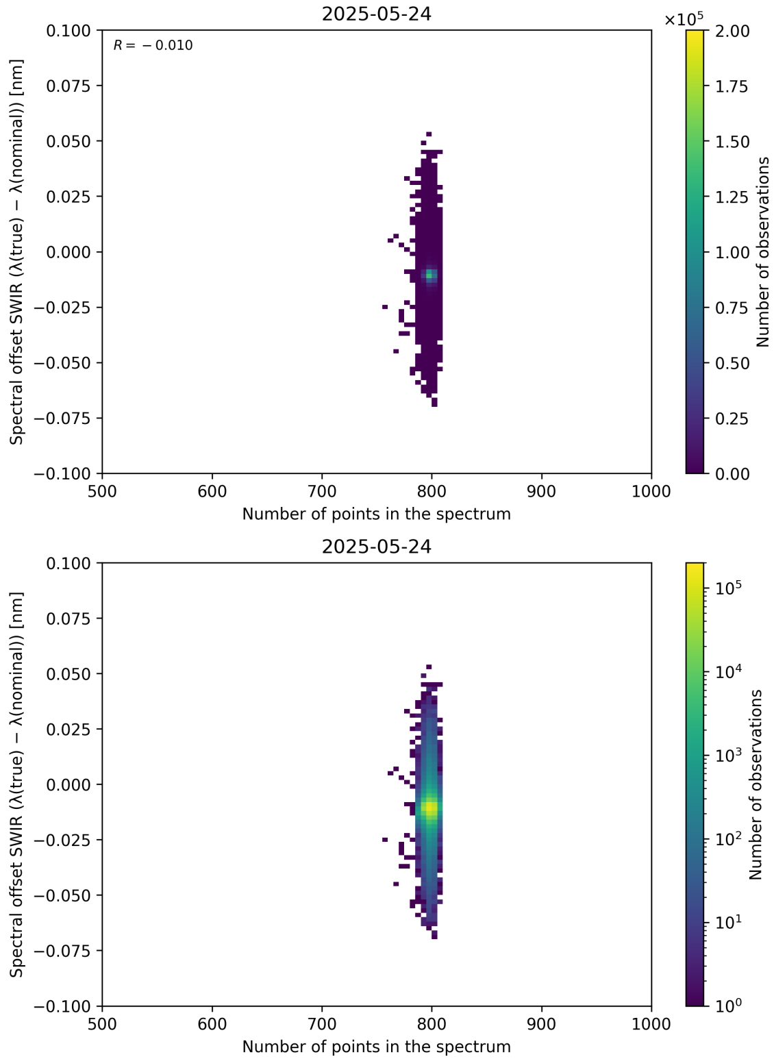
Figure 93: Scatter density plot of “Number of points in the spectrum” against “Spectral offset SWIR ( \lambda_{\text{true}} - \lambda_{\text{nominal}} )” for 2025-05-23 to 2025-05-25.
