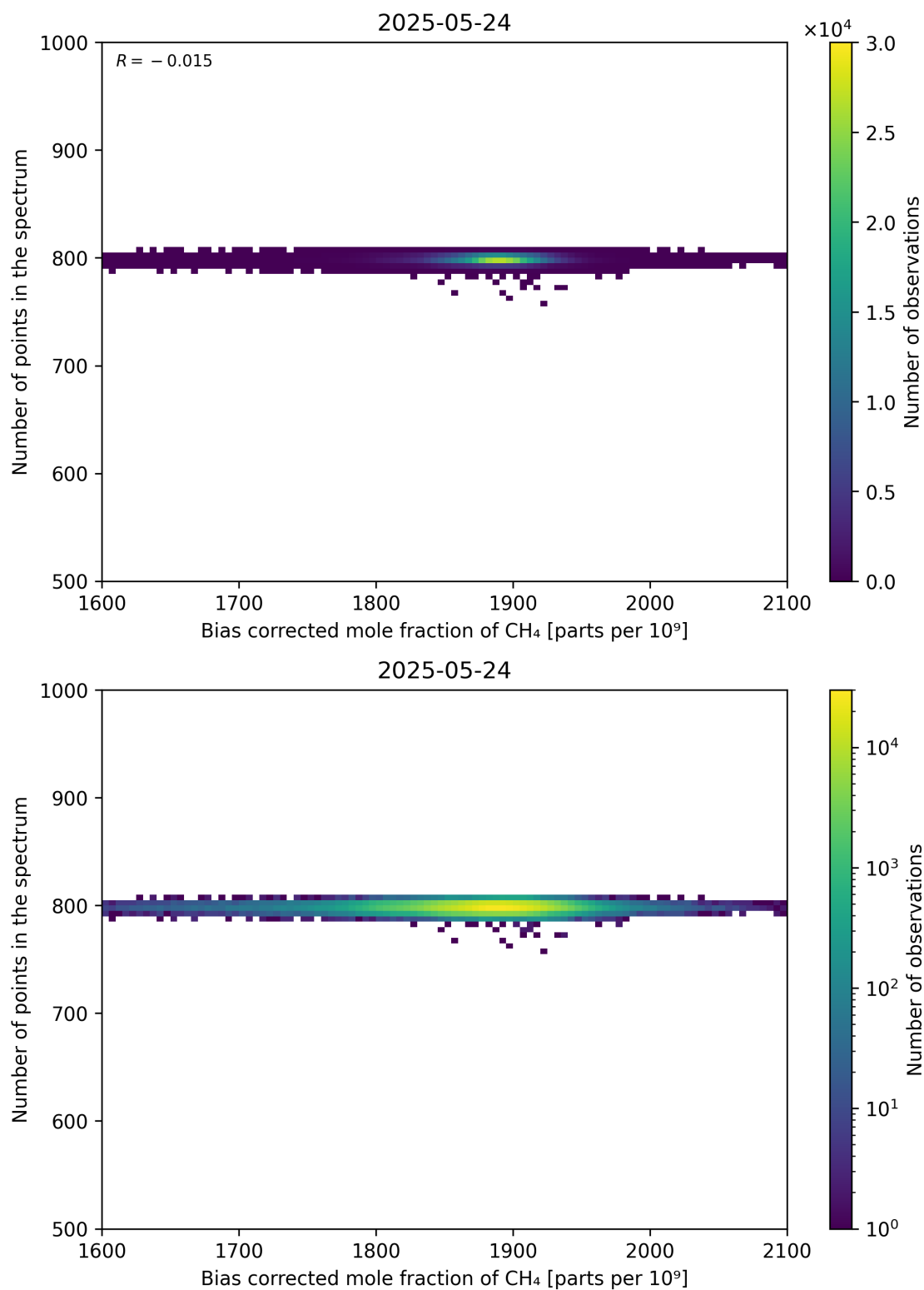
Figure 68: Scatter density plot of “Bias corrected mole fraction of CH 4 ” against “Number of points in the spectrum” for 2025-05-23 to 2025-05-25.
