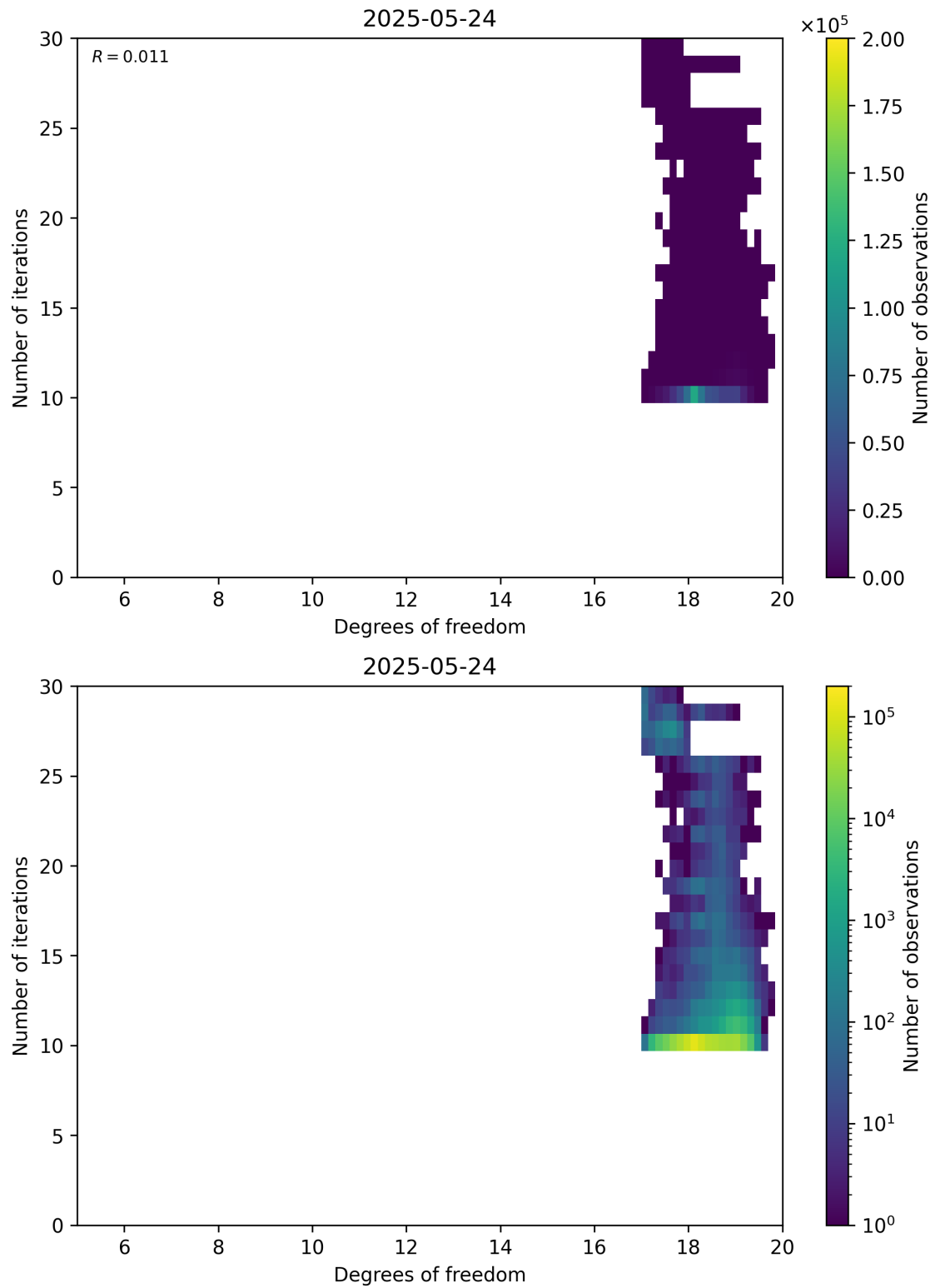
Figure 52: Scatter density plot of “Degrees of freedom” against “Number of iterations” for 2025-05-23 to 2025-05-25.
