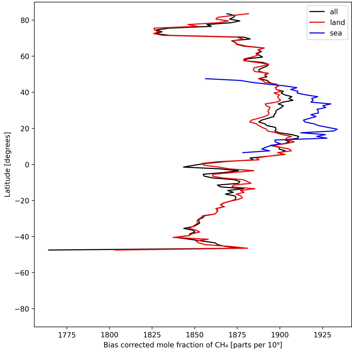
Figure 14: Zonal average of “Bias corrected mole fraction of CH 4 ” for 2025-05-23 to 2025-05-25.
