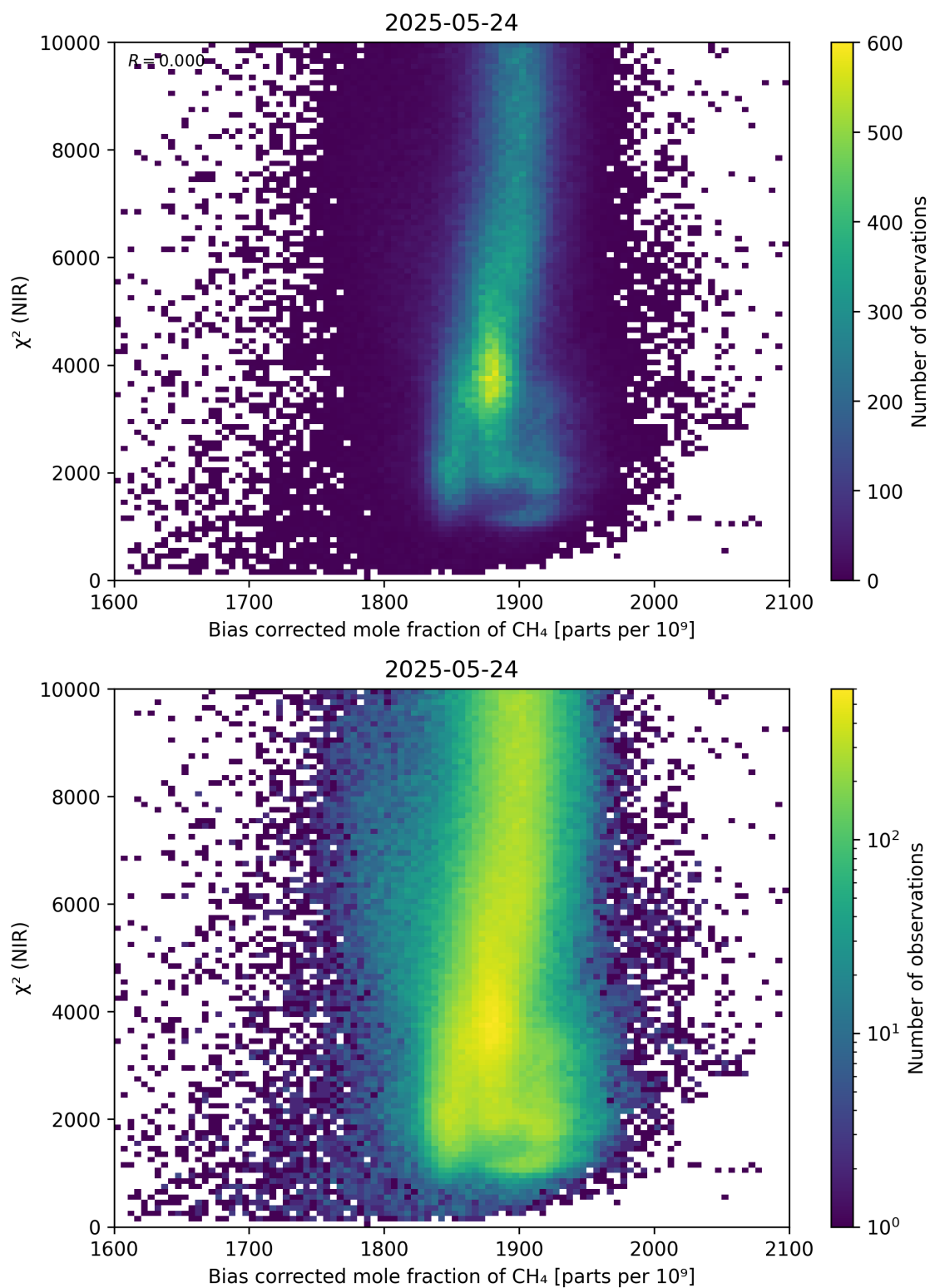
Figure 63: Scatter density plot of “Bias corrected mole fraction of \text{CH}_4 ” against “ \chi^2 (NIR)” for 2025-05-23 to 2025-05-25.
