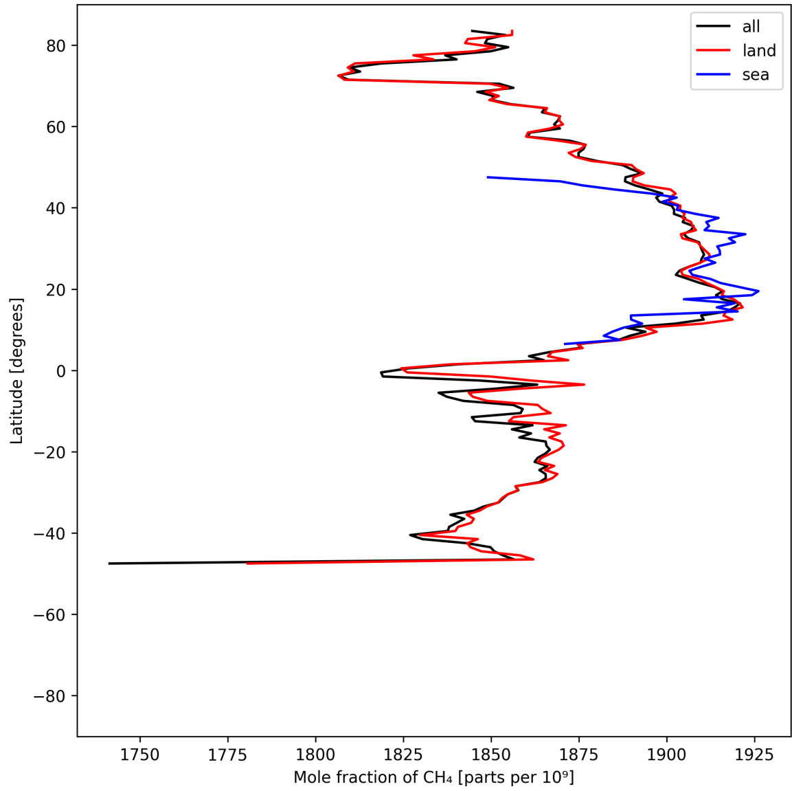
Figure 12: Zonal average of “Mole fraction of CH 4 ” for 2025-05-23 to 2025-05-25.
