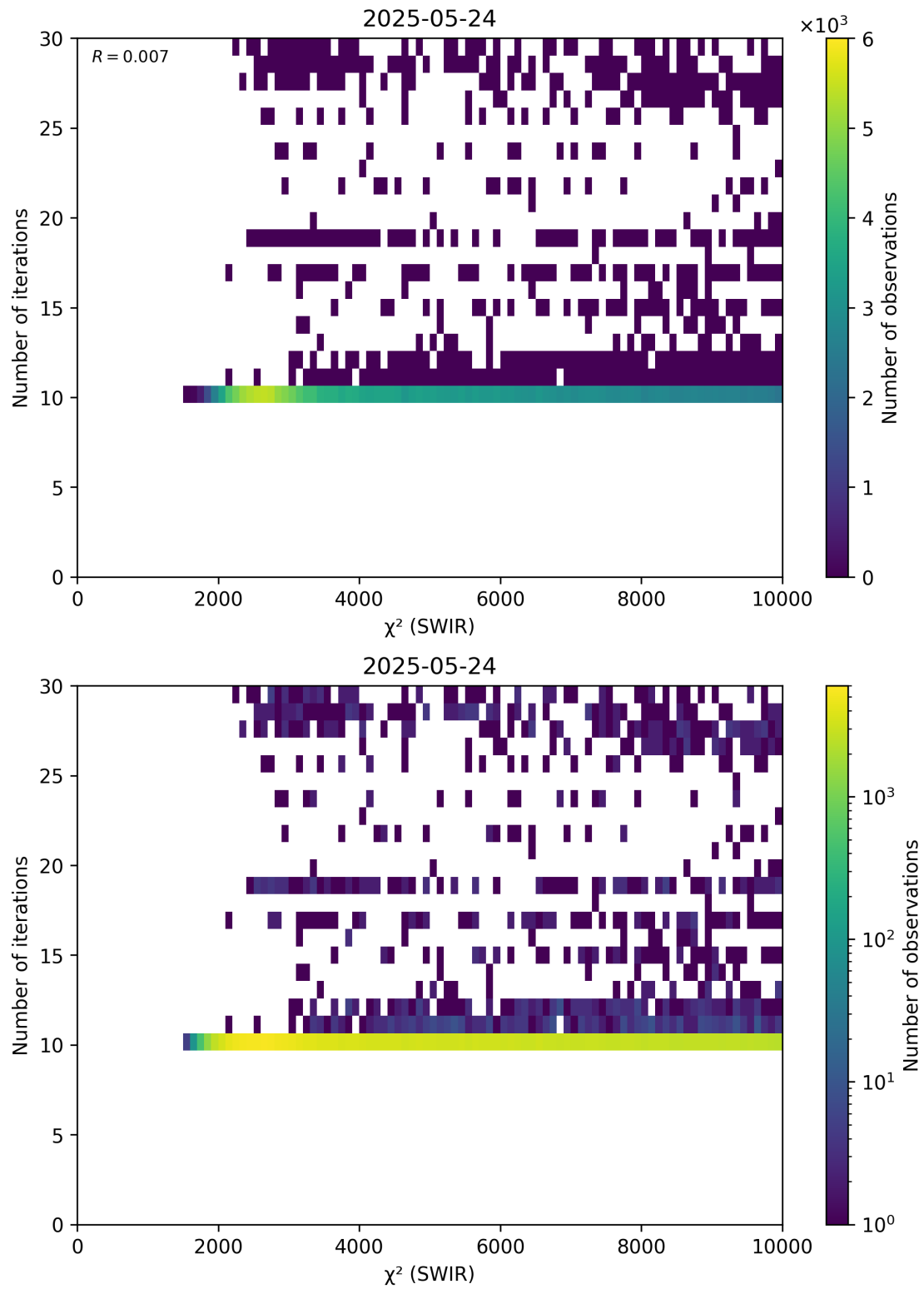
Figure 50: Scatter density plot of “ \chi^2 (SWIR)” against “Number of iterations” for 2025-05-23 to 2025-05-25.
