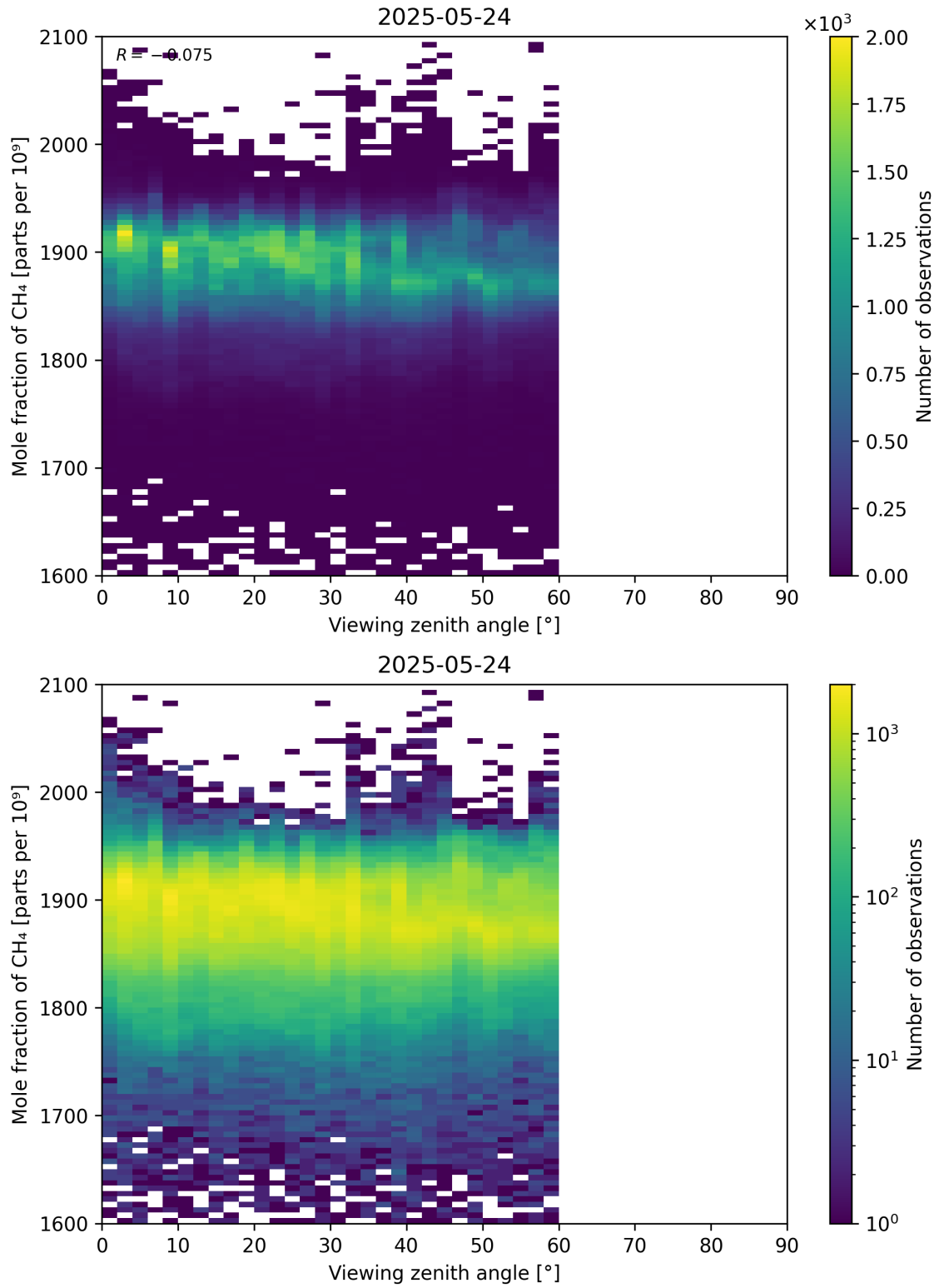
Figure 110: Scatter density plot of “Viewing zenith angle” against “Mole fraction of CH 4 ” for 2025-05-23 to 2025-05-25.
