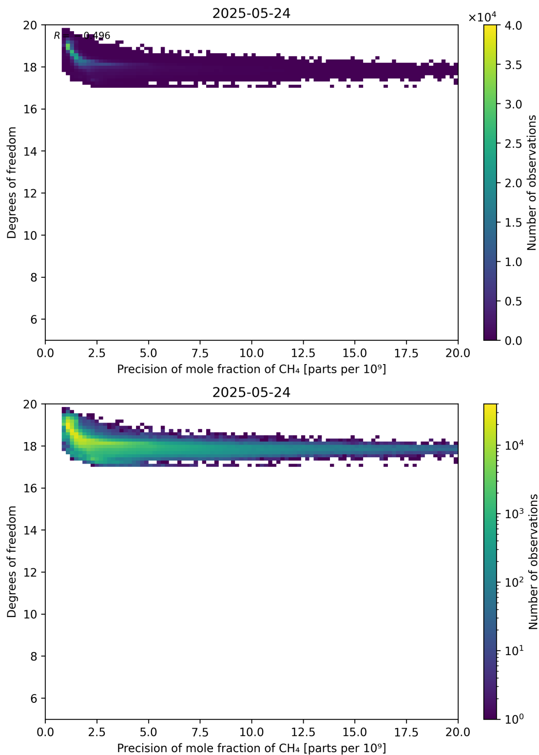
Figure 80: Scatter density plot of “Precision of mole fraction of CH 4 ” against “Degrees of freedom” for 2025-05-23 to 2025-05-25.
