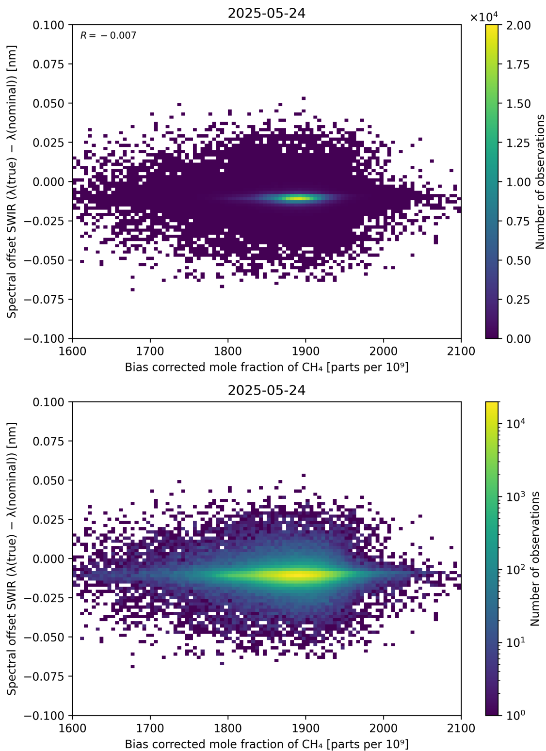
Figure 69: Scatter density plot of “Bias corrected mole fraction of \text{CH}_4 ” against “Spectral offset SWIR ( \lambda_{\text{true}} - \lambda_{\text{nominal}} )” for 2025-05-23 to 2025-05-25.
