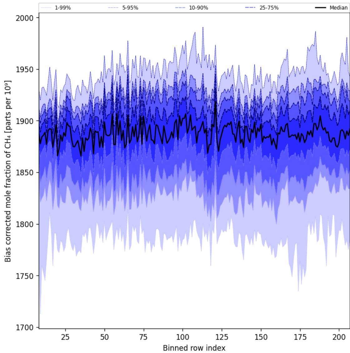
Figure 36: Along track statistics of “Bias corrected mole fraction of CH 4 ” for 2025-05-23 to 2025-05-25
