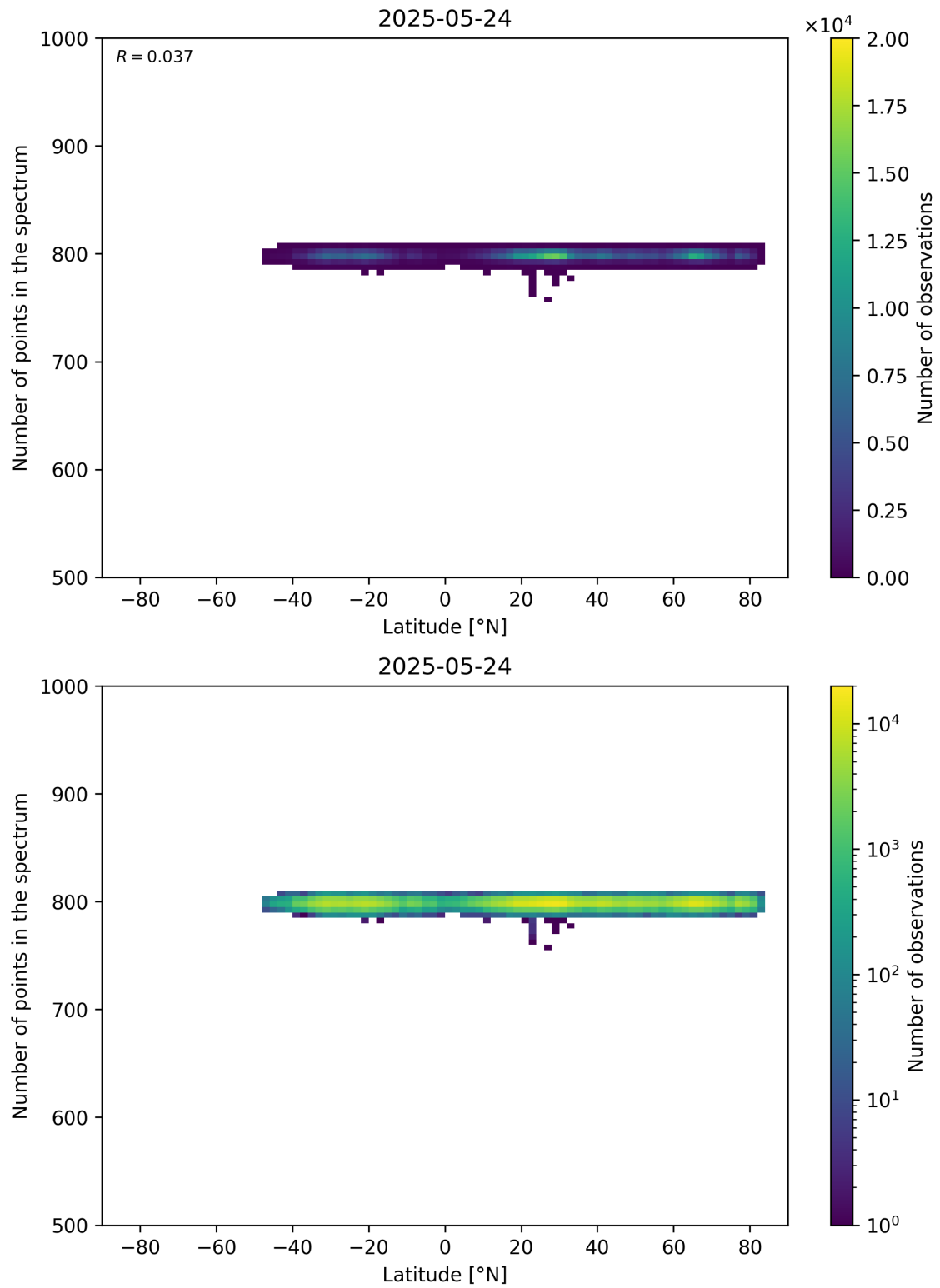
Figure 61: Scatter density plot of “Latitude” against “Number of points in the spectrum” for 2025-05-23 to 2025-05-25.
