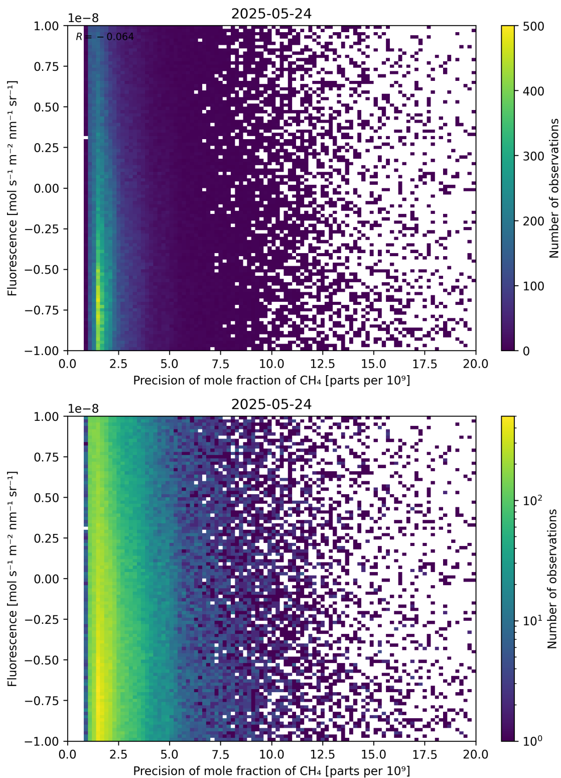
Figure 81: Scatter density plot of “Precision of mole fraction of \text{CH}_4 ” against “Fluorescence” for 2025-05-23 to 2025-05-25.
