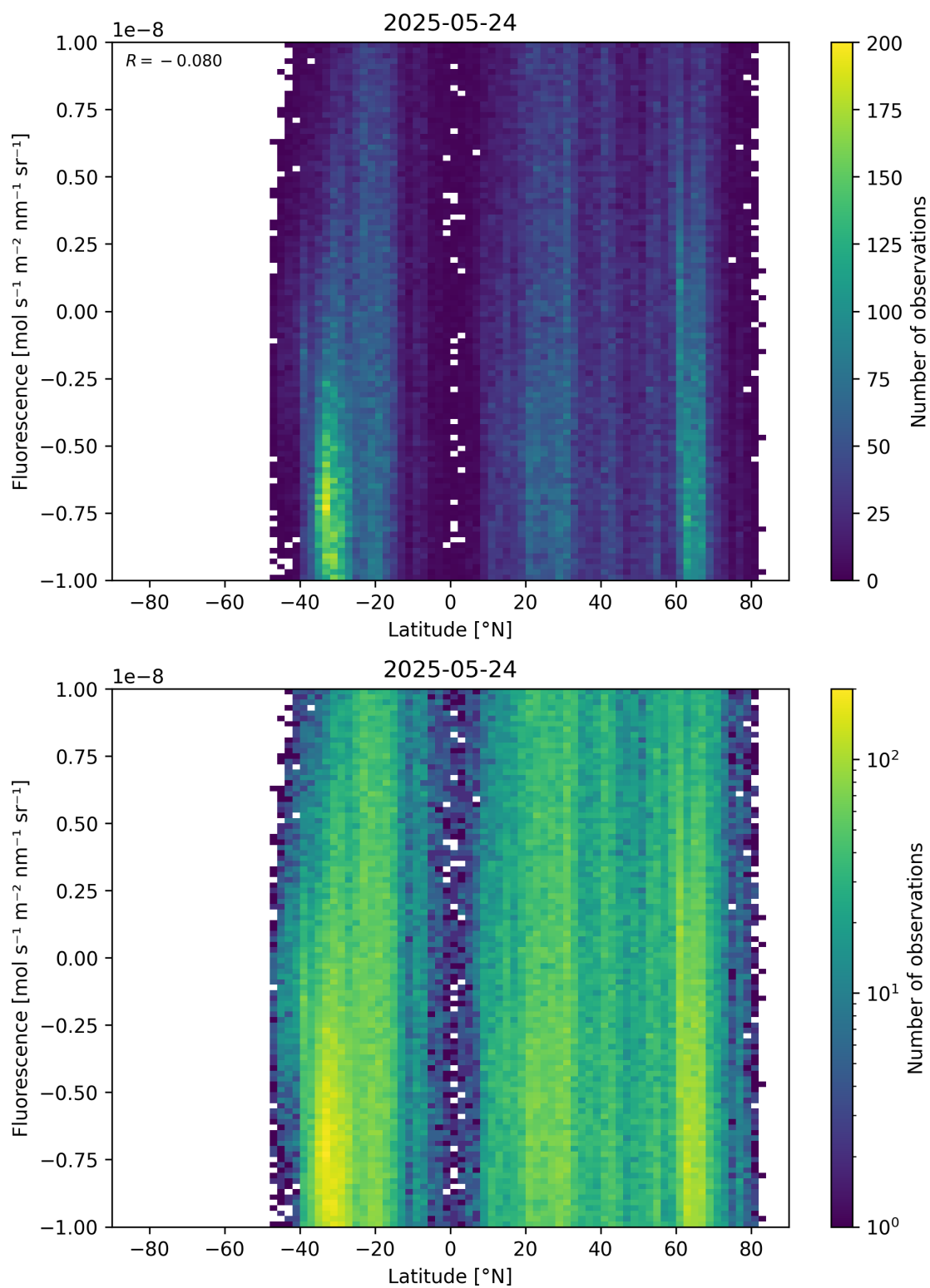
Figure 56: Scatter density plot of “Latitude” against “Fluorescence” for 2025-05-23 to 2025-05-25.
