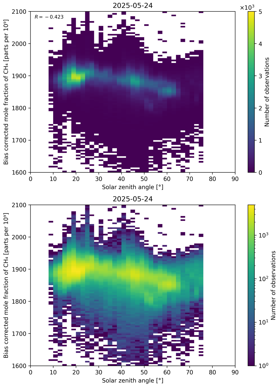
Figure 100: Scatter density plot of “Solar zenith angle” against “Bias corrected mole fraction of CH 4 ” for 2025-05-23 to 2025-05-25.
