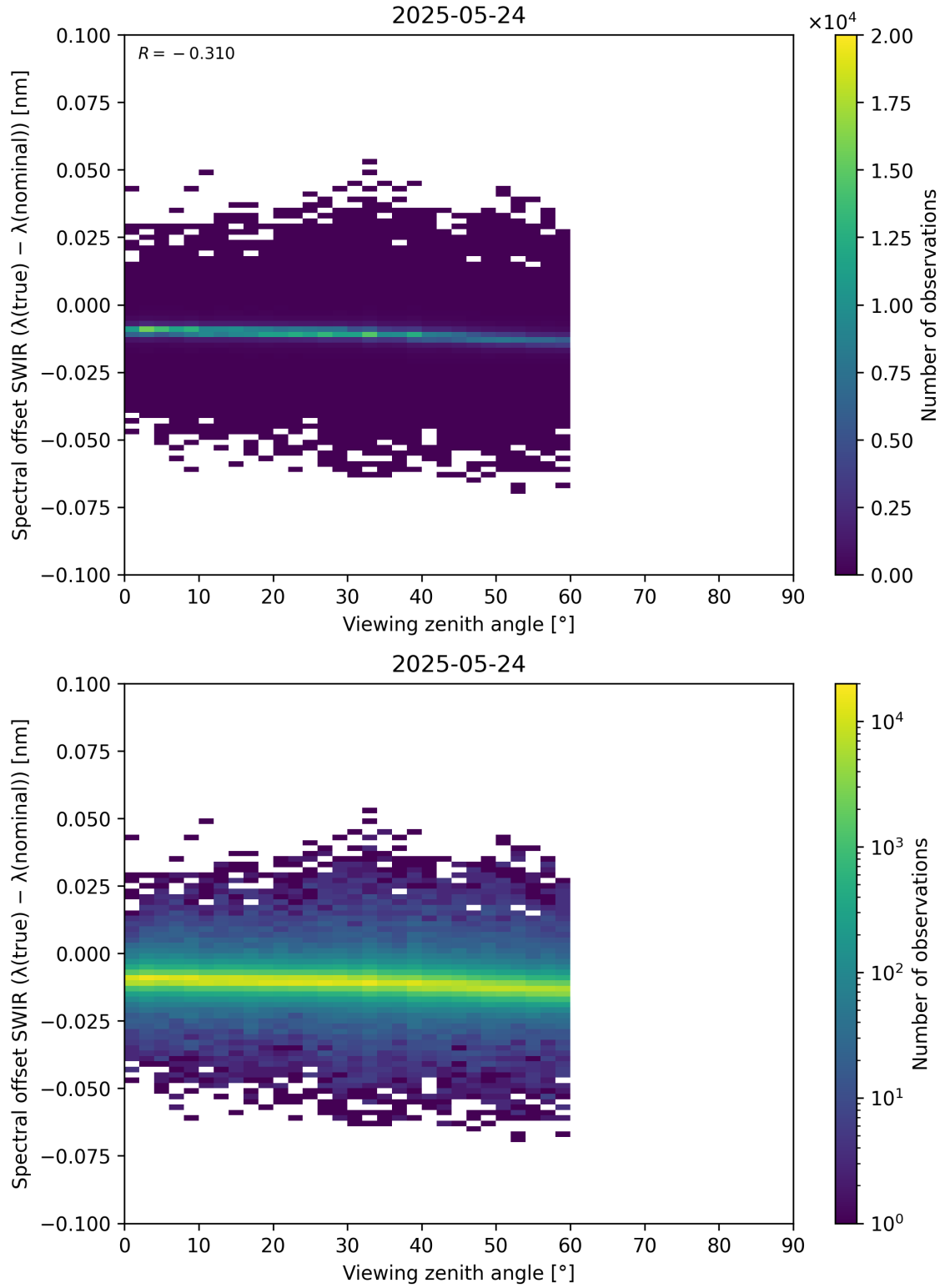
Figure 116: Scatter density plot of “Viewing zenith angle” against “Spectral offset SWIR ( \lambda_{\text{true}} - \lambda_{\text{nominal}} )” for 2025-05-23 to 2025-05-25.
