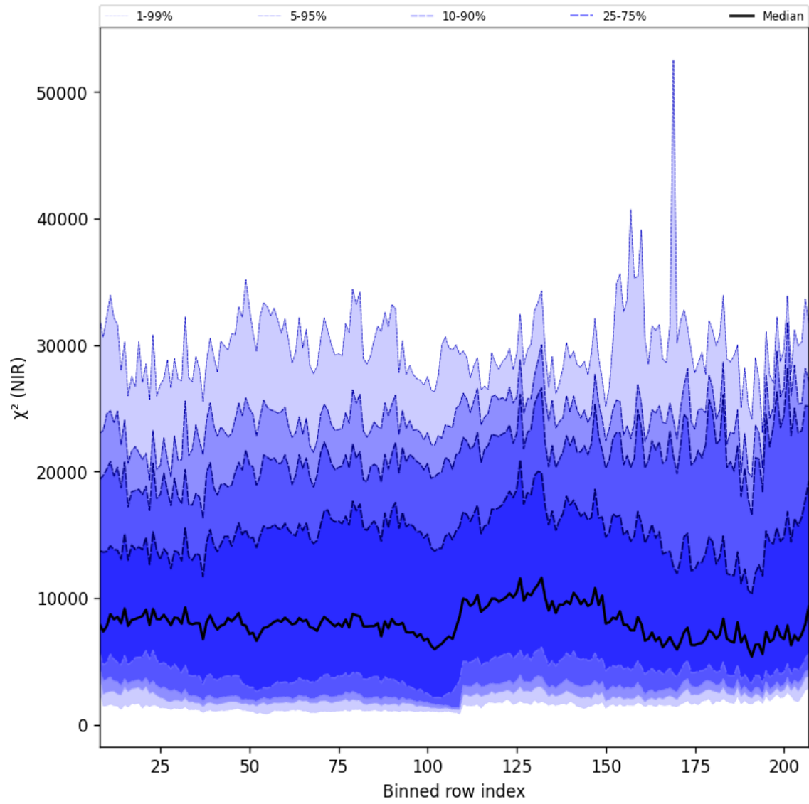
Figure 40: Along track statistics of “ \chi^2 (NIR)” for 2025-05-23 to 2025-05-25
