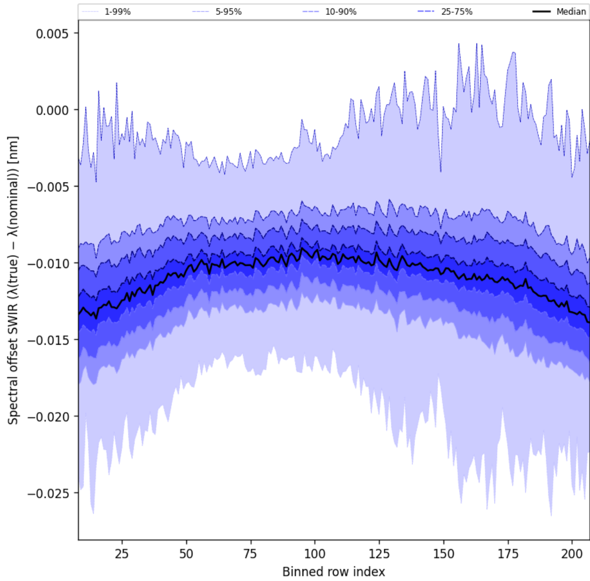
Figure 38: Along track statistics of “Spectral offset SWIR ( \lambda_{\text{true}} - \lambda_{\text{nominal}} )” for 2025-05-23 to 2025-05-25
