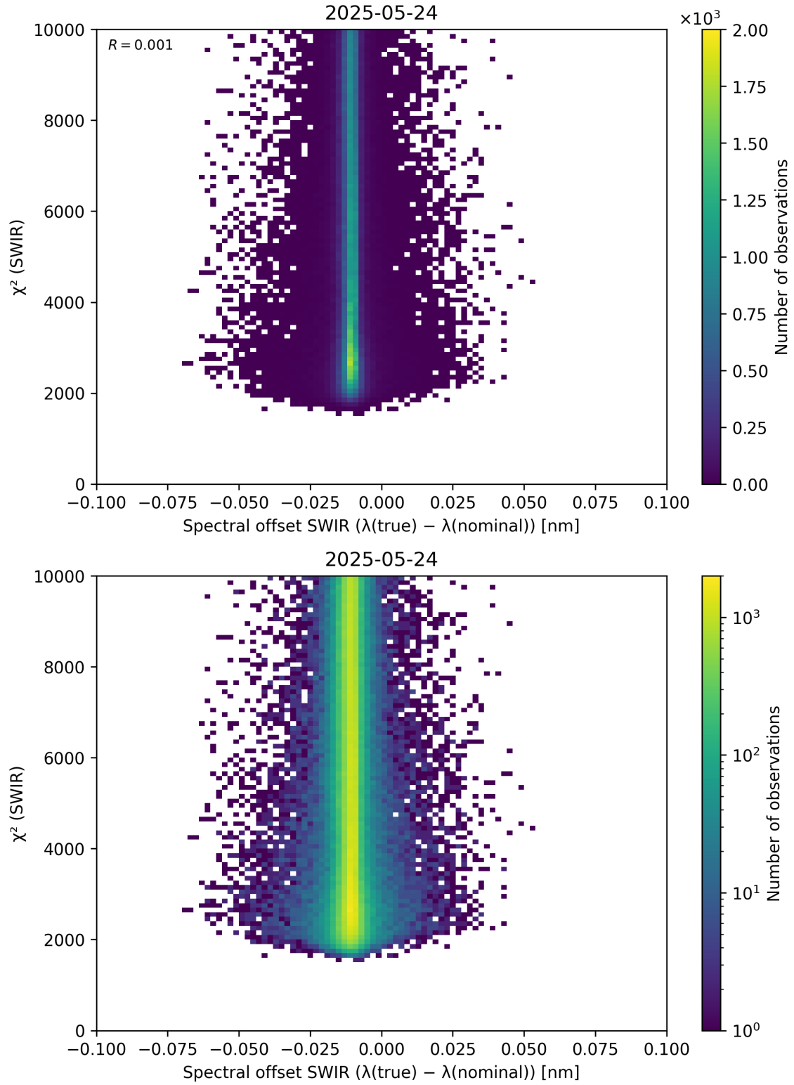
Figure 118: Scatter density plot of “Spectral offset SWIR ( \lambda_{\text{true}} - \lambda_{\text{nominal}} )” against “ \chi^2 (SWIR)” for 2025-05-23 to 2025-05-25.
