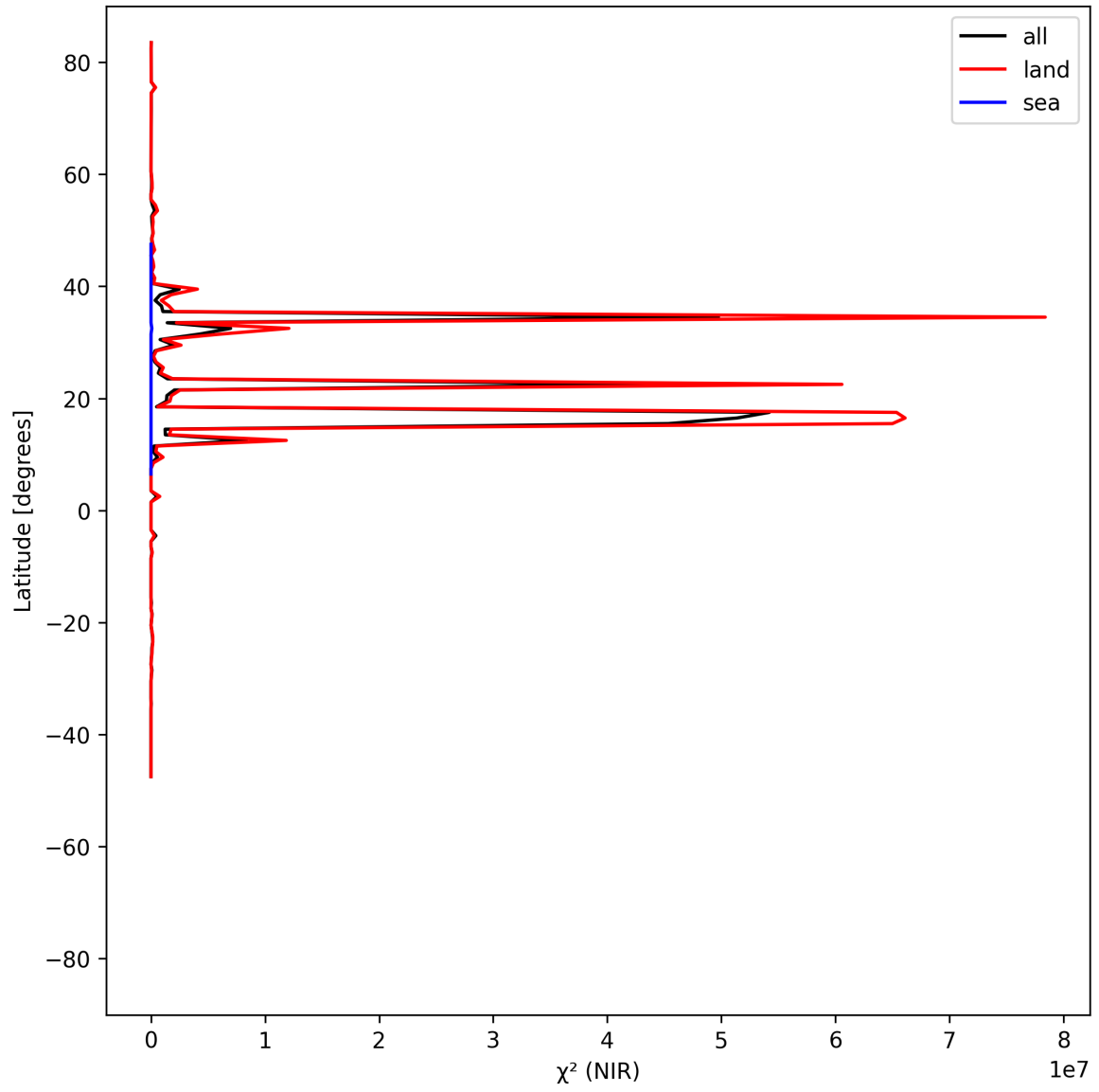
Figure 18: Zonal average of “ \chi^2 (NIR)” for 2025-05-23 to 2025-05-25.
