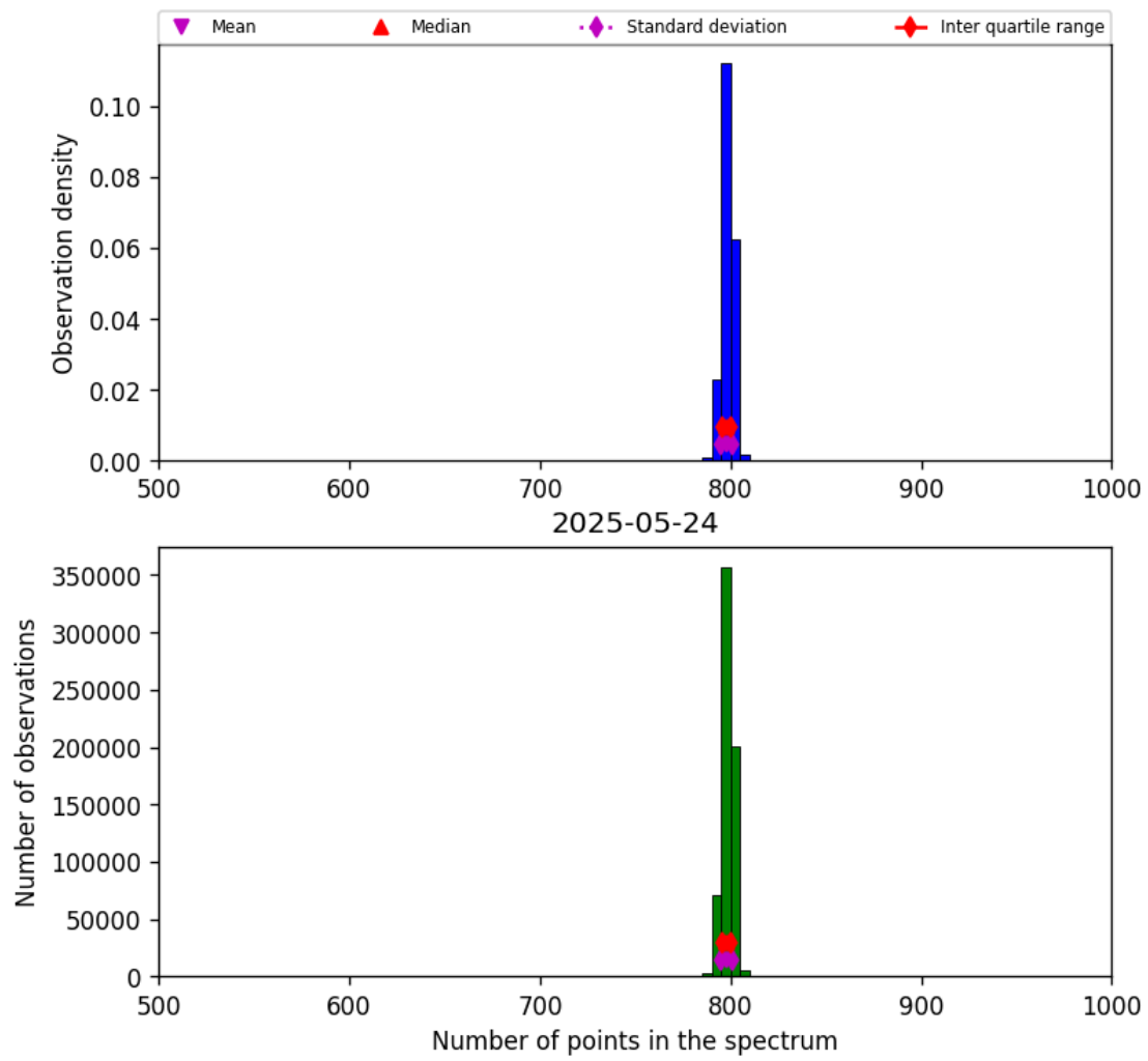
Figure 26: Histogram of “Number of points in the spectrum” for 2025-05-23 to 2025-05-25
