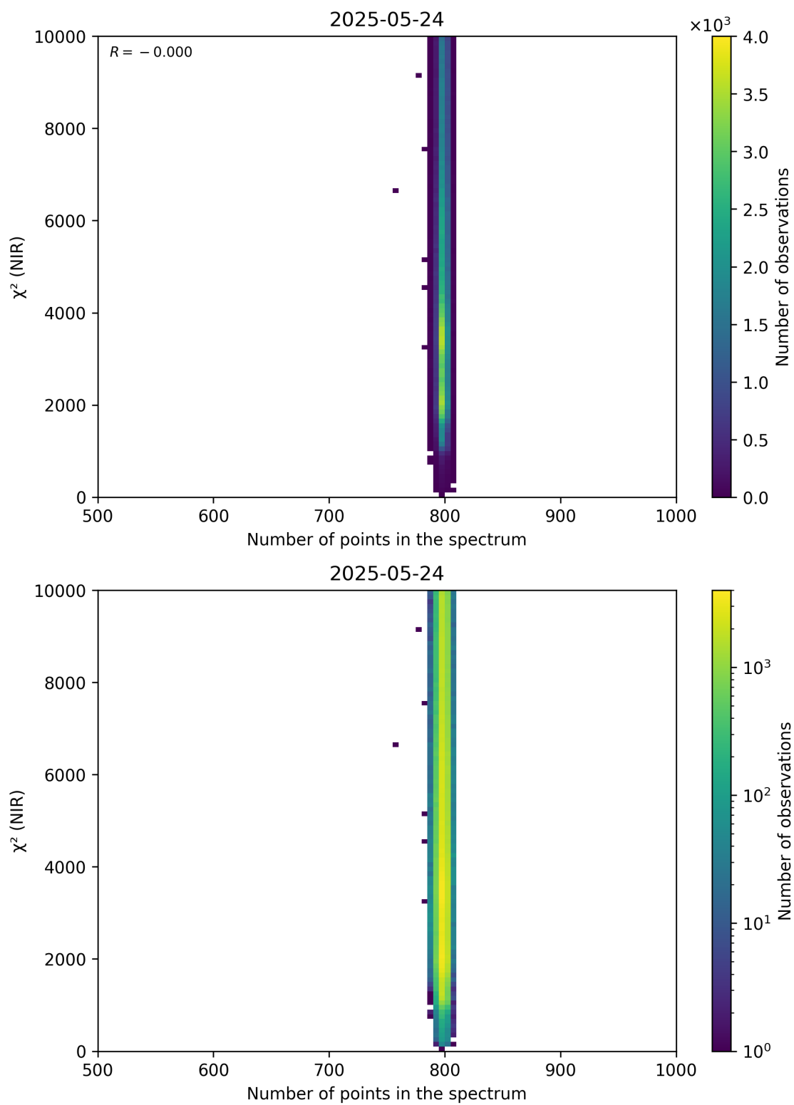
Figure 88: Scatter density plot of “Number of points in the spectrum” against “ \chi^2 (NIR)” for 2025-05-23 to 2025-05-25.
