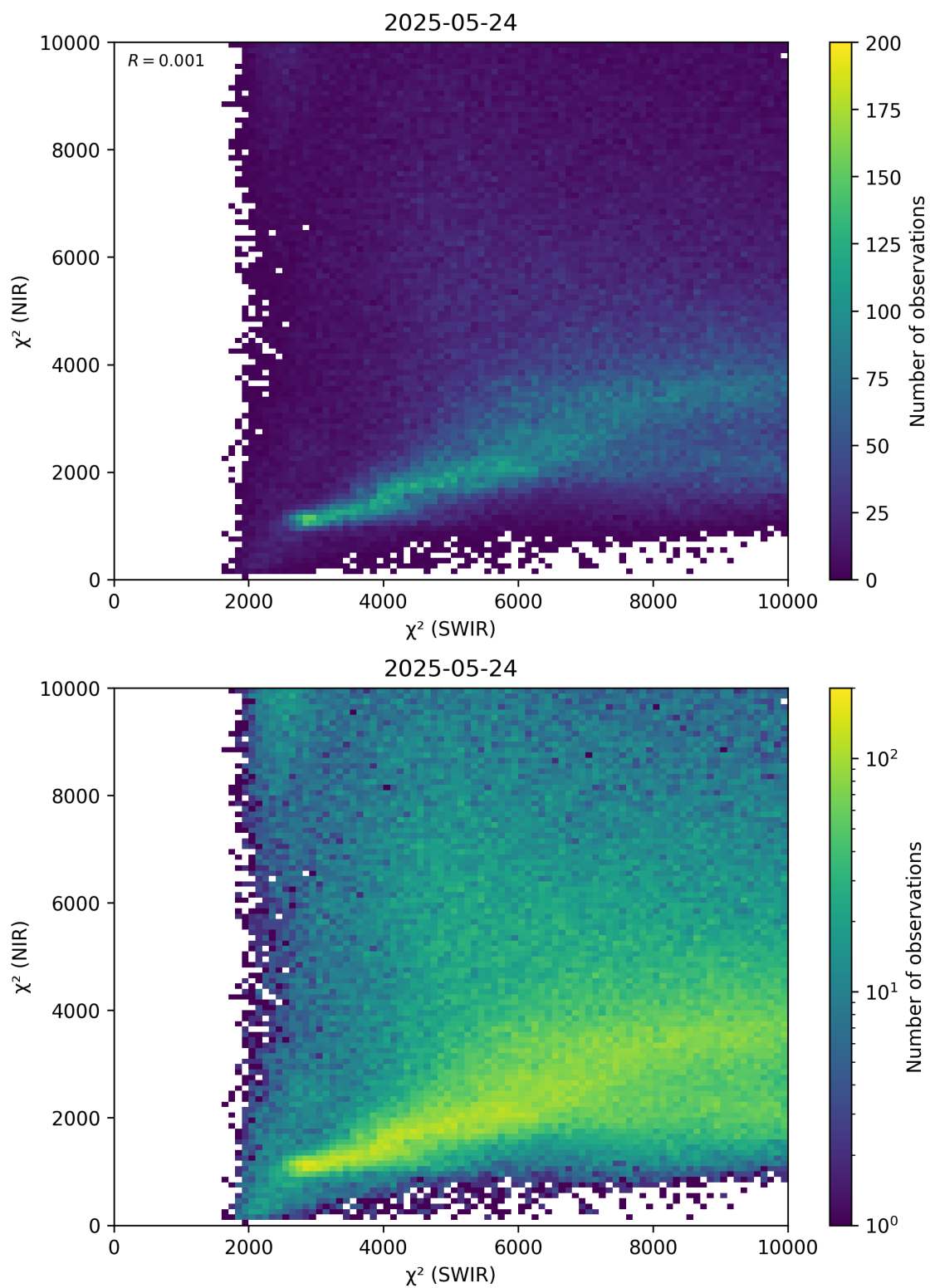
Figure 47: Scatter density plot of “ \chi^2 (SWIR)” against “ \chi^2 (NIR)” for 2025-05-23 to 2025-05-25.
