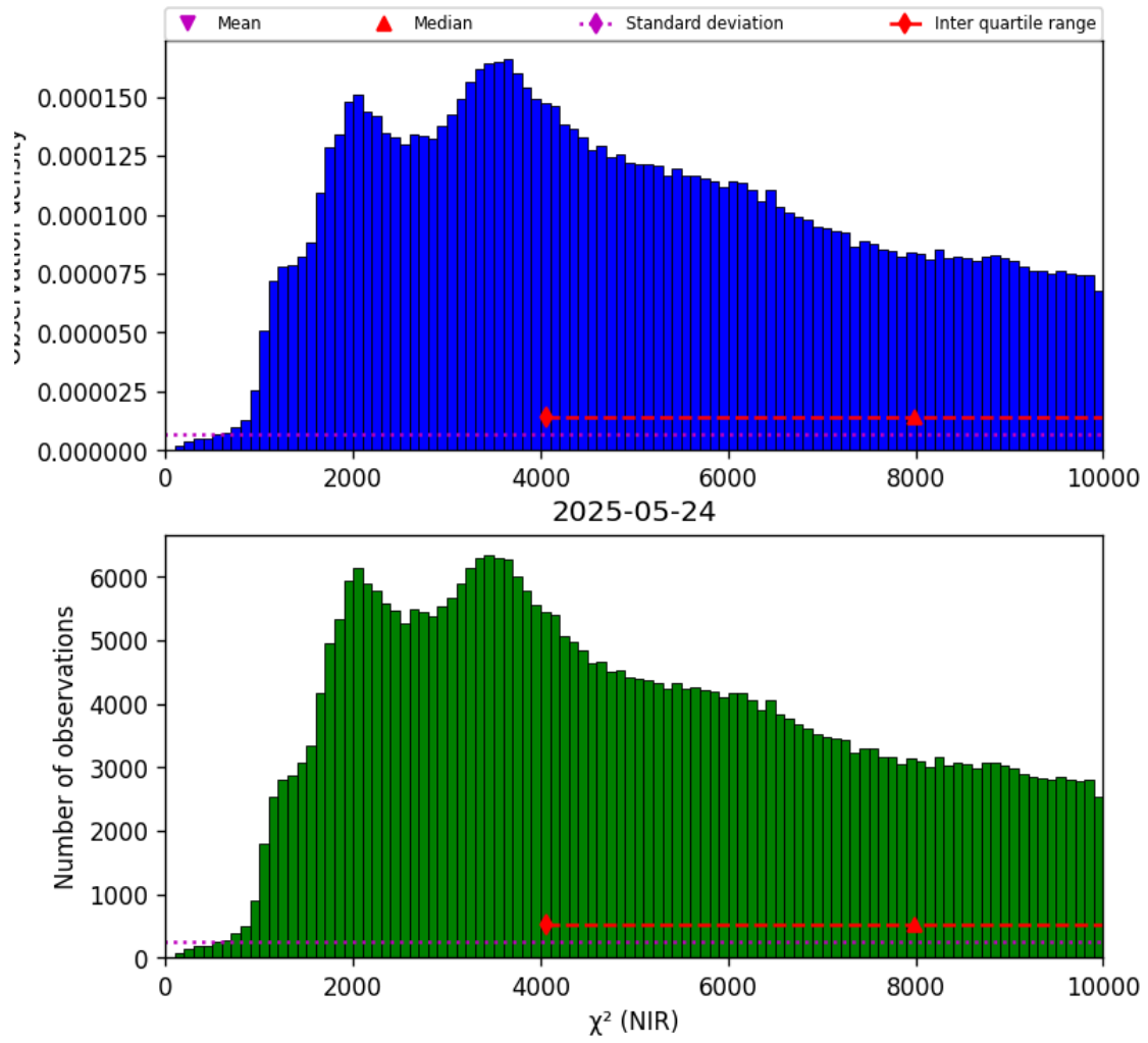
Figure 29: Histogram of “ \chi^2 (NIR)” for 2025-05-23 to 2025-05-25
