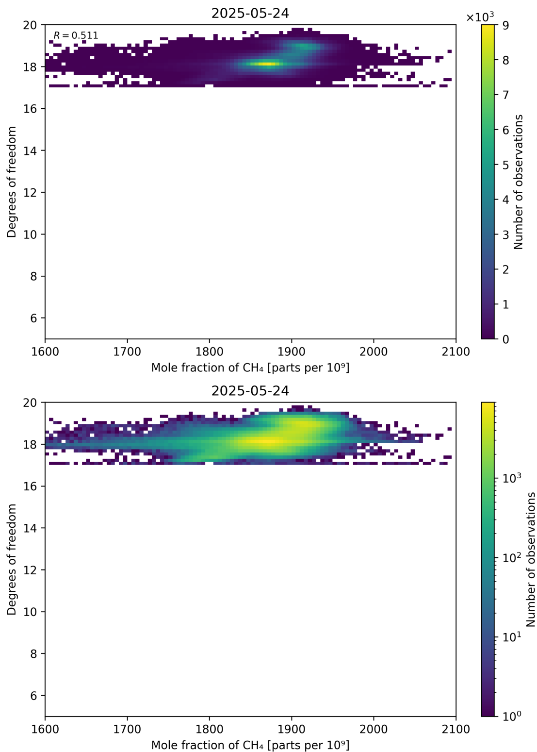
Figure 72: Scatter density plot of “Mole fraction of CH 4 ” against “Degrees of freedom” for 2025-05-23 to 2025-05-25.
