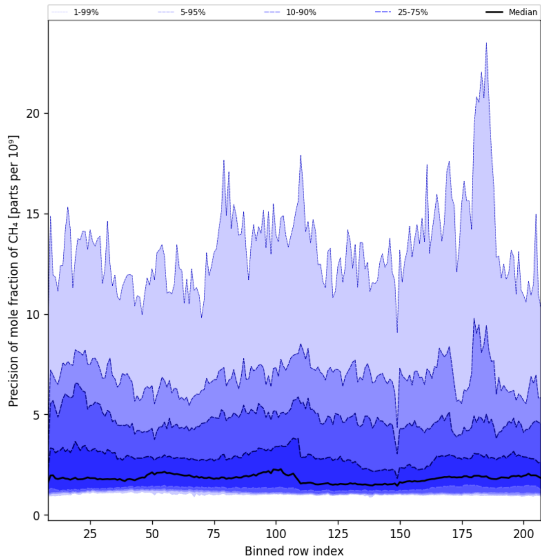
Figure 35: Along track statistics of “Precision of mole fraction of CH 4 ” for 2025-05-23 to 2025-05-25
