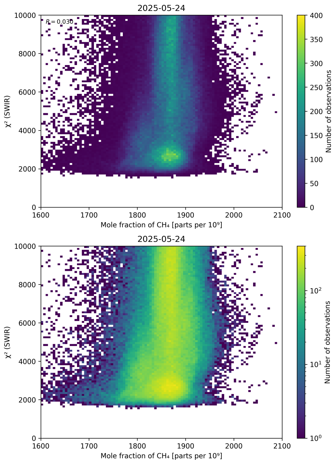
Figure 71: Scatter density plot of “Mole fraction of CH 4 ” against “ \chi^2 (SWIR)” for 2025-05-23 to 2025-05-25.
