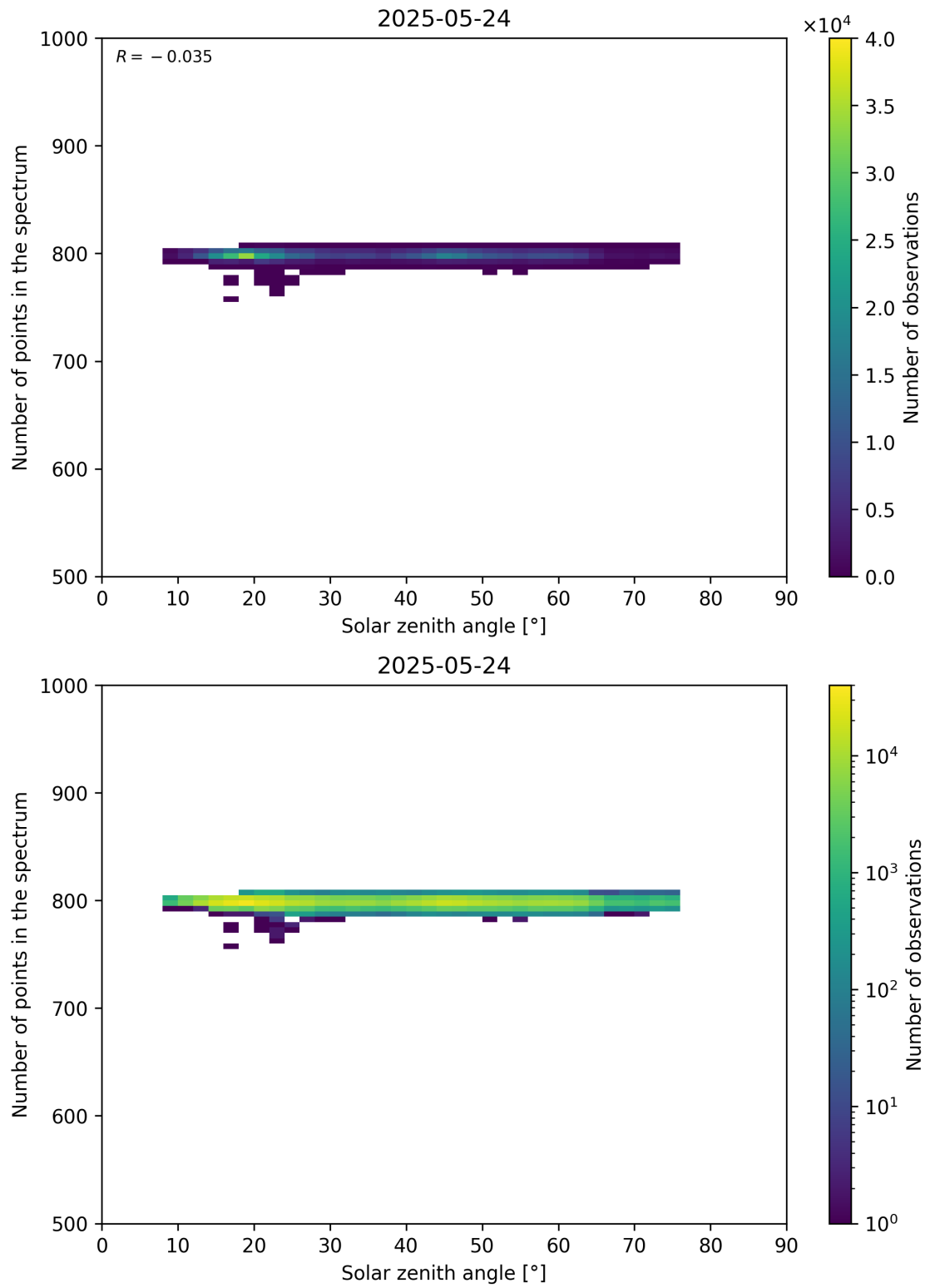
Figure 103: Scatter density plot of “Solar zenith angle” against “Number of points in the spectrum” for 2025-05-23 to 2025-05-25.
