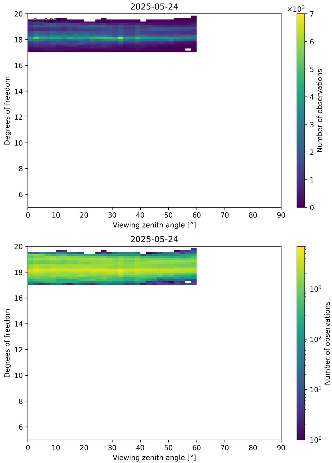
Figure 107: Scatter density plot of “Viewing zenith angle” against “Degrees of freedom” for 2025-05-23 to 2025-05-25.
