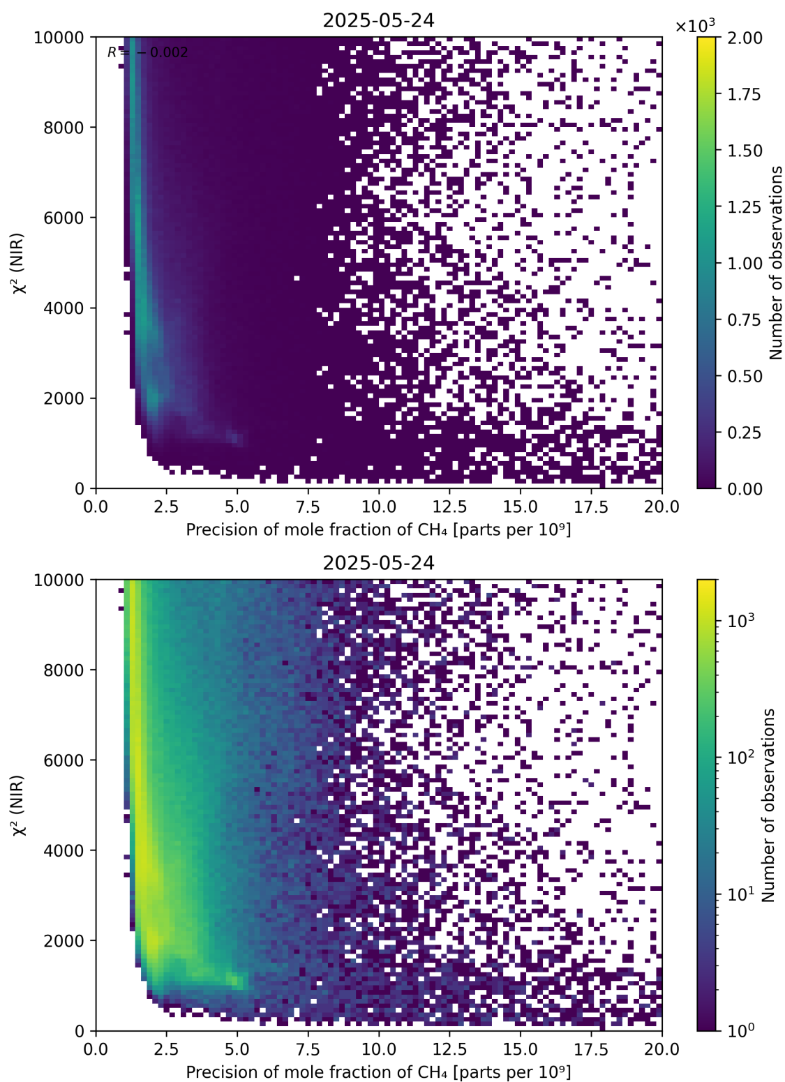
Figure 78: Scatter density plot of “Precision of mole fraction of \text{CH}_4 ” against “ \chi^2 (NIR)” for 2025-05-23 to 2025-05-25.
