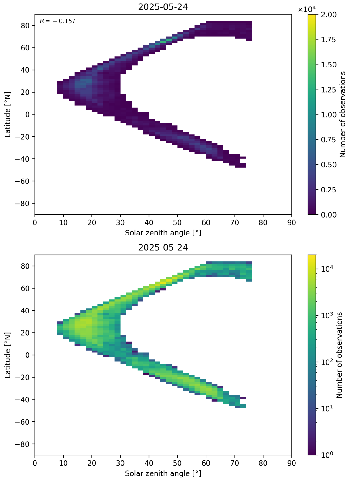
Figure 98: Scatter density plot of “Solar zenith angle” against “Latitude” for 2025-05-23 to 2025-05-25.
