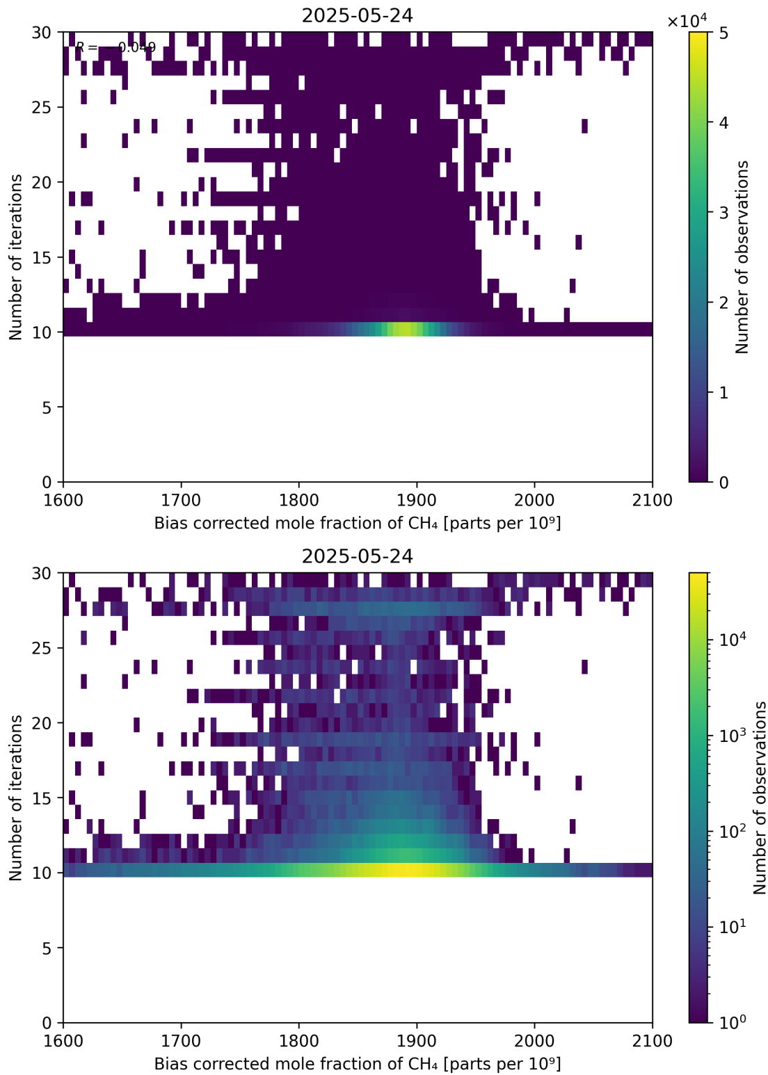
Figure 67: Scatter density plot of “Bias corrected mole fraction of CH 4 ” against “Number of iterations” for 2025-05-23 to 2025-05-25.
