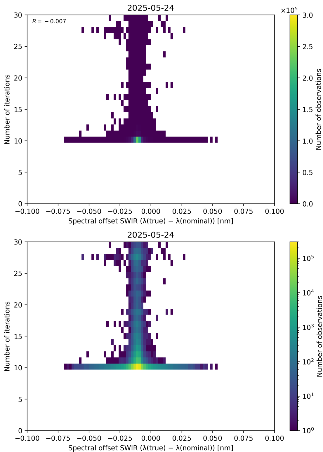
Figure 121: Scatter density plot of “Spectral offset SWIR ( \lambda_{\text{true}} - \lambda_{\text{nominal}} )” against “Number of iterations” for 2025-05-23 to 2025-05-25.
