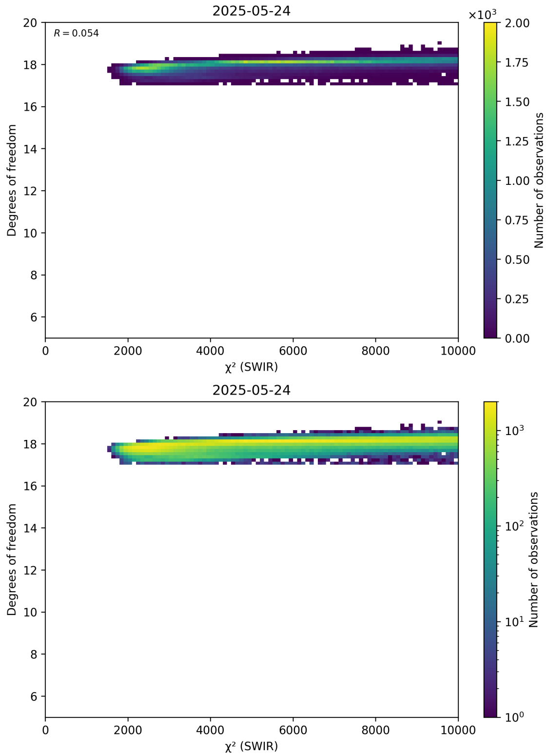
Figure 48: Scatter density plot of “ \chi^2 (SWIR)” against “Degrees of freedom” for 2025-05-23 to 2025-05-25.
