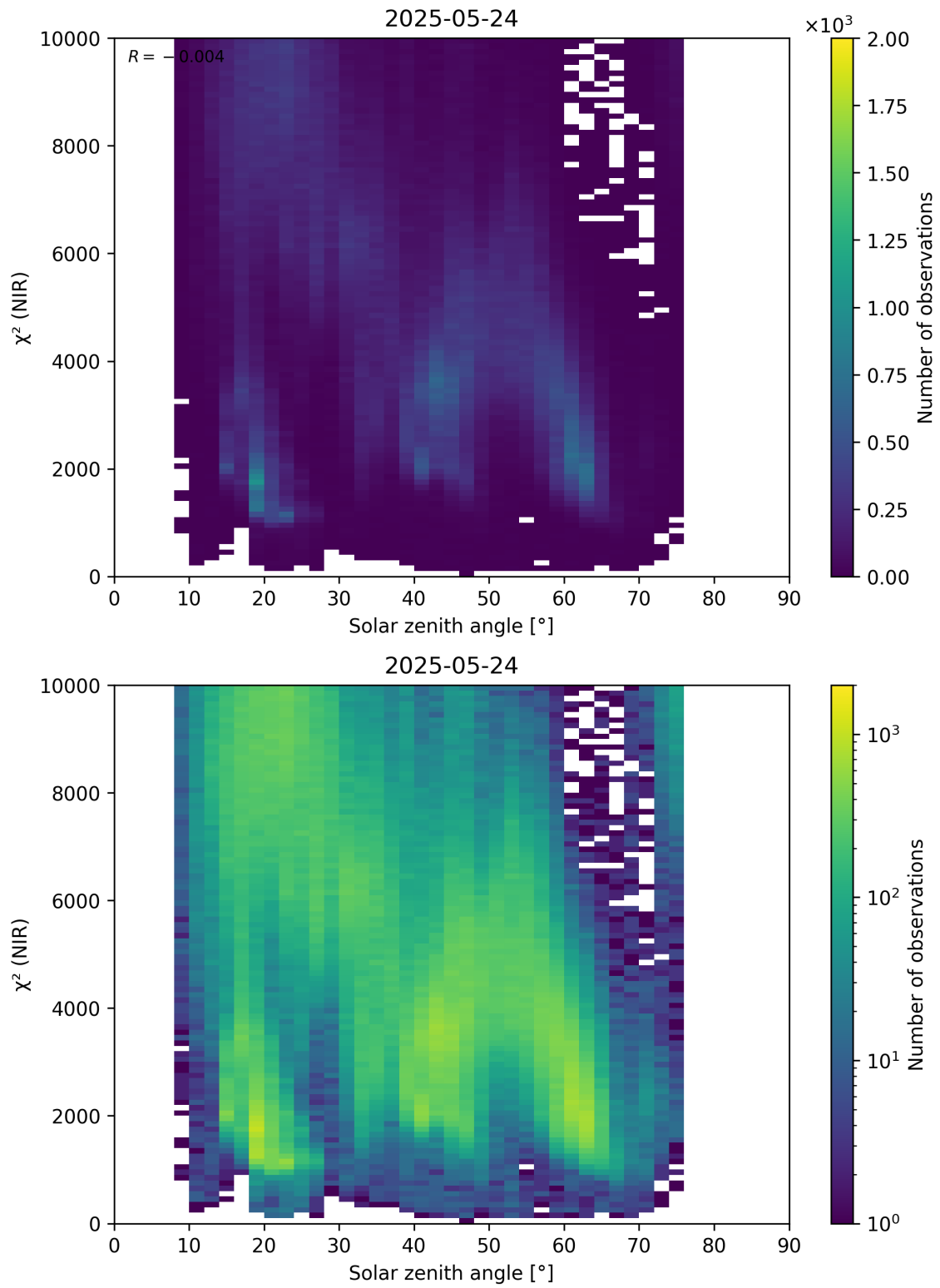
Figure 94: Scatter density plot of “Solar zenith angle” against “ \chi^2 (NIR)” for 2025-05-23 to 2025-05-25.
