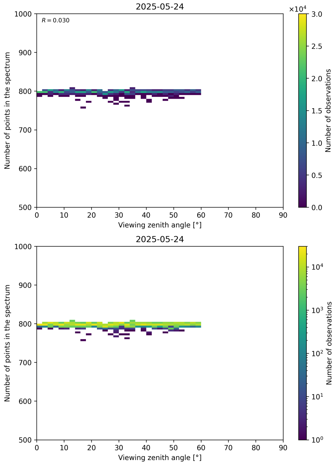
Figure 114: Scatter density plot of “Viewing zenith angle” against “Number of points in the spectrum” for 2025-05-23 to 2025-05-25.
