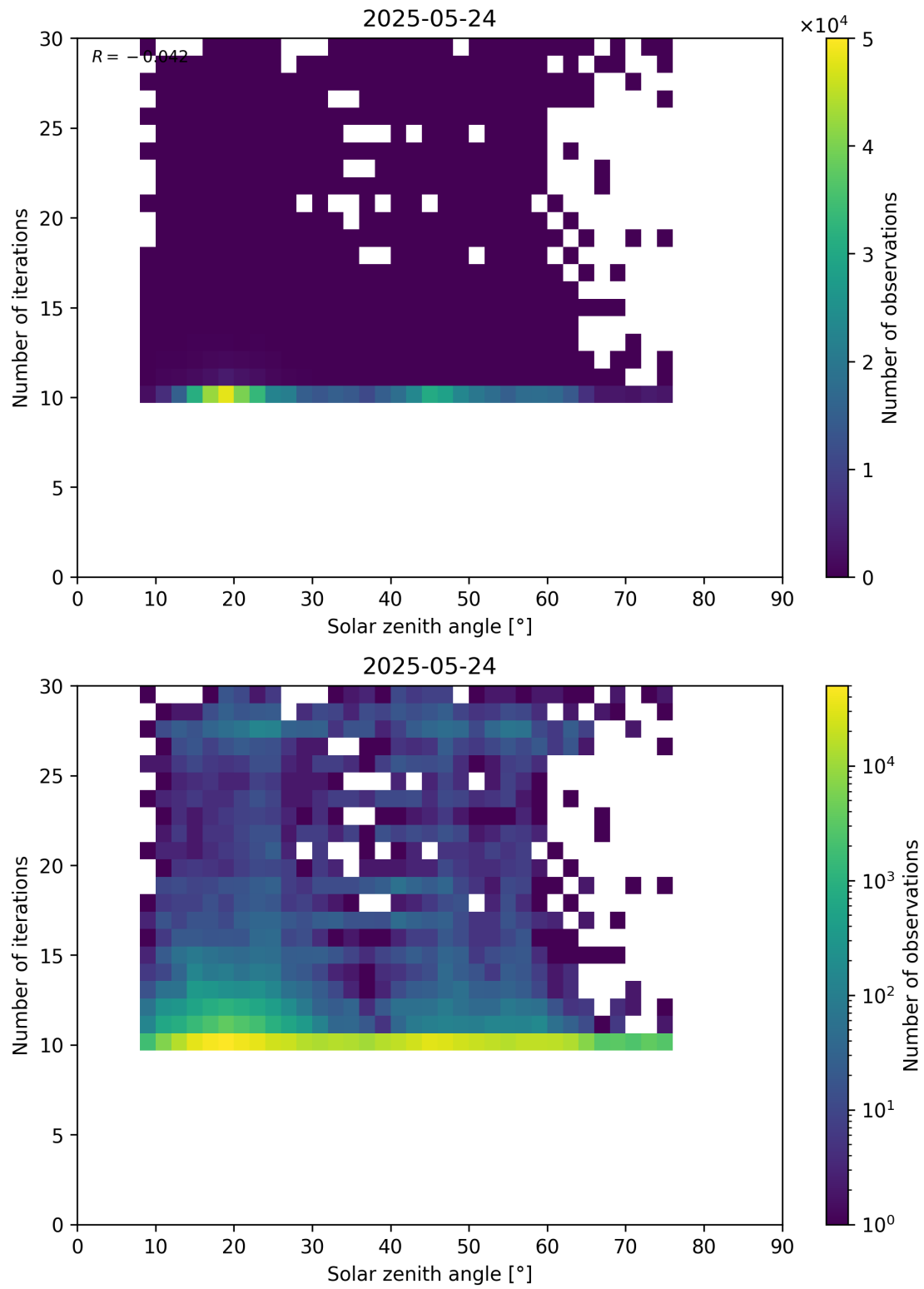
Figure 102: Scatter density plot of “Solar zenith angle” against “Number of iterations” for 2025-05-23 to 2025-05-25.
