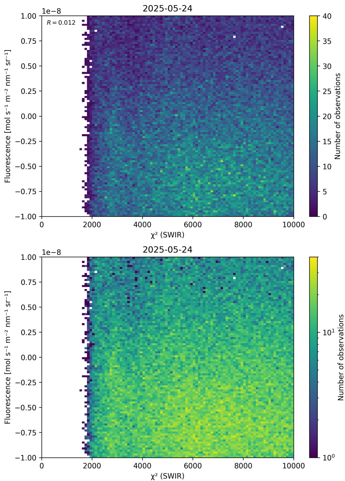
Figure 49: Scatter density plot of “ \chi^2 (SWIR)” against “Fluorescence” for 2025-05-23 to 2025-05-25.
