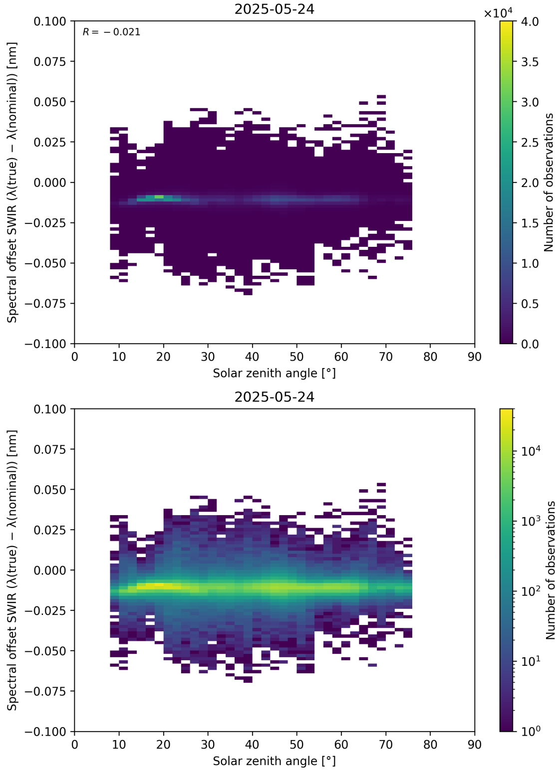
Figure 104: Scatter density plot of “Solar zenith angle” against “Spectral offset SWIR ( \lambda_{\text{true}} - \lambda_{\text{nominal}} )” for 2025-05-23 to 2025-05-25.
