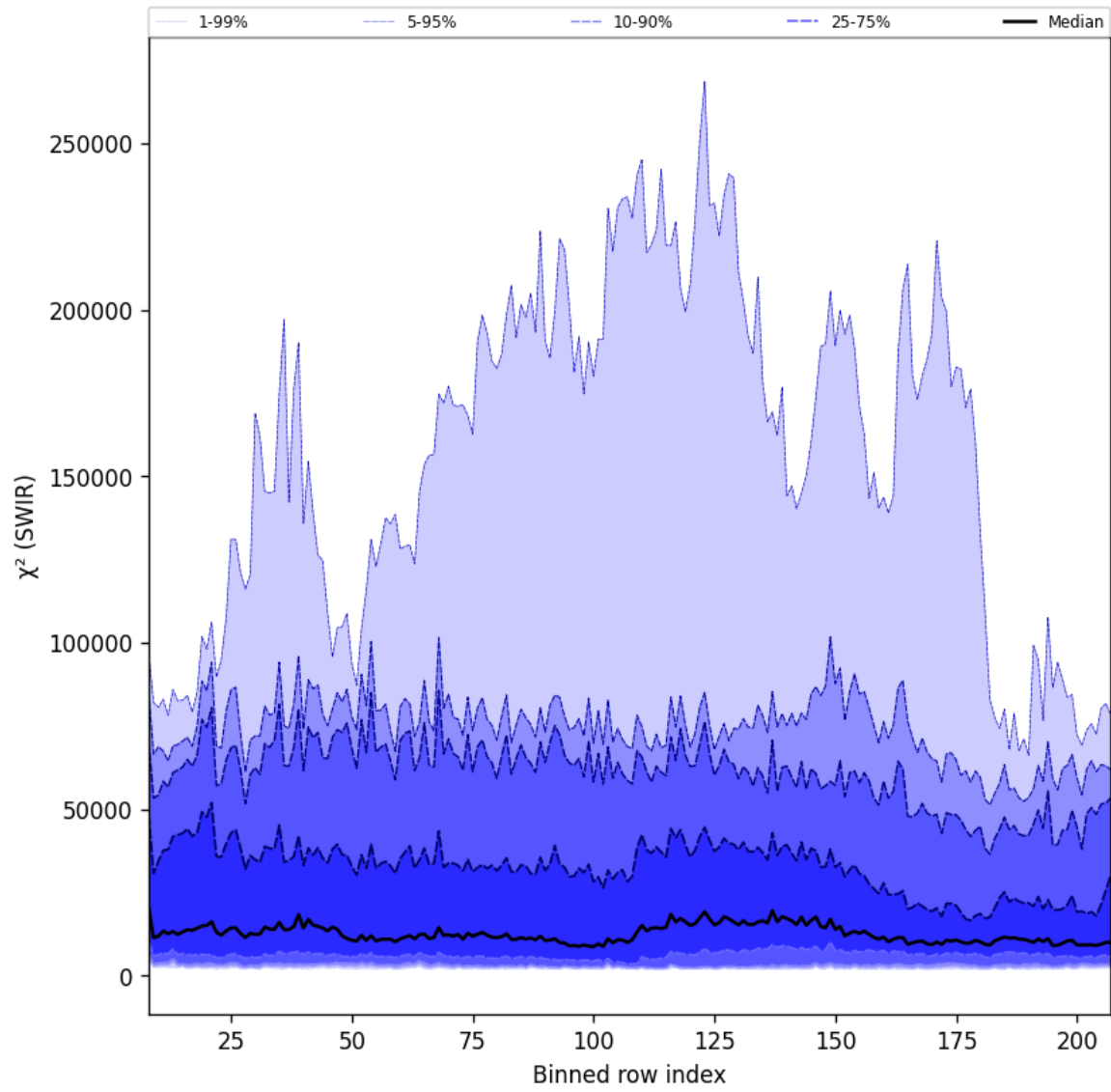
Figure 39: Along track statistics of “ \chi^2 (SWIR)” for 2025-05-23 to 2025-05-25
