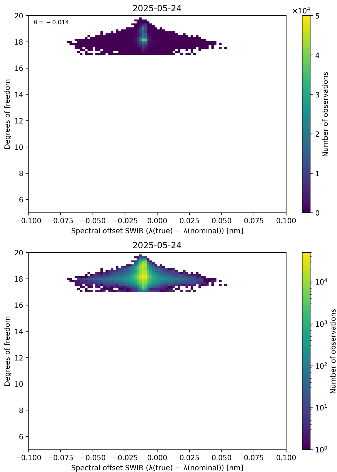
Figure 119: Scatter density plot of “Spectral offset SWIR ( \lambda_{\text{true}} - \lambda_{\text{nominal}} )” against “Degrees of freedom” for 2025-05-23 to 2025-05-25.
