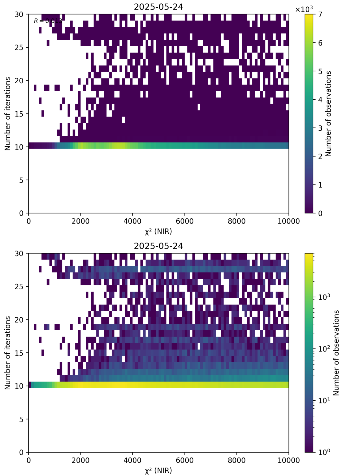
Figure 46: Scatter density plot of “ \chi^2 (NIR)” against “Number of iterations” for 2025-05-23 to 2025-05-25.
