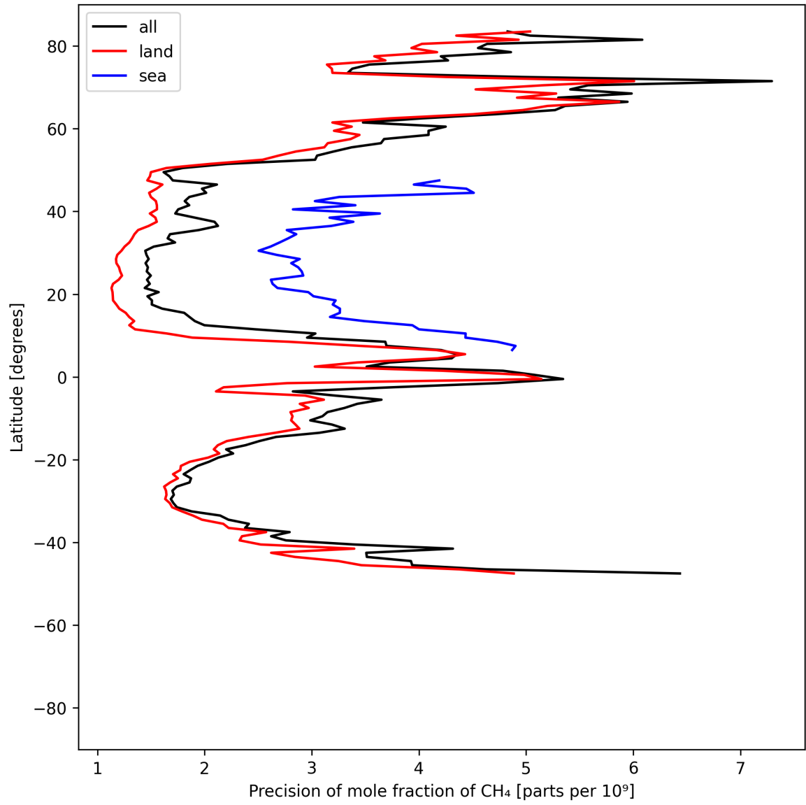
Figure 13: Zonal average of “Precision of mole fraction of CH 4 ” for 2025-05-23 to 2025-05-25.
