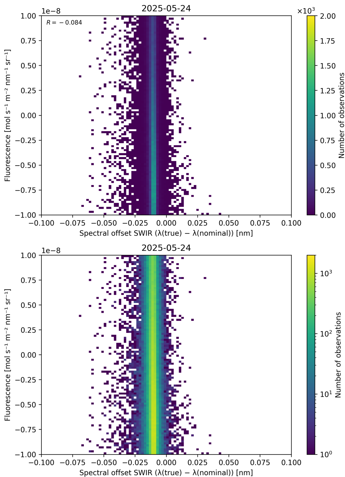
Figure 120: Scatter density plot of “Spectral offset SWIR ( \lambda_{\text{true}} - \lambda_{\text{nominal}} )” against “Fluorescence” for 2025-05-23 to 2025-05-25.
