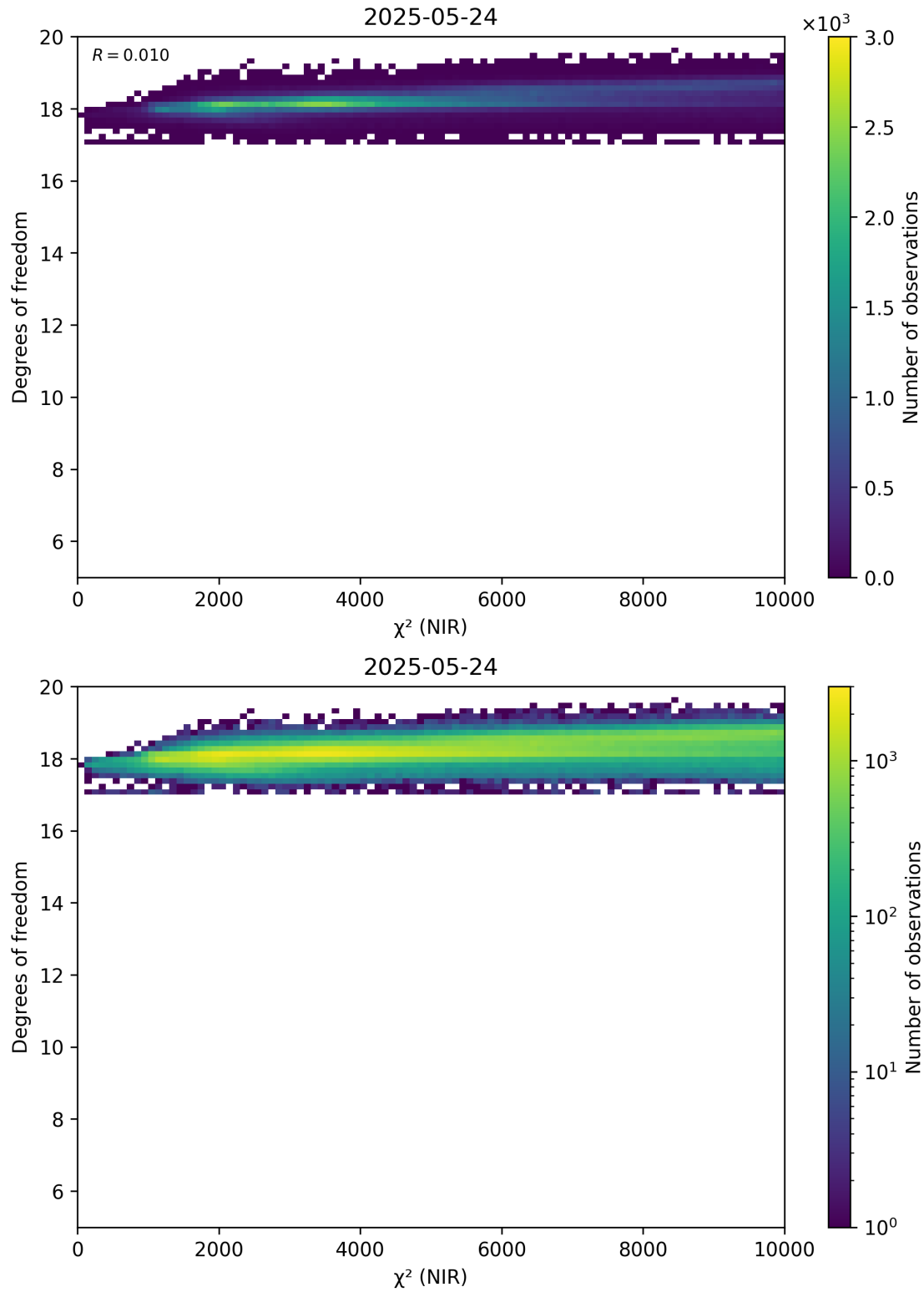
Figure 44: Scatter density plot of “ \chi^2 (NIR)” against “Degrees of freedom” for 2025-05-23 to 2025-05-25.
