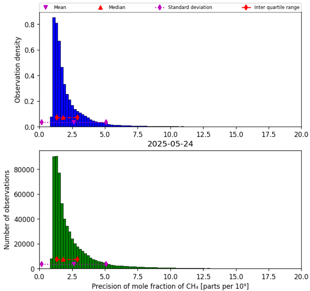
Figure 24: Histogram of “Precision of mole fraction of CH 4 ” for 2025-05-23 to 2025-05-25
