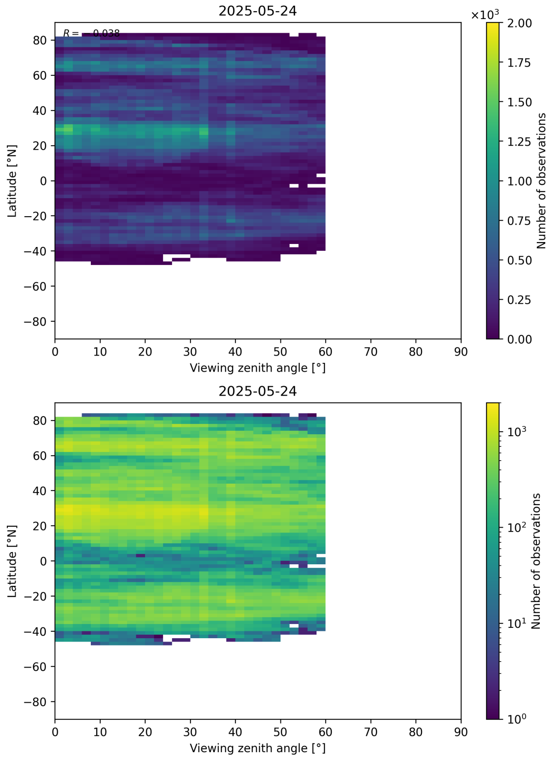
Figure 109: Scatter density plot of “Viewing zenith angle” against “Latitude” for 2025-05-23 to 2025-05-25.
