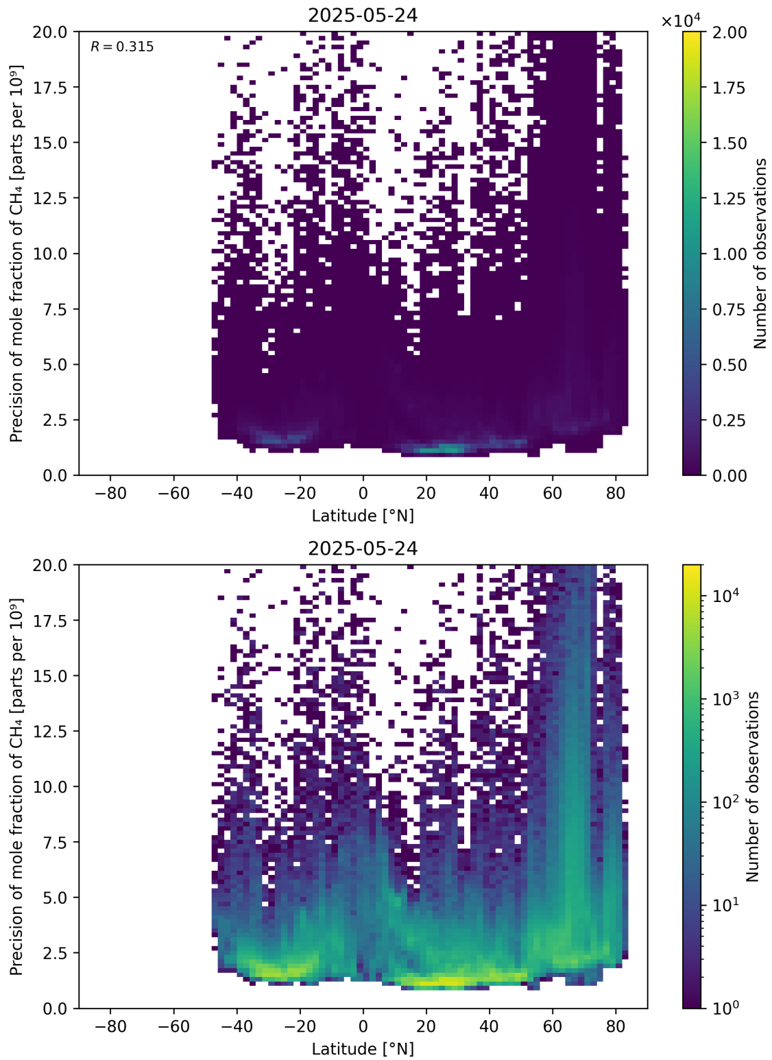
Figure 59: Scatter density plot of “Latitude” against “Precision of mole fraction of \text{CH}_4 ” for 2025-05-23 to 2025-05-25.
