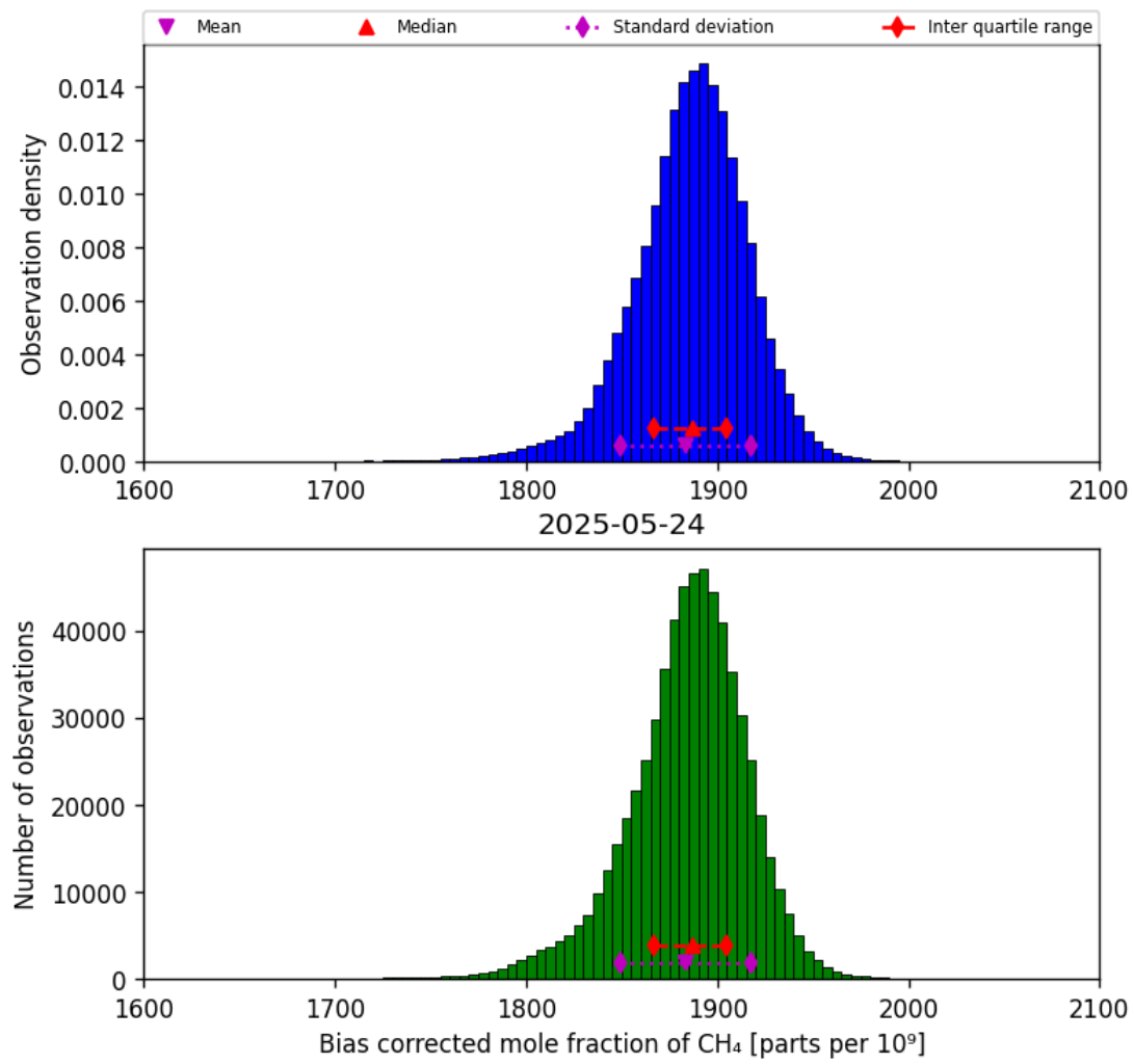
Figure 25: Histogram of “Bias corrected mole fraction of CH 4 ” for 2025-05-23 to 2025-05-25
