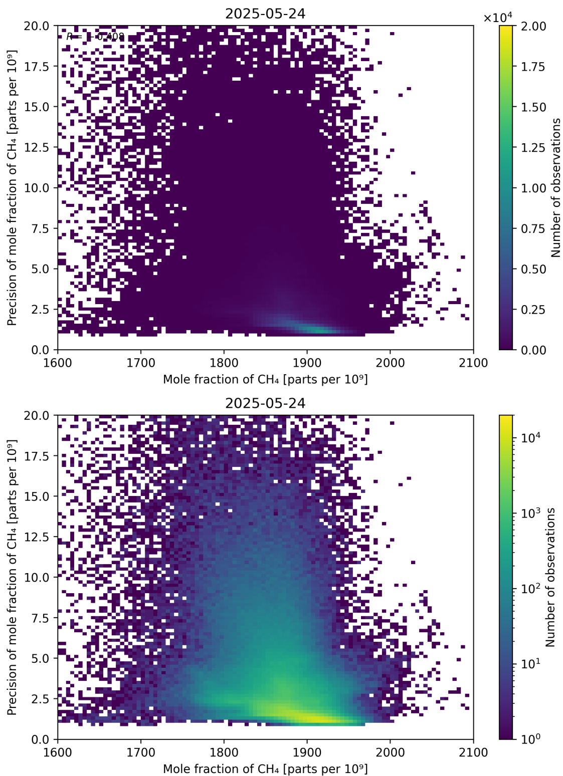
Figure 75: Scatter density plot of “Mole fraction of CH 4 ” against “Precision of mole fraction of CH 4 ” for 2025-05-23 to 2025-05-25.
