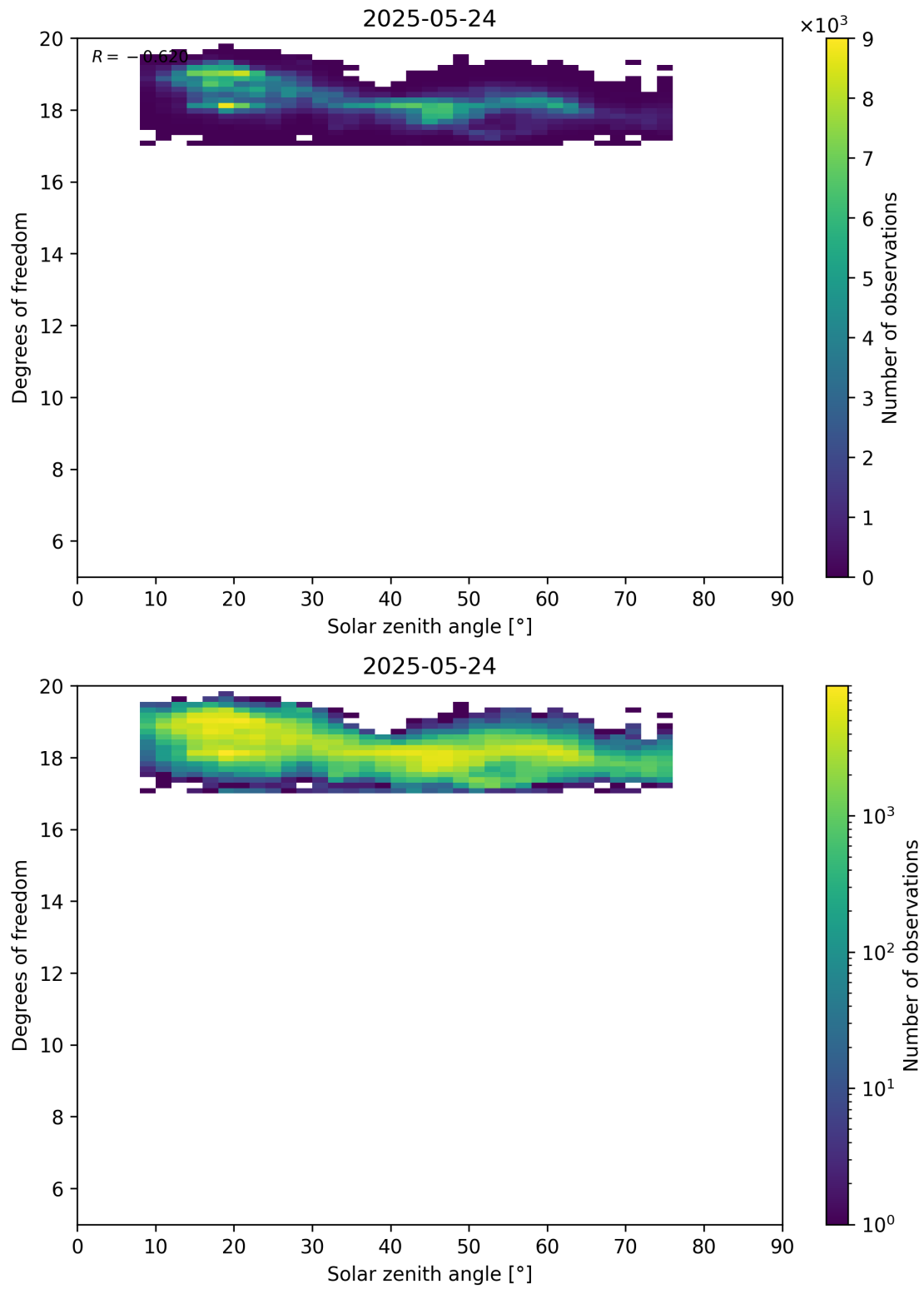
Figure 96: Scatter density plot of “Solar zenith angle” against “Degrees of freedom” for 2025-05-23 to 2025-05-25.
