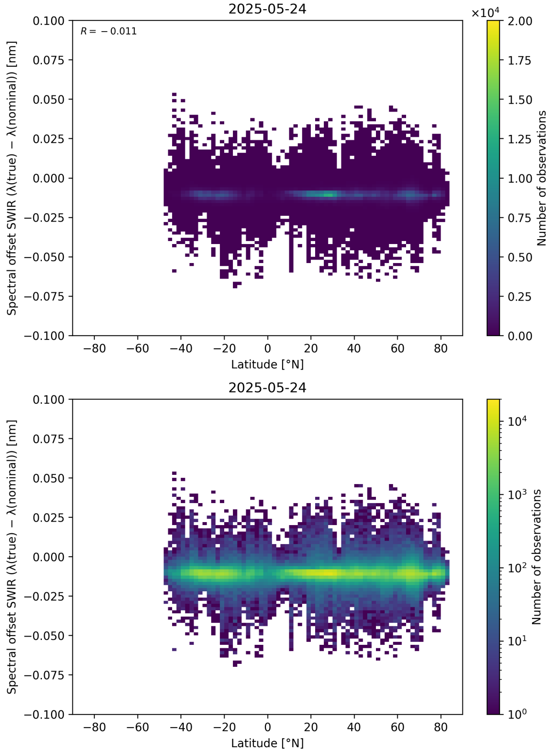
Figure 62: Scatter density plot of “Latitude” against “Spectral offset SWIR ( \lambda_{\text{true}} - \lambda_{\text{nominal}} )” for 2025-05-23 to 2025-05-25.
