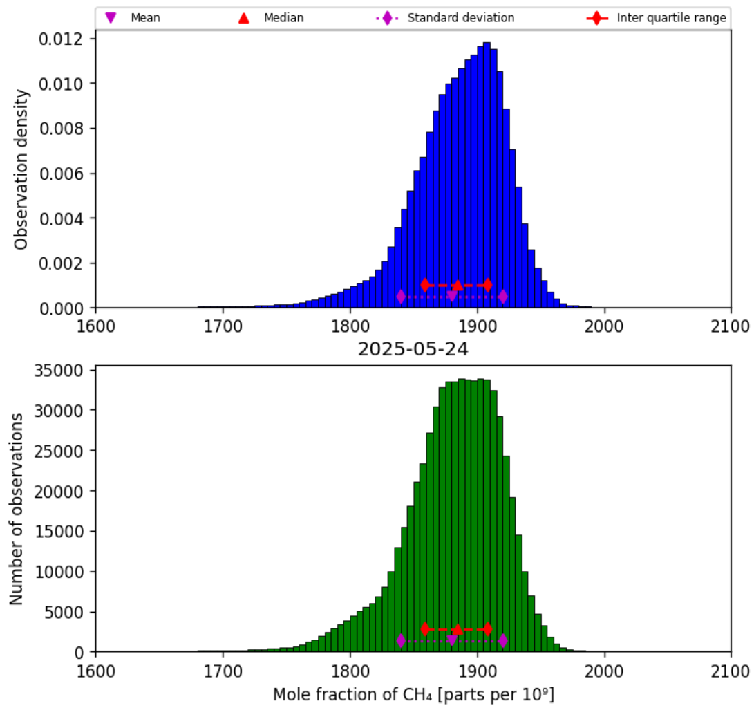
Figure 23: Histogram of “Mole fraction of CH 4 ” for 2025-05-23 to 2025-05-25
