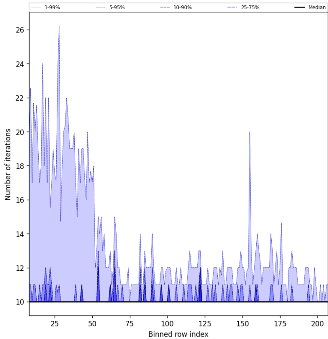
Figure 42: Along track statistics of “Number of iterations” for 2025-05-23 to 2025-05-25
