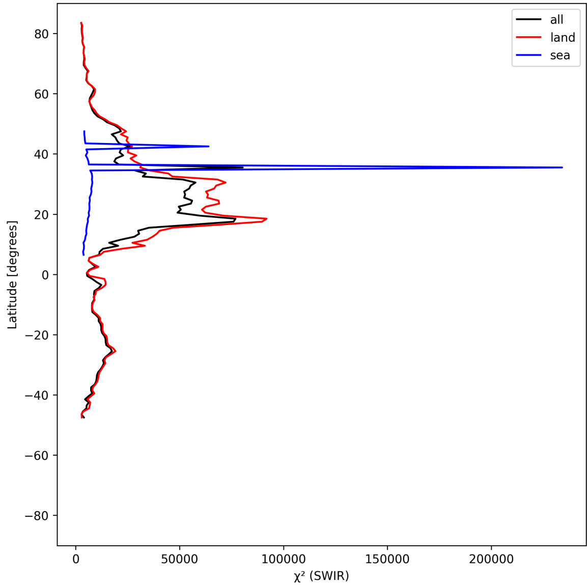
Figure 17: Zonal average of “ \chi^2 (SWIR)” for 2025-05-23 to 2025-05-25.
