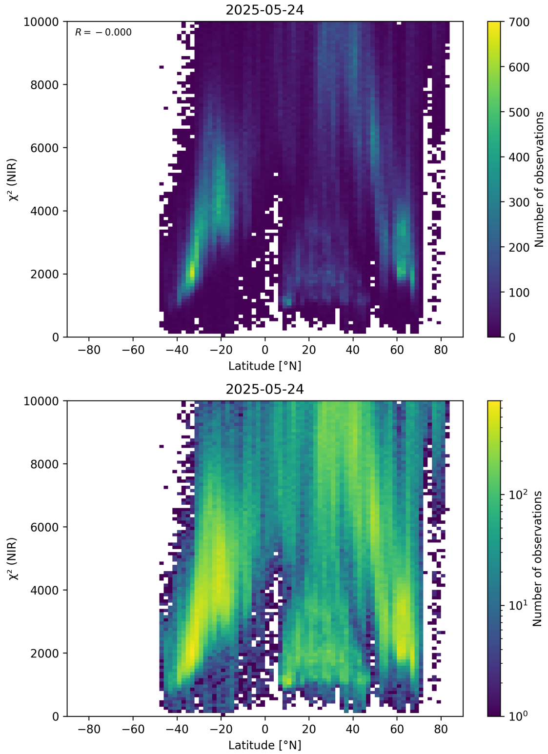
Figure 53: Scatter density plot of “Latitude” against “ \chi^2 (NIR)” for 2025-05-23 to 2025-05-25.
