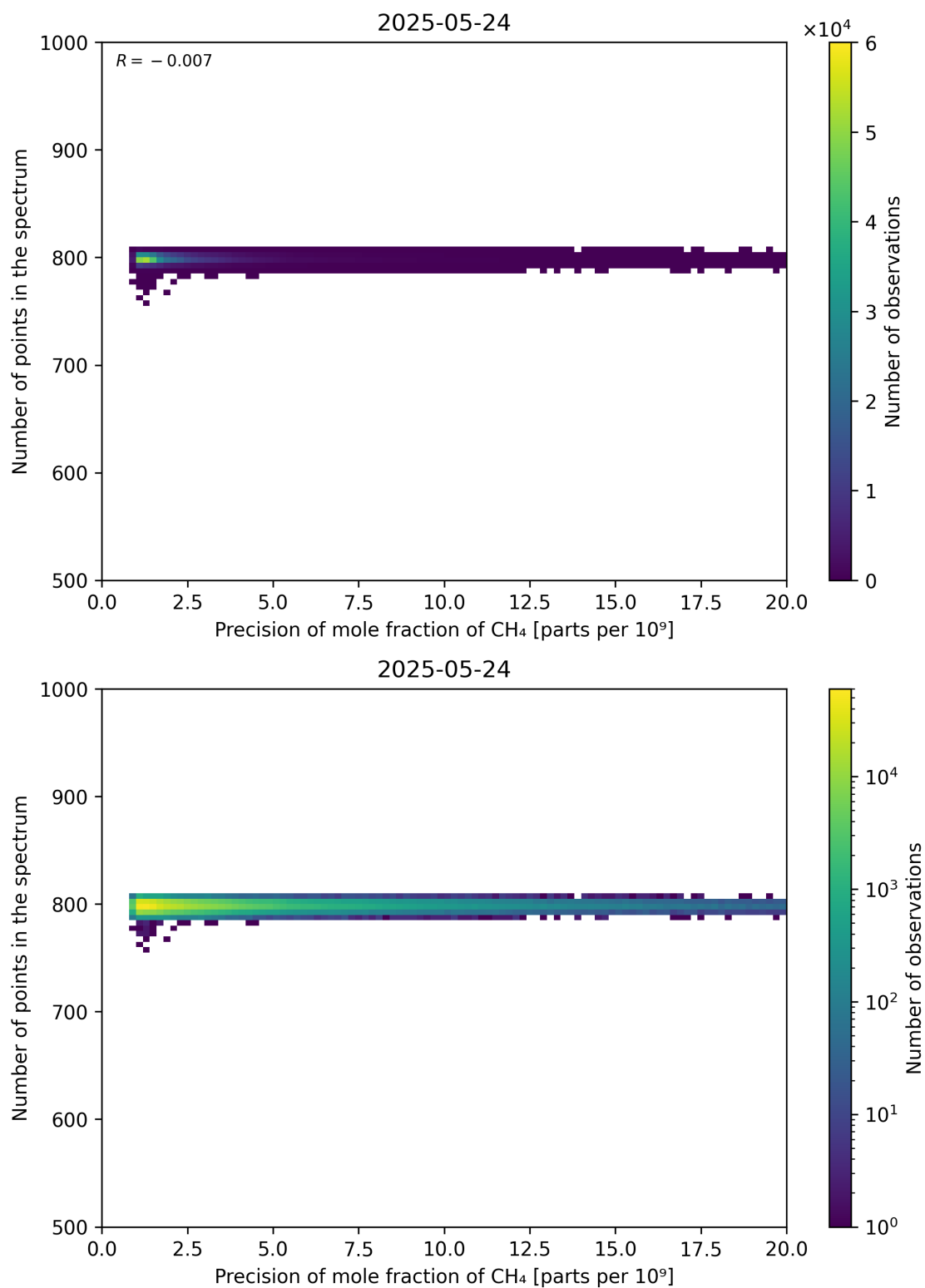
Figure 84: Scatter density plot of “Precision of mole fraction of CH 4 ” against “Number of points in the spectrum” for 2025-05-23 to 2025-05-25.
