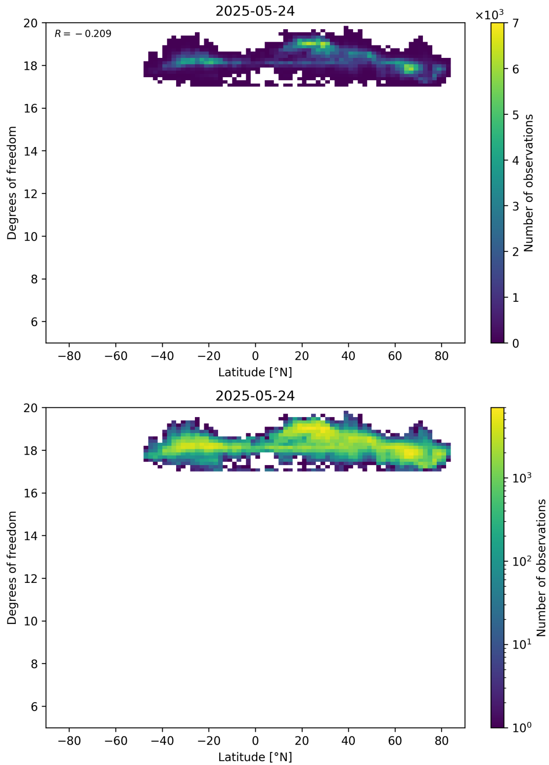
Figure 55: Scatter density plot of “Latitude” against “Degrees of freedom” for 2025-05-23 to 2025-05-25.
