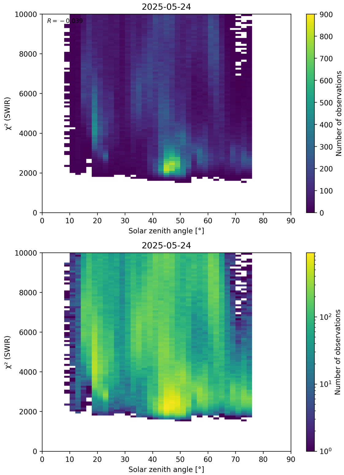
Figure 95: Scatter density plot of “Solar zenith angle” against “ \chi^2 (SWIR)” for 2025-05-23 to 2025-05-25.
