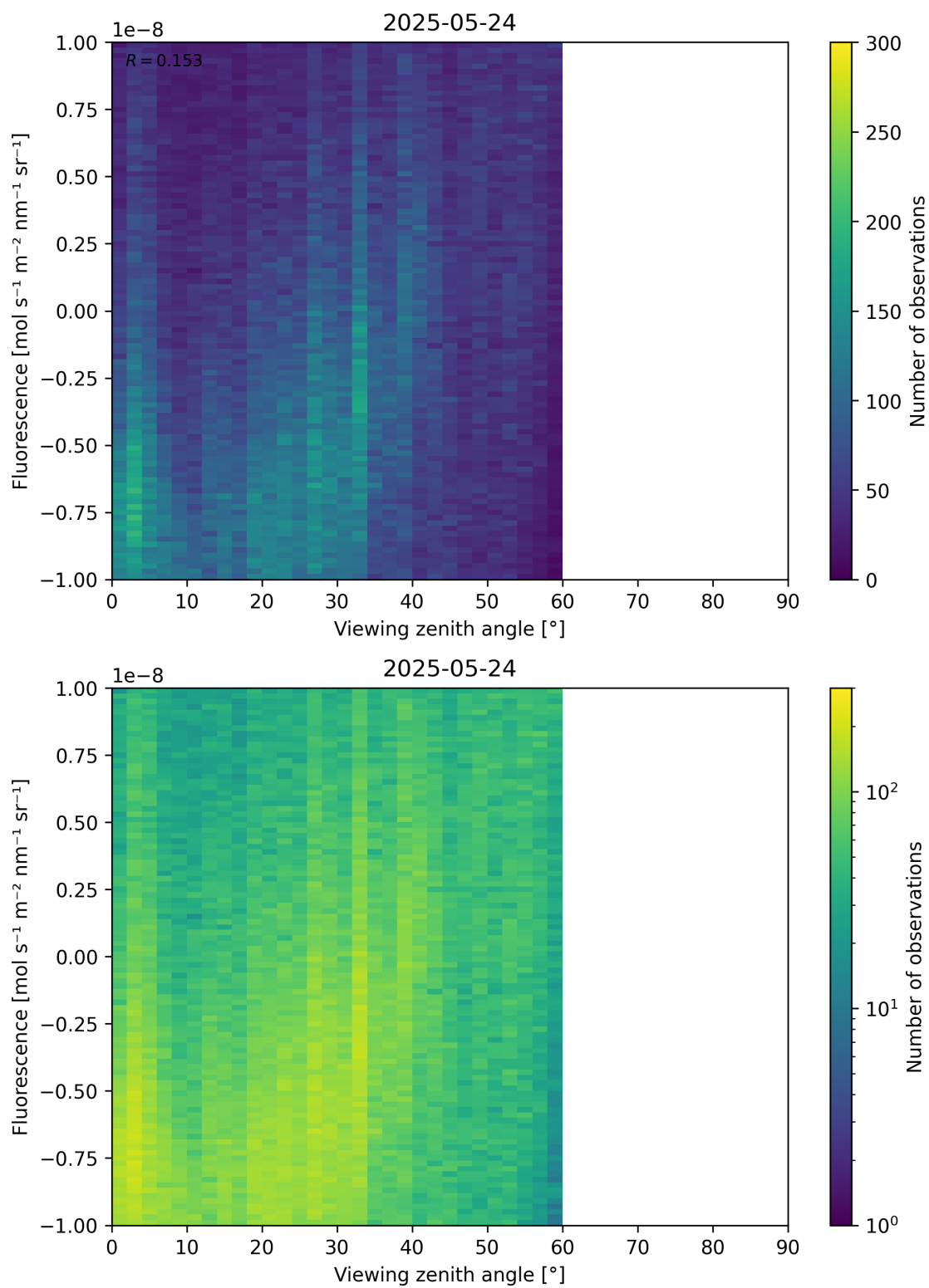
Figure 108: Scatter density plot of “Viewing zenith angle” against “Fluorescence” for 2025-05-23 to 2025-05-25.
