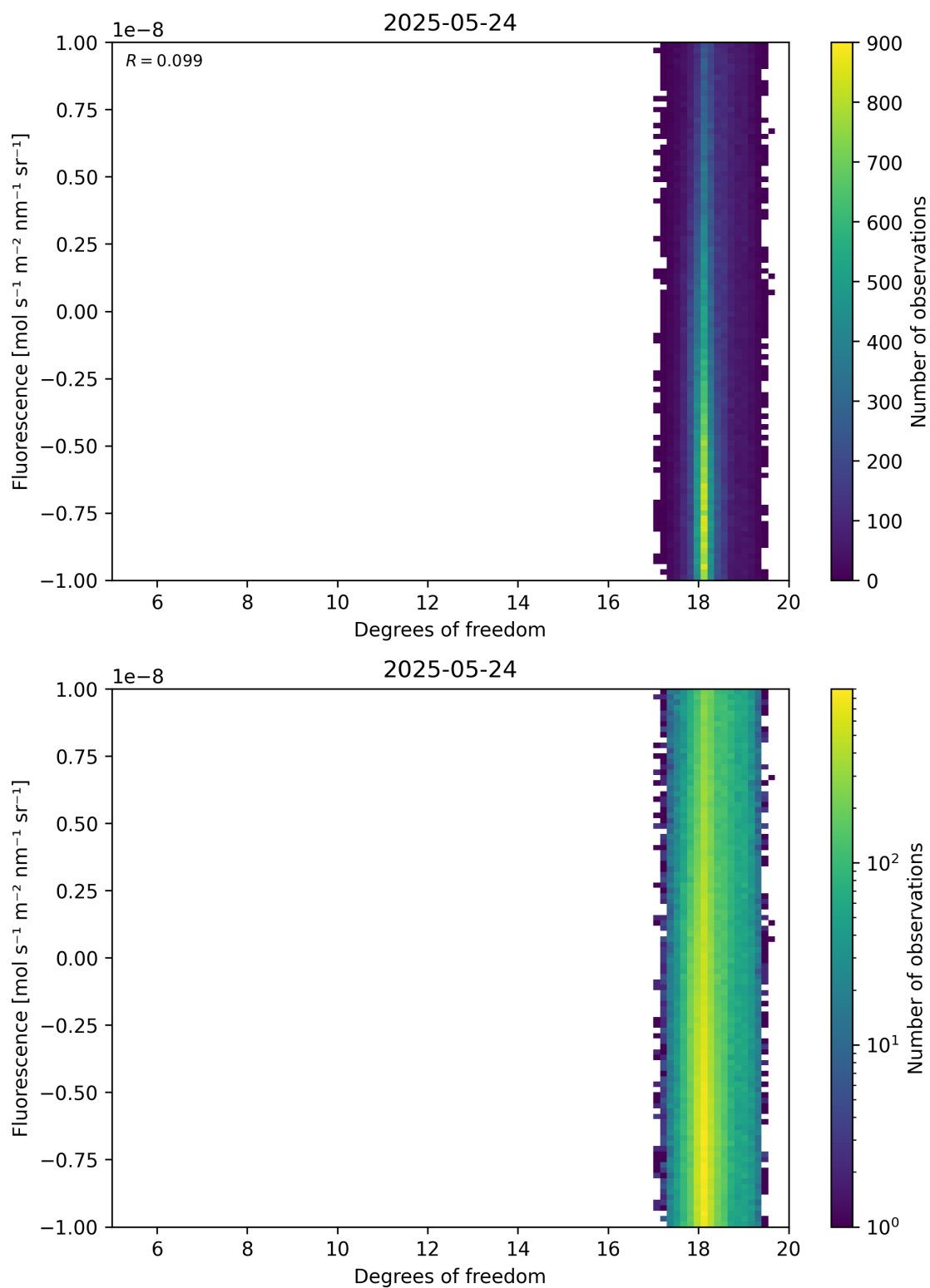
Figure 51: Scatter density plot of “Degrees of freedom” against “Fluorescence” for 2025-05-23 to 2025-05-25.
