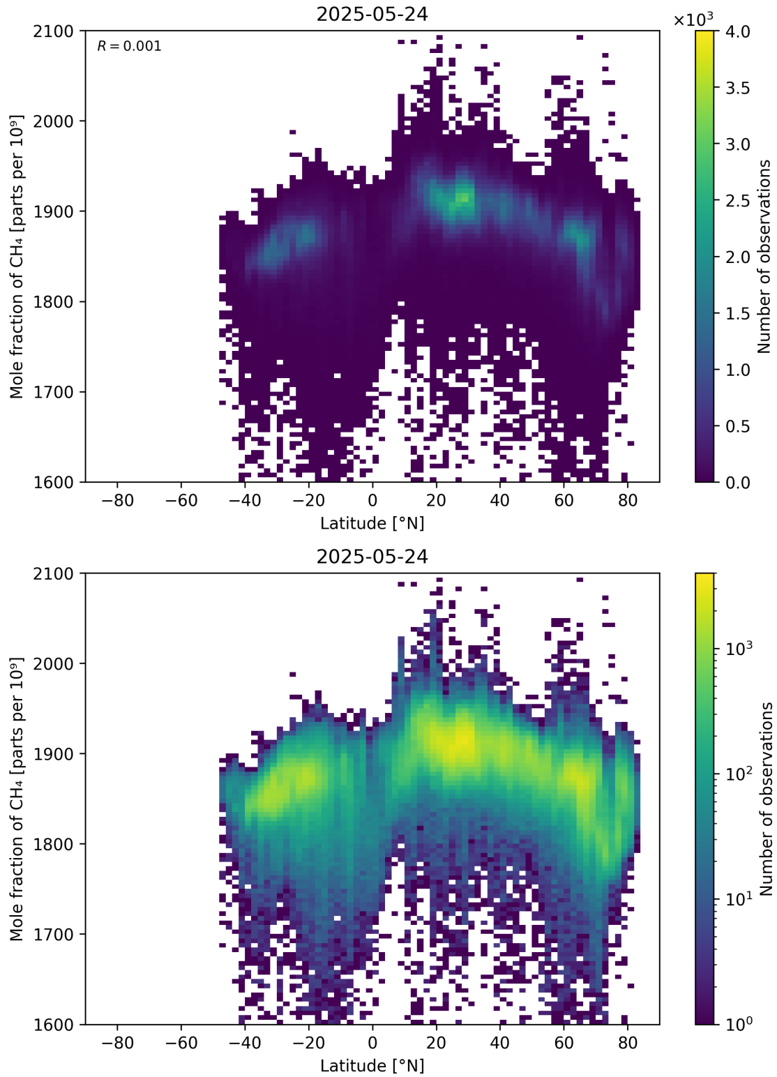
Figure 57: Scatter density plot of “Latitude” against “Mole fraction of \text{CH}_4 ” for 2025-05-23 to 2025-05-25.
