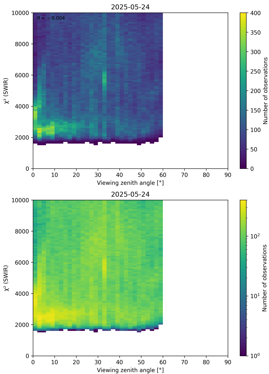
Figure 106: Scatter density plot of “Viewing zenith angle” against “ \chi^2 (SWIR)” for 2025-05-23 to 2025-05-25.
