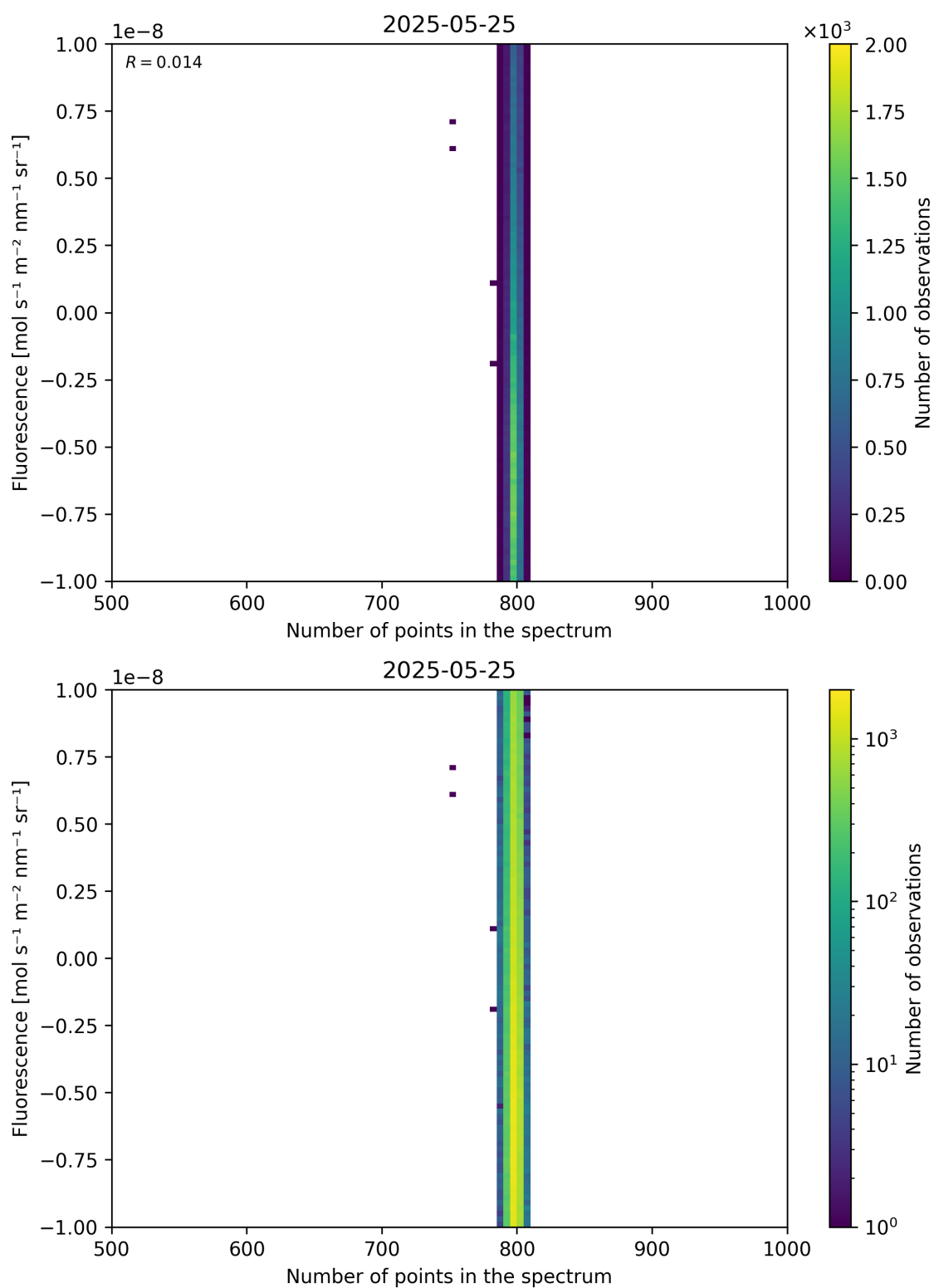
Figure 91: Scatter density plot of “Number of points in the spectrum” against “Fluorescence” for 2025-05-24 to 2025-05-26.
