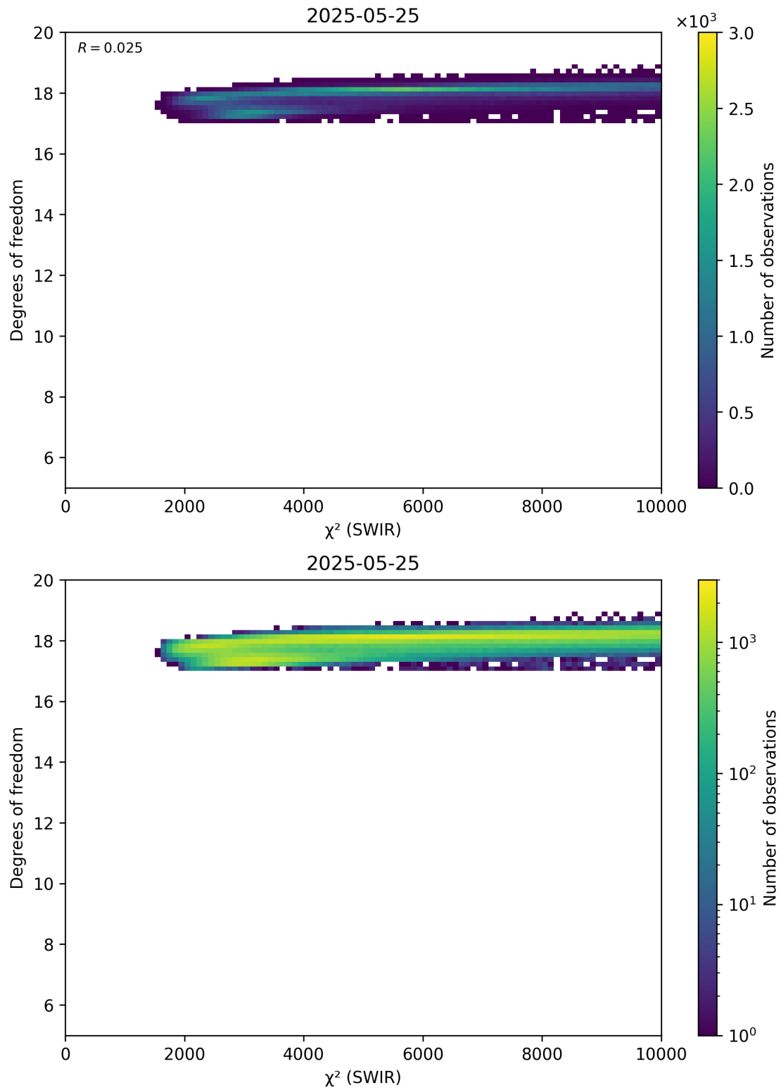
Figure 48: Scatter density plot of “ \chi^2 (SWIR)” against “Degrees of freedom” for 2025-05-24 to 2025-05-26.
