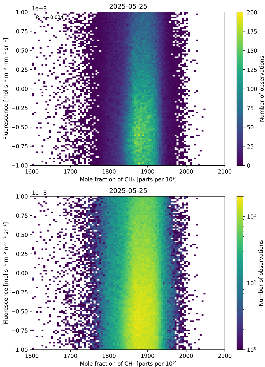
Figure 73: Scatter density plot of “Mole fraction of CH 4 ” against “Fluorescence” for 2025-05-24 to 2025-05-26.
