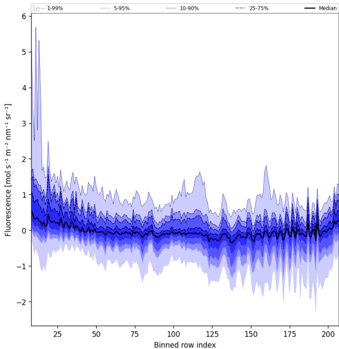
Figure 43: Along track statistics of "Fluorescence" for 2025-05-24 to 2025-05-26
