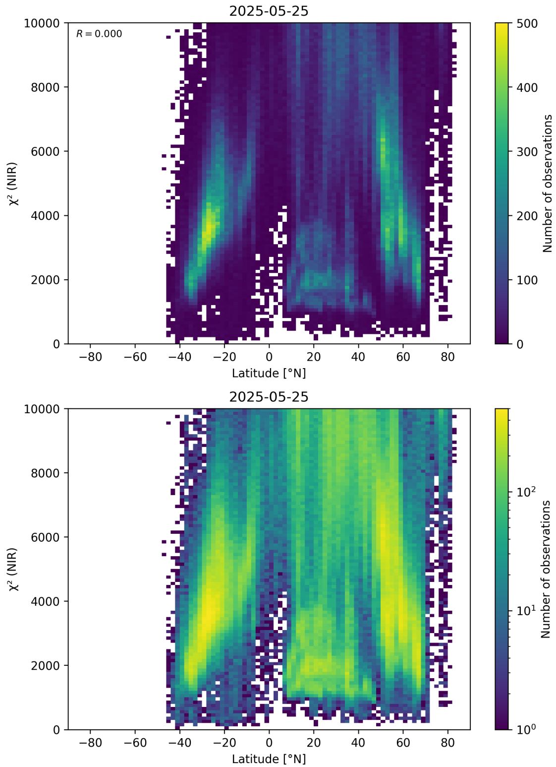
Figure 53: Scatter density plot of “Latitude” against “ \chi^2 (NIR)” for 2025-05-24 to 2025-05-26.
