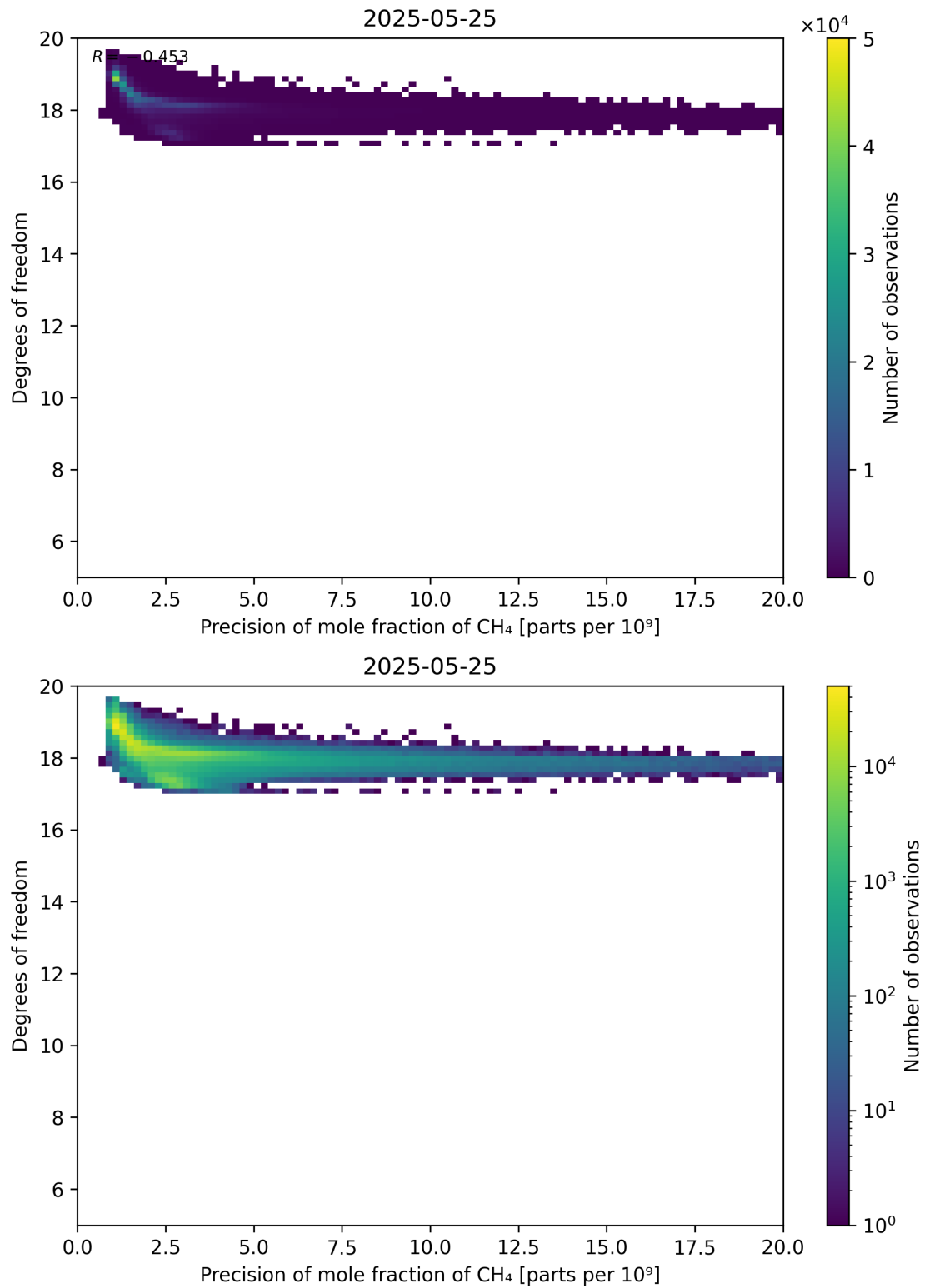
Figure 80: Scatter density plot of “Precision of mole fraction of CH 4 ” against “Degrees of freedom” for 2025-05-24 to 2025-05-26.
