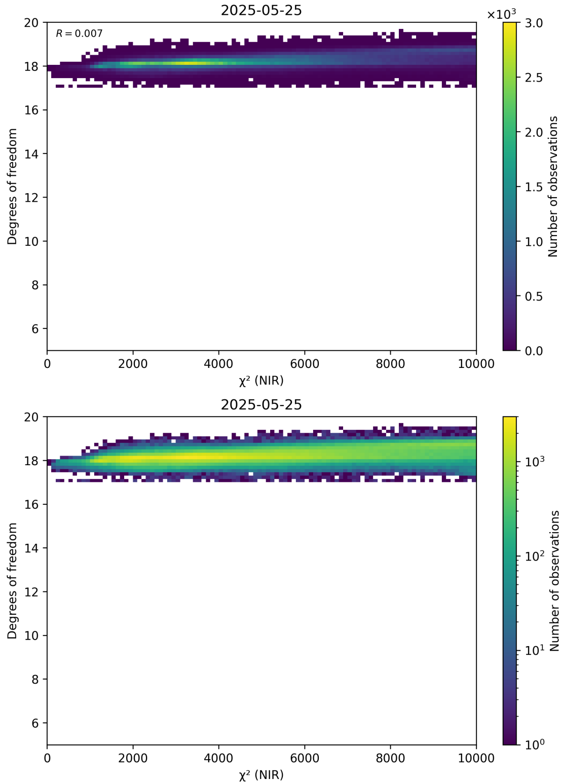
Figure 44: Scatter density plot of “ \chi^2 (NIR)” against “Degrees of freedom” for 2025-05-24 to 2025-05-26.
