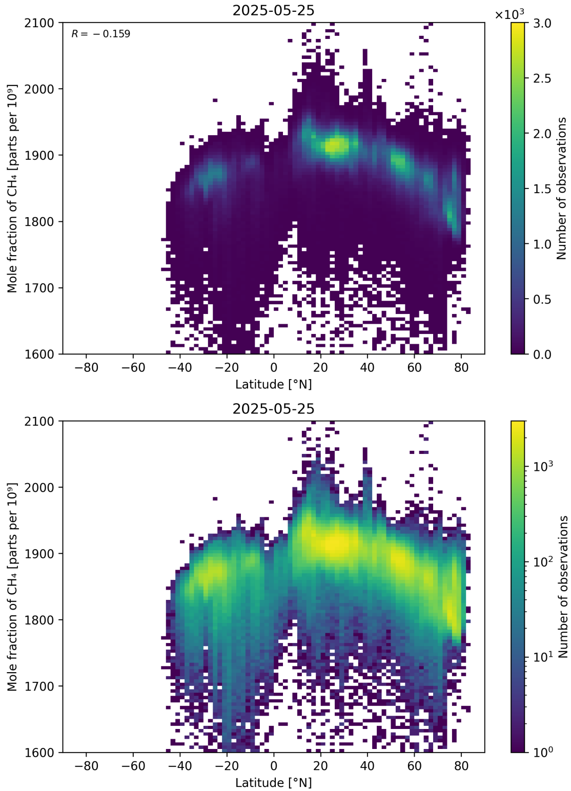
Figure 57: Scatter density plot of “Latitude” against “Mole fraction of \text{CH}_4 ” for 2025-05-24 to 2025-05-26.
