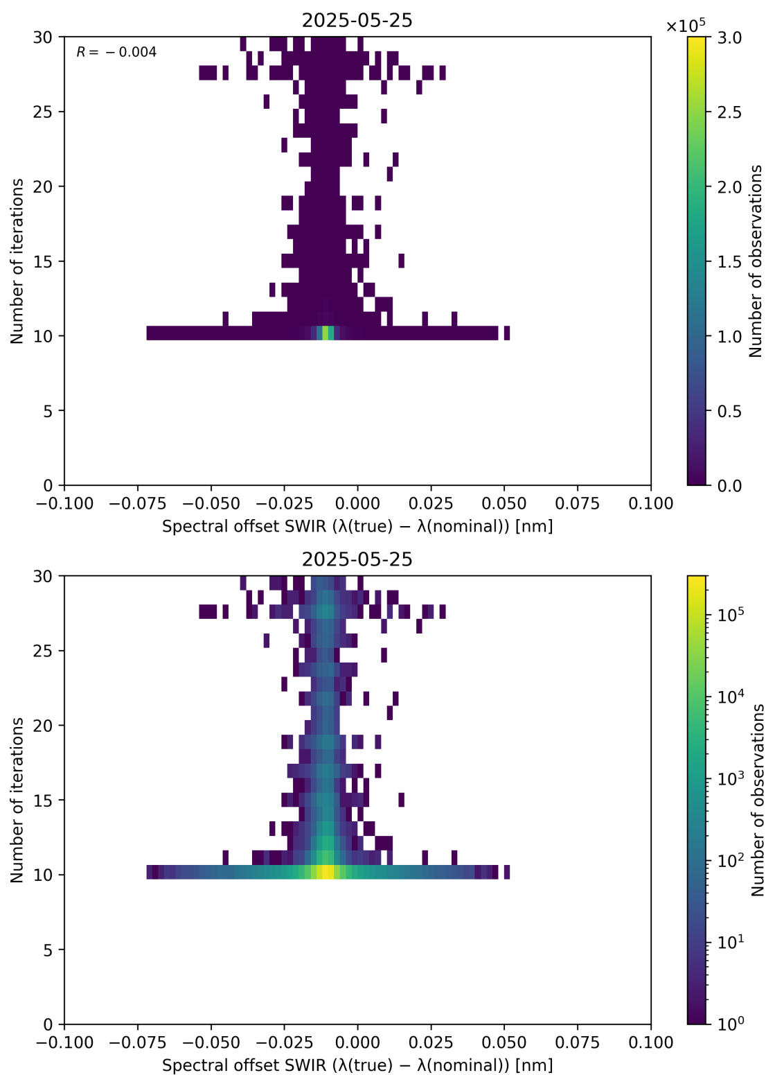
Figure 121: Scatter density plot of “Spectral offset SWIR ( \lambda_{\text{true}} - \lambda_{\text{nominal}} )” against “Number of iterations” for 2025-05-24 to 2025-05-26.
