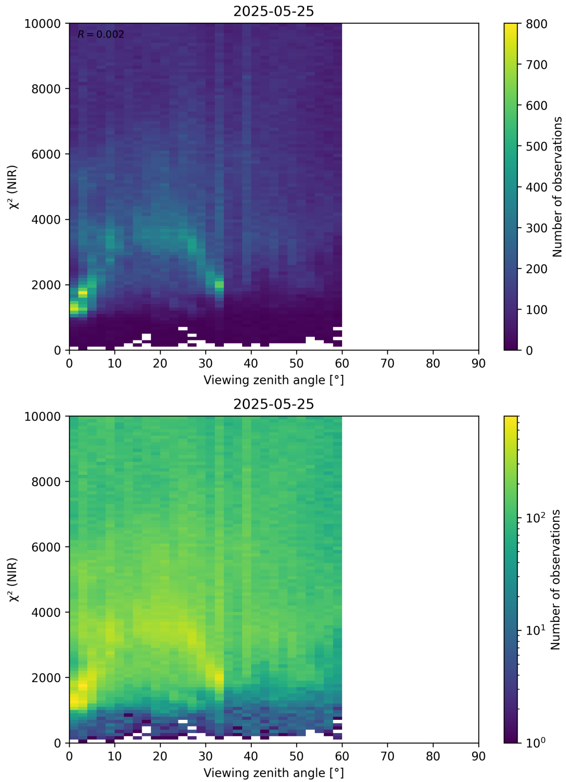
Figure 105: Scatter density plot of “Viewing zenith angle” against “ \chi^2 (NIR)” for 2025-05-24 to 2025-05-26.
