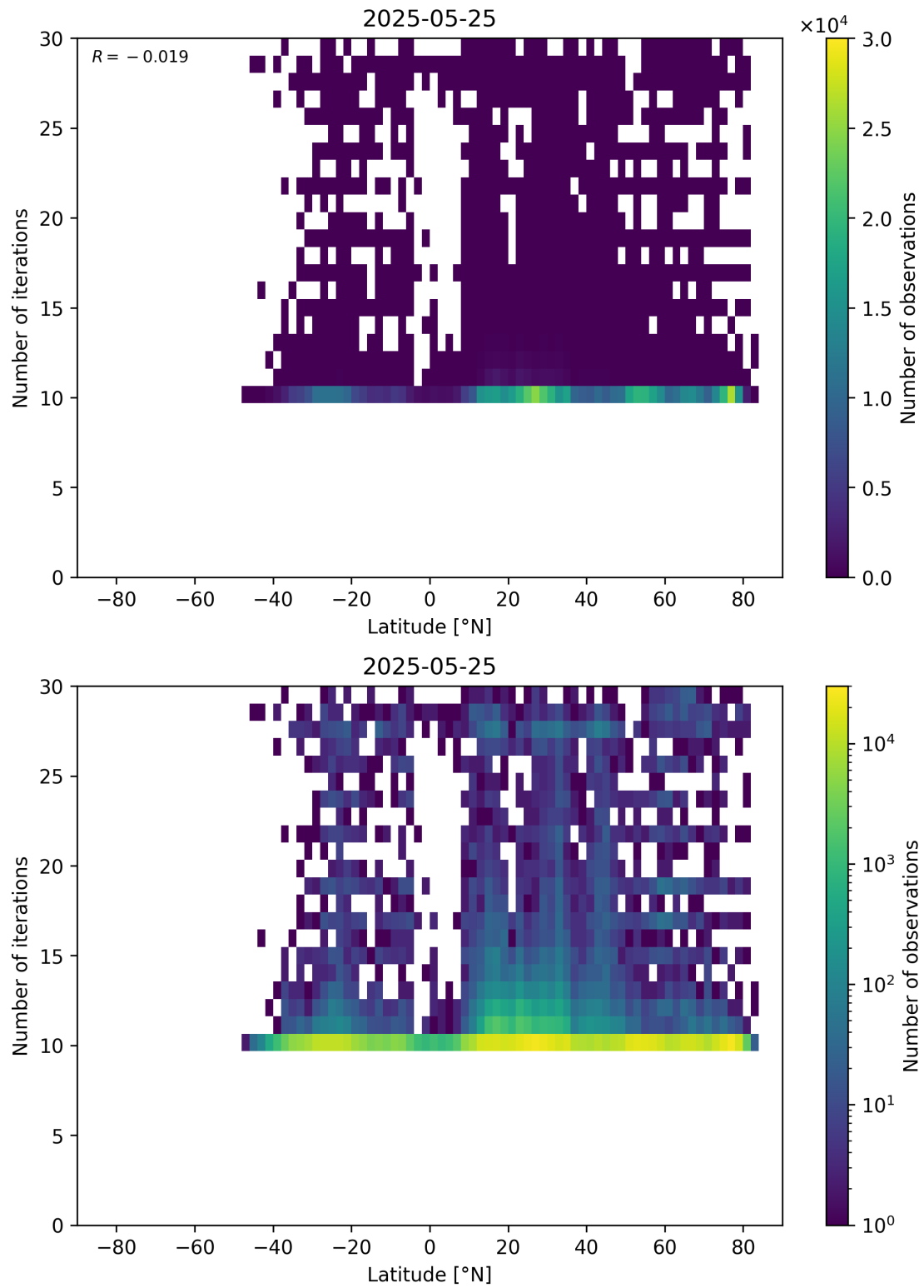
Figure 60: Scatter density plot of “Latitude” against “Number of iterations” for 2025-05-24 to 2025-05-26.
