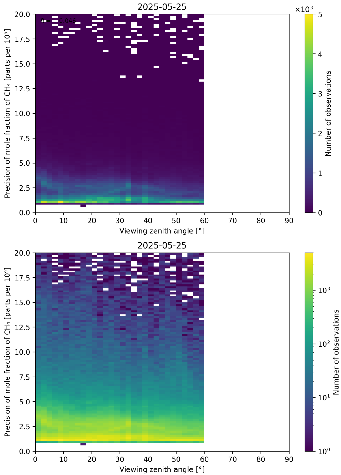
Figure 112: Scatter density plot of “Viewing zenith angle” against “Precision of mole fraction of CH 4 ” for 2025-05-24 to 2025-05-26.
