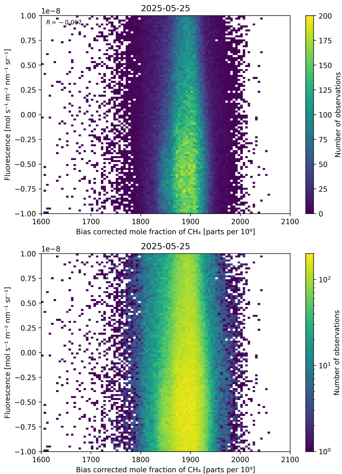
Figure 66: Scatter density plot of “Bias corrected mole fraction of \text{CH}_4 ” against “Fluorescence” for 2025-05-24 to 2025-05-26.
