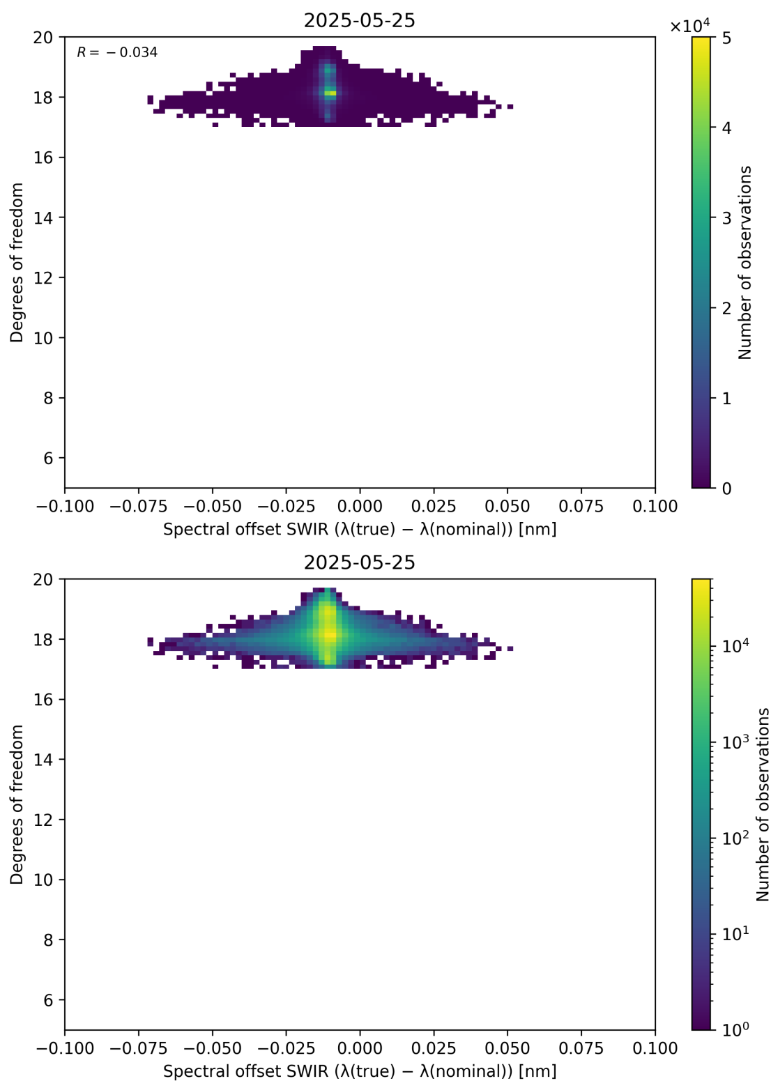
Figure 119: Scatter density plot of “Spectral offset SWIR ( \lambda_{\text{true}} - \lambda_{\text{nominal}} )” against “Degrees of freedom” for 2025-05-24 to 2025-05-26.
