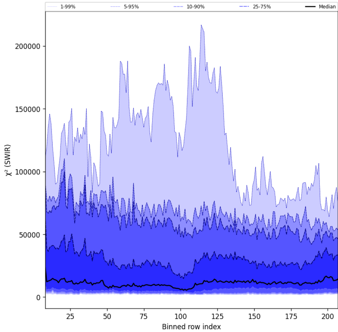
Figure 39: Along track statistics of “ \chi^2 (SWIR)” for 2025-05-24 to 2025-05-26
