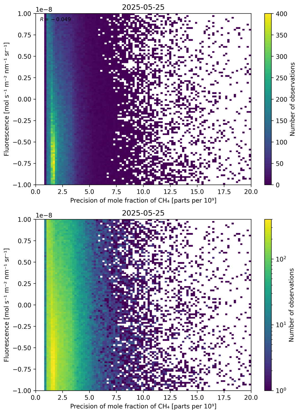
Figure 81: Scatter density plot of “Precision of mole fraction of \text{CH}_4 ” against “Fluorescence” for 2025-05-24 to 2025-05-26.
