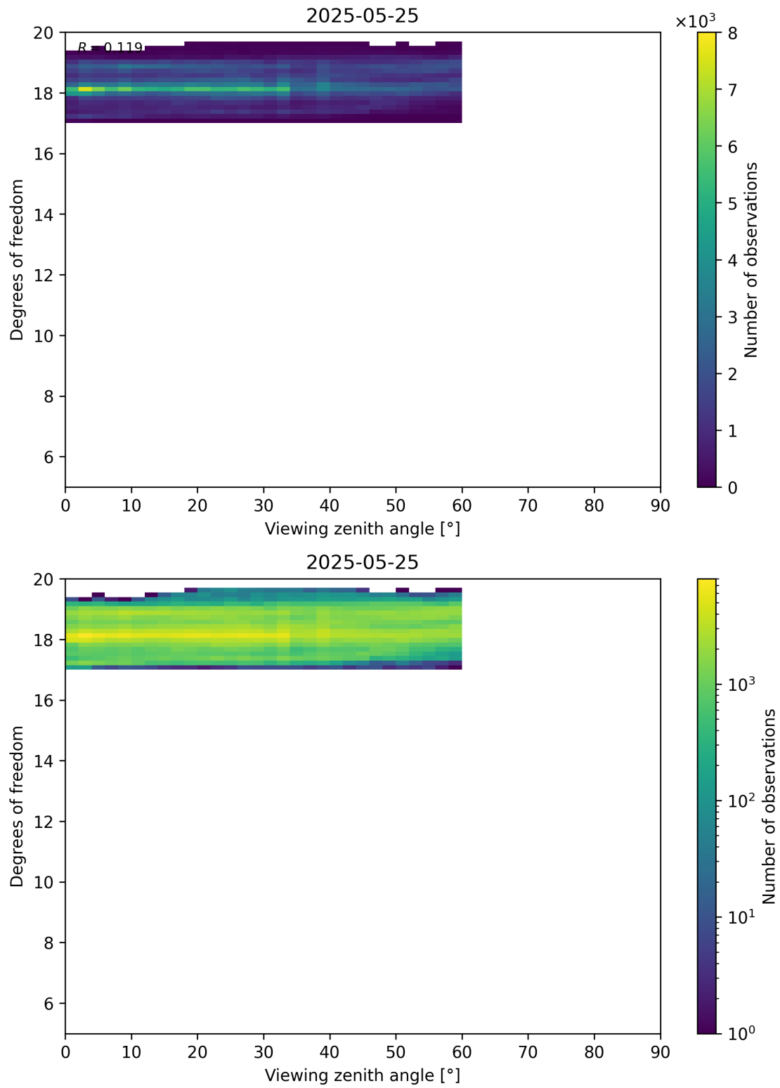
Figure 107: Scatter density plot of “Viewing zenith angle” against “Degrees of freedom” for 2025-05-24 to 2025-05-26.
