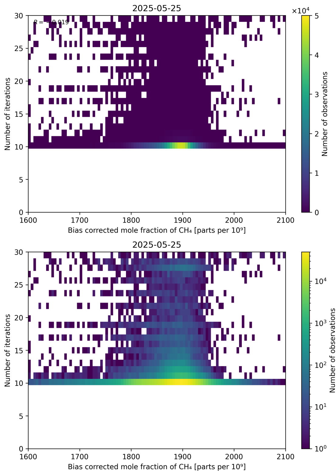
Figure 67: Scatter density plot of “Bias corrected mole fraction of \text{CH}_4 ” against “Number of iterations” for 2025-05-24 to 2025-05-26.
