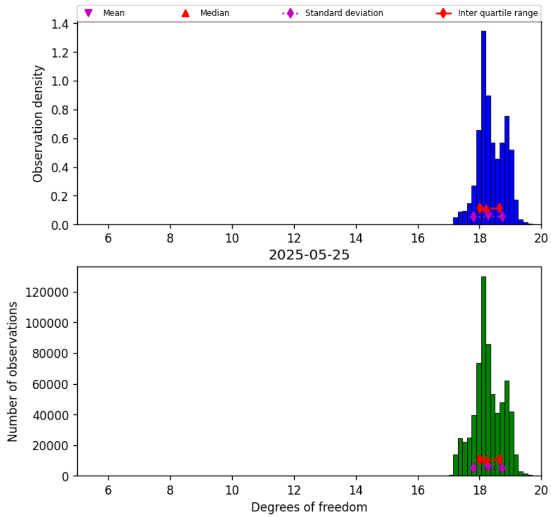
Figure 30: Histogram of “Degrees of freedom” for 2025-05-24 to 2025-05-26
