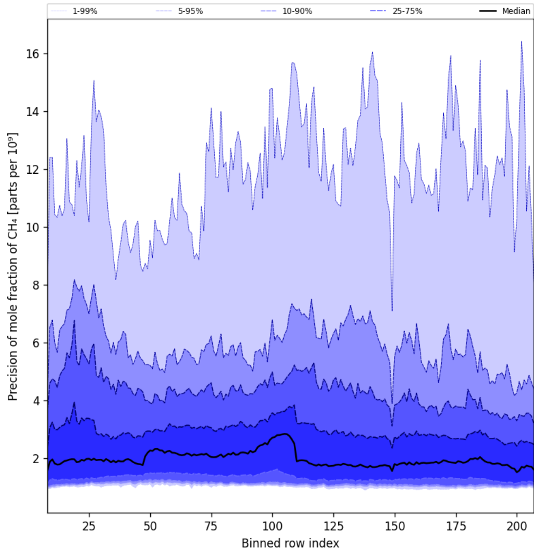
Figure 35: Along track statistics of “Precision of mole fraction of CH 4 ” for 2025-05-24 to 2025-05-26
