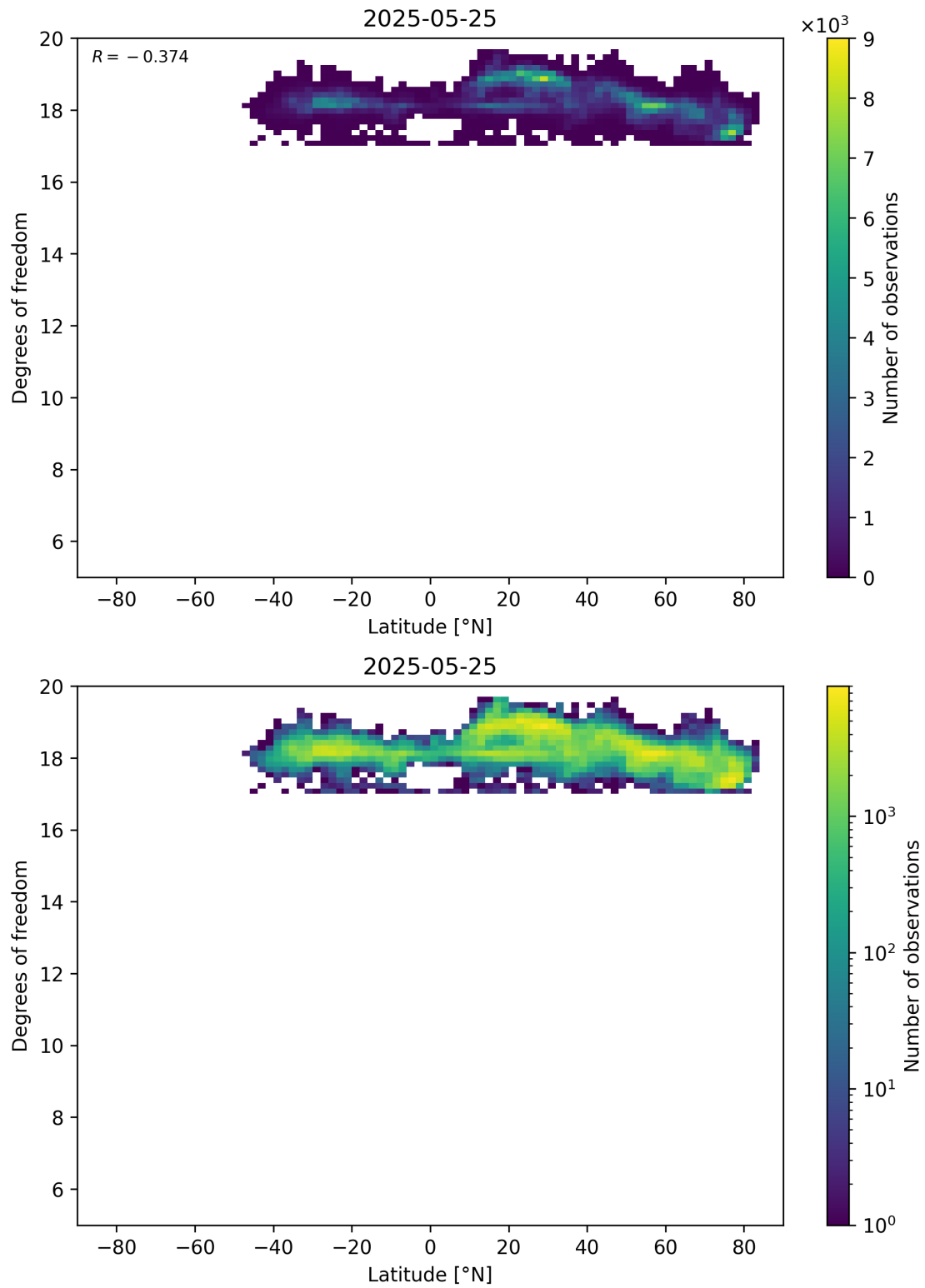
Figure 55: Scatter density plot of “Latitude” against “Degrees of freedom” for 2025-05-24 to 2025-05-26.
