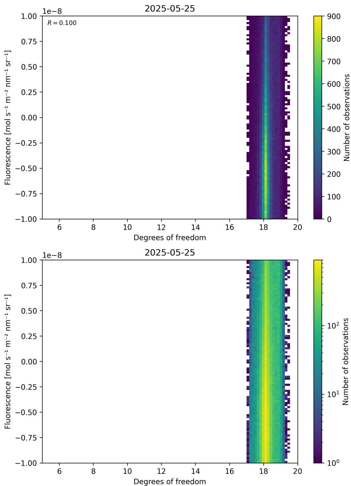
Figure 51: Scatter density plot of “Degrees of freedom” against “Fluorescence” for 2025-05-24 to 2025-05-26.
