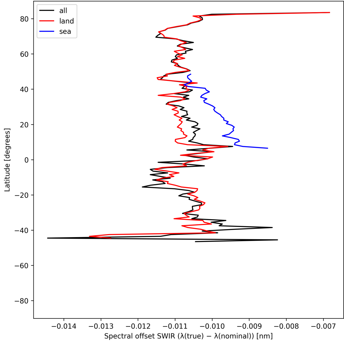
Figure 16: Zonal average of “Spectral offset SWIR ( \lambda_{\text{true}} - \lambda_{\text{nominal}} )” for 2025-05-24 to 2025-05-26.
