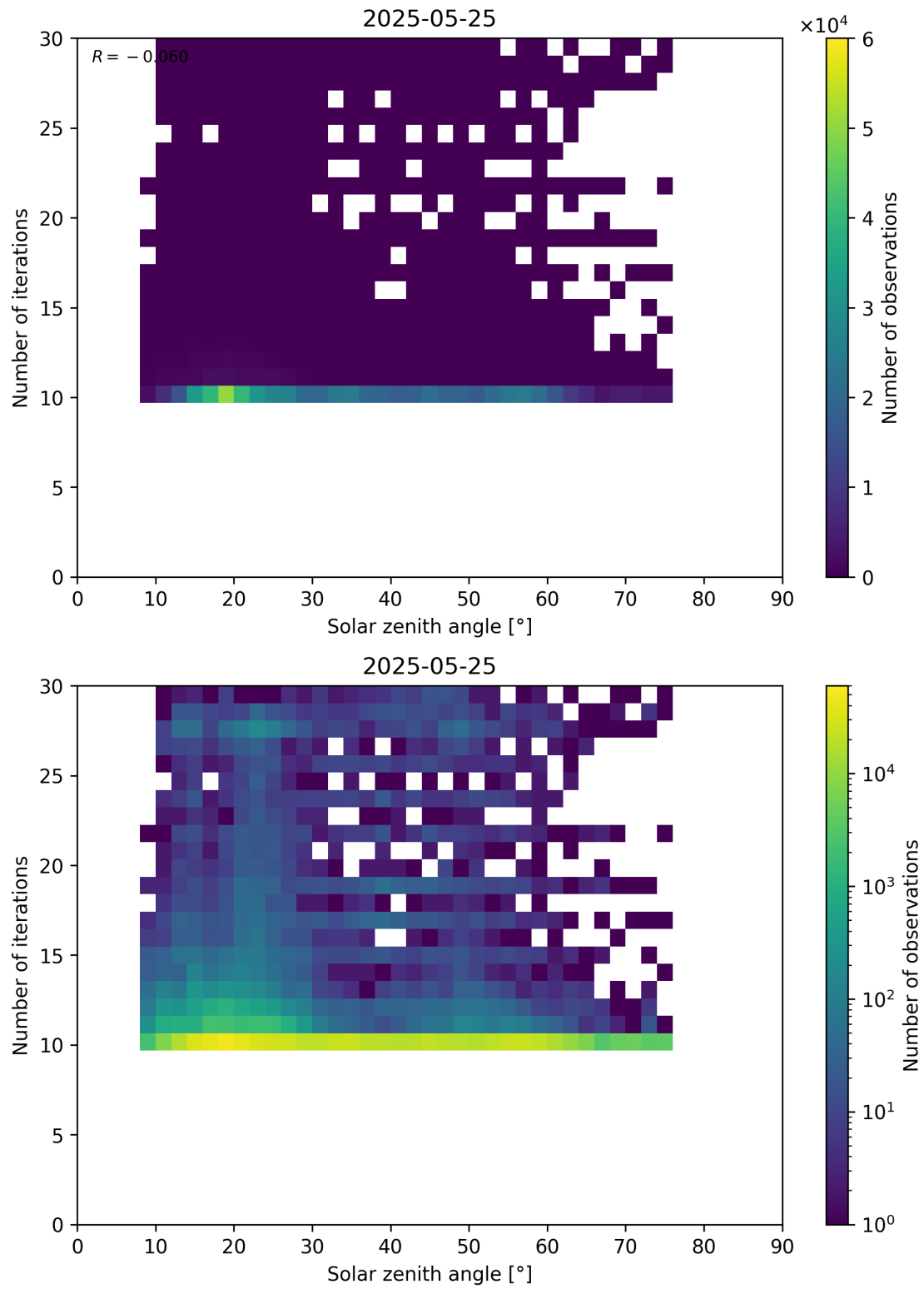
Figure 102: Scatter density plot of “Solar zenith angle” against “Number of iterations” for 2025-05-24 to 2025-05-26.
