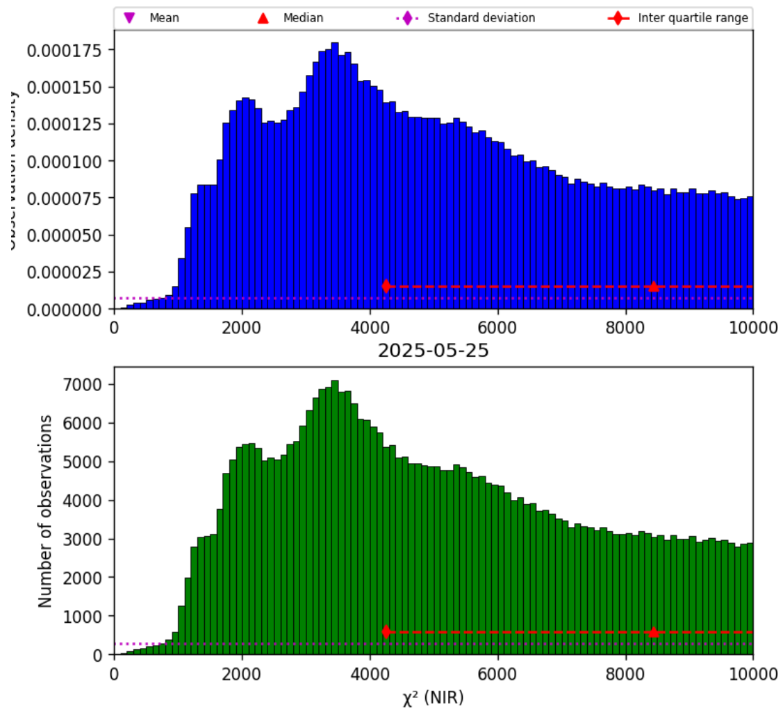
Figure 29: Histogram of “ \chi^2 (NIR)” for 2025-05-24 to 2025-05-26
