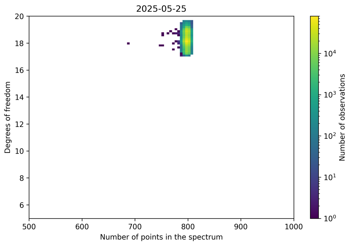
Figure 90: Scatter density plot of “Number of points in the spectrum” against “Degrees of freedom” for 2025-05-24 to 2025-05-26.
