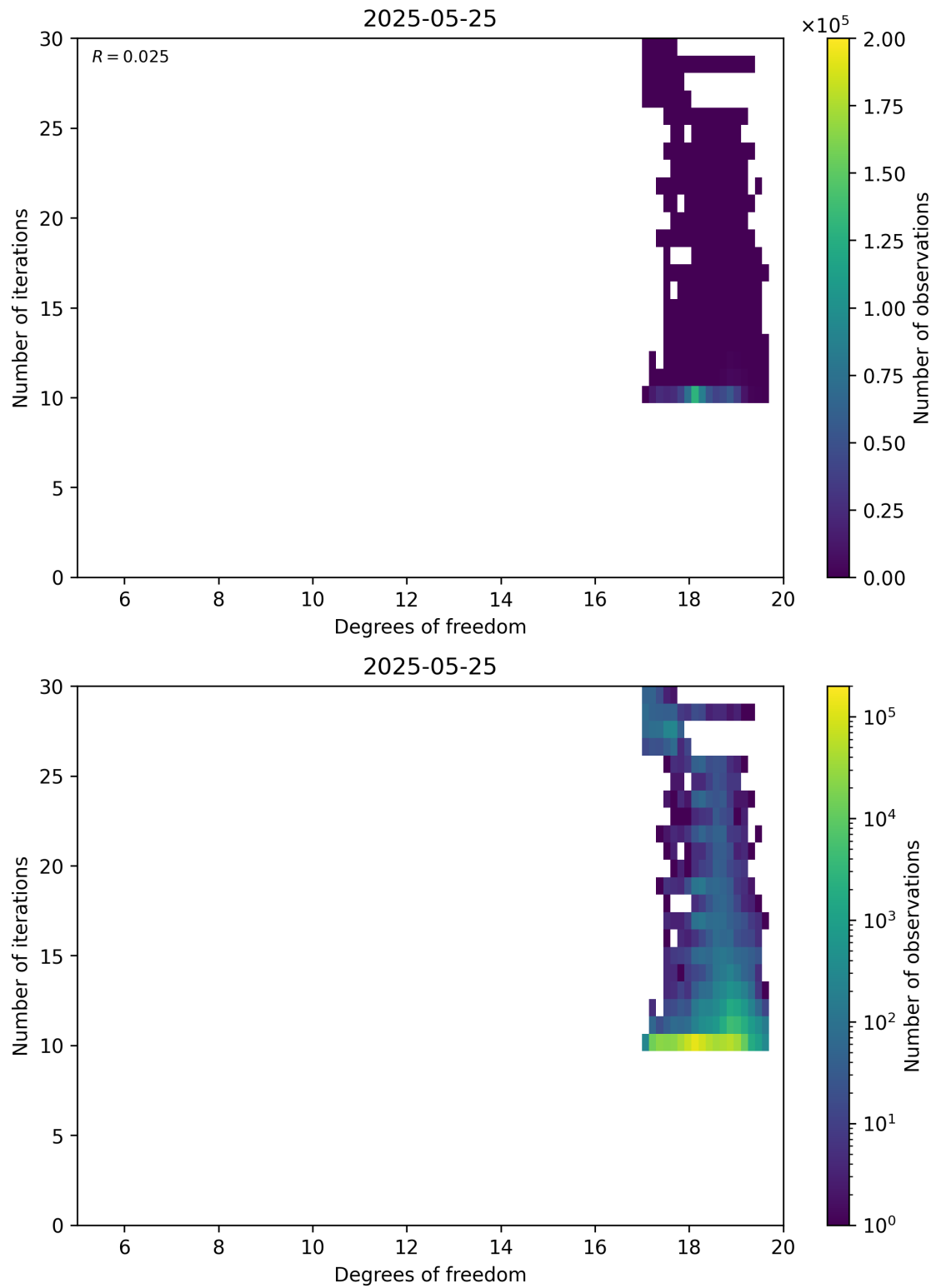
Figure 52: Scatter density plot of “Degrees of freedom” against “Number of iterations” for 2025-05-24 to 2025-05-26.
