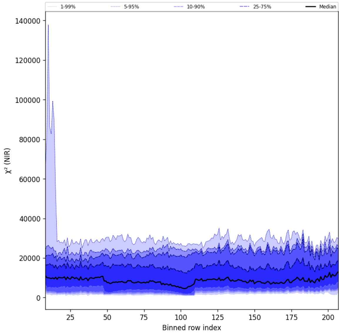
Figure 40: Along track statistics of “ \chi^2 (NIR)” for 2025-05-24 to 2025-05-26
