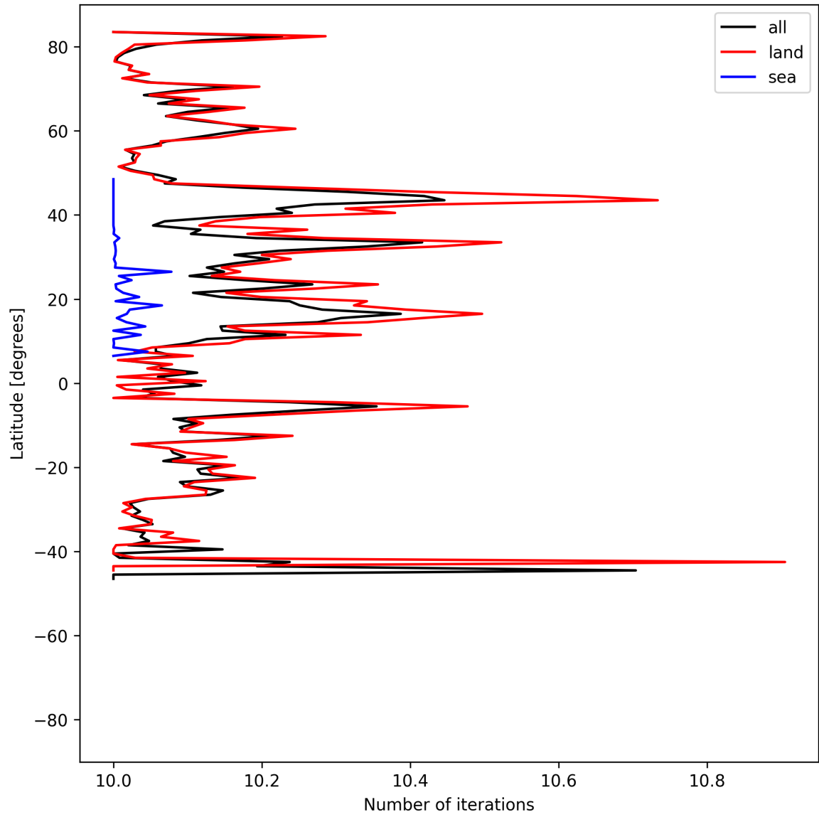
Figure 20: Zonal average of “Number of iterations” for 2025-05-24 to 2025-05-26.
