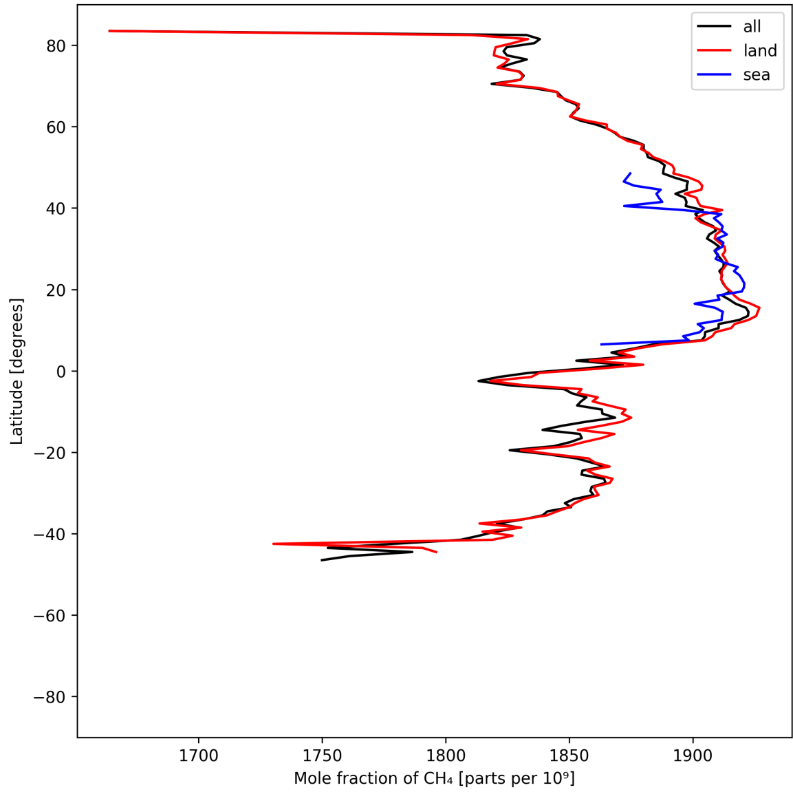
Figure 12: Zonal average of “Mole fraction of CH 4 ” for 2025-05-24 to 2025-05-26.
