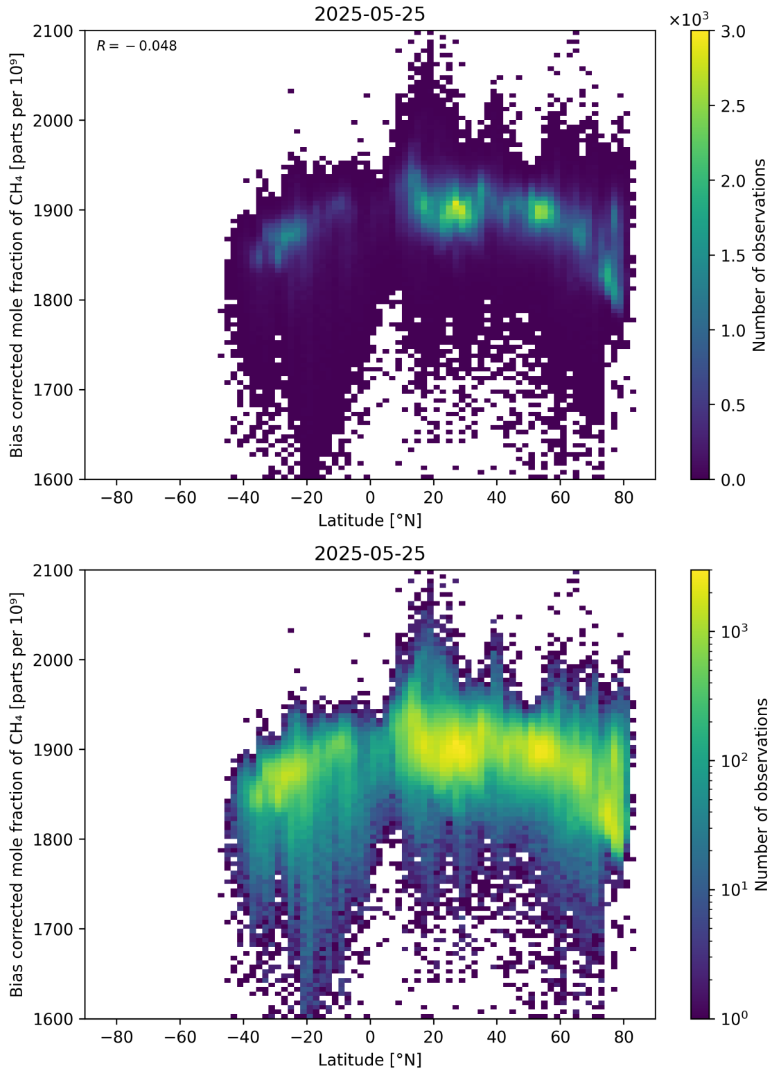
Figure 58: Scatter density plot of “Latitude” against “Bias corrected mole fraction of CH 4 ” for 2025-05-24 to 2025-05-26.
