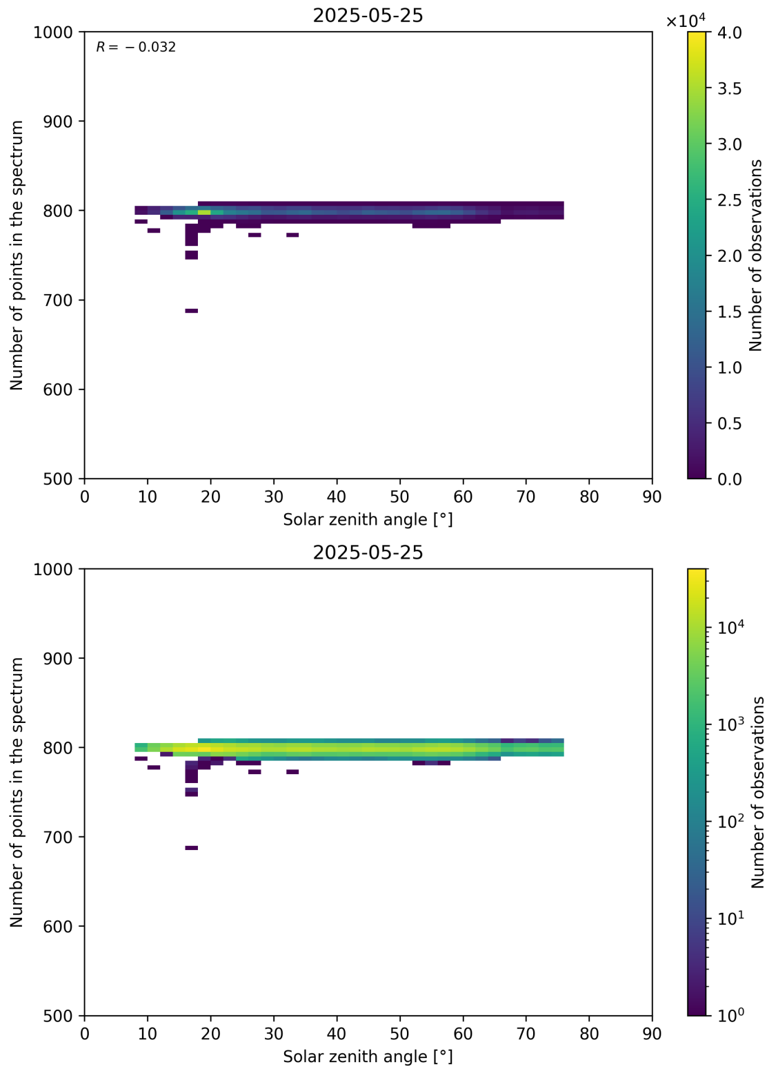
Figure 103: Scatter density plot of “Solar zenith angle” against “Number of points in the spectrum” for 2025-05-24 to 2025-05-26.
