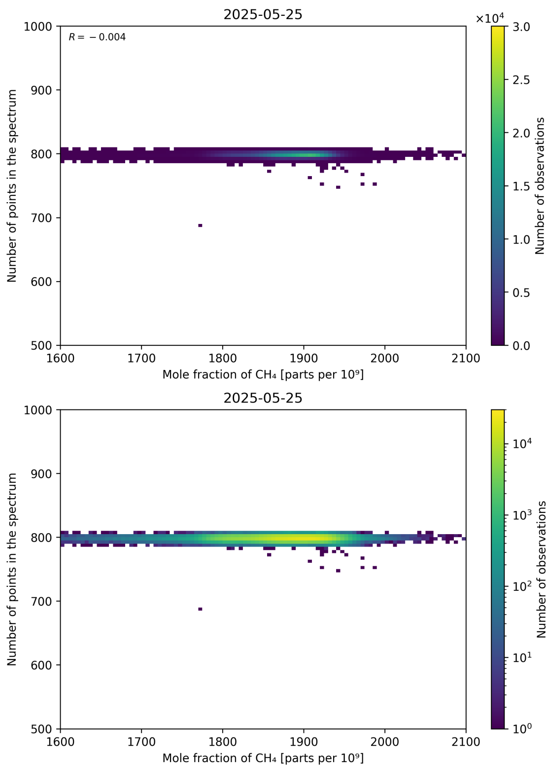
Figure 77: Scatter density plot of “Mole fraction of CH 4 ” against “Number of points in the spectrum” for 2025-05-24 to 2025-05-26.
