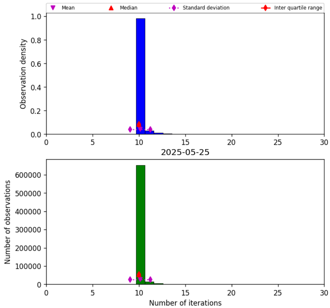
Figure 31: Histogram of “Number of iterations” for 2025-05-24 to 2025-05-26
