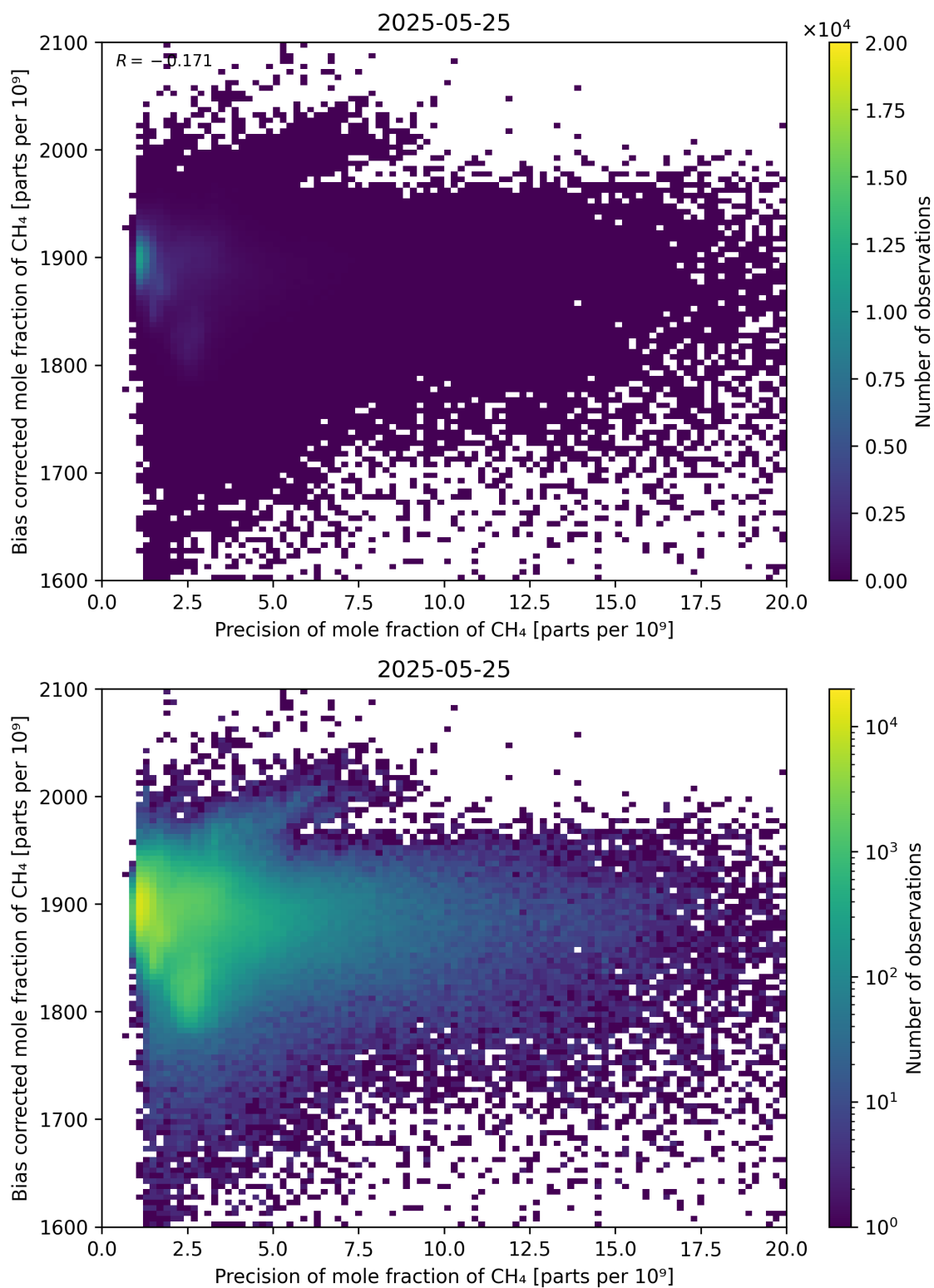
Figure 82: Scatter density plot of “Precision of mole fraction of CH 4 ” against “Bias corrected mole fraction of CH 4 ” for 2025-05-24 to 2025-05-26.
