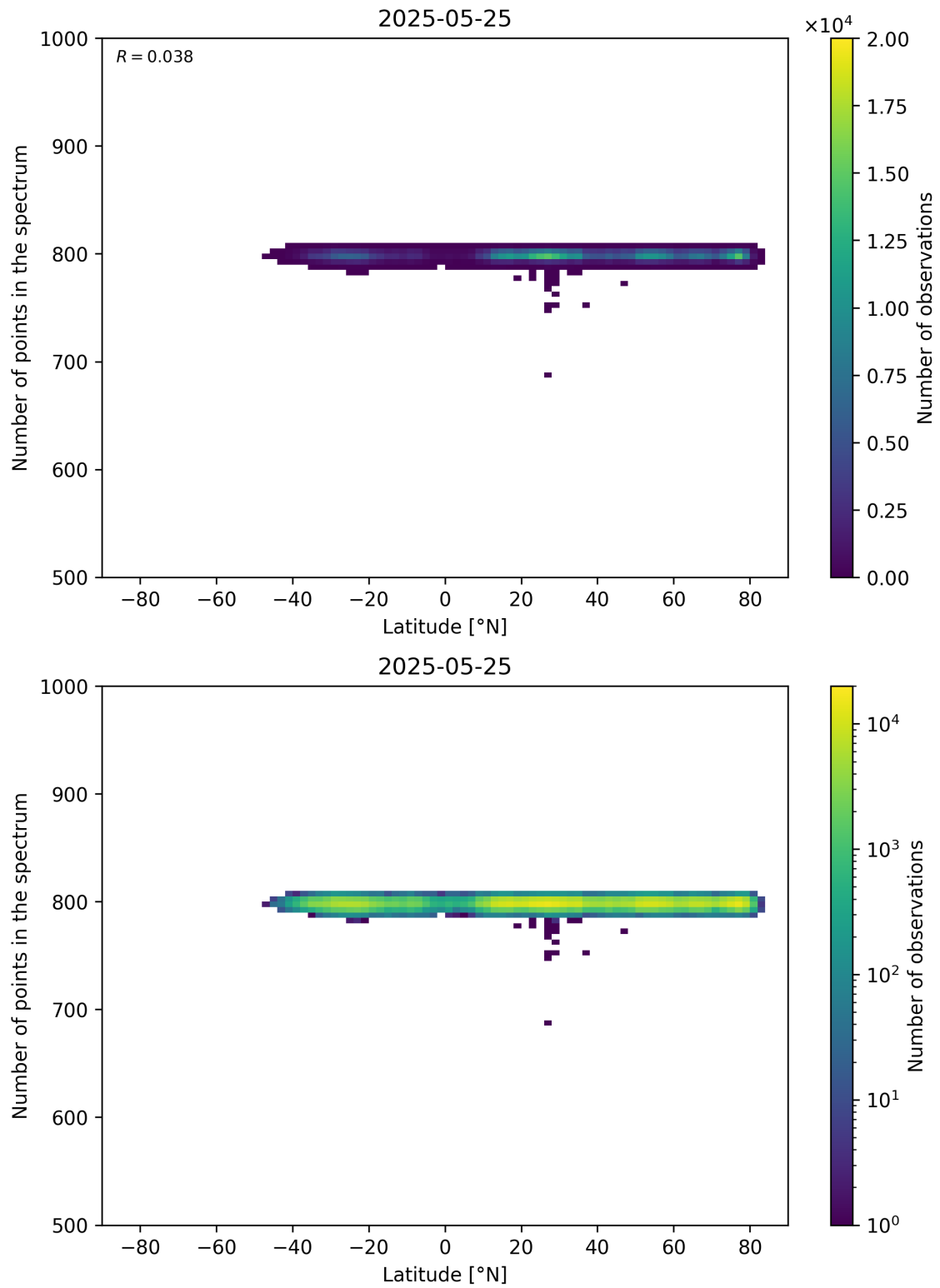
Figure 61: Scatter density plot of “Latitude” against “Number of points in the spectrum” for 2025-05-24 to 2025-05-26.
