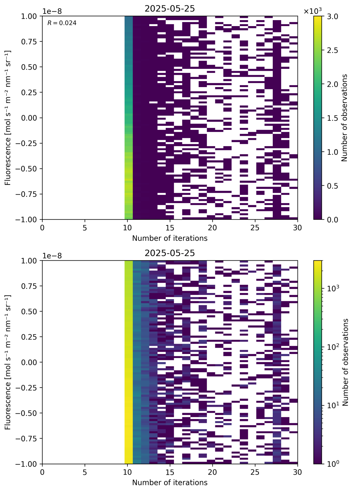
Figure 87: Scatter density plot of "Number of iterations" against "Fluorescence" for 2025-05-24 to 2025-05-26.
