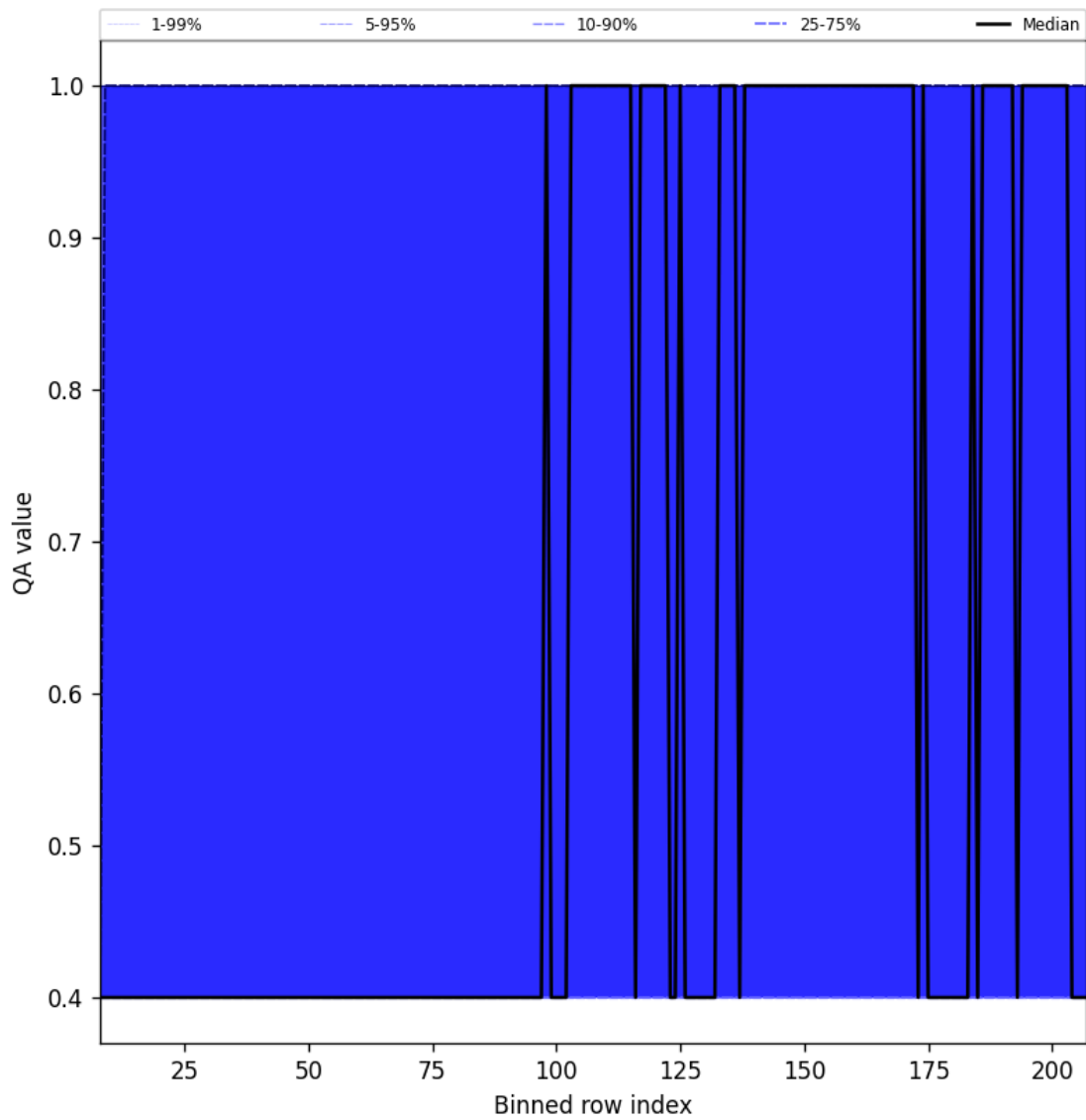
Figure 33: Along track statistics of “QA value” for 2025-05-24 to 2025-05-26
