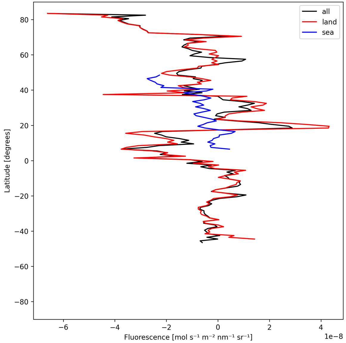
Figure 21: Zonal average of “Fluorescence” for 2025-05-24 to 2025-05-26.
