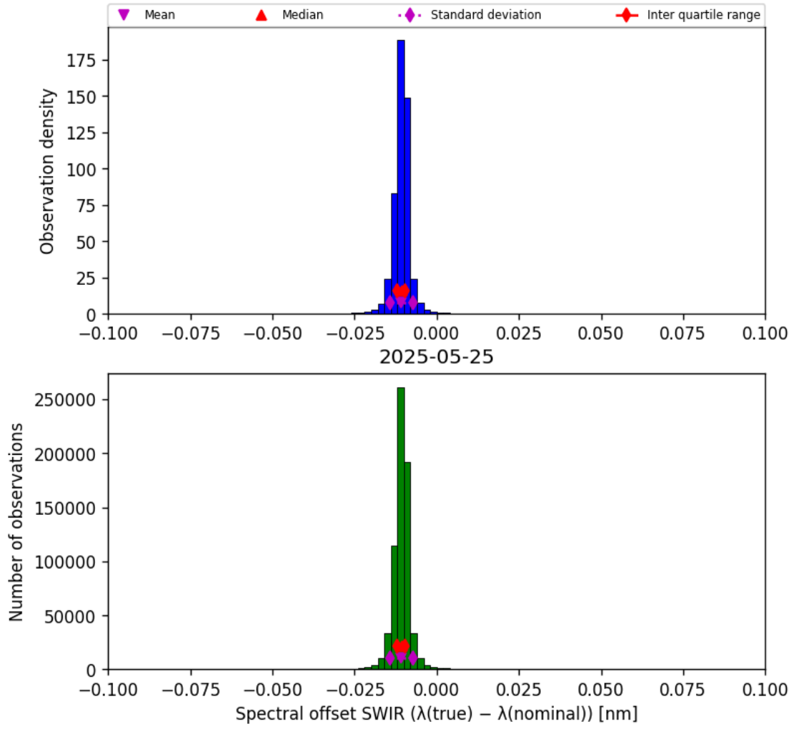
Figure 27: Histogram of “Spectral offset SWIR ( \lambda_{\text{true}} - \lambda_{\text{nominal}} )” for 2025-05-24 to 2025-05-26
