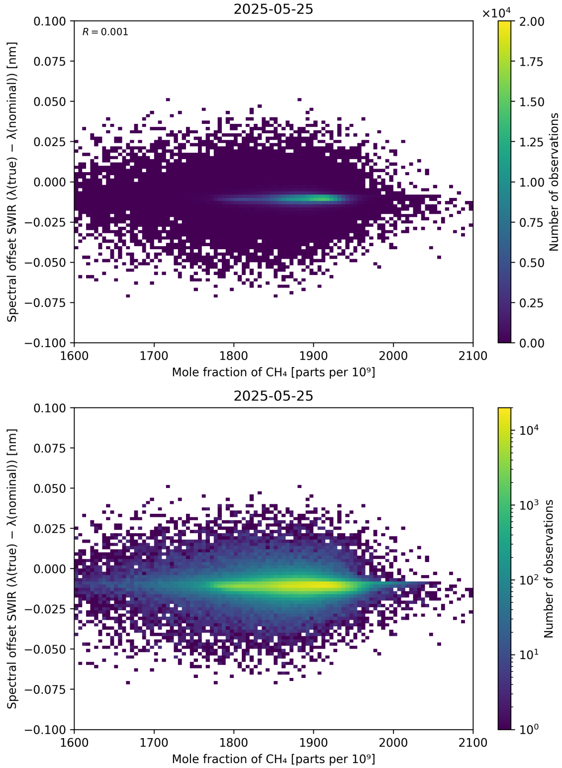
Figure 86: Scatter density plot of “Mole fraction of CH 4 ” against “Spectral offset SWIR ( \lambda_{\text{true}} - \lambda_{\text{nominal}} )” for 2025-05-24 to 2025-05-26.
