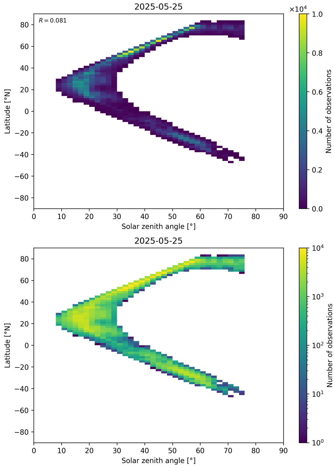
Figure 98: Scatter density plot of “Solar zenith angle” against “Latitude” for 2025-05-24 to 2025-05-26.
