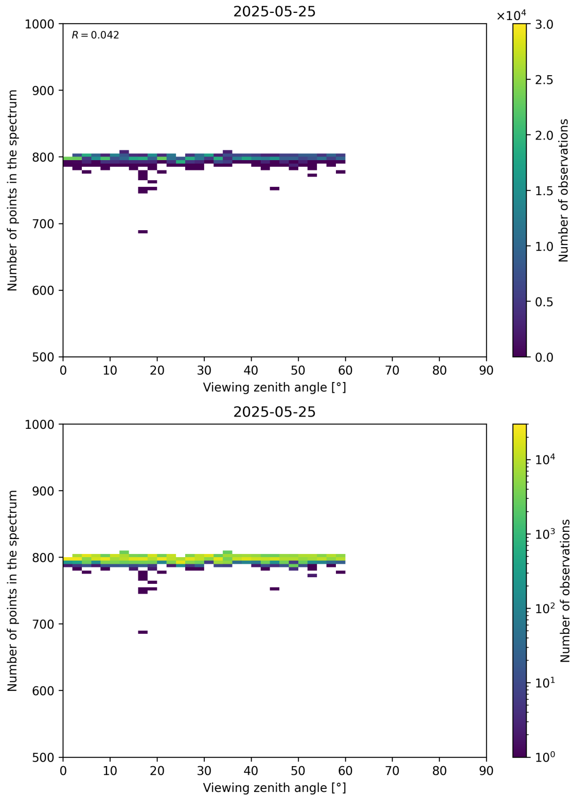
Figure 114: Scatter density plot of “Viewing zenith angle” against “Number of points in the spectrum” for 2025-05-24 to 2025-05-26.
