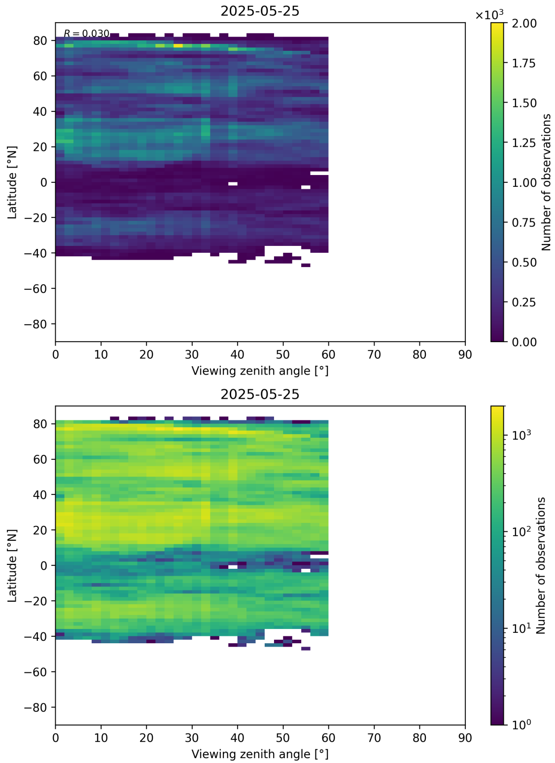
Figure 109: Scatter density plot of “Viewing zenith angle” against “Latitude” for 2025-05-24 to 2025-05-26.
