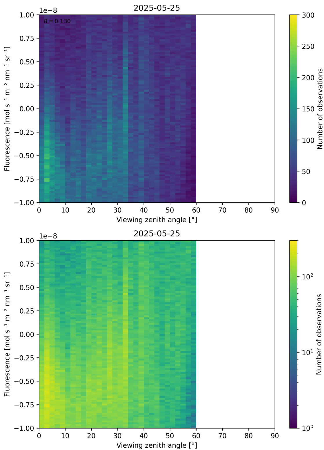
Figure 108: Scatter density plot of “Viewing zenith angle” against “Fluorescence” for 2025-05-24 to 2025-05-26.
