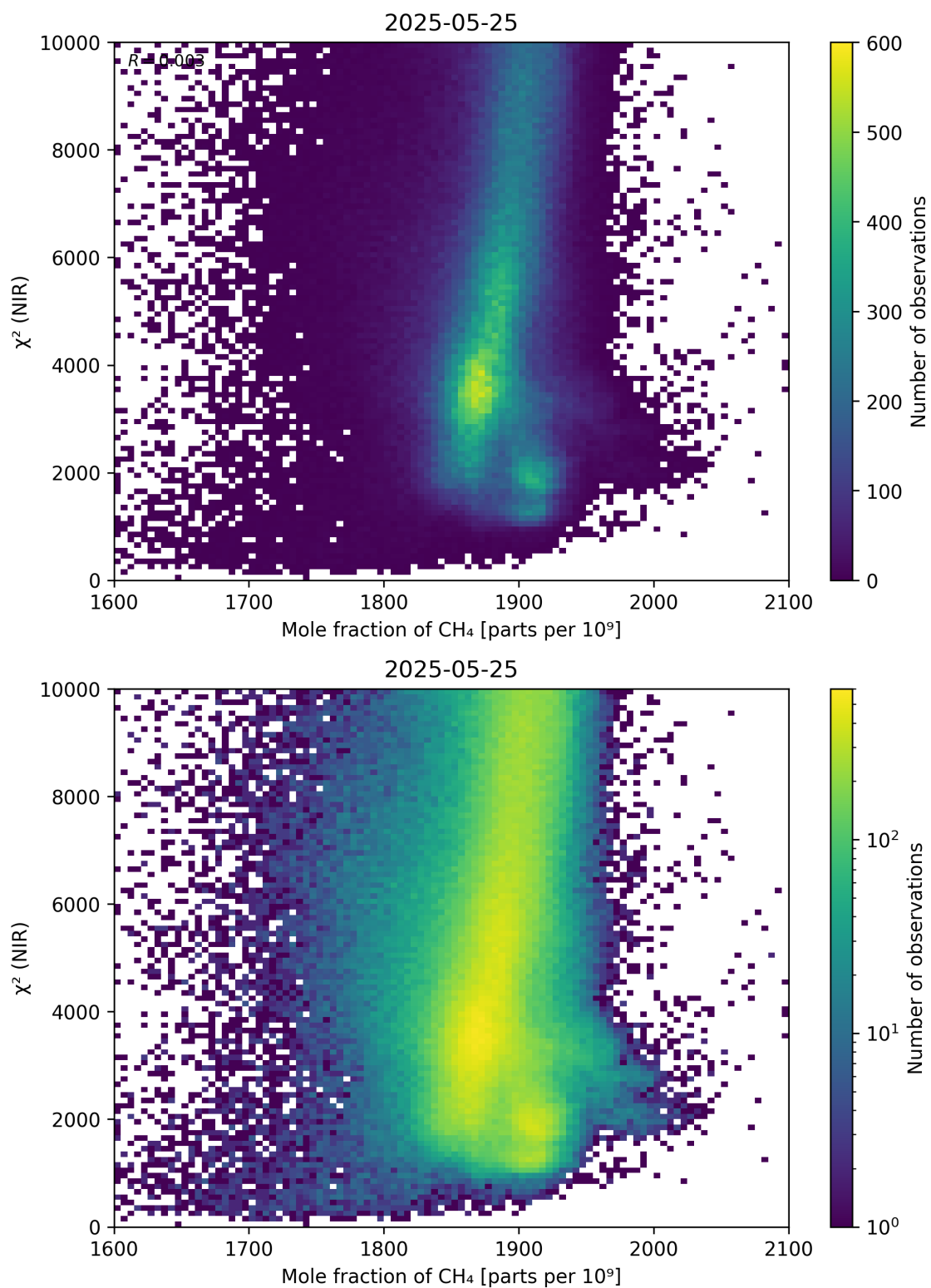
Figure 70: Scatter density plot of “Mole fraction of \text{CH}_4 ” against “ \chi^2 (NIR)” for 2025-05-24 to 2025-05-26.
