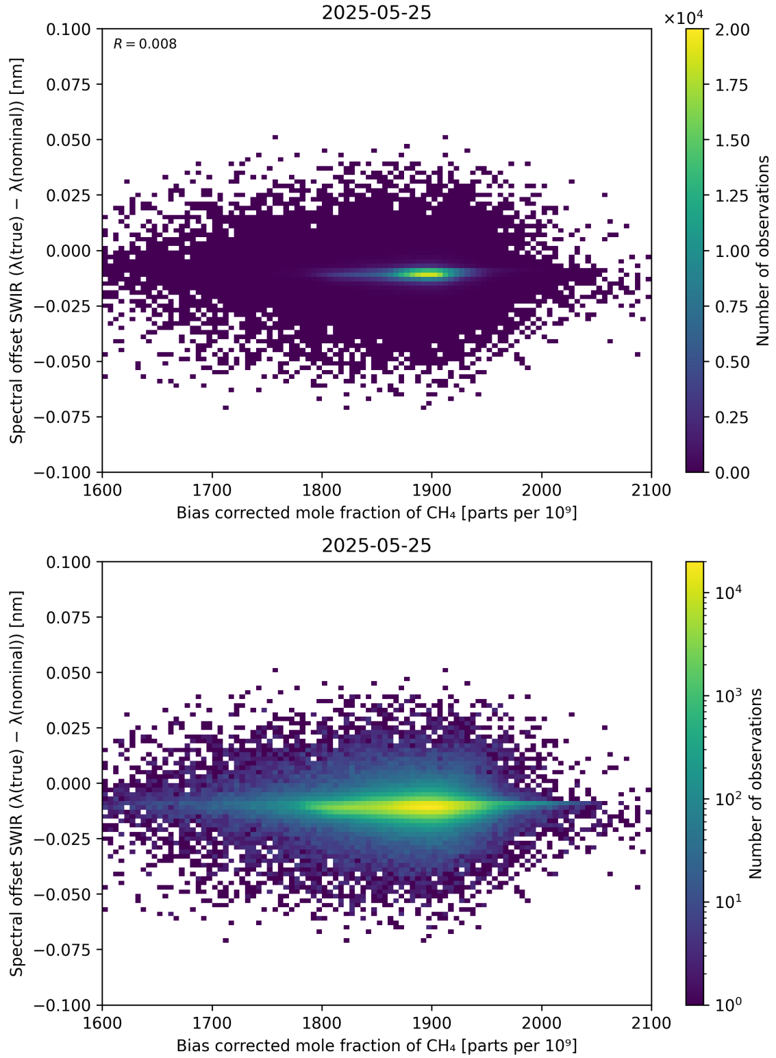
Figure 69: Scatter density plot of “Bias corrected mole fraction of \text{CH}_4 ” against “Spectral offset SWIR ( \lambda_{\text{true}} - \lambda_{\text{nominal}} )” for 2025-05-24 to 2025-05-26.
