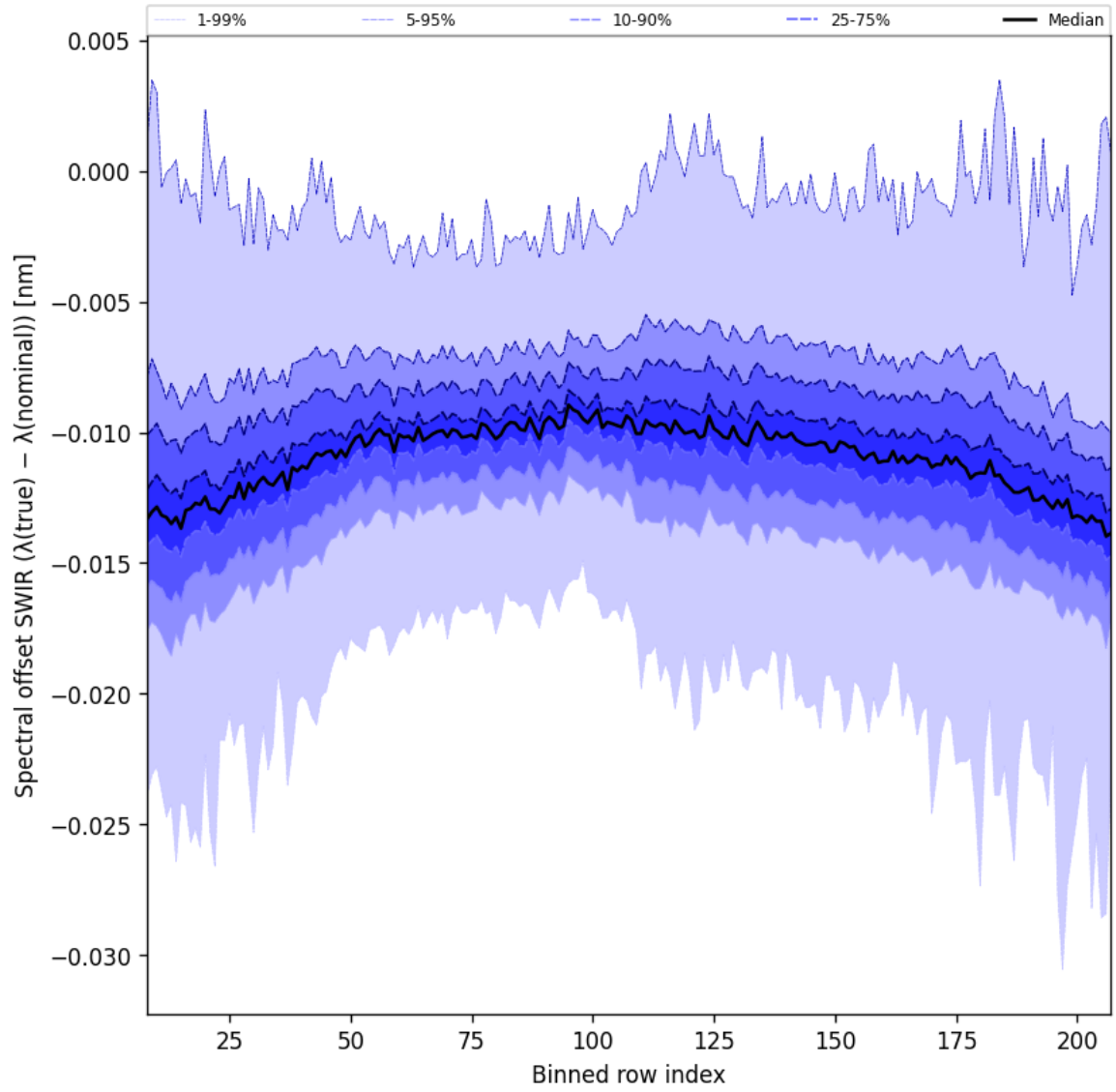
Figure 38: Along track statistics of “Spectral offset SWIR ( \lambda_{\text{true}} - \lambda_{\text{nominal}} )” for 2025-05-24 to 2025-05-26
