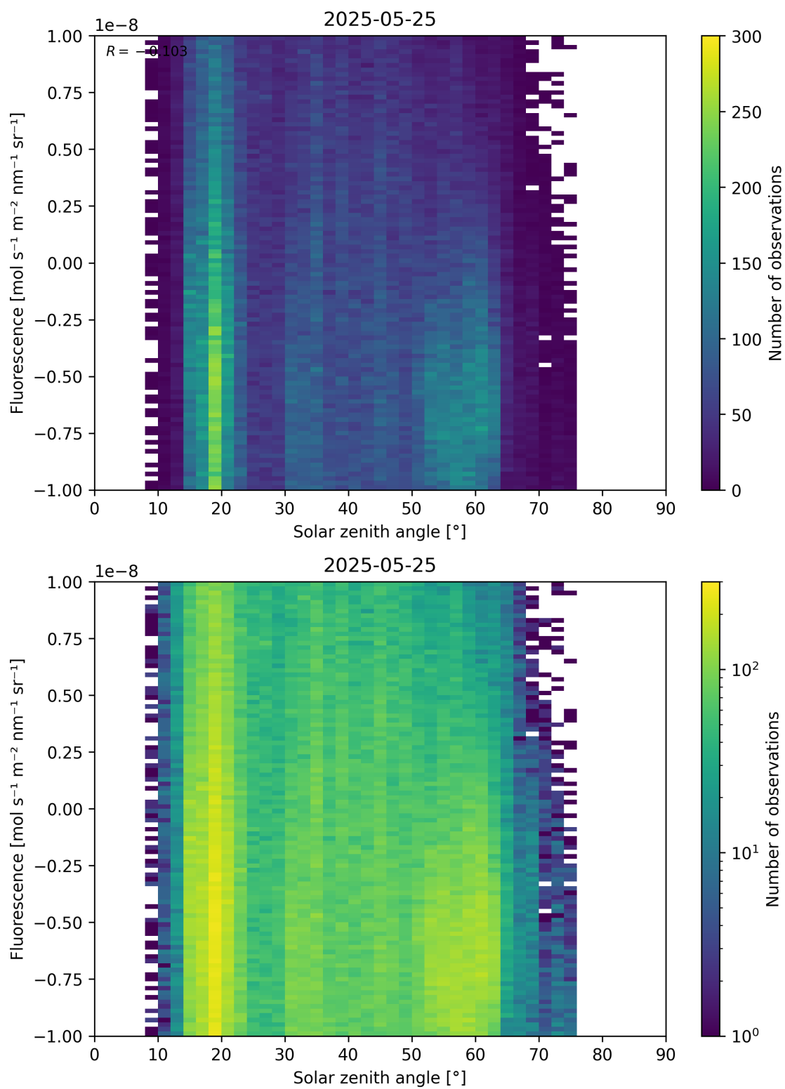
Figure 97: Scatter density plot of “Solar zenith angle” against “Fluorescence” for 2025-05-24 to 2025-05-26.
