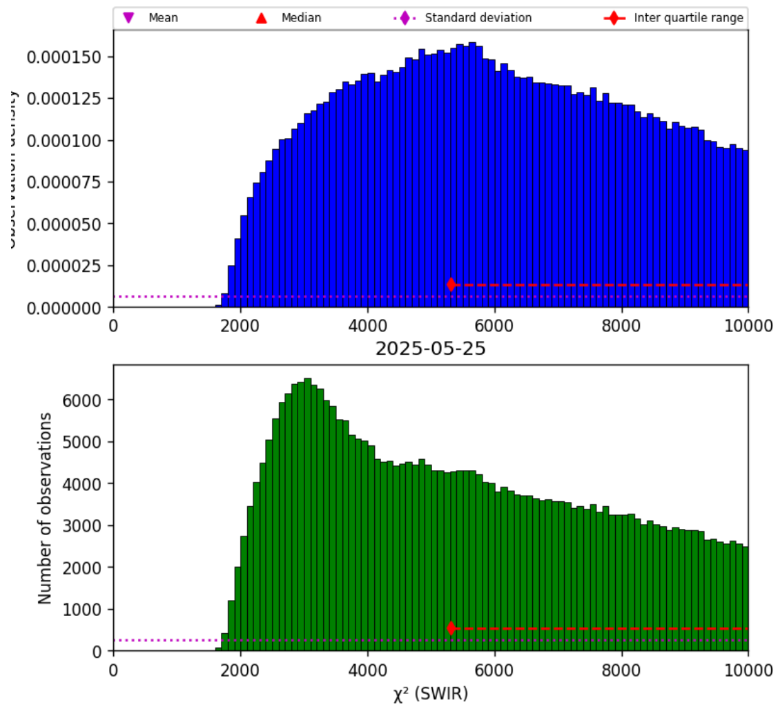
Figure 28: Histogram of “ \chi^2 (SWIR)” for 2025-05-24 to 2025-05-26
