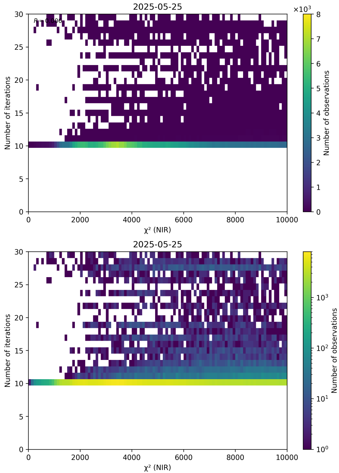
Figure 46: Scatter density plot of “ \chi^2 (NIR)” against “Number of iterations” for 2025-05-24 to 2025-05-26.
