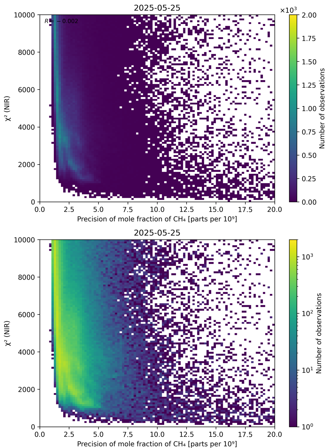
Figure 78: Scatter density plot of “Precision of mole fraction of CH 4 ” against “ \chi^2 (NIR)” for 2025-05-24 to 2025-05-26.
