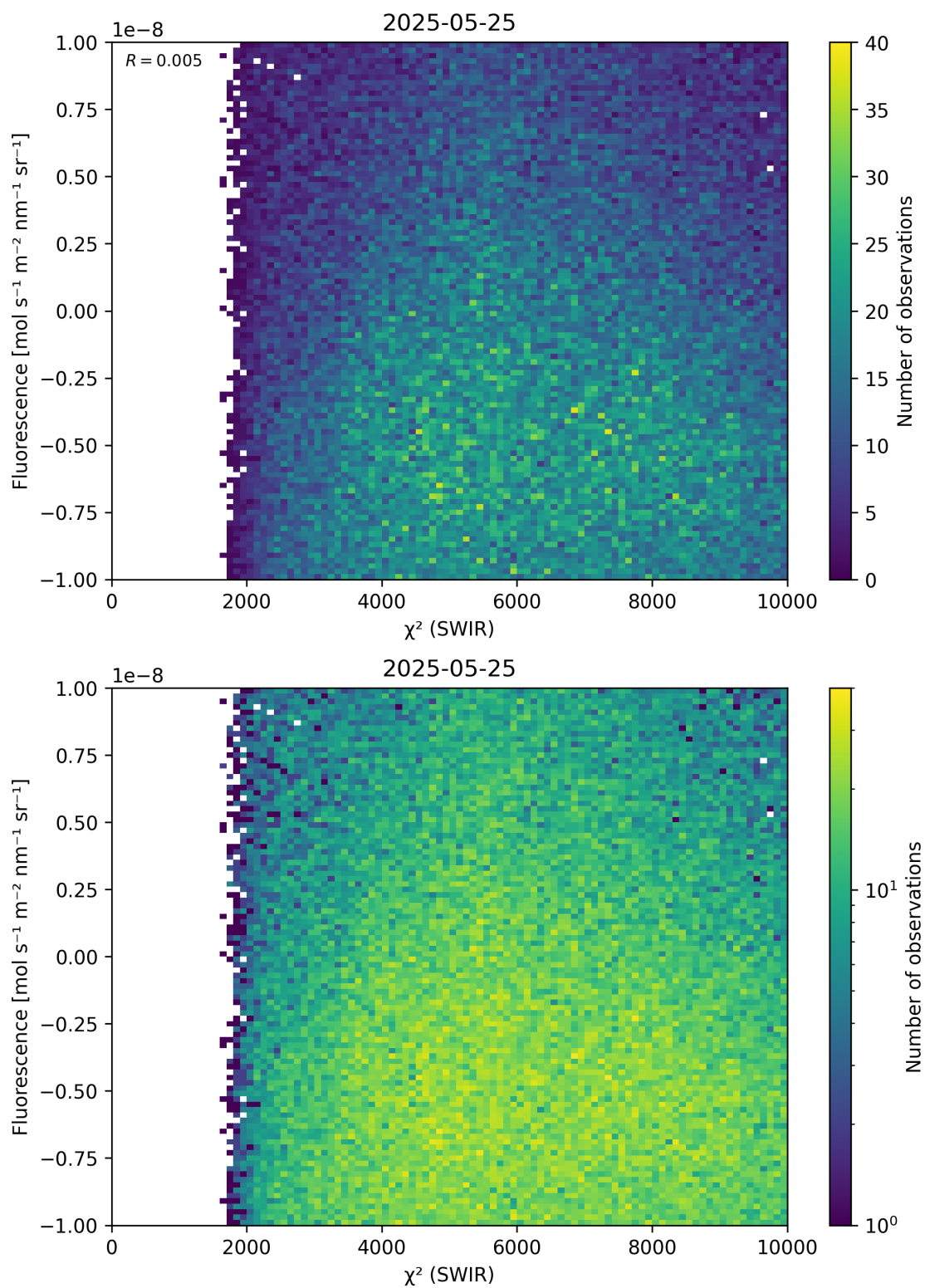
Figure 49: Scatter density plot of “ \chi^2 (SWIR)” against “Fluorescence” for 2025-05-24 to 2025-05-26.
