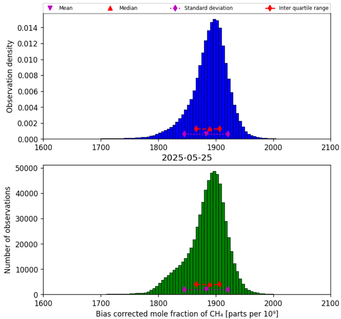
Figure 25: Histogram of “Bias corrected mole fraction of CH 4 ” for 2025-05-24 to 2025-05-26
