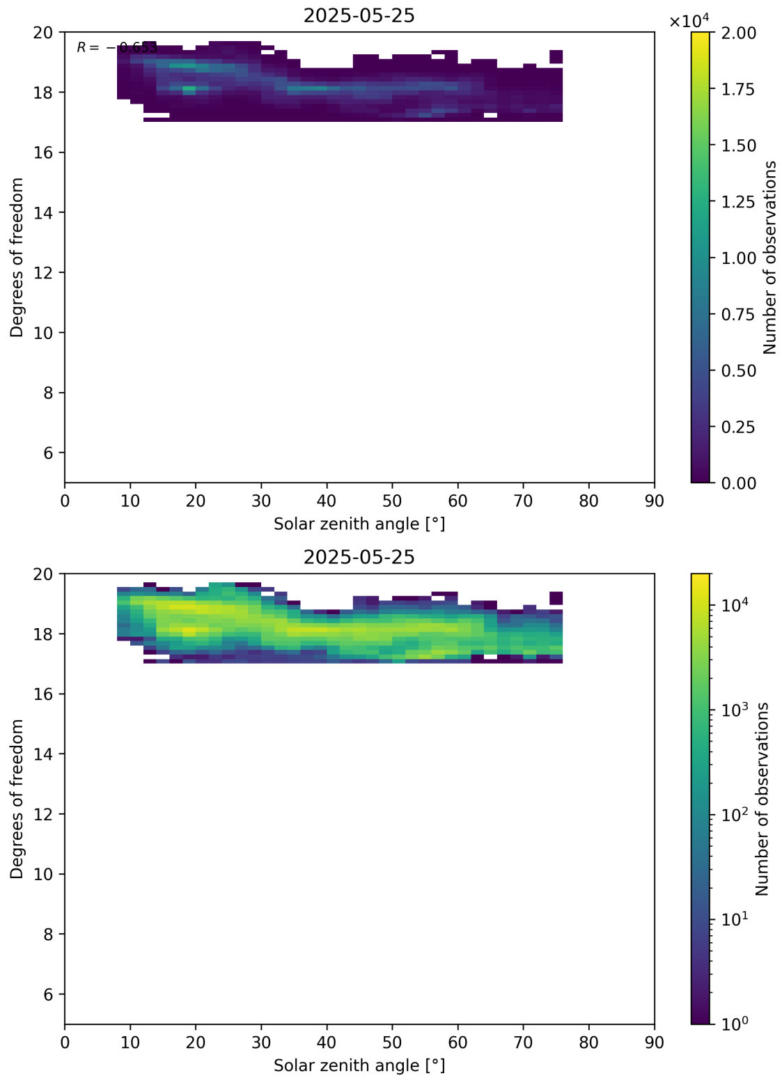
Figure 96: Scatter density plot of “Solar zenith angle” against “Degrees of freedom” for 2025-05-24 to 2025-05-26.
