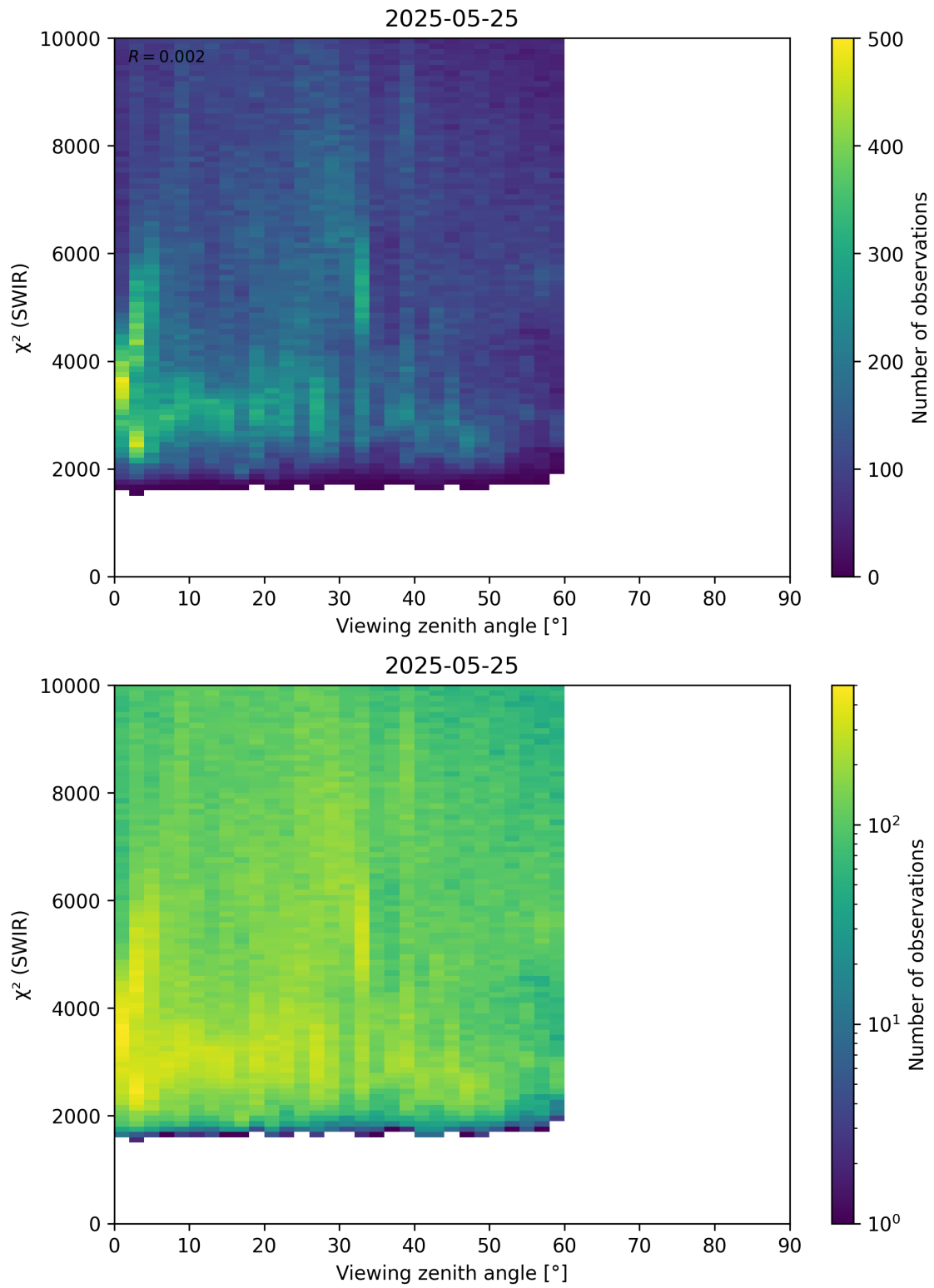
Figure 106: Scatter density plot of “Viewing zenith angle” against “ \chi^2 (SWIR)” for 2025-05-24 to 2025-05-26.
