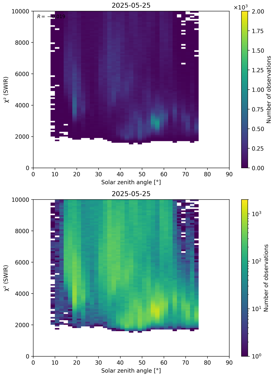
Figure 95: Scatter density plot of “Solar zenith angle” against “ \chi^2 (SWIR)” for 2025-05-24 to 2025-05-26.
