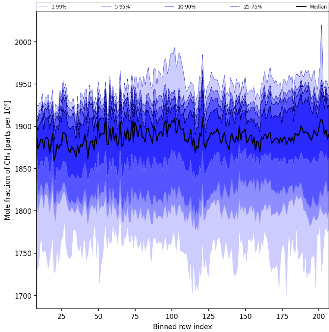
Figure 34: Along track statistics of “Mole fraction of CH 4 ” for 2025-05-24 to 2025-05-26
