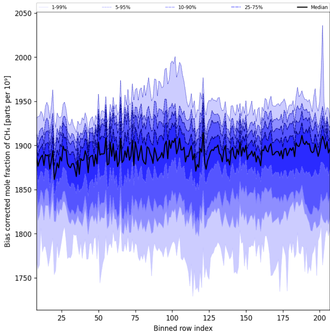
Figure 36: Along track statistics of “Bias corrected mole fraction of CH 4 ” for 2025-05-24 to 2025-05-26
