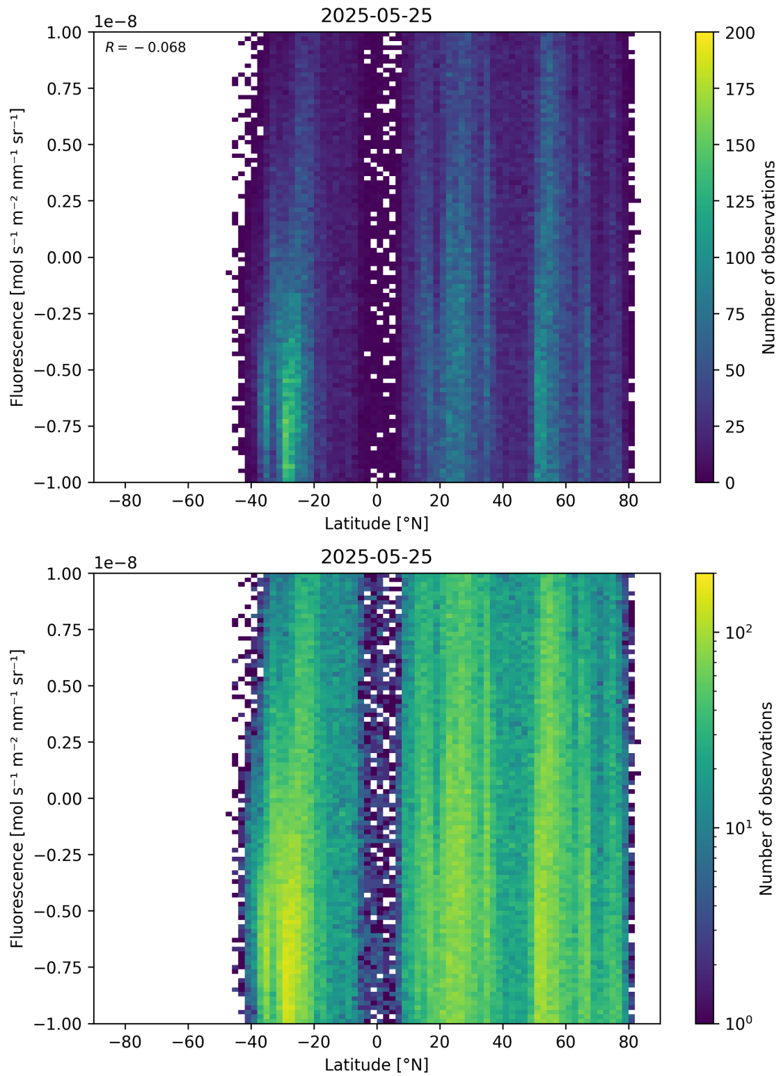
Figure 56: Scatter density plot of “Latitude” against “Fluorescence” for 2025-05-24 to 2025-05-26.
