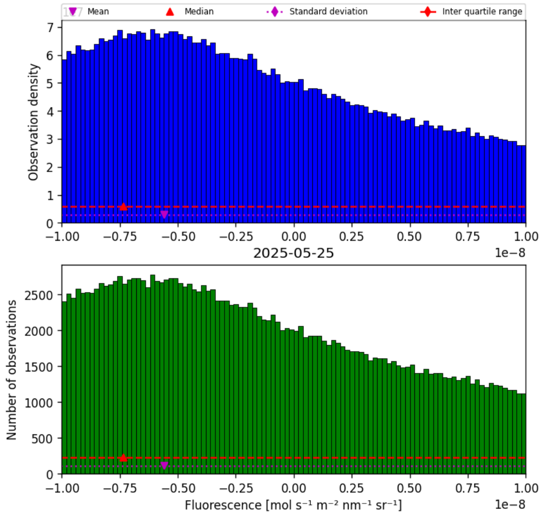
Figure 32: Histogram of “Fluorescence” for 2025-05-24 to 2025-05-26
