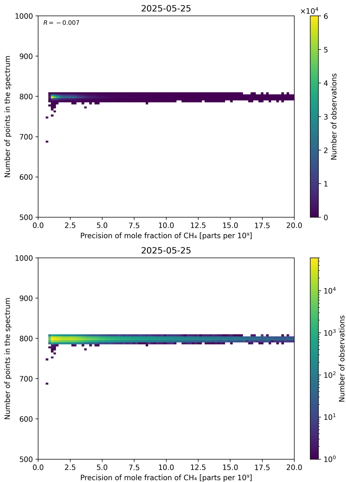
Figure 84: Scatter density plot of “Precision of mole fraction of CH 4 ” against “Number of points in the spectrum” for 2025-05-24 to 2025-05-26.
