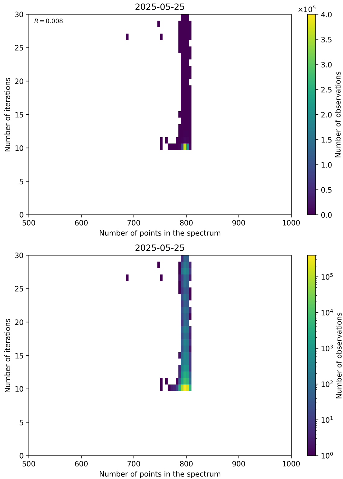
Figure 92: Scatter density plot of “Number of points in the spectrum” against “Number of iterations” for 2025-05-24 to 2025-05-26.
