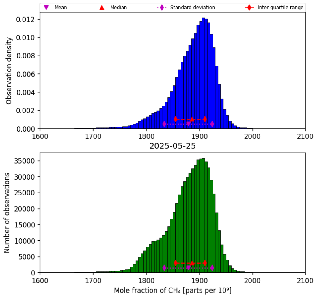
Figure 23: Histogram of “Mole fraction of CH 4 ” for 2025-05-24 to 2025-05-26
