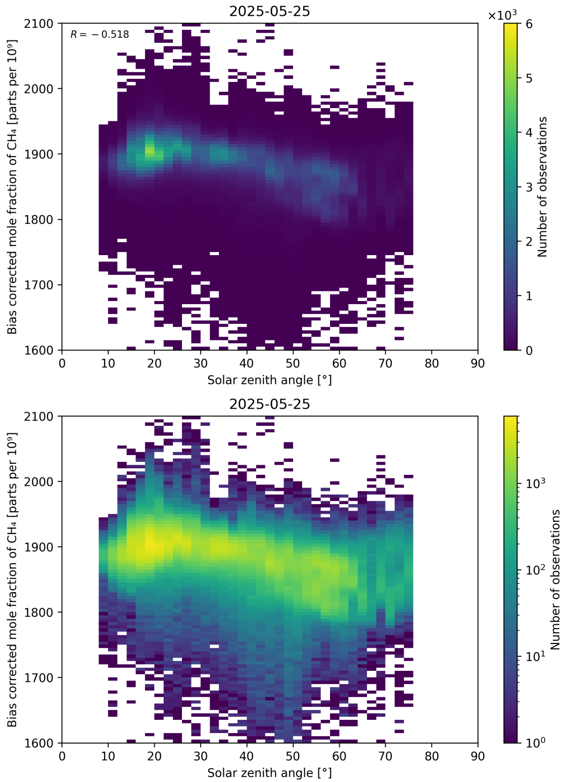
Figure 100: Scatter density plot of “Solar zenith angle” against “Bias corrected mole fraction of CH 4 ” for 2025-05-24 to 2025-05-26.
