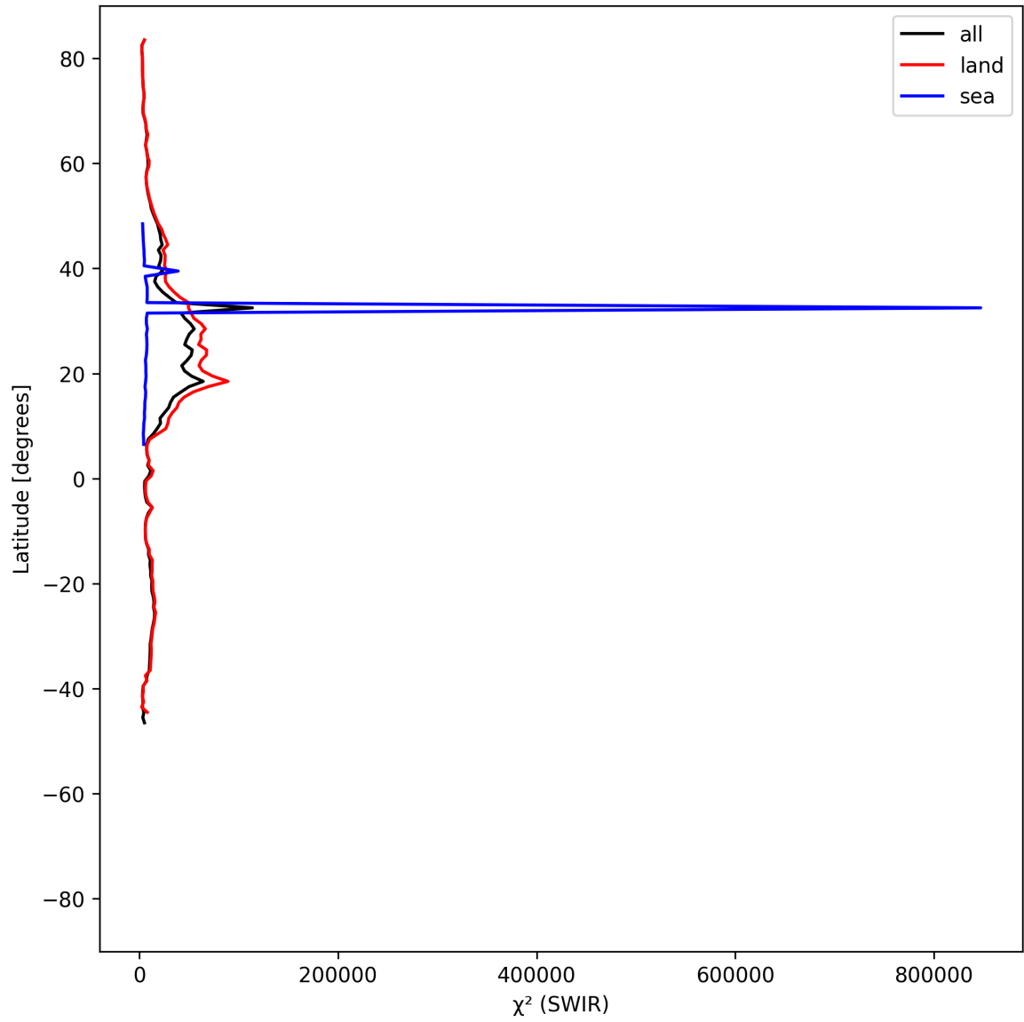
Figure 17: Zonal average of “ \chi^2 (SWIR)” for 2025-05-24 to 2025-05-26.
