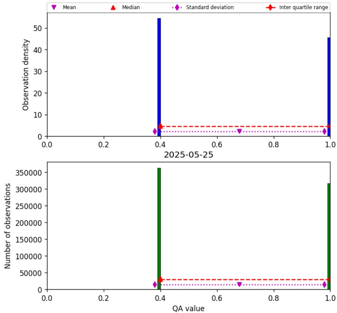
Figure 22: Histogram of “QA value” for 2025-05-24 to 2025-05-26
