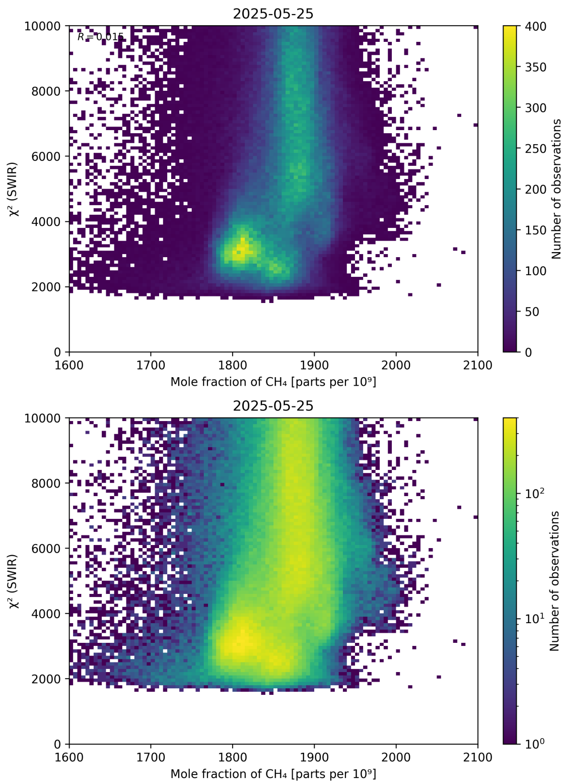
Figure 71: Scatter density plot of “Mole fraction of \text{CH}_4 ” against “ \chi^2 (SWIR)” for 2025-05-24 to 2025-05-26.
