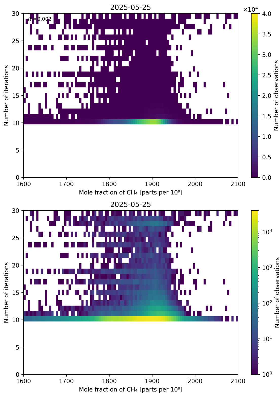
Figure 76: Scatter density plot of “Mole fraction of CH 4 ” against “Number of iterations” for 2025-05-24 to 2025-05-26.
