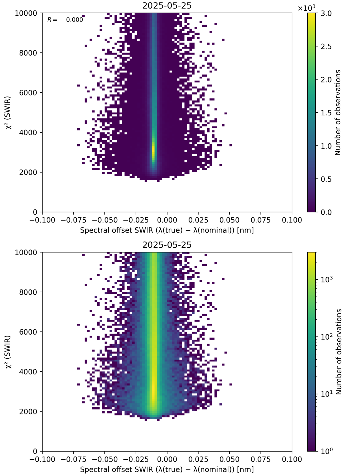
Figure 118: Scatter density plot of “Spectral offset SWIR ( \lambda_{\text{true}} - \lambda_{\text{nominal}} )” against “ \chi^2 (SWIR)” for 2025-05-24 to 2025-05-26.
