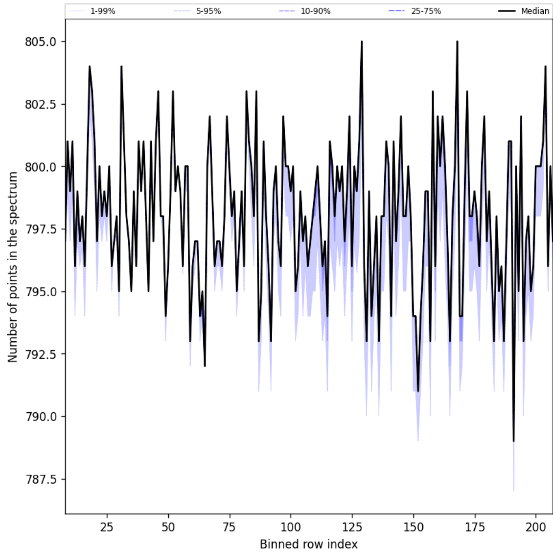
Figure 37: Along track statistics of “Number of points in the spectrum” for 2025-05-24 to 2025-05-26
