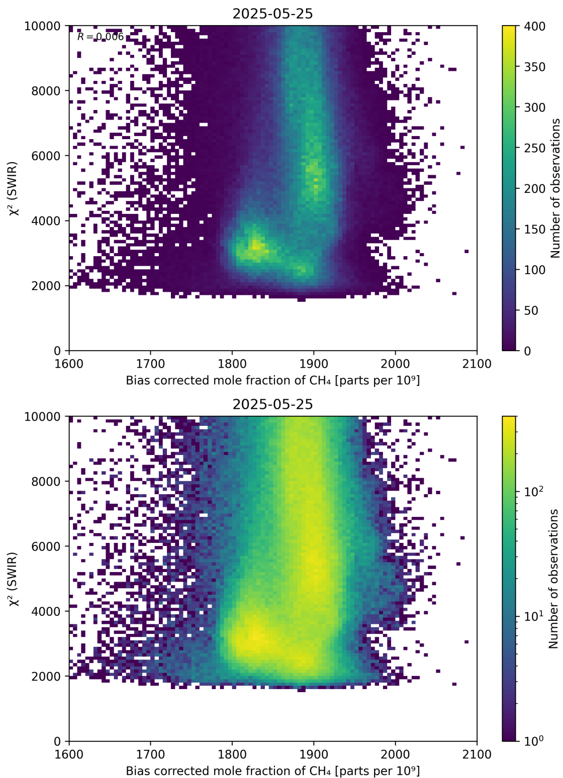
Figure 64: Scatter density plot of “Bias corrected mole fraction of \text{CH}_4 ” against “ \chi^2 (SWIR)” for 2025-05-24 to 2025-05-26.
