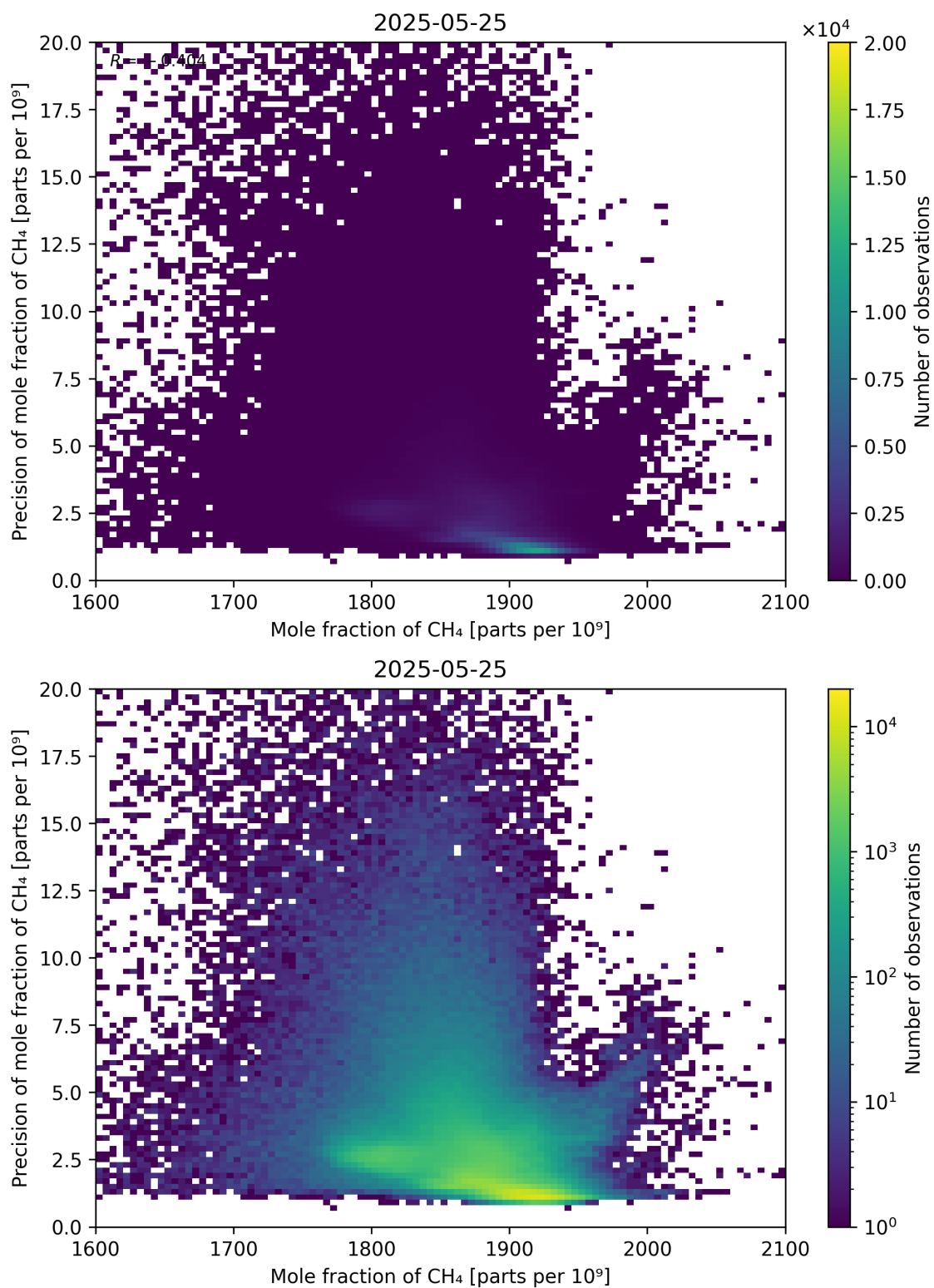
Figure 75: Scatter density plot of “Mole fraction of CH 4 ” against “Precision of mole fraction of CH 4 ” for 2025-05-24 to 2025-05-26.
