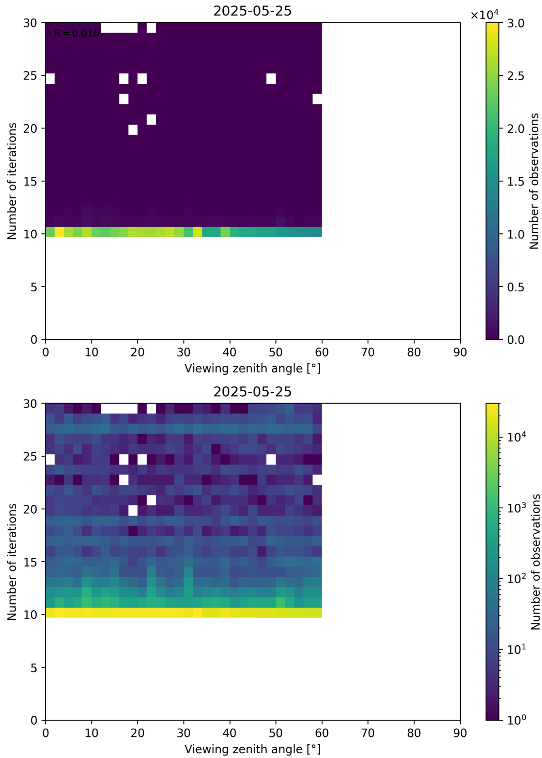
Figure 113: Scatter density plot of “Viewing zenith angle” against “Number of iterations” for 2025-05-24 to 2025-05-26.
