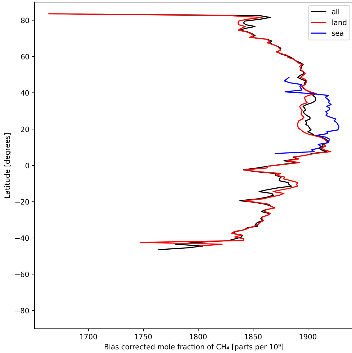
Figure 14: Zonal average of “Bias corrected mole fraction of \text{CH}_4 ” for 2025-05-24 to 2025-05-26.
