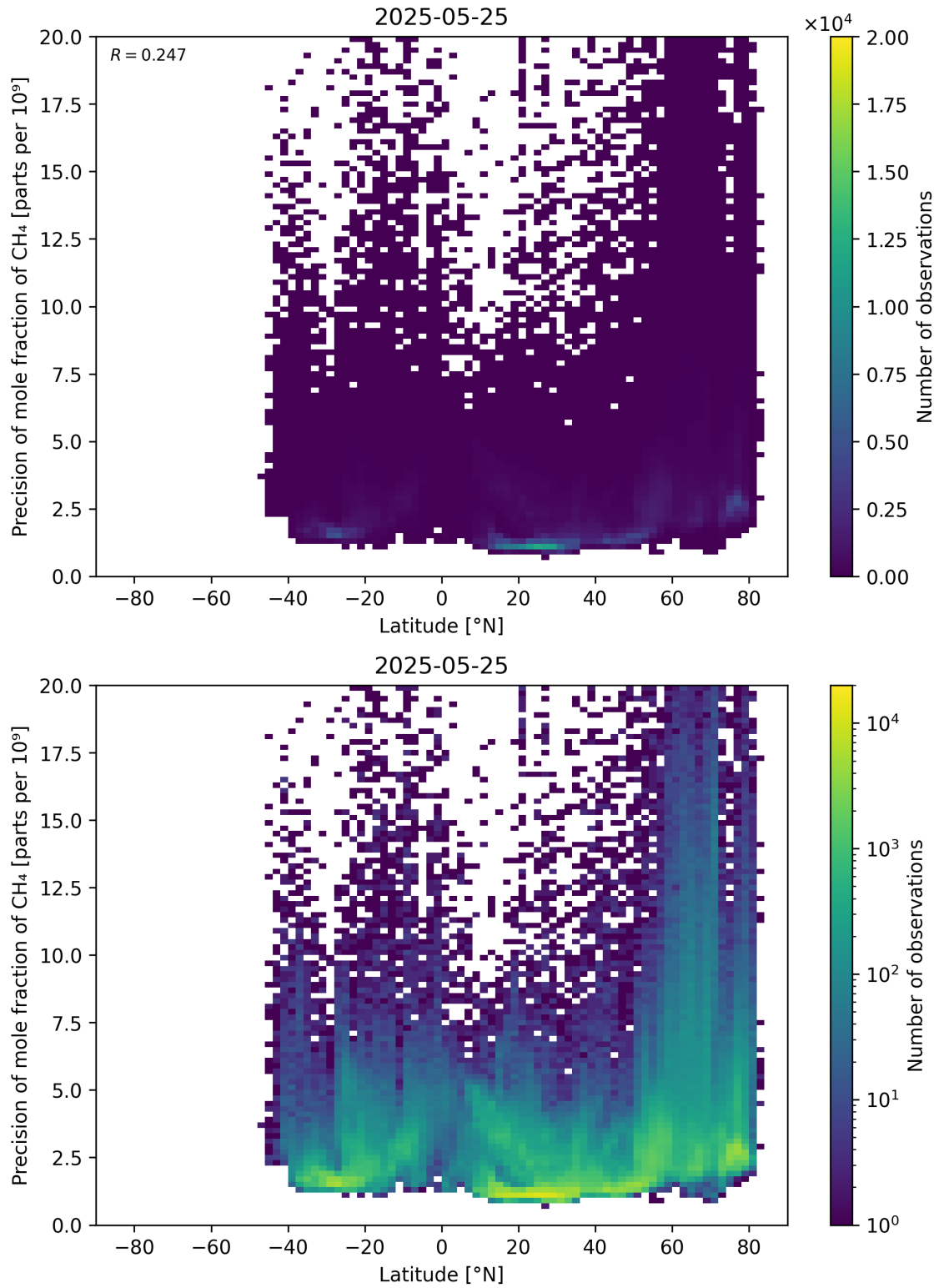
Figure 59: Scatter density plot of “Latitude” against “Precision of mole fraction of \text{CH}_4 ” for 2025-05-24 to 2025-05-26.
