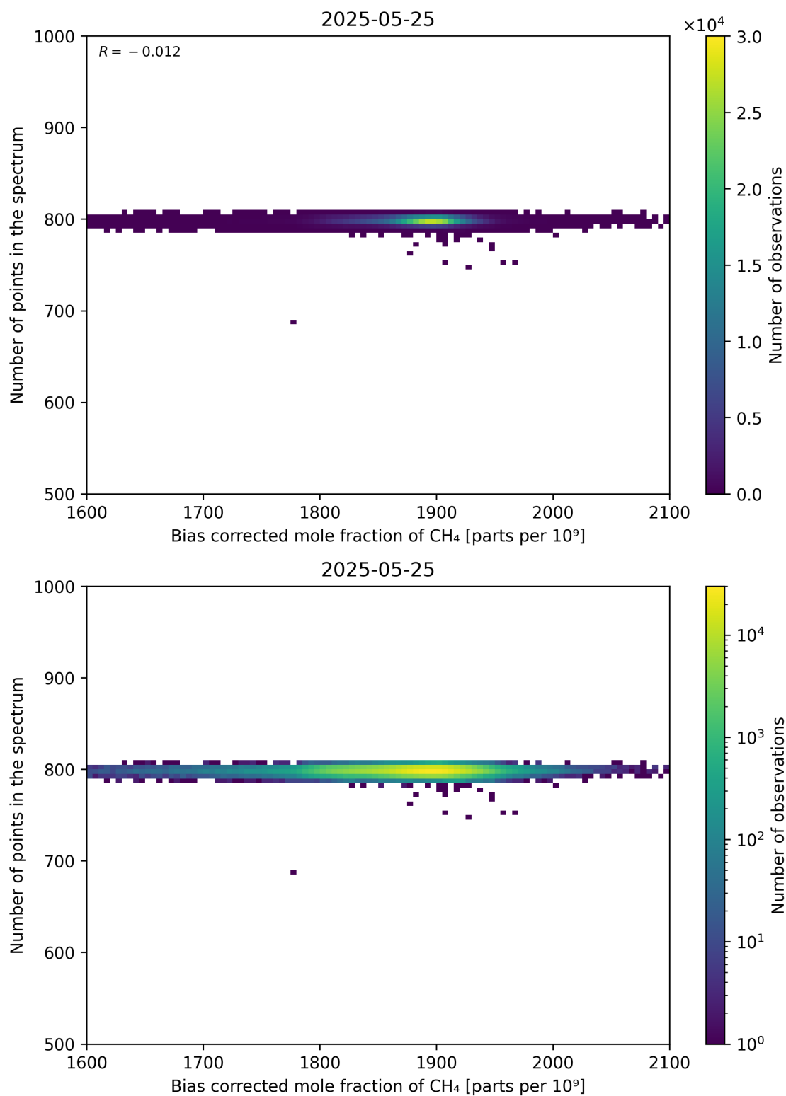
Figure 68: Scatter density plot of “Bias corrected mole fraction of CH 4 ” against “Number of points in the spectrum” for 2025-05-24 to 2025-05-26.
