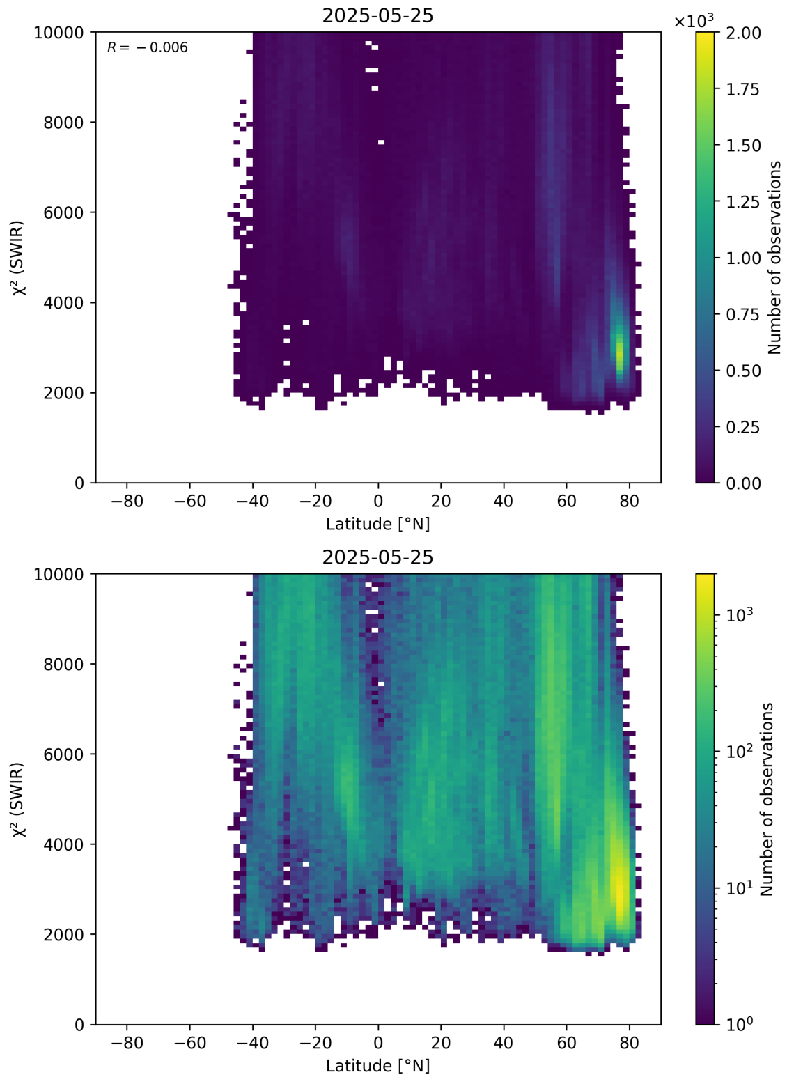
Figure 54: Scatter density plot of “Latitude” against “ \chi^2 (SWIR)” for 2025-05-24 to 2025-05-26.
