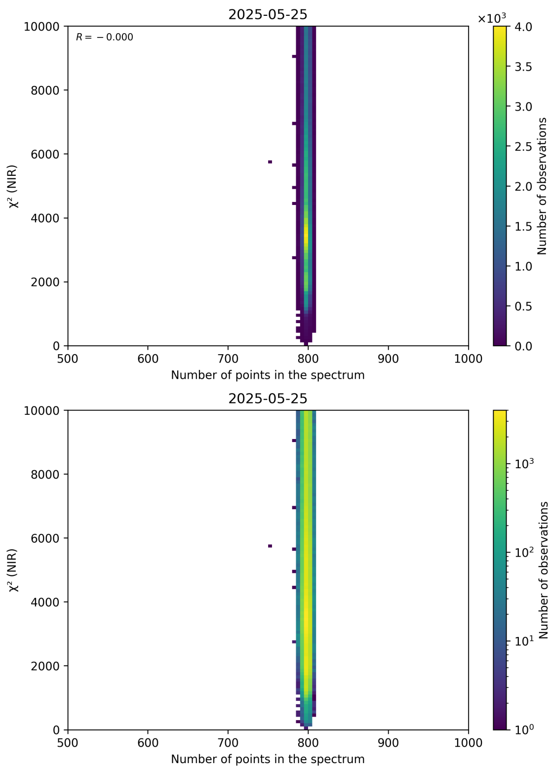
Figure 88: Scatter density plot of “Number of points in the spectrum” against “ \chi^2 (NIR)” for 2025-05-24 to 2025-05-26.
