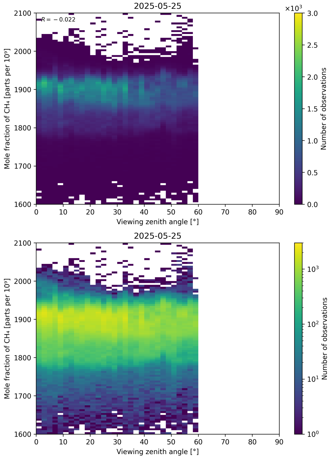
Figure 110: Scatter density plot of “Viewing zenith angle” against “Mole fraction of CH 4 ” for 2025-05-24 to 2025-05-26.
