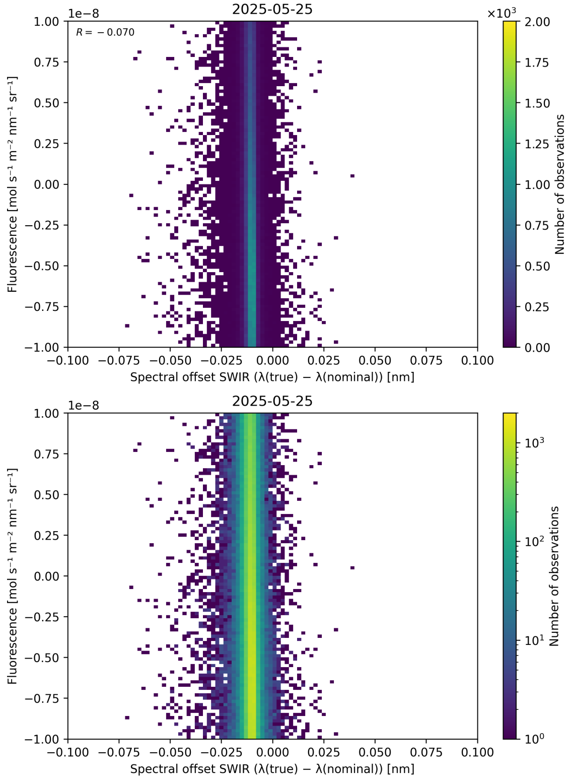
Figure 120: Scatter density plot of “Spectral offset SWIR ( \lambda_{\text{true}} - \lambda_{\text{nominal}} )” against “Fluorescence” for 2025-05-24 to 2025-05-26.
