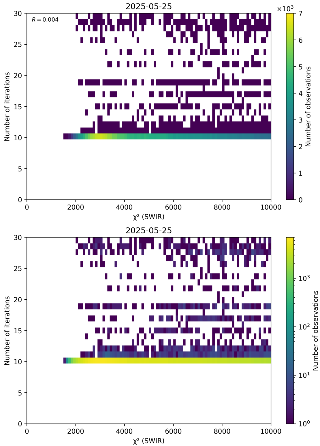
Figure 50: Scatter density plot of “ \chi^2 (SWIR)” against “Number of iterations” for 2025-05-24 to 2025-05-26.
