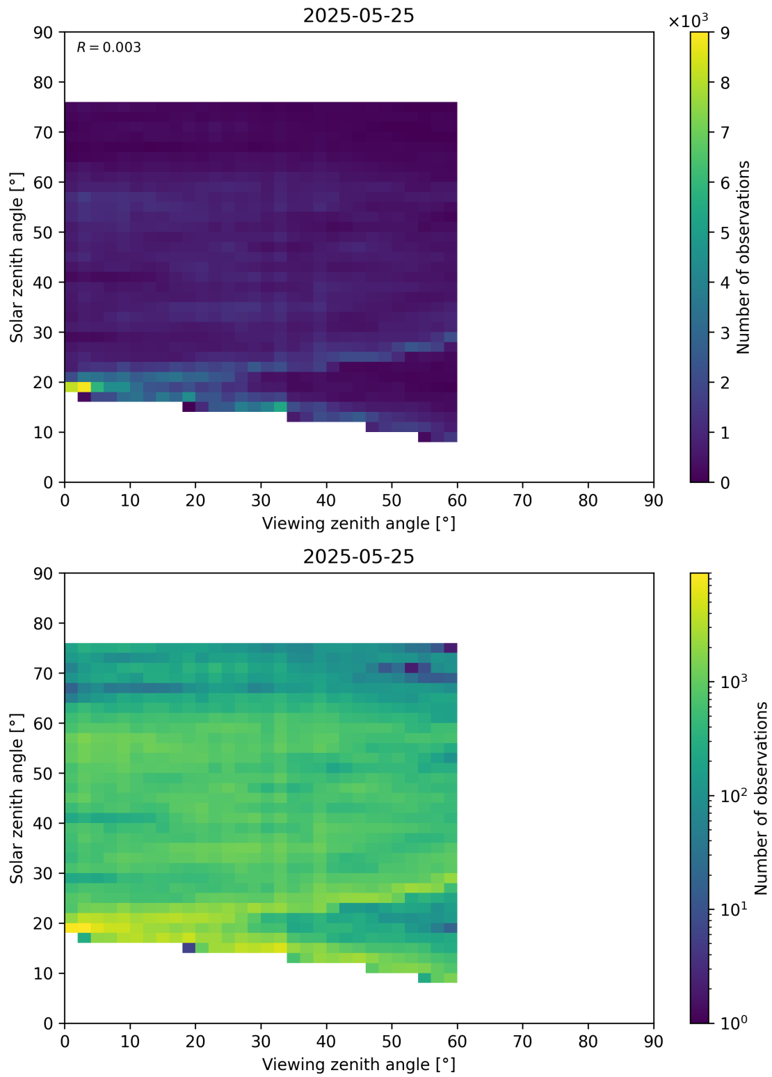
Figure 115: Scatter density plot of “Viewing zenith angle” against “Solar zenith angle” for 2025-05-24 to 2025-05-26.
