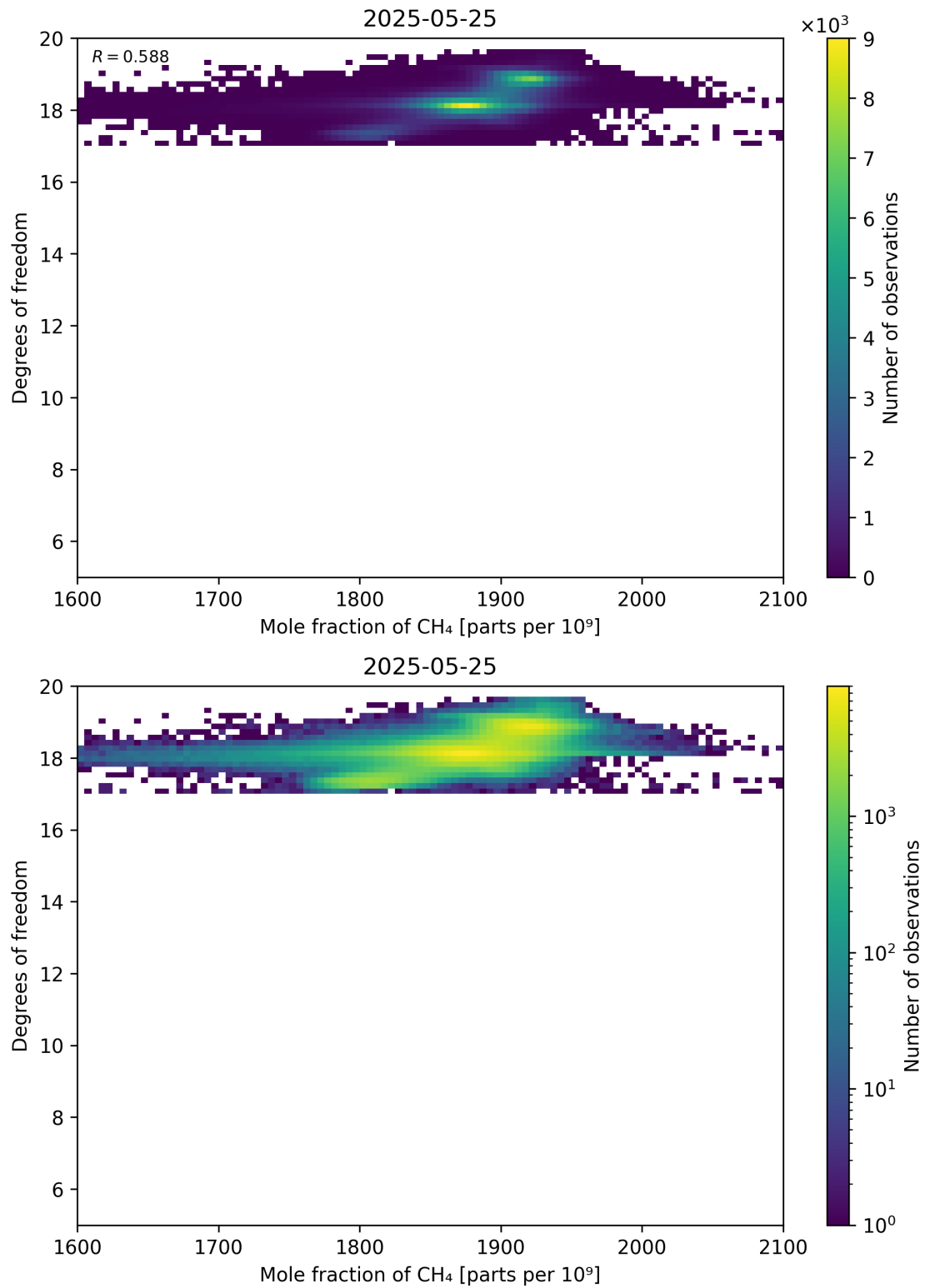
Figure 72: Scatter density plot of “Mole fraction of CH 4 ” against “Degrees of freedom” for 2025-05-24 to 2025-05-26.
