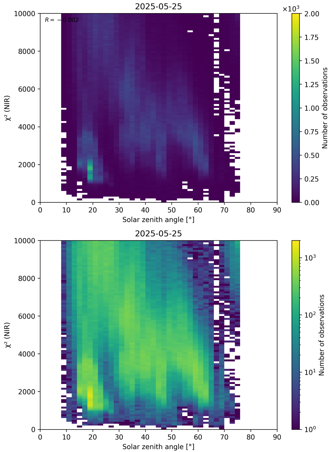
Figure 94: Scatter density plot of “Solar zenith angle” against “ \chi^2 (NIR)” for 2025-05-24 to 2025-05-26.
