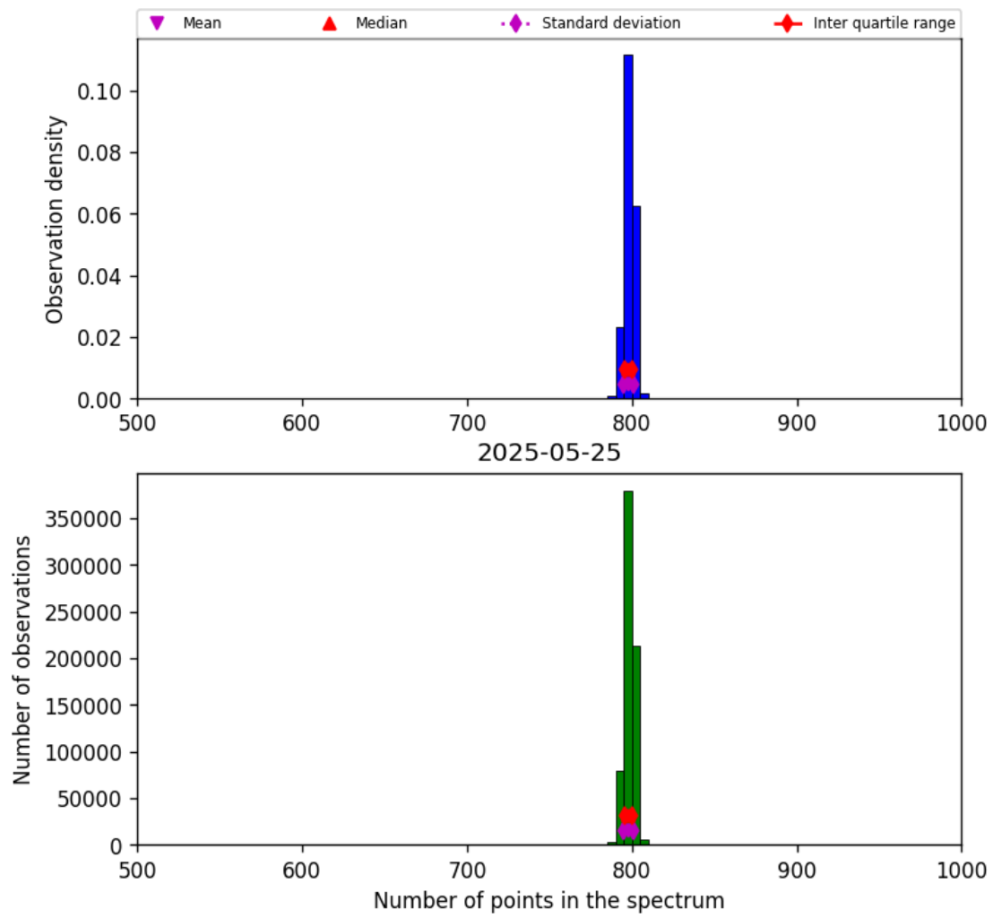
Figure 26: Histogram of “Number of points in the spectrum” for 2025-05-24 to 2025-05-26
