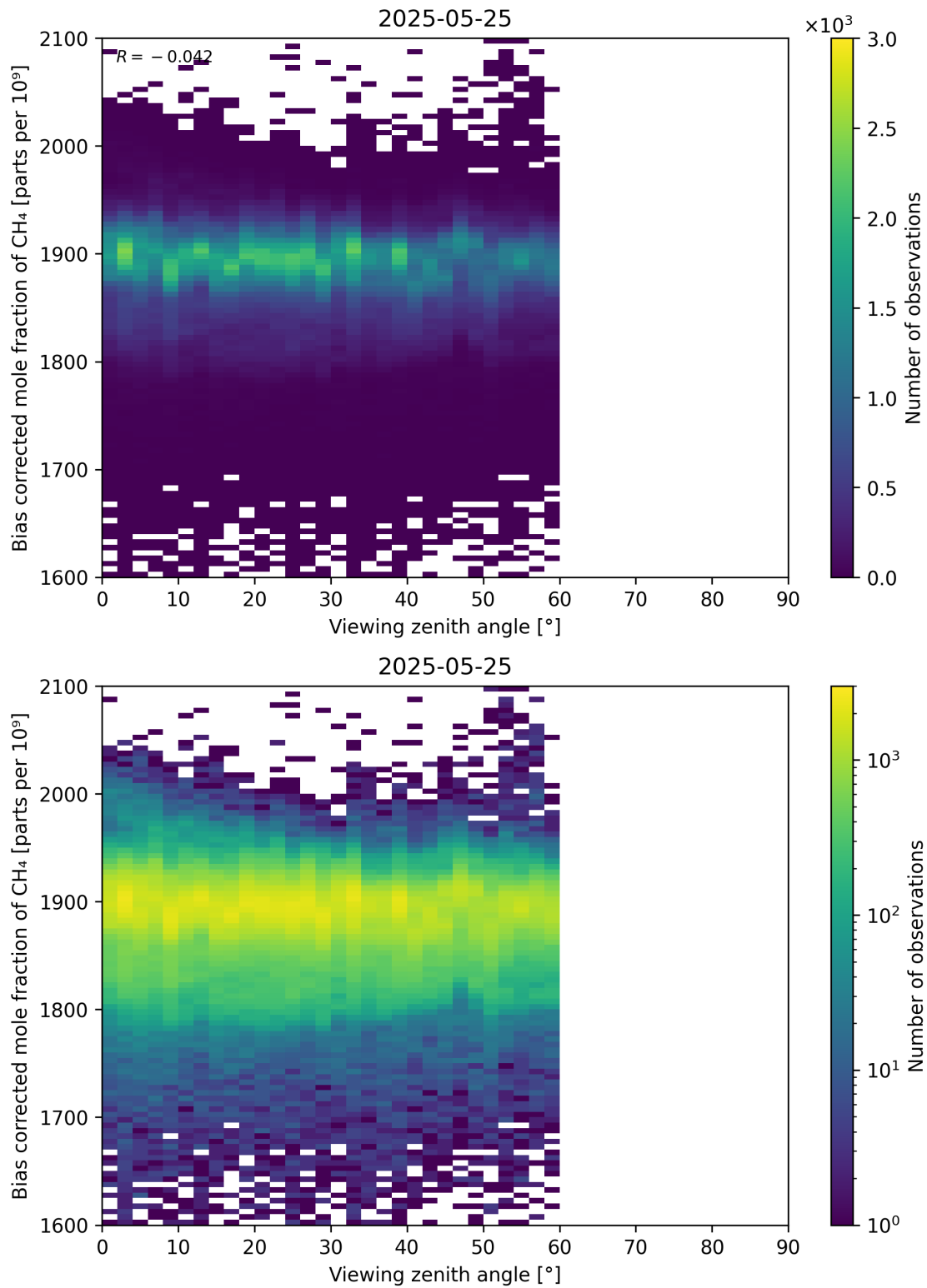
Figure 111: Scatter density plot of “Viewing zenith angle” against “Bias corrected mole fraction of CH 4 ” for 2025-05-24 to 2025-05-26.
