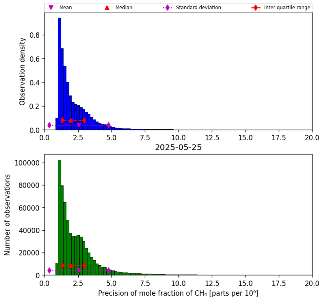
Figure 24: Histogram of “Precision of mole fraction of CH 4 ” for 2025-05-24 to 2025-05-26
