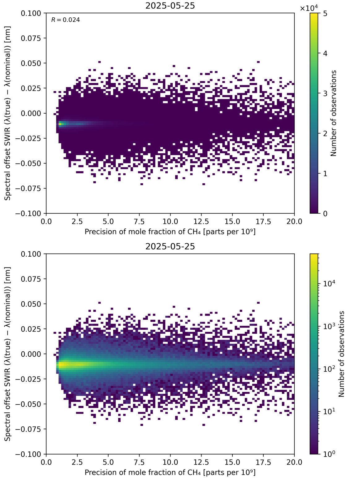
Figure 85: Scatter density plot of “Precision of mole fraction of \text{CH}_4 ” against “Spectral offset SWIR ( \lambda_{\text{true}} - \lambda_{\text{nominal}} )” for 2025-05-24 to 2025-05-26.
