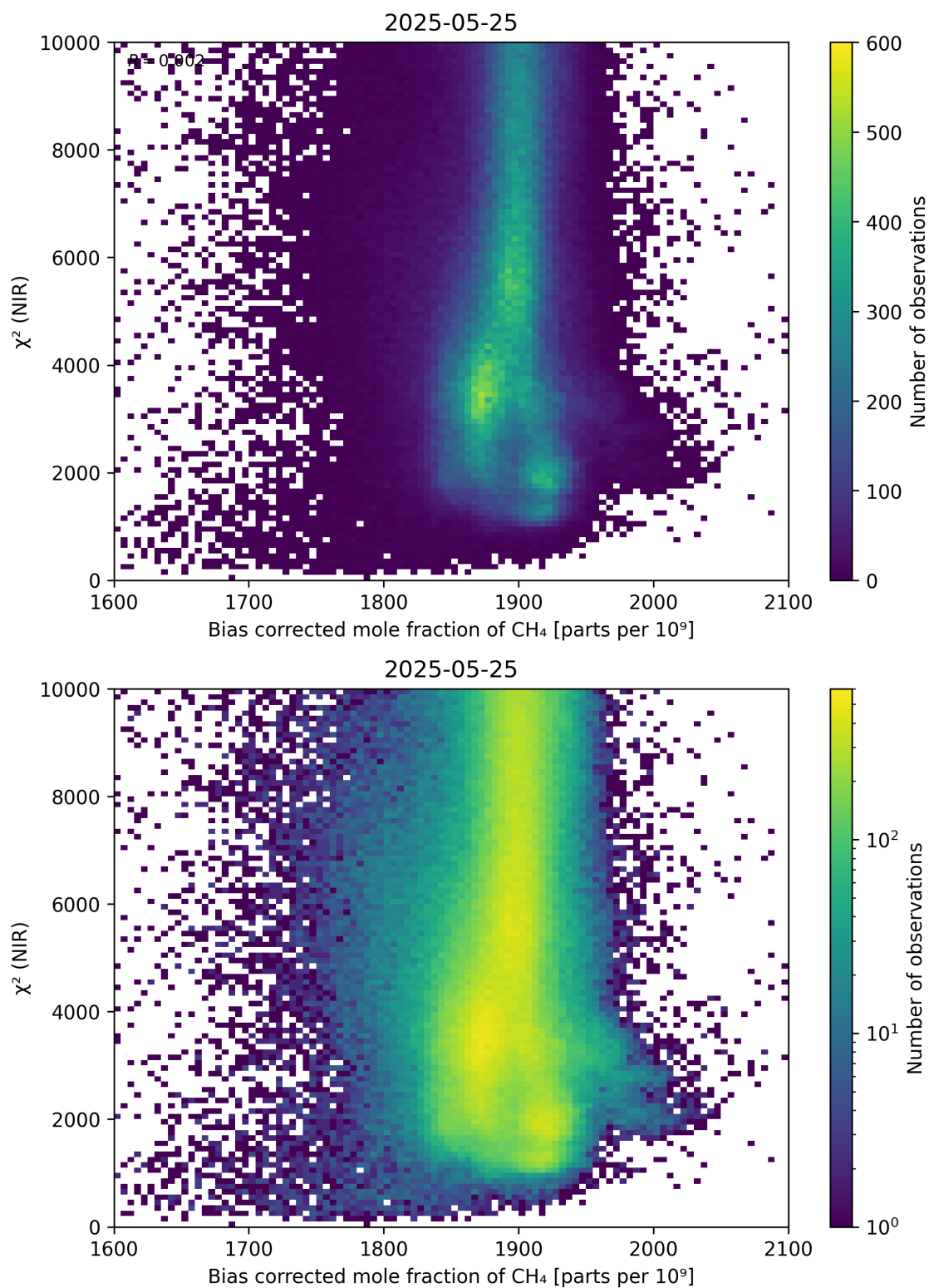
Figure 63: Scatter density plot of “Bias corrected mole fraction of \text{CH}_4 ” against “ \chi^2 (NIR)” for 2025-05-24 to 2025-05-26.
