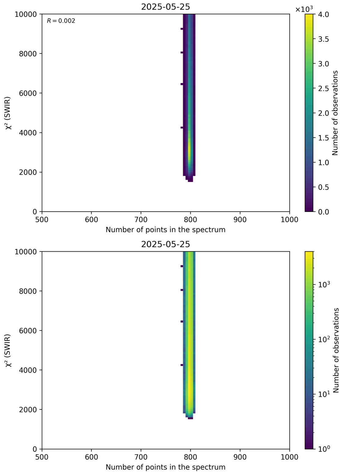
Figure 89: Scatter density plot of “Number of points in the spectrum” against “ \chi^2 (SWIR)” for 2025-05-24 to 2025-05-26.
