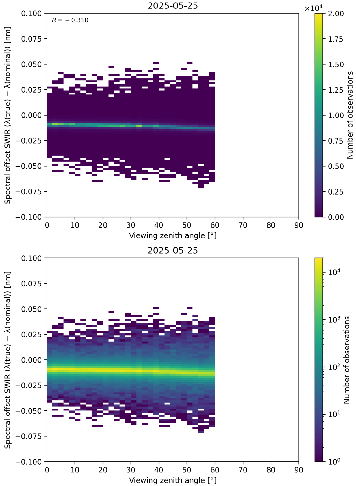
Figure 116: Scatter density plot of “Viewing zenith angle” against “Spectral offset SWIR ( \lambda_{\text{true}} - \lambda_{\text{nominal}} )” for 2025-05-24 to 2025-05-26.
