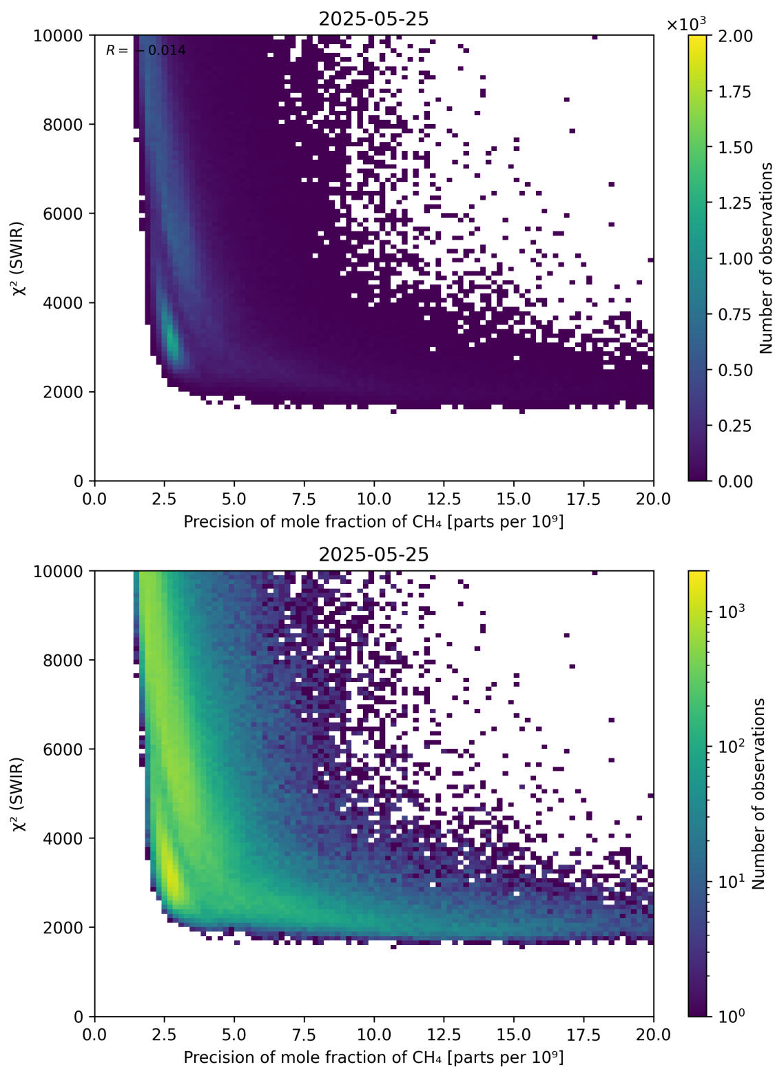
Figure 79: Scatter density plot of “Precision of mole fraction of \text{CH}_4 ” against “ \chi^2 (SWIR)” for 2025-05-24 to 2025-05-26.
