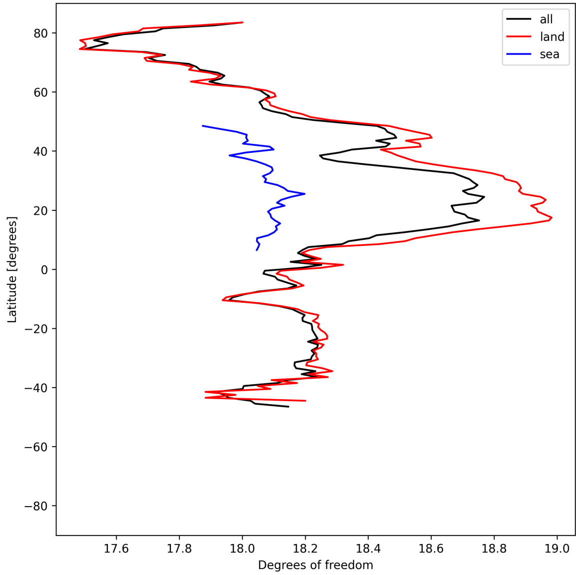
Figure 19: Zonal average of “Degrees of freedom” for 2025-05-24 to 2025-05-26.
