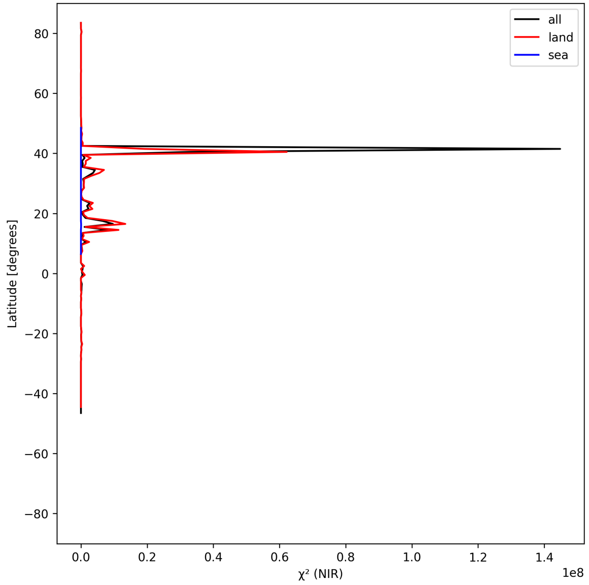
Figure 18: Zonal average of “ \chi^2 (NIR)” for 2025-05-24 to 2025-05-26.
