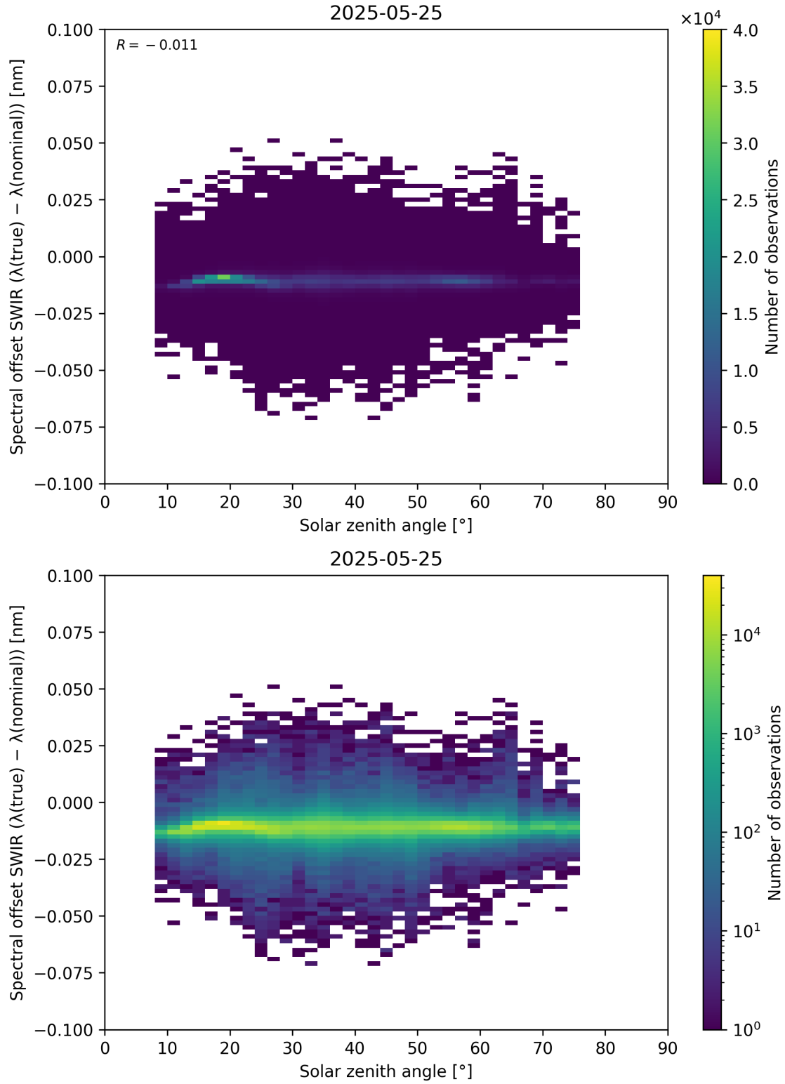
Figure 104: Scatter density plot of “Solar zenith angle” against “Spectral offset SWIR ( \lambda_{\text{true}} - \lambda_{\text{nominal}} )” for 2025-05-24 to 2025-05-26.
