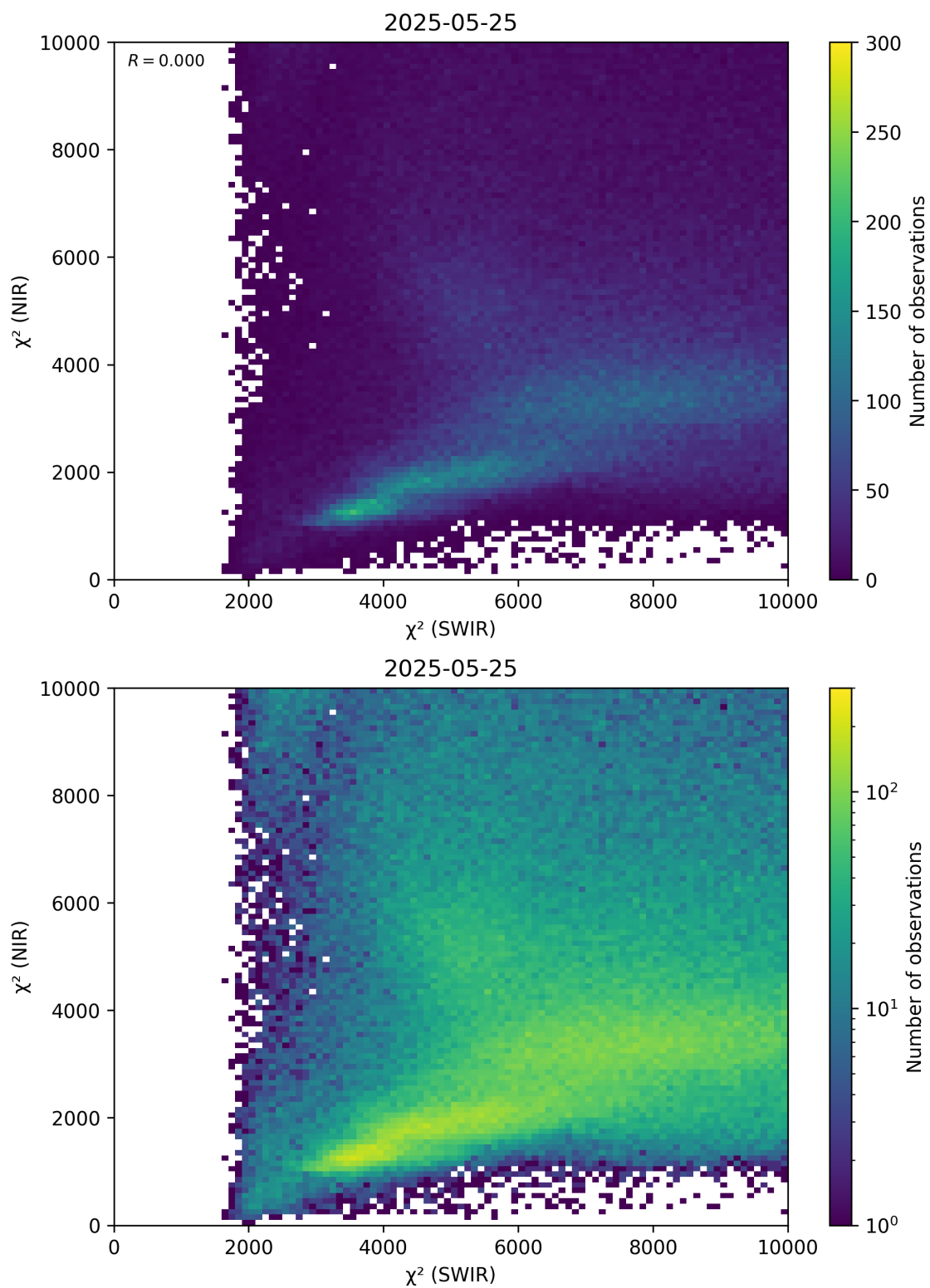
Figure 47: Scatter density plot of “ \chi^2 (SWIR)” against “ \chi^2 (NIR)” for 2025-05-24 to 2025-05-26.
