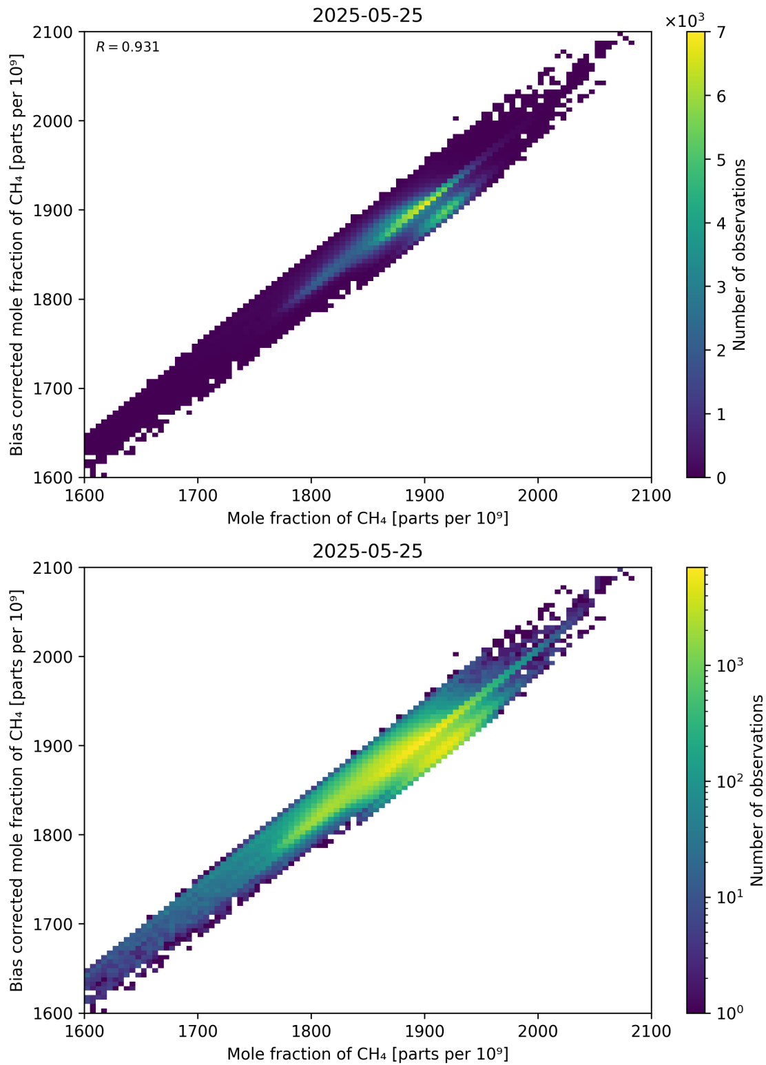
Figure 74: Scatter density plot of “Mole fraction of CH 4 ” against “Bias corrected mole fraction of CH 4 ” for 2025-05-24 to 2025-05-26.
