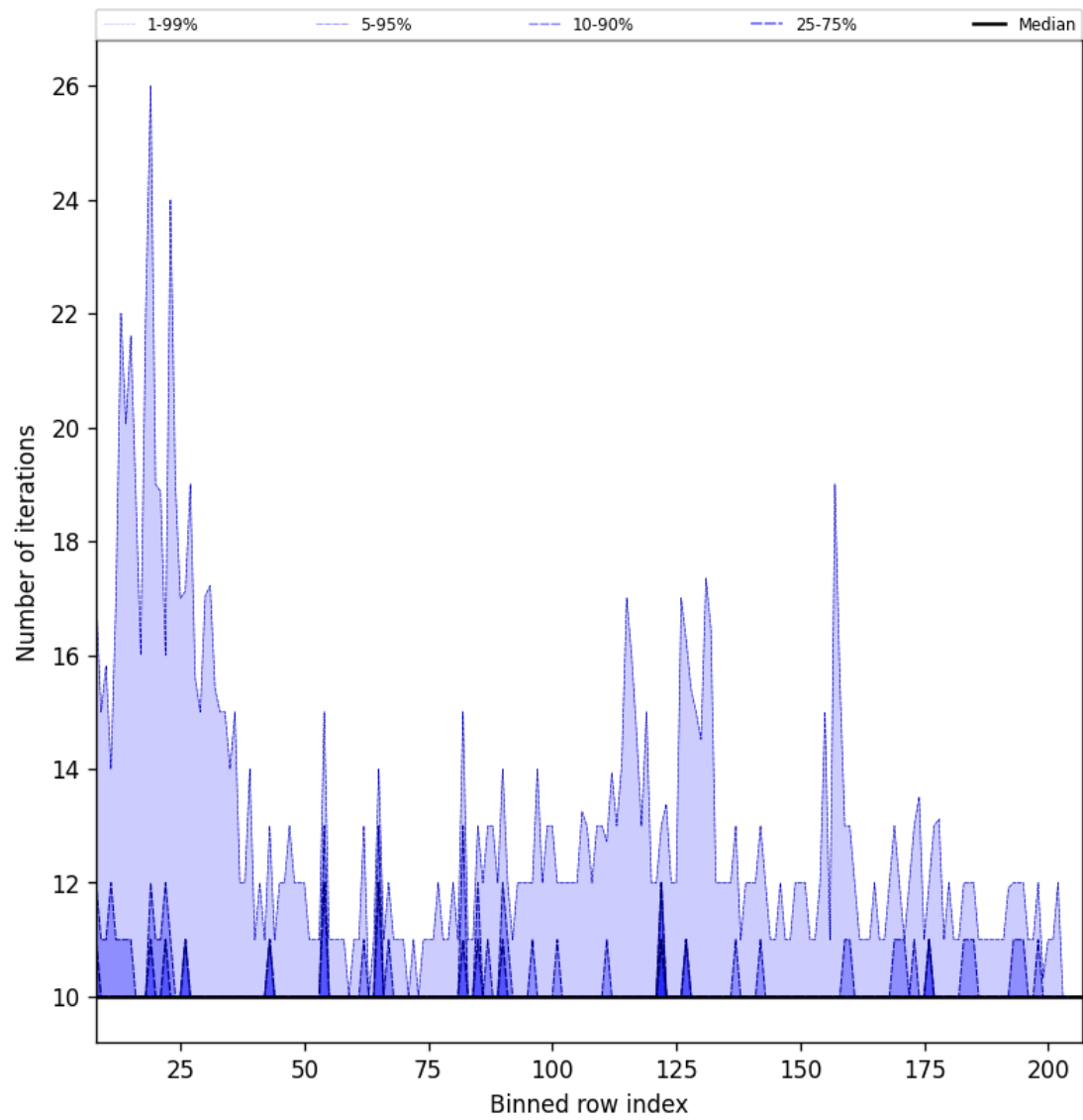
Figure 42: Along track statistics of “Number of iterations” for 2025-05-24 to 2025-05-26
