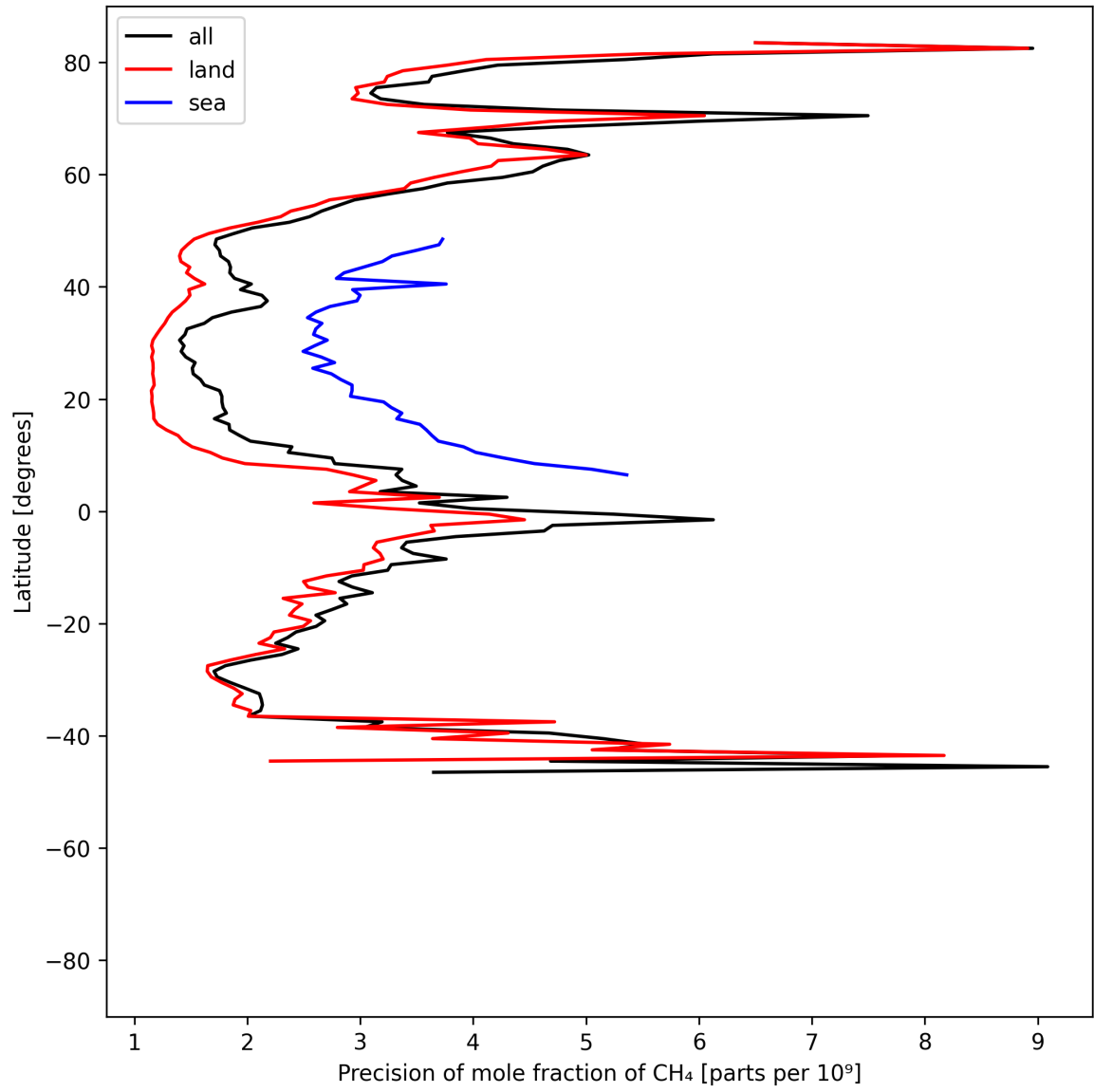
Figure 13: Zonal average of “Precision of mole fraction of CH 4 ” for 2025-05-24 to 2025-05-26.
