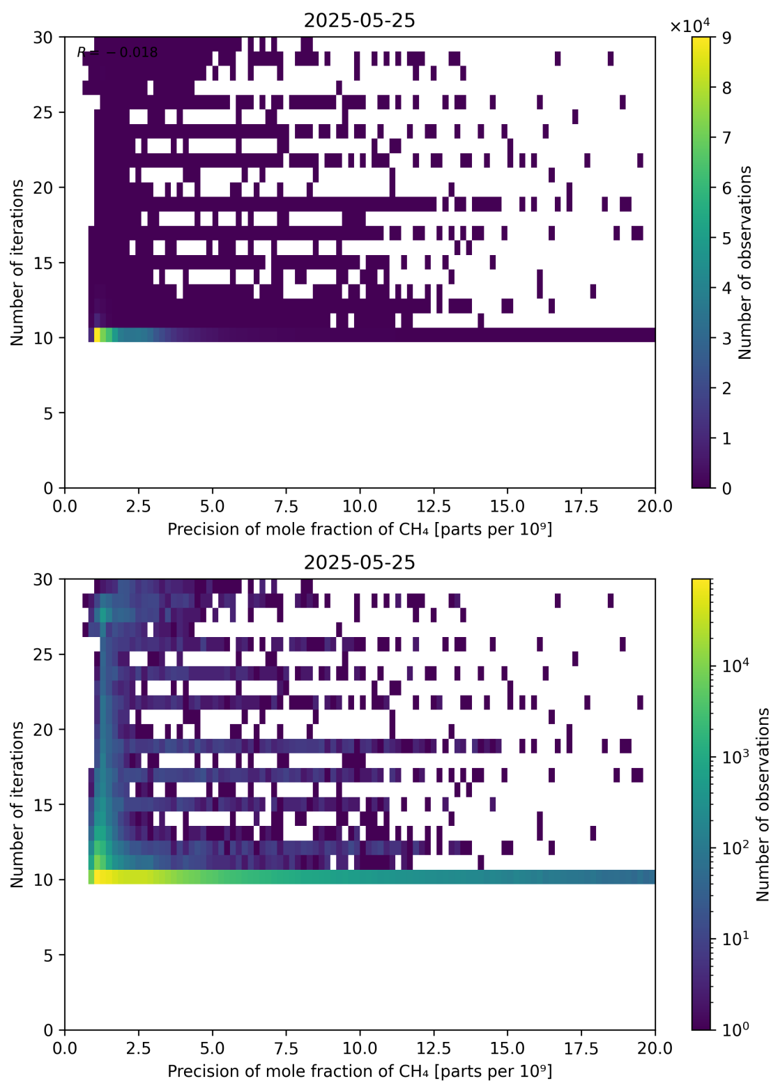
Figure 83: Scatter density plot of “Precision of mole fraction of CH 4 ” against “Number of iterations” for 2025-05-24 to 2025-05-26.
