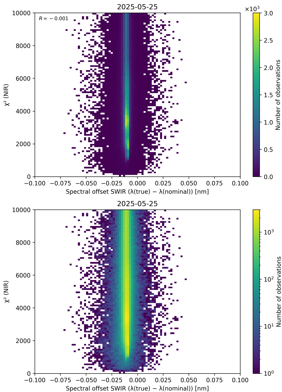
Figure 117: Scatter density plot of “Spectral offset SWIR ( \lambda_{\text{true}} - \lambda_{\text{nominal}} )” against “ \chi^2 (NIR)” for 2025-05-24 to 2025-05-26.
