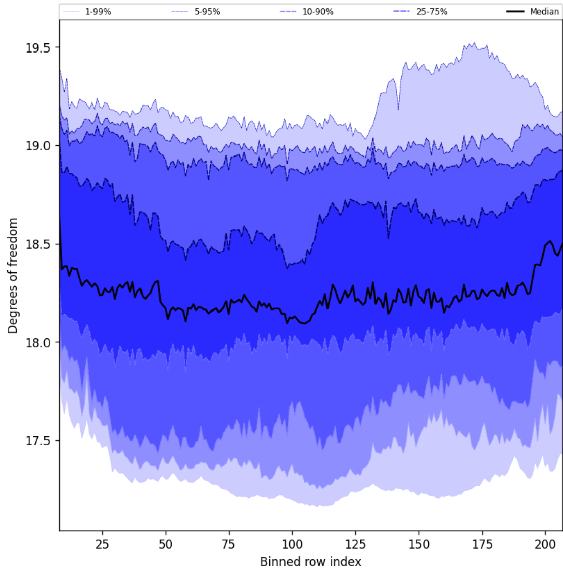
Figure 41: Along track statistics of “Degrees of freedom” for 2025-05-24 to 2025-05-26
