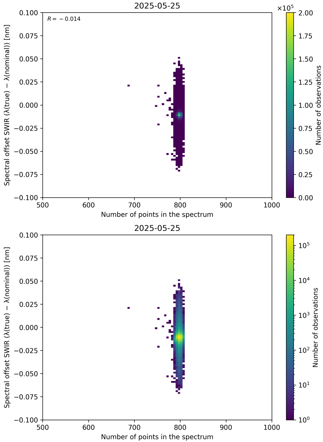
Figure 93: Scatter density plot of “Number of points in the spectrum” against “Spectral offset SWIR ( \lambda_{\text{true}} - \lambda_{\text{nominal}} )” for 2025-05-24 to 2025-05-26.
