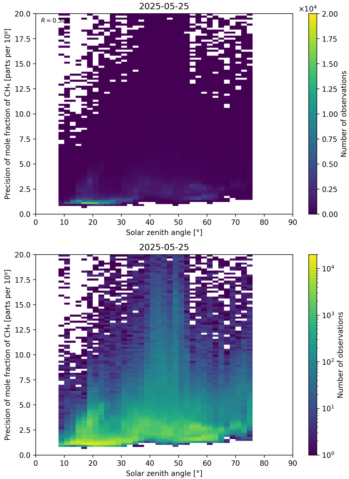
Figure 101: Scatter density plot of “Solar zenith angle” against “Precision of mole fraction of CH 4 ” for 2025-05-24 to 2025-05-26.
