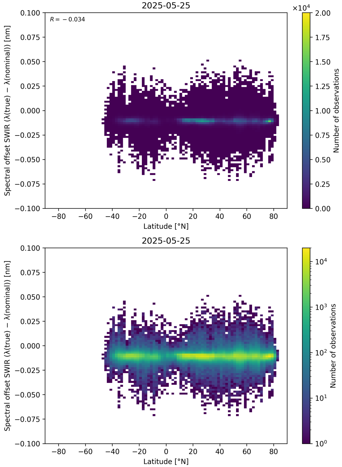
Figure 62: Scatter density plot of “Latitude” against “Spectral offset SWIR ( \lambda_{\text{true}} - \lambda_{\text{nominal}} )” for 2025-05-24 to 2025-05-26.
