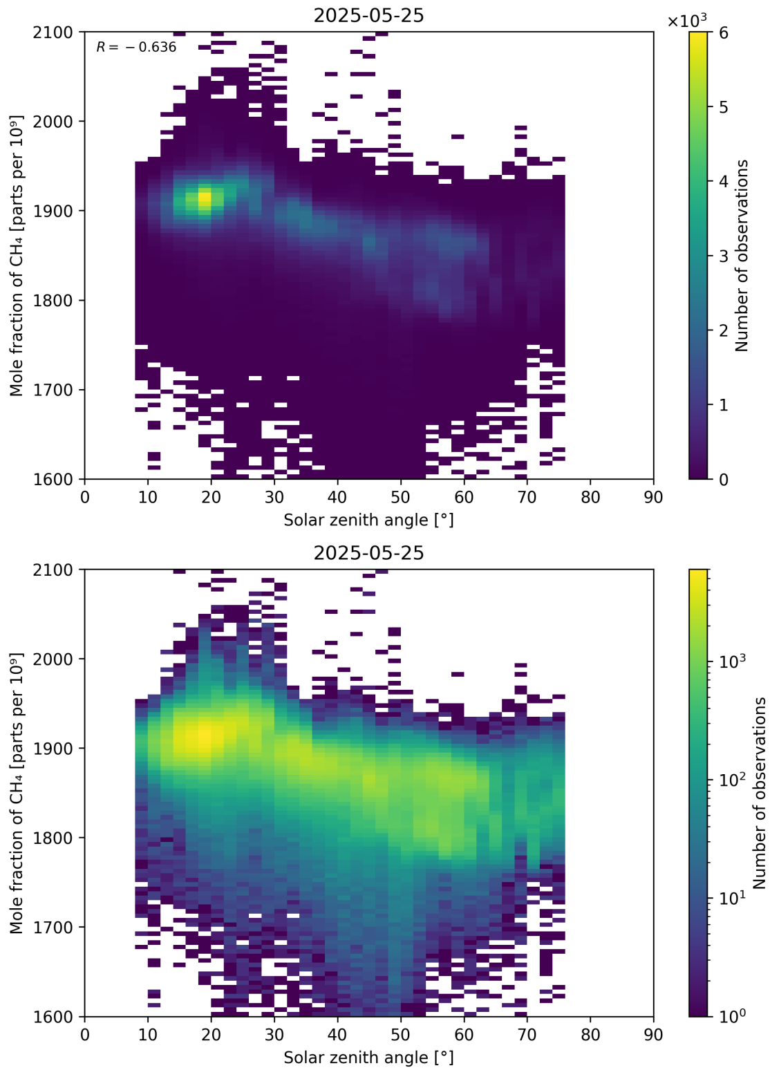
Figure 99: Scatter density plot of “Solar zenith angle” against “Mole fraction of \text{CH}_4 ” for 2025-05-24 to 2025-05-26.
