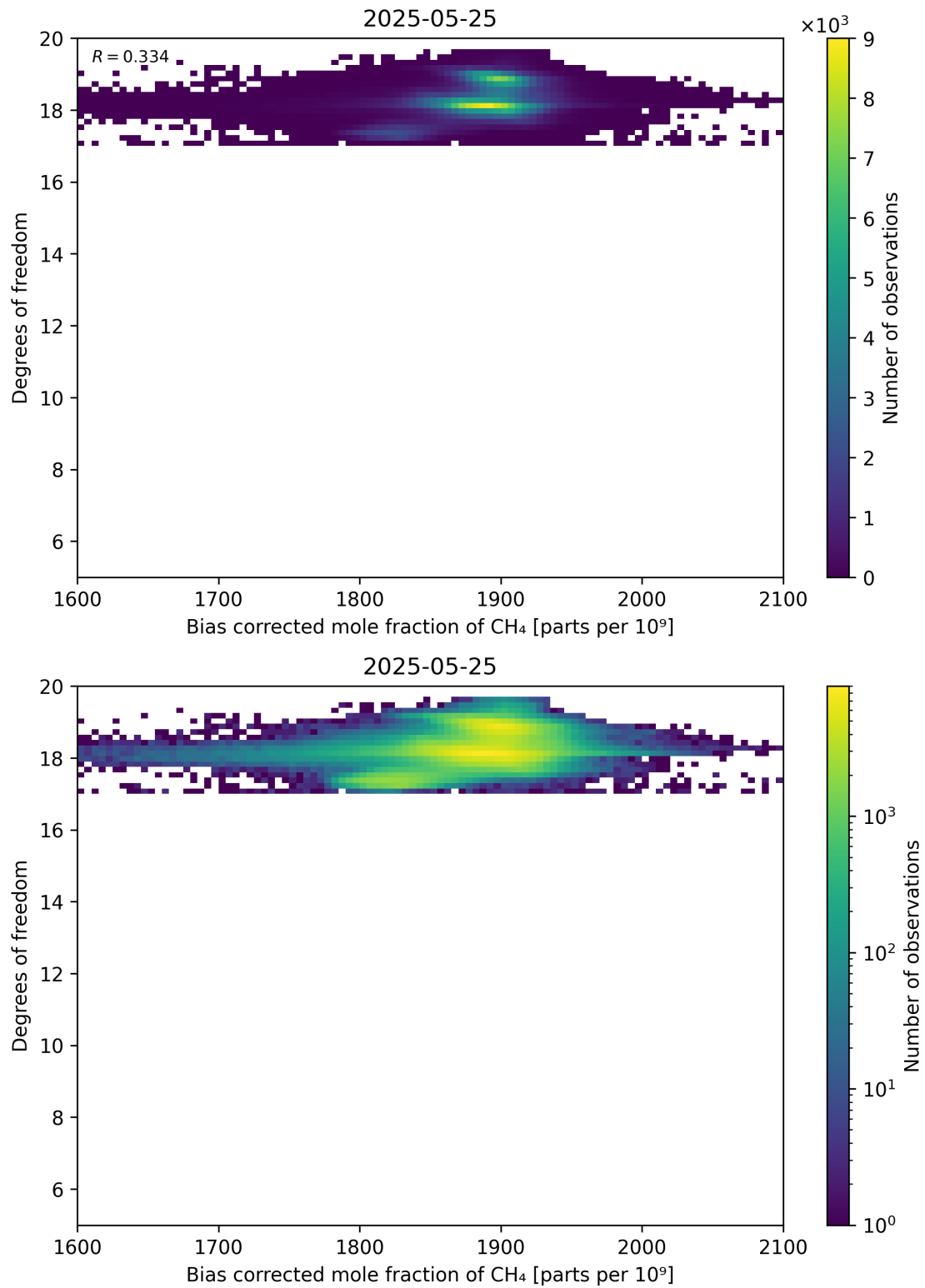
Figure 65: Scatter density plot of “Bias corrected mole fraction of CH 4 ” against “Degrees of freedom” for 2025-05-24 to 2025-05-26.
