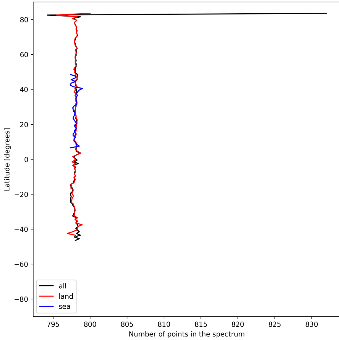
Figure 15: Zonal average of “Number of points in the spectrum” for 2025-05-24 to 2025-05-26.
