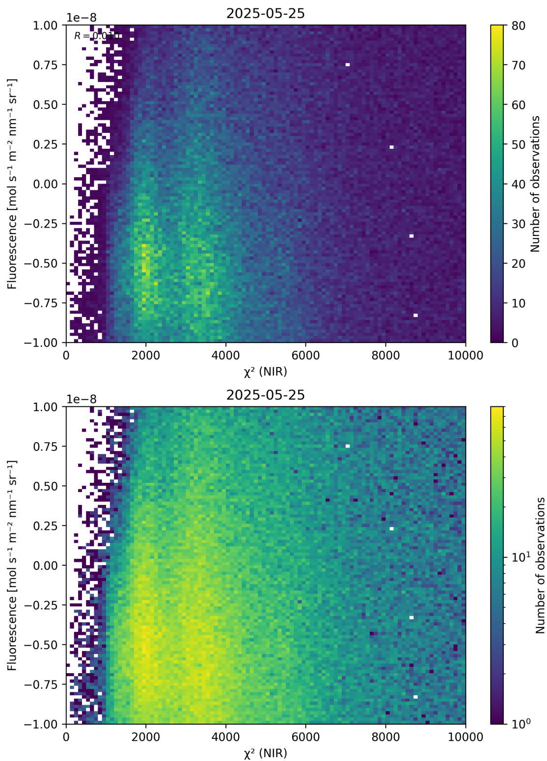
Figure 45: Scatter density plot of “ \chi^2 (NIR)” against “Fluorescence” for 2025-05-24 to 2025-05-26.
