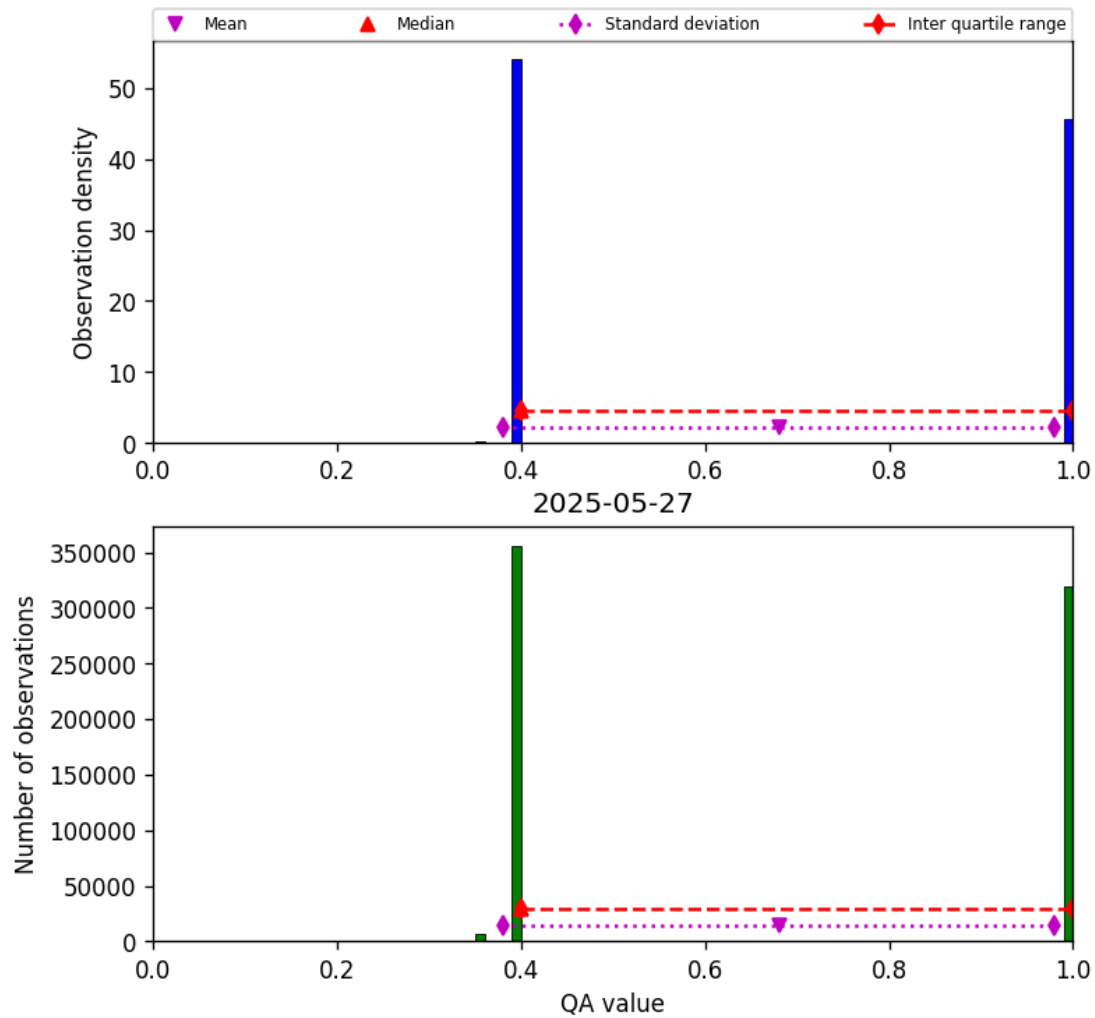
Figure 22: Histogram of “QA value” for 2025-05-26 to 2025-05-28
