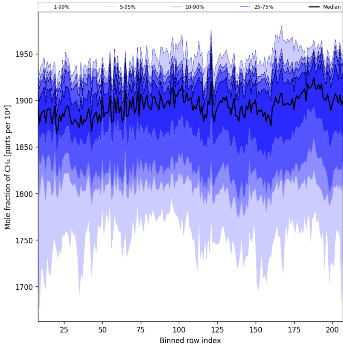
Figure 34: Along track statistics of “Mole fraction of CH 4 ” for 2025-05-26 to 2025-05-28
