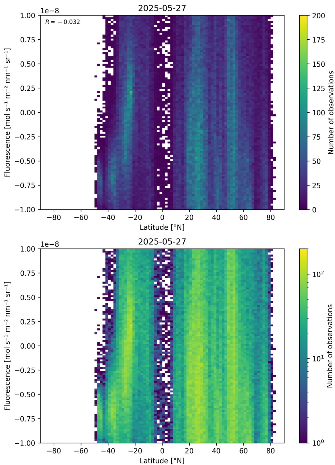
Figure 56: Scatter density plot of “Latitude” against “Fluorescence” for 2025-05-26 to 2025-05-28.
