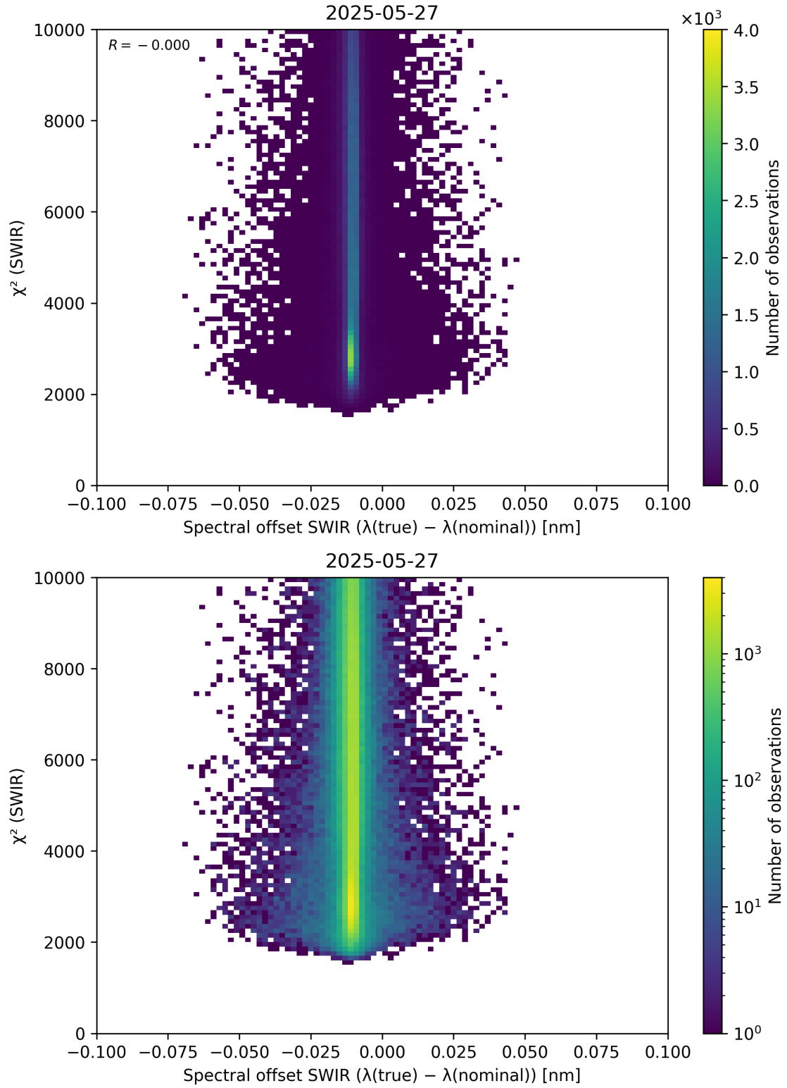
Figure 118: Scatter density plot of “Spectral offset SWIR ( \lambda_{\text{true}} - \lambda_{\text{nominal}} )” against “ \chi^2 (SWIR)” for 2025-05-26 to 2025-05-28.
