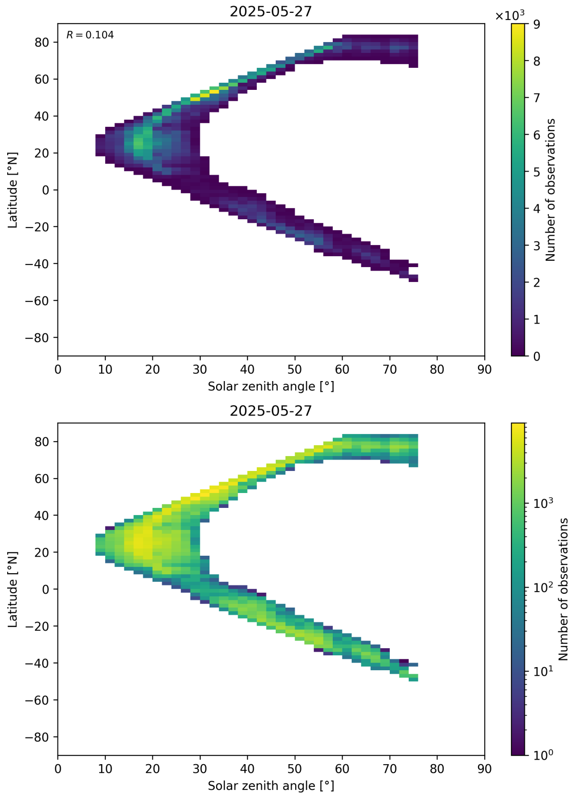
Figure 98: Scatter density plot of “Solar zenith angle” against “Latitude” for 2025-05-26 to 2025-05-28.
