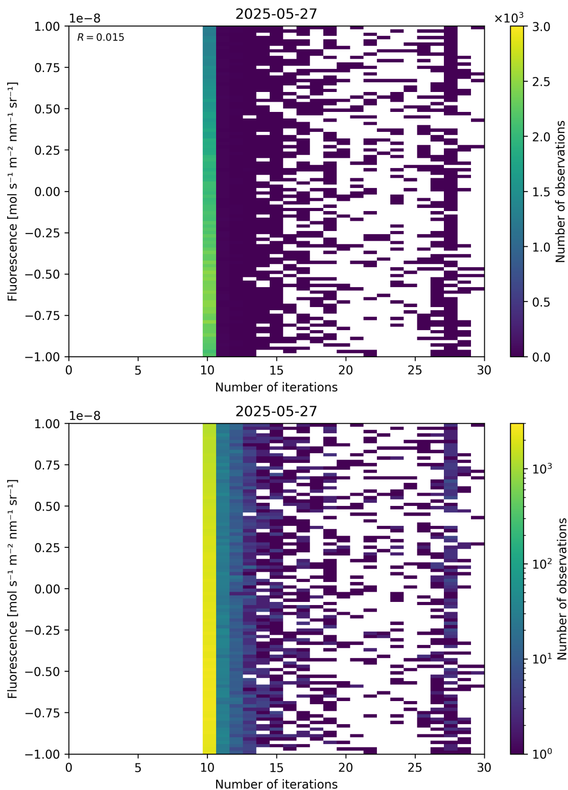
Figure 87: Scatter density plot of "Number of iterations" against "Fluorescence" for 2025-05-26 to 2025-05-28.
