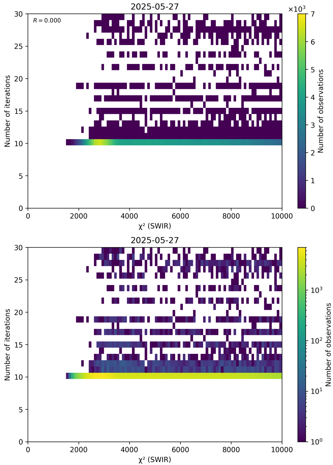
Figure 50: Scatter density plot of “ \chi^2 (SWIR)” against “Number of iterations” for 2025-05-26 to 2025-05-28.
