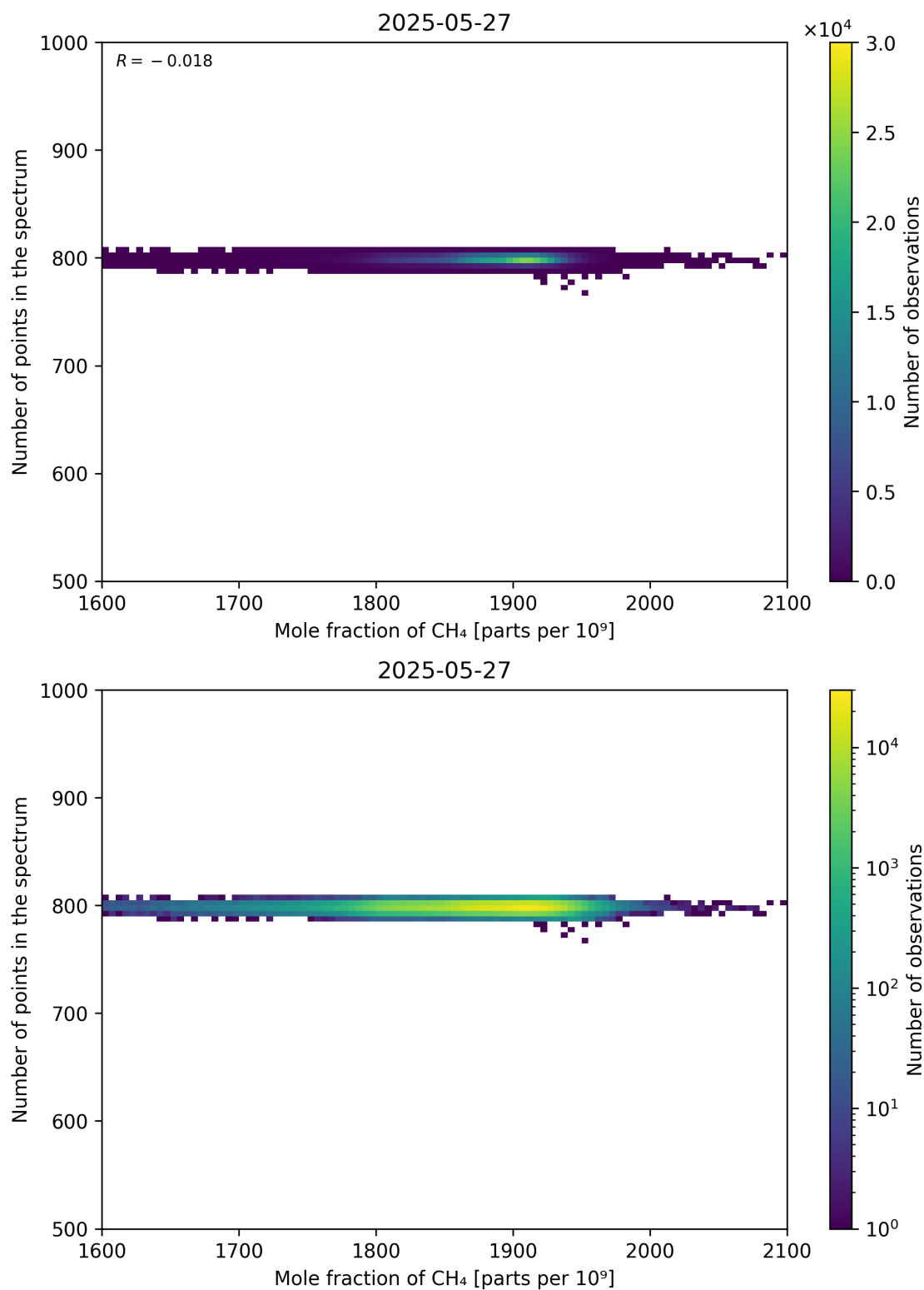
Figure 77: Scatter density plot of “Mole fraction of CH 4 ” against “Number of points in the spectrum” for 2025-05-26 to 2025-05-28.
