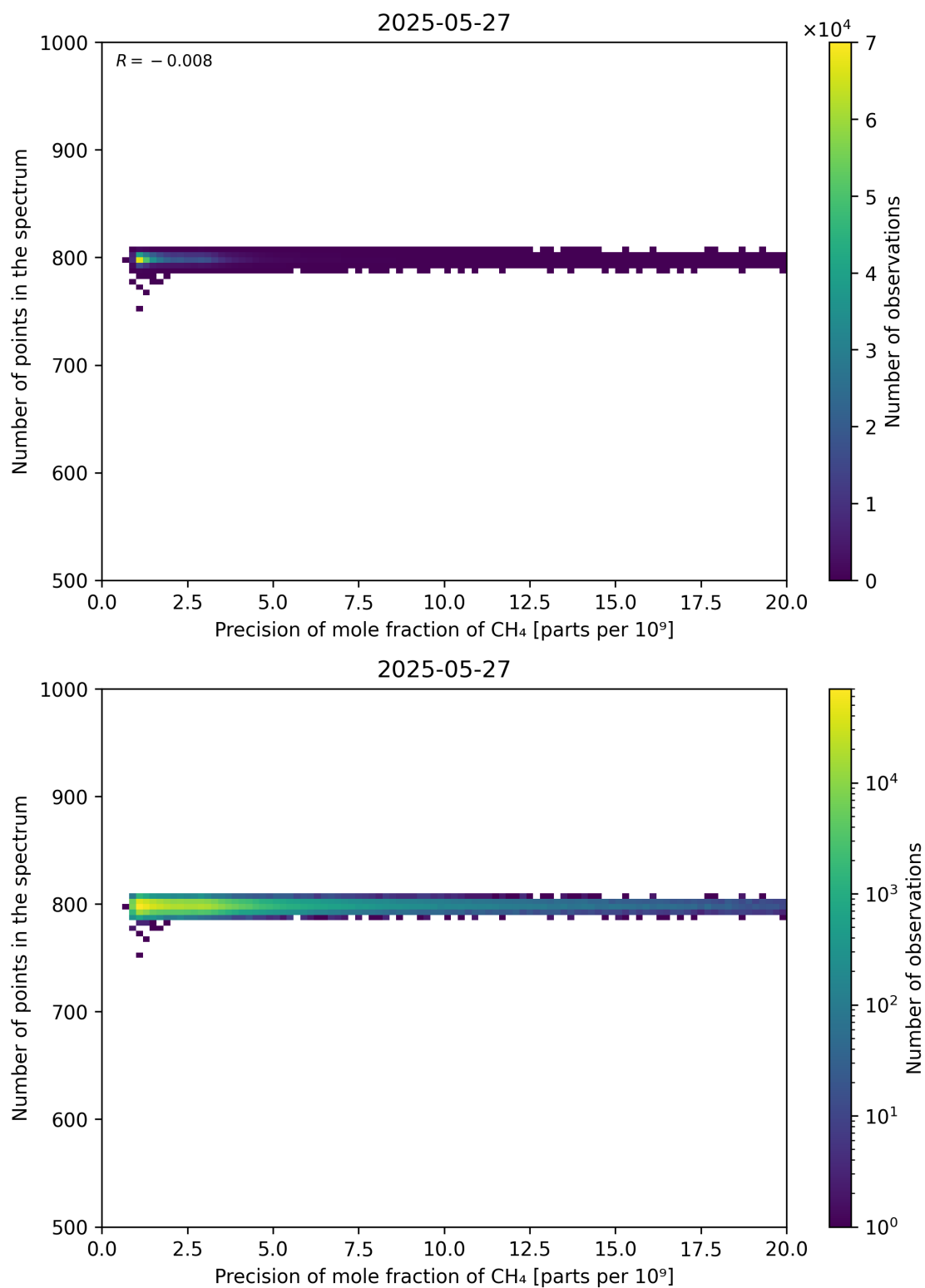
Figure 84: Scatter density plot of “Precision of mole fraction of CH 4 ” against “Number of points in the spectrum” for 2025-05-26 to 2025-05-28.
