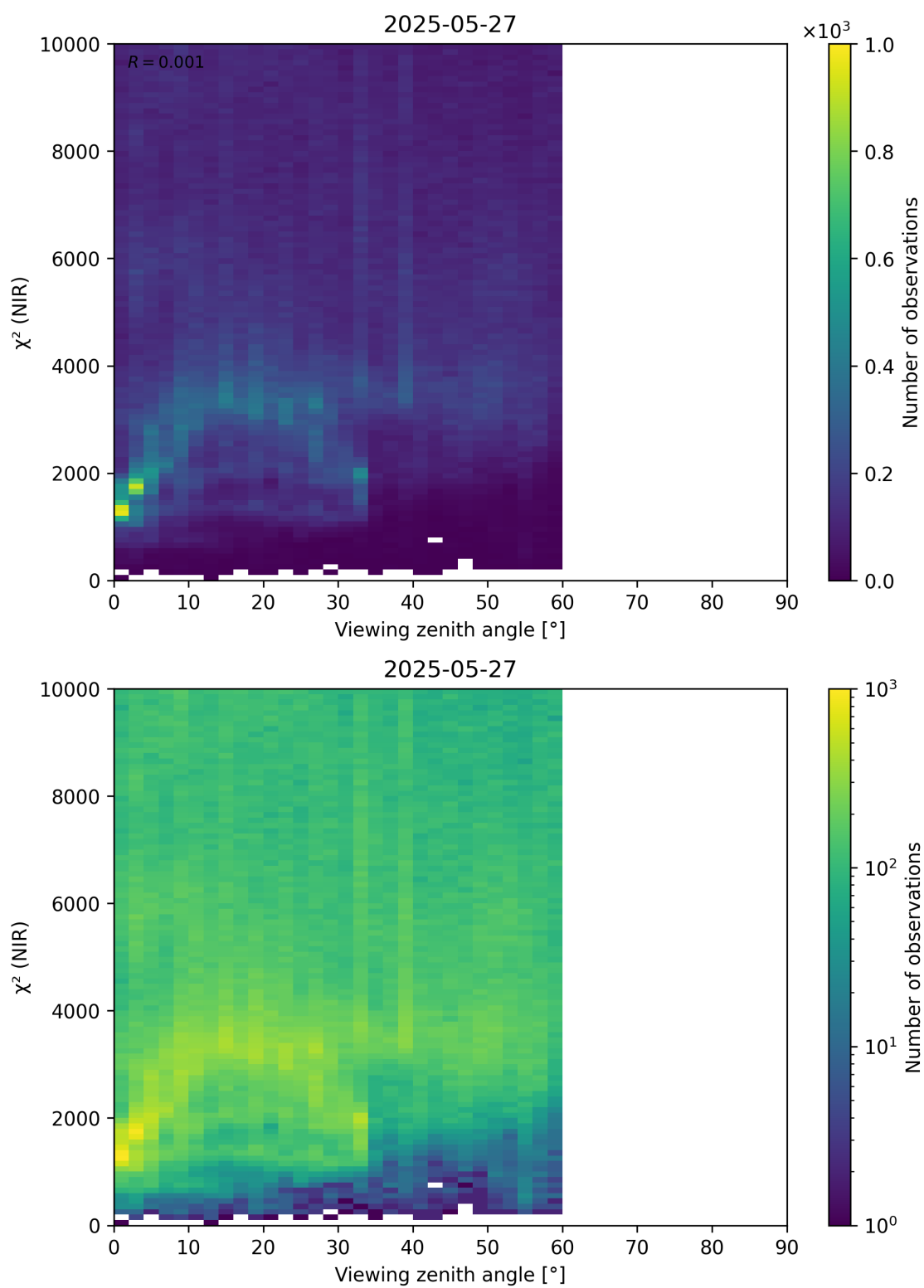
Figure 105: Scatter density plot of “Viewing zenith angle” against “ \chi^2 (NIR)” for 2025-05-26 to 2025-05-28.
