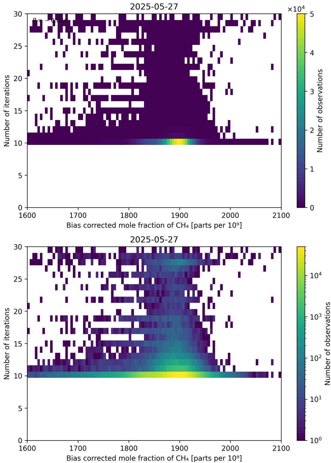
Figure 67: Scatter density plot of “Bias corrected mole fraction of \text{CH}_4 ” against “Number of iterations” for 2025-05-26 to 2025-05-28.
