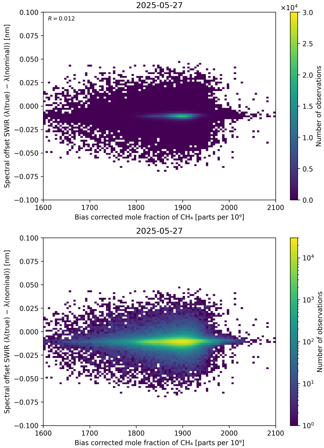
Figure 69: Scatter density plot of “Bias corrected mole fraction of CH 4 ” against “Spectral offset SWIR ( \lambda_{\text{true}} - \lambda_{\text{nominal}} )” for 2025-05-26 to 2025-05-28.
