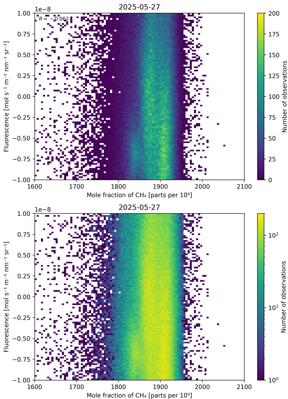
Figure 73: Scatter density plot of “Mole fraction of \text{CH}_4 ” against “Fluorescence” for 2025-05-26 to 2025-05-28.
