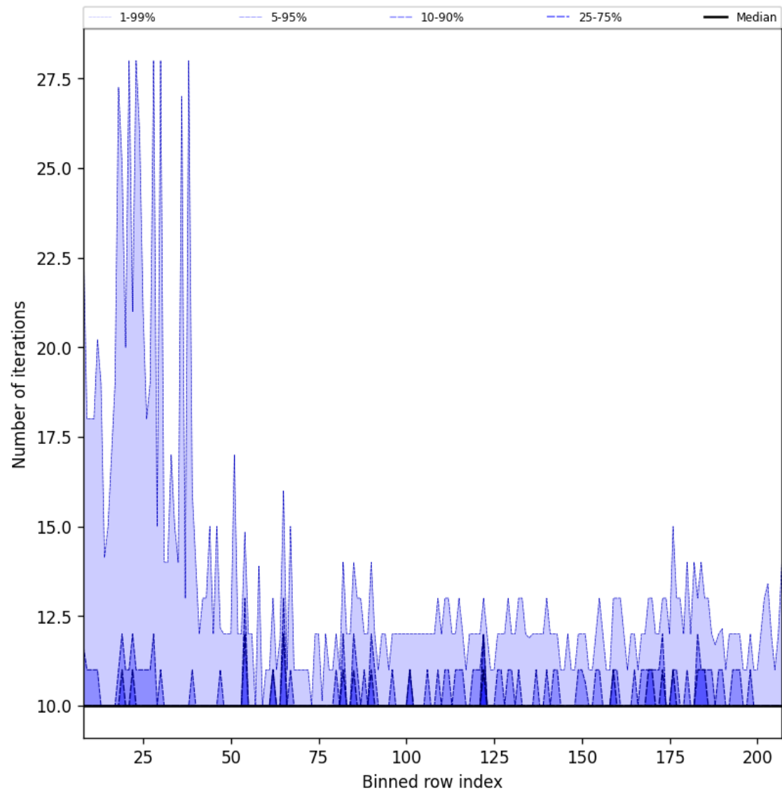
Figure 42: Along track statistics of “Number of iterations” for 2025-05-26 to 2025-05-28
