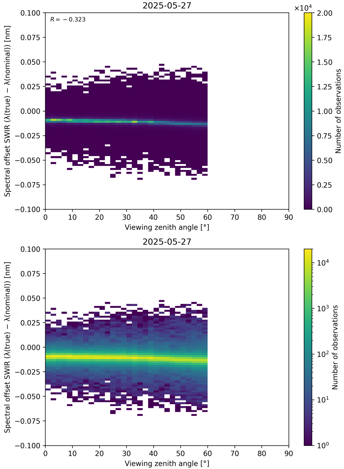
Figure 116: Scatter density plot of “Viewing zenith angle” against “Spectral offset SWIR ( \lambda_{\text{true}} - \lambda_{\text{nominal}} )” for 2025-05-26 to 2025-05-28.
