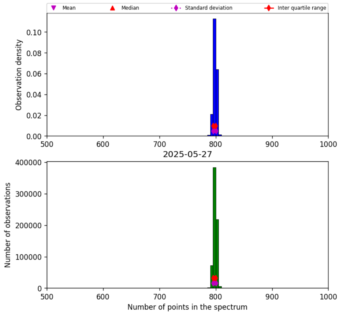
Figure 26: Histogram of “Number of points in the spectrum” for 2025-05-26 to 2025-05-28
