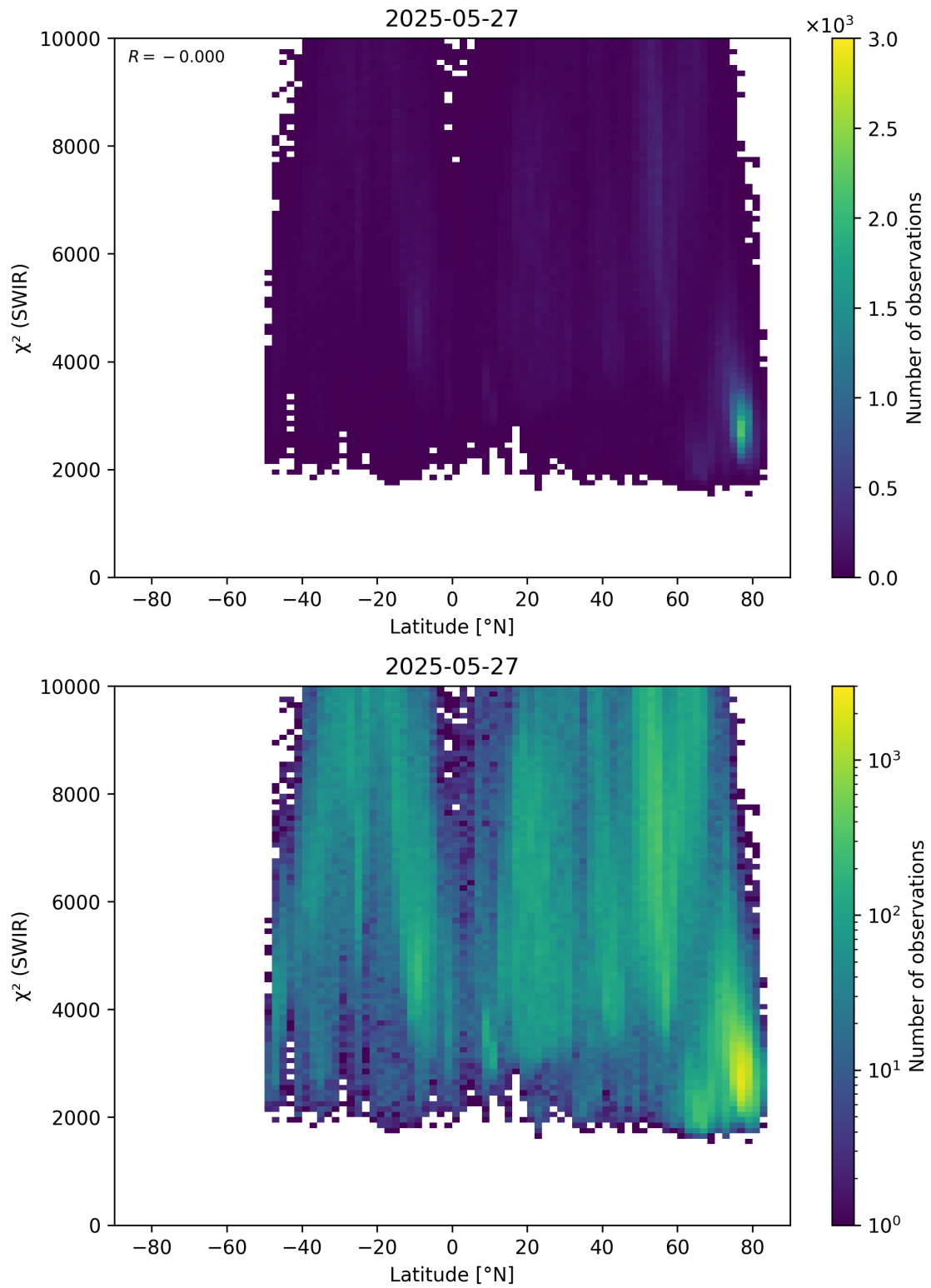
Figure 54: Scatter density plot of “Latitude” against “ \chi^2 (SWIR)” for 2025-05-26 to 2025-05-28.
