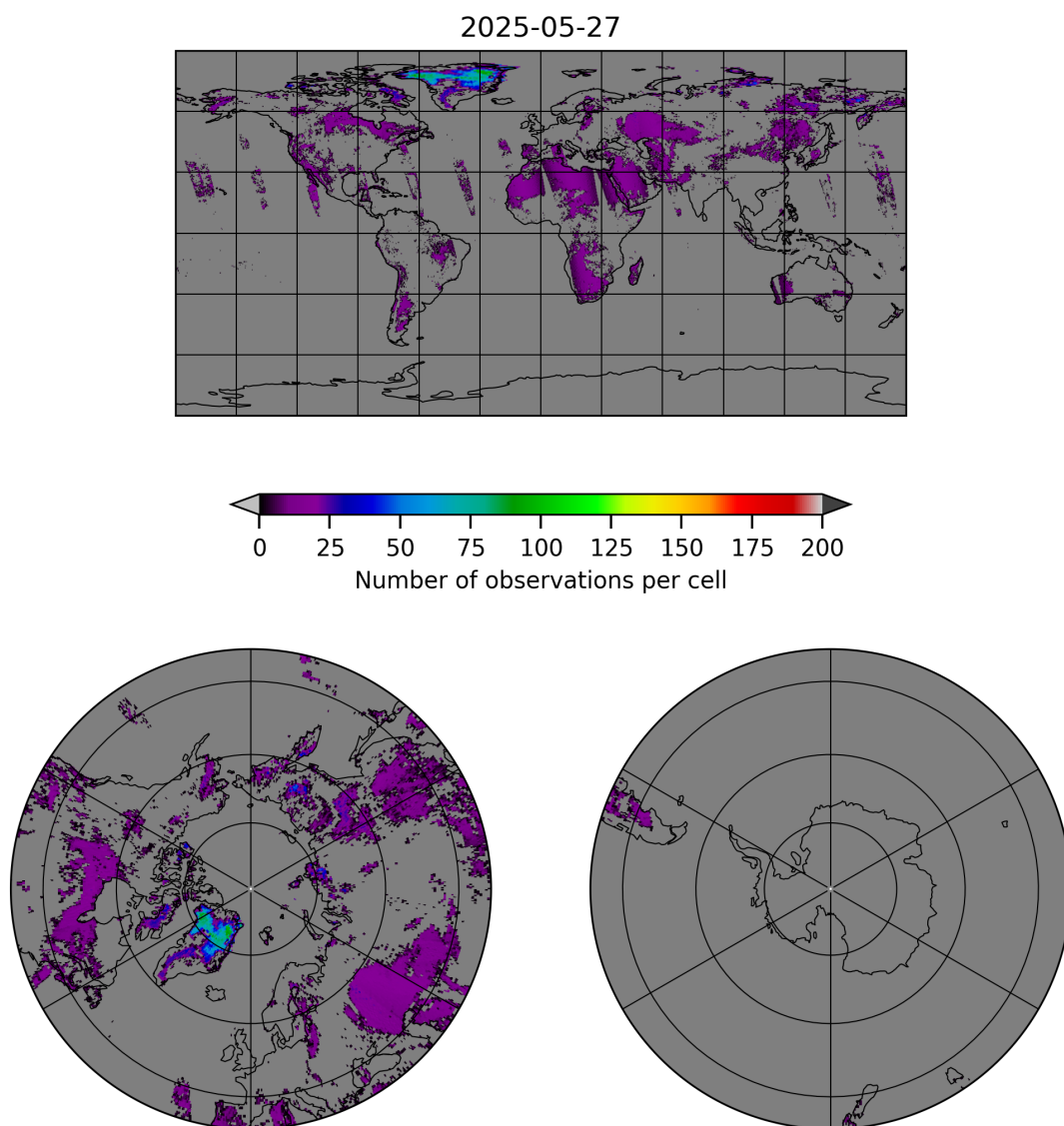
Figure 10: Map of the number of observations for 2025-05-26 to 2025-05-28
