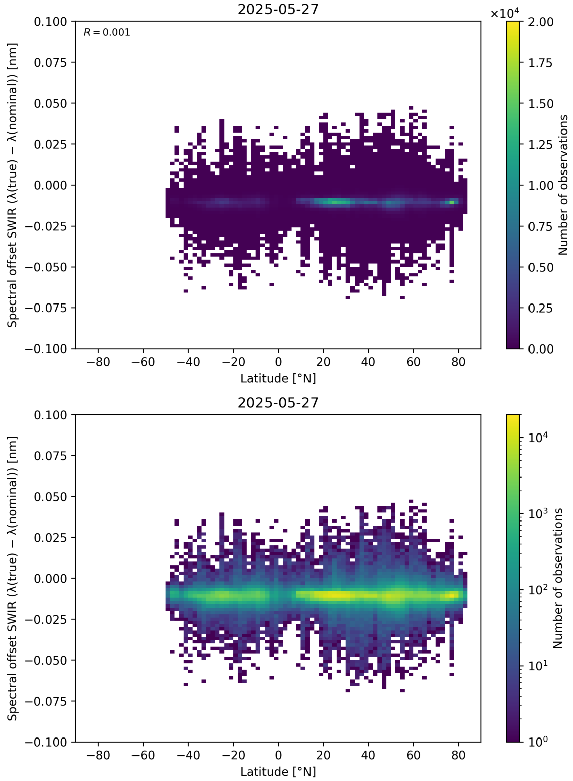
Figure 62: Scatter density plot of “Latitude” against “Spectral offset SWIR ( \lambda_{\text{true}} - \lambda_{\text{nominal}} )” for 2025-05-26 to 2025-05-28.
