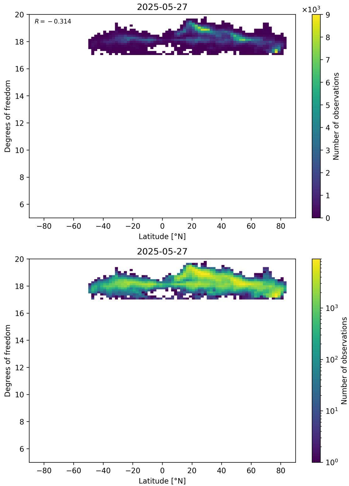
Figure 55: Scatter density plot of “Latitude” against “Degrees of freedom” for 2025-05-26 to 2025-05-28.
