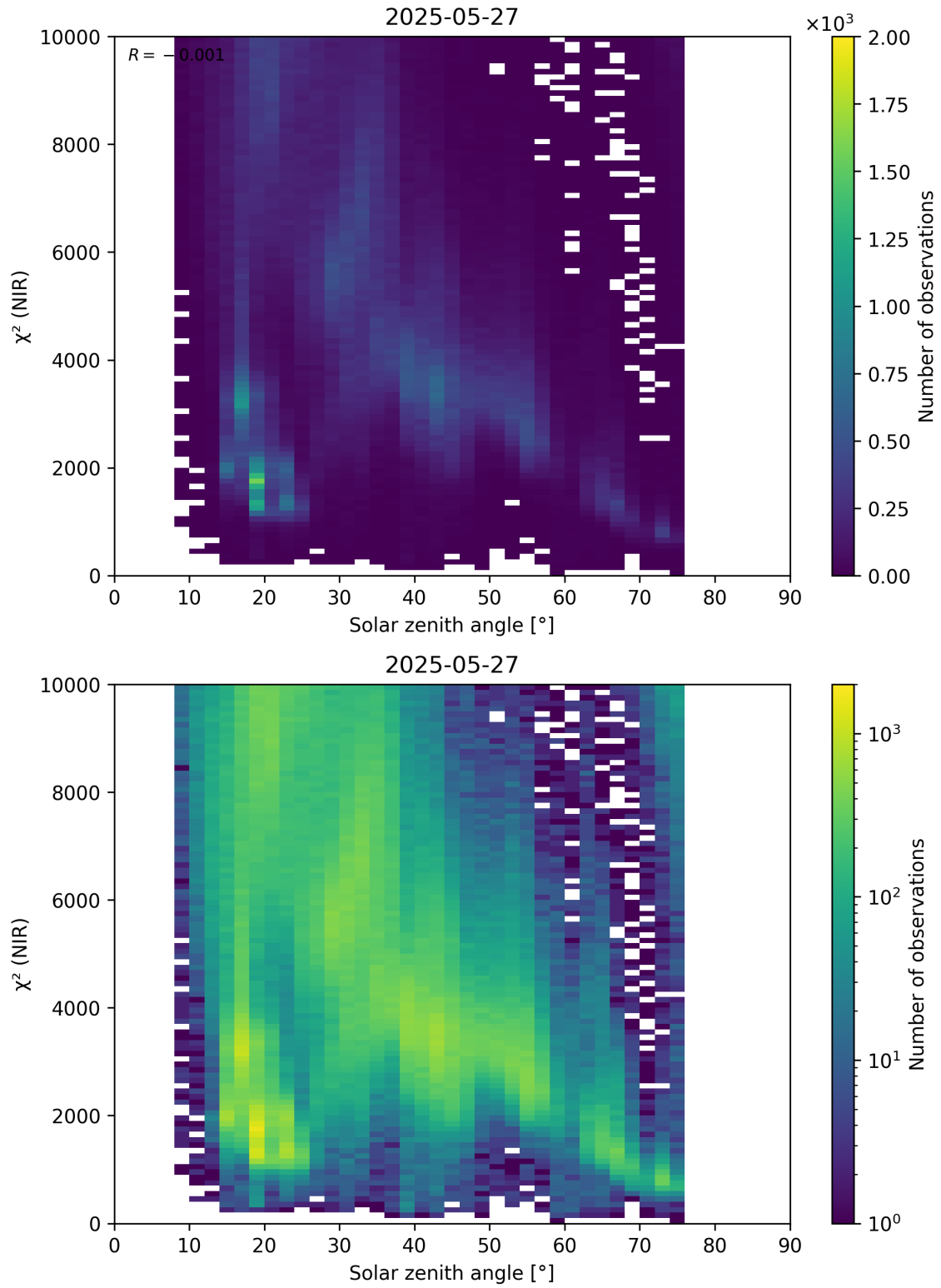
Figure 94: Scatter density plot of “Solar zenith angle” against “ \chi^2 (NIR)” for 2025-05-26 to 2025-05-28.
