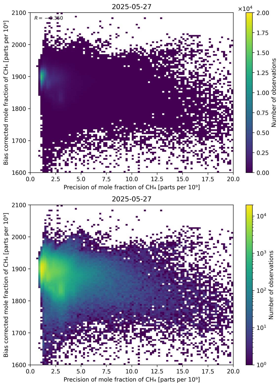
Figure 82: Scatter density plot of “Precision of mole fraction of CH 4 ” against “Bias corrected mole fraction of CH 4 ” for 2025-05-26 to 2025-05-28.
