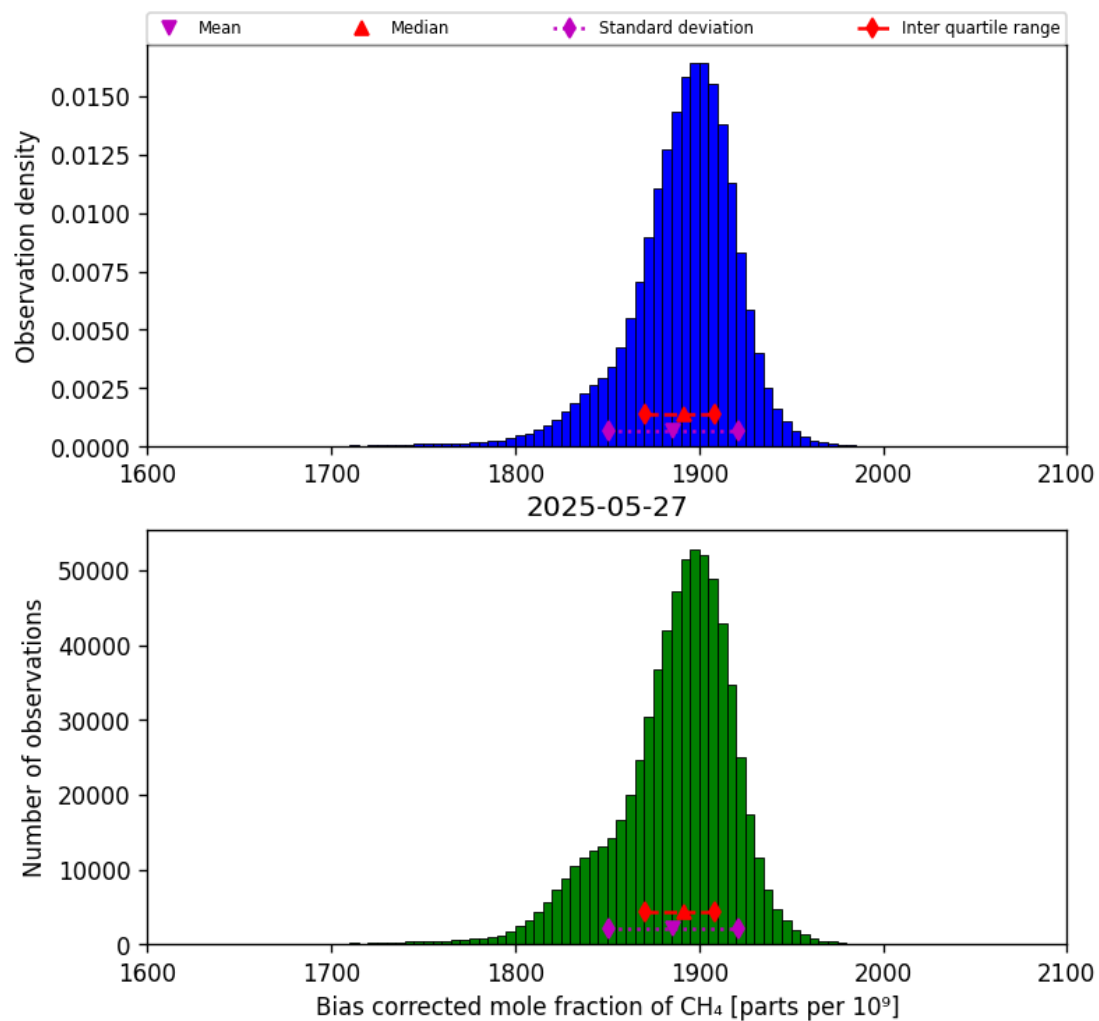
Figure 25: Histogram of “Bias corrected mole fraction of CH 4 ” for 2025-05-26 to 2025-05-28
