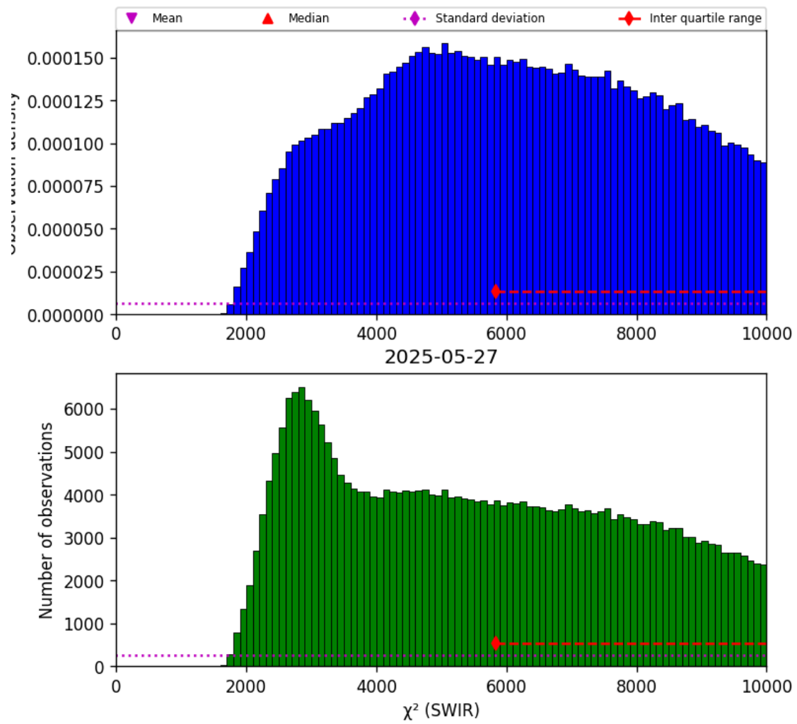
Figure 28: Histogram of “ \chi^2 (SWIR)” for 2025-05-26 to 2025-05-28
