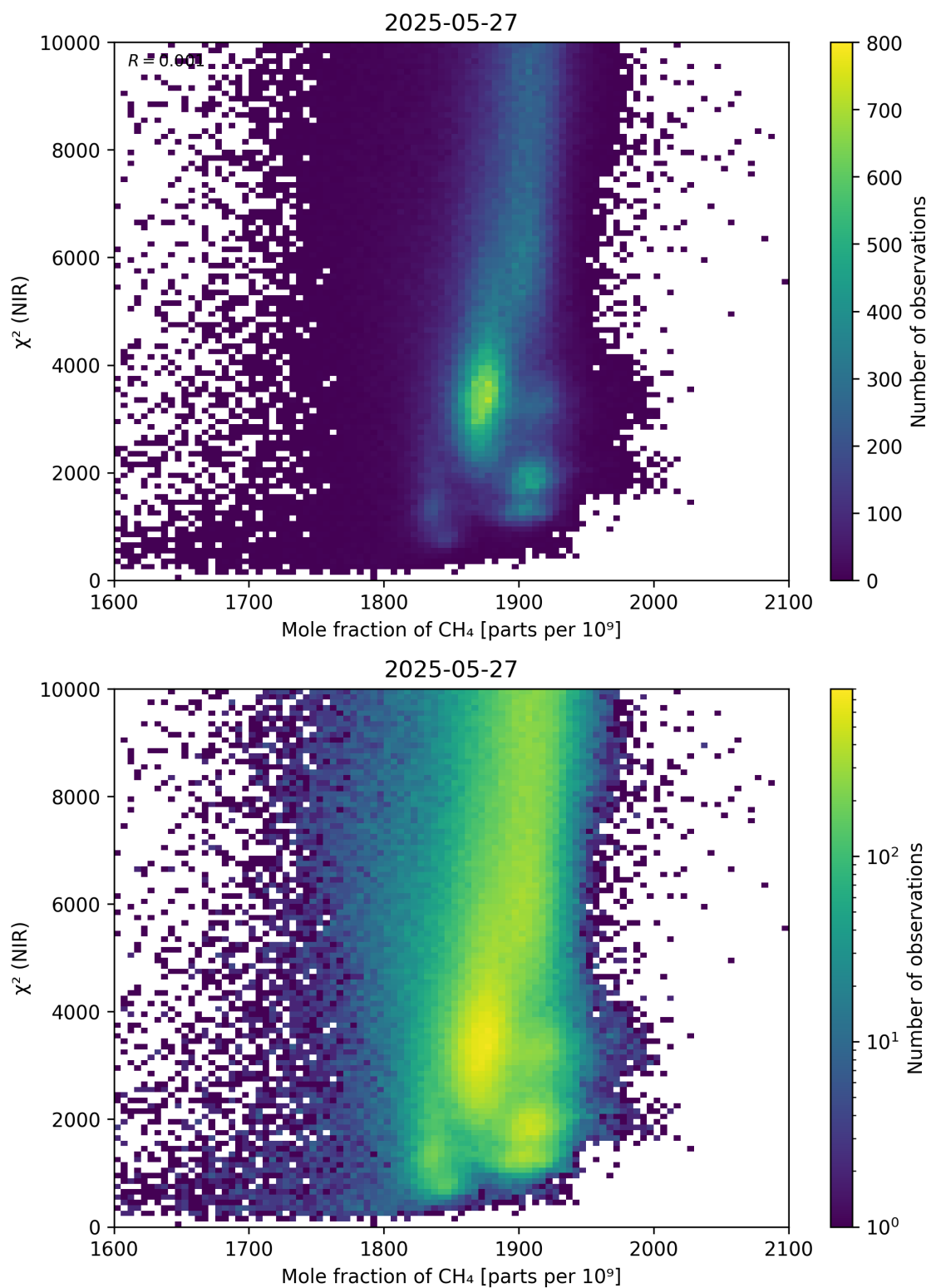
Figure 70: Scatter density plot of “Mole fraction of \text{CH}_4 ” against “ \chi^2 (NIR)” for 2025-05-26 to 2025-05-28.
