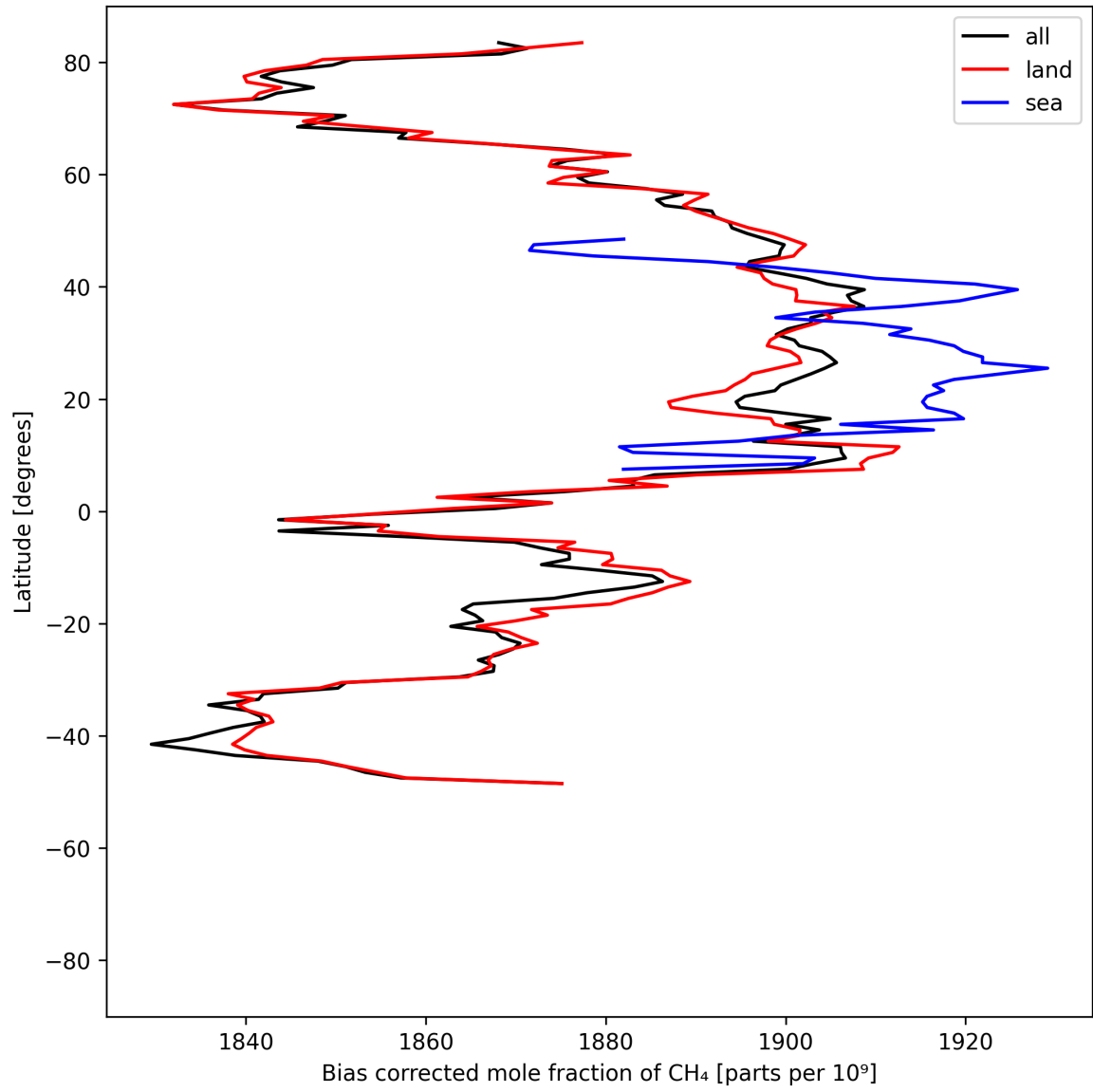
Figure 14: Zonal average of “Bias corrected mole fraction of CH 4 ” for 2025-05-26 to 2025-05-28.
