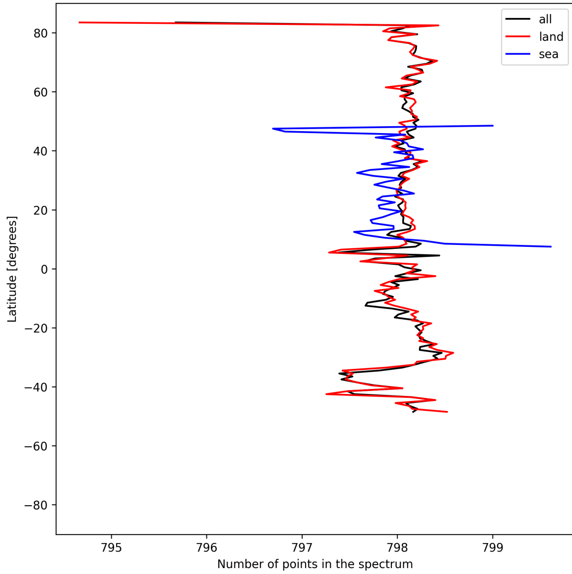
Figure 15: Zonal average of “Number of points in the spectrum” for 2025-05-26 to 2025-05-28.
