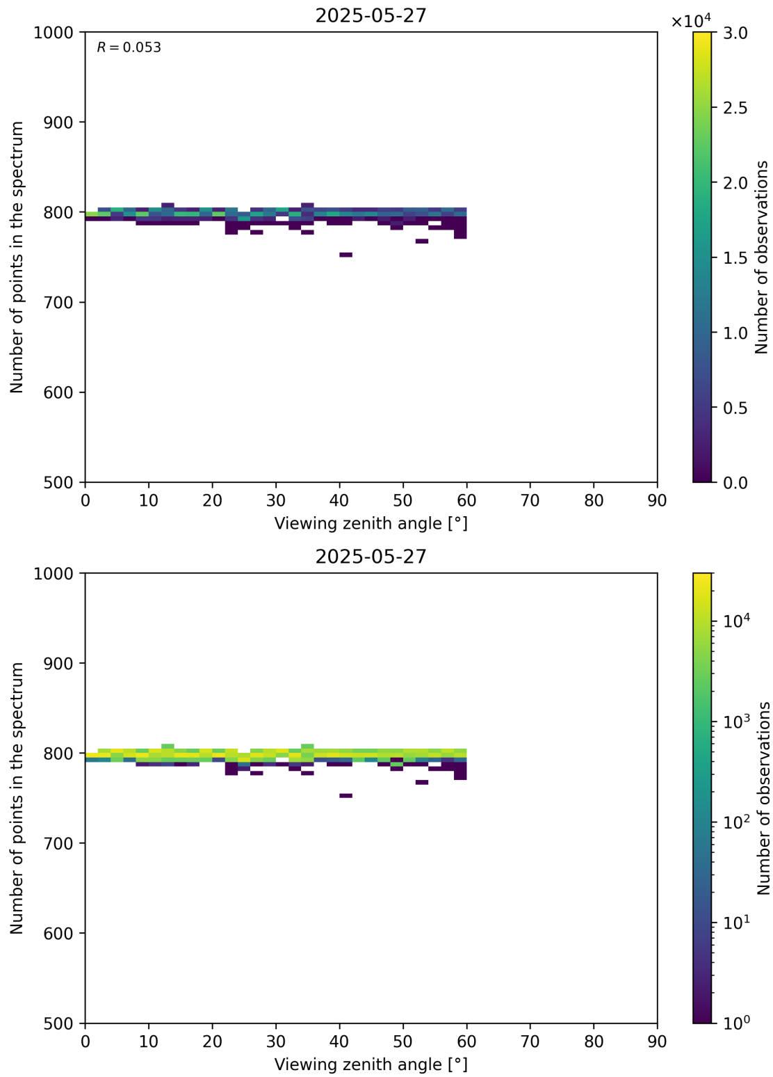
Figure 114: Scatter density plot of “Viewing zenith angle” against “Number of points in the spectrum” for 2025-05-26 to 2025-05-28.
