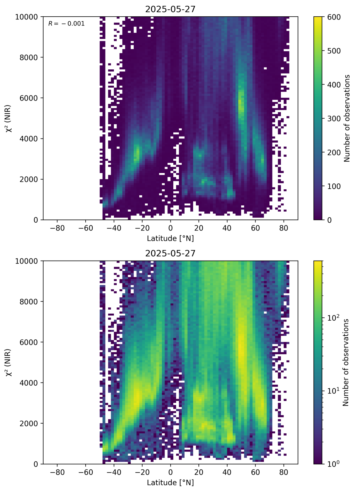
Figure 53: Scatter density plot of “Latitude” against “ \chi^2 (NIR)” for 2025-05-26 to 2025-05-28.
