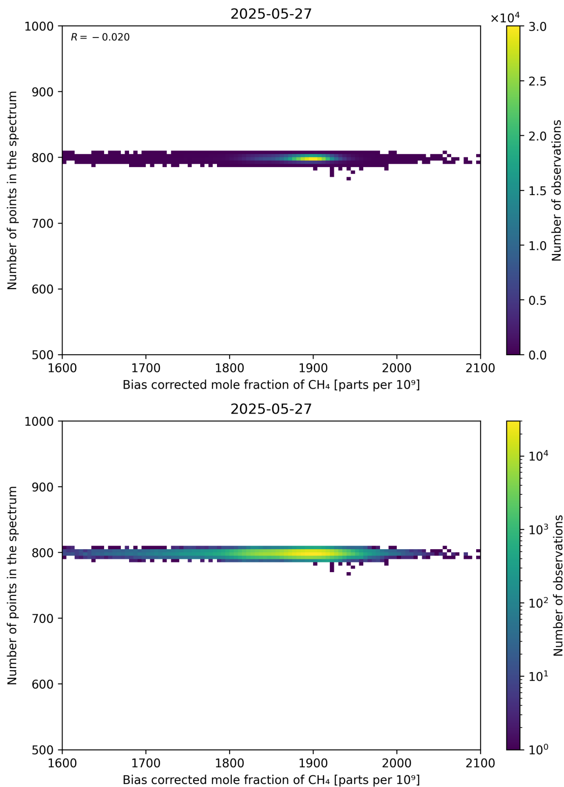
Figure 68: Scatter density plot of “Bias corrected mole fraction of CH 4 ” against “Number of points in the spectrum” for 2025-05-26 to 2025-05-28.
