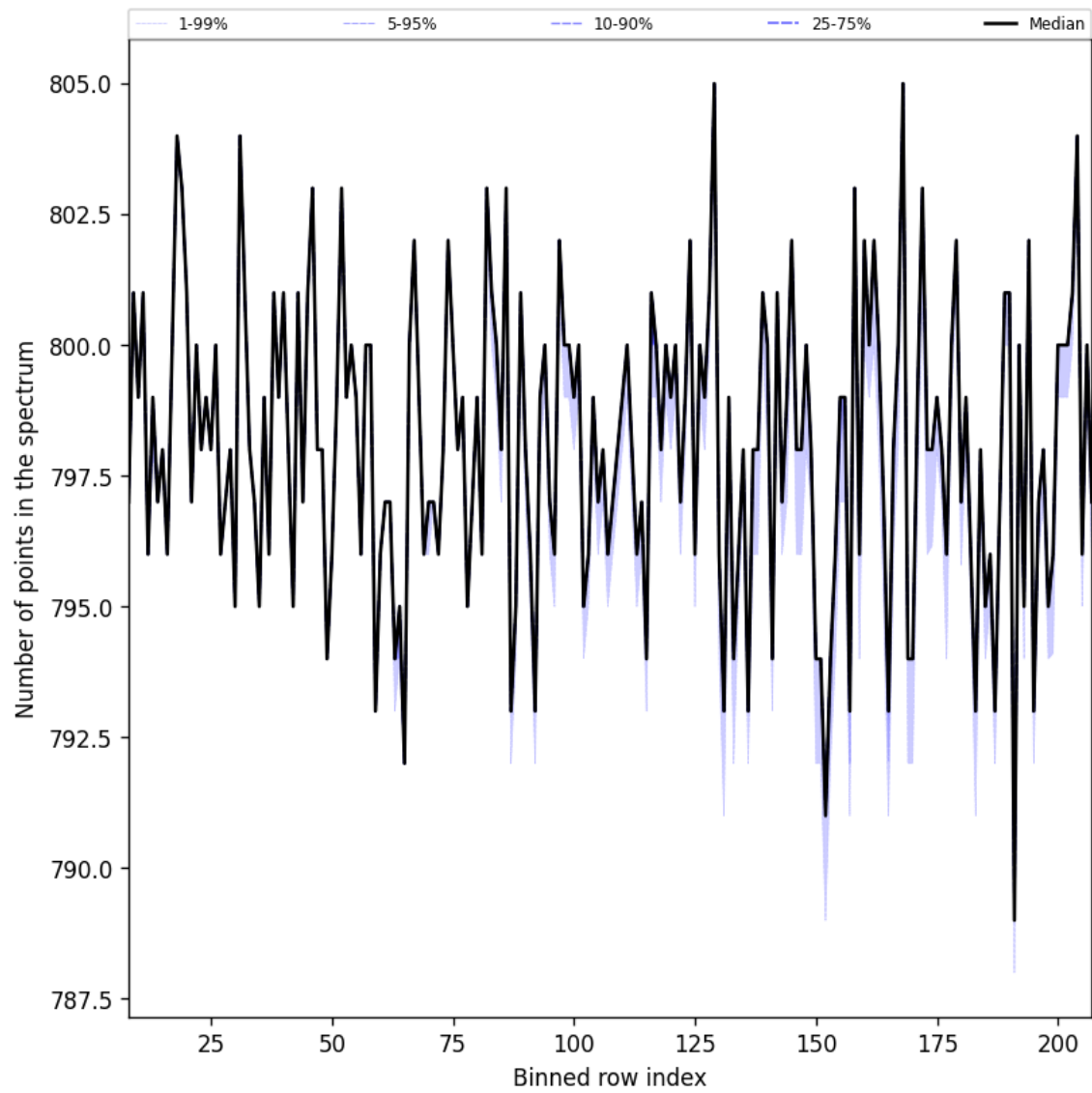
Figure 37: Along track statistics of “Number of points in the spectrum” for 2025-05-26 to 2025-05-28
