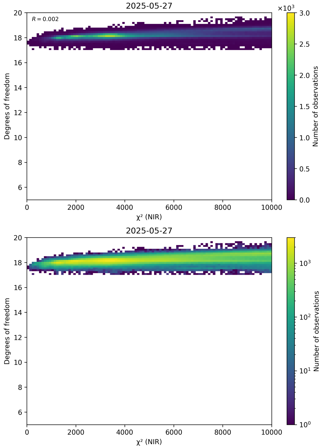
Figure 44: Scatter density plot of “ \chi^2 (NIR)” against “Degrees of freedom” for 2025-05-26 to 2025-05-28.
