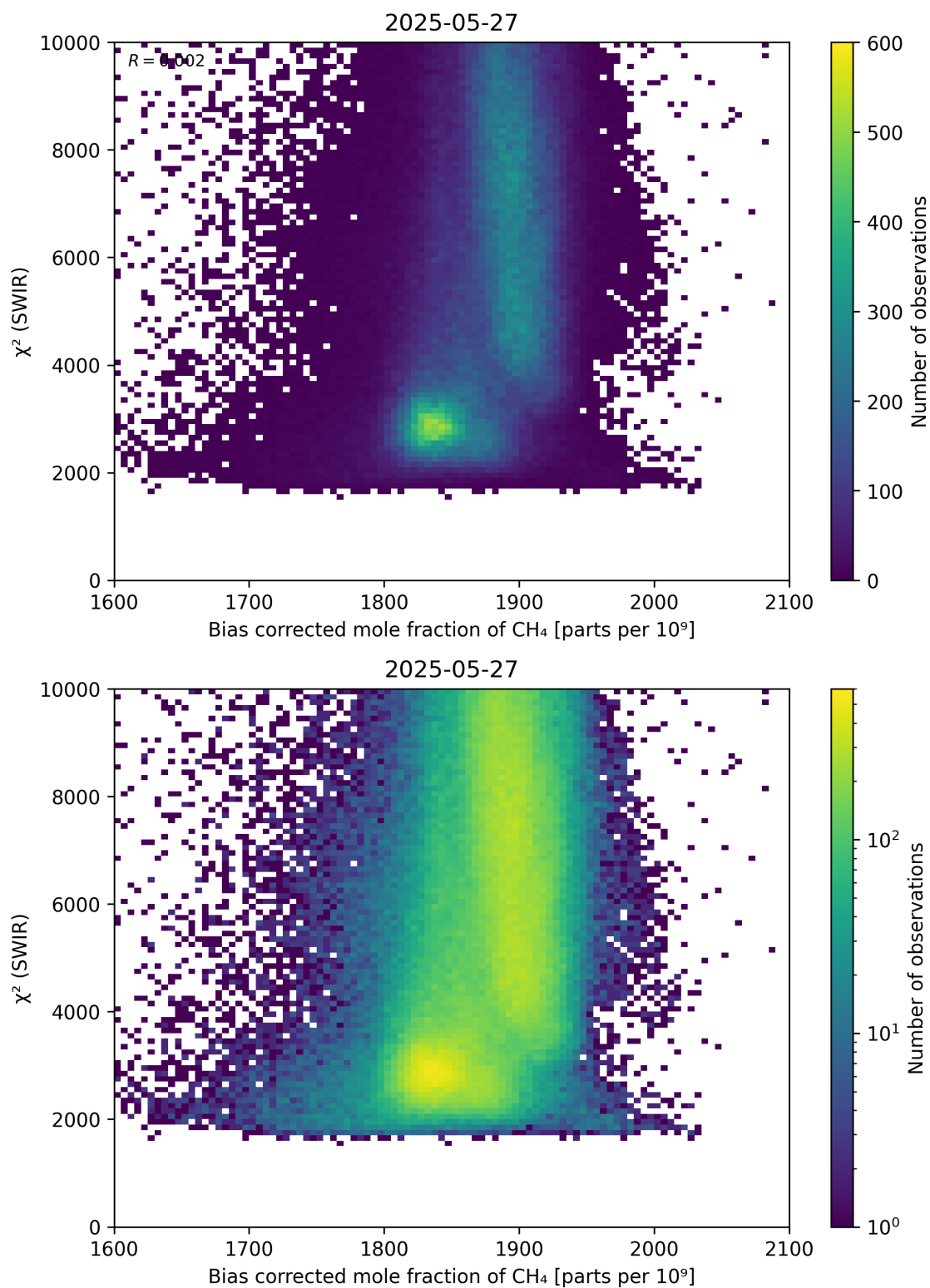
Figure 64: Scatter density plot of “Bias corrected mole fraction of \text{CH}_4 ” against “ \chi^2 (SWIR)” for 2025-05-26 to 2025-05-28.
