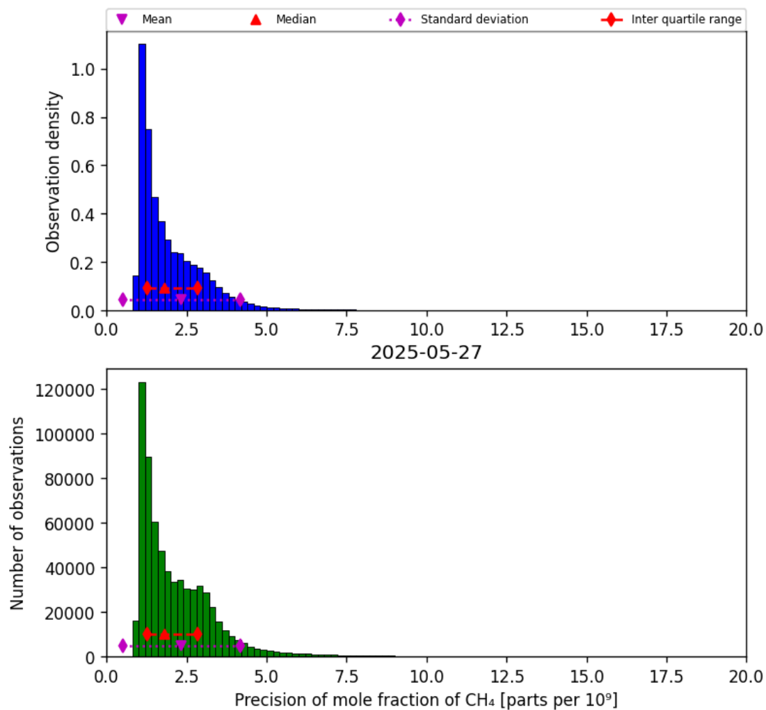
Figure 24: Histogram of “Precision of mole fraction of CH 4 ” for 2025-05-26 to 2025-05-28
