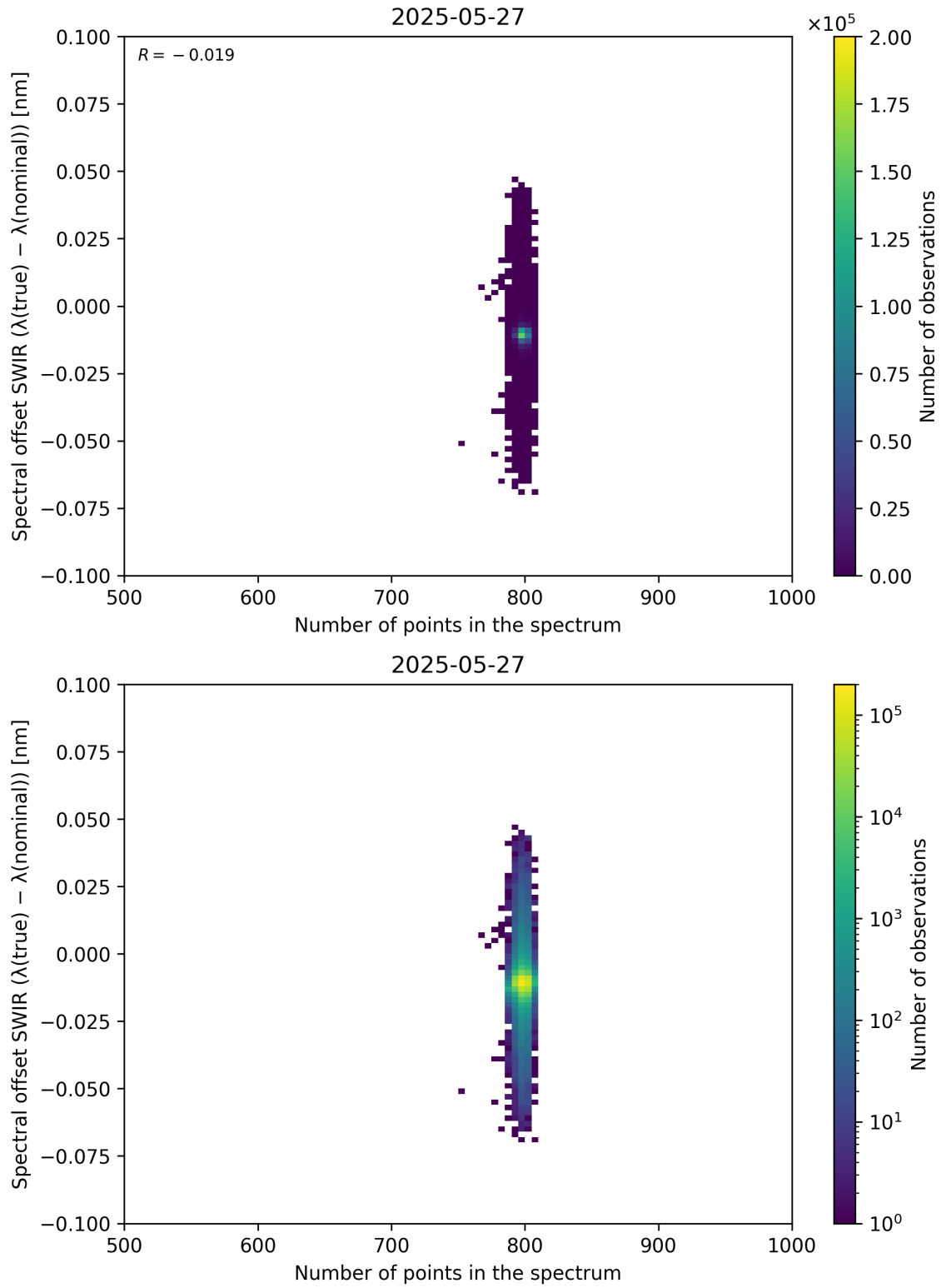
Figure 93: Scatter density plot of “Number of points in the spectrum” against “Spectral offset SWIR ( \lambda_{\text{true}} - \lambda_{\text{nominal}} )” for 2025-05-26 to 2025-05-28.
