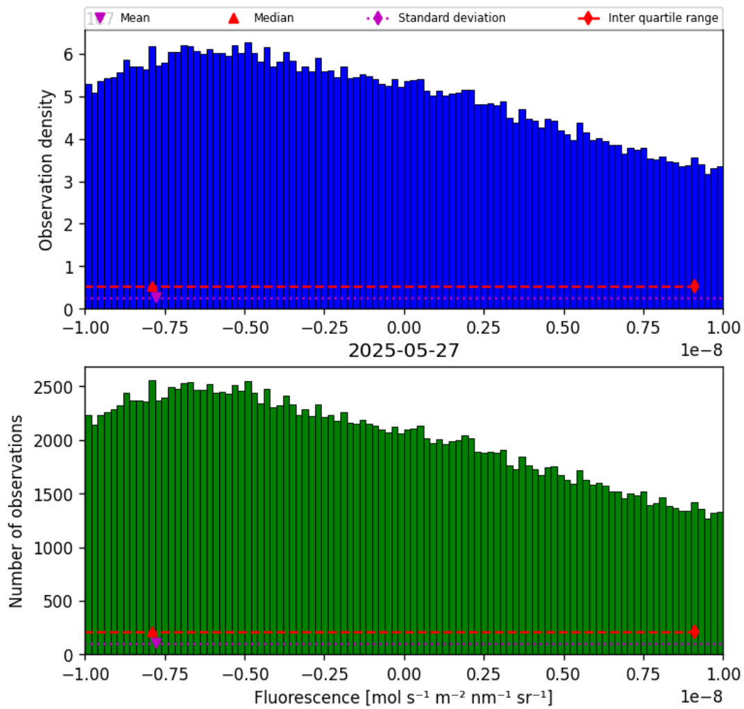
Figure 32: Histogram of “Fluorescence” for 2025-05-26 to 2025-05-28
