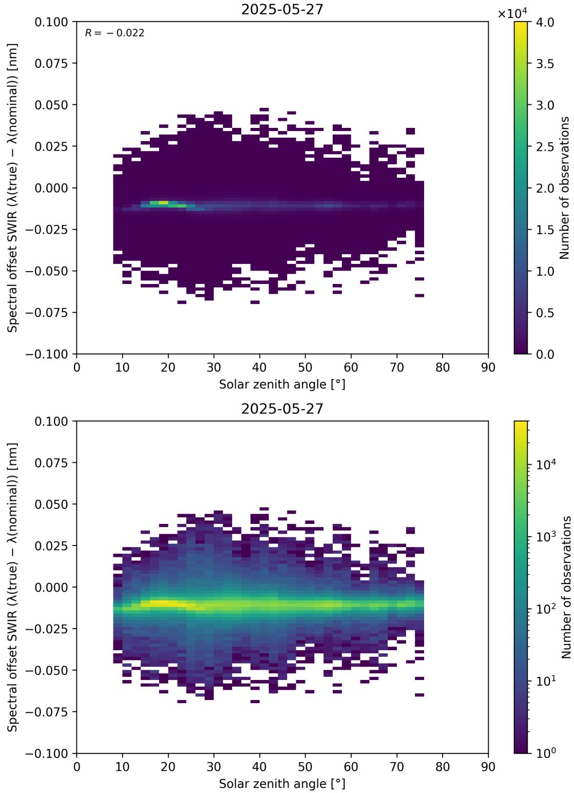
Figure 104: Scatter density plot of “Solar zenith angle” against “Spectral offset SWIR ( \lambda_{\text{true}} - \lambda_{\text{nominal}} )” for 2025-05-26 to 2025-05-28.
