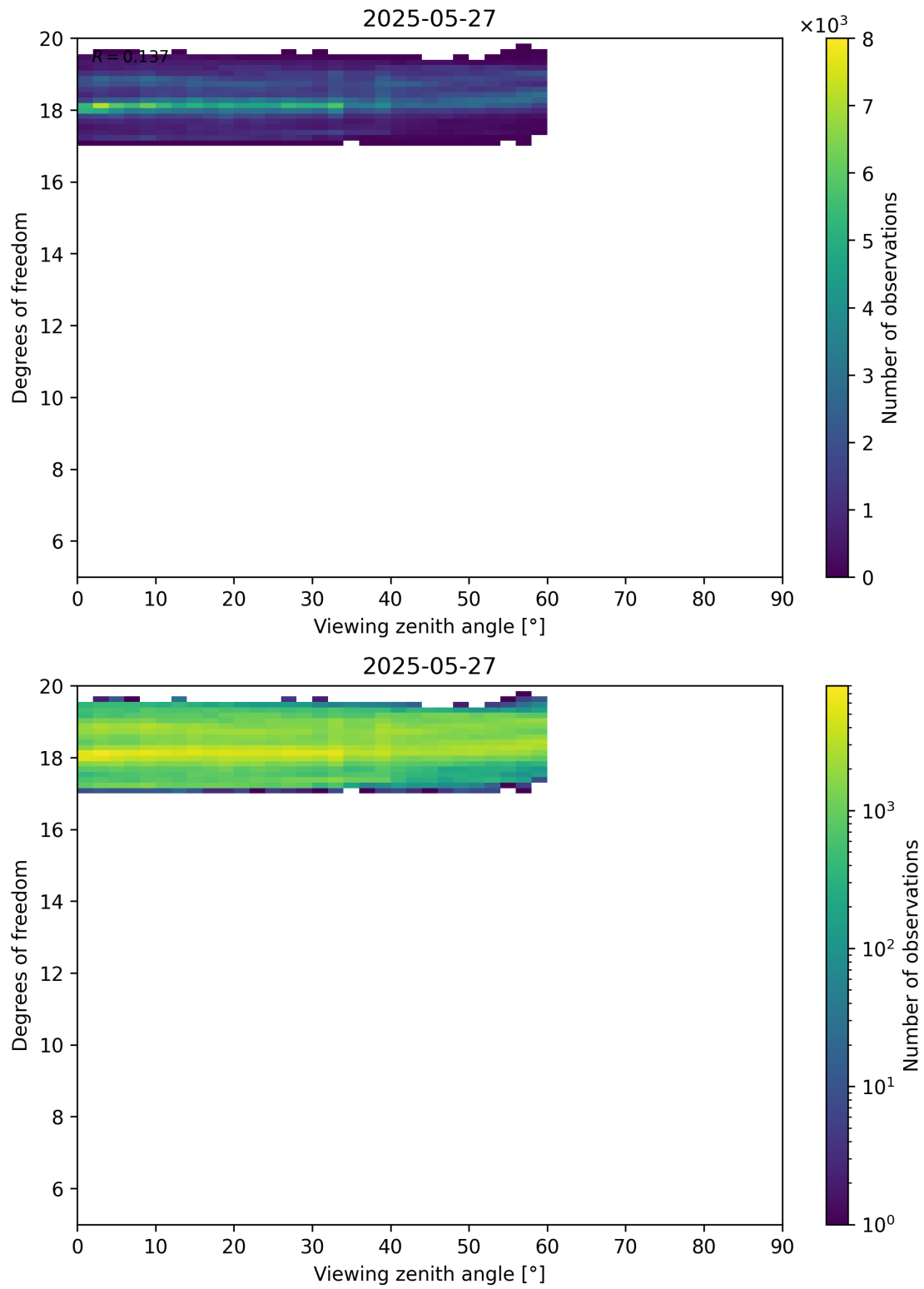
Figure 107: Scatter density plot of “Viewing zenith angle” against “Degrees of freedom” for 2025-05-26 to 2025-05-28.
