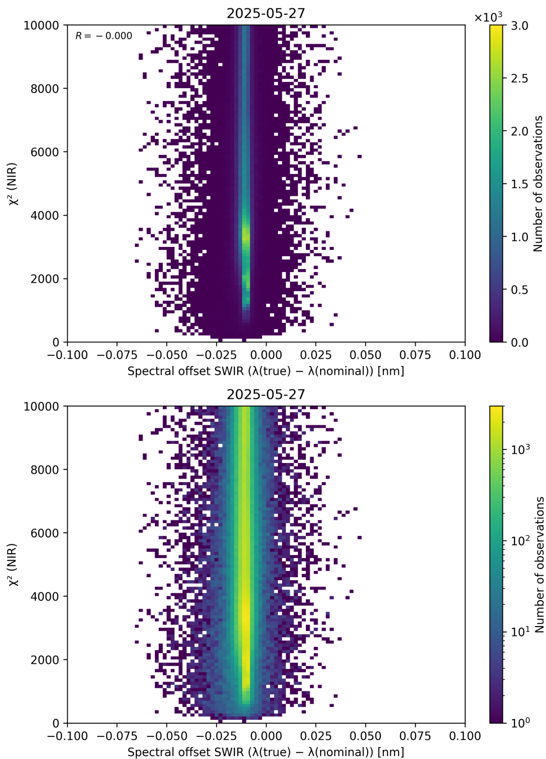
Figure 117: Scatter density plot of “Spectral offset SWIR ( \lambda_{\text{true}} - \lambda_{\text{nominal}} )” against “ \chi^2 (NIR)” for 2025-05-26 to 2025-05-28.
