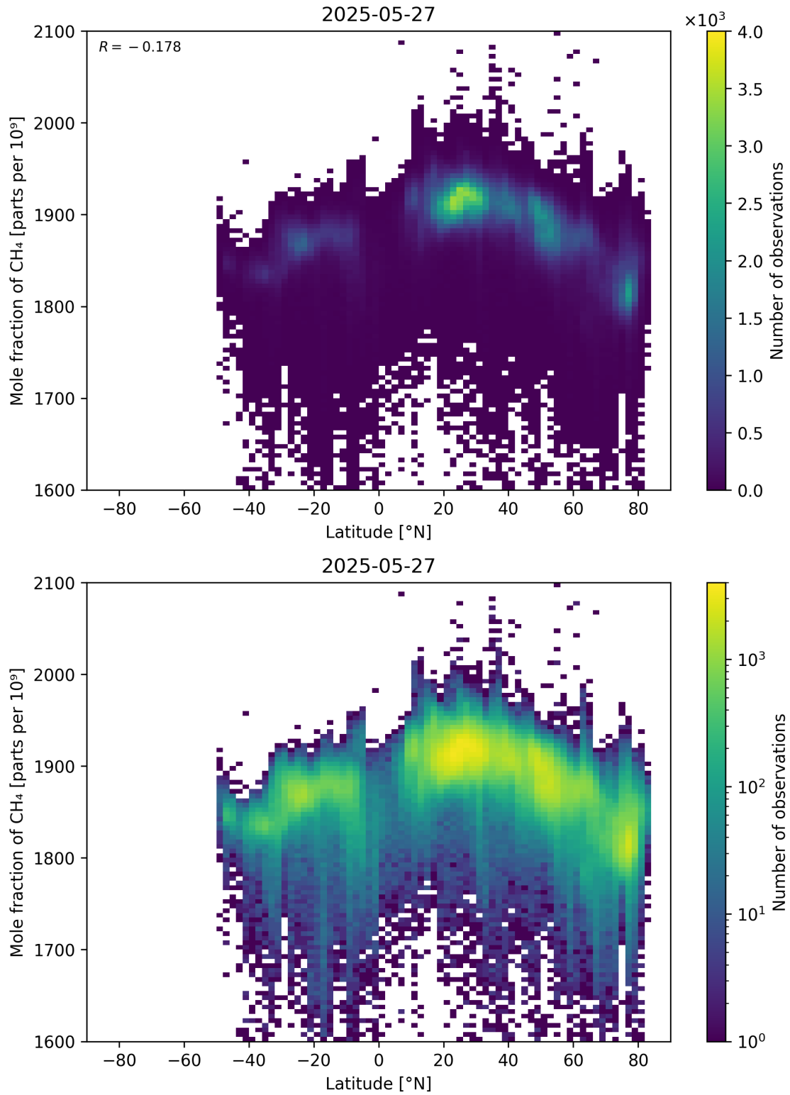
Figure 57: Scatter density plot of “Latitude” against “Mole fraction of CH 4 ” for 2025-05-26 to 2025-05-28.
