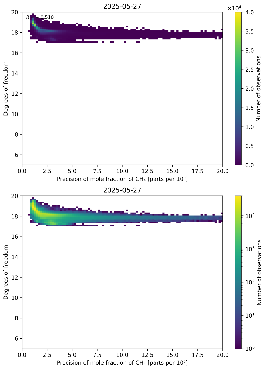
Figure 80: Scatter density plot of “Precision of mole fraction of CH 4 ” against “Degrees of freedom” for 2025-05-26 to 2025-05-28.
