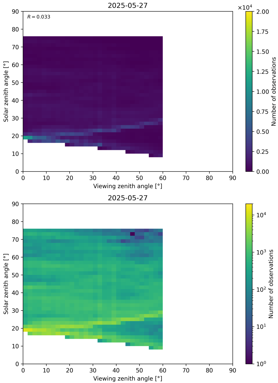
Figure 115: Scatter density plot of “Viewing zenith angle” against “Solar zenith angle” for 2025-05-26 to 2025-05-28.
