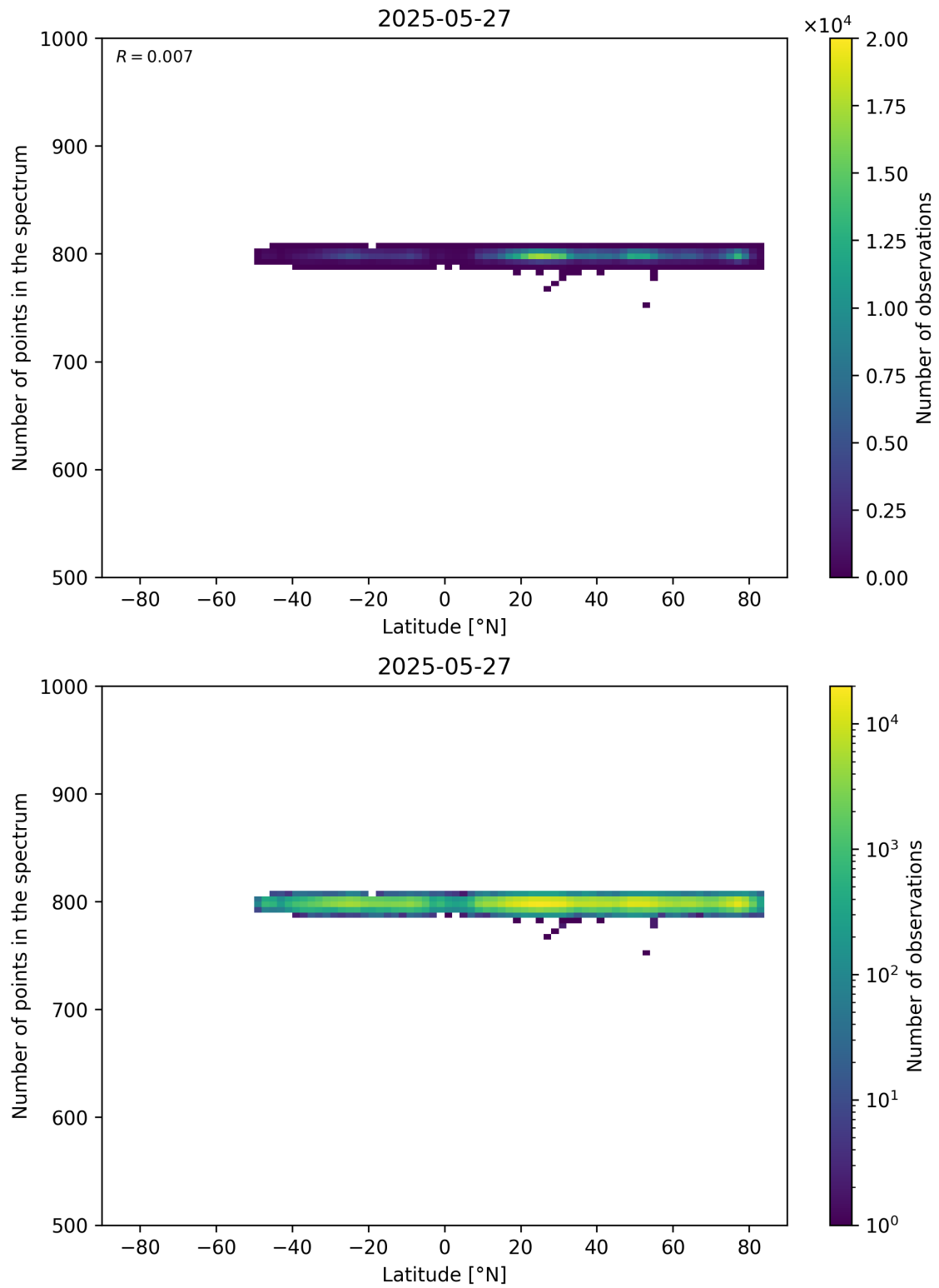
Figure 61: Scatter density plot of “Latitude” against “Number of points in the spectrum” for 2025-05-26 to 2025-05-28.
