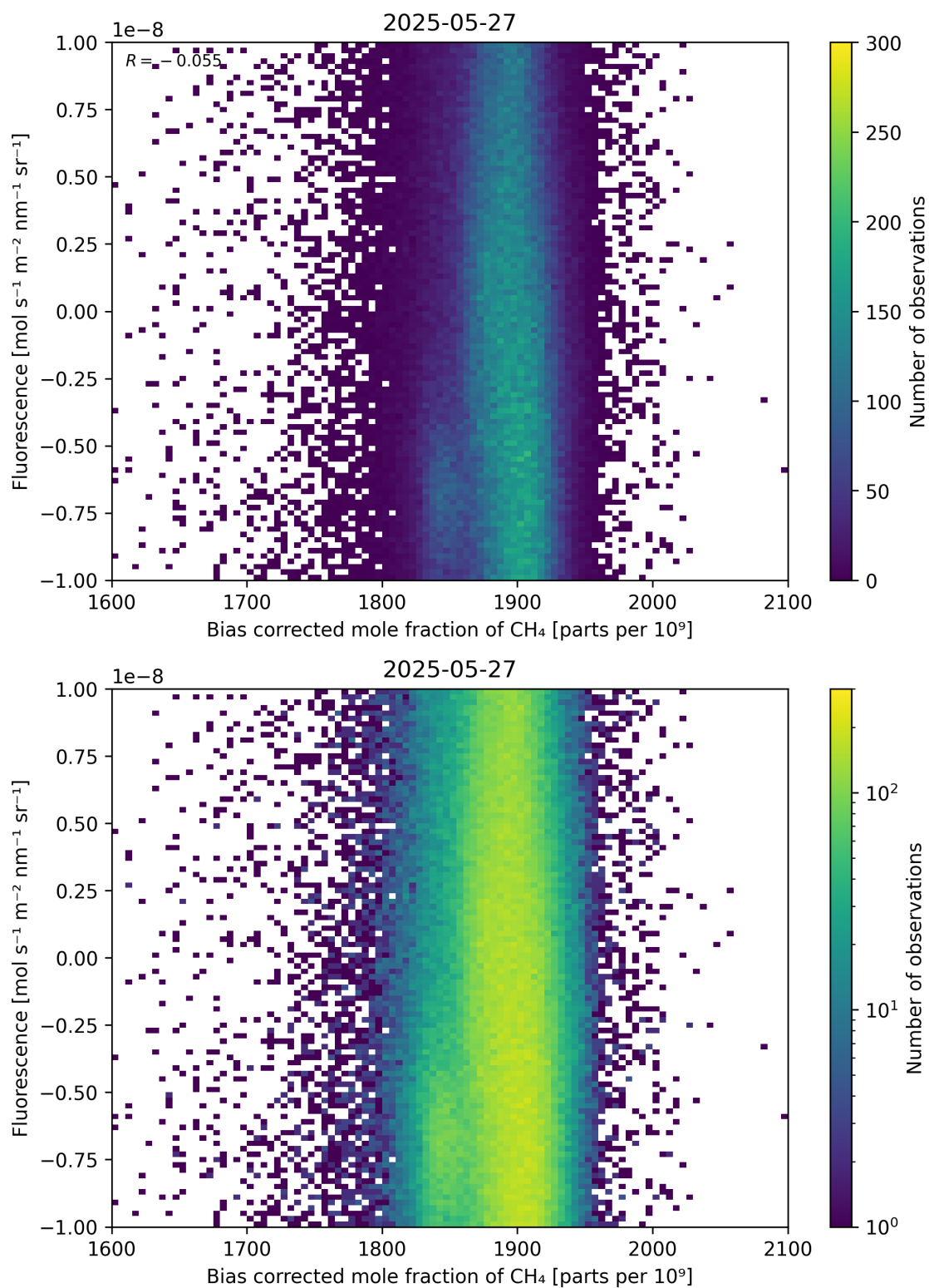
Figure 66: Scatter density plot of “Bias corrected mole fraction of \text{CH}_4 ” against “Fluorescence” for 2025-05-26 to 2025-05-28.
