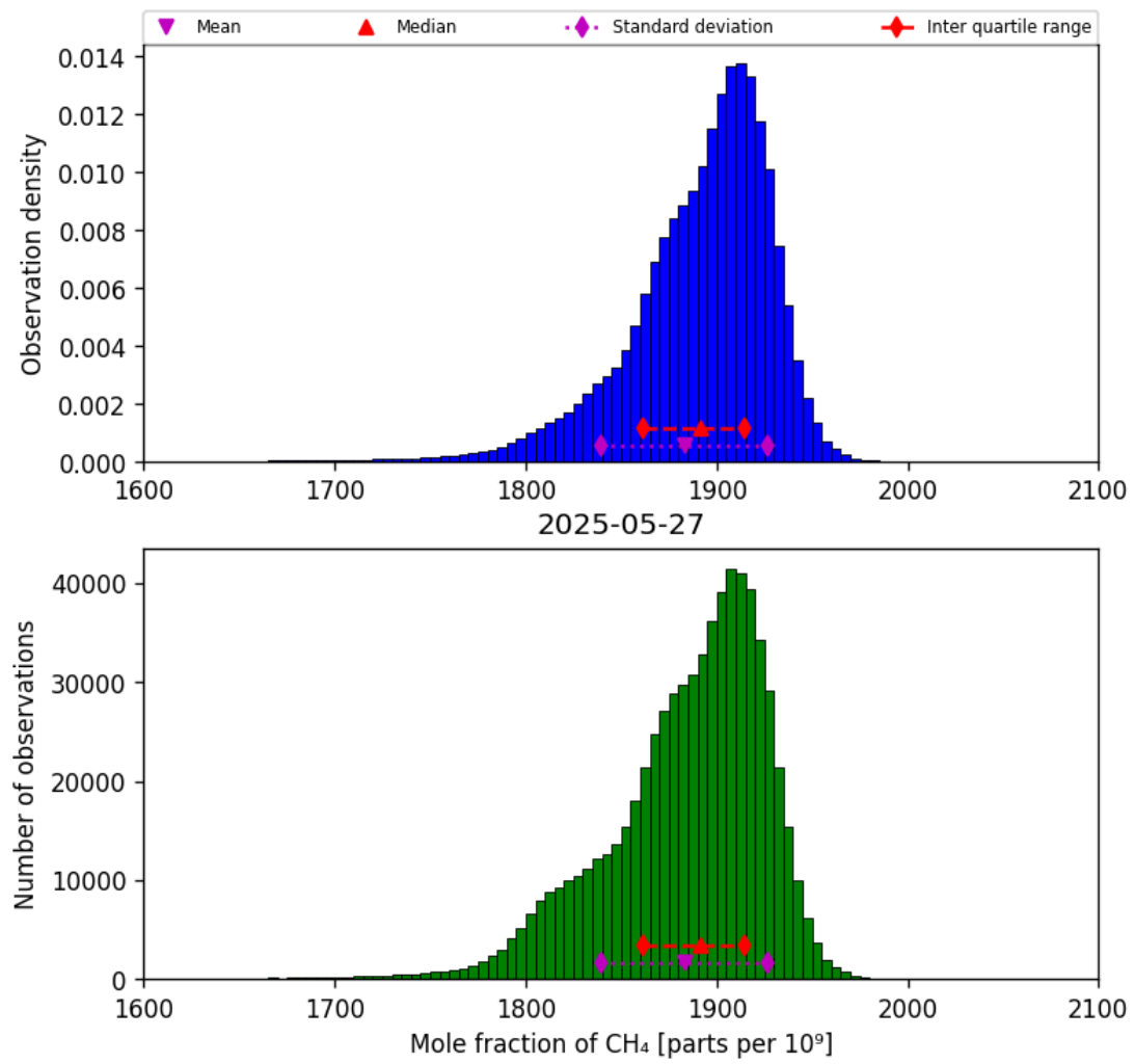
Figure 23: Histogram of “Mole fraction of CH 4 ” for 2025-05-26 to 2025-05-28
