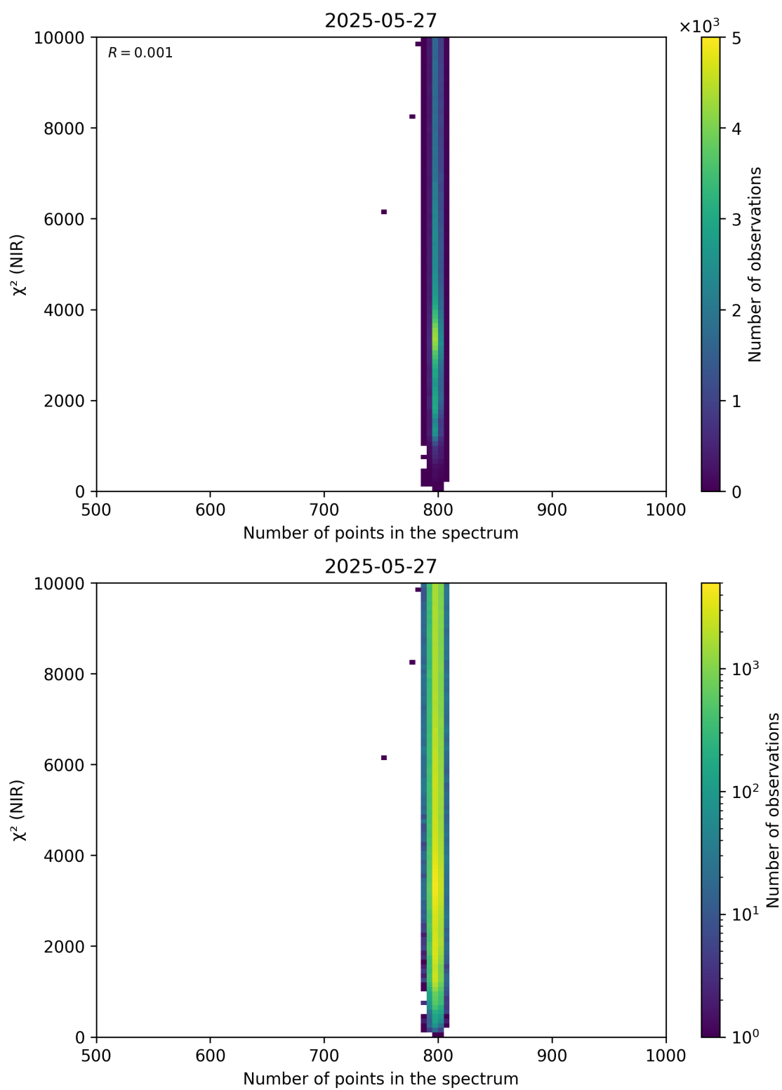
Figure 88: Scatter density plot of “Number of points in the spectrum” against “ \chi^2 (NIR)” for 2025-05-26 to 2025-05-28.
