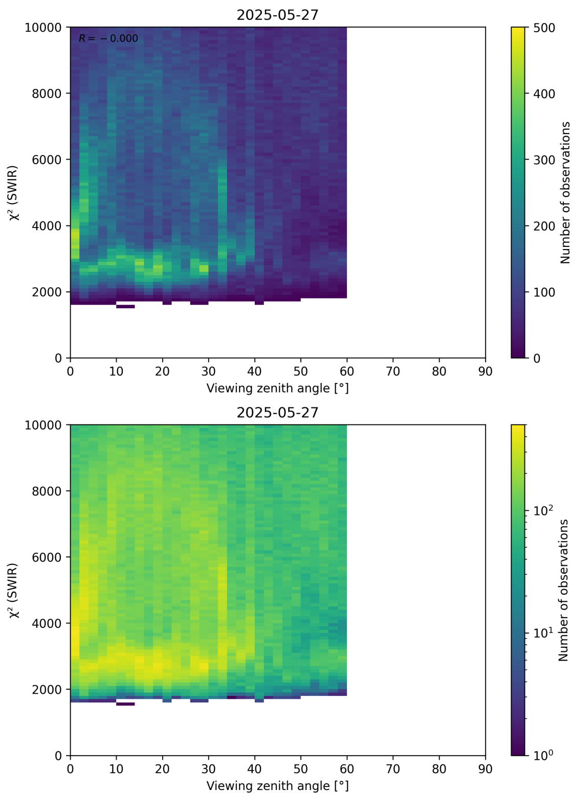
Figure 106: Scatter density plot of “Viewing zenith angle” against “ \chi^2 (SWIR)” for 2025-05-26 to 2025-05-28.
