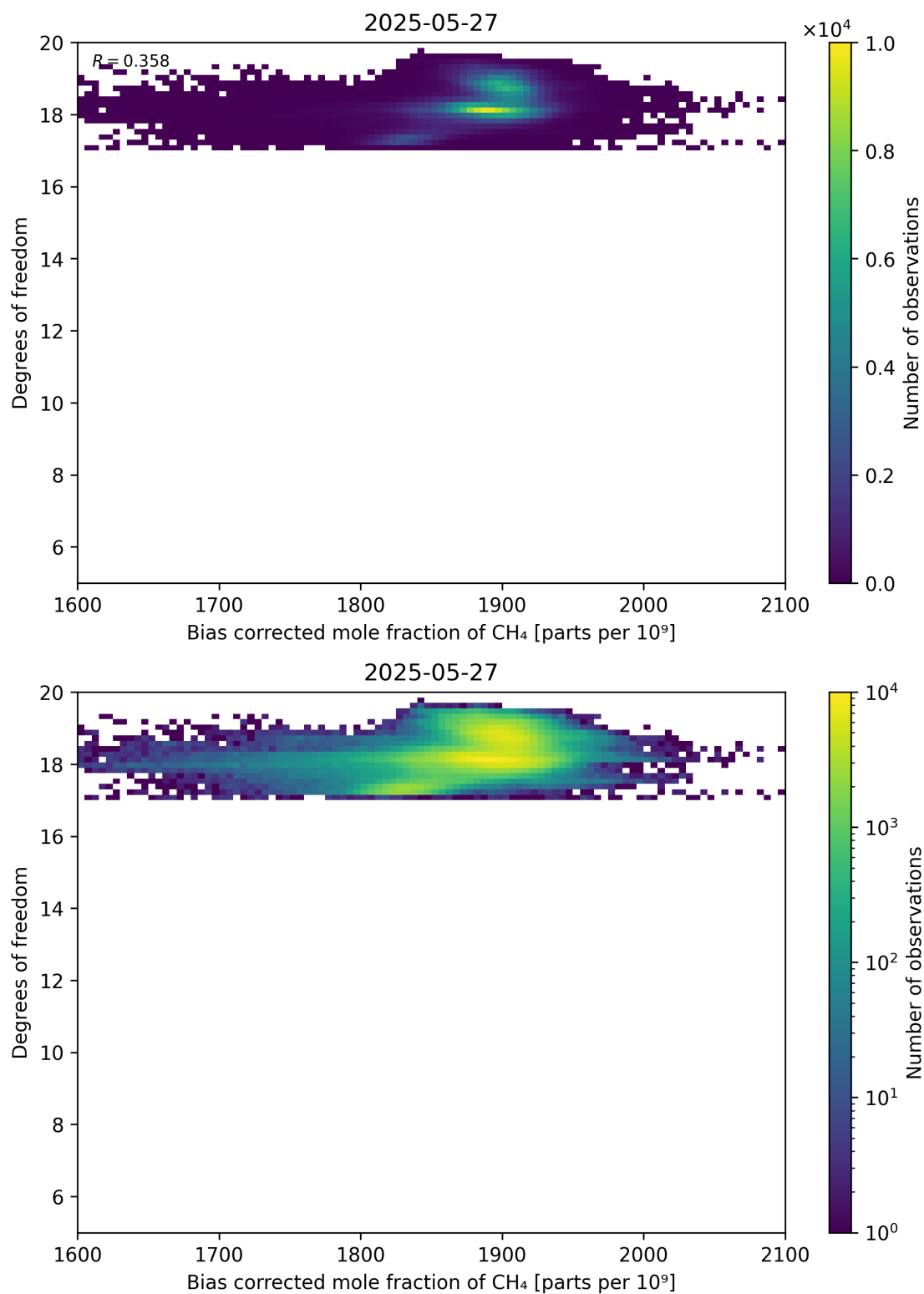
Figure 65: Scatter density plot of “Bias corrected mole fraction of CH 4 ” against “Degrees of freedom” for 2025-05-26 to 2025-05-28.
