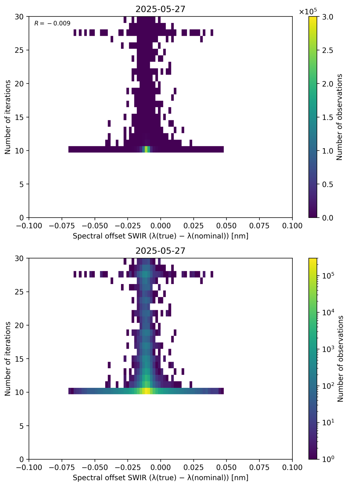
Figure 121: Scatter density plot of “Spectral offset SWIR ( \lambda_{\text{true}} - \lambda_{\text{nominal}} )” against “Number of iterations” for 2025-05-26 to 2025-05-28.
