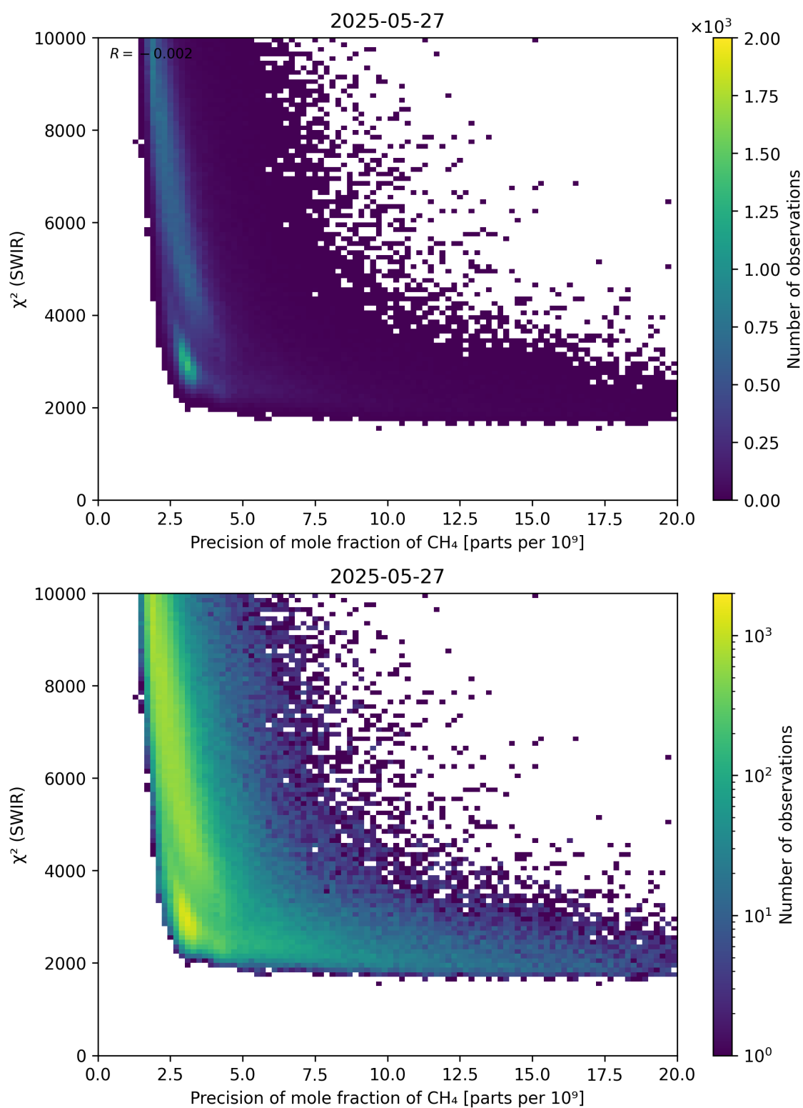
Figure 79: Scatter density plot of “Precision of mole fraction of CH 4 ” against “ \chi^2 (SWIR)” for 2025-05-26 to 2025-05-28.
