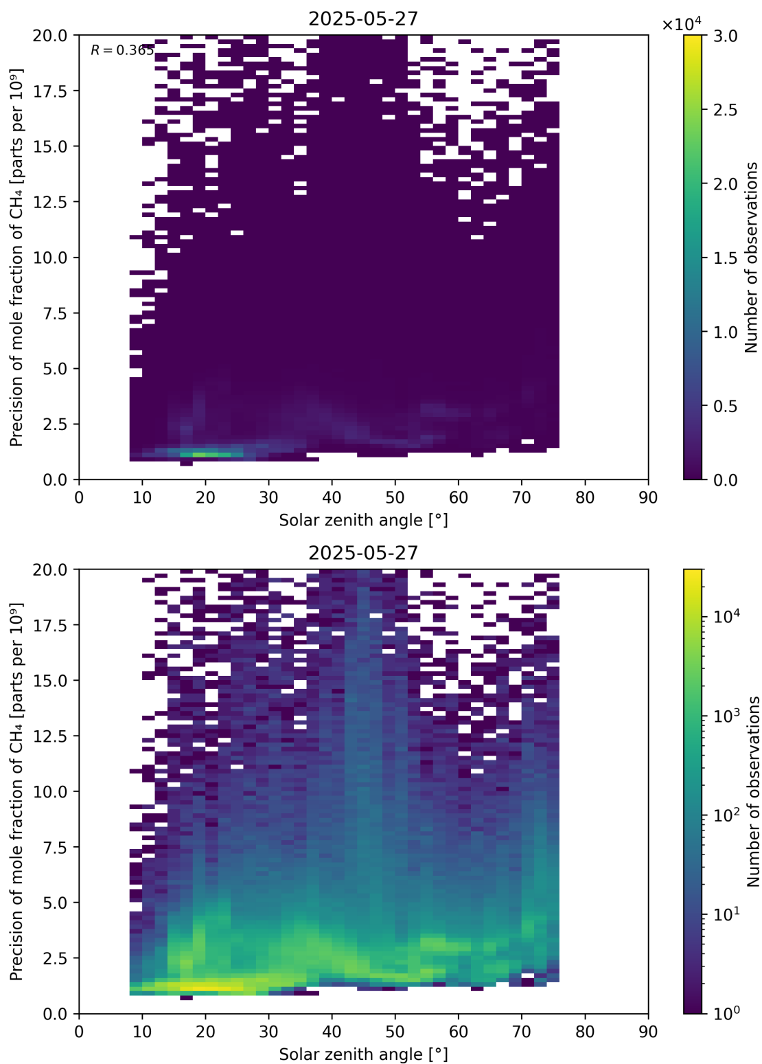
Figure 101: Scatter density plot of “Solar zenith angle” against “Precision of mole fraction of \text{CH}_4 ” for 2025-05-26 to 2025-05-28.
