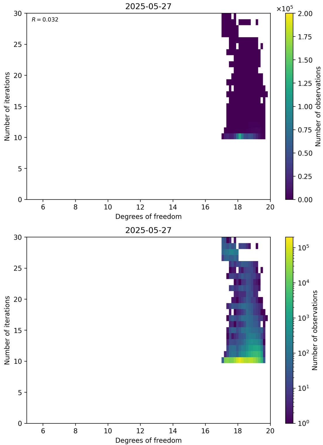
Figure 52: Scatter density plot of “Degrees of freedom” against “Number of iterations” for 2025-05-26 to 2025-05-28.
