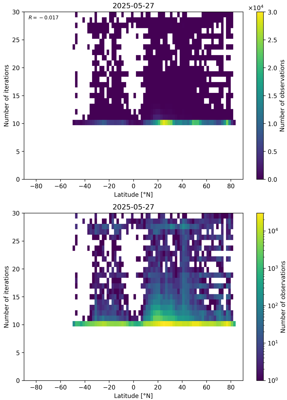
Figure 60: Scatter density plot of “Latitude” against “Number of iterations” for 2025-05-26 to 2025-05-28.
