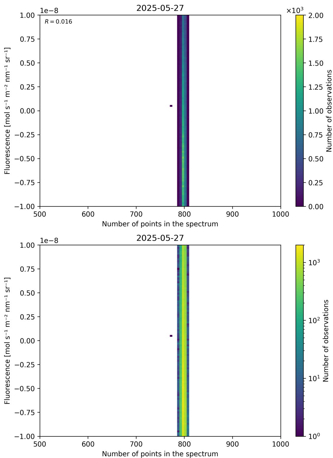
Figure 91: Scatter density plot of “Number of points in the spectrum” against “Fluorescence” for 2025-05-26 to 2025-05-28.
