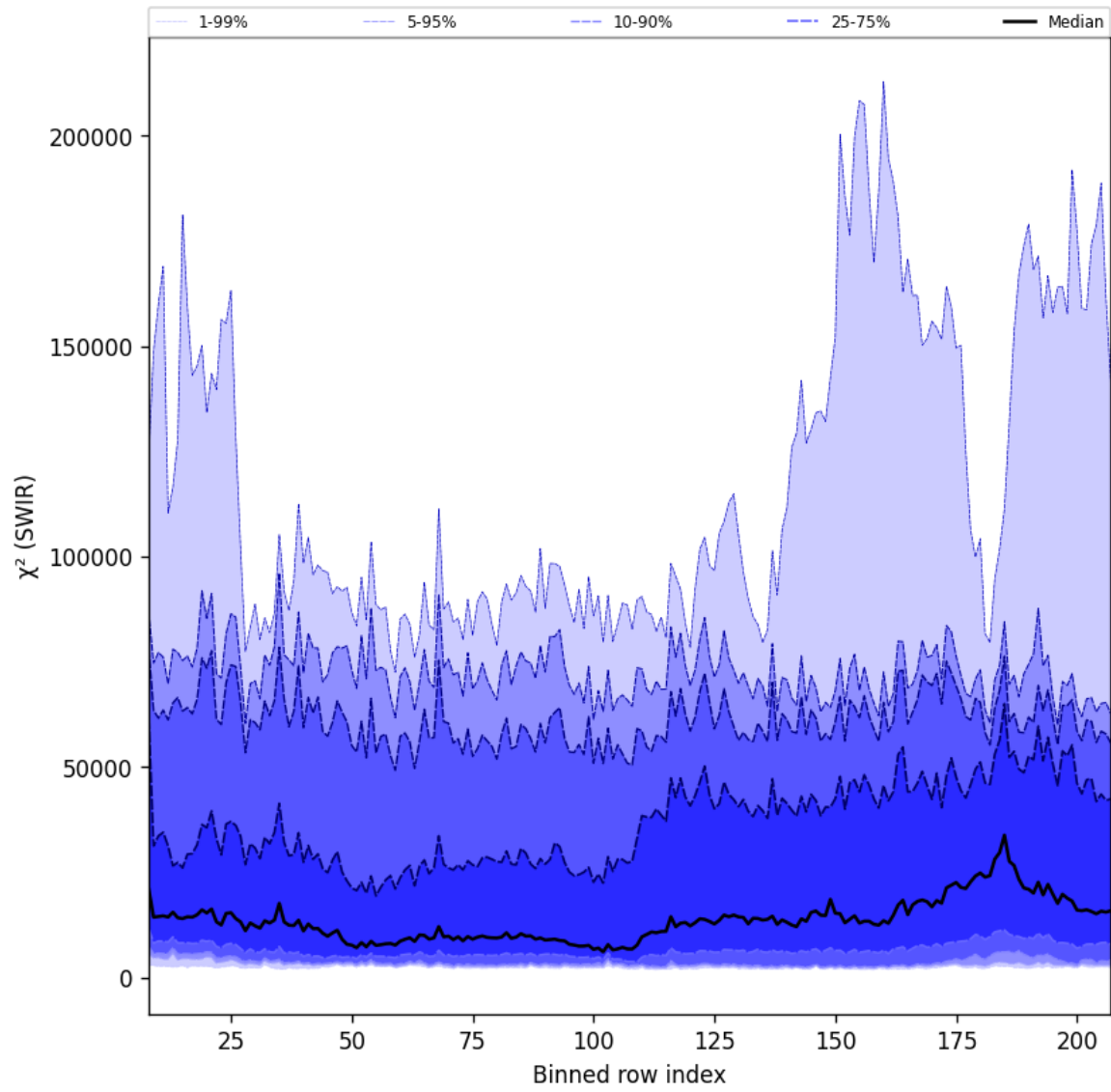
Figure 39: Along track statistics of “ \chi^2 (SWIR)” for 2025-05-26 to 2025-05-28
