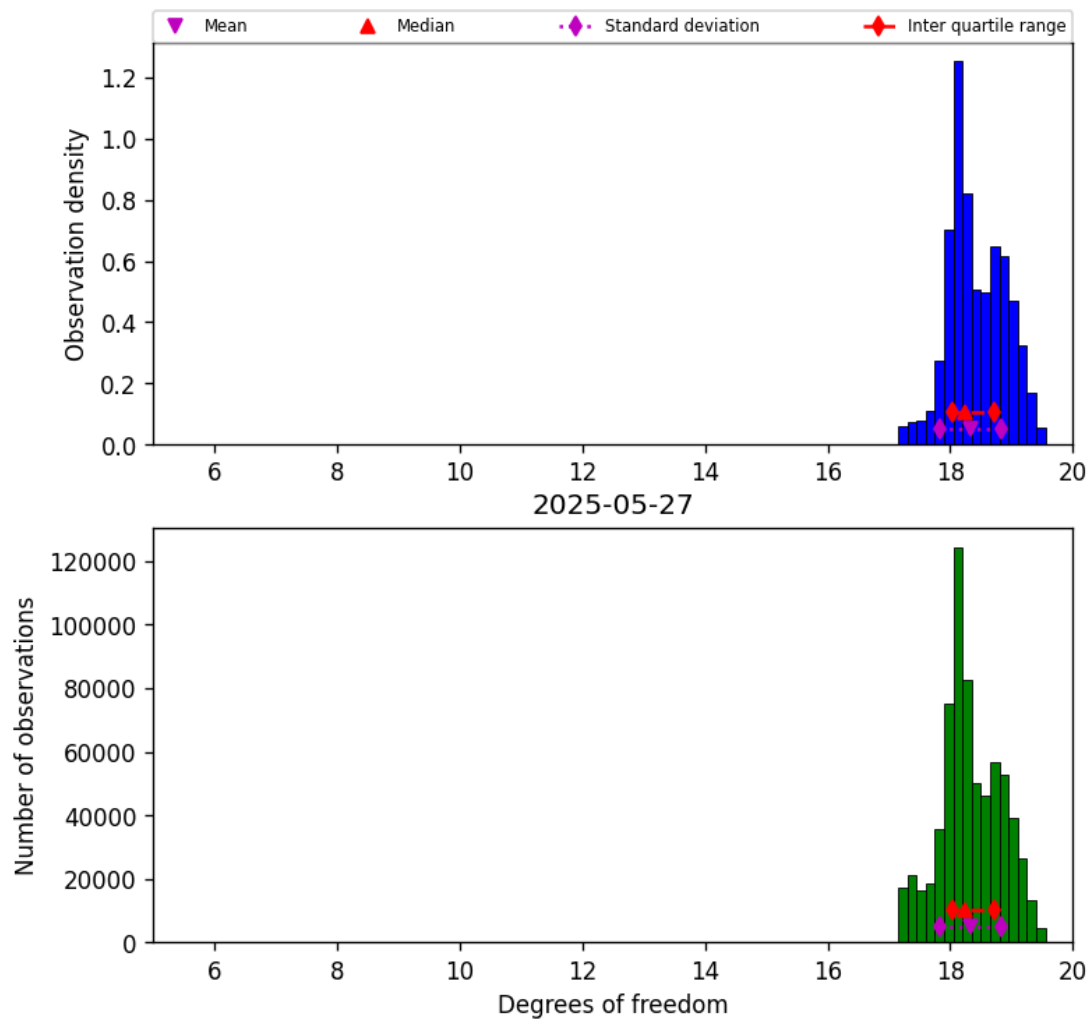
Figure 30: Histogram of “Degrees of freedom” for 2025-05-26 to 2025-05-28
