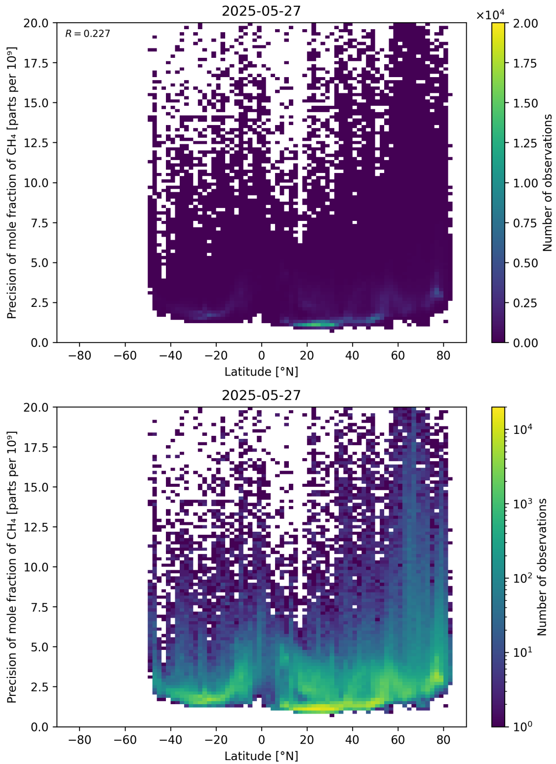
Figure 59: Scatter density plot of “Latitude” against “Precision of mole fraction of CH 4 ” for 2025-05-26 to 2025-05-28.
