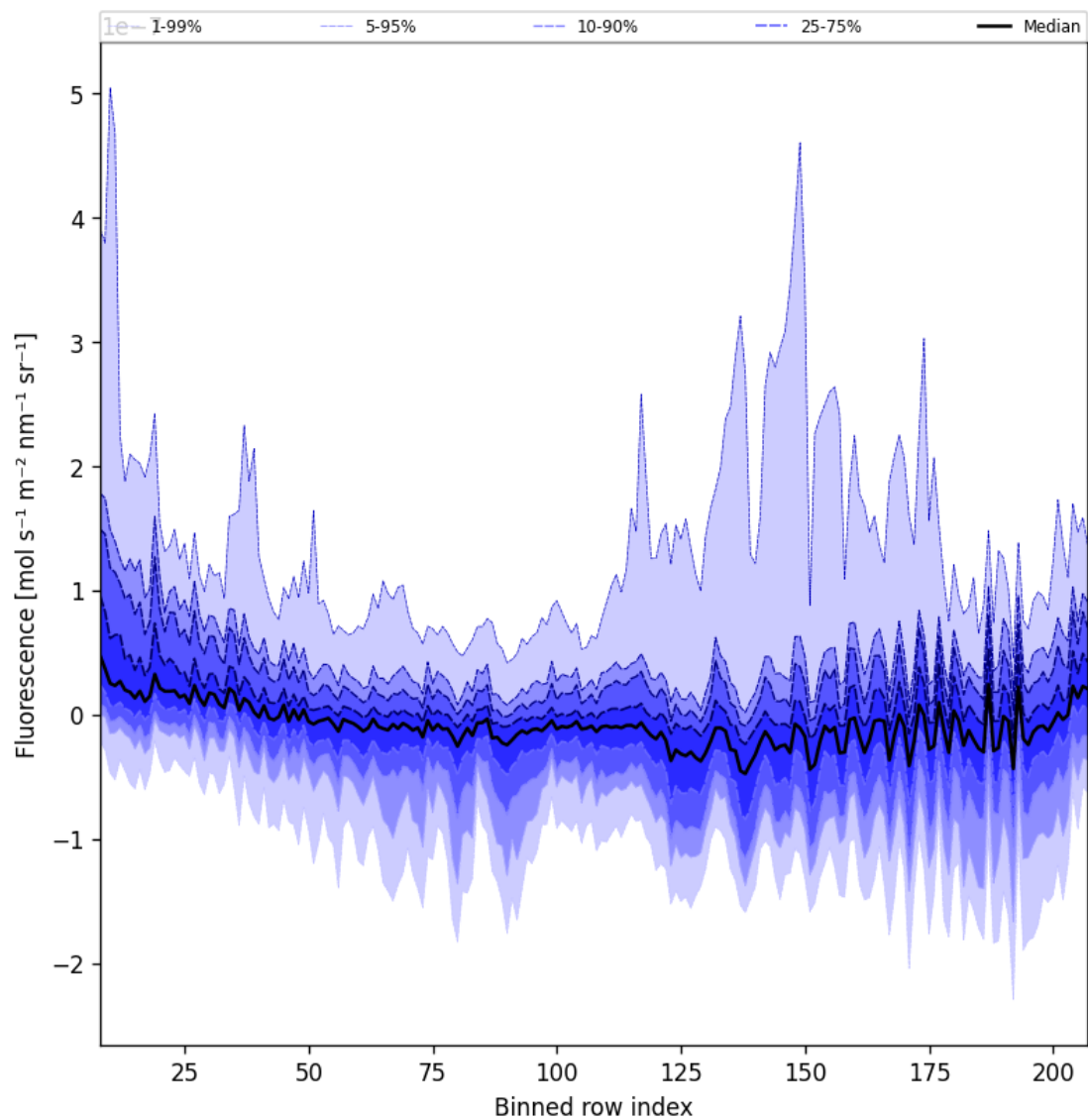
Figure 43: Along track statistics of “Fluorescence” for 2025-05-26 to 2025-05-28
