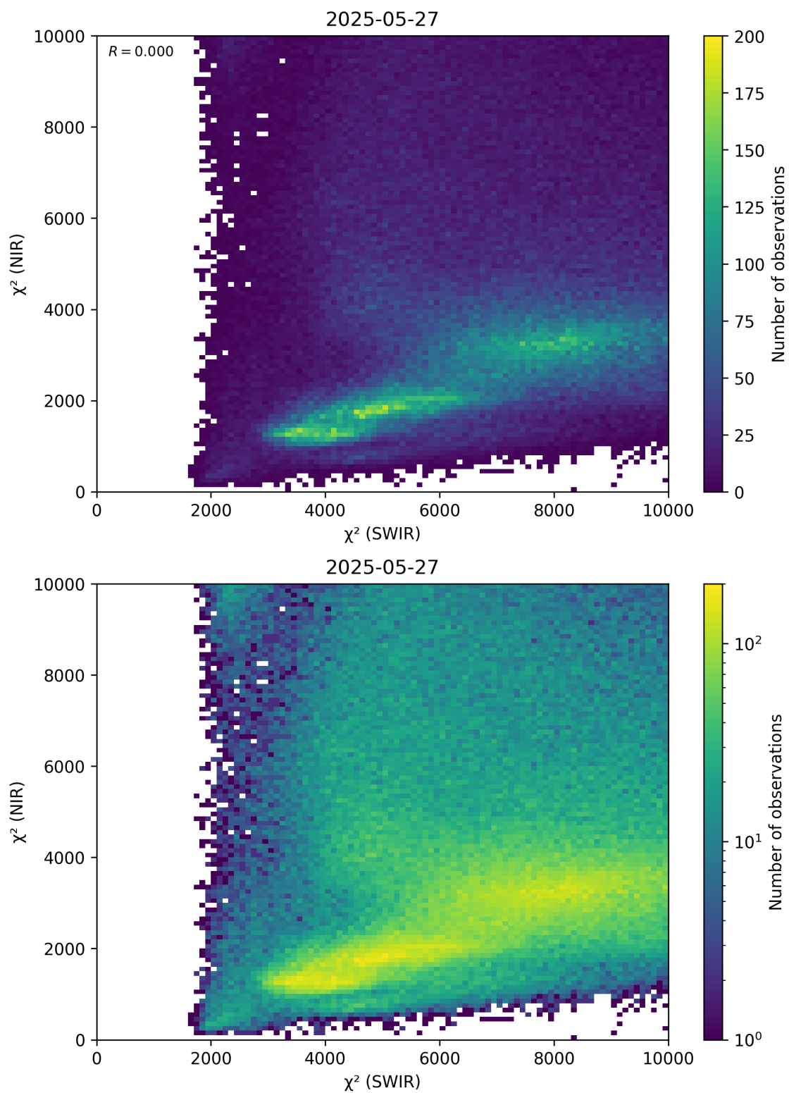
Figure 47: Scatter density plot of “ \chi^2 (SWIR)” against “ \chi^2 (NIR)” for 2025-05-26 to 2025-05-28.
