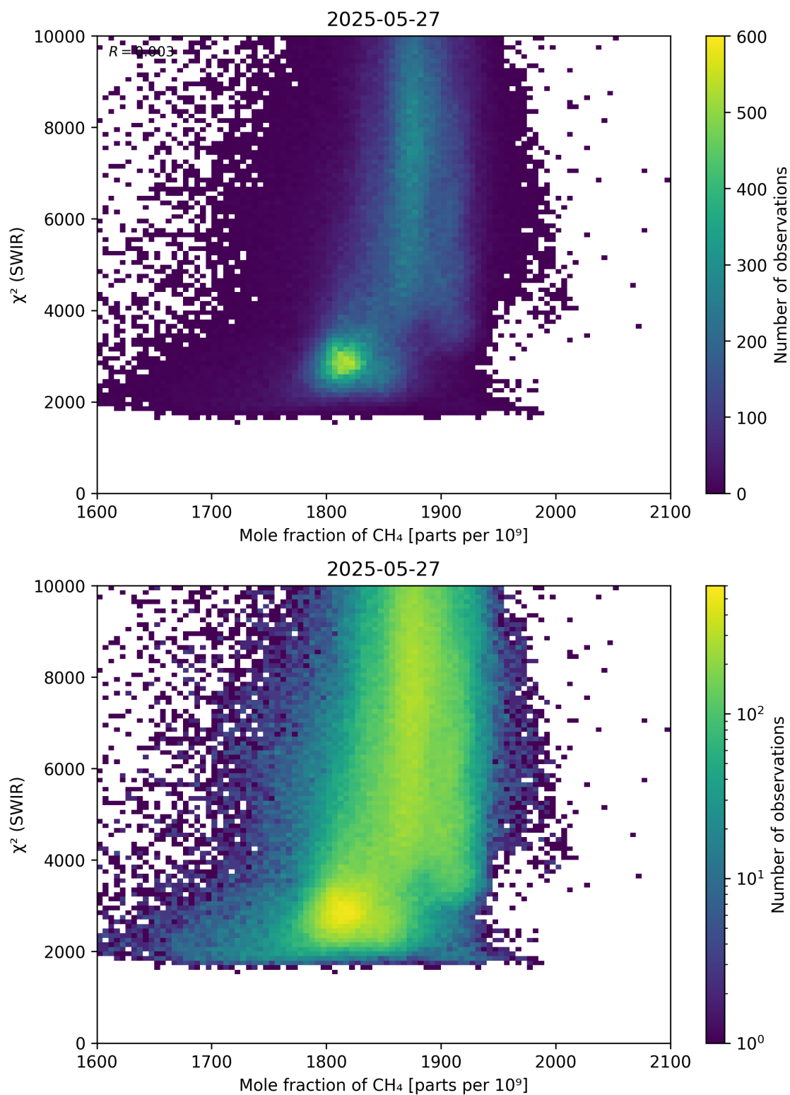
Figure 71: Scatter density plot of “Mole fraction of \text{CH}_4 ” against “ \chi^2 (SWIR)” for 2025-05-26 to 2025-05-28.
