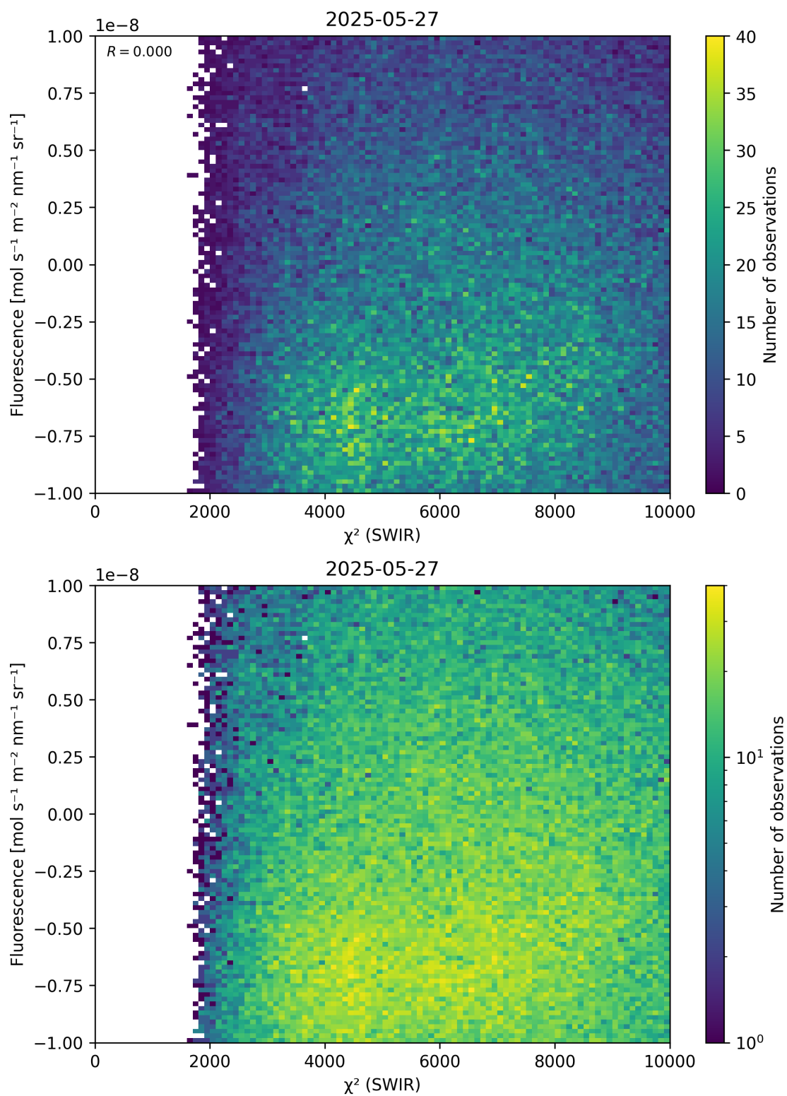
Figure 49: Scatter density plot of “ \chi^2 (SWIR)” against “Fluorescence” for 2025-05-26 to 2025-05-28.
