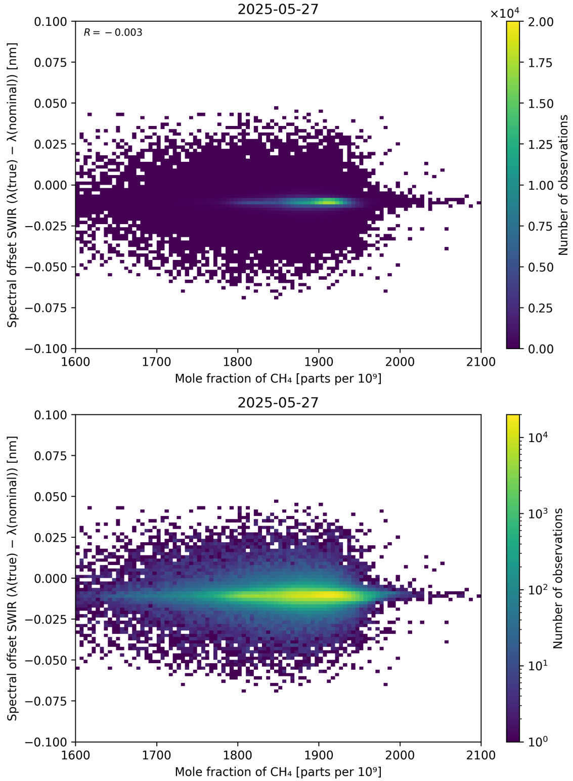
Figure 86: Scatter density plot of “Mole fraction of CH 4 ” against “Spectral offset SWIR ( \lambda_{\text{true}} - \lambda_{\text{nominal}} )” for 2025-05-26 to 2025-05-28.
