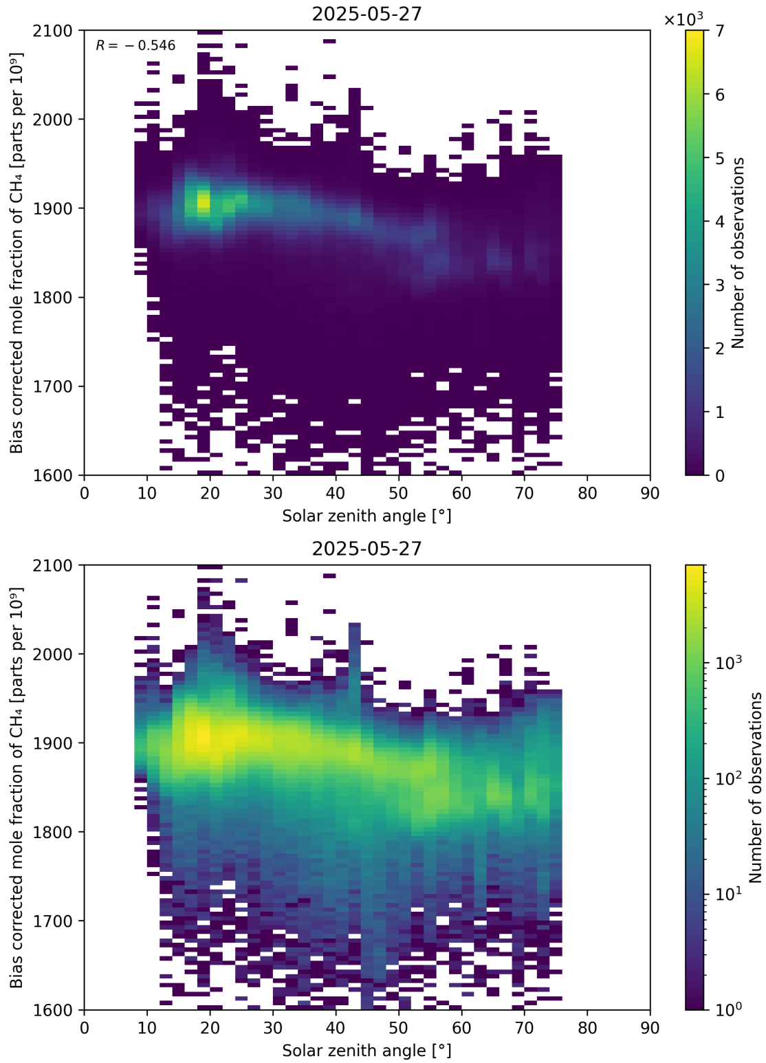
Figure 100: Scatter density plot of “Solar zenith angle” against “Bias corrected mole fraction of CH 4 ” for 2025-05-26 to 2025-05-28.
