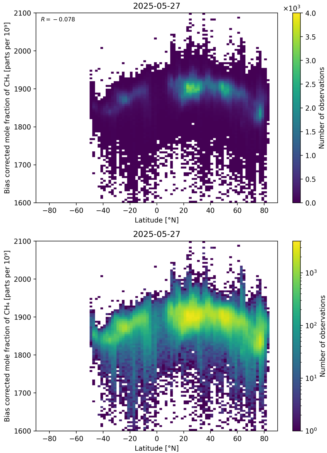
Figure 58: Scatter density plot of “Latitude” against “Bias corrected mole fraction of \text{CH}_4 ” for 2025-05-26 to 2025-05-28.
