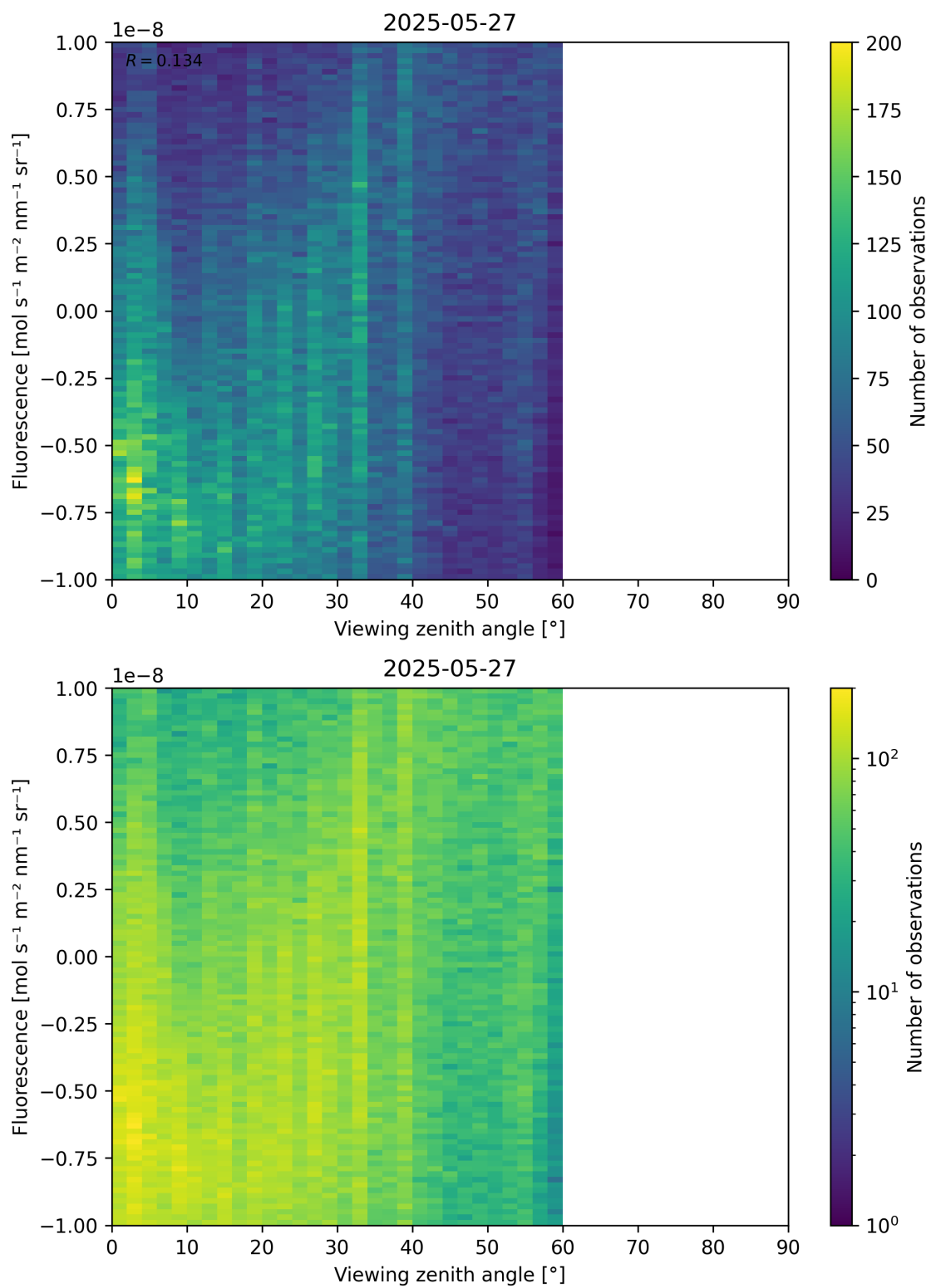
Figure 108: Scatter density plot of “Viewing zenith angle” against “Fluorescence” for 2025-05-26 to 2025-05-28.
