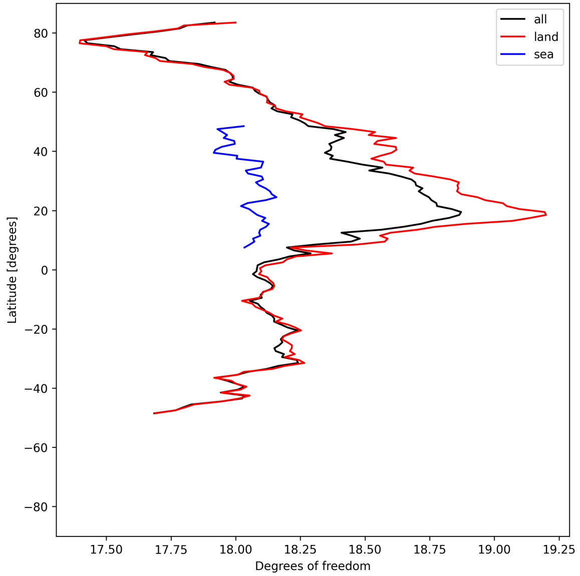
Figure 19: Zonal average of “Degrees of freedom” for 2025-05-26 to 2025-05-28.
