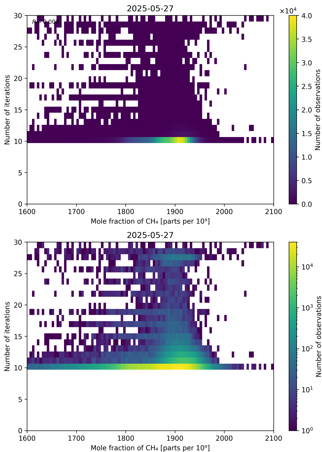
Figure 76: Scatter density plot of “Mole fraction of CH 4 ” against “Number of iterations” for 2025-05-26 to 2025-05-28.
