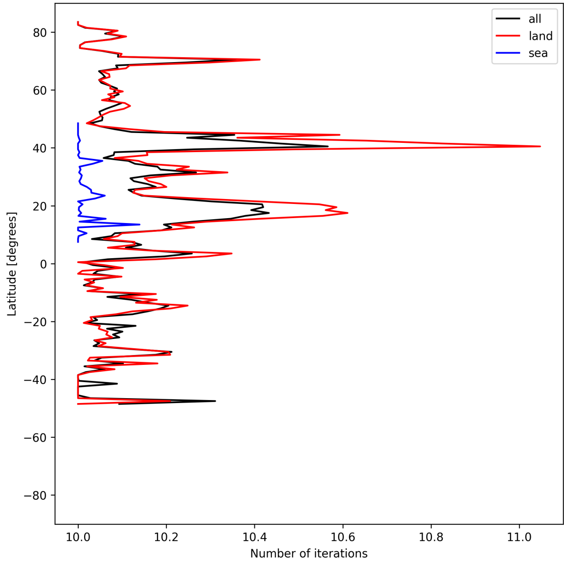
Figure 20: Zonal average of “Number of iterations” for 2025-05-26 to 2025-05-28.
