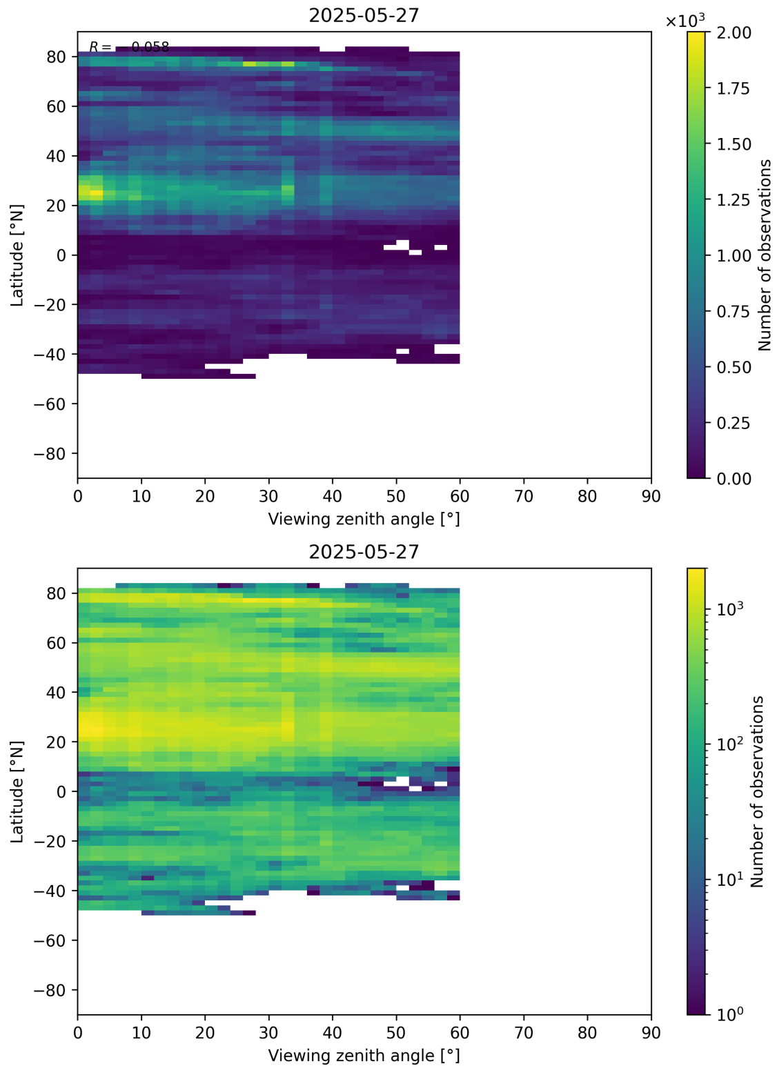
Figure 109: Scatter density plot of “Viewing zenith angle” against “Latitude” for 2025-05-26 to 2025-05-28.
