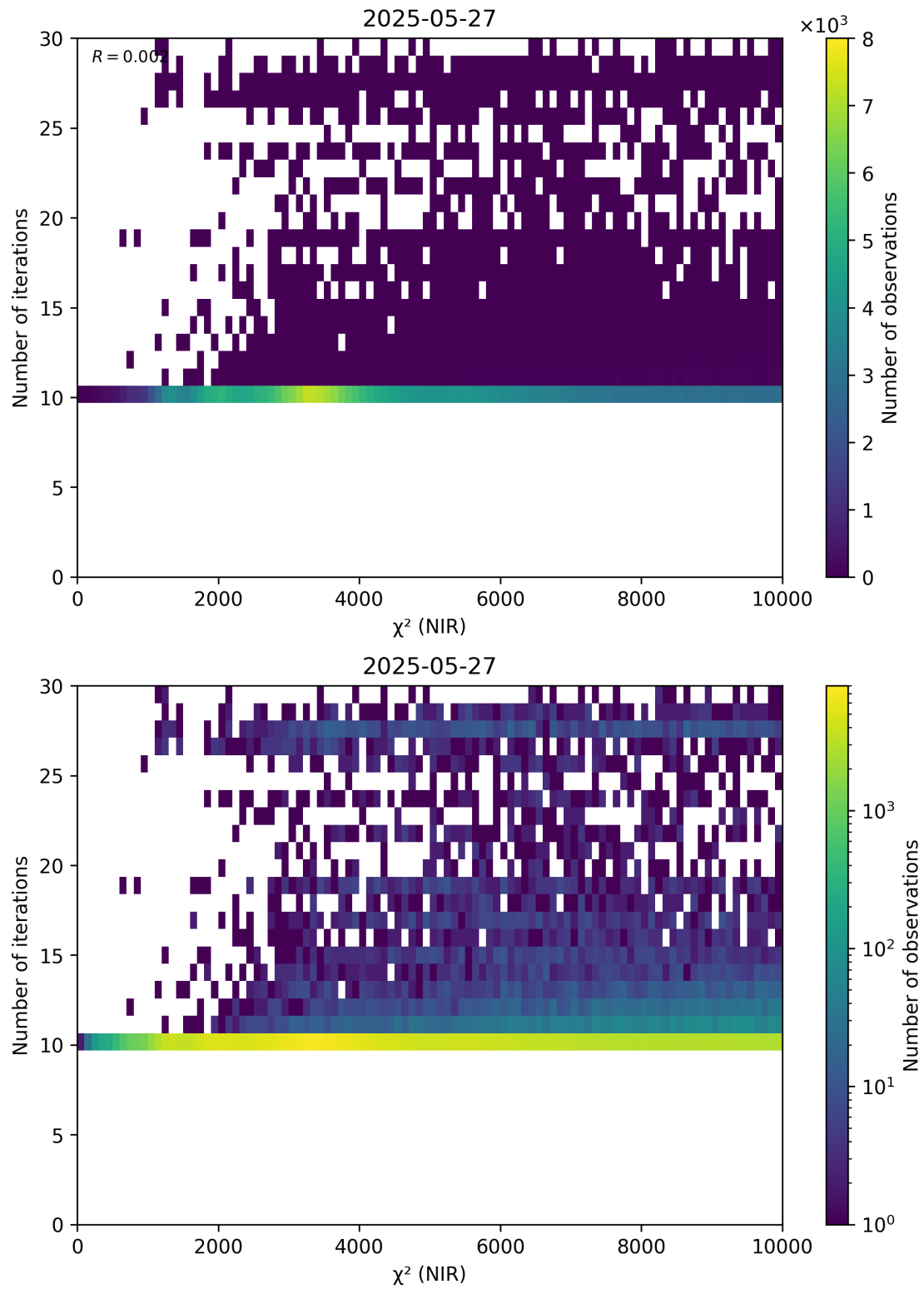
Figure 46: Scatter density plot of “ \chi^2 (NIR)” against “Number of iterations” for 2025-05-26 to 2025-05-28.
