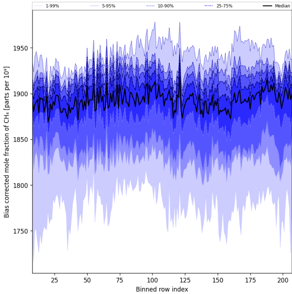
Figure 36: Along track statistics of “Bias corrected mole fraction of CH 4 ” for 2025-05-26 to 2025-05-28
