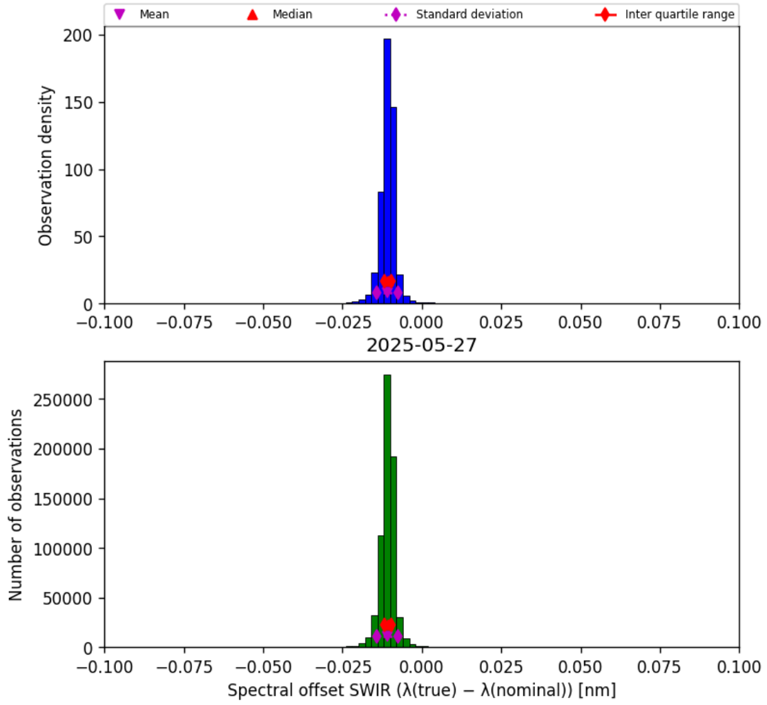
Figure 27: Histogram of “Spectral offset SWIR ( \lambda_{\text{true}} - \lambda_{\text{nominal}} )” for 2025-05-26 to 2025-05-28
