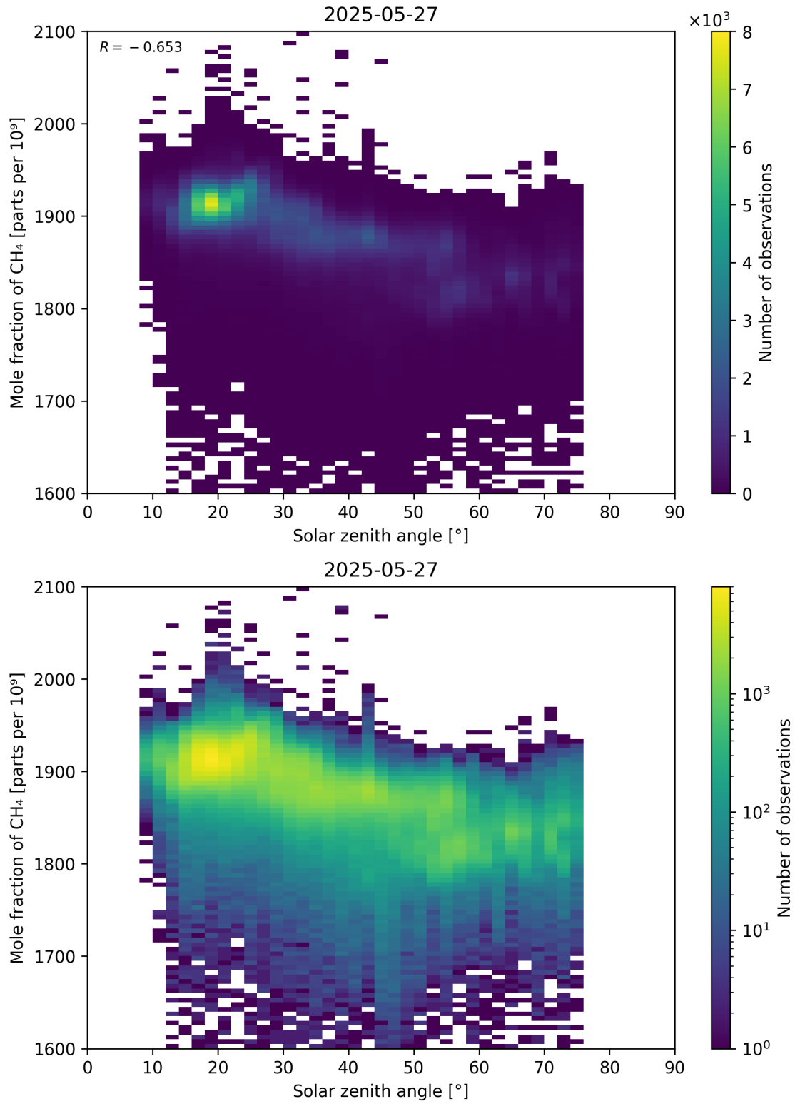
Figure 99: Scatter density plot of “Solar zenith angle” against “Mole fraction of CH 4 ” for 2025-05-26 to 2025-05-28.
