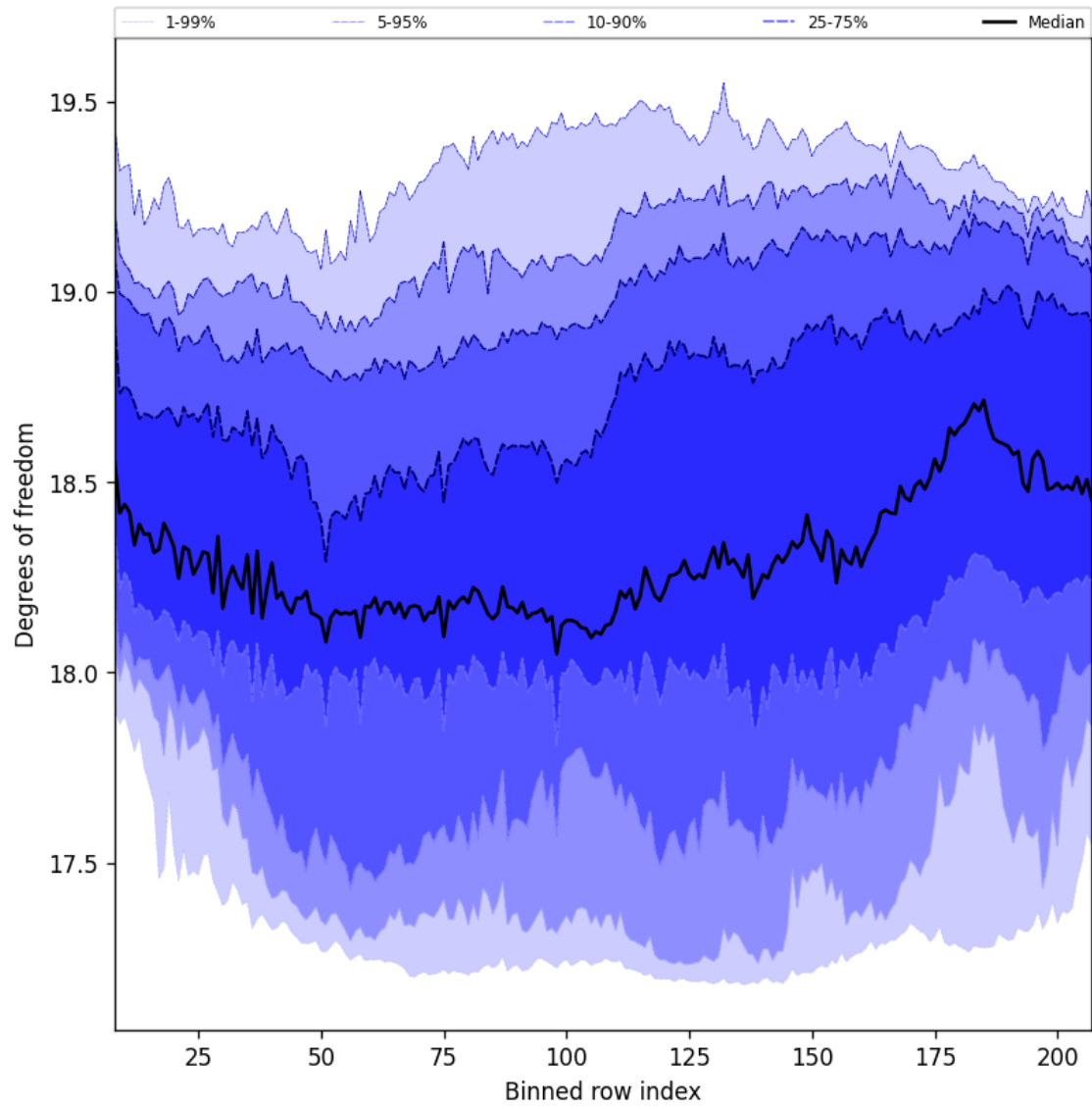
Figure 41: Along track statistics of “Degrees of freedom” for 2025-05-26 to 2025-05-28
