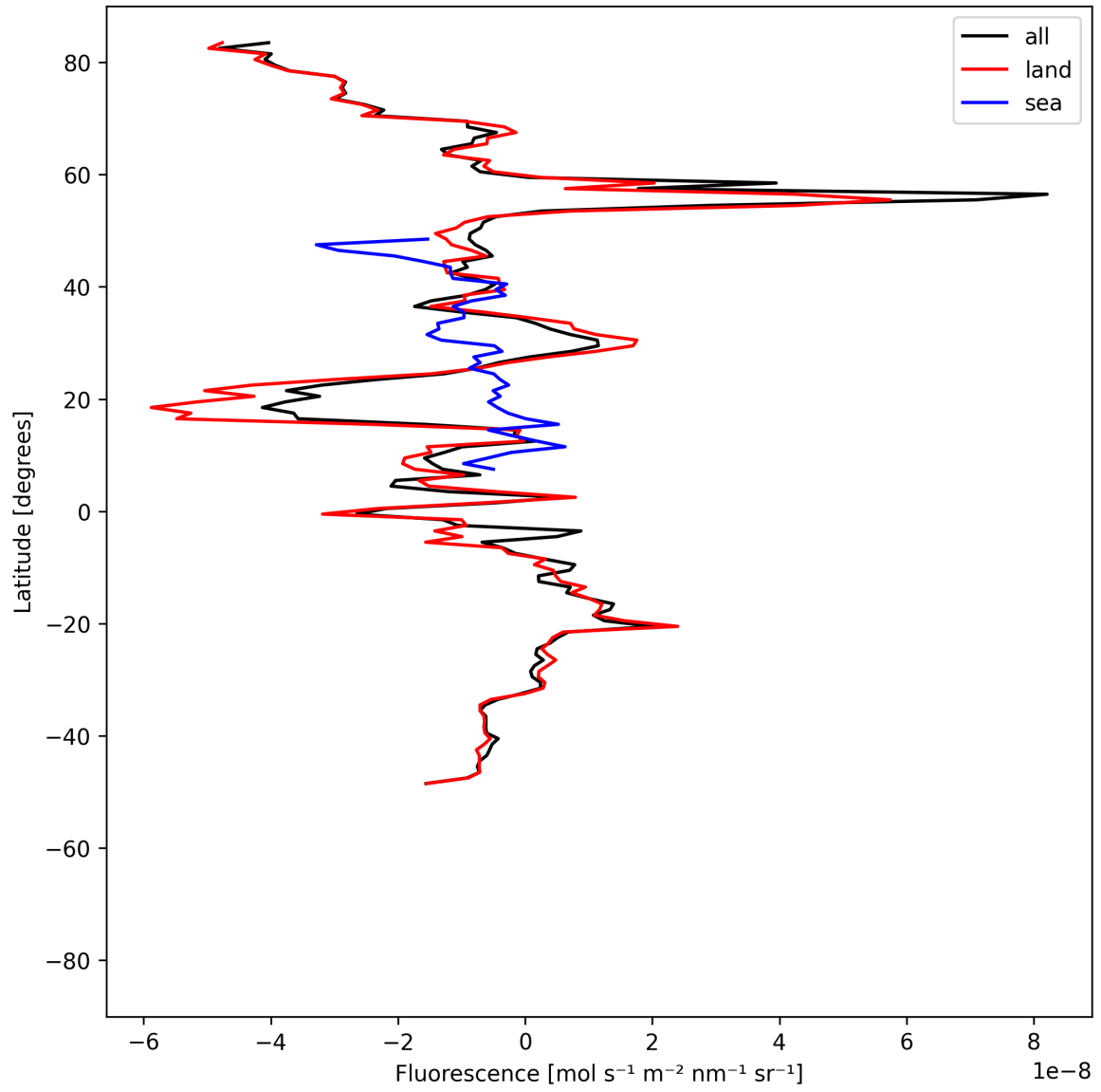
Figure 21: Zonal average of “Fluorescence” for 2025-05-26 to 2025-05-28.
