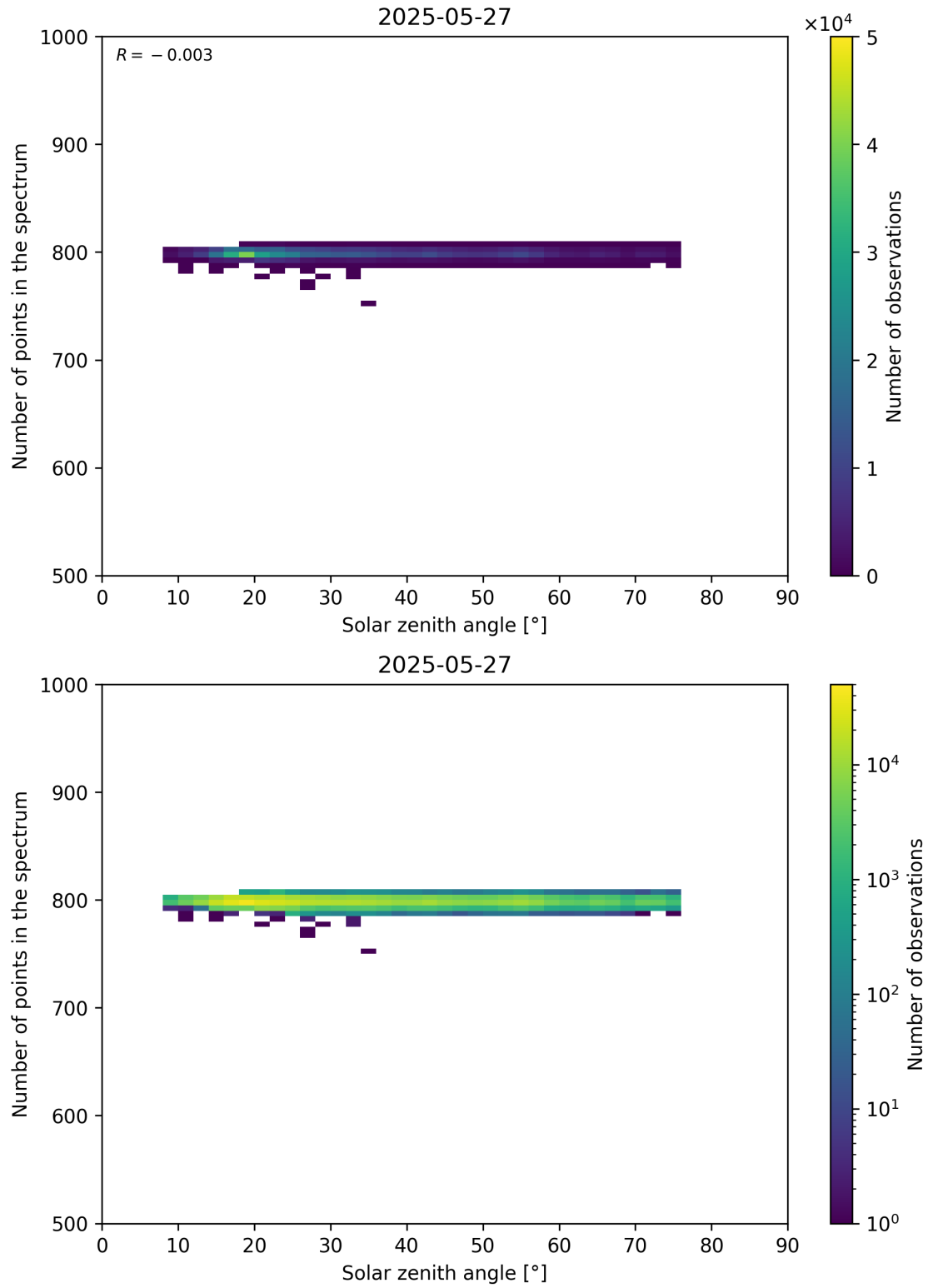
Figure 103: Scatter density plot of “Solar zenith angle” against “Number of points in the spectrum” for 2025-05-26 to 2025-05-28.
