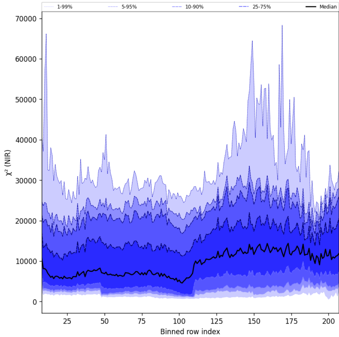
Figure 40: Along track statistics of " \chi^2 (NIR)" for 2025-05-26 to 2025-05-28
