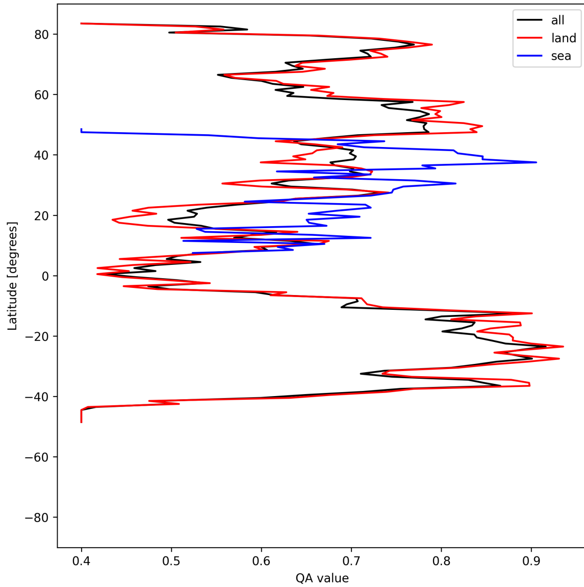
Figure 11: Zonal average of “QA value” for 2025-05-26 to 2025-05-28.
