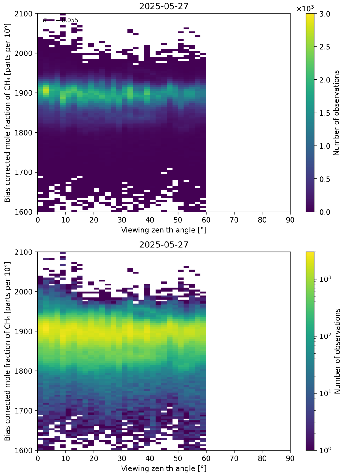
Figure 111: Scatter density plot of “Viewing zenith angle” against “Bias corrected mole fraction of CH 4 ” for 2025-05-26 to 2025-05-28.
