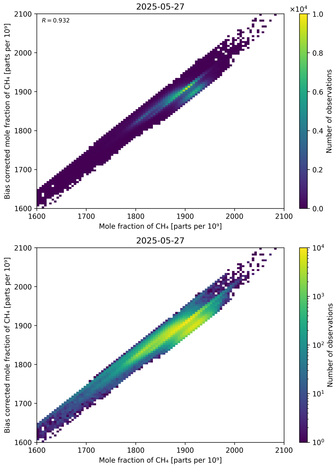
Figure 74: Scatter density plot of “Mole fraction of CH 4 ” against “Bias corrected mole fraction of CH 4 ” for 2025-05-26 to 2025-05-28.
