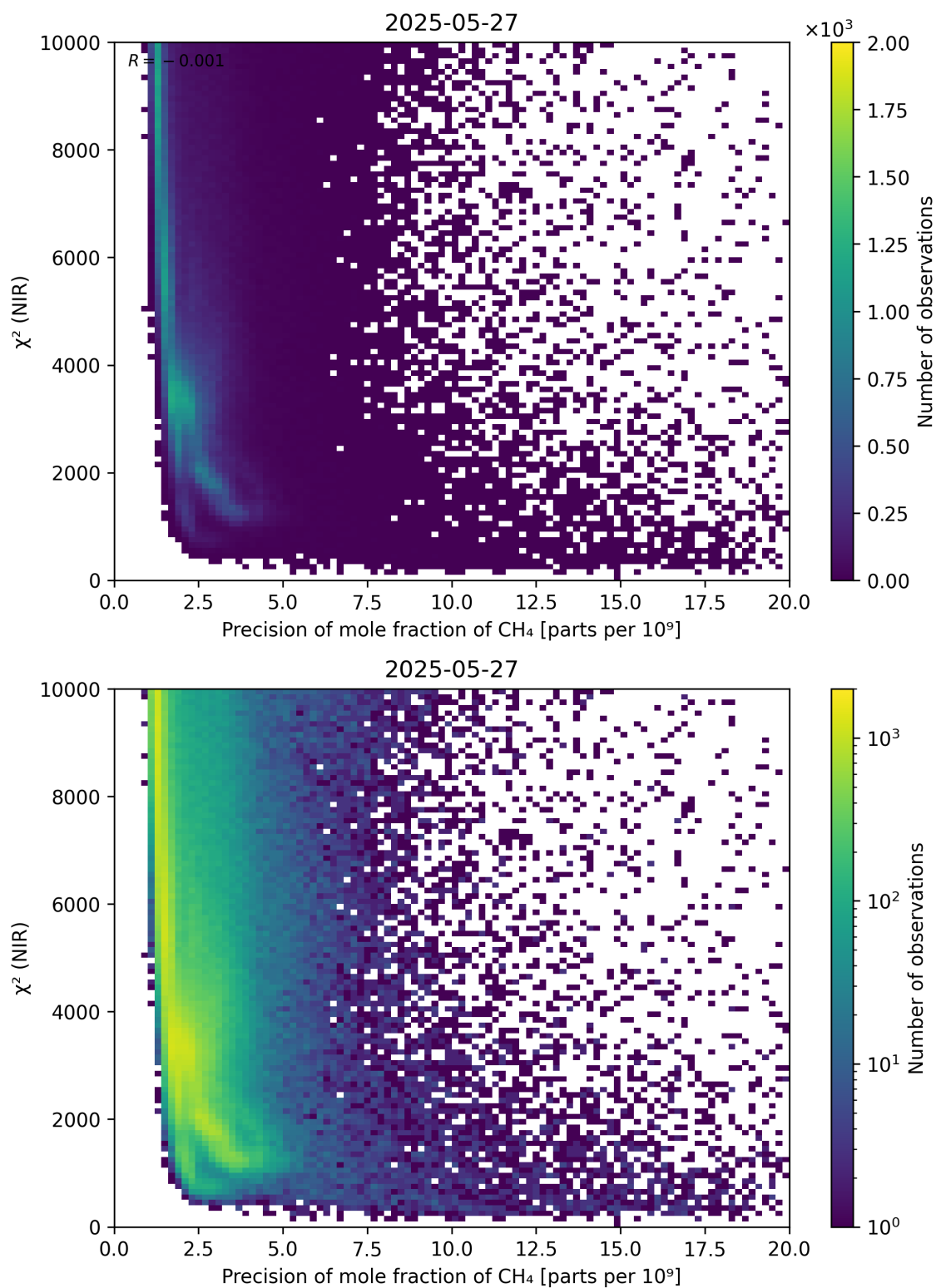
Figure 78: Scatter density plot of “Precision of mole fraction of CH 4 ” against “ \chi^2 (NIR)” for 2025-05-26 to 2025-05-28.
