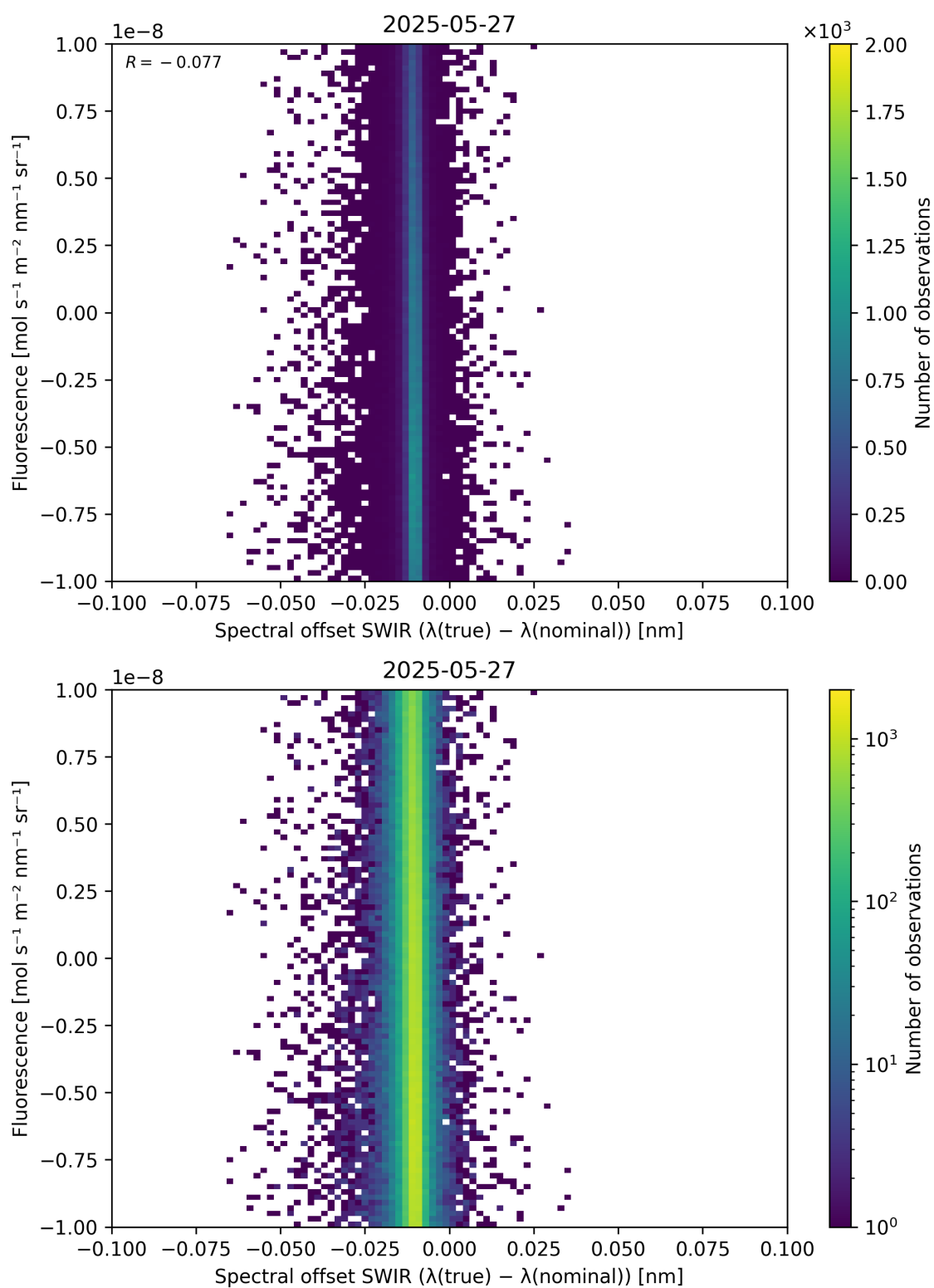
Figure 120: Scatter density plot of “Spectral offset SWIR ( \lambda_{\text{true}} - \lambda_{\text{nominal}} )” against “Fluorescence” for 2025-05-26 to 2025-05-28.
