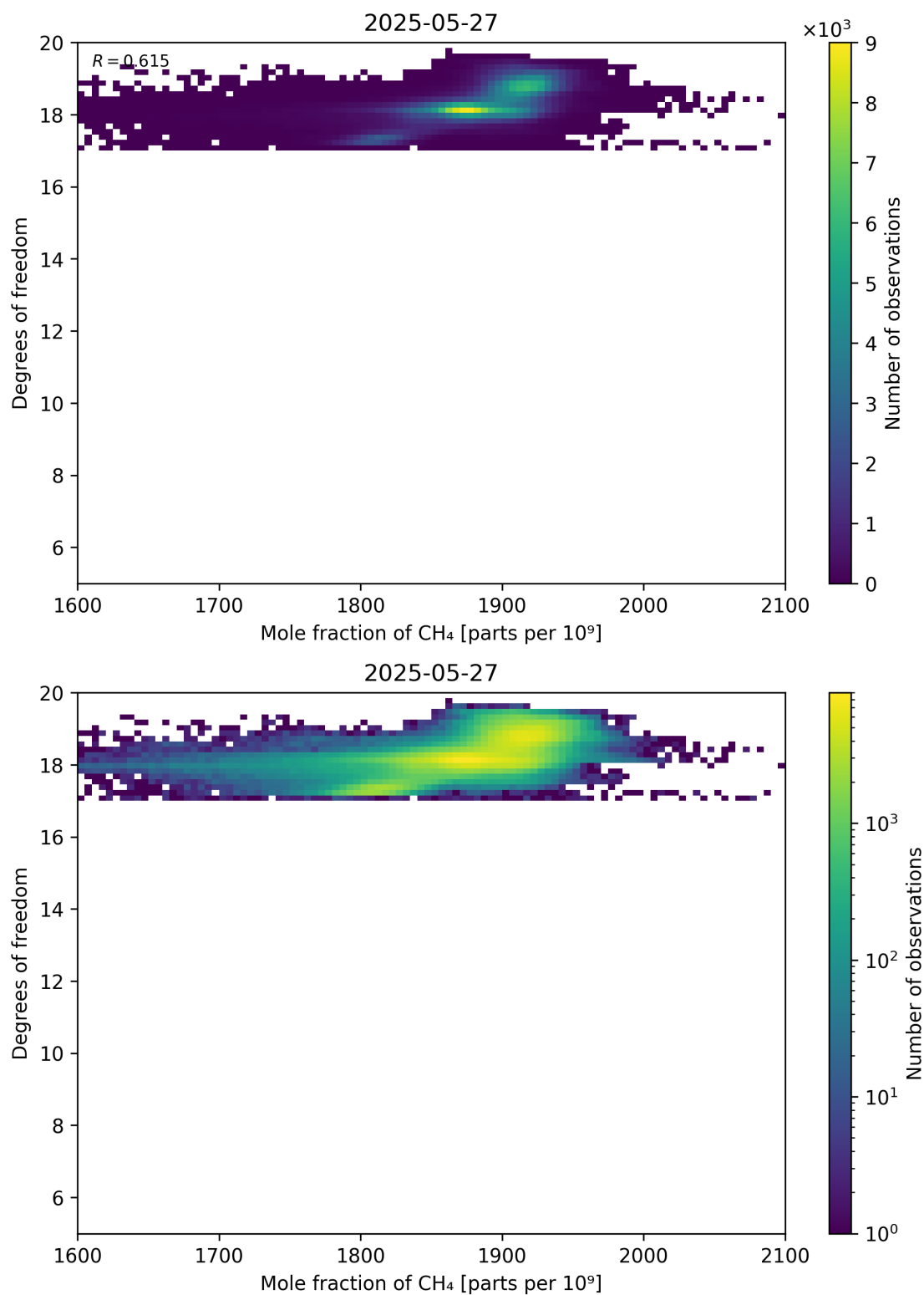
Figure 72: Scatter density plot of “Mole fraction of CH 4 ” against “Degrees of freedom” for 2025-05-26 to 2025-05-28.
