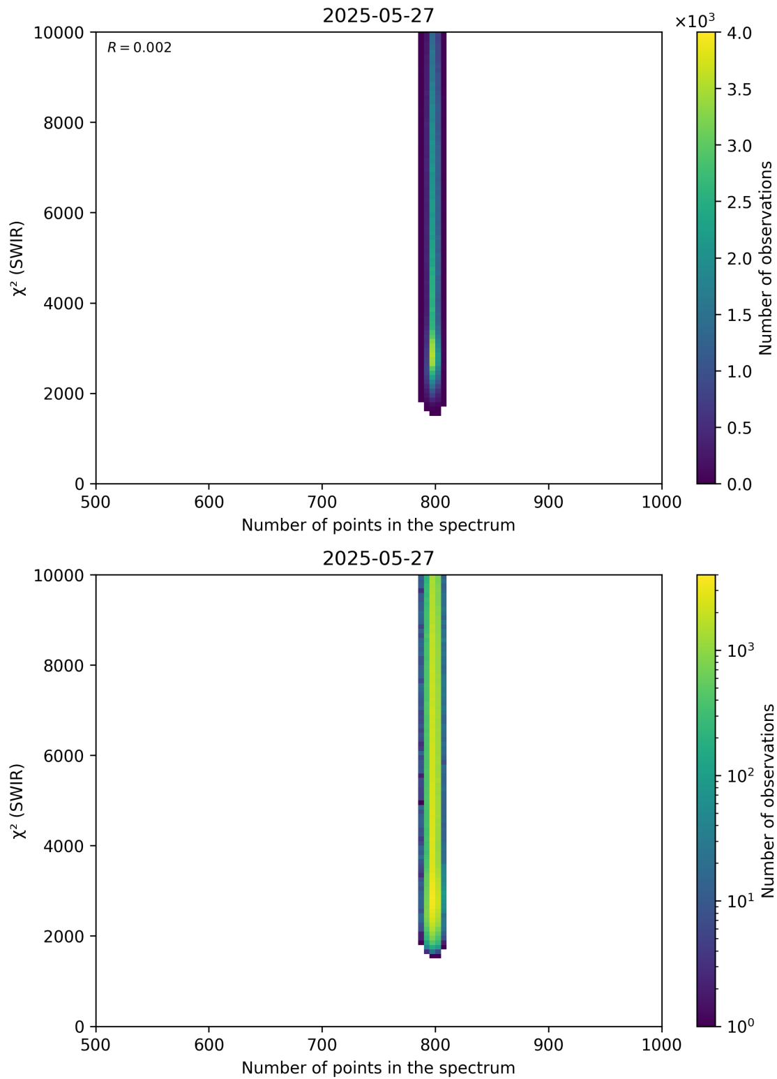
Figure 89: Scatter density plot of “Number of points in the spectrum” against “ \chi^2 (SWIR)” for 2025-05-26 to 2025-05-28.
