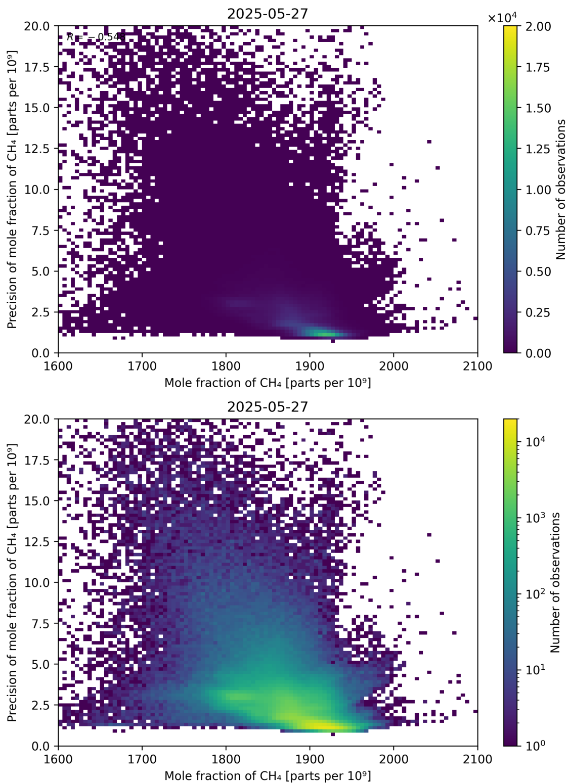
Figure 75: Scatter density plot of “Mole fraction of CH 4 ” against “Precision of mole fraction of CH 4 ” for 2025-05-26 to 2025-05-28.
