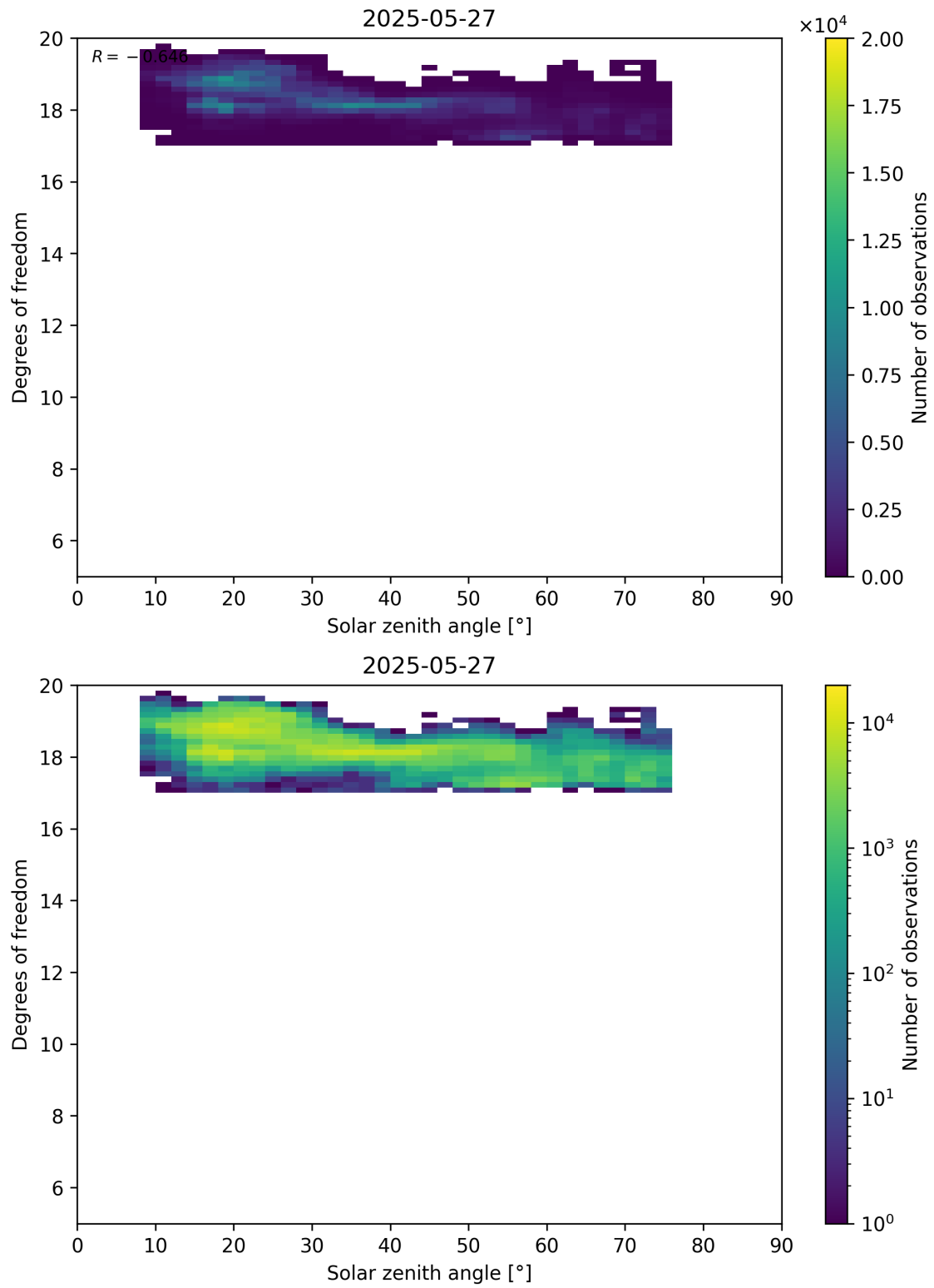
Figure 96: Scatter density plot of “Solar zenith angle” against “Degrees of freedom” for 2025-05-26 to 2025-05-28.
