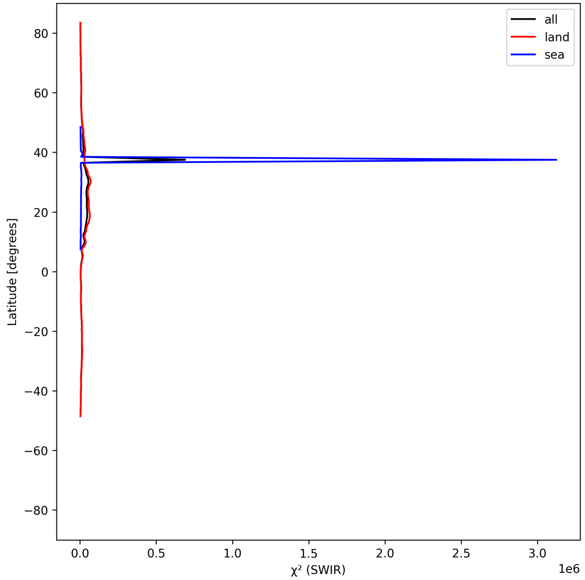
Figure 17: Zonal average of “ \chi^2 (SWIR)” for 2025-05-26 to 2025-05-28.
