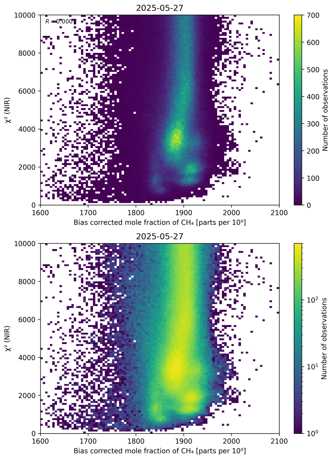
Figure 63: Scatter density plot of “Bias corrected mole fraction of CH 4 ” against “ \chi^2 (NIR)” for 2025-05-26 to 2025-05-28.
