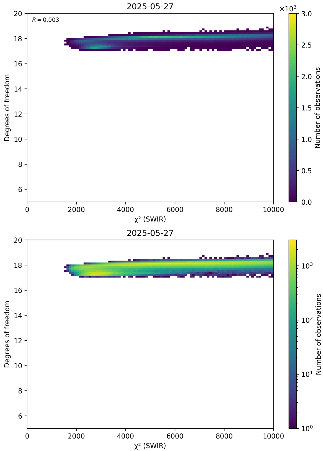
Figure 48: Scatter density plot of “ \chi^2 (SWIR)” against “Degrees of freedom” for 2025-05-26 to 2025-05-28.
