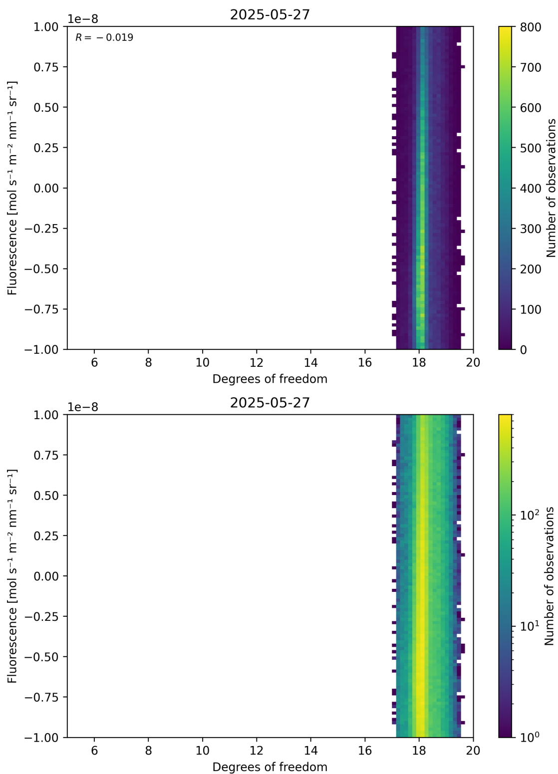
Figure 51: Scatter density plot of “Degrees of freedom” against “Fluorescence” for 2025-05-26 to 2025-05-28.
