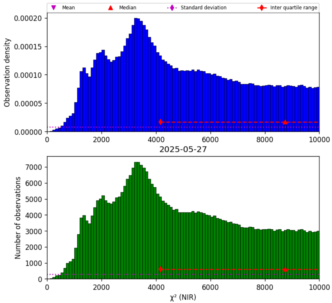
Figure 29: Histogram of " \chi^2 (NIR)" for 2025-05-26 to 2025-05-28
