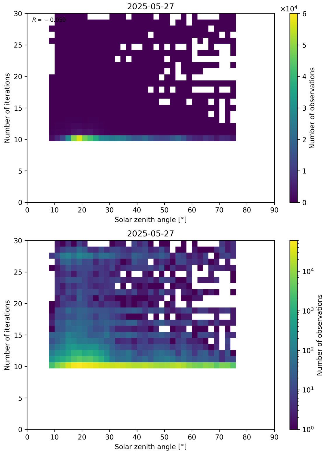
Figure 102: Scatter density plot of “Solar zenith angle” against “Number of iterations” for 2025-05-26 to 2025-05-28.
