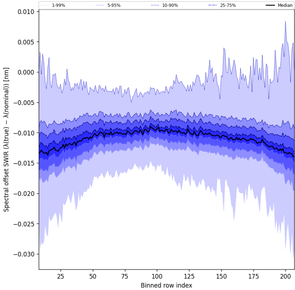
Figure 38: Along track statistics of “Spectral offset SWIR ( \lambda_{\text{true}} - \lambda_{\text{nominal}} )” for 2025-05-26 to 2025-05-28
