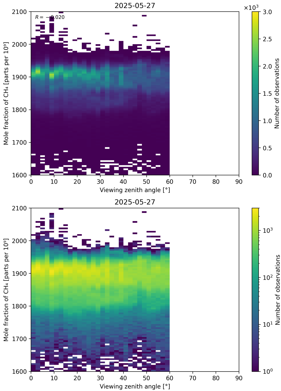
Figure 110: Scatter density plot of “Viewing zenith angle” against “Mole fraction of CH 4 ” for 2025-05-26 to 2025-05-28.
