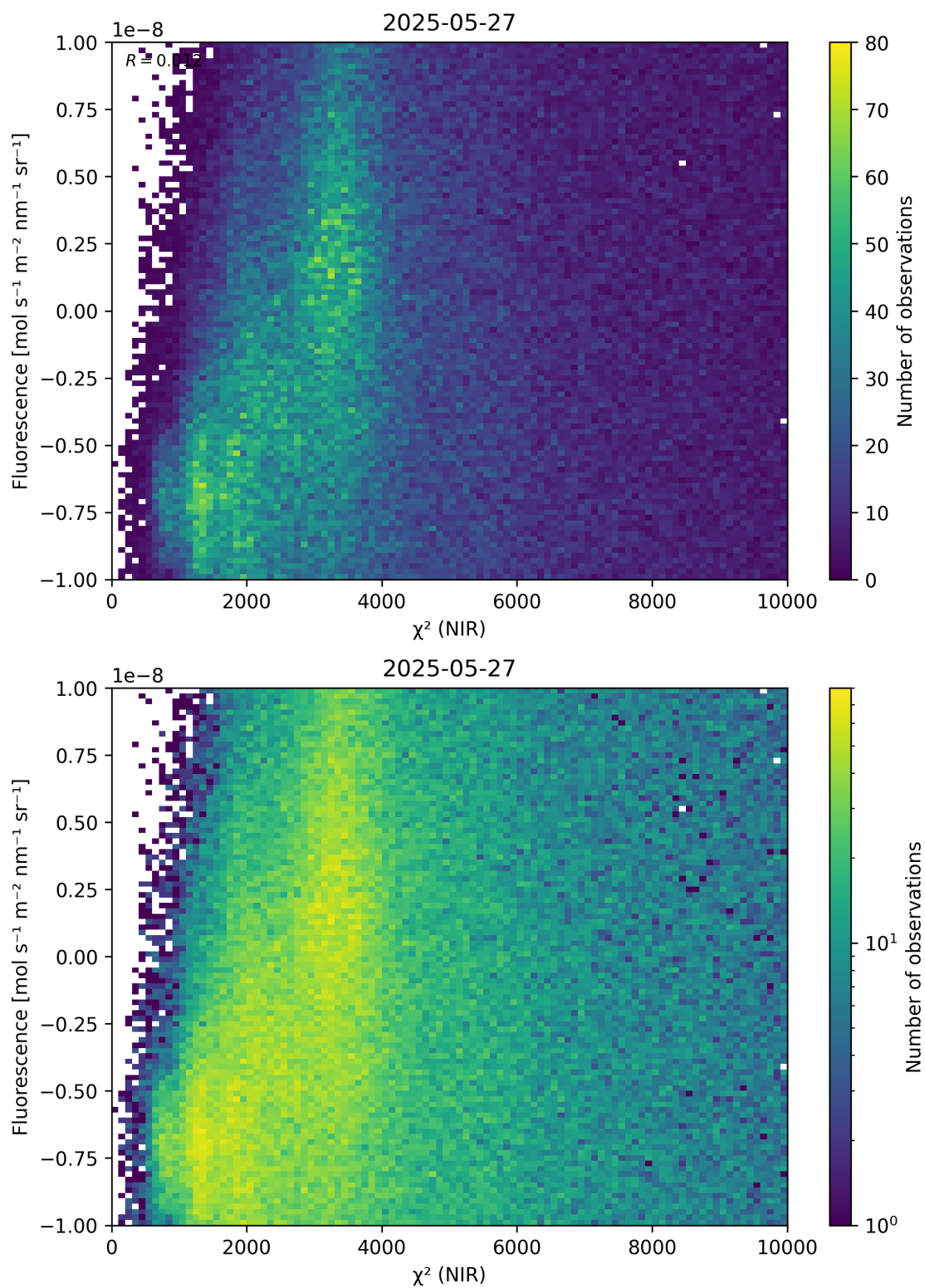
Figure 45: Scatter density plot of “ \chi^2 (NIR)” against “Fluorescence” for 2025-05-26 to 2025-05-28.
