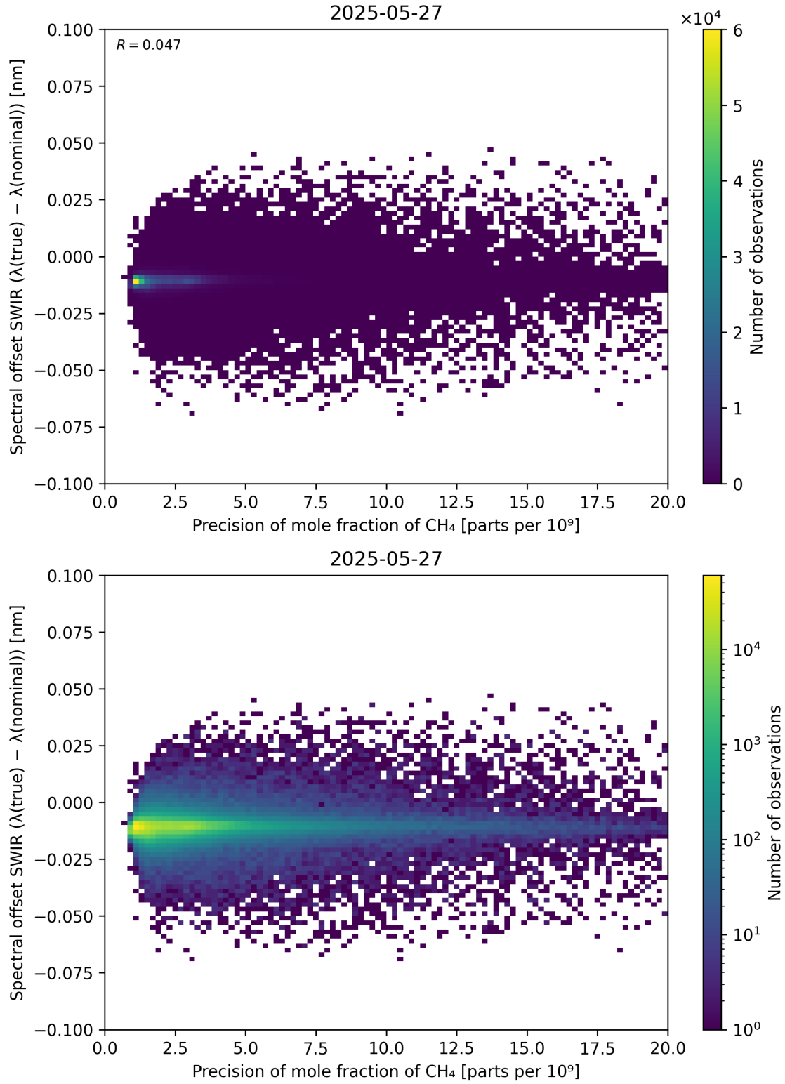
Figure 85: Scatter density plot of “Precision of mole fraction of CH 4 ” against “Spectral offset SWIR ( \lambda_{\text{true}} - \lambda_{\text{nominal}} )” for 2025-05-26 to 2025-05-28.
