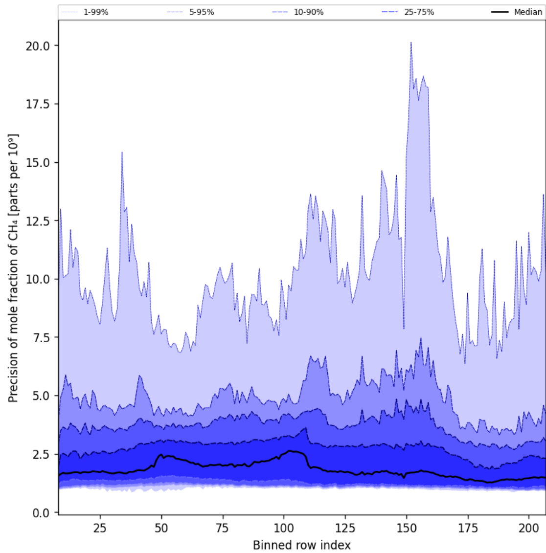
Figure 35: Along track statistics of “Precision of mole fraction of CH 4 ” for 2025-05-26 to 2025-05-28
