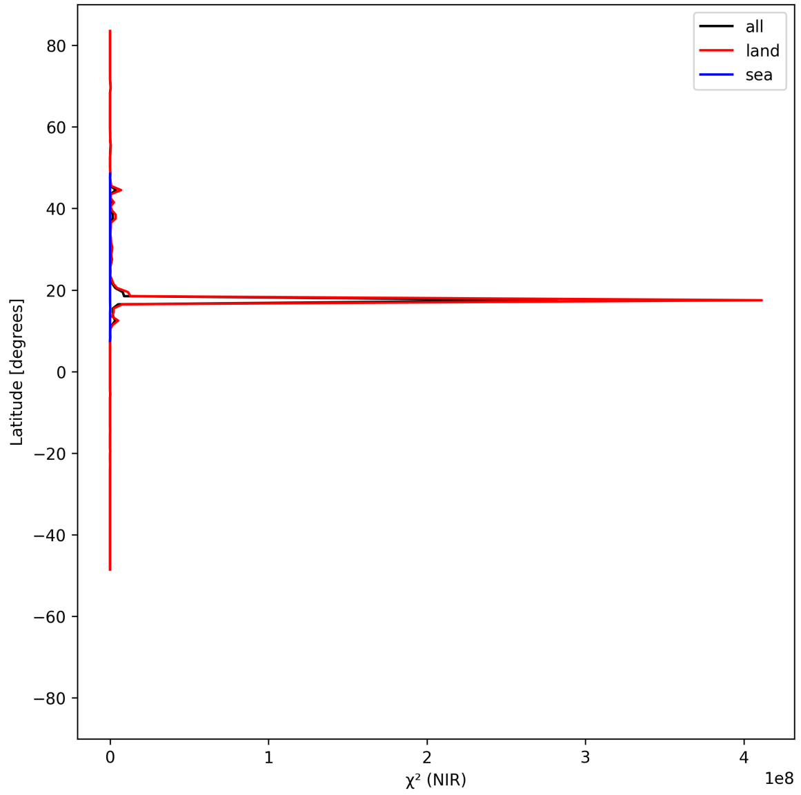
Figure 18: Zonal average of “ \chi^2 (NIR)” for 2025-05-26 to 2025-05-28.
