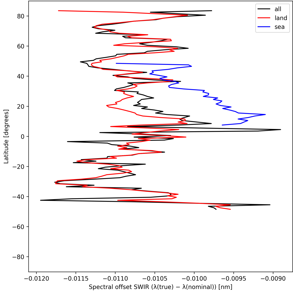
Figure 16: Zonal average of “Spectral offset SWIR ( \lambda_{\text{true}} - \lambda_{\text{nominal}} )” for 2025-05-26 to 2025-05-28.
