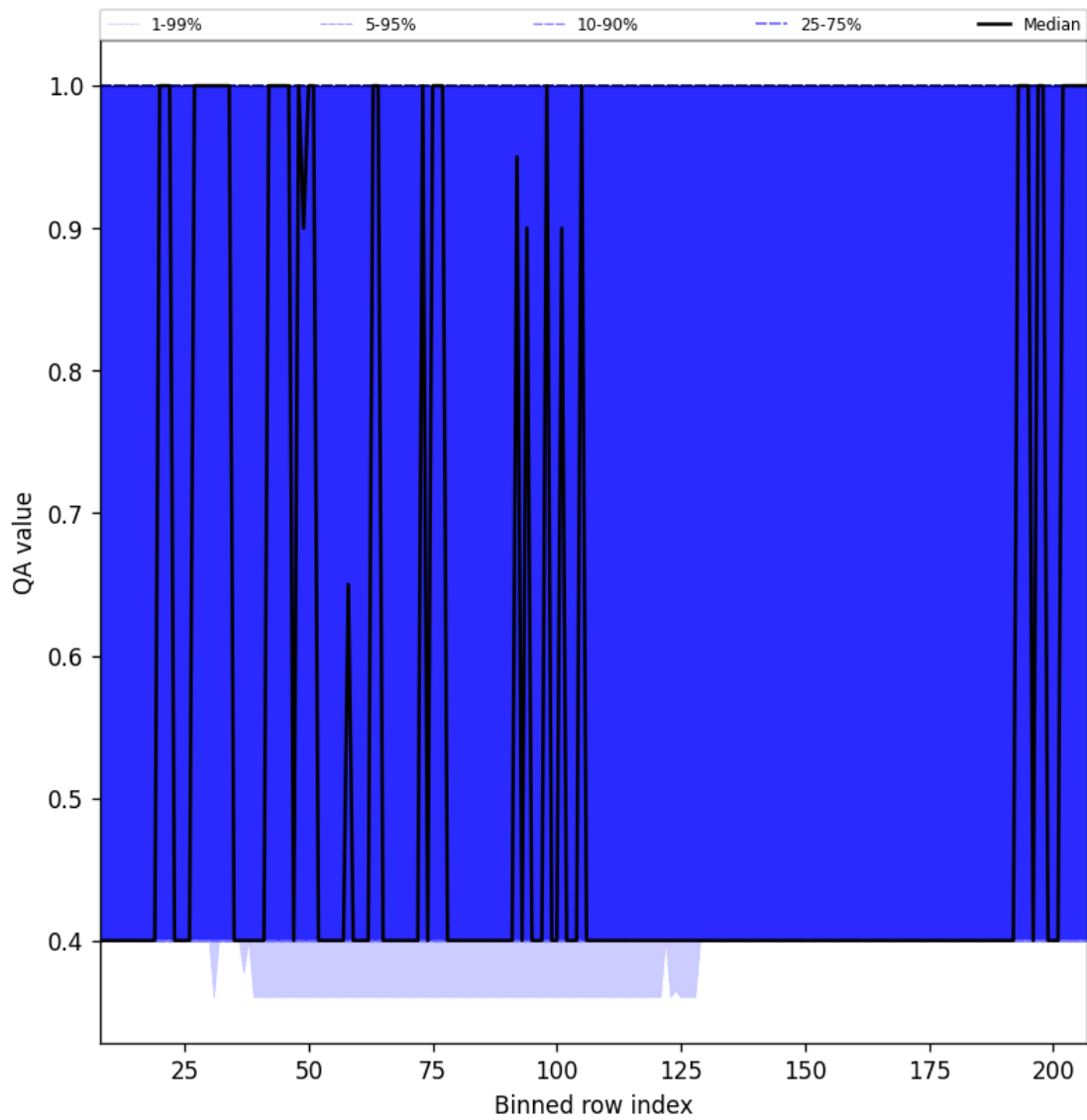
Figure 33: Along track statistics of “QA value” for 2025-05-26 to 2025-05-28
