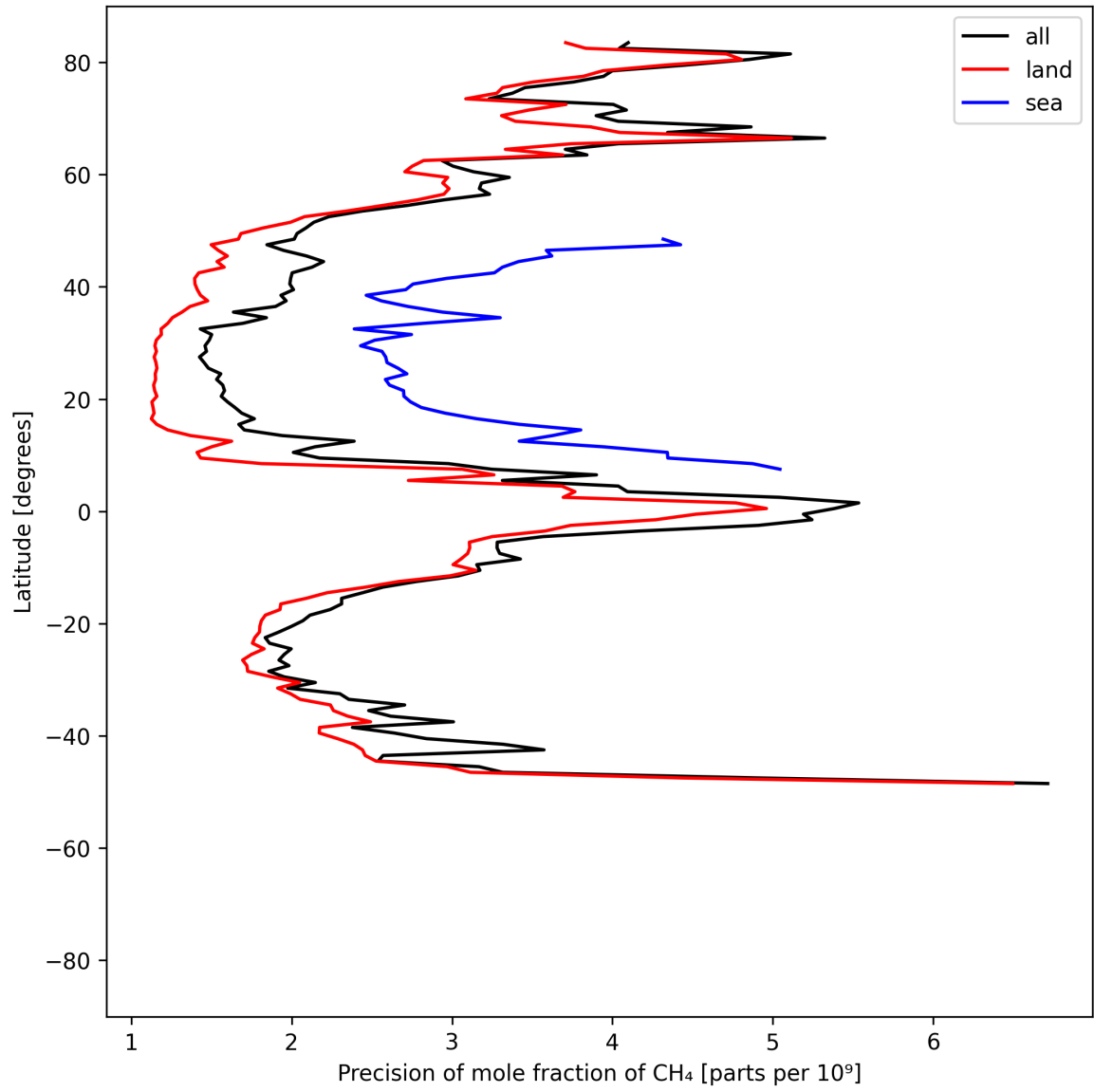
Figure 13: Zonal average of “Precision of mole fraction of CH 4 ” for 2025-05-26 to 2025-05-28.
