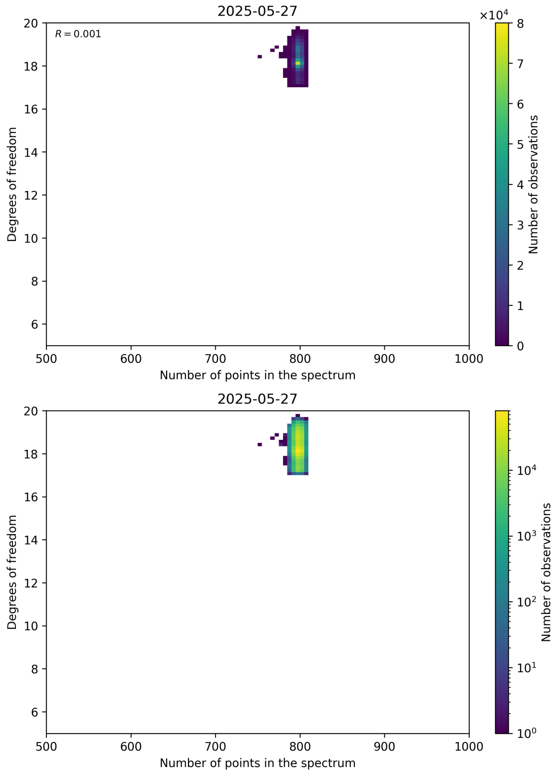
Figure 90: Scatter density plot of “Number of points in the spectrum” against “Degrees of freedom” for 2025-05-26 to 2025-05-28.
