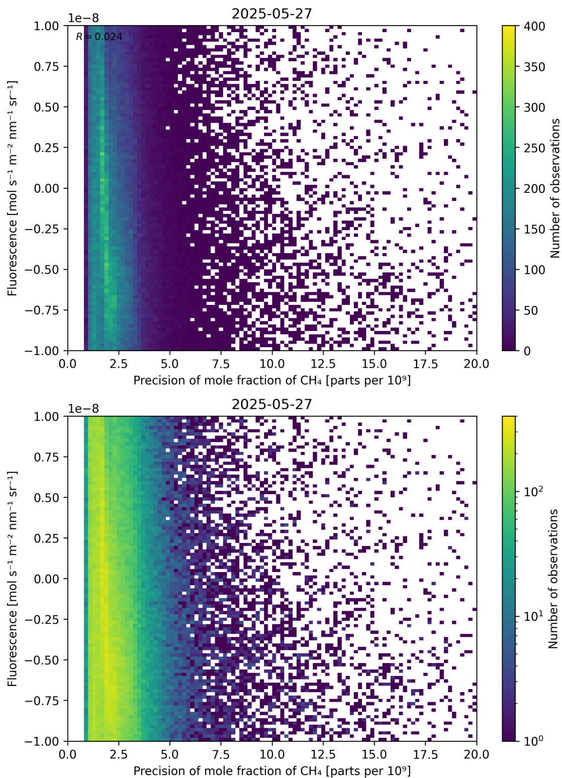
Figure 81: Scatter density plot of “Precision of mole fraction of \text{CH}_4 ” against “Fluorescence” for 2025-05-26 to 2025-05-28.
