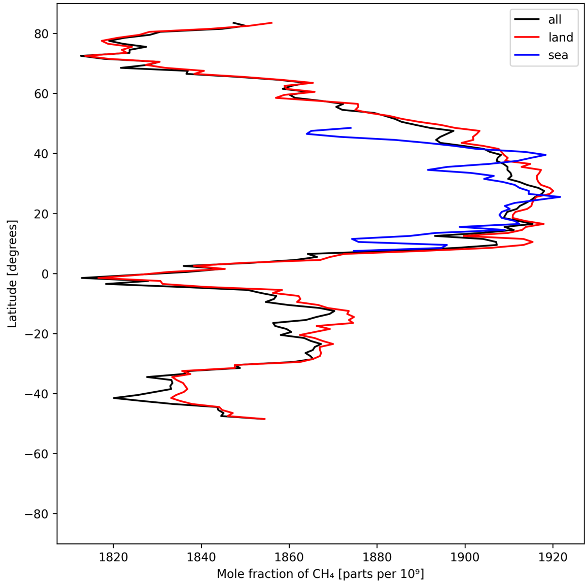
Figure 12: Zonal average of “Mole fraction of CH 4 ” for 2025-05-26 to 2025-05-28.
