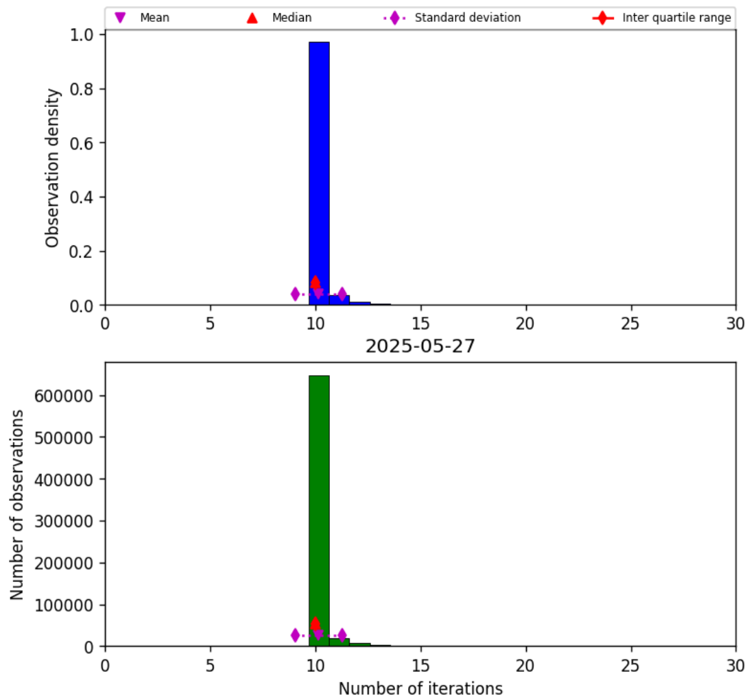
Figure 31: Histogram of “Number of iterations” for 2025-05-26 to 2025-05-28
