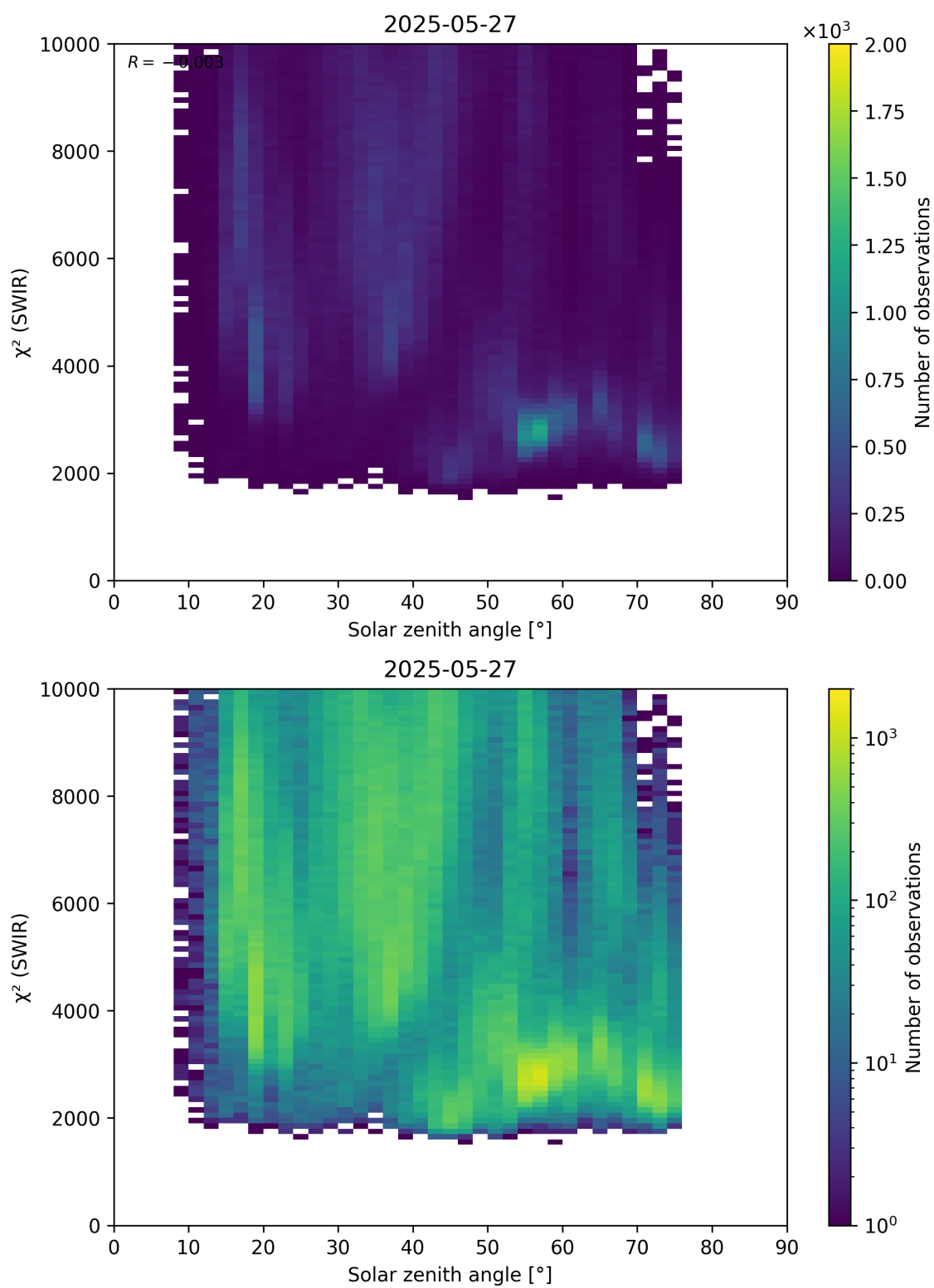
Figure 95: Scatter density plot of “Solar zenith angle” against “ \chi^2 (SWIR)” for 2025-05-26 to 2025-05-28.
