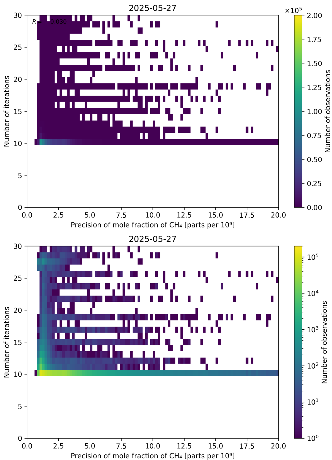
Figure 83: Scatter density plot of “Precision of mole fraction of CH 4 ” against “Number of iterations” for 2025-05-26 to 2025-05-28.
