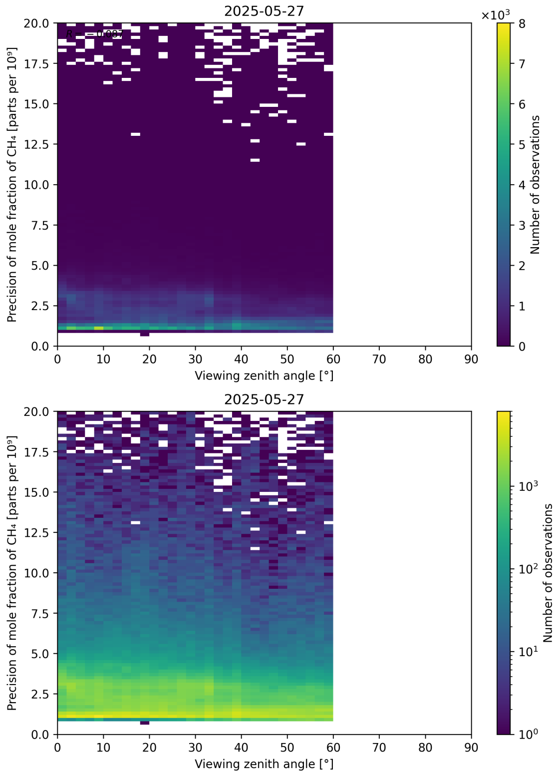
Figure 112: Scatter density plot of “Viewing zenith angle” against “Precision of mole fraction of CH 4 ” for 2025-05-26 to 2025-05-28.
