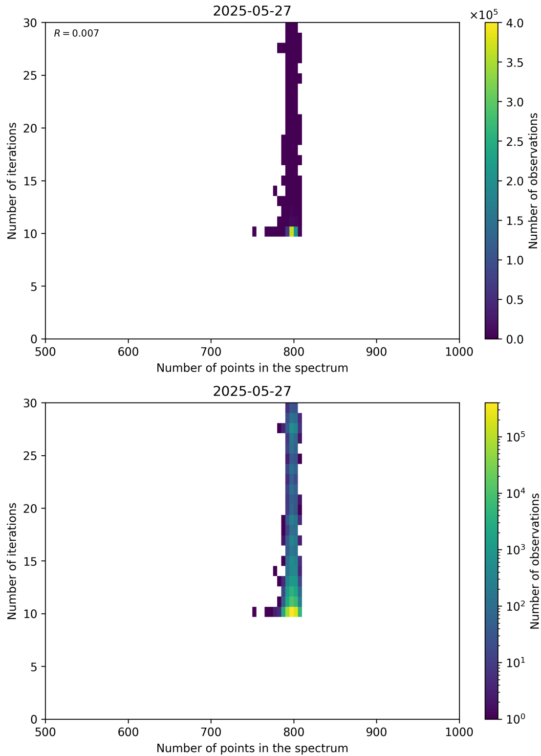
Figure 92: Scatter density plot of “Number of points in the spectrum” against “Number of iterations” for 2025-05-26 to 2025-05-28.
