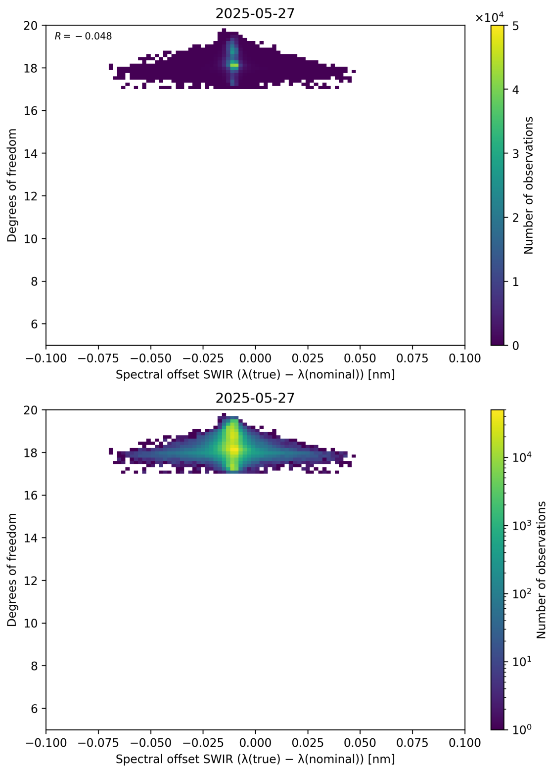
Figure 119: Scatter density plot of “Spectral offset SWIR ( \lambda_{\text{true}} - \lambda_{\text{nominal}} )” against “Degrees of freedom” for 2025-05-26 to 2025-05-28.
