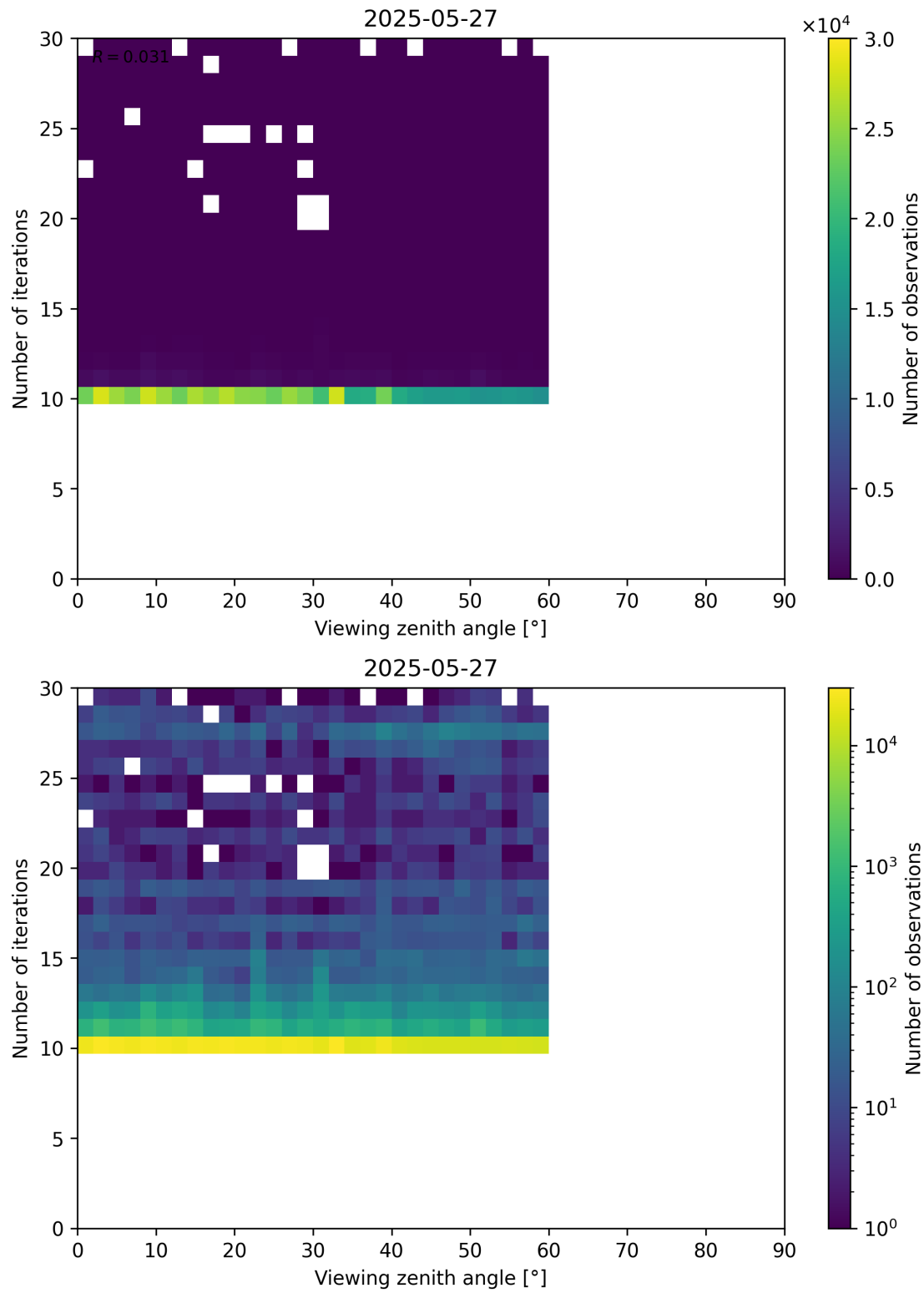
Figure 113: Scatter density plot of “Viewing zenith angle” against “Number of iterations” for 2025-05-26 to 2025-05-28.
