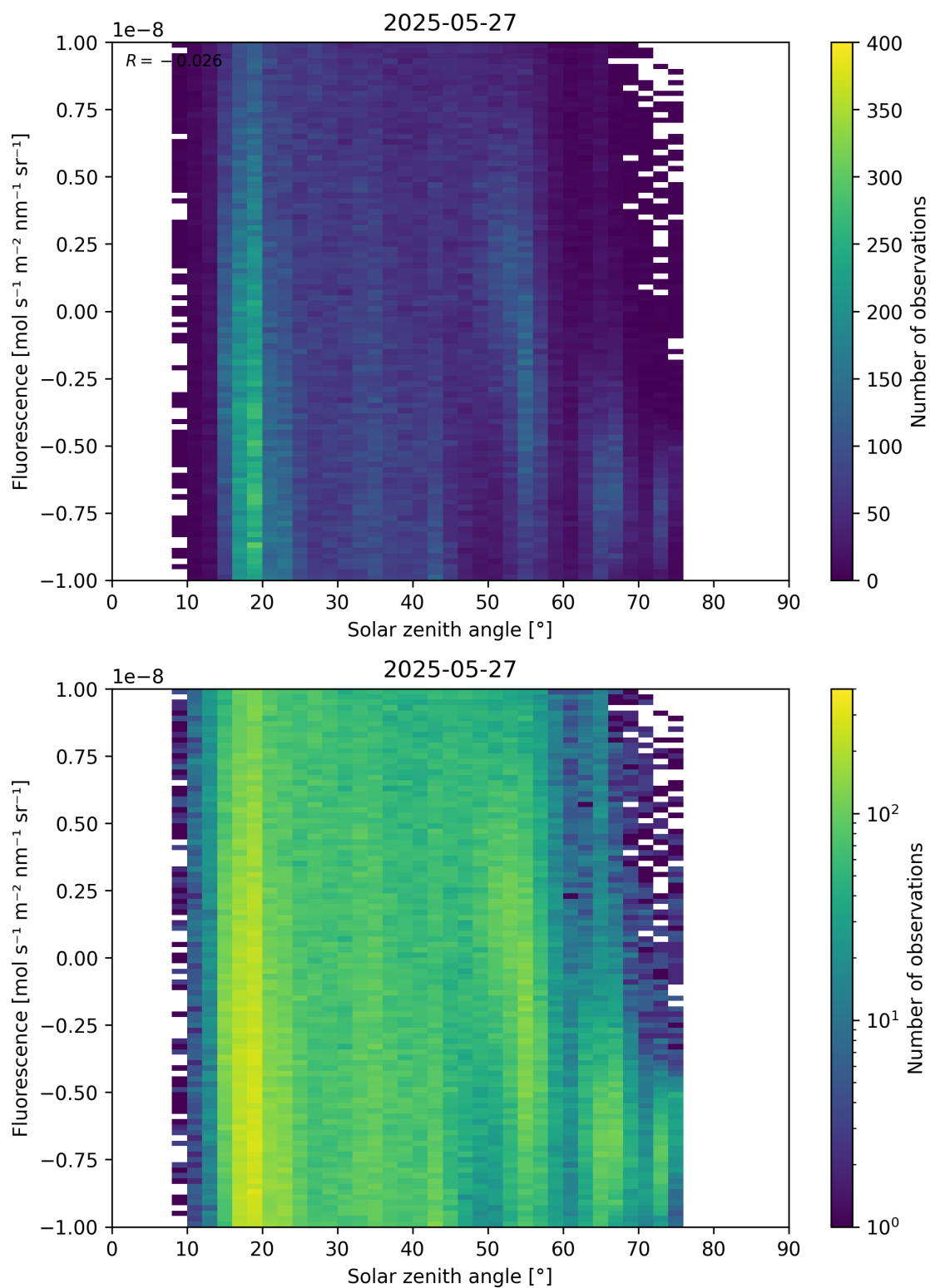
Figure 97: Scatter density plot of “Solar zenith angle” against “Fluorescence” for 2025-05-26 to 2025-05-28.
