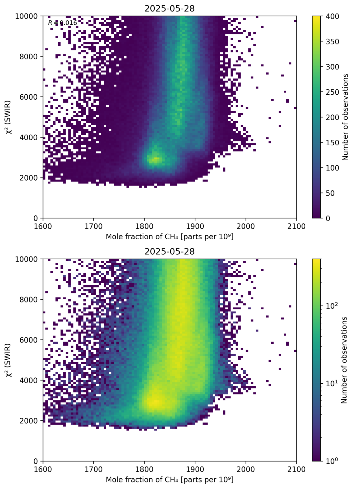
Figure 71: Scatter density plot of “Mole fraction of \text{CH}_4 ” against “ \chi^2 (SWIR)” for 2025-05-27 to 2025-05-29.
