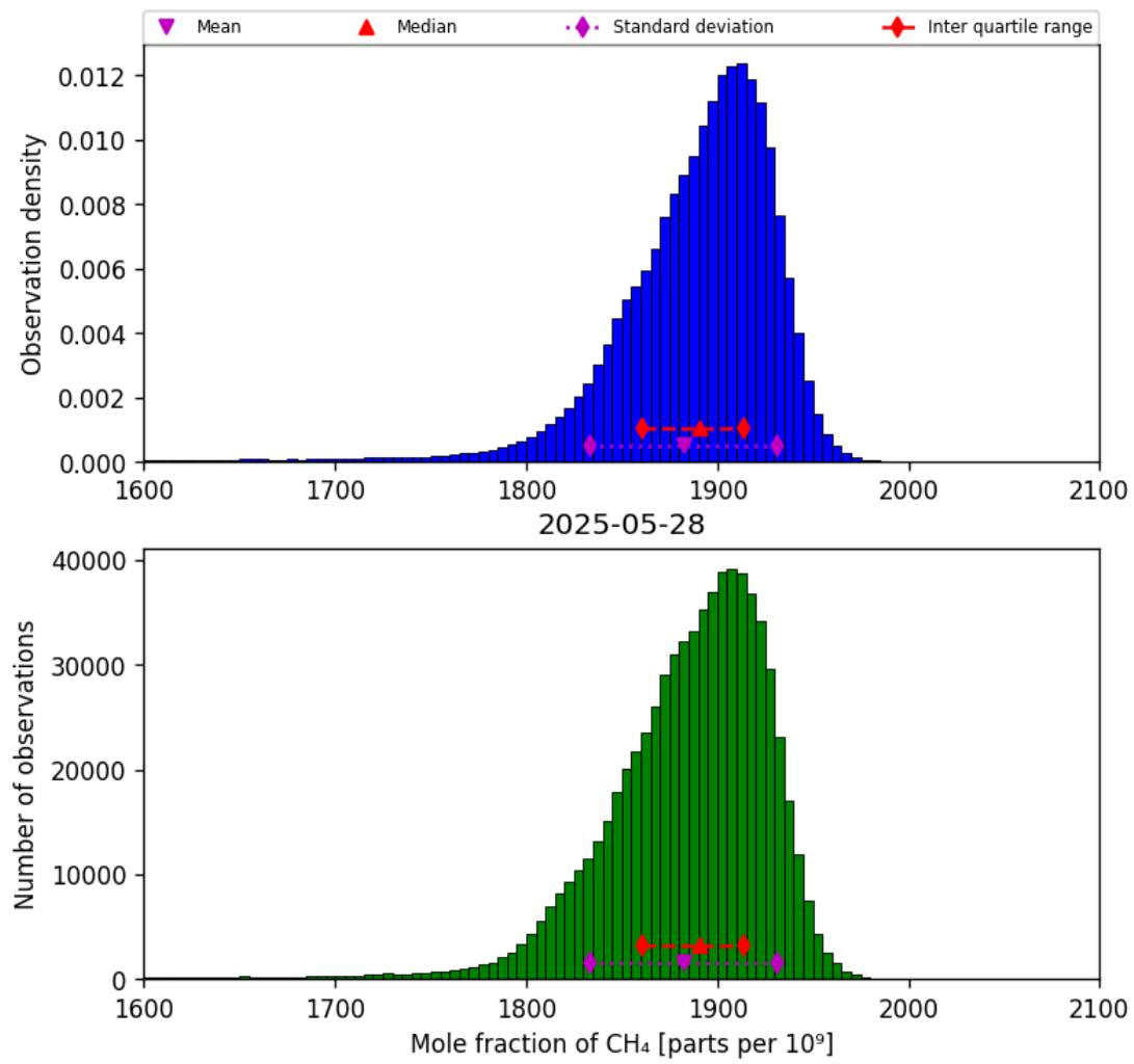
Figure 23: Histogram of “Mole fraction of CH 4 ” for 2025-05-27 to 2025-05-29
