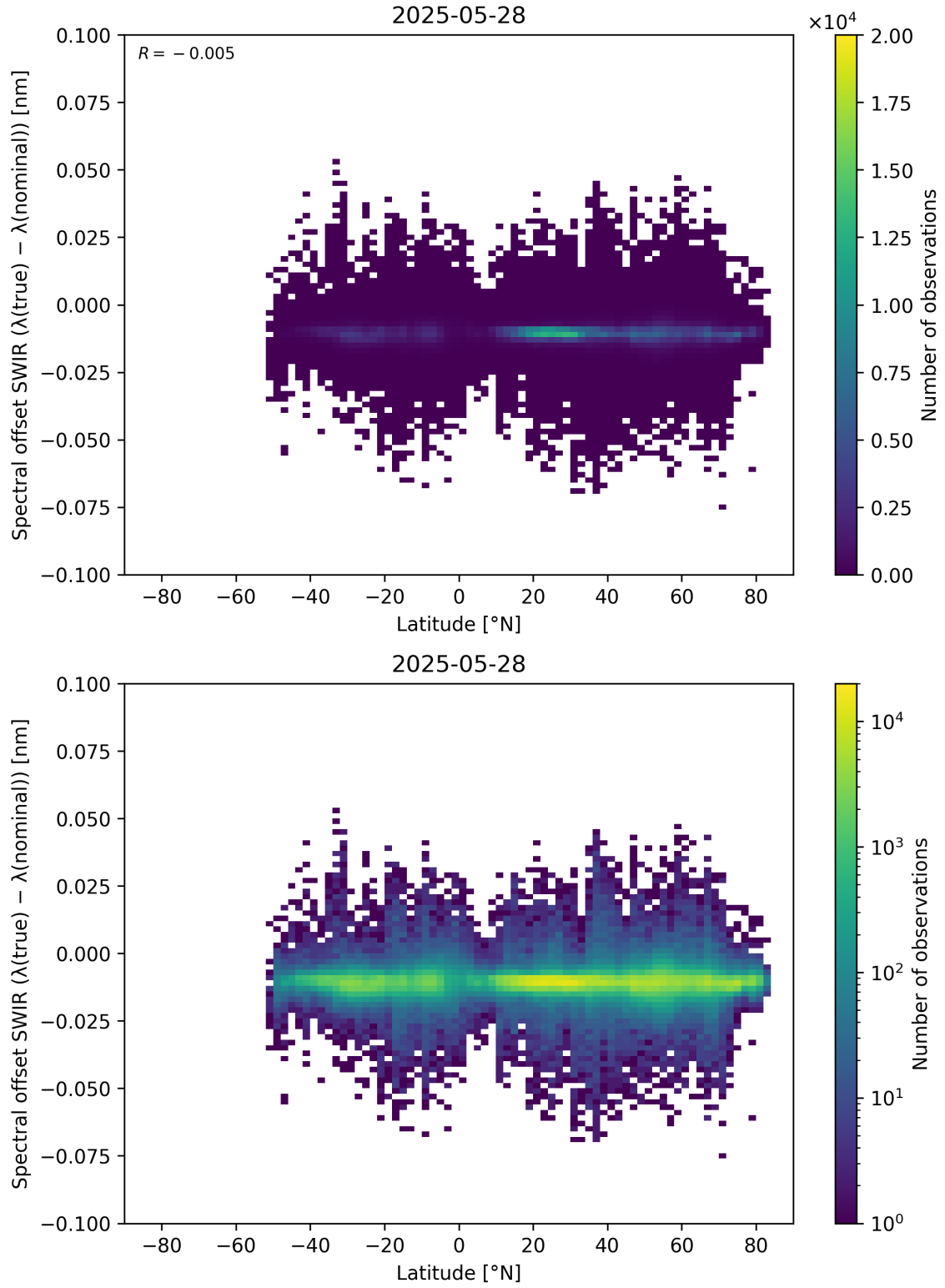
Figure 62: Scatter density plot of “Latitude” against “Spectral offset SWIR ( \lambda_{\text{true}} - \lambda_{\text{nominal}} )” for 2025-05-27 to 2025-05-29.
