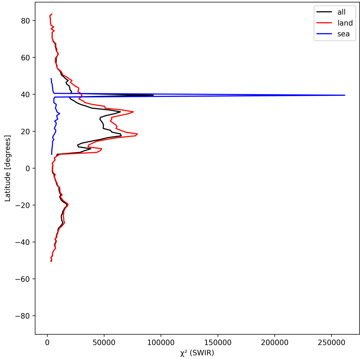
Figure 17: Zonal average of “ \chi^2 (SWIR)” for 2025-05-27 to 2025-05-29.
