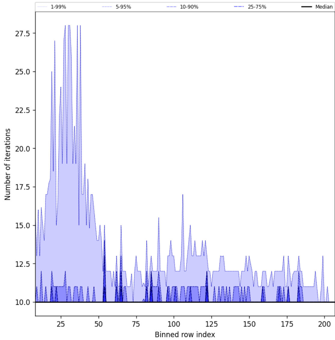
Figure 42: Along track statistics of “Number of iterations” for 2025-05-27 to 2025-05-29
