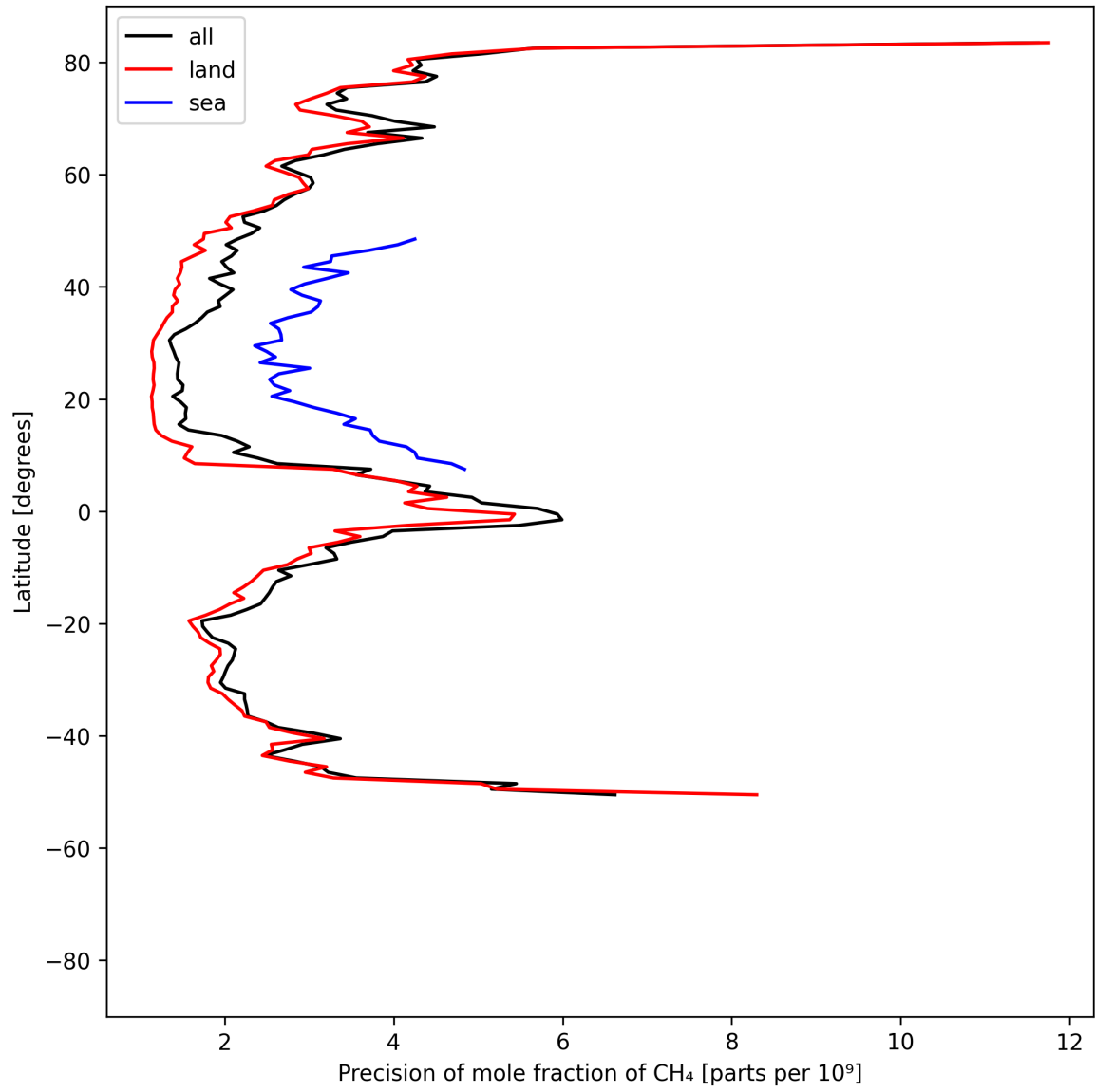
Figure 13: Zonal average of “Precision of mole fraction of CH 4 ” for 2025-05-27 to 2025-05-29.
