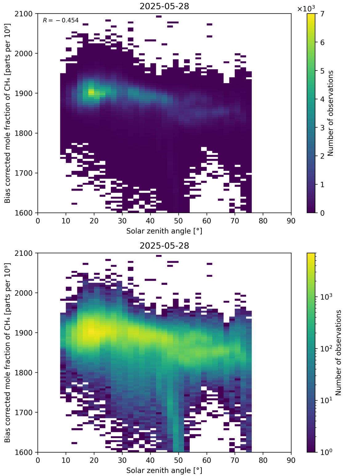
Figure 100: Scatter density plot of “Solar zenith angle” against “Bias corrected mole fraction of \text{CH}_4 ” for 2025-05-27 to 2025-05-29.
