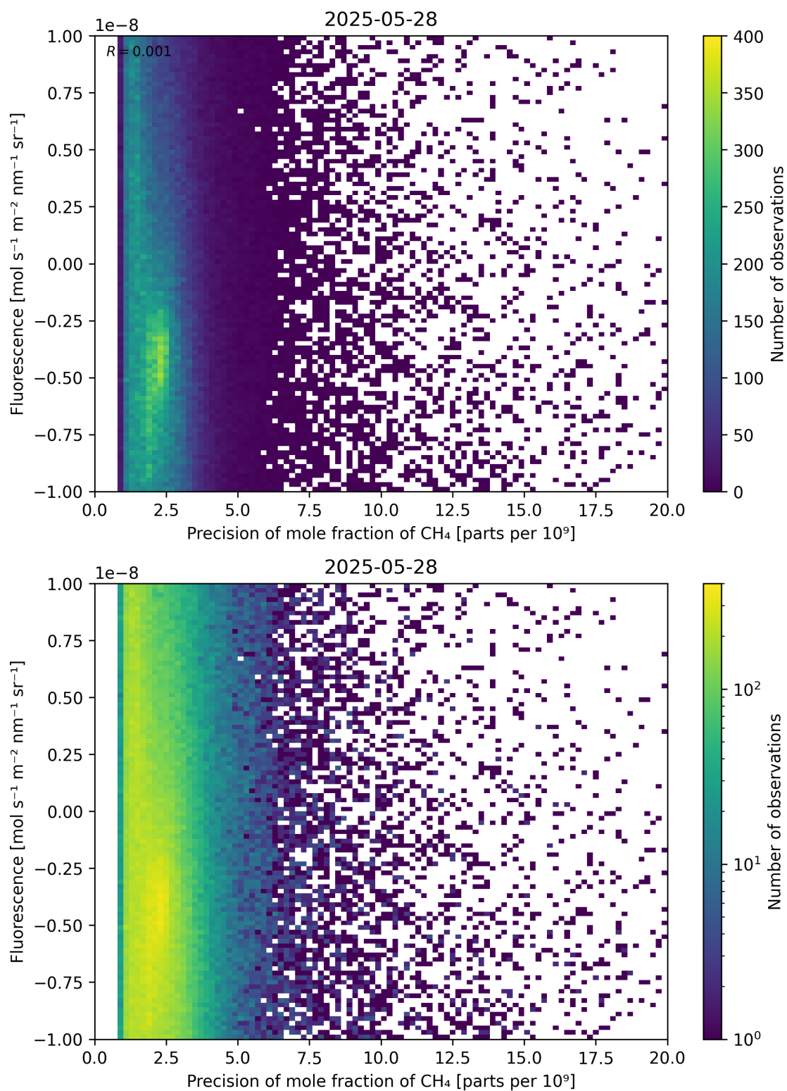
Figure 81: Scatter density plot of “Precision of mole fraction of \text{CH}_4 ” against “Fluorescence” for 2025-05-27 to 2025-05-29.
