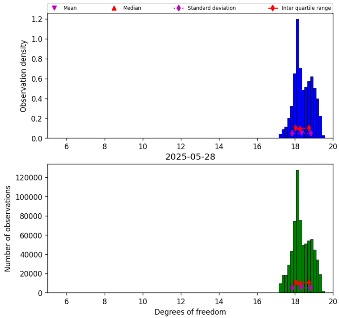
Figure 30: Histogram of “Degrees of freedom” for 2025-05-27 to 2025-05-29
