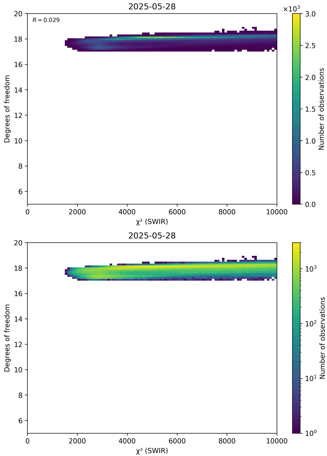
Figure 48: Scatter density plot of “ \chi^2 (SWIR)” against “Degrees of freedom” for 2025-05-27 to 2025-05-29.
