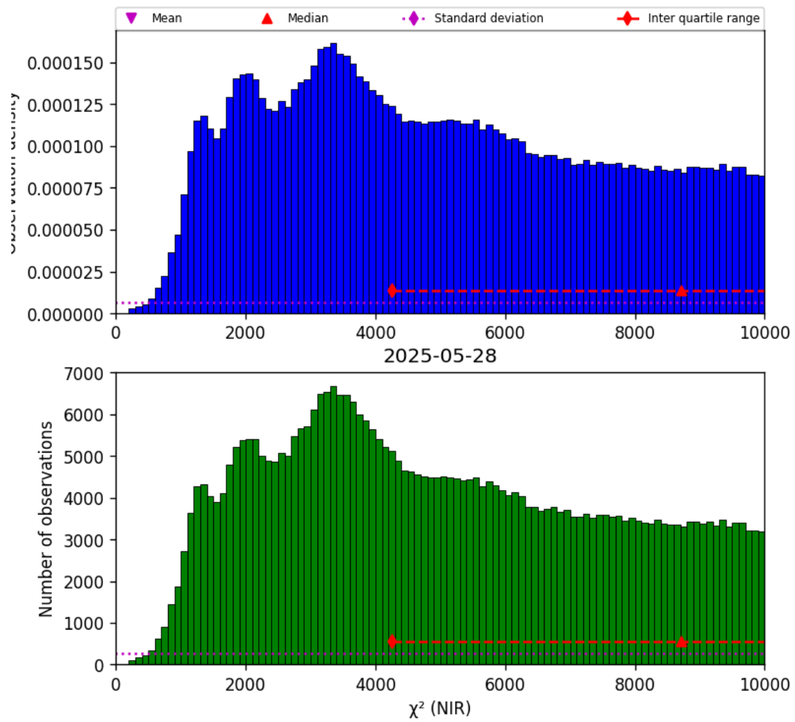
Figure 29: Histogram of “ \chi^2 (NIR)” for 2025-05-27 to 2025-05-29
