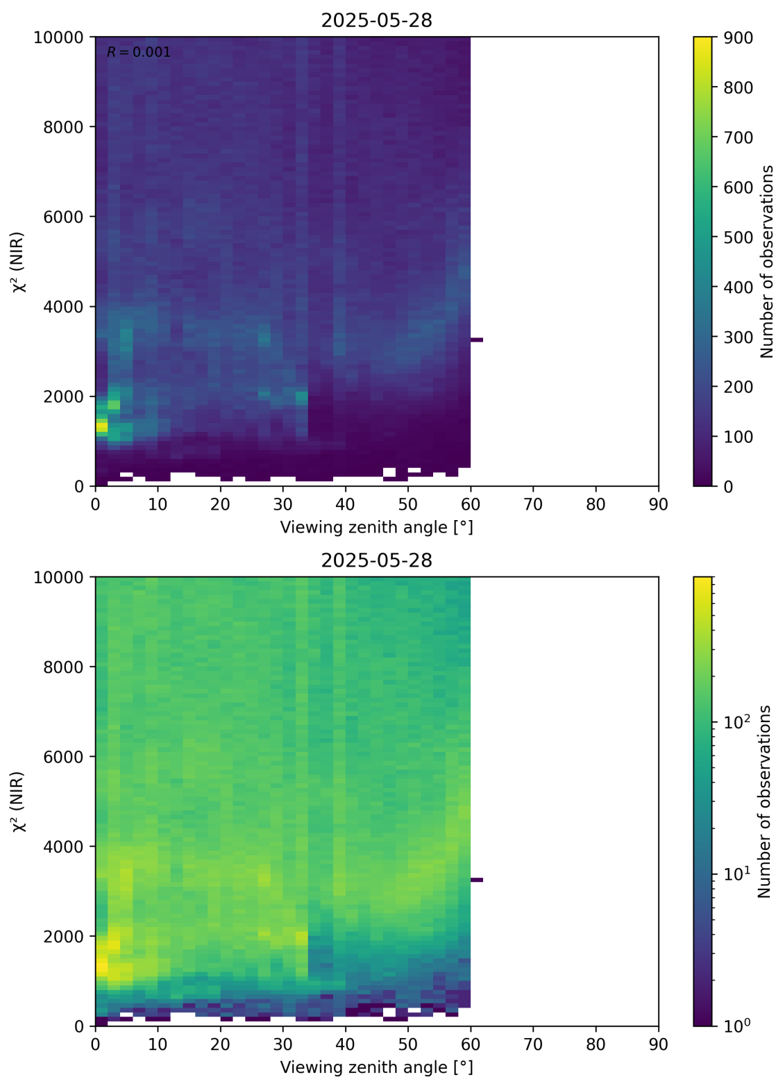
Figure 105: Scatter density plot of “Viewing zenith angle” against “ \chi^2 (NIR)” for 2025-05-27 to 2025-05-29.
