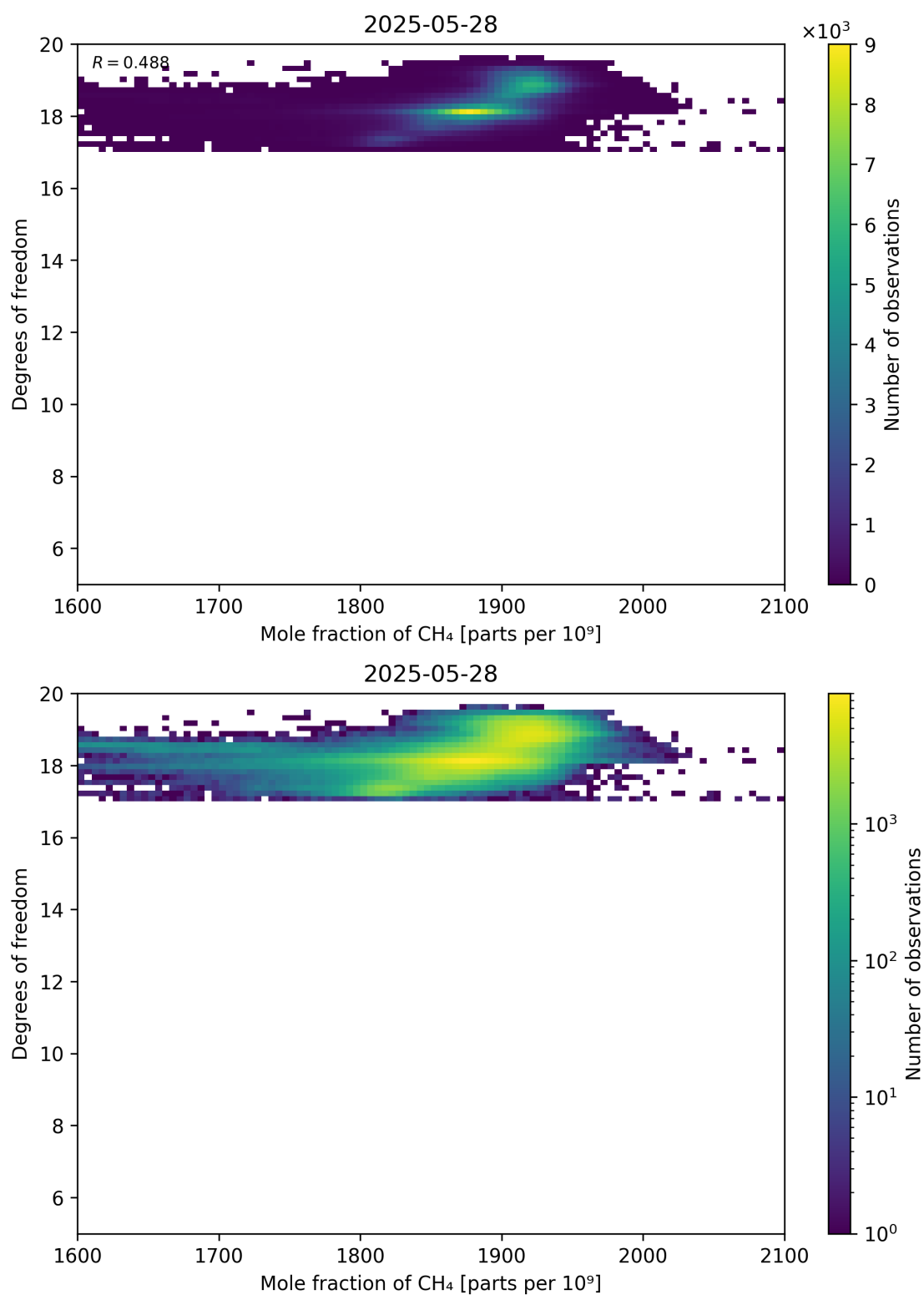
Figure 72: Scatter density plot of “Mole fraction of CH 4 ” against “Degrees of freedom” for 2025-05-27 to 2025-05-29.
