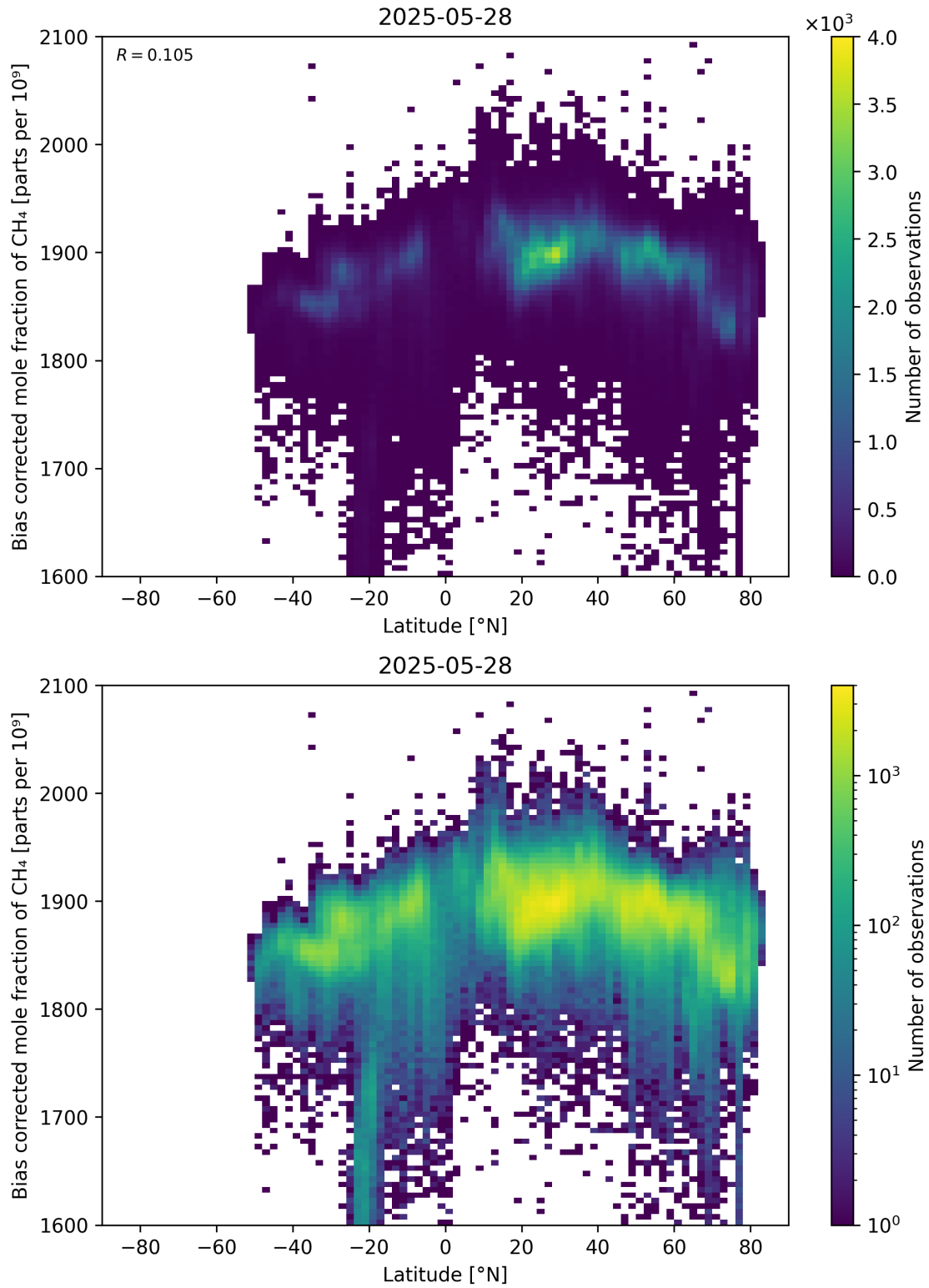
Figure 58: Scatter density plot of “Latitude” against “Bias corrected mole fraction of \text{CH}_4 ” for 2025-05-27 to 2025-05-29.
