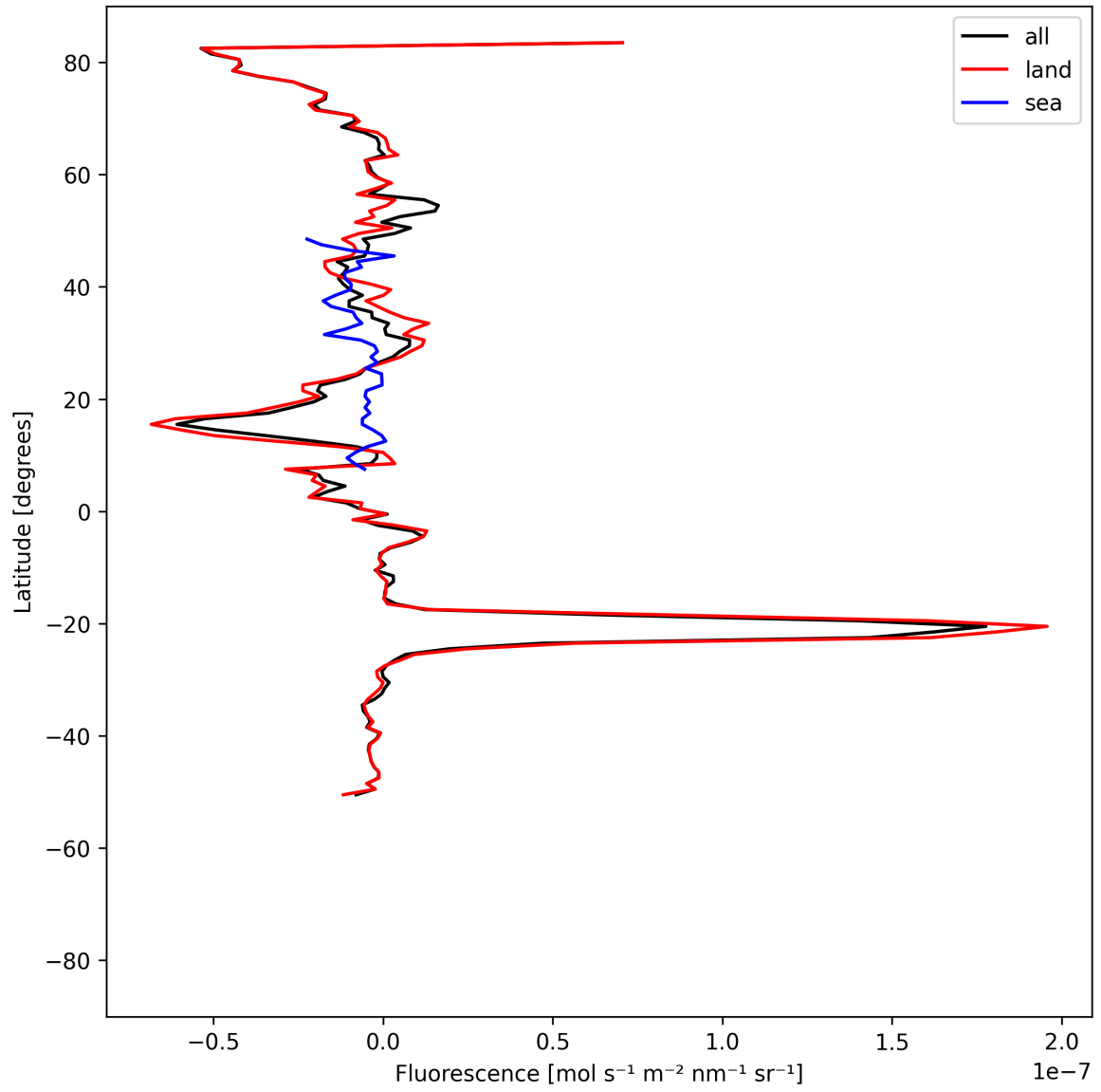
Figure 21: Zonal average of “Fluorescence” for 2025-05-27 to 2025-05-29.
