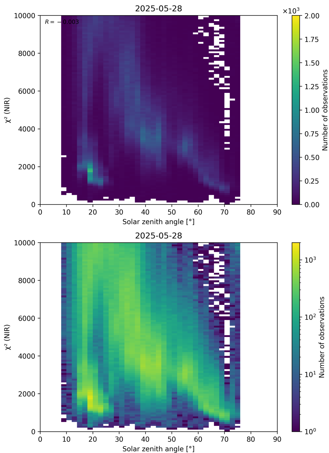
Figure 94: Scatter density plot of “Solar zenith angle” against “ \chi^2 (NIR)” for 2025-05-27 to 2025-05-29.
