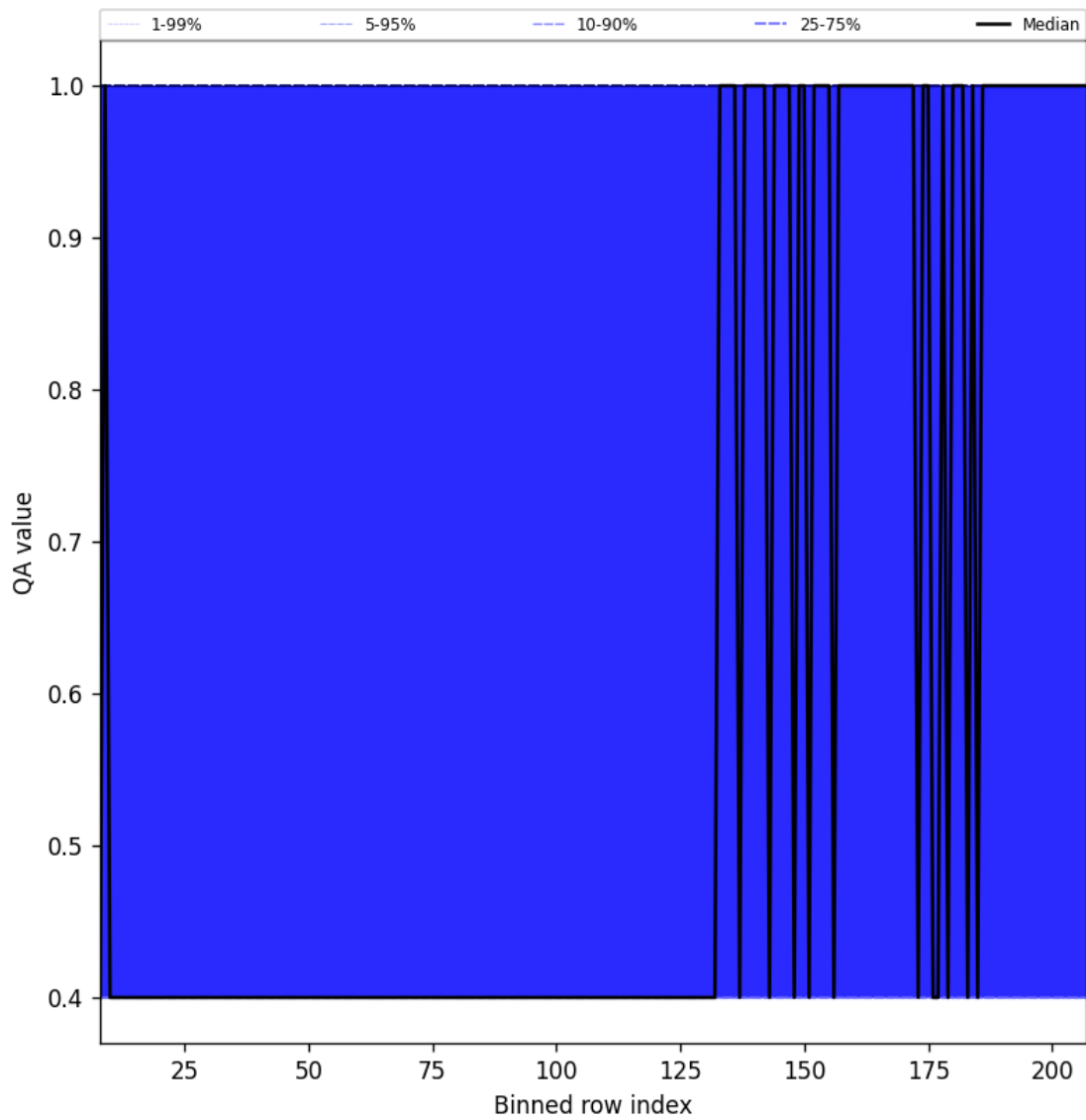
Figure 33: Along track statistics of “QA value” for 2025-05-27 to 2025-05-29
