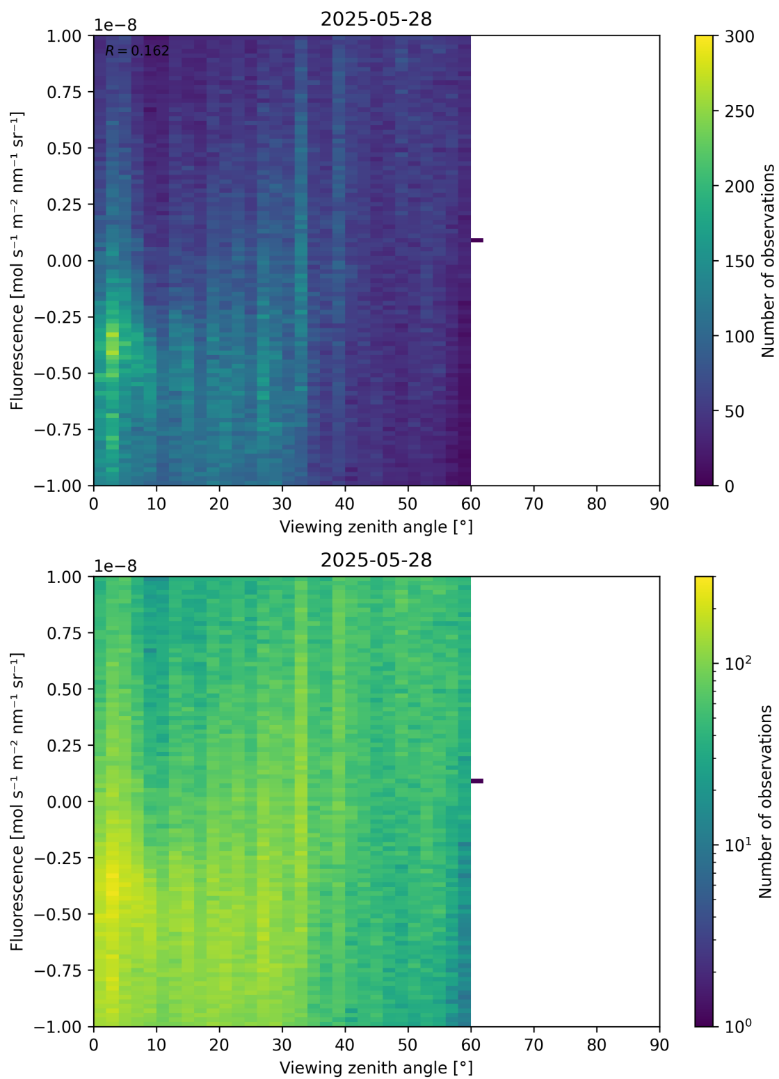
Figure 108: Scatter density plot of “Viewing zenith angle” against “Fluorescence” for 2025-05-27 to 2025-05-29.
