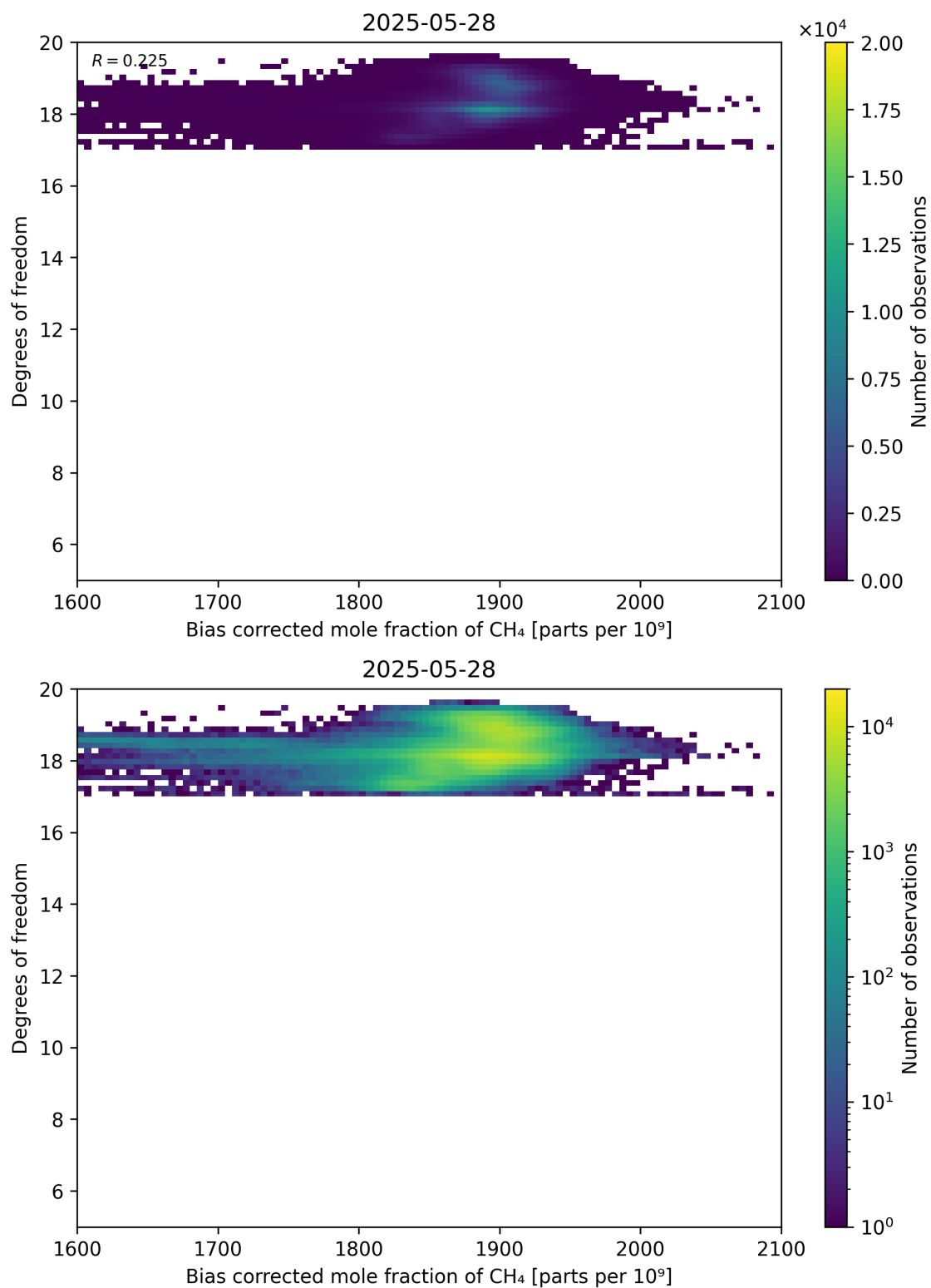
Figure 65: Scatter density plot of “Bias corrected mole fraction of CH 4 ” against “Degrees of freedom” for 2025-05-27 to 2025-05-29.
