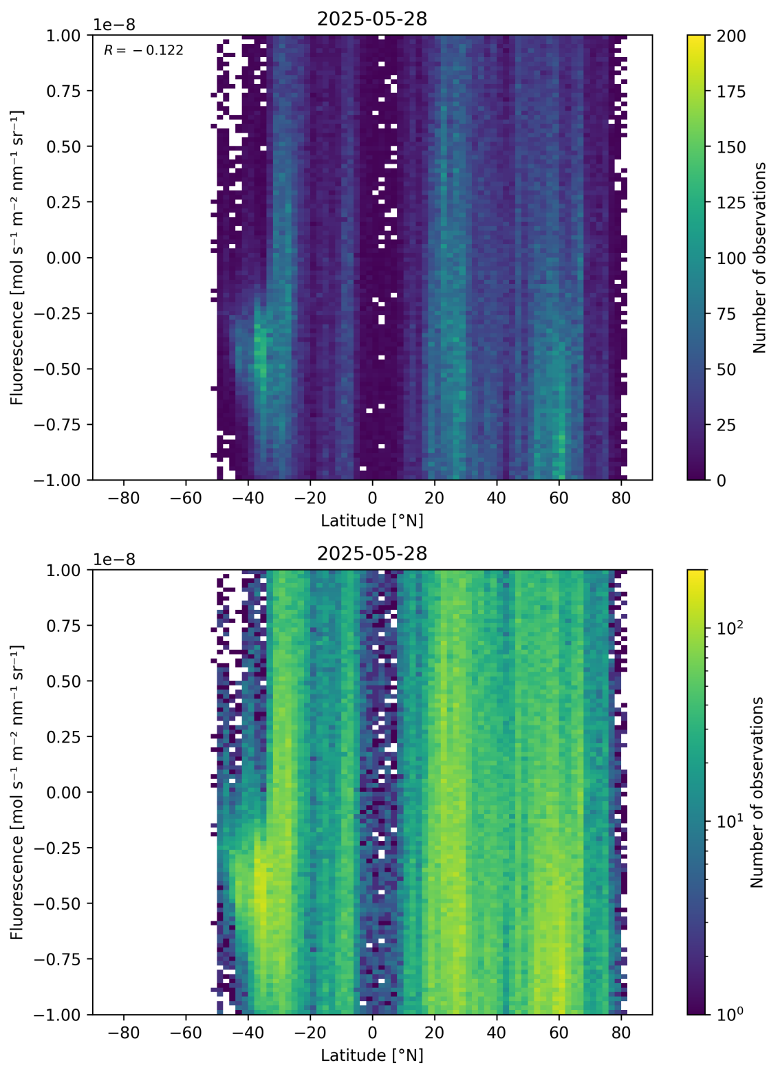
Figure 56: Scatter density plot of “Latitude” against “Fluorescence” for 2025-05-27 to 2025-05-29.
