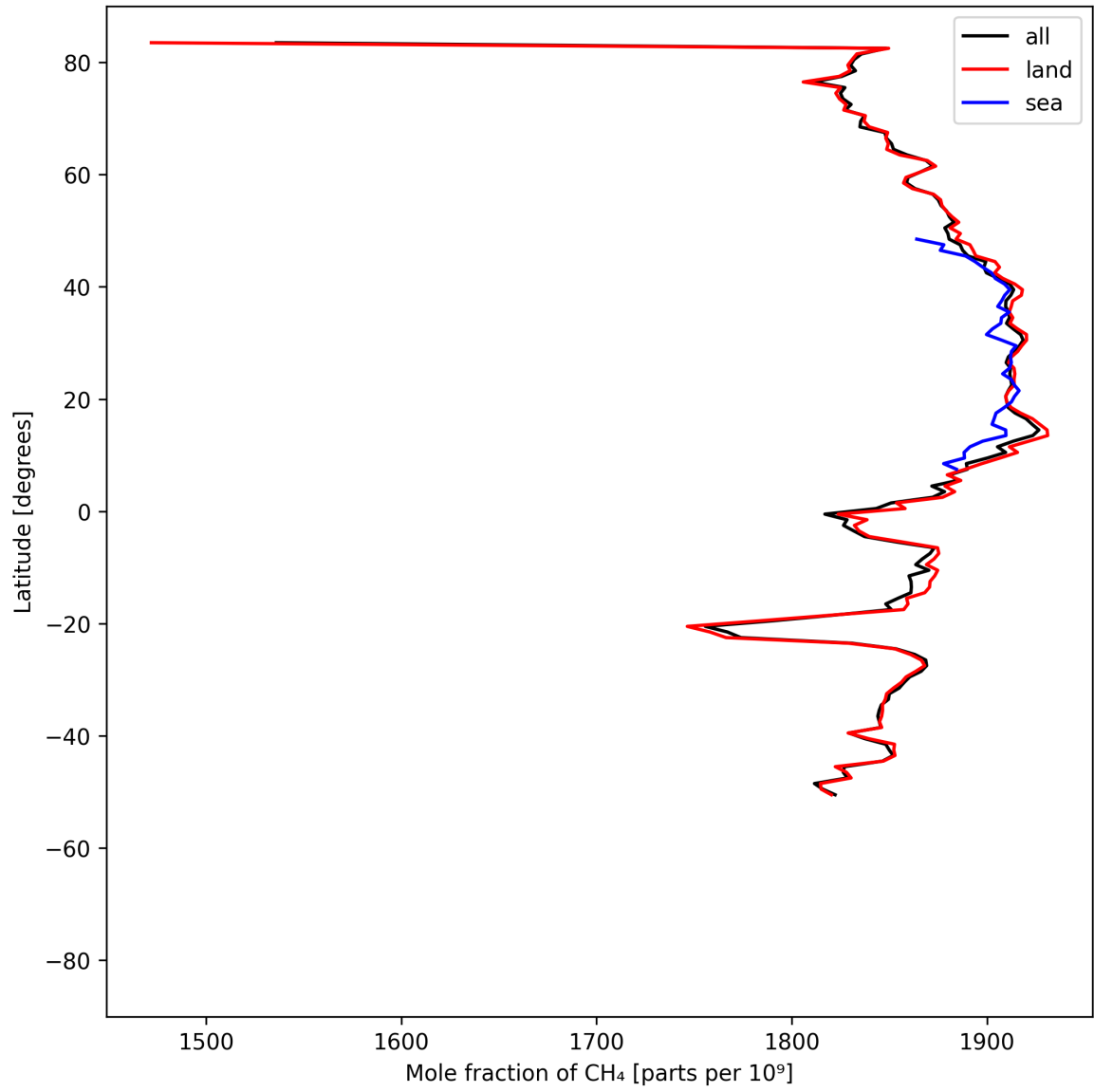
Figure 12: Zonal average of “Mole fraction of \text{CH}_4 ” for 2025-05-27 to 2025-05-29.
