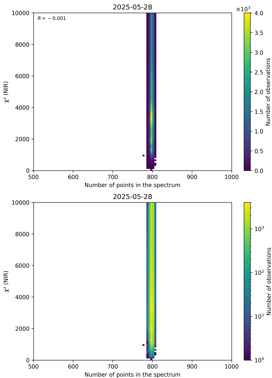
Figure 88: Scatter density plot of “Number of points in the spectrum” against “ \chi^2 (NIR)” for 2025-05-27 to 2025-05-29.
