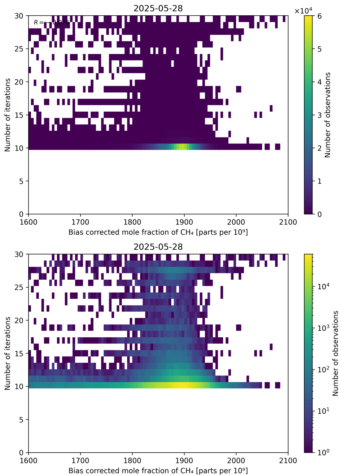
Figure 67: Scatter density plot of “Bias corrected mole fraction of \text{CH}_4 ” against “Number of iterations” for 2025-05-27 to 2025-05-29.
