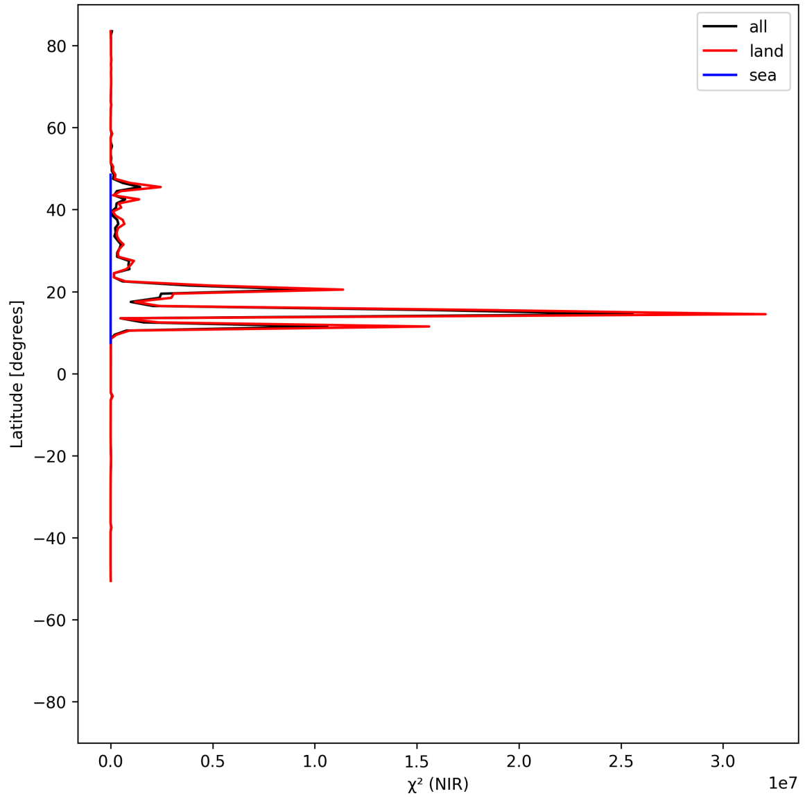
Figure 18: Zonal average of “ \chi^2 (NIR)” for 2025-05-27 to 2025-05-29.
