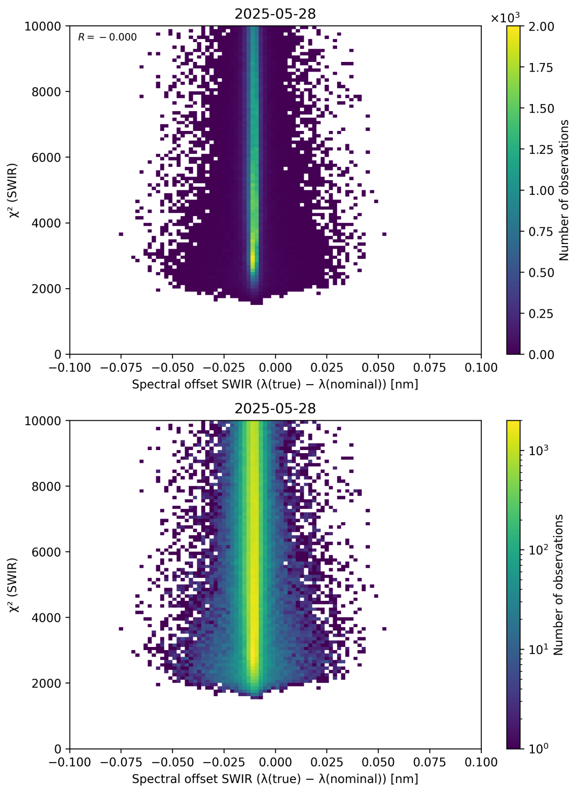
Figure 118: Scatter density plot of “Spectral offset SWIR ( \lambda_{\text{true}} - \lambda_{\text{nominal}} )” against “ \chi^2 (SWIR)” for 2025-05-27 to 2025-05-29.
