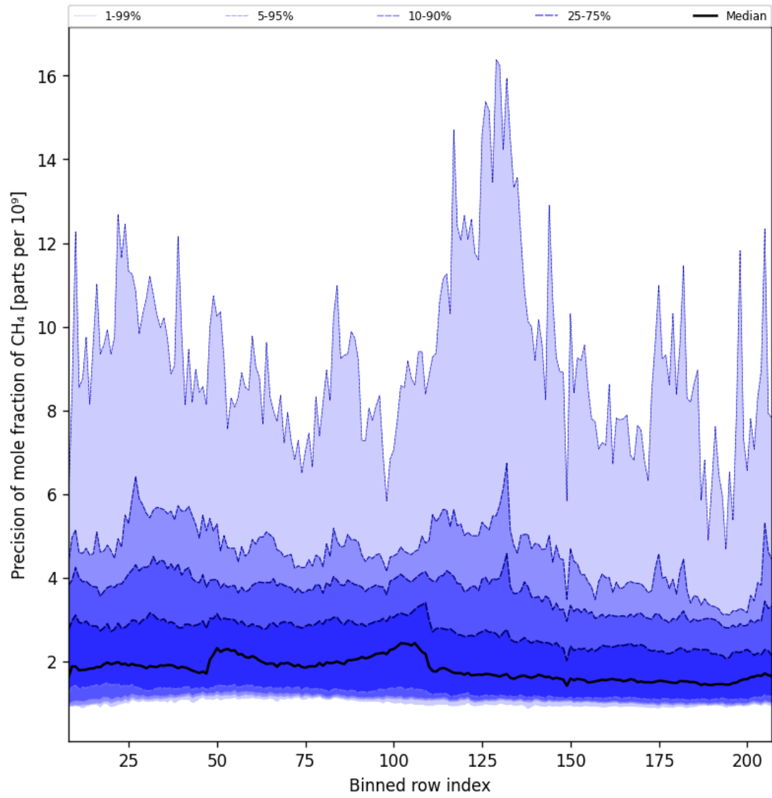
Figure 35: Along track statistics of “Precision of mole fraction of CH 4 ” for 2025-05-27 to 2025-05-29
