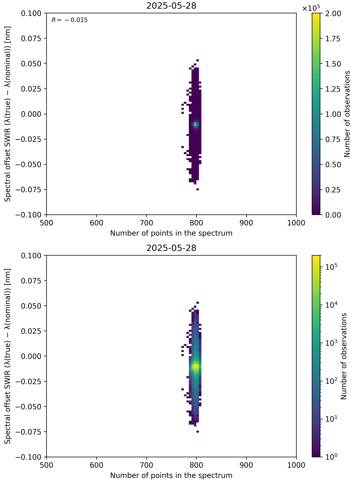
Figure 93: Scatter density plot of “Number of points in the spectrum” against “Spectral offset SWIR ( \lambda_{\text{true}} - \lambda_{\text{nominal}} )” for 2025-05-27 to 2025-05-29.
