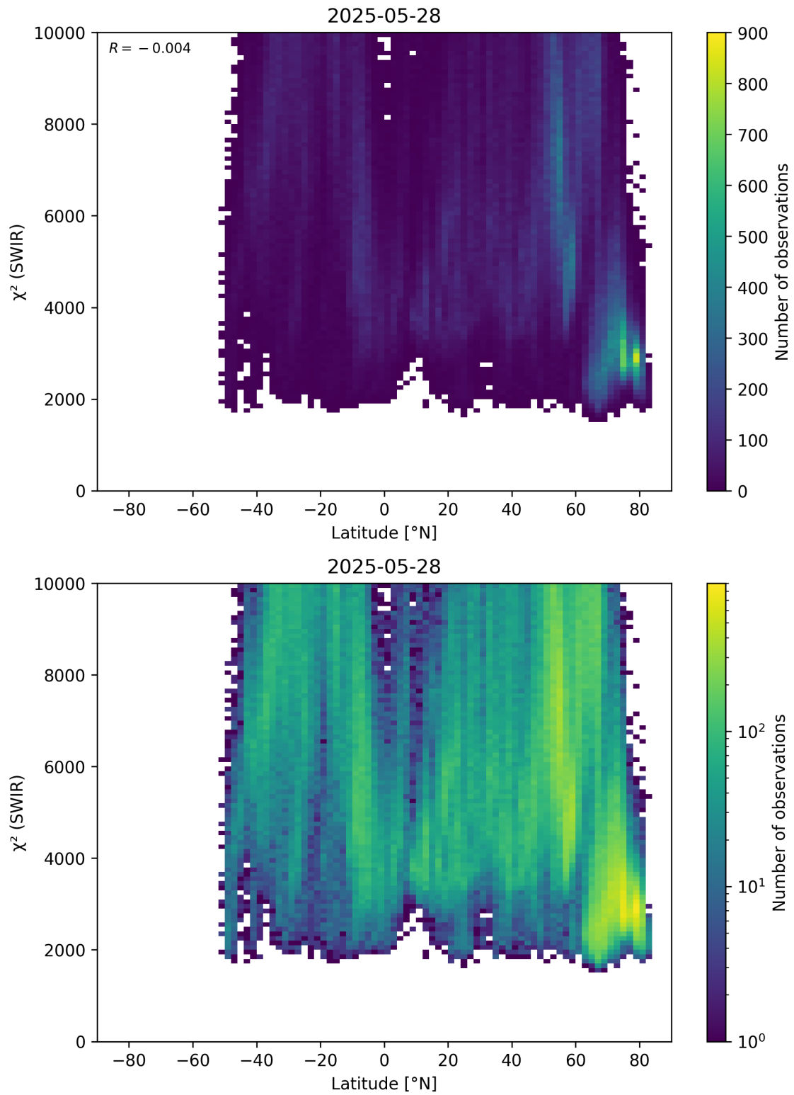
Figure 54: Scatter density plot of “Latitude” against “ \chi^2 (SWIR)” for 2025-05-27 to 2025-05-29.
