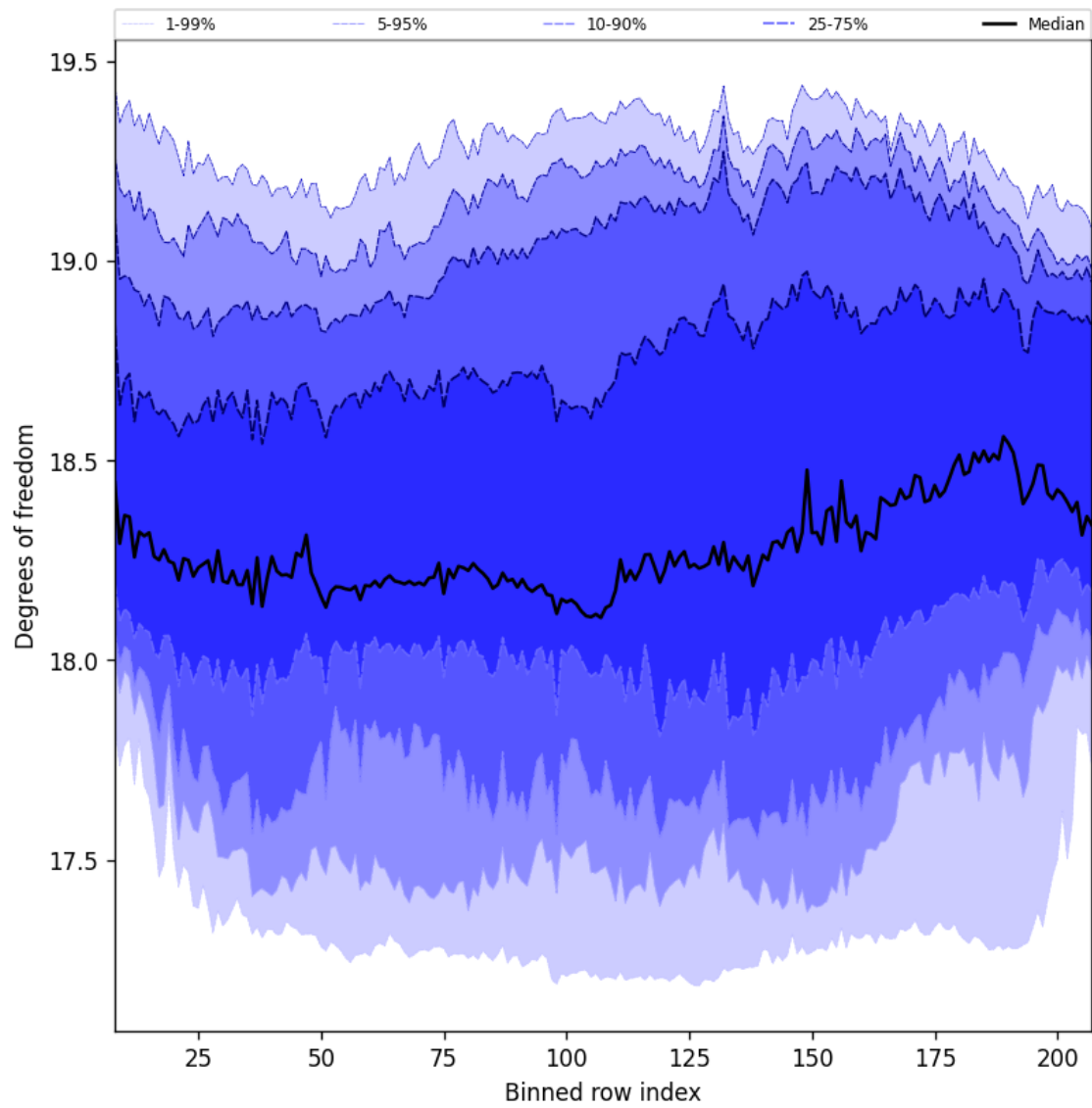
Figure 41: Along track statistics of “Degrees of freedom” for 2025-05-27 to 2025-05-29
