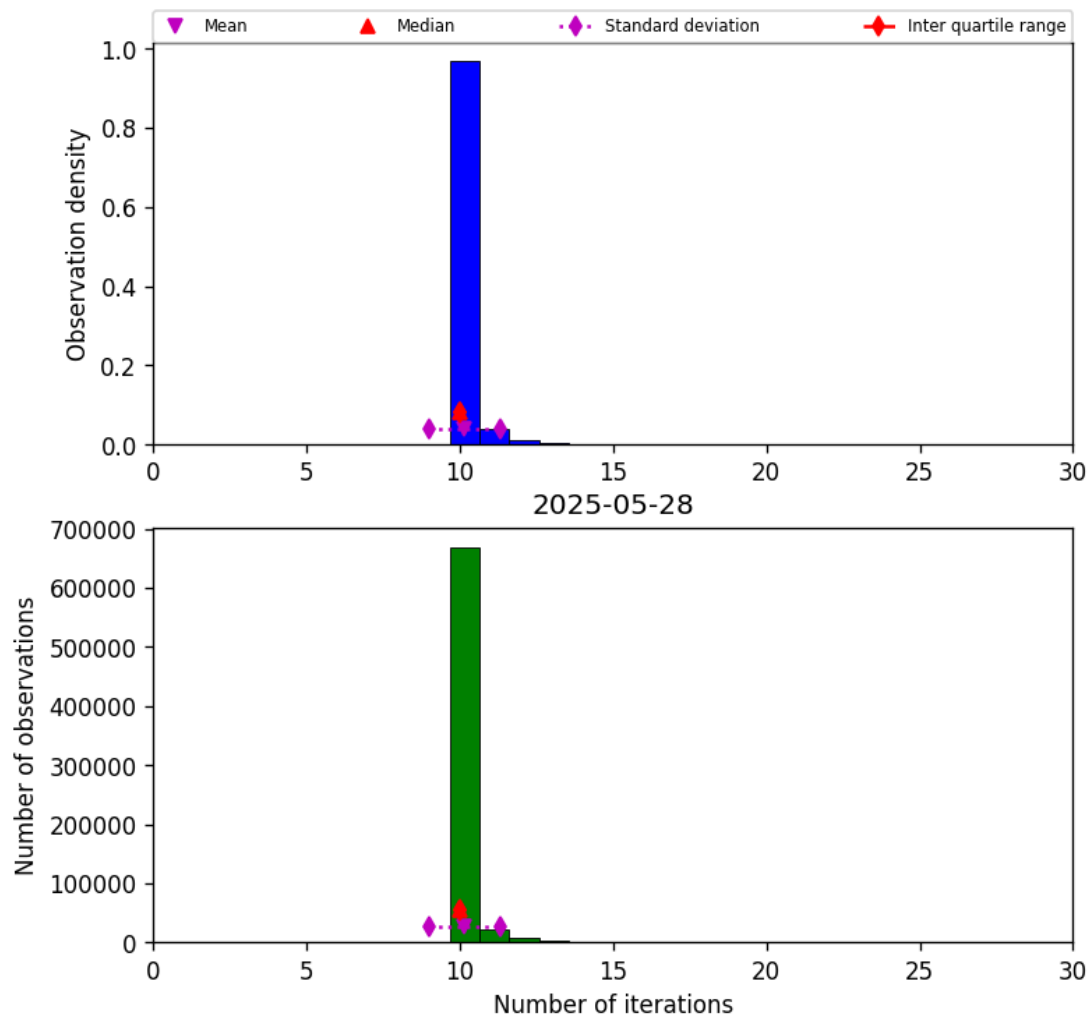
Figure 31: Histogram of “Number of iterations” for 2025-05-27 to 2025-05-29
