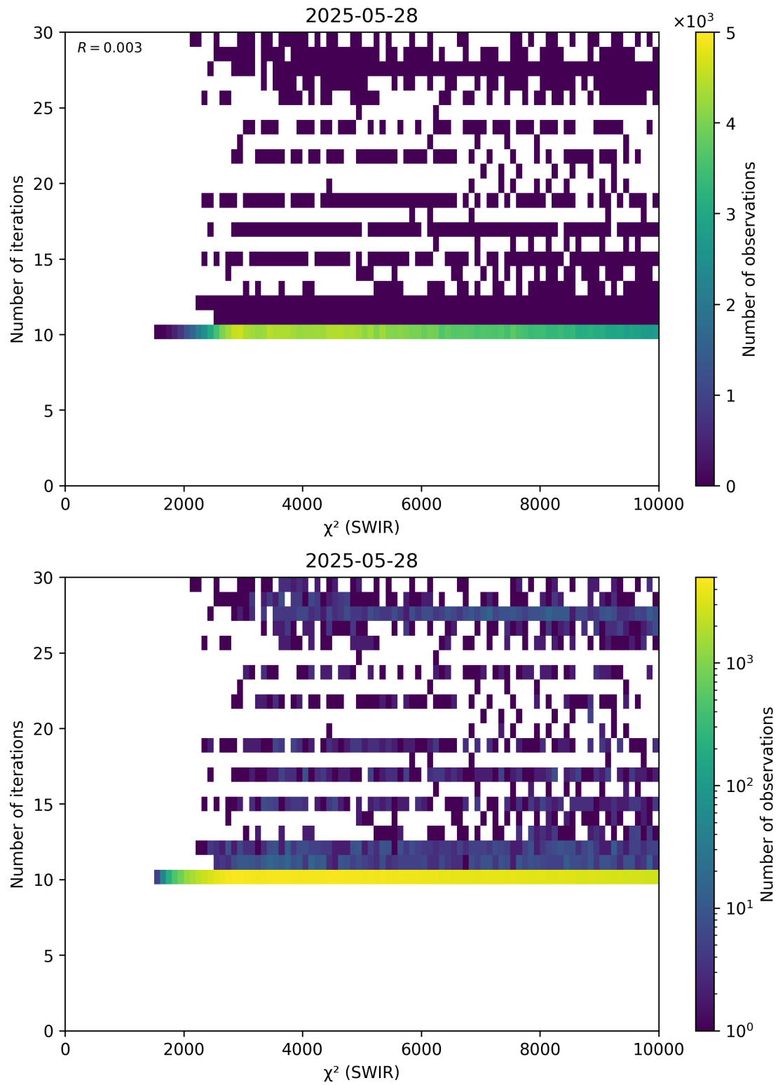
Figure 50: Scatter density plot of “ \chi^2 (SWIR)” against “Number of iterations” for 2025-05-27 to 2025-05-29.
