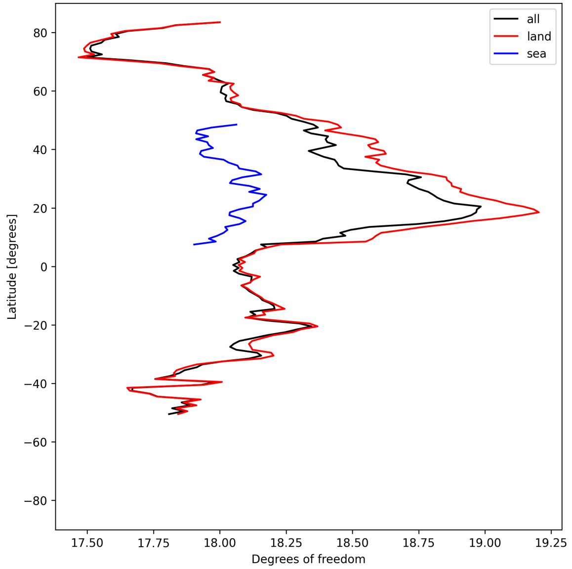
Figure 19: Zonal average of “Degrees of freedom” for 2025-05-27 to 2025-05-29.
