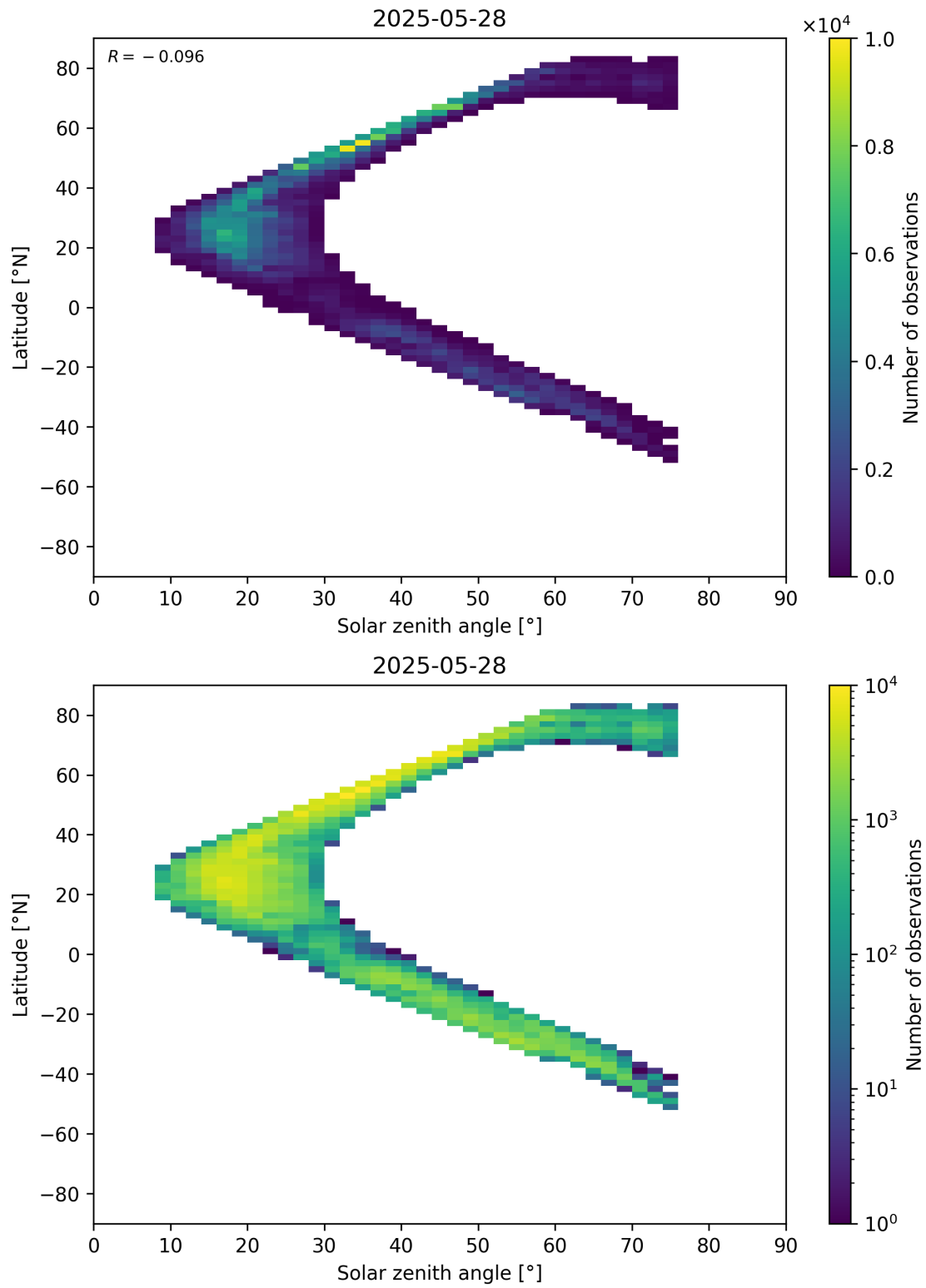
Figure 98: Scatter density plot of “Solar zenith angle” against “Latitude” for 2025-05-27 to 2025-05-29.
