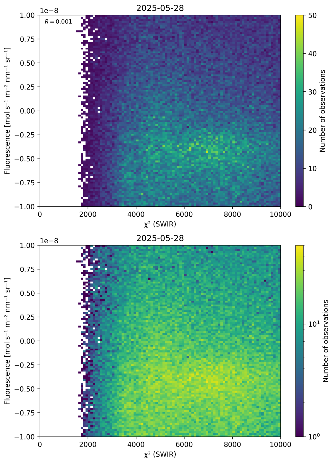
Figure 49: Scatter density plot of “ \chi^2 (SWIR)” against “Fluorescence” for 2025-05-27 to 2025-05-29.
