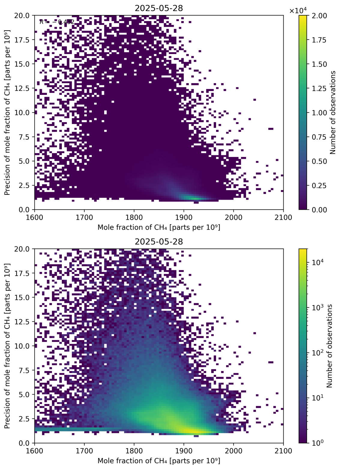
Figure 75: Scatter density plot of “Mole fraction of CH 4 ” against “Precision of mole fraction of CH 4 ” for 2025-05-27 to 2025-05-29.
