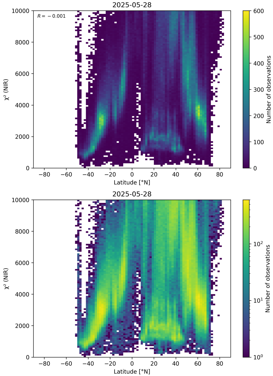
Figure 53: Scatter density plot of “Latitude” against “ \chi^2 (NIR)” for 2025-05-27 to 2025-05-29.
