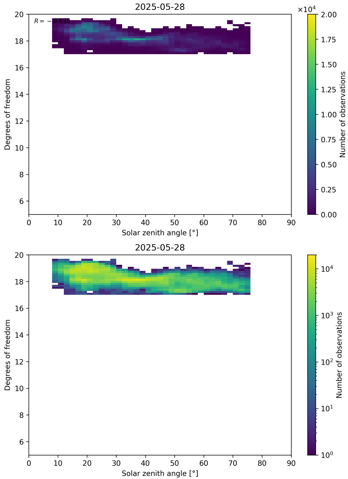
Figure 96: Scatter density plot of “Solar zenith angle” against “Degrees of freedom” for 2025-05-27 to 2025-05-29.
