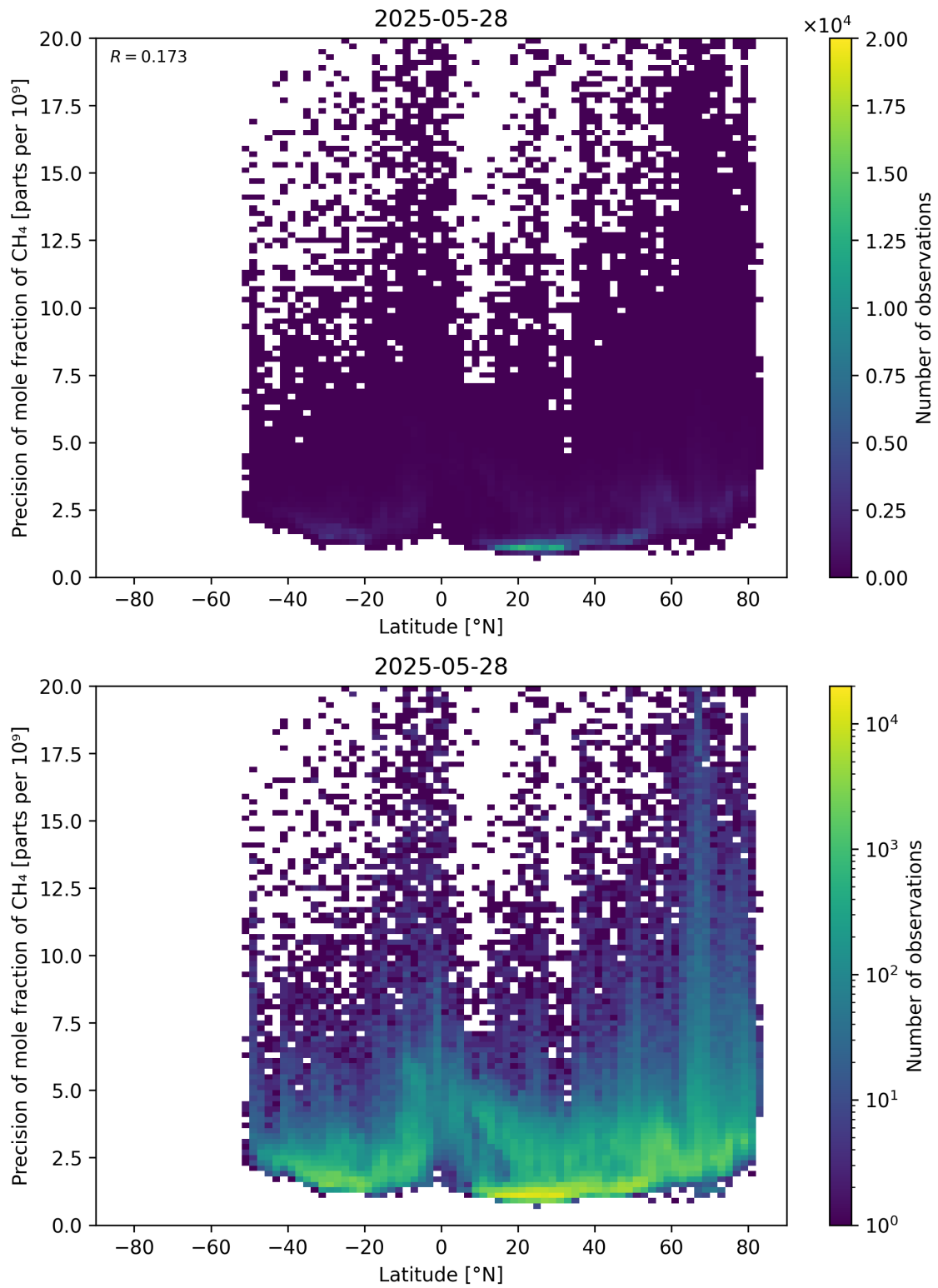
Figure 59: Scatter density plot of “Latitude” against “Precision of mole fraction of \text{CH}_4 ” for 2025-05-27 to 2025-05-29.
