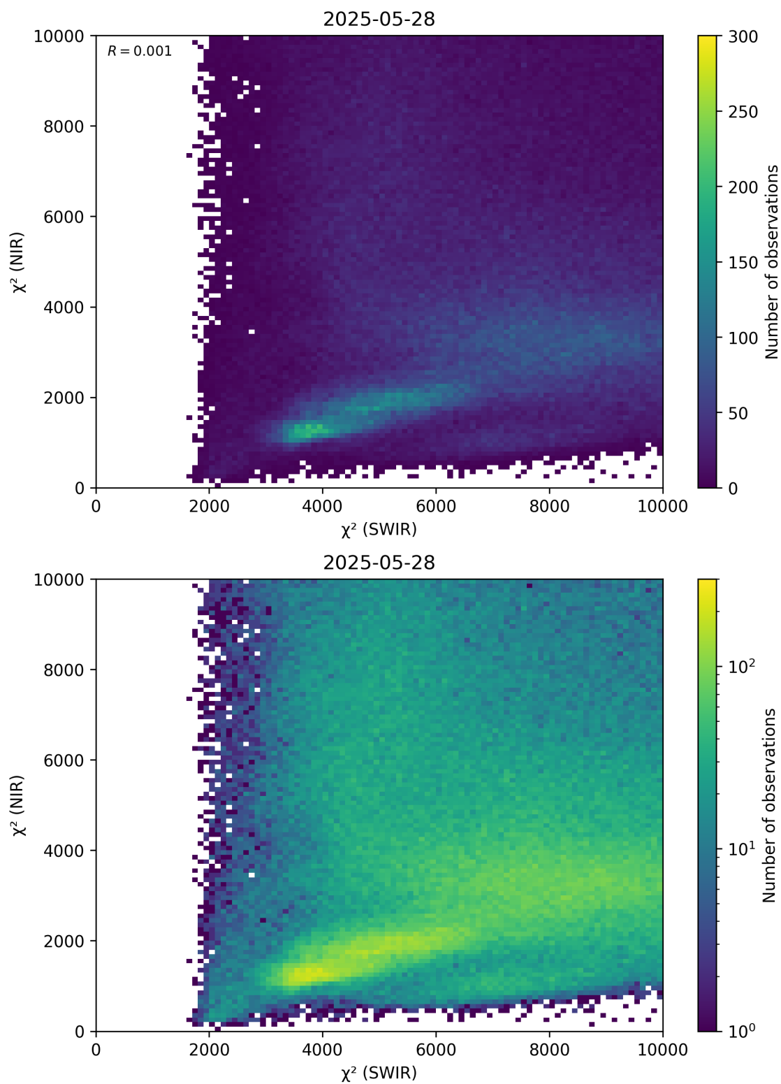
Figure 47: Scatter density plot of “ \chi^2 (SWIR)” against “ \chi^2 (NIR)” for 2025-05-27 to 2025-05-29.
