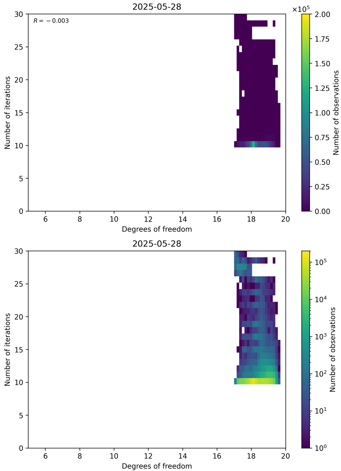
Figure 52: Scatter density plot of “Degrees of freedom” against “Number of iterations” for 2025-05-27 to 2025-05-29.
