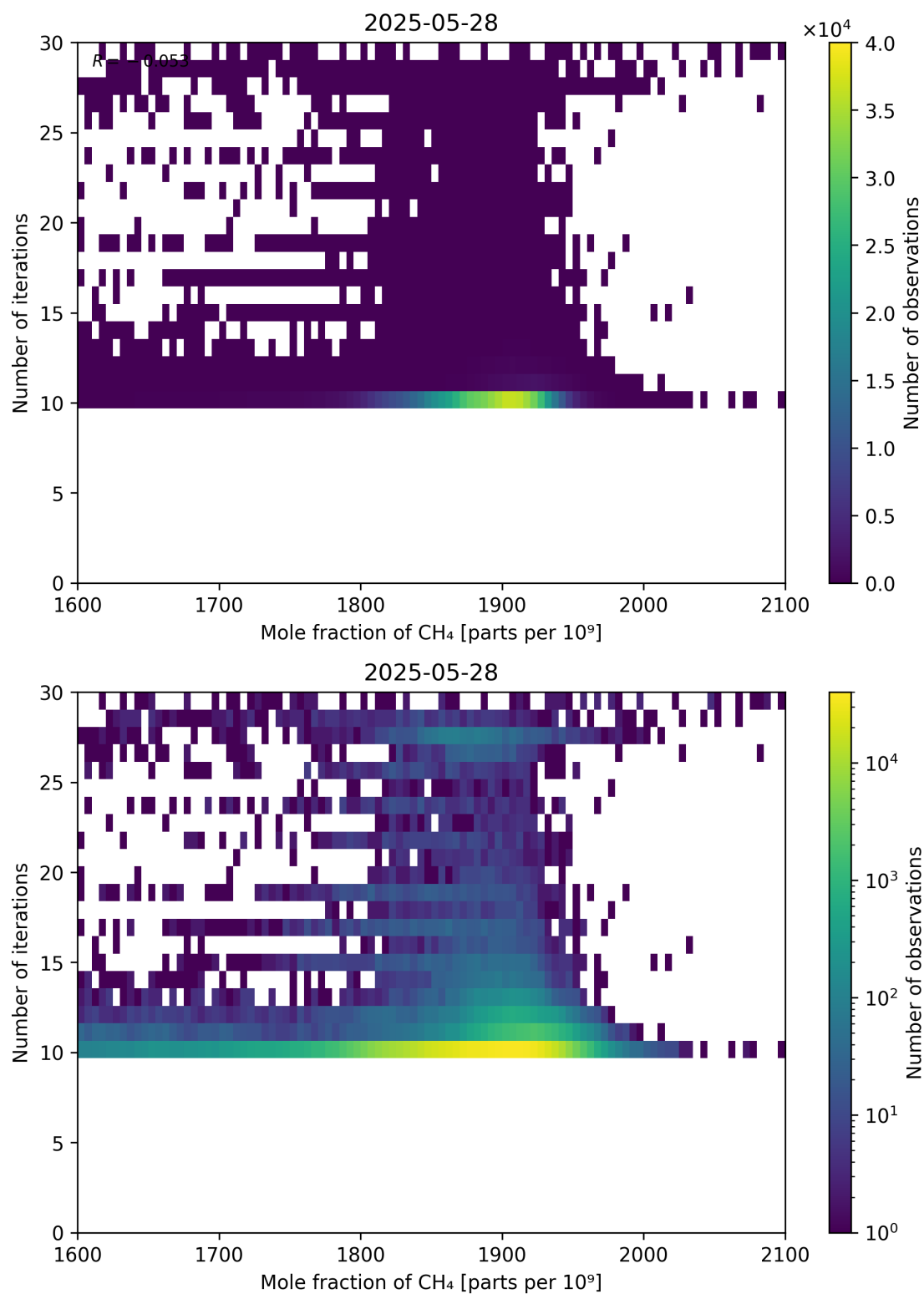
Figure 76: Scatter density plot of “Mole fraction of CH 4 ” against “Number of iterations” for 2025-05-27 to 2025-05-29.
