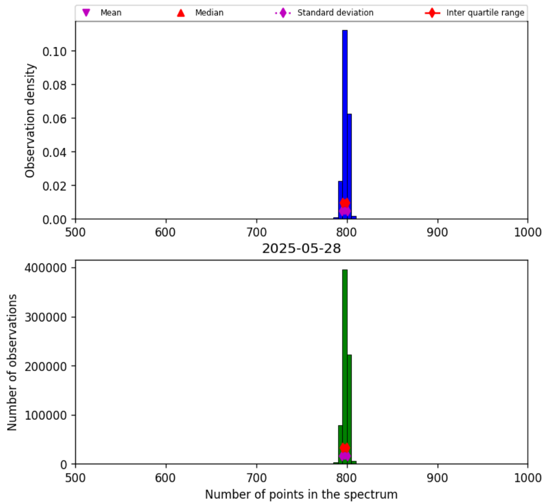
Figure 26: Histogram of “Number of points in the spectrum” for 2025-05-27 to 2025-05-29
