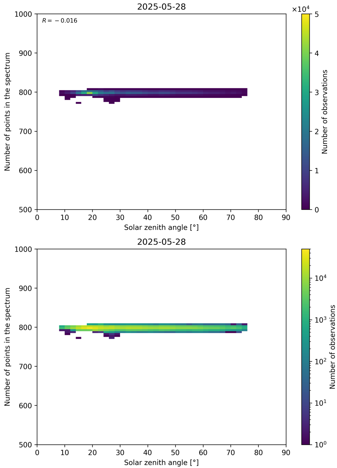
Figure 103: Scatter density plot of “Solar zenith angle” against “Number of points in the spectrum” for 2025-05-27 to 2025-05-29.
