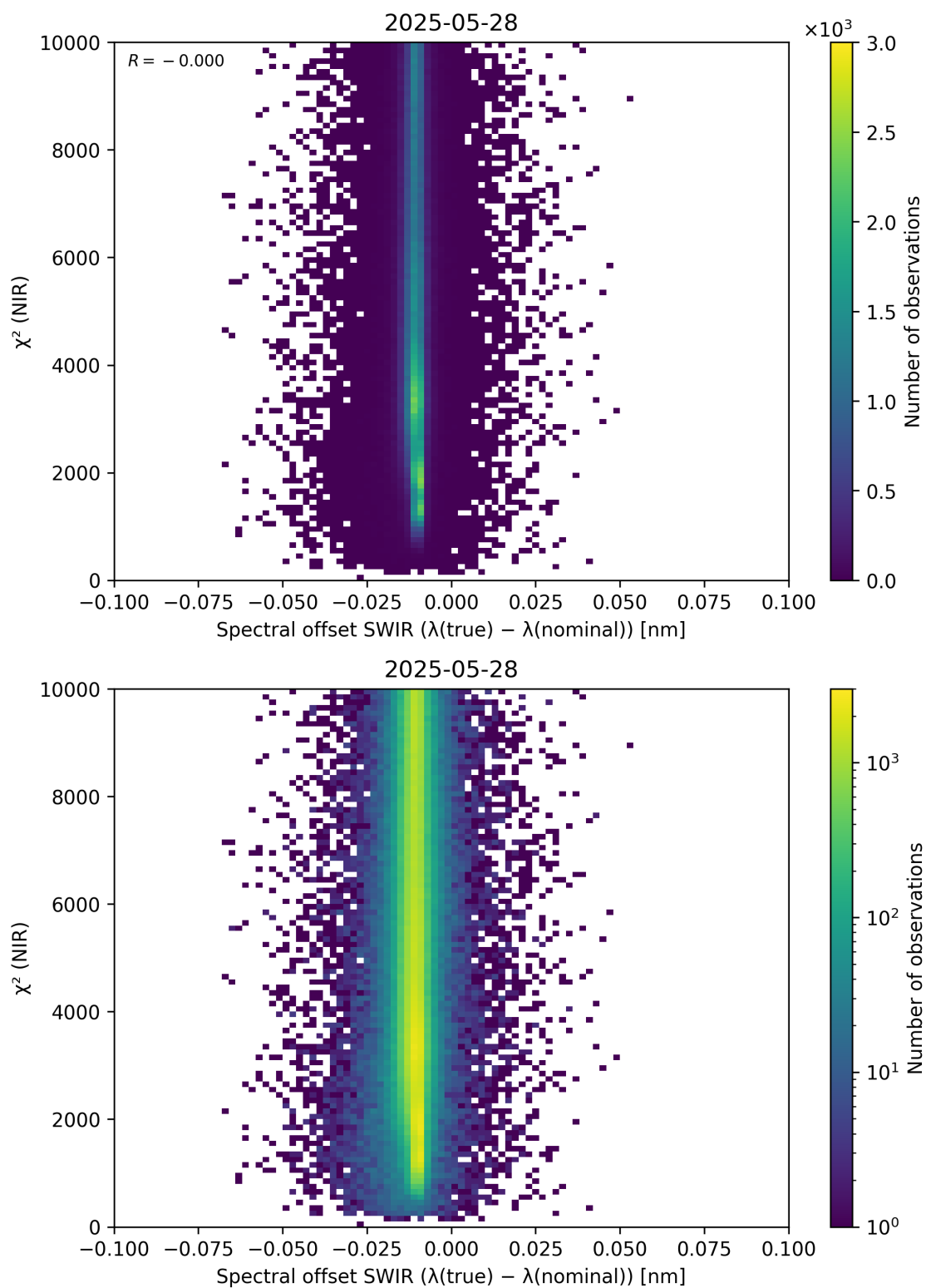
Figure 117: Scatter density plot of “Spectral offset SWIR ( \lambda_{\text{true}} - \lambda_{\text{nominal}} )” against “ \chi^2 (NIR)” for 2025-05-27 to 2025-05-29.
