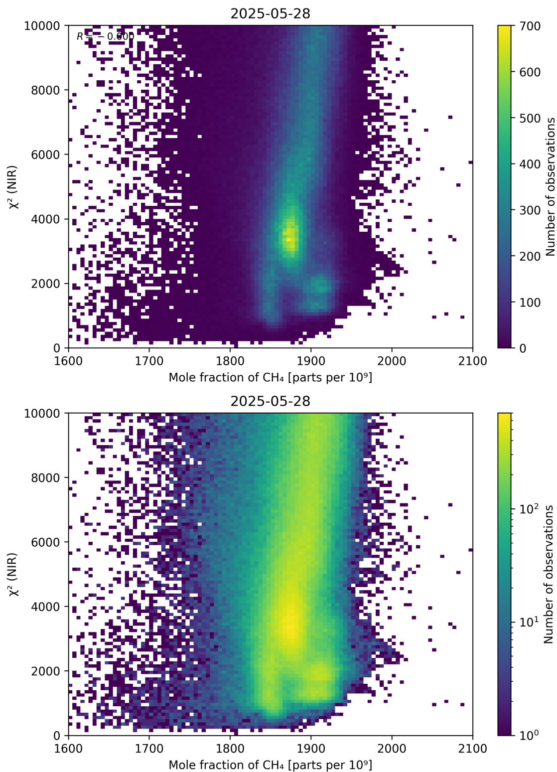
Figure 70: Scatter density plot of “Mole fraction of \text{CH}_4 ” against “ \chi^2 (NIR)” for 2025-05-27 to 2025-05-29.
