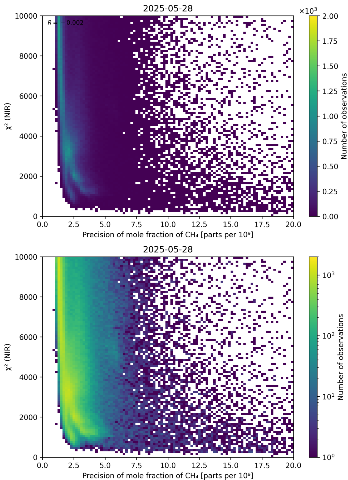
Figure 78: Scatter density plot of “Precision of mole fraction of CH 4 ” against “ \chi^2 (NIR)” for 2025-05-27 to 2025-05-29.
