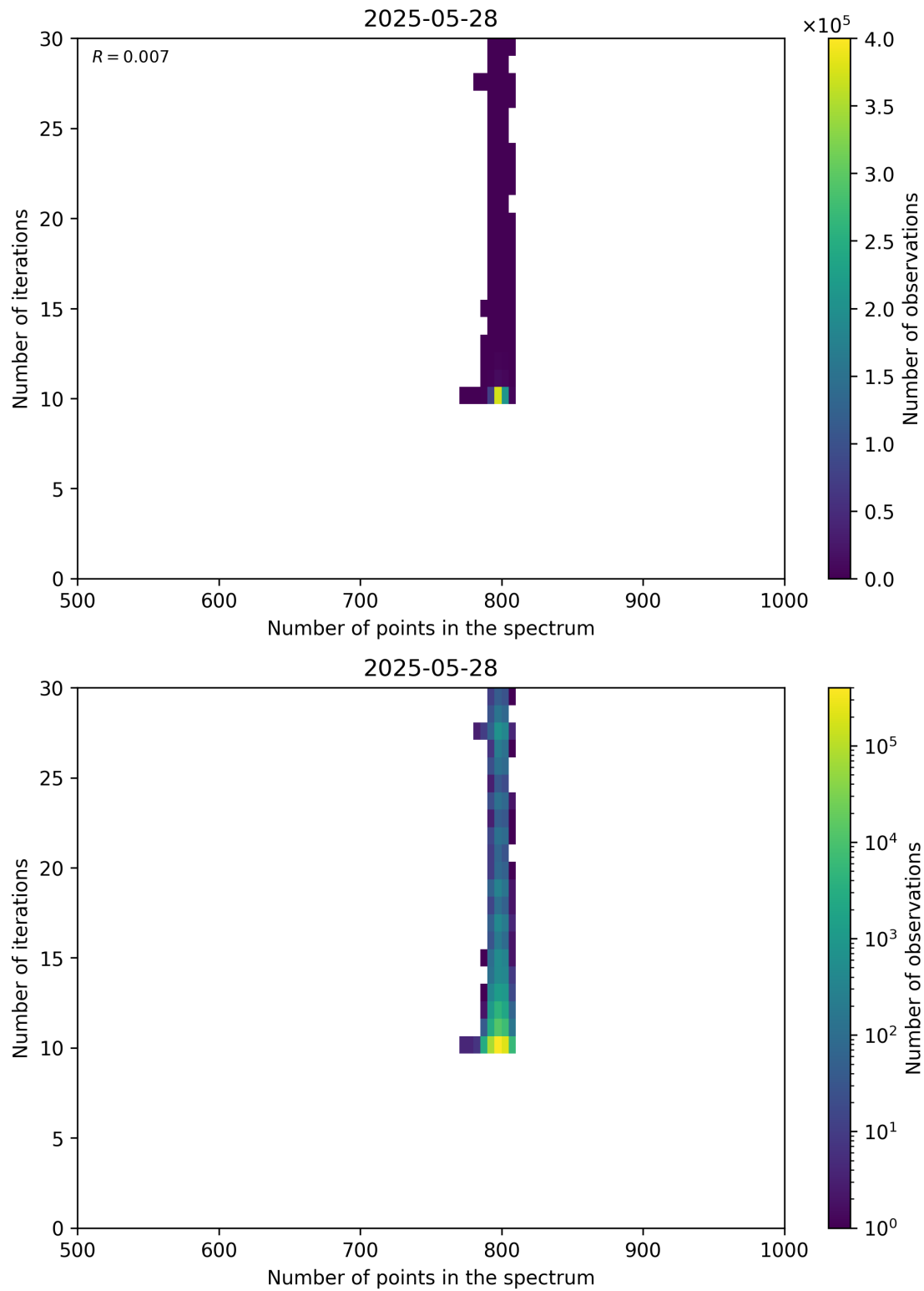
Figure 92: Scatter density plot of “Number of points in the spectrum” against “Number of iterations” for 2025-05-27 to 2025-05-29.
