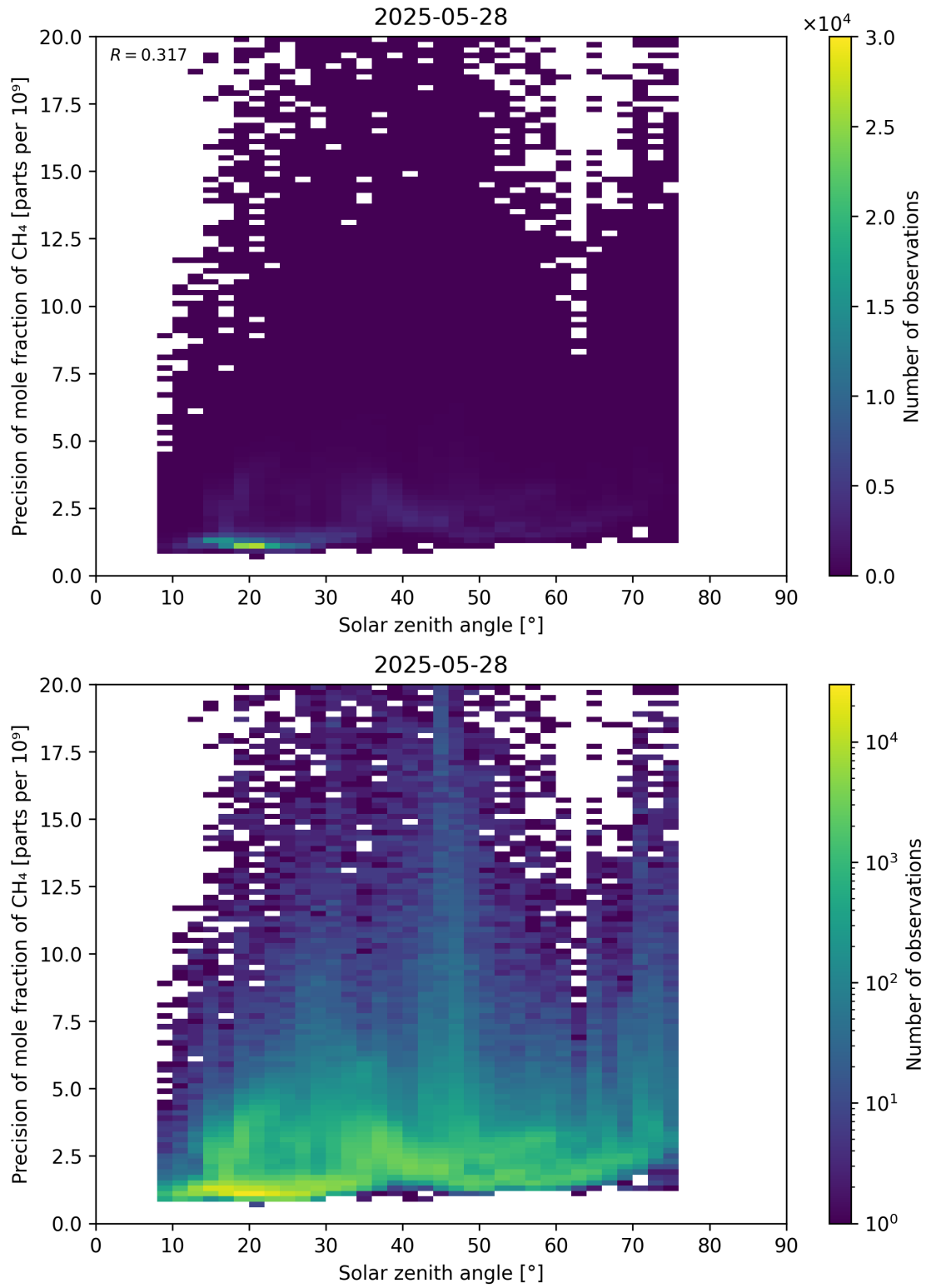
Figure 101: Scatter density plot of “Solar zenith angle” against “Precision of mole fraction of \text{CH}_4 ” for 2025-05-27 to 2025-05-29.
