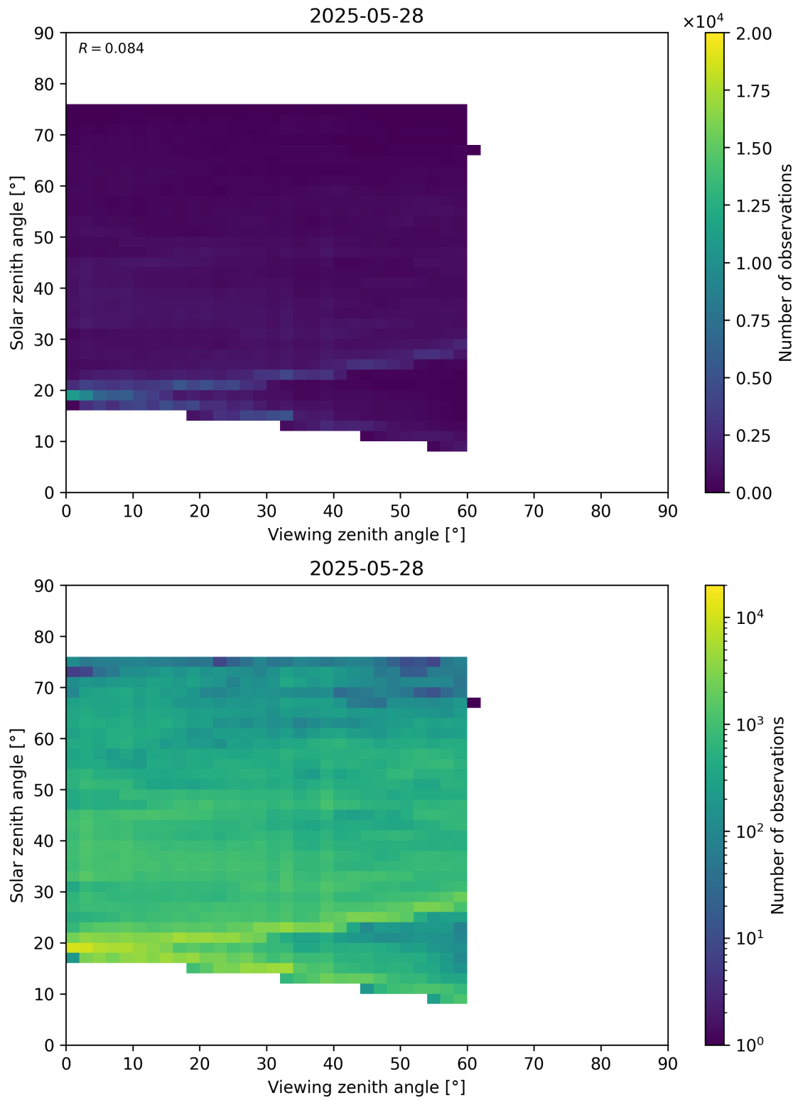
Figure 115: Scatter density plot of “Viewing zenith angle” against “Solar zenith angle” for 2025-05-27 to 2025-05-29.
