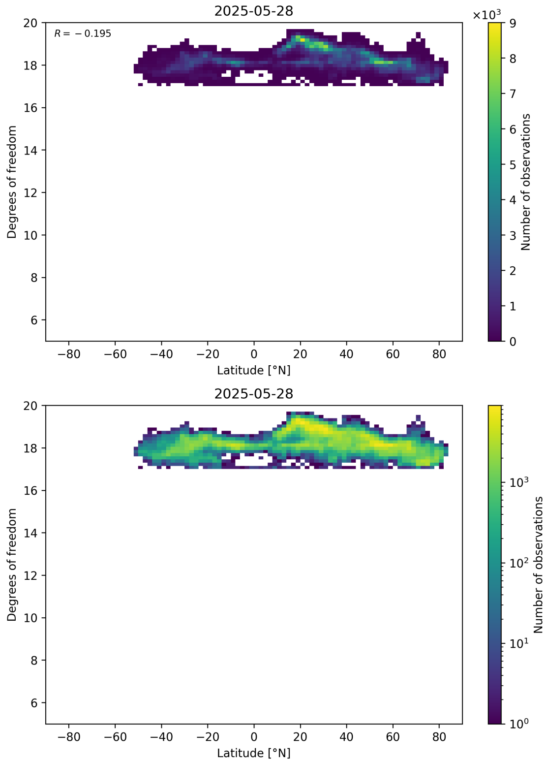
Figure 55: Scatter density plot of “Latitude” against “Degrees of freedom” for 2025-05-27 to 2025-05-29.
