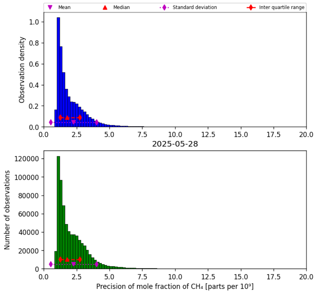
Figure 24: Histogram of “Precision of mole fraction of CH 4 ” for 2025-05-27 to 2025-05-29
