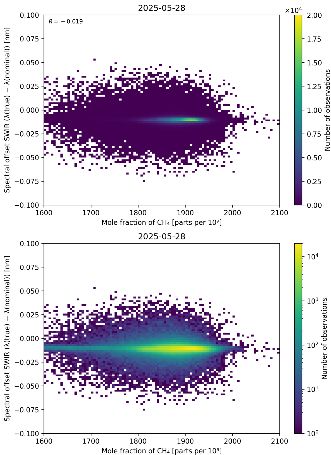
Figure 86: Scatter density plot of “Mole fraction of CH 4 ” against “Spectral offset SWIR ( \lambda_{\text{true}} - \lambda_{\text{nominal}} )” for 2025-05-27 to 2025-05-29.
