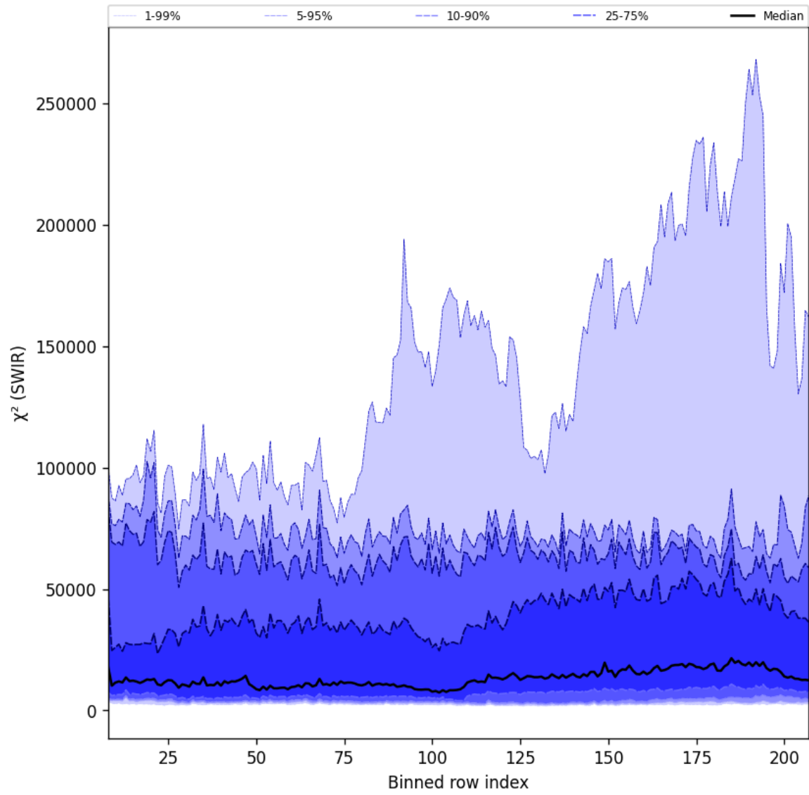
Figure 39: Along track statistics of “ \chi^2 (SWIR)” for 2025-05-27 to 2025-05-29
