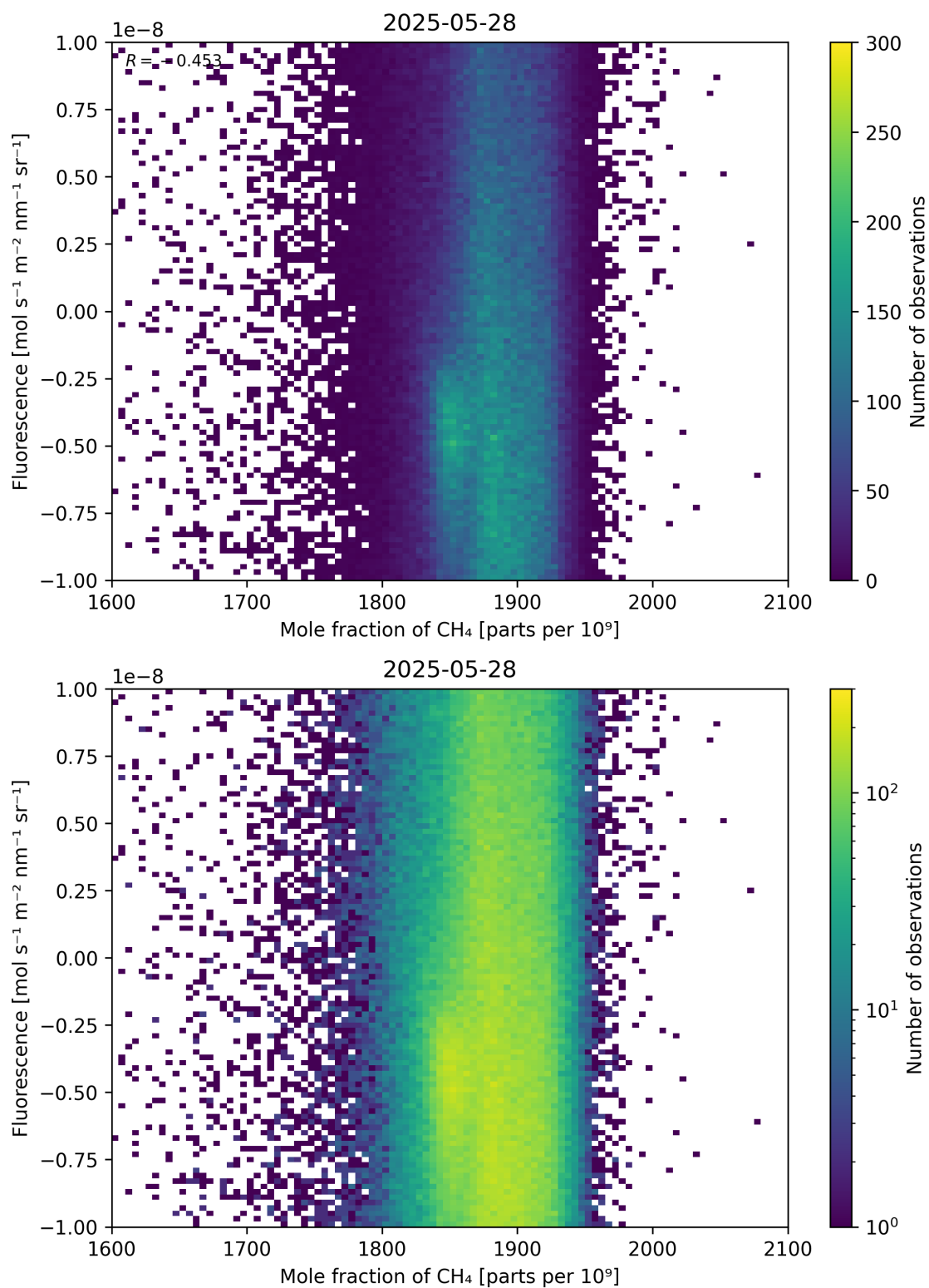
Figure 73: Scatter density plot of “Mole fraction of CH 4 ” against “Fluorescence” for 2025-05-27 to 2025-05-29.
