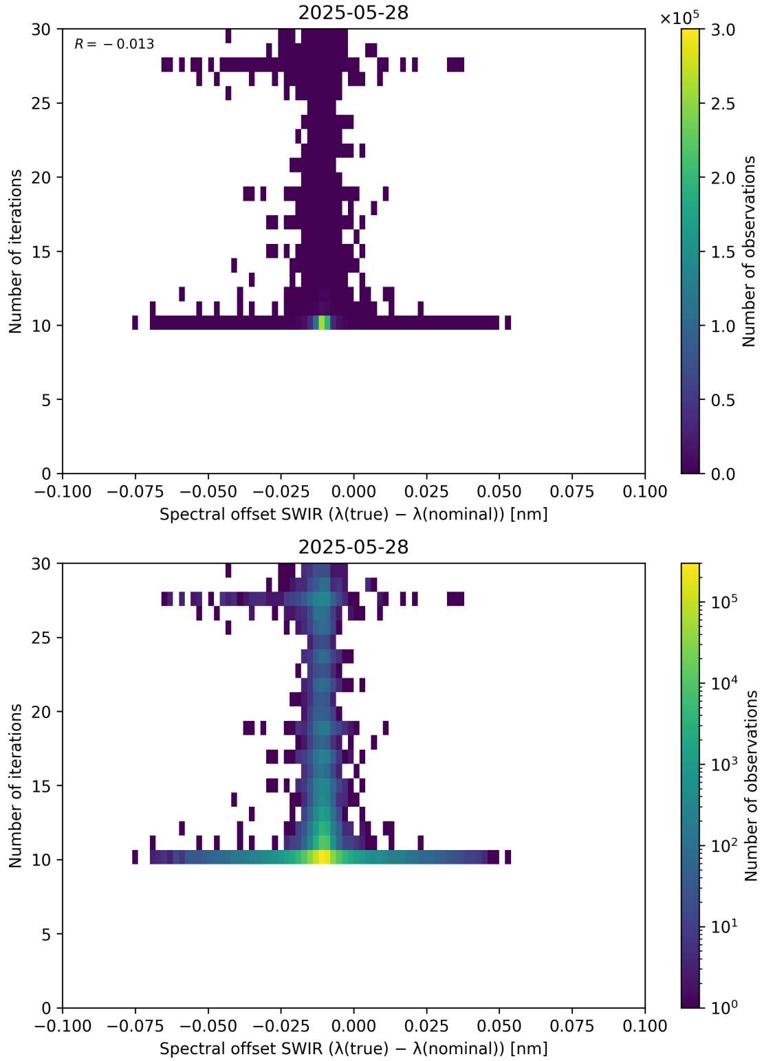
Figure 121: Scatter density plot of “Spectral offset SWIR ( \lambda_{\text{true}} - \lambda_{\text{nominal}} )” against “Number of iterations” for 2025-05-27 to 2025-05-29.
