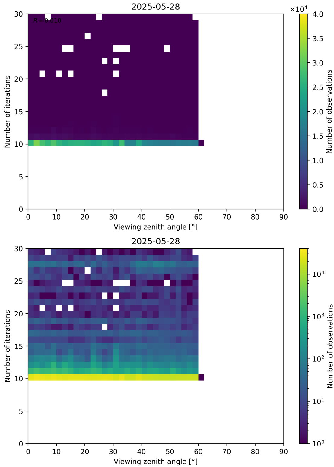
Figure 113: Scatter density plot of “Viewing zenith angle” against “Number of iterations” for 2025-05-27 to 2025-05-29.
