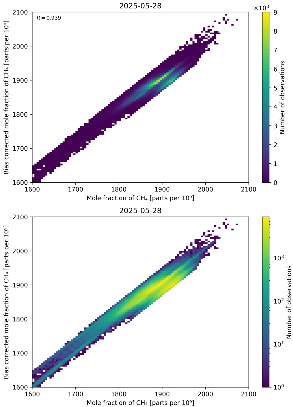
Figure 74: Scatter density plot of “Mole fraction of CH 4 ” against “Bias corrected mole fraction of CH 4 ” for 2025-05-27 to 2025-05-29.
