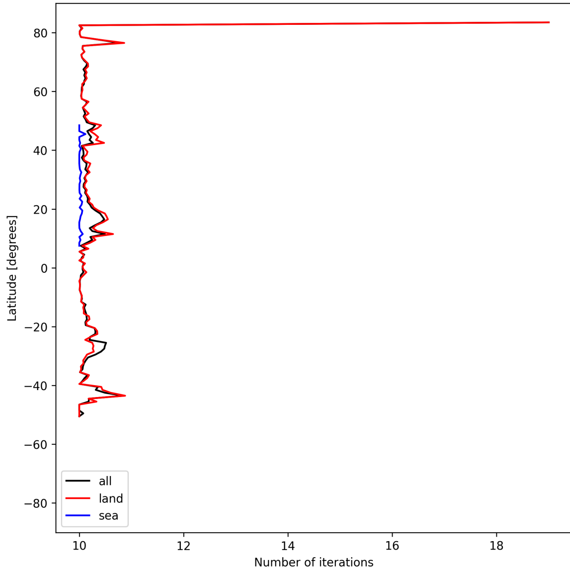
Figure 20: Zonal average of “Number of iterations” for 2025-05-27 to 2025-05-29.
