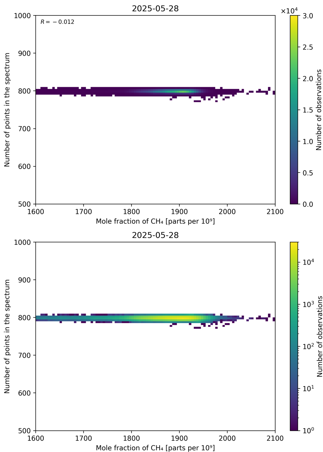
Figure 77: Scatter density plot of “Mole fraction of CH 4 ” against “Number of points in the spectrum” for 2025-05-27 to 2025-05-29.
