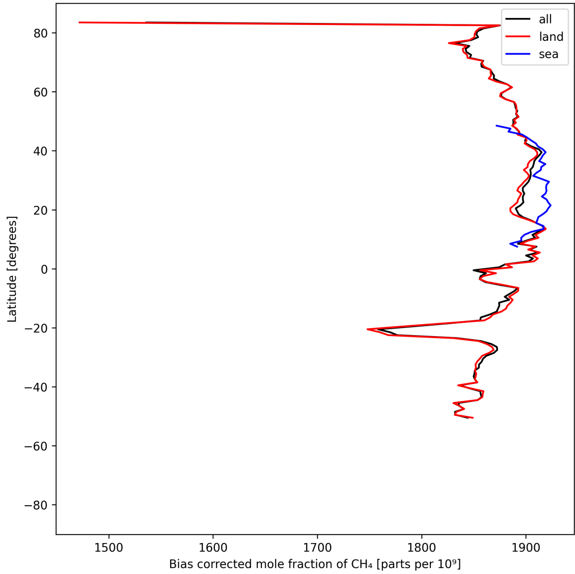
Figure 14: Zonal average of “Bias corrected mole fraction of \text{CH}_4 ” for 2025-05-27 to 2025-05-29.
