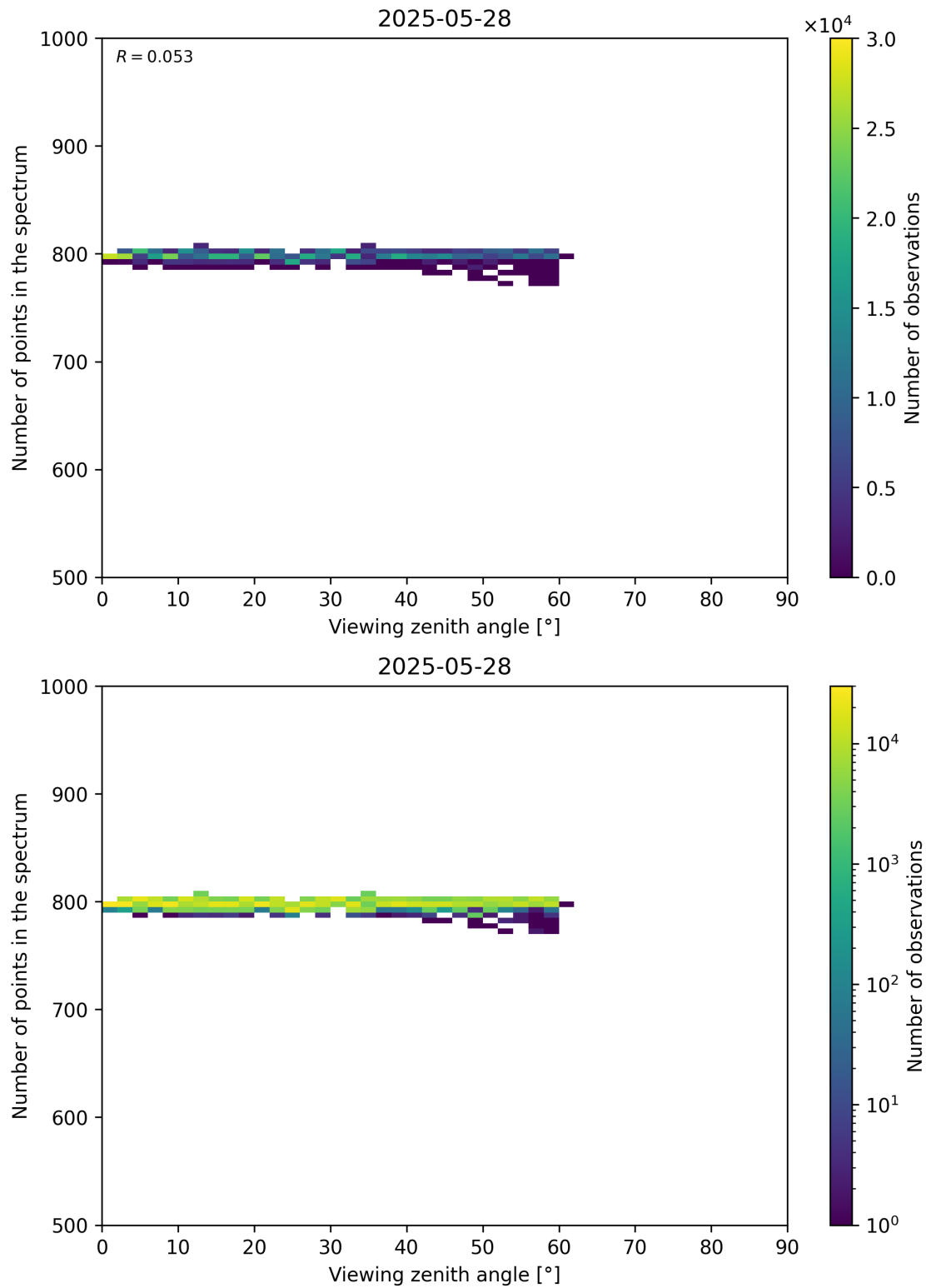
Figure 114: Scatter density plot of “Viewing zenith angle” against “Number of points in the spectrum” for 2025-05-27 to 2025-05-29.
