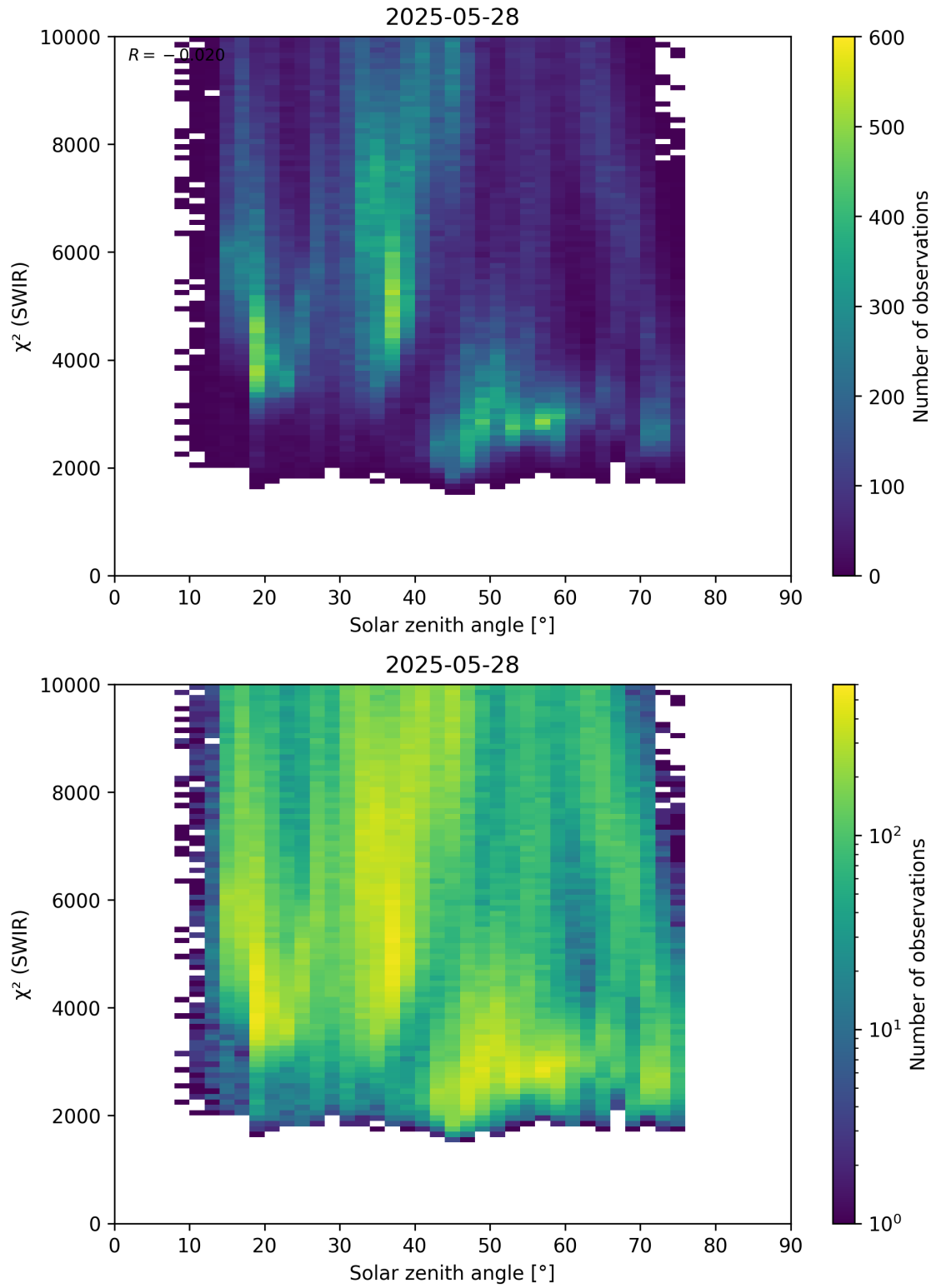
Figure 95: Scatter density plot of “Solar zenith angle” against “ \chi^2 (SWIR)” for 2025-05-27 to 2025-05-29.
