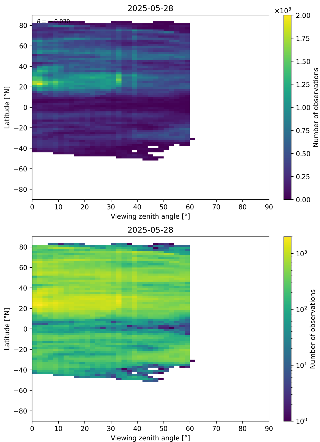
Figure 109: Scatter density plot of “Viewing zenith angle” against “Latitude” for 2025-05-27 to 2025-05-29.
