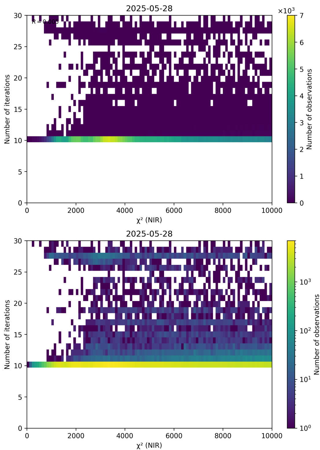
Figure 46: Scatter density plot of “ \chi^2 (NIR)” against “Number of iterations” for 2025-05-27 to 2025-05-29.
