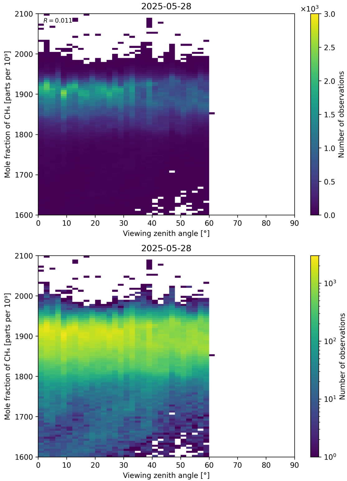
Figure 110: Scatter density plot of “Viewing zenith angle” against “Mole fraction of \text{CH}_4 ” for 2025-05-27 to 2025-05-29.
