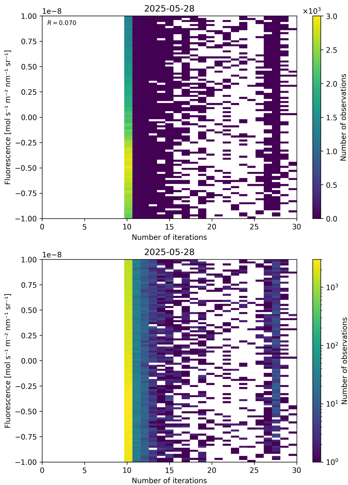
Figure 87: Scatter density plot of “Number of iterations” against “Fluorescence” for 2025-05-27 to 2025-05-29.
