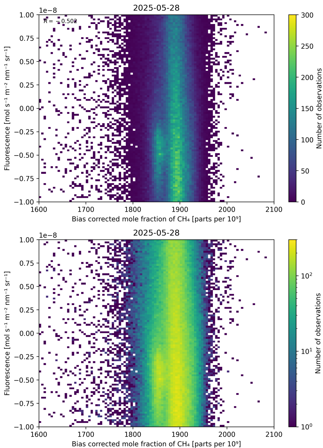
Figure 66: Scatter density plot of “Bias corrected mole fraction of \text{CH}_4 ” against “Fluorescence” for 2025-05-27 to 2025-05-29.
