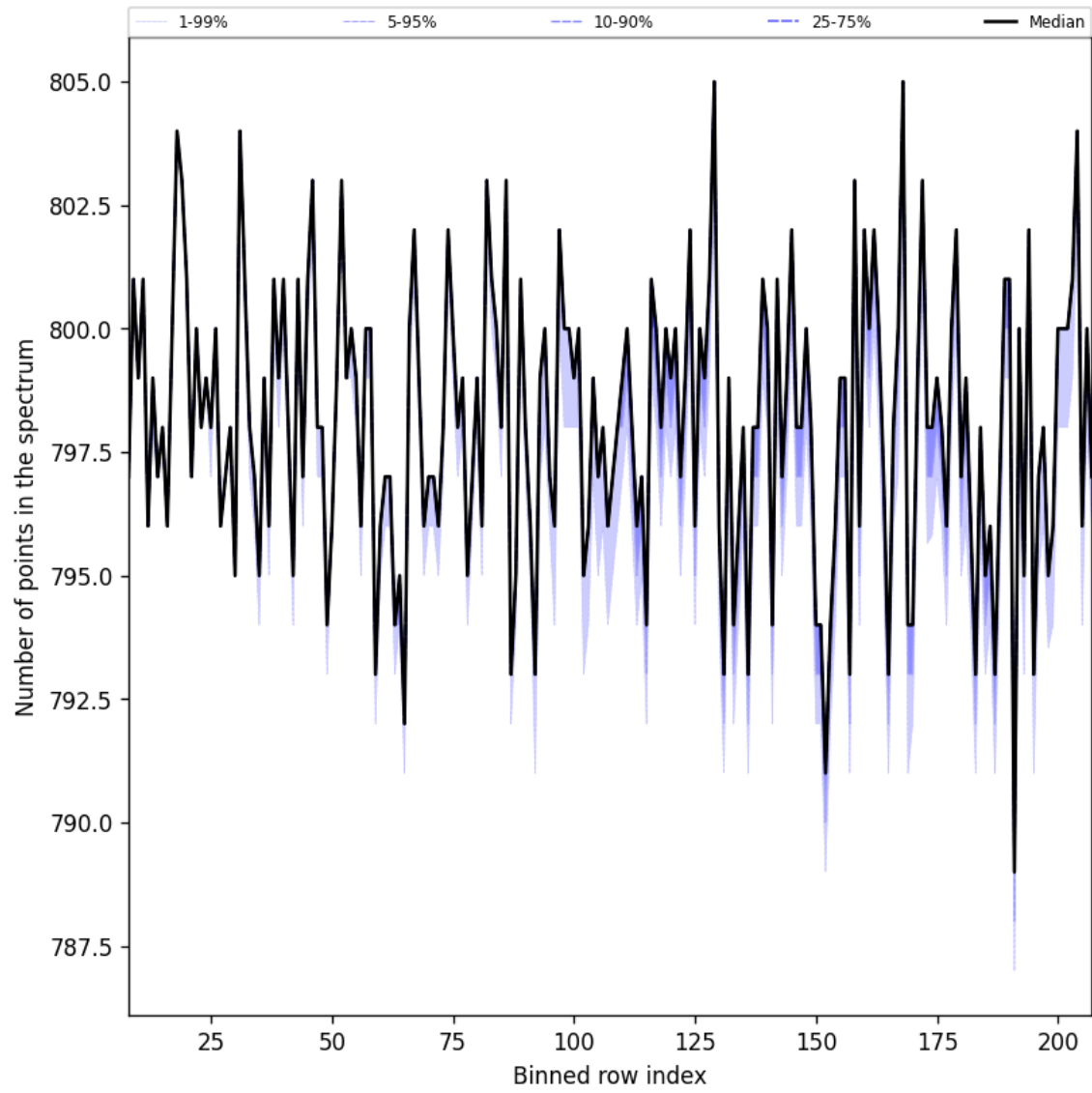
Figure 37: Along track statistics of “Number of points in the spectrum” for 2025-05-27 to 2025-05-29
