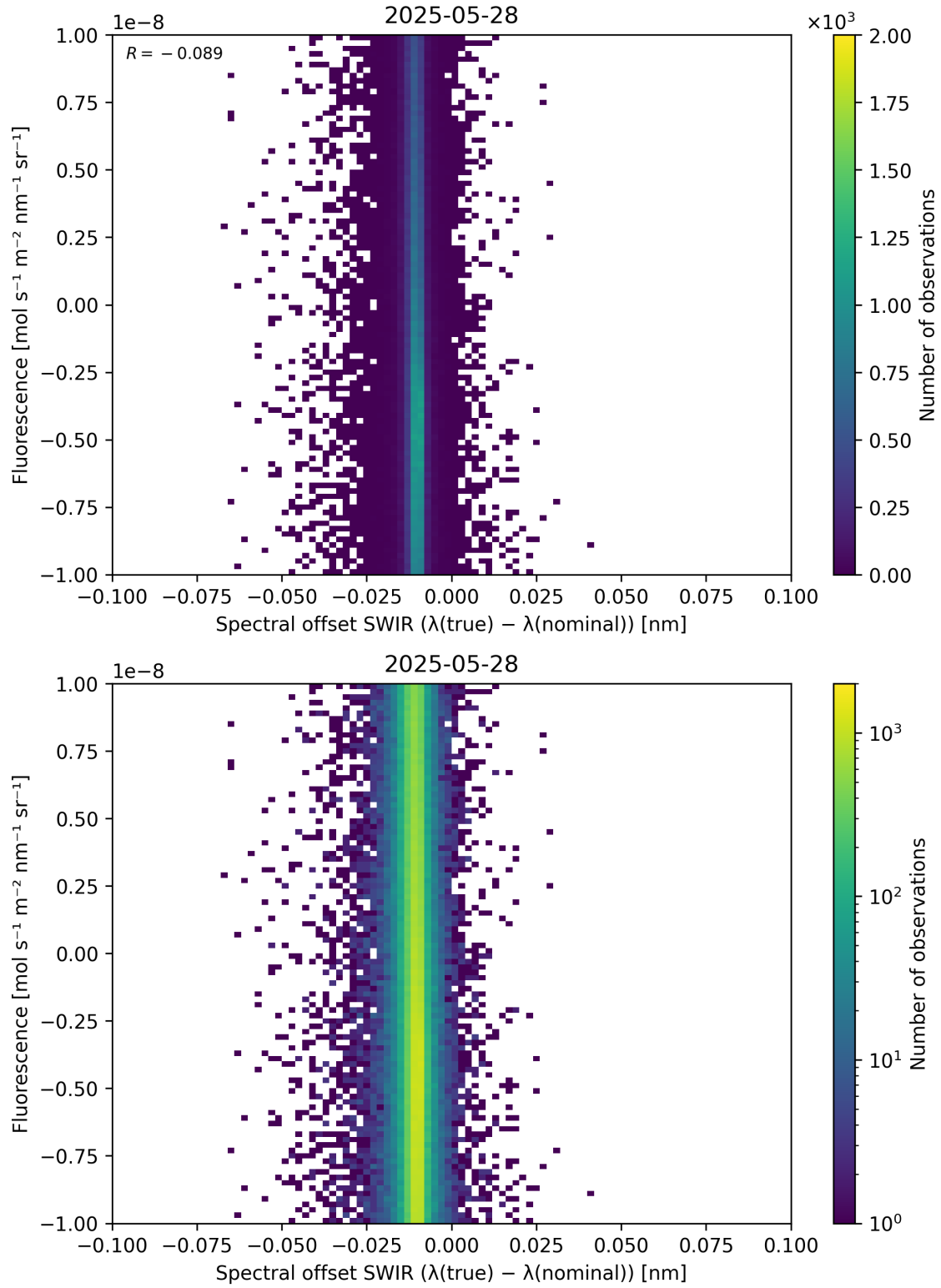
Figure 120: Scatter density plot of “Spectral offset SWIR ( \lambda_{\text{true}} - \lambda_{\text{nominal}} )” against “Fluorescence” for 2025-05-27 to 2025-05-29.
