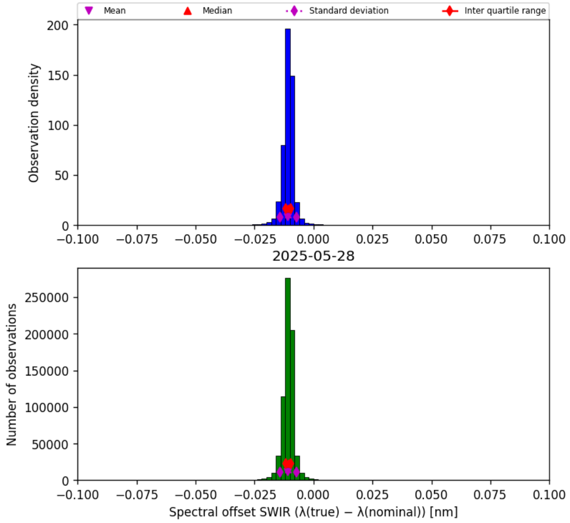
Figure 27: Histogram of “Spectral offset SWIR ( \lambda_{\text{true}} - \lambda_{\text{nominal}} )” for 2025-05-27 to 2025-05-29
