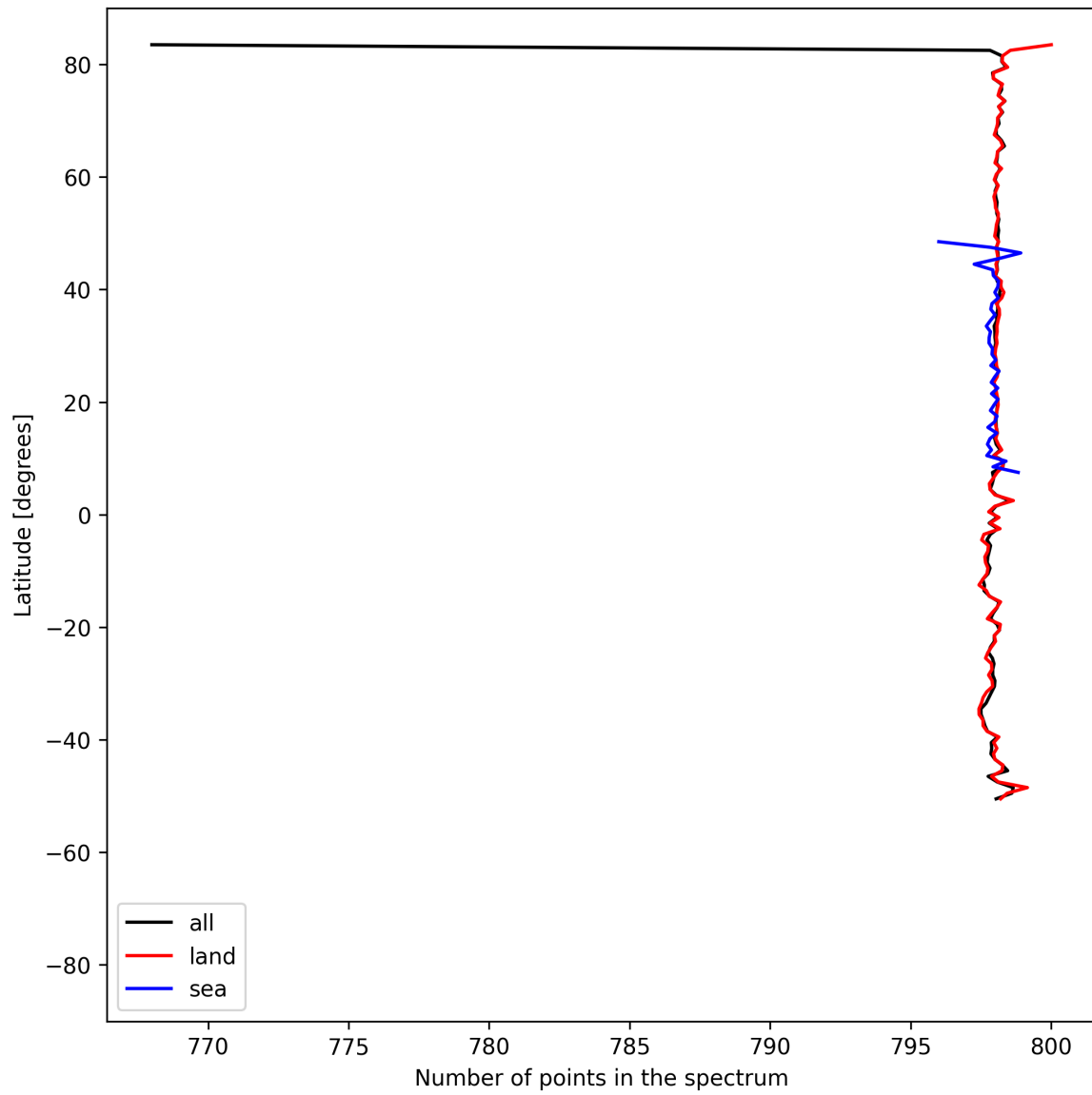
Figure 15: Zonal average of “Number of points in the spectrum” for 2025-05-27 to 2025-05-29.
