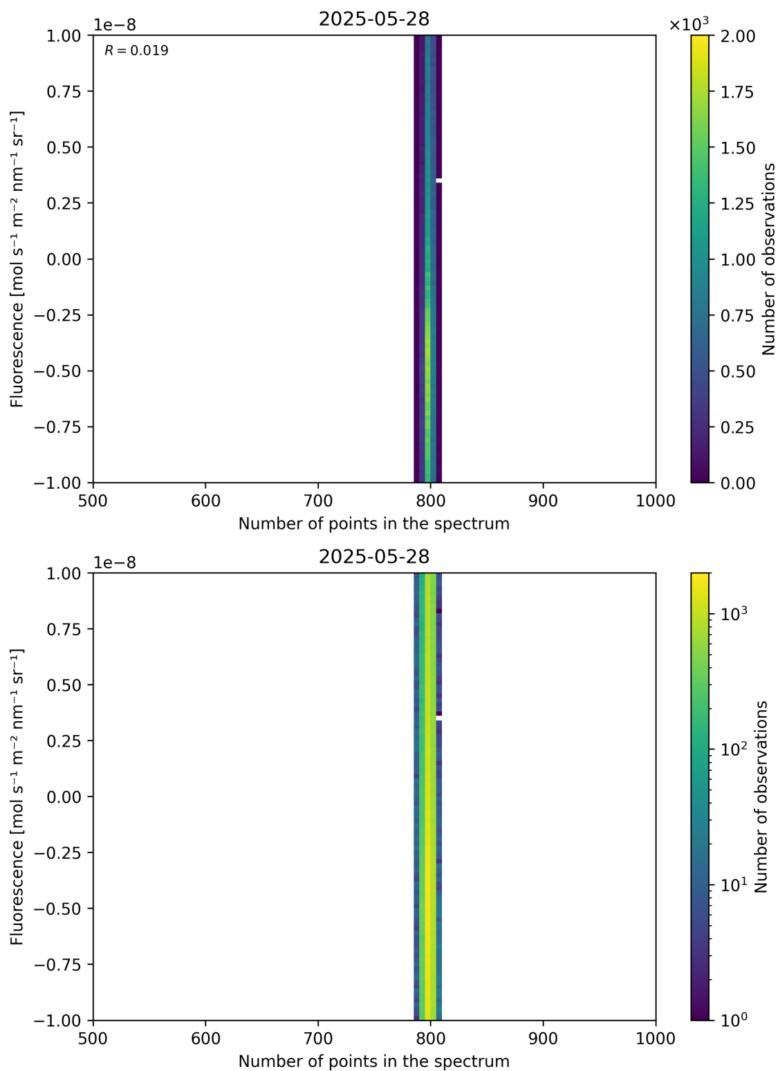
Figure 91: Scatter density plot of “Number of points in the spectrum” against “Fluorescence” for 2025-05-27 to 2025-05-29.
