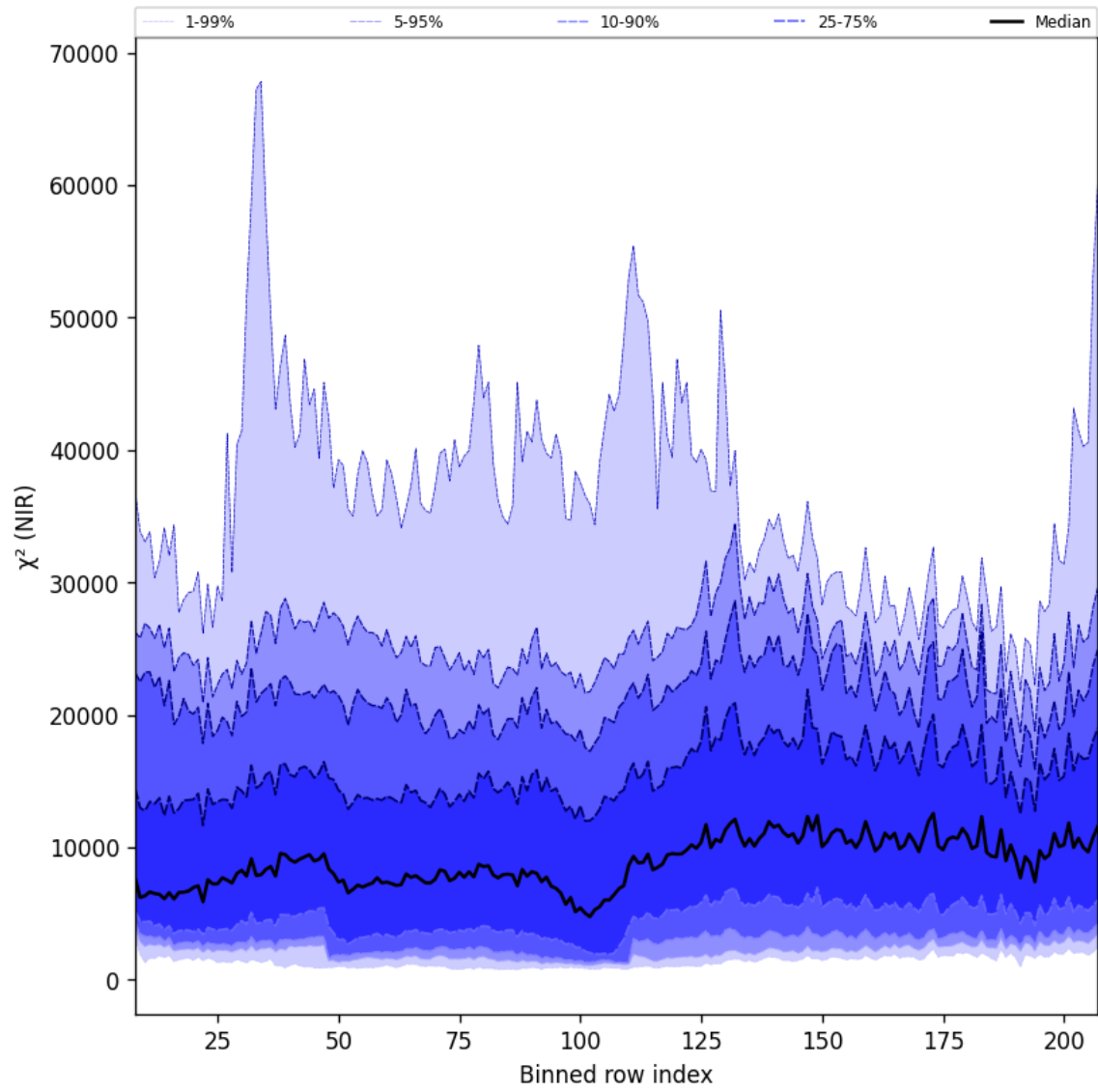
Figure 40: Along track statistics of “ \chi^2 (NIR)” for 2025-05-27 to 2025-05-29
