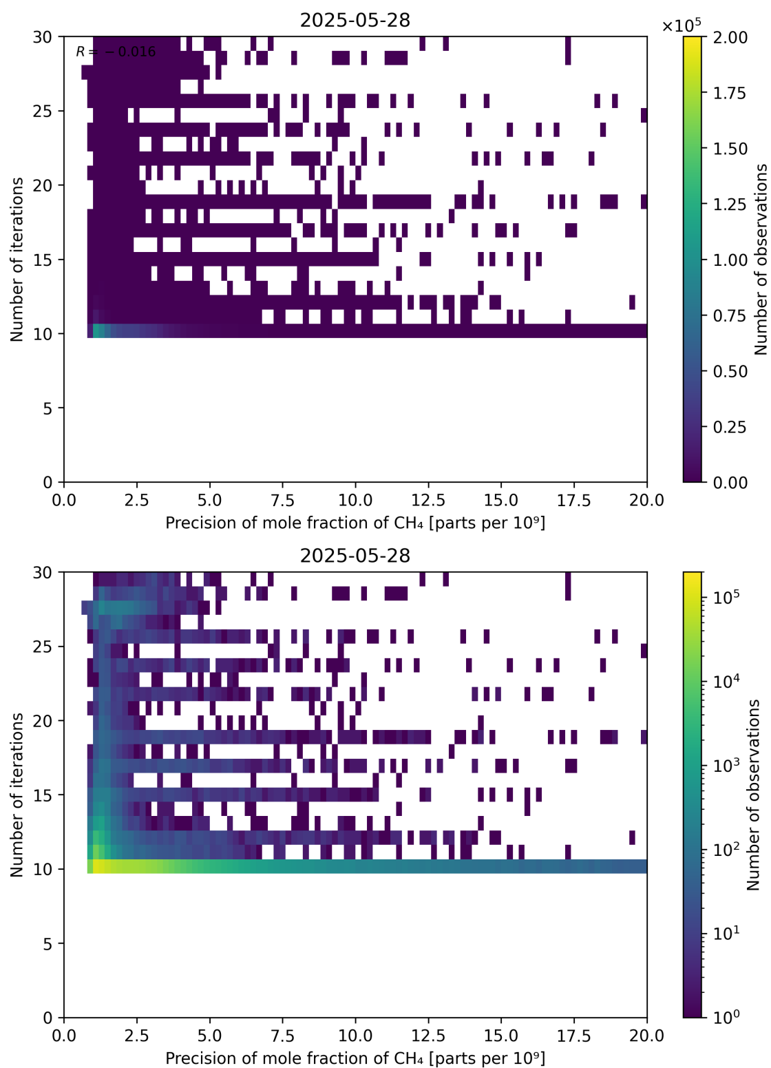
Figure 83: Scatter density plot of “Precision of mole fraction of CH 4 ” against “Number of iterations” for 2025-05-27 to 2025-05-29.
