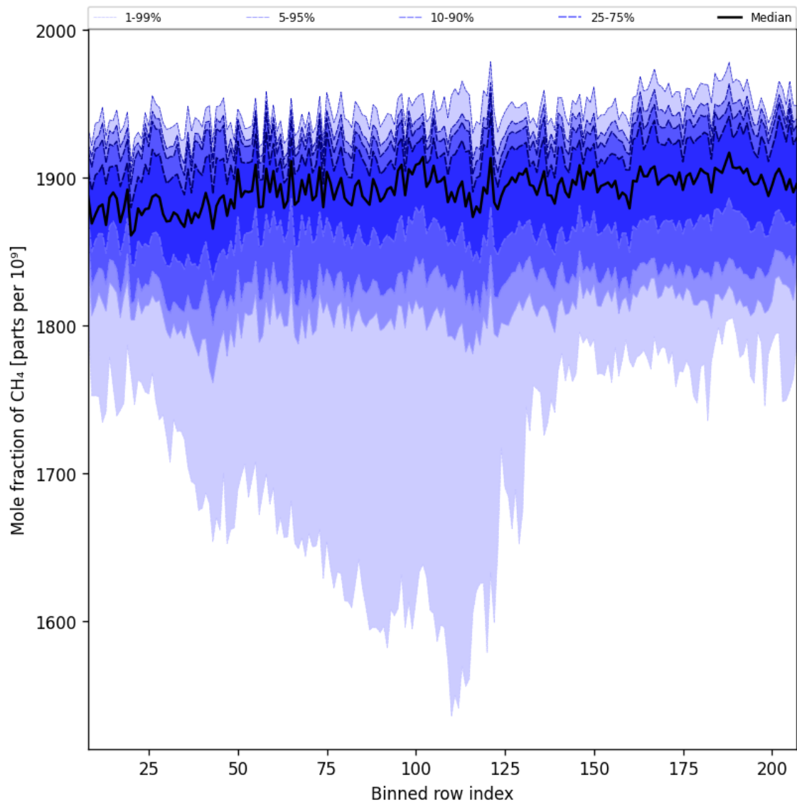
Figure 34: Along track statistics of “Mole fraction of CH 4 ” for 2025-05-27 to 2025-05-29
