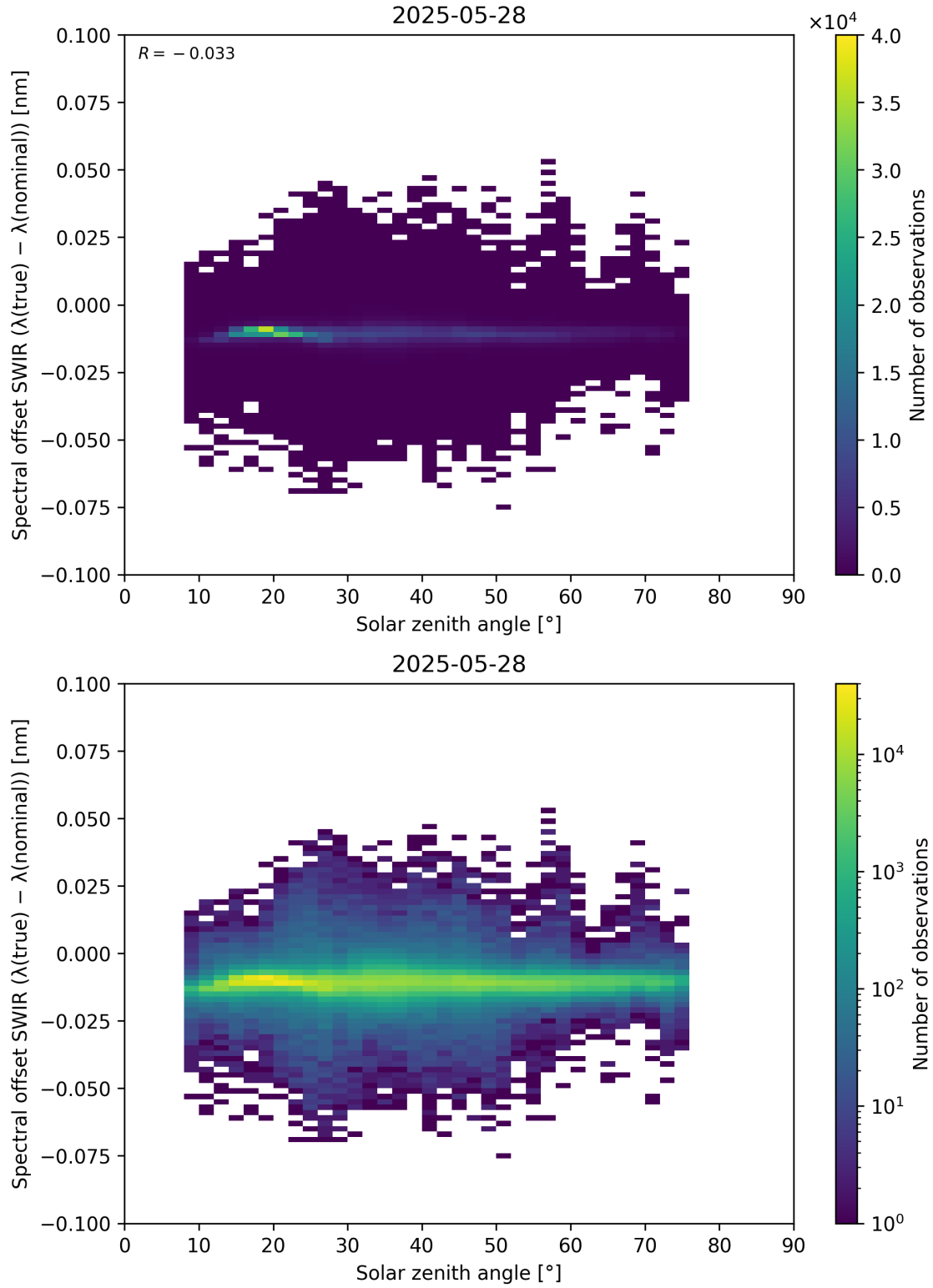
Figure 104: Scatter density plot of “Solar zenith angle” against “Spectral offset SWIR ( \lambda_{\text{true}} - \lambda_{\text{nominal}} )” for 2025-05-27 to 2025-05-29.
