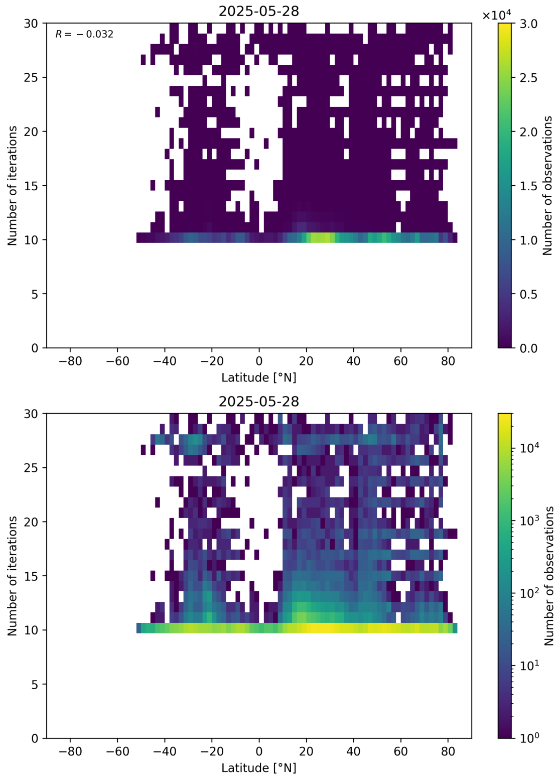
Figure 60: Scatter density plot of “Latitude” against “Number of iterations” for 2025-05-27 to 2025-05-29.
