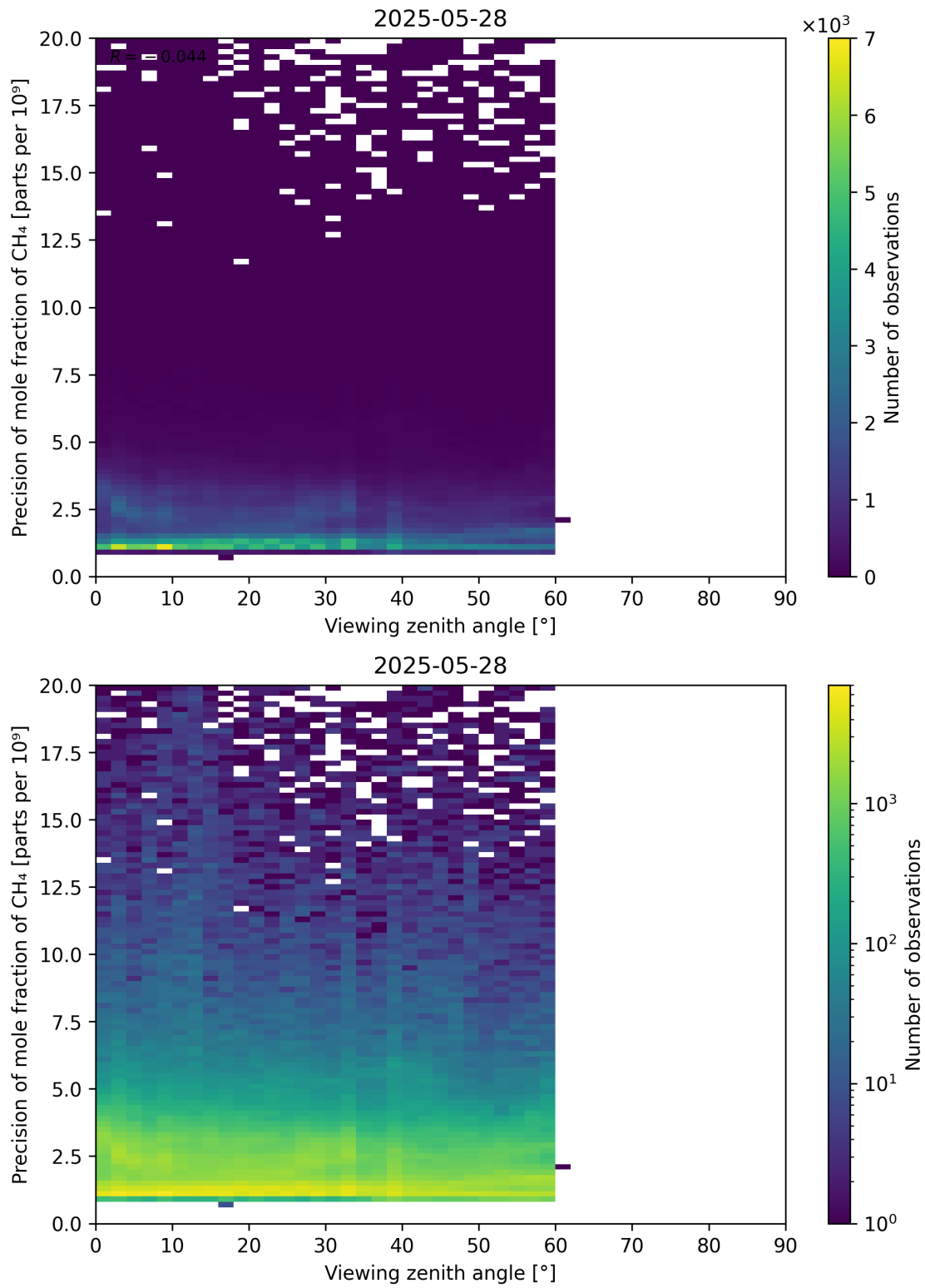
Figure 112: Scatter density plot of “Viewing zenith angle” against “Precision of mole fraction of CH 4 ” for 2025-05-27 to 2025-05-29.
