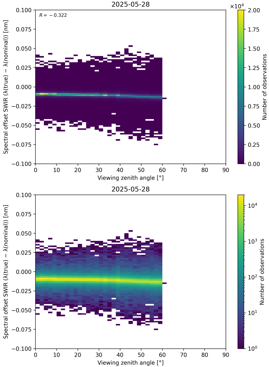
Figure 116: Scatter density plot of “Viewing zenith angle” against “Spectral offset SWIR ( \lambda_{\text{true}} - \lambda_{\text{nominal}} )” for 2025-05-27 to 2025-05-29.
