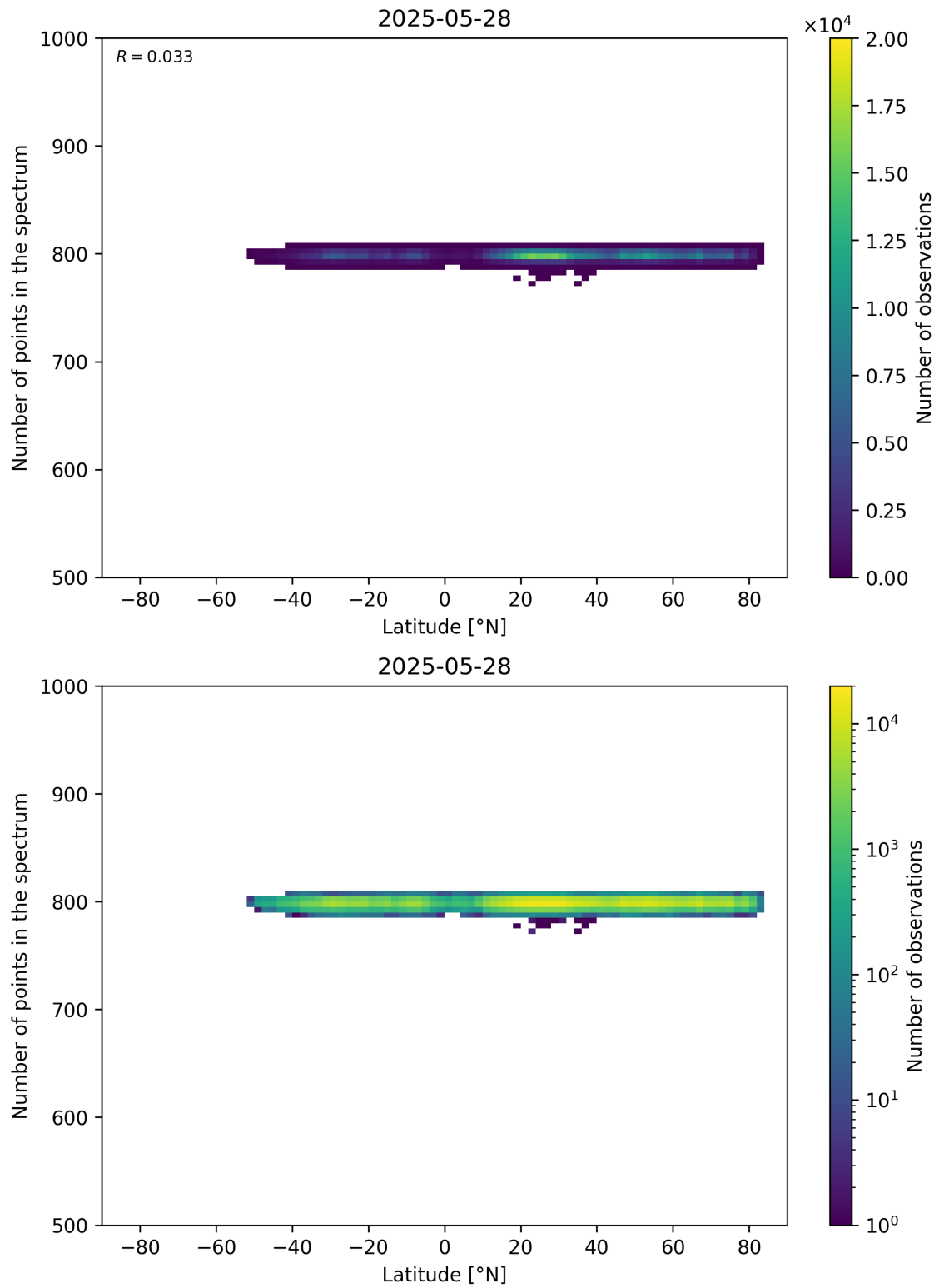
Figure 61: Scatter density plot of “Latitude” against “Number of points in the spectrum” for 2025-05-27 to 2025-05-29.
