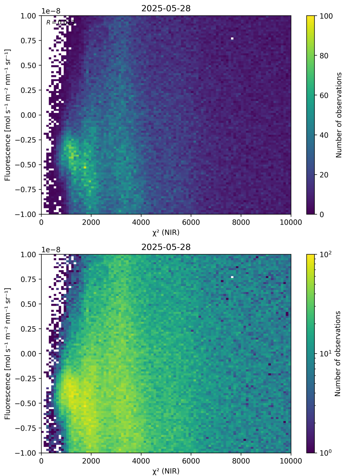
Figure 45: Scatter density plot of “ \chi^2 (NIR)” against “Fluorescence” for 2025-05-27 to 2025-05-29.
