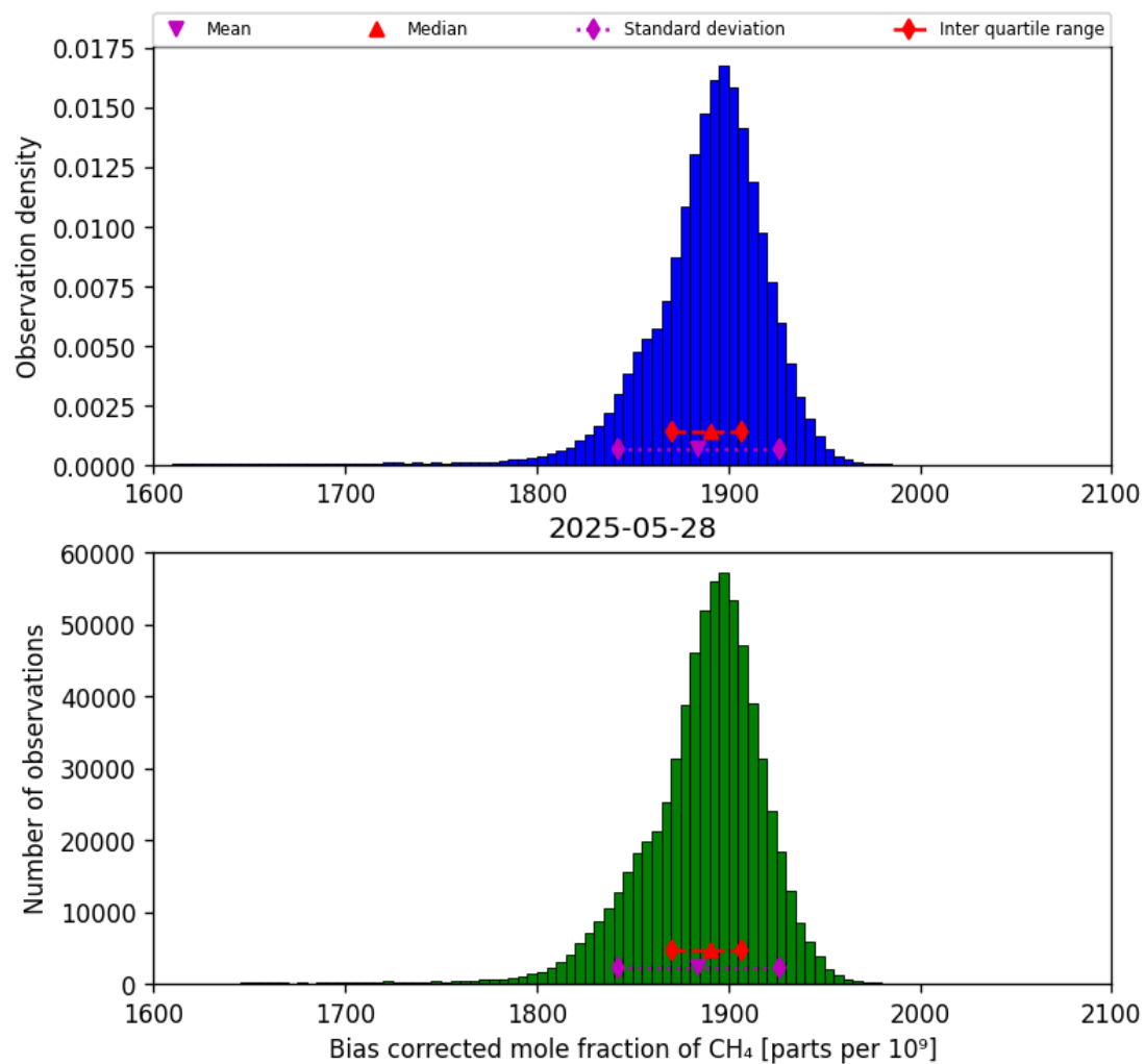
Figure 25: Histogram of “Bias corrected mole fraction of CH 4 ” for 2025-05-27 to 2025-05-29
