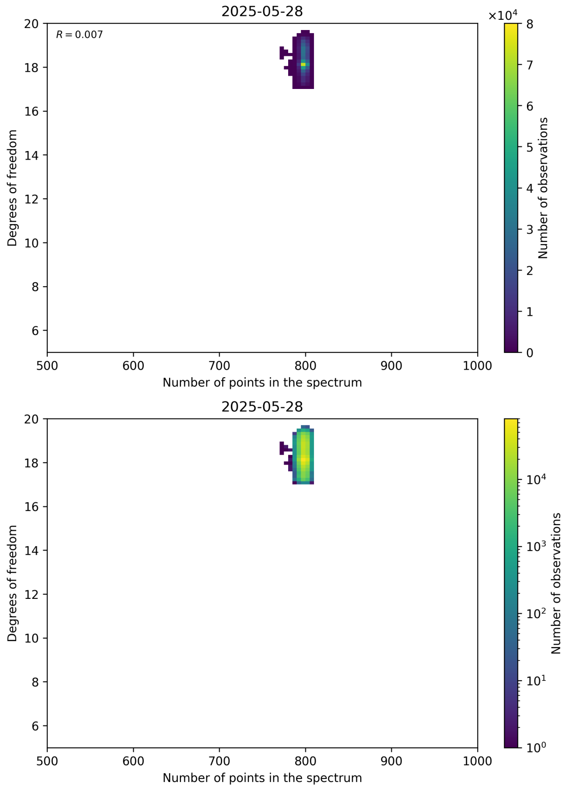
Figure 90: Scatter density plot of “Number of points in the spectrum” against “Degrees of freedom” for 2025-05-27 to 2025-05-29.
