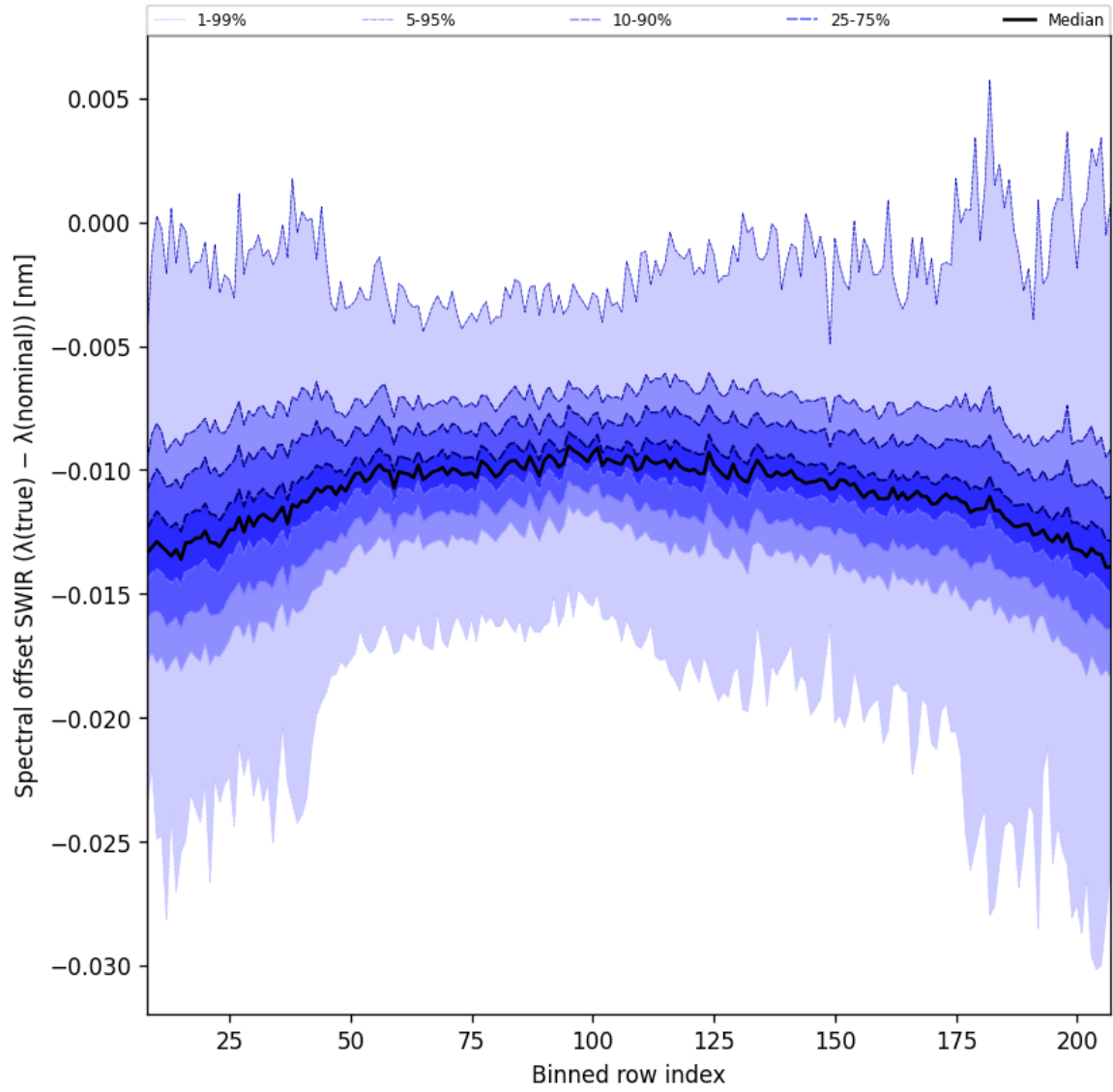
Figure 38: Along track statistics of “Spectral offset SWIR ( \lambda_{\text{true}} - \lambda_{\text{nominal}} )” for 2025-05-27 to 2025-05-29
