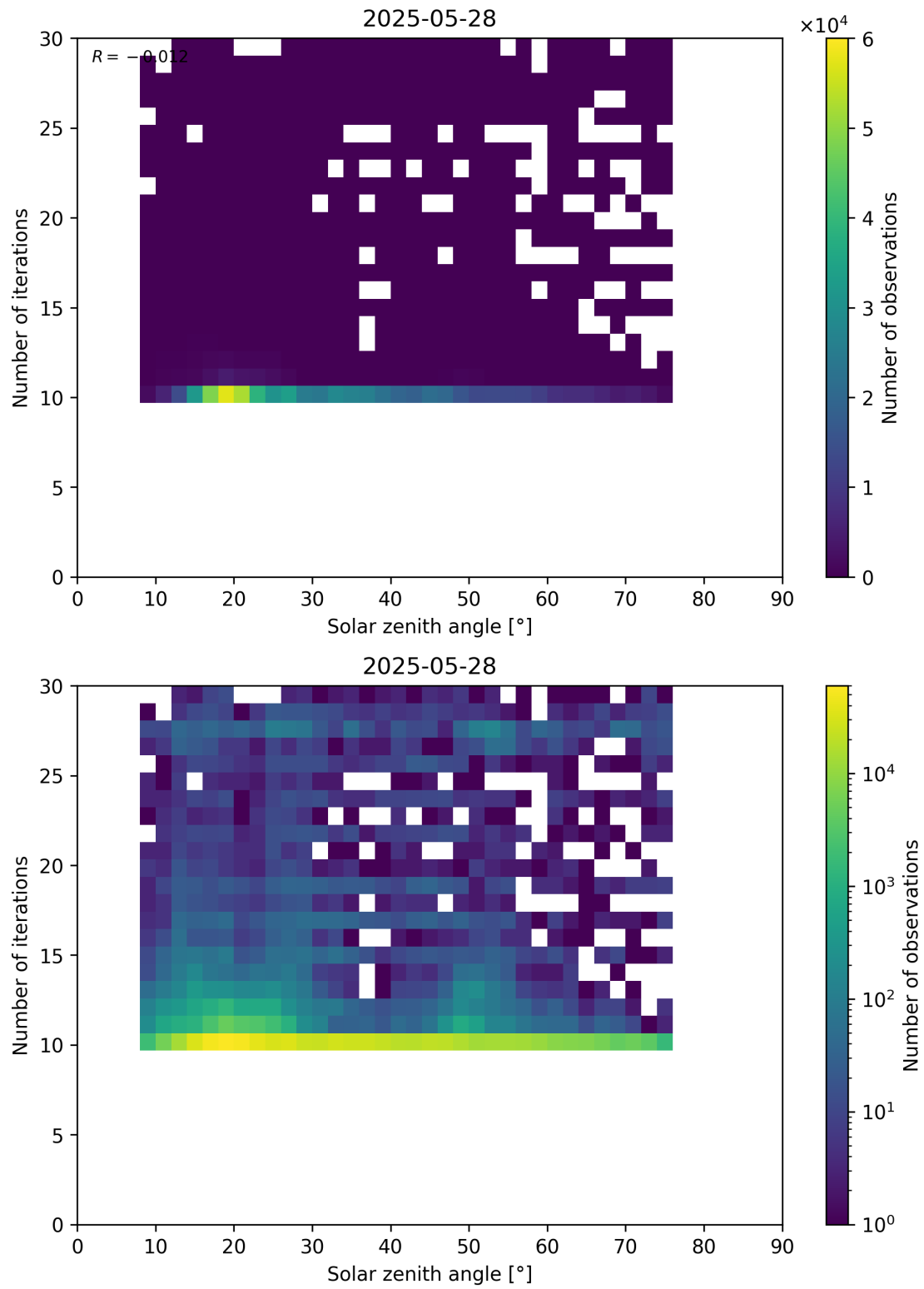
Figure 102: Scatter density plot of “Solar zenith angle” against “Number of iterations” for 2025-05-27 to 2025-05-29.
