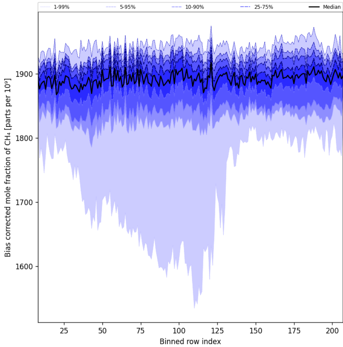
Figure 36: Along track statistics of “Bias corrected mole fraction of CH 4 ” for 2025-05-27 to 2025-05-29
