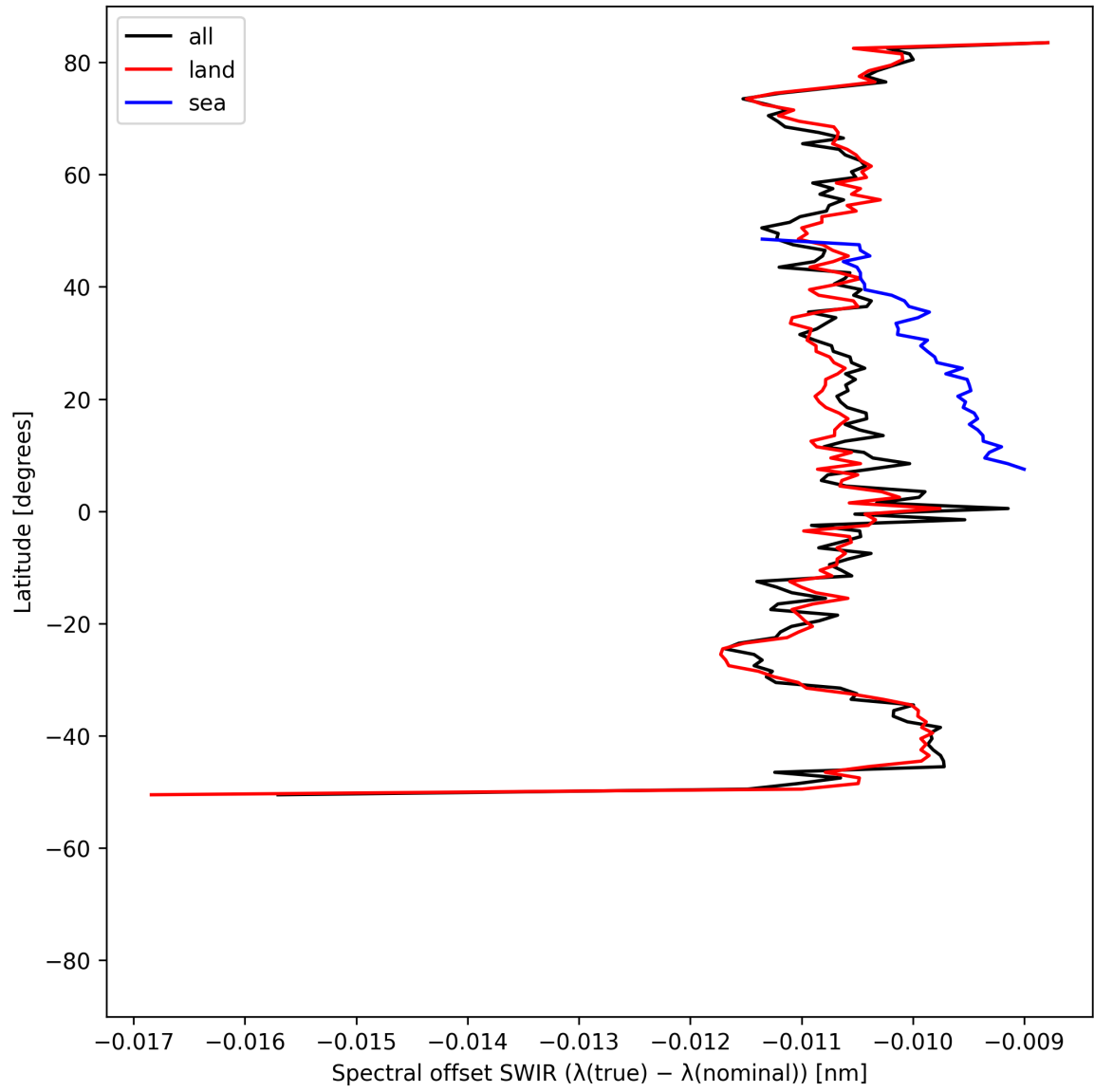
Figure 16: Zonal average of “Spectral offset SWIR ( \lambda_{\text{true}} - \lambda_{\text{nominal}} )” for 2025-05-27 to 2025-05-29.
