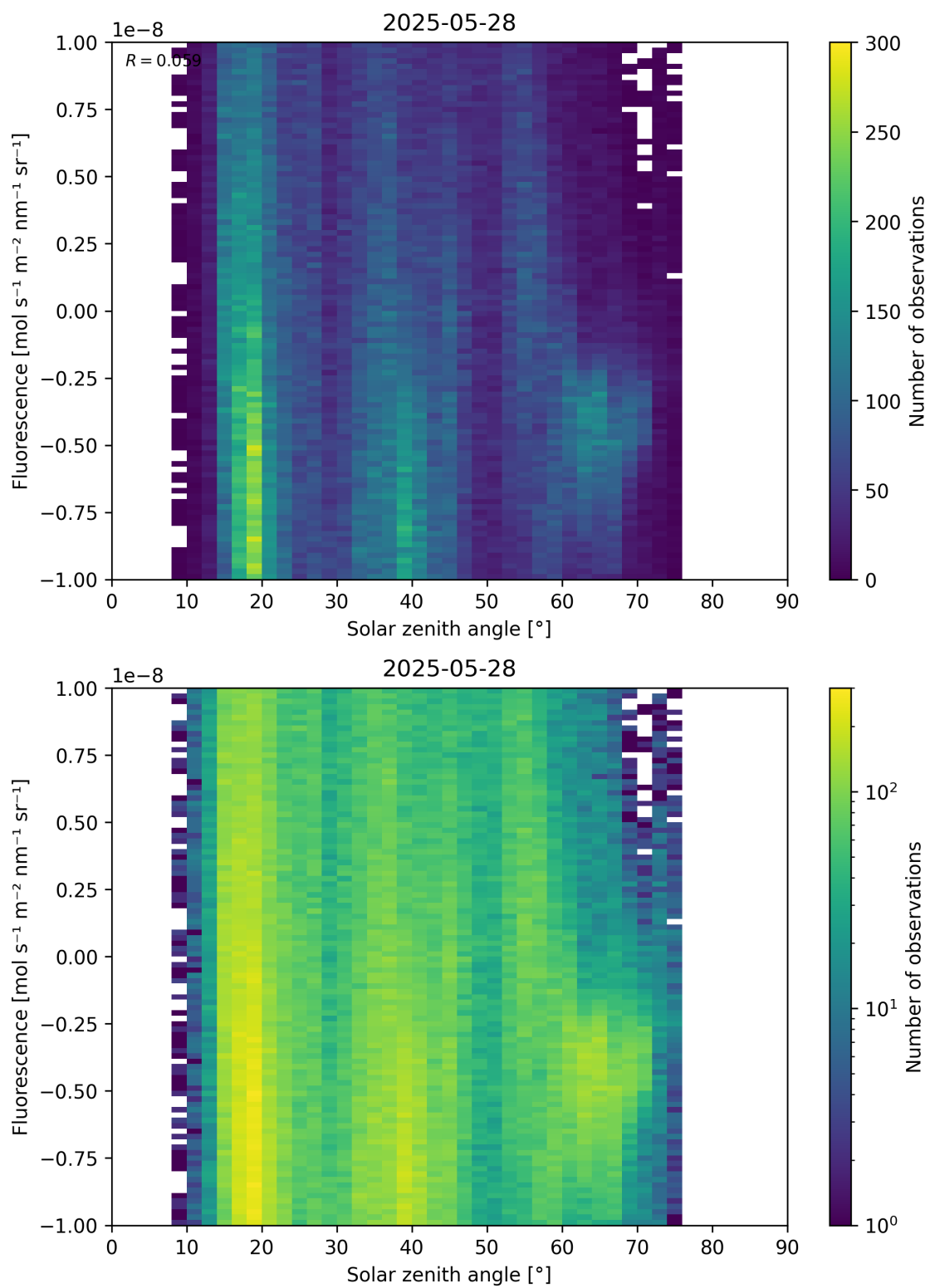
Figure 97: Scatter density plot of “Solar zenith angle” against “Fluorescence” for 2025-05-27 to 2025-05-29.
