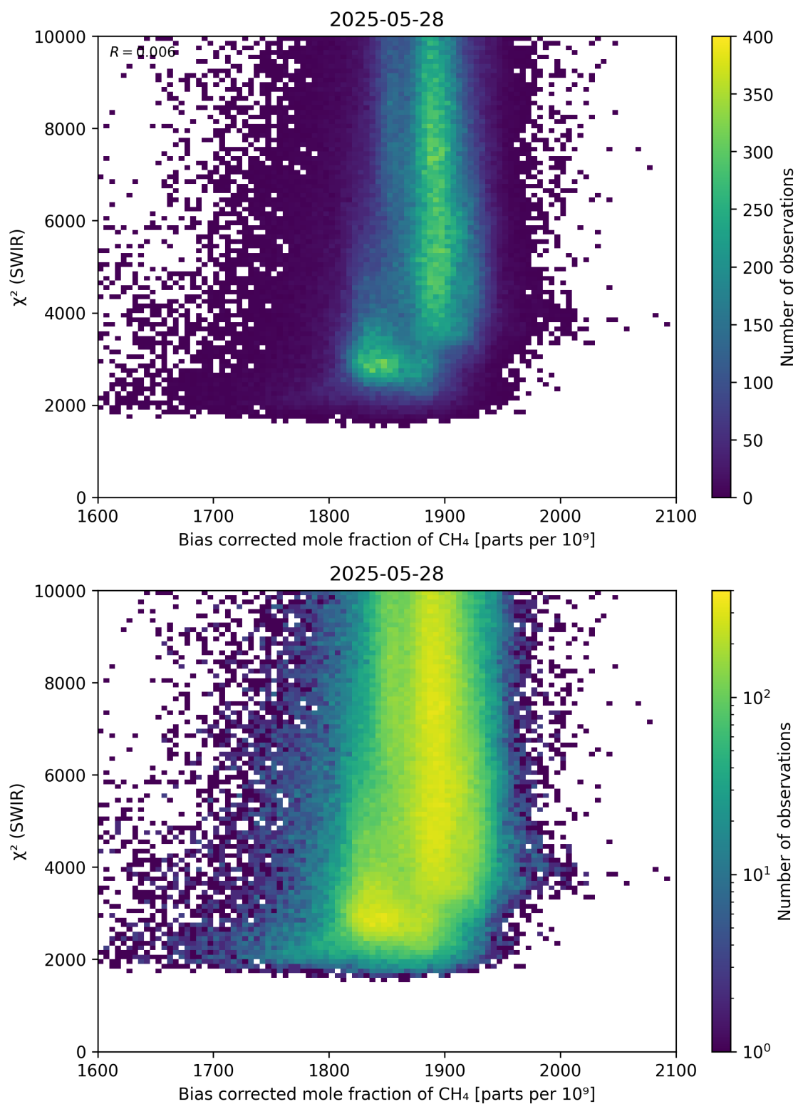
Figure 64: Scatter density plot of “Bias corrected mole fraction of \text{CH}_4 ” against “ \chi^2 (SWIR)” for 2025-05-27 to 2025-05-29.
