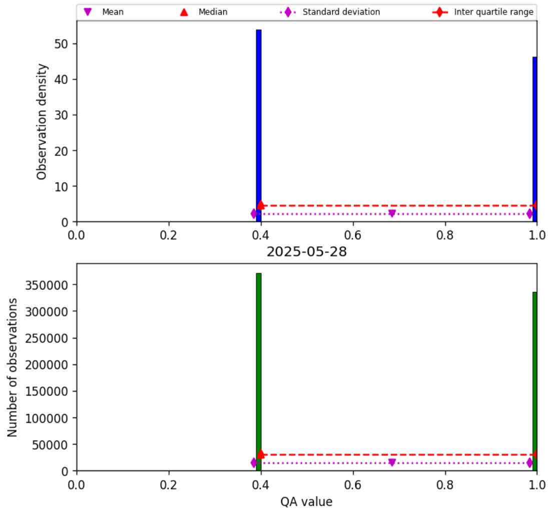
Figure 22: Histogram of “QA value” for 2025-05-27 to 2025-05-29
