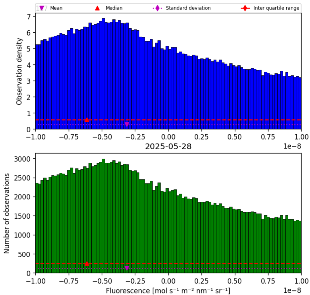
Figure 32: Histogram of “Fluorescence” for 2025-05-27 to 2025-05-29
