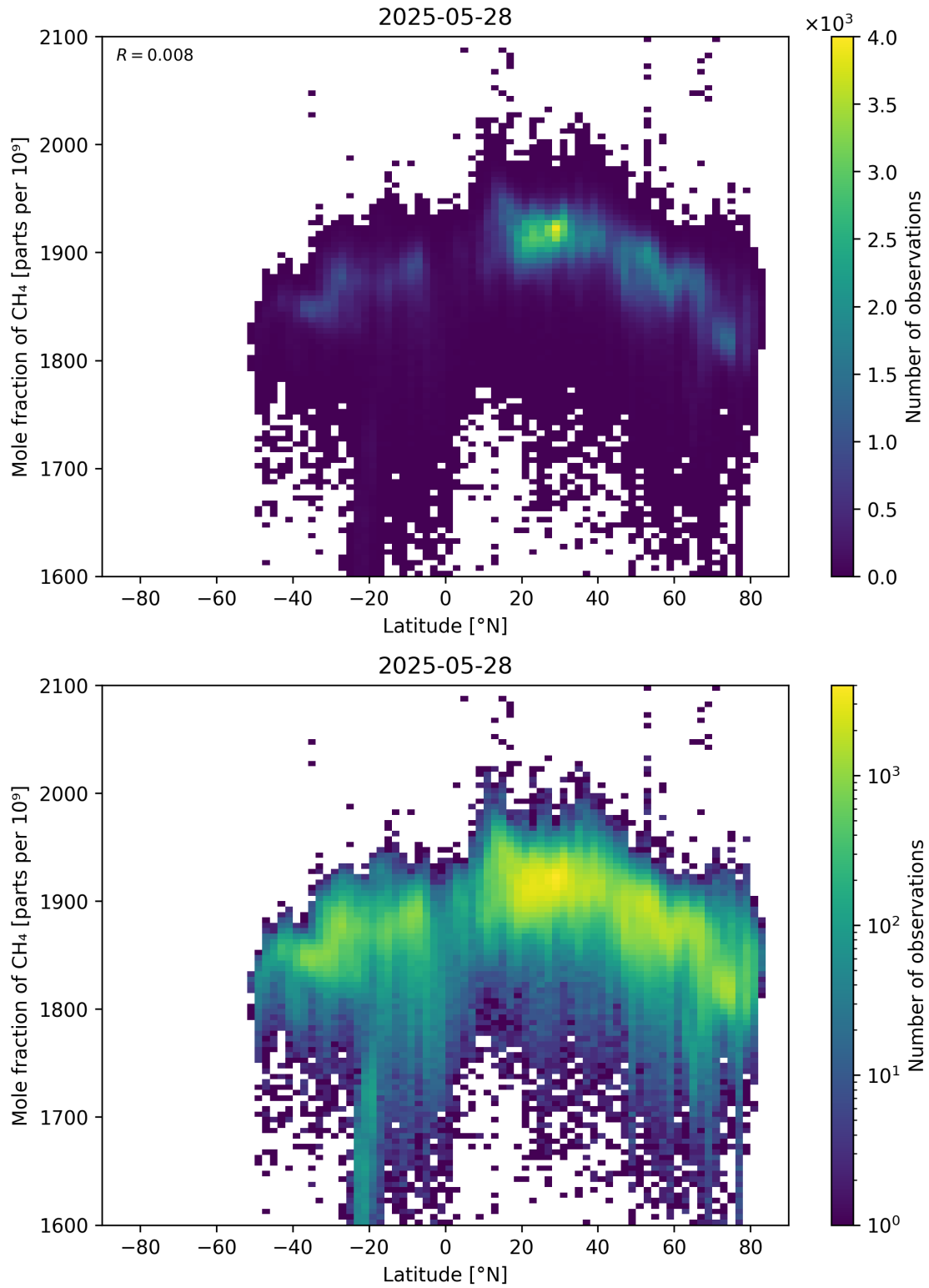
Figure 57: Scatter density plot of “Latitude” against “Mole fraction of CH 4 ” for 2025-05-27 to 2025-05-29.
