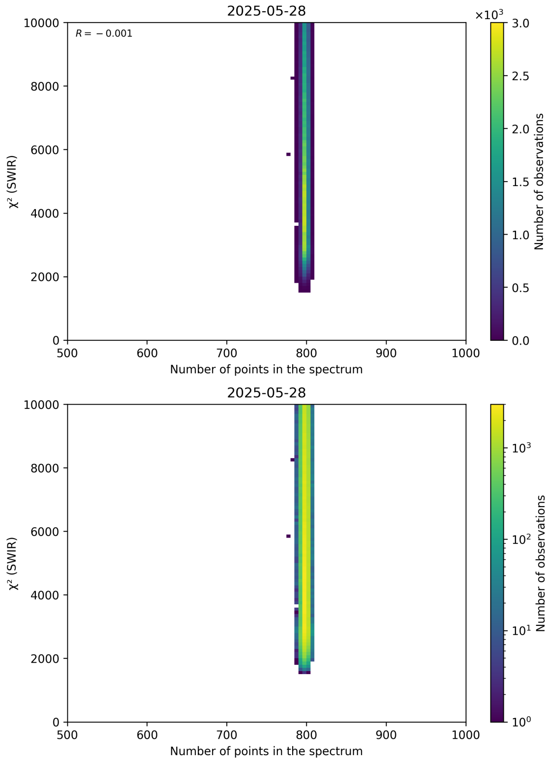
Figure 89: Scatter density plot of “Number of points in the spectrum” against “ \chi^2 (SWIR)” for 2025-05-27 to 2025-05-29.
