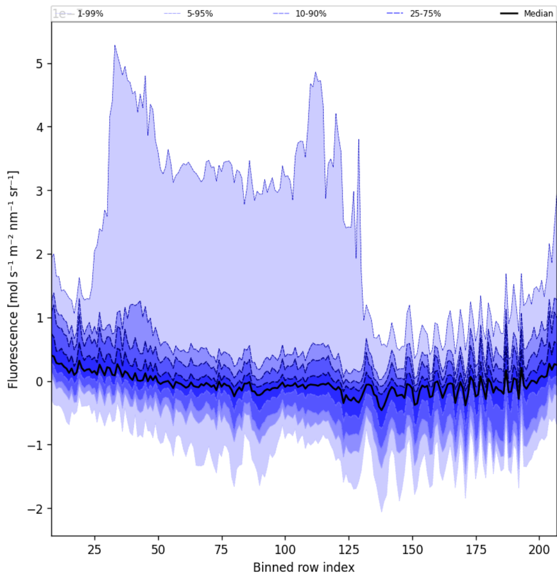
Figure 43: Along track statistics of "Fluorescence" for 2025-05-27 to 2025-05-29
