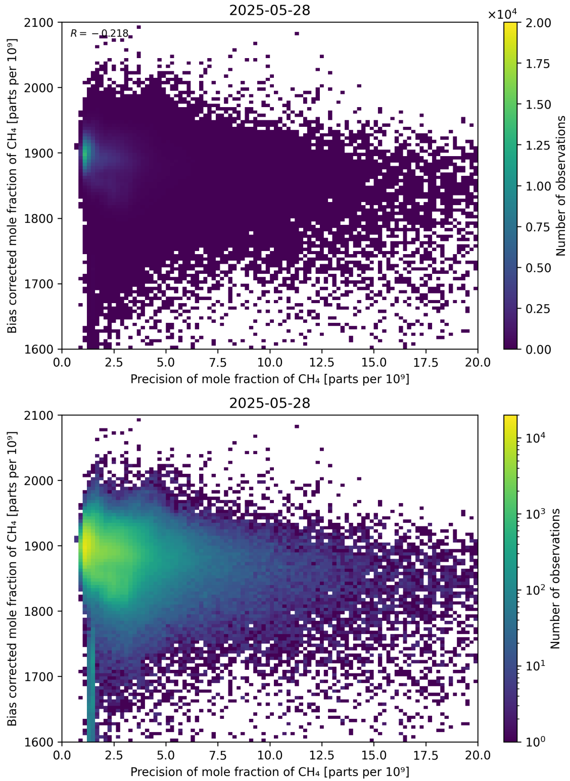
Figure 82: Scatter density plot of “Precision of mole fraction of CH 4 ” against “Bias corrected mole fraction of CH 4 ” for 2025-05-27 to 2025-05-29.
