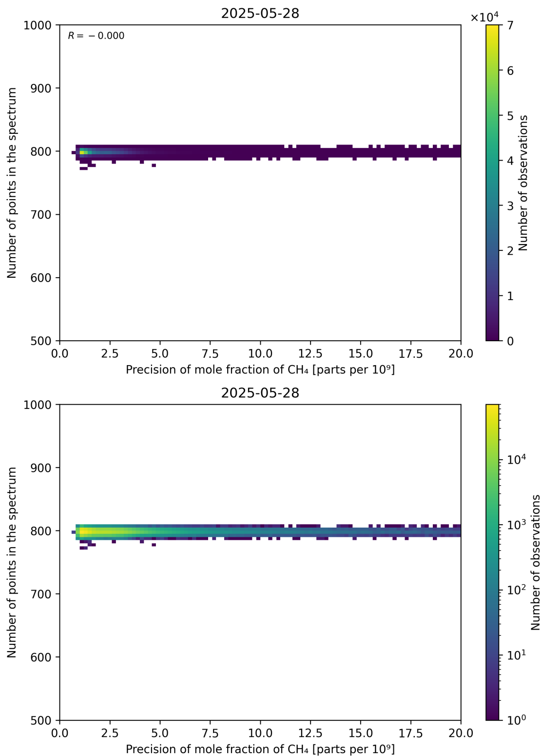
Figure 84: Scatter density plot of “Precision of mole fraction of CH 4 ” against “Number of points in the spectrum” for 2025-05-27 to 2025-05-29.
