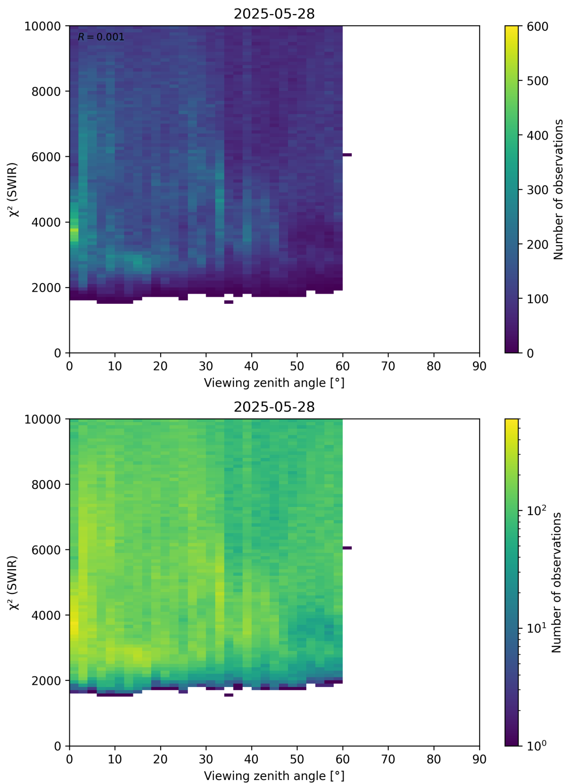
Figure 106: Scatter density plot of “Viewing zenith angle” against “ \chi^2 (SWIR)” for 2025-05-27 to 2025-05-29.
