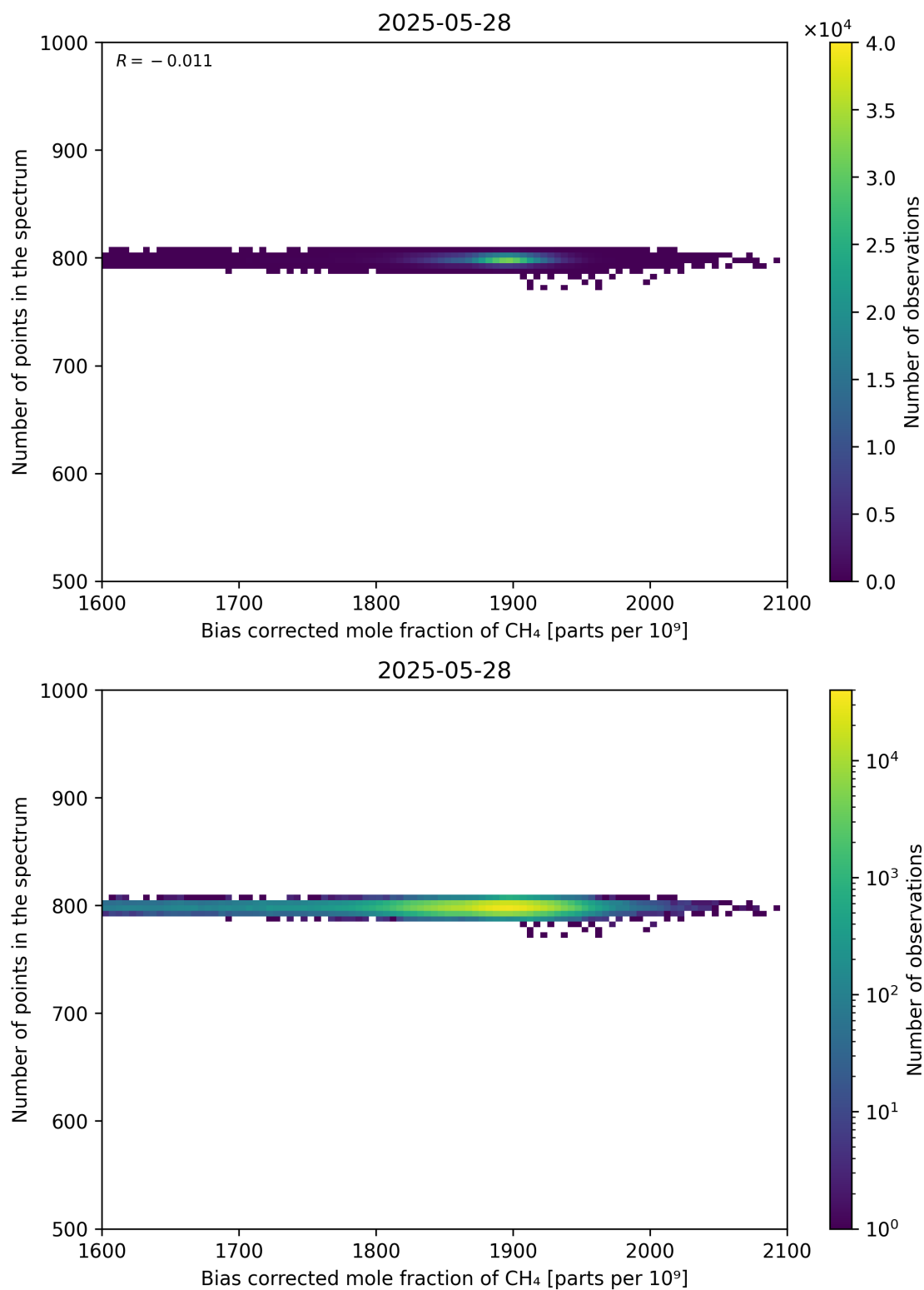
Figure 68: Scatter density plot of “Bias corrected mole fraction of CH 4 ” against “Number of points in the spectrum” for 2025-05-27 to 2025-05-29.
