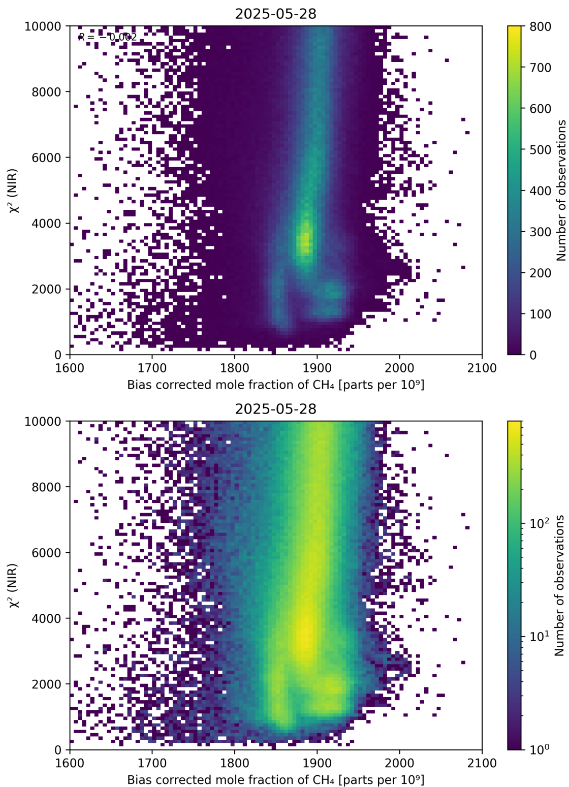
Figure 63: Scatter density plot of “Bias corrected mole fraction of \text{CH}_4 ” against “ \chi^2 (NIR)” for 2025-05-27 to 2025-05-29.
