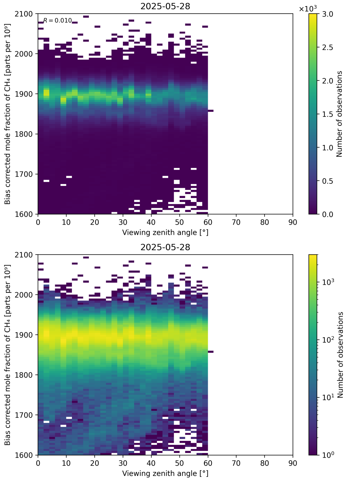
Figure 111: Scatter density plot of “Viewing zenith angle” against “Bias corrected mole fraction of CH 4 ” for 2025-05-27 to 2025-05-29.
