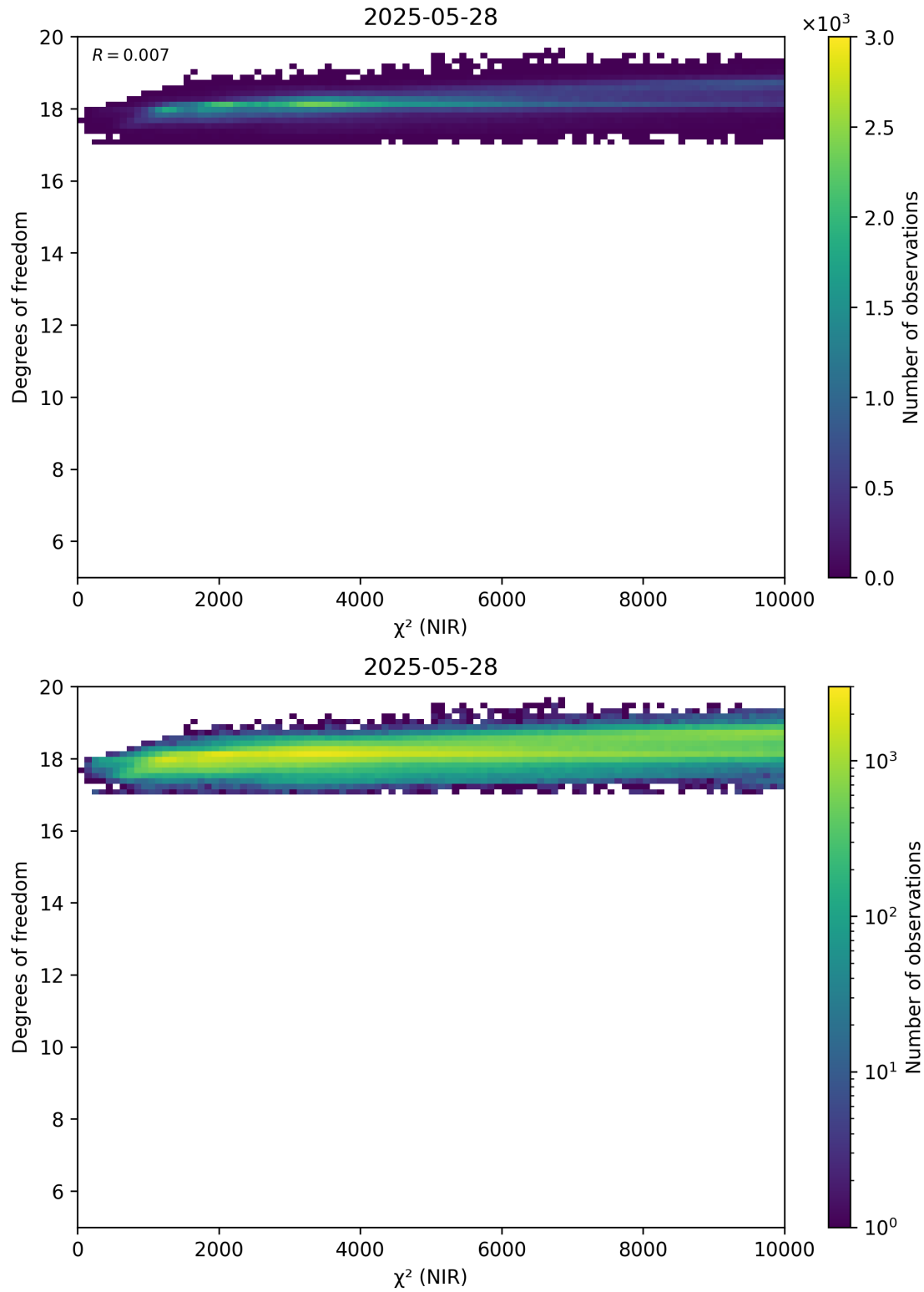
Figure 44: Scatter density plot of “ \chi^2 (NIR)” against “Degrees of freedom” for 2025-05-27 to 2025-05-29.
