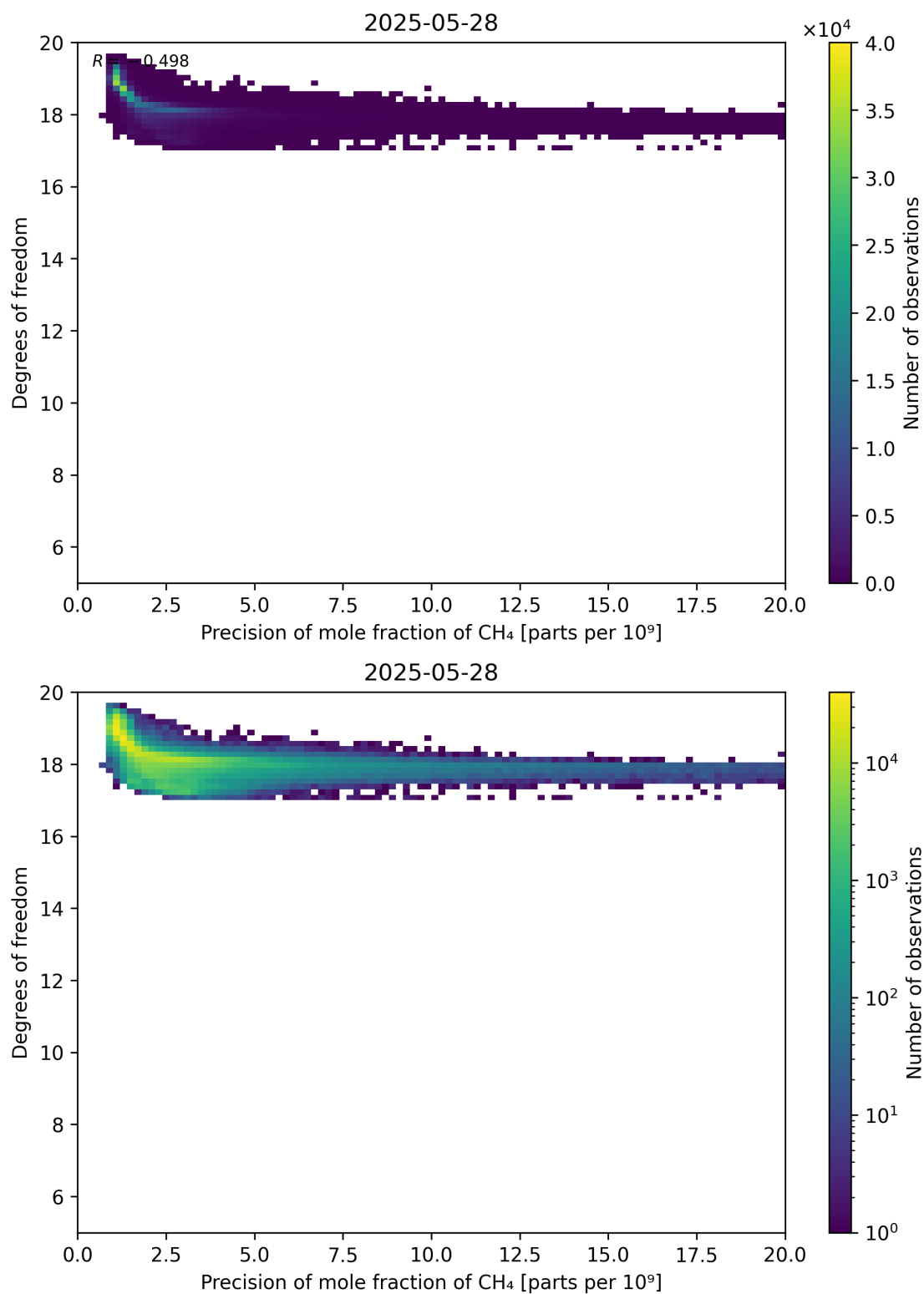
Figure 80: Scatter density plot of “Precision of mole fraction of CH 4 ” against “Degrees of freedom” for 2025-05-27 to 2025-05-29.
