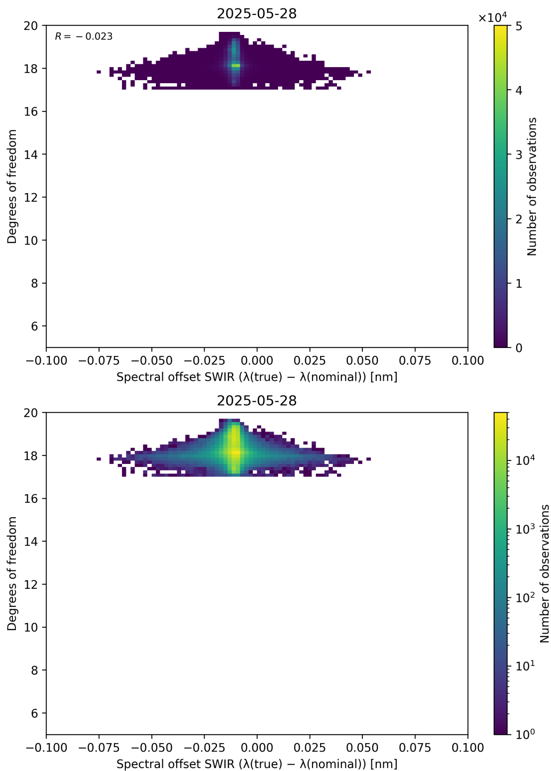
Figure 119: Scatter density plot of “Spectral offset SWIR ( \lambda_{\text{true}} - \lambda_{\text{nominal}} )” against “Degrees of freedom” for 2025-05-27 to 2025-05-29.
