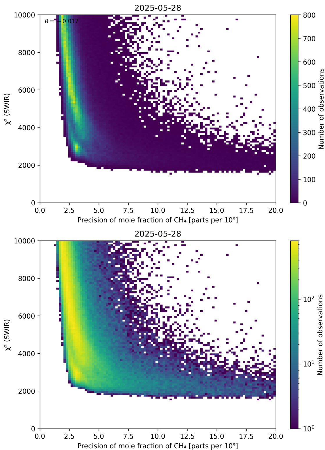
Figure 79: Scatter density plot of “Precision of mole fraction of \text{CH}_4 ” against “ \chi^2 (SWIR)” for 2025-05-27 to 2025-05-29.
