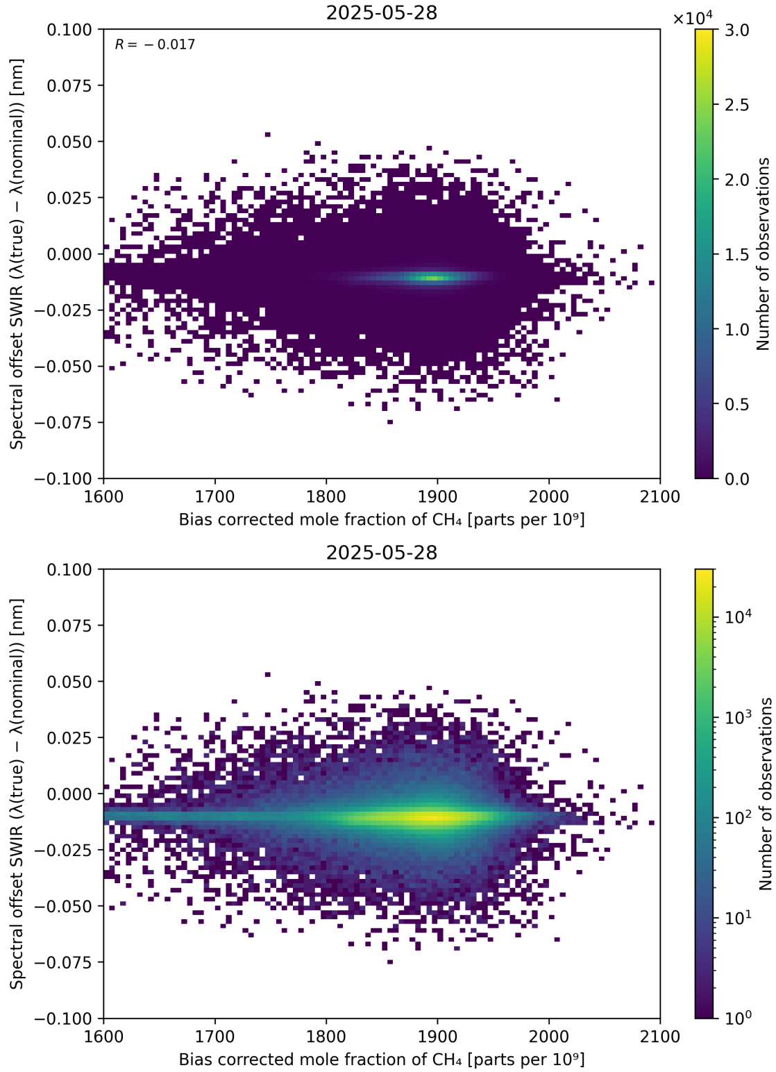
Figure 69: Scatter density plot of “Bias corrected mole fraction of \text{CH}_4 ” against “Spectral offset SWIR ( \lambda_{\text{true}} - \lambda_{\text{nominal}} )” for 2025-05-27 to 2025-05-29.
