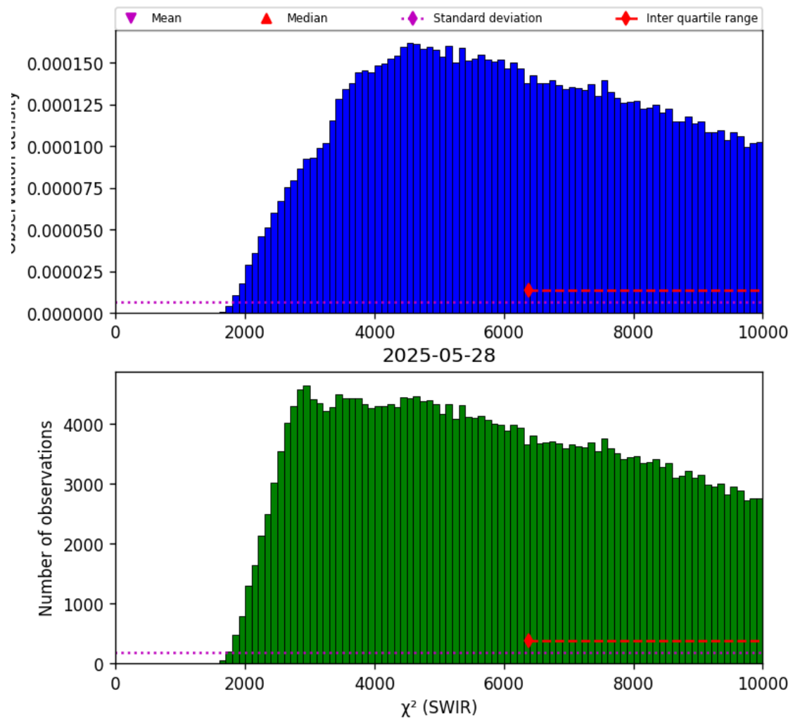
Figure 28: Histogram of “ \chi^2 (SWIR)” for 2025-05-27 to 2025-05-29
