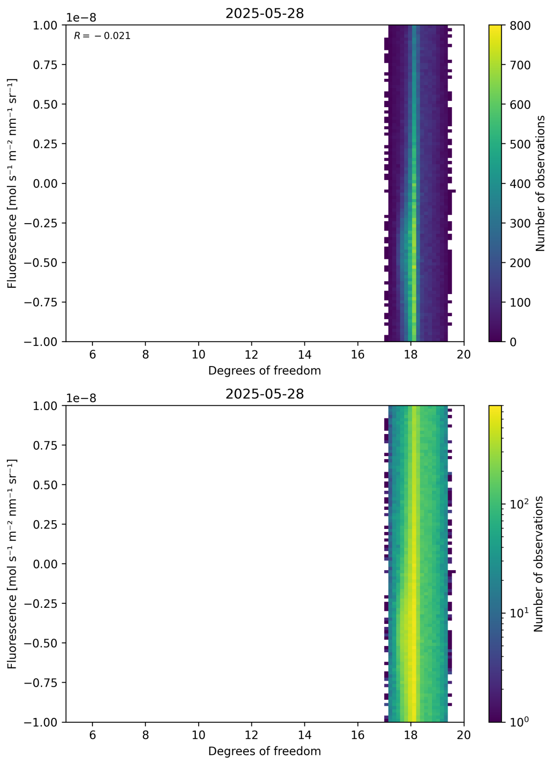
Figure 51: Scatter density plot of “Degrees of freedom” against “Fluorescence” for 2025-05-27 to 2025-05-29.
