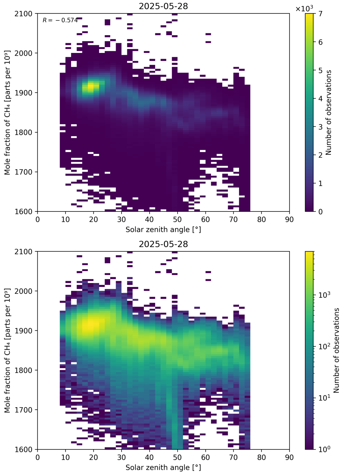
Figure 99: Scatter density plot of “Solar zenith angle” against “Mole fraction of CH 4 ” for 2025-05-27 to 2025-05-29.
