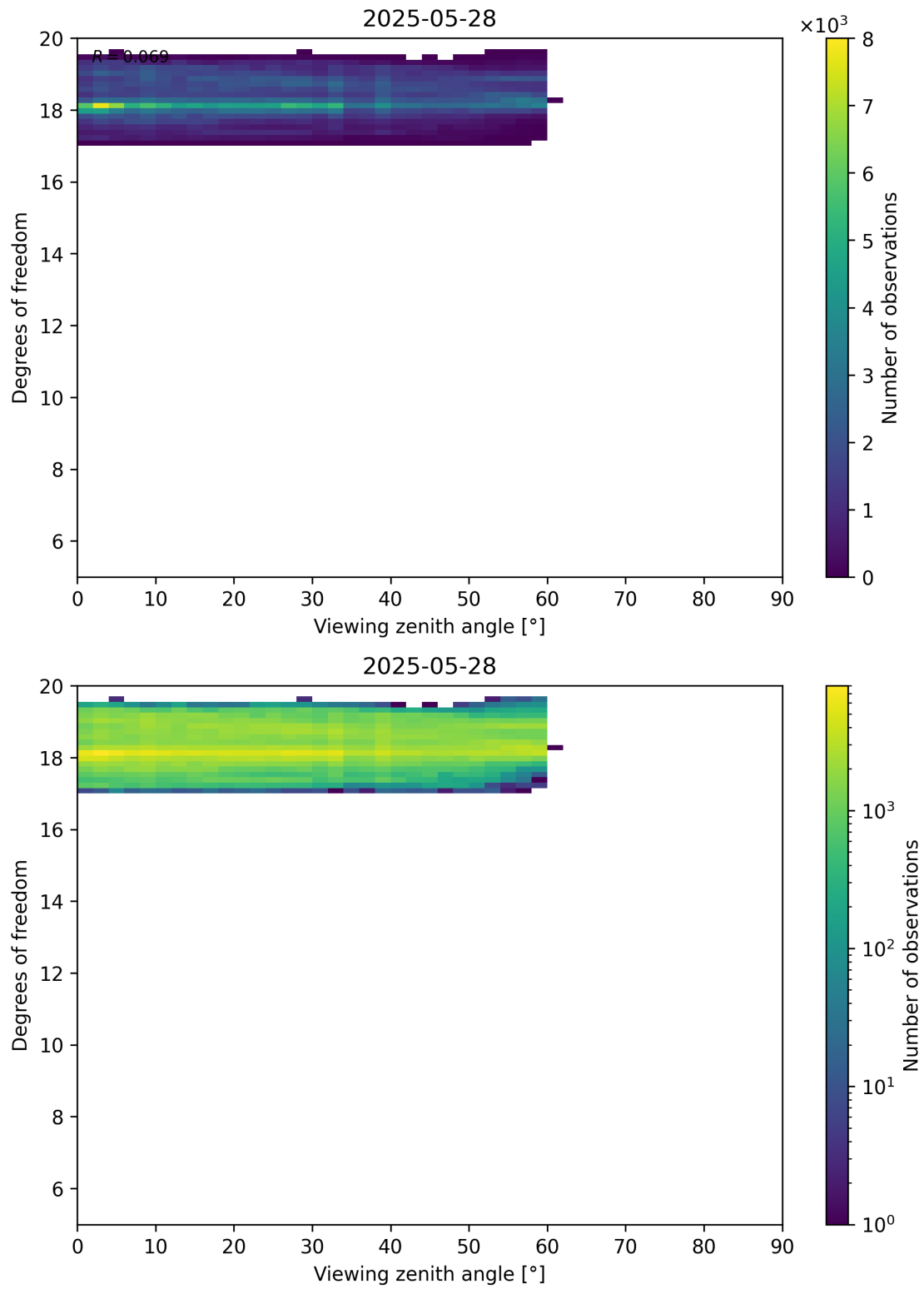
Figure 107: Scatter density plot of “Viewing zenith angle” against “Degrees of freedom” for 2025-05-27 to 2025-05-29.
