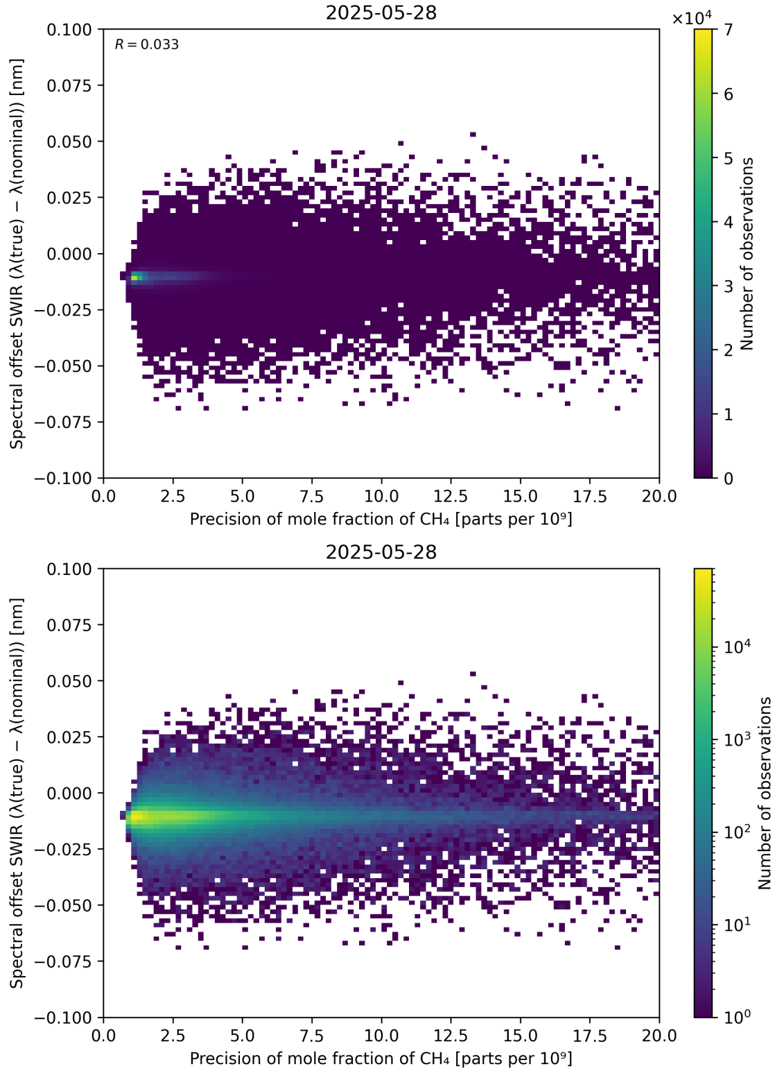
Figure 85: Scatter density plot of “Precision of mole fraction of \text{CH}_4 ” against “Spectral offset SWIR ( \lambda_{\text{true}} - \lambda_{\text{nominal}} )” for 2025-05-27 to 2025-05-29.
