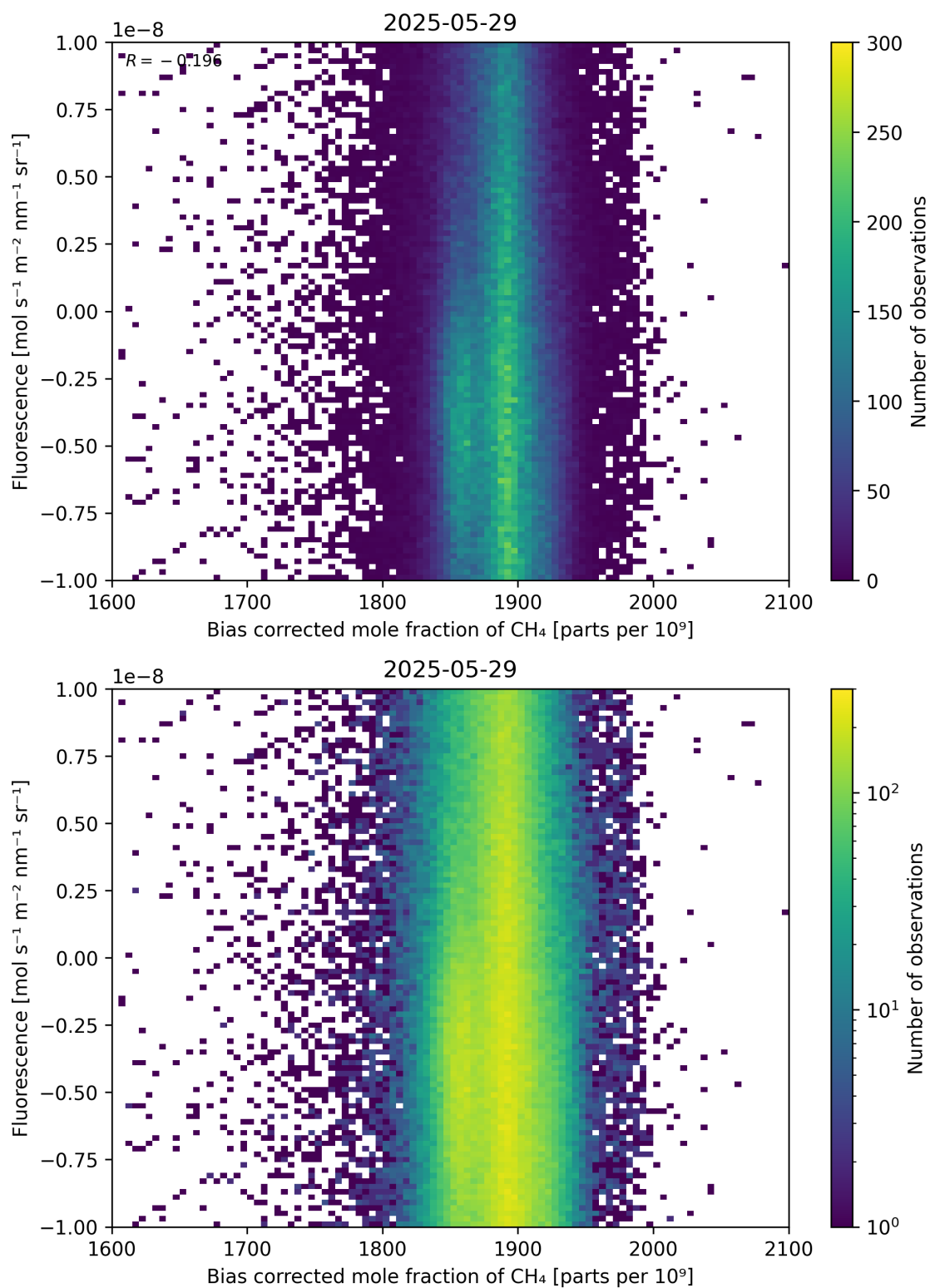
Figure 66: Scatter density plot of “Bias corrected mole fraction of \text{CH}_4 ” against “Fluorescence” for 2025-05-28 to 2025-05-30.
