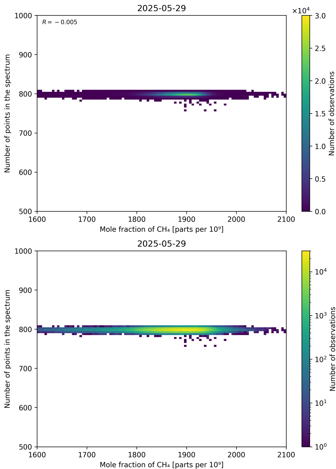
Figure 77: Scatter density plot of “Mole fraction of CH 4 ” against “Number of points in the spectrum” for 2025-05-28 to 2025-05-30.
