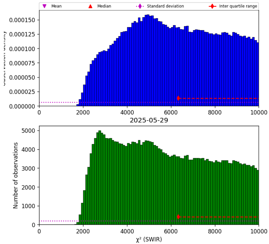
Figure 28: Histogram of “ \chi^2 (SWIR)” for 2025-05-28 to 2025-05-30
