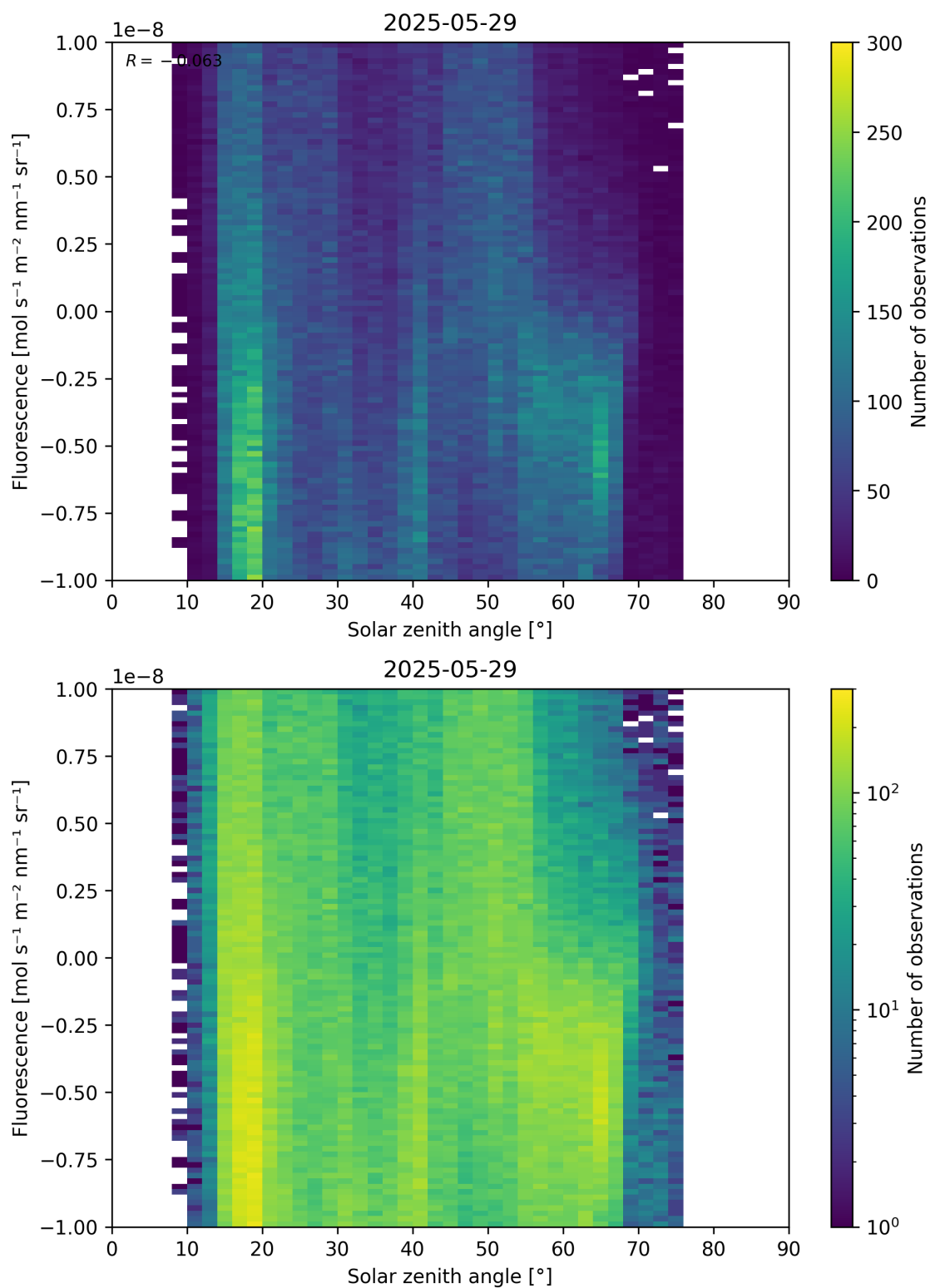
Figure 97: Scatter density plot of “Solar zenith angle” against “Fluorescence” for 2025-05-28 to 2025-05-30.
