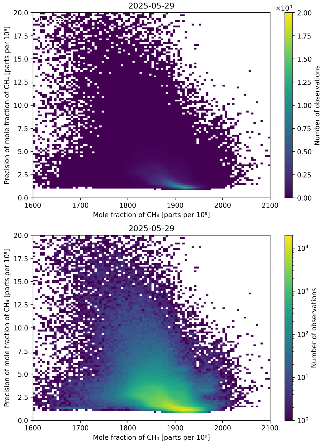
Figure 75: Scatter density plot of “Mole fraction of CH 4 ” against “Precision of mole fraction of CH 4 ” for 2025-05-28 to 2025-05-30.
