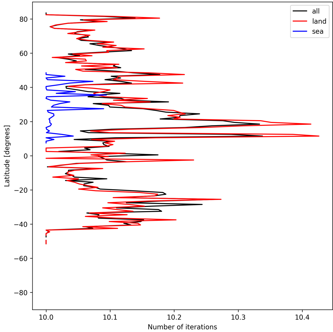
Figure 20: Zonal average of “Number of iterations” for 2025-05-28 to 2025-05-30.
