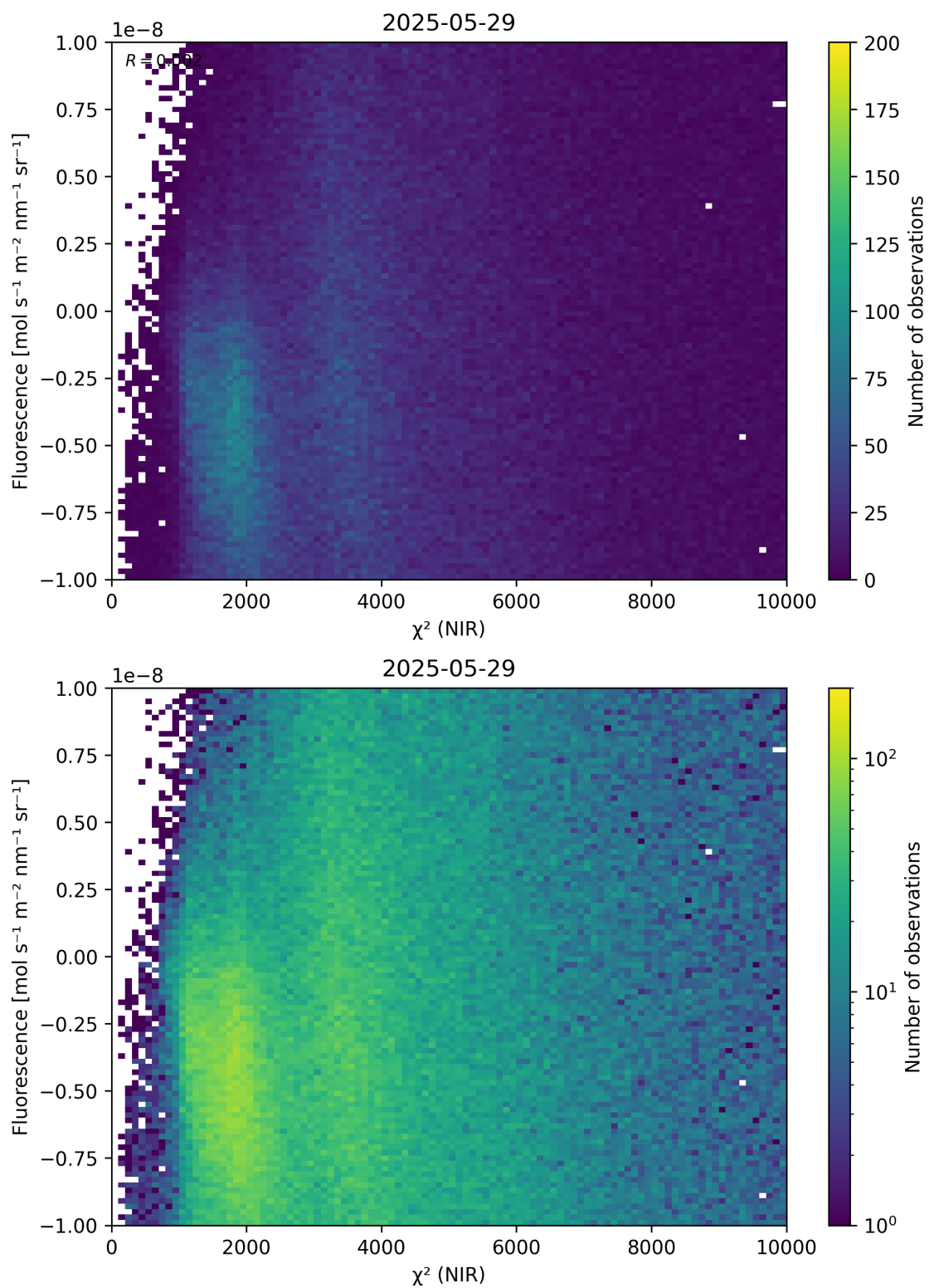
Figure 45: Scatter density plot of “ \chi^2 (NIR)” against “Fluorescence” for 2025-05-28 to 2025-05-30.
