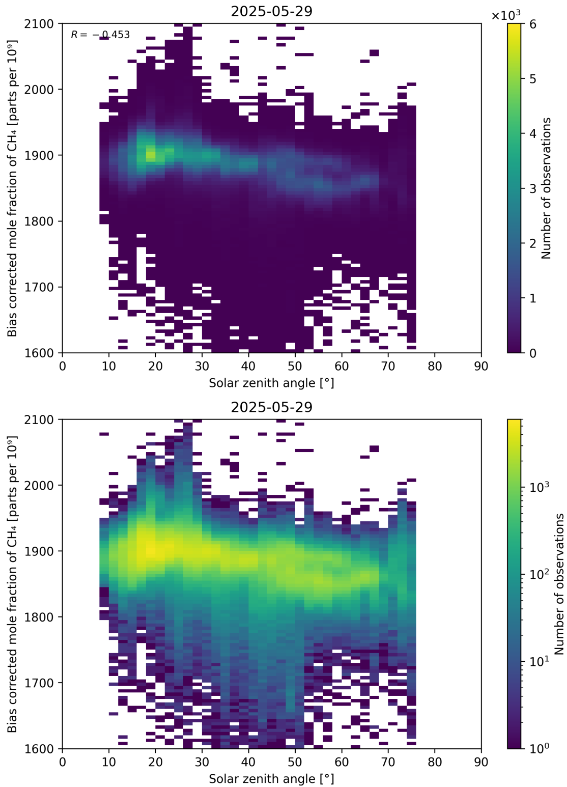
Figure 100: Scatter density plot of “Solar zenith angle” against “Bias corrected mole fraction of \text{CH}_4 ” for 2025-05-28 to 2025-05-30.
