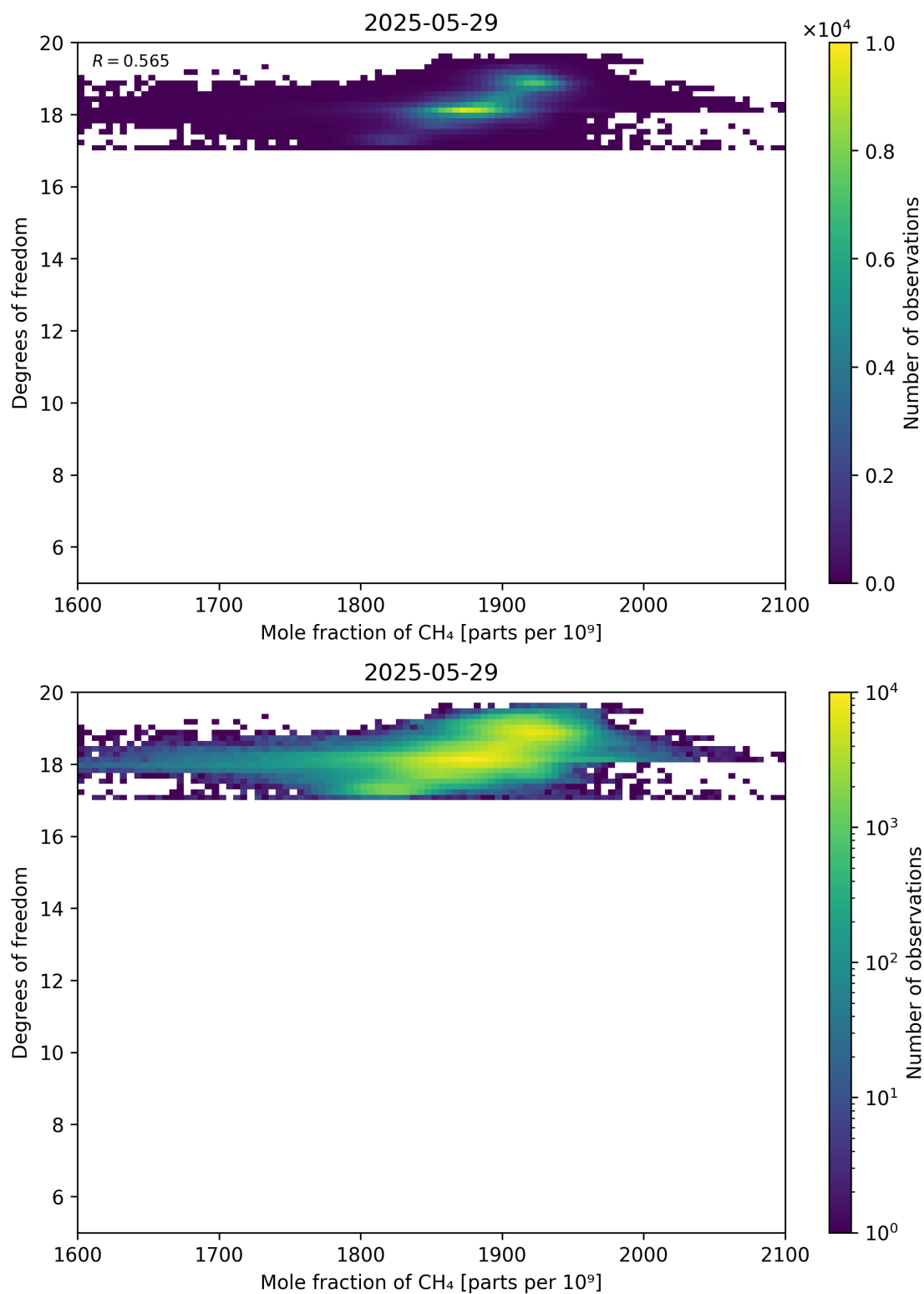
Figure 72: Scatter density plot of “Mole fraction of CH 4 ” against “Degrees of freedom” for 2025-05-28 to 2025-05-30.
