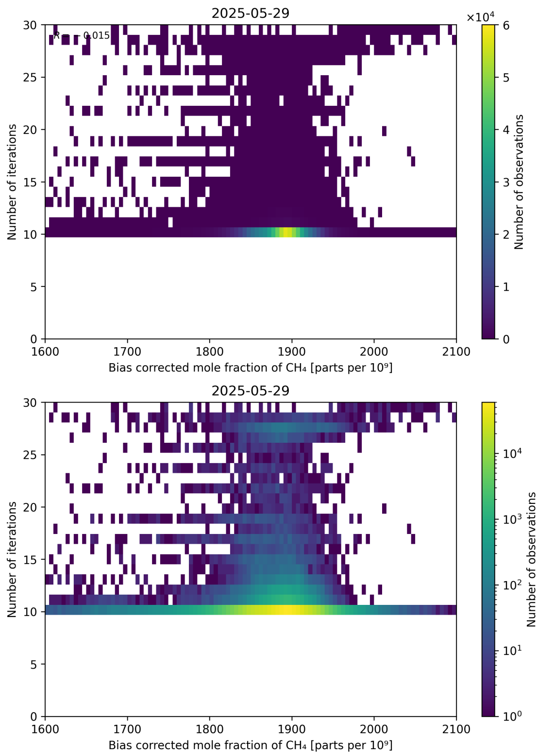
Figure 67: Scatter density plot of “Bias corrected mole fraction of CH 4 ” against “Number of iterations” for 2025-05-28 to 2025-05-30.
