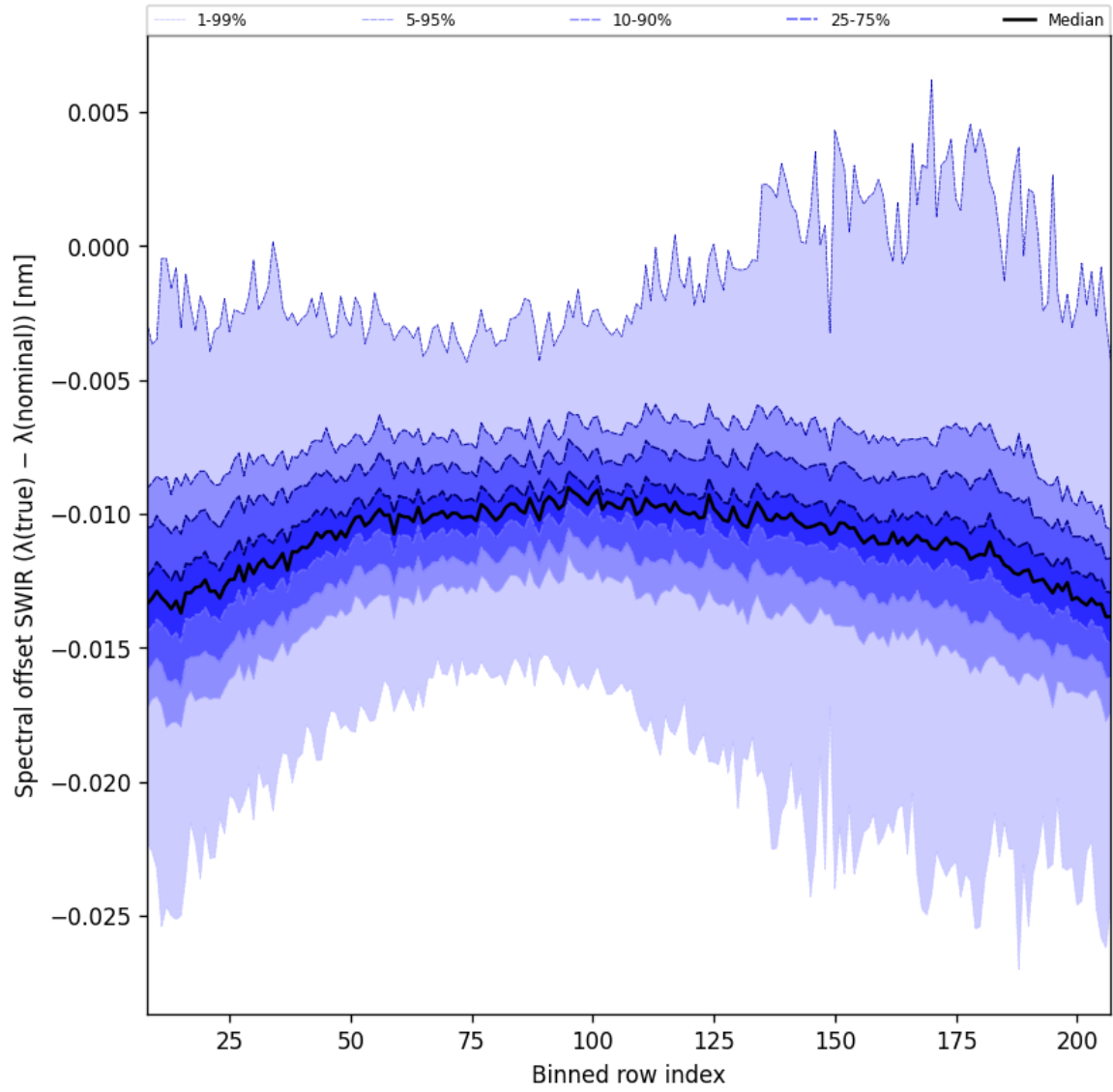
Figure 38: Along track statistics of “Spectral offset SWIR ( \lambda_{\text{true}} - \lambda_{\text{nominal}} )” for 2025-05-28 to 2025-05-30
