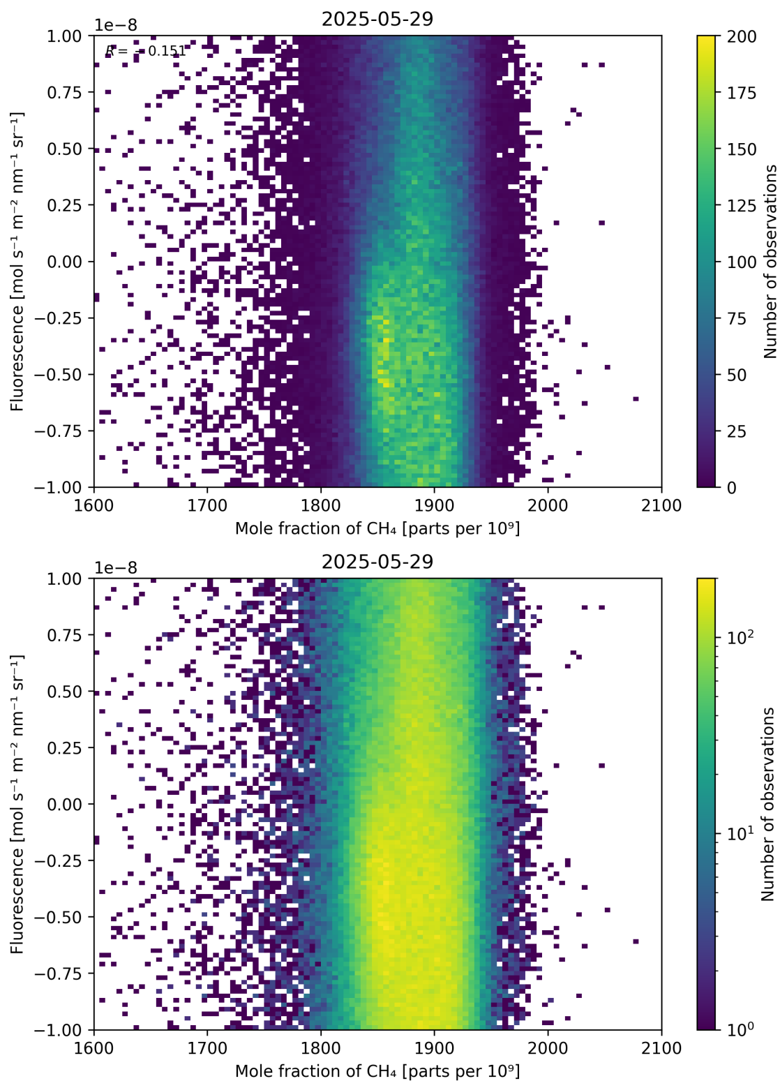
Figure 73: Scatter density plot of “Mole fraction of CH 4 ” against “Fluorescence” for 2025-05-28 to 2025-05-30.
