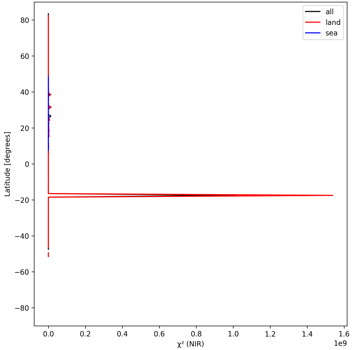
Figure 18: Zonal average of “ \chi^2 (NIR)” for 2025-05-28 to 2025-05-30.
