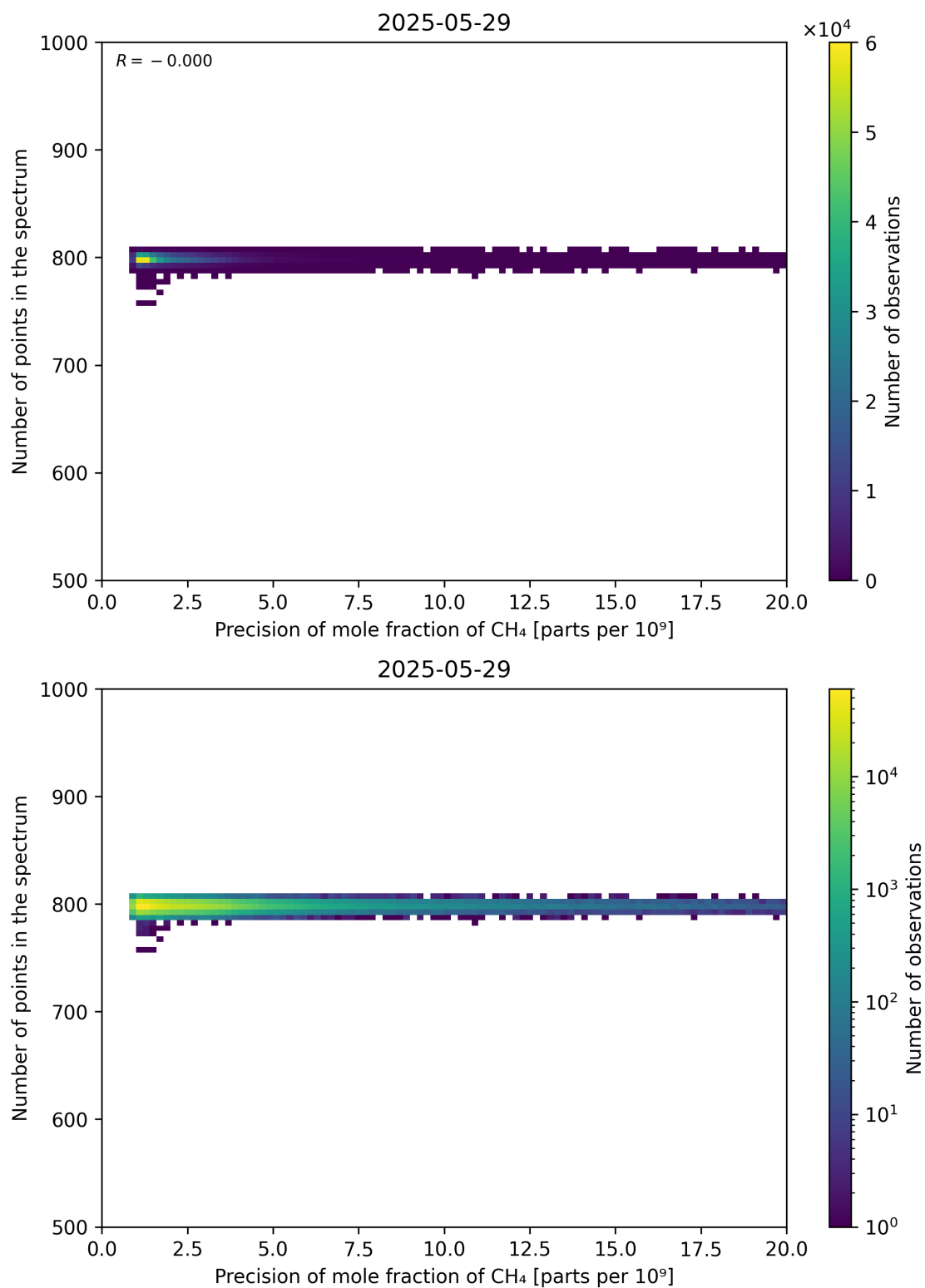
Figure 84: Scatter density plot of “Precision of mole fraction of CH 4 ” against “Number of points in the spectrum” for 2025-05-28 to 2025-05-30.
