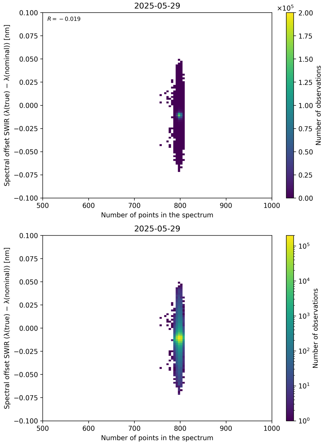
Figure 93: Scatter density plot of “Number of points in the spectrum” against “Spectral offset SWIR ( \lambda_{\text{true}} - \lambda_{\text{nominal}} )” for 2025-05-28 to 2025-05-30.
