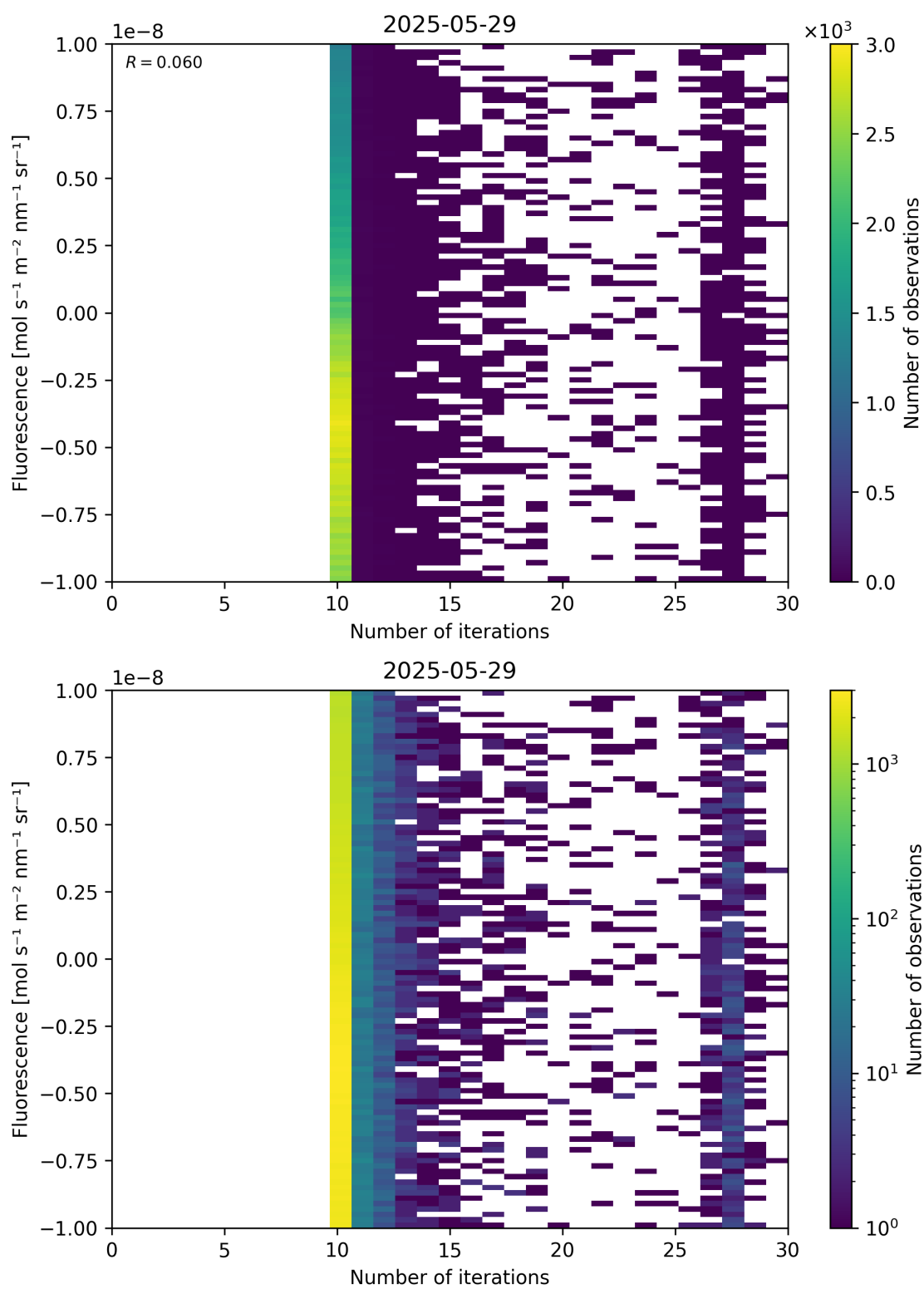
Figure 87: Scatter density plot of "Number of iterations" against "Fluorescence" for 2025-05-28 to 2025-05-30.
