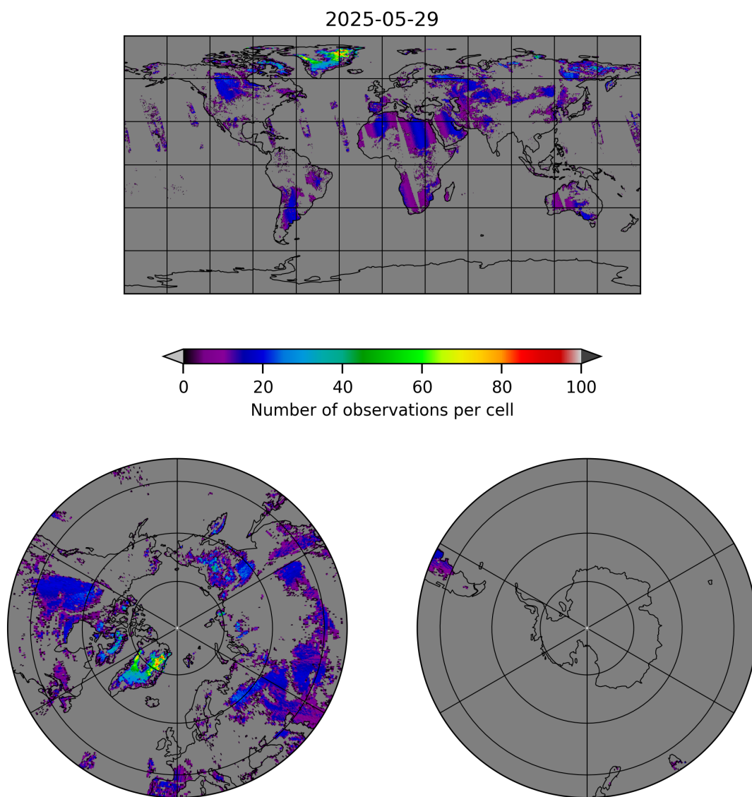
Figure 10: Map of the number of observations for 2025-05-28 to 2025-05-30
