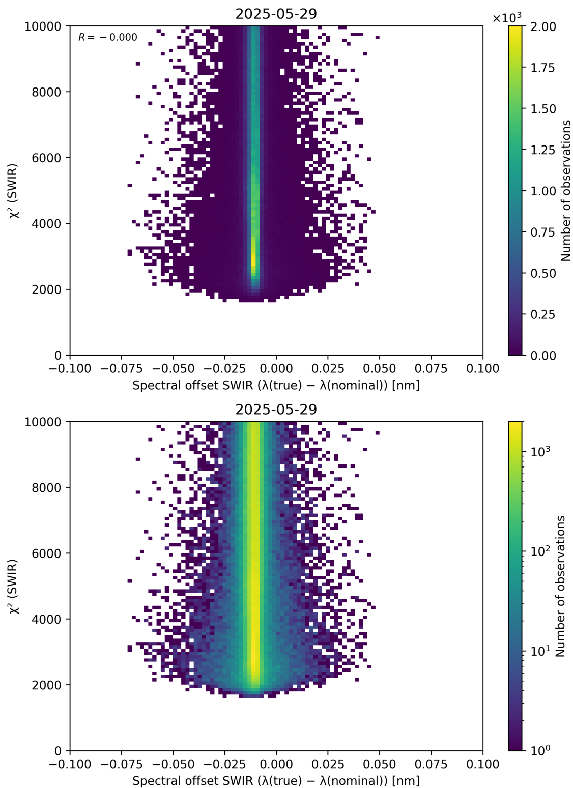
Figure 118: Scatter density plot of “Spectral offset SWIR ( \lambda_{\text{true}} - \lambda_{\text{nominal}} )” against “ \chi^2 (SWIR)” for 2025-05-28 to 2025-05-30.
