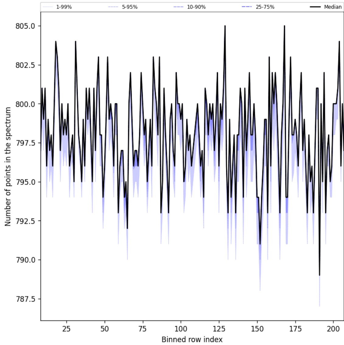
Figure 37: Along track statistics of “Number of points in the spectrum” for 2025-05-28 to 2025-05-30
