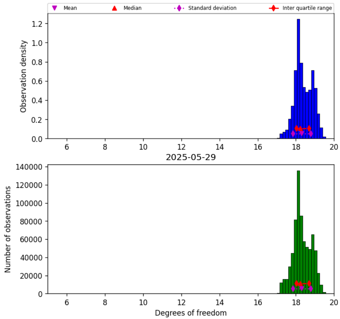
Figure 30: Histogram of “Degrees of freedom” for 2025-05-28 to 2025-05-30
