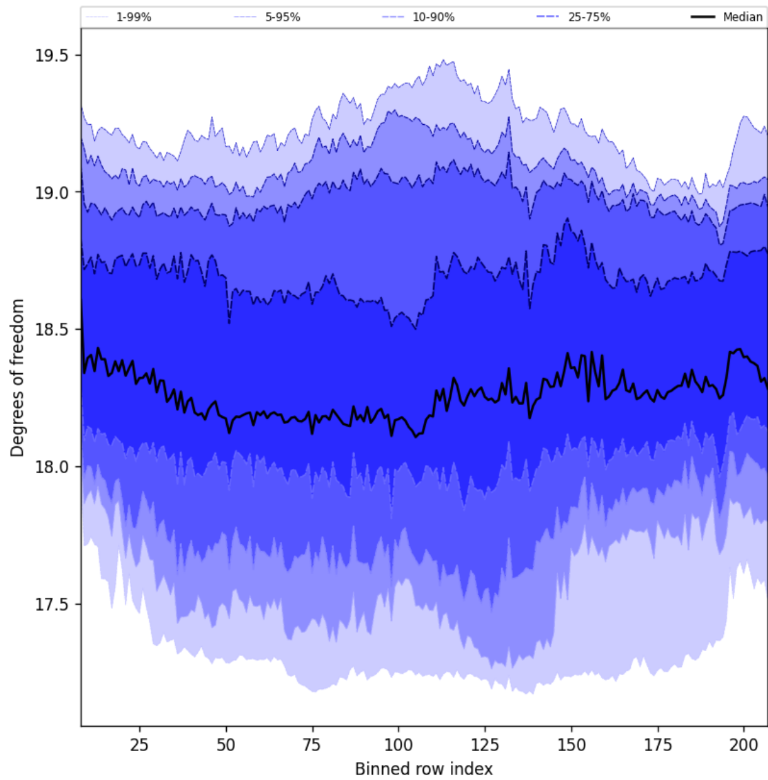
Figure 41: Along track statistics of “Degrees of freedom” for 2025-05-28 to 2025-05-30
