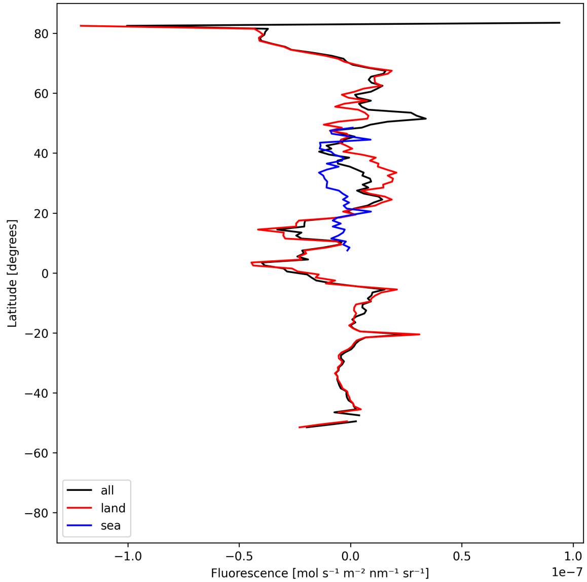
Figure 21: Zonal average of “Fluorescence” for 2025-05-28 to 2025-05-30.
