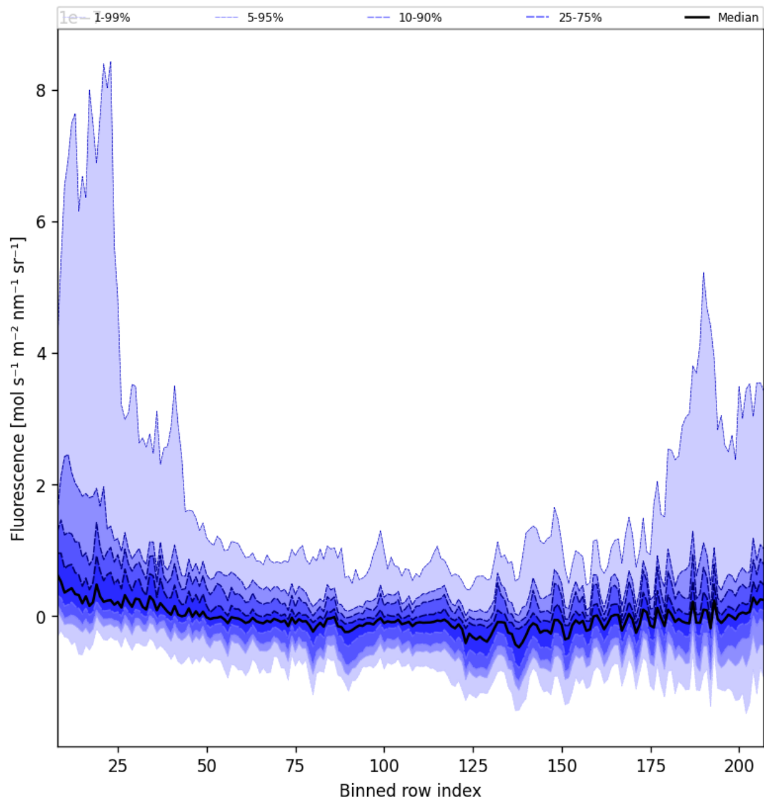
Figure 43: Along track statistics of “Fluorescence” for 2025-05-28 to 2025-05-30
