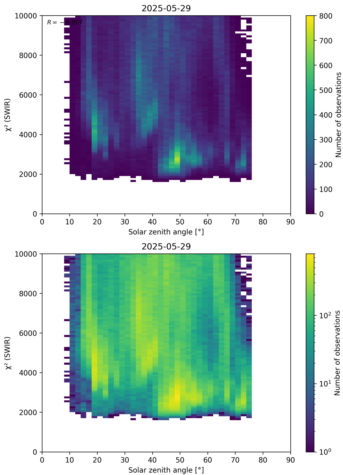
Figure 95: Scatter density plot of “Solar zenith angle” against “ \chi^2 (SWIR)” for 2025-05-28 to 2025-05-30.
