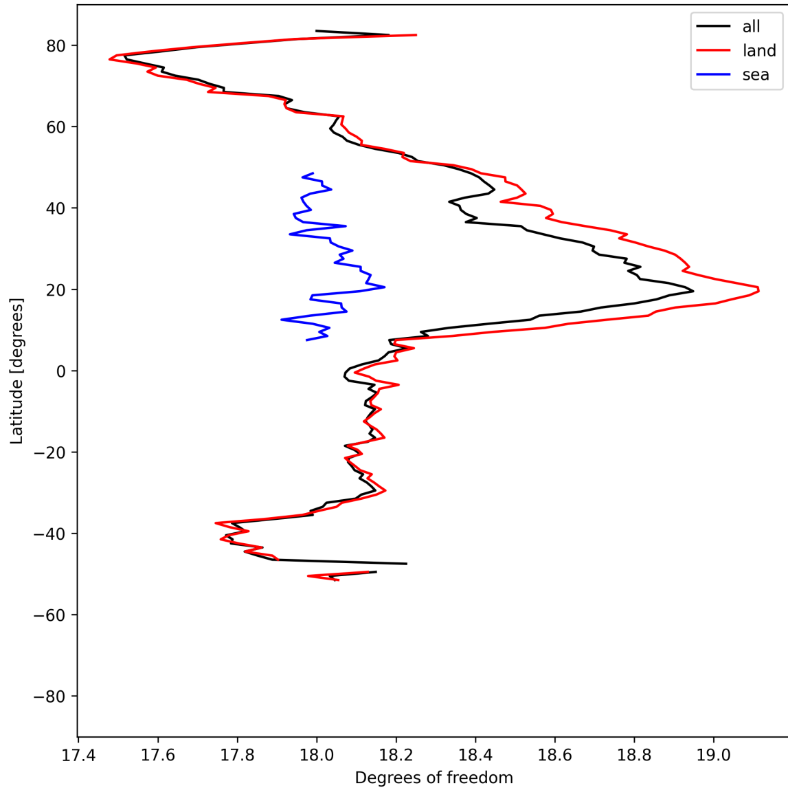
Figure 19: Zonal average of “Degrees of freedom” for 2025-05-28 to 2025-05-30.
