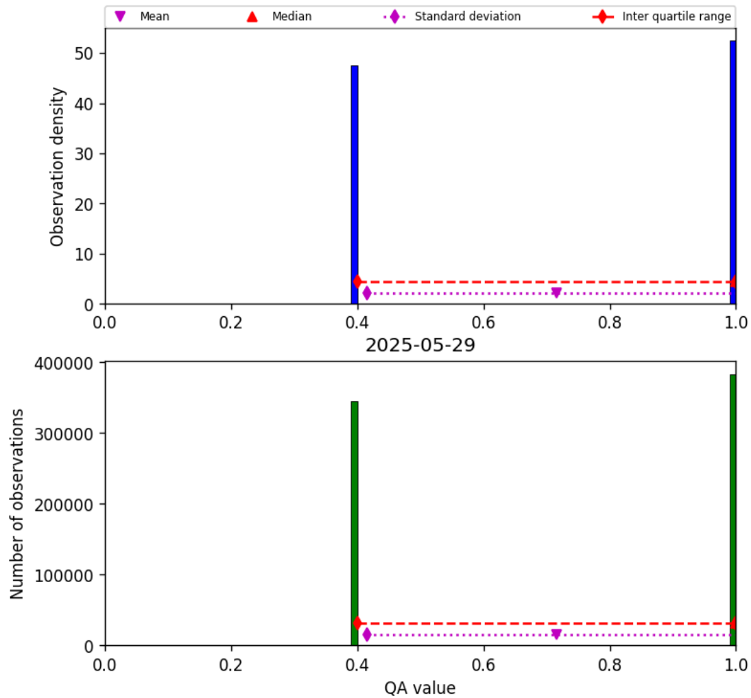
Figure 22: Histogram of “QA value” for 2025-05-28 to 2025-05-30
