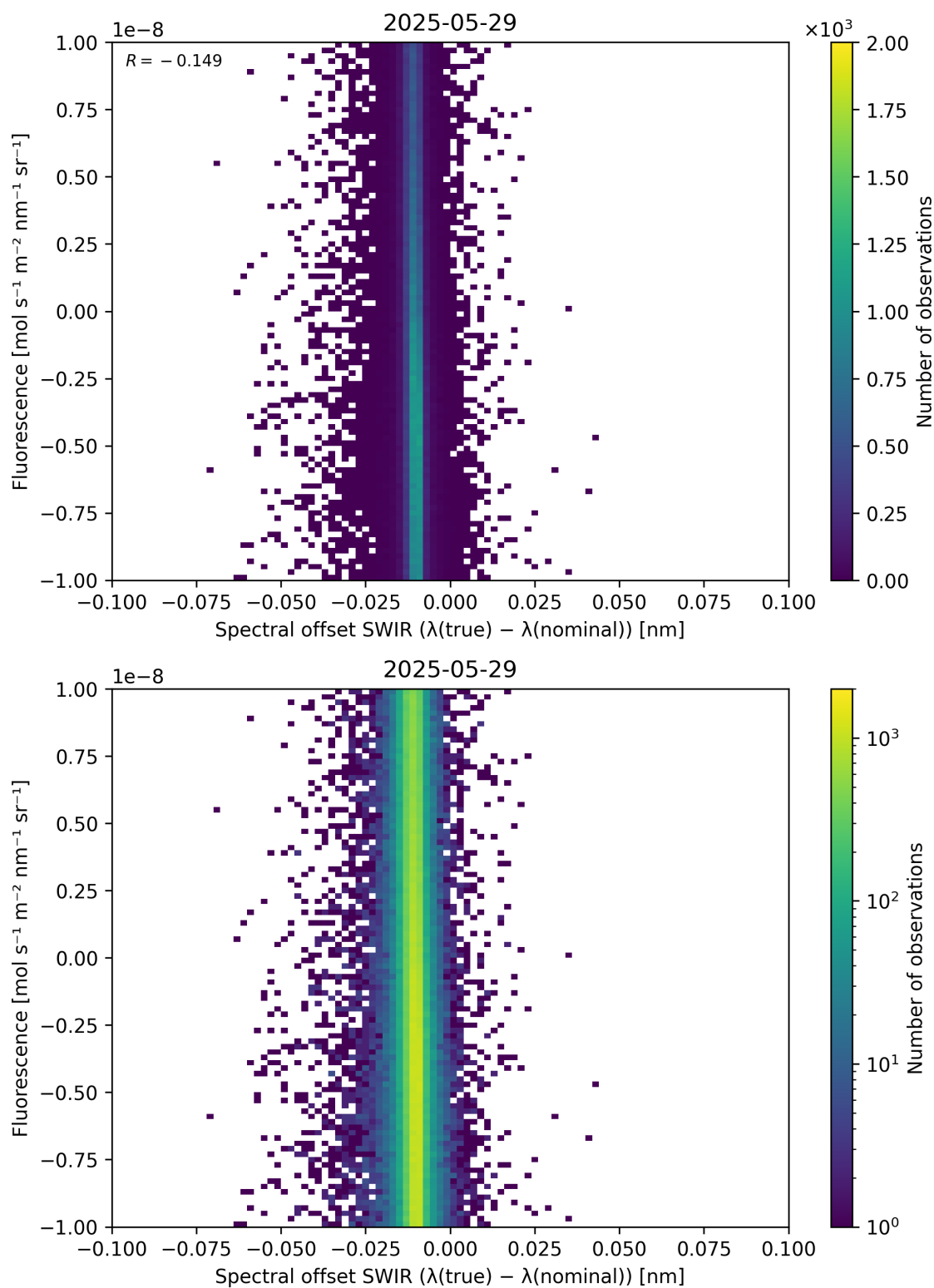
Figure 120: Scatter density plot of “Spectral offset SWIR ( \lambda_{\text{true}} - \lambda_{\text{nominal}} )” against “Fluorescence” for 2025-05-28 to 2025-05-30.
