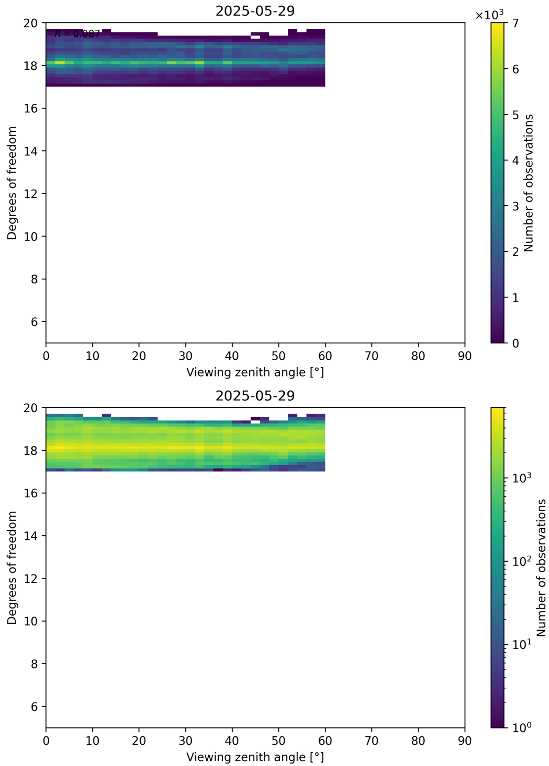
Figure 107: Scatter density plot of “Viewing zenith angle” against “Degrees of freedom” for 2025-05-28 to 2025-05-30.
