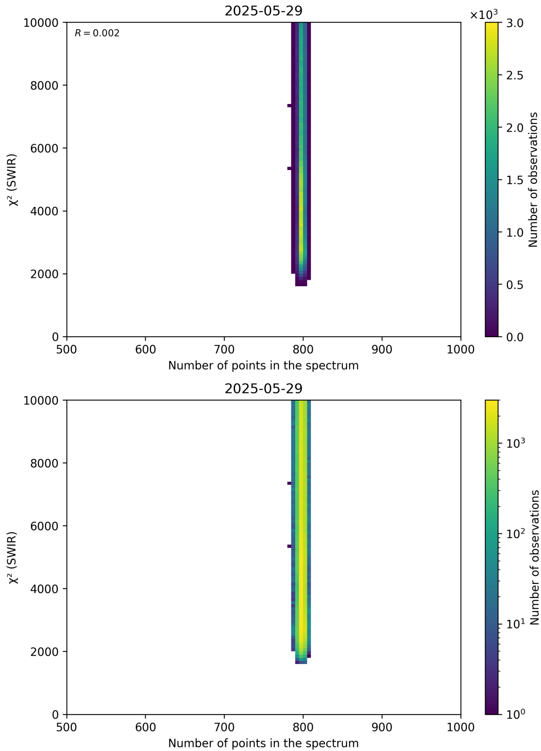
Figure 89: Scatter density plot of “Number of points in the spectrum” against “ \chi^2 (SWIR)” for 2025-05-28 to 2025-05-30.
