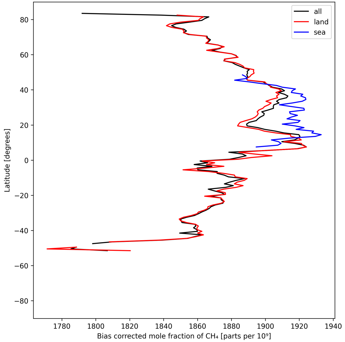
Figure 14: Zonal average of “Bias corrected mole fraction of CH 4 ” for 2025-05-28 to 2025-05-30.
