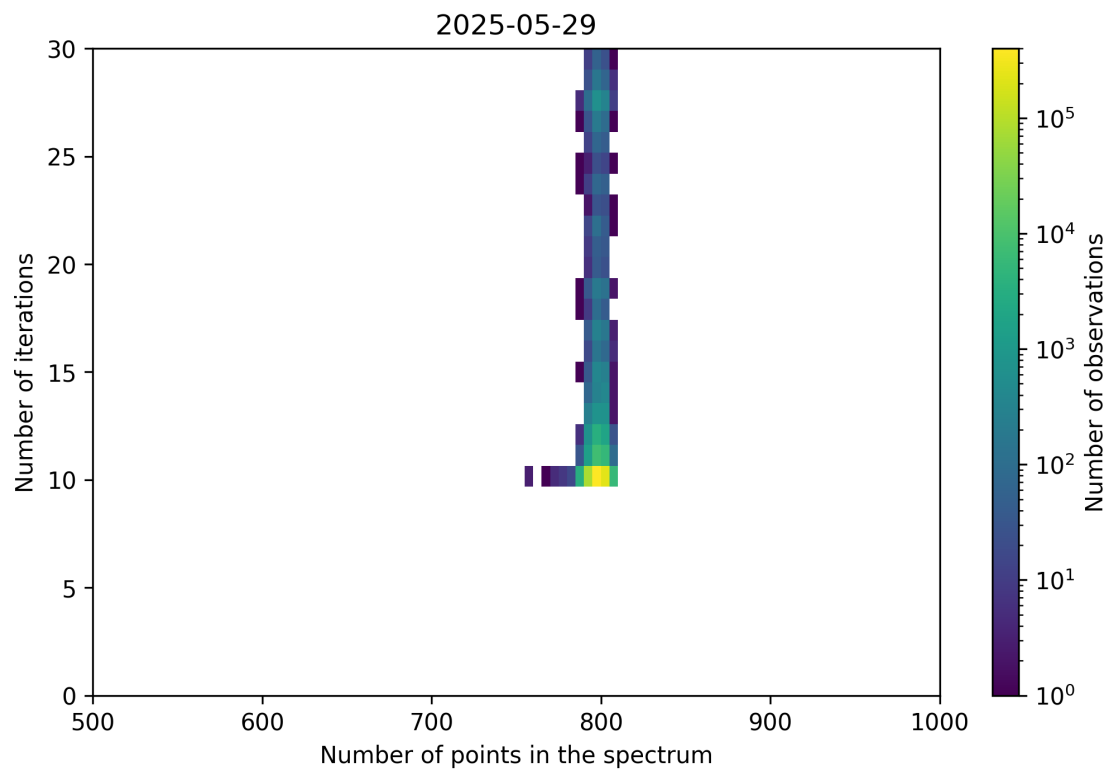
Figure 92: Scatter density plot of “Number of points in the spectrum” against “Number of iterations” for 2025-05-28 to 2025-05-30.
