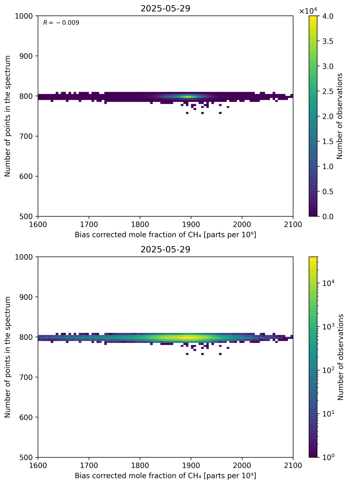
Figure 68: Scatter density plot of “Bias corrected mole fraction of CH 4 ” against “Number of points in the spectrum” for 2025-05-28 to 2025-05-30.
