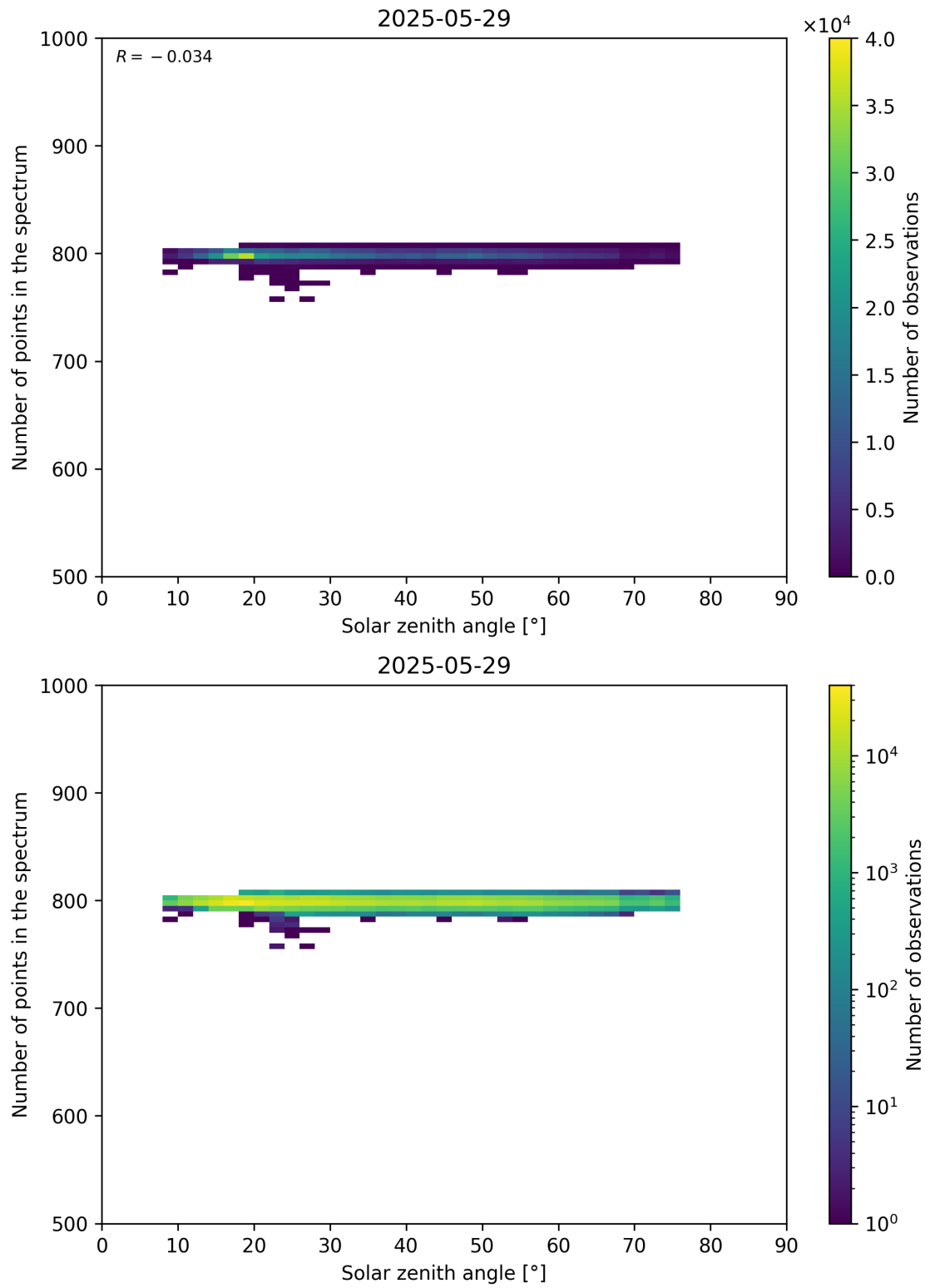
Figure 103: Scatter density plot of “Solar zenith angle” against “Number of points in the spectrum” for 2025-05-28 to 2025-05-30.
