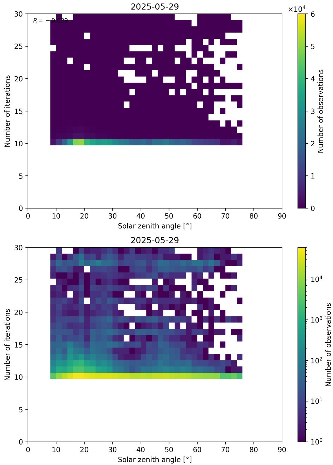
Figure 102: Scatter density plot of “Solar zenith angle” against “Number of iterations” for 2025-05-28 to 2025-05-30.
