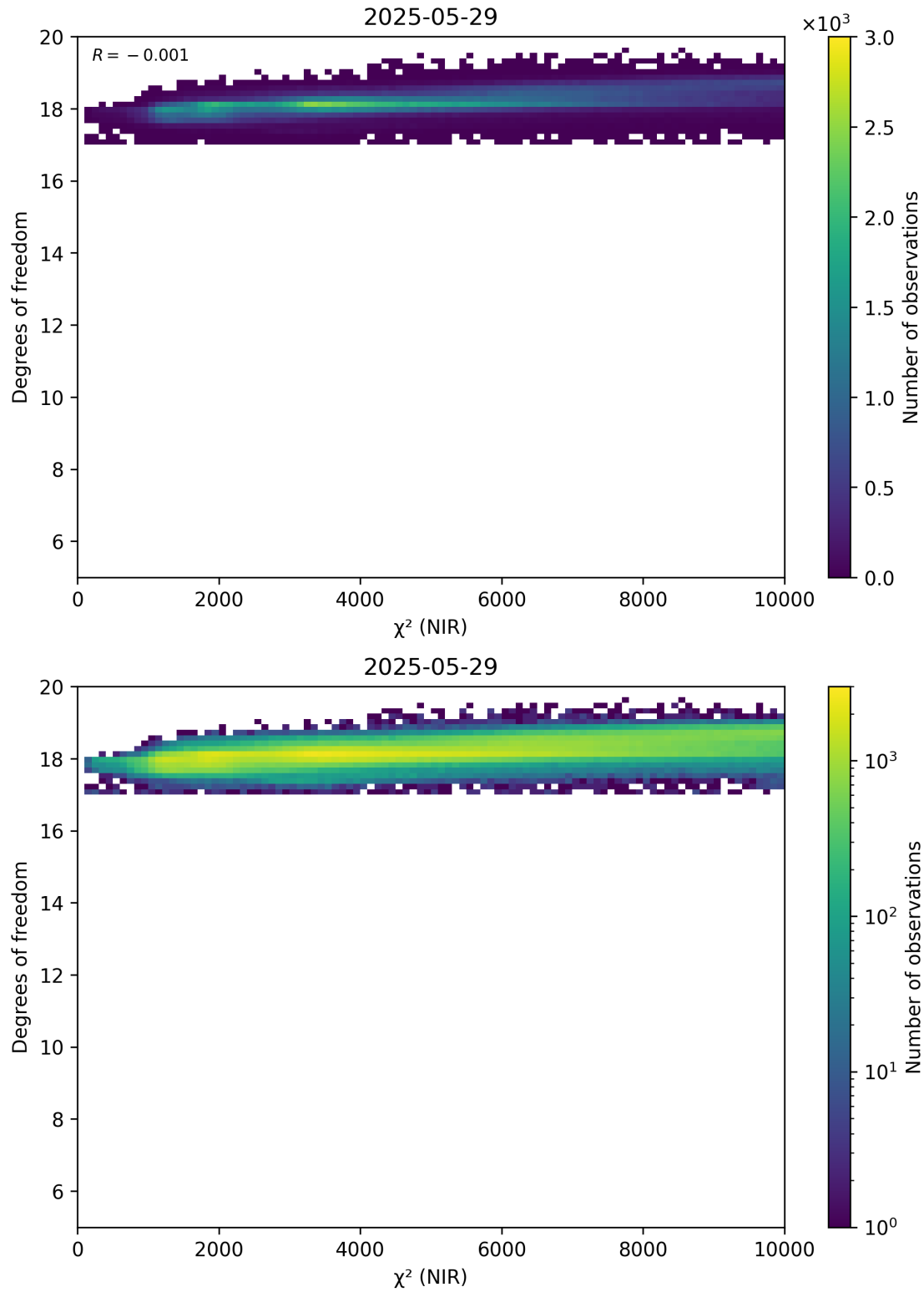
Figure 44: Scatter density plot of “ \chi^2 (NIR)” against “Degrees of freedom” for 2025-05-28 to 2025-05-30.
