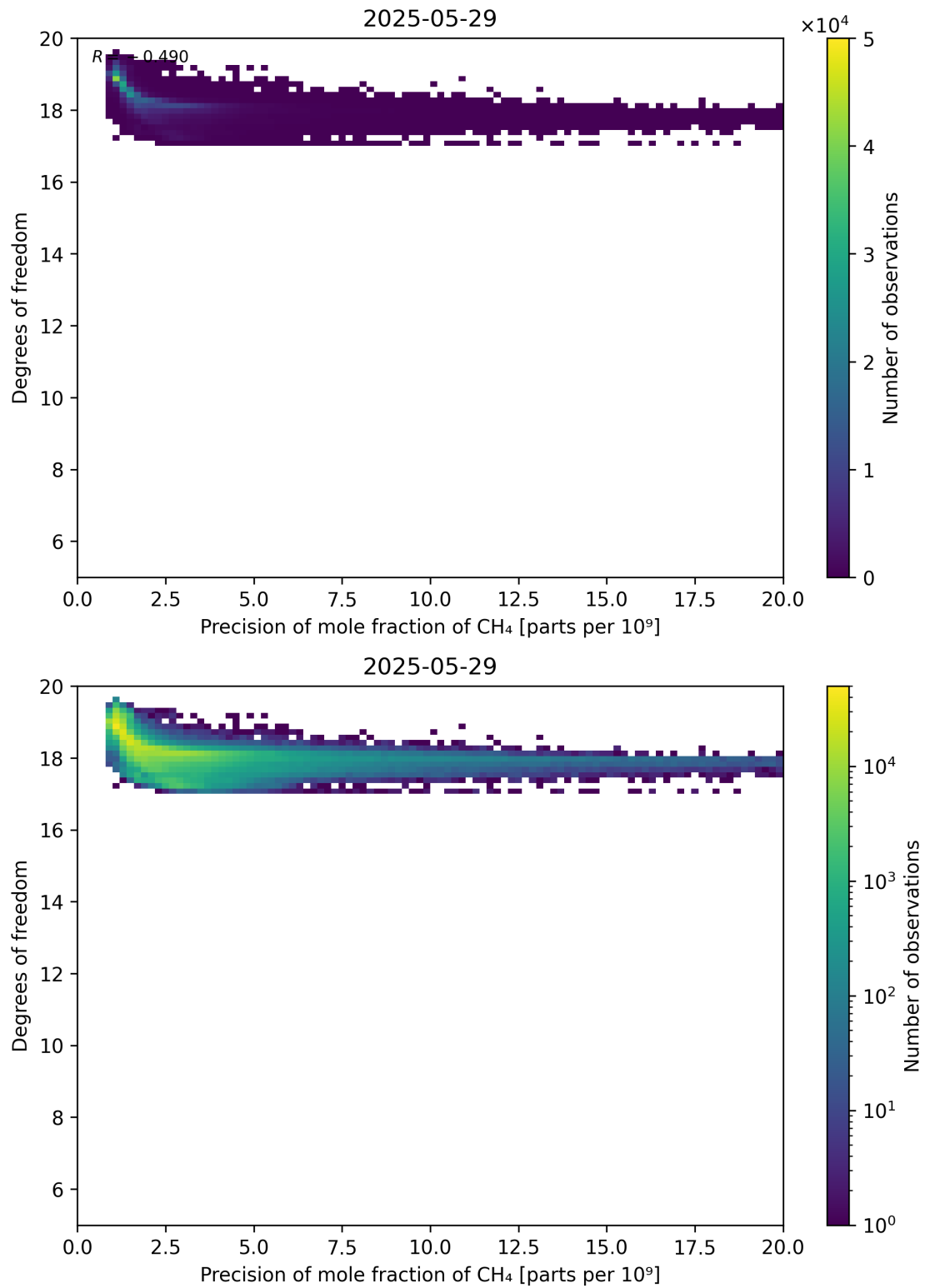
Figure 80: Scatter density plot of “Precision of mole fraction of CH 4 ” against “Degrees of freedom” for 2025-05-28 to 2025-05-30.
