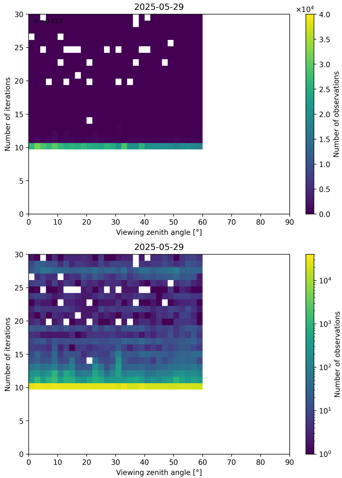
Figure 113: Scatter density plot of “Viewing zenith angle” against “Number of iterations” for 2025-05-28 to 2025-05-30.
