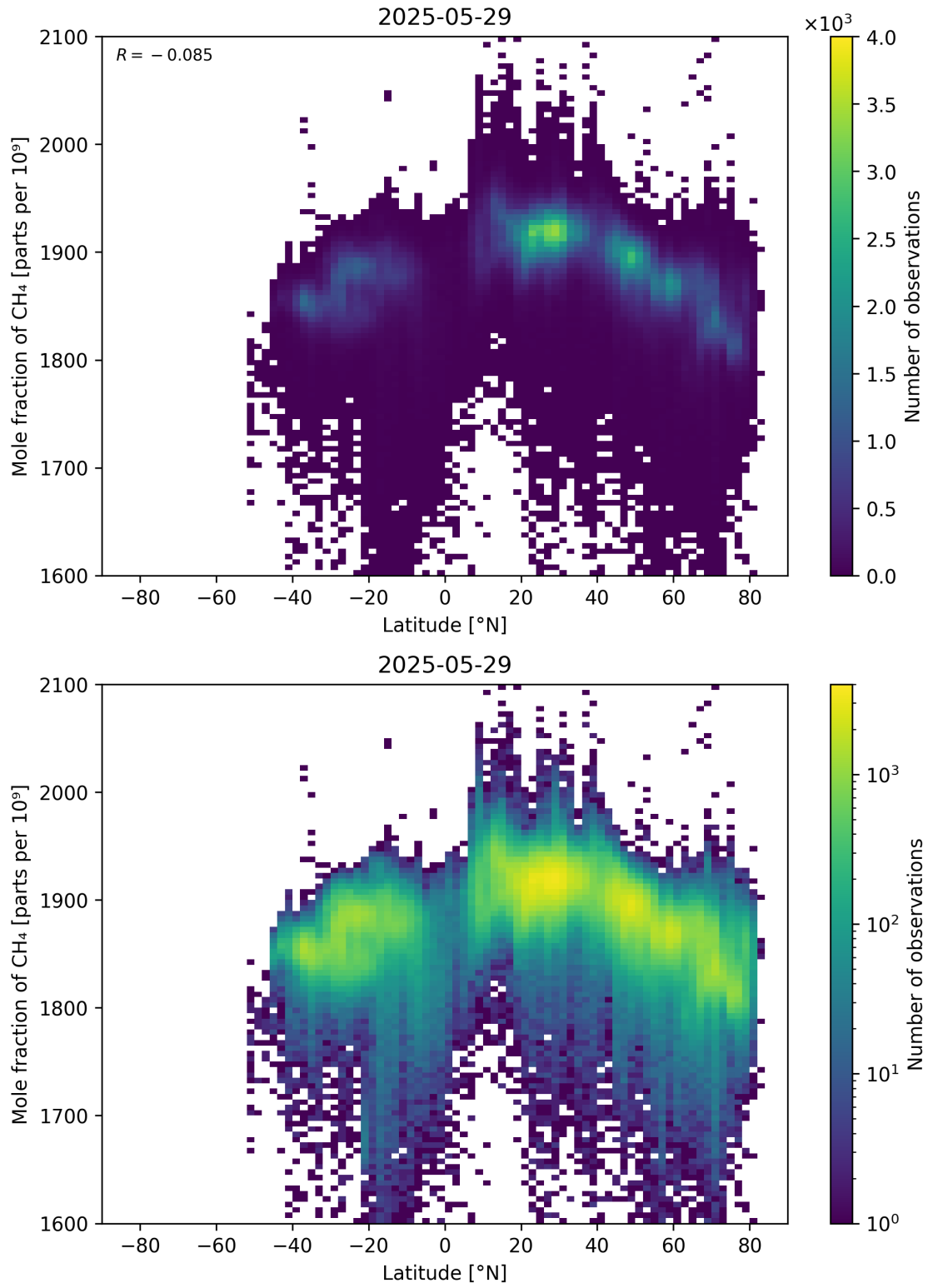
Figure 57: Scatter density plot of “Latitude” against “Mole fraction of CH 4 ” for 2025-05-28 to 2025-05-30.
