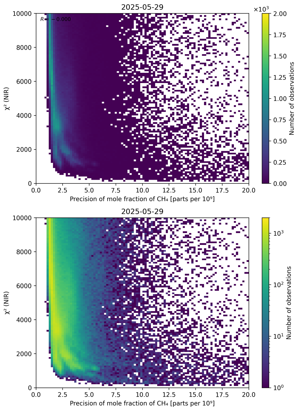
Figure 78: Scatter density plot of “Precision of mole fraction of CH 4 ” against “ \chi^2 (NIR)” for 2025-05-28 to 2025-05-30.
