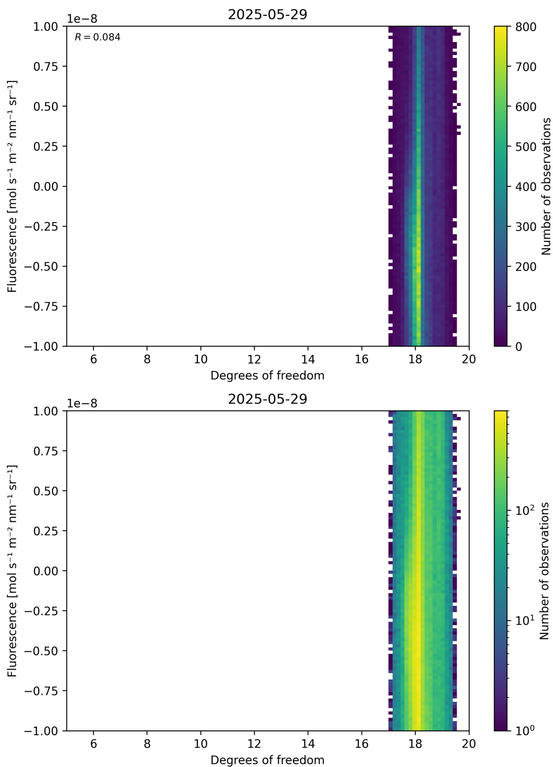
Figure 51: Scatter density plot of “Degrees of freedom” against “Fluorescence” for 2025-05-28 to 2025-05-30.
