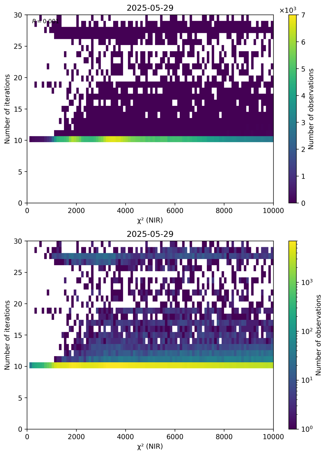
Figure 46: Scatter density plot of “ \chi^2 (NIR)” against “Number of iterations” for 2025-05-28 to 2025-05-30.
