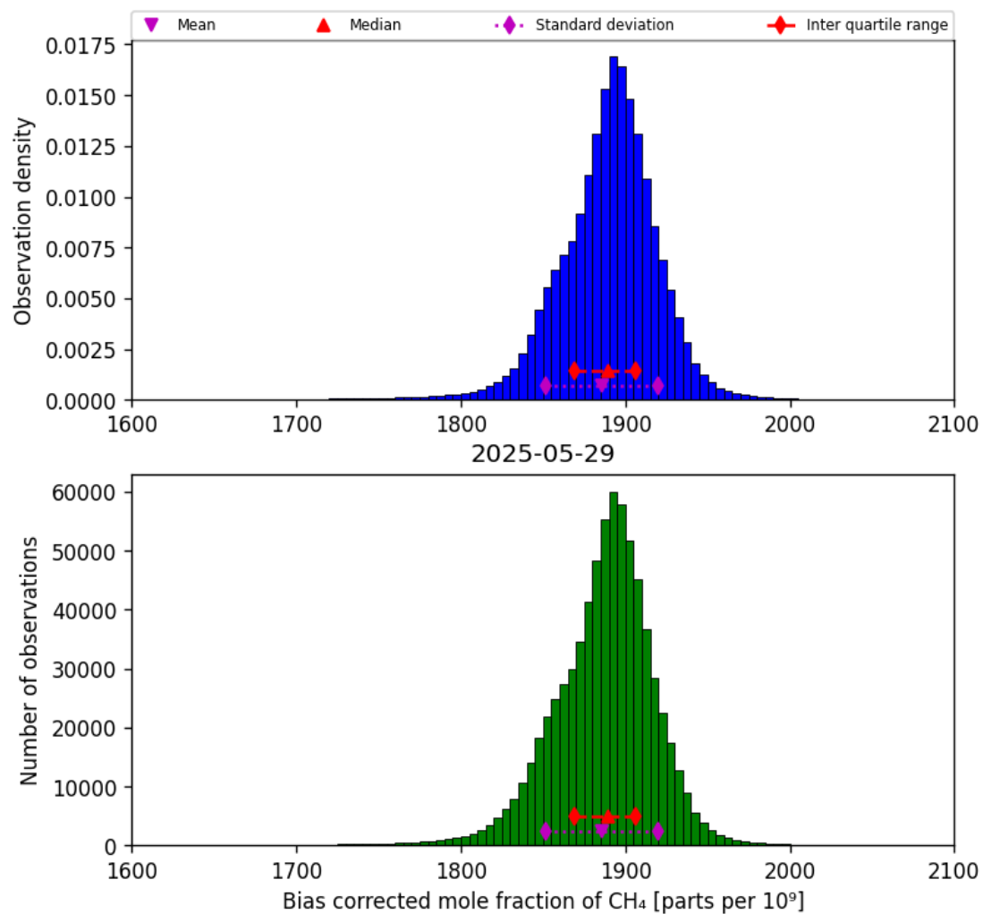
Figure 25: Histogram of “Bias corrected mole fraction of CH 4 ” for 2025-05-28 to 2025-05-30
