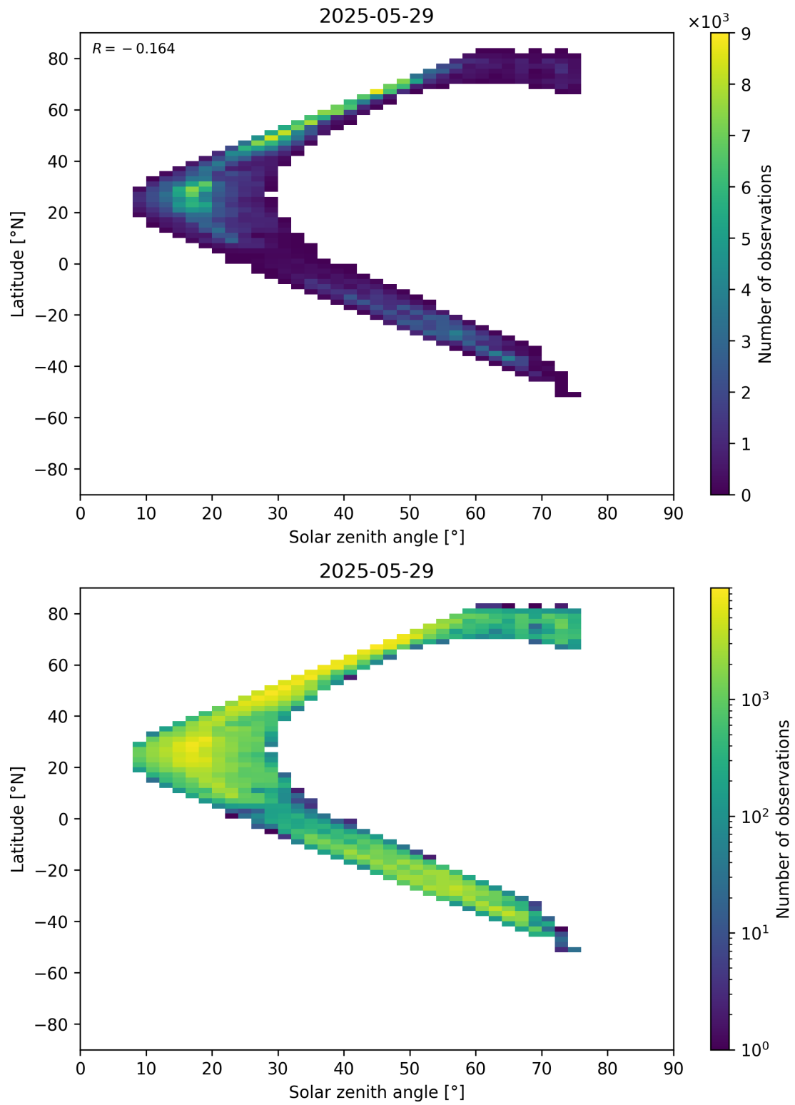
Figure 98: Scatter density plot of “Solar zenith angle” against “Latitude” for 2025-05-28 to 2025-05-30.
