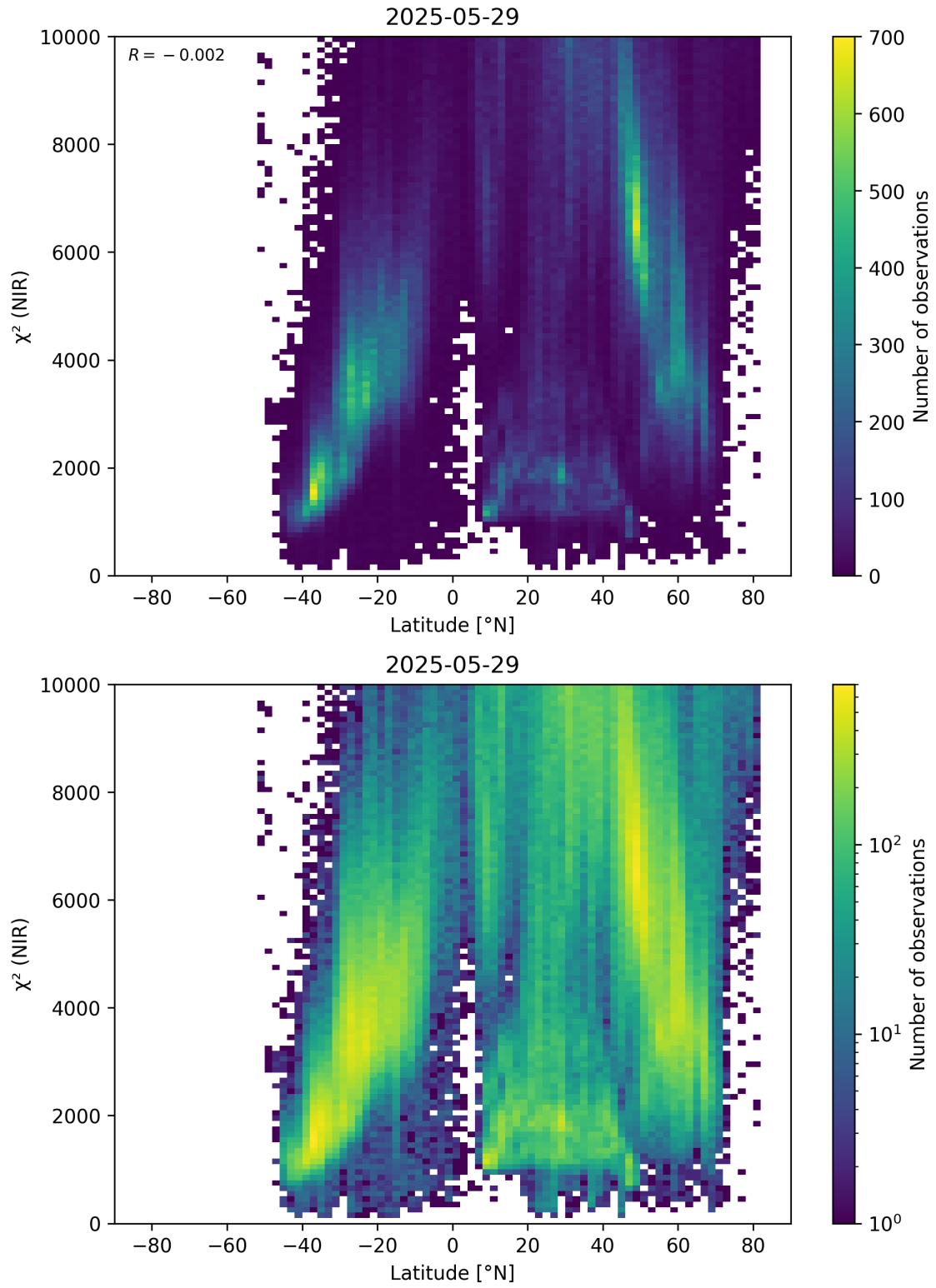
Figure 53: Scatter density plot of “Latitude” against “ \chi^2 (NIR)” for 2025-05-28 to 2025-05-30.
