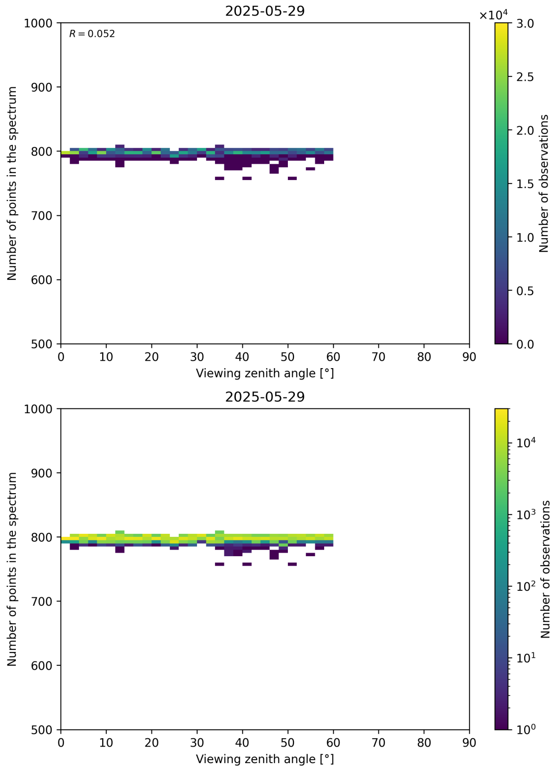
Figure 114: Scatter density plot of “Viewing zenith angle” against “Number of points in the spectrum” for 2025-05-28 to 2025-05-30.
