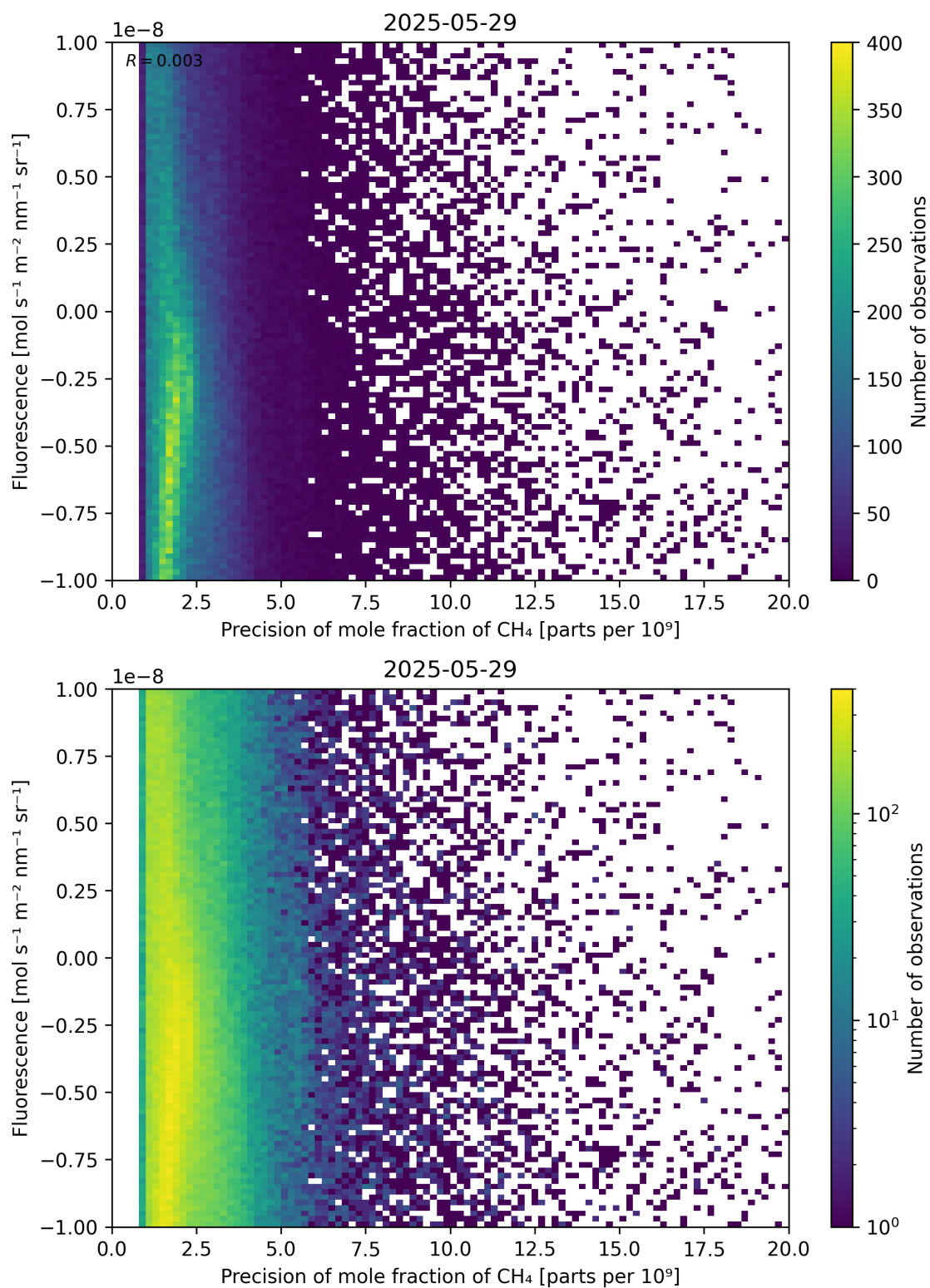
Figure 81: Scatter density plot of “Precision of mole fraction of CH 4 ” against “Fluorescence” for 2025-05-28 to 2025-05-30.
