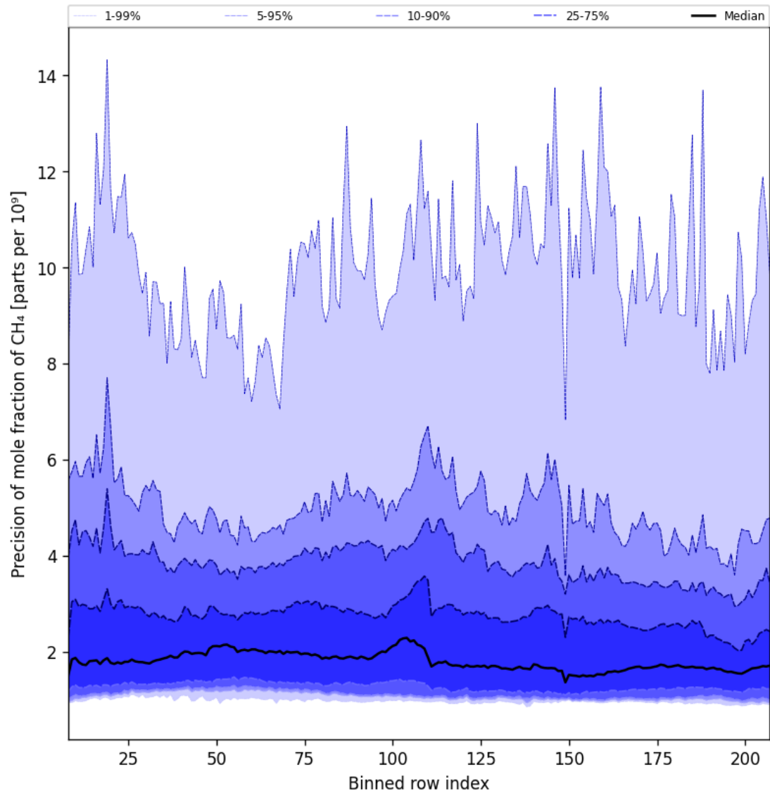
Figure 35: Along track statistics of “Precision of mole fraction of CH 4 ” for 2025-05-28 to 2025-05-30
