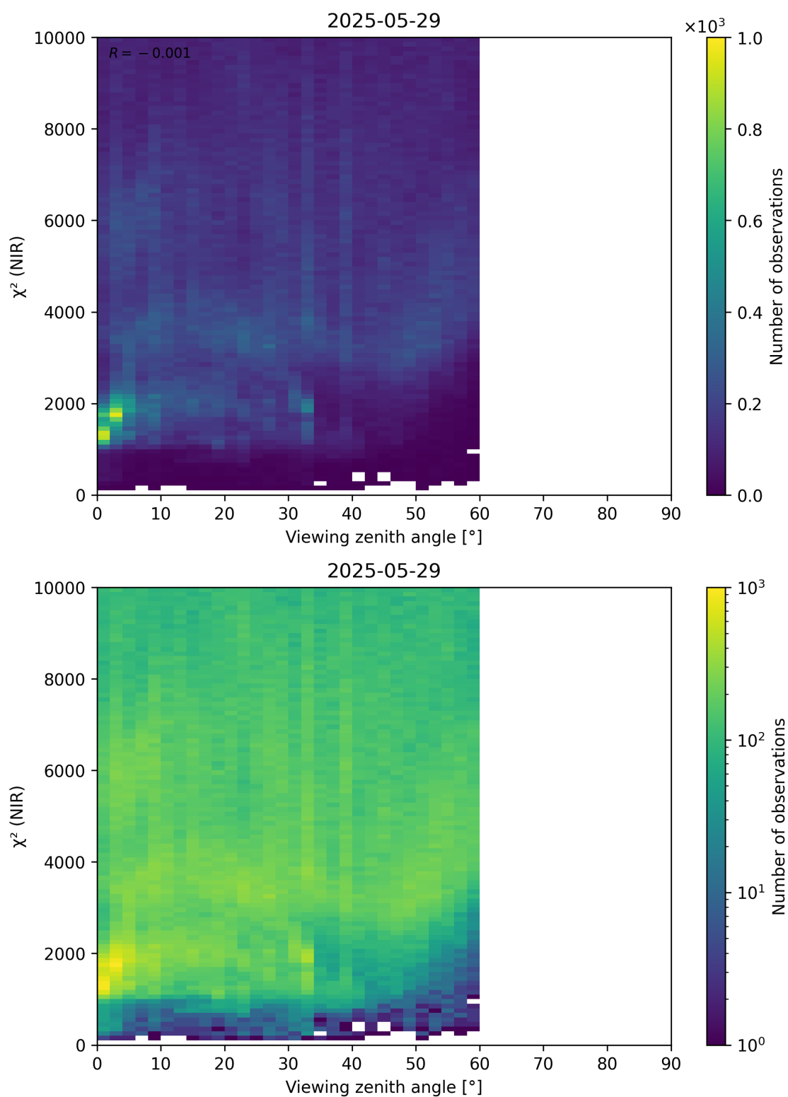
Figure 105: Scatter density plot of “Viewing zenith angle” against “ \chi^2 (NIR)” for 2025-05-28 to 2025-05-30.
