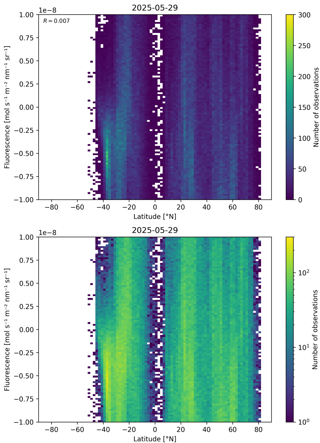
Figure 56: Scatter density plot of “Latitude” against “Fluorescence” for 2025-05-28 to 2025-05-30.
