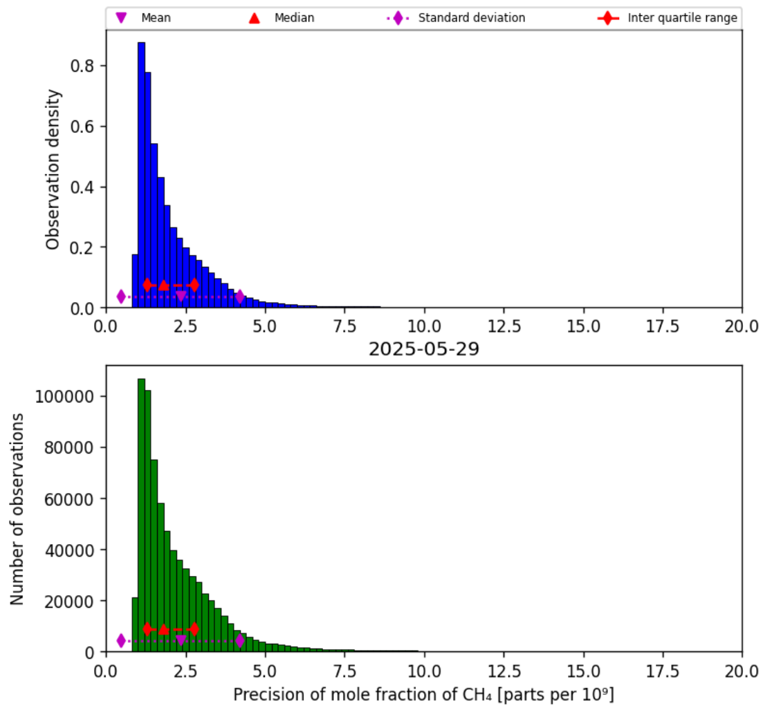
Figure 24: Histogram of “Precision of mole fraction of CH 4 ” for 2025-05-28 to 2025-05-30
