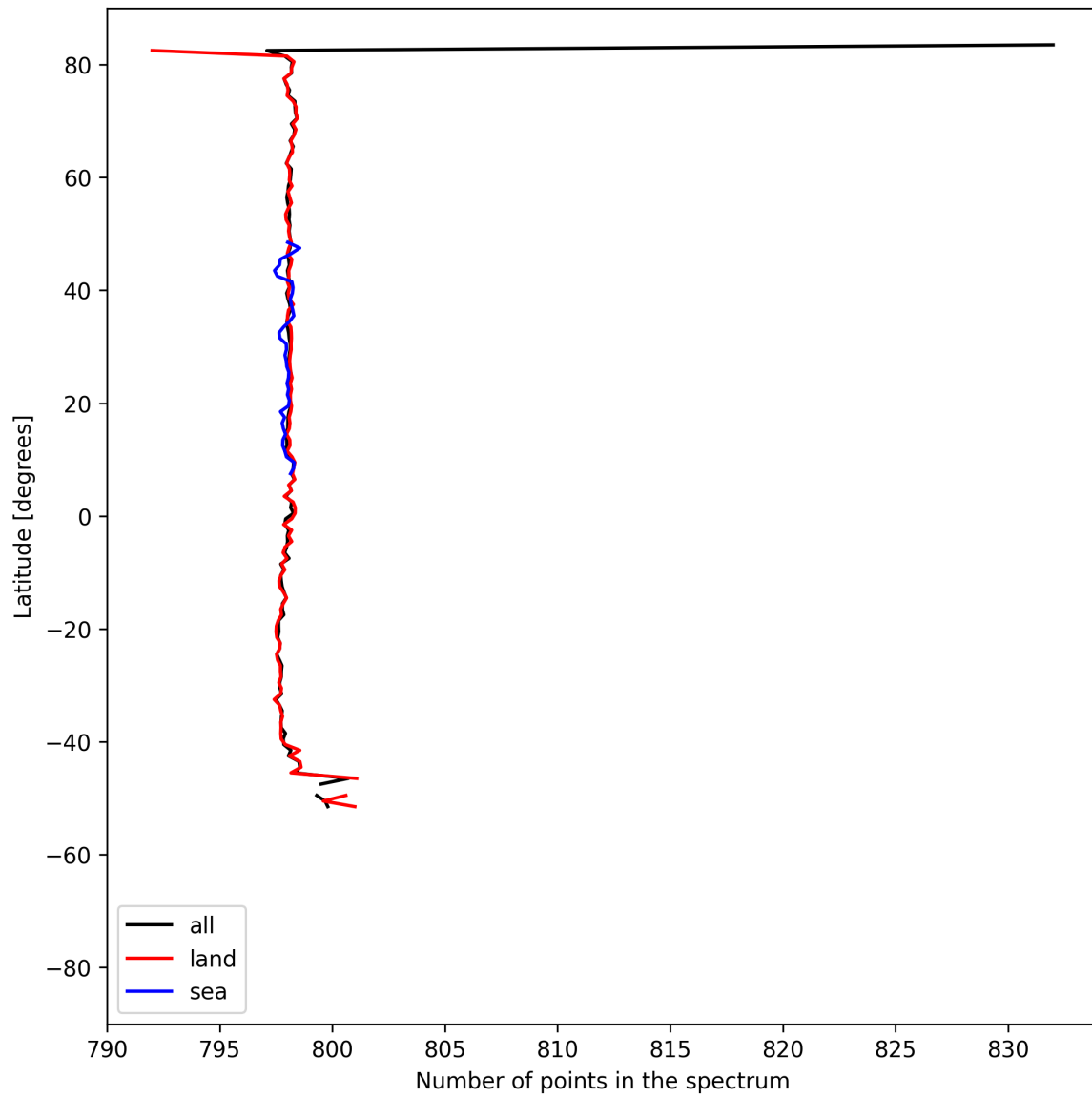
Figure 15: Zonal average of “Number of points in the spectrum” for 2025-05-28 to 2025-05-30.
