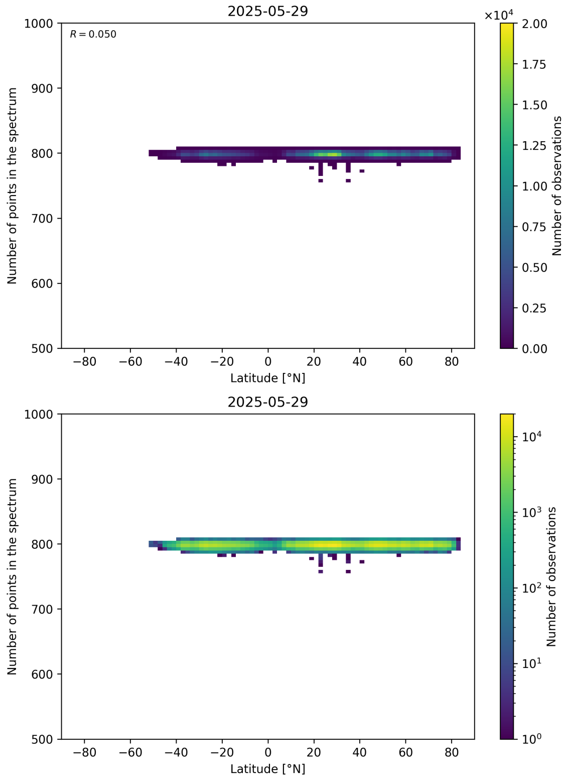
Figure 61: Scatter density plot of “Latitude” against “Number of points in the spectrum” for 2025-05-28 to 2025-05-30.
