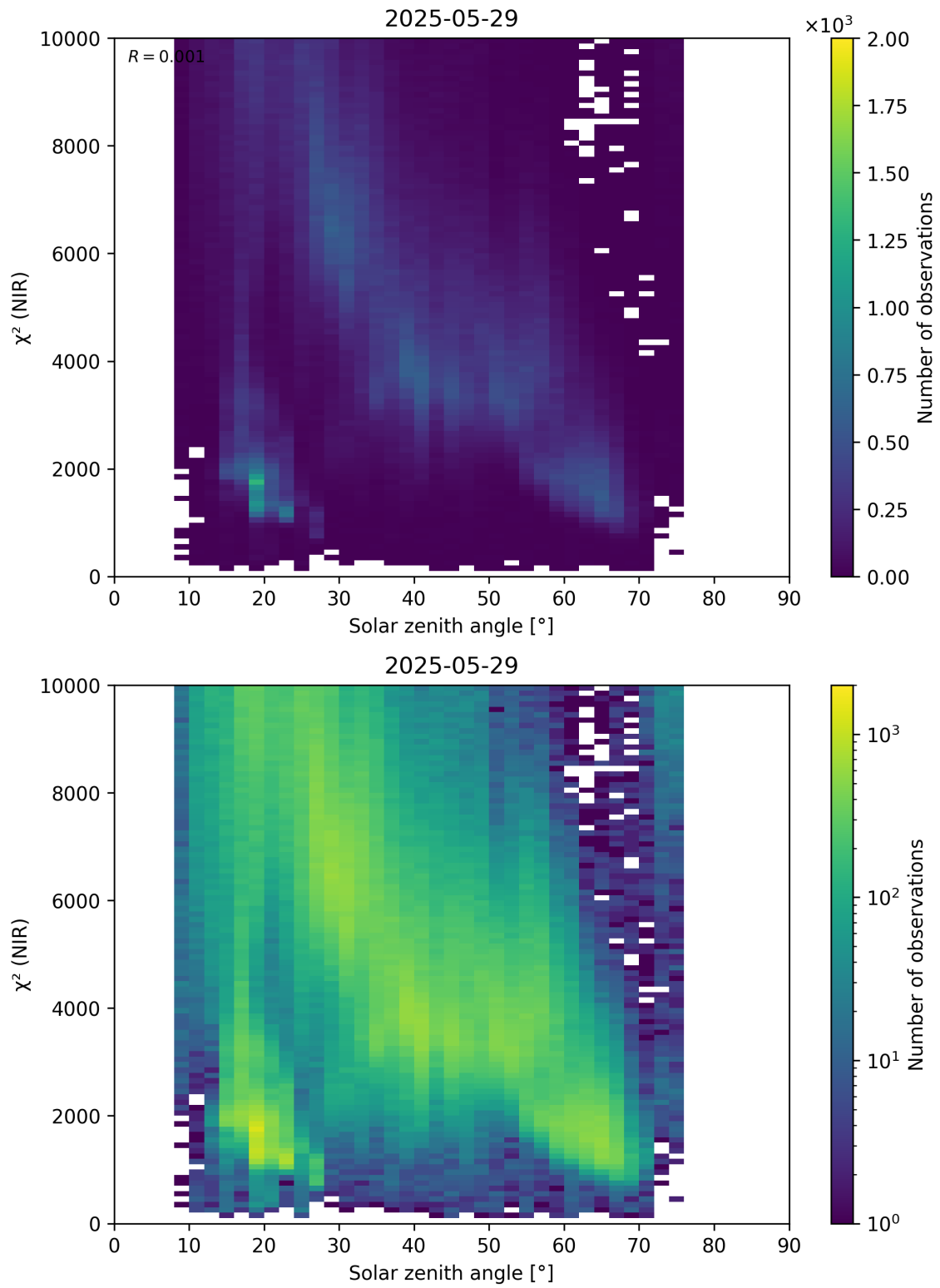
Figure 94: Scatter density plot of “Solar zenith angle” against “ \chi^2 (NIR)” for 2025-05-28 to 2025-05-30.
