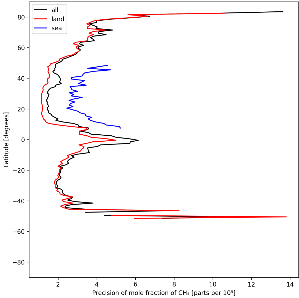
Figure 13: Zonal average of “Precision of mole fraction of CH 4 ” for 2025-05-28 to 2025-05-30.
