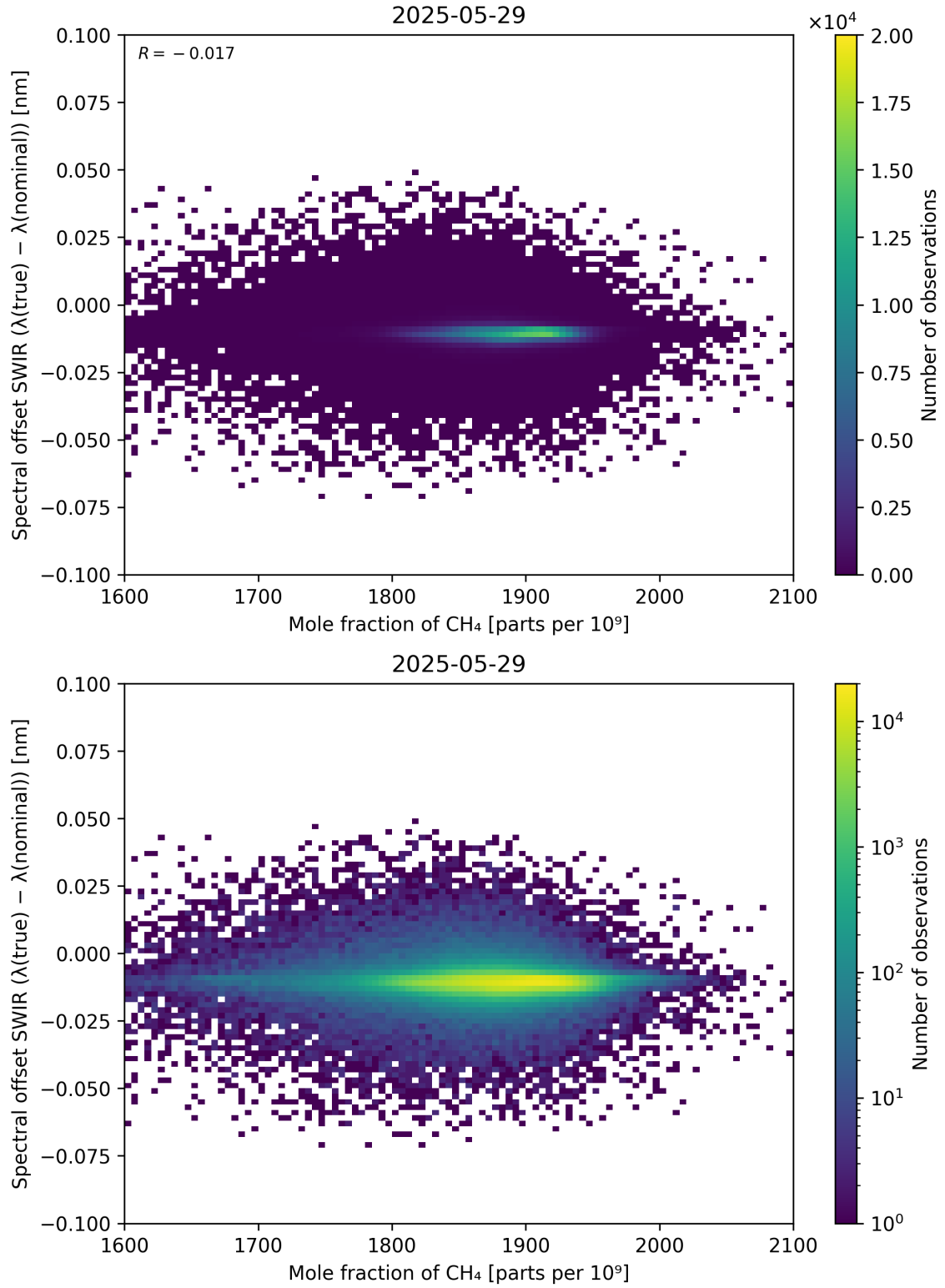
Figure 86: Scatter density plot of “Mole fraction of \text{CH}_4 ” against “Spectral offset SWIR ( \lambda_{\text{true}} - \lambda_{\text{nominal}} )” for 2025-05-28 to 2025-05-30.
