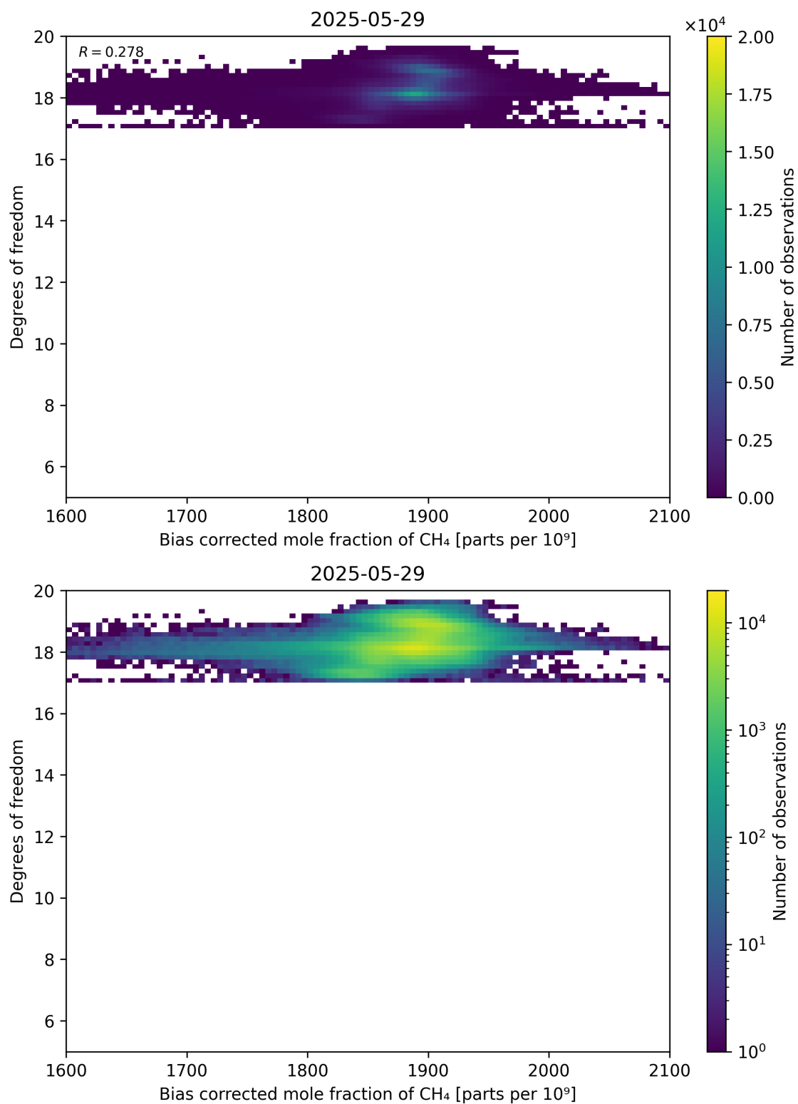
Figure 65: Scatter density plot of “Bias corrected mole fraction of CH 4 ” against “Degrees of freedom” for 2025-05-28 to 2025-05-30.
