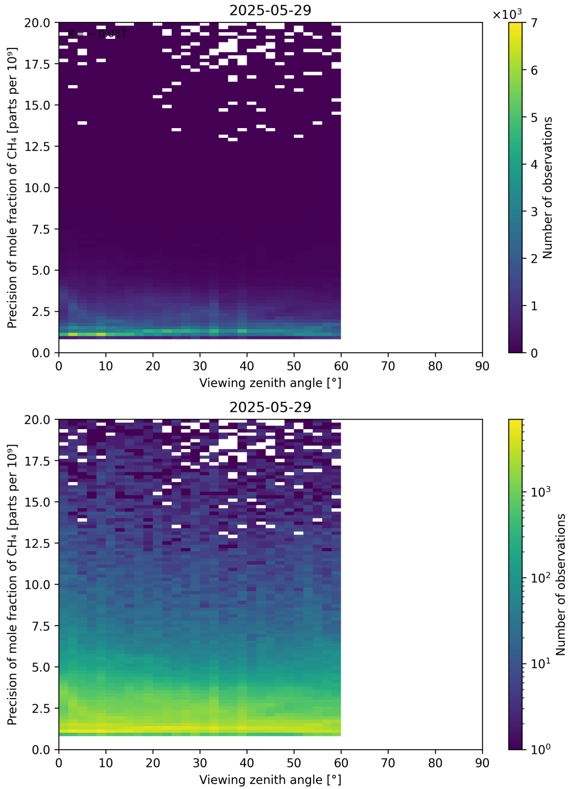
Figure 112: Scatter density plot of “Viewing zenith angle” against “Precision of mole fraction of CH 4 ” for 2025-05-28 to 2025-05-30.
