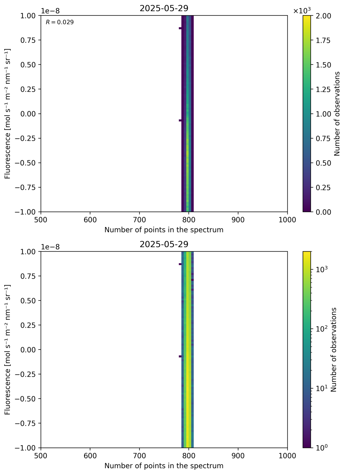
Figure 91: Scatter density plot of “Number of points in the spectrum” against “Fluorescence” for 2025-05-28 to 2025-05-30.
