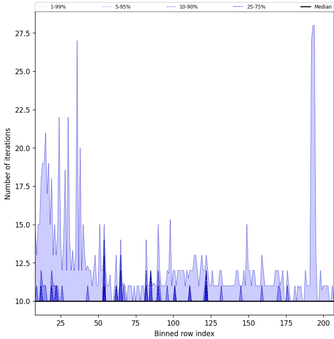
Figure 42: Along track statistics of “Number of iterations” for 2025-05-28 to 2025-05-30
