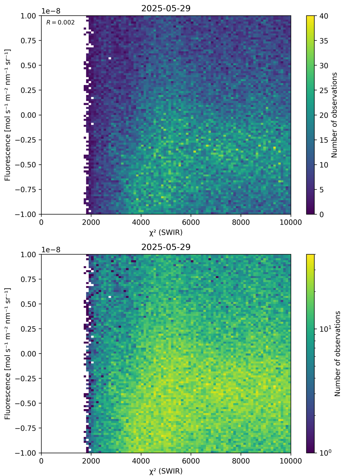
Figure 49: Scatter density plot of “ \chi^2 (SWIR)” against “Fluorescence” for 2025-05-28 to 2025-05-30.
