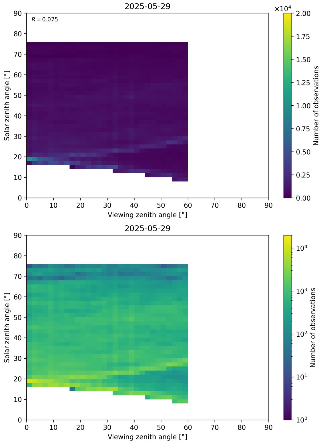
Figure 115: Scatter density plot of “Viewing zenith angle” against “Solar zenith angle” for 2025-05-28 to 2025-05-30.
