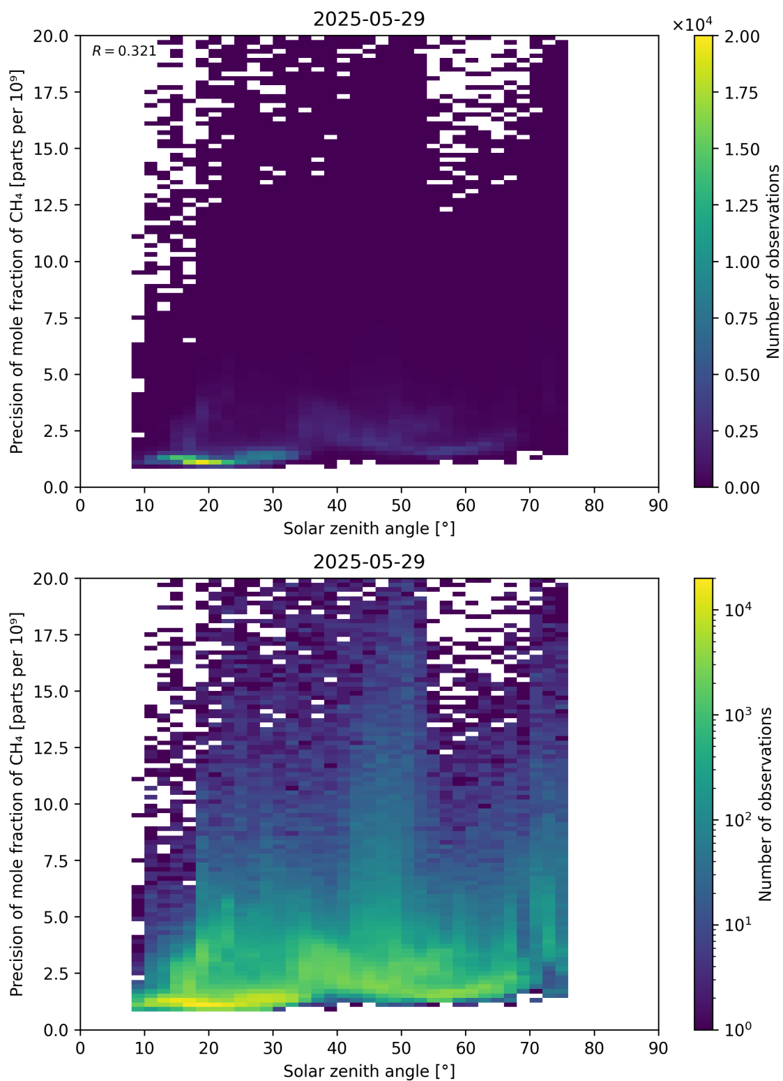
Figure 101: Scatter density plot of “Solar zenith angle” against “Precision of mole fraction of CH 4 ” for 2025-05-28 to 2025-05-30.
