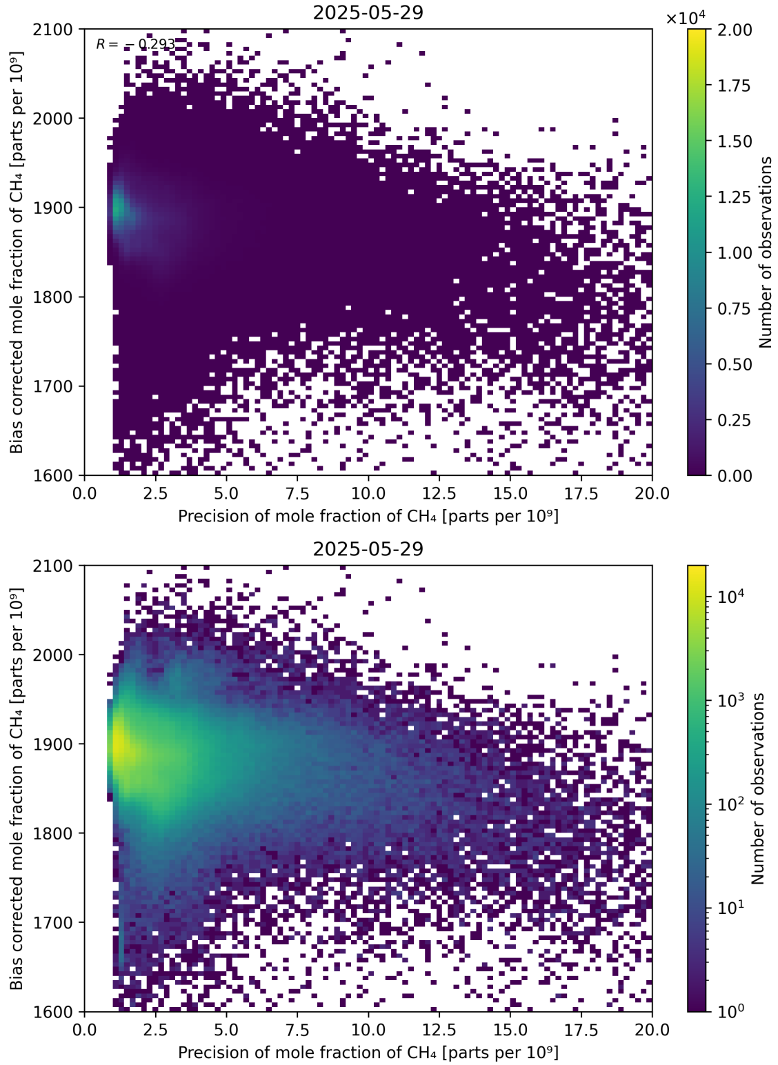
Figure 82: Scatter density plot of “Precision of mole fraction of CH 4 ” against “Bias corrected mole fraction of CH 4 ” for 2025-05-28 to 2025-05-30.
