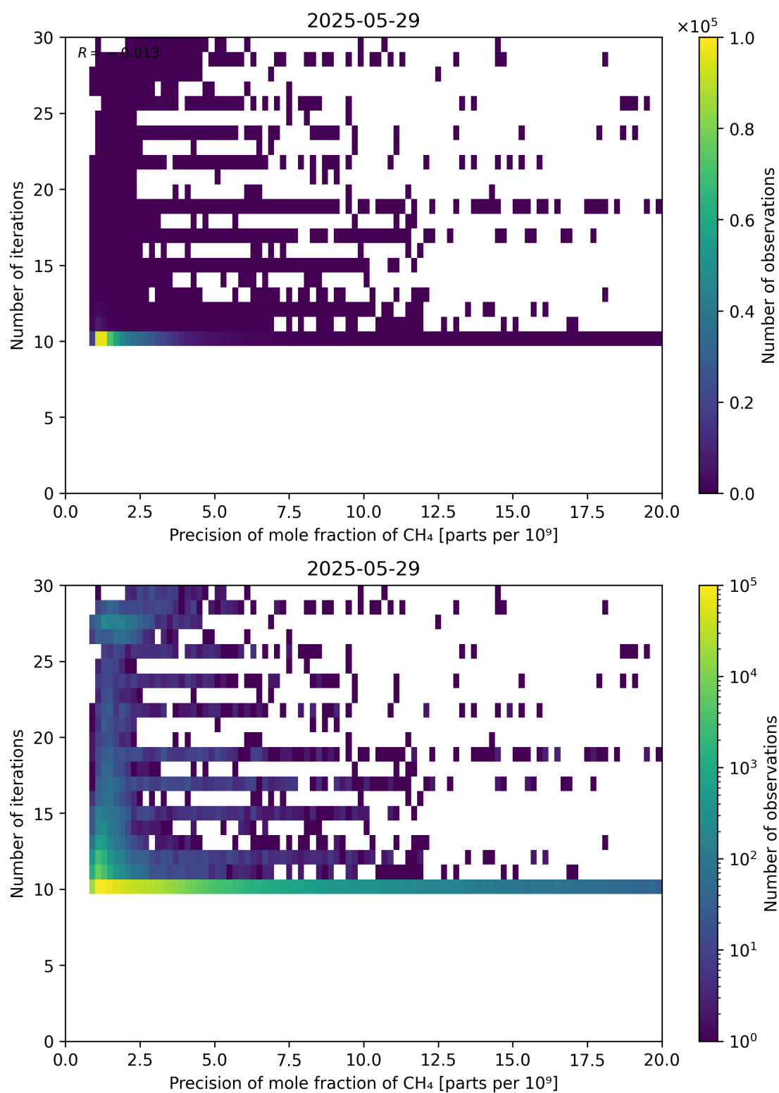
Figure 83: Scatter density plot of “Precision of mole fraction of CH 4 ” against “Number of iterations” for 2025-05-28 to 2025-05-30.
