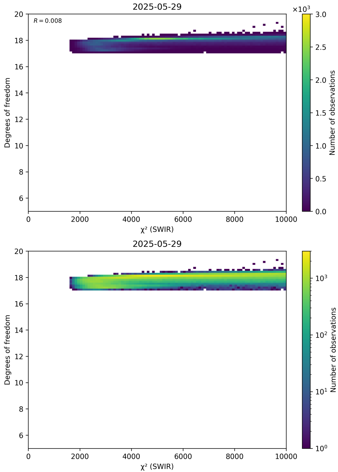
Figure 48: Scatter density plot of “ \chi^2 (SWIR)” against “Degrees of freedom” for 2025-05-28 to 2025-05-30.
