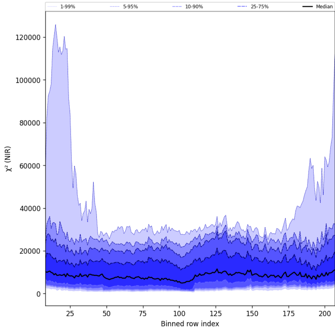
Figure 40: Along track statistics of “ \chi^2 (NIR)” for 2025-05-28 to 2025-05-30
