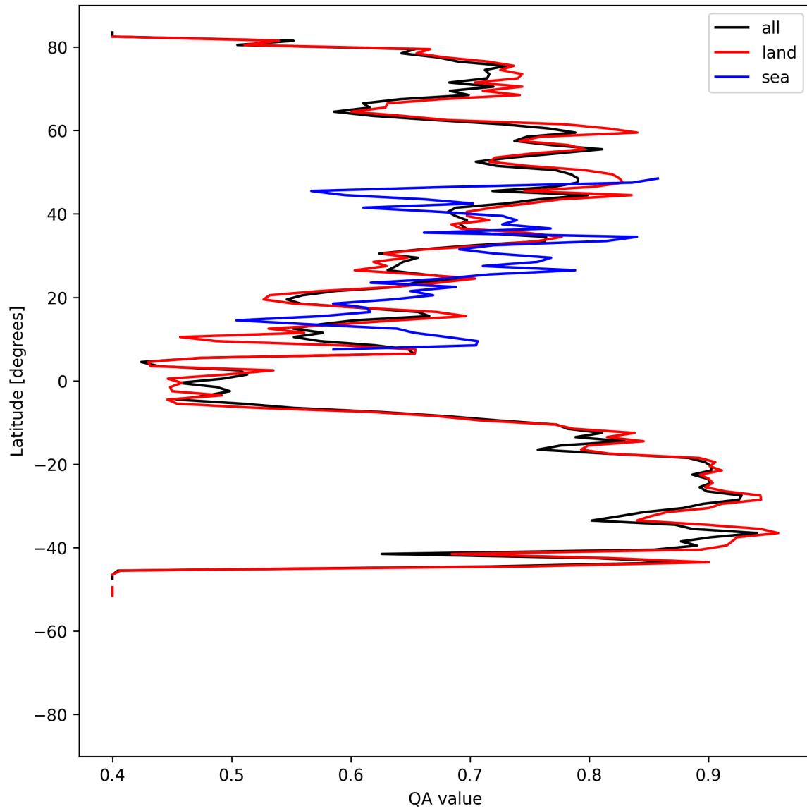
Figure 11: Zonal average of “QA value” for 2025-05-28 to 2025-05-30.
