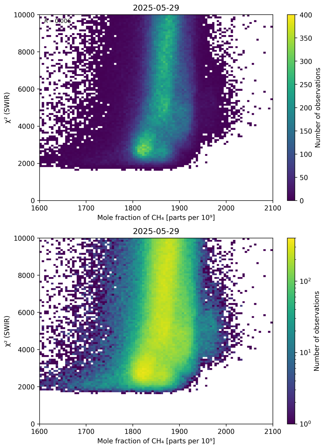
Figure 71: Scatter density plot of “Mole fraction of \text{CH}_4 ” against “ \chi^2 (SWIR)” for 2025-05-28 to 2025-05-30.
