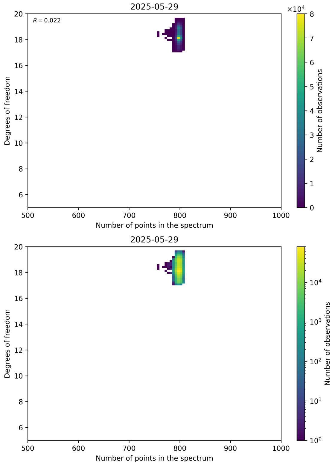
Figure 90: Scatter density plot of “Number of points in the spectrum” against “Degrees of freedom” for 2025-05-28 to 2025-05-30.
