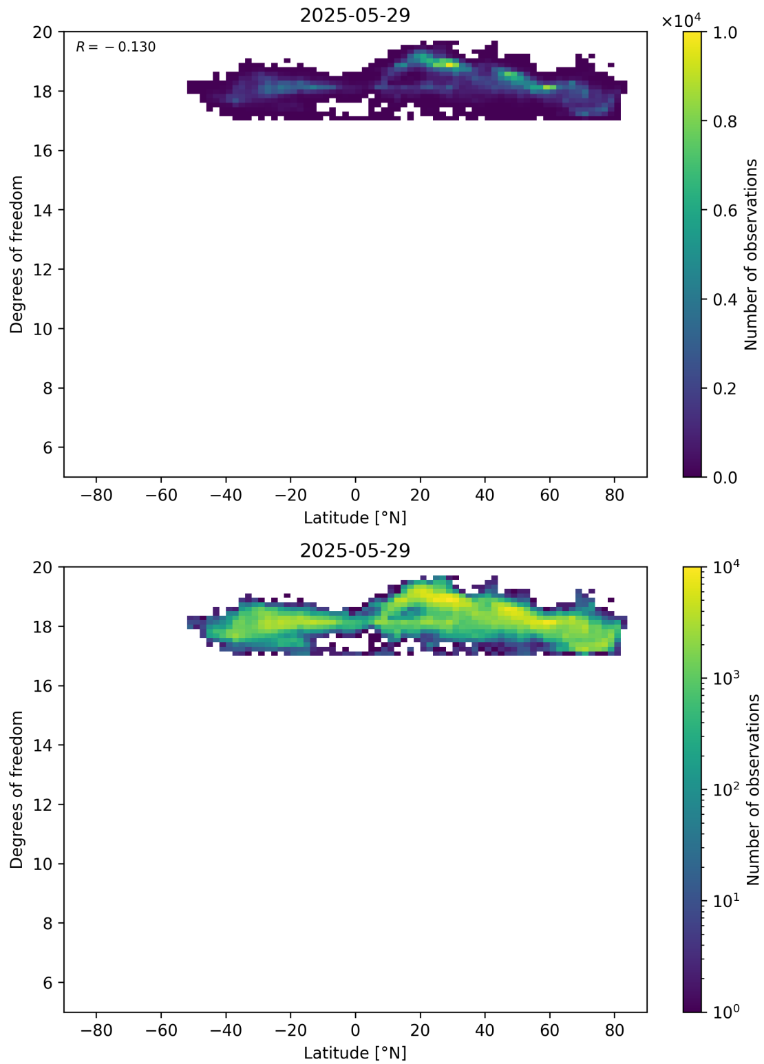
Figure 55: Scatter density plot of “Latitude” against “Degrees of freedom” for 2025-05-28 to 2025-05-30.
