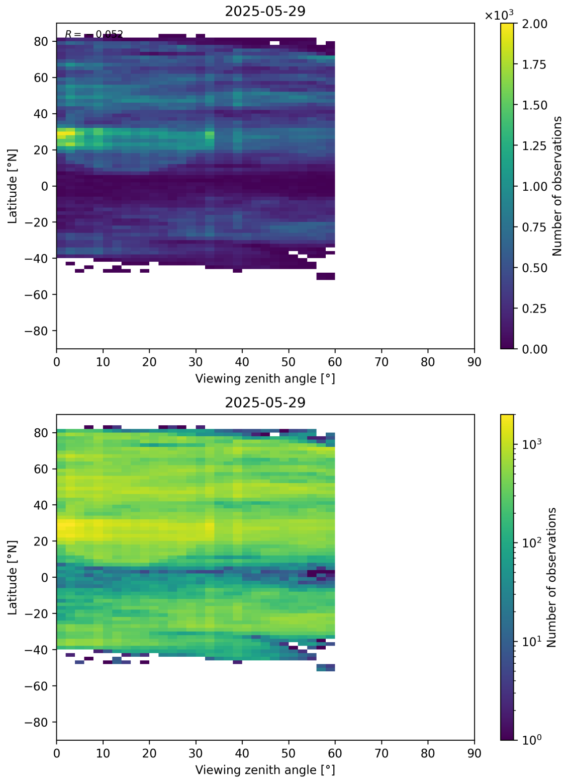
Figure 109: Scatter density plot of “Viewing zenith angle” against “Latitude” for 2025-05-28 to 2025-05-30.
