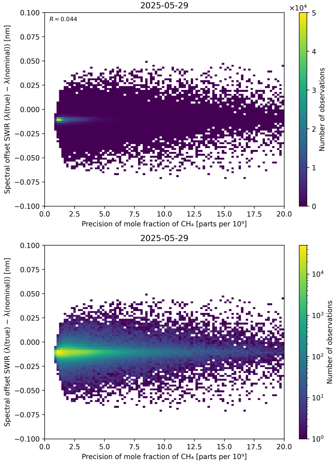
Figure 85: Scatter density plot of “Precision of mole fraction of CH 4 ” against “Spectral offset SWIR ( \lambda_{\text{true}} - \lambda_{\text{nominal}} )” for 2025-05-28 to 2025-05-30.
