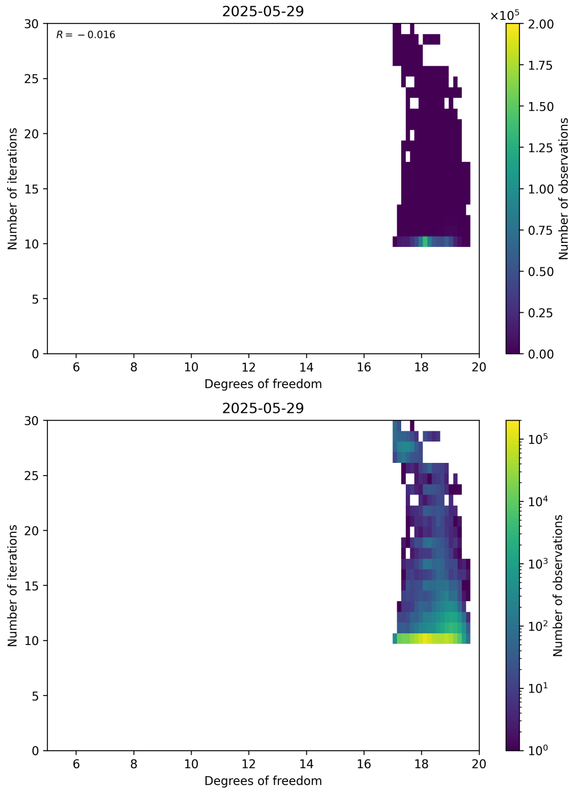
Figure 52: Scatter density plot of “Degrees of freedom” against “Number of iterations” for 2025-05-28 to 2025-05-30.
