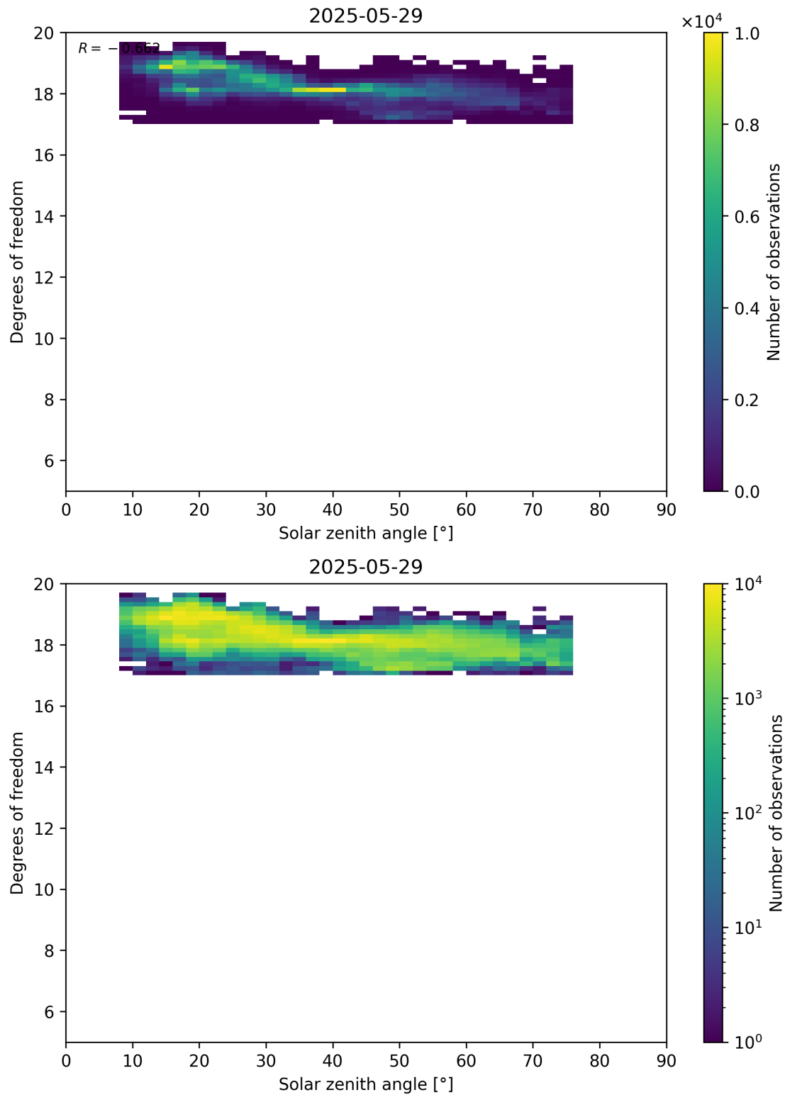
Figure 96: Scatter density plot of “Solar zenith angle” against “Degrees of freedom” for 2025-05-28 to 2025-05-30.
