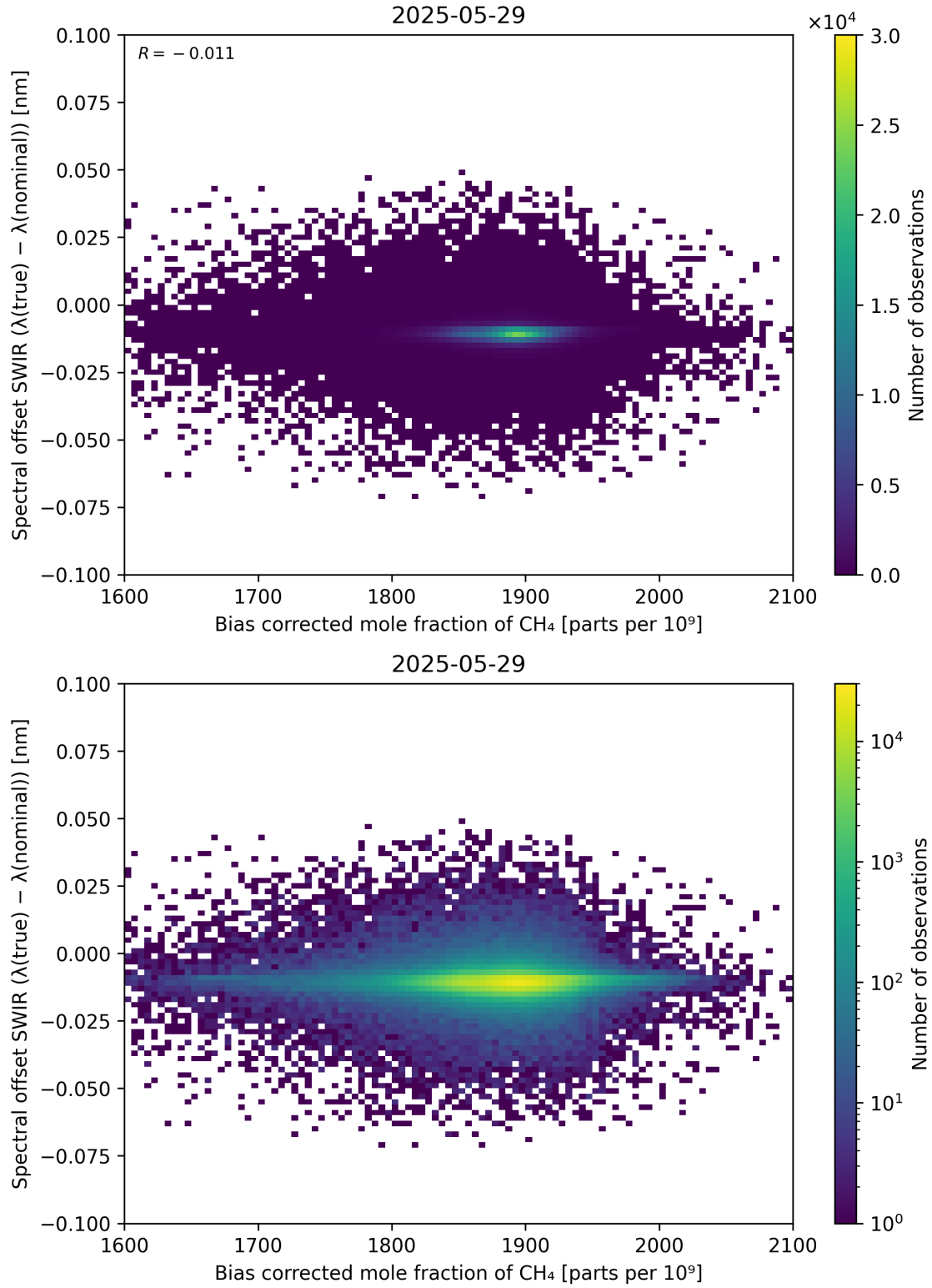
Figure 69: Scatter density plot of “Bias corrected mole fraction of \text{CH}_4 ” against “Spectral offset SWIR ( \lambda_{\text{true}} - \lambda_{\text{nominal}} )” for 2025-05-28 to 2025-05-30.
