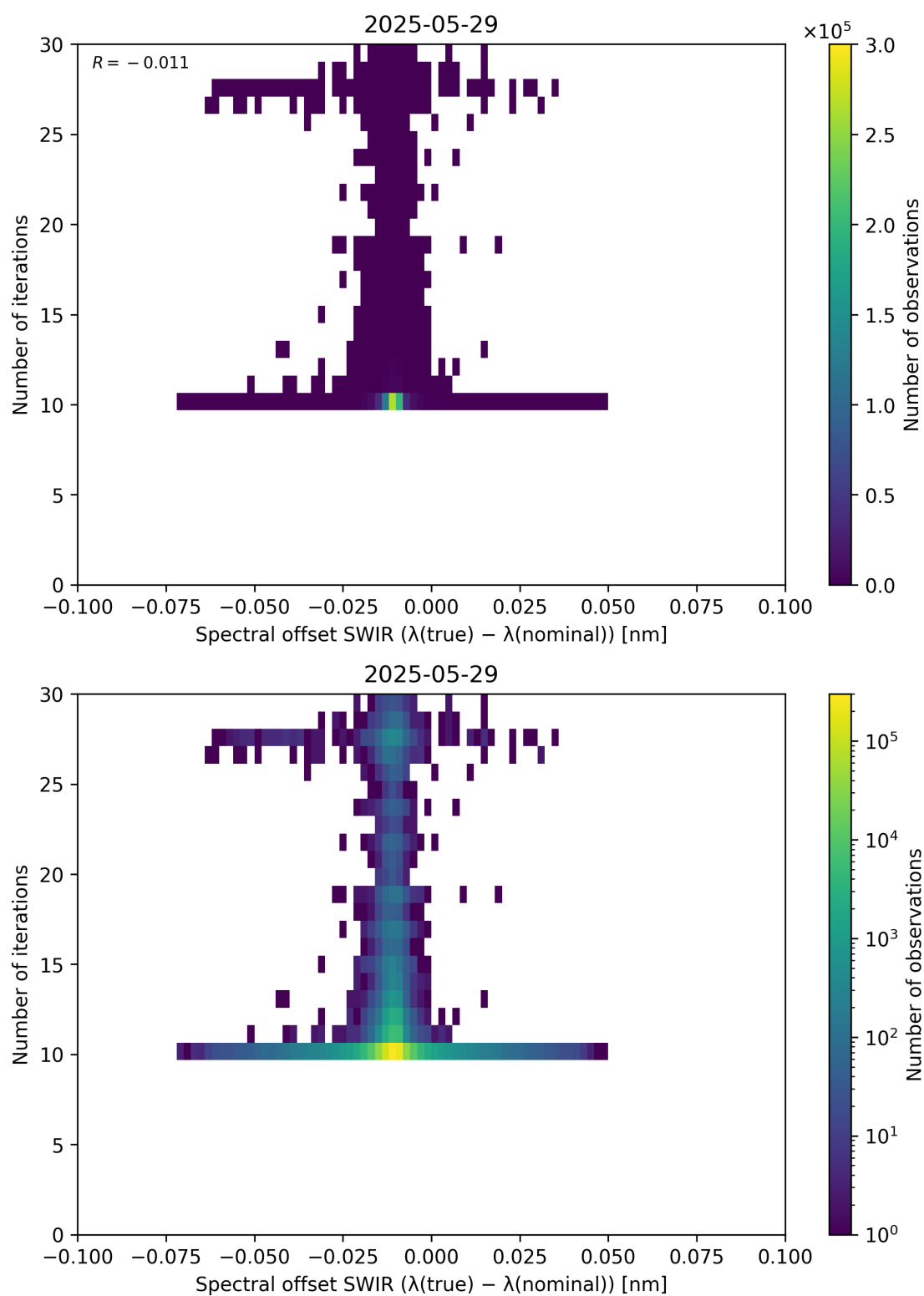
Figure 121: Scatter density plot of “Spectral offset SWIR ( \lambda_{\text{true}} - \lambda_{\text{nominal}} )” against “Number of iterations” for 2025-05-28 to 2025-05-30.
