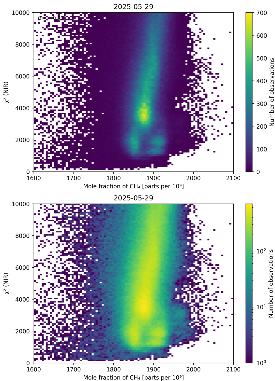
Figure 70: Scatter density plot of “Mole fraction of CH 4 ” against “ \chi^2 (NIR)” for 2025-05-28 to 2025-05-30.
