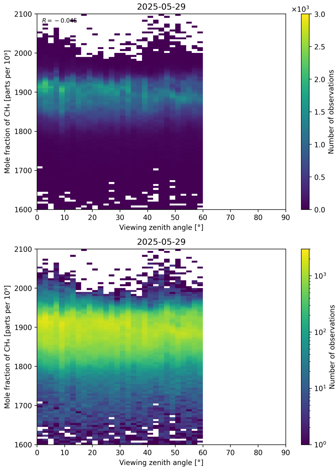
Figure 110: Scatter density plot of “Viewing zenith angle” against “Mole fraction of CH 4 ” for 2025-05-28 to 2025-05-30.
