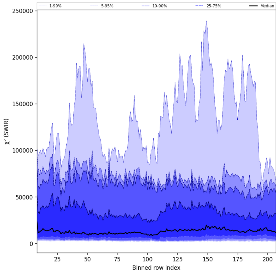
Figure 39: Along track statistics of “ \chi^2 (SWIR)” for 2025-05-28 to 2025-05-30
