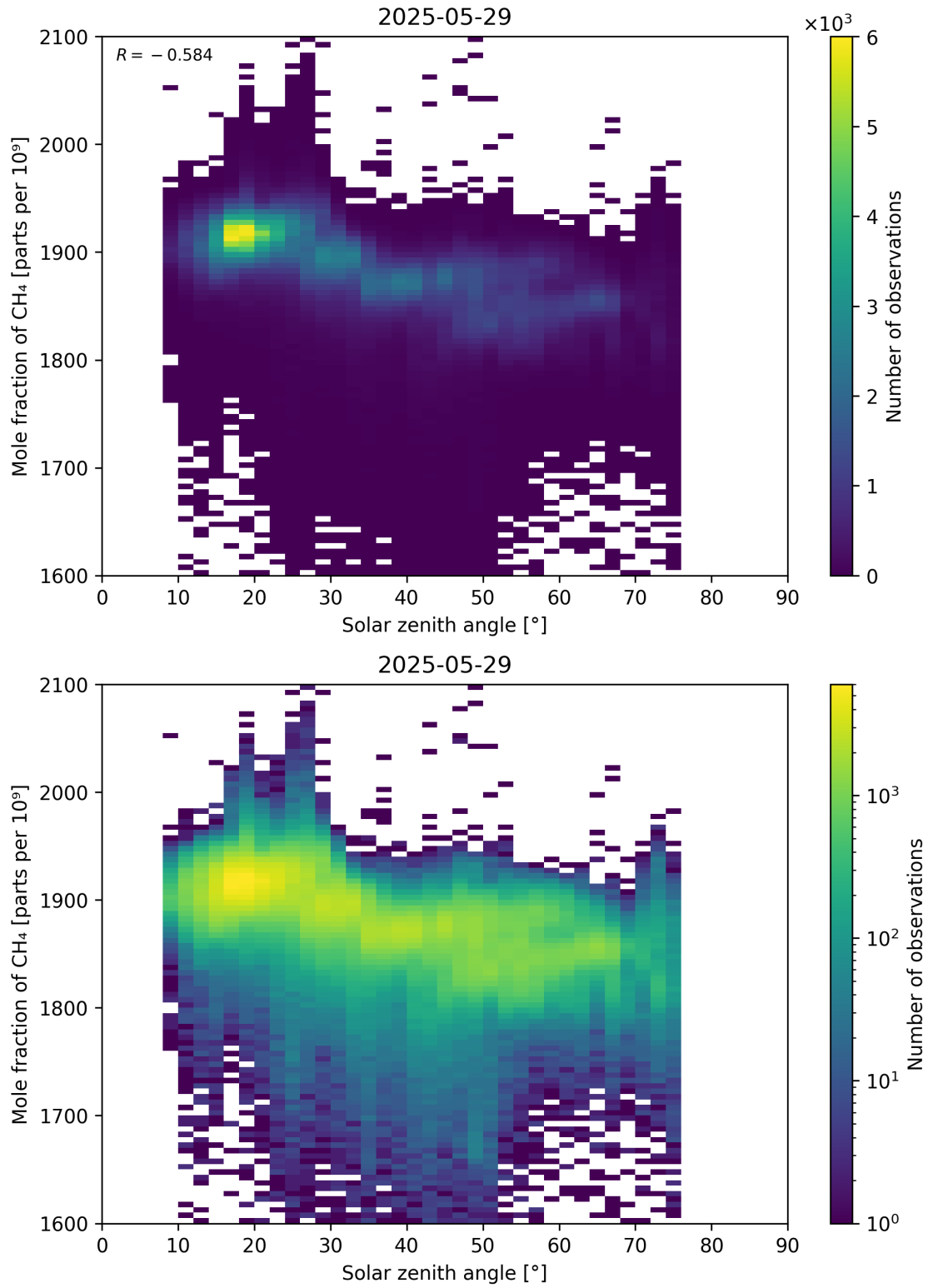
Figure 99: Scatter density plot of “Solar zenith angle” against “Mole fraction of \text{CH}_4 ” for 2025-05-28 to 2025-05-30.
