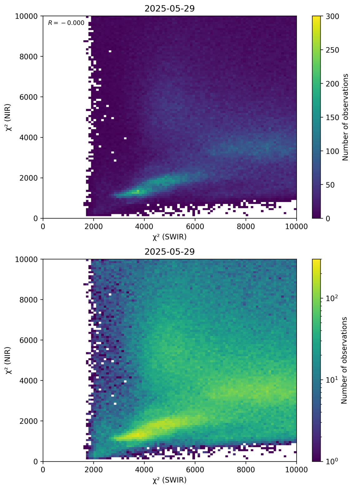
Figure 47: Scatter density plot of “ \chi^2 (SWIR)” against “ \chi^2 (NIR)” for 2025-05-28 to 2025-05-30.
