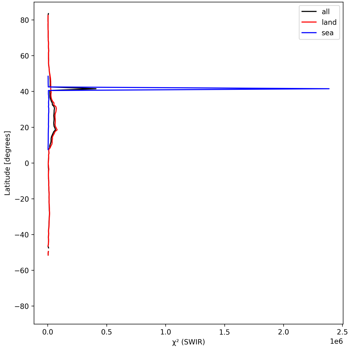
Figure 17: Zonal average of “ \chi^2 (SWIR)” for 2025-05-28 to 2025-05-30.
