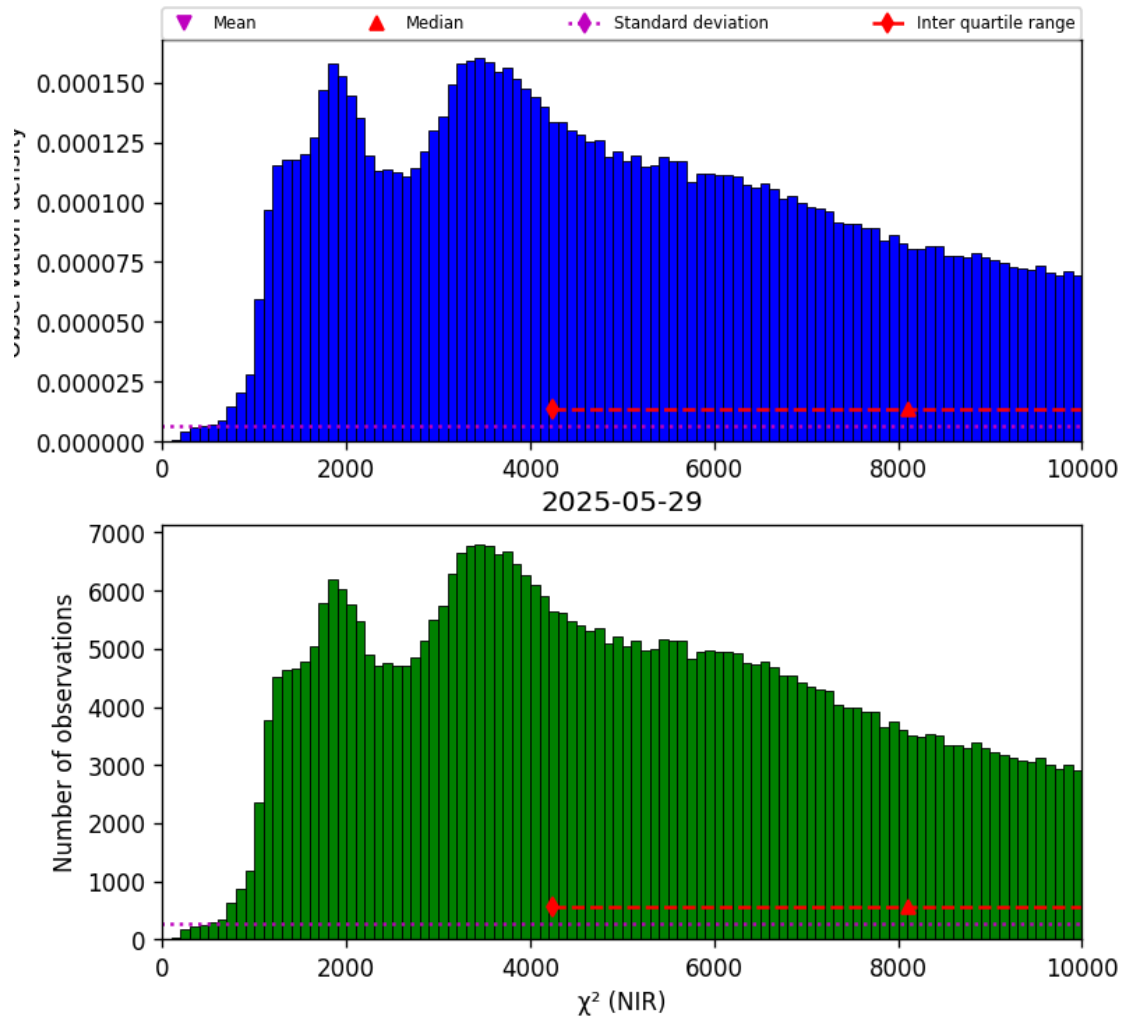
Figure 29: Histogram of “ \chi^2 (NIR)” for 2025-05-28 to 2025-05-30
