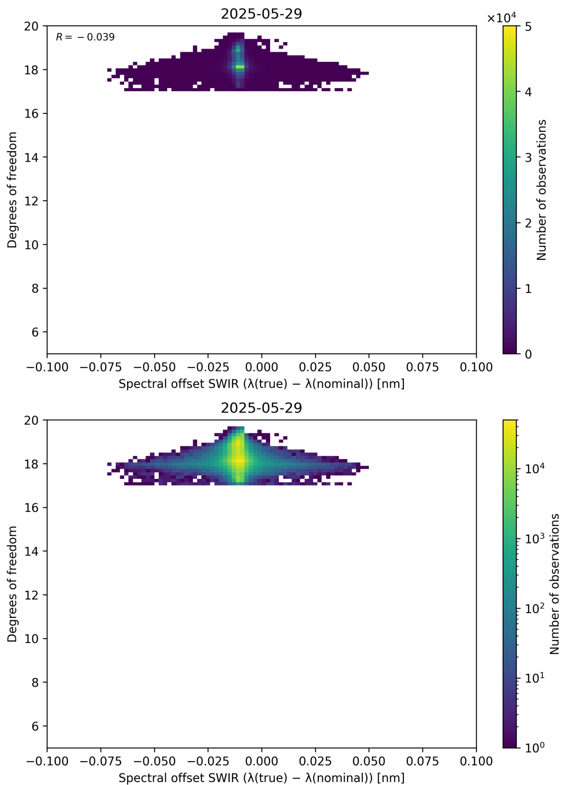
Figure 119: Scatter density plot of “Spectral offset SWIR ( \lambda_{\text{true}} - \lambda_{\text{nominal}} )” against “Degrees of freedom” for 2025-05-28 to 2025-05-30.
