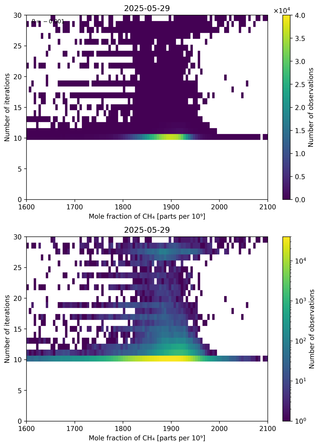
Figure 76: Scatter density plot of “Mole fraction of CH 4 ” against “Number of iterations” for 2025-05-28 to 2025-05-30.
