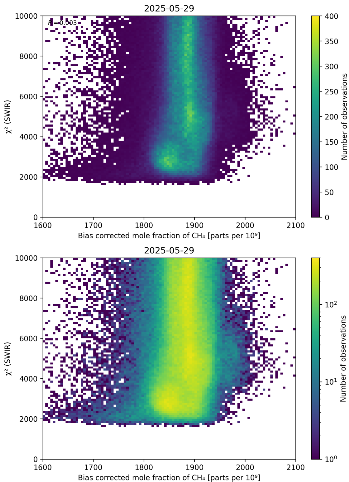
Figure 64: Scatter density plot of “Bias corrected mole fraction of \text{CH}_4 ” against “ \chi^2 (SWIR)” for 2025-05-28 to 2025-05-30.
