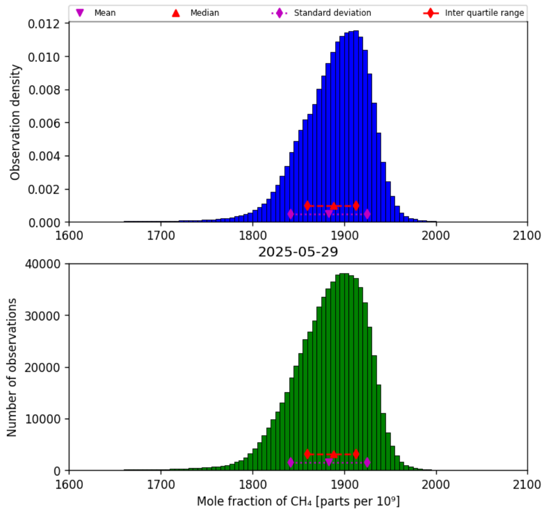
Figure 23: Histogram of “Mole fraction of CH 4 ” for 2025-05-28 to 2025-05-30
