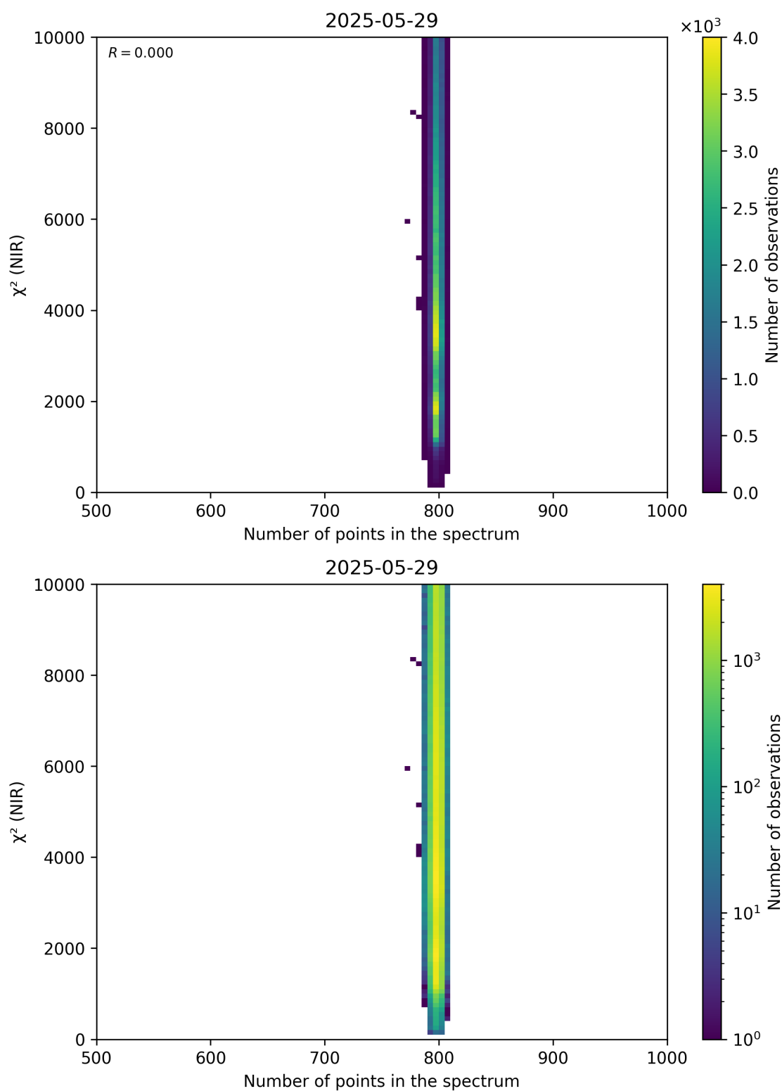
Figure 88: Scatter density plot of “Number of points in the spectrum” against “ \chi^2 (NIR)” for 2025-05-28 to 2025-05-30.
