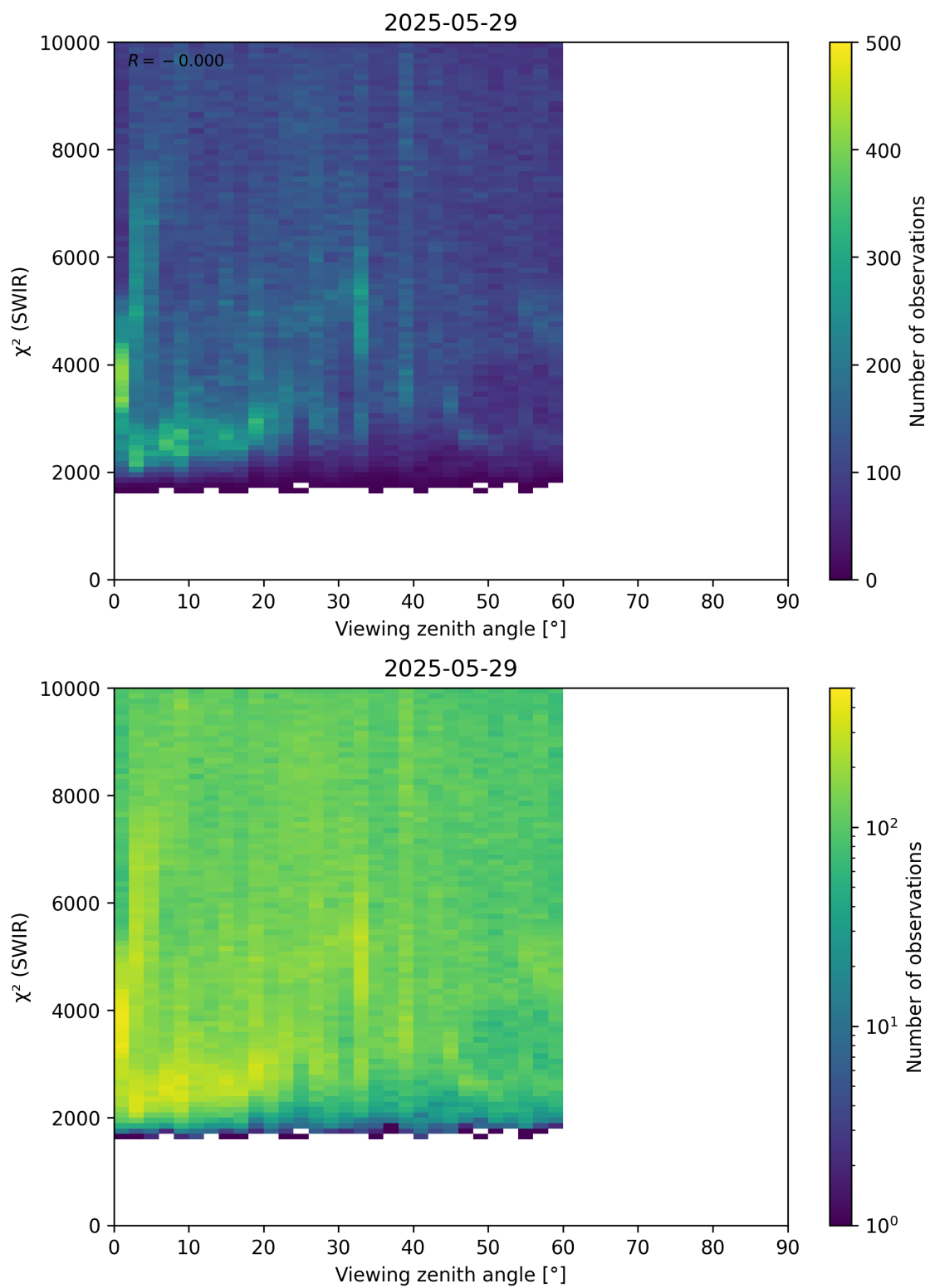
Figure 106: Scatter density plot of “Viewing zenith angle” against “ \chi^2 (SWIR)” for 2025-05-28 to 2025-05-30.
