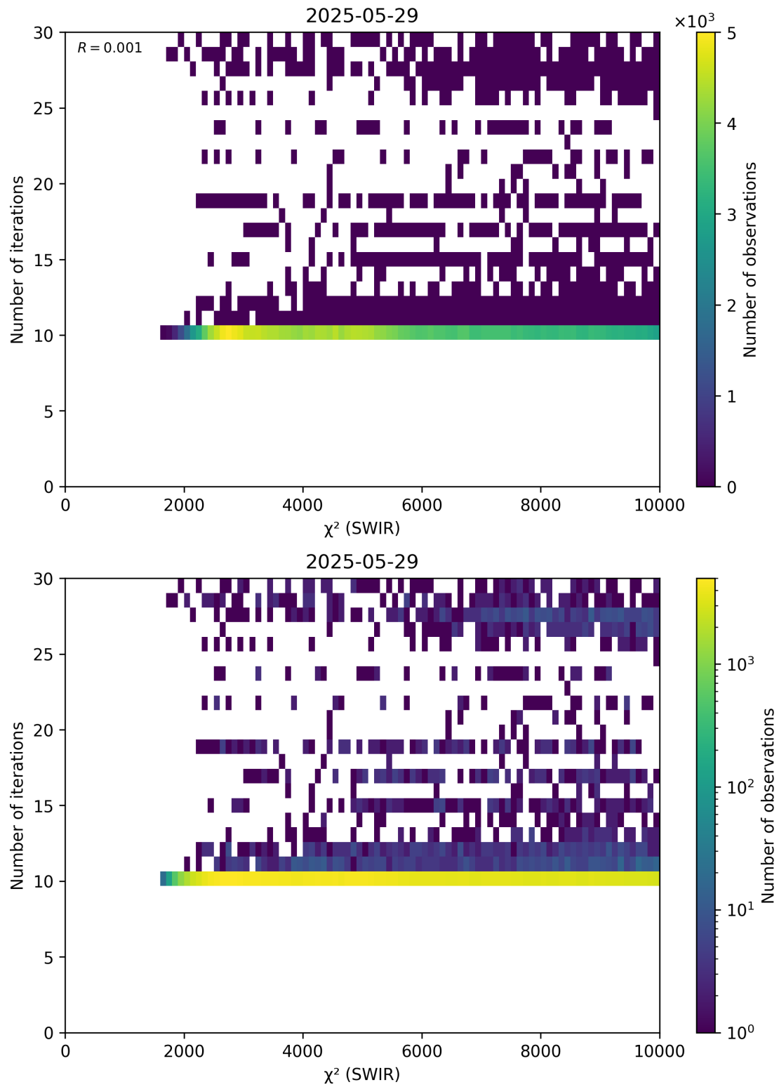
Figure 50: Scatter density plot of “ \chi^2 (SWIR)” against “Number of iterations” for 2025-05-28 to 2025-05-30.
