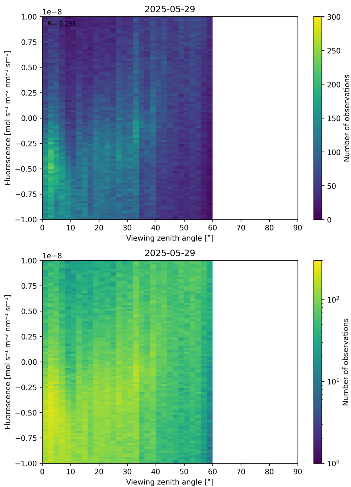
Figure 108: Scatter density plot of “Viewing zenith angle” against “Fluorescence” for 2025-05-28 to 2025-05-30.
