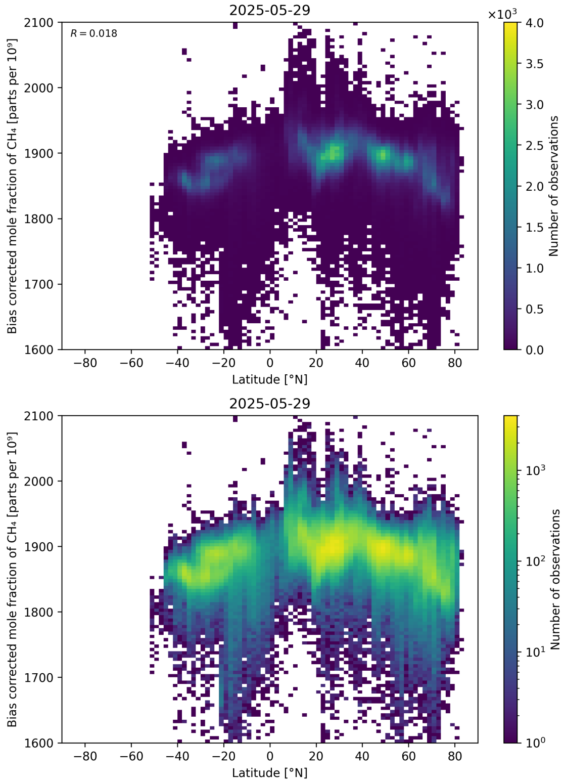
Figure 58: Scatter density plot of “Latitude” against “Bias corrected mole fraction of \text{CH}_4 ” for 2025-05-28 to 2025-05-30.
