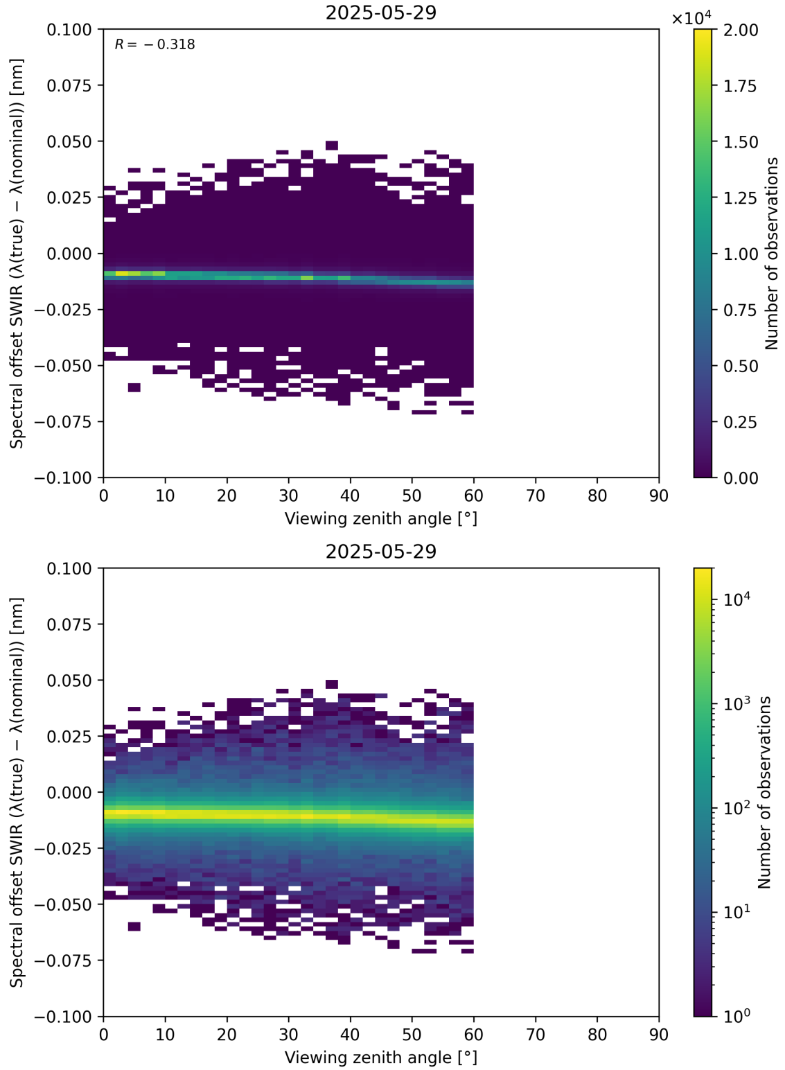
Figure 116: Scatter density plot of “Viewing zenith angle” against “Spectral offset SWIR ( \lambda_{\text{true}} - \lambda_{\text{nominal}} )” for 2025-05-28 to 2025-05-30.
