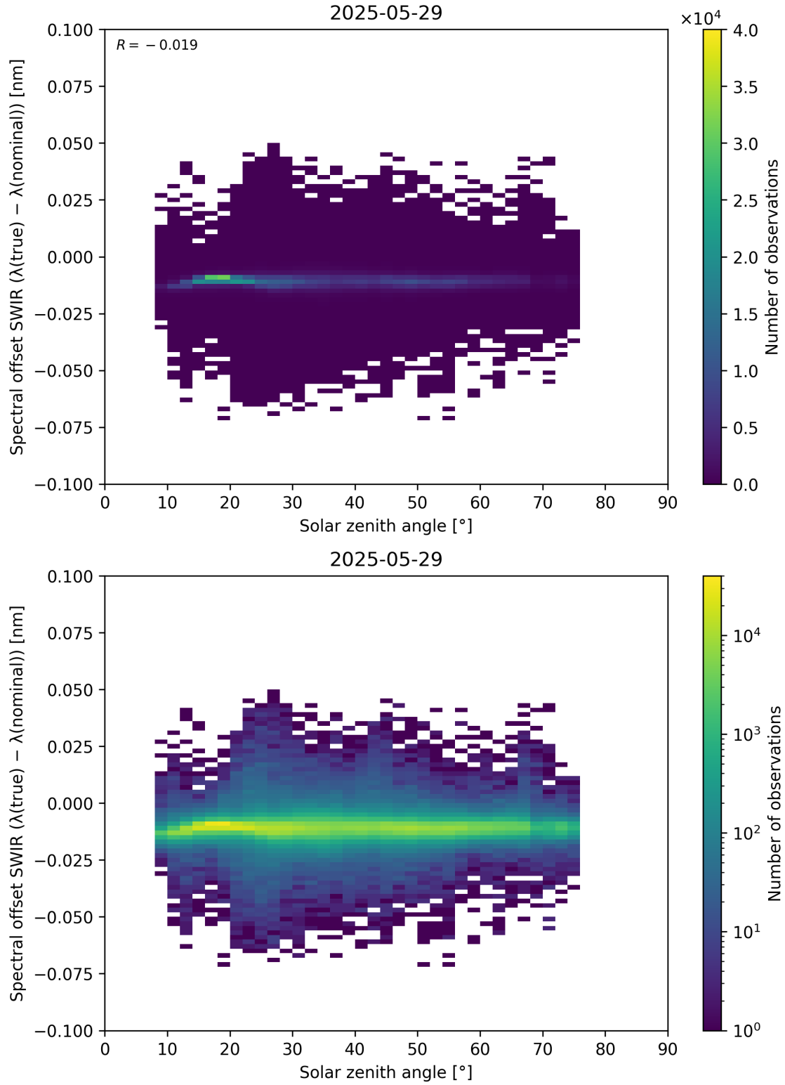
Figure 104: Scatter density plot of “Solar zenith angle” against “Spectral offset SWIR ( \lambda_{\text{true}} - \lambda_{\text{nominal}} )” for 2025-05-28 to 2025-05-30.
