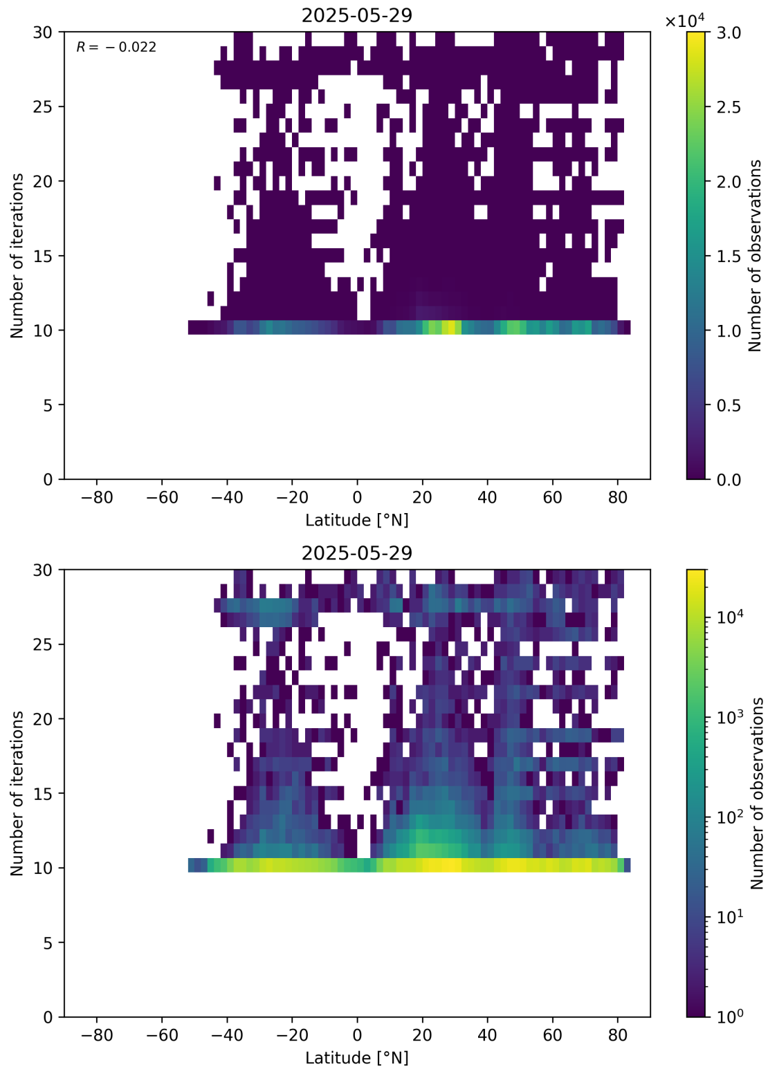
Figure 60: Scatter density plot of “Latitude” against “Number of iterations” for 2025-05-28 to 2025-05-30.
