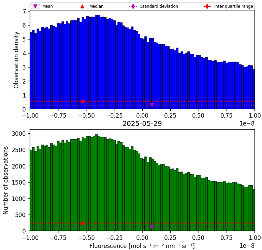
Figure 32: Histogram of “Fluorescence” for 2025-05-28 to 2025-05-30
