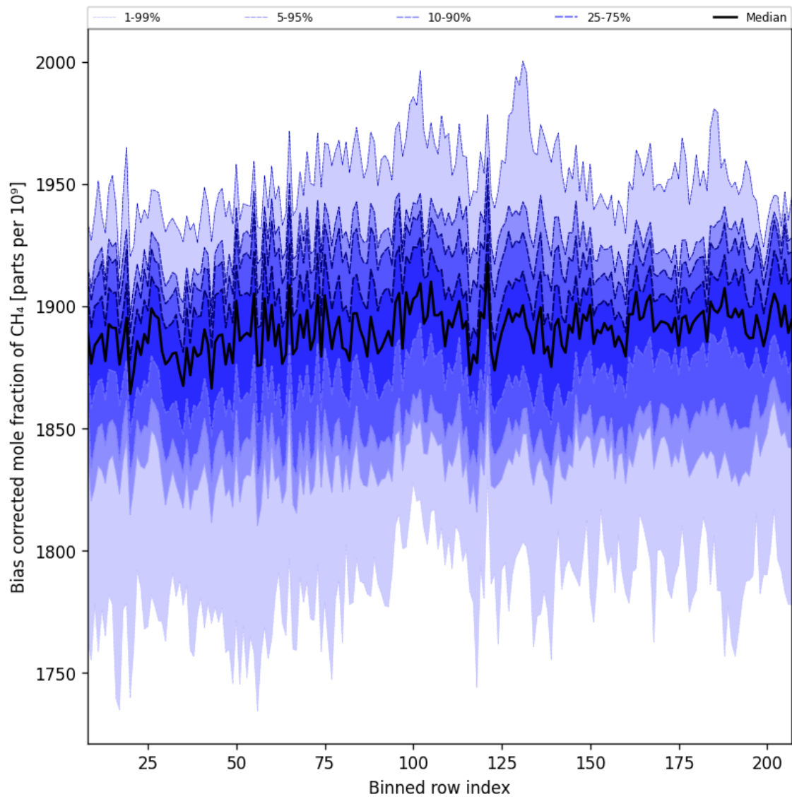
Figure 36: Along track statistics of “Bias corrected mole fraction of CH 4 ” for 2025-05-28 to 2025-05-30
