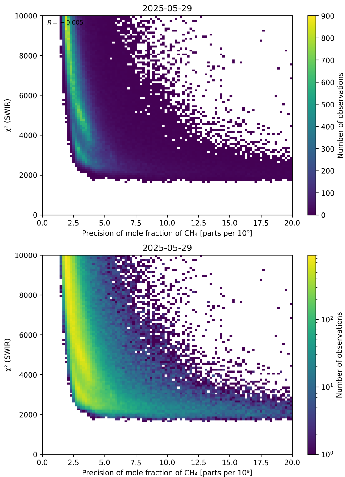
Figure 79: Scatter density plot of “Precision of mole fraction of CH 4 ” against “ \chi^2 (SWIR)” for 2025-05-28 to 2025-05-30.
