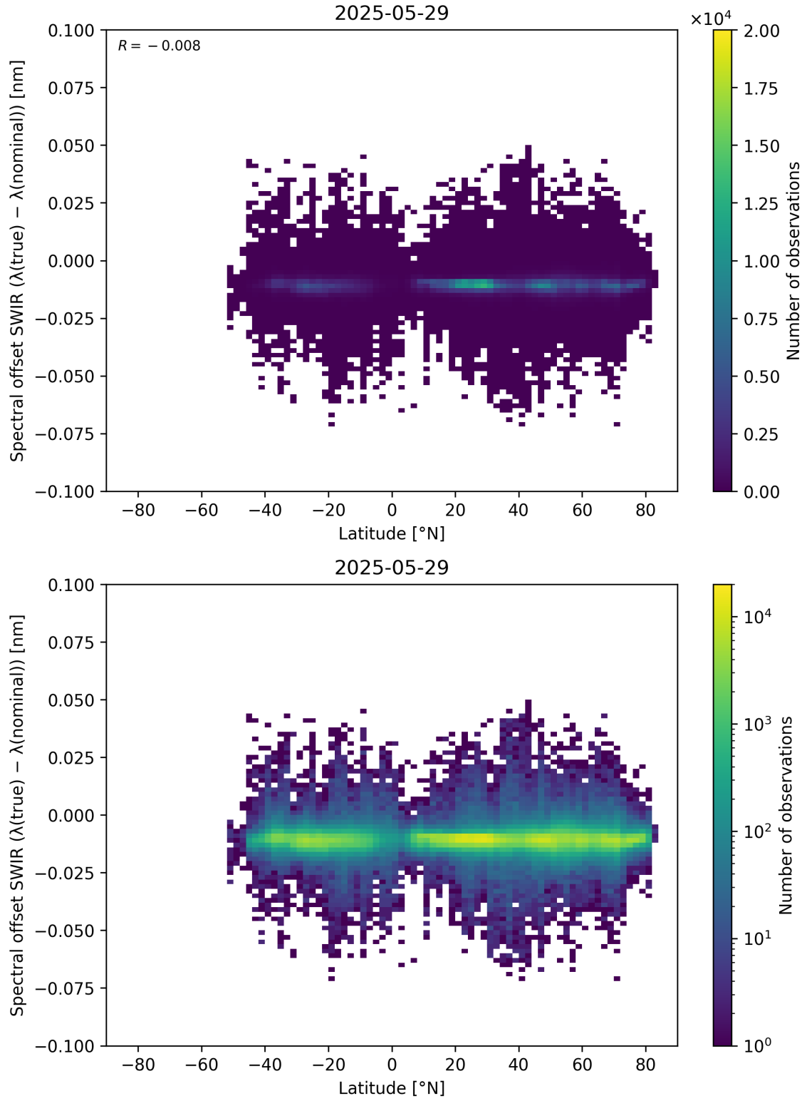
Figure 62: Scatter density plot of “Latitude” against “Spectral offset SWIR ( \lambda_{\text{true}} - \lambda_{\text{nominal}} )” for 2025-05-28 to 2025-05-30.
