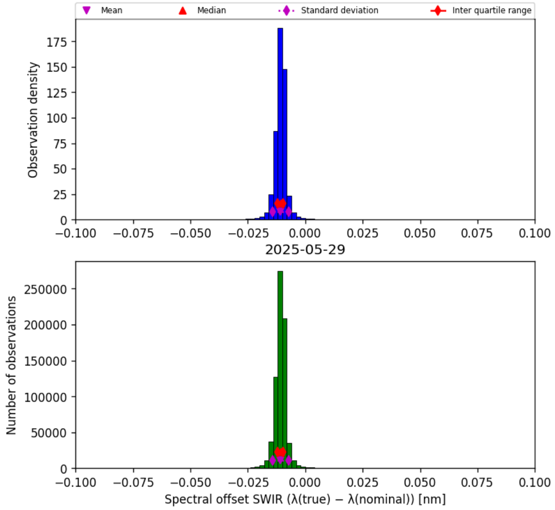
Figure 27: Histogram of “Spectral offset SWIR ( \lambda_{\text{true}} - \lambda_{\text{nominal}} )” for 2025-05-28 to 2025-05-30
