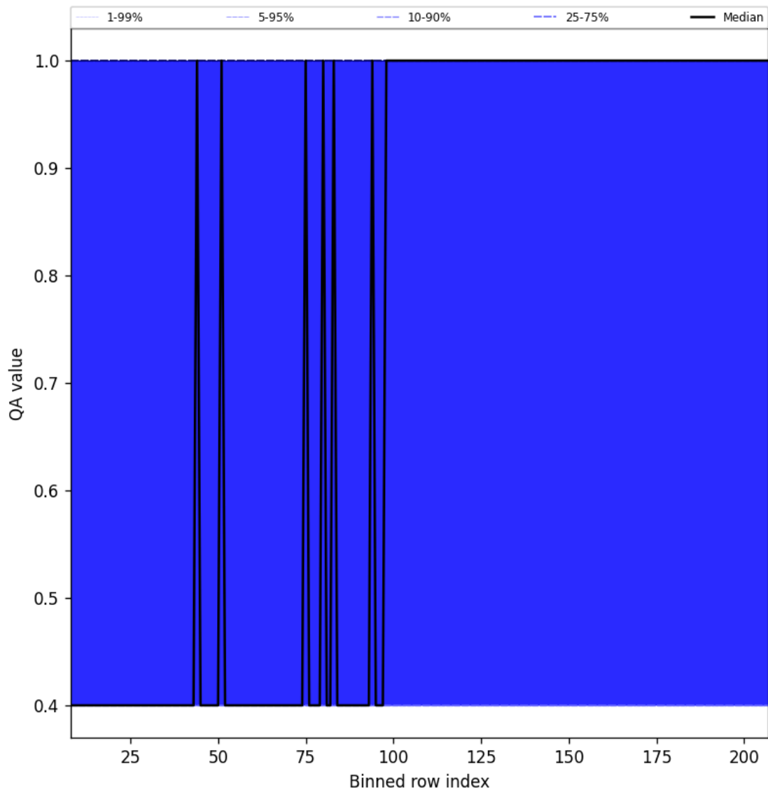
Figure 33: Along track statistics of “QA value” for 2025-05-28 to 2025-05-30
