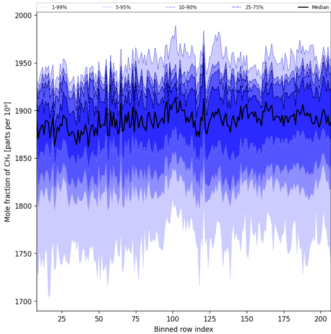
Figure 34: Along track statistics of “Mole fraction of CH 4 ” for 2025-05-28 to 2025-05-30
