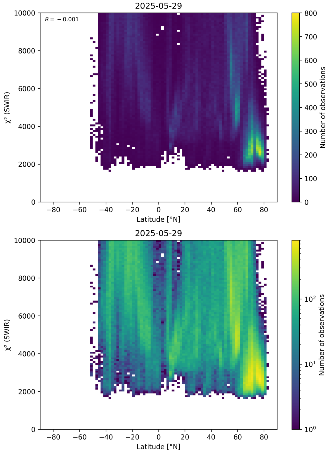
Figure 54: Scatter density plot of “Latitude” against “ \chi^2 (SWIR)” for 2025-05-28 to 2025-05-30.
