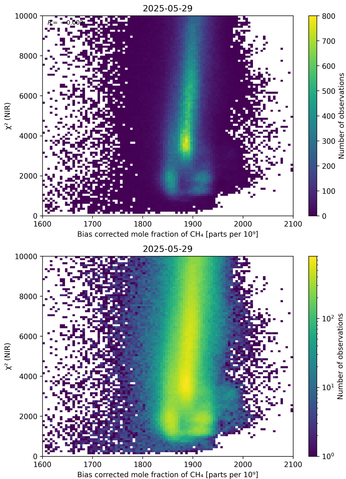
Figure 63: Scatter density plot of “Bias corrected mole fraction of \text{CH}_4 ” against “ \chi^2 (NIR)” for 2025-05-28 to 2025-05-30.
