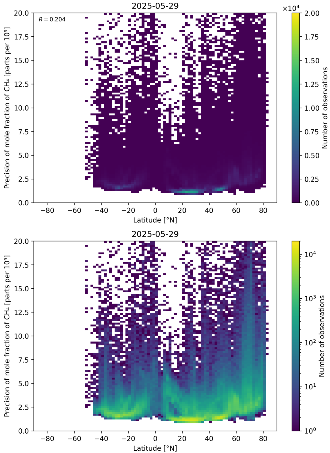
Figure 59: Scatter density plot of “Latitude” against “Precision of mole fraction of \text{CH}_4 ” for 2025-05-28 to 2025-05-30.
