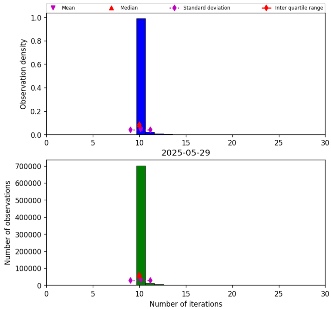
Figure 31: Histogram of “Number of iterations” for 2025-05-28 to 2025-05-30
