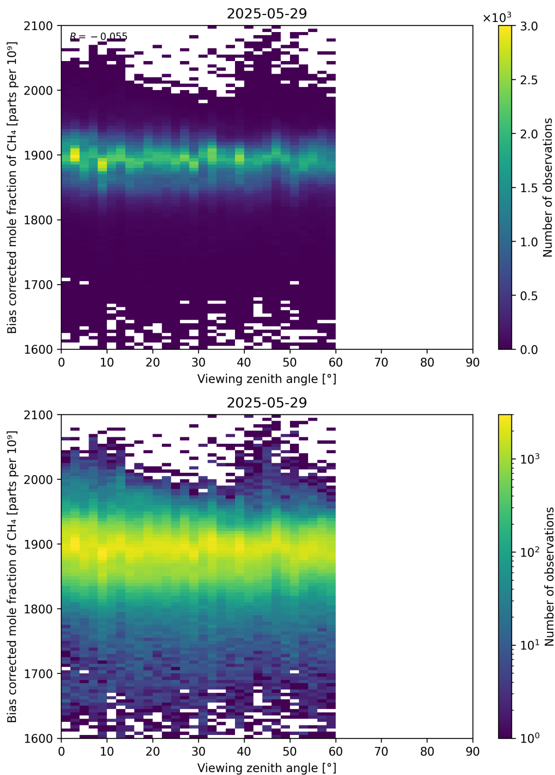
Figure 111: Scatter density plot of “Viewing zenith angle” against “Bias corrected mole fraction of CH 4 ” for 2025-05-28 to 2025-05-30.
