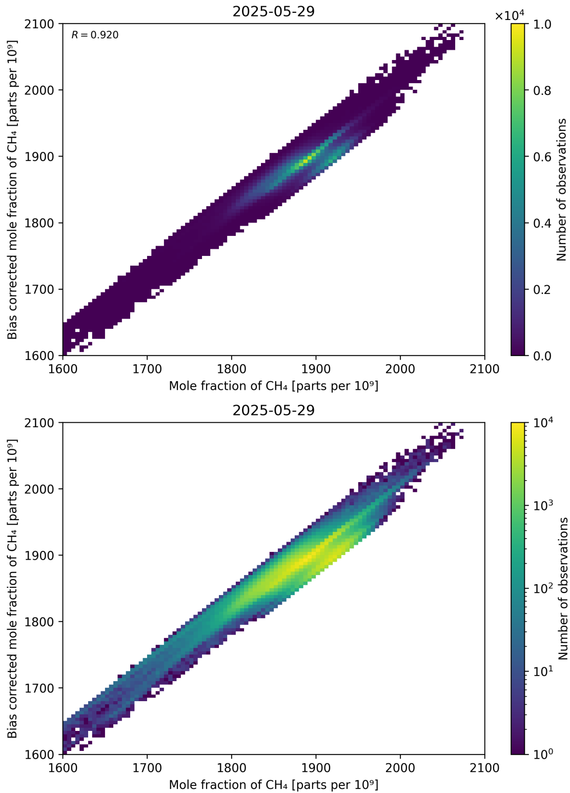
Figure 74: Scatter density plot of “Mole fraction of CH 4 ” against “Bias corrected mole fraction of CH 4 ” for 2025-05-28 to 2025-05-30.
