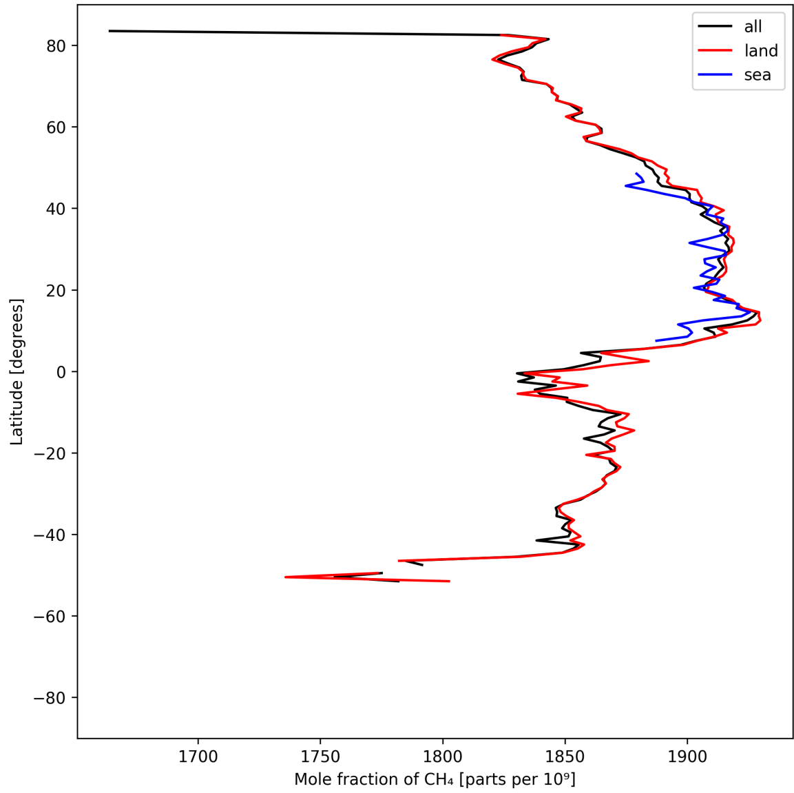
Figure 12: Zonal average of “Mole fraction of CH 4 ” for 2025-05-28 to 2025-05-30.
