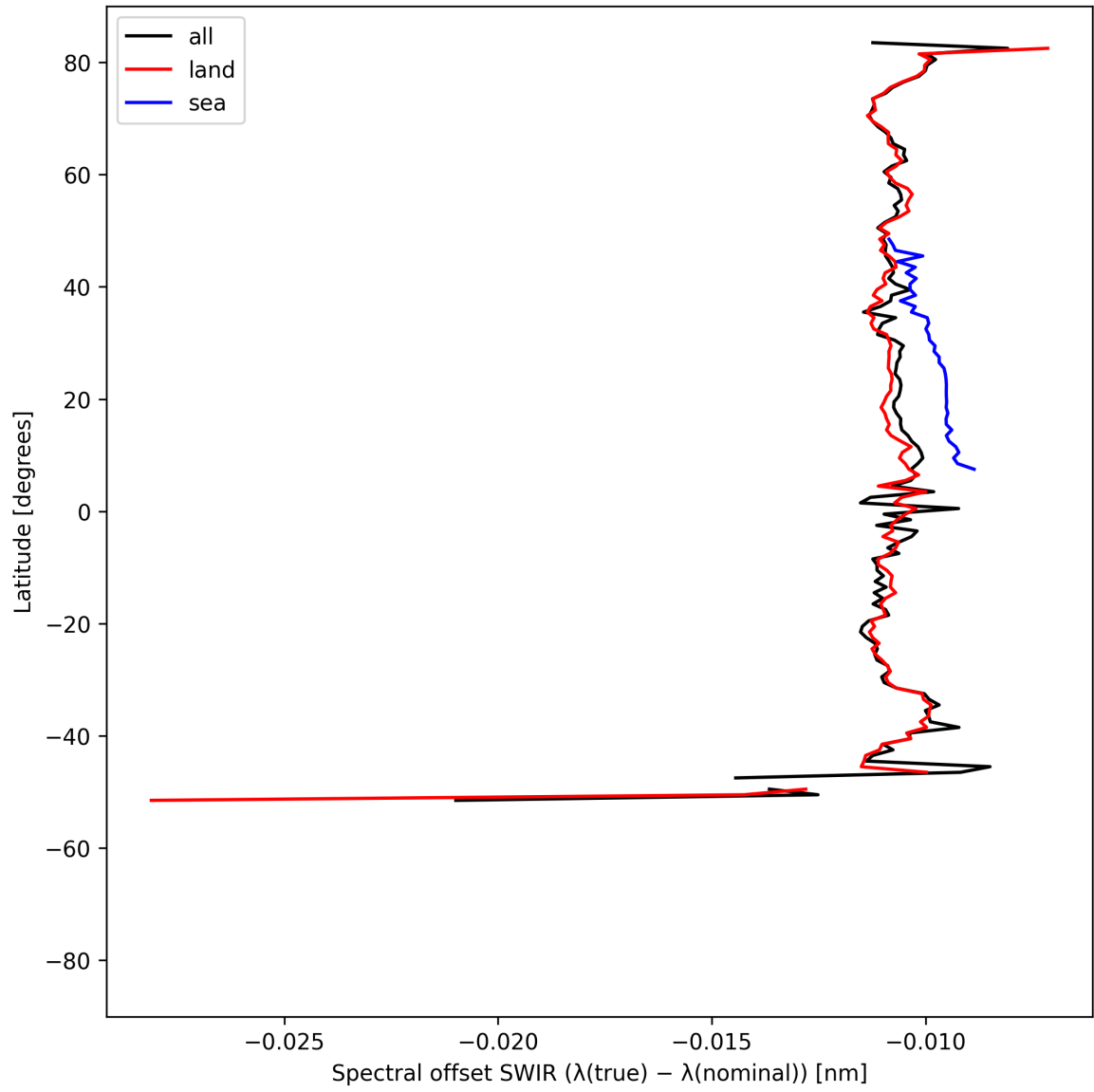
Figure 16: Zonal average of “Spectral offset SWIR ( \lambda_{\text{true}} - \lambda_{\text{nominal}} )” for 2025-05-28 to 2025-05-30.
