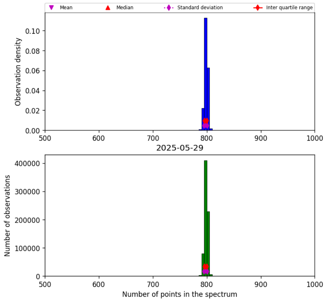
Figure 26: Histogram of “Number of points in the spectrum” for 2025-05-28 to 2025-05-30
