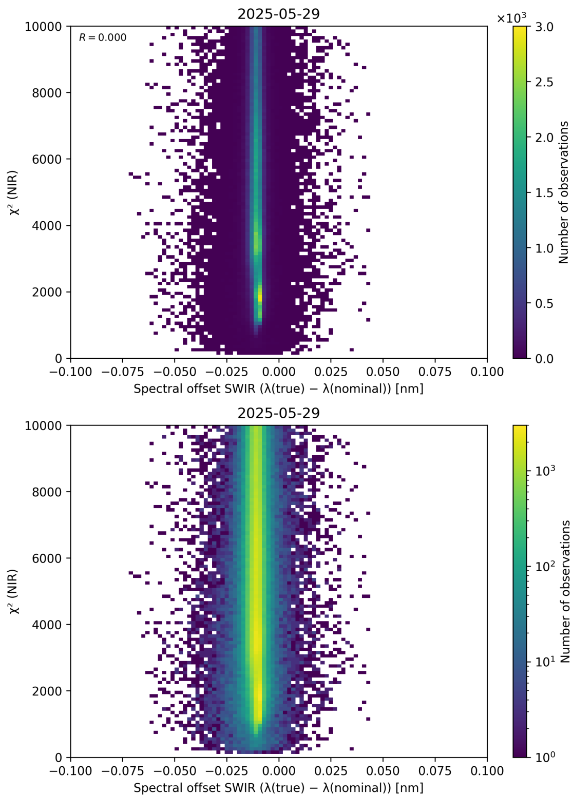
Figure 117: Scatter density plot of “Spectral offset SWIR ( \lambda_{\text{true}} - \lambda_{\text{nominal}} )” against “ \chi^2 (NIR)” for 2025-05-28 to 2025-05-30.
