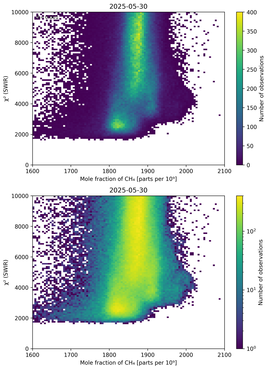
Figure 71: Scatter density plot of “Mole fraction of CH 4 ” against “ \chi^2 (SWIR)” for 2025-05-29 to 2025-05-31.
