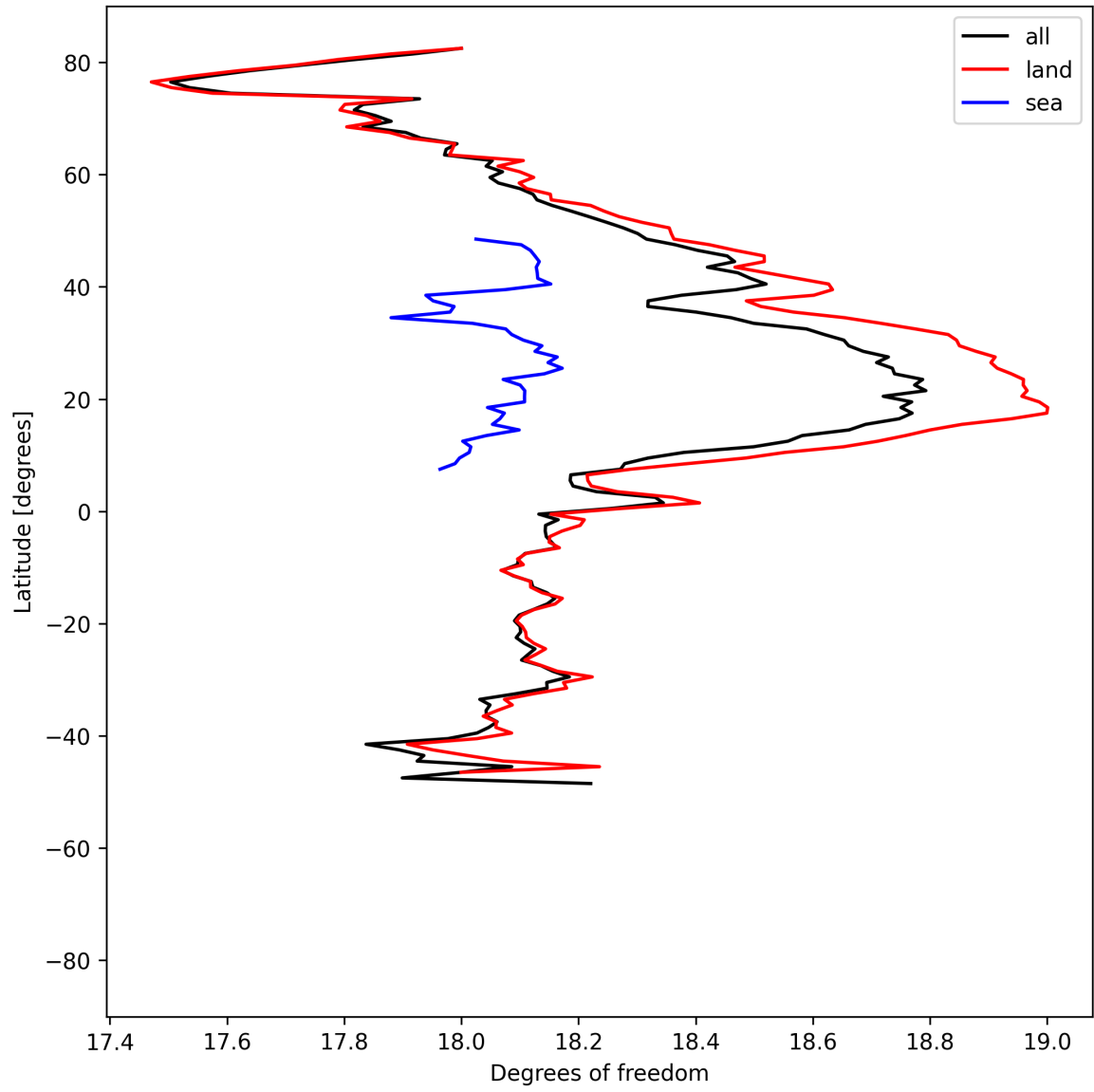
Figure 19: Zonal average of “Degrees of freedom” for 2025-05-29 to 2025-05-31.
