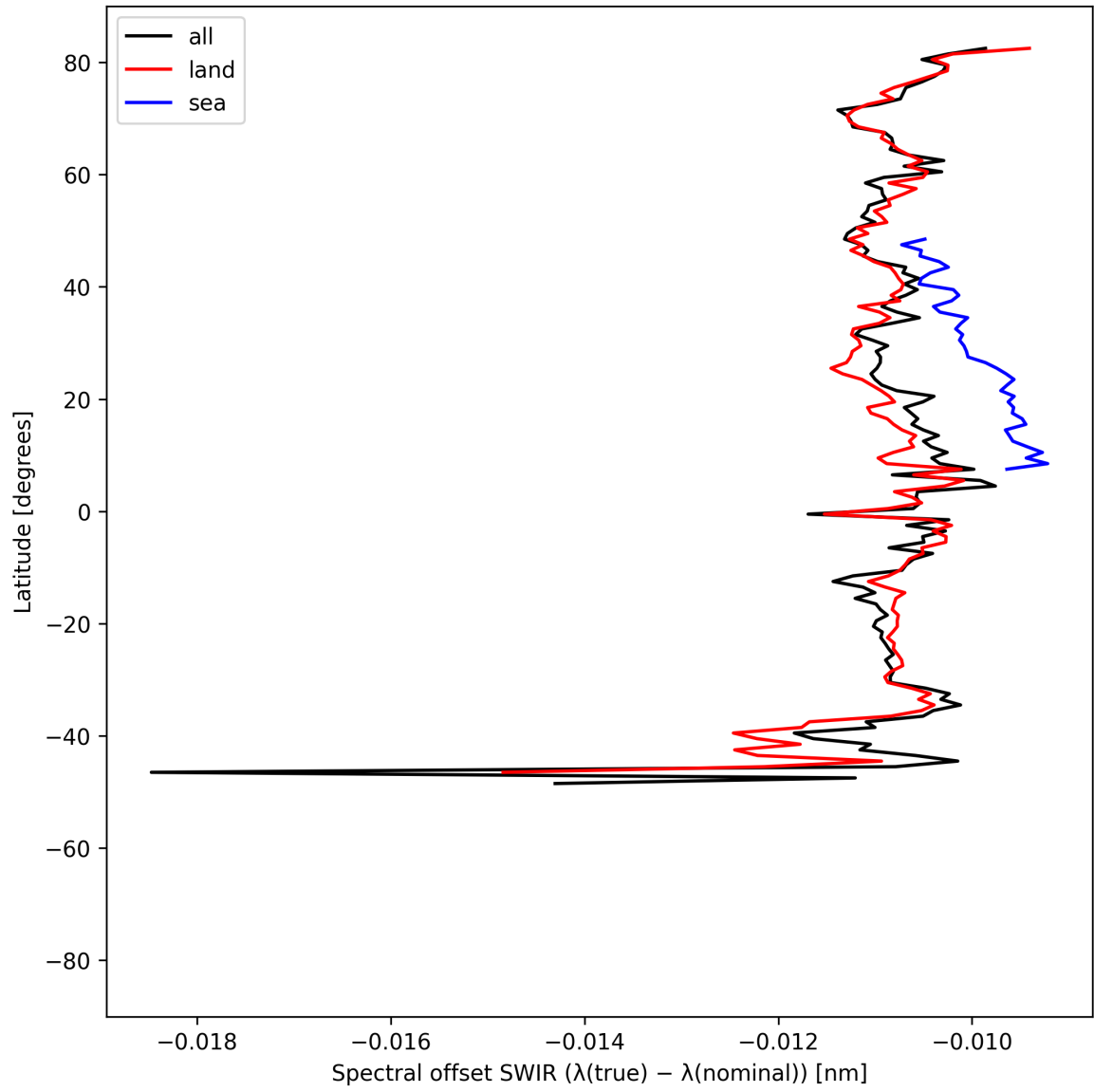
Figure 16: Zonal average of “Spectral offset SWIR ( \lambda_{\text{true}} - \lambda_{\text{nominal}} )” for 2025-05-29 to 2025-05-31.
