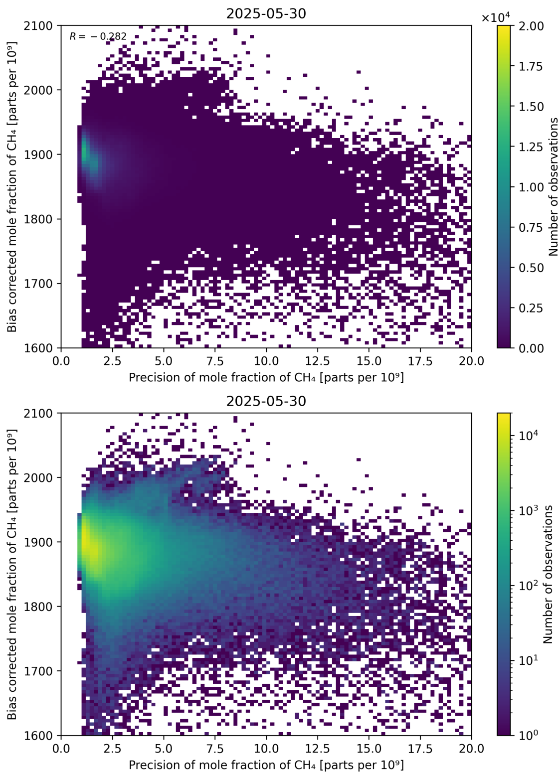
Figure 82: Scatter density plot of “Precision of mole fraction of CH 4 ” against “Bias corrected mole fraction of CH 4 ” for 2025-05-29 to 2025-05-31.
