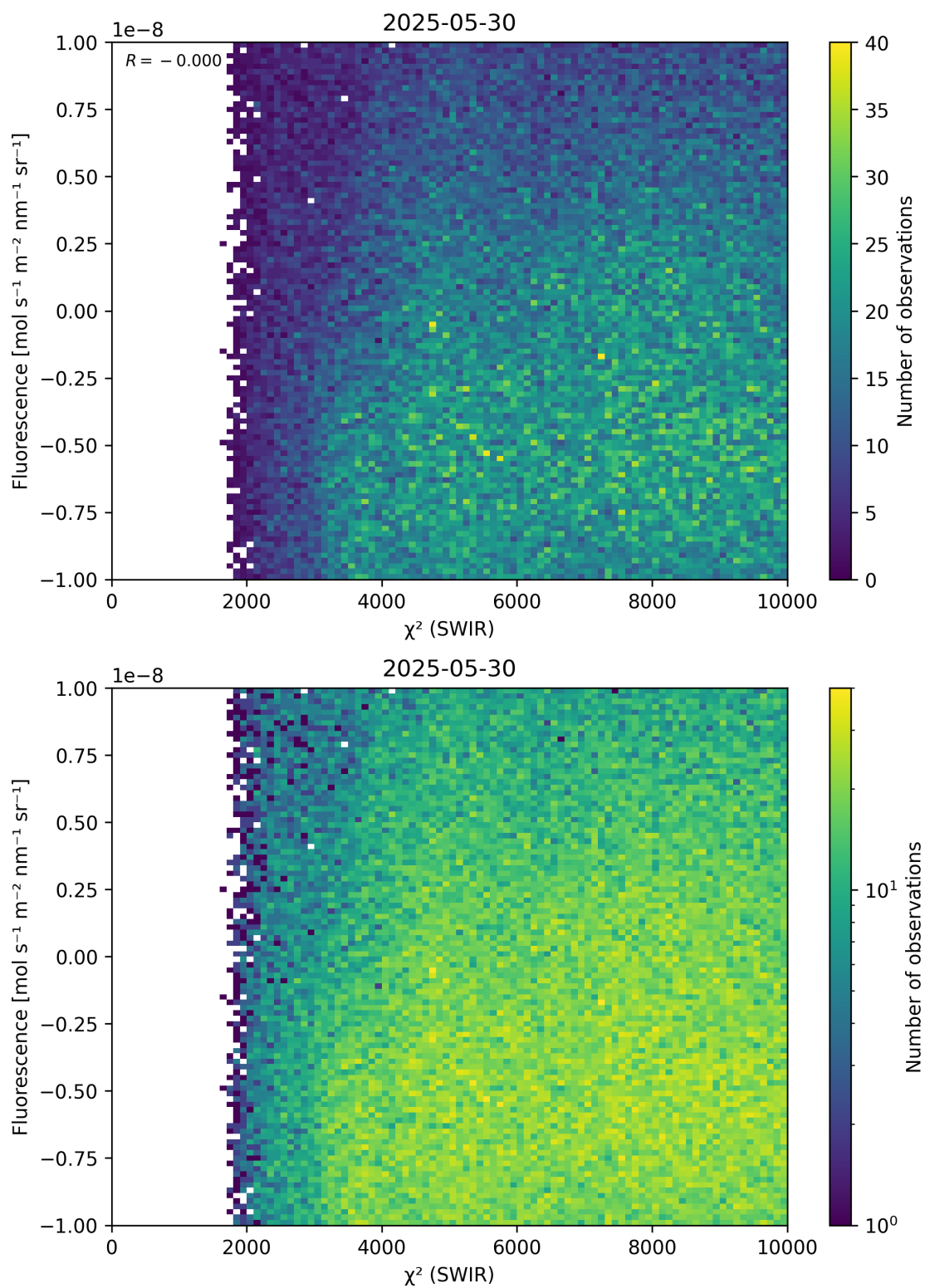
Figure 49: Scatter density plot of “ \chi^2 (SWIR)” against “Fluorescence” for 2025-05-29 to 2025-05-31.
