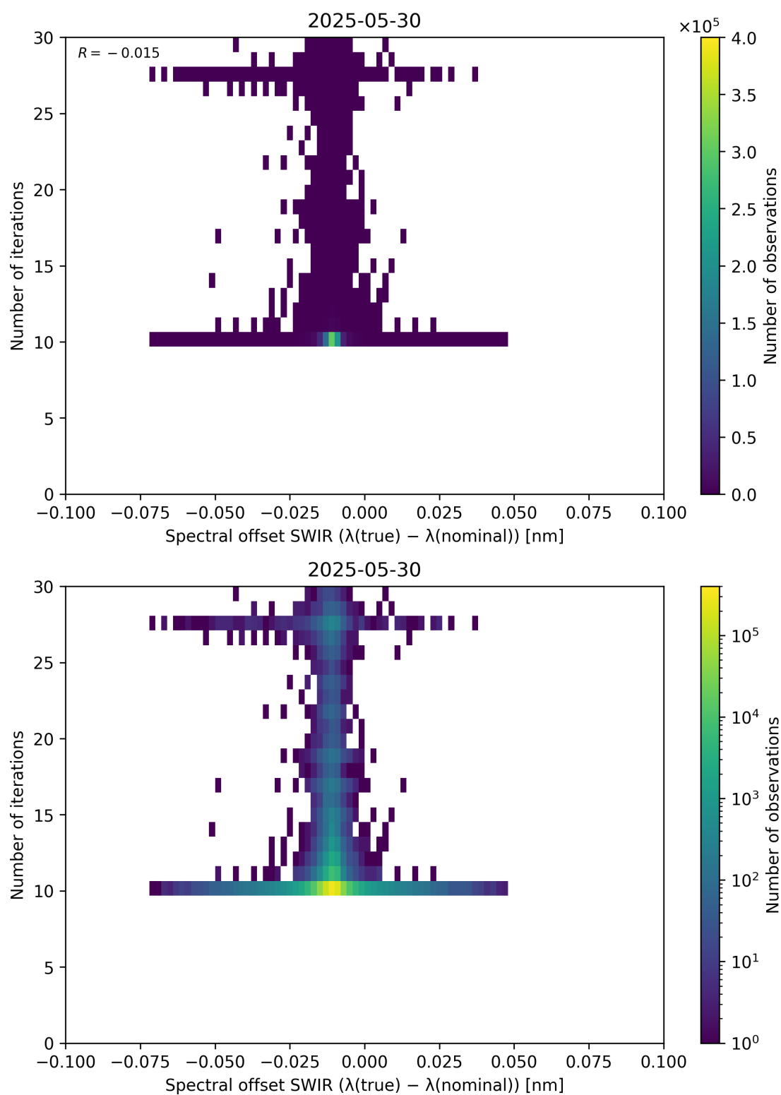
Figure 121: Scatter density plot of “Spectral offset SWIR ( \lambda_{\text{true}} - \lambda_{\text{nominal}} )” against “Number of iterations” for 2025-05-29 to 2025-05-31.
