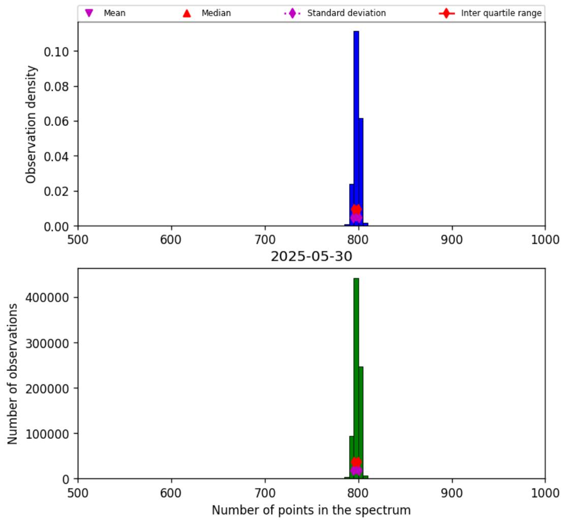
Figure 26: Histogram of “Number of points in the spectrum” for 2025-05-29 to 2025-05-31
