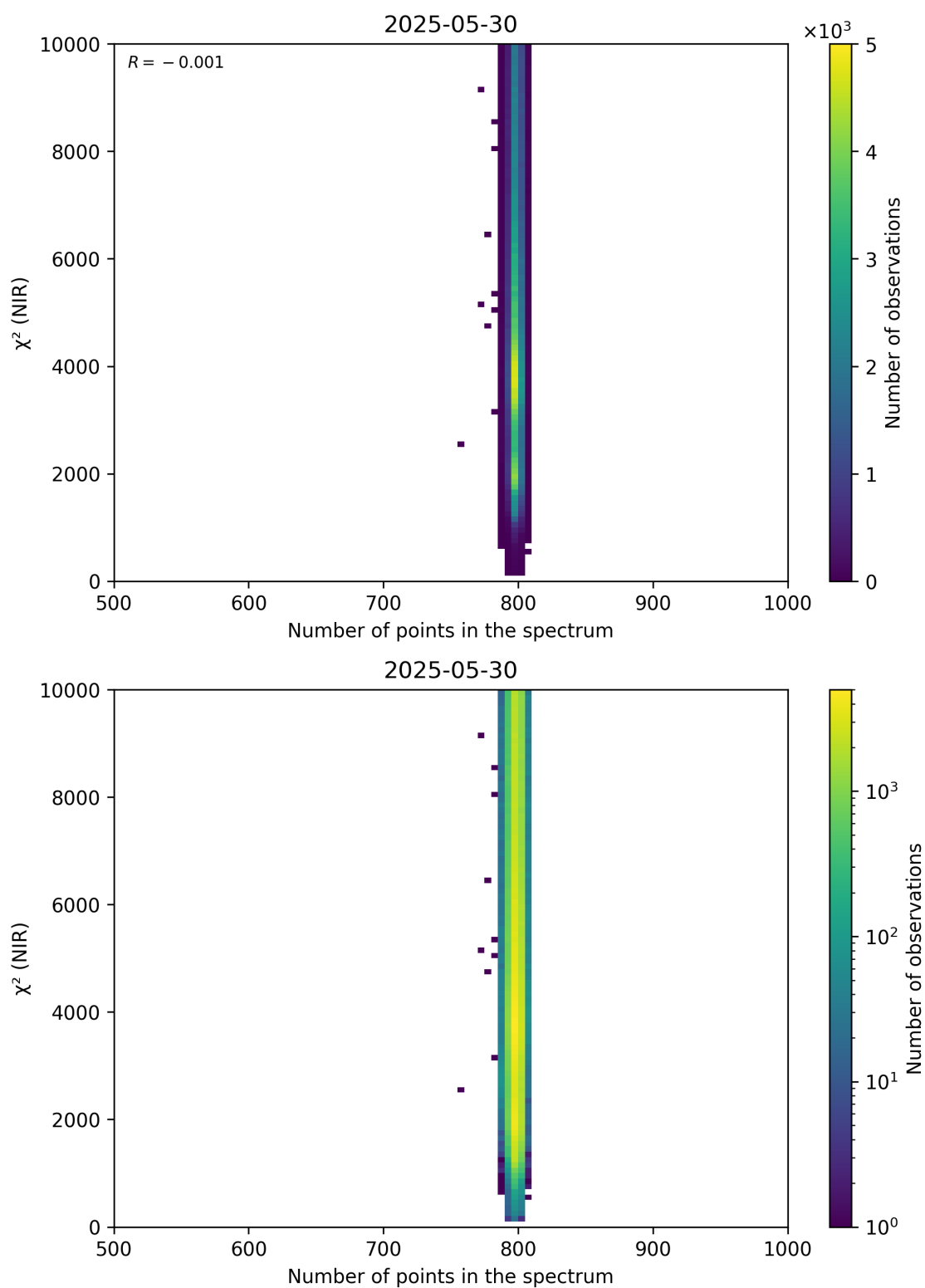
Figure 88: Scatter density plot of “Number of points in the spectrum” against “ \chi^2 (NIR)” for 2025-05-29 to 2025-05-31.
