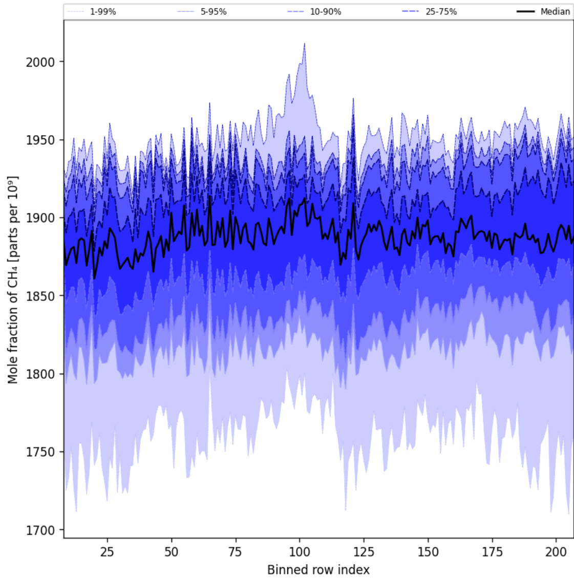
Figure 34: Along track statistics of “Mole fraction of CH 4 ” for 2025-05-29 to 2025-05-31
