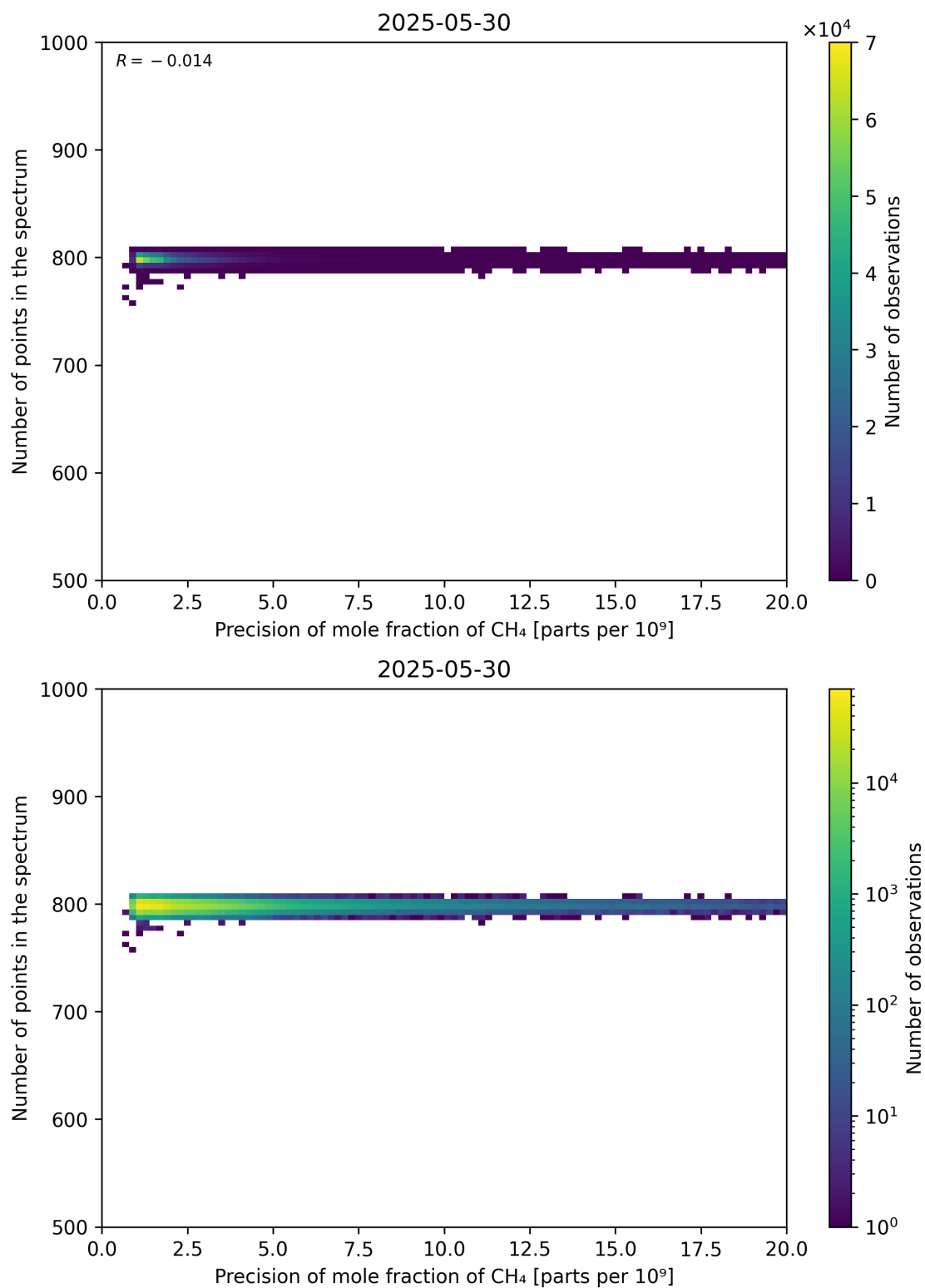
Figure 84: Scatter density plot of “Precision of mole fraction of CH 4 ” against “Number of points in the spectrum” for 2025-05-29 to 2025-05-31.
