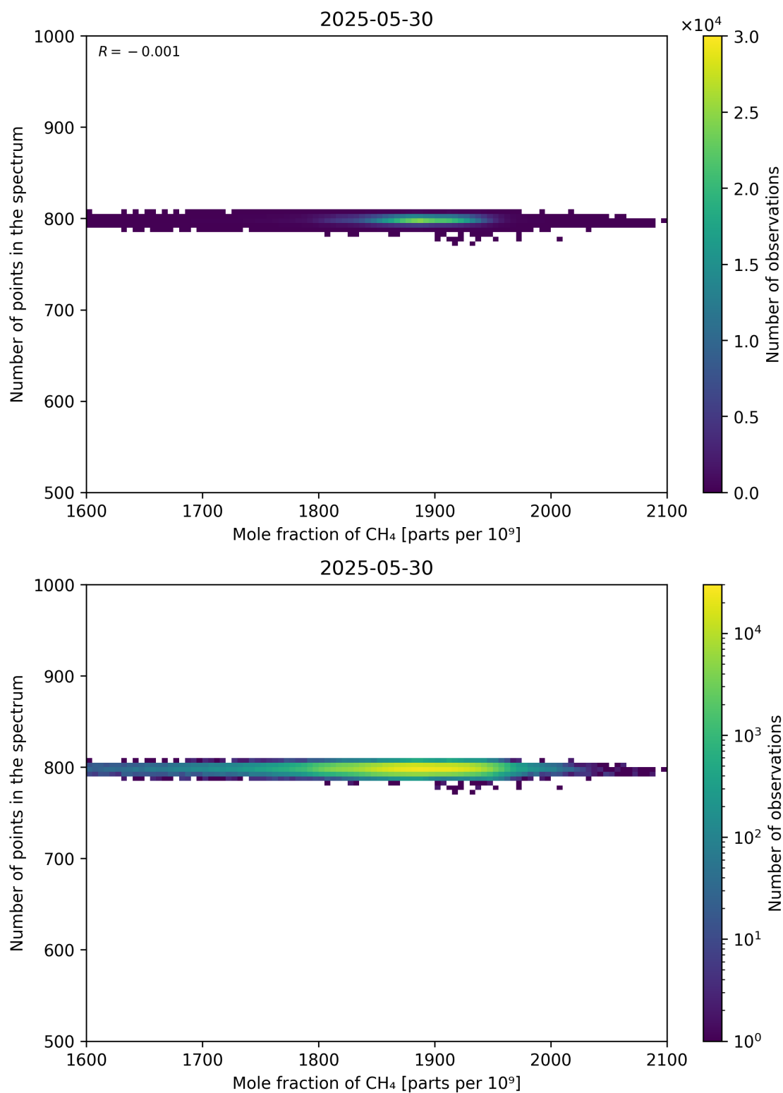
Figure 77: Scatter density plot of “Mole fraction of CH 4 ” against “Number of points in the spectrum” for 2025-05-29 to 2025-05-31.
