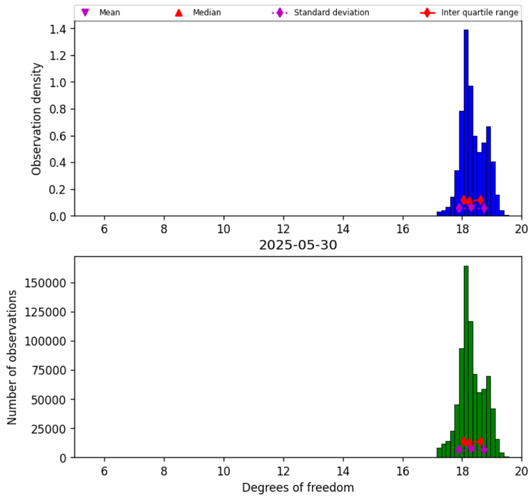
Figure 30: Histogram of “Degrees of freedom” for 2025-05-29 to 2025-05-31
