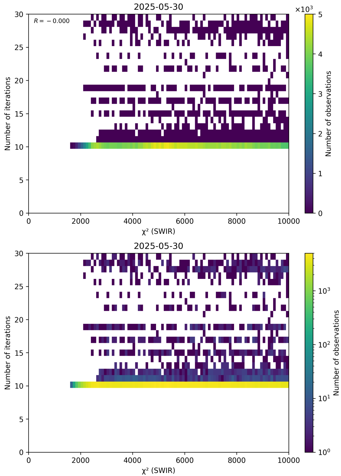
Figure 50: Scatter density plot of “ \chi^2 (SWIR)” against “Number of iterations” for 2025-05-29 to 2025-05-31.
