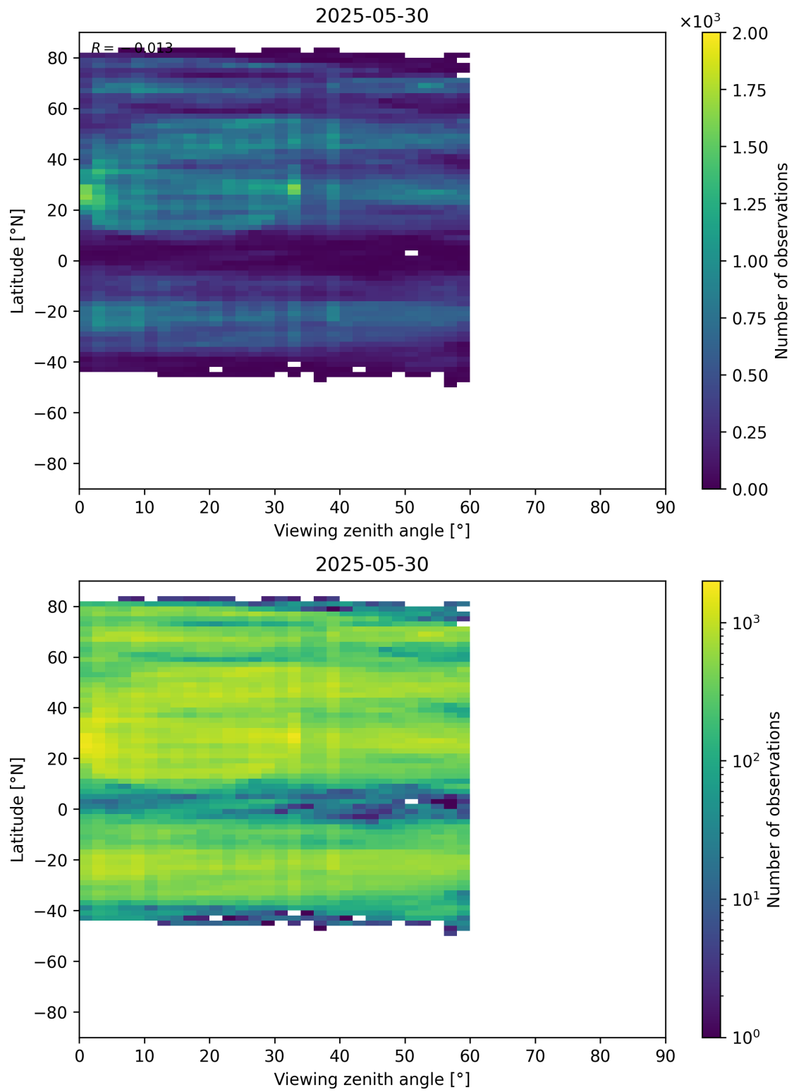
Figure 109: Scatter density plot of “Viewing zenith angle” against “Latitude” for 2025-05-29 to 2025-05-31.
