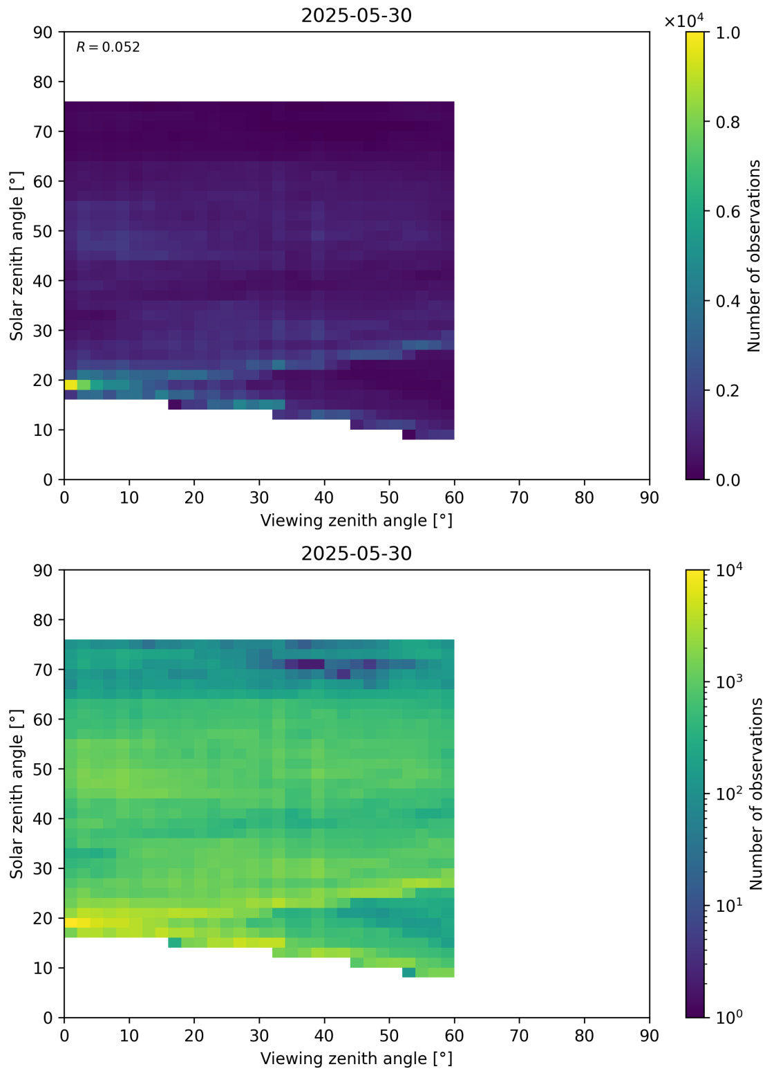
Figure 115: Scatter density plot of “Viewing zenith angle” against “Solar zenith angle” for 2025-05-29 to 2025-05-31.
