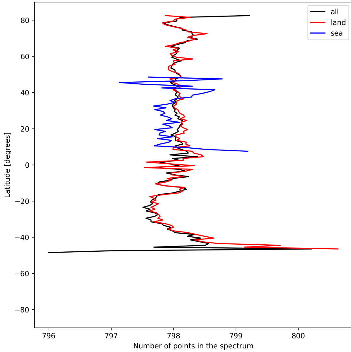
Figure 15: Zonal average of “Number of points in the spectrum” for 2025-05-29 to 2025-05-31.
