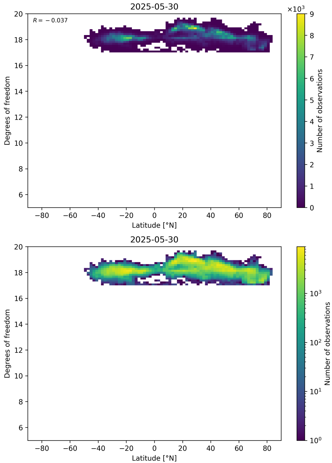
Figure 55: Scatter density plot of “Latitude” against “Degrees of freedom” for 2025-05-29 to 2025-05-31.
