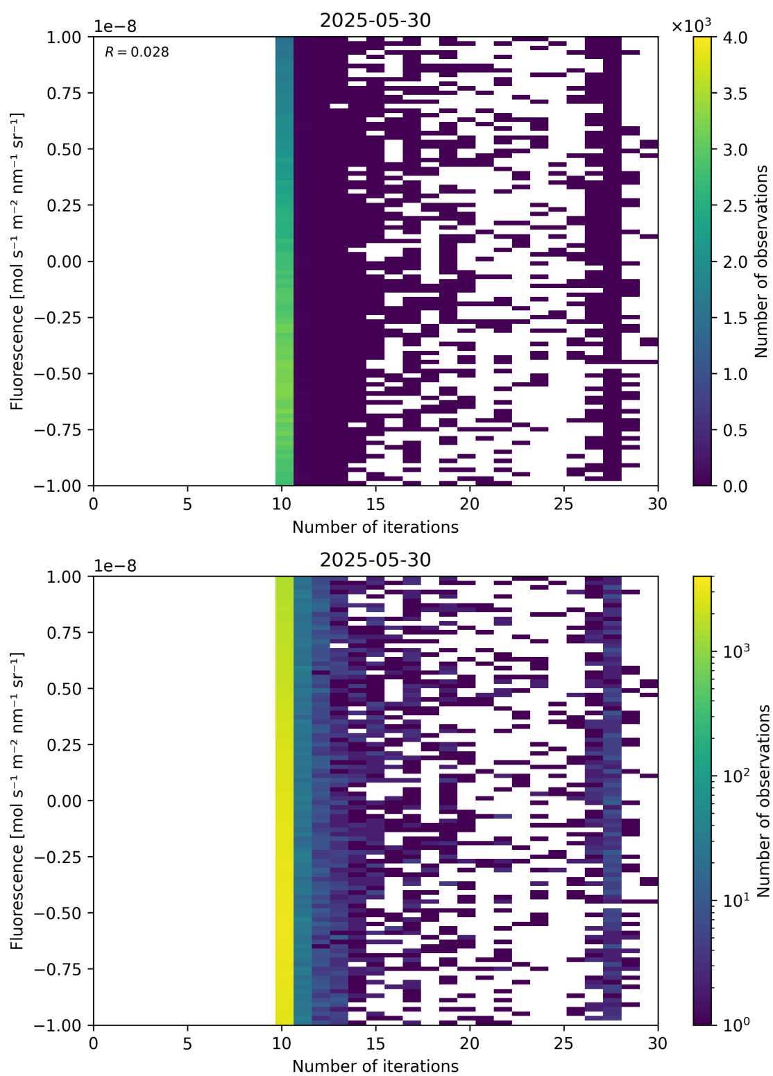
Figure 87: Scatter density plot of “Number of iterations” against “Fluorescence” for 2025-05-29 to 2025-05-31.
