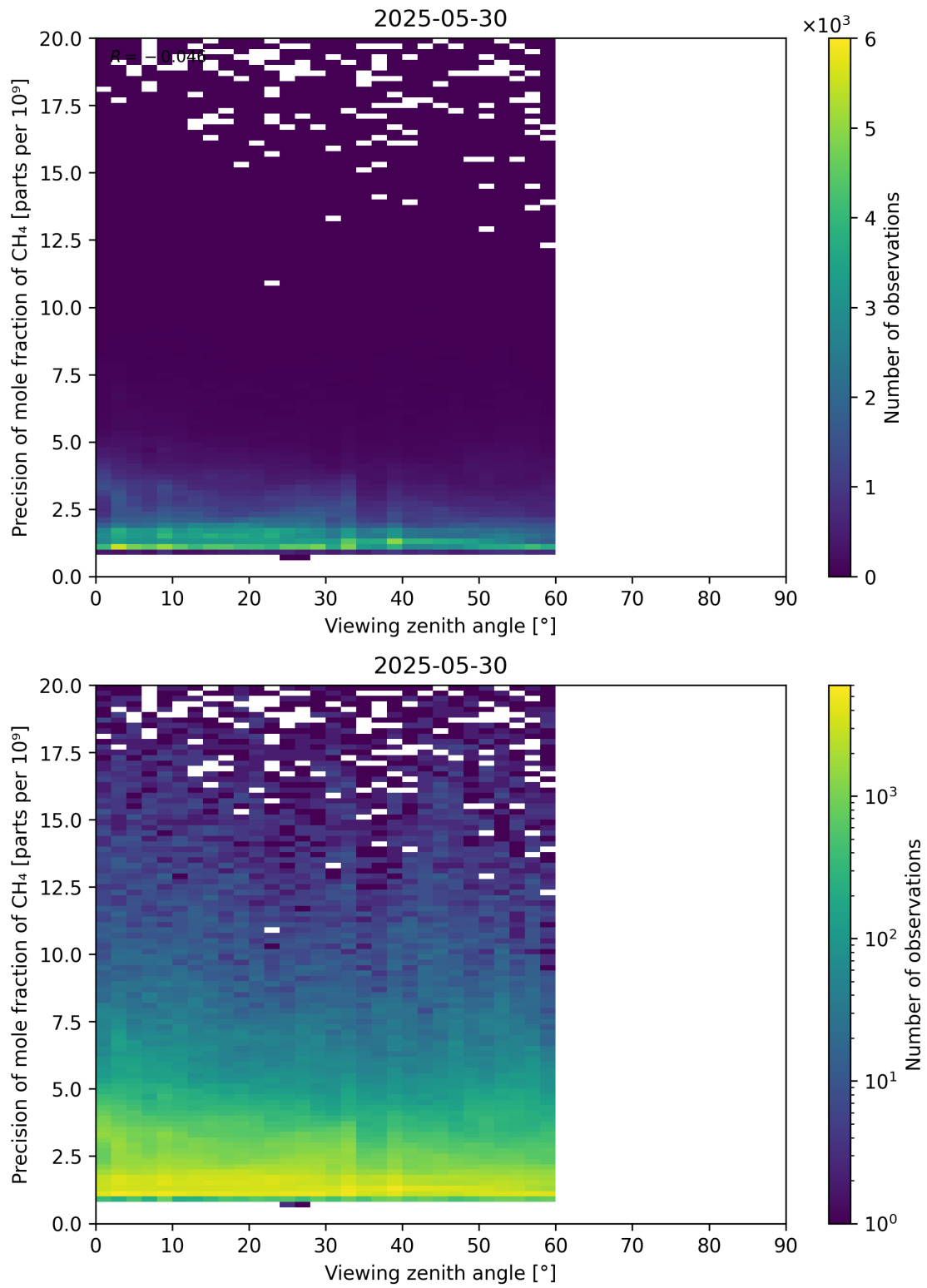
Figure 112: Scatter density plot of “Viewing zenith angle” against “Precision of mole fraction of CH 4 ” for 2025-05-29 to 2025-05-31.
