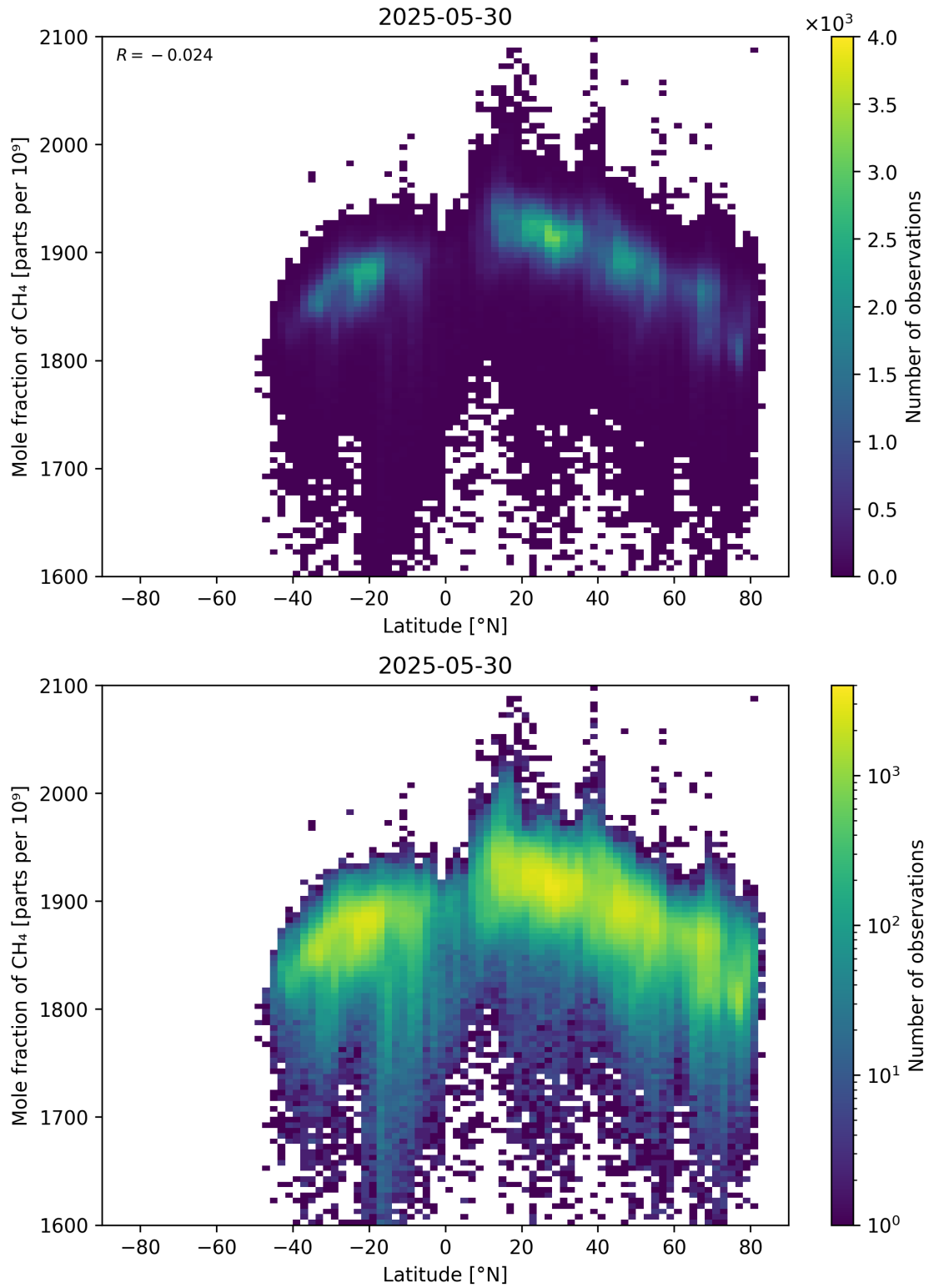
Figure 57: Scatter density plot of “Latitude” against “Mole fraction of CH 4 ” for 2025-05-29 to 2025-05-31.
