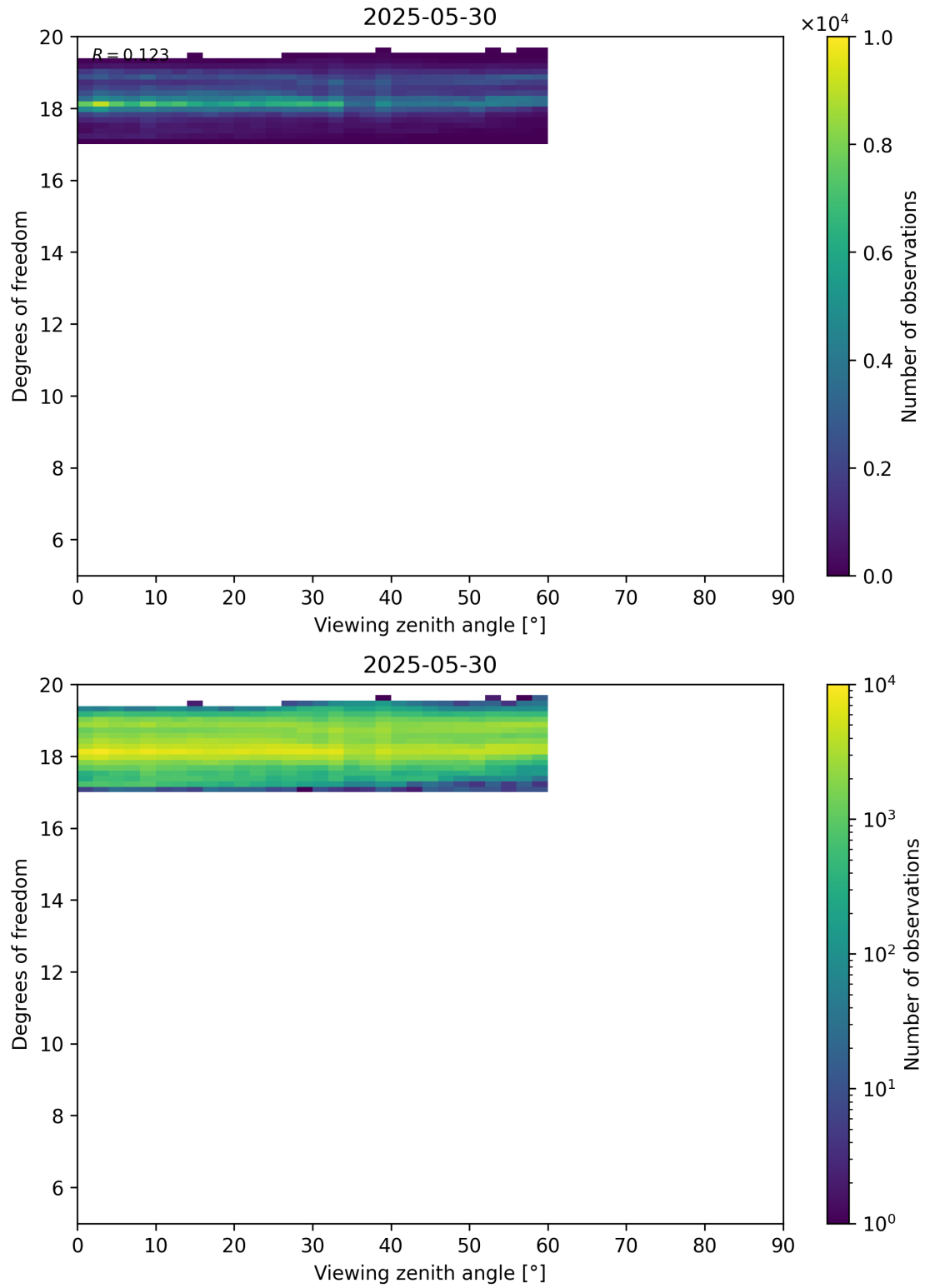
Figure 107: Scatter density plot of “Viewing zenith angle” against “Degrees of freedom” for 2025-05-29 to 2025-05-31.
