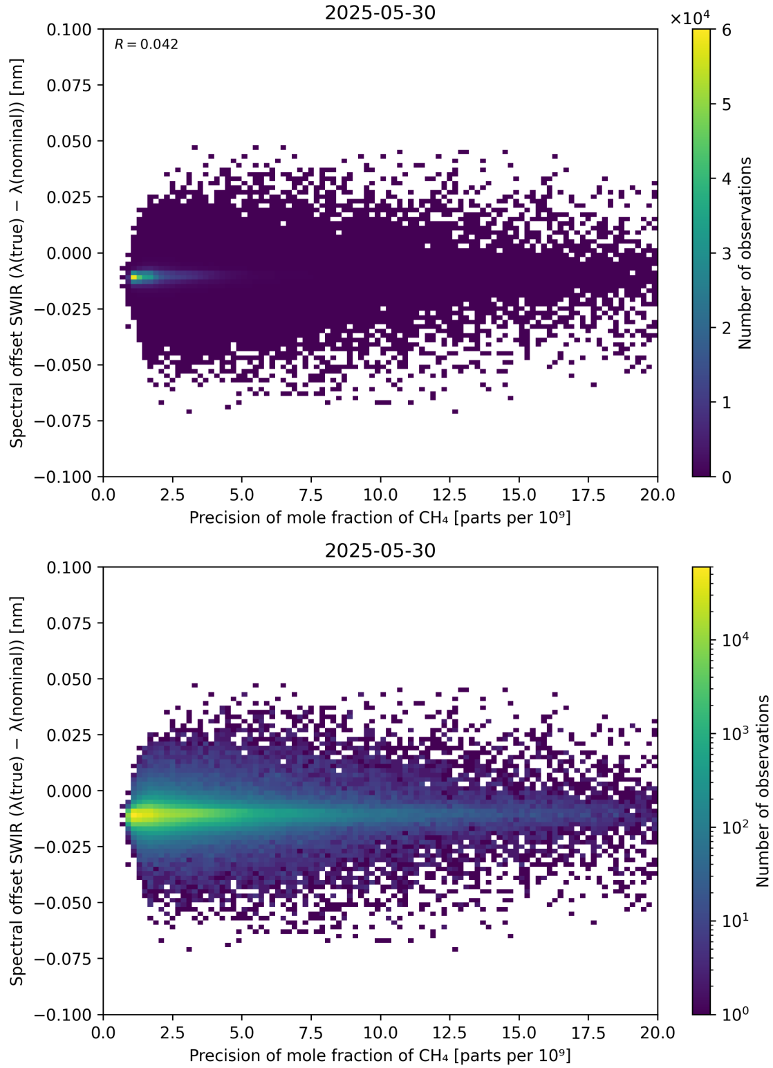
Figure 85: Scatter density plot of “Precision of mole fraction of CH 4 ” against “Spectral offset SWIR ( \lambda_{\text{true}} - \lambda_{\text{nominal}} )” for 2025-05-29 to 2025-05-31.
