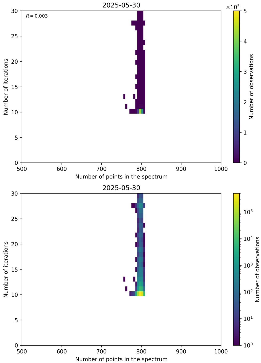
Figure 92: Scatter density plot of “Number of points in the spectrum” against “Number of iterations” for 2025-05-29 to 2025-05-31.
