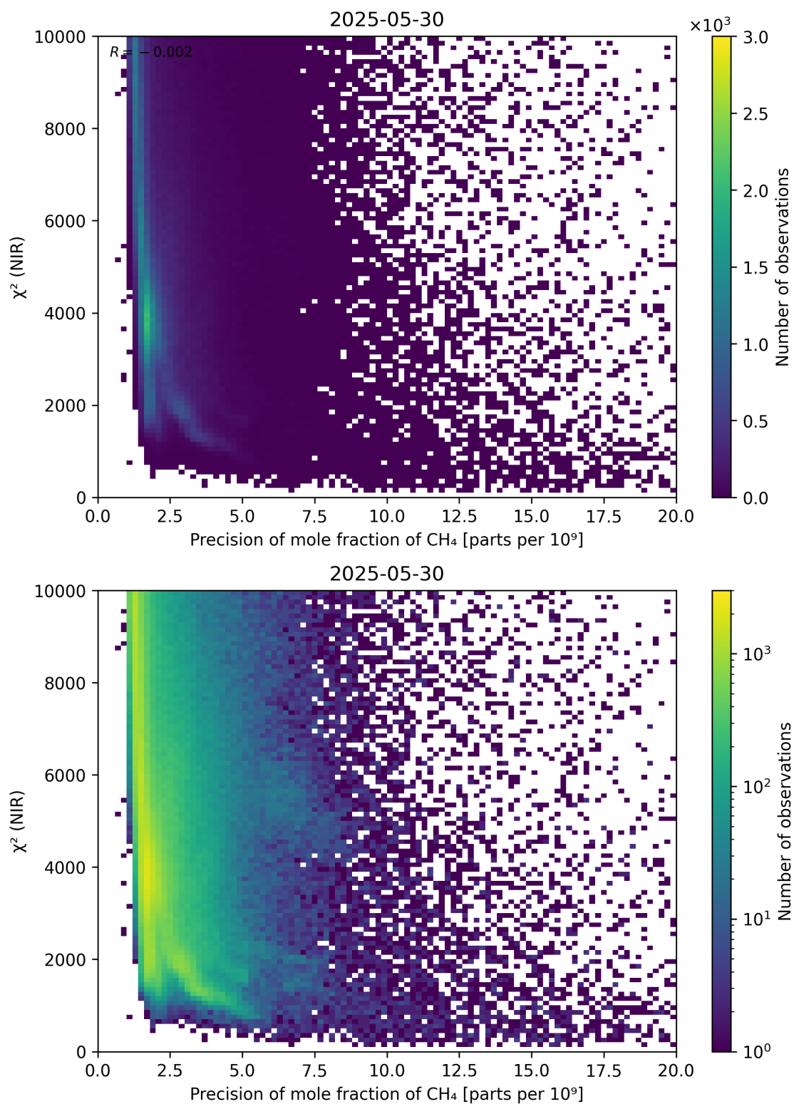
Figure 78: Scatter density plot of “Precision of mole fraction of \text{CH}_4 ” against “ \chi^2 (NIR)” for 2025-05-29 to 2025-05-31.
