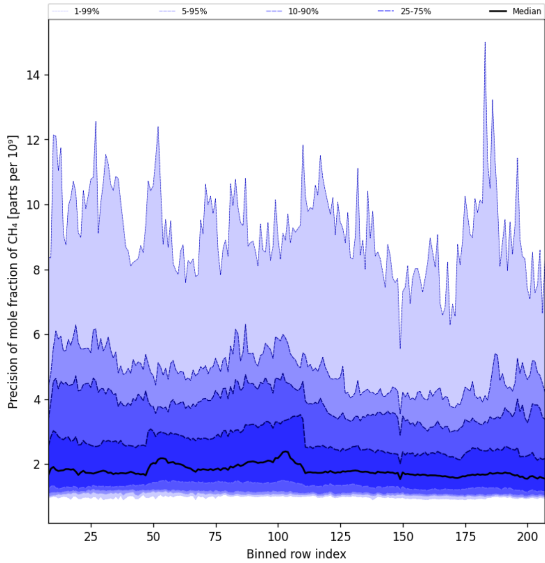
Figure 35: Along track statistics of “Precision of mole fraction of CH 4 ” for 2025-05-29 to 2025-05-31
