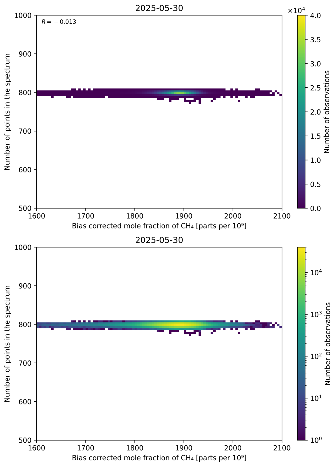
Figure 68: Scatter density plot of “Bias corrected mole fraction of CH 4 ” against “Number of points in the spectrum” for 2025-05-29 to 2025-05-31.
