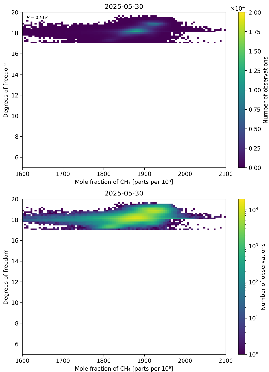
Figure 72: Scatter density plot of “Mole fraction of CH 4 ” against “Degrees of freedom” for 2025-05-29 to 2025-05-31.
