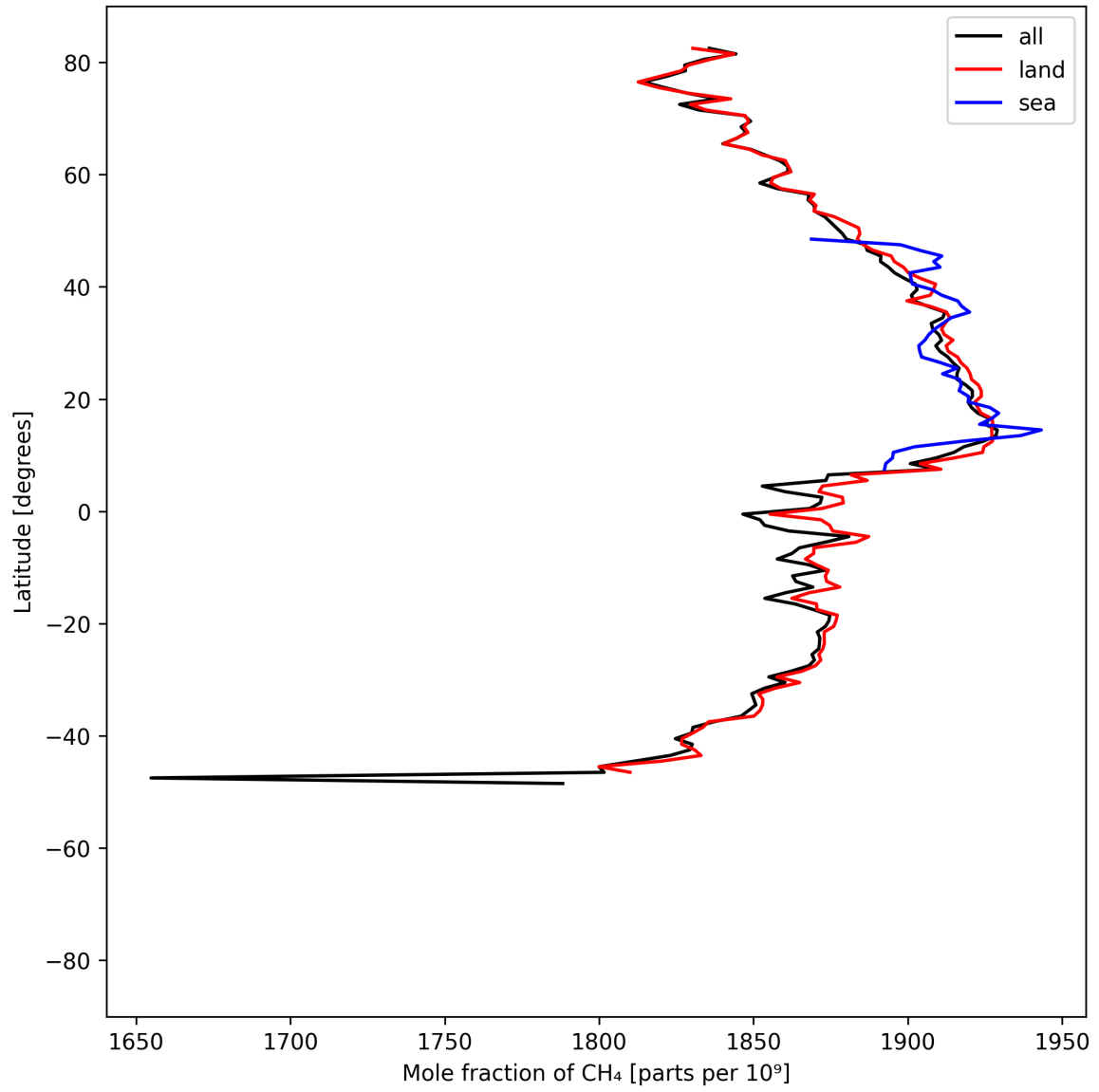
Figure 12: Zonal average of “Mole fraction of CH 4 ” for 2025-05-29 to 2025-05-31.
