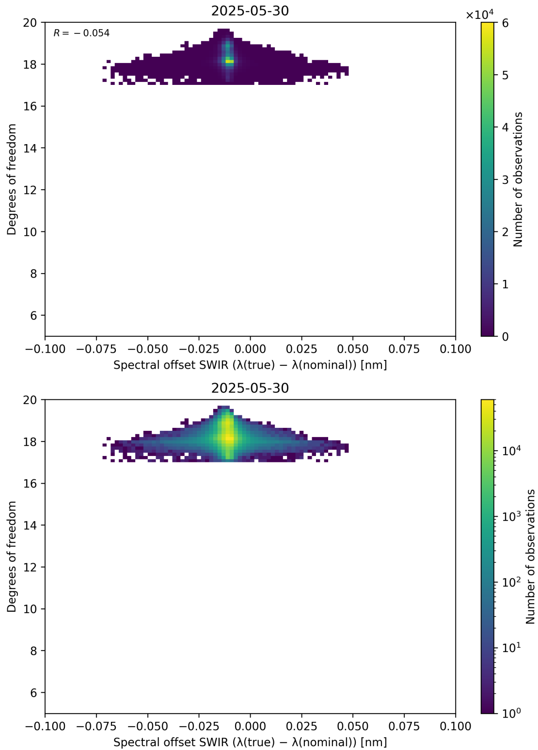
Figure 119: Scatter density plot of “Spectral offset SWIR ( \lambda_{\text{true}} - \lambda_{\text{nominal}} )” against “Degrees of freedom” for 2025-05-29 to 2025-05-31.
