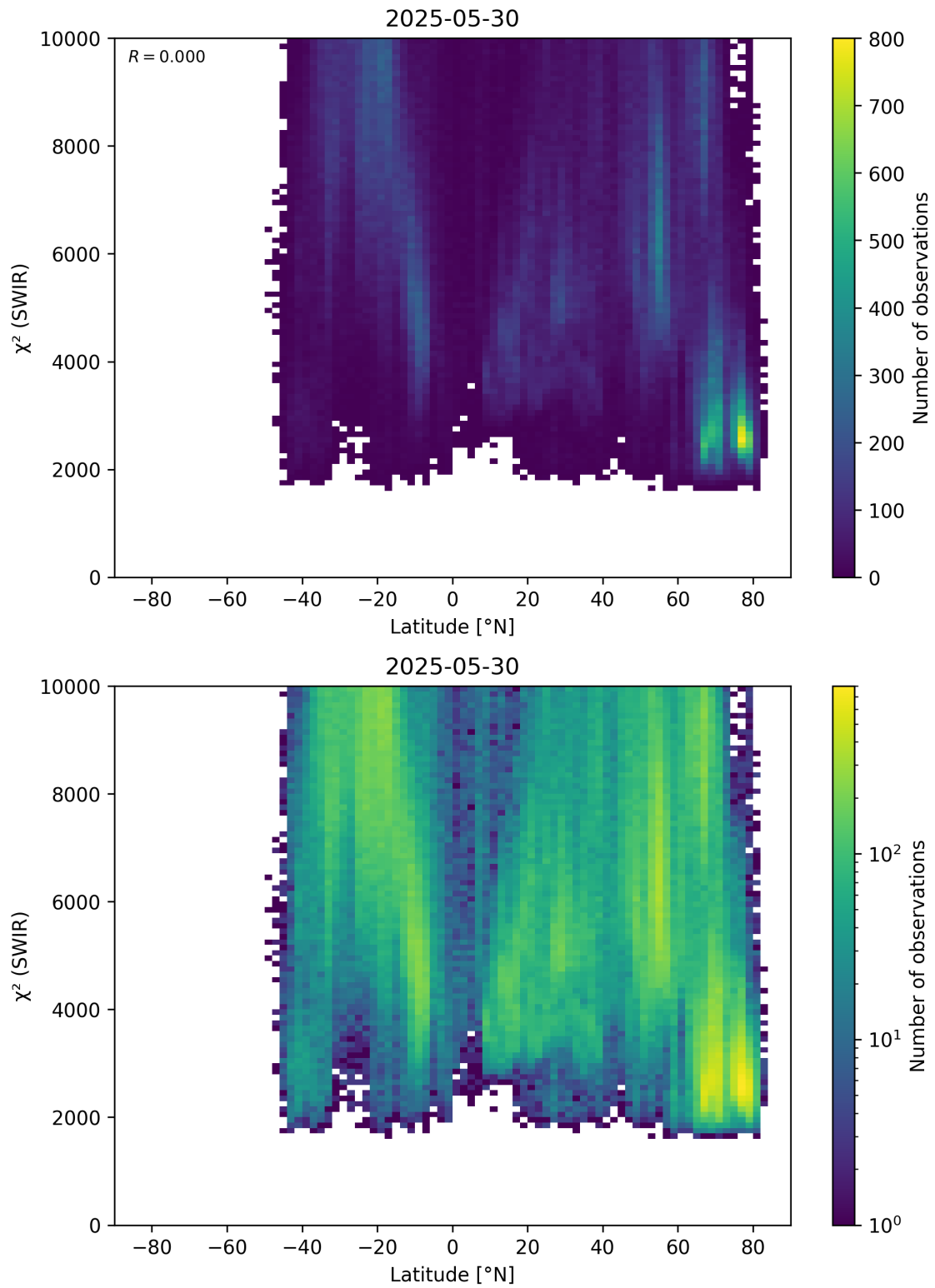
Figure 54: Scatter density plot of “Latitude” against “ \chi^2 (SWIR)” for 2025-05-29 to 2025-05-31.
