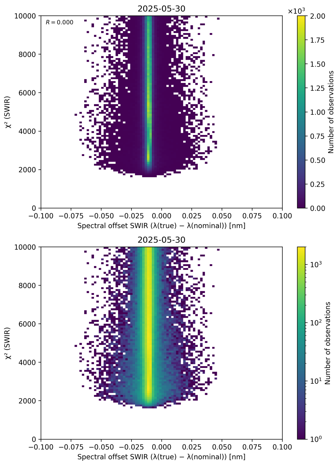
Figure 118: Scatter density plot of “Spectral offset SWIR ( \lambda_{\text{true}} - \lambda_{\text{nominal}} )” against “ \chi^2 (SWIR)” for 2025-05-29 to 2025-05-31.
