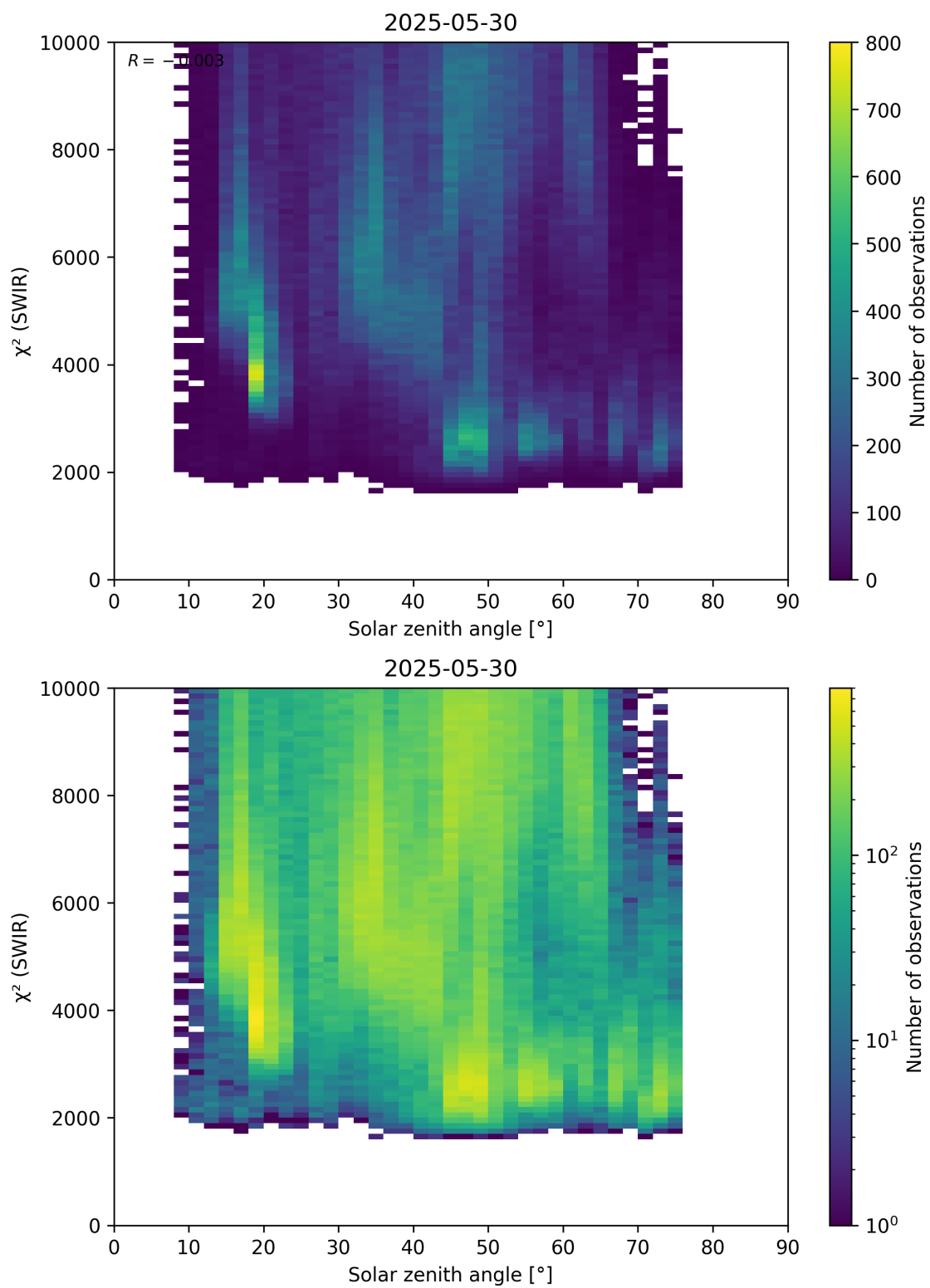
Figure 95: Scatter density plot of “Solar zenith angle” against “ \chi^2 (SWIR)” for 2025-05-29 to 2025-05-31.
