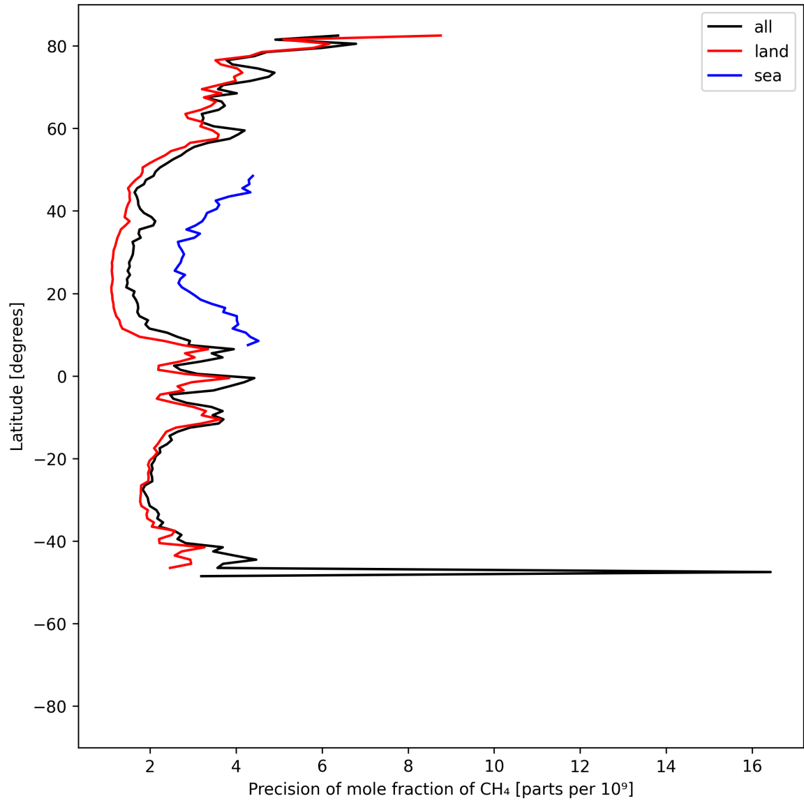
Figure 13: Zonal average of “Precision of mole fraction of CH 4 ” for 2025-05-29 to 2025-05-31.
