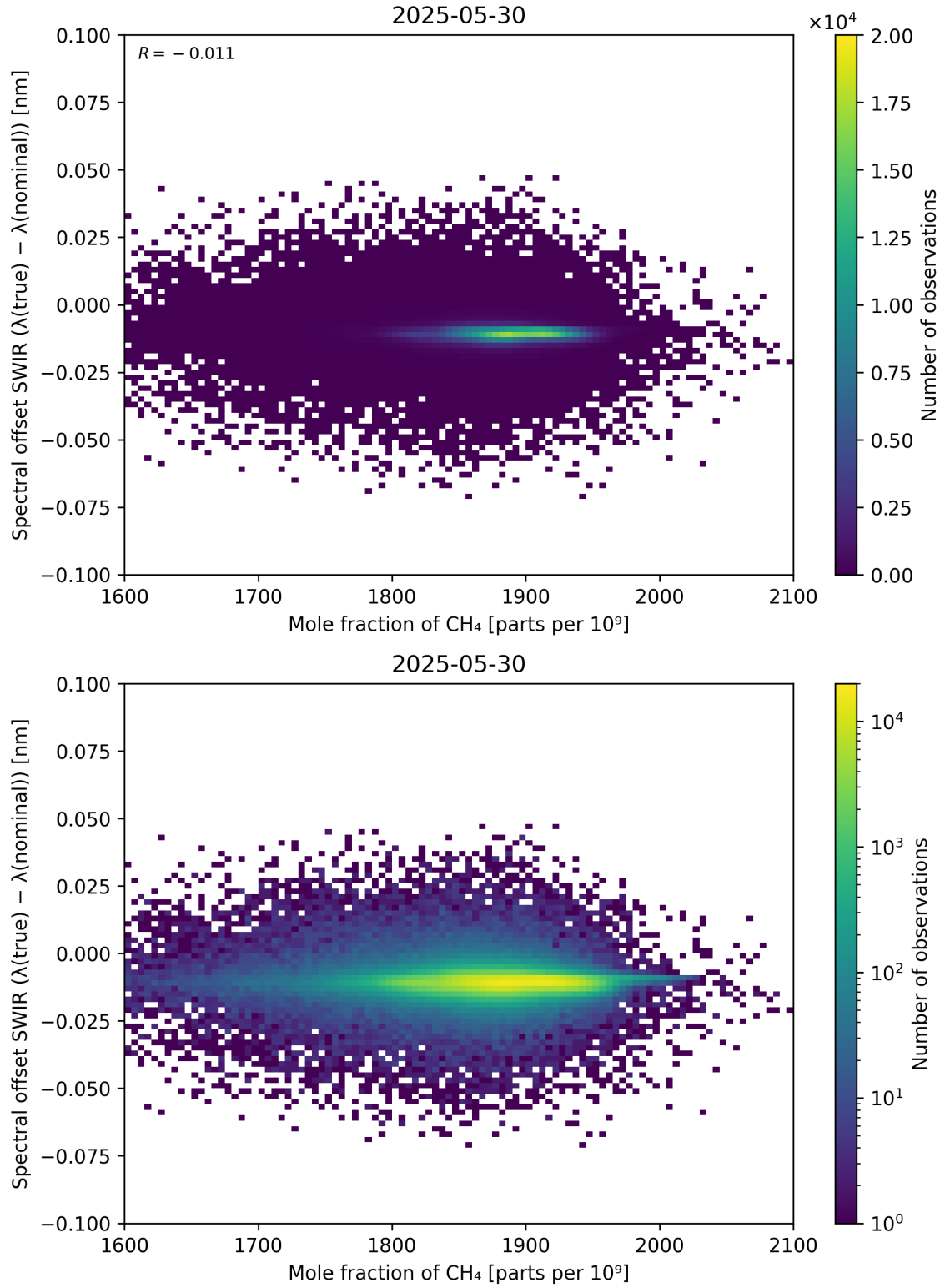
Figure 86: Scatter density plot of “Mole fraction of CH 4 ” against “Spectral offset SWIR ( \lambda_{\text{true}} - \lambda_{\text{nominal}} )” for 2025-05-29 to 2025-05-31.
