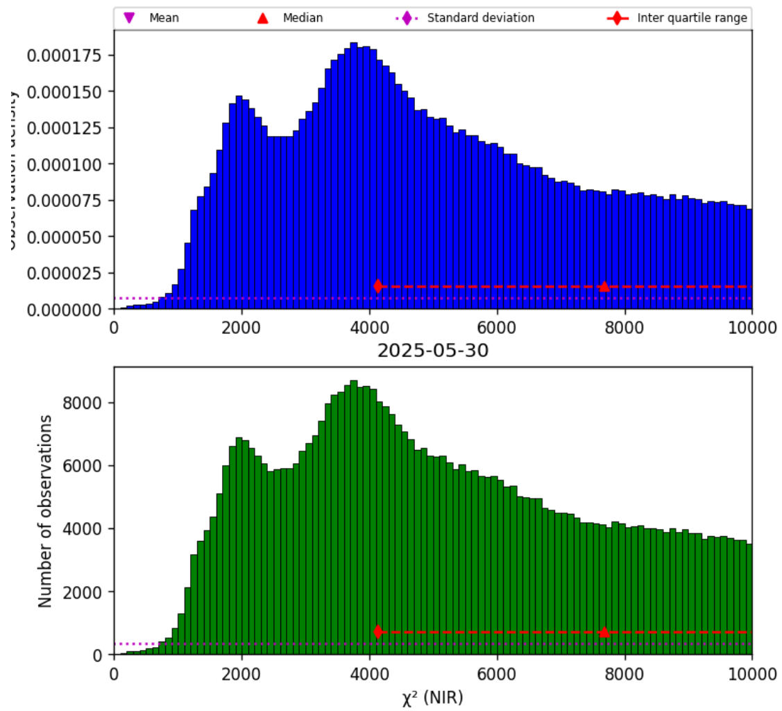
Figure 29: Histogram of “ \chi^2 (NIR)” for 2025-05-29 to 2025-05-31
