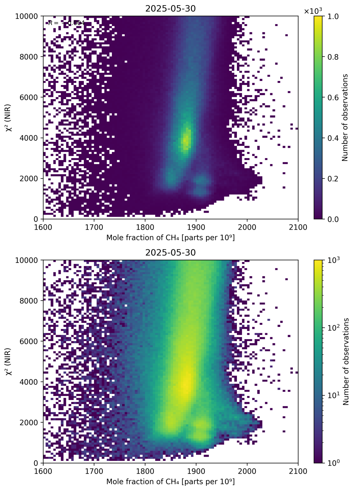
Figure 70: Scatter density plot of “Mole fraction of \text{CH}_4 ” against “ \chi^2 (NIR)” for 2025-05-29 to 2025-05-31.
