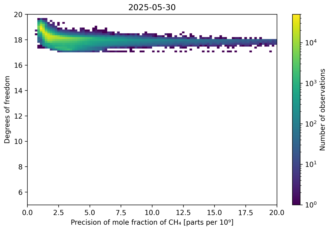
Figure 80: Scatter density plot of “Precision of mole fraction of CH 4 ” against “Degrees of freedom” for 2025-05-29 to 2025-05-31.
