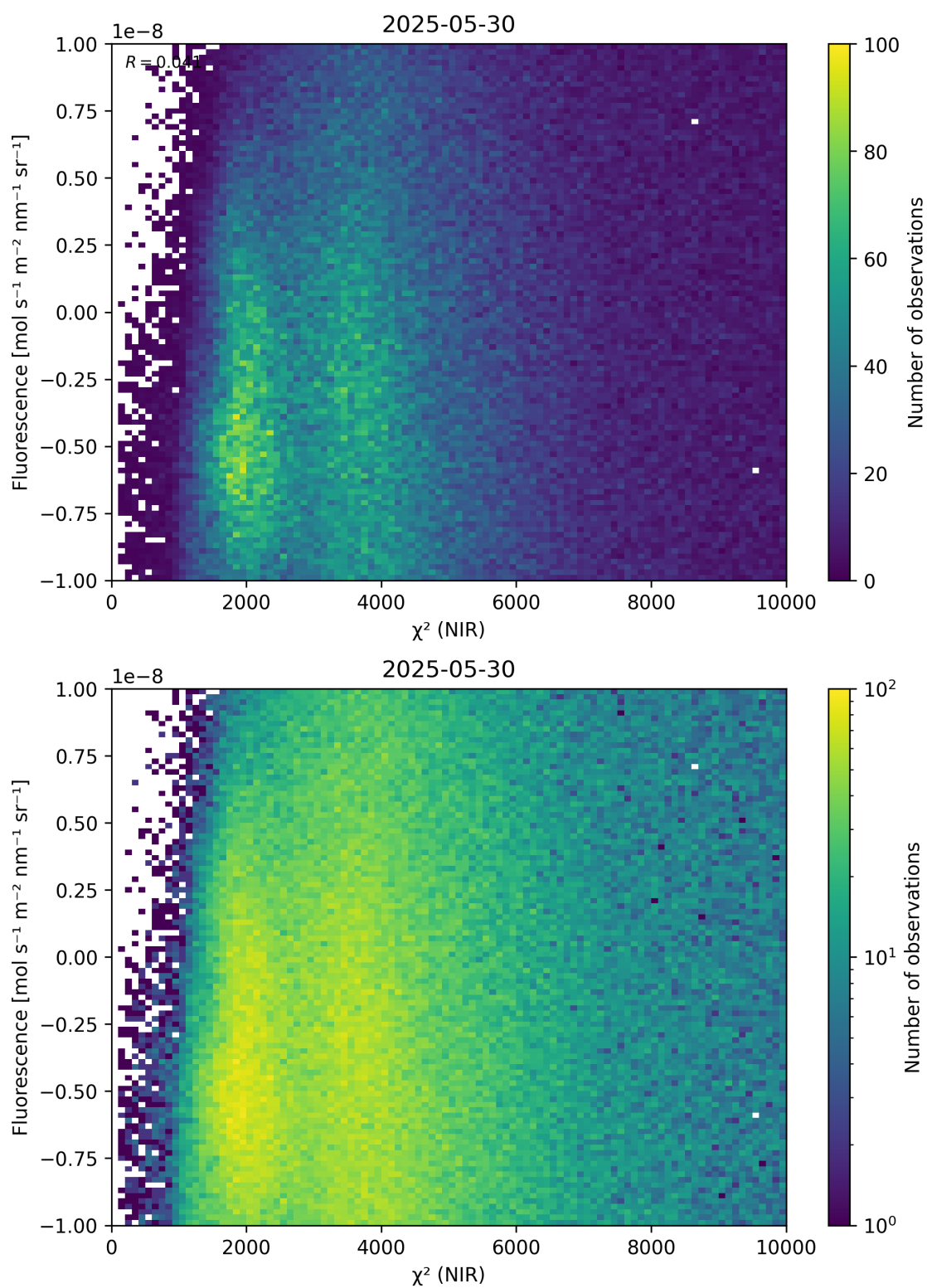
Figure 45: Scatter density plot of “ \chi^2 (NIR)” against “Fluorescence” for 2025-05-29 to 2025-05-31.
