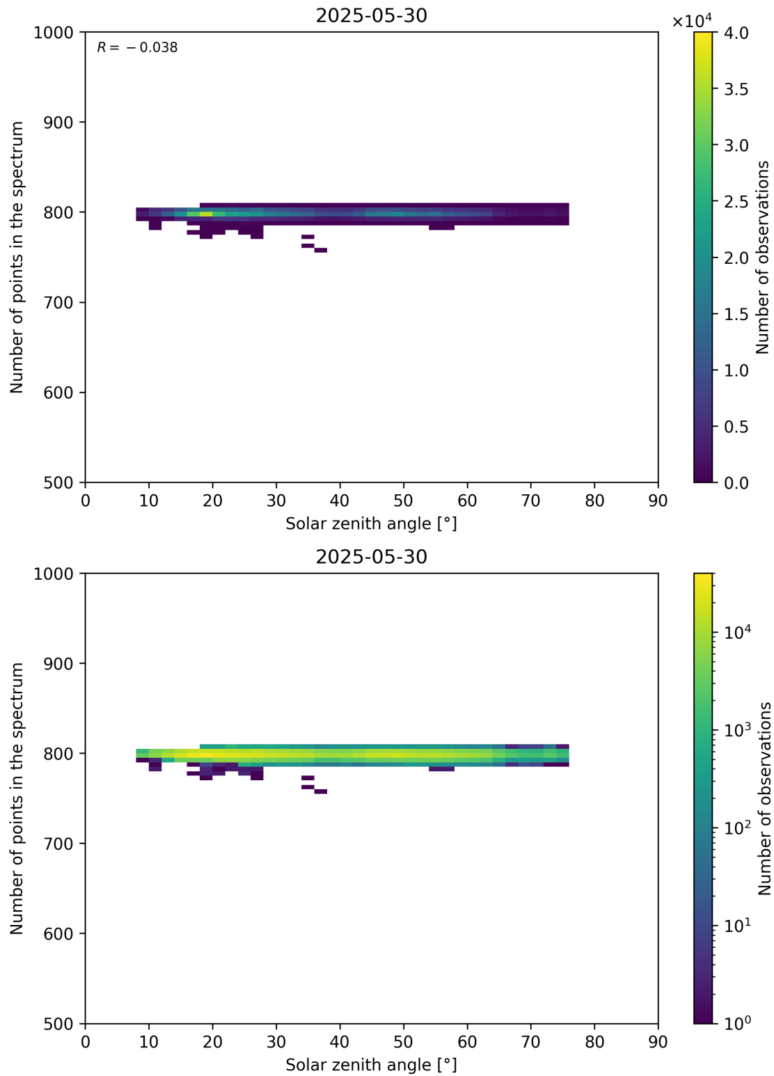
Figure 103: Scatter density plot of “Solar zenith angle” against “Number of points in the spectrum” for 2025-05-29 to 2025-05-31.
