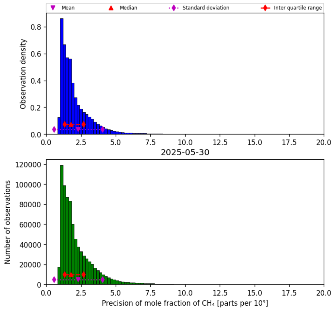
Figure 24: Histogram of “Precision of mole fraction of CH 4 ” for 2025-05-29 to 2025-05-31
