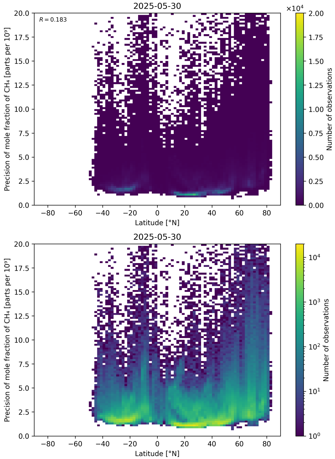
Figure 59: Scatter density plot of “Latitude” against “Precision of mole fraction of \text{CH}_4 ” for 2025-05-29 to 2025-05-31.
