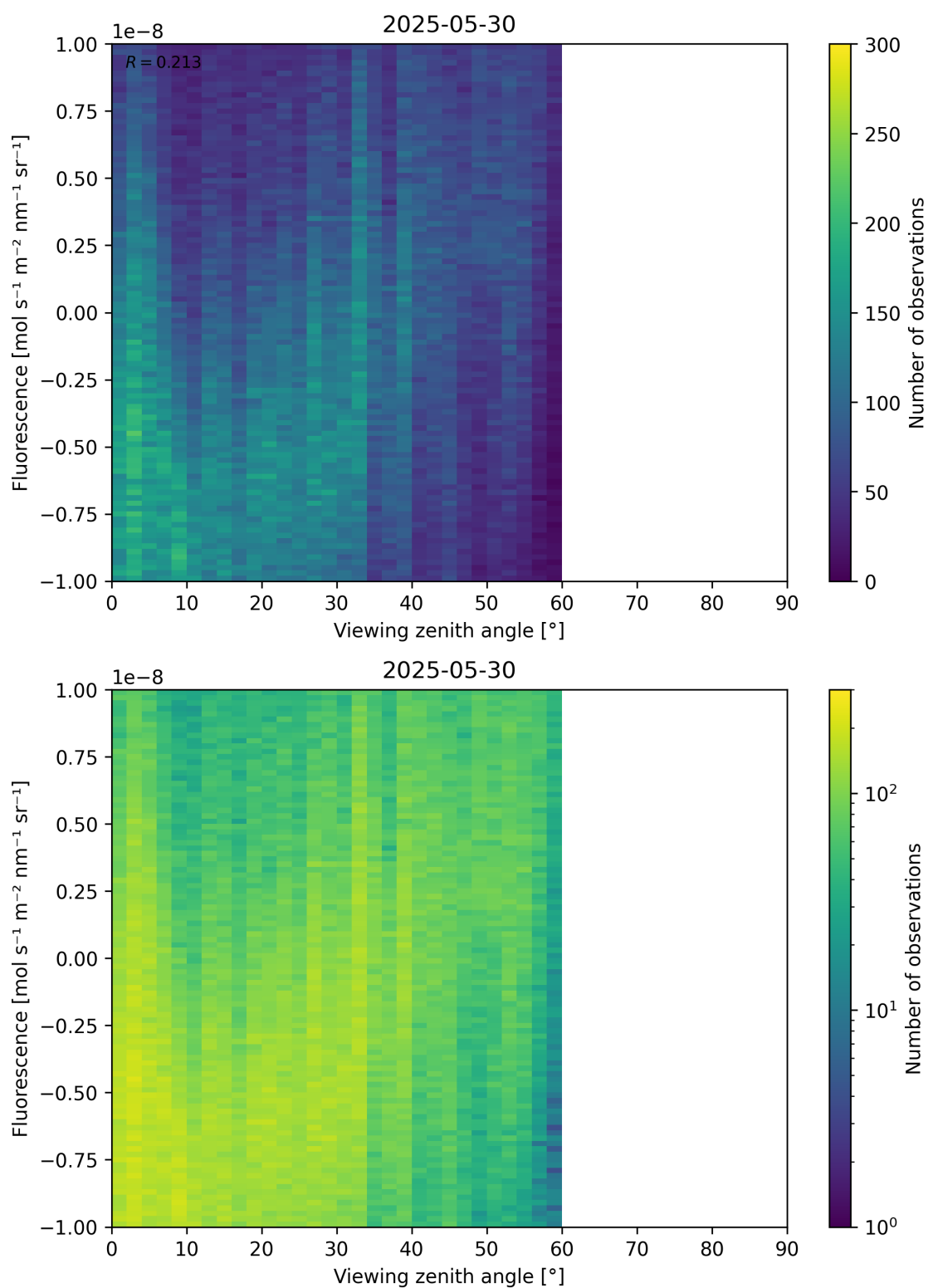
Figure 108: Scatter density plot of “Viewing zenith angle” against “Fluorescence” for 2025-05-29 to 2025-05-31.
