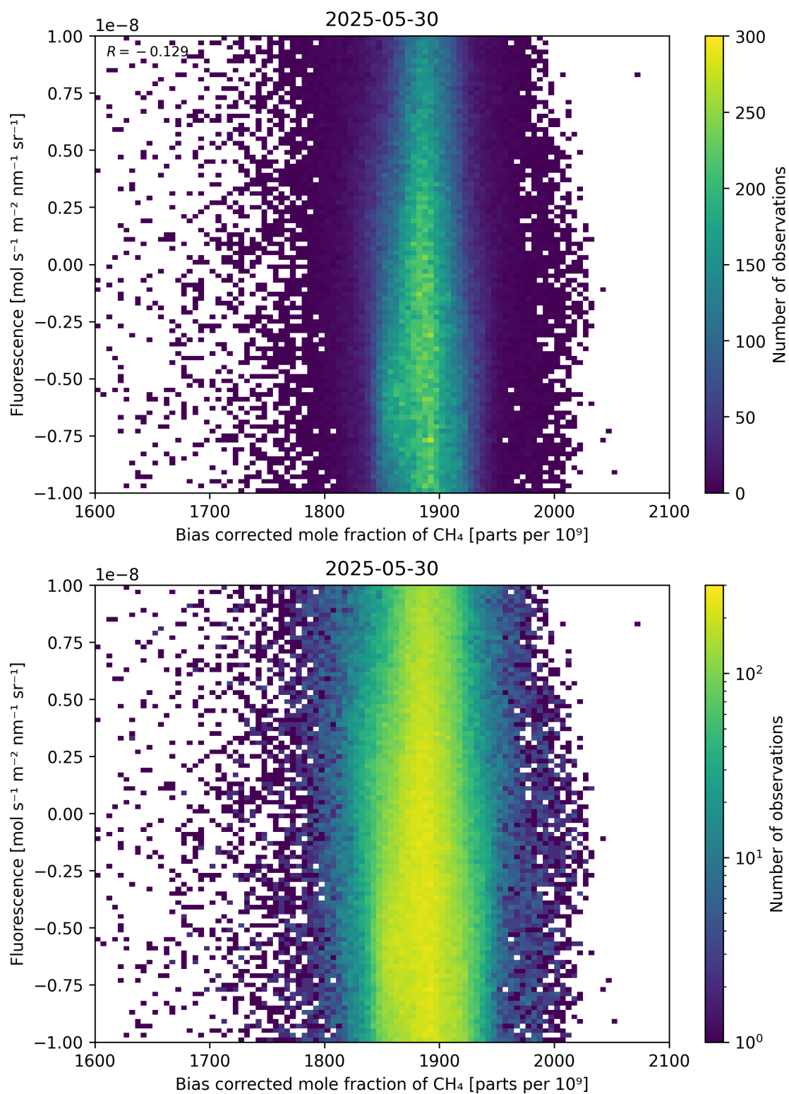
Figure 66: Scatter density plot of “Bias corrected mole fraction of \text{CH}_4 ” against “Fluorescence” for 2025-05-29 to 2025-05-31.
