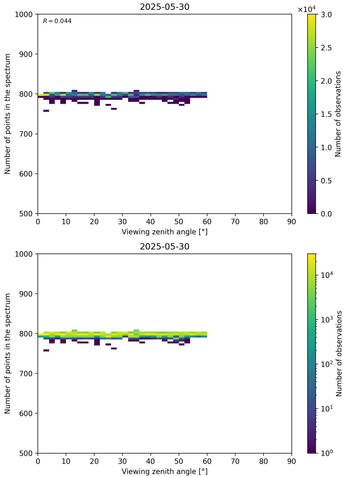
Figure 114: Scatter density plot of “Viewing zenith angle” against “Number of points in the spectrum” for 2025-05-29 to 2025-05-31.
