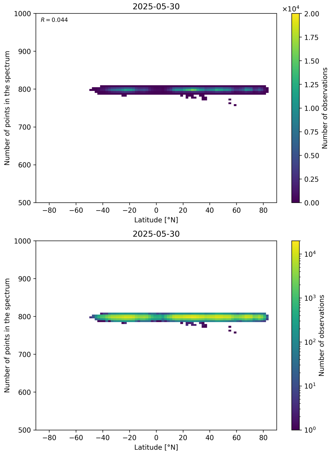
Figure 61: Scatter density plot of “Latitude” against “Number of points in the spectrum” for 2025-05-29 to 2025-05-31.
