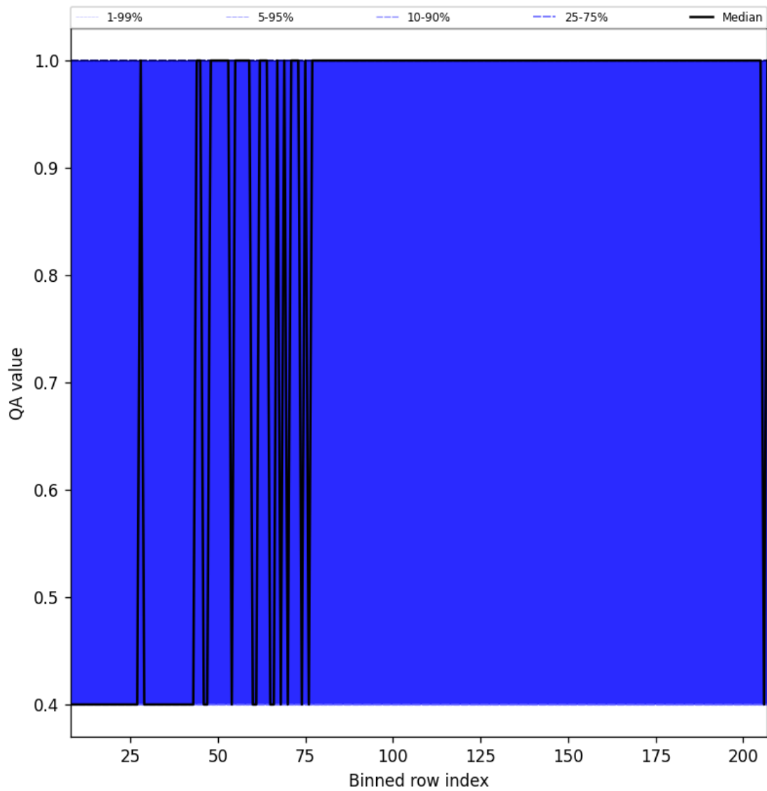
Figure 33: Along track statistics of “QA value” for 2025-05-29 to 2025-05-31
