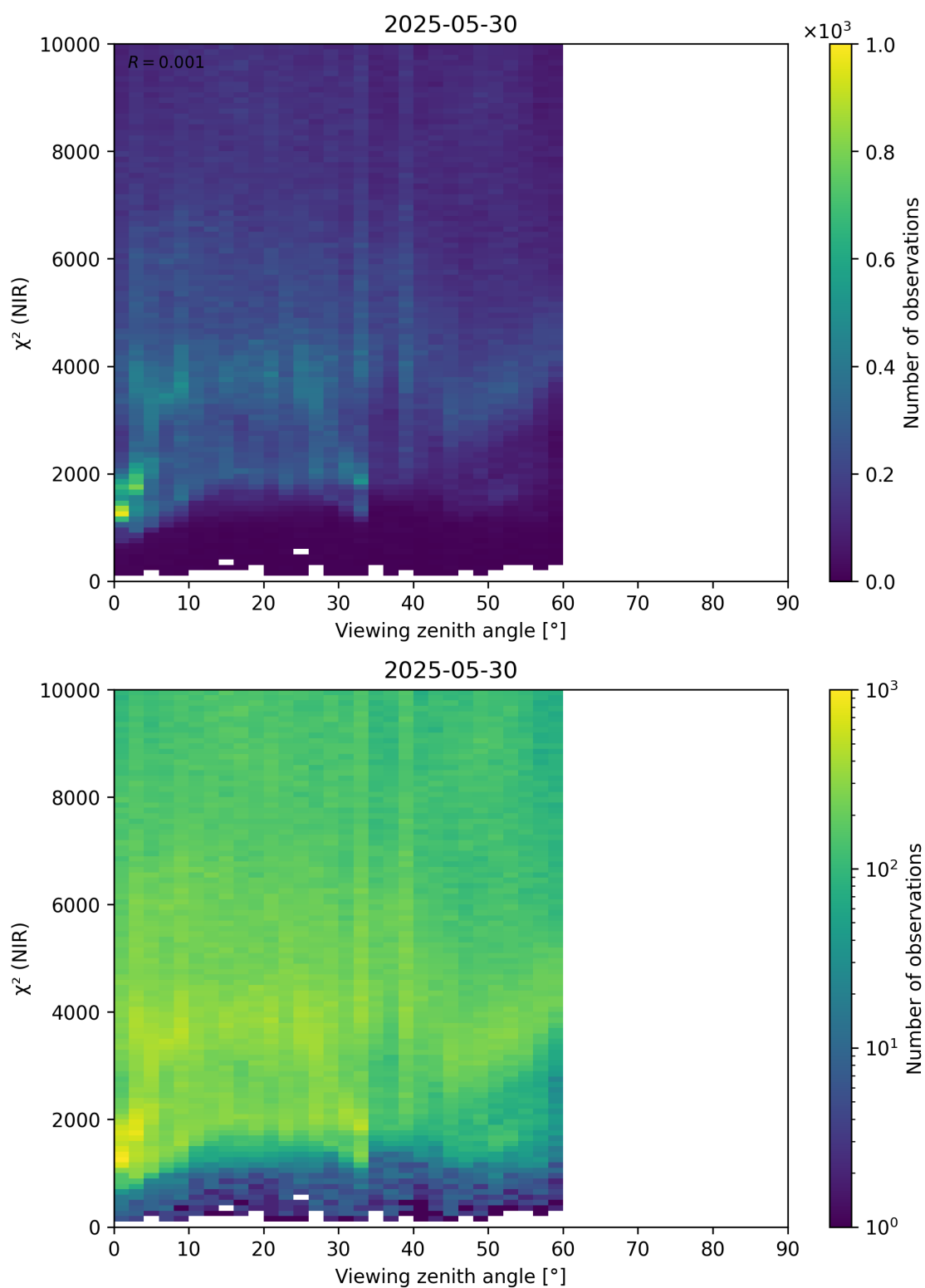
Figure 105: Scatter density plot of “Viewing zenith angle” against “ \chi^2 (NIR)” for 2025-05-29 to 2025-05-31.
