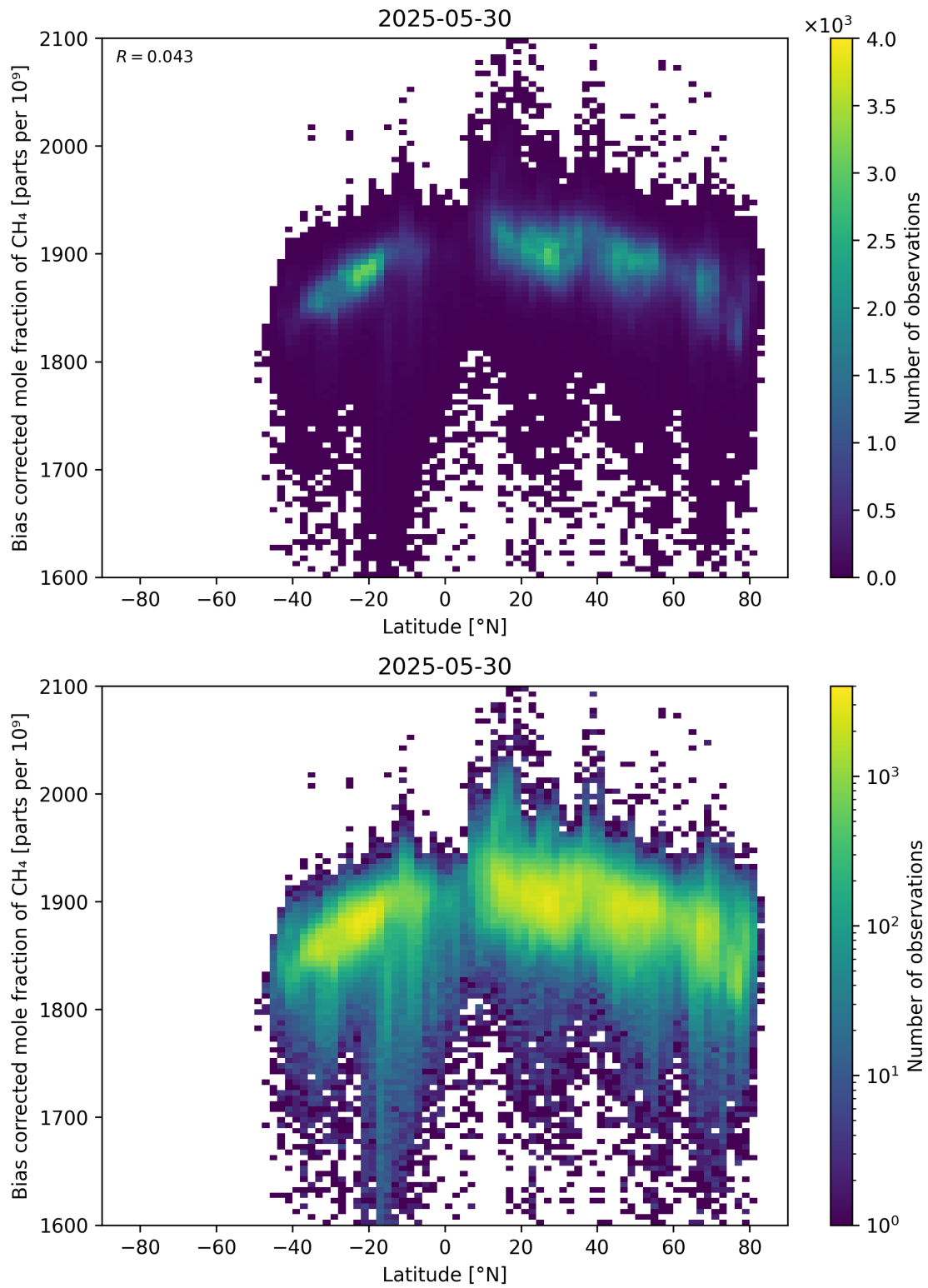
Figure 58: Scatter density plot of “Latitude” against “Bias corrected mole fraction of CH 4 ” for 2025-05-29 to 2025-05-31.
