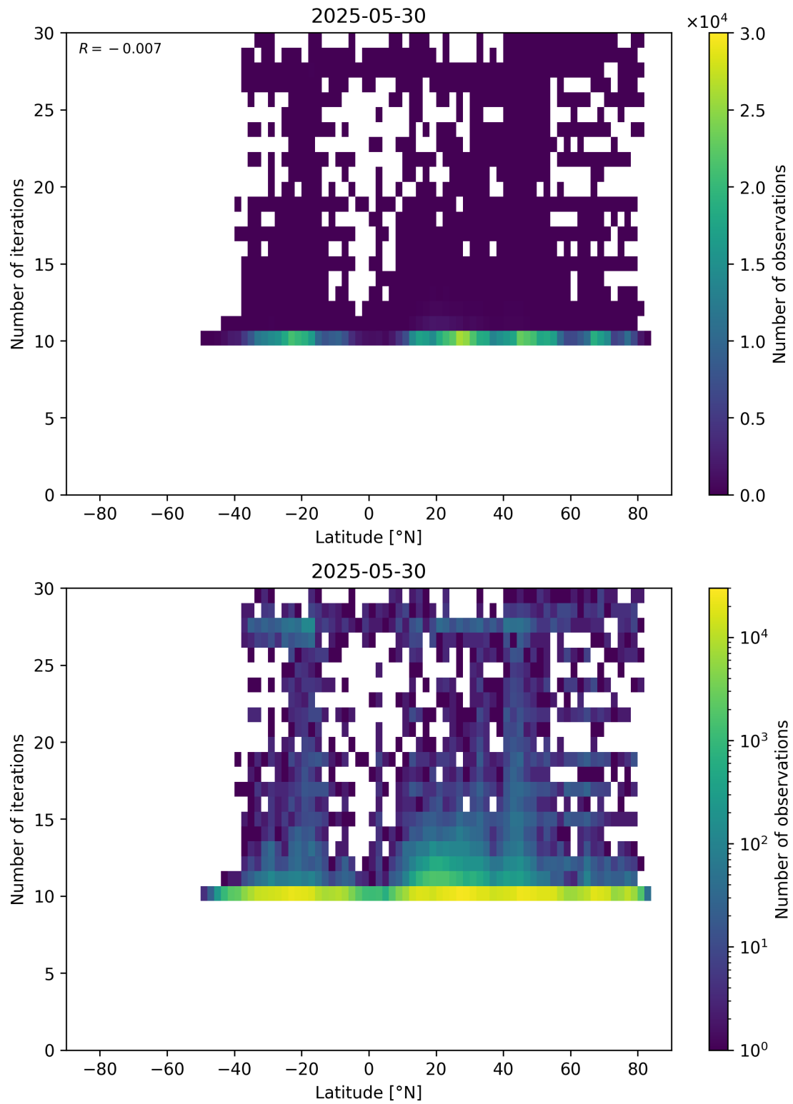
Figure 60: Scatter density plot of “Latitude” against “Number of iterations” for 2025-05-29 to 2025-05-31.
