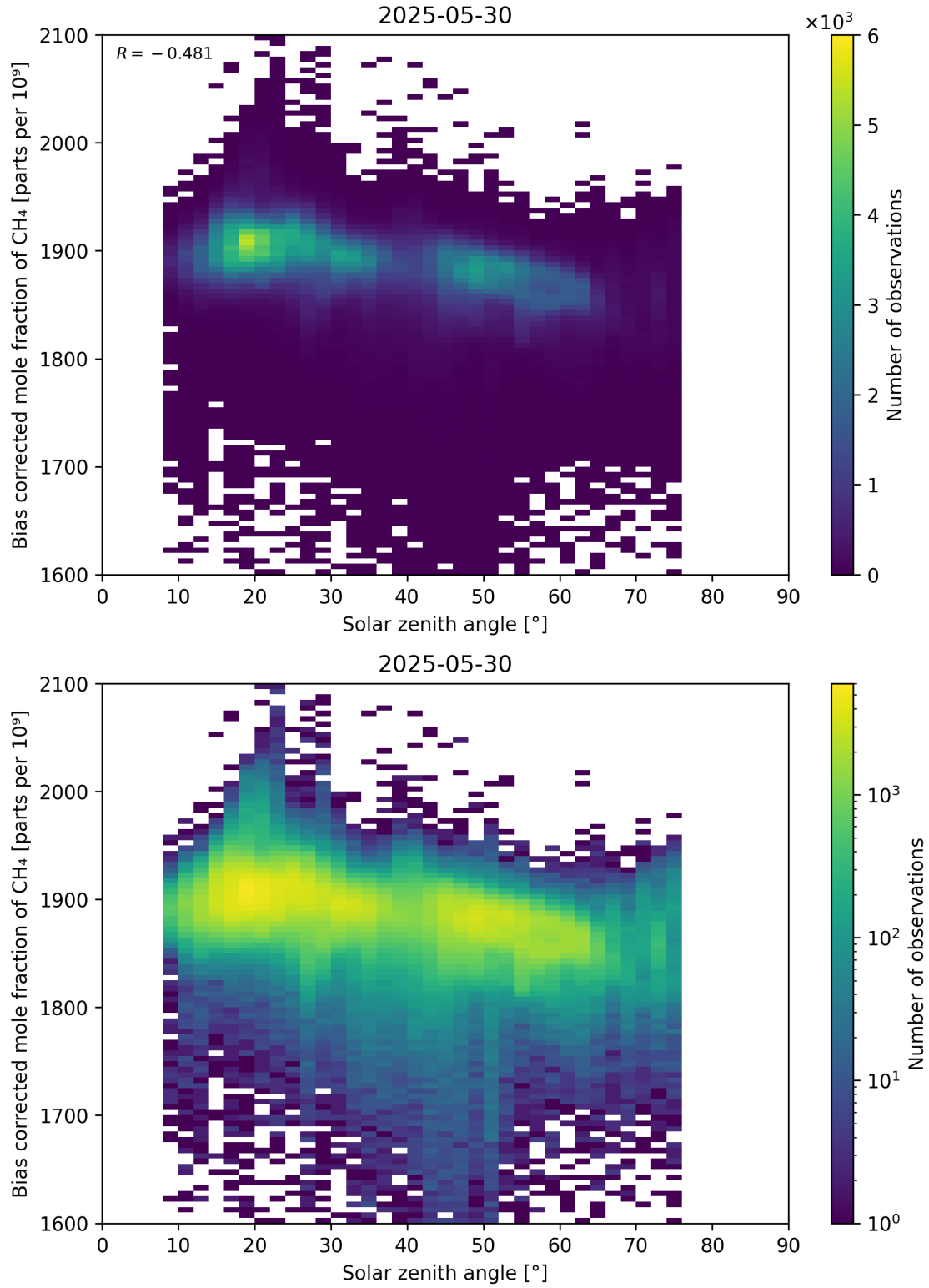
Figure 100: Scatter density plot of “Solar zenith angle” against “Bias corrected mole fraction of \text{CH}_4 ” for 2025-05-29 to 2025-05-31.
