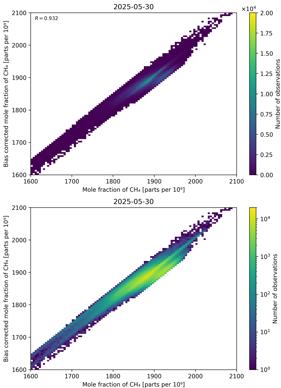
Figure 74: Scatter density plot of “Mole fraction of CH 4 ” against “Bias corrected mole fraction of CH 4 ” for 2025-05-29 to 2025-05-31.
