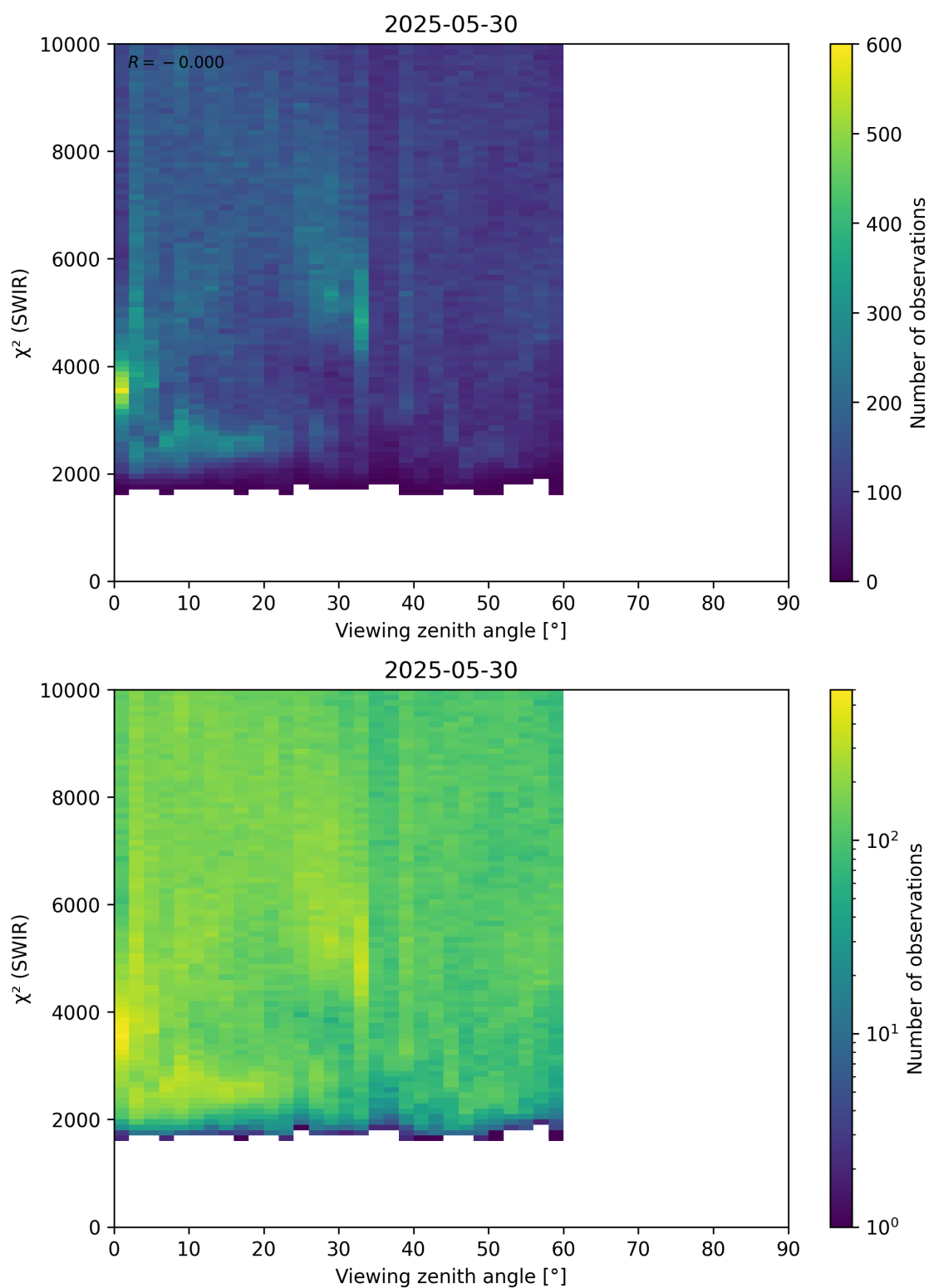
Figure 106: Scatter density plot of “Viewing zenith angle” against “ \chi^2 (SWIR)” for 2025-05-29 to 2025-05-31.
