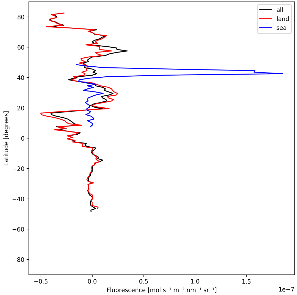
Figure 21: Zonal average of “Fluorescence” for 2025-05-29 to 2025-05-31.
