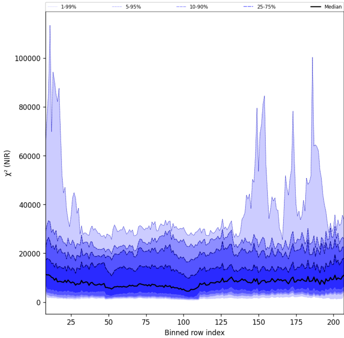
Figure 40: Along track statistics of “ \chi^2 (NIR)” for 2025-05-29 to 2025-05-31
