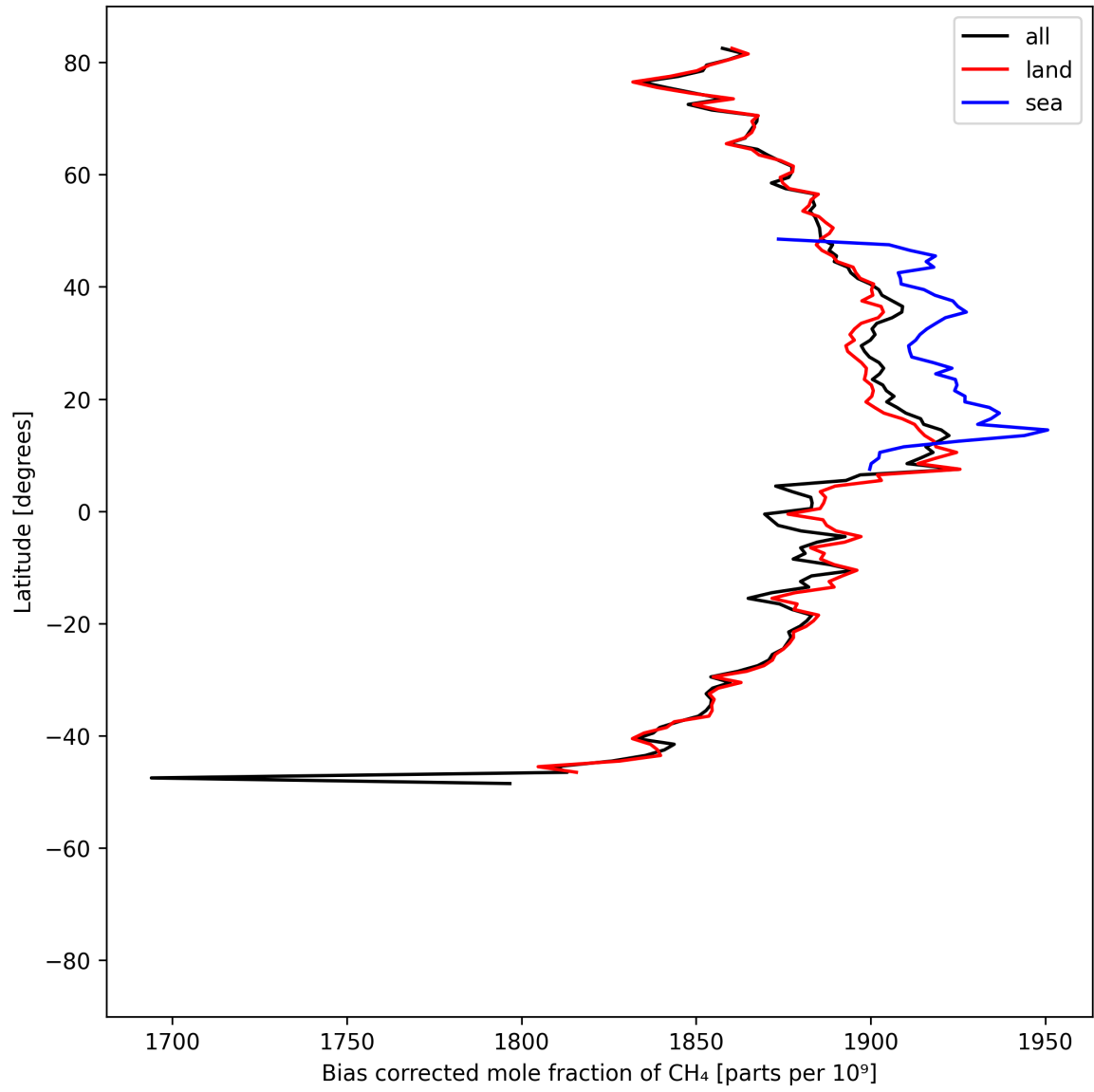
Figure 14: Zonal average of “Bias corrected mole fraction of CH 4 ” for 2025-05-29 to 2025-05-31.
