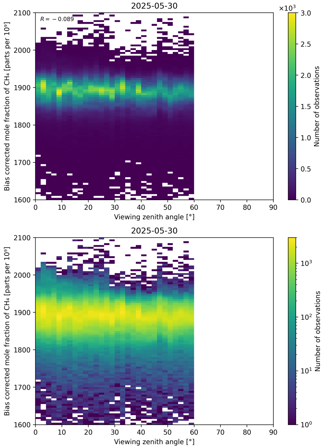
Figure 111: Scatter density plot of “Viewing zenith angle” against “Bias corrected mole fraction of CH 4 ” for 2025-05-29 to 2025-05-31.
