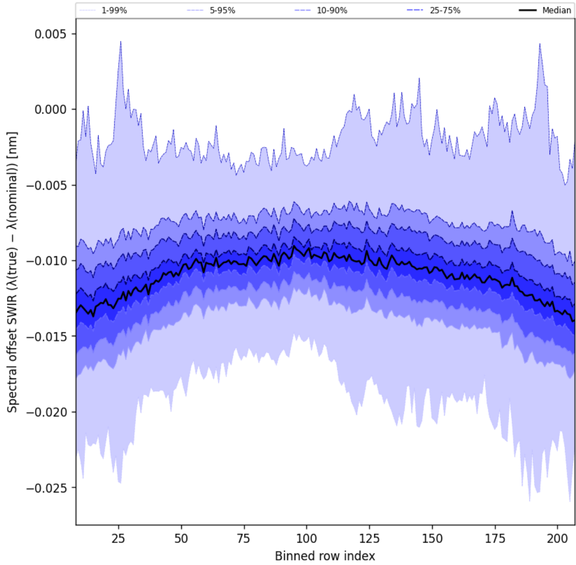
Figure 38: Along track statistics of “Spectral offset SWIR ( \lambda_{\text{true}} - \lambda_{\text{nominal}} )” for 2025-05-29 to 2025-05-31
