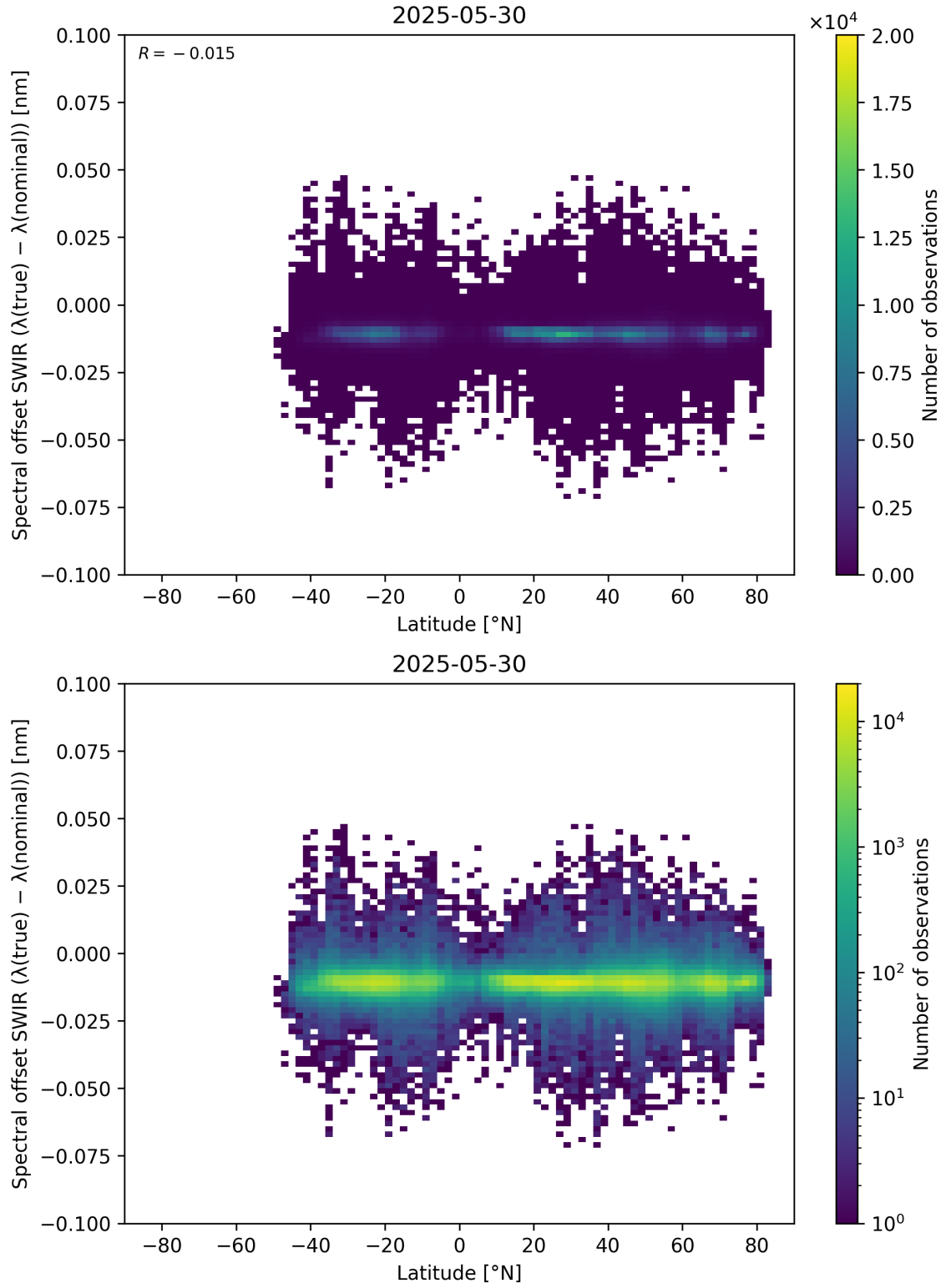
Figure 62: Scatter density plot of “Latitude” against “Spectral offset SWIR ( \lambda_{\text{true}} - \lambda_{\text{nominal}} )” for 2025-05-29 to 2025-05-31.
