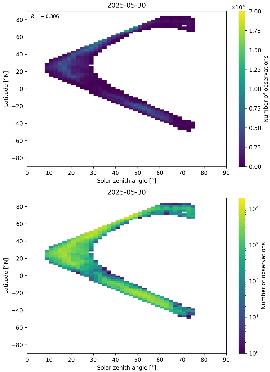
Figure 98: Scatter density plot of “Solar zenith angle” against “Latitude” for 2025-05-29 to 2025-05-31.
