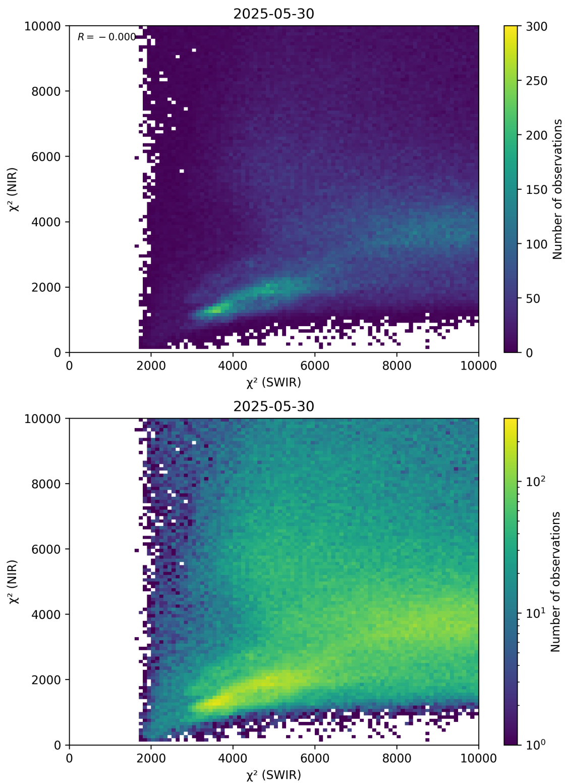
Figure 47: Scatter density plot of “ \chi^2 (SWIR)” against “ \chi^2 (NIR)” for 2025-05-29 to 2025-05-31.
