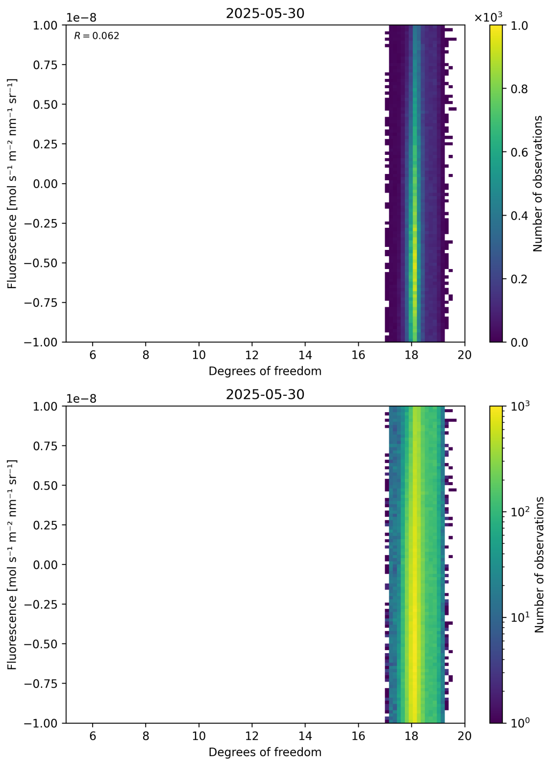
Figure 51: Scatter density plot of “Degrees of freedom” against “Fluorescence” for 2025-05-29 to 2025-05-31.
