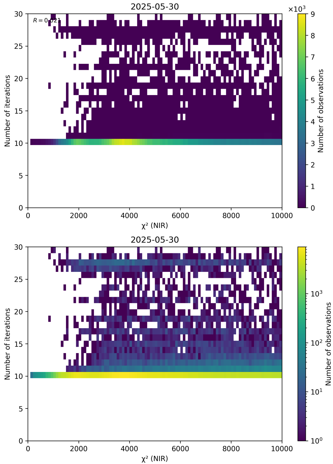
Figure 46: Scatter density plot of “ \chi^2 (NIR)” against “Number of iterations” for 2025-05-29 to 2025-05-31.
