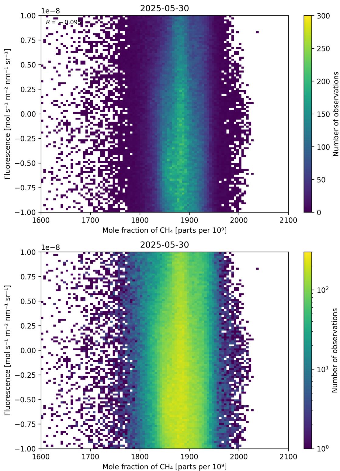
Figure 73: Scatter density plot of “Mole fraction of \text{CH}_4 ” against “Fluorescence” for 2025-05-29 to 2025-05-31.
