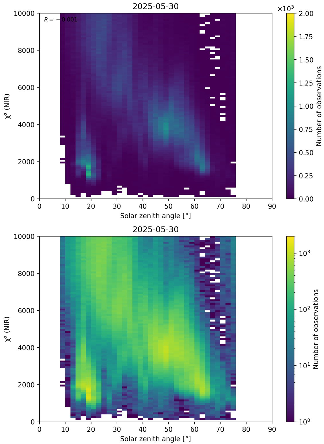
Figure 94: Scatter density plot of “Solar zenith angle” against “ \chi^2 (NIR)” for 2025-05-29 to 2025-05-31.
