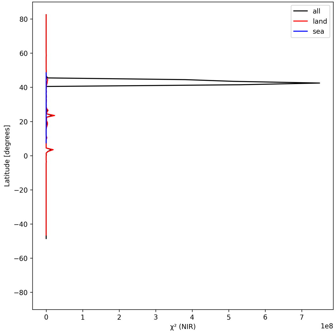
Figure 18: Zonal average of “ \chi^2 (NIR)” for 2025-05-29 to 2025-05-31.
