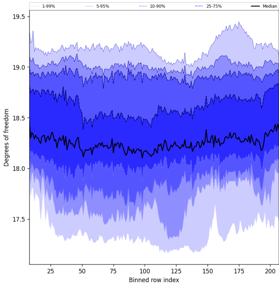
Figure 41: Along track statistics of “Degrees of freedom” for 2025-05-29 to 2025-05-31
