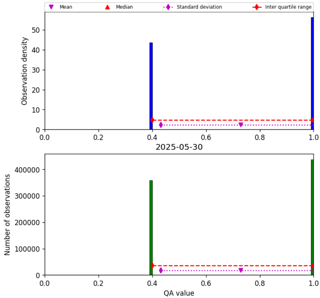
Figure 22: Histogram of “QA value” for 2025-05-29 to 2025-05-31
