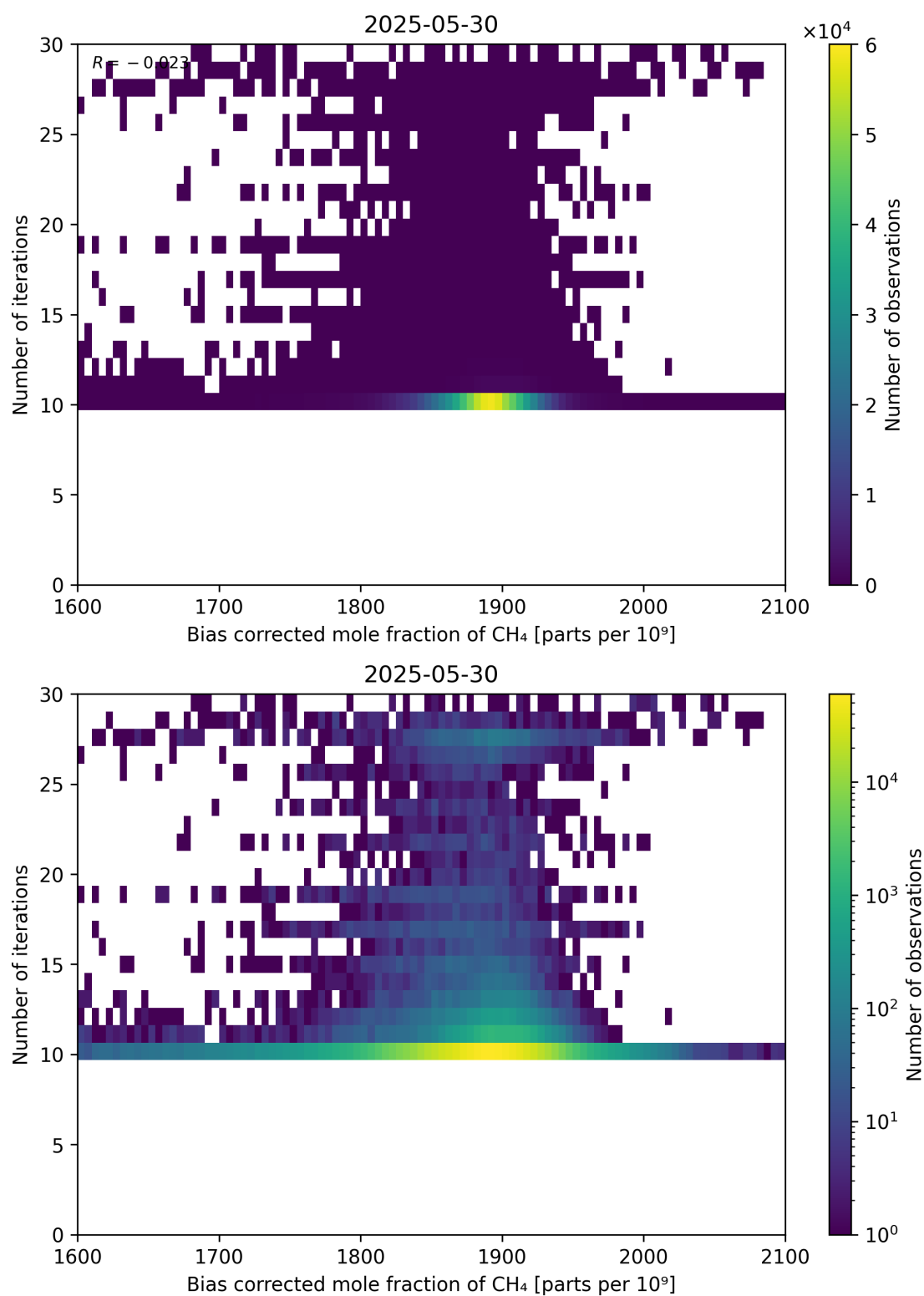
Figure 67: Scatter density plot of “Bias corrected mole fraction of \text{CH}_4 ” against “Number of iterations” for 2025-05-29 to 2025-05-31.
