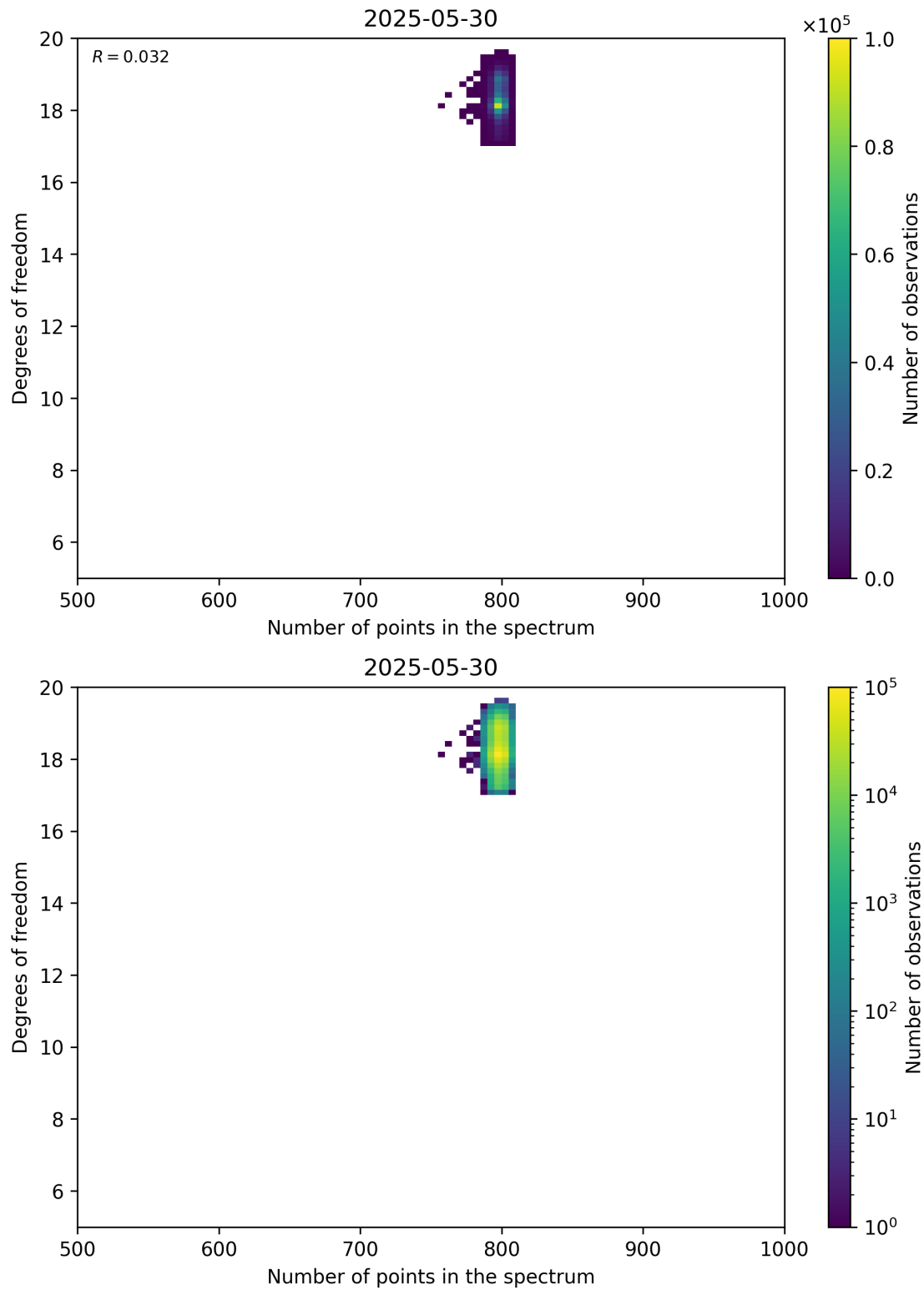
Figure 90: Scatter density plot of “Number of points in the spectrum” against “Degrees of freedom” for 2025-05-29 to 2025-05-31.
