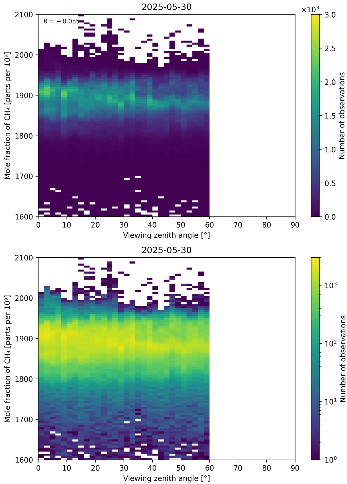
Figure 110: Scatter density plot of “Viewing zenith angle” against “Mole fraction of CH 4 ” for 2025-05-29 to 2025-05-31.
