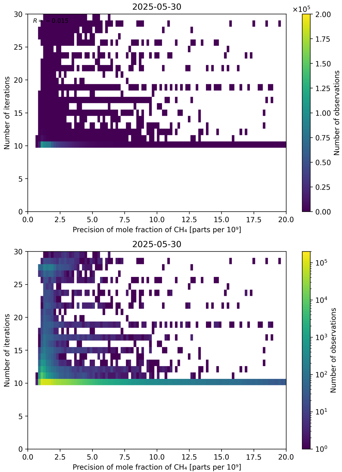
Figure 83: Scatter density plot of “Precision of mole fraction of CH 4 ” against “Number of iterations” for 2025-05-29 to 2025-05-31.
