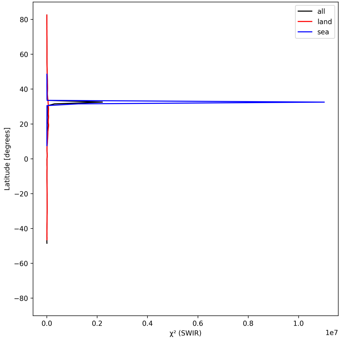
Figure 17: Zonal average of “ \chi^2 (SWIR)” for 2025-05-29 to 2025-05-31.
