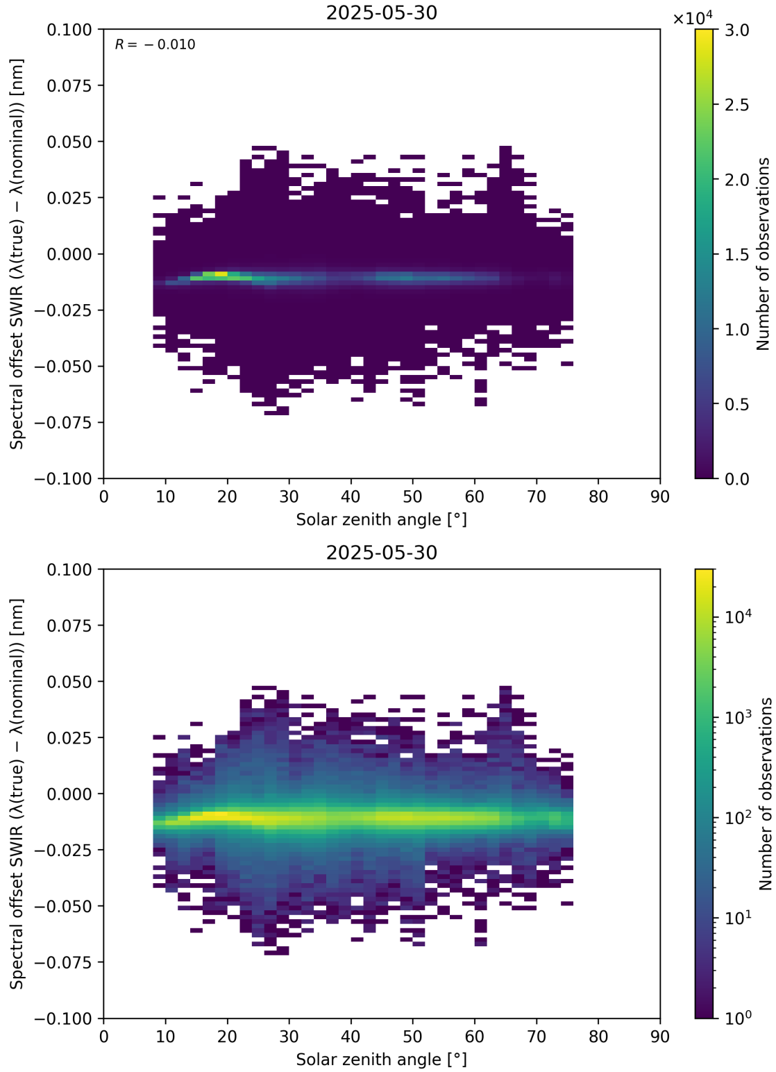
Figure 104: Scatter density plot of “Solar zenith angle” against “Spectral offset SWIR ( \lambda_{\text{true}} - \lambda_{\text{nominal}} )” for 2025-05-29 to 2025-05-31.
