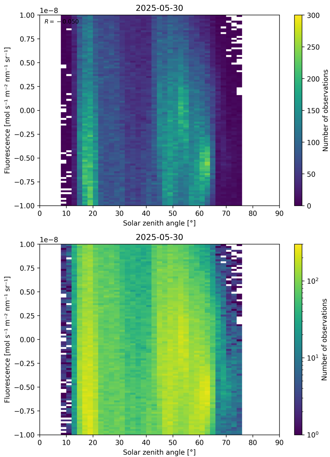
Figure 97: Scatter density plot of “Solar zenith angle” against “Fluorescence” for 2025-05-29 to 2025-05-31.
