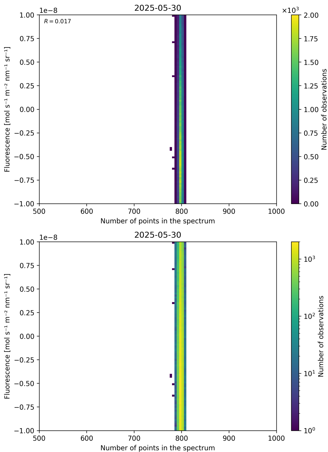
Figure 91: Scatter density plot of “Number of points in the spectrum” against “Fluorescence” for 2025-05-29 to 2025-05-31.
