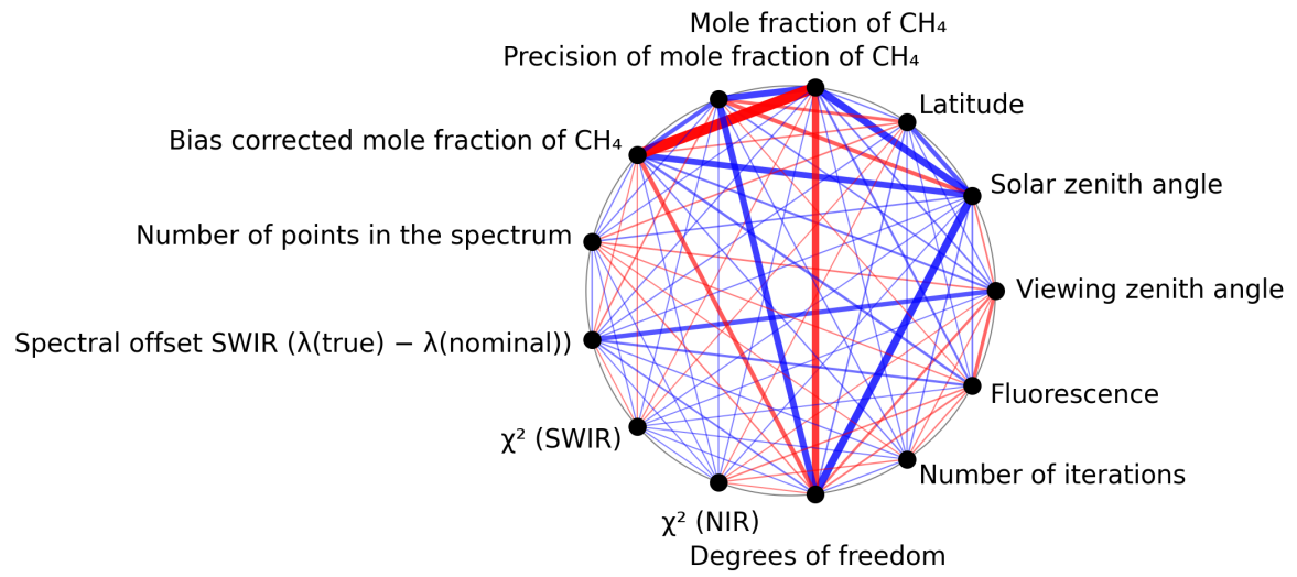
Figure 1: Map of correlation graph for 2025-05-29 to 2025-05-31.
