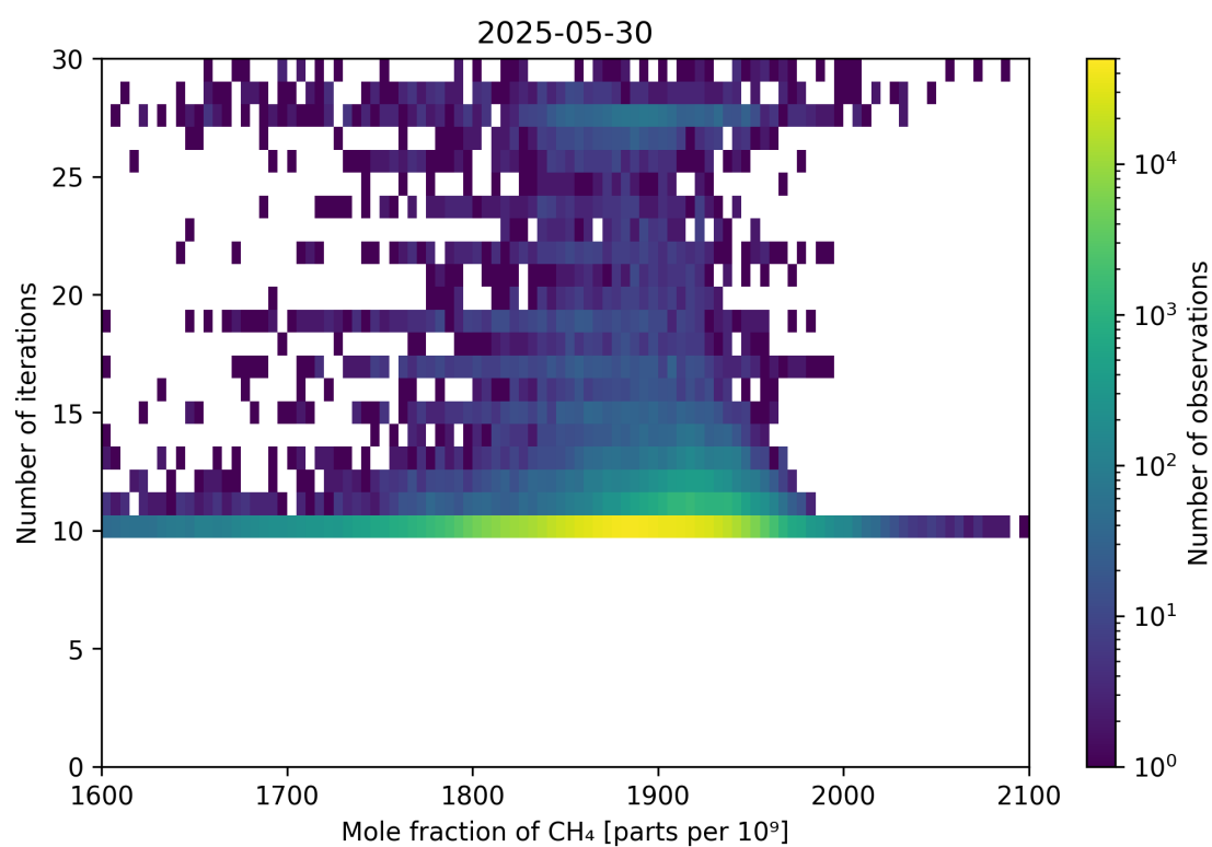
Figure 76: Scatter density plot of “Mole fraction of CH 4 ” against “Number of iterations” for 2025-05-29 to 2025-05-31.
