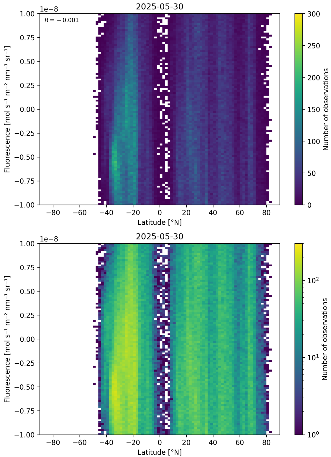
Figure 56: Scatter density plot of “Latitude” against “Fluorescence” for 2025-05-29 to 2025-05-31.
