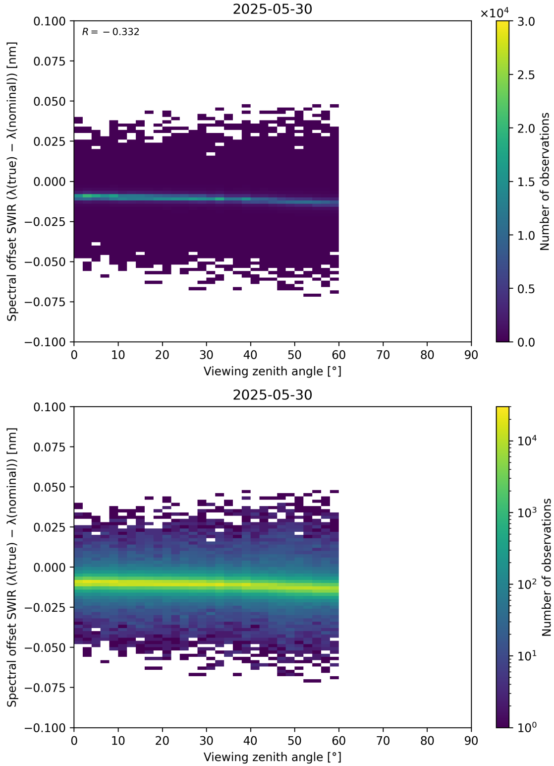
Figure 116: Scatter density plot of “Viewing zenith angle” against “Spectral offset SWIR ( \lambda_{\text{true}} - \lambda_{\text{nominal}} )” for 2025-05-29 to 2025-05-31.
