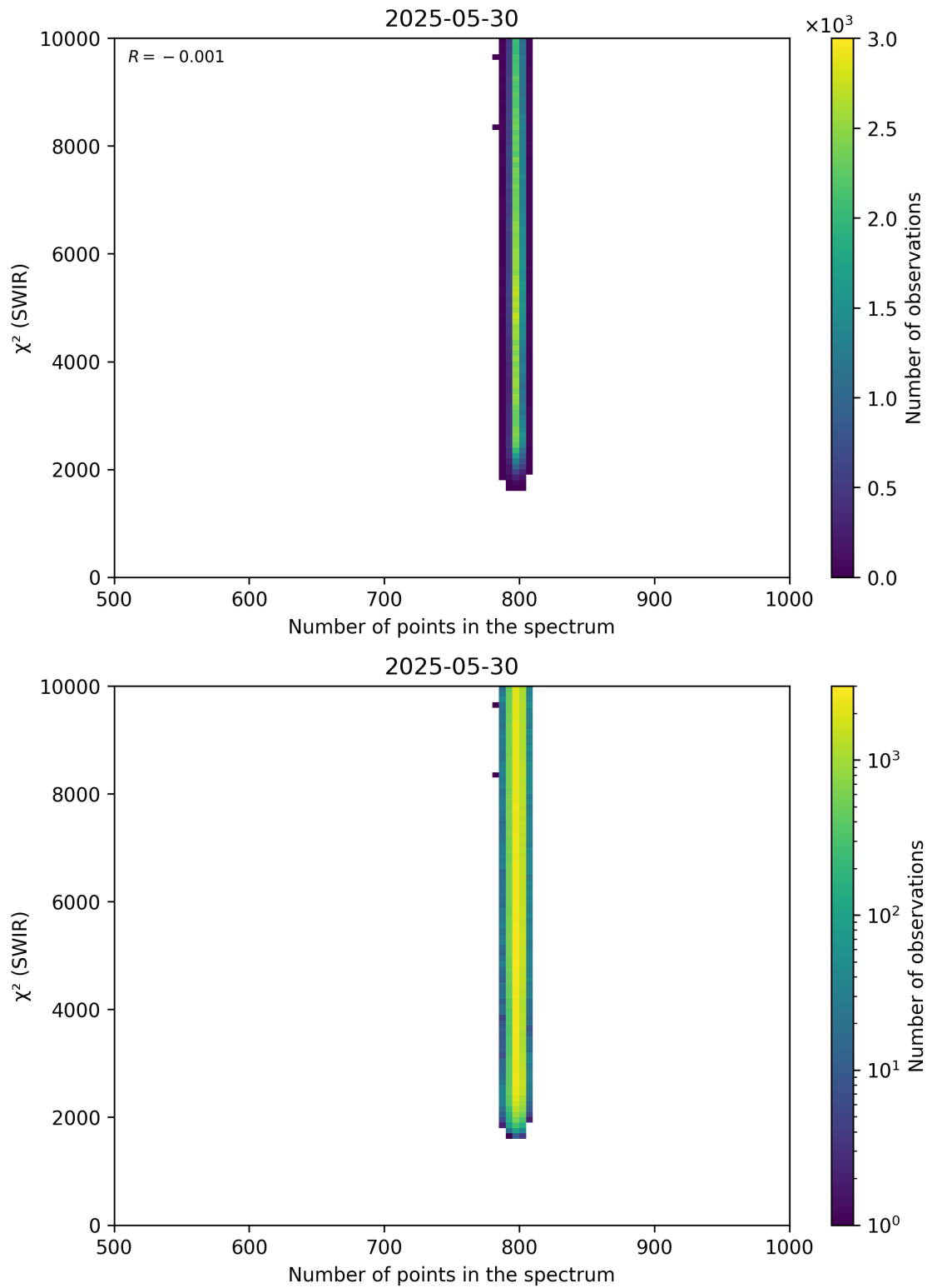
Figure 89: Scatter density plot of “Number of points in the spectrum” against “ \chi^2 (SWIR)” for 2025-05-29 to 2025-05-31.
