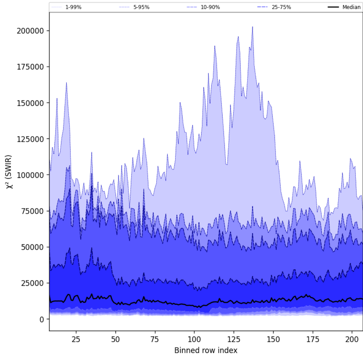
Figure 39: Along track statistics of " \chi^2 (SWIR)" for 2025-05-29 to 2025-05-31
