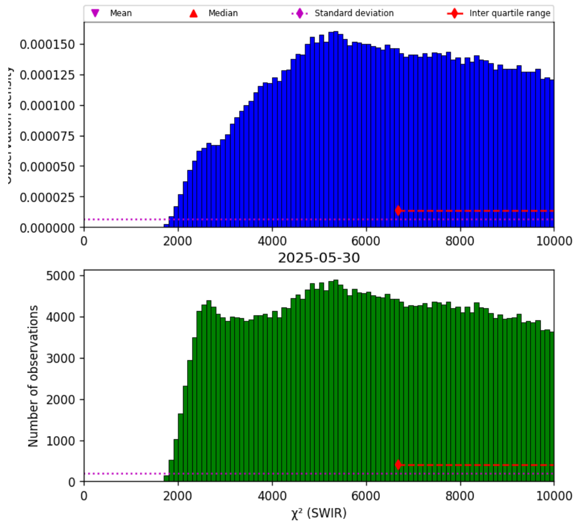
Figure 28: Histogram of “ \chi^2 (SWIR)” for 2025-05-29 to 2025-05-31
