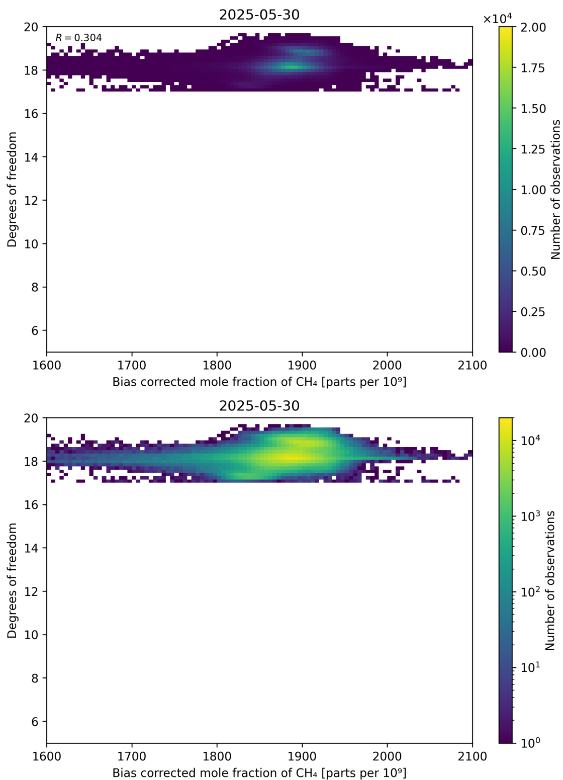
Figure 65: Scatter density plot of “Bias corrected mole fraction of CH 4 ” against “Degrees of freedom” for 2025-05-29 to 2025-05-31.
