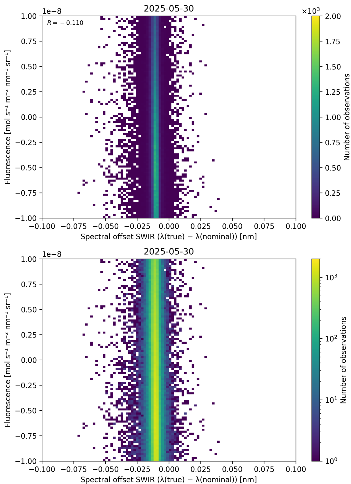
Figure 120: Scatter density plot of “Spectral offset SWIR ( \lambda_{\text{true}} - \lambda_{\text{nominal}} )” against “Fluorescence” for 2025-05-29 to 2025-05-31.
