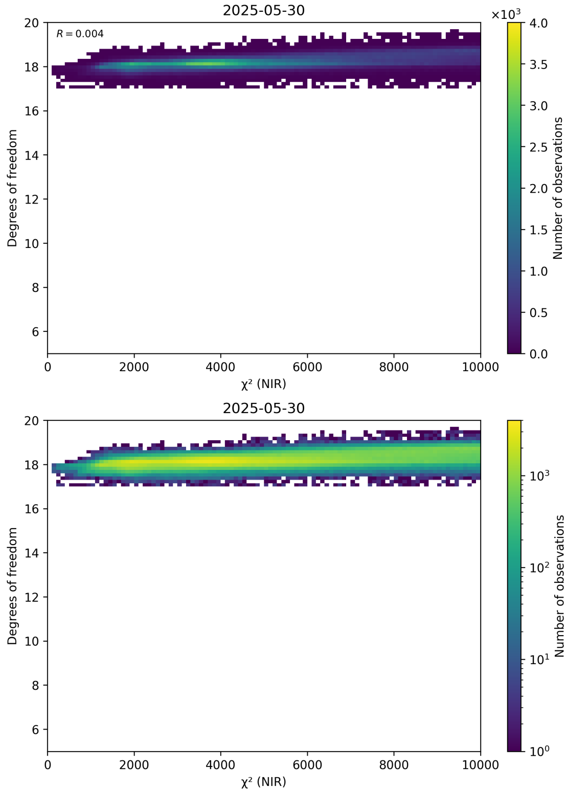
Figure 44: Scatter density plot of “ \chi^2 (NIR)” against “Degrees of freedom” for 2025-05-29 to 2025-05-31.
