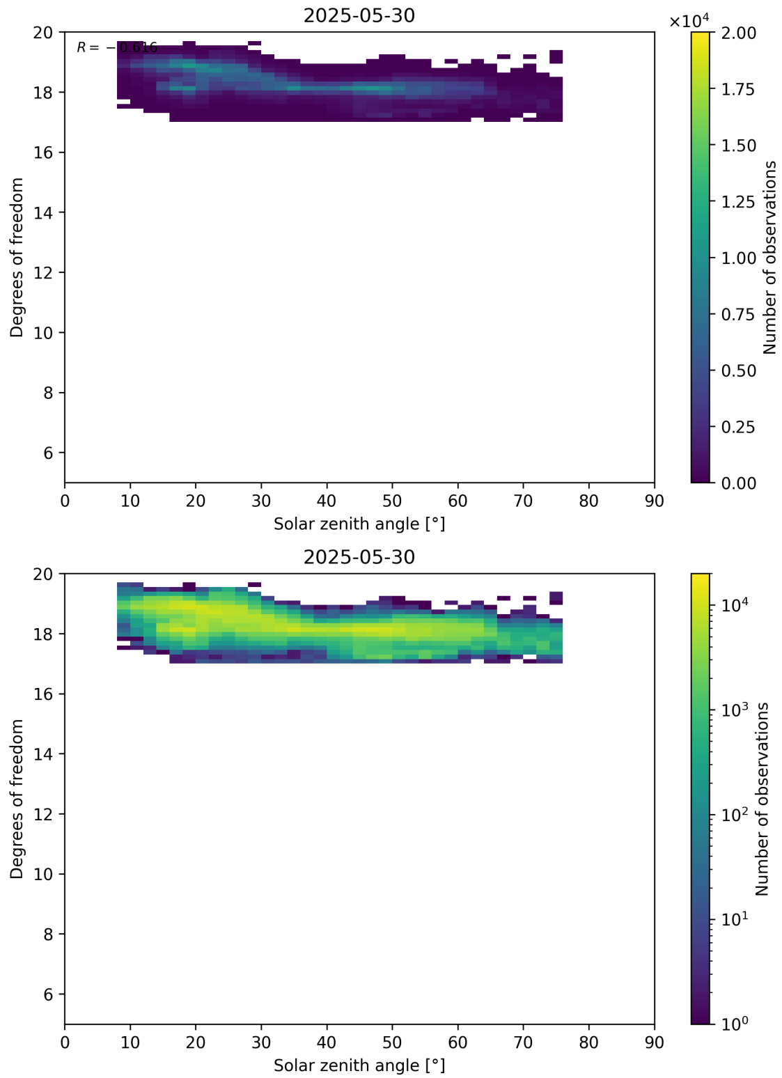
Figure 96: Scatter density plot of “Solar zenith angle” against “Degrees of freedom” for 2025-05-29 to 2025-05-31.
