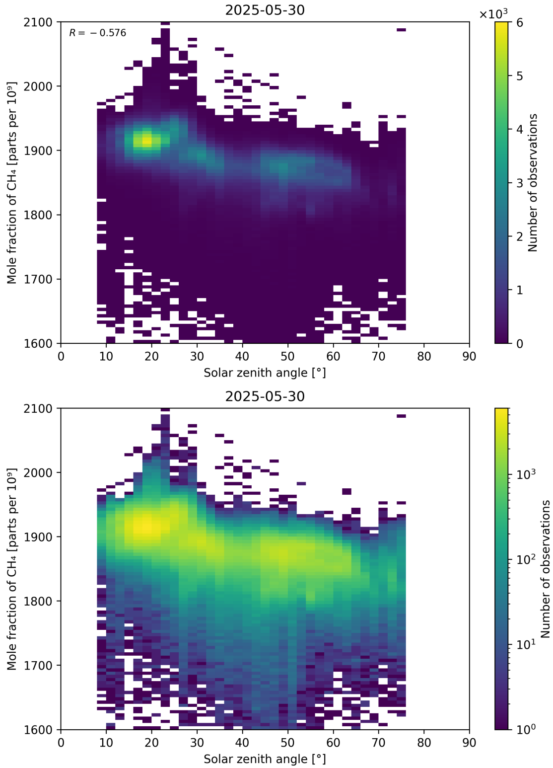
Figure 99: Scatter density plot of “Solar zenith angle” against “Mole fraction of \text{CH}_4 ” for 2025-05-29 to 2025-05-31.
