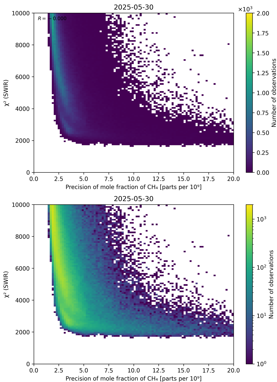
Figure 79: Scatter density plot of “Precision of mole fraction of CH 4 ” against “ \chi^2 (SWIR)” for 2025-05-29 to 2025-05-31.
