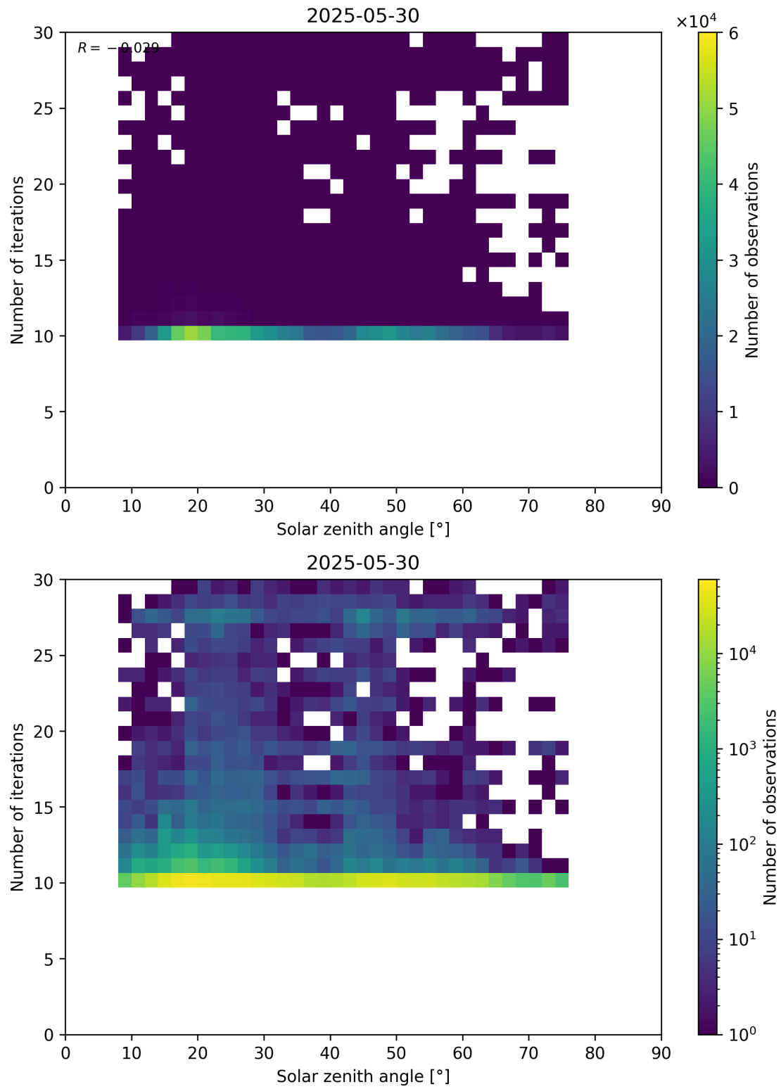
Figure 102: Scatter density plot of “Solar zenith angle” against “Number of iterations” for 2025-05-29 to 2025-05-31.
