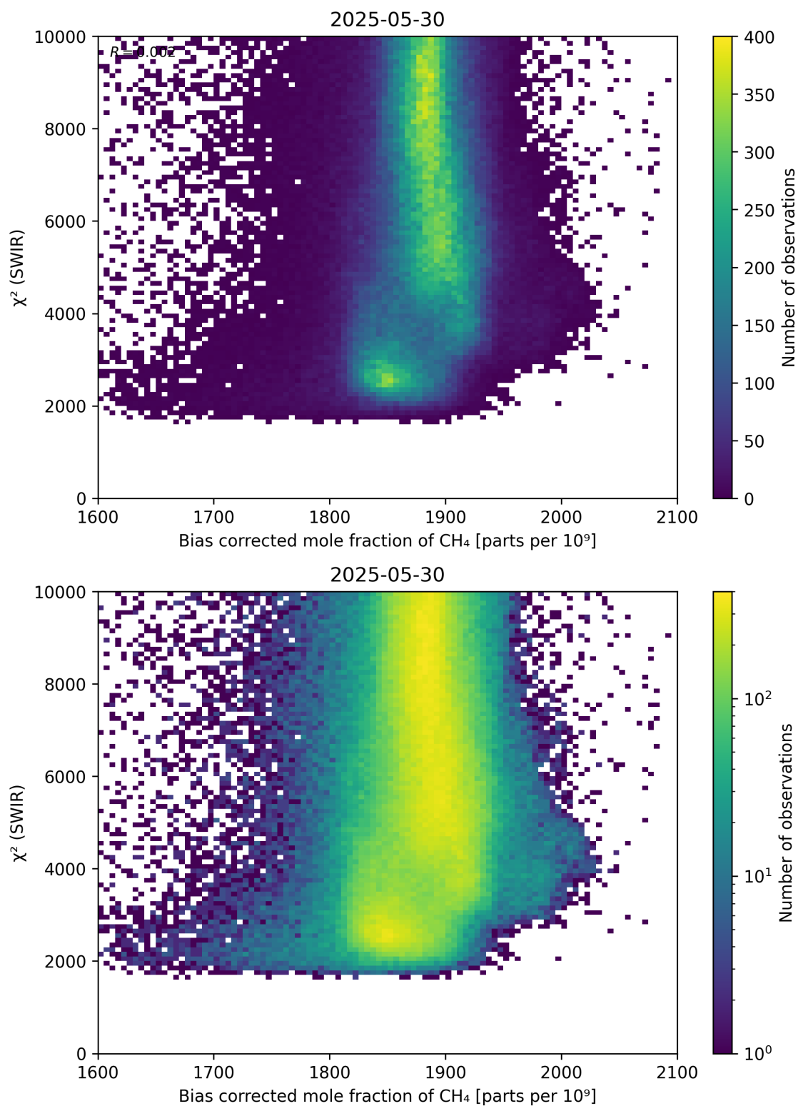
Figure 64: Scatter density plot of “Bias corrected mole fraction of \text{CH}_4 ” against “ \chi^2 (SWIR)” for 2025-05-29 to 2025-05-31.
