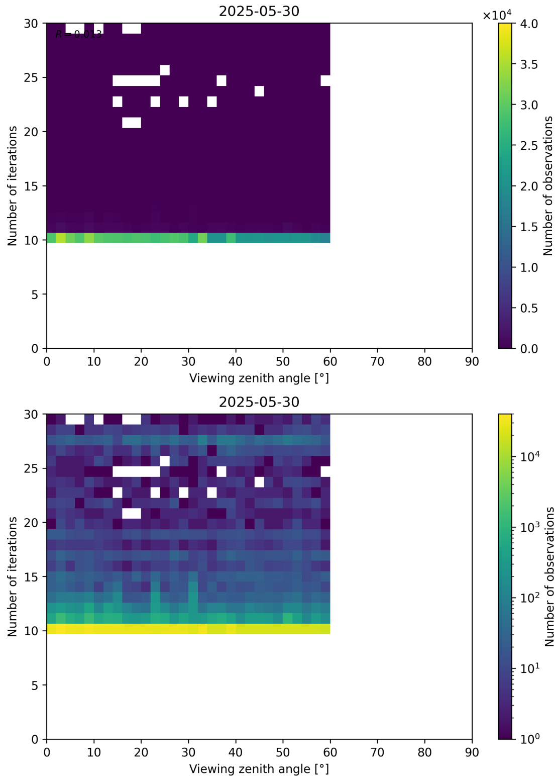
Figure 113: Scatter density plot of “Viewing zenith angle” against “Number of iterations” for 2025-05-29 to 2025-05-31.
