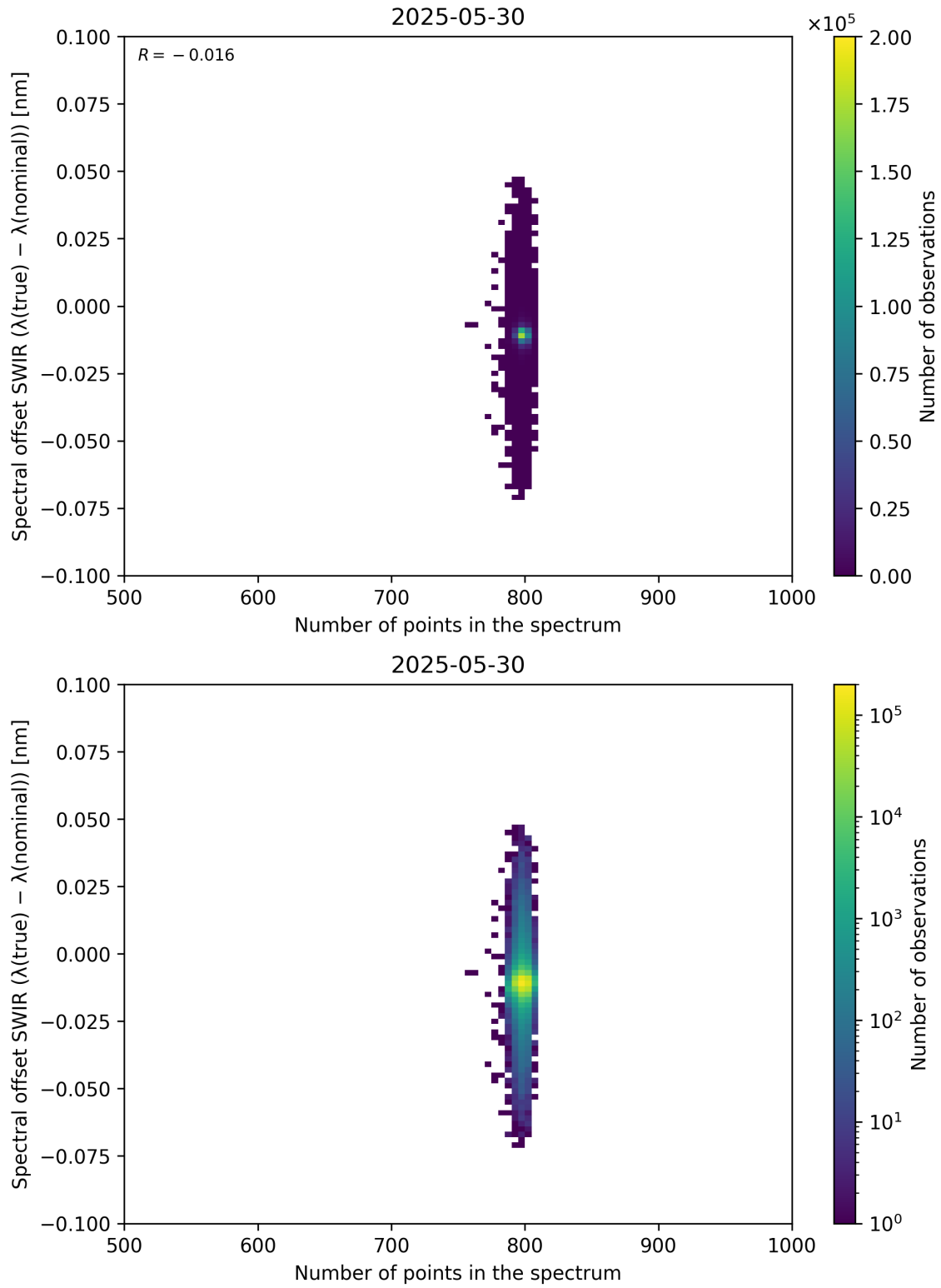
Figure 93: Scatter density plot of “Number of points in the spectrum” against “Spectral offset SWIR ( \lambda_{\text{true}} - \lambda_{\text{nominal}} )” for 2025-05-29 to 2025-05-31.
