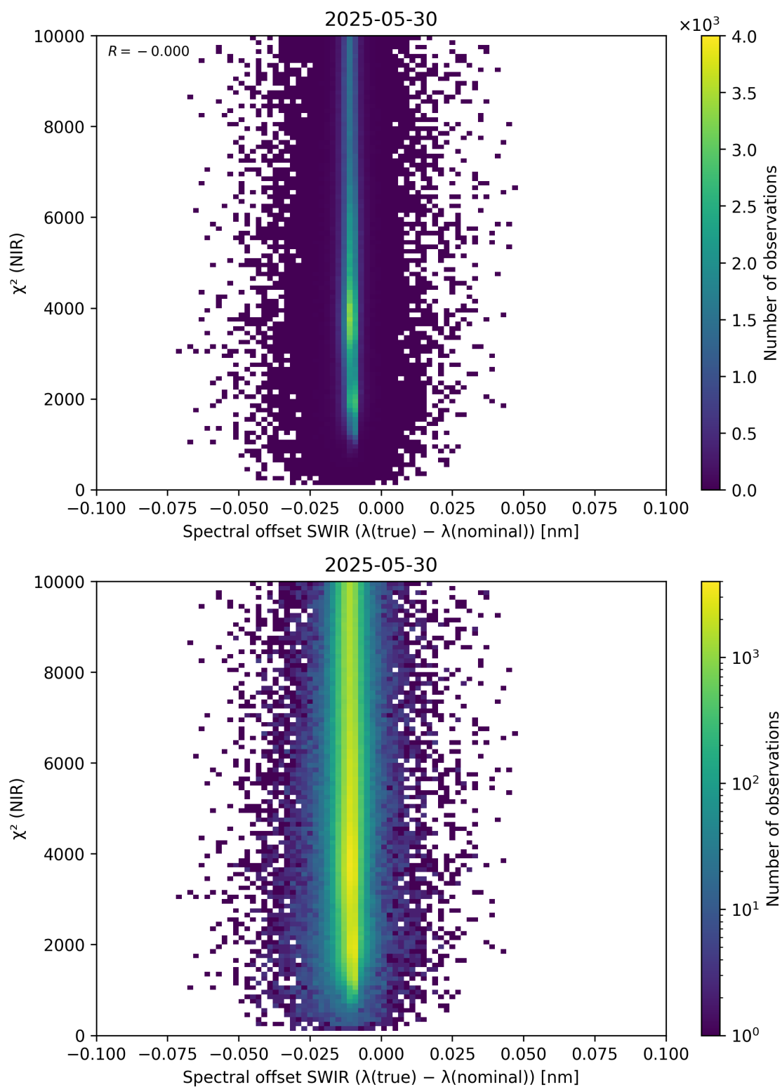
Figure 117: Scatter density plot of “Spectral offset SWIR ( \lambda_{\text{true}} - \lambda_{\text{nominal}} )” against “ \chi^2 (NIR)” for 2025-05-29 to 2025-05-31.
