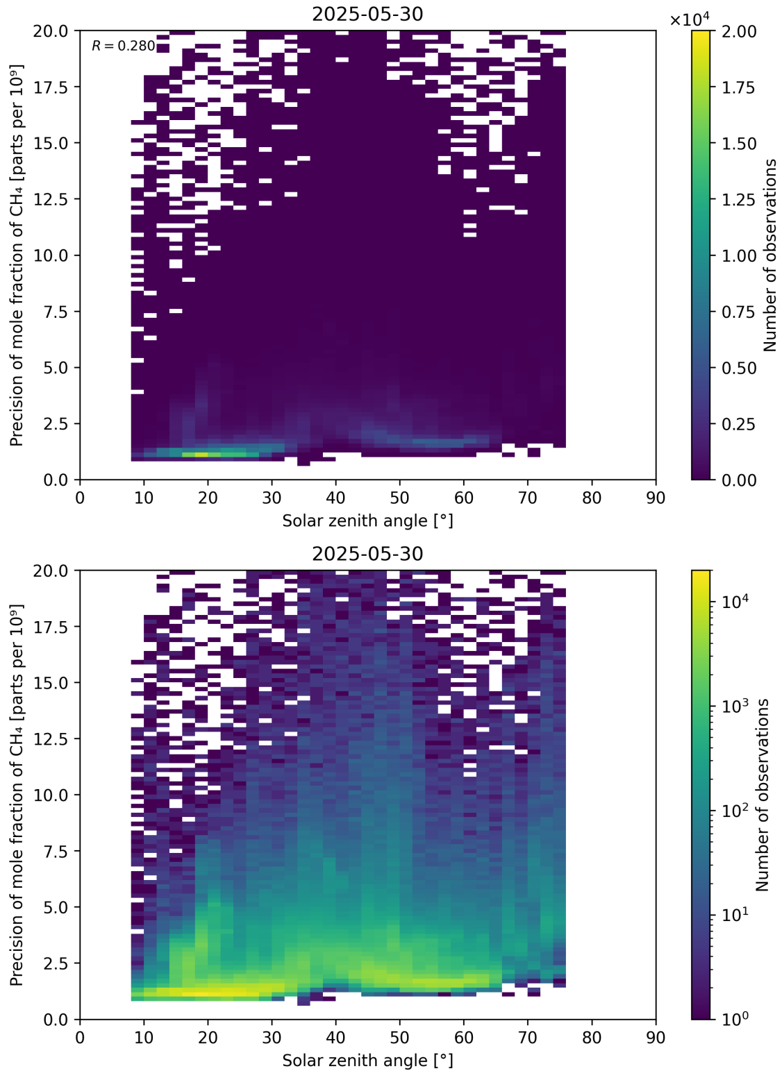
Figure 101: Scatter density plot of “Solar zenith angle” against “Precision of mole fraction of \text{CH}_4 ” for 2025-05-29 to 2025-05-31.
