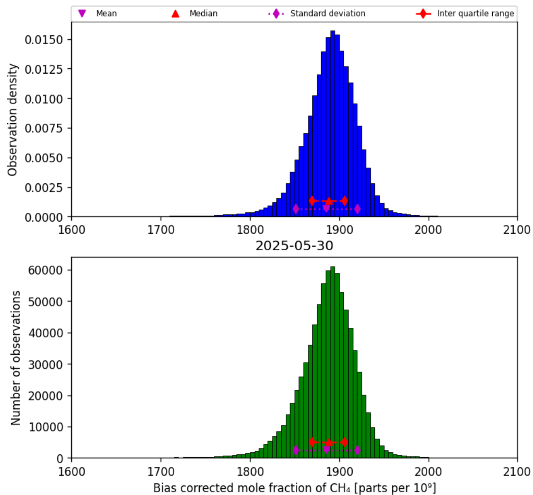
Figure 25: Histogram of “Bias corrected mole fraction of CH 4 ” for 2025-05-29 to 2025-05-31
