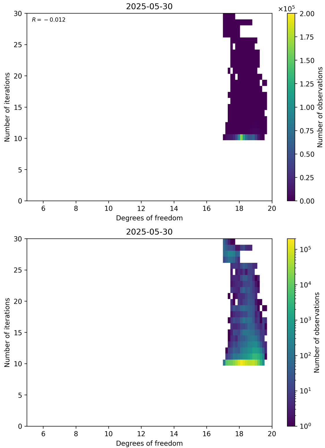
Figure 52: Scatter density plot of “Degrees of freedom” against “Number of iterations” for 2025-05-29 to 2025-05-31.
