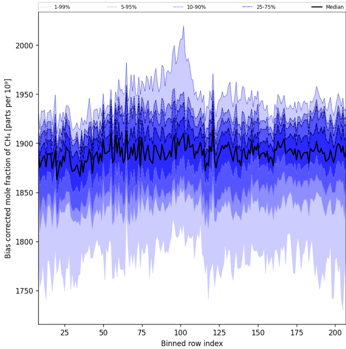
Figure 36: Along track statistics of “Bias corrected mole fraction of CH 4 ” for 2025-05-29 to 2025-05-31
