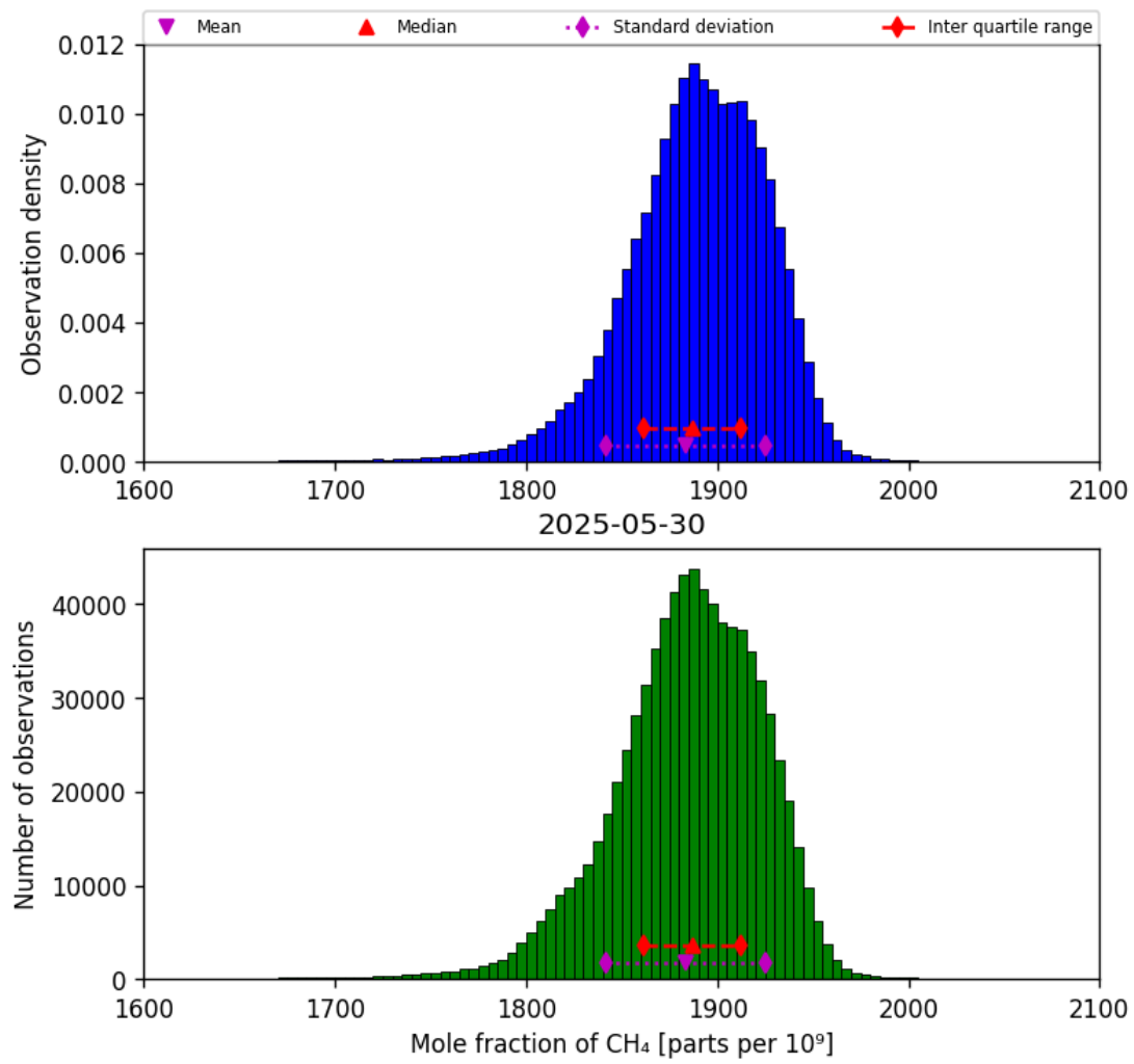
Figure 23: Histogram of “Mole fraction of CH 4 ” for 2025-05-29 to 2025-05-31
