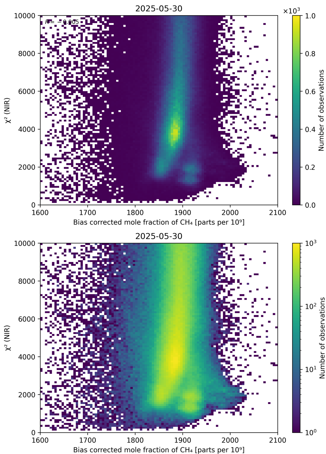
Figure 63: Scatter density plot of “Bias corrected mole fraction of \text{CH}_4 ” against “ \chi^2 (NIR)” for 2025-05-29 to 2025-05-31.
