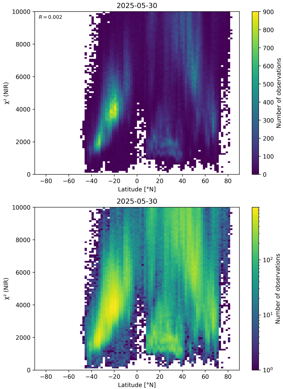
Figure 53: Scatter density plot of “Latitude” against “ \chi^2 (NIR)” for 2025-05-29 to 2025-05-31.
