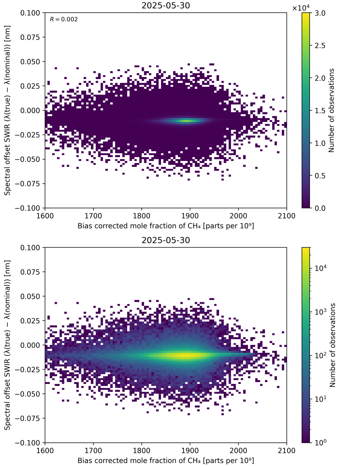
Figure 69: Scatter density plot of “Bias corrected mole fraction of CH 4 ” against “Spectral offset SWIR ( \lambda_{\text{true}} - \lambda_{\text{nominal}} )” for 2025-05-29 to 2025-05-31.
