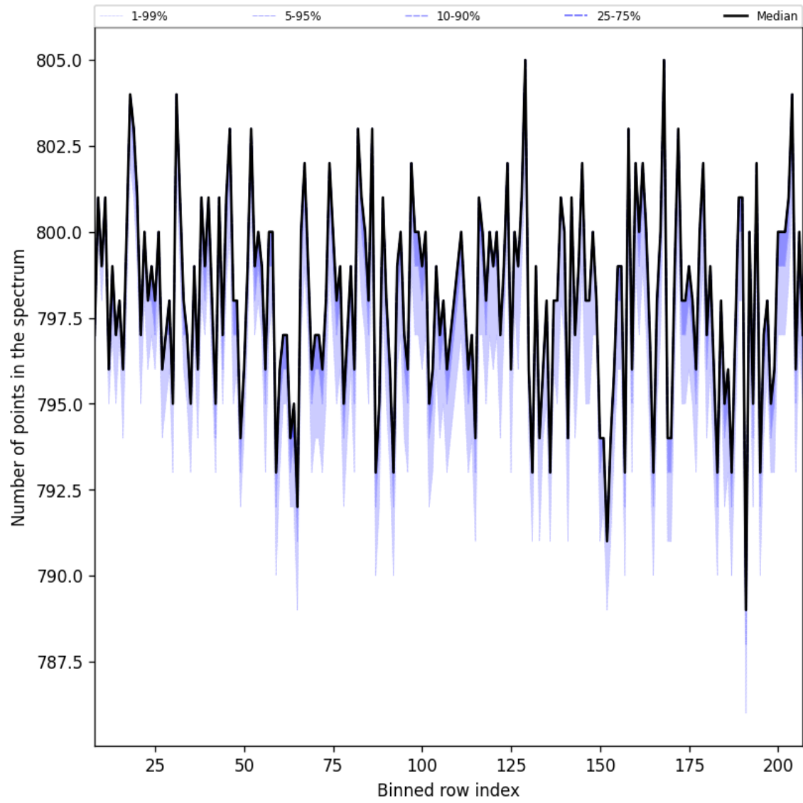
Figure 37: Along track statistics of “Number of points in the spectrum” for 2025-05-29 to 2025-05-31
