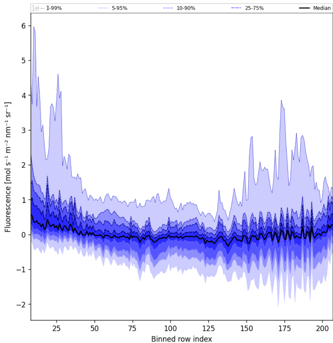
Figure 43: Along track statistics of “Fluorescence” for 2025-05-29 to 2025-05-31
