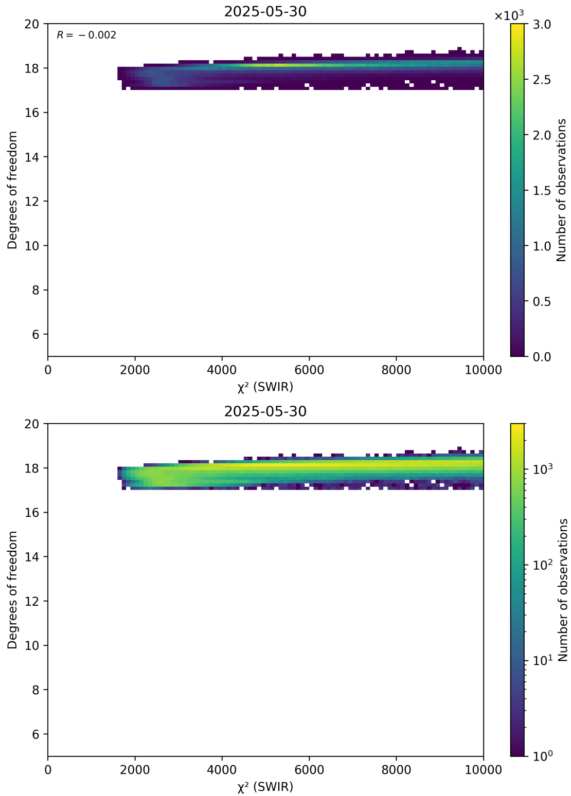
Figure 48: Scatter density plot of “ \chi^2 (SWIR)” against “Degrees of freedom” for 2025-05-29 to 2025-05-31.
