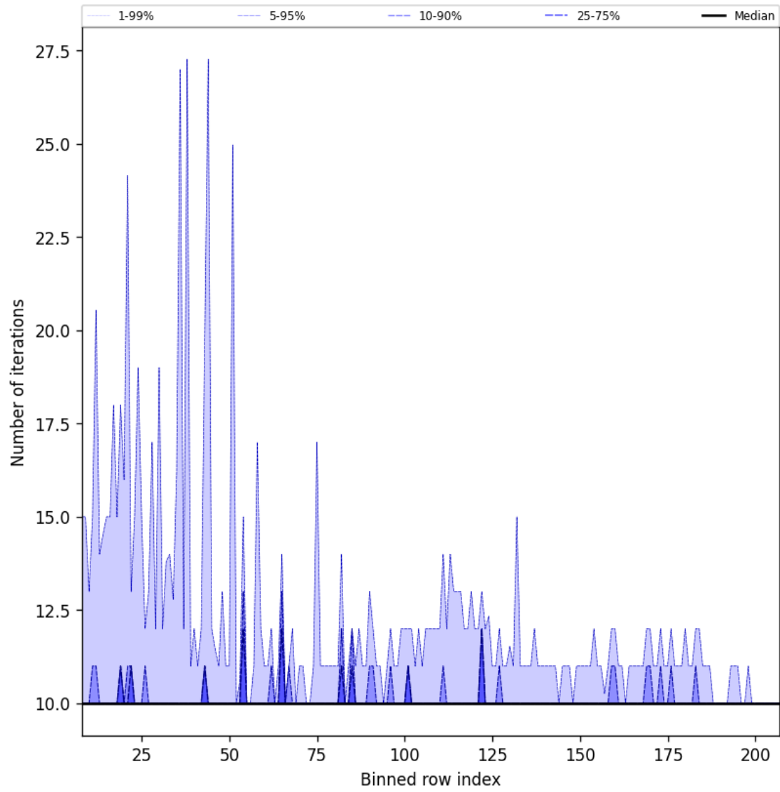
Figure 42: Along track statistics of “Number of iterations” for 2025-05-29 to 2025-05-31
