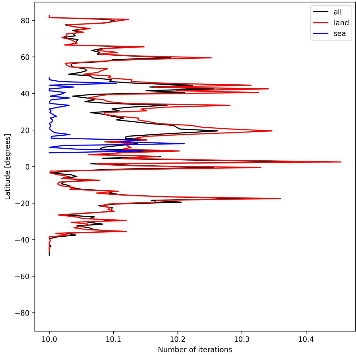
Figure 20: Zonal average of “Number of iterations” for 2025-05-29 to 2025-05-31.
