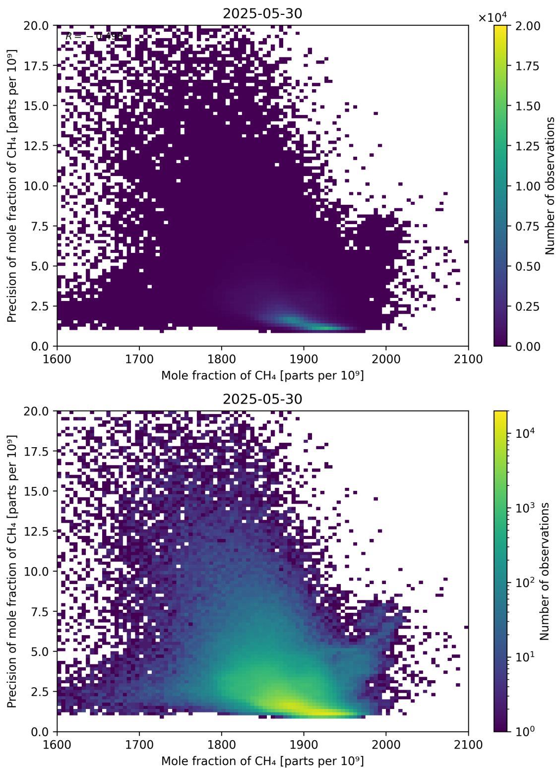
Figure 75: Scatter density plot of “Mole fraction of CH 4 ” against “Precision of mole fraction of CH 4 ” for 2025-05-29 to 2025-05-31.
