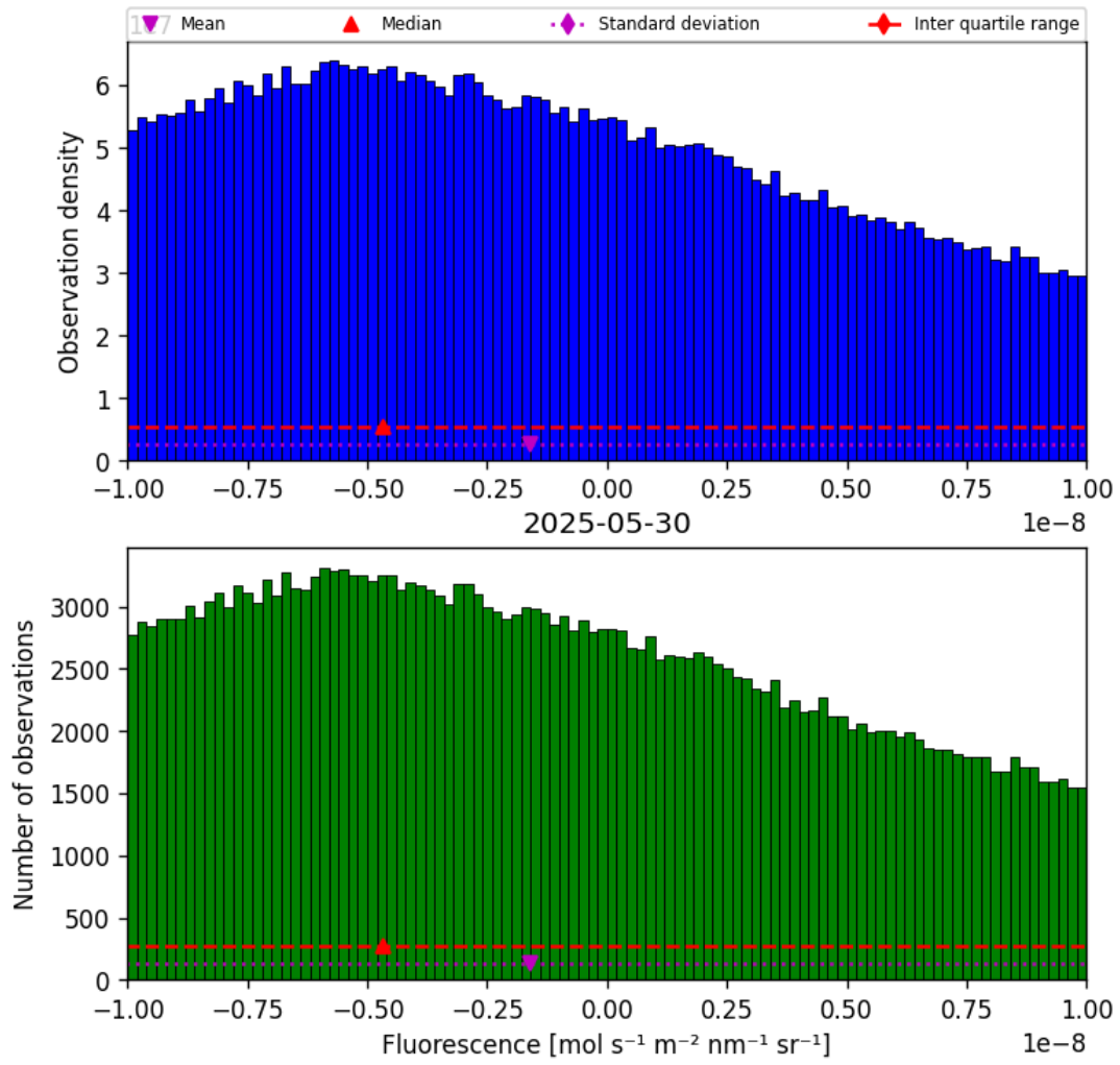
Figure 32: Histogram of “Fluorescence” for 2025-05-29 to 2025-05-31
