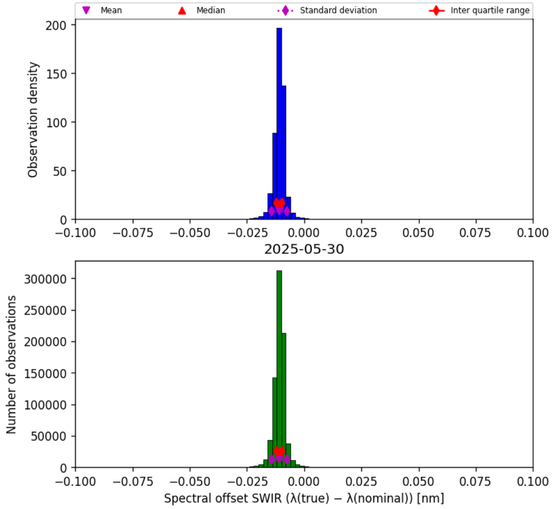
Figure 27: Histogram of “Spectral offset SWIR ( \lambda_{\text{true}} - \lambda_{\text{nominal}} )” for 2025-05-29 to 2025-05-31
