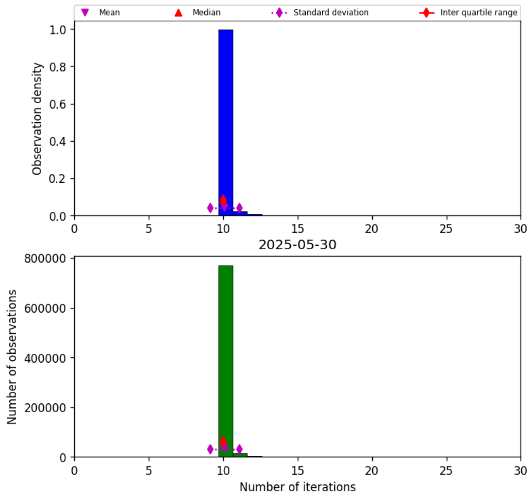
Figure 31: Histogram of “Number of iterations” for 2025-05-29 to 2025-05-31
