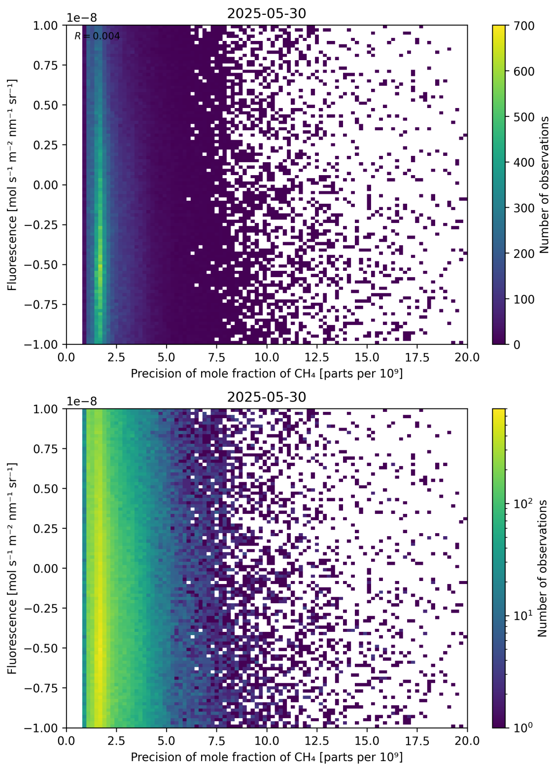
Figure 81: Scatter density plot of “Precision of mole fraction of \text{CH}_4 ” against “Fluorescence” for 2025-05-29 to 2025-05-31.
