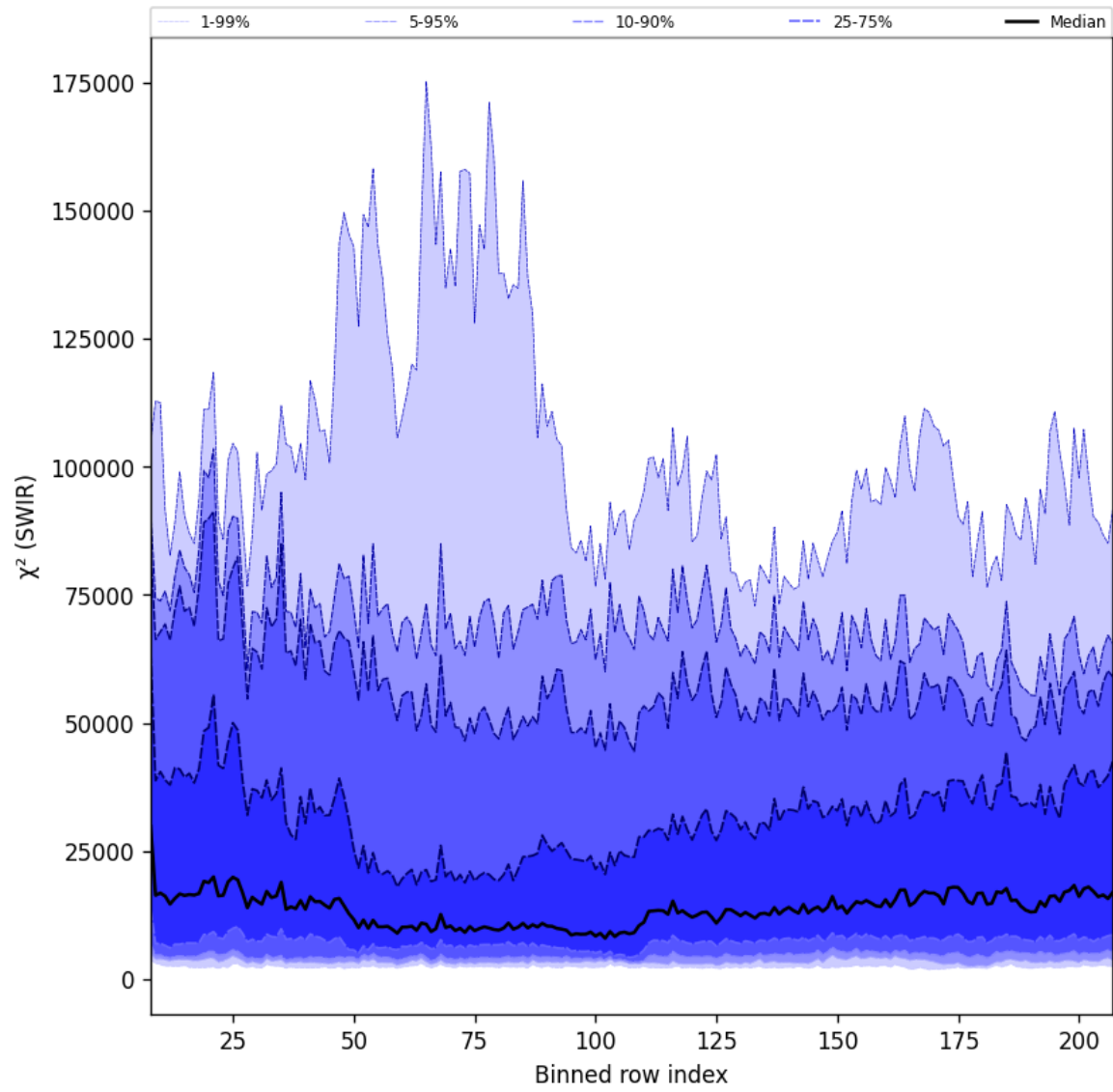
Figure 39: Along track statistics of “ \chi^2 (SWIR)” for 2025-05-31 to 2025-06-01
