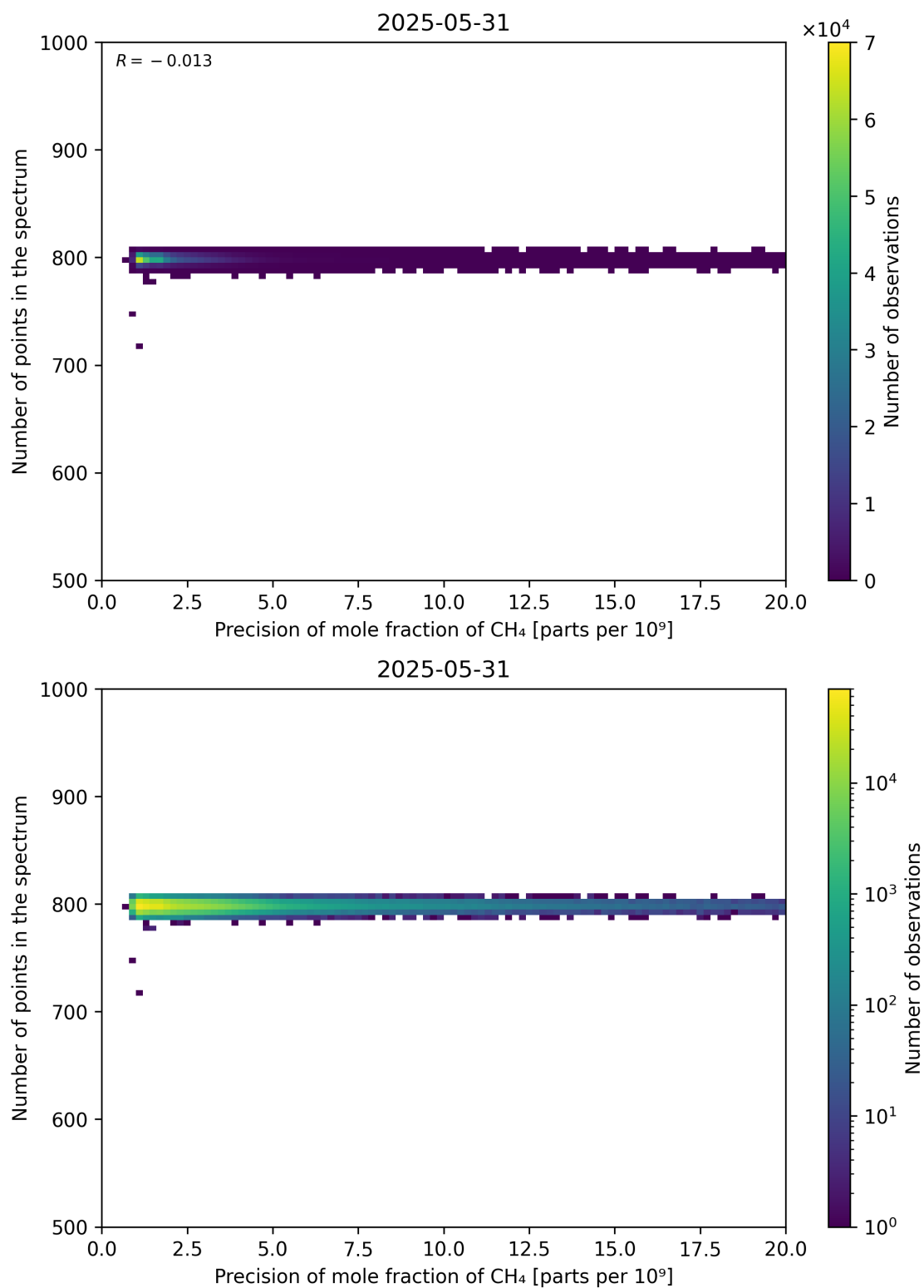
Figure 84: Scatter density plot of “Precision of mole fraction of CH 4 ” against “Number of points in the spectrum” for 2025-05-31 to 2025-06-01.
