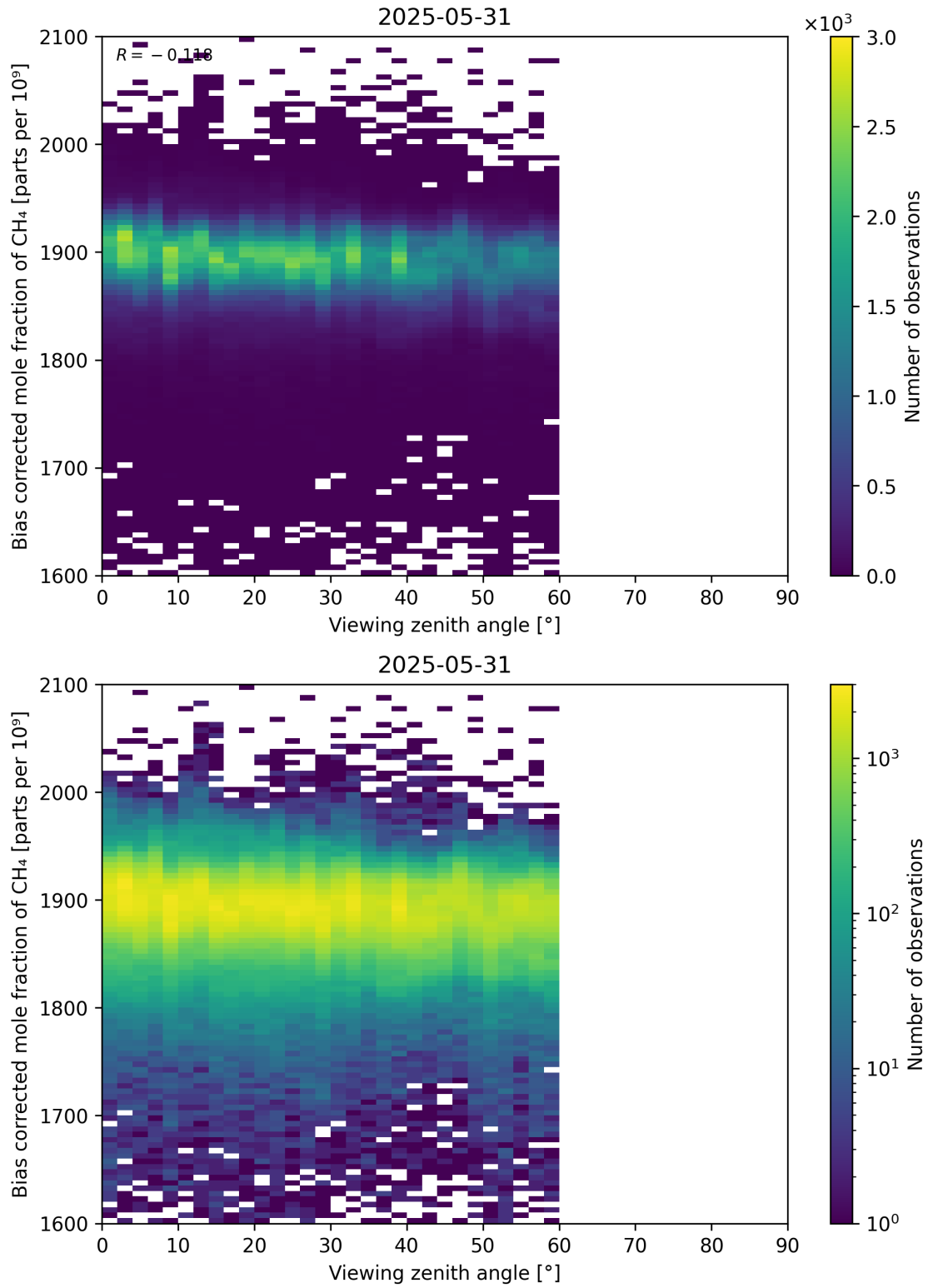
Figure 111: Scatter density plot of “Viewing zenith angle” against “Bias corrected mole fraction of CH 4 ” for 2025-05-31 to 2025-06-01.
