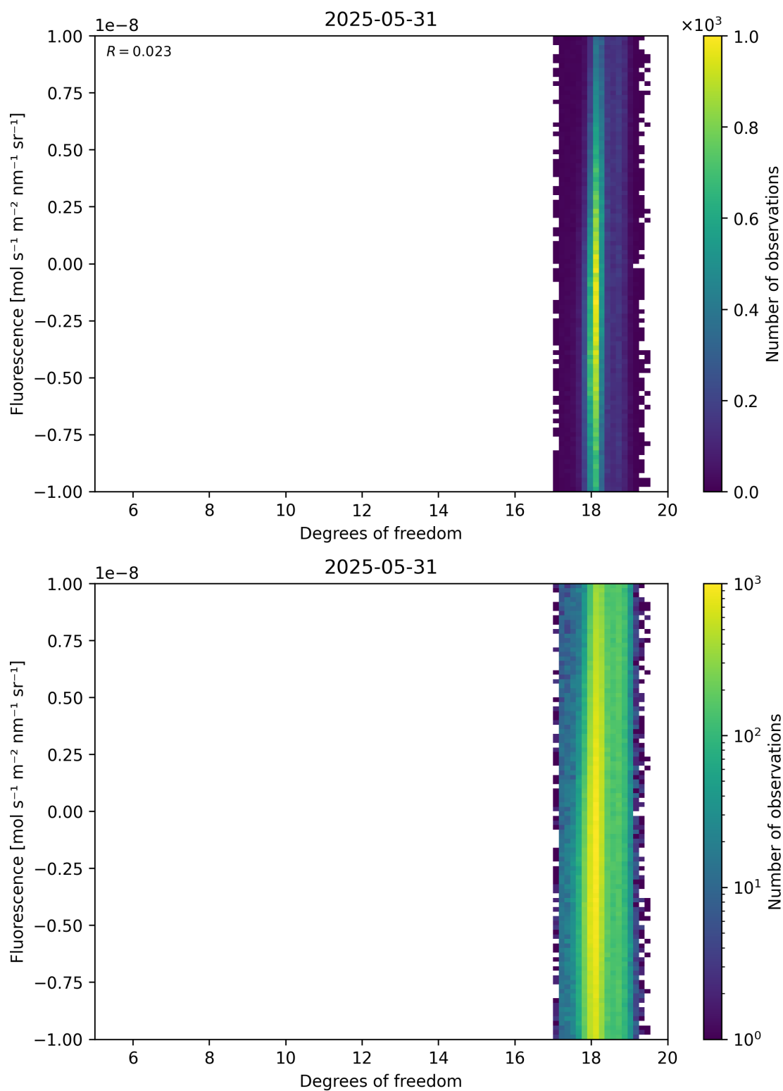
Figure 51: Scatter density plot of “Degrees of freedom” against “Fluorescence” for 2025-05-31 to 2025-06-01.
