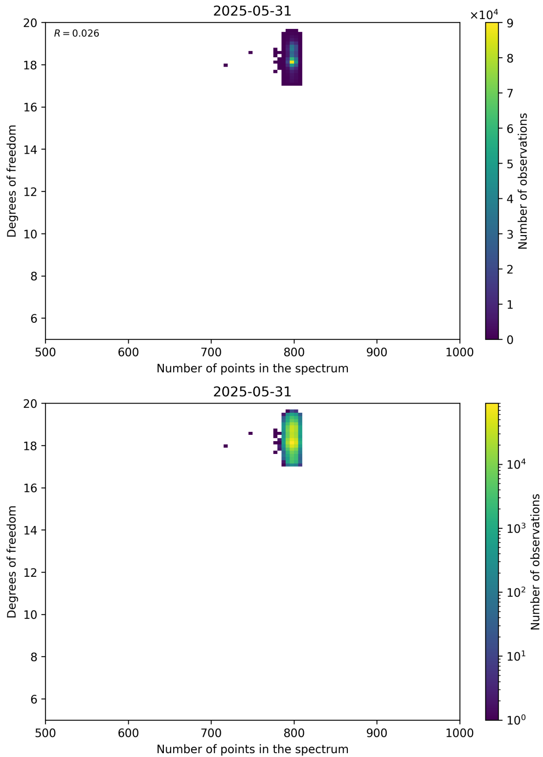
Figure 90: Scatter density plot of “Number of points in the spectrum” against “Degrees of freedom” for 2025-05-31 to 2025-06-01.
