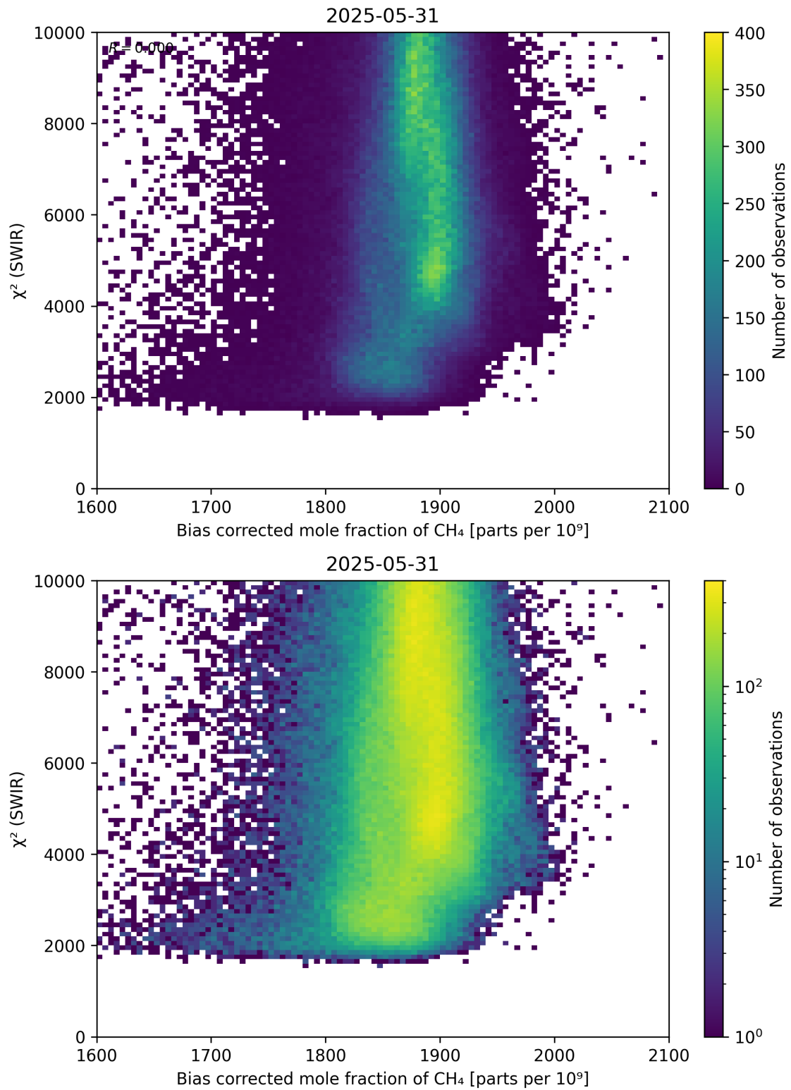
Figure 64: Scatter density plot of “Bias corrected mole fraction of \text{CH}_4 ” against “ \chi^2 (SWIR)” for 2025-05-31 to 2025-06-01.
