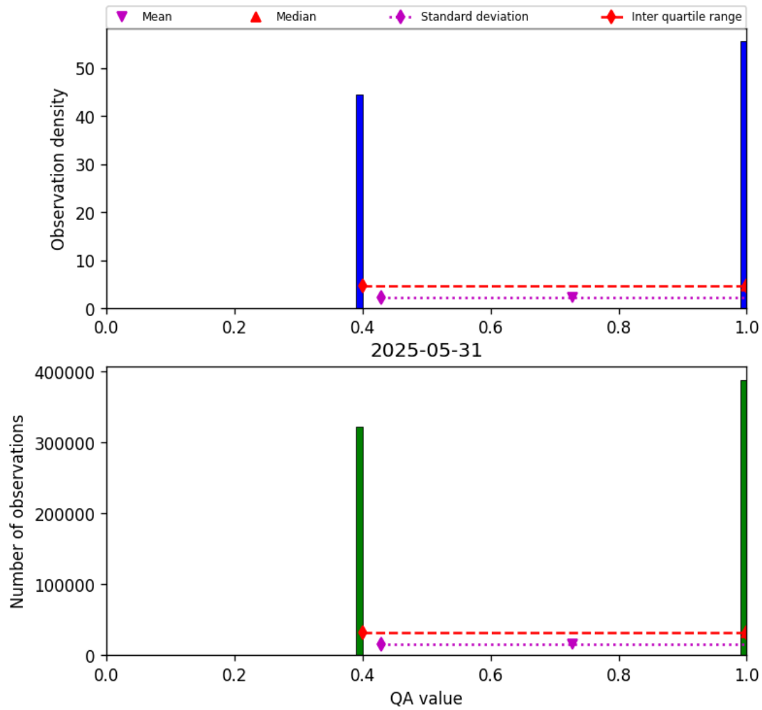
Figure 22: Histogram of “QA value” for 2025-05-31 to 2025-06-01
