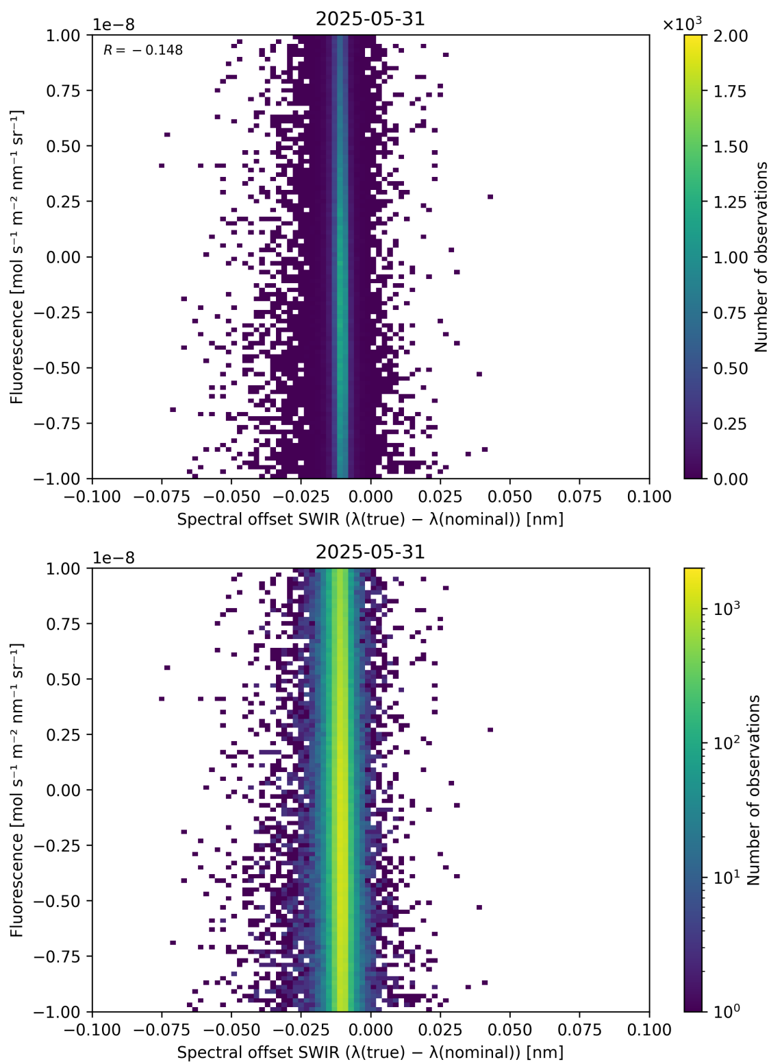
Figure 120: Scatter density plot of “Spectral offset SWIR ( \lambda_{\text{true}} - \lambda_{\text{nominal}} )” against “Fluorescence” for 2025-05-31 to 2025-06-01.
