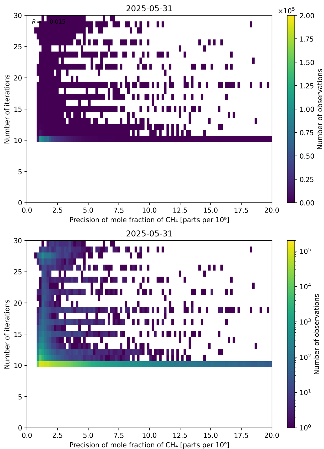
Figure 83: Scatter density plot of “Precision of mole fraction of \text{CH}_4 ” against “Number of iterations” for 2025-05-31 to 2025-06-01.
