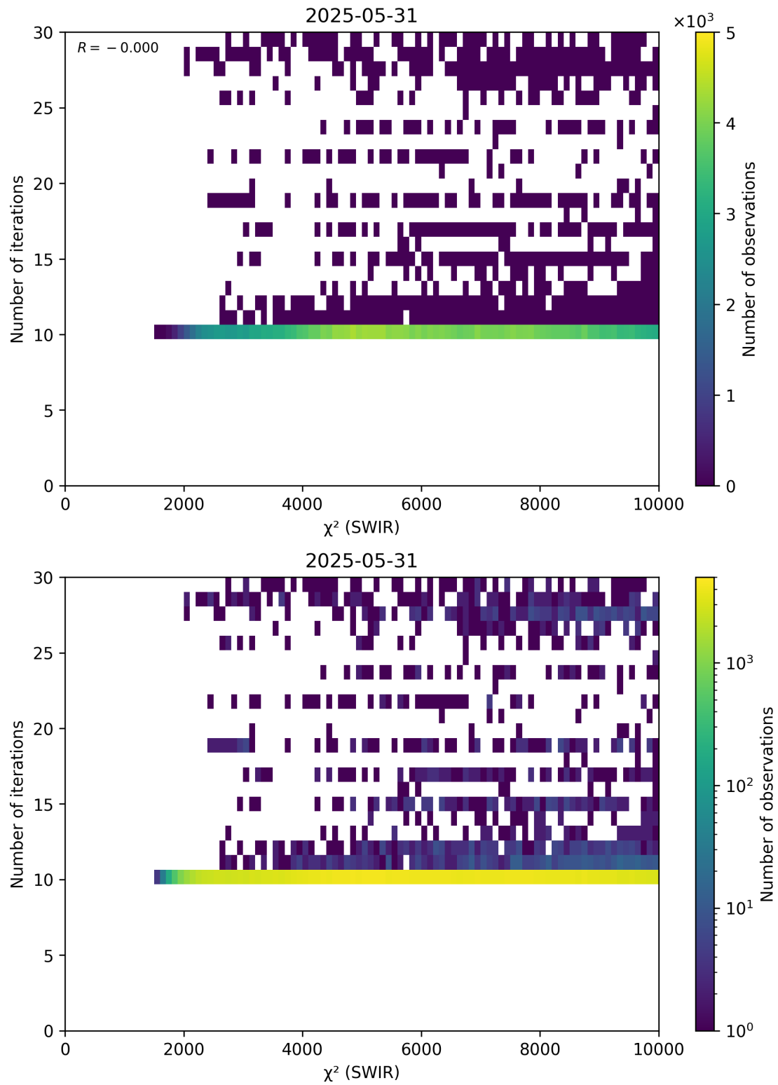
Figure 50: Scatter density plot of “ \chi^2 (SWIR)” against “Number of iterations” for 2025-05-31 to 2025-06-01.
