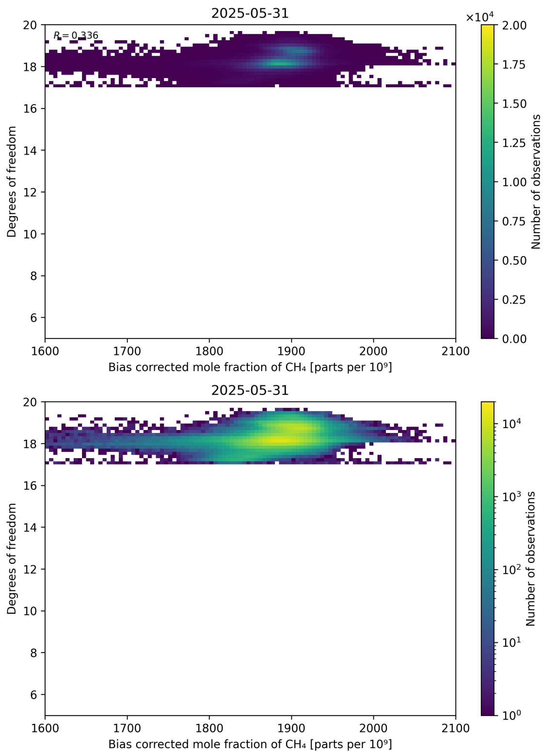
Figure 65: Scatter density plot of “Bias corrected mole fraction of CH 4 ” against “Degrees of freedom” for 2025-05-31 to 2025-06-01.
