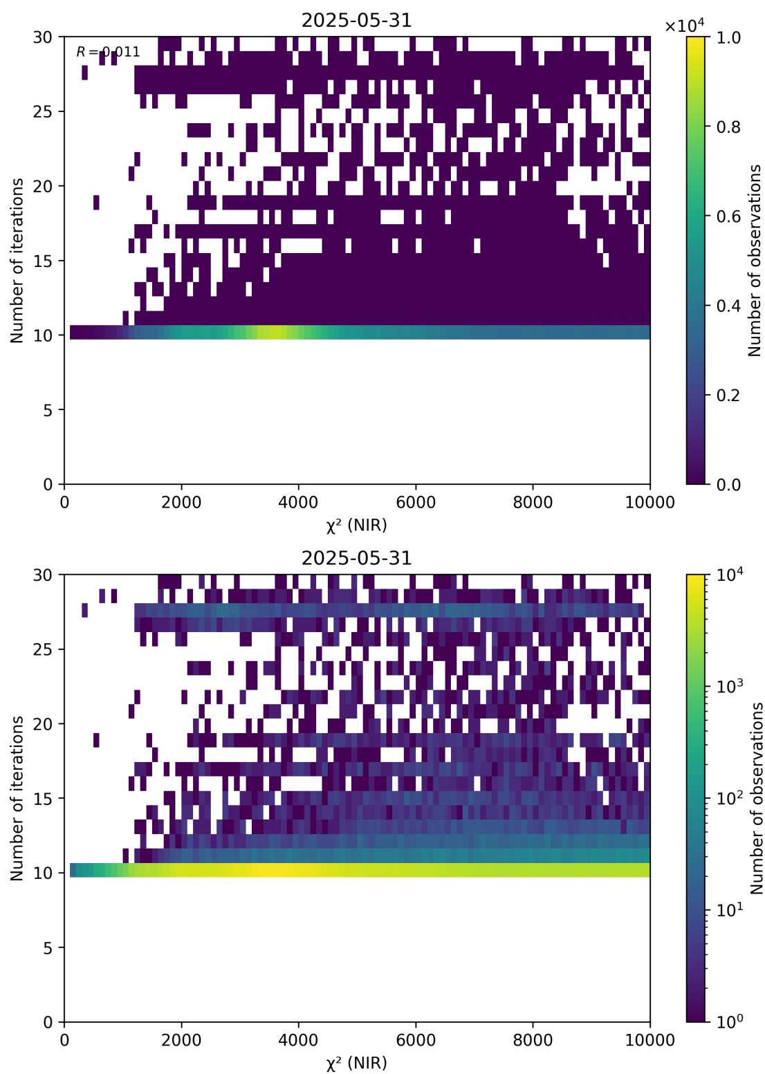
Figure 46: Scatter density plot of “ \chi^2 (NIR)” against “Number of iterations” for 2025-05-31 to 2025-06-01.
