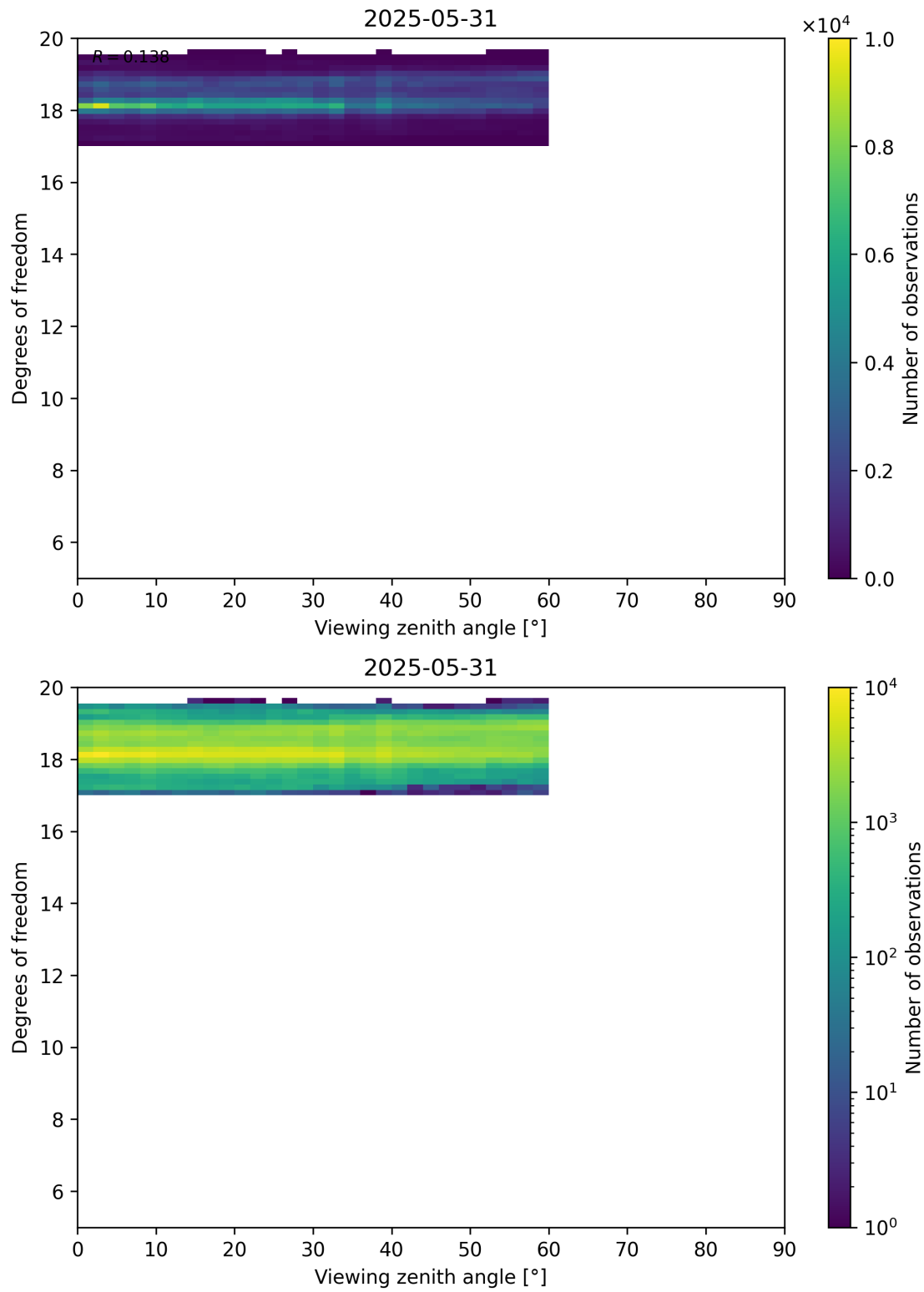
Figure 107: Scatter density plot of “Viewing zenith angle” against “Degrees of freedom” for 2025-05-31 to 2025-06-01.
