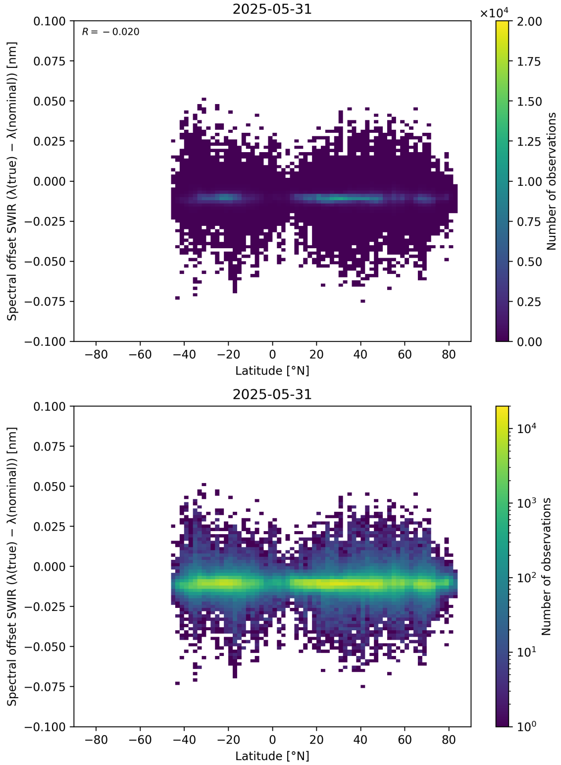
Figure 62: Scatter density plot of “Latitude” against “Spectral offset SWIR ( \lambda_{\text{true}} - \lambda_{\text{nominal}} )” for 2025-05-31 to 2025-06-01.
