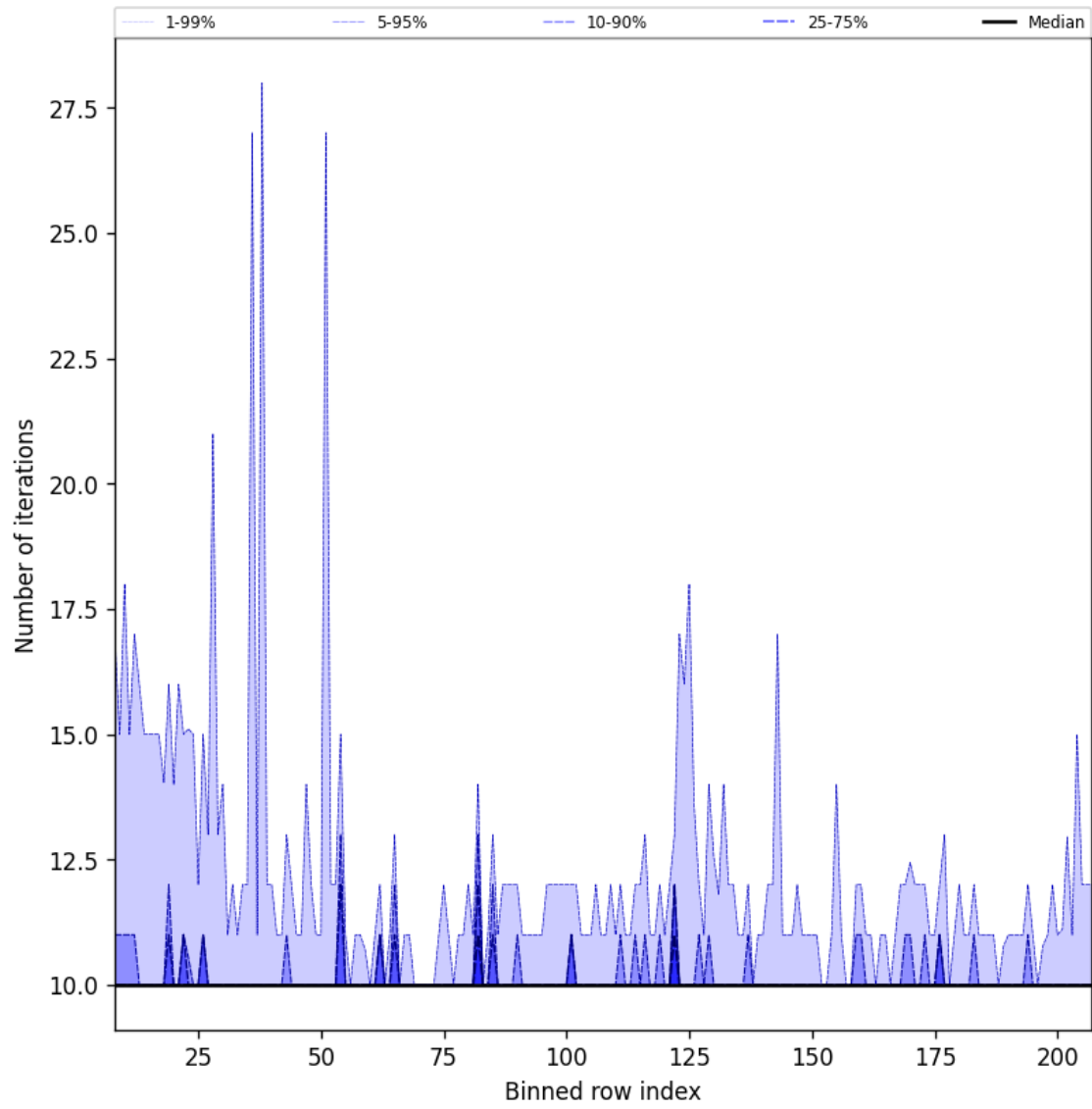
Figure 42: Along track statistics of “Number of iterations” for 2025-05-31 to 2025-06-01
