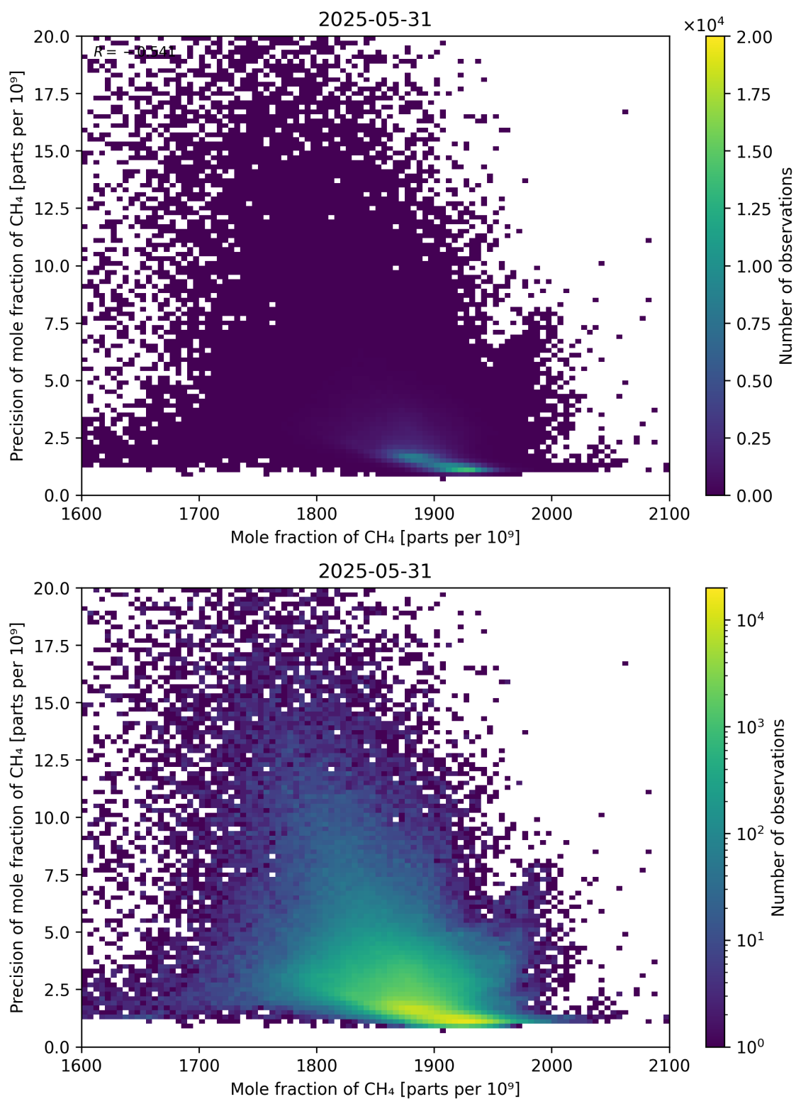
Figure 75: Scatter density plot of “Mole fraction of CH 4 ” against “Precision of mole fraction of CH 4 ” for 2025-05-31 to 2025-06-01.
