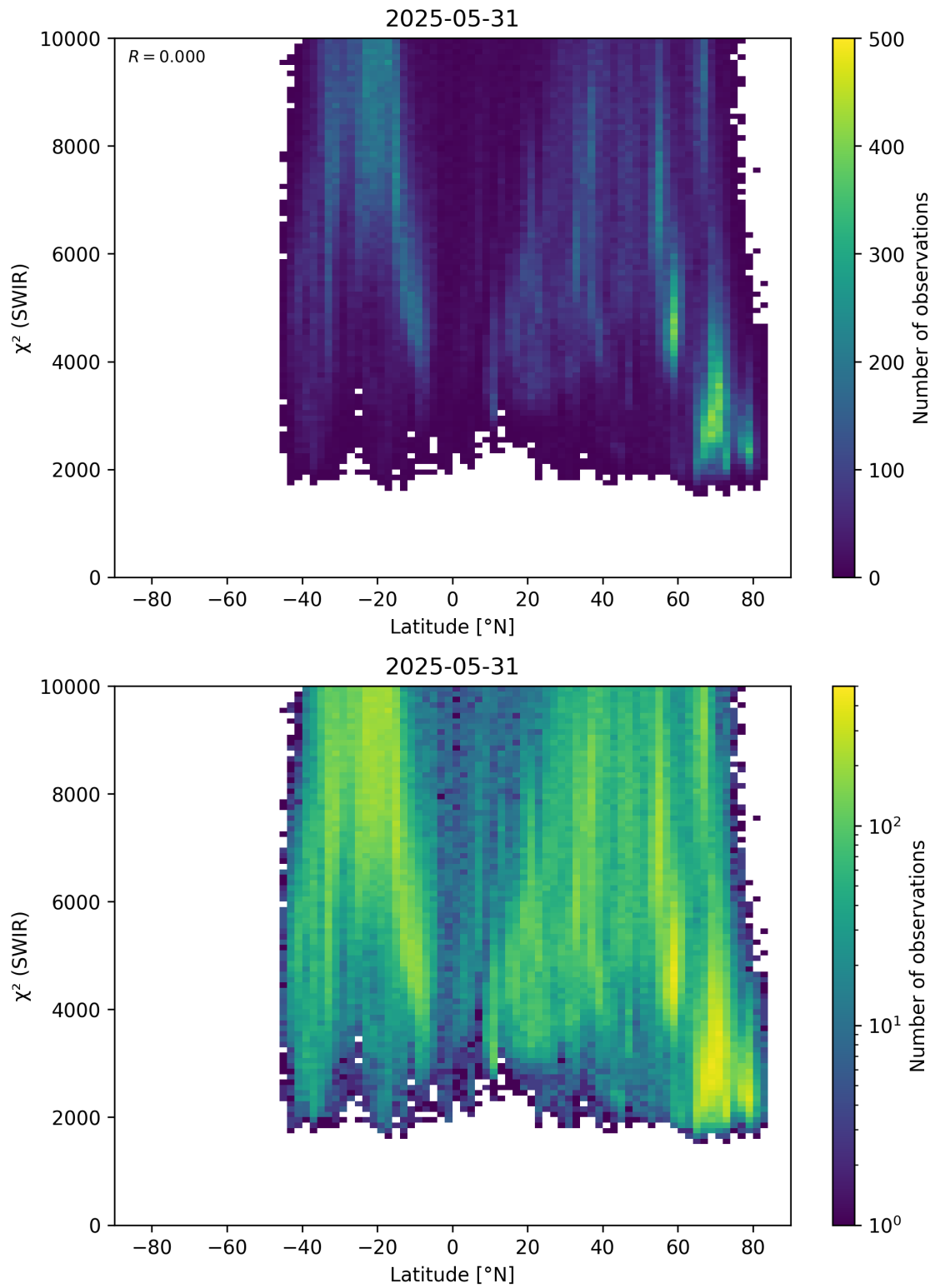
Figure 54: Scatter density plot of “Latitude” against “ \chi^2 (SWIR)” for 2025-05-31 to 2025-06-01.
