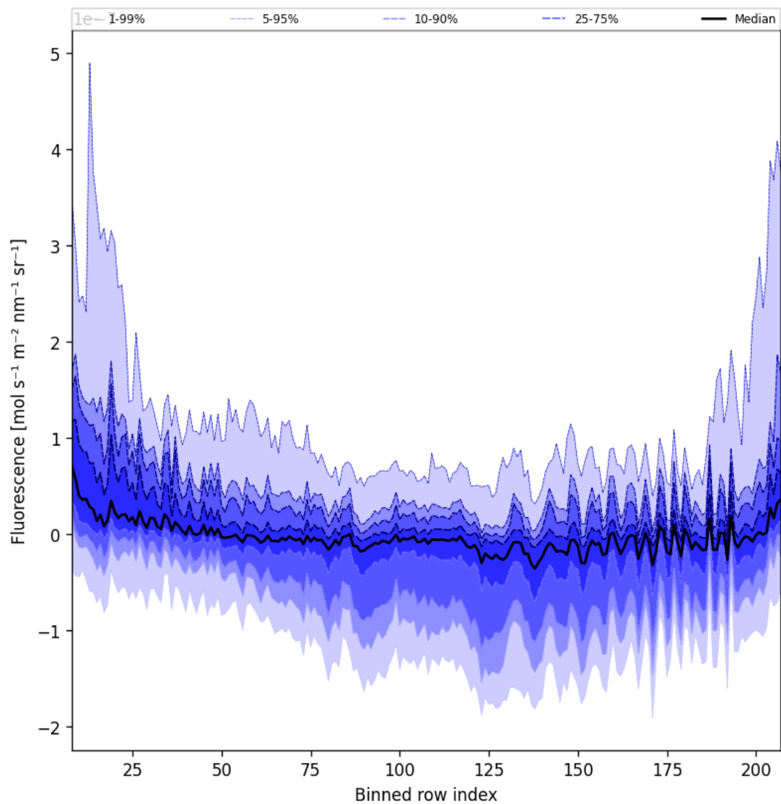
Figure 43: Along track statistics of “Fluorescence” for 2025-05-31 to 2025-06-01
