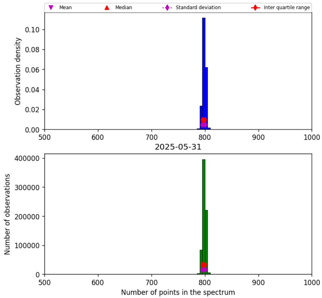
Figure 26: Histogram of “Number of points in the spectrum” for 2025-05-31 to 2025-06-01
