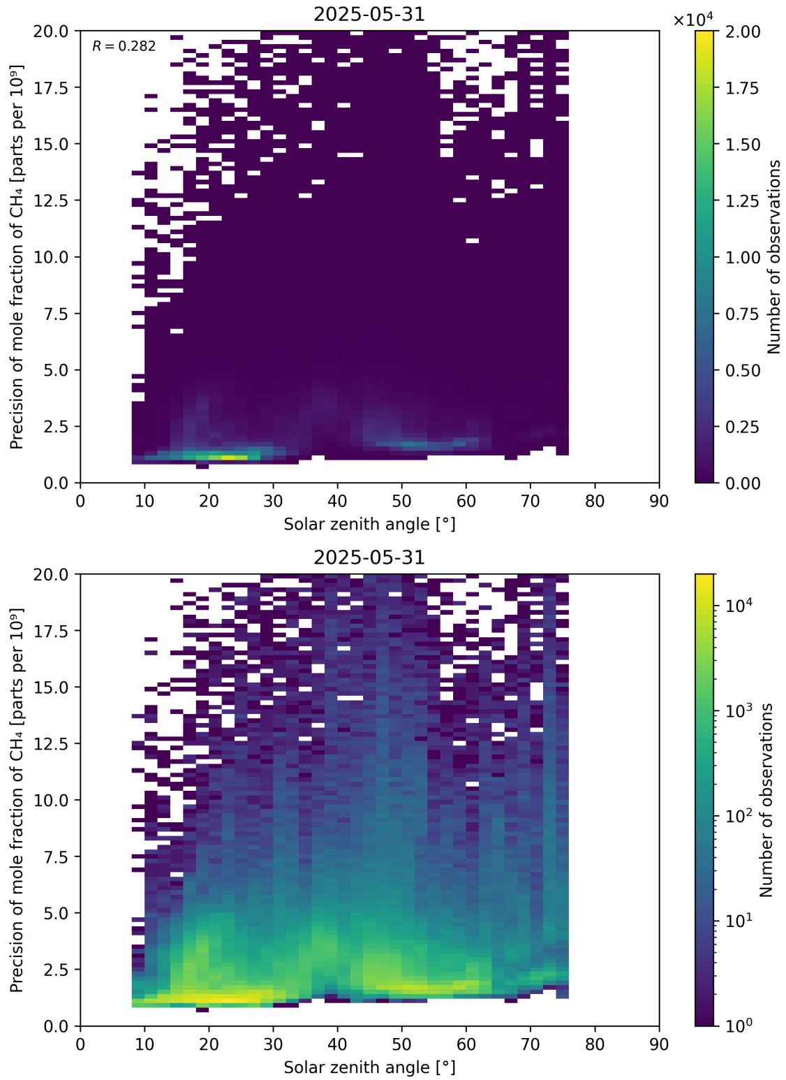
Figure 101: Scatter density plot of “Solar zenith angle” against “Precision of mole fraction of CH 4 ” for 2025-05-31 to 2025-06-01.
