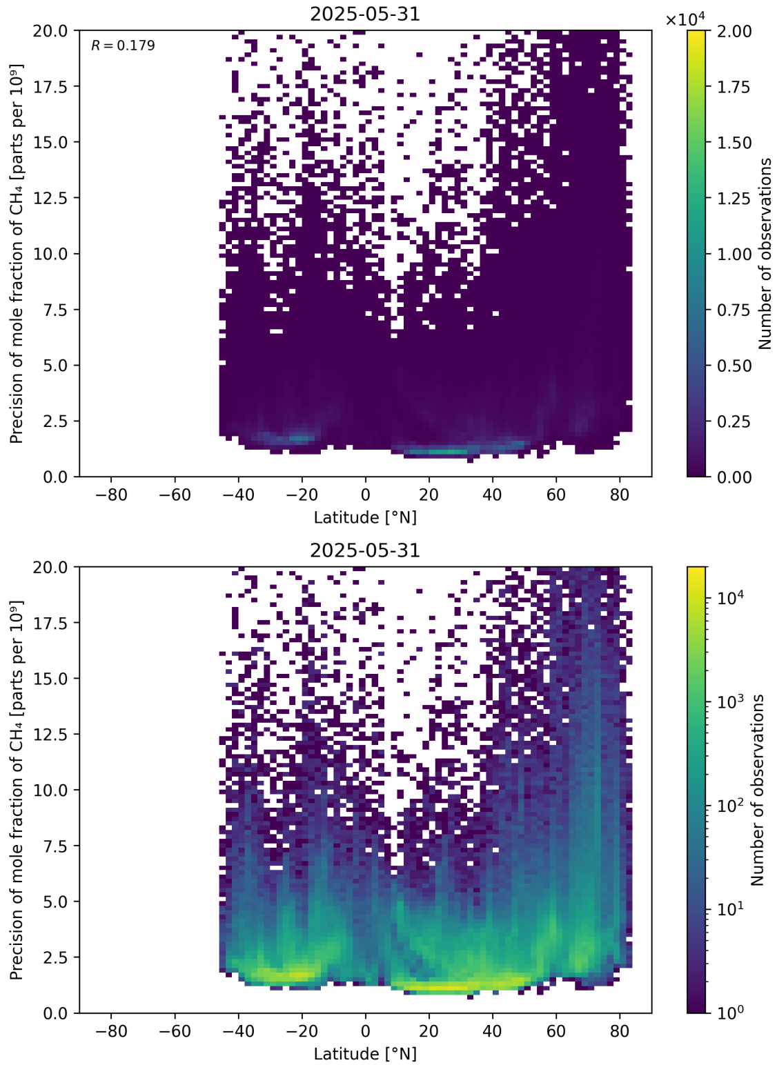
Figure 59: Scatter density plot of “Latitude” against “Precision of mole fraction of \text{CH}_4 ” for 2025-05-31 to 2025-06-01.
