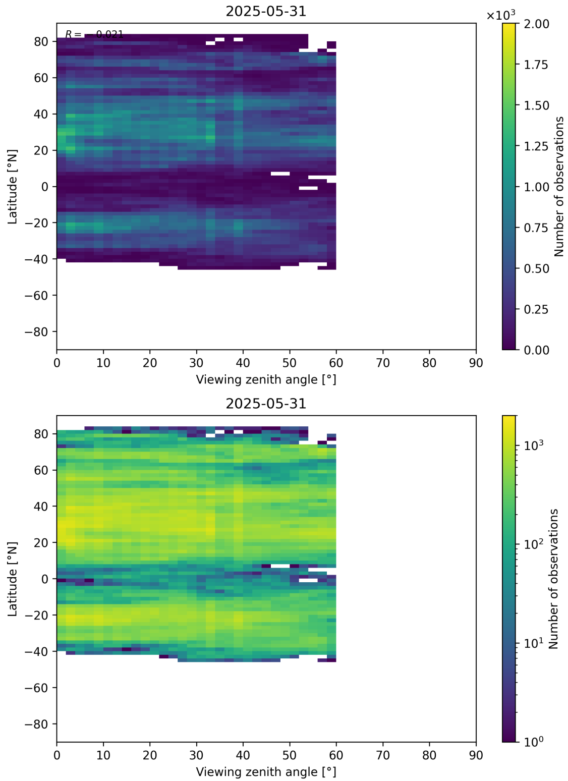
Figure 109: Scatter density plot of “Viewing zenith angle” against “Latitude” for 2025-05-31 to 2025-06-01.
