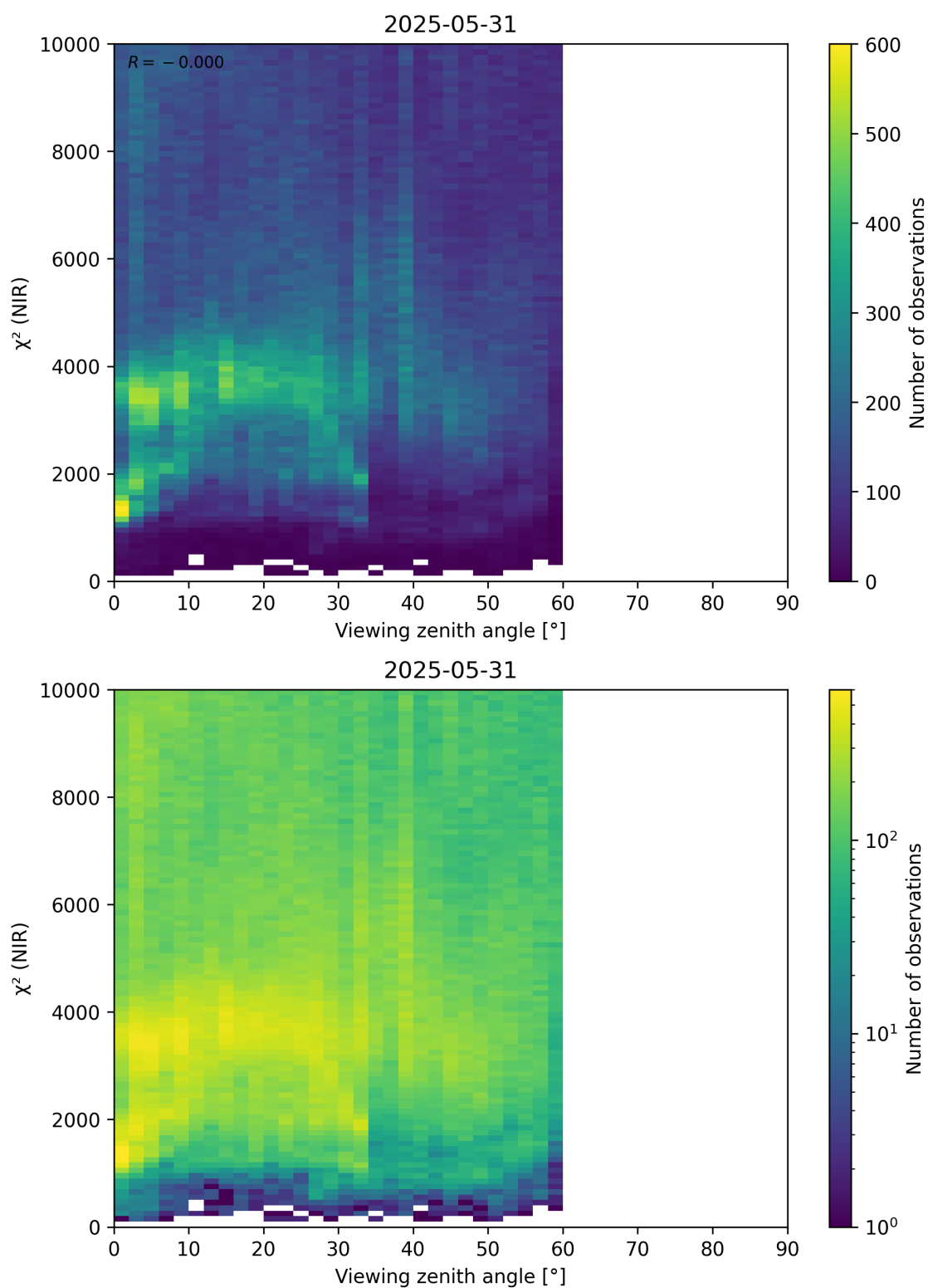
Figure 105: Scatter density plot of “Viewing zenith angle” against “ \chi^2 (NIR)” for 2025-05-31 to 2025-06-01.
