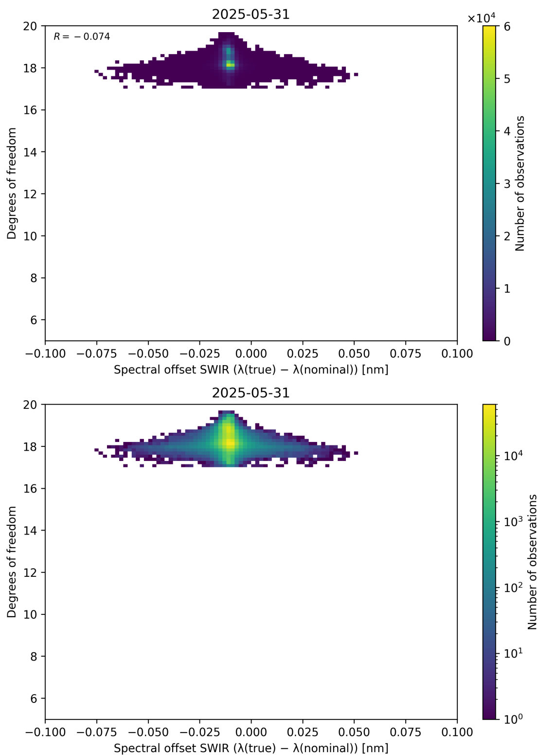
Figure 119: Scatter density plot of “Spectral offset SWIR ( \lambda_{\text{true}} - \lambda_{\text{nominal}} )” against “Degrees of freedom” for 2025-05-31 to 2025-06-01.
