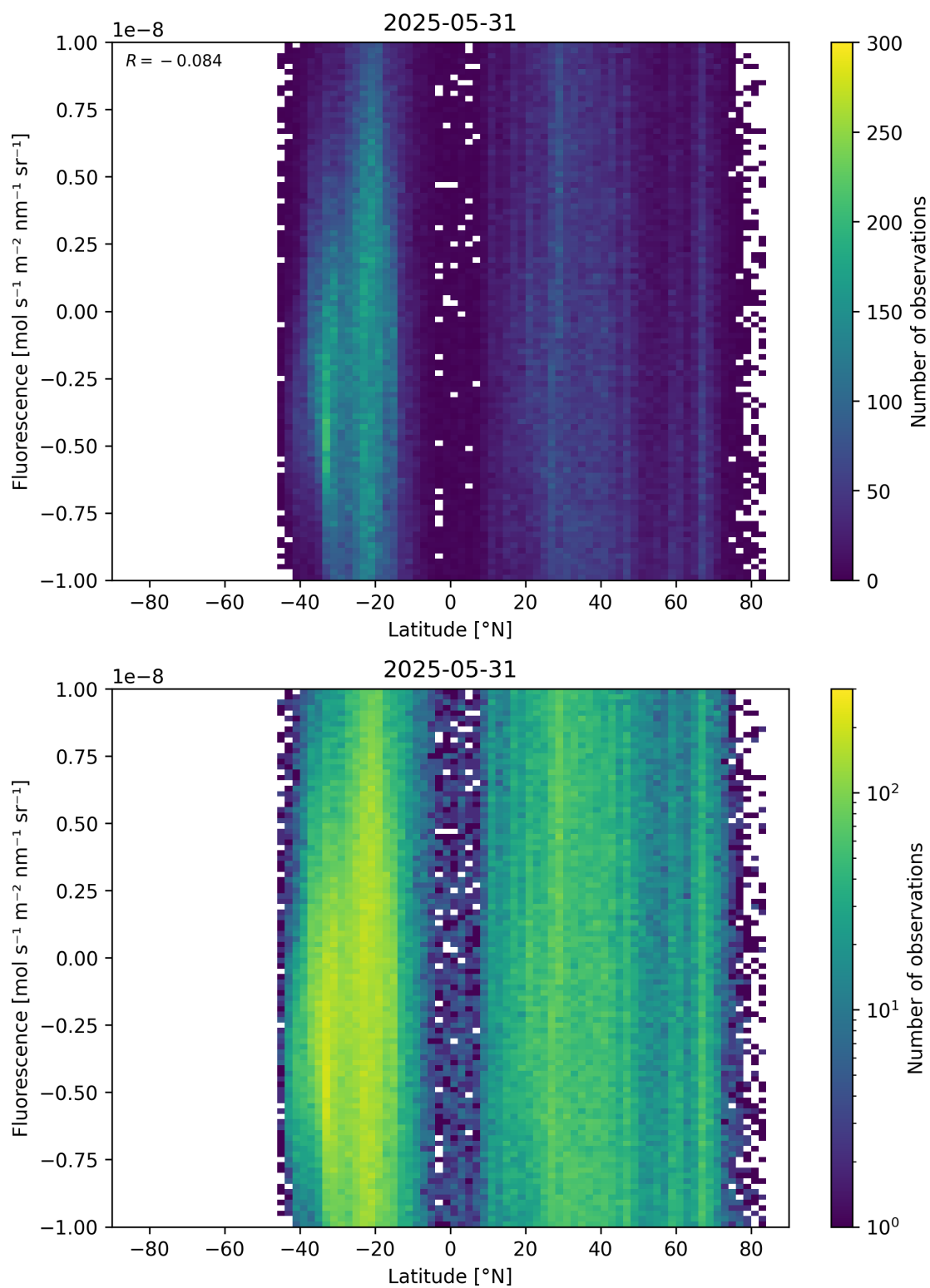
Figure 56: Scatter density plot of “Latitude” against “Fluorescence” for 2025-05-31 to 2025-06-01.
