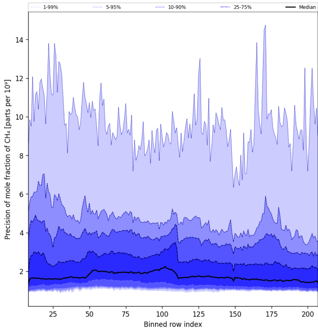
Figure 35: Along track statistics of “Precision of mole fraction of CH 4 ” for 2025-05-31 to 2025-06-01
