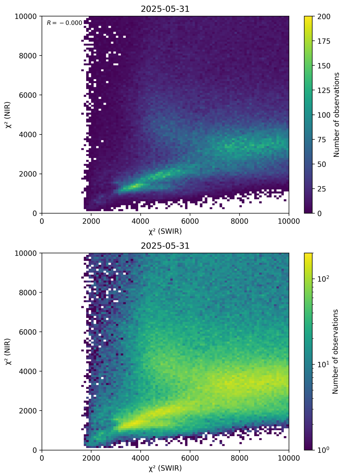
Figure 47: Scatter density plot of “ \chi^2 (SWIR)” against “ \chi^2 (NIR)” for 2025-05-31 to 2025-06-01.
