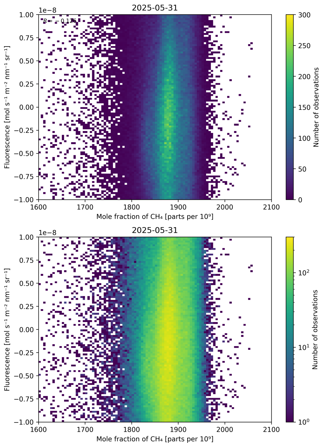
Figure 73: Scatter density plot of “Mole fraction of \text{CH}_4 ” against “Fluorescence” for 2025-05-31 to 2025-06-01.
