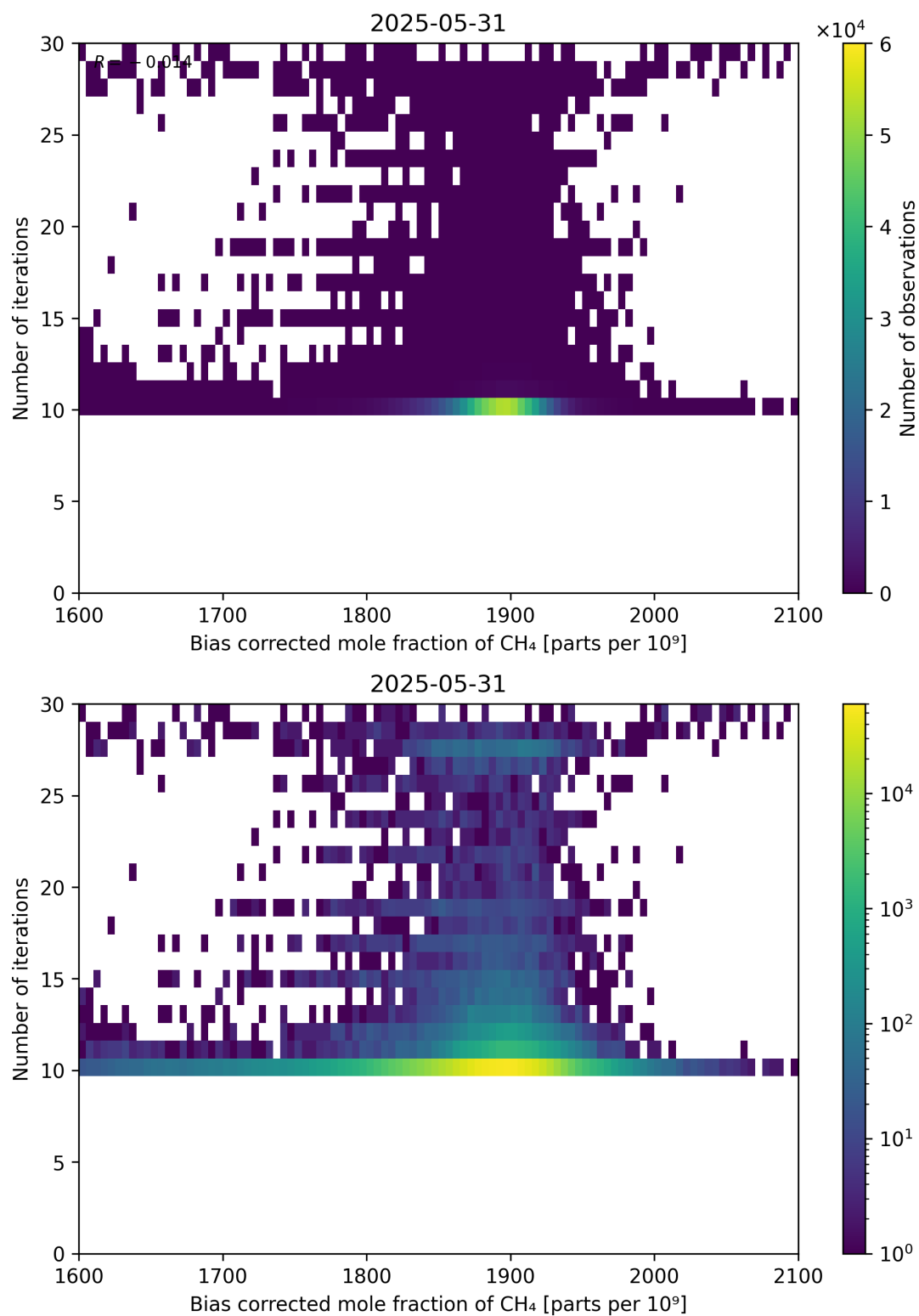
Figure 67: Scatter density plot of “Bias corrected mole fraction of CH 4 ” against “Number of iterations” for 2025-05-31 to 2025-06-01.
