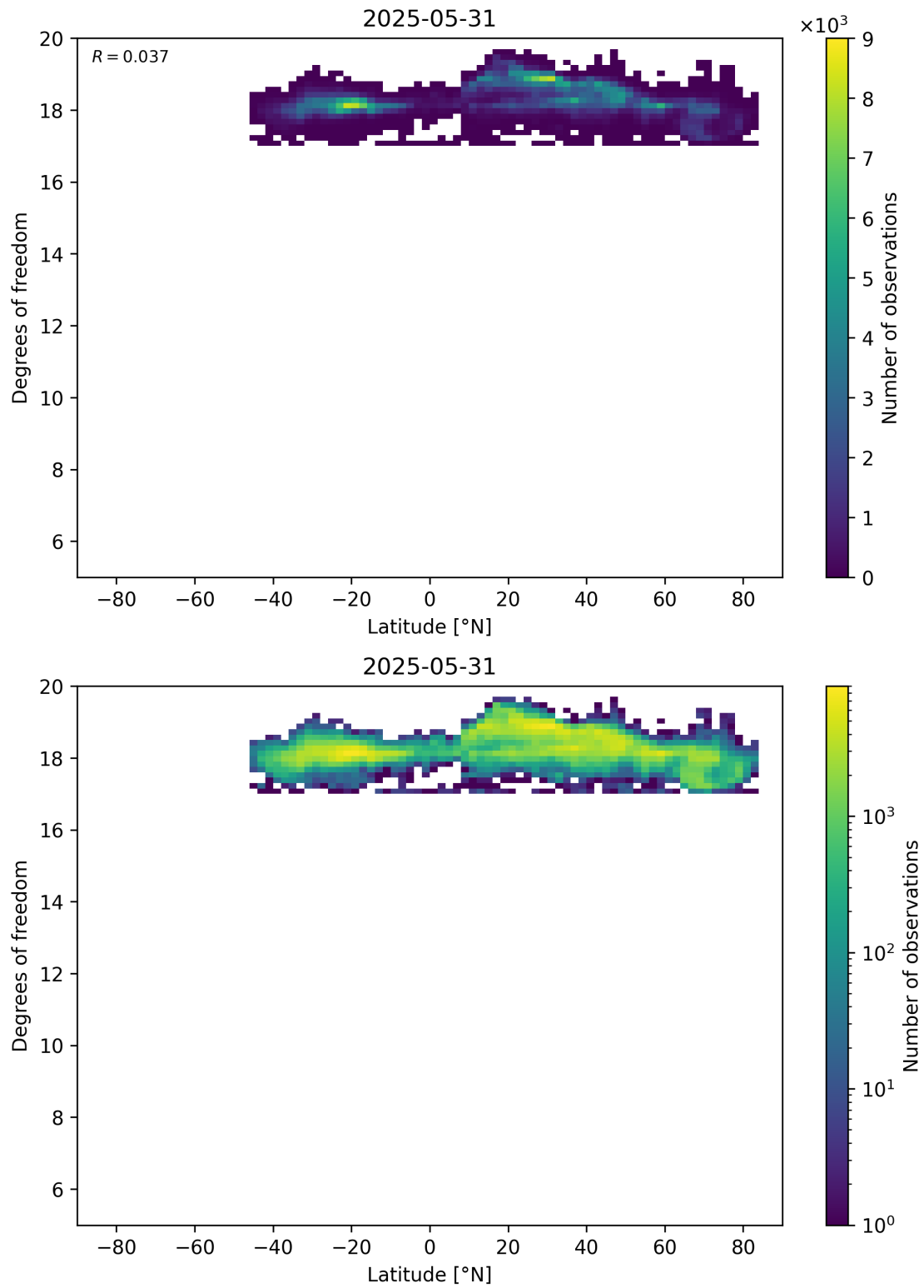
Figure 55: Scatter density plot of “Latitude” against “Degrees of freedom” for 2025-05-31 to 2025-06-01.
