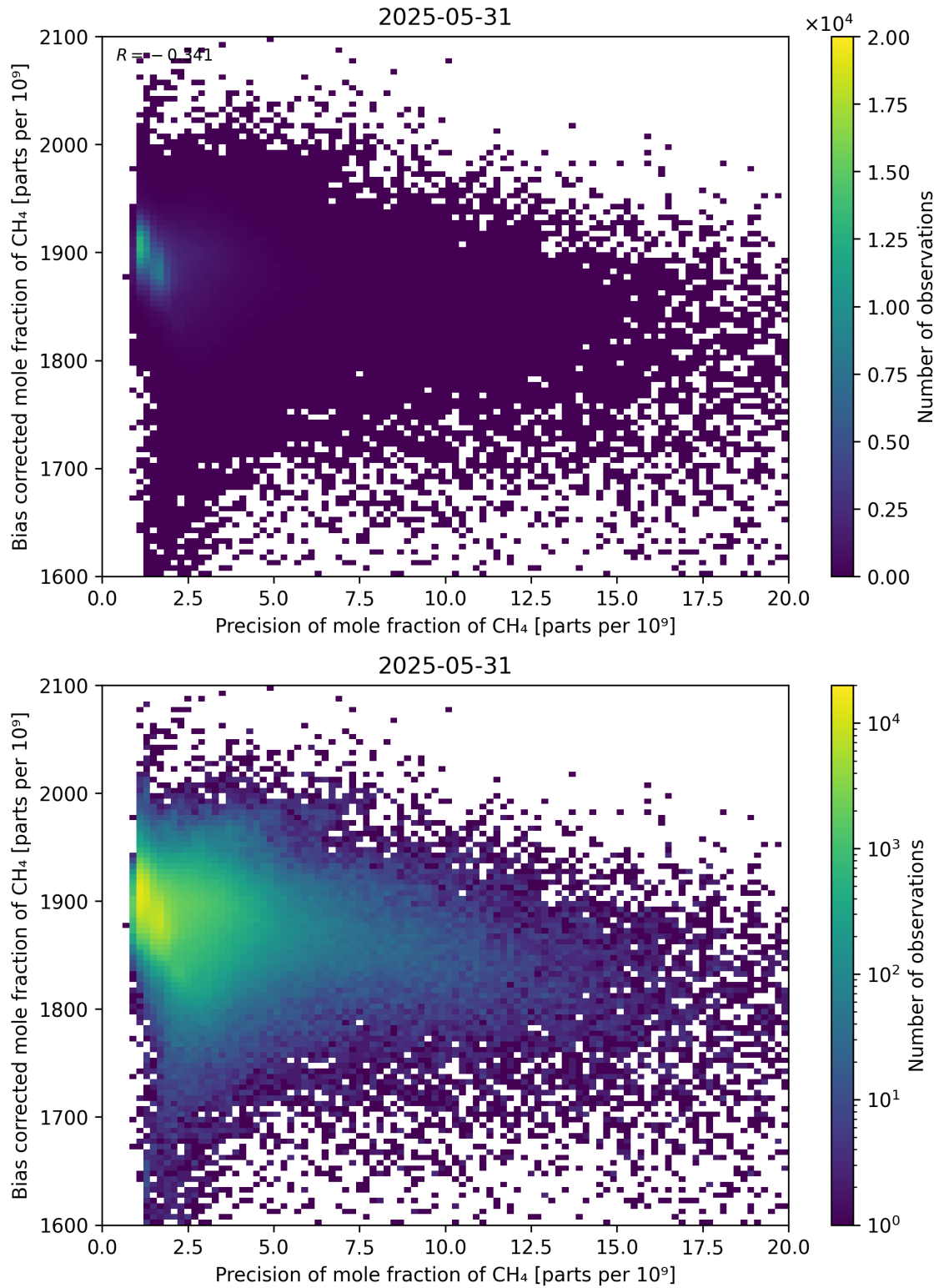
Figure 82: Scatter density plot of “Precision of mole fraction of CH 4 ” against “Bias corrected mole fraction of CH 4 ” for 2025-05-31 to 2025-06-01.
