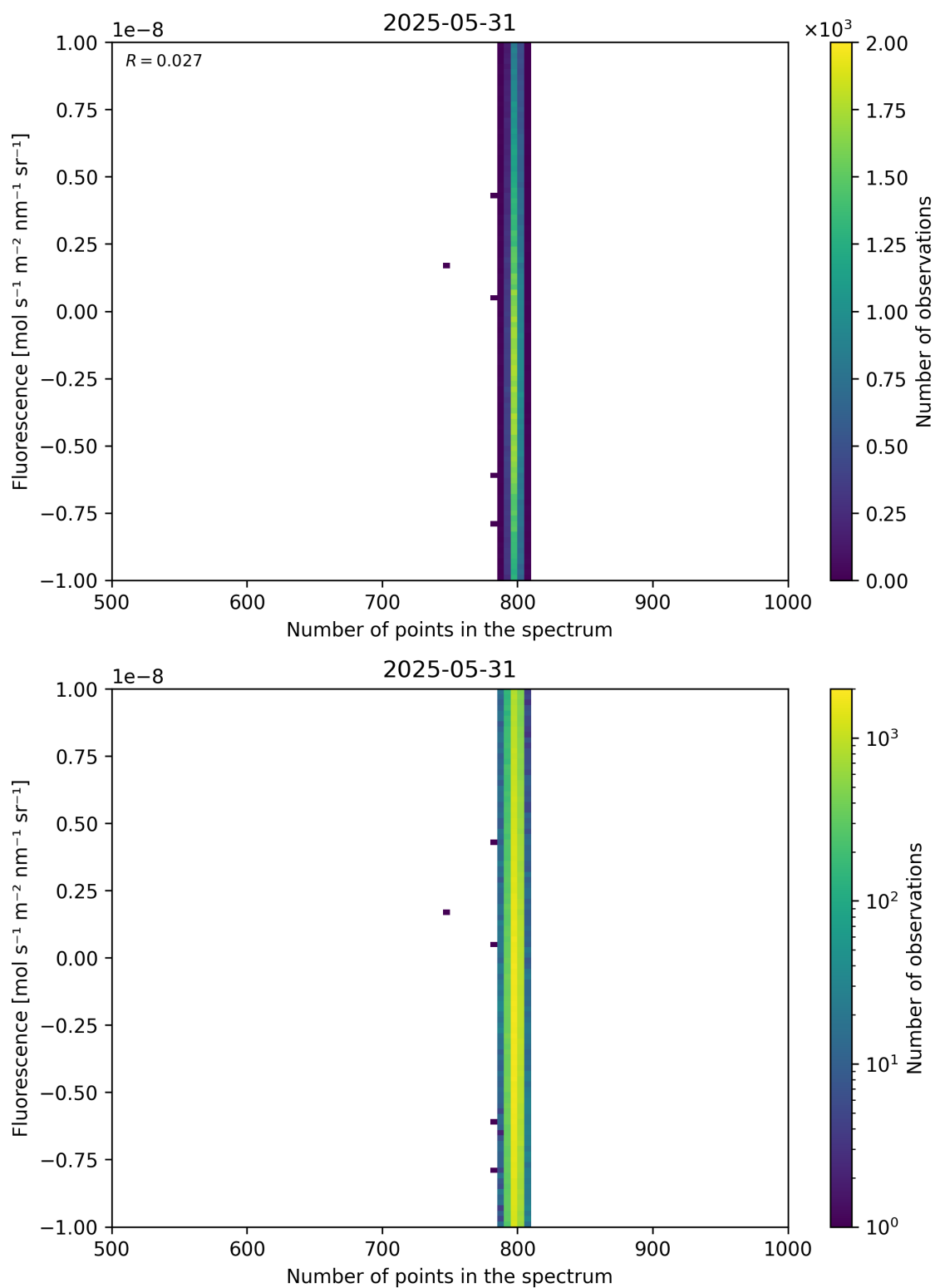
Figure 91: Scatter density plot of “Number of points in the spectrum” against “Fluorescence” for 2025-05-31 to 2025-06-01.
