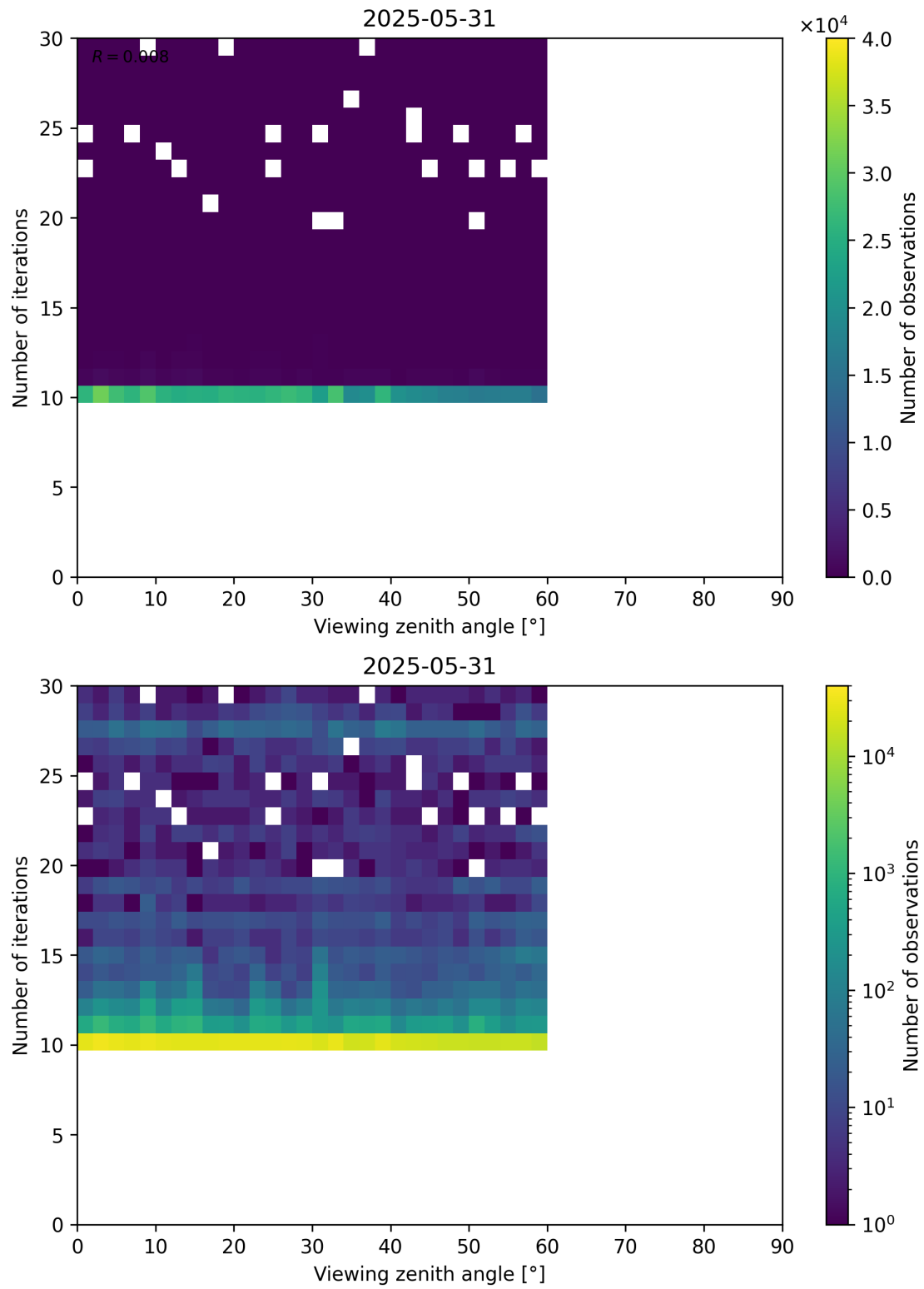
Figure 113: Scatter density plot of “Viewing zenith angle” against “Number of iterations” for 2025-05-31 to 2025-06-01.
