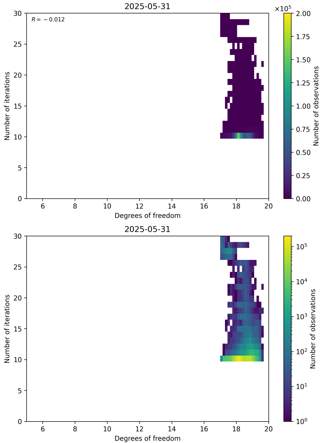
Figure 52: Scatter density plot of “Degrees of freedom” against “Number of iterations” for 2025-05-31 to 2025-06-01.
