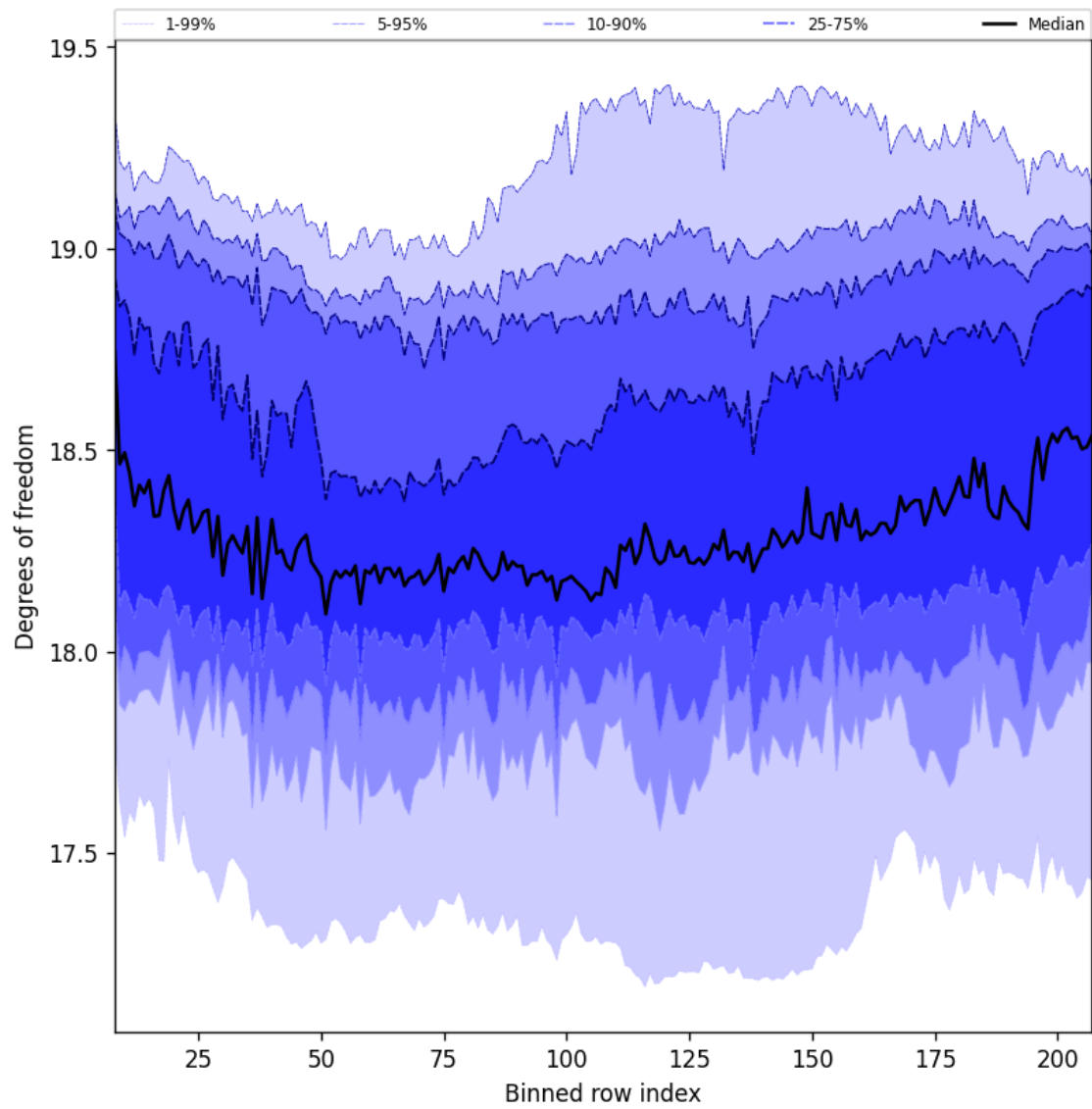
Figure 41: Along track statistics of “Degrees of freedom” for 2025-05-31 to 2025-06-01
