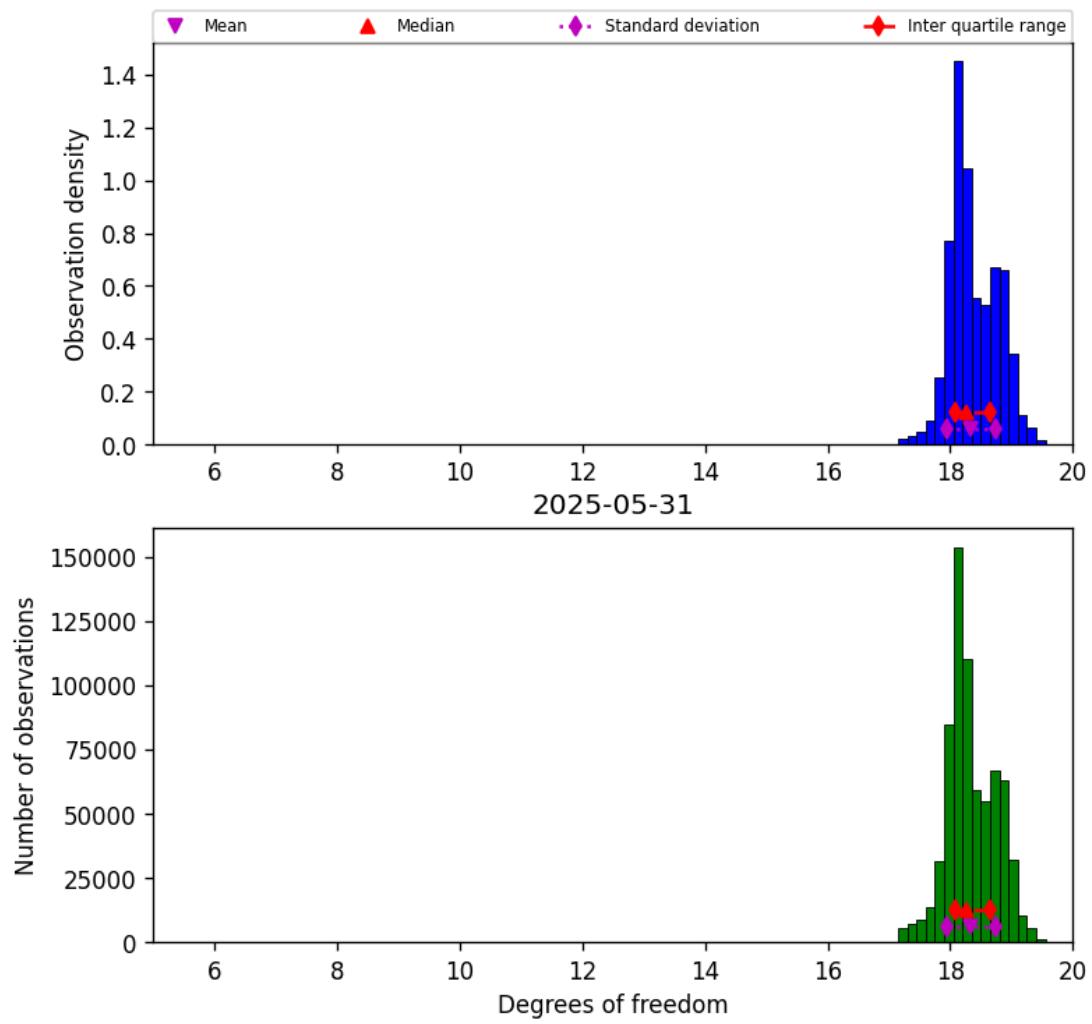
Figure 30: Histogram of “Degrees of freedom” for 2025-05-31 to 2025-06-01
