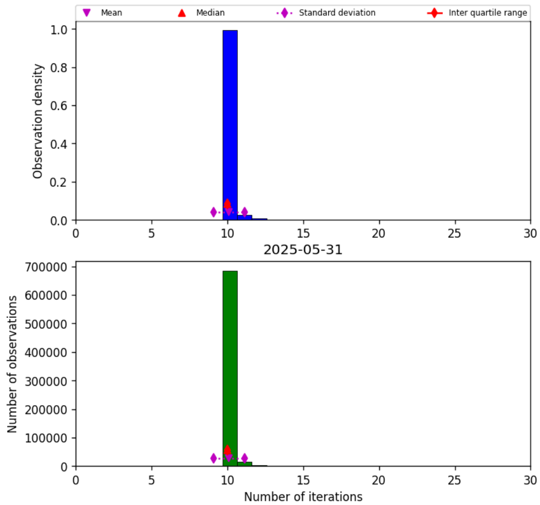
Figure 31: Histogram of “Number of iterations” for 2025-05-31 to 2025-06-01
