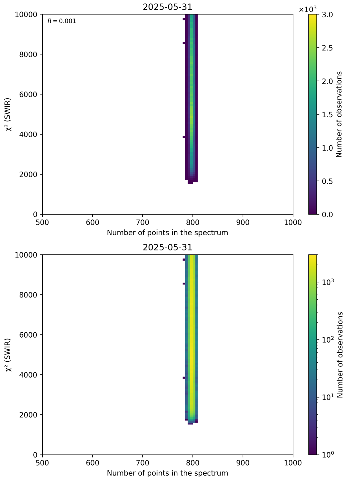
Figure 89: Scatter density plot of “Number of points in the spectrum” against “ \chi^2 (SWIR)” for 2025-05-31 to 2025-06-01.
