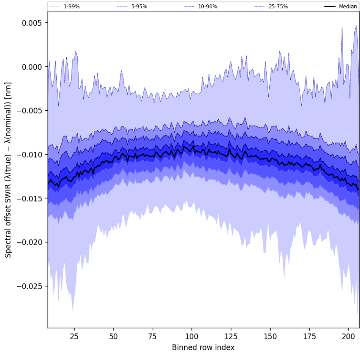
Figure 38: Along track statistics of “Spectral offset SWIR ( \lambda_{\text{true}} - \lambda_{\text{nominal}} )” for 2025-05-31 to 2025-06-01
