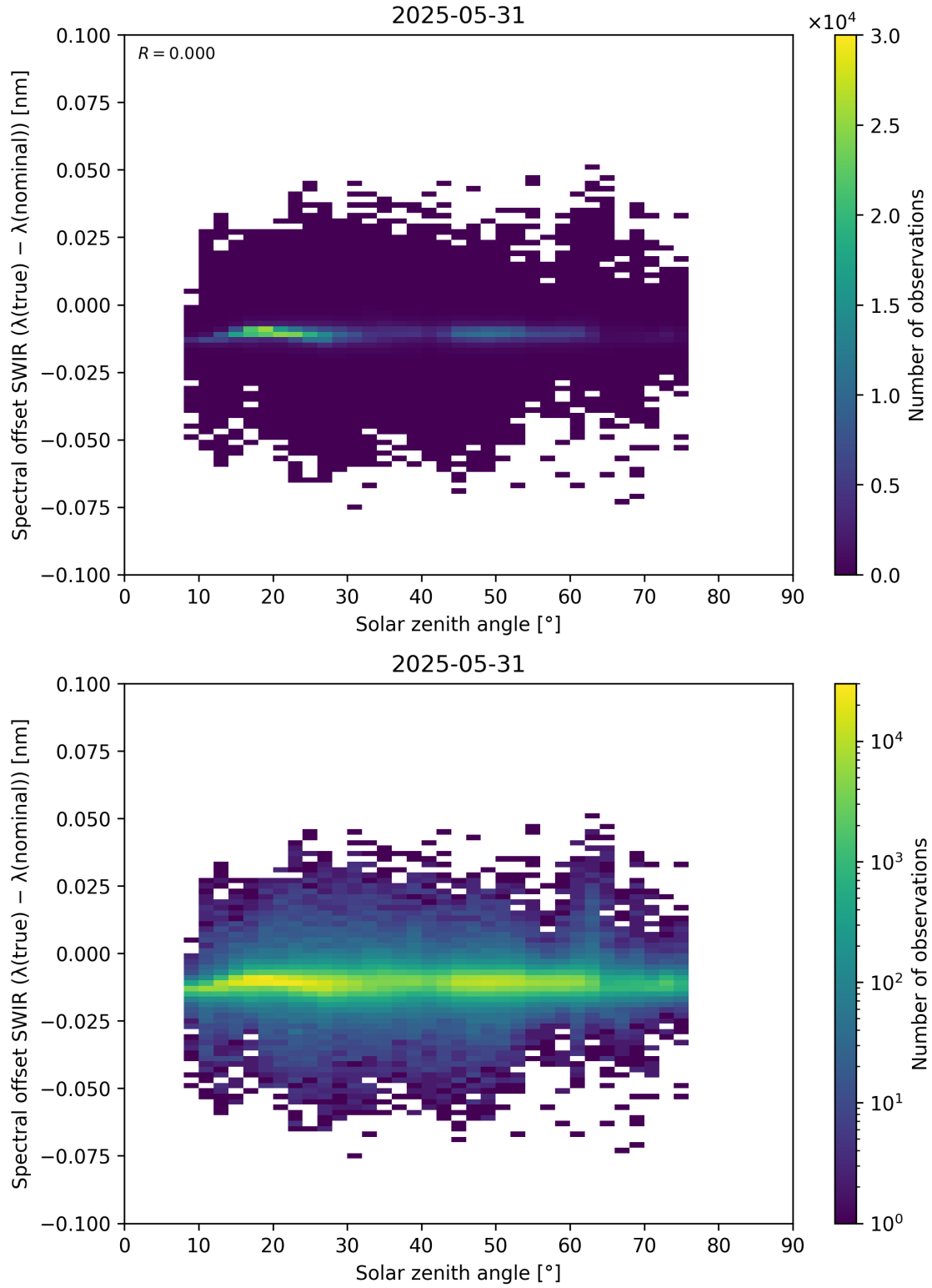
Figure 104: Scatter density plot of “Solar zenith angle” against “Spectral offset SWIR ( \lambda_{\text{true}} - \lambda_{\text{nominal}} )” for 2025-05-31 to 2025-06-01.
