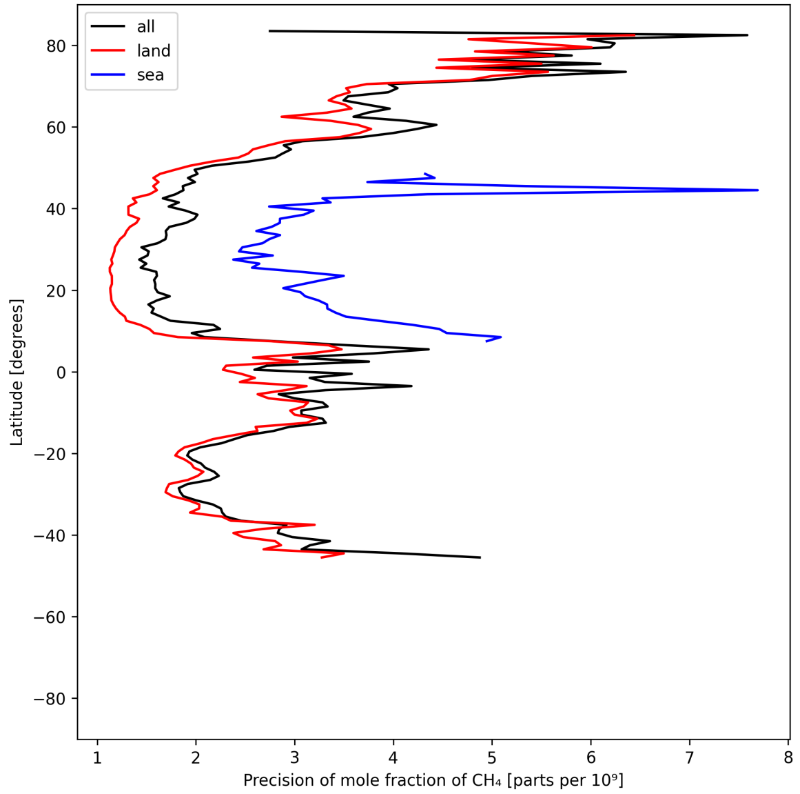
Figure 13: Zonal average of “Precision of mole fraction of CH 4 ” for 2025-05-31 to 2025-06-01.
