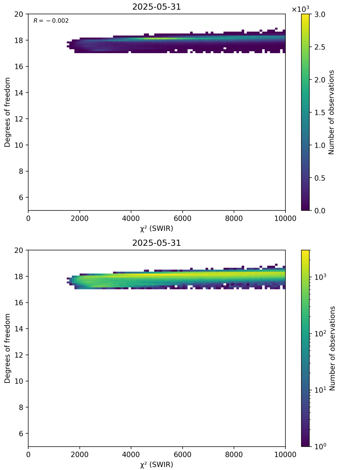
Figure 48: Scatter density plot of “ \chi^2 (SWIR)” against “Degrees of freedom” for 2025-05-31 to 2025-06-01.
