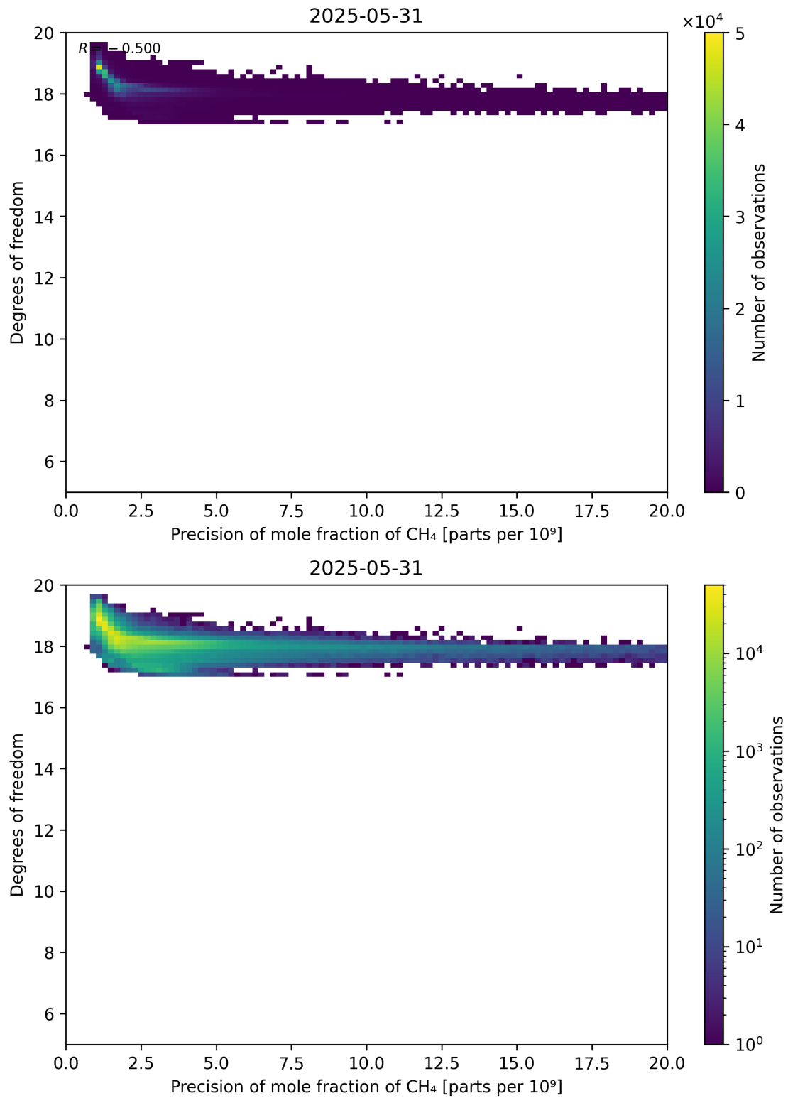
Figure 80: Scatter density plot of “Precision of mole fraction of CH 4 ” against “Degrees of freedom” for 2025-05-31 to 2025-06-01.
