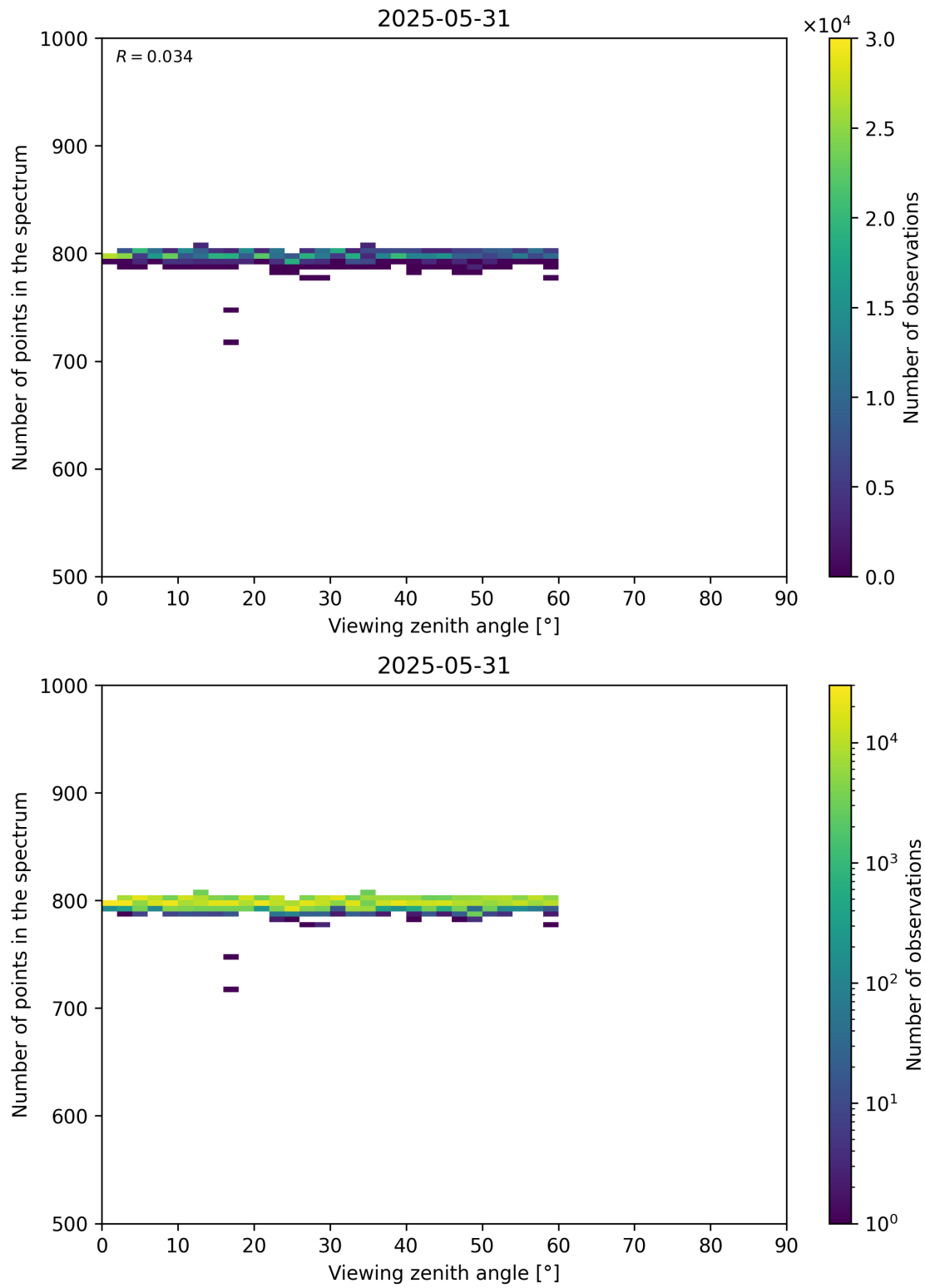
Figure 114: Scatter density plot of “Viewing zenith angle” against “Number of points in the spectrum” for 2025-05-31 to 2025-06-01.
