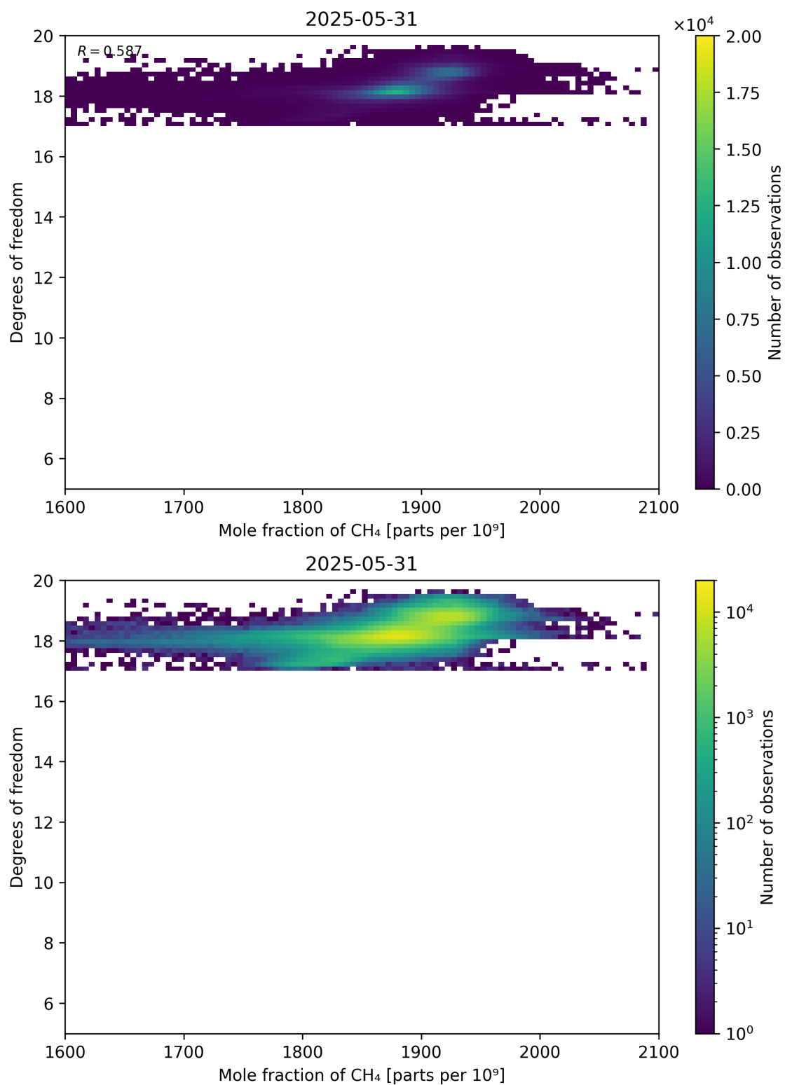
Figure 72: Scatter density plot of “Mole fraction of CH 4 ” against “Degrees of freedom” for 2025-05-31 to 2025-06-01.
