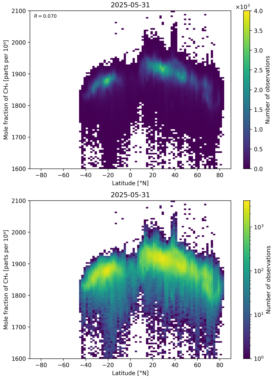
Figure 57: Scatter density plot of “Latitude” against “Mole fraction of \text{CH}_4 ” for 2025-05-31 to 2025-06-01.
