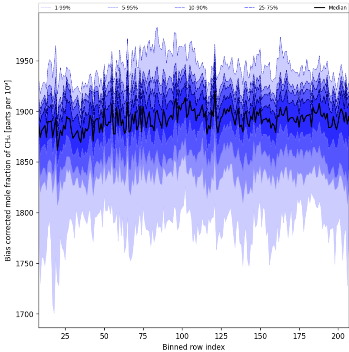
Figure 36: Along track statistics of “Bias corrected mole fraction of CH 4 ” for 2025-05-31 to 2025-06-01
