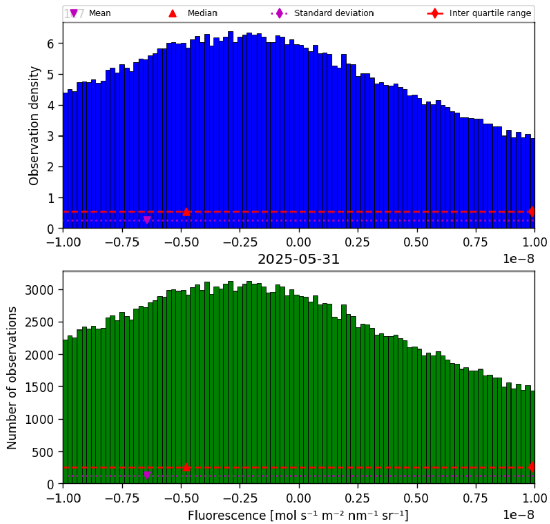
Figure 32: Histogram of “Fluorescence” for 2025-05-31 to 2025-06-01
