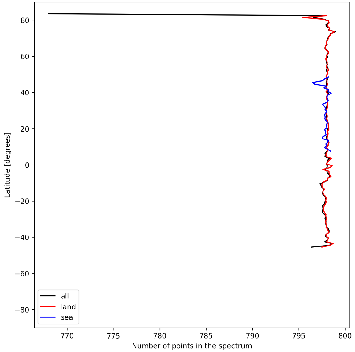
Figure 15: Zonal average of “Number of points in the spectrum” for 2025-05-31 to 2025-06-01.
