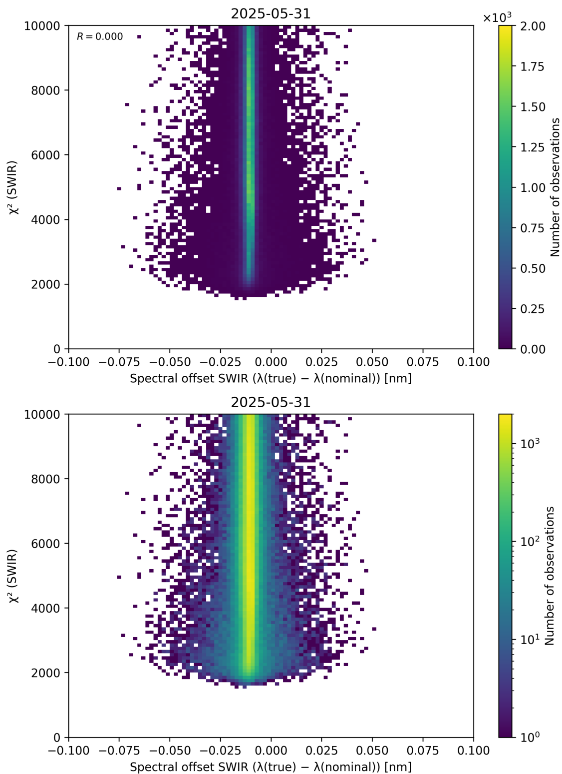
Figure 118: Scatter density plot of “Spectral offset SWIR ( \lambda_{\text{true}} - \lambda_{\text{nominal}} )” against “ \chi^2 (SWIR)” for 2025-05-31 to 2025-06-01.
