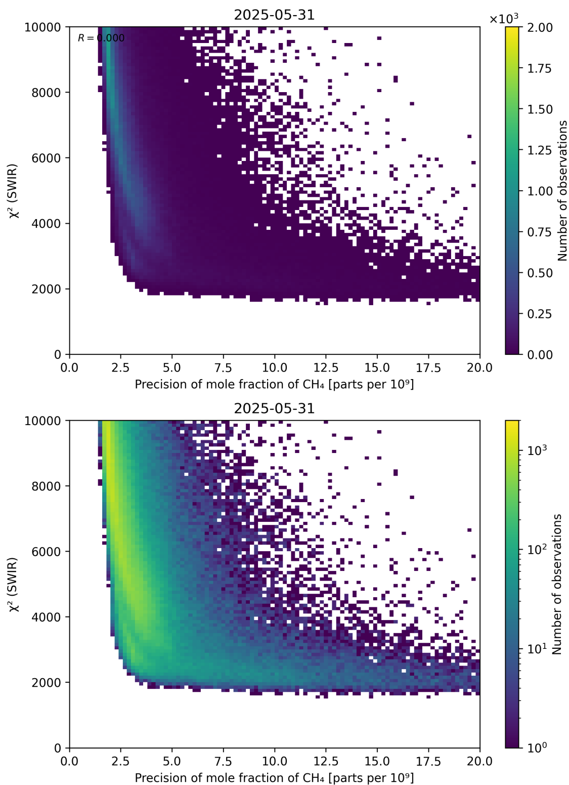
Figure 79: Scatter density plot of “Precision of mole fraction of \text{CH}_4 ” against “ \chi^2 (SWIR)” for 2025-05-31 to 2025-06-01.
