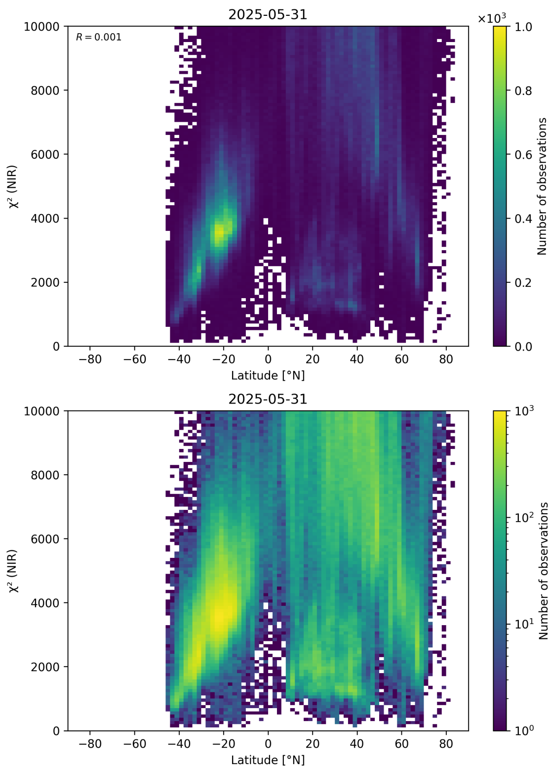
Figure 53: Scatter density plot of “Latitude” against “ \chi^2 (NIR)” for 2025-05-31 to 2025-06-01.
