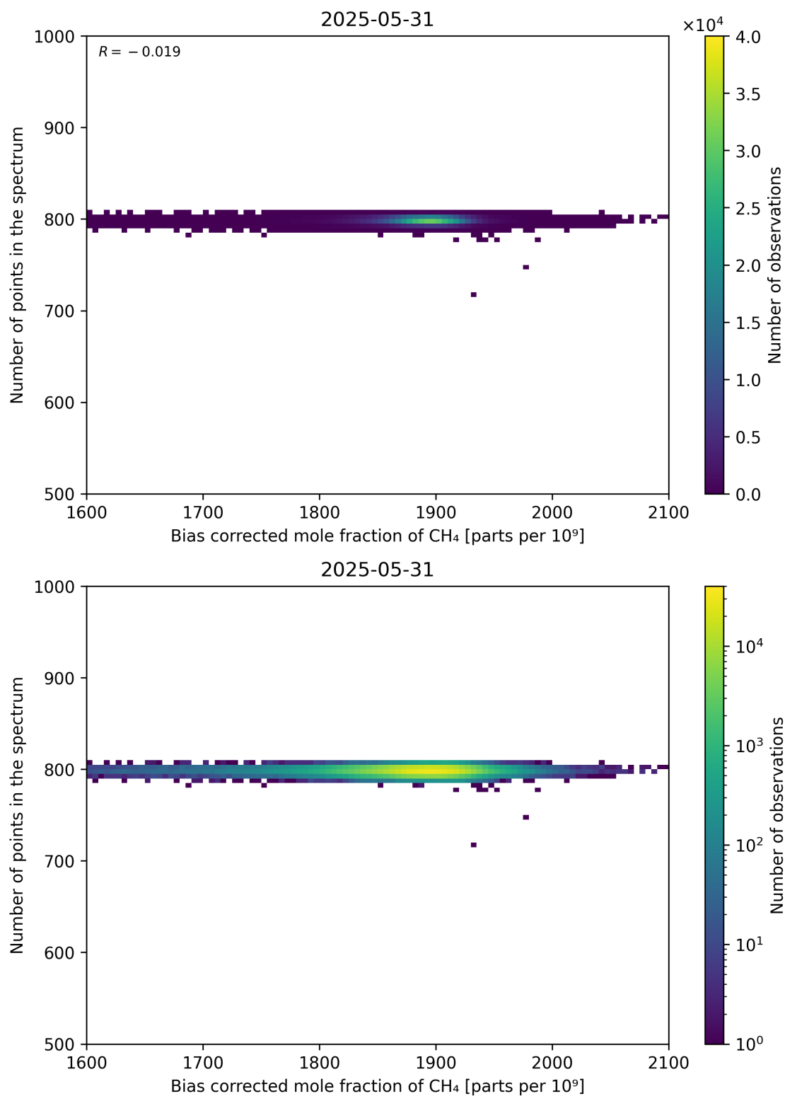
Figure 68: Scatter density plot of “Bias corrected mole fraction of CH 4 ” against “Number of points in the spectrum” for 2025-05-31 to 2025-06-01.
