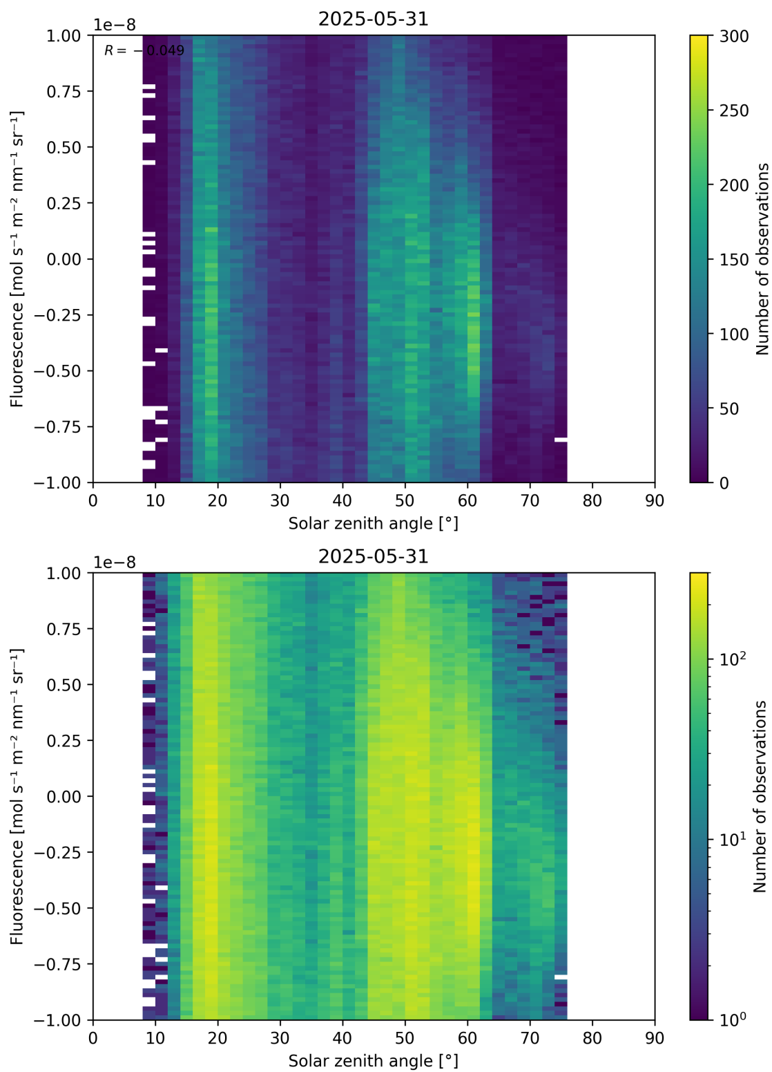
Figure 97: Scatter density plot of “Solar zenith angle” against “Fluorescence” for 2025-05-31 to 2025-06-01.
