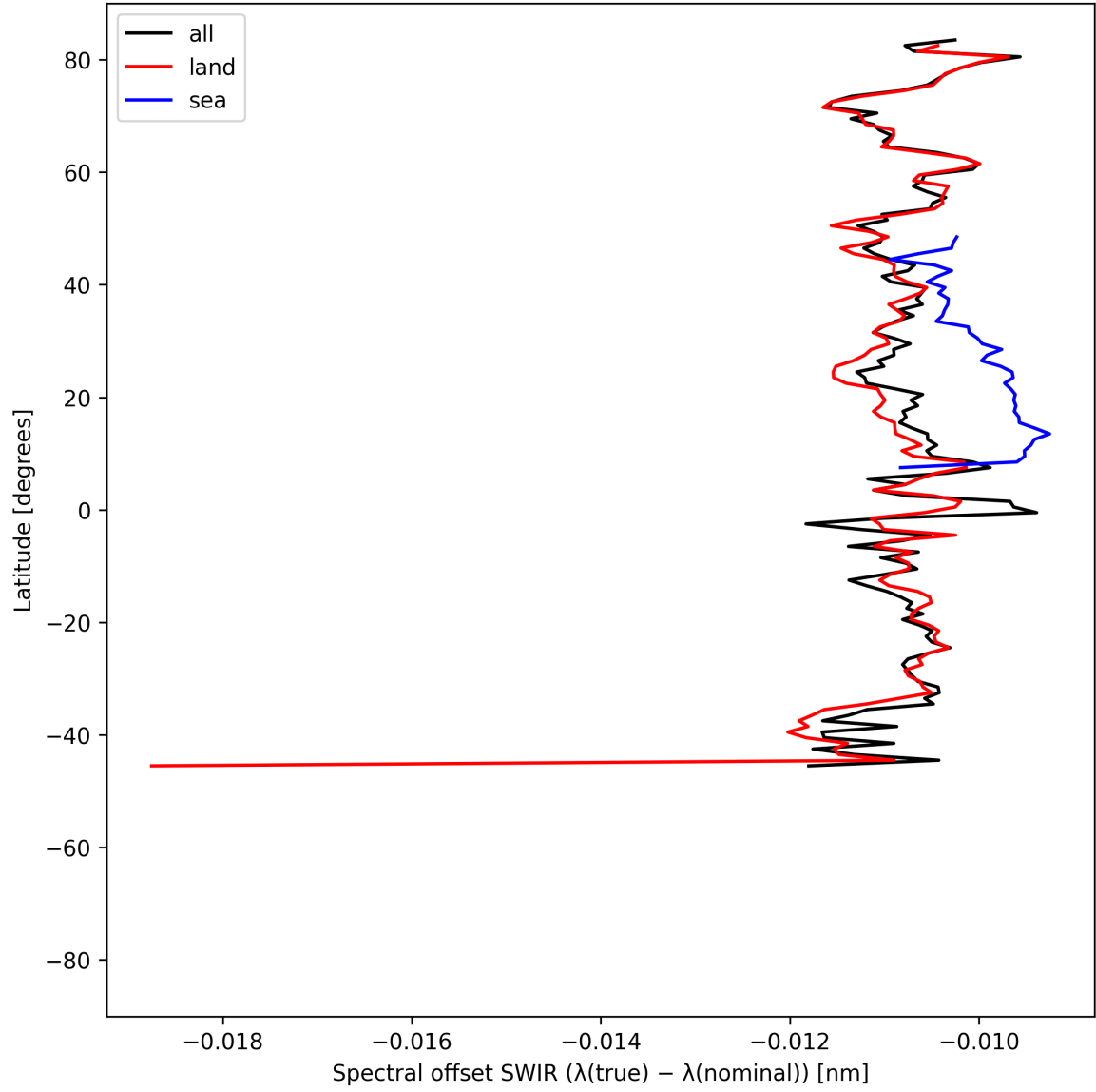
Figure 16: Zonal average of “Spectral offset SWIR ( \lambda_{\text{true}} - \lambda_{\text{nominal}} )” for 2025-05-31 to 2025-06-01.
