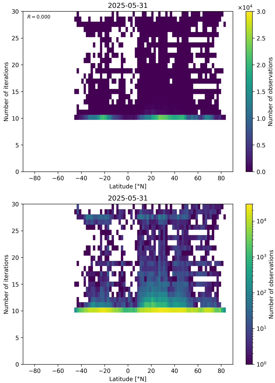
Figure 60: Scatter density plot of “Latitude” against “Number of iterations” for 2025-05-31 to 2025-06-01.
