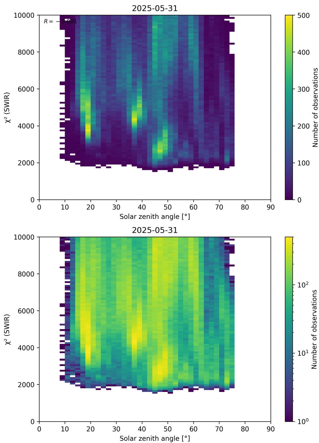
Figure 95: Scatter density plot of “Solar zenith angle” against “ \chi^2 (SWIR)” for 2025-05-31 to 2025-06-01.
