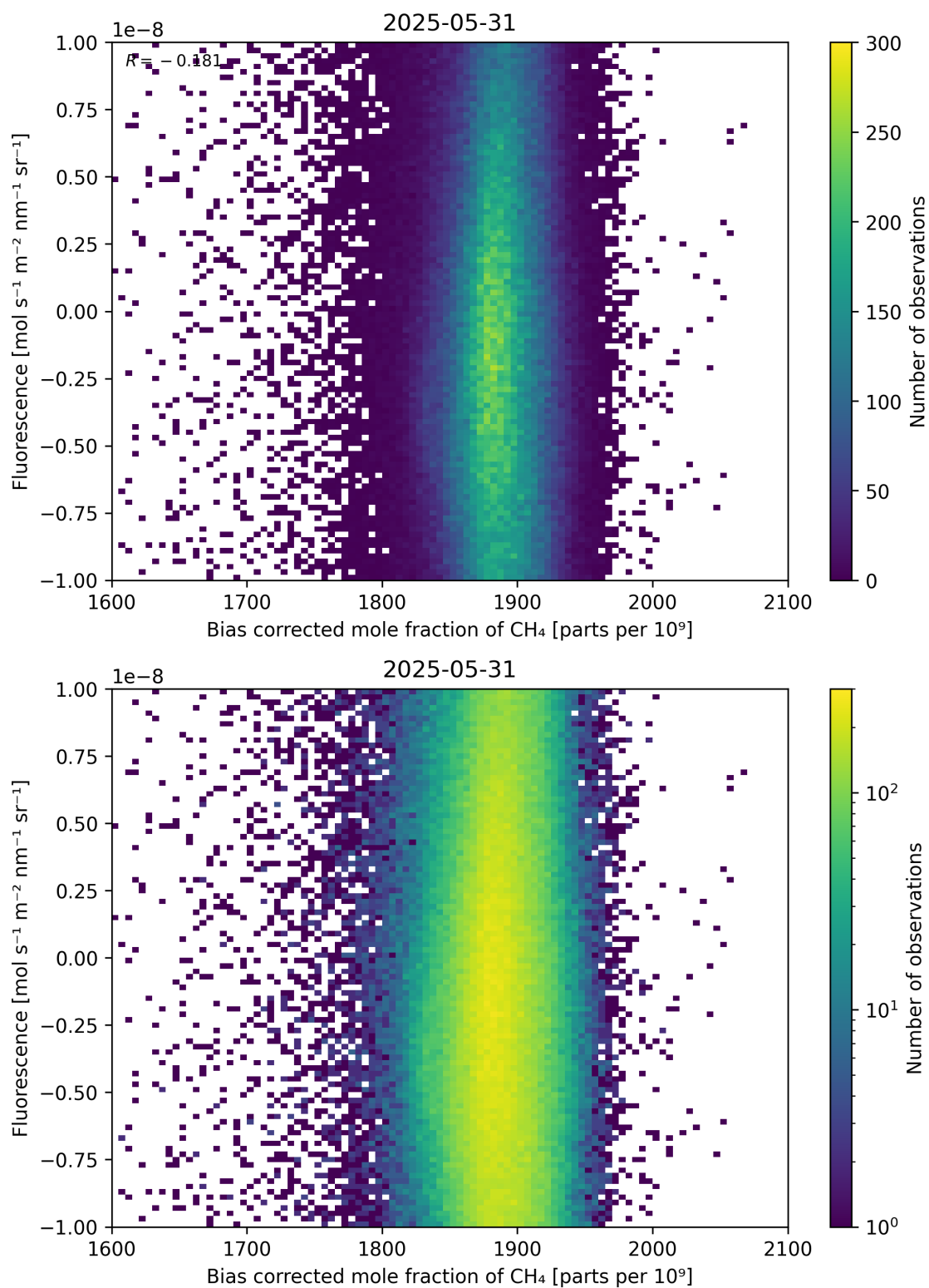
Figure 66: Scatter density plot of “Bias corrected mole fraction of CH 4 ” against “Fluorescence” for 2025-05-31 to 2025-06-01.
