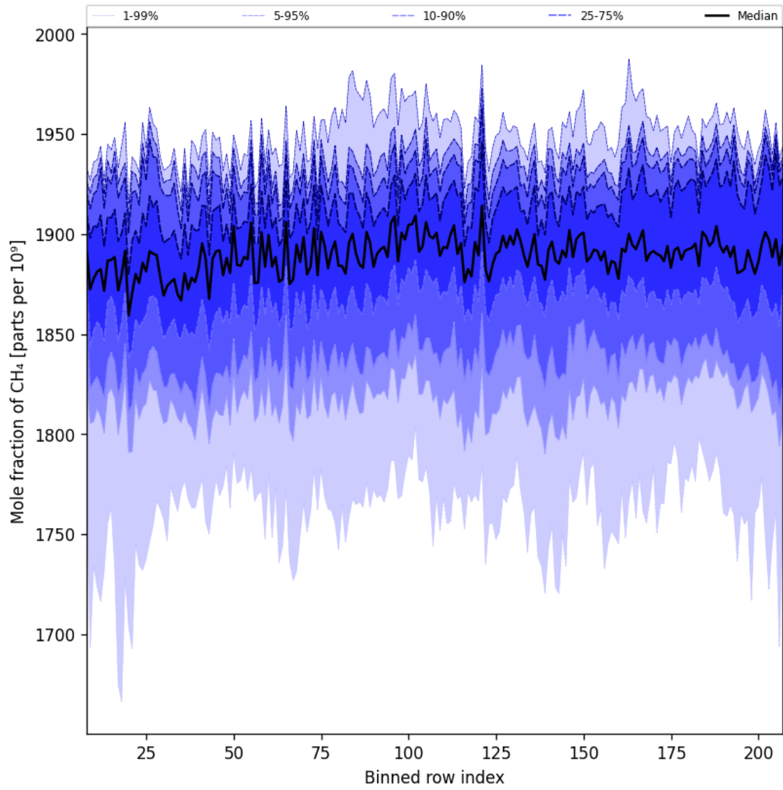
Figure 34: Along track statistics of “Mole fraction of CH 4 ” for 2025-05-31 to 2025-06-01
