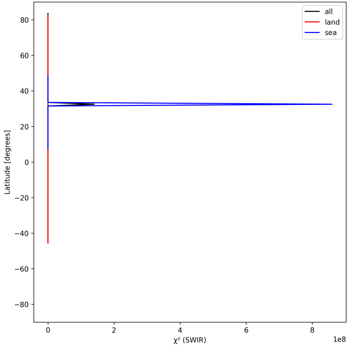
Figure 17: Zonal average of “ \chi^2 (SWIR)” for 2025-05-31 to 2025-06-01.
