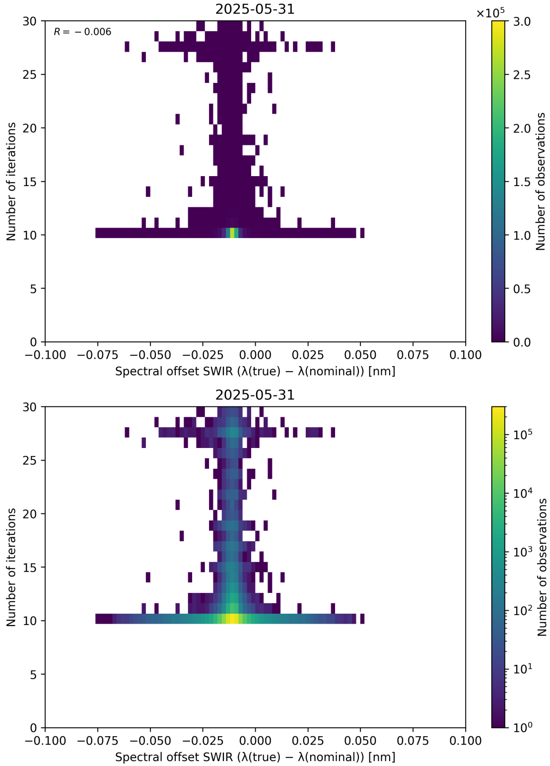
Figure 121: Scatter density plot of “Spectral offset SWIR ( \lambda_{\text{true}} - \lambda_{\text{nominal}} )” against “Number of iterations” for 2025-05-31 to 2025-06-01.
