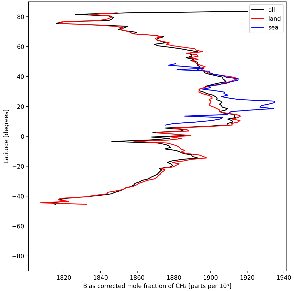
Figure 14: Zonal average of “Bias corrected mole fraction of CH 4 ” for 2025-05-31 to 2025-06-01.
