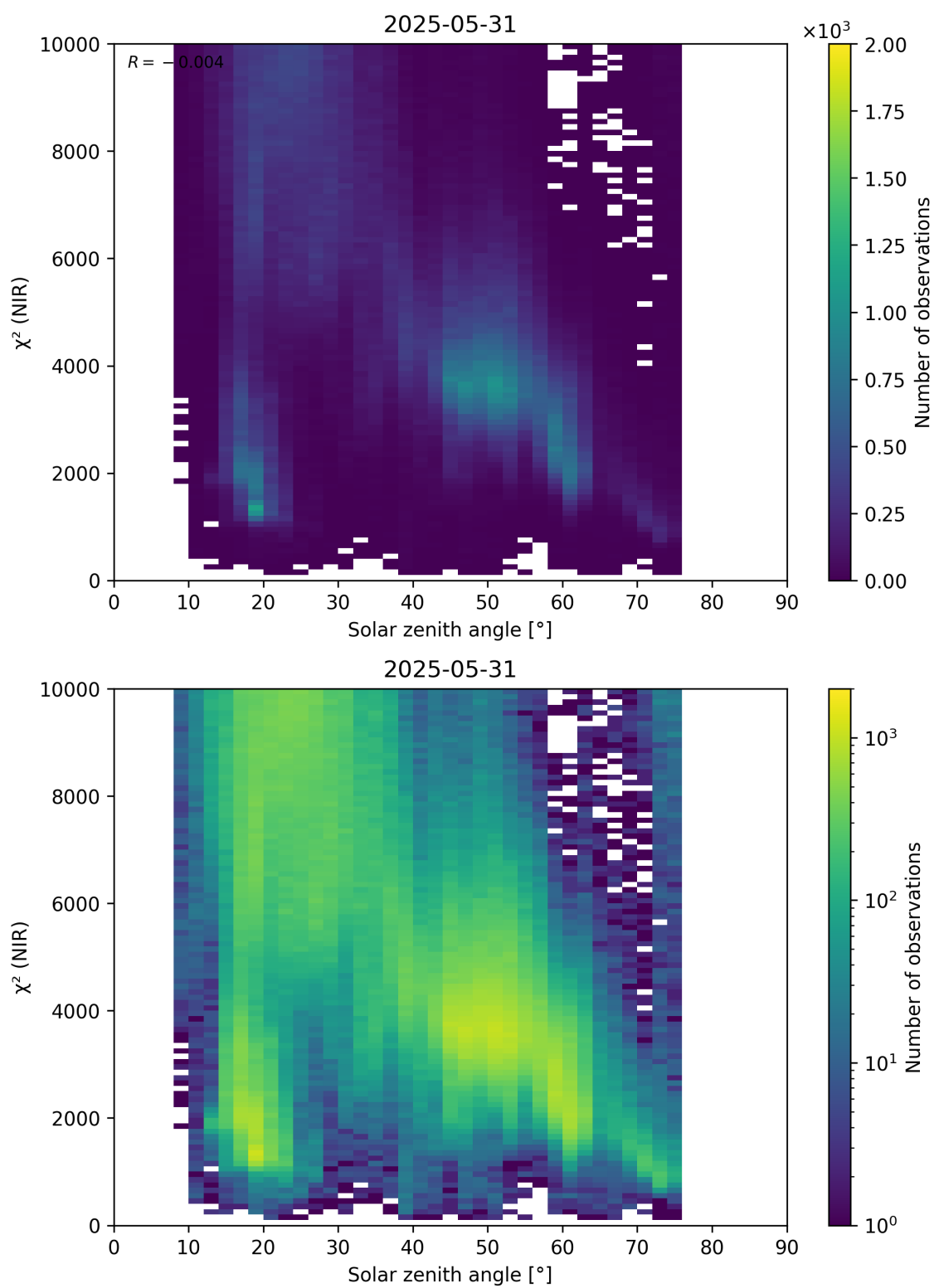
Figure 94: Scatter density plot of “Solar zenith angle” against “ \chi^2 (NIR)” for 2025-05-31 to 2025-06-01.
