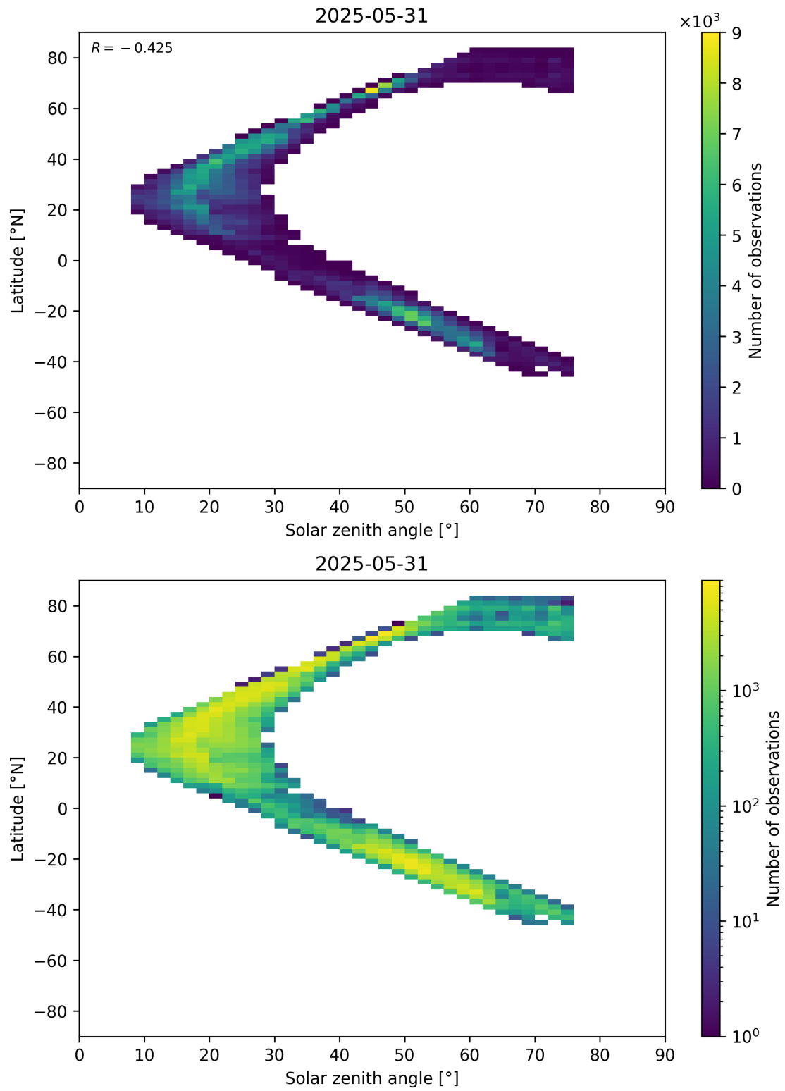
Figure 98: Scatter density plot of “Solar zenith angle” against “Latitude” for 2025-05-31 to 2025-06-01.
