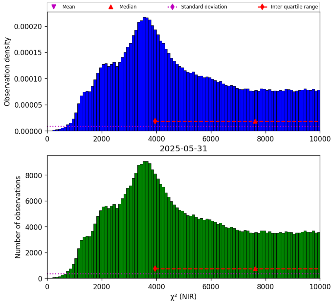
Figure 29: Histogram of " \chi^2 (NIR)" for 2025-05-31 to 2025-06-01
