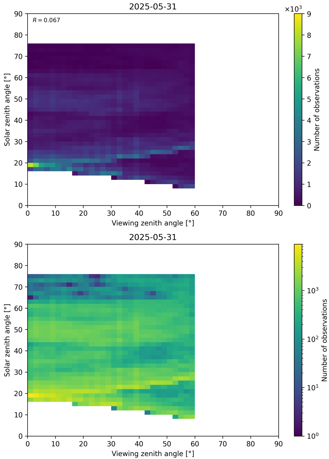
Figure 115: Scatter density plot of “Viewing zenith angle” against “Solar zenith angle” for 2025-05-31 to 2025-06-01.
