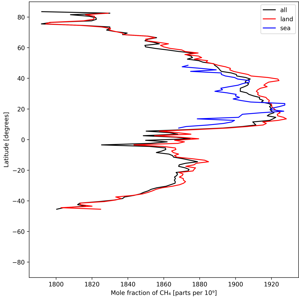
Figure 12: Zonal average of “Mole fraction of CH 4 ” for 2025-05-31 to 2025-06-01.
