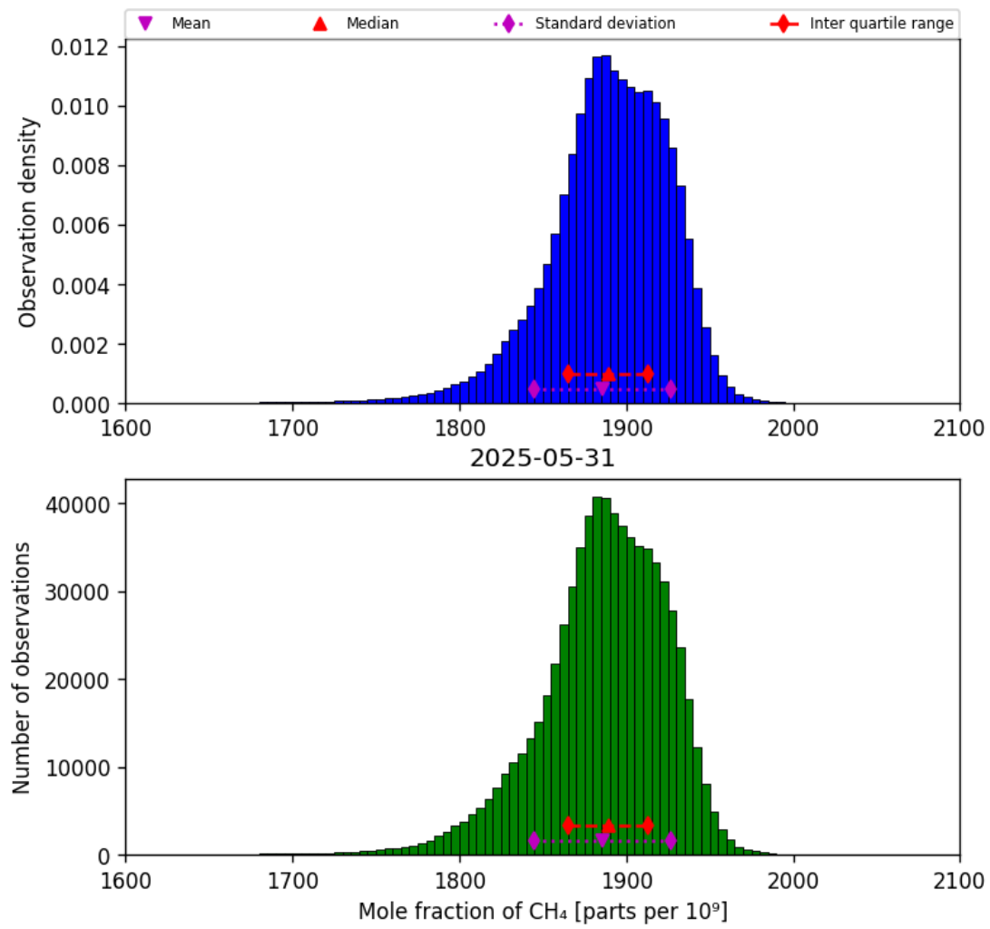
Figure 23: Histogram of “Mole fraction of CH 4 ” for 2025-05-31 to 2025-06-01
