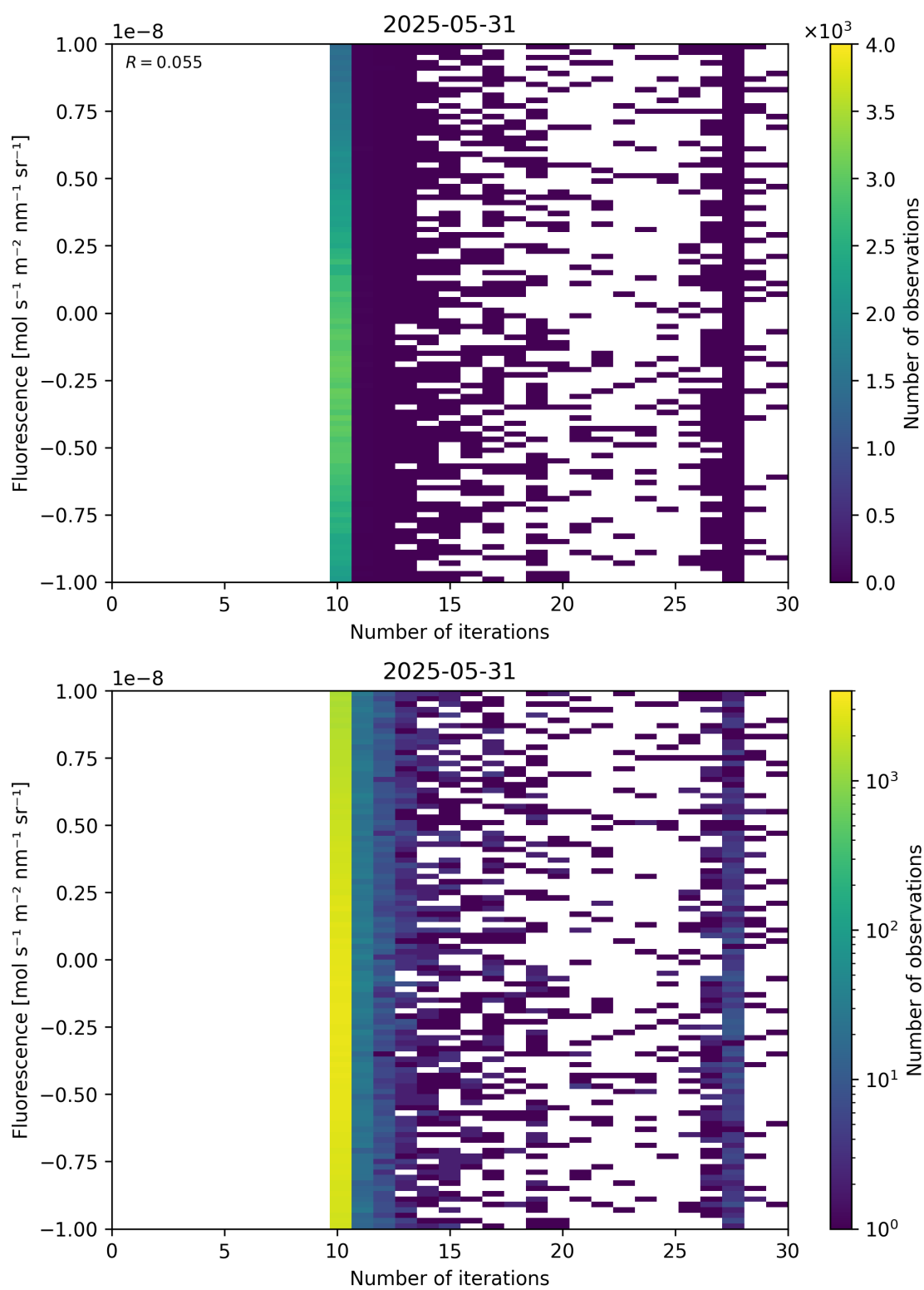
Figure 87: Scatter density plot of “Number of iterations” against “Fluorescence” for 2025-05-31 to 2025-06-01.
