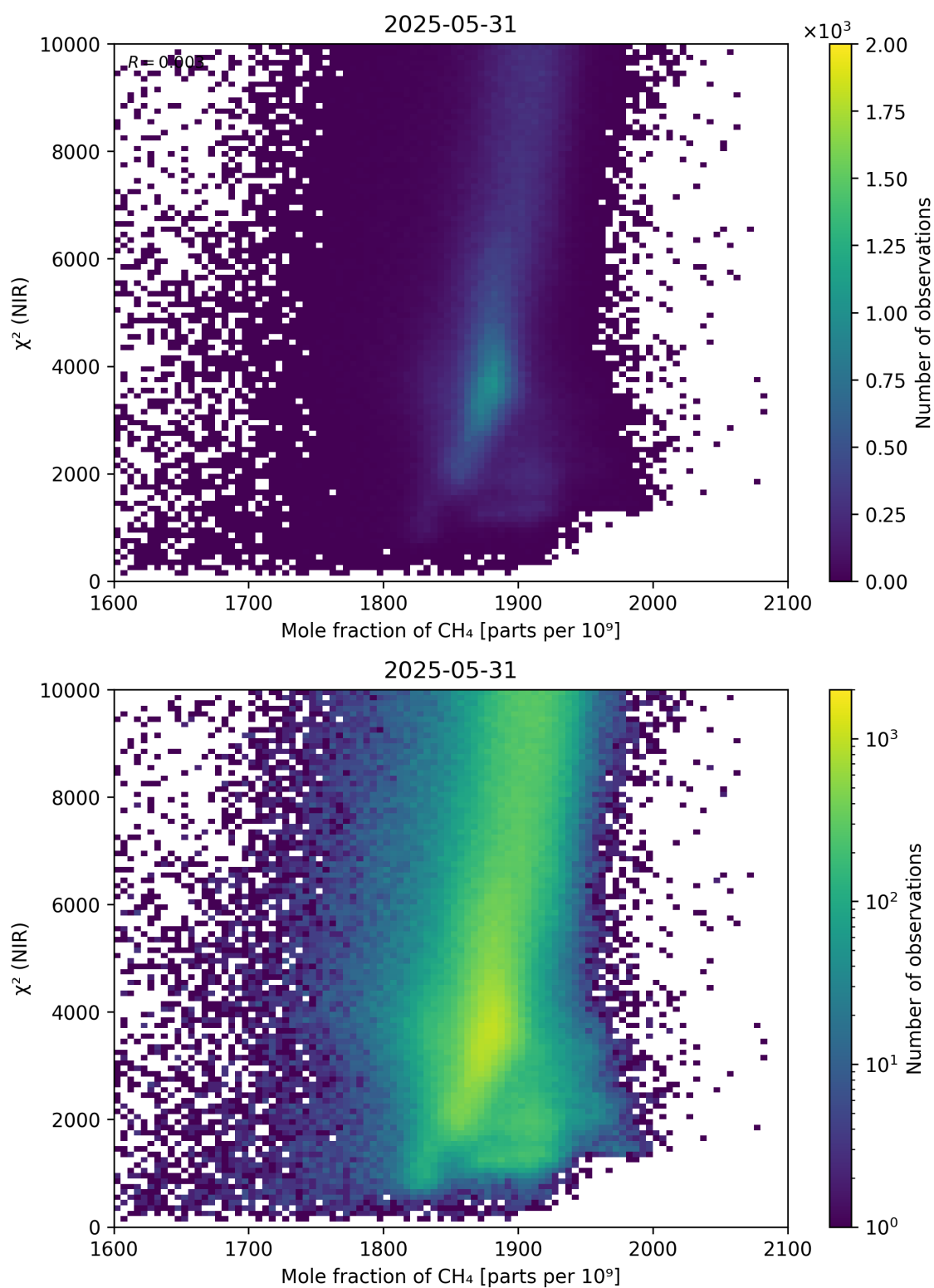
Figure 70: Scatter density plot of “Mole fraction of \text{CH}_4 ” against “ \chi^2 (NIR)” for 2025-05-31 to 2025-06-01.
