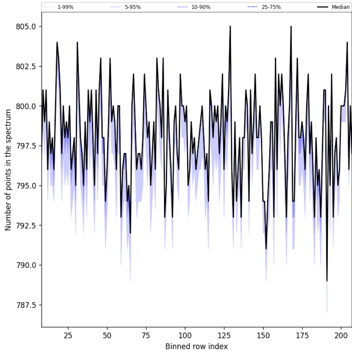
Figure 37: Along track statistics of “Number of points in the spectrum” for 2025-05-31 to 2025-06-01
