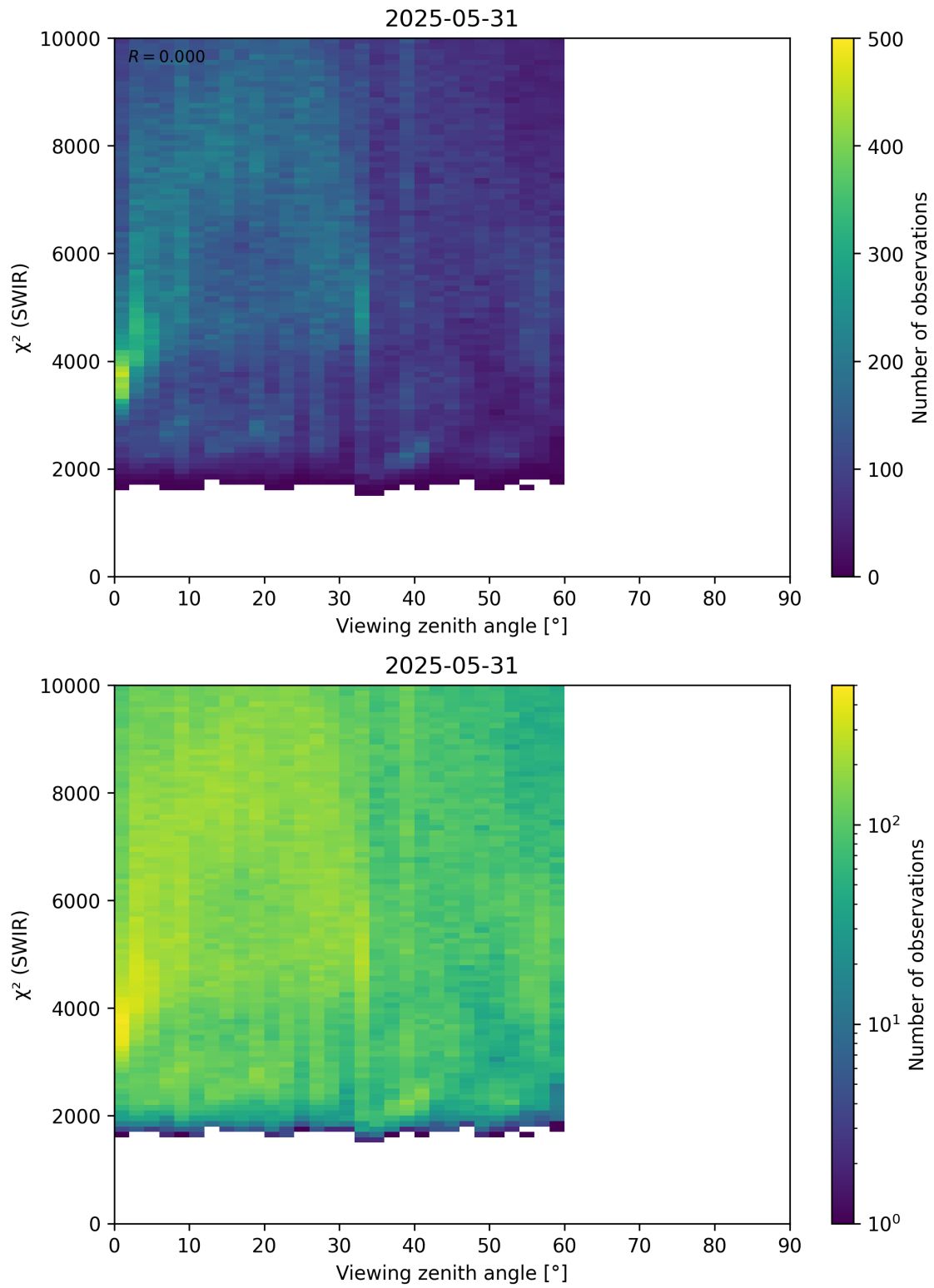
Figure 106: Scatter density plot of “Viewing zenith angle” against “ \chi^2 (SWIR)” for 2025-05-31 to 2025-06-01.
