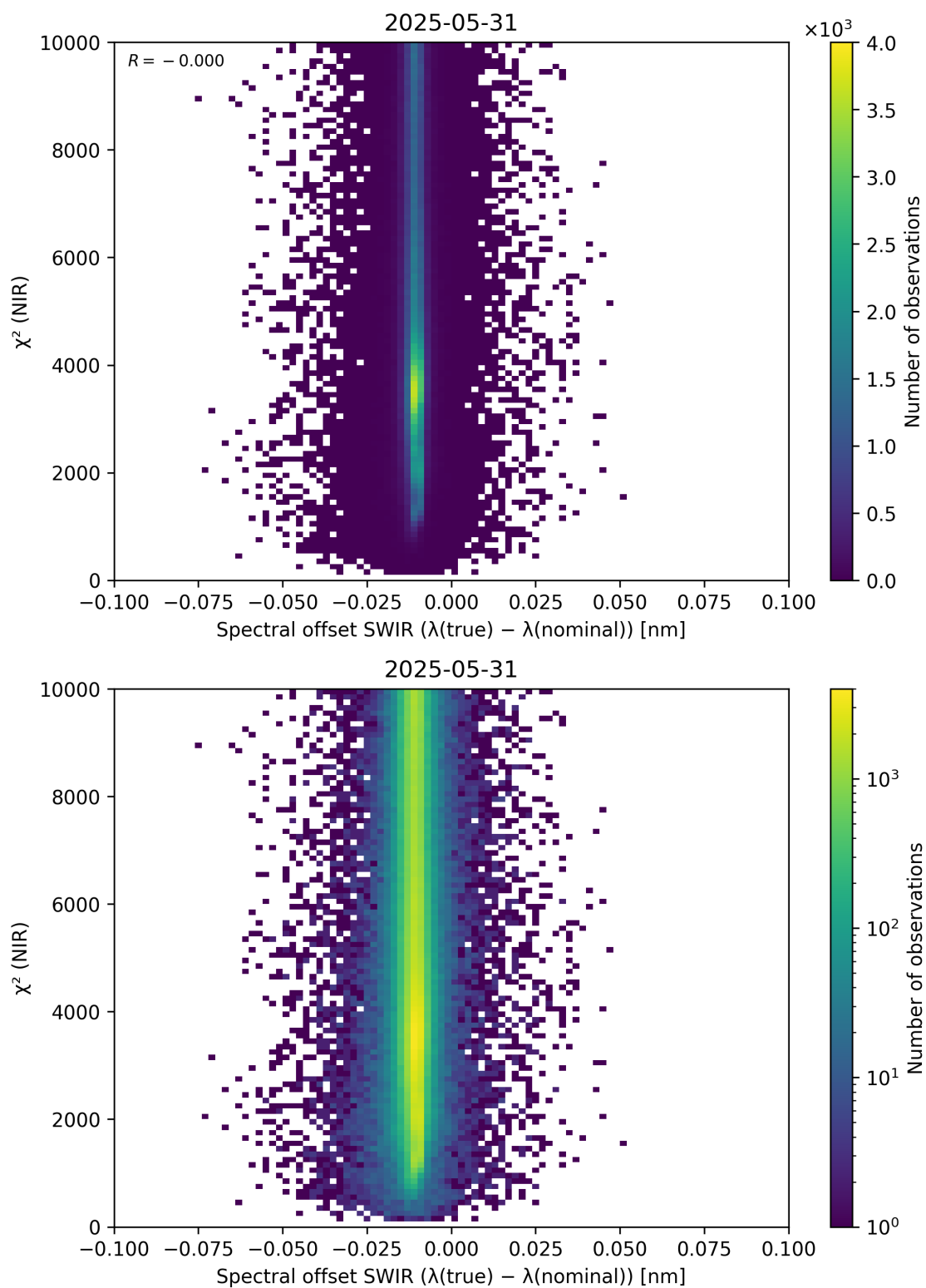
Figure 117: Scatter density plot of “Spectral offset SWIR ( \lambda_{\text{true}} - \lambda_{\text{nominal}} )” against “ \chi^2 (NIR)” for 2025-05-31 to 2025-06-01.
