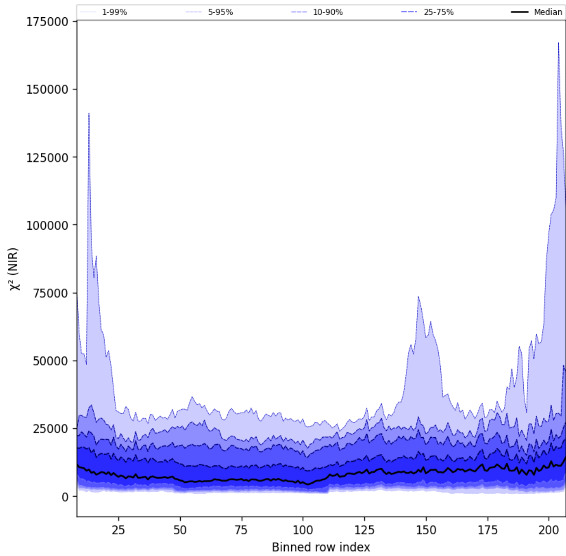
Figure 40: Along track statistics of “ \chi^2 (NIR)” for 2025-05-31 to 2025-06-01
