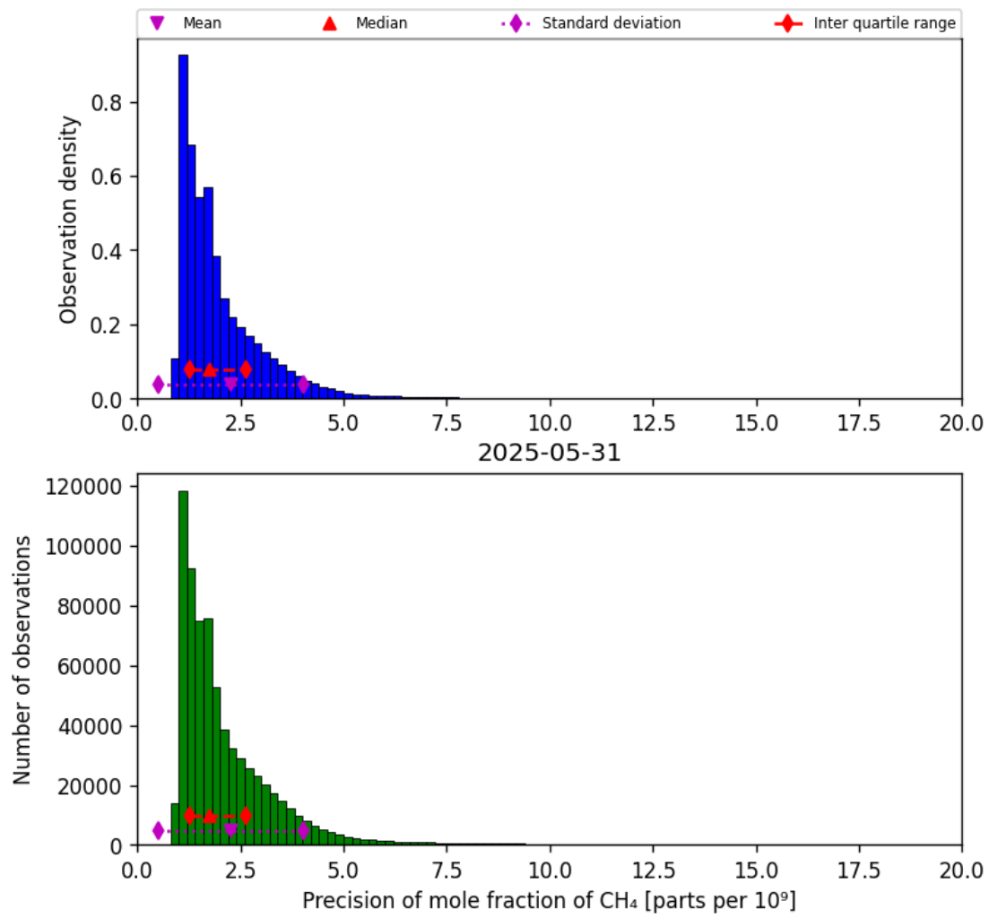
Figure 24: Histogram of “Precision of mole fraction of CH 4 ” for 2025-05-31 to 2025-06-01
