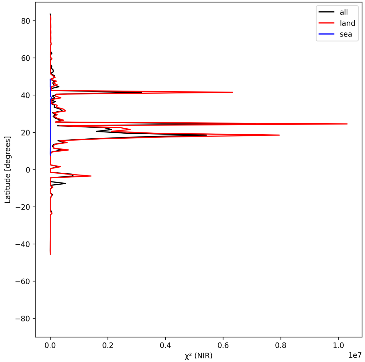
Figure 18: Zonal average of “ \chi^2 (NIR)” for 2025-05-31 to 2025-06-01.
