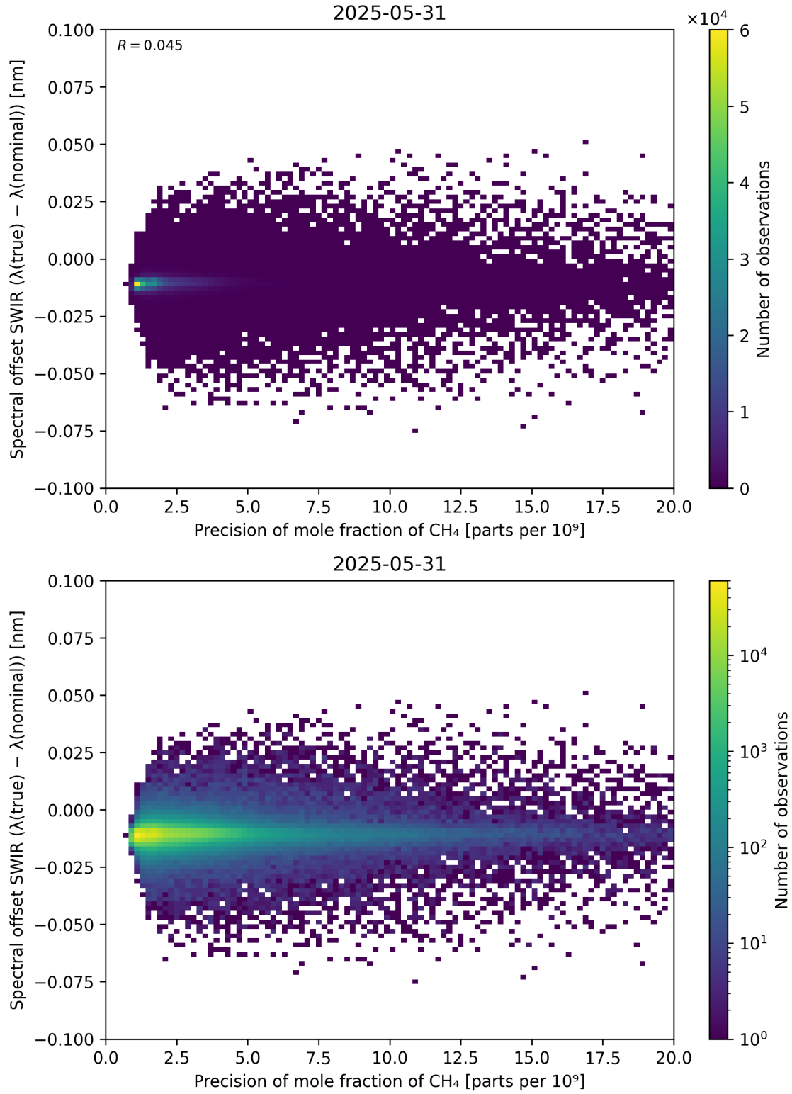
Figure 85: Scatter density plot of “Precision of mole fraction of \text{CH}_4 ” against “Spectral offset SWIR ( \lambda_{\text{true}} - \lambda_{\text{nominal}} )” for 2025-05-31 to 2025-06-01.
