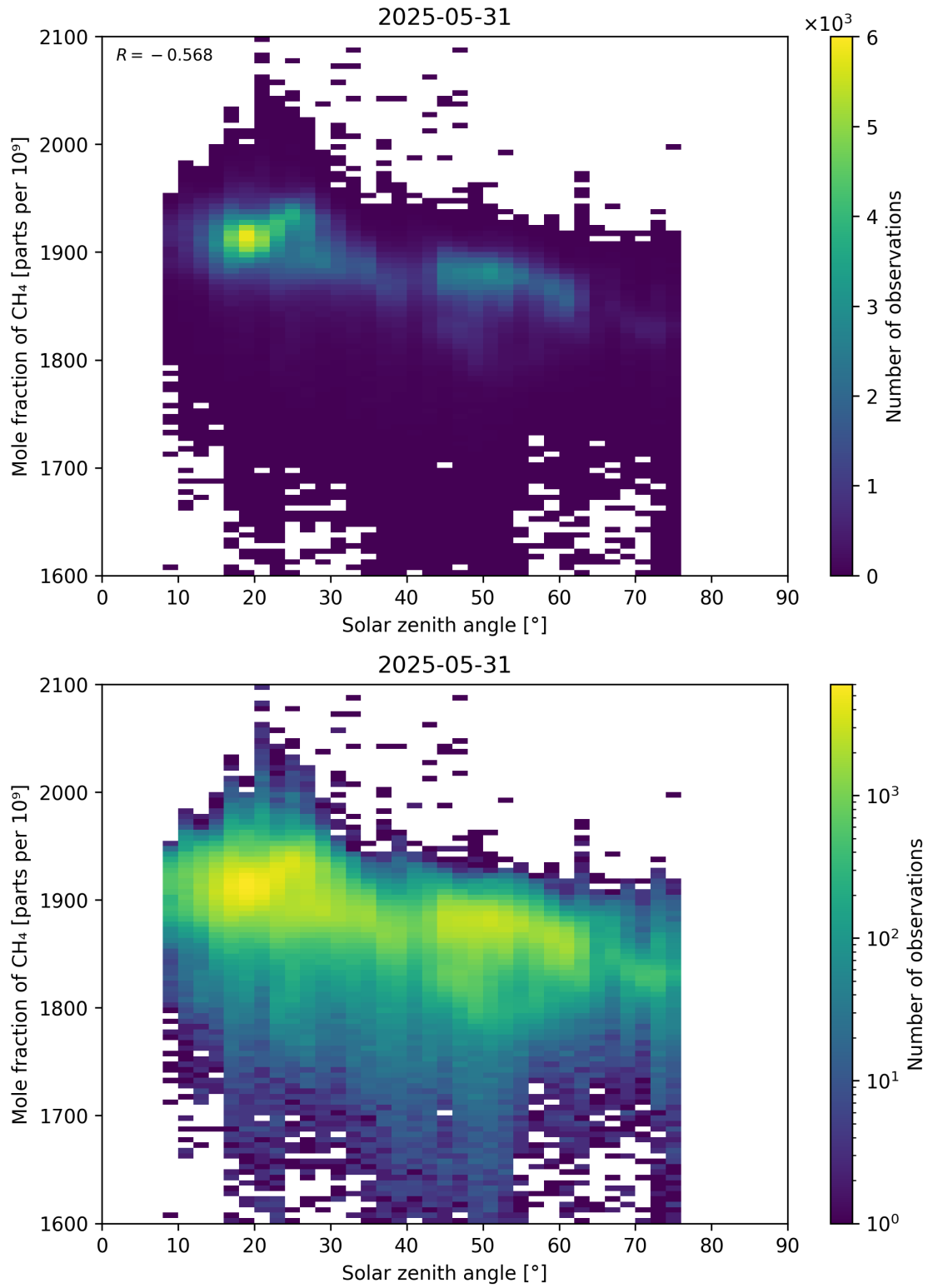
Figure 99: Scatter density plot of “Solar zenith angle” against “Mole fraction of CH 4 ” for 2025-05-31 to 2025-06-01.
