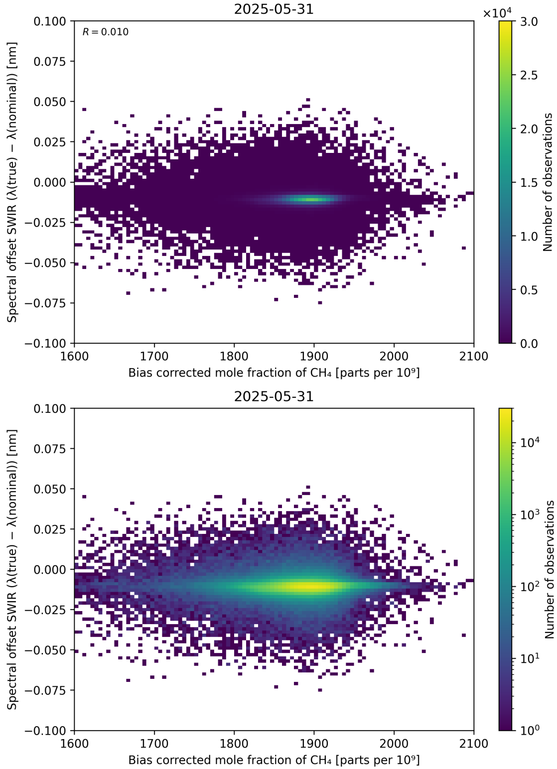
Figure 69: Scatter density plot of “Bias corrected mole fraction of \text{CH}_4 ” against “Spectral offset SWIR ( \lambda_{\text{true}} - \lambda_{\text{nominal}} )” for 2025-05-31 to 2025-06-01.
