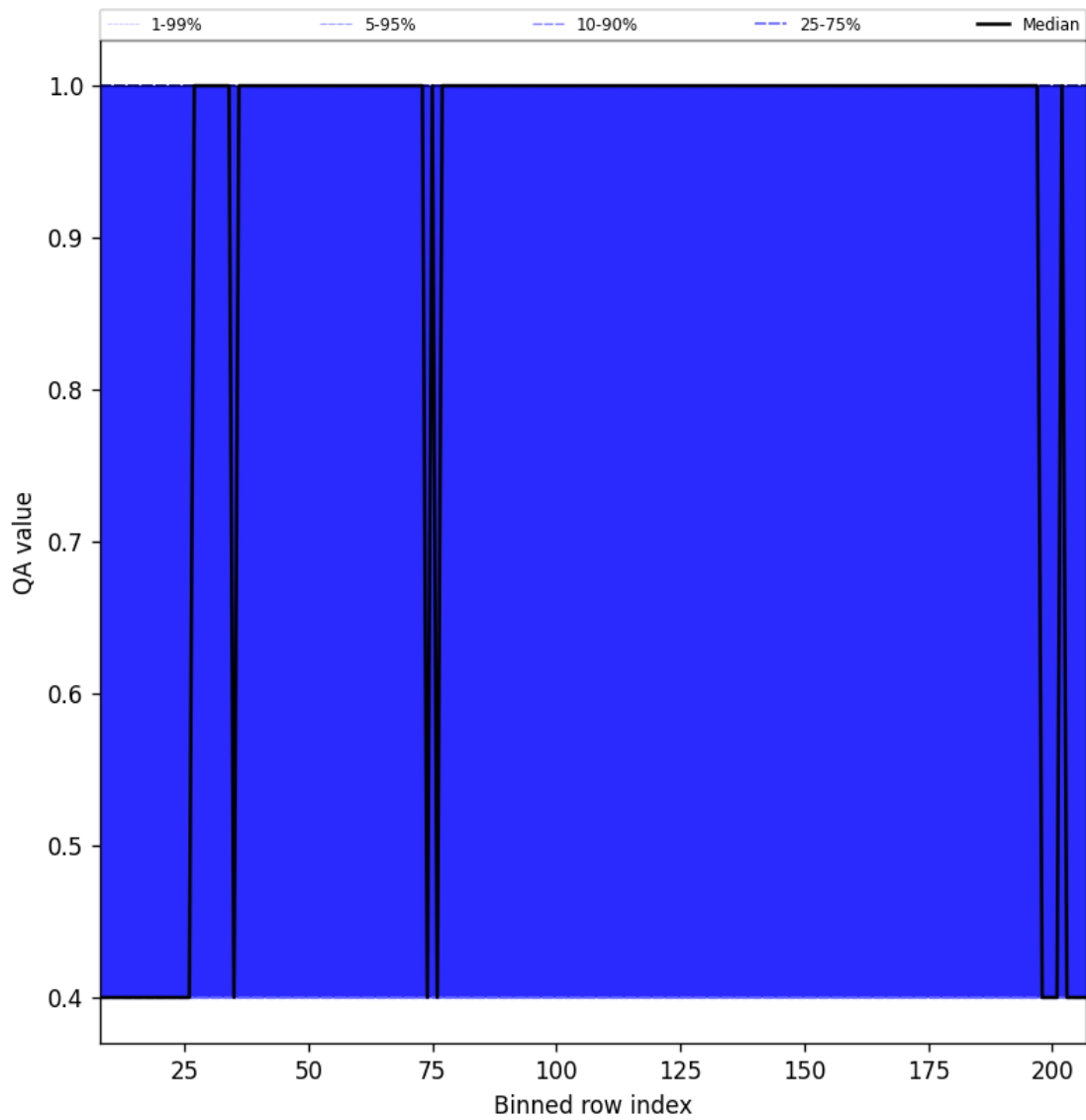
Figure 33: Along track statistics of “QA value” for 2025-05-31 to 2025-06-01
