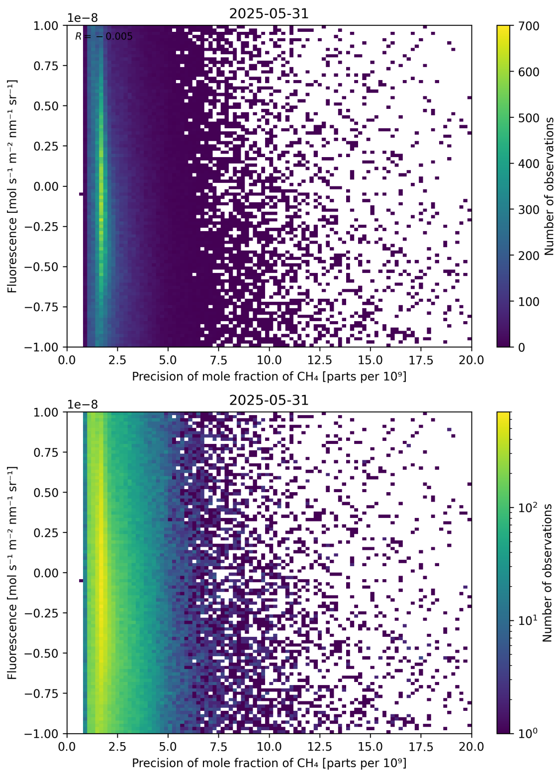
Figure 81: Scatter density plot of “Precision of mole fraction of CH 4 ” against “Fluorescence” for 2025-05-31 to 2025-06-01.
