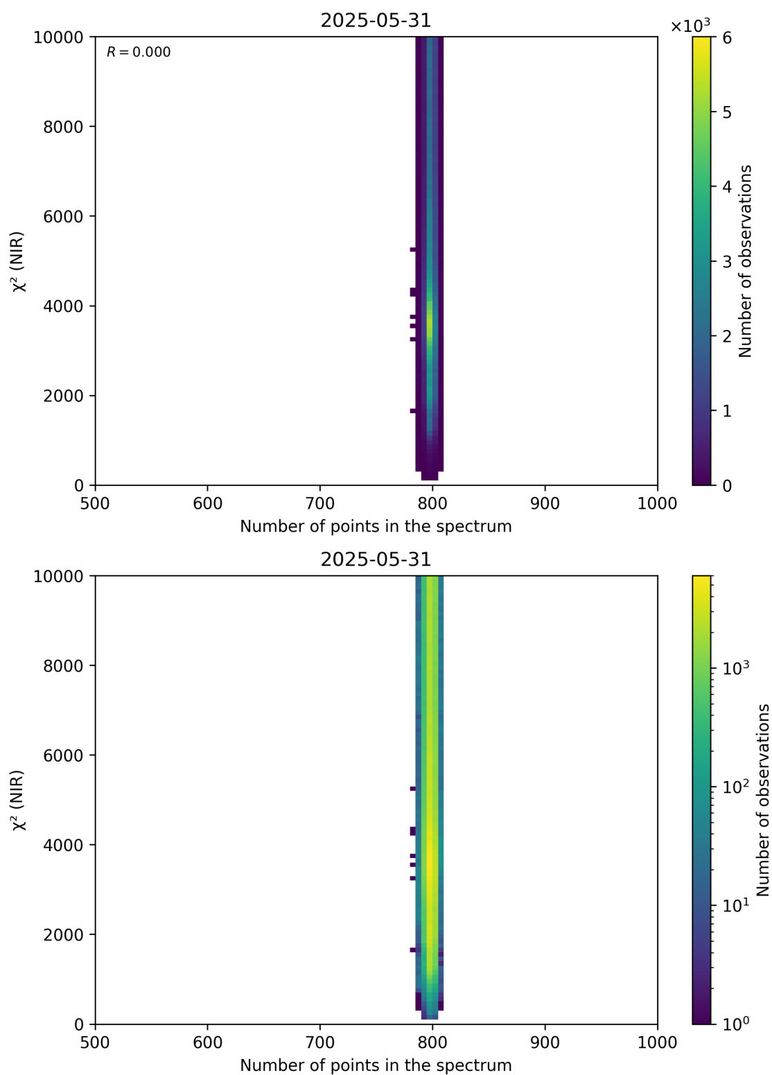
Figure 88: Scatter density plot of “Number of points in the spectrum” against “ \chi^2 (NIR)” for 2025-05-31 to 2025-06-01.
