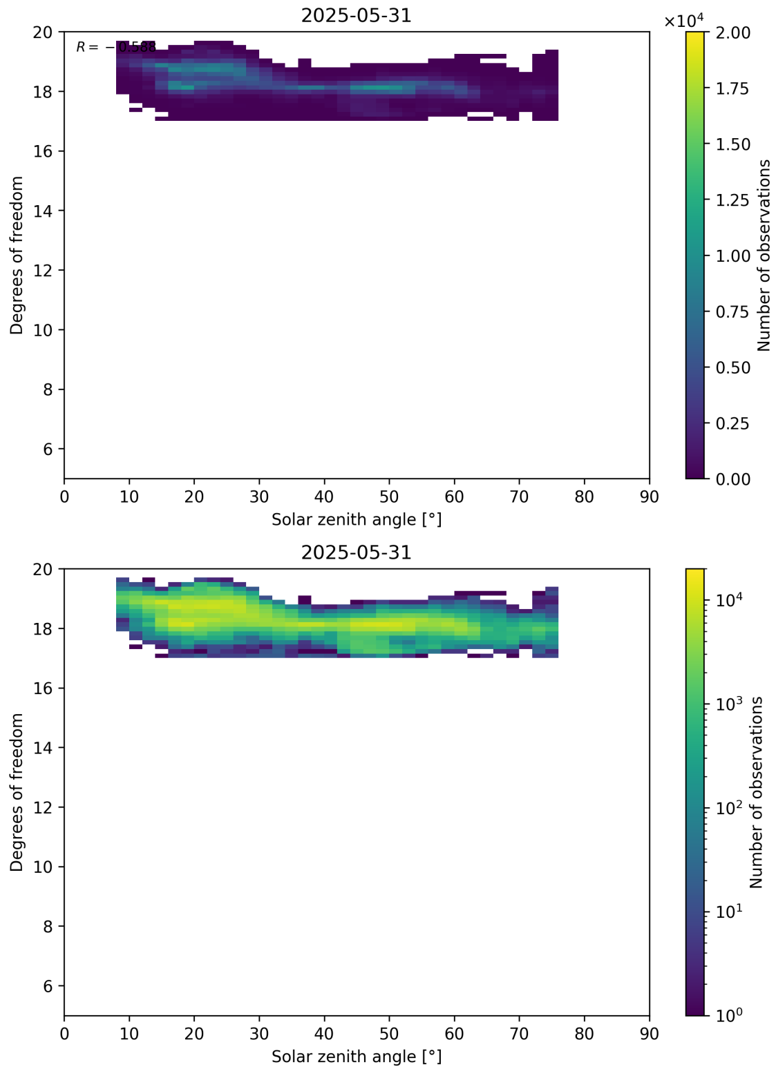
Figure 96: Scatter density plot of “Solar zenith angle” against “Degrees of freedom” for 2025-05-31 to 2025-06-01.
