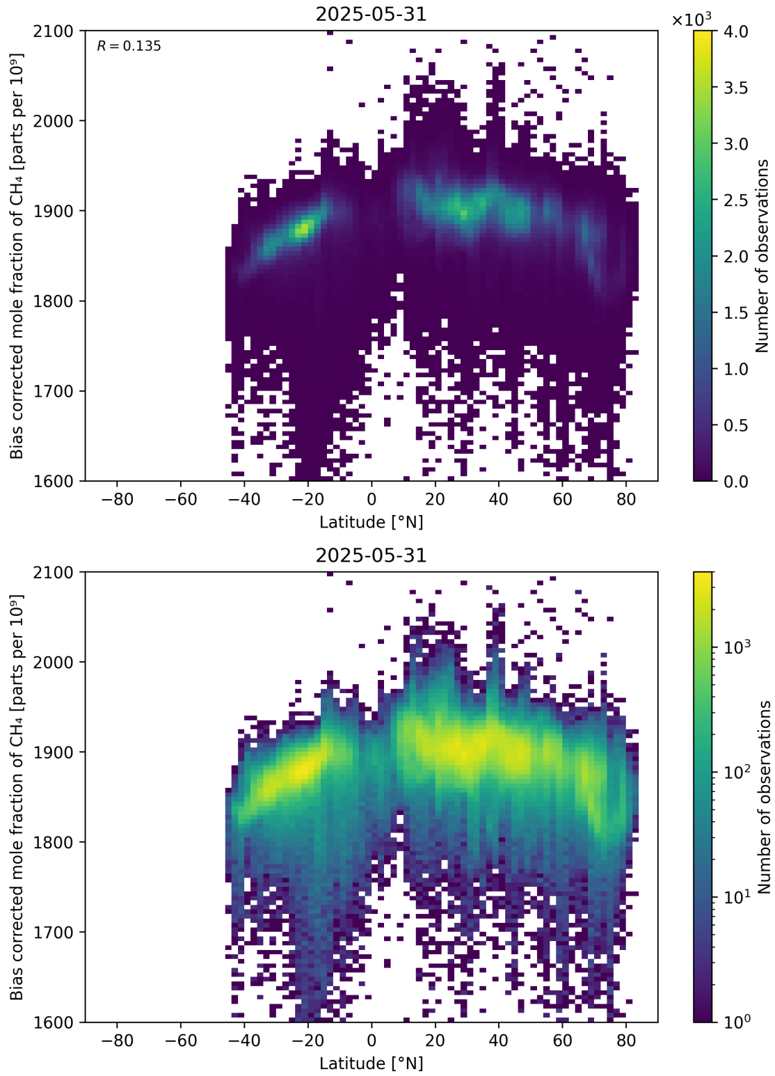
Figure 58: Scatter density plot of “Latitude” against “Bias corrected mole fraction of CH 4 ” for 2025-05-31 to 2025-06-01.
