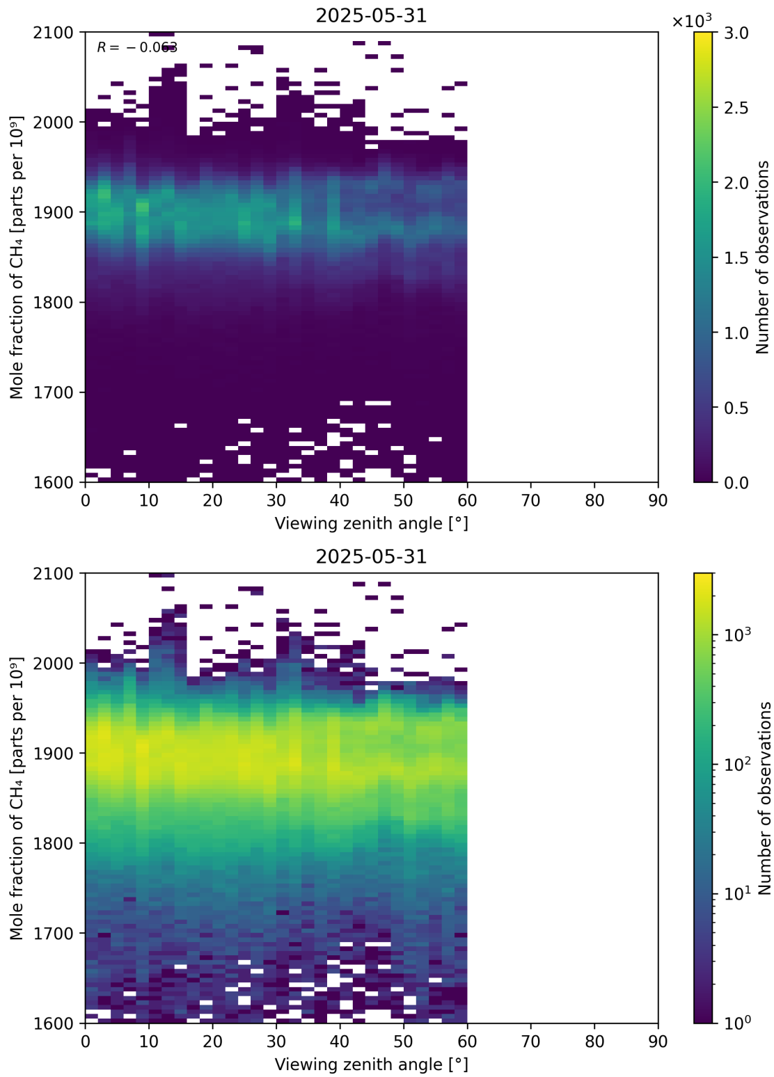
Figure 110: Scatter density plot of “Viewing zenith angle” against “Mole fraction of CH 4 ” for 2025-05-31 to 2025-06-01.
