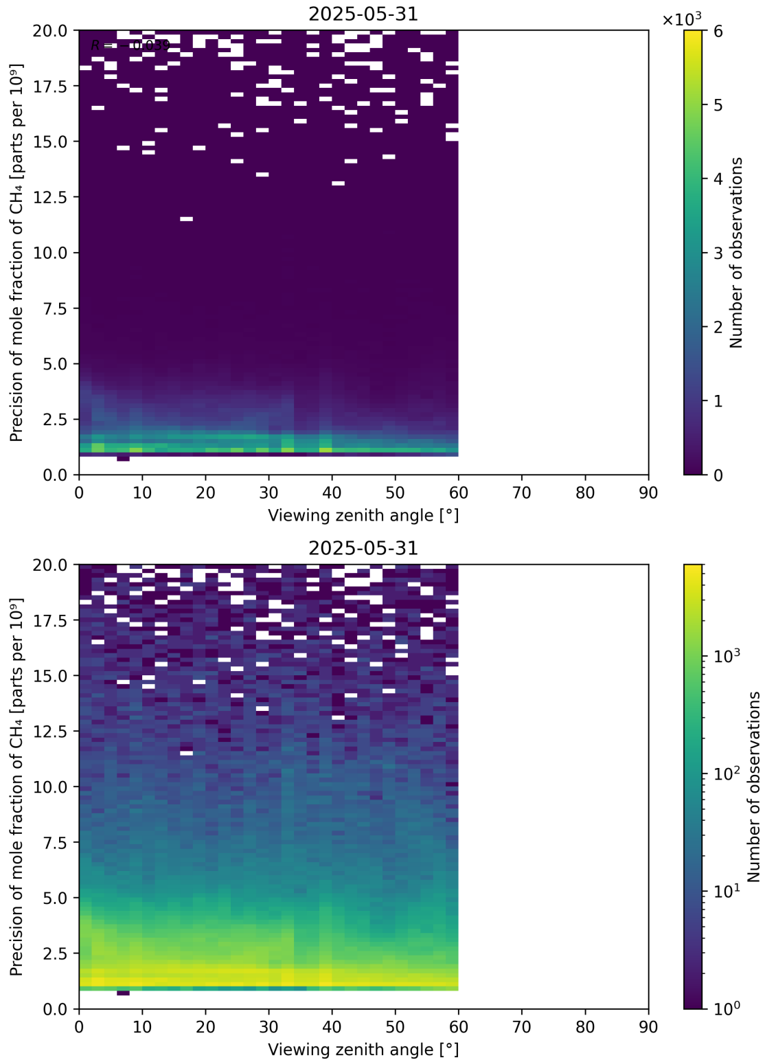
Figure 112: Scatter density plot of “Viewing zenith angle” against “Precision of mole fraction of CH 4 ” for 2025-05-31 to 2025-06-01.
