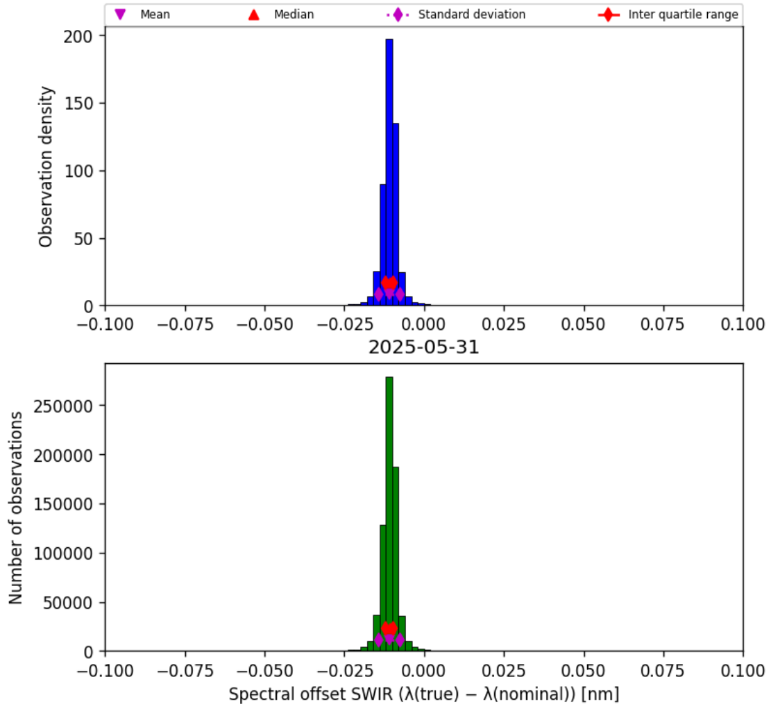
Figure 27: Histogram of “Spectral offset SWIR ( \lambda_{\text{true}} - \lambda_{\text{nominal}} )” for 2025-05-31 to 2025-06-01
