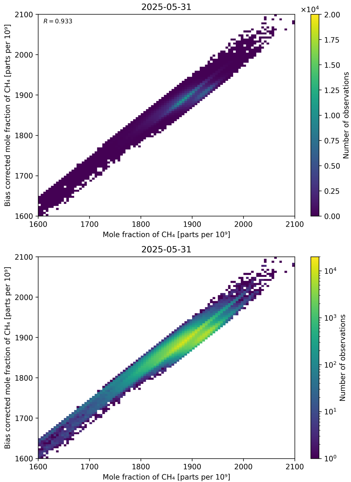
Figure 74: Scatter density plot of “Mole fraction of CH 4 ” against “Bias corrected mole fraction of CH 4 ” for 2025-05-31 to 2025-06-01.
