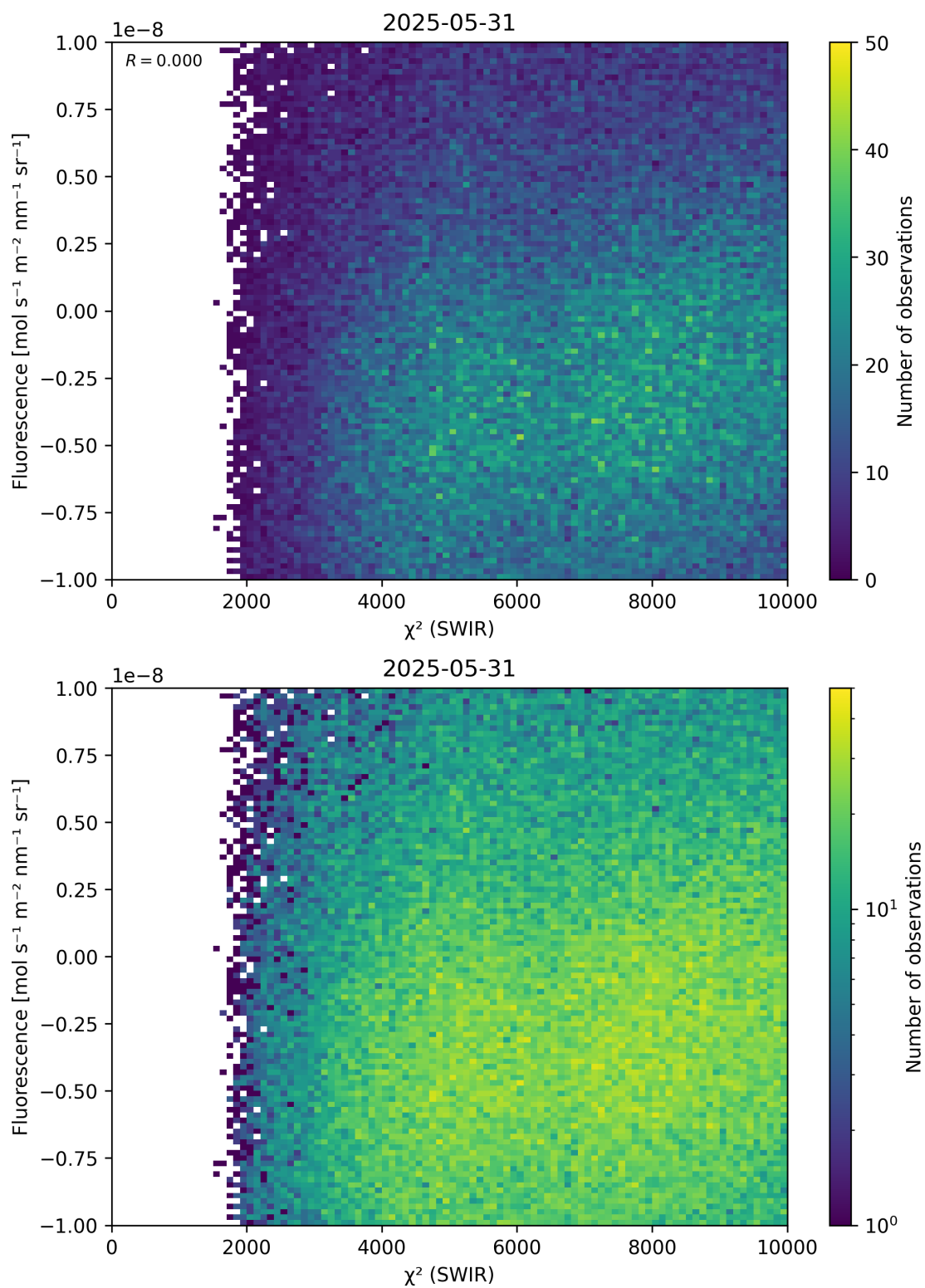
Figure 49: Scatter density plot of “ \chi^2 (SWIR)” against “Fluorescence” for 2025-05-31 to 2025-06-01.
