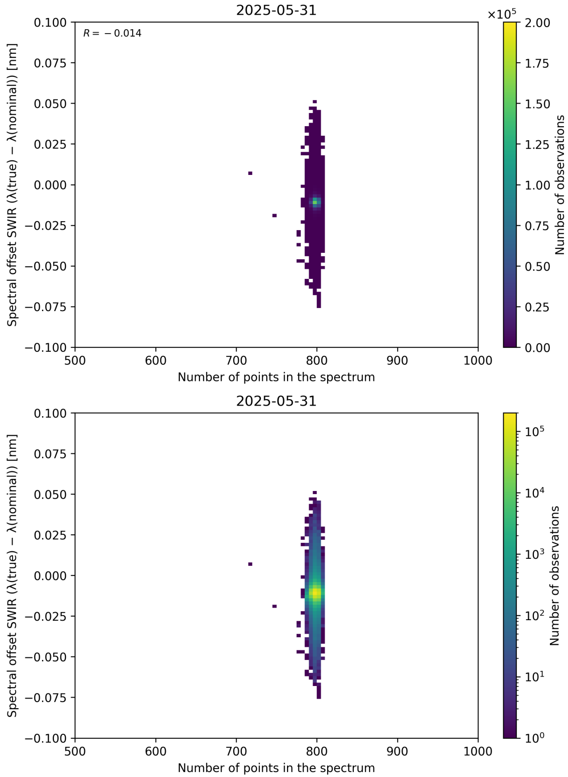
Figure 93: Scatter density plot of “Number of points in the spectrum” against “Spectral offset SWIR ( \lambda_{\text{true}} - \lambda_{\text{nominal}} )” for 2025-05-31 to 2025-06-01.
