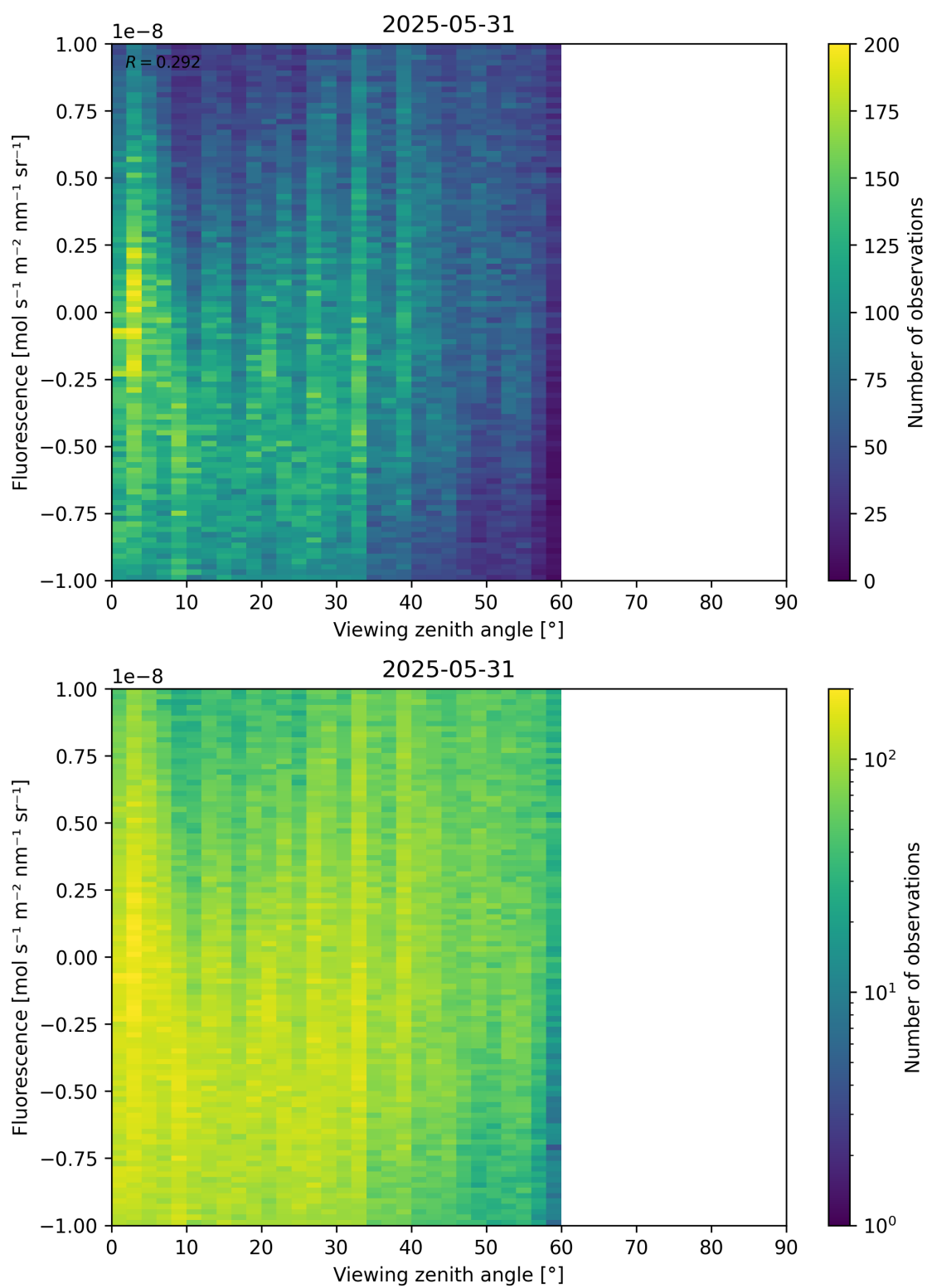
Figure 108: Scatter density plot of “Viewing zenith angle” against “Fluorescence” for 2025-05-31 to 2025-06-01.
