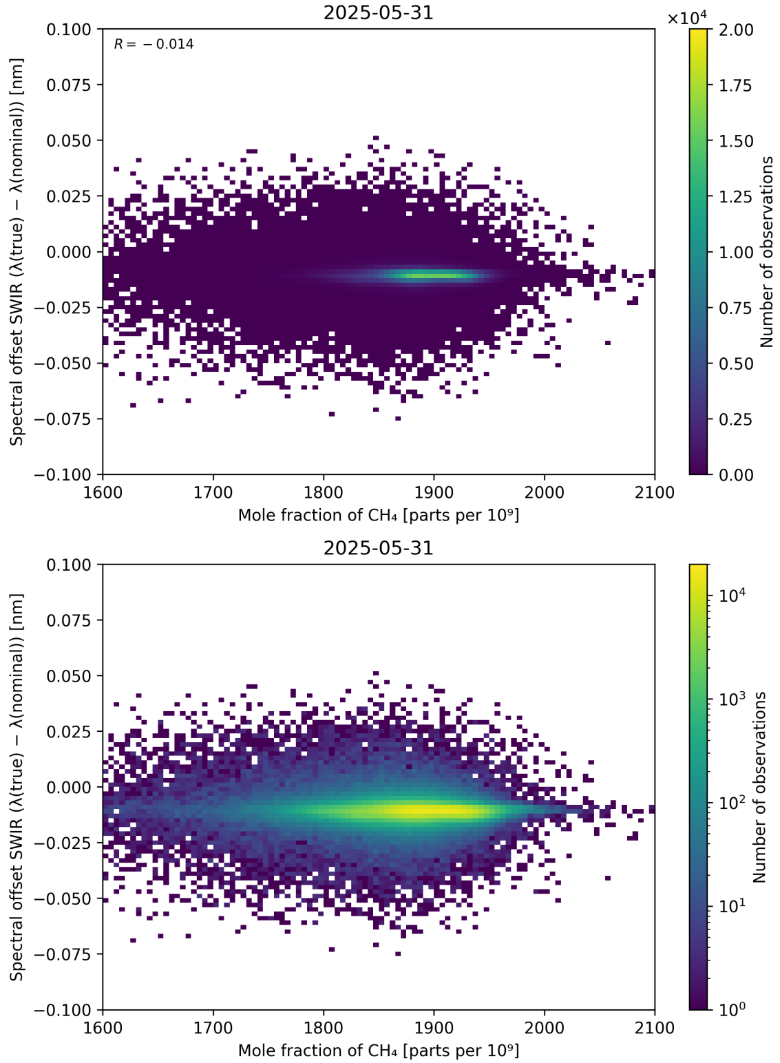
Figure 86: Scatter density plot of “Mole fraction of CH 4 ” against “Spectral offset SWIR ( \lambda_{\text{true}} - \lambda_{\text{nominal}} )” for 2025-05-31 to 2025-06-01.
