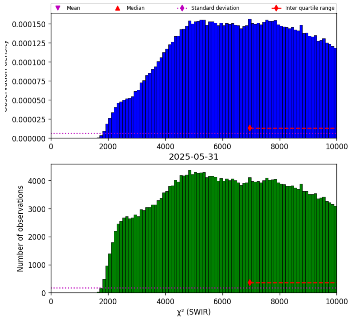
Figure 28: Histogram of “ \chi^2 (SWIR)” for 2025-05-31 to 2025-06-01
