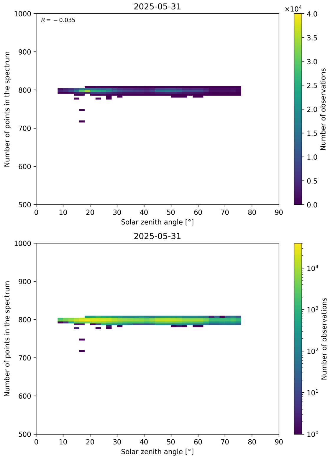
Figure 103: Scatter density plot of “Solar zenith angle” against “Number of points in the spectrum” for 2025-05-31 to 2025-06-01.
