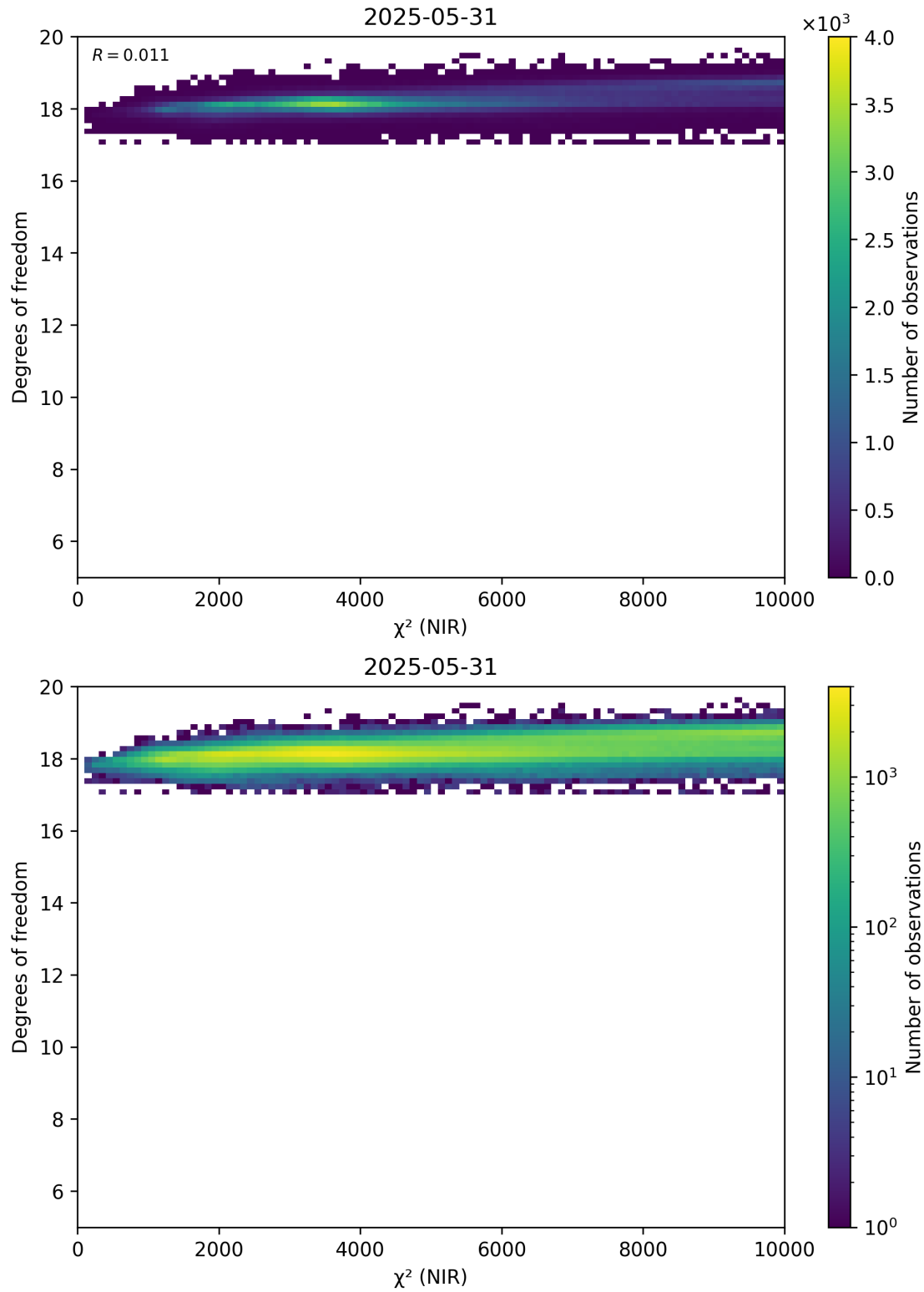
Figure 44: Scatter density plot of “ \chi^2 (NIR)” against “Degrees of freedom” for 2025-05-31 to 2025-06-01.
