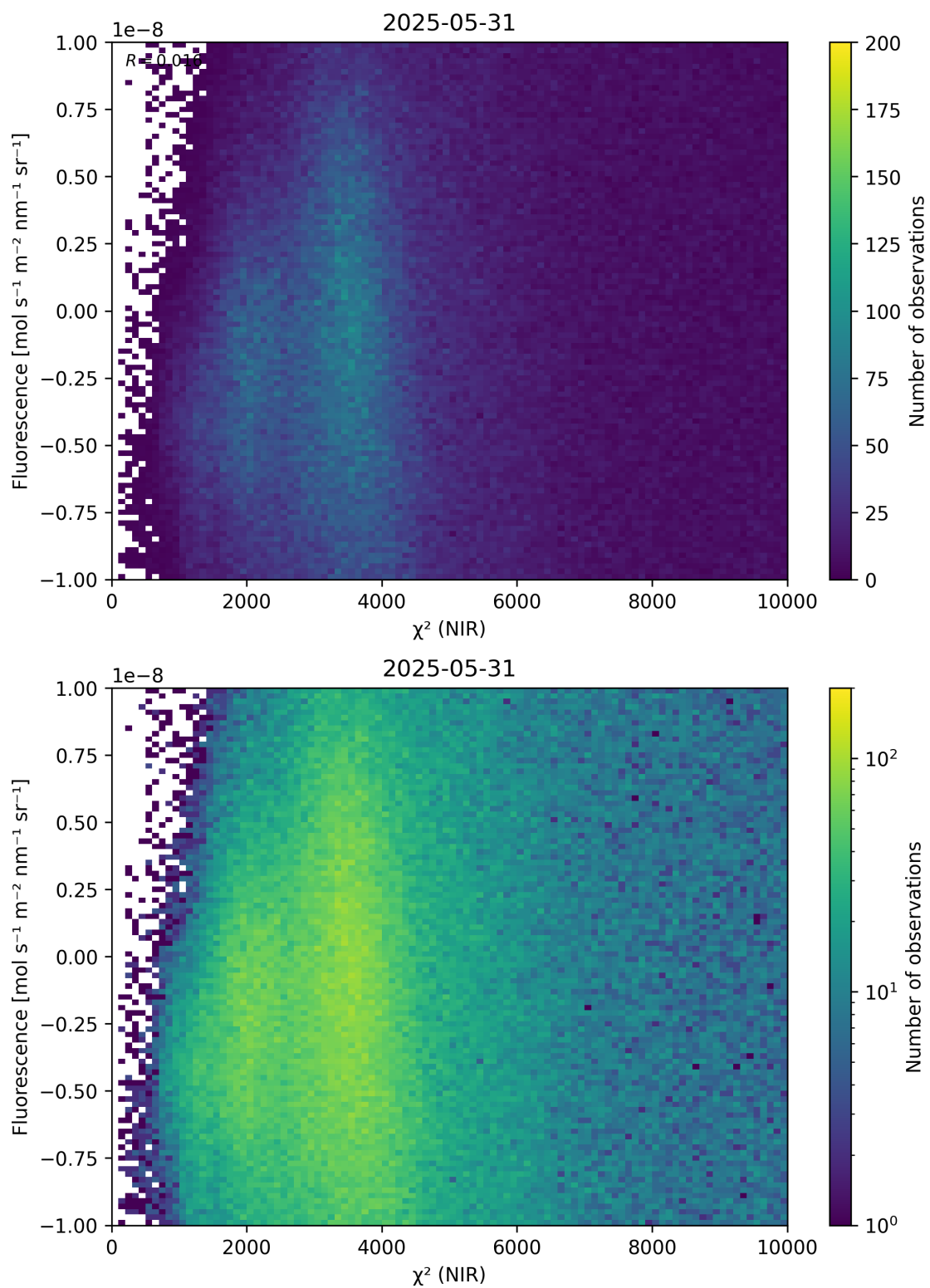
Figure 45: Scatter density plot of “ \chi^2 (NIR)” against “Fluorescence” for 2025-05-31 to 2025-06-01.
