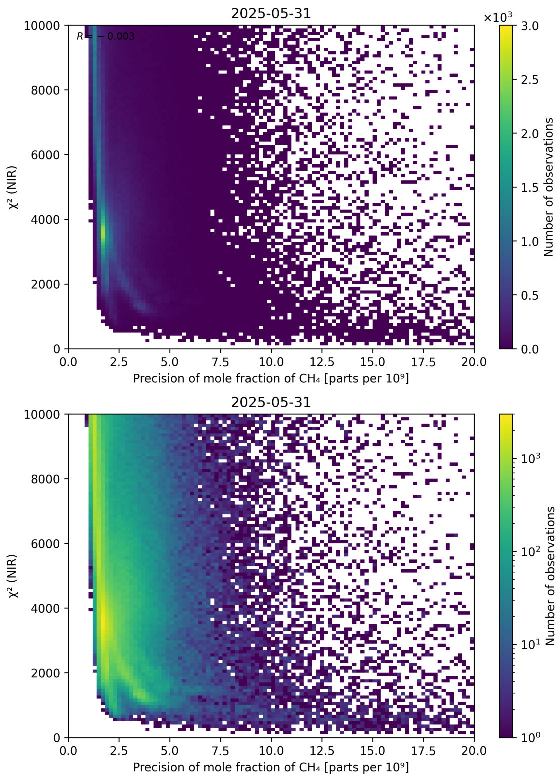
Figure 78: Scatter density plot of “Precision of mole fraction of CH 4 ” against “ \chi^2 (NIR)” for 2025-05-31 to 2025-06-01.
