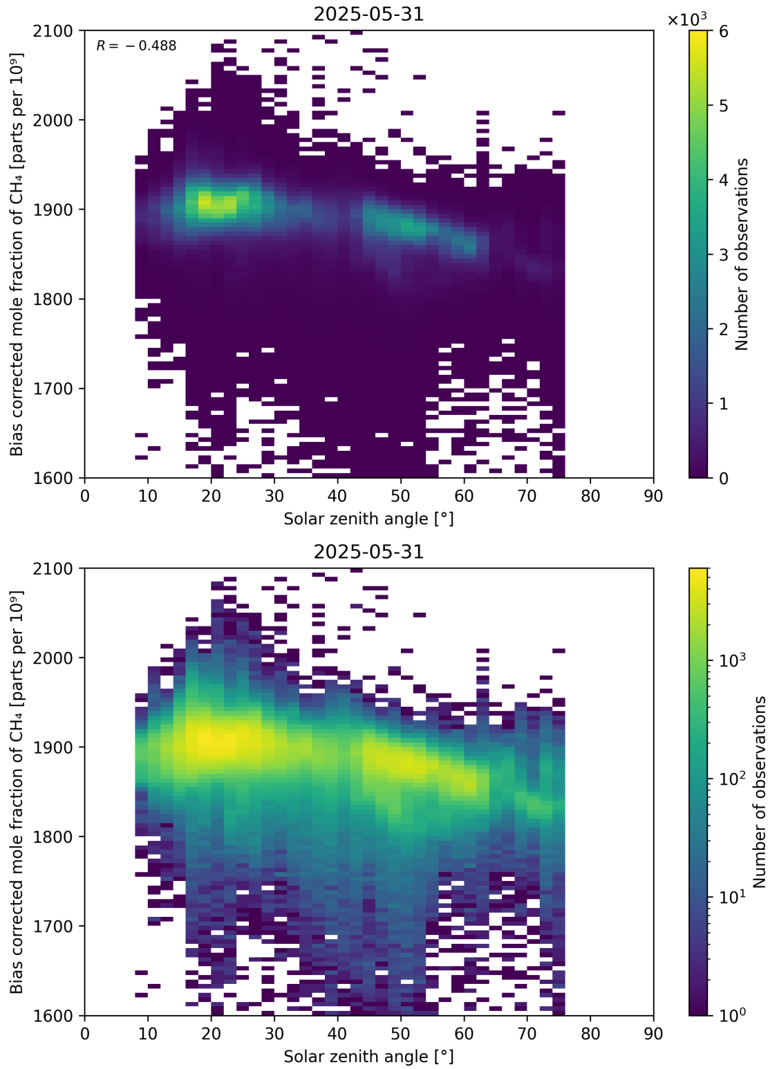
Figure 100: Scatter density plot of “Solar zenith angle” against “Bias corrected mole fraction of CH 4 ” for 2025-05-31 to 2025-06-01.
