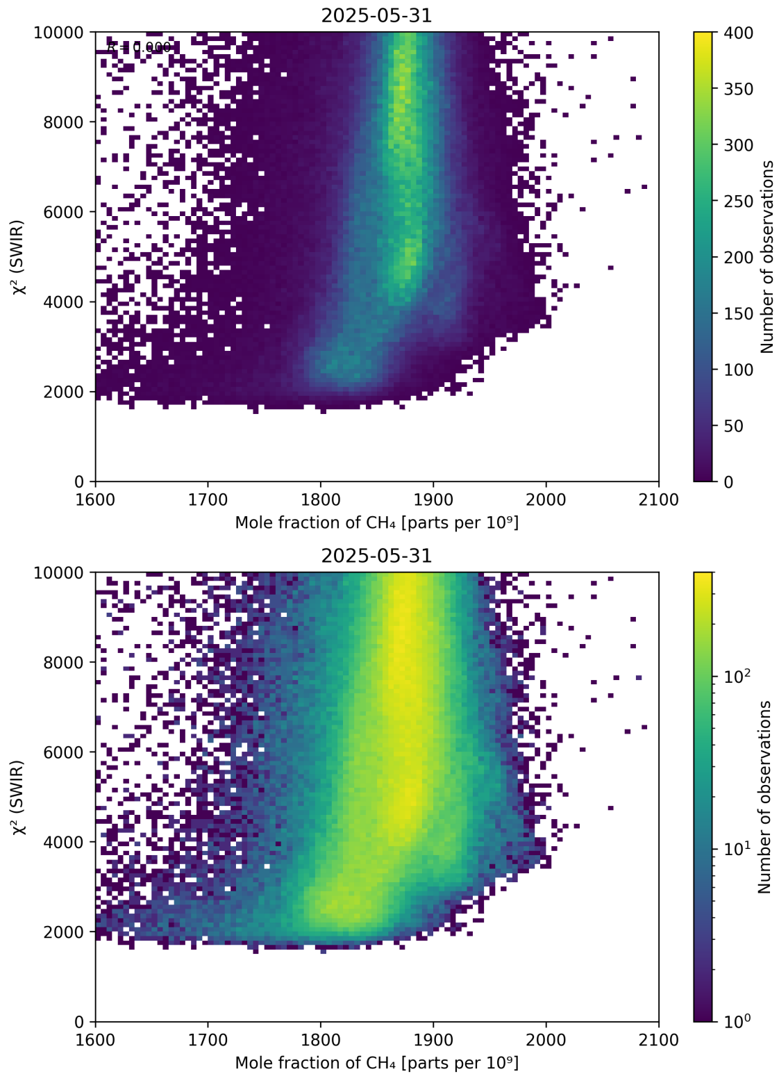
Figure 71: Scatter density plot of “Mole fraction of CH 4 ” against “ \chi^2 (SWIR)” for 2025-05-31 to 2025-06-01.
