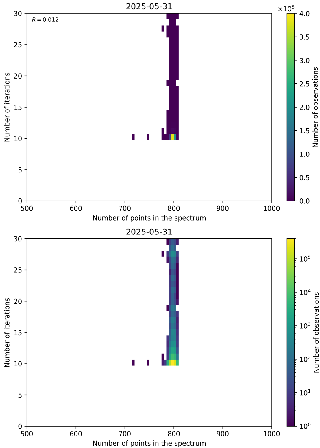
Figure 92: Scatter density plot of “Number of points in the spectrum” against “Number of iterations” for 2025-05-31 to 2025-06-01.
