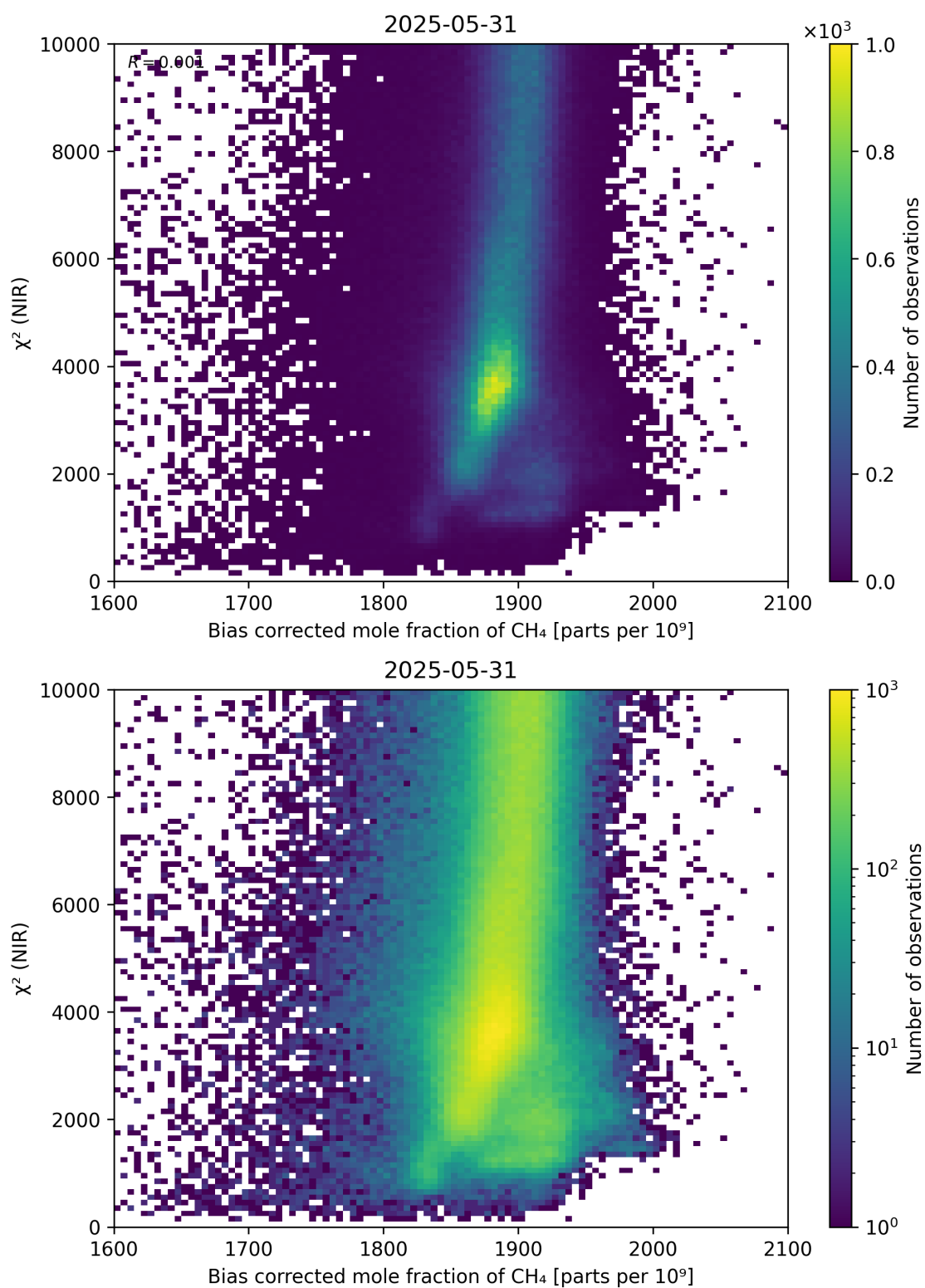
Figure 63: Scatter density plot of “Bias corrected mole fraction of \text{CH}_4 ” against “ \chi^2 (NIR)” for 2025-05-31 to 2025-06-01.
