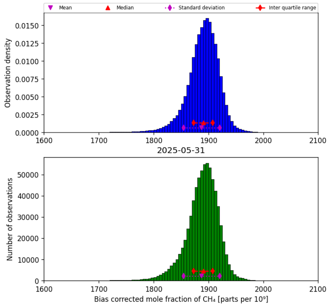
Figure 25: Histogram of "Bias corrected mole fraction of CH 4 " for 2025-05-31 to 2025-06-01
