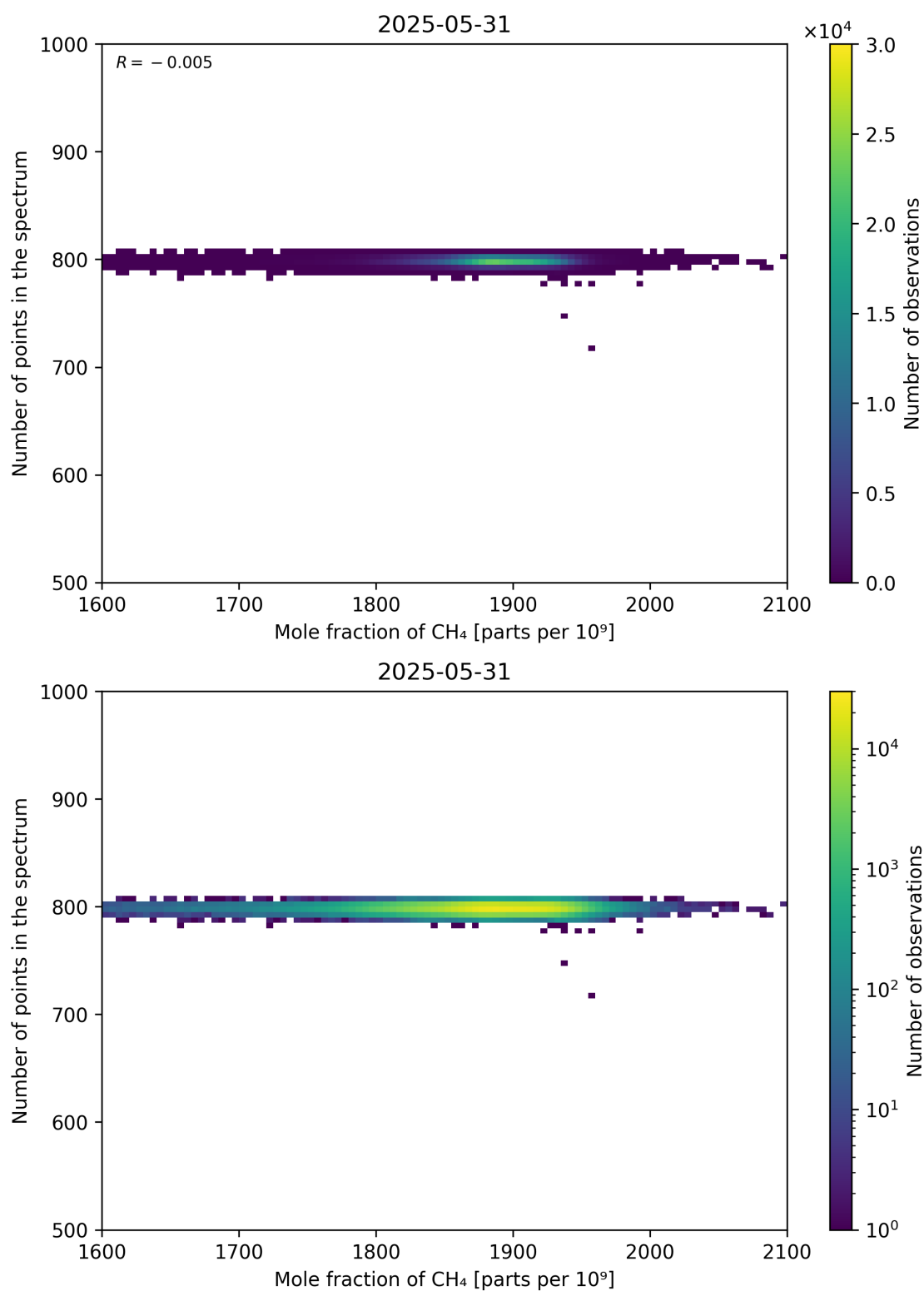
Figure 77: Scatter density plot of “Mole fraction of CH 4 ” against “Number of points in the spectrum” for 2025-05-31 to 2025-06-01.
