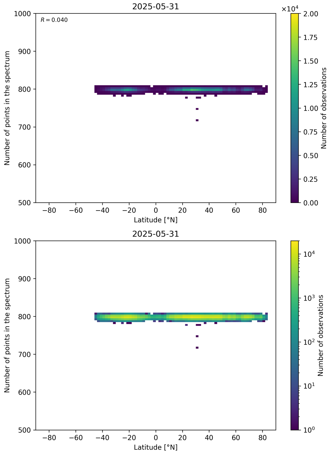
Figure 61: Scatter density plot of “Latitude” against “Number of points in the spectrum” for 2025-05-31 to 2025-06-01.
