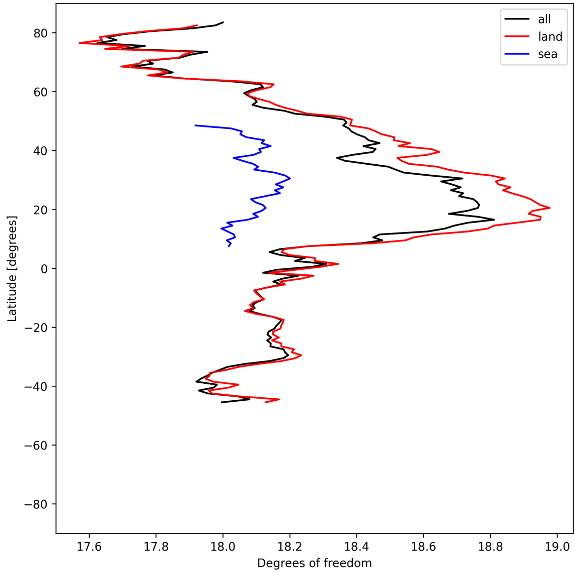
Figure 19: Zonal average of “Degrees of freedom” for 2025-05-31 to 2025-06-01.
