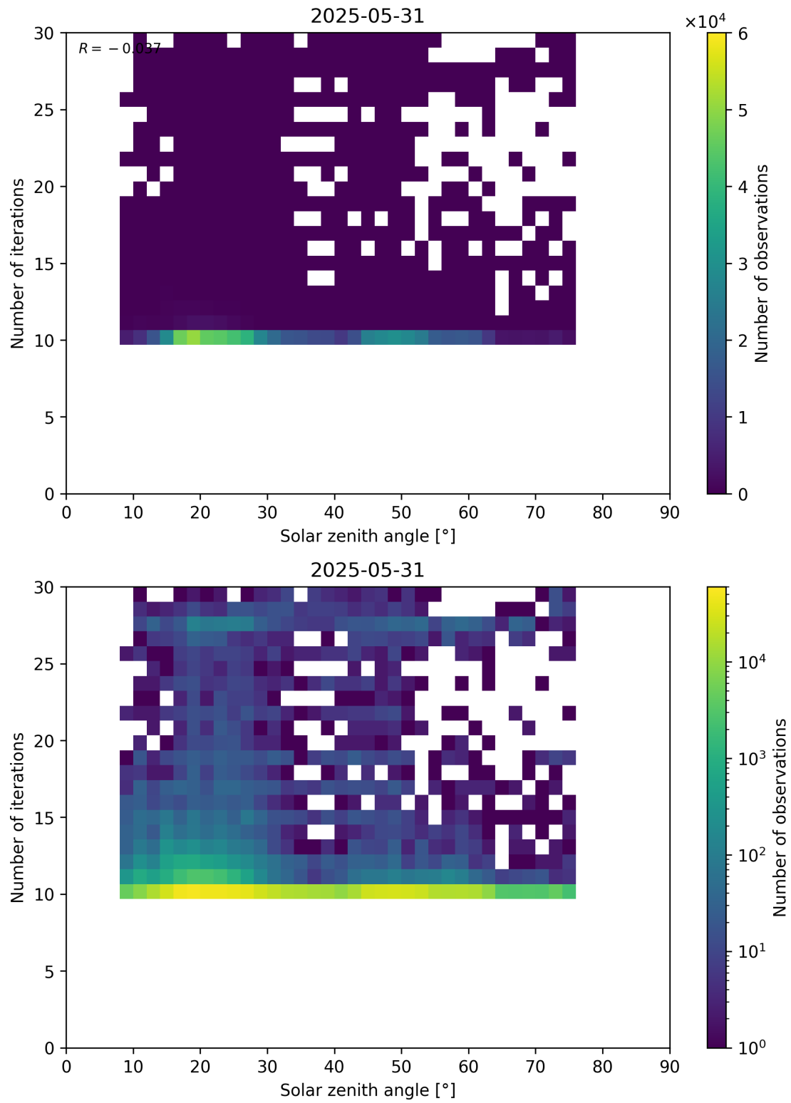
Figure 102: Scatter density plot of “Solar zenith angle” against “Number of iterations” for 2025-05-31 to 2025-06-01.
