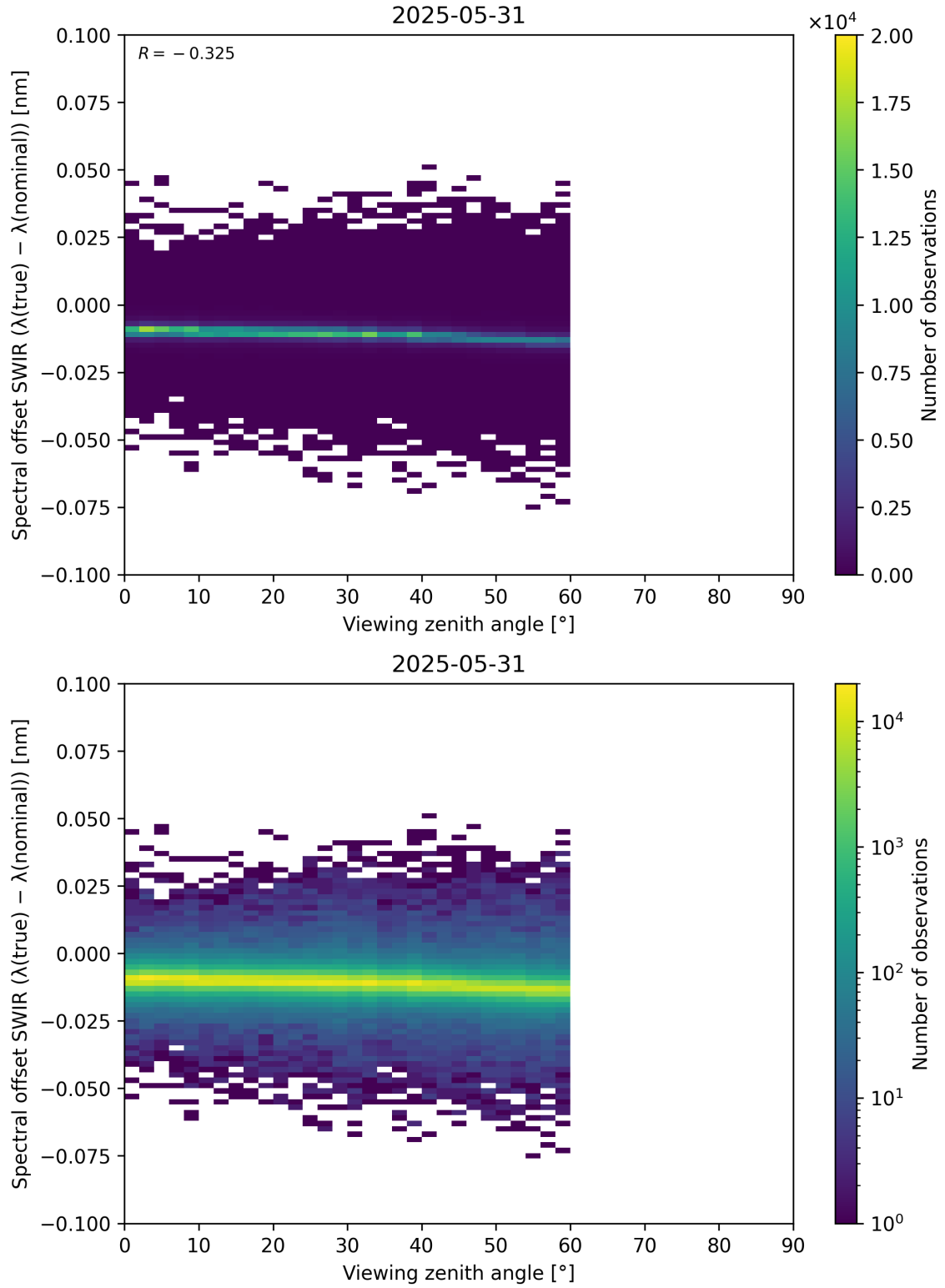
Figure 116: Scatter density plot of “Viewing zenith angle” against “Spectral offset SWIR ( \lambda_{\text{true}} - \lambda_{\text{nominal}} )” for 2025-05-31 to 2025-06-01.
