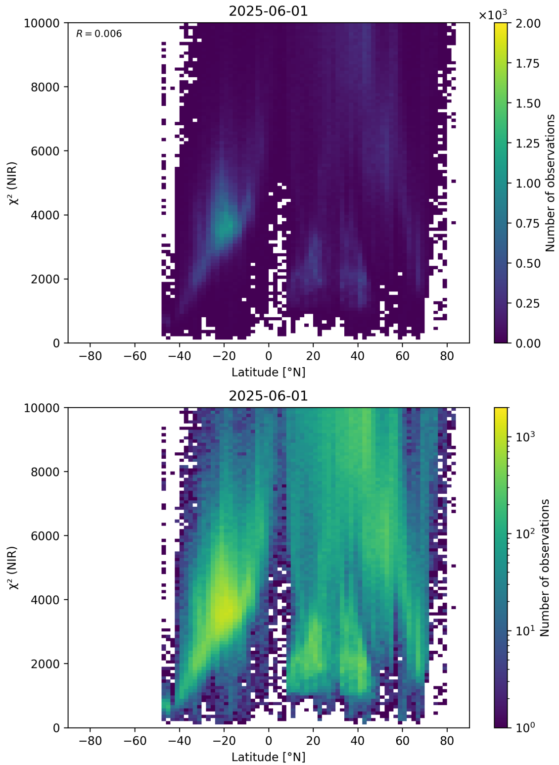
Figure 53: Scatter density plot of “Latitude” against “ \chi^2 (NIR)” for 2025-06-01 to 2025-06-02.
