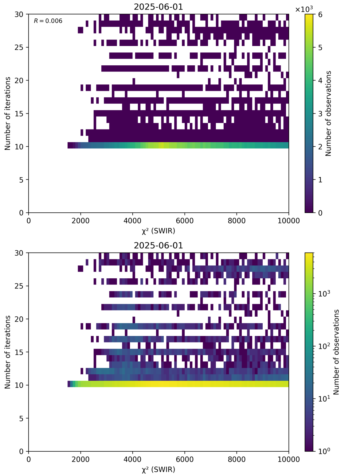
Figure 50: Scatter density plot of “ \chi^2 (SWIR)” against “Number of iterations” for 2025-06-01 to 2025-06-02.
