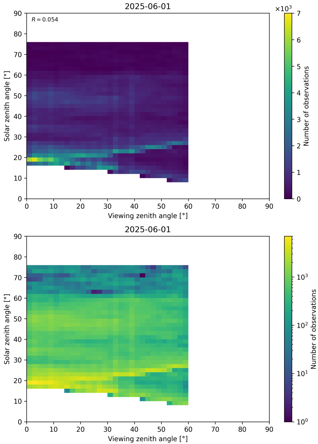
Figure 115: Scatter density plot of “Viewing zenith angle” against “Solar zenith angle” for 2025-06-01 to 2025-06-02.
