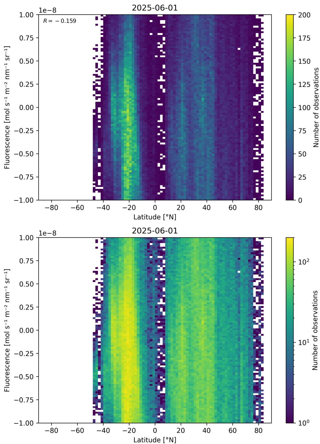
Figure 56: Scatter density plot of “Latitude” against “Fluorescence” for 2025-06-01 to 2025-06-02.
