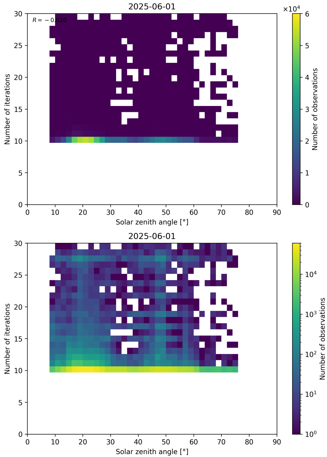
Figure 102: Scatter density plot of “Solar zenith angle” against “Number of iterations” for 2025-06-01 to 2025-06-02.
