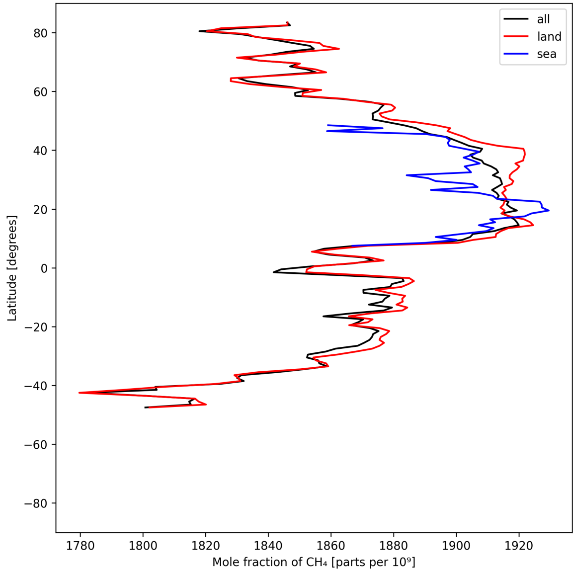
Figure 12: Zonal average of “Mole fraction of \text{CH}_4 ” for 2025-06-01 to 2025-06-02.
