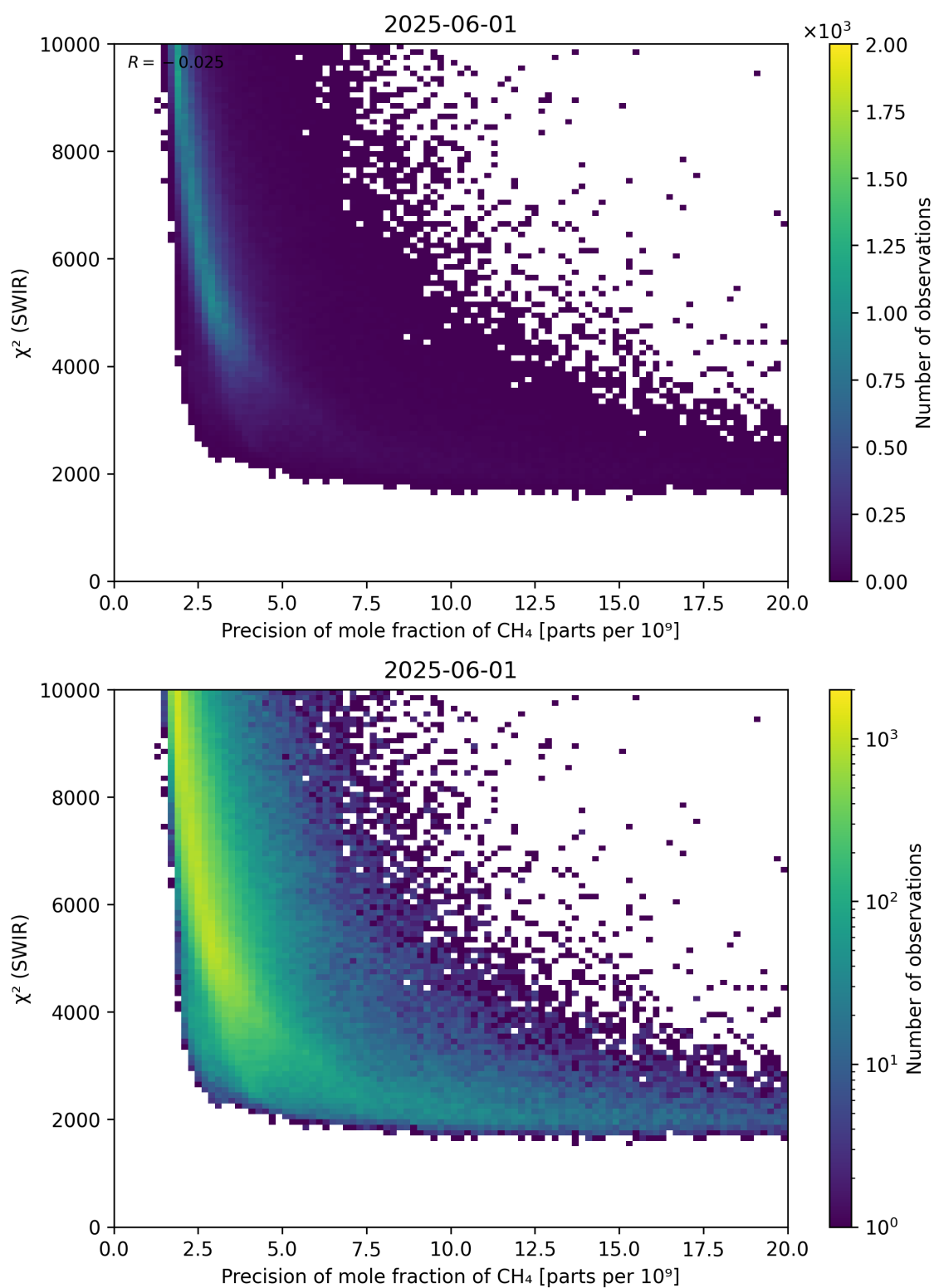
Figure 79: Scatter density plot of “Precision of mole fraction of \text{CH}_4 ” against “ \chi^2 (SWIR)” for 2025-06-01 to 2025-06-02.
