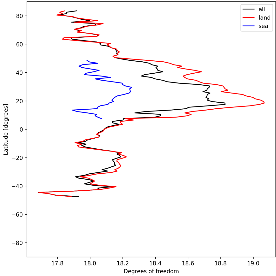
Figure 19: Zonal average of “Degrees of freedom” for 2025-06-01 to 2025-06-02.
