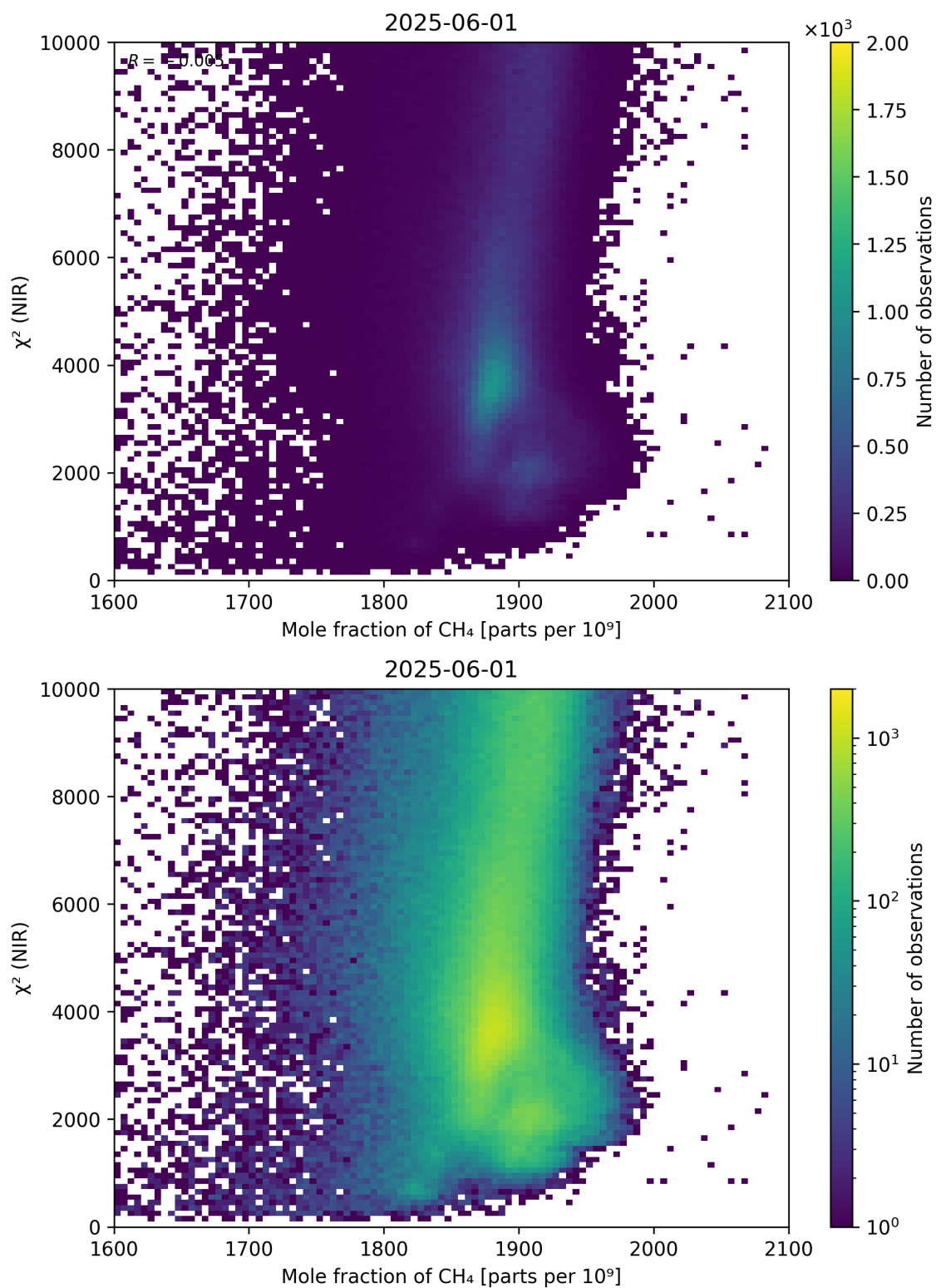
Figure 70: Scatter density plot of “Mole fraction of \text{CH}_4 ” against “ \chi^2 (NIR)” for 2025-06-01 to 2025-06-02.
