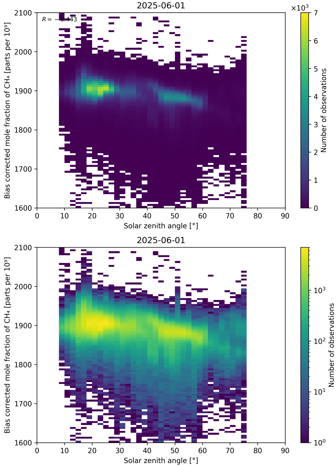
Figure 100: Scatter density plot of “Solar zenith angle” against “Bias corrected mole fraction of CH 4 ” for 2025-06-01 to 2025-06-02.
