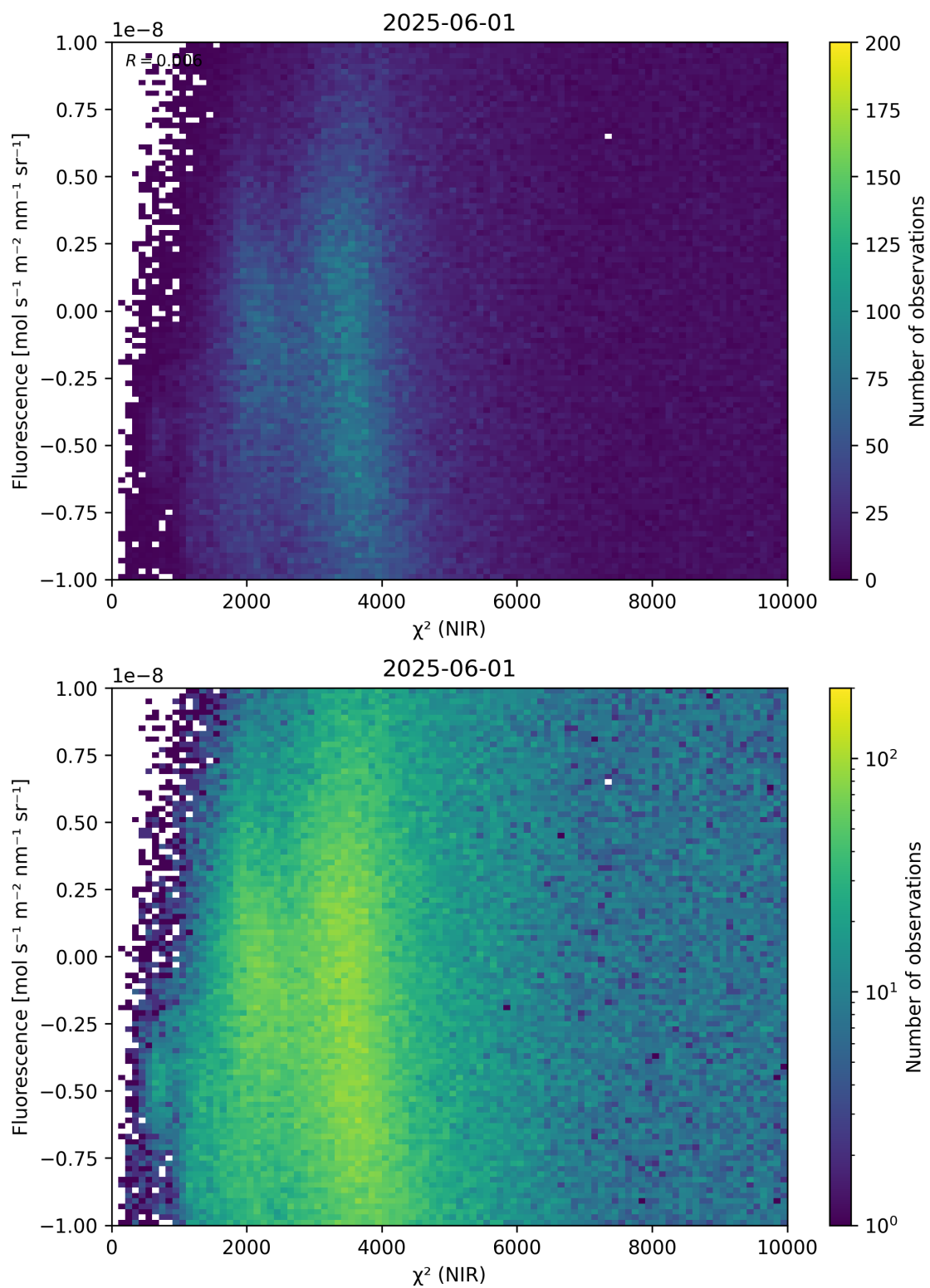
Figure 45: Scatter density plot of “ \chi^2 (NIR)” against “Fluorescence” for 2025-06-01 to 2025-06-02.
