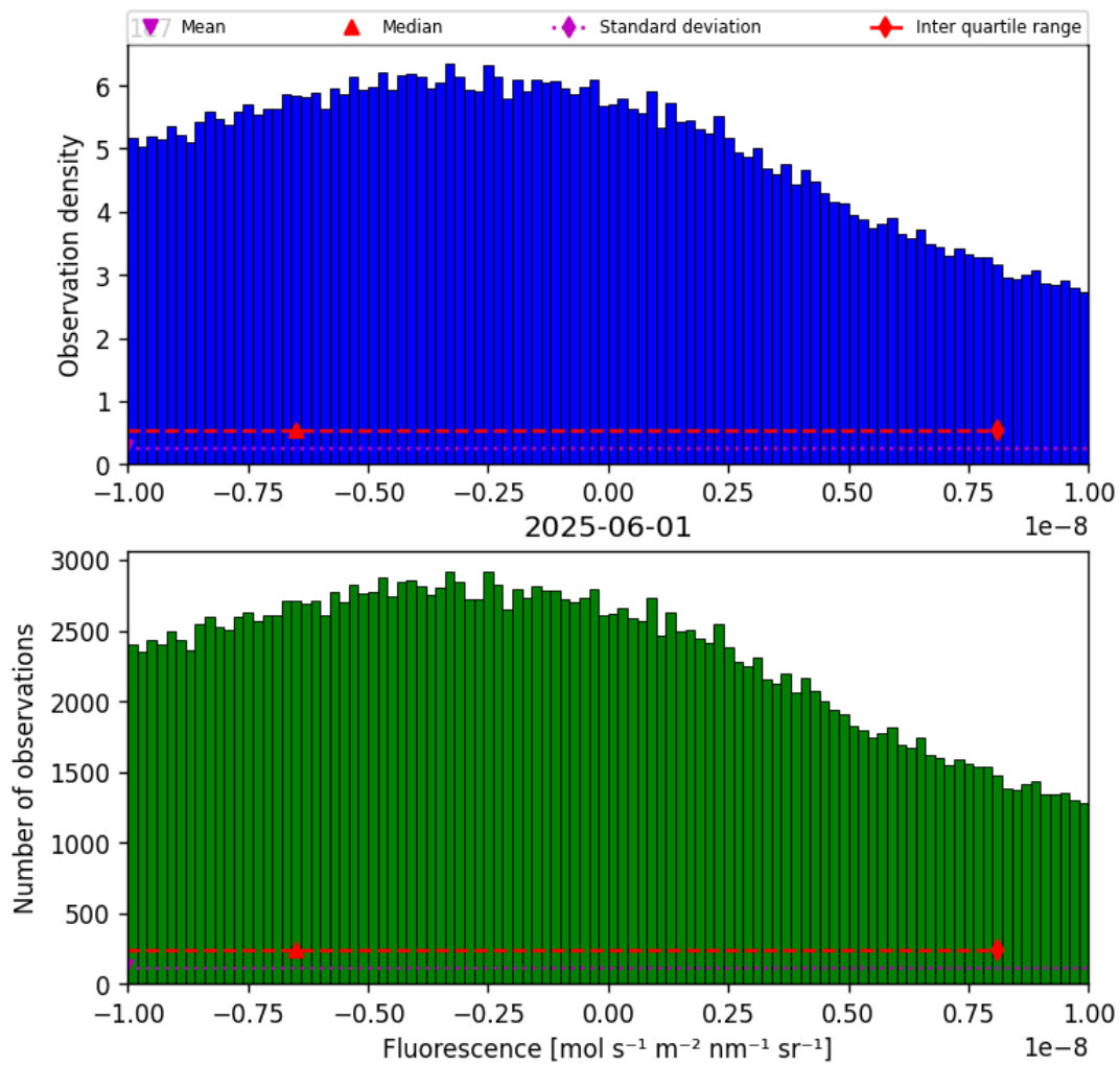
Figure 32: Histogram of “Fluorescence” for 2025-06-01 to 2025-06-02
