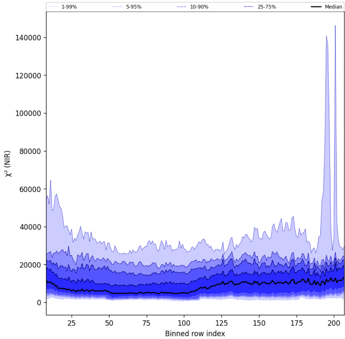
Figure 40: Along track statistics of “ \chi^2 (NIR)” for 2025-06-01 to 2025-06-02
