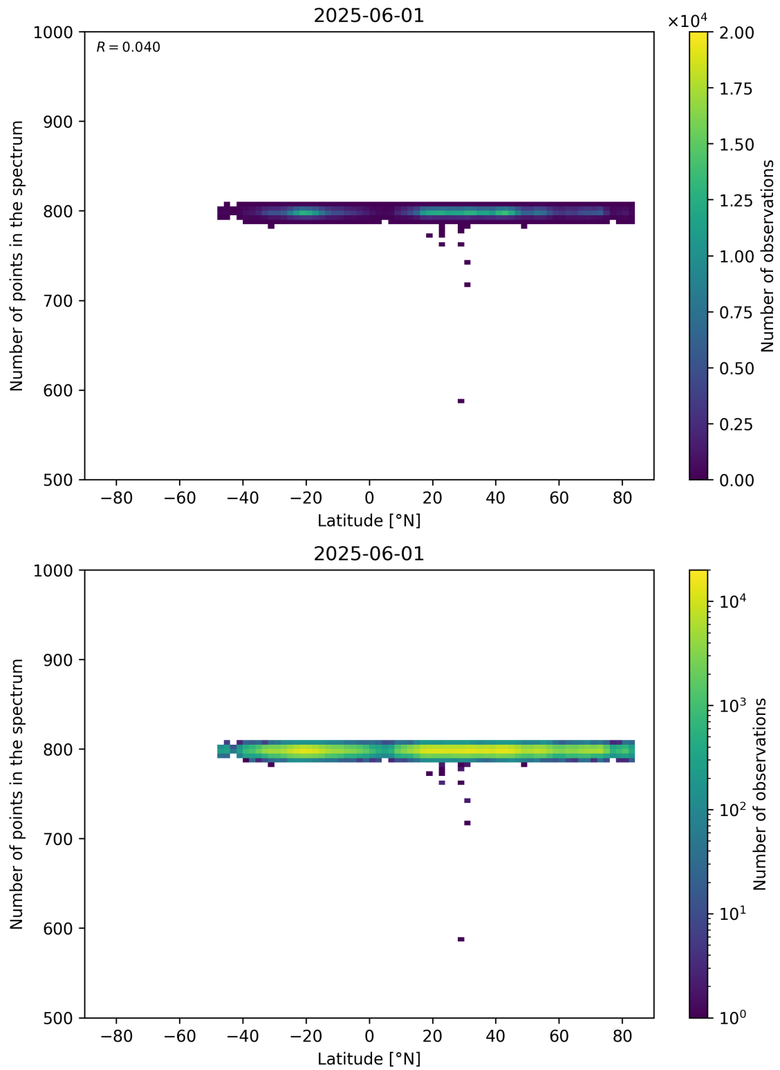
Figure 61: Scatter density plot of “Latitude” against “Number of points in the spectrum” for 2025-06-01 to 2025-06-02.
