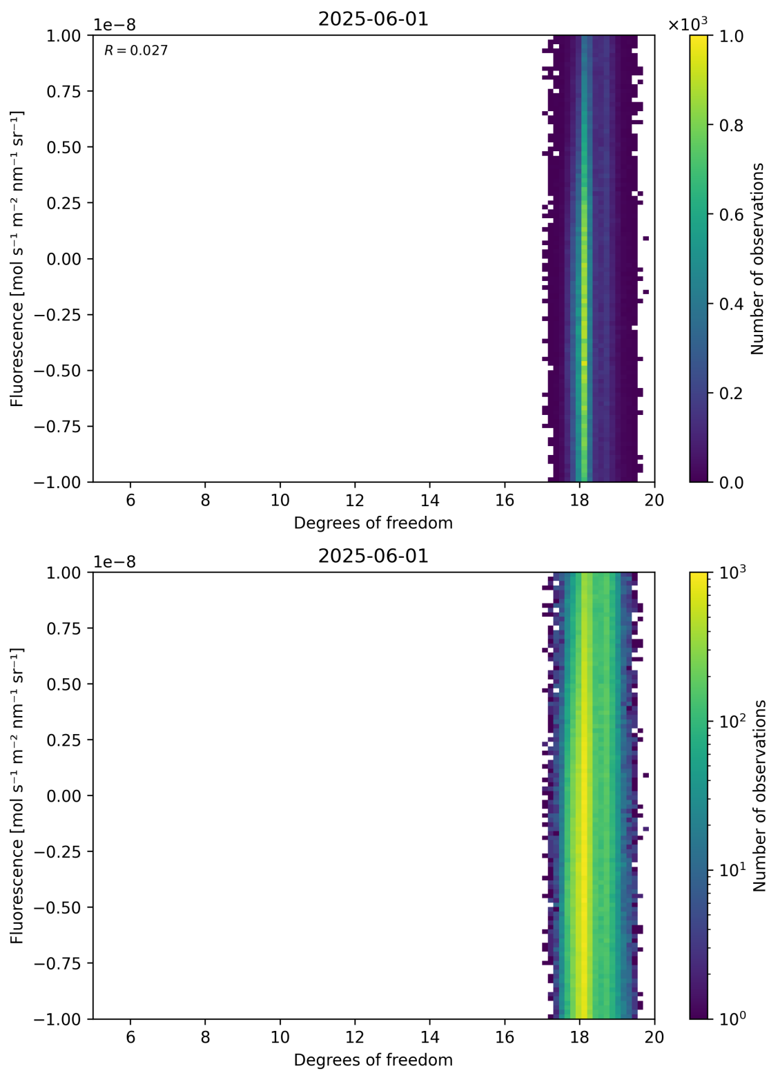
Figure 51: Scatter density plot of “Degrees of freedom” against “Fluorescence” for 2025-06-01 to 2025-06-02.
