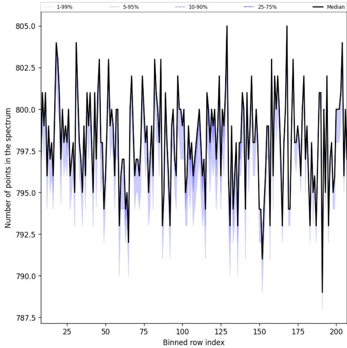
Figure 37: Along track statistics of “Number of points in the spectrum” for 2025-06-01 to 2025-06-02
