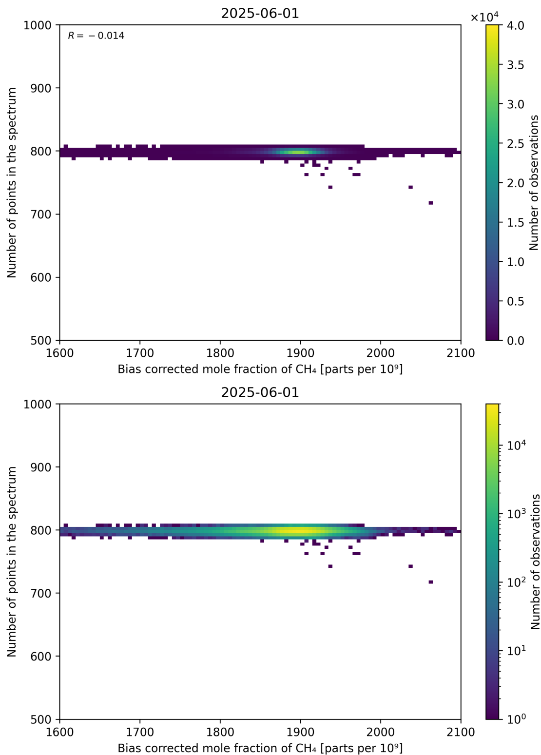
Figure 68: Scatter density plot of “Bias corrected mole fraction of CH 4 ” against “Number of points in the spectrum” for 2025-06-01 to 2025-06-02.
