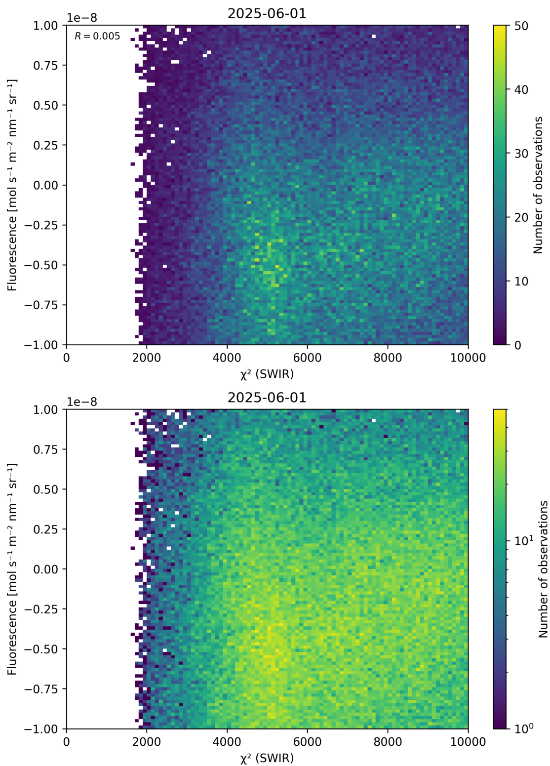
Figure 49: Scatter density plot of “ \chi^2 (SWIR)” against “Fluorescence” for 2025-06-01 to 2025-06-02.
