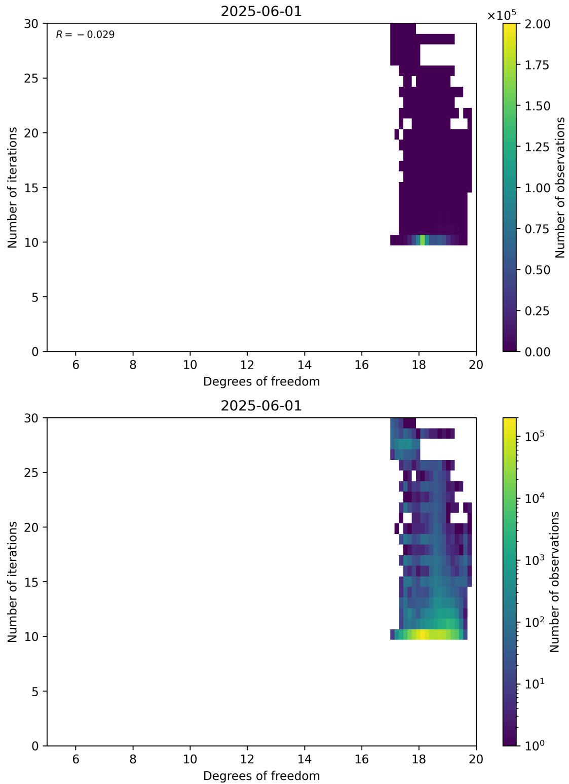
Figure 52: Scatter density plot of “Degrees of freedom” against “Number of iterations” for 2025-06-01 to 2025-06-02.
