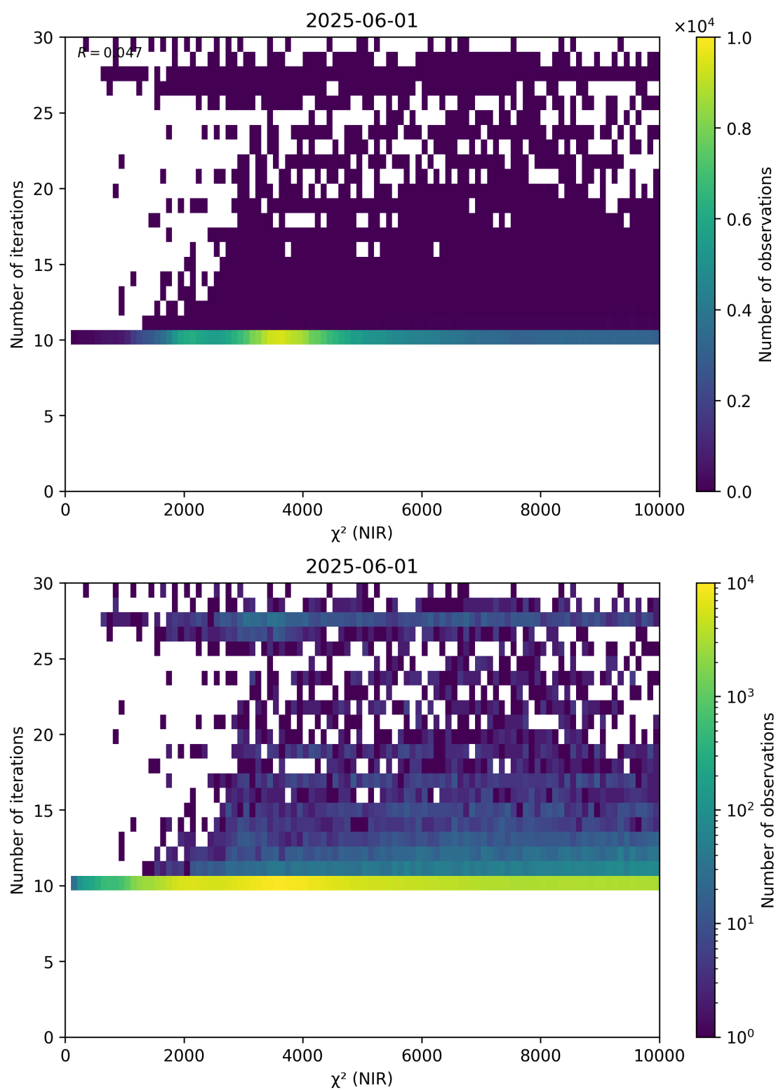
Figure 46: Scatter density plot of “ \chi^2 (NIR)” against “Number of iterations” for 2025-06-01 to 2025-06-02.
