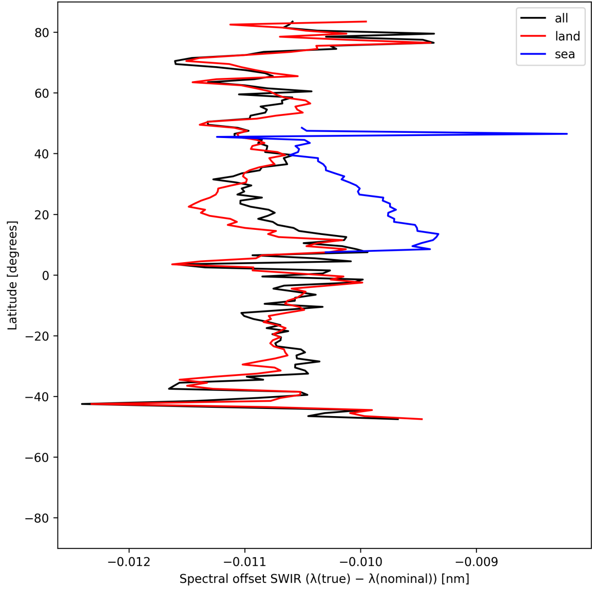
Figure 16: Zonal average of “Spectral offset SWIR ( \lambda_{\text{true}} - \lambda_{\text{nominal}} )” for 2025-06-01 to 2025-06-02.
