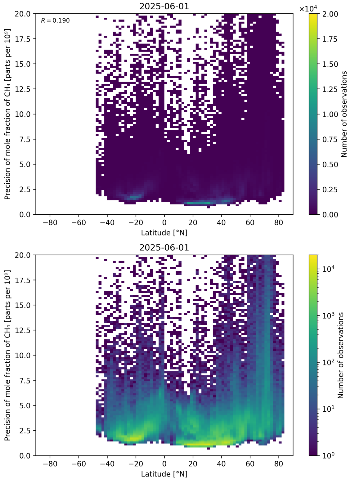
Figure 59: Scatter density plot of “Latitude” against “Precision of mole fraction of \text{CH}_4 ” for 2025-06-01 to 2025-06-02.
