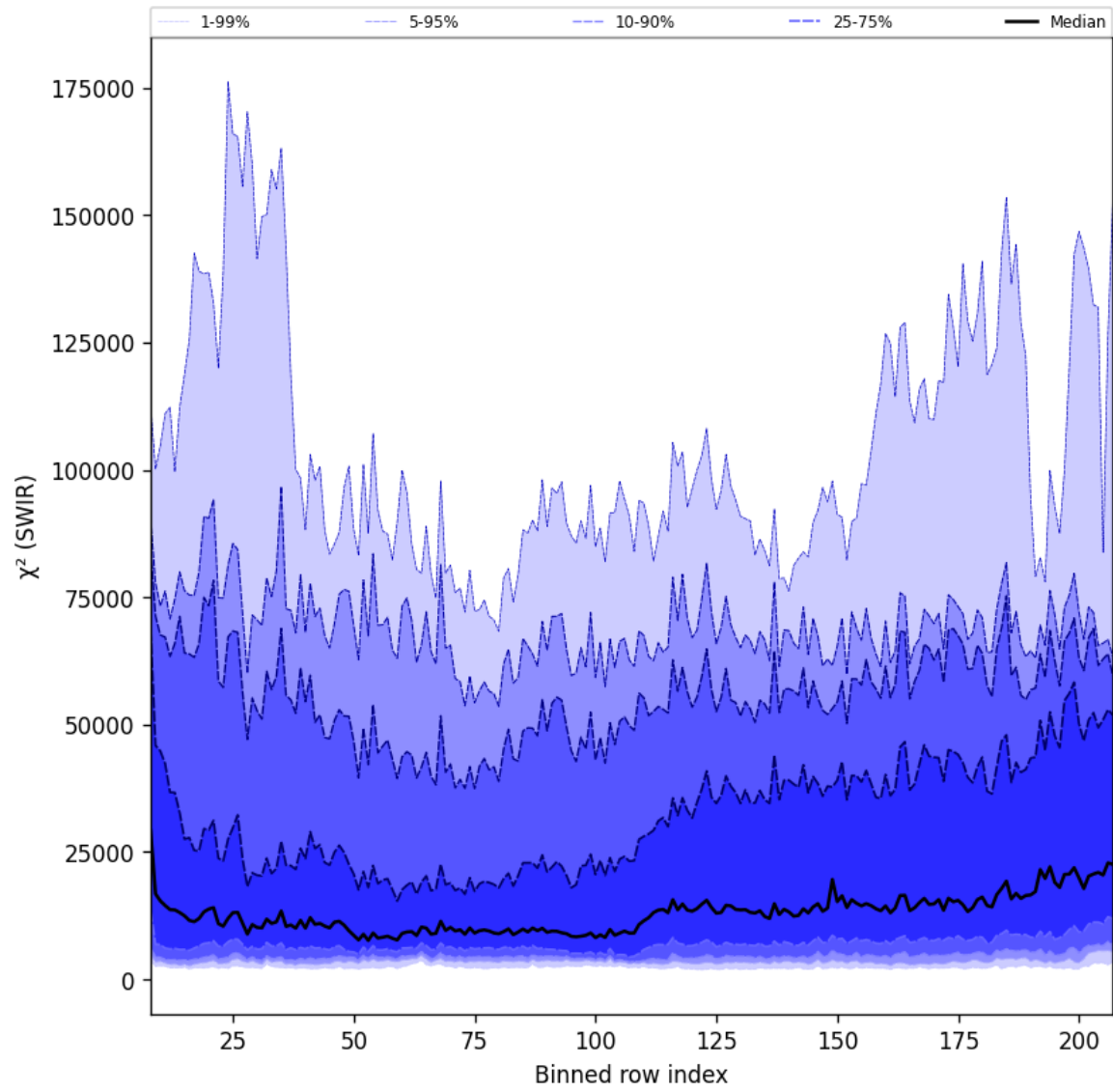
Figure 39: Along track statistics of " \chi^2 (SWIR)" for 2025-06-01 to 2025-06-02
