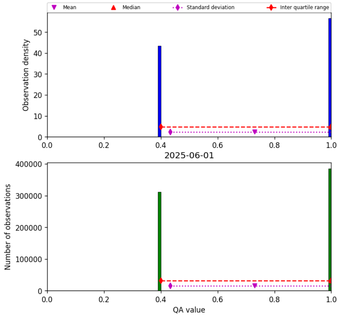
Figure 22: Histogram of “QA value” for 2025-06-01 to 2025-06-02
