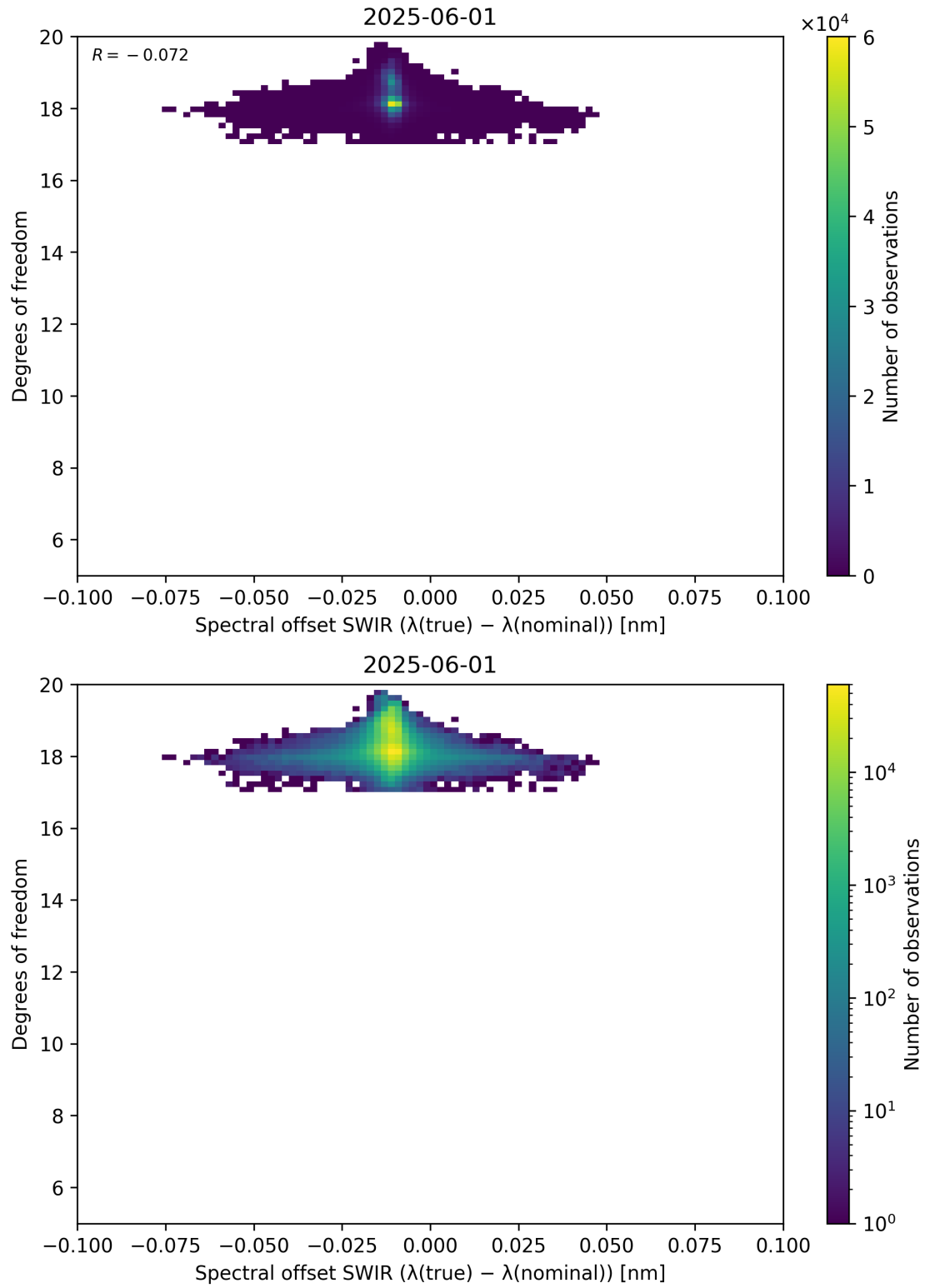
Figure 119: Scatter density plot of “Spectral offset SWIR ( \lambda_{\text{true}} - \lambda_{\text{nominal}} )” against “Degrees of freedom” for 2025-06-01 to 2025-06-02.
