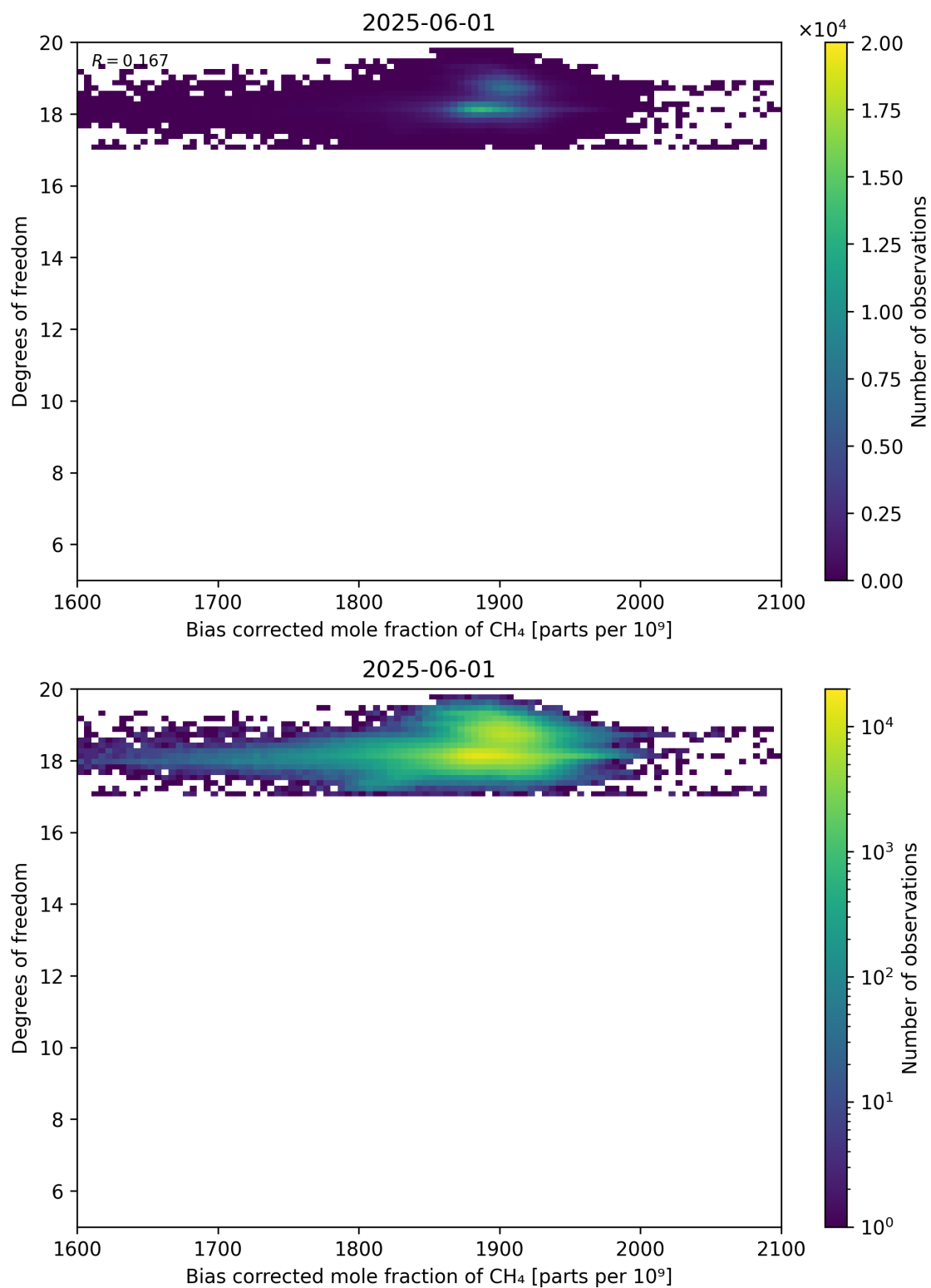
Figure 65: Scatter density plot of “Bias corrected mole fraction of CH 4 ” against “Degrees of freedom” for 2025-06-01 to 2025-06-02.
