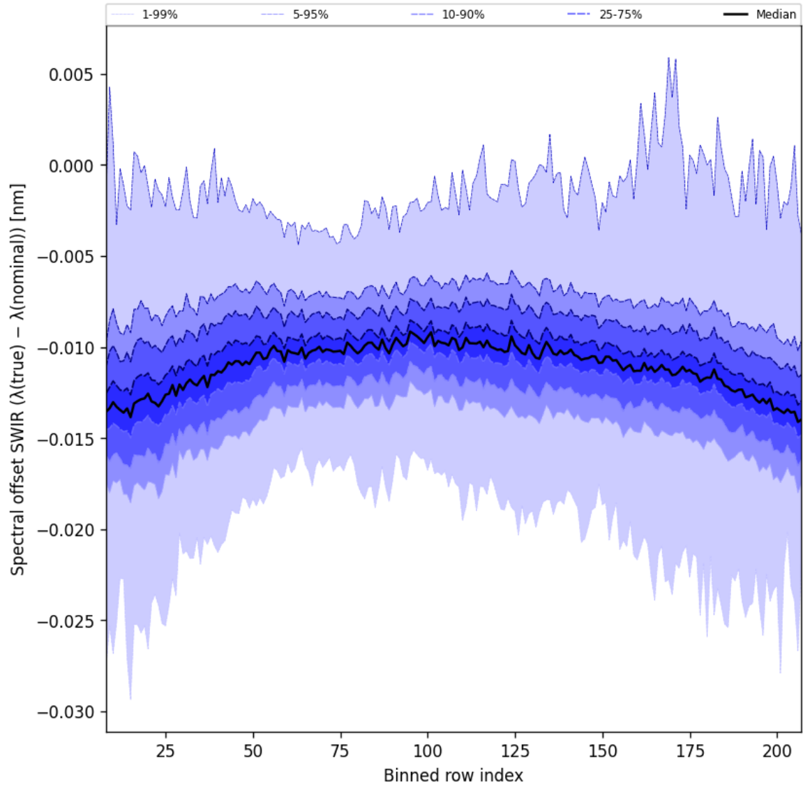
Figure 38: Along track statistics of “Spectral offset SWIR ( \lambda_{\text{true}} - \lambda_{\text{nominal}} )” for 2025-06-01 to 2025-06-02
