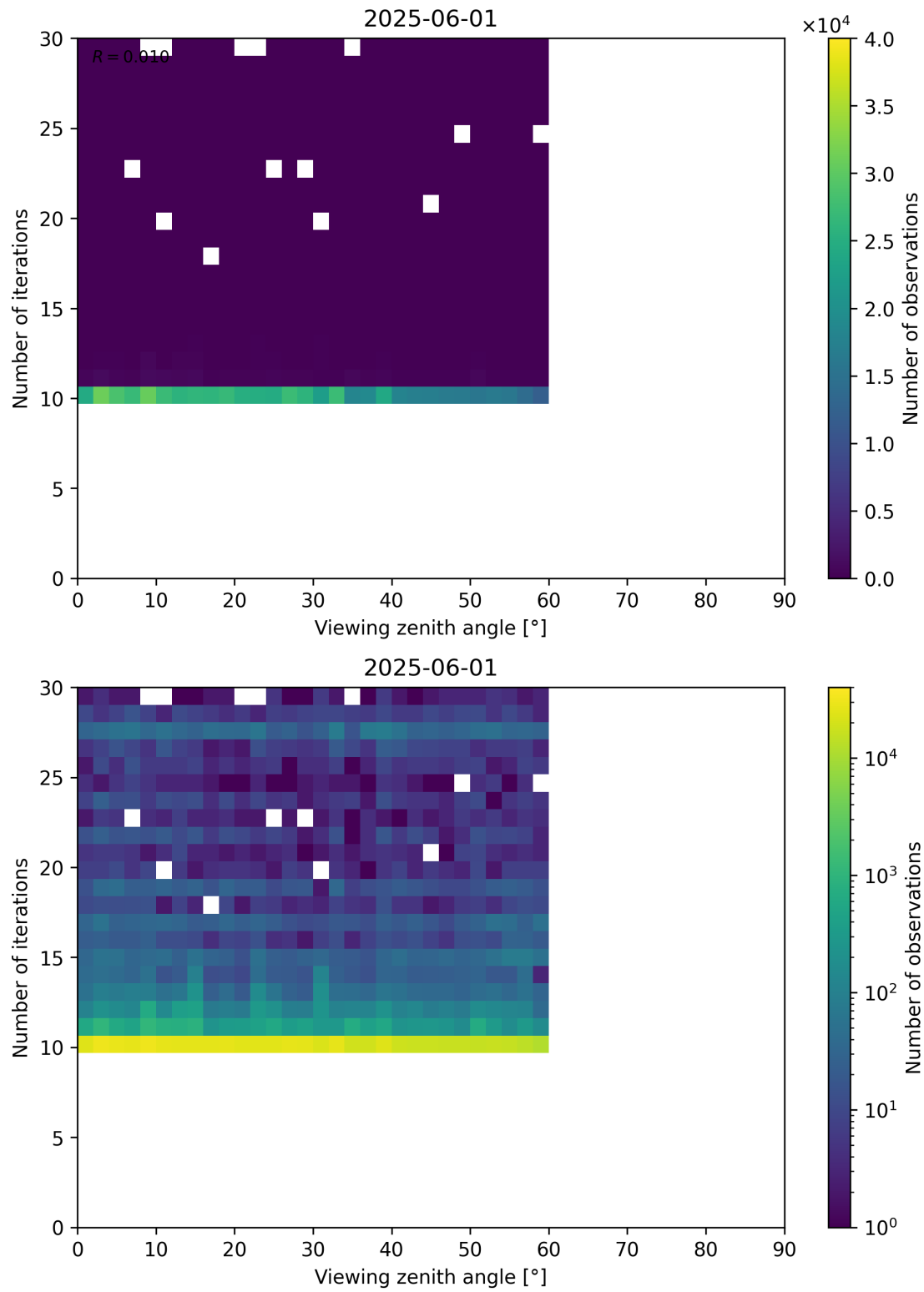
Figure 113: Scatter density plot of “Viewing zenith angle” against “Number of iterations” for 2025-06-01 to 2025-06-02.
