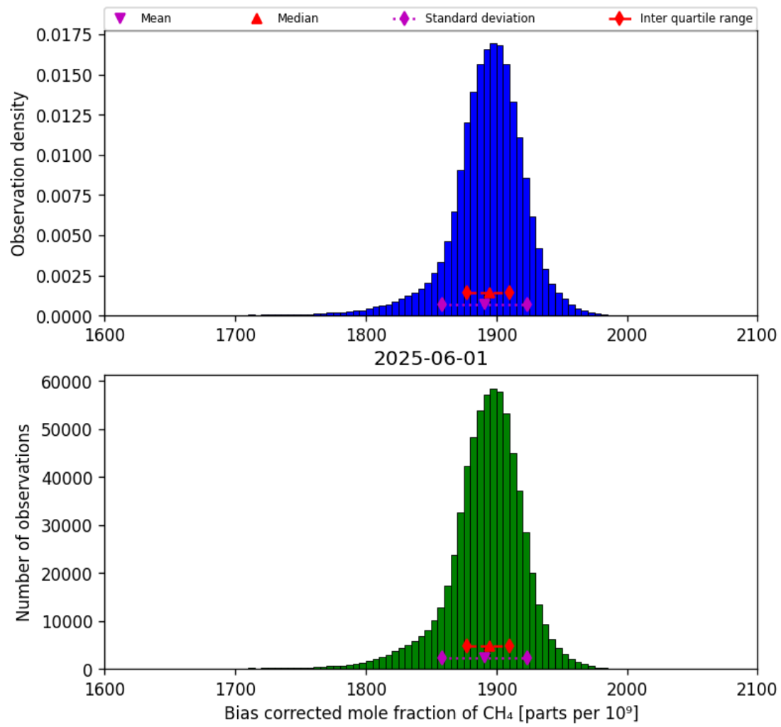
Figure 25: Histogram of “Bias corrected mole fraction of CH 4 ” for 2025-06-01 to 2025-06-02
