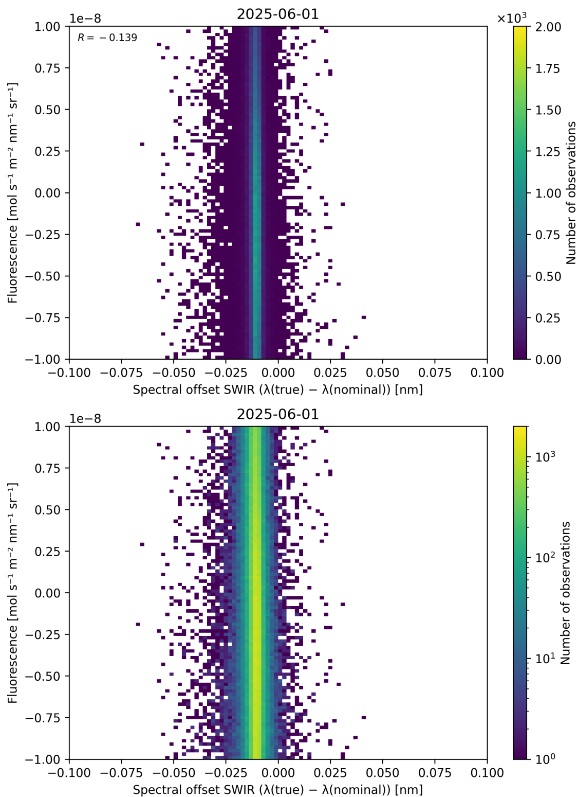
Figure 120: Scatter density plot of “Spectral offset SWIR ( \lambda_{\text{true}} - \lambda_{\text{nominal}} )” against “Fluorescence” for 2025-06-01 to 2025-06-02.
