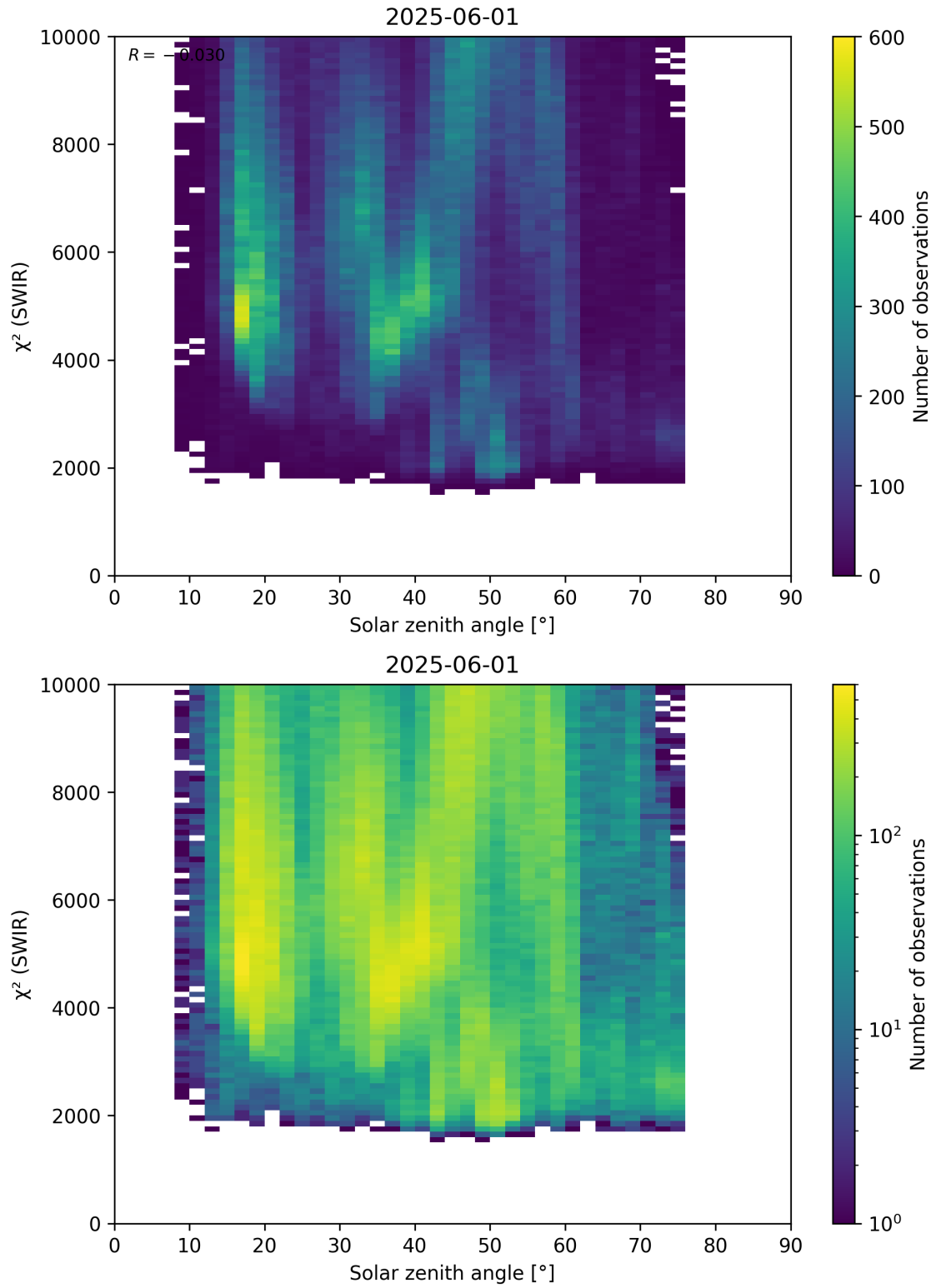
Figure 95: Scatter density plot of “Solar zenith angle” against “ \chi^2 (SWIR)” for 2025-06-01 to 2025-06-02.
