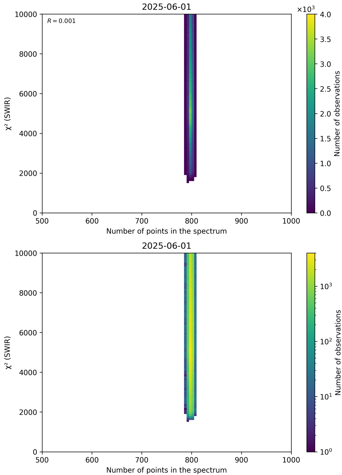
Figure 89: Scatter density plot of “Number of points in the spectrum” against “ \chi^2 (SWIR)” for 2025-06-01 to 2025-06-02.
