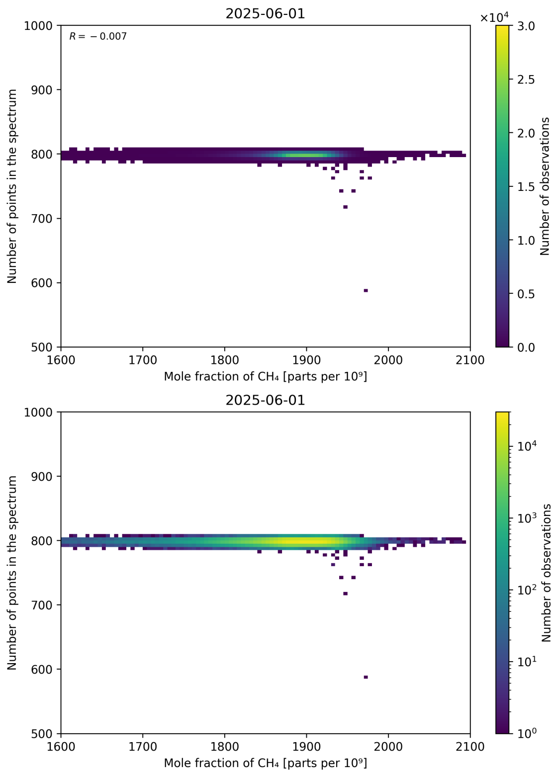
Figure 77: Scatter density plot of “Mole fraction of CH 4 ” against “Number of points in the spectrum” for 2025-06-01 to 2025-06-02.
