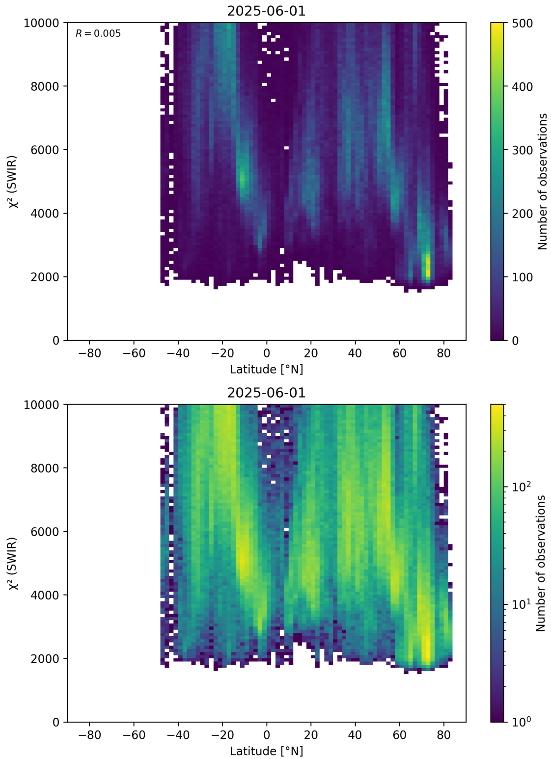
Figure 54: Scatter density plot of “Latitude” against “ \chi^2 (SWIR)” for 2025-06-01 to 2025-06-02.
