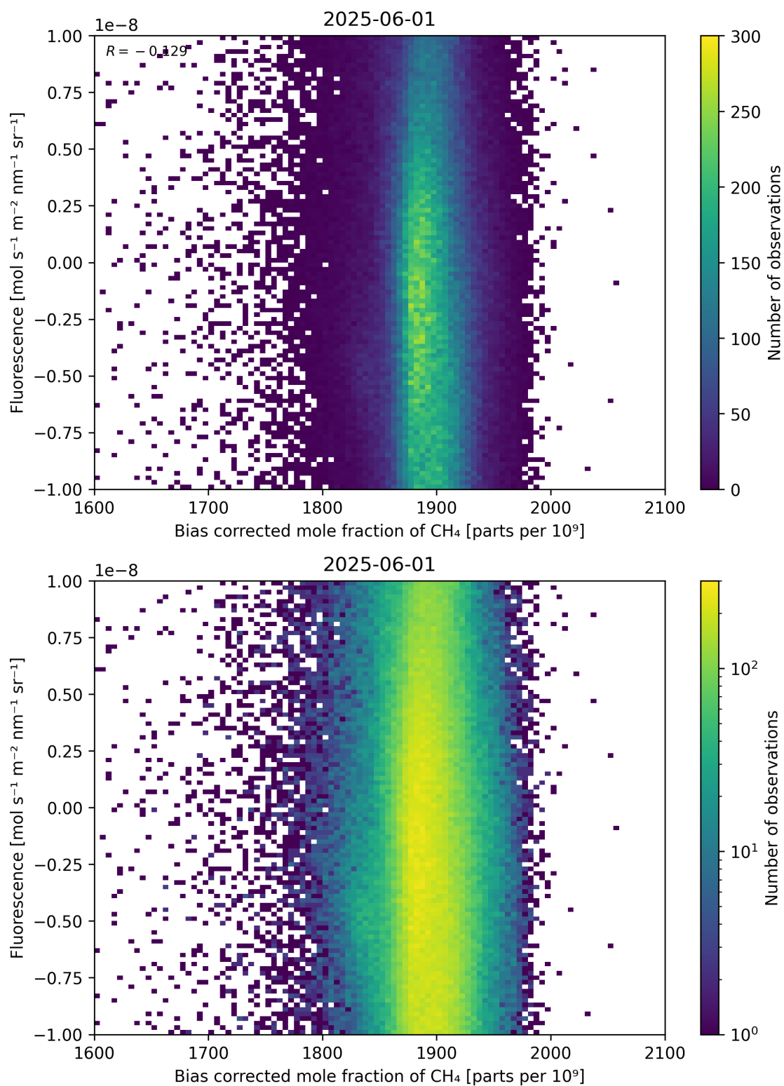
Figure 66: Scatter density plot of “Bias corrected mole fraction of \text{CH}_4 ” against “Fluorescence” for 2025-06-01 to 2025-06-02.
