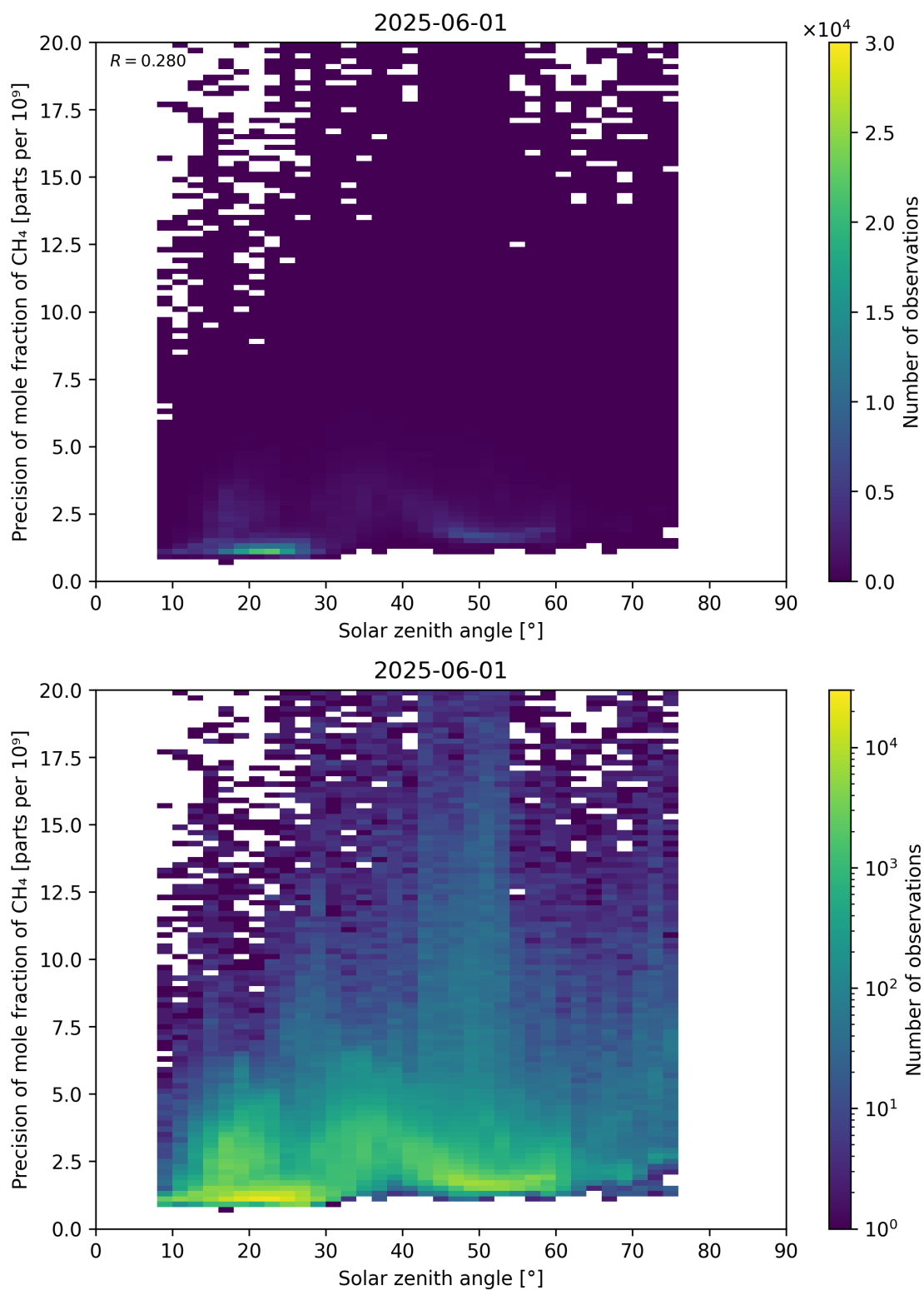
Figure 101: Scatter density plot of “Solar zenith angle” against “Precision of mole fraction of \text{CH}_4 ” for 2025-06-01 to 2025-06-02.
