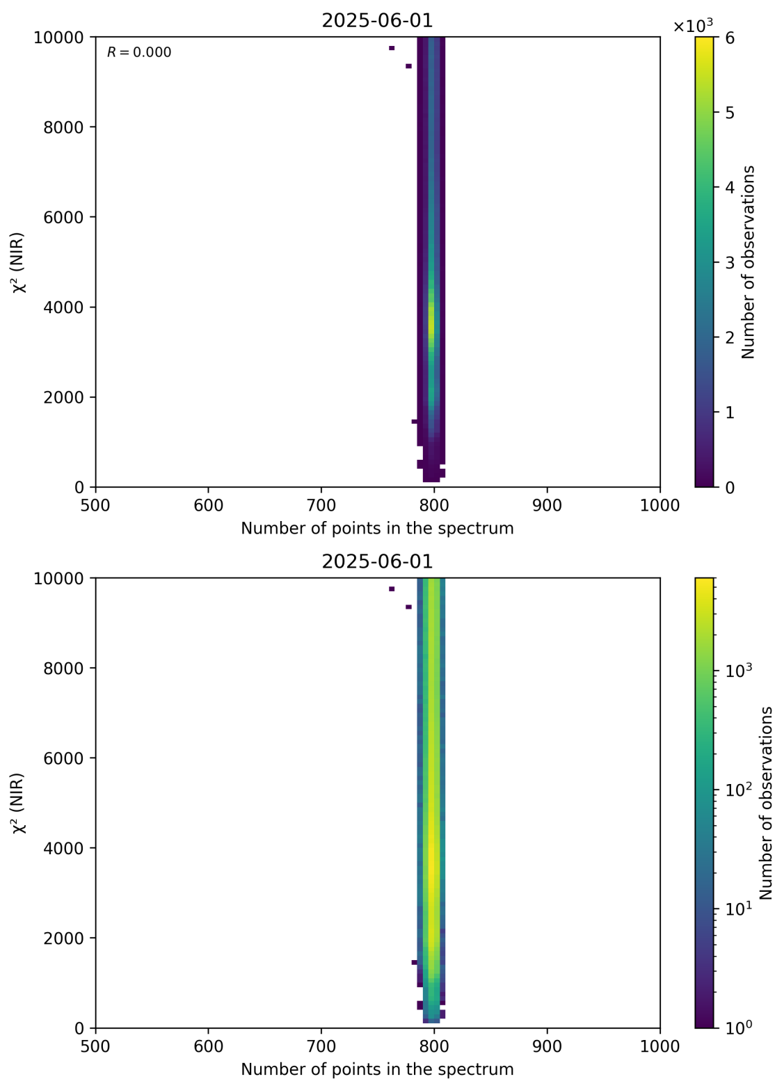
Figure 88: Scatter density plot of “Number of points in the spectrum” against “ \chi^2 (NIR)” for 2025-06-01 to 2025-06-02.
