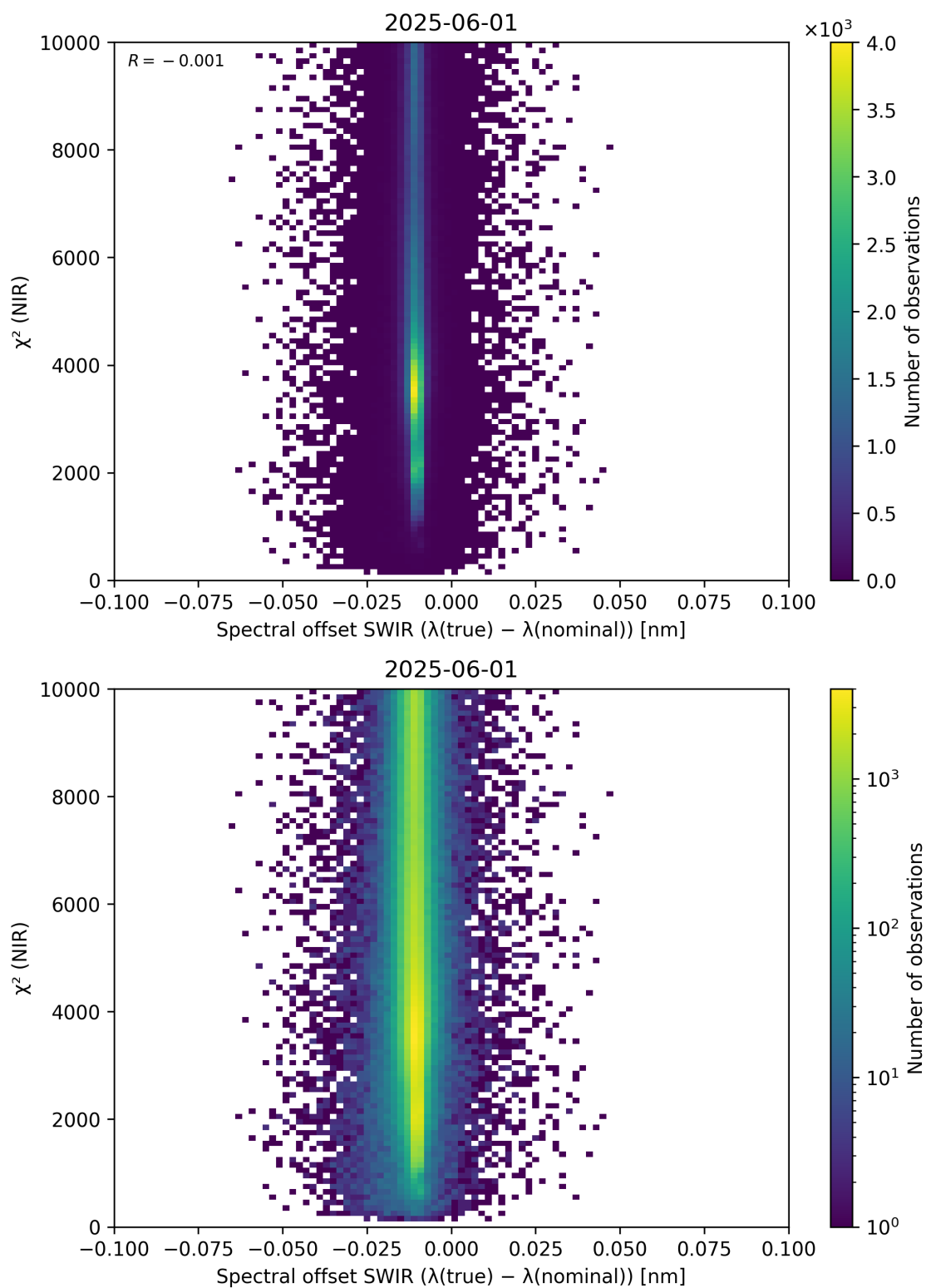
Figure 117: Scatter density plot of “Spectral offset SWIR ( \lambda_{\text{true}} - \lambda_{\text{nominal}} )” against “ \chi^2 (NIR)” for 2025-06-01 to 2025-06-02.
