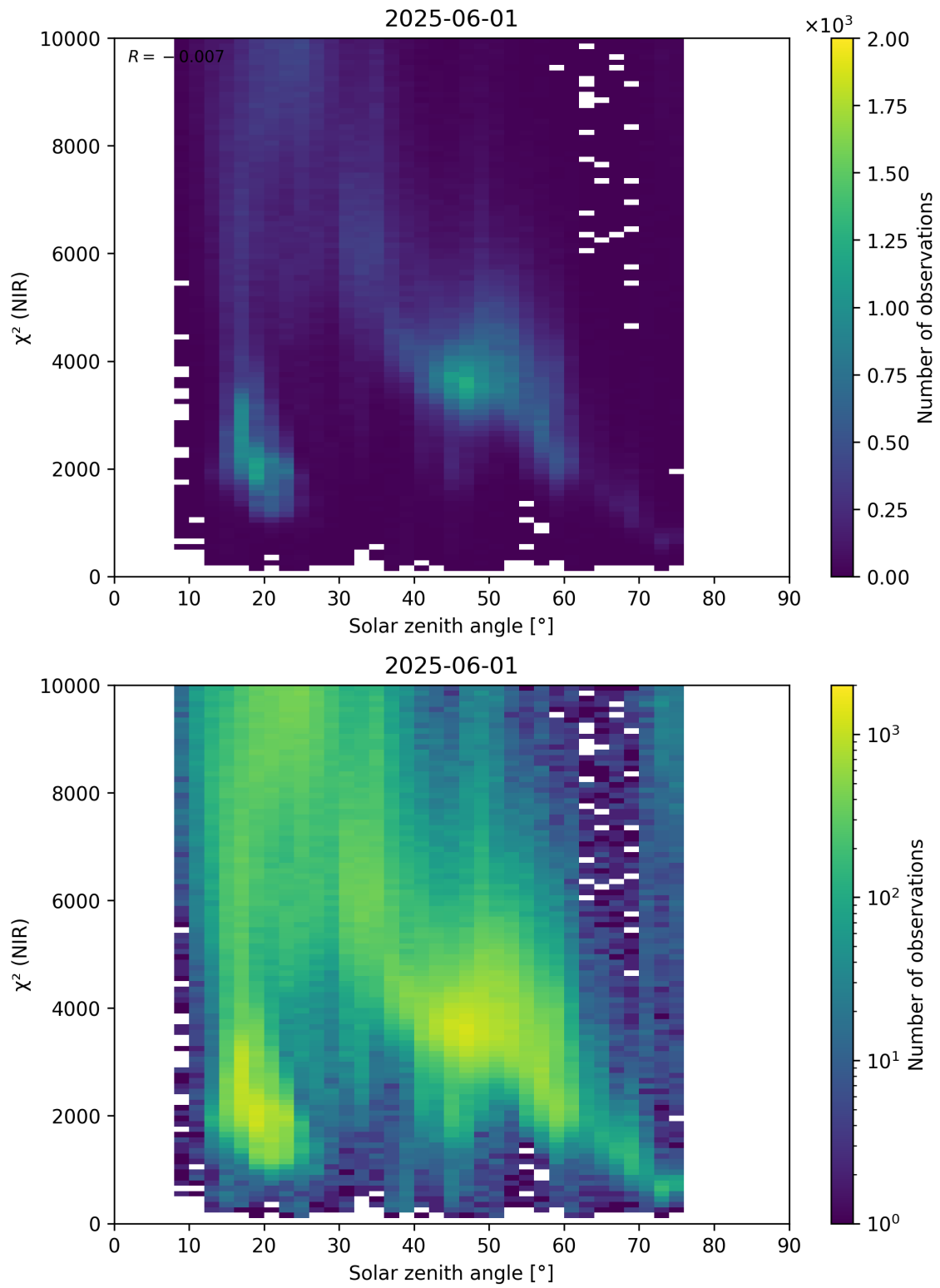
Figure 94: Scatter density plot of “Solar zenith angle” against “ \chi^2 (NIR)” for 2025-06-01 to 2025-06-02.
