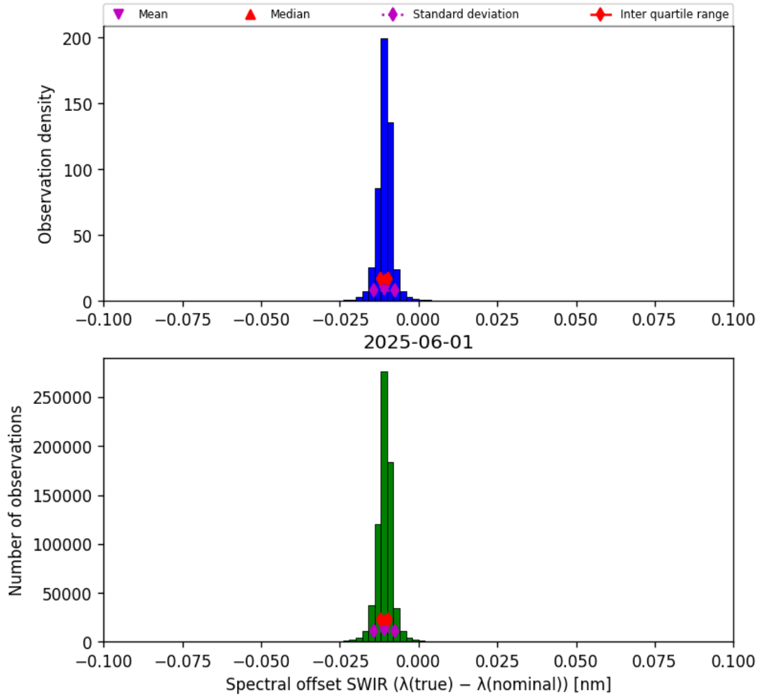
Figure 27: Histogram of “Spectral offset SWIR ( \lambda_{\text{true}} - \lambda_{\text{nominal}} )” for 2025-06-01 to 2025-06-02
