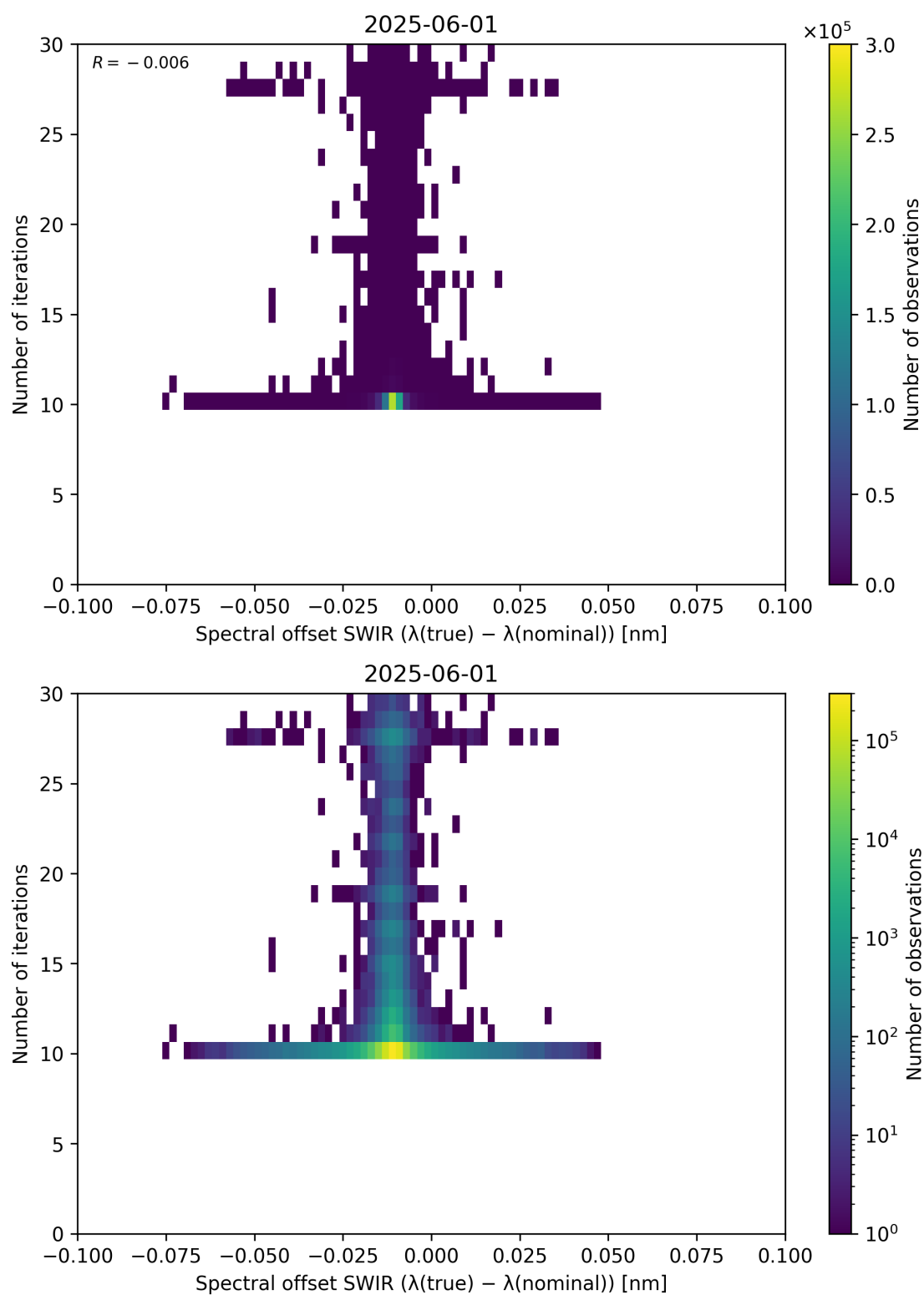
Figure 121: Scatter density plot of “Spectral offset SWIR ( \lambda_{\text{true}} - \lambda_{\text{nominal}} )” against “Number of iterations” for 2025-06-01 to 2025-06-02.
