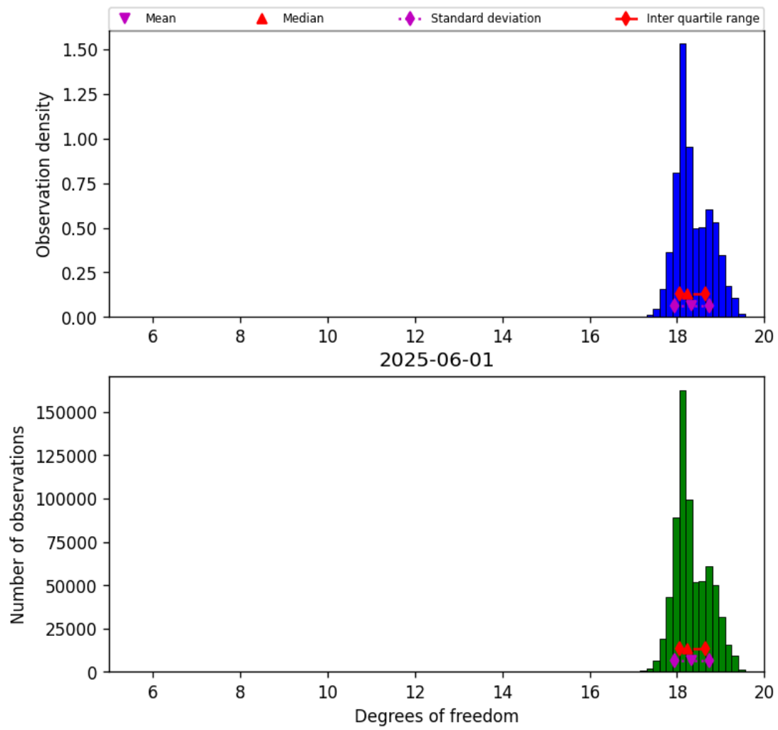
Figure 30: Histogram of “Degrees of freedom” for 2025-06-01 to 2025-06-02
