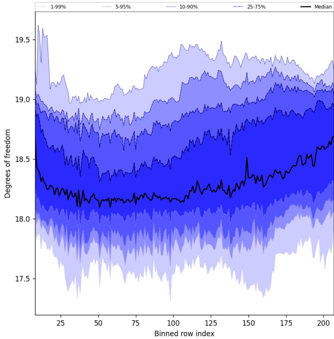
Figure 41: Along track statistics of “Degrees of freedom” for 2025-06-01 to 2025-06-02
