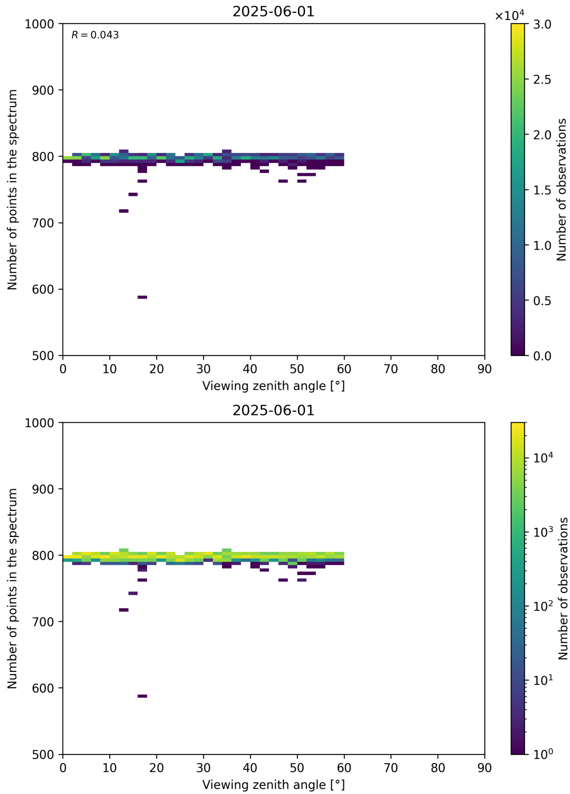
Figure 114: Scatter density plot of “Viewing zenith angle” against “Number of points in the spectrum” for 2025-06-01 to 2025-06-02.
