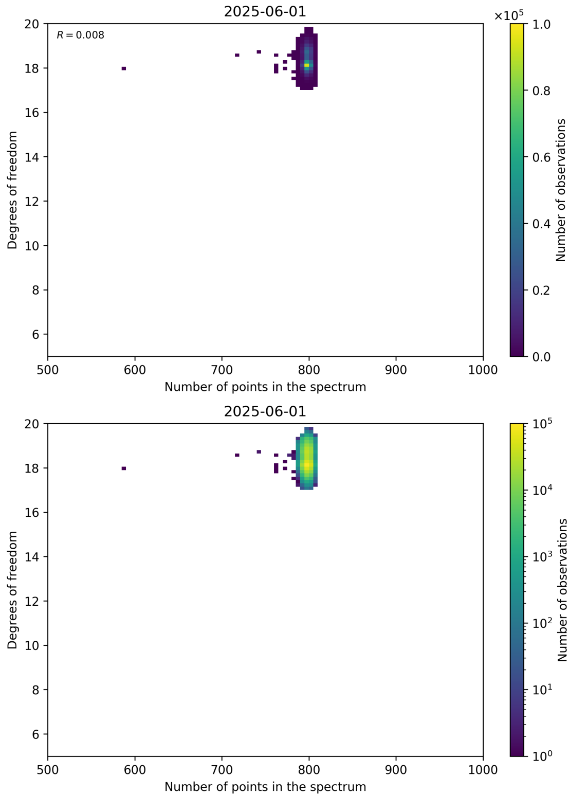
Figure 90: Scatter density plot of “Number of points in the spectrum” against “Degrees of freedom” for 2025-06-01 to 2025-06-02.
