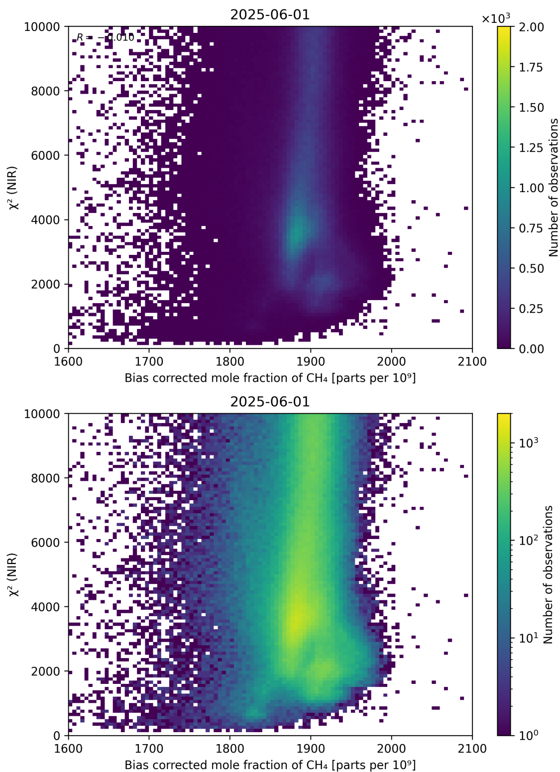
Figure 63: Scatter density plot of “Bias corrected mole fraction of \text{CH}_4 ” against “ \chi^2 (NIR)” for 2025-06-01 to 2025-06-02.
