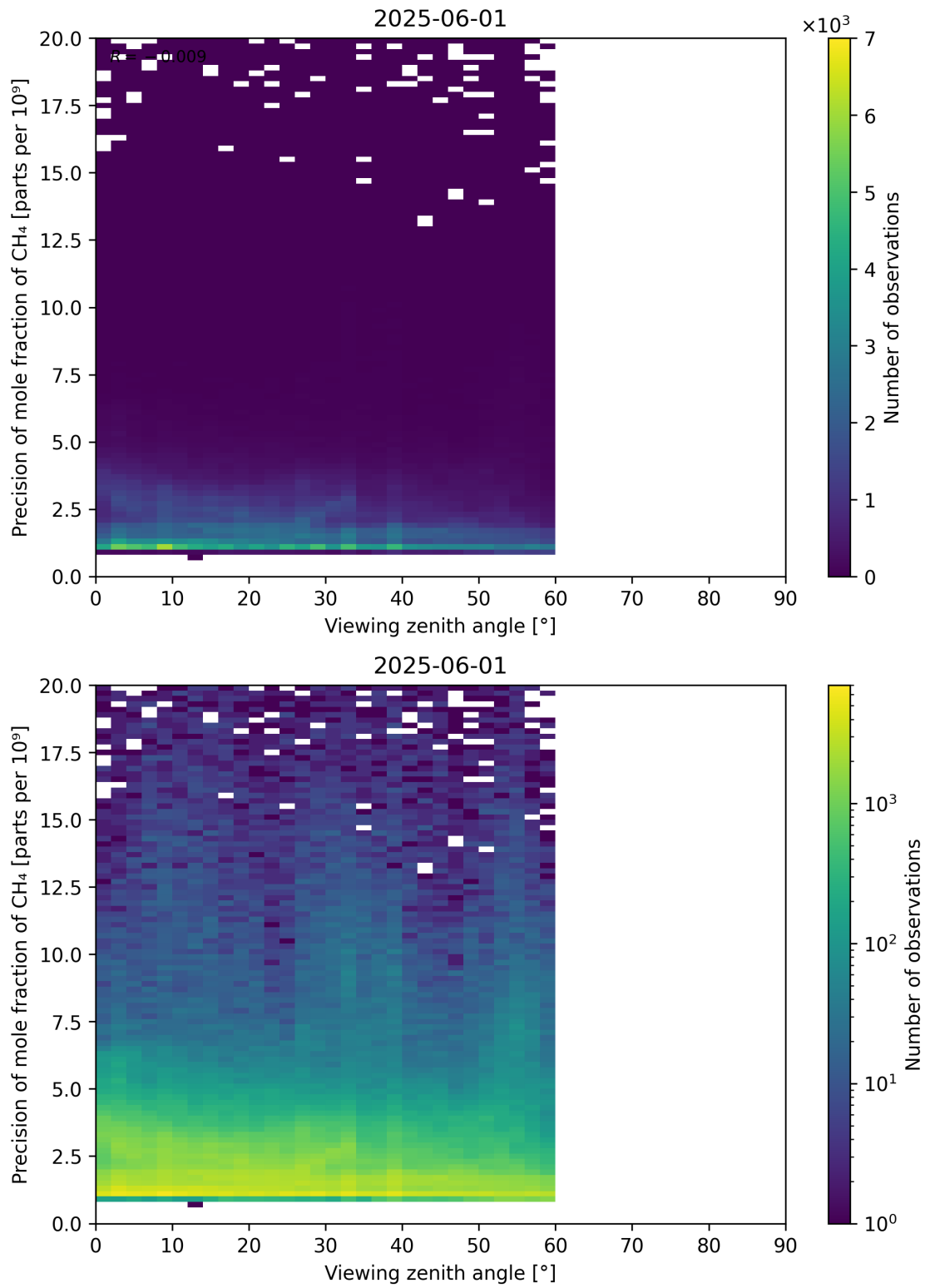
Figure 112: Scatter density plot of “Viewing zenith angle” against “Precision of mole fraction of CH 4 ” for 2025-06-01 to 2025-06-02.
