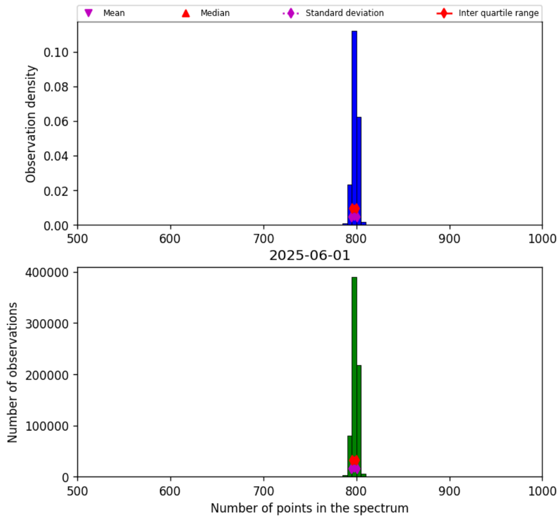
Figure 26: Histogram of “Number of points in the spectrum” for 2025-06-01 to 2025-06-02
