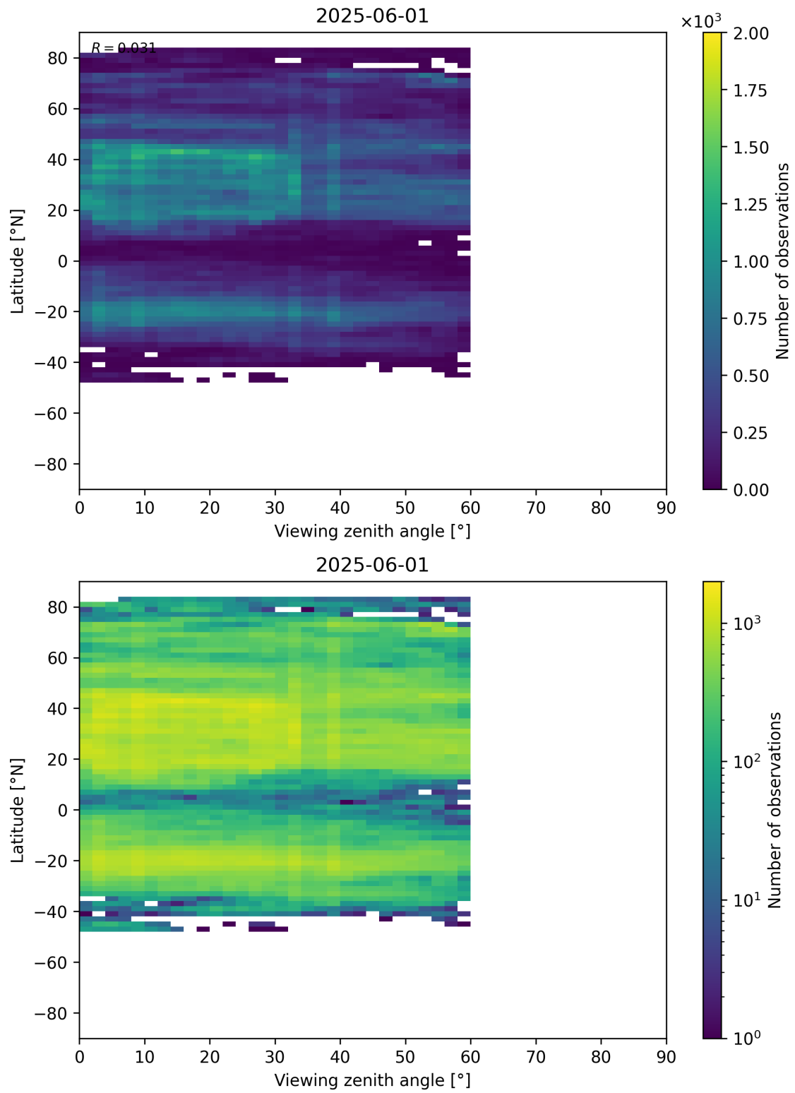
Figure 109: Scatter density plot of “Viewing zenith angle” against “Latitude” for 2025-06-01 to 2025-06-02.
