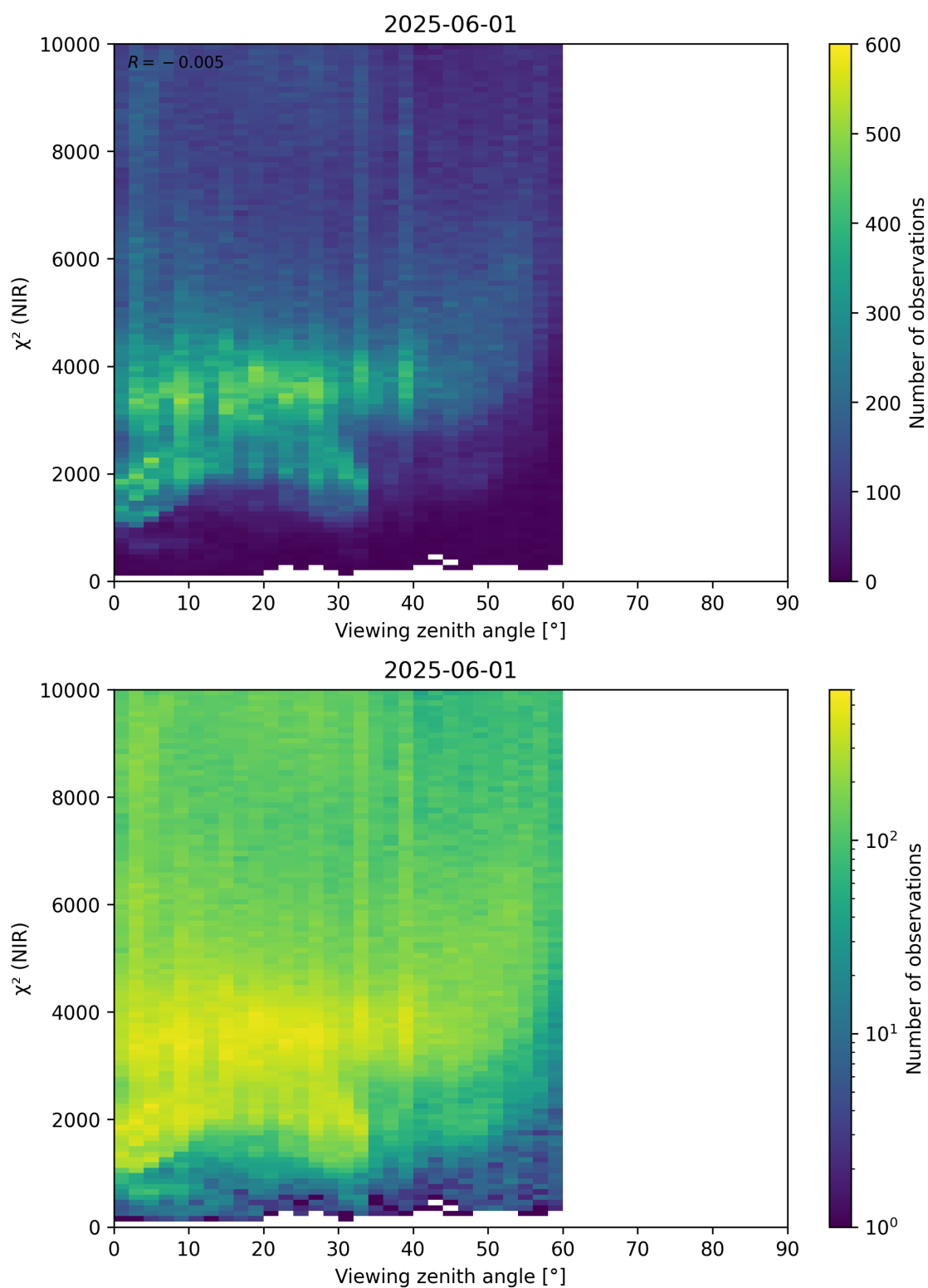
Figure 105: Scatter density plot of “Viewing zenith angle” against “ \chi^2 (NIR)” for 2025-06-01 to 2025-06-02.
