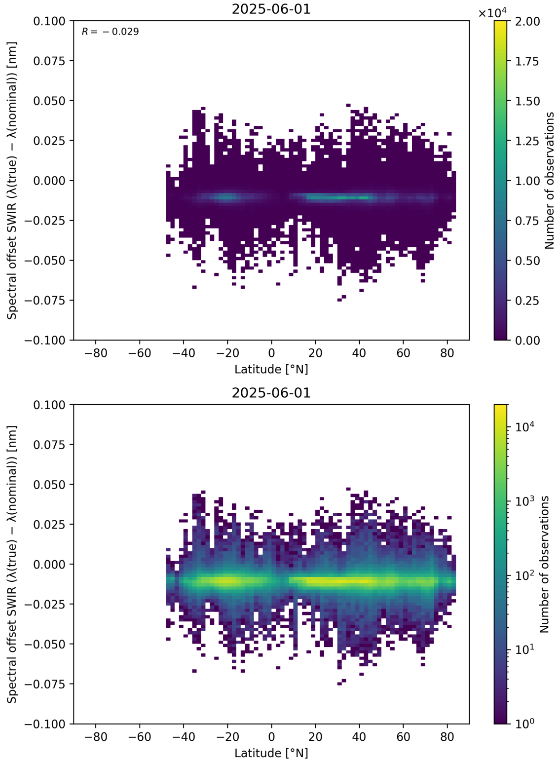
Figure 62: Scatter density plot of “Latitude” against “Spectral offset SWIR ( \lambda_{\text{true}} - \lambda_{\text{nominal}} )” for 2025-06-01 to 2025-06-02.
