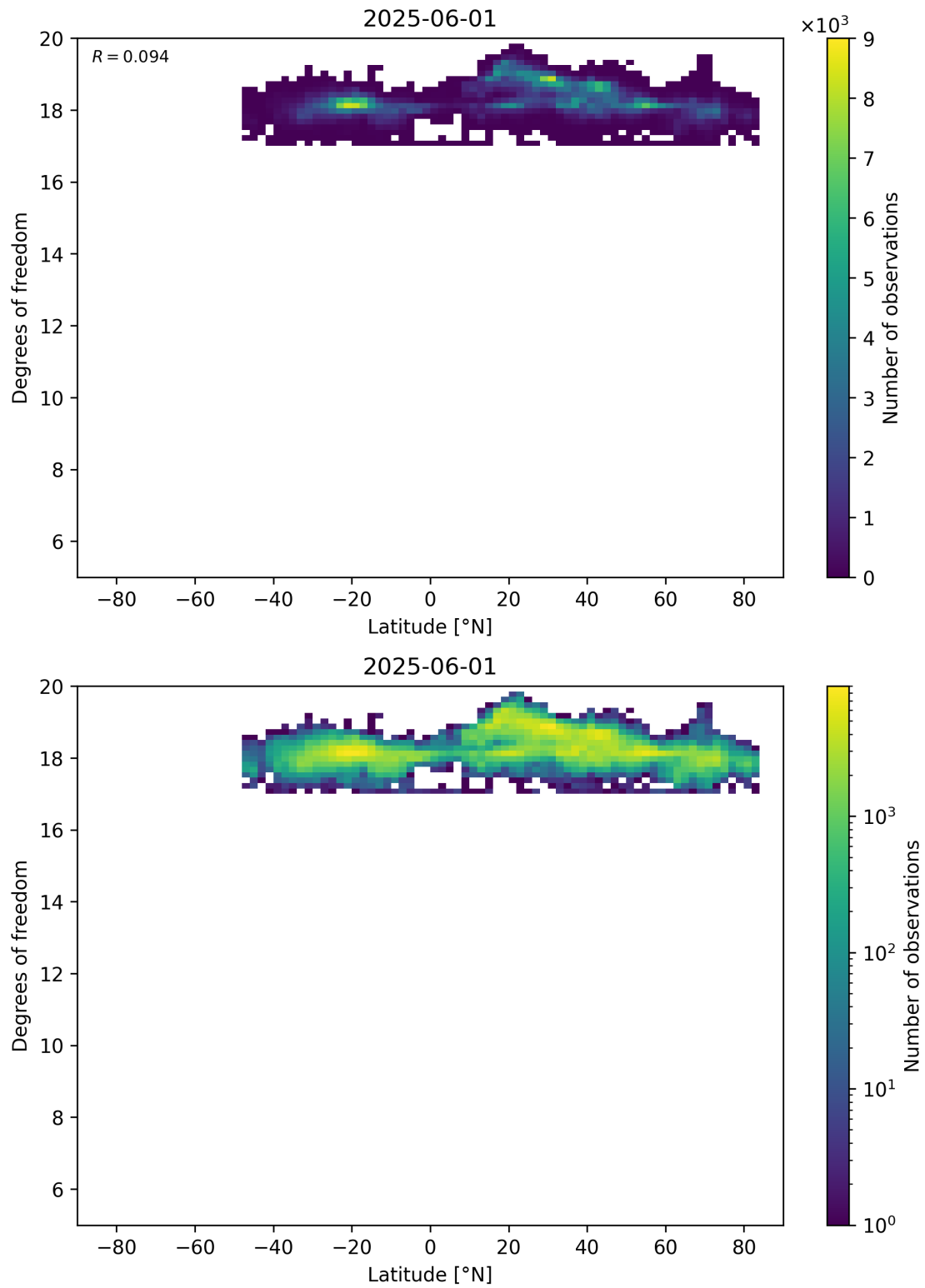
Figure 55: Scatter density plot of “Latitude” against “Degrees of freedom” for 2025-06-01 to 2025-06-02.
