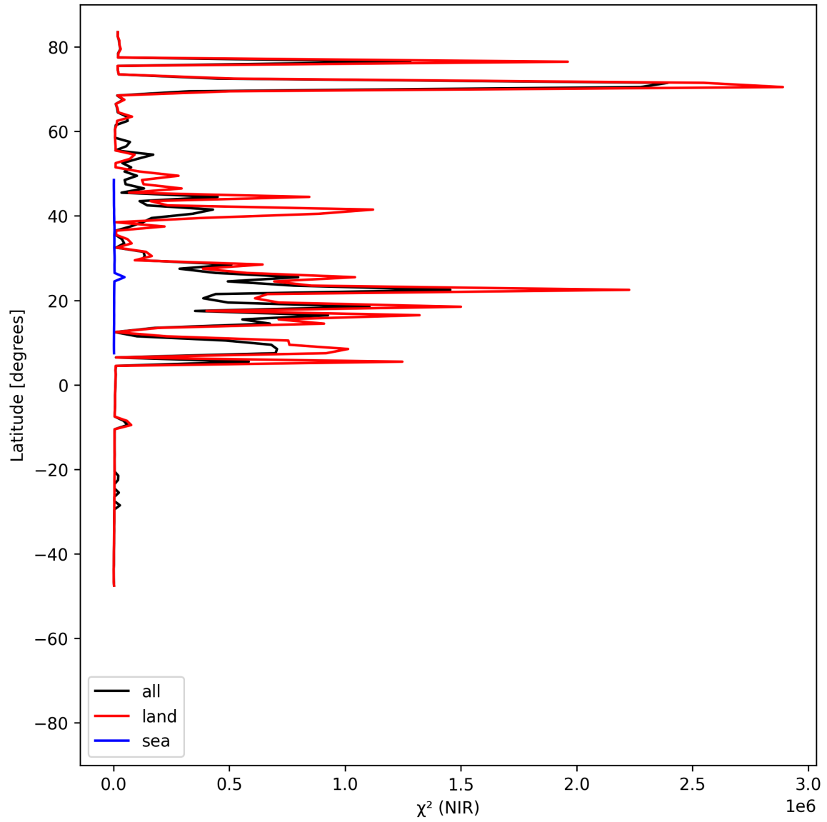
Figure 18: Zonal average of “ \chi^2 (NIR)” for 2025-06-01 to 2025-06-02.
