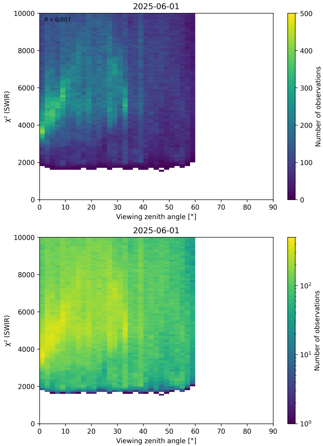
Figure 106: Scatter density plot of “Viewing zenith angle” against “ \chi^2 (SWIR)” for 2025-06-01 to 2025-06-02.
