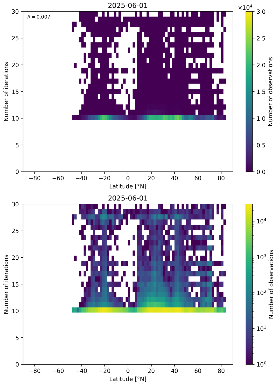
Figure 60: Scatter density plot of “Latitude” against “Number of iterations” for 2025-06-01 to 2025-06-02.
