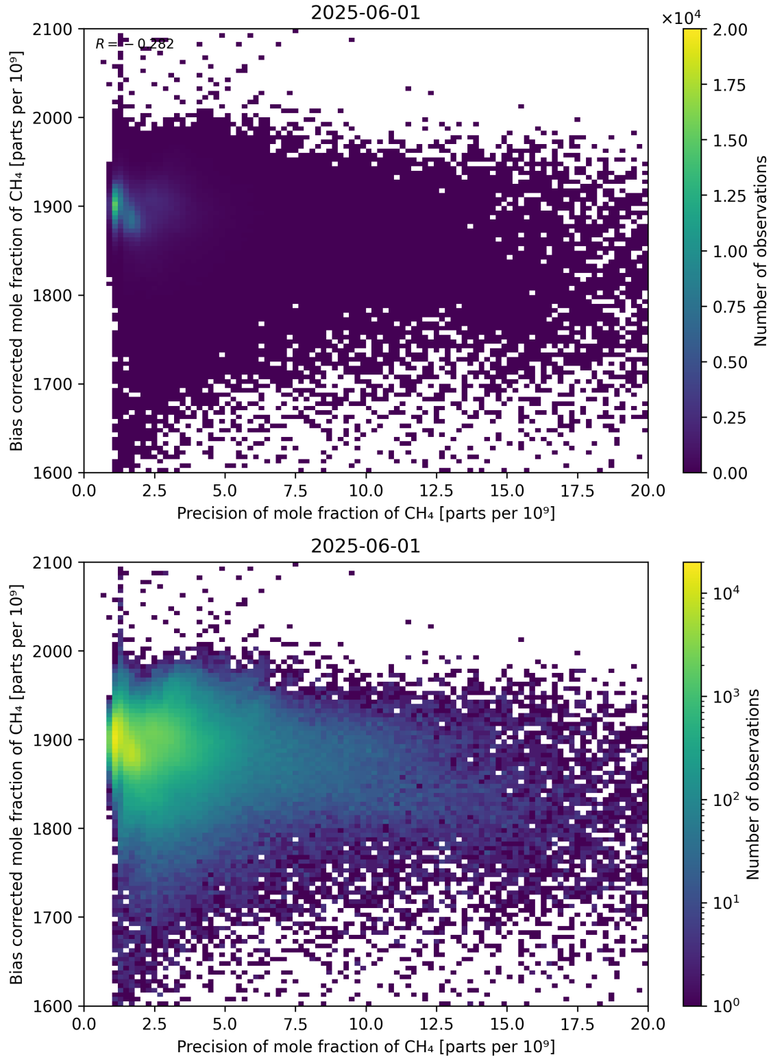
Figure 82: Scatter density plot of “Precision of mole fraction of CH 4 ” against “Bias corrected mole fraction of CH 4 ” for 2025-06-01 to 2025-06-02.
