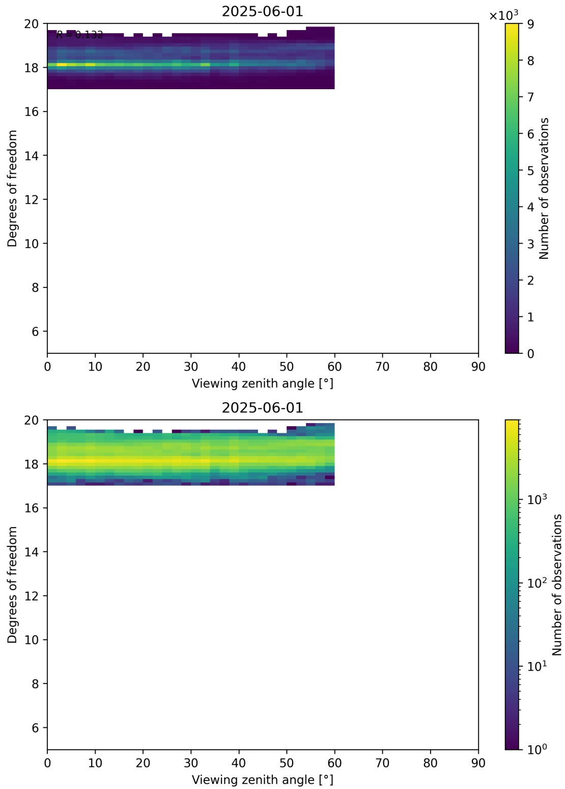
Figure 107: Scatter density plot of “Viewing zenith angle” against “Degrees of freedom” for 2025-06-01 to 2025-06-02.
