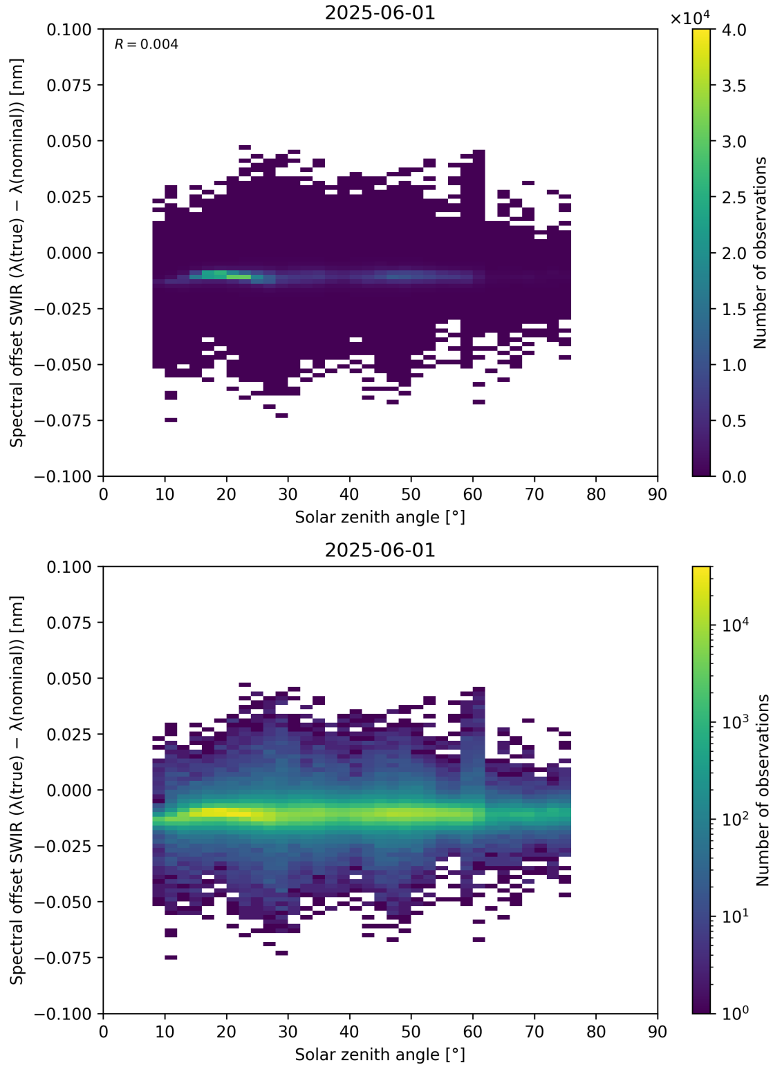
Figure 104: Scatter density plot of “Solar zenith angle” against “Spectral offset SWIR ( \lambda_{\text{true}} - \lambda_{\text{nominal}} )” for 2025-06-01 to 2025-06-02.
