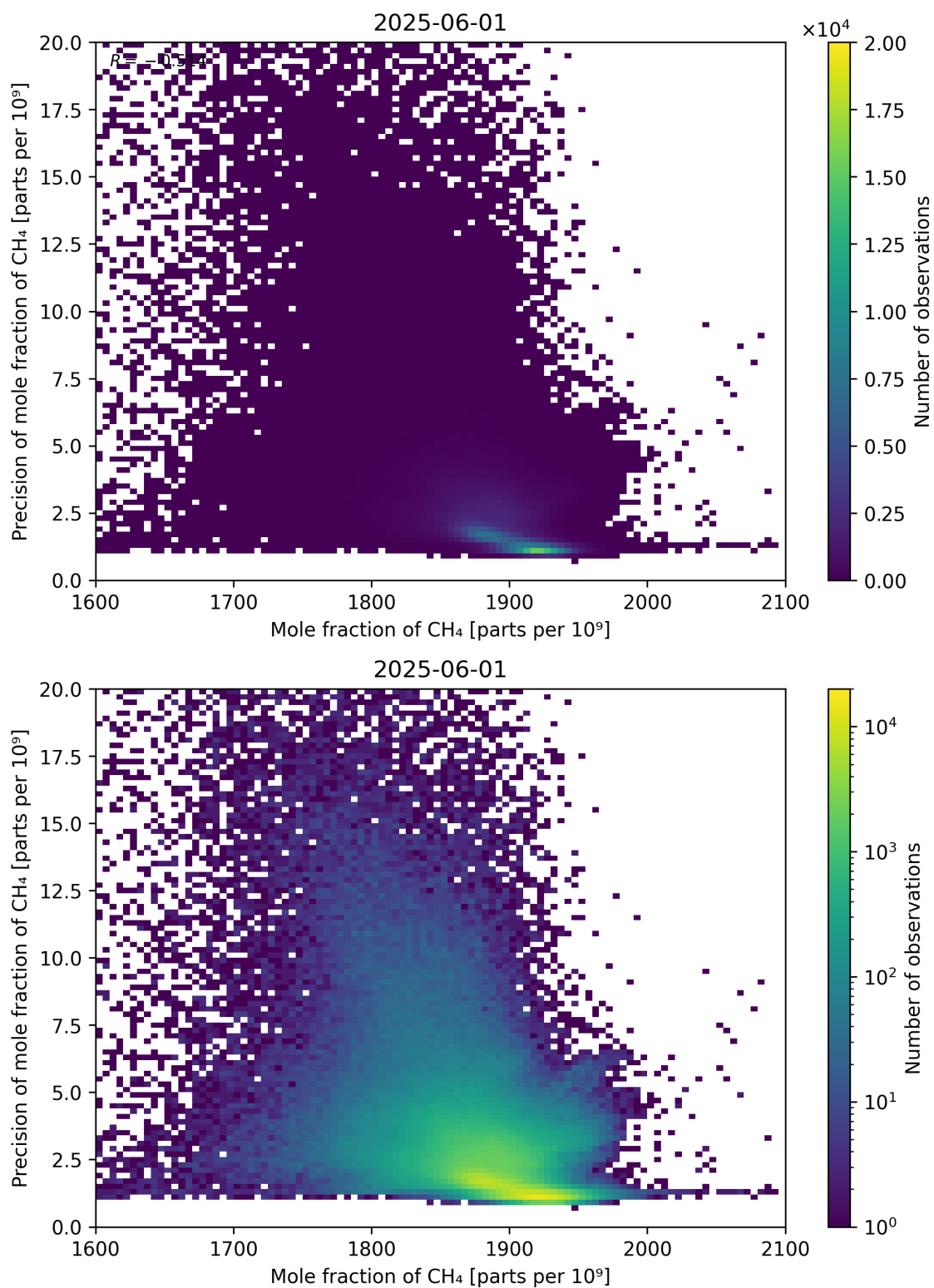
Figure 75: Scatter density plot of “Mole fraction of CH 4 ” against “Precision of mole fraction of CH 4 ” for 2025-06-01 to 2025-06-02.
