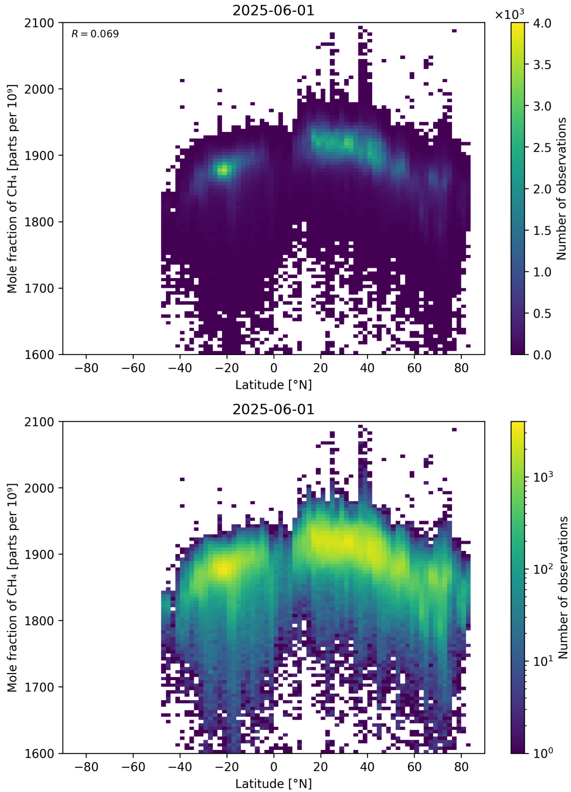
Figure 57: Scatter density plot of “Latitude” against “Mole fraction of CH 4 ” for 2025-06-01 to 2025-06-02.
