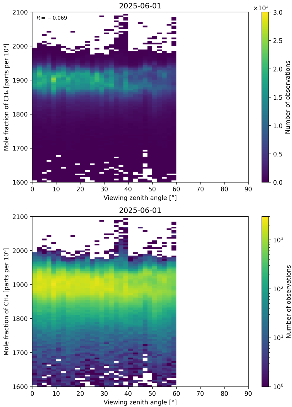
Figure 110: Scatter density plot of “Viewing zenith angle” against “Mole fraction of CH 4 ” for 2025-06-01 to 2025-06-02.
