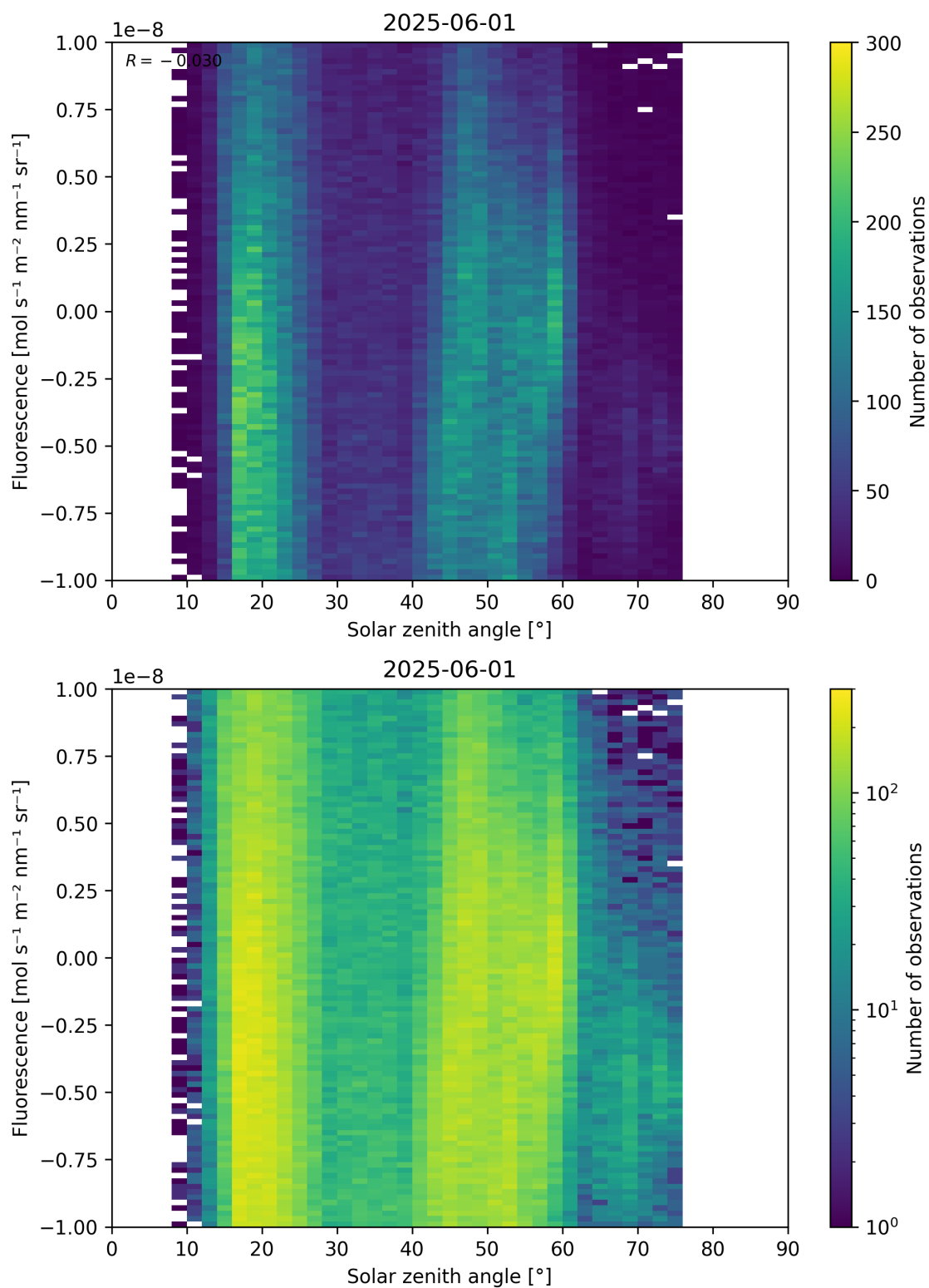
Figure 97: Scatter density plot of “Solar zenith angle” against “Fluorescence” for 2025-06-01 to 2025-06-02.
