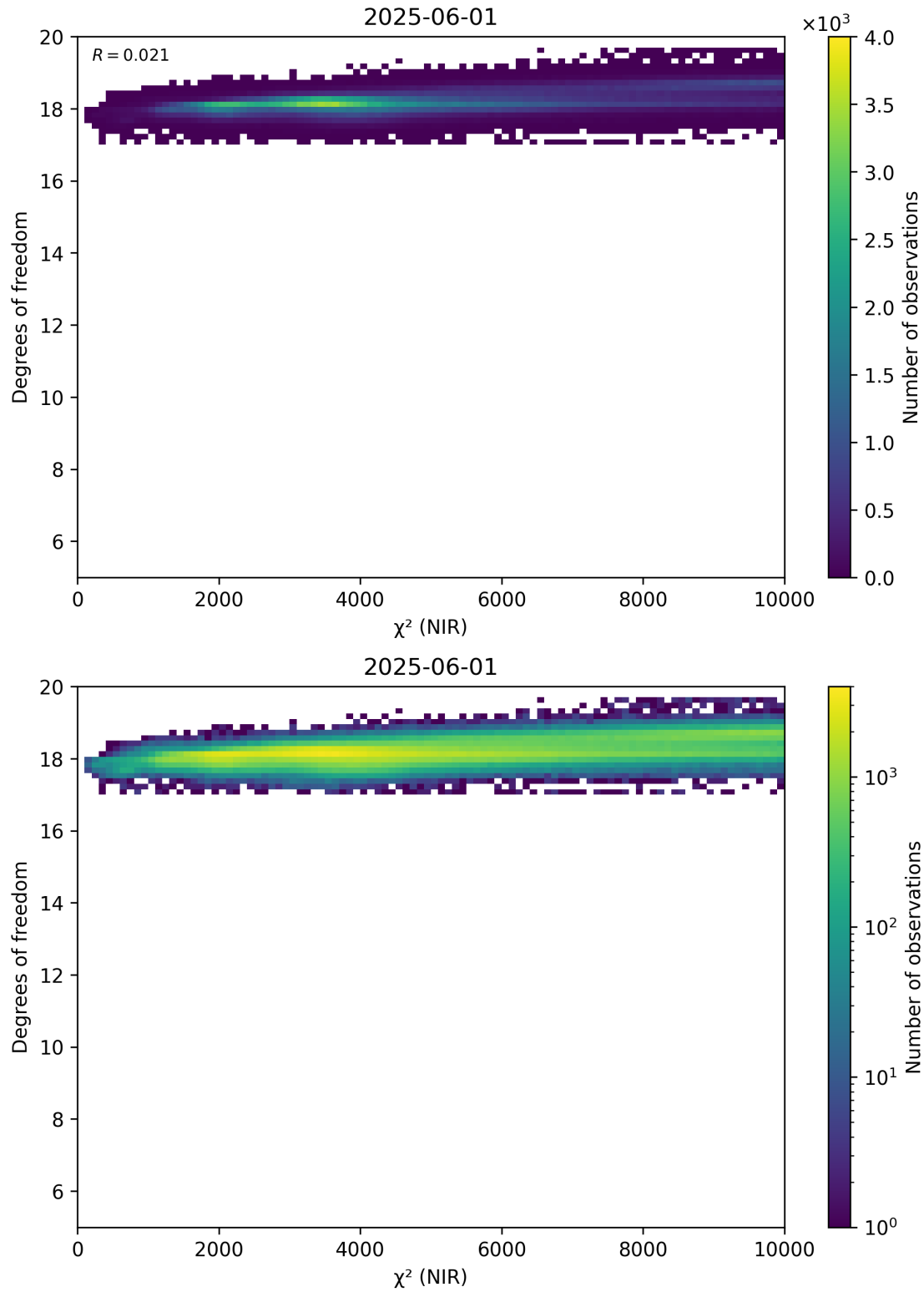
Figure 44: Scatter density plot of “ \chi^2 (NIR)” against “Degrees of freedom” for 2025-06-01 to 2025-06-02.
