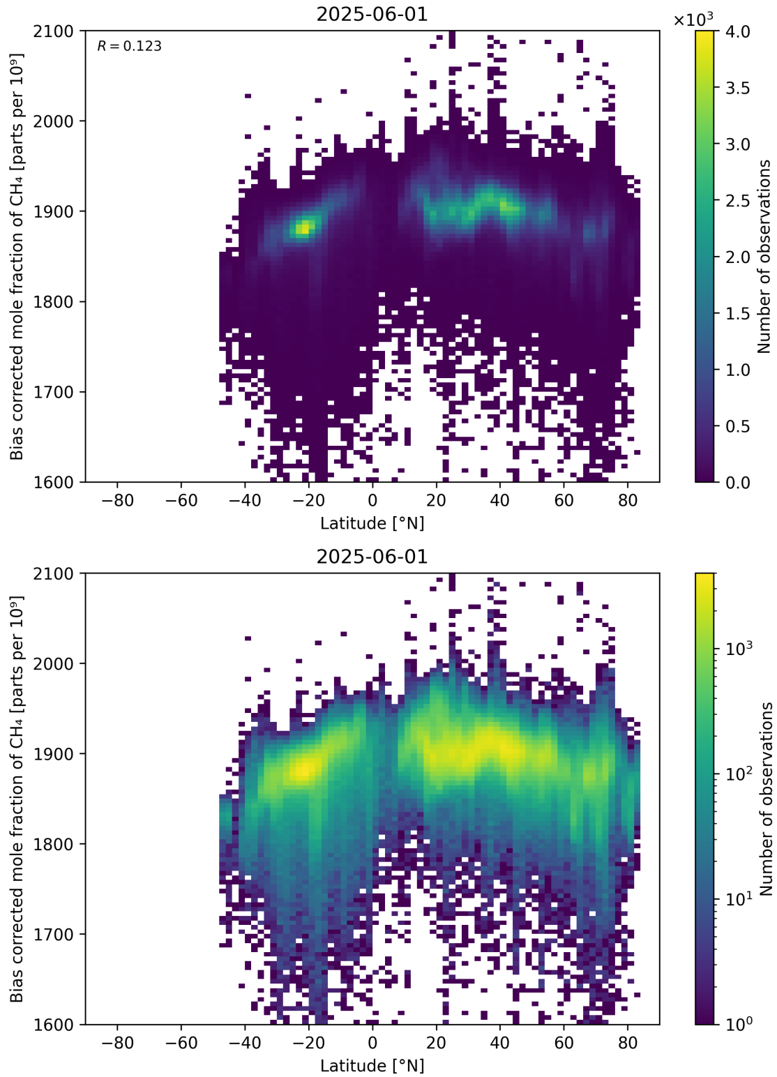
Figure 58: Scatter density plot of “Latitude” against “Bias corrected mole fraction of CH 4 ” for 2025-06-01 to 2025-06-02.
