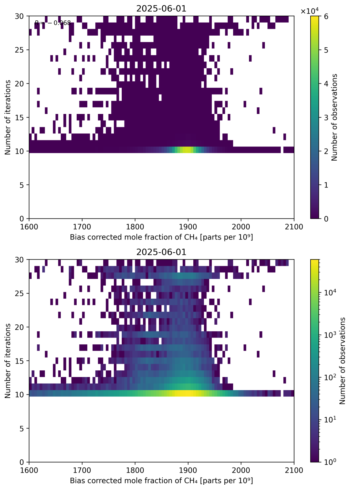
Figure 67: Scatter density plot of “Bias corrected mole fraction of CH 4 ” against “Number of iterations” for 2025-06-01 to 2025-06-02.
