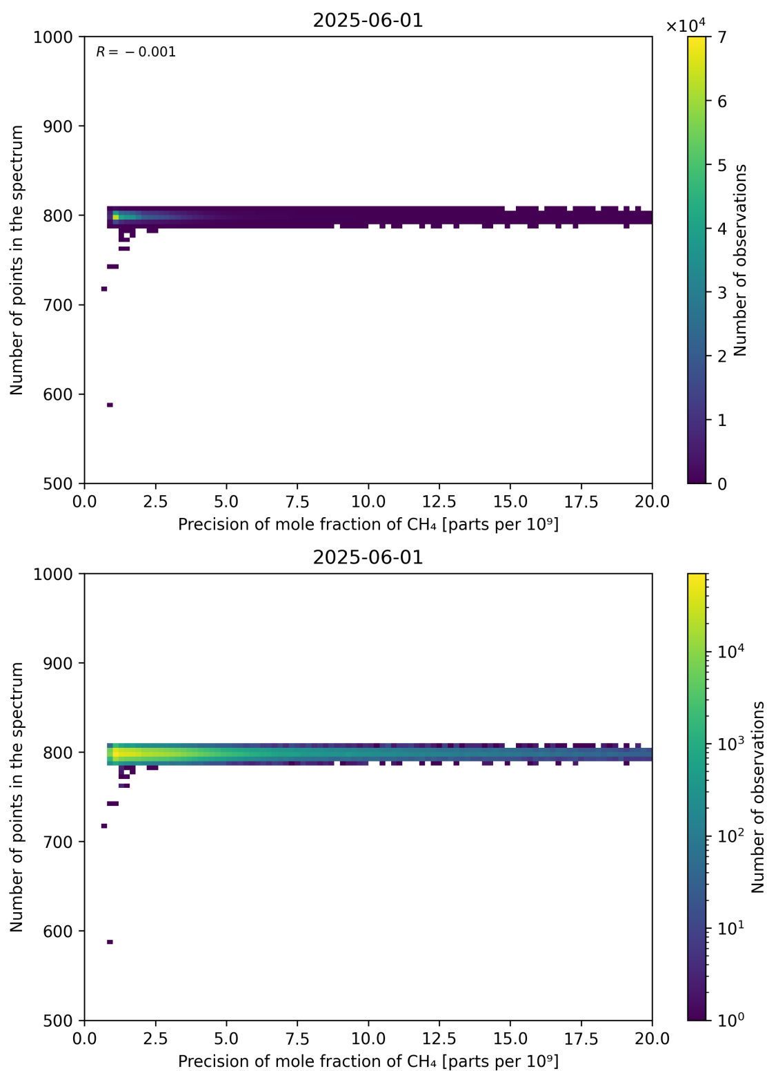
Figure 84: Scatter density plot of “Precision of mole fraction of CH 4 ” against “Number of points in the spectrum” for 2025-06-01 to 2025-06-02.
