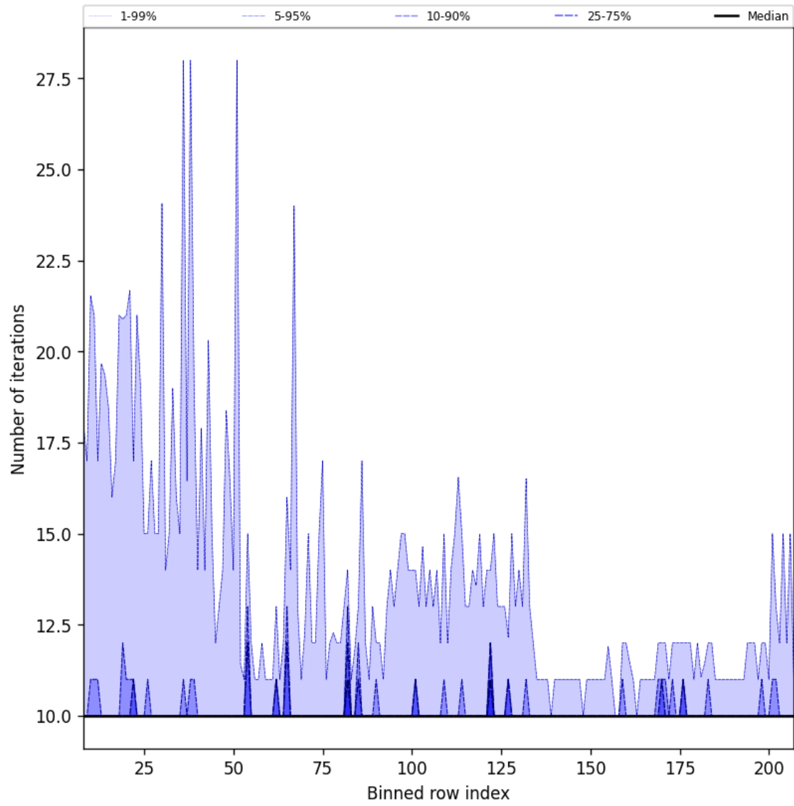
Figure 42: Along track statistics of “Number of iterations” for 2025-06-01 to 2025-06-02
