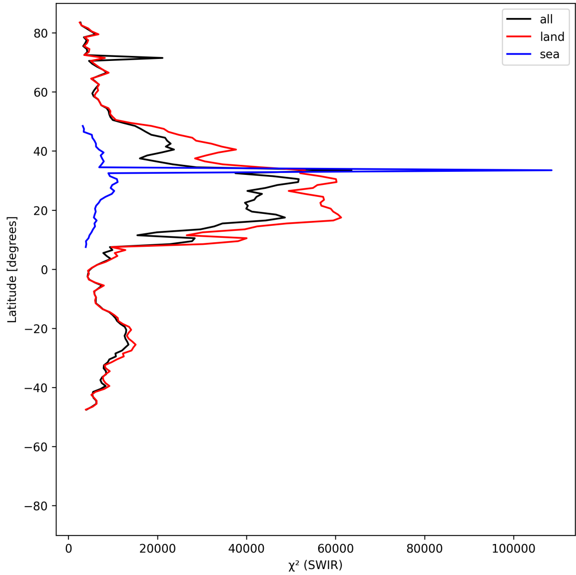
Figure 17: Zonal average of “ \chi^2 (SWIR)” for 2025-06-01 to 2025-06-02.
