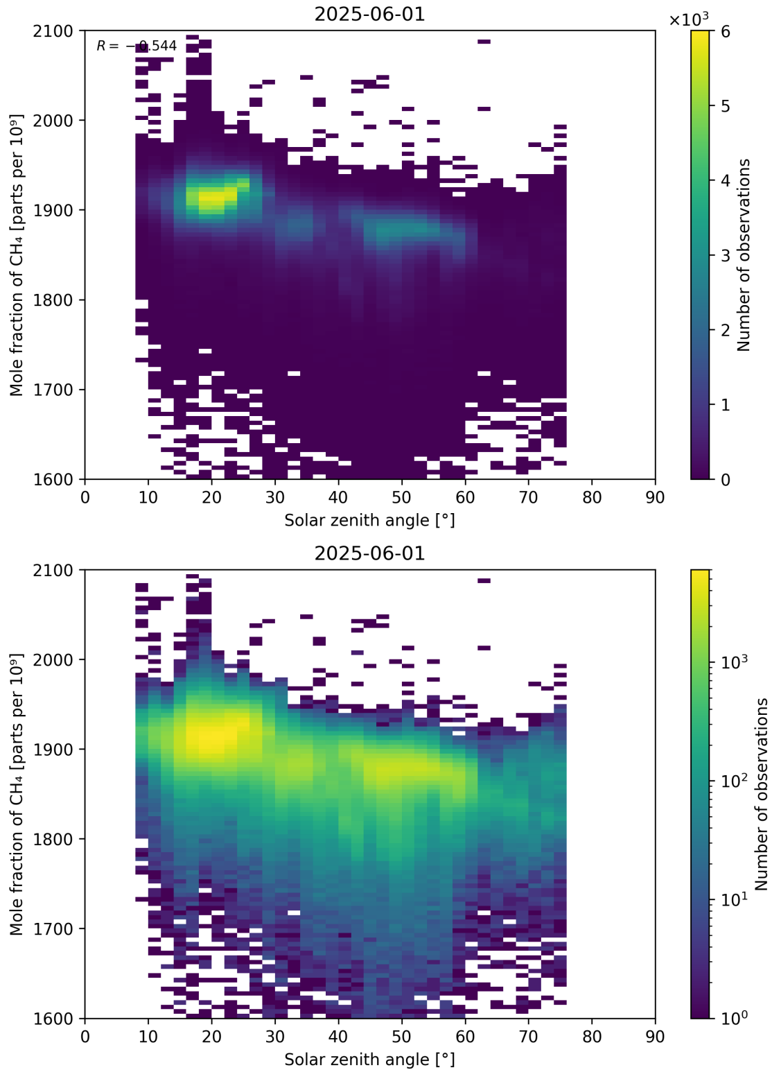
Figure 99: Scatter density plot of “Solar zenith angle” against “Mole fraction of CH 4 ” for 2025-06-01 to 2025-06-02.
