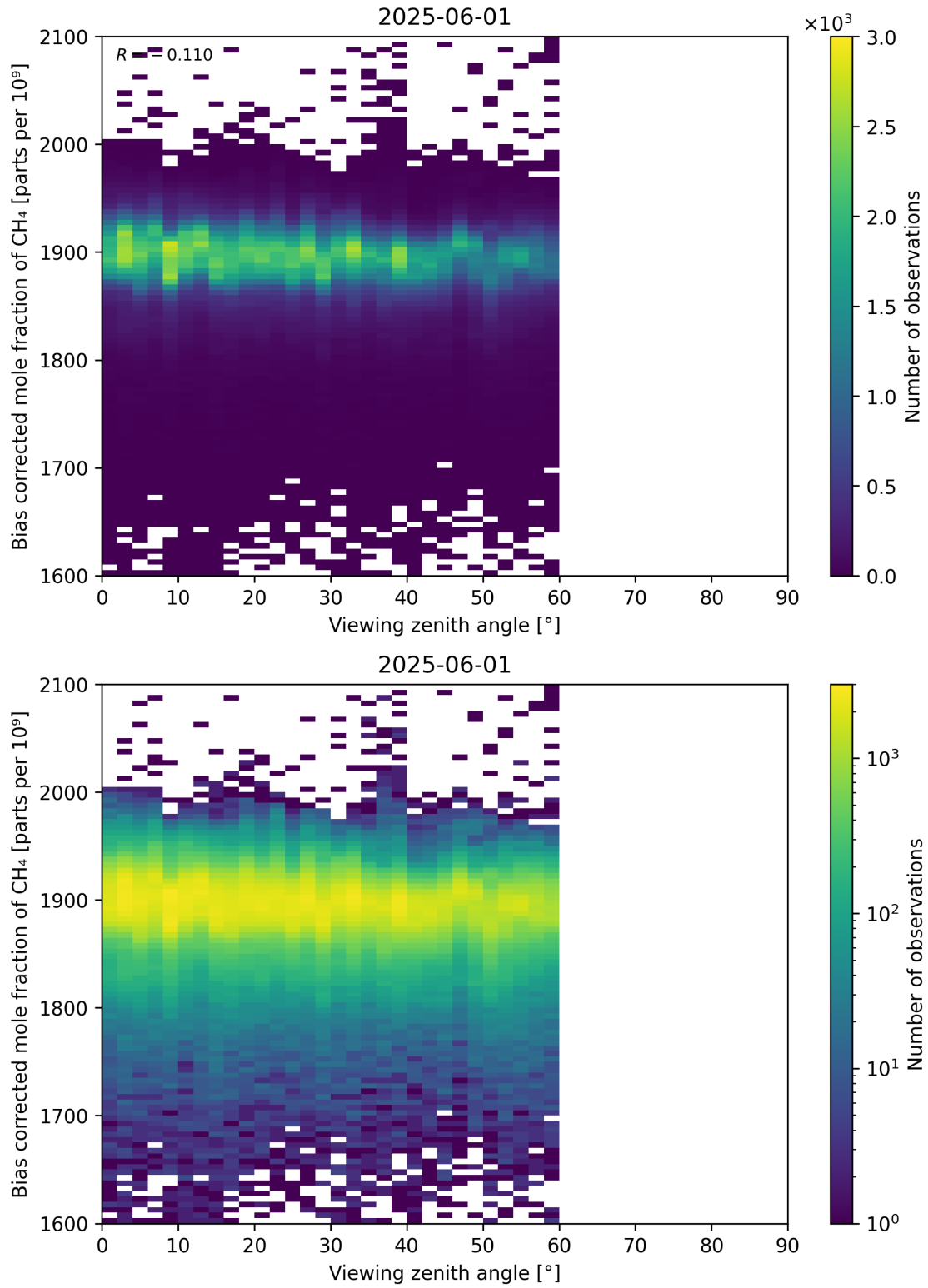
Figure 111: Scatter density plot of “Viewing zenith angle” against “Bias corrected mole fraction of CH 4 ” for 2025-06-01 to 2025-06-02.
