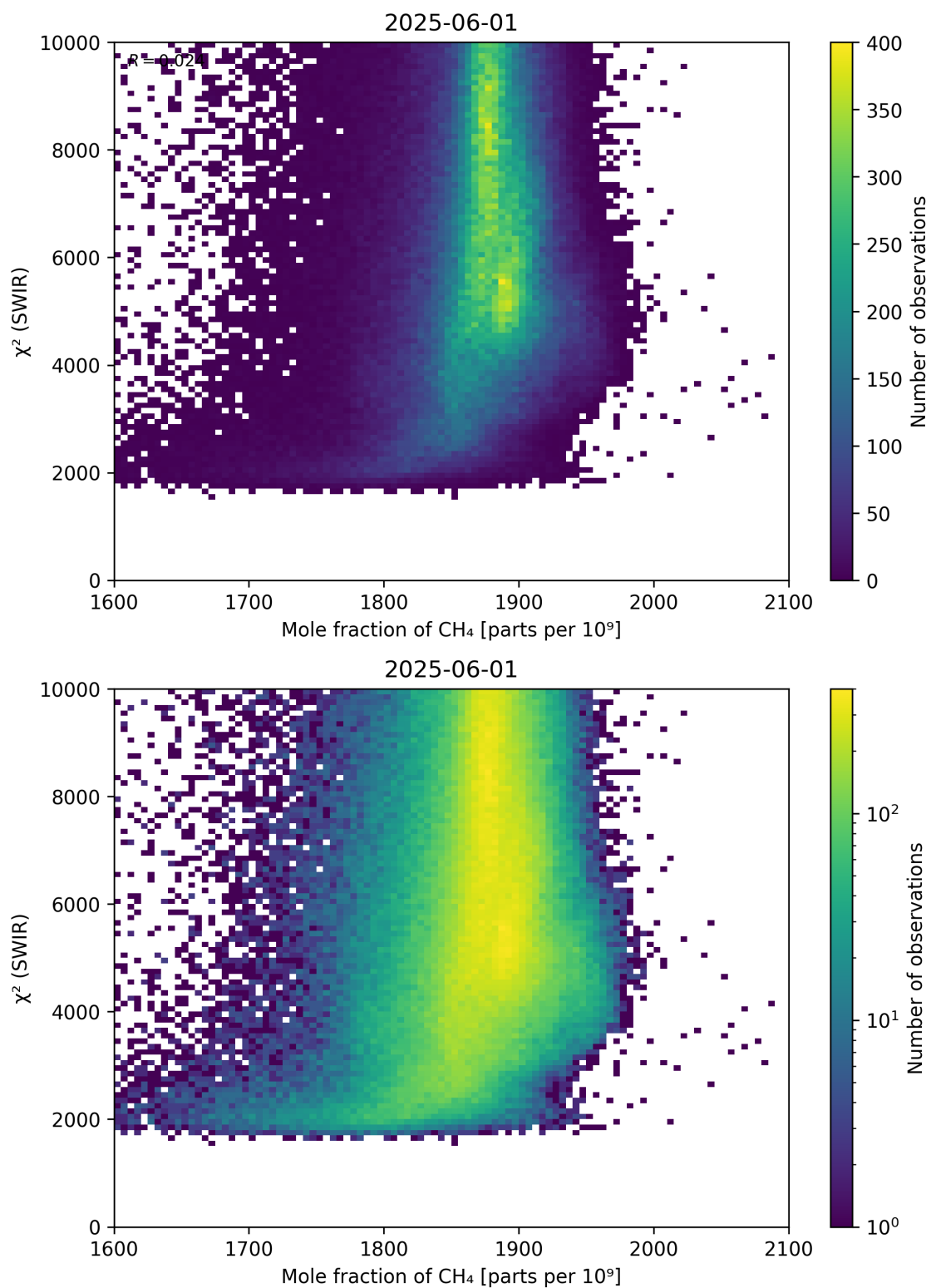
Figure 71: Scatter density plot of “Mole fraction of \text{CH}_4 ” against “ \chi^2 (SWIR)” for 2025-06-01 to 2025-06-02.
