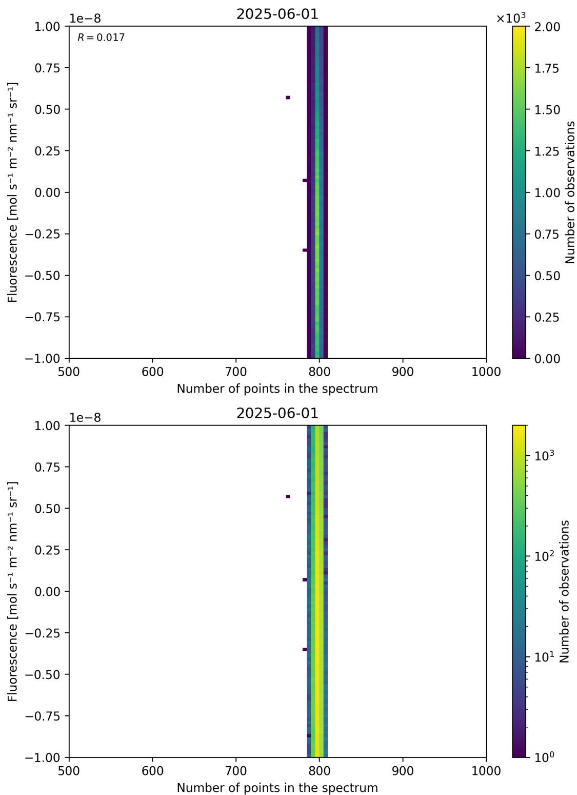
Figure 91: Scatter density plot of “Number of points in the spectrum” against “Fluorescence” for 2025-06-01 to 2025-06-02.
