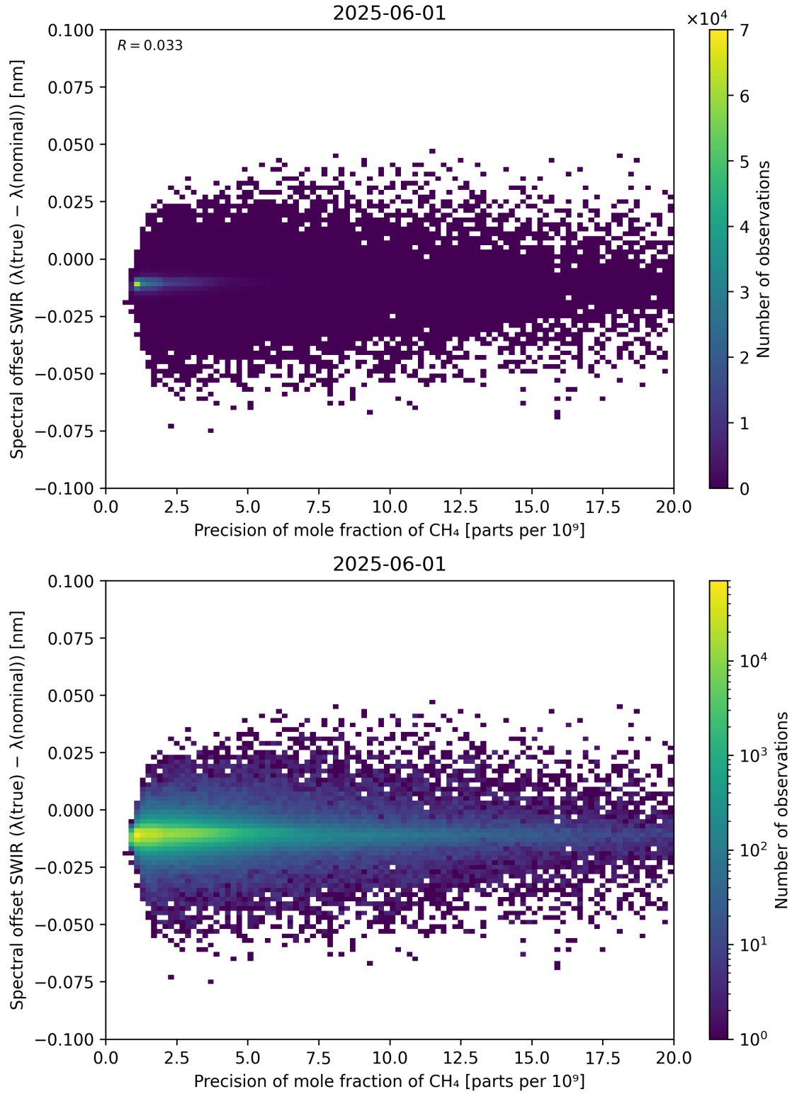
Figure 85: Scatter density plot of “Precision of mole fraction of \text{CH}_4 ” against “Spectral offset SWIR ( \lambda_{\text{true}} - \lambda_{\text{nominal}} )” for 2025-06-01 to 2025-06-02.
