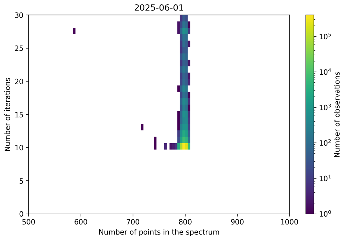
Figure 92: Scatter density plot of “Number of points in the spectrum” against “Number of iterations” for 2025-06-01 to 2025-06-02.
