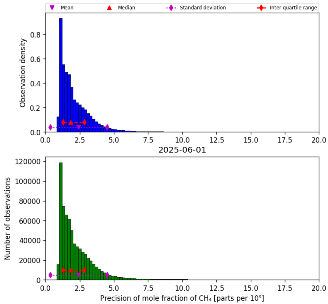
Figure 24: Histogram of “Precision of mole fraction of CH 4 ” for 2025-06-01 to 2025-06-02
