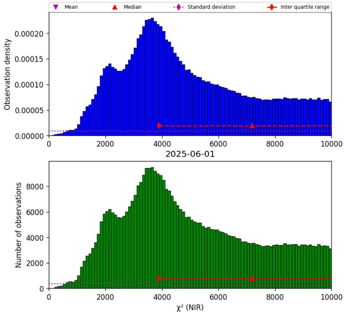
Figure 29: Histogram of " \chi^2 (NIR)" for 2025-06-01 to 2025-06-02
