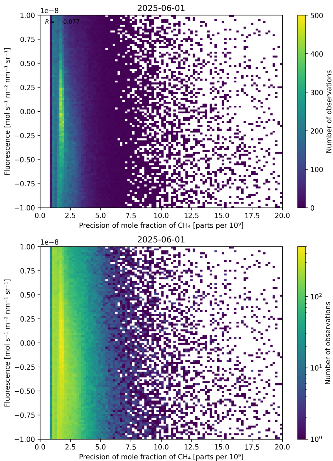
Figure 81: Scatter density plot of “Precision of mole fraction of \text{CH}_4 ” against “Fluorescence” for 2025-06-01 to 2025-06-02.
