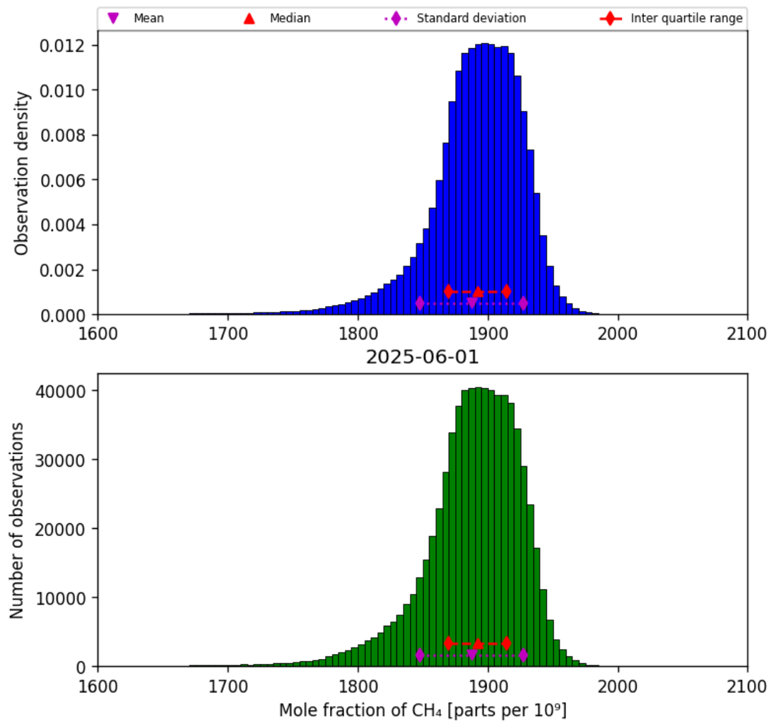
Figure 23: Histogram of “Mole fraction of CH 4 ” for 2025-06-01 to 2025-06-02
