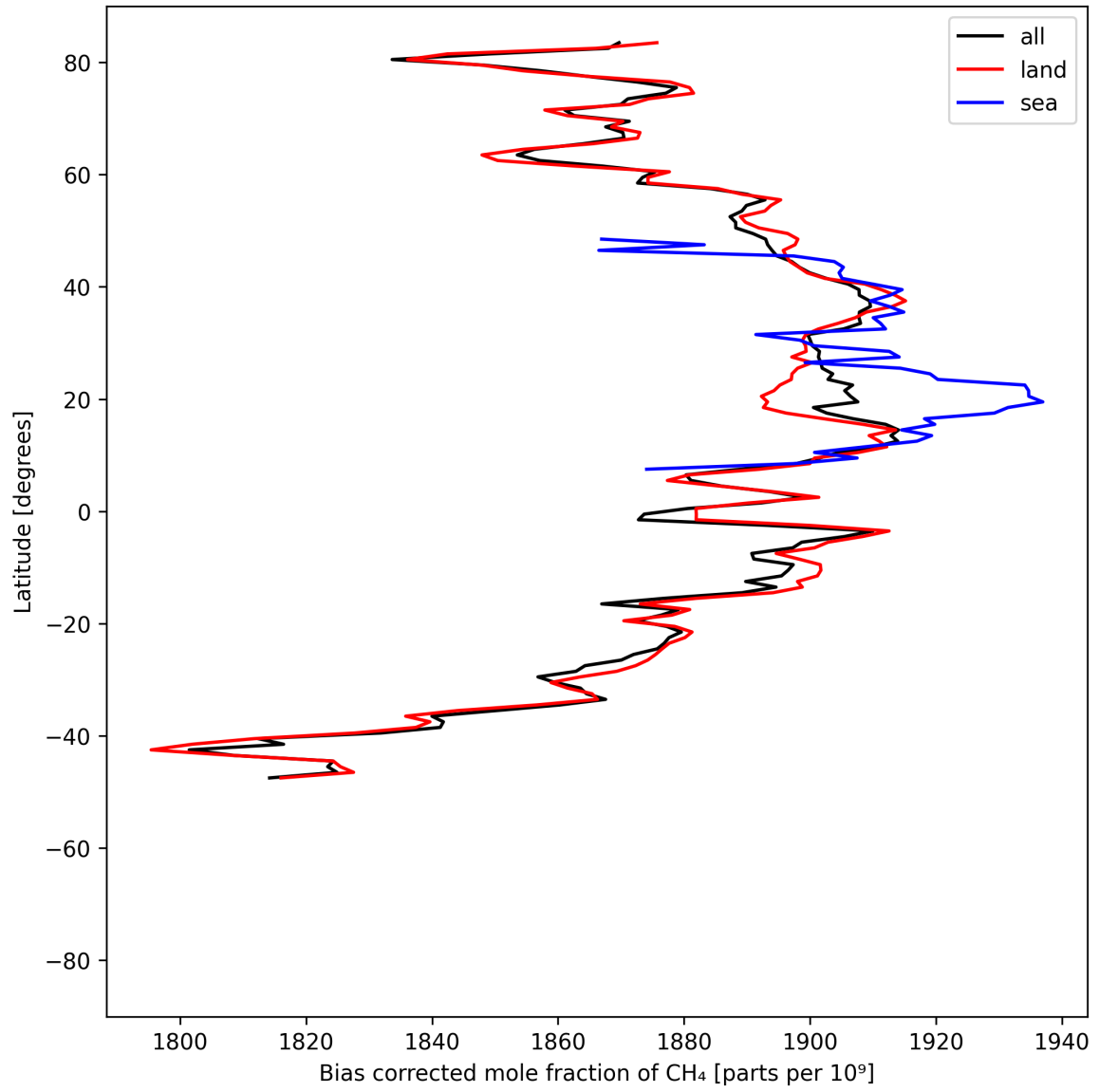
Figure 14: Zonal average of “Bias corrected mole fraction of CH 4 ” for 2025-06-01 to 2025-06-02.
