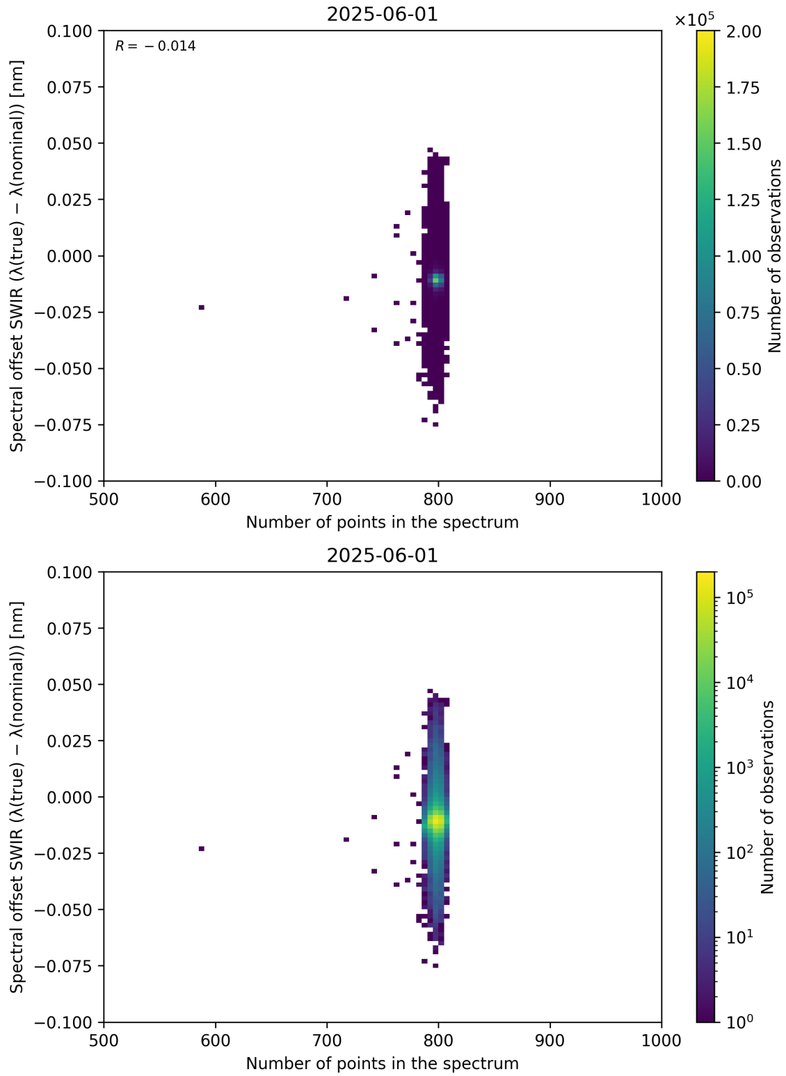
Figure 93: Scatter density plot of “Number of points in the spectrum” against “Spectral offset SWIR ( \lambda_{\text{true}} - \lambda_{\text{nominal}} )” for 2025-06-01 to 2025-06-02.
