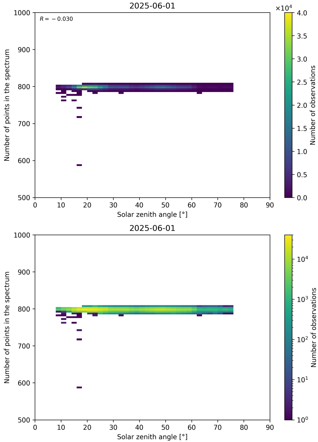
Figure 103: Scatter density plot of “Solar zenith angle” against “Number of points in the spectrum” for 2025-06-01 to 2025-06-02.
