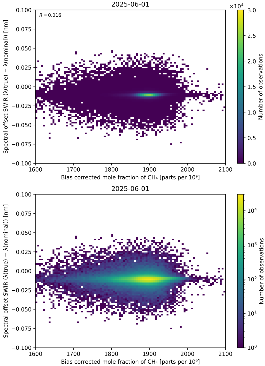
Figure 69: Scatter density plot of “Bias corrected mole fraction of \text{CH}_4 ” against “Spectral offset SWIR ( \lambda_{\text{true}} - \lambda_{\text{nominal}} )” for 2025-06-01 to 2025-06-02.
