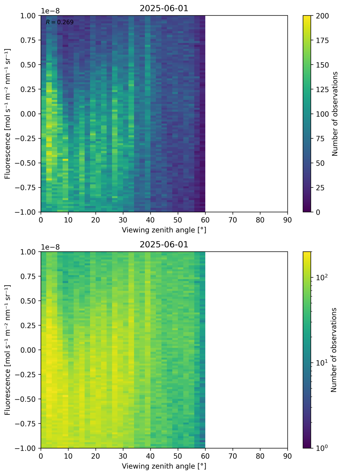
Figure 108: Scatter density plot of “Viewing zenith angle” against “Fluorescence” for 2025-06-01 to 2025-06-02.
