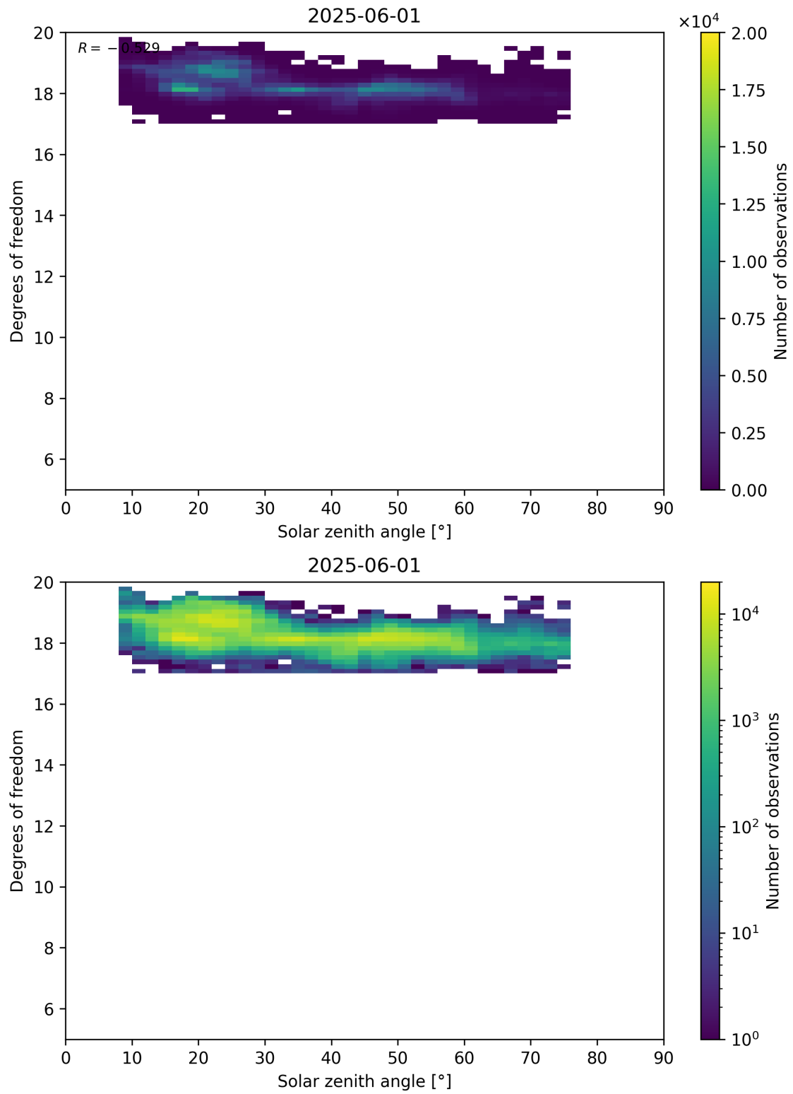
Figure 96: Scatter density plot of “Solar zenith angle” against “Degrees of freedom” for 2025-06-01 to 2025-06-02.
