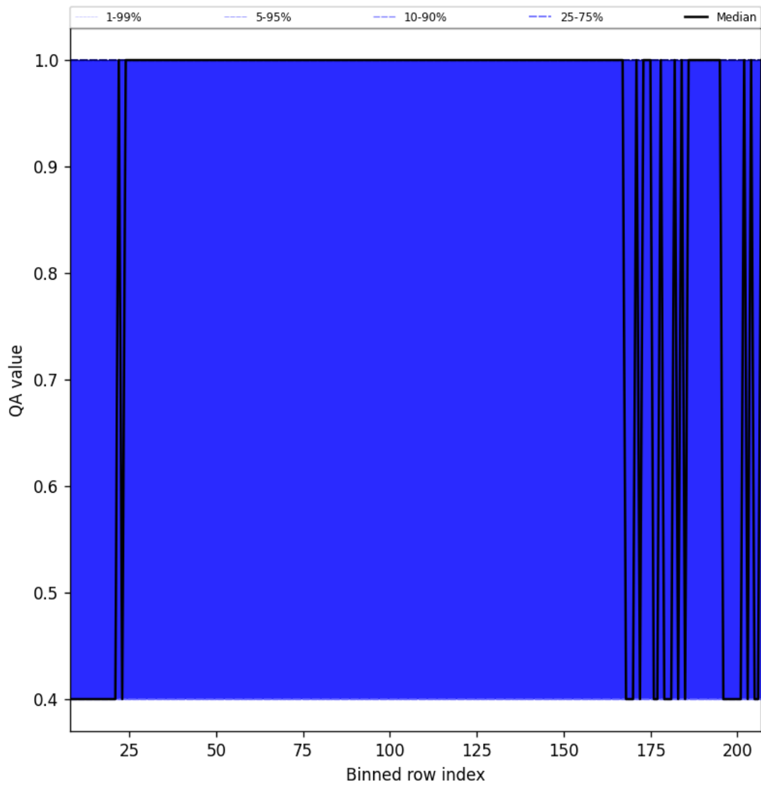
Figure 33: Along track statistics of “QA value” for 2025-06-01 to 2025-06-02
