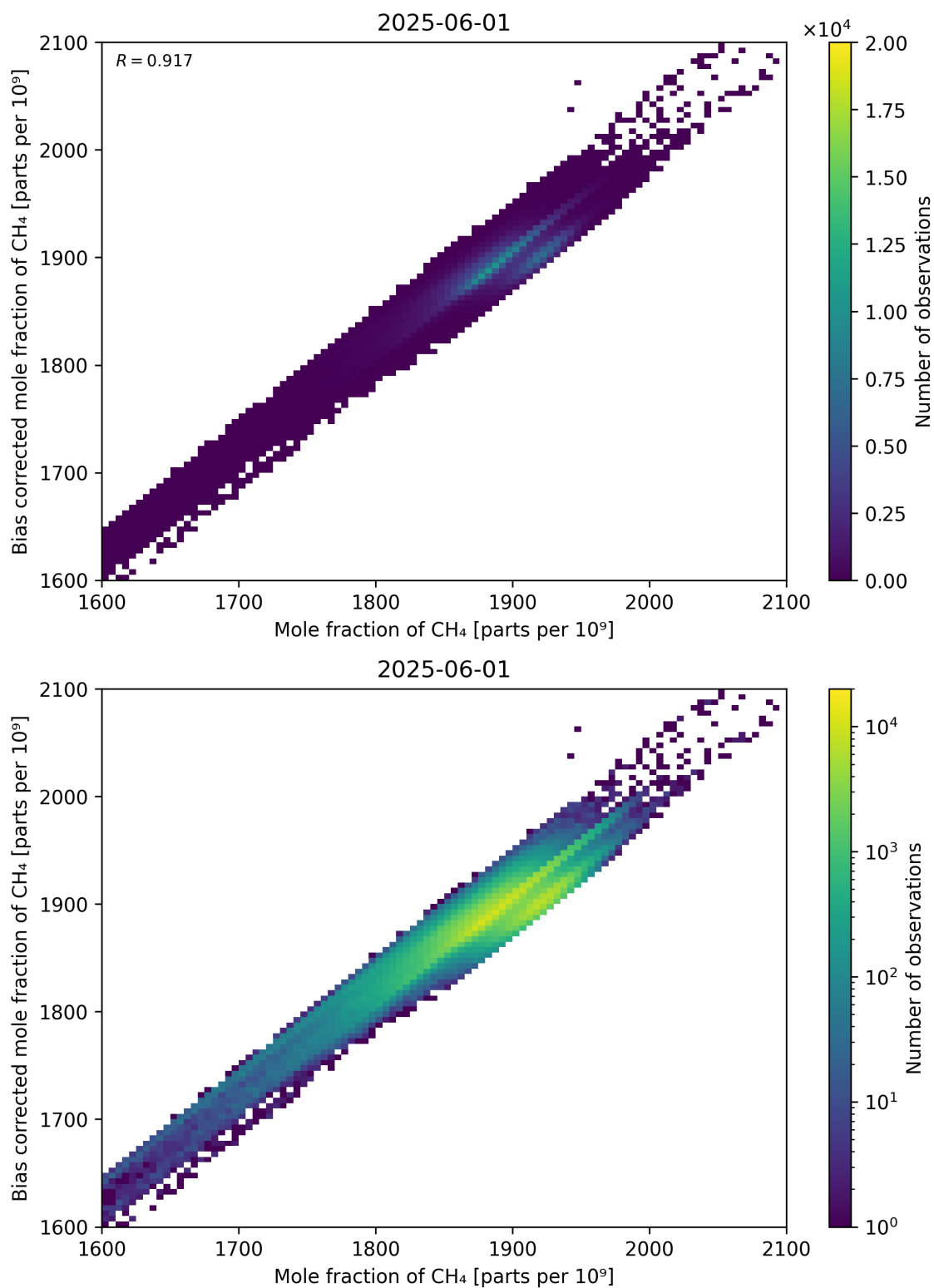
Figure 74: Scatter density plot of “Mole fraction of CH 4 ” against “Bias corrected mole fraction of CH 4 ” for 2025-06-01 to 2025-06-02.
