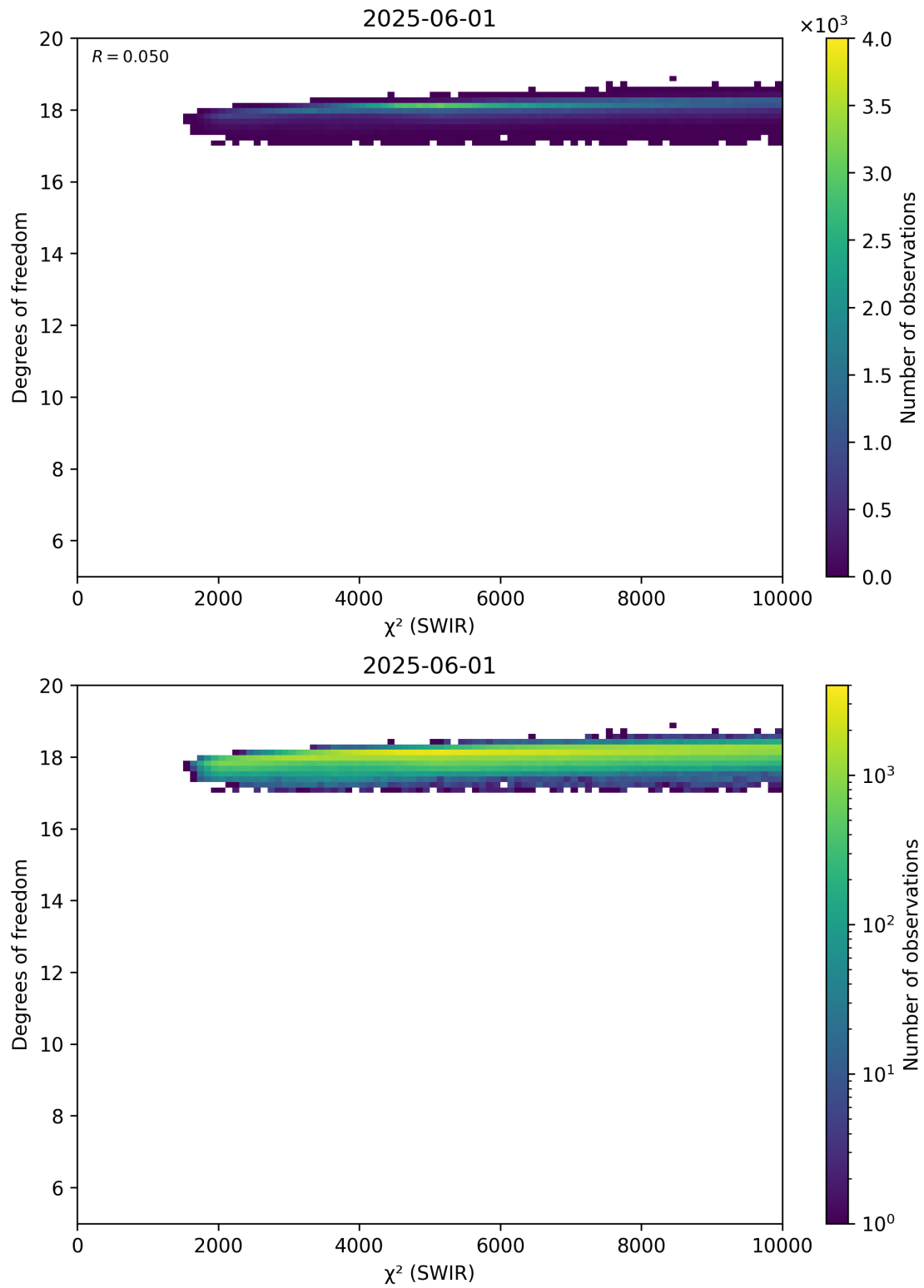
Figure 48: Scatter density plot of “ \chi^2 (SWIR)” against “Degrees of freedom” for 2025-06-01 to 2025-06-02.
