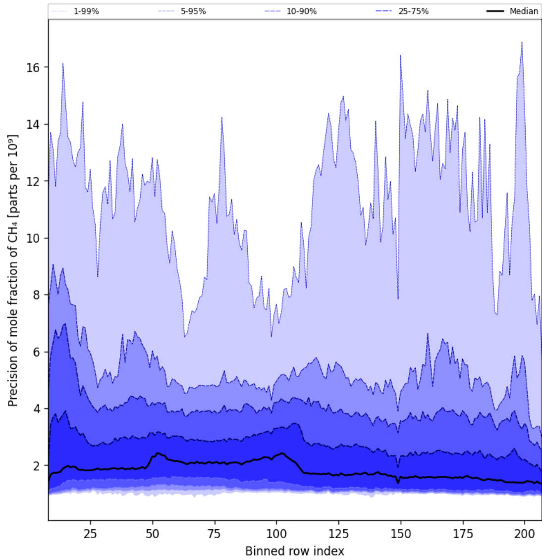
Figure 35: Along track statistics of “Precision of mole fraction of CH 4 ” for 2025-06-01 to 2025-06-02
