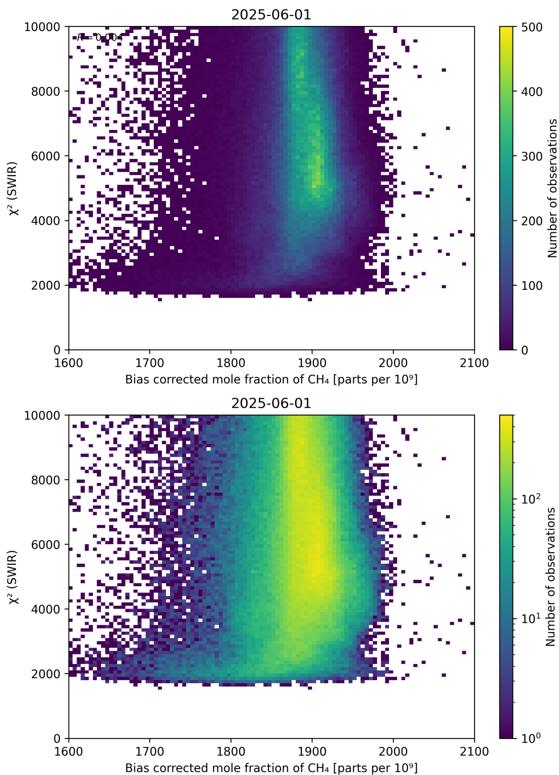
Figure 64: Scatter density plot of “Bias corrected mole fraction of CH 4 ” against “ \chi^2 (SWIR)” for 2025-06-01 to 2025-06-02.
