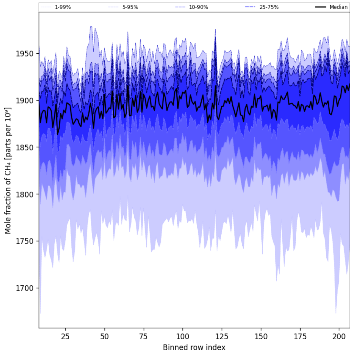
Figure 34: Along track statistics of “Mole fraction of CH 4 ” for 2025-06-01 to 2025-06-02
