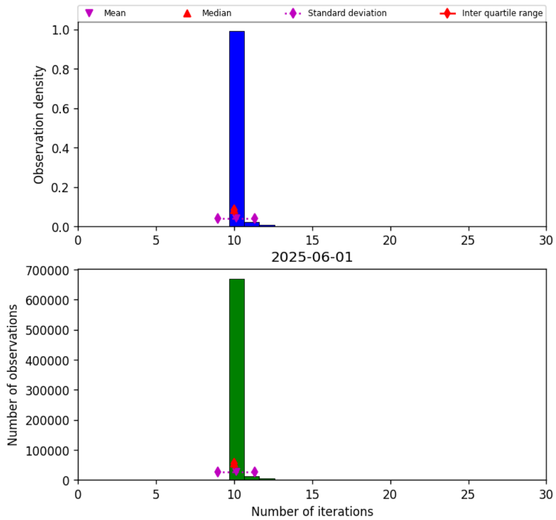
Figure 31: Histogram of “Number of iterations” for 2025-06-01 to 2025-06-02
