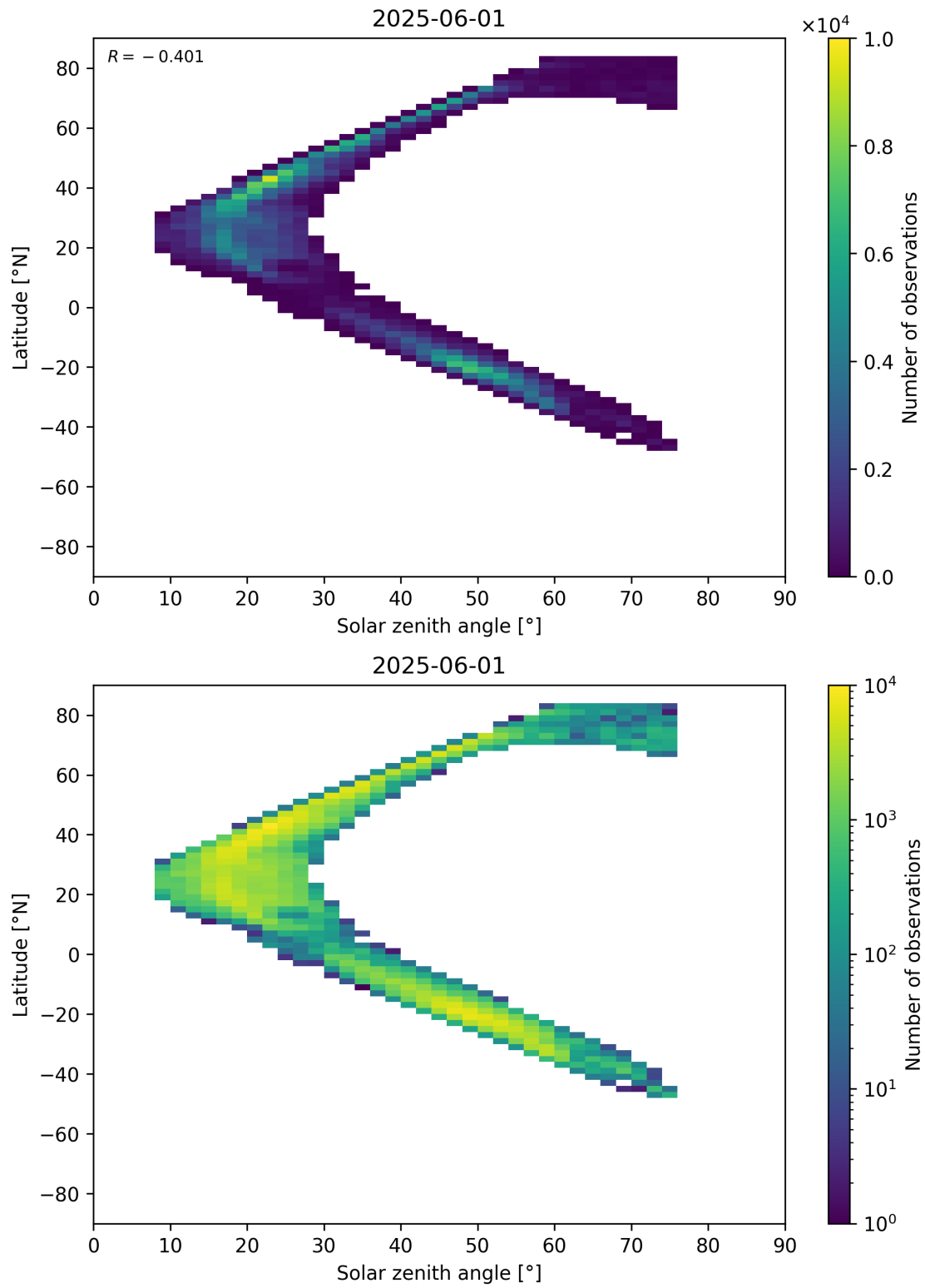
Figure 98: Scatter density plot of “Solar zenith angle” against “Latitude” for 2025-06-01 to 2025-06-02.
