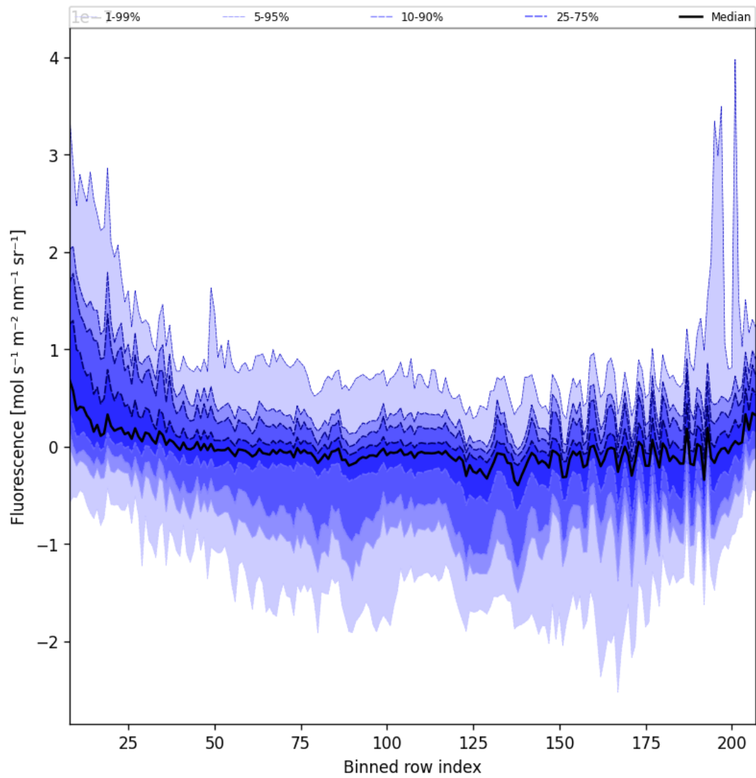
Figure 43: Along track statistics of “Fluorescence” for 2025-06-01 to 2025-06-02
