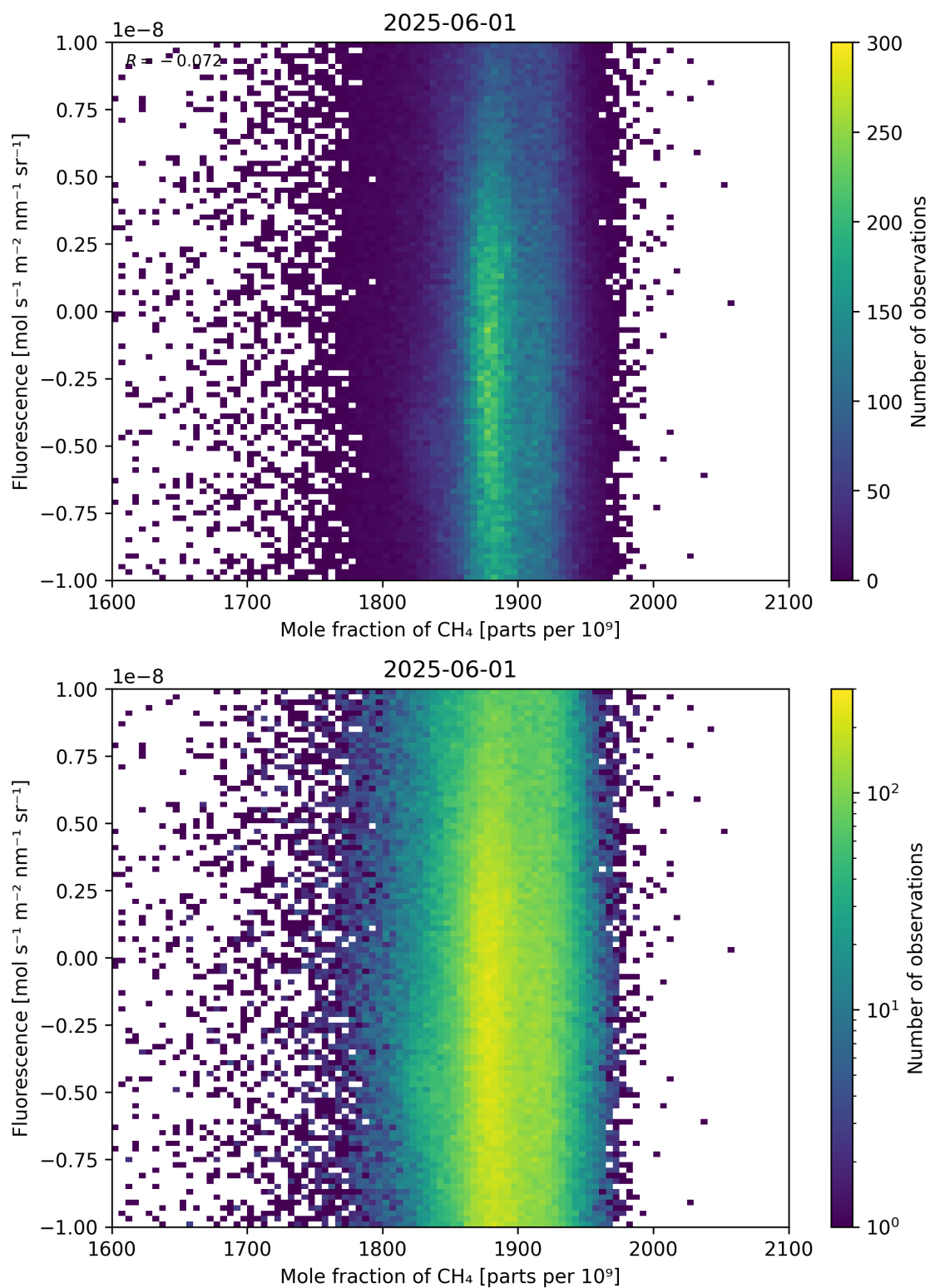
Figure 73: Scatter density plot of “Mole fraction of \text{CH}_4 ” against “Fluorescence” for 2025-06-01 to 2025-06-02.
