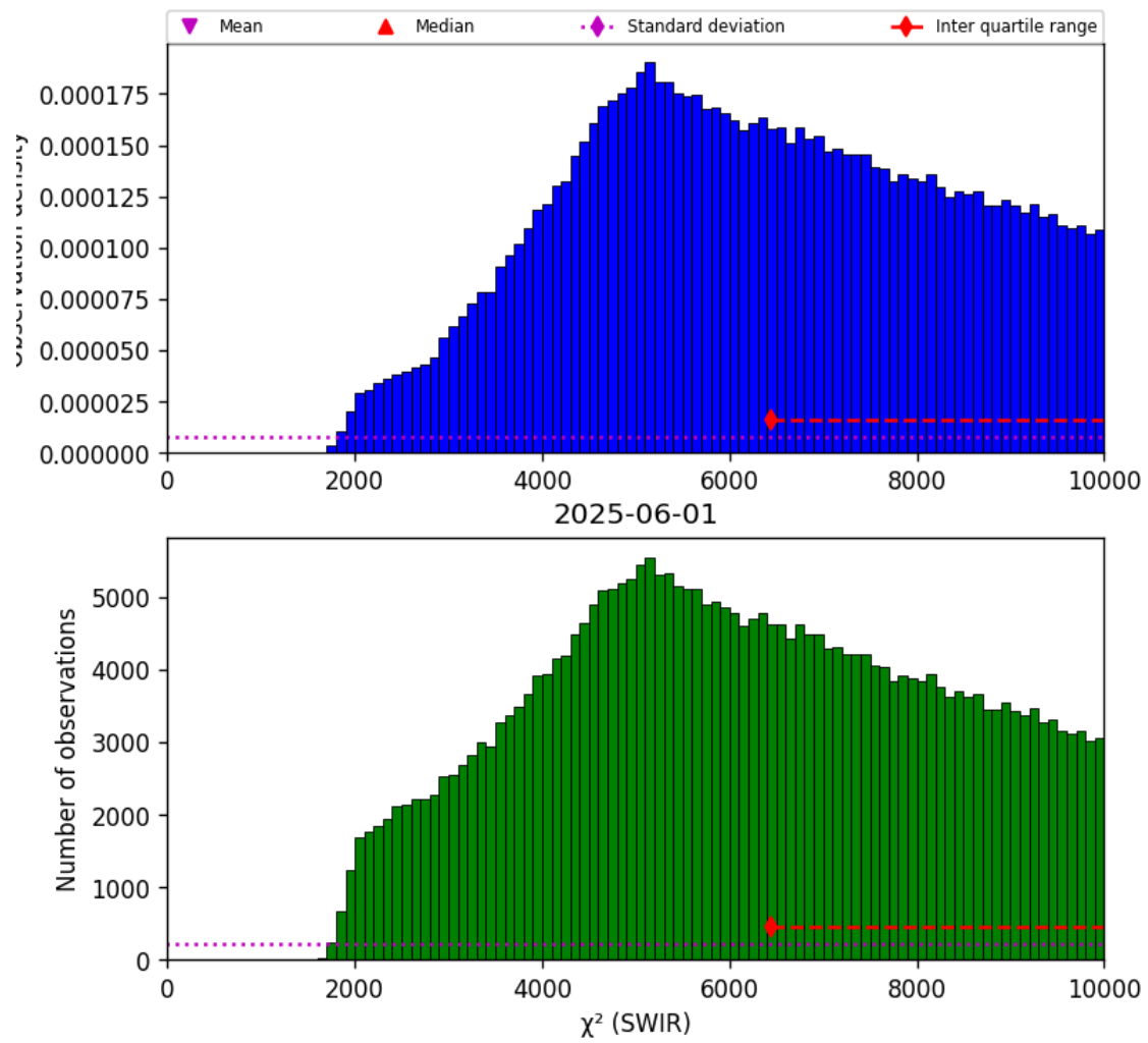
Figure 28: Histogram of “ \chi^2 (SWIR)” for 2025-06-01 to 2025-06-02
