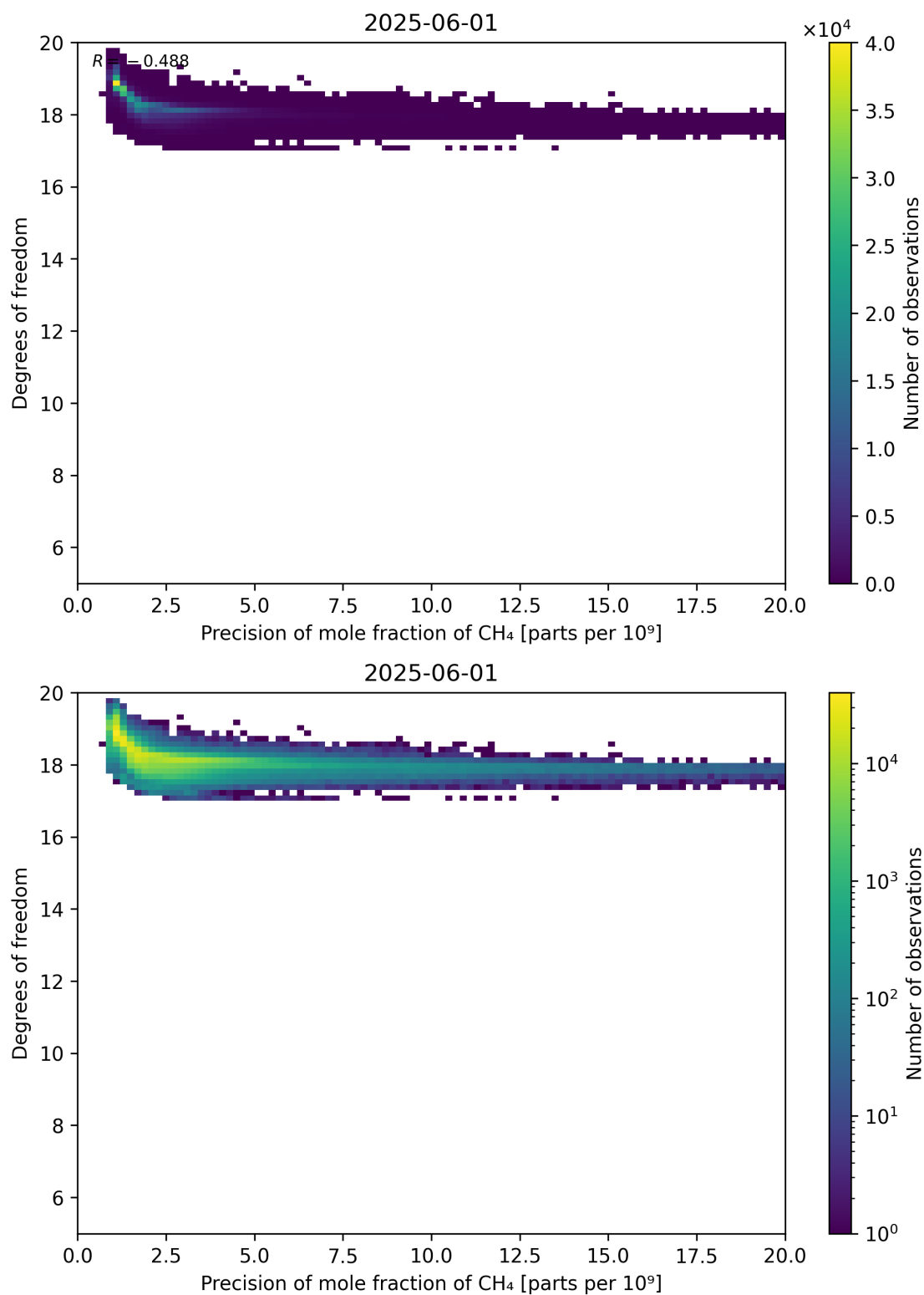
Figure 80: Scatter density plot of “Precision of mole fraction of CH 4 ” against “Degrees of freedom” for 2025-06-01 to 2025-06-02.
