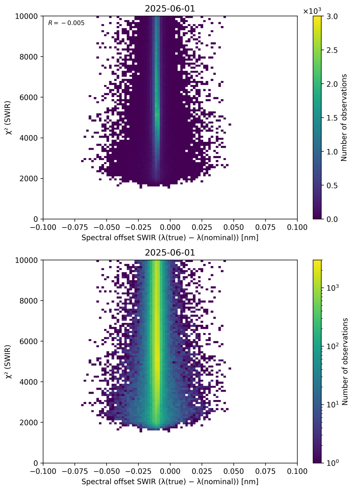
Figure 118: Scatter density plot of “Spectral offset SWIR ( \lambda_{\text{true}} - \lambda_{\text{nominal}} )” against “ \chi^2 (SWIR)” for 2025-06-01 to 2025-06-02.
