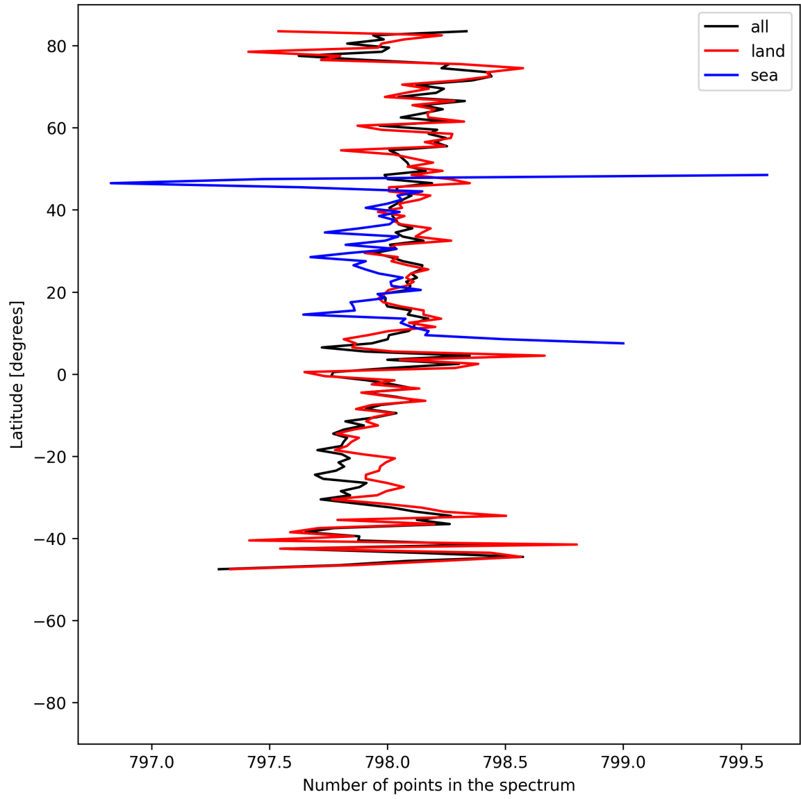
Figure 15: Zonal average of “Number of points in the spectrum” for 2025-06-01 to 2025-06-02.
