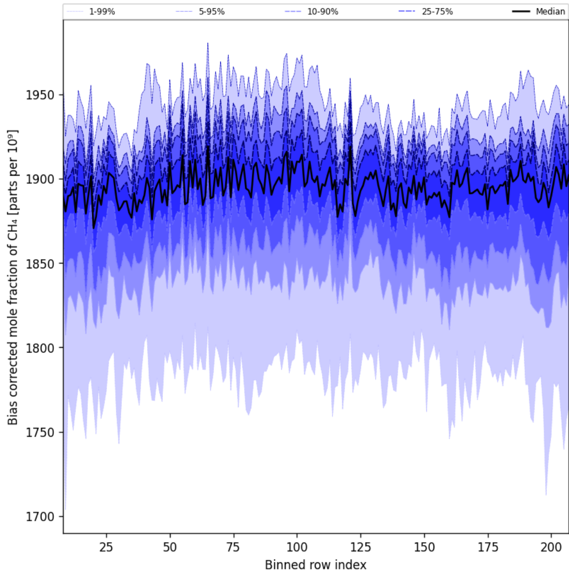
Figure 36: Along track statistics of “Bias corrected mole fraction of CH 4 ” for 2025-06-01 to 2025-06-02
