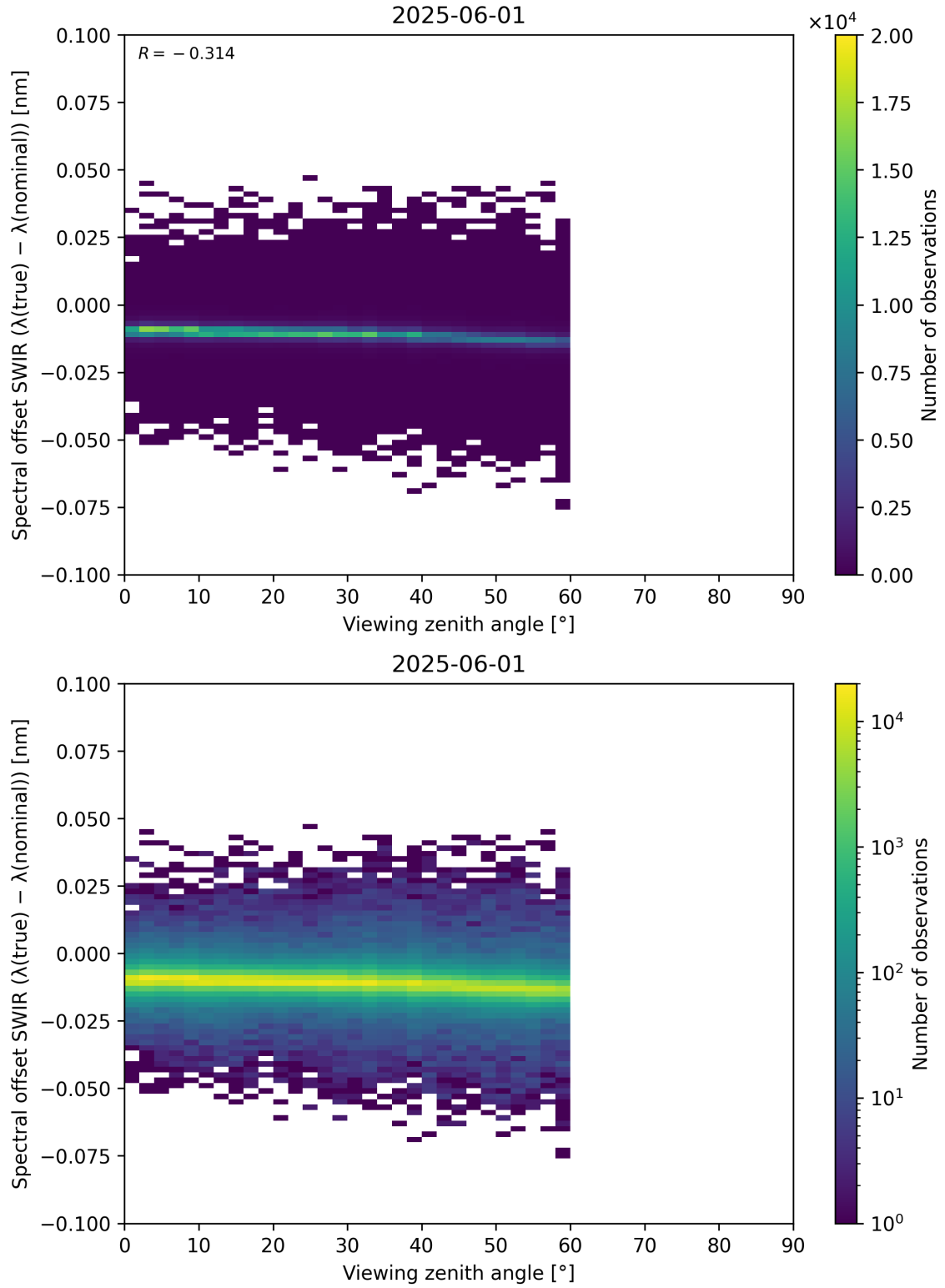
Figure 116: Scatter density plot of “Viewing zenith angle” against “Spectral offset SWIR ( \lambda_{\text{true}} - \lambda_{\text{nominal}} )” for 2025-06-01 to 2025-06-02.
