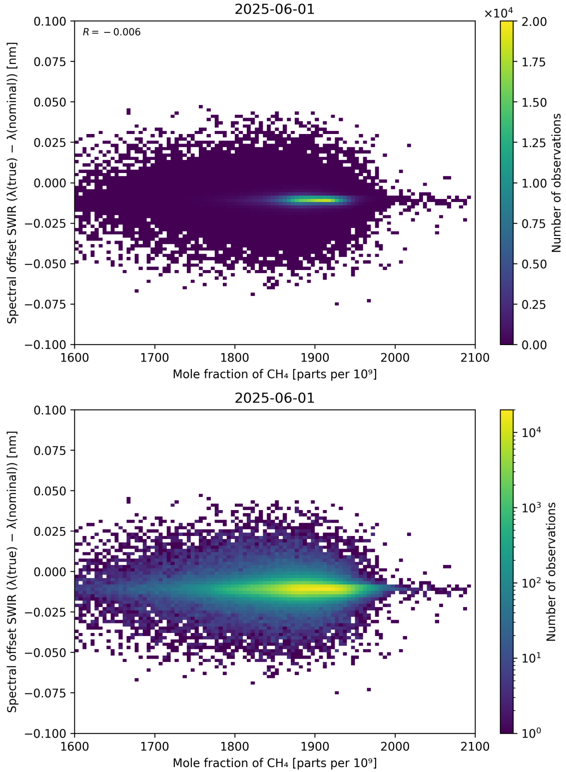
Figure 86: Scatter density plot of “Mole fraction of CH 4 ” against “Spectral offset SWIR ( \lambda_{\text{true}} - \lambda_{\text{nominal}} )” for 2025-06-01 to 2025-06-02.
