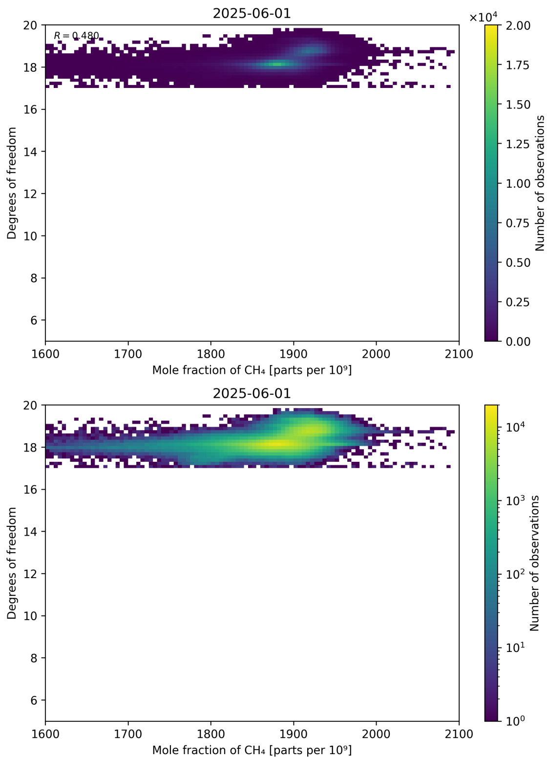
Figure 72: Scatter density plot of “Mole fraction of CH 4 ” against “Degrees of freedom” for 2025-06-01 to 2025-06-02.
