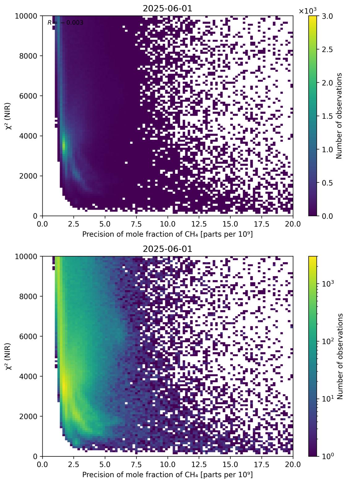
Figure 78: Scatter density plot of “Precision of mole fraction of CH 4 ” against “ \chi^2 (NIR)” for 2025-06-01 to 2025-06-02.
