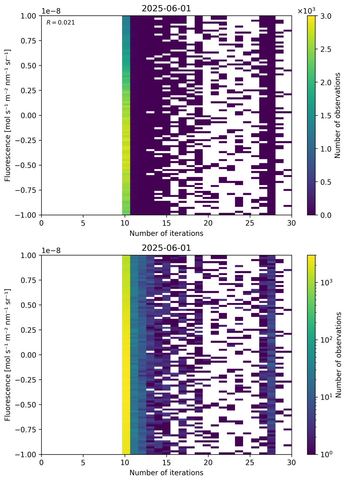
Figure 87: Scatter density plot of “Number of iterations” against “Fluorescence” for 2025-06-01 to 2025-06-02.
