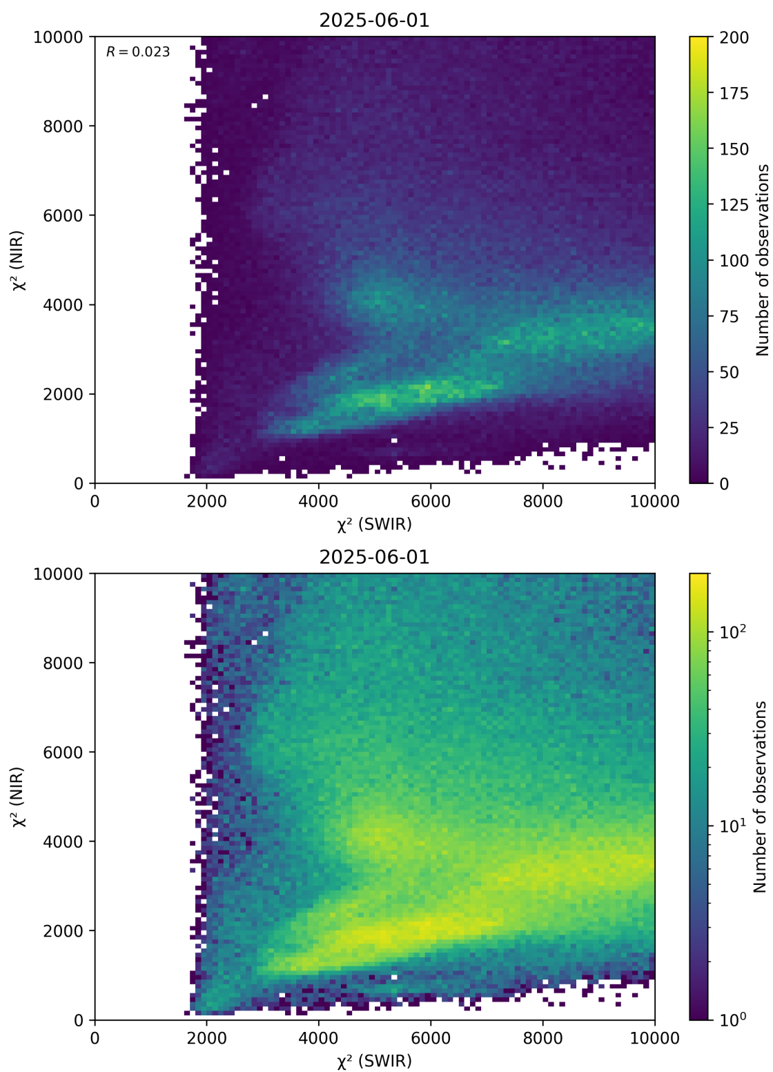
Figure 47: Scatter density plot of “ \chi^2 (SWIR)” against “ \chi^2 (NIR)” for 2025-06-01 to 2025-06-02.
