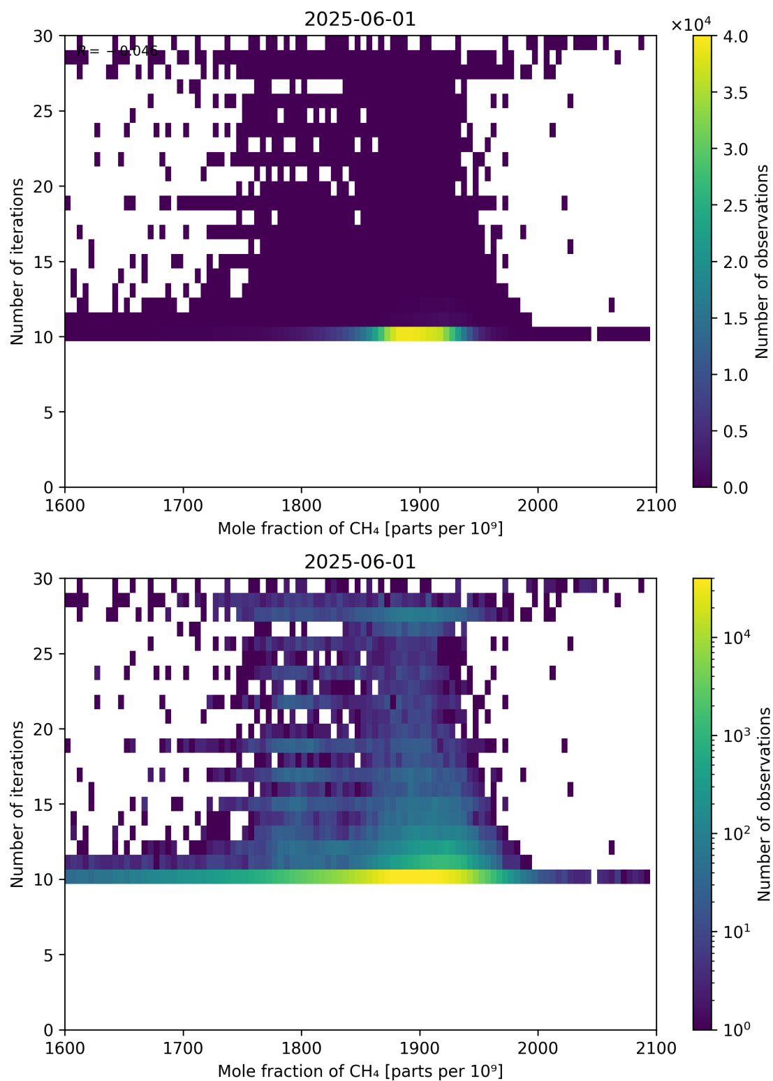
Figure 76: Scatter density plot of “Mole fraction of CH 4 ” against “Number of iterations” for 2025-06-01 to 2025-06-02.
