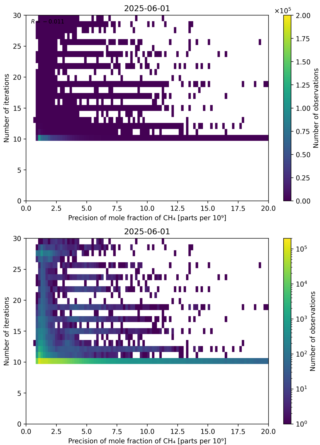
Figure 83: Scatter density plot of “Precision of mole fraction of CH 4 ” against “Number of iterations” for 2025-06-01 to 2025-06-02.
