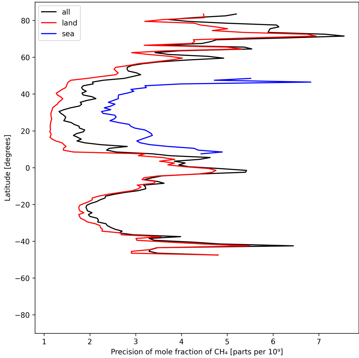
Figure 13: Zonal average of “Precision of mole fraction of CH 4 ” for 2025-06-01 to 2025-06-02.
