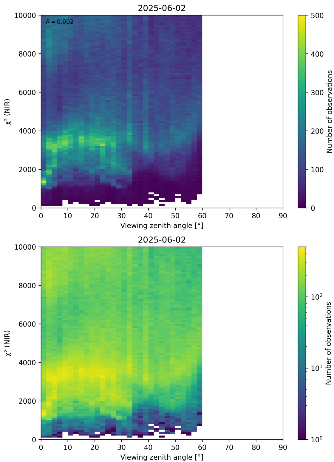
Figure 105: Scatter density plot of “Viewing zenith angle” against “ \chi^2 (NIR)” for 2025-06-01 to 2025-06-03.
