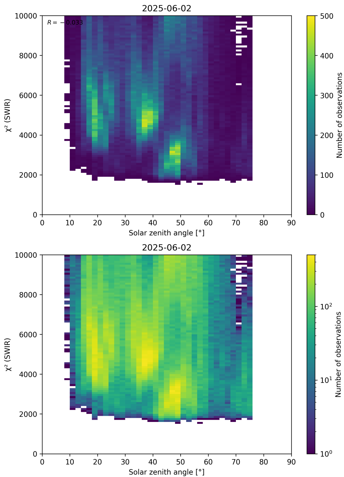
Figure 95: Scatter density plot of “Solar zenith angle” against “ \chi^2 (SWIR)” for 2025-06-01 to 2025-06-03.
