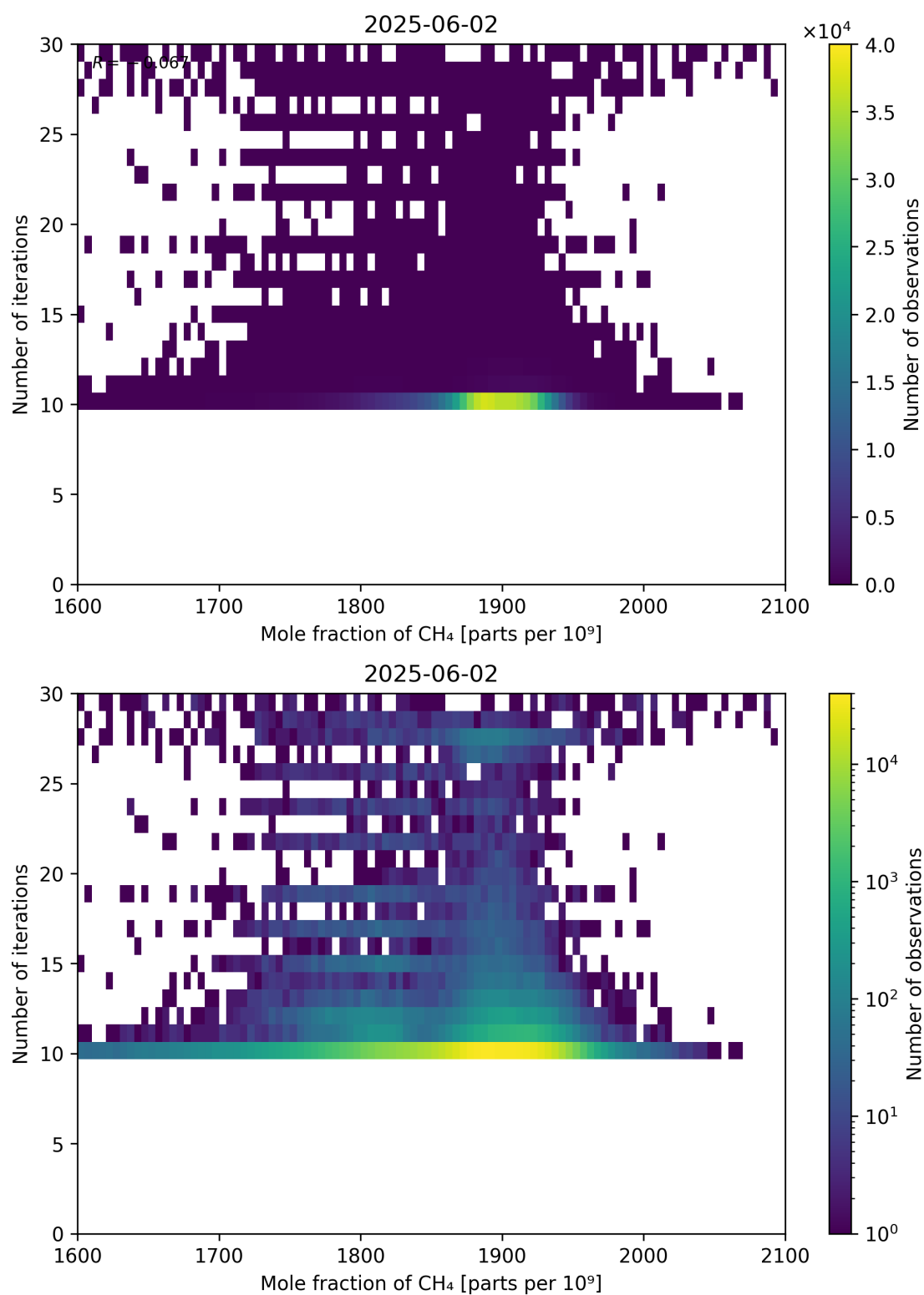
Figure 76: Scatter density plot of “Mole fraction of CH 4 ” against “Number of iterations” for 2025-06-01 to 2025-06-03.
