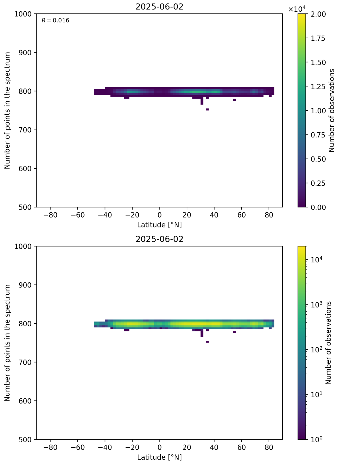
Figure 61: Scatter density plot of “Latitude” against “Number of points in the spectrum” for 2025-06-01 to 2025-06-03.
