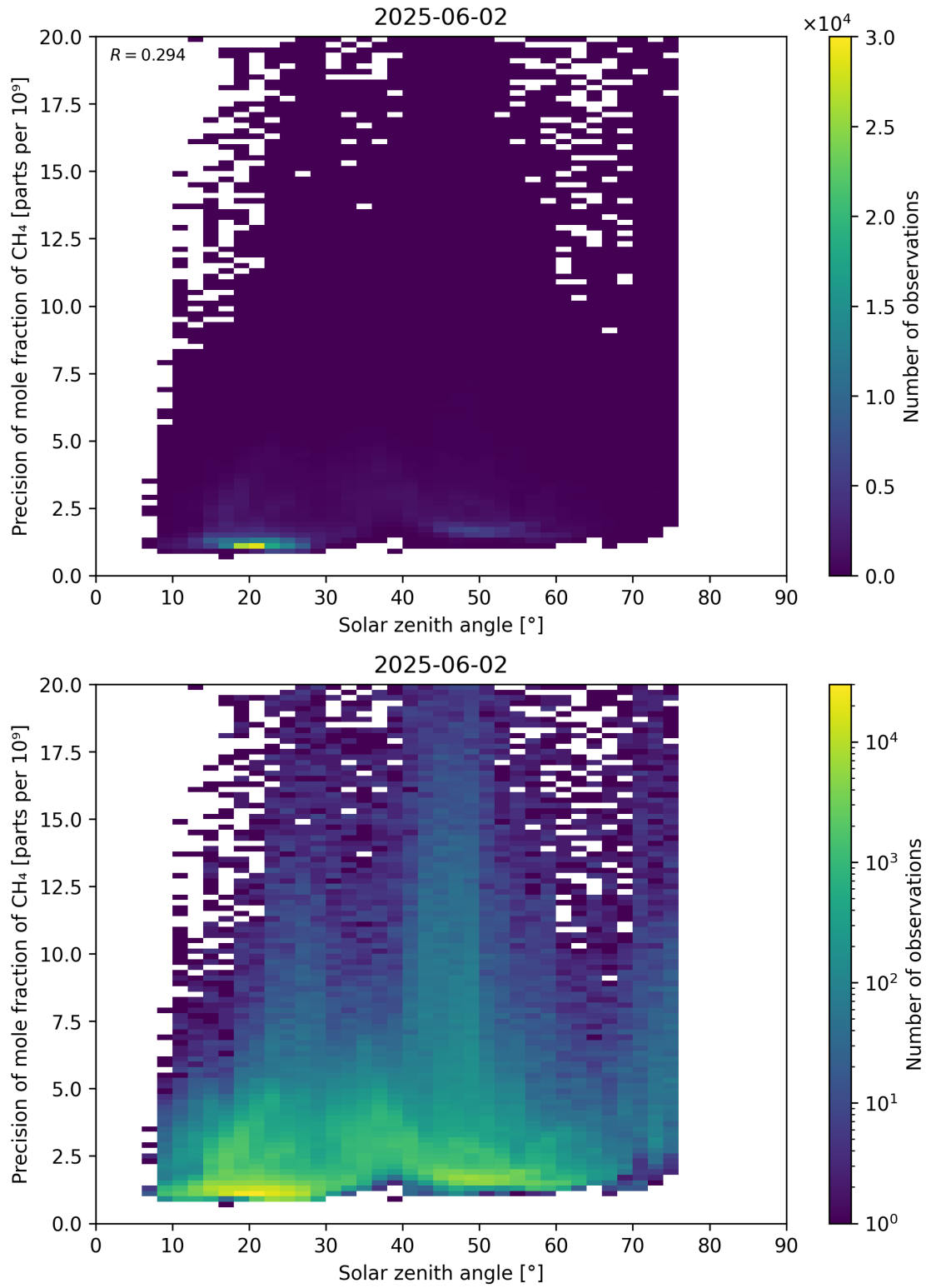
Figure 101: Scatter density plot of “Solar zenith angle” against “Precision of mole fraction of CH 4 ” for 2025-06-01 to 2025-06-03.
