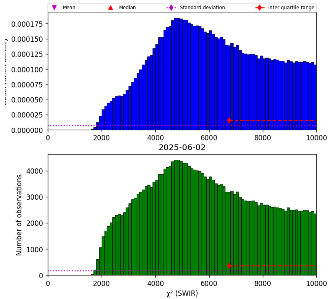
Figure 28: Histogram of “ \chi^2 (SWIR)” for 2025-06-01 to 2025-06-03
