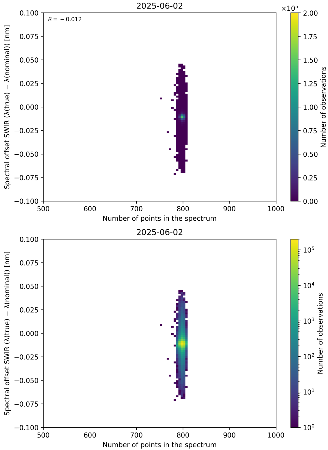
Figure 93: Scatter density plot of “Number of points in the spectrum” against “Spectral offset SWIR ( \lambda_{\text{true}} - \lambda_{\text{nominal}} )” for 2025-06-01 to 2025-06-03.
