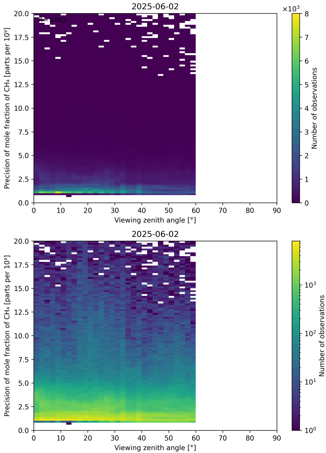
Figure 112: Scatter density plot of “Viewing zenith angle” against “Precision of mole fraction of CH 4 ” for 2025-06-01 to 2025-06-03.
