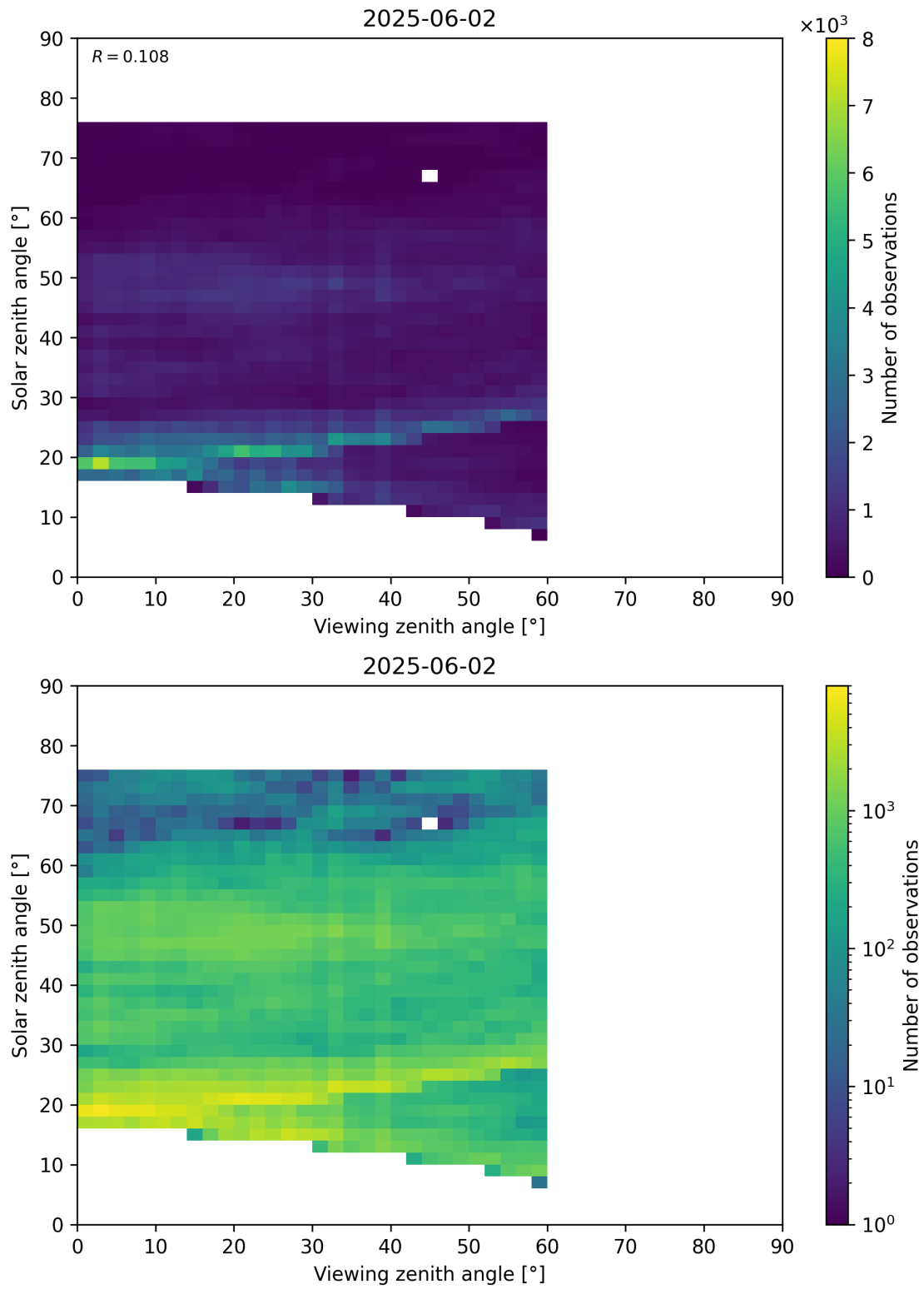
Figure 115: Scatter density plot of “Viewing zenith angle” against “Solar zenith angle” for 2025-06-01 to 2025-06-03.
