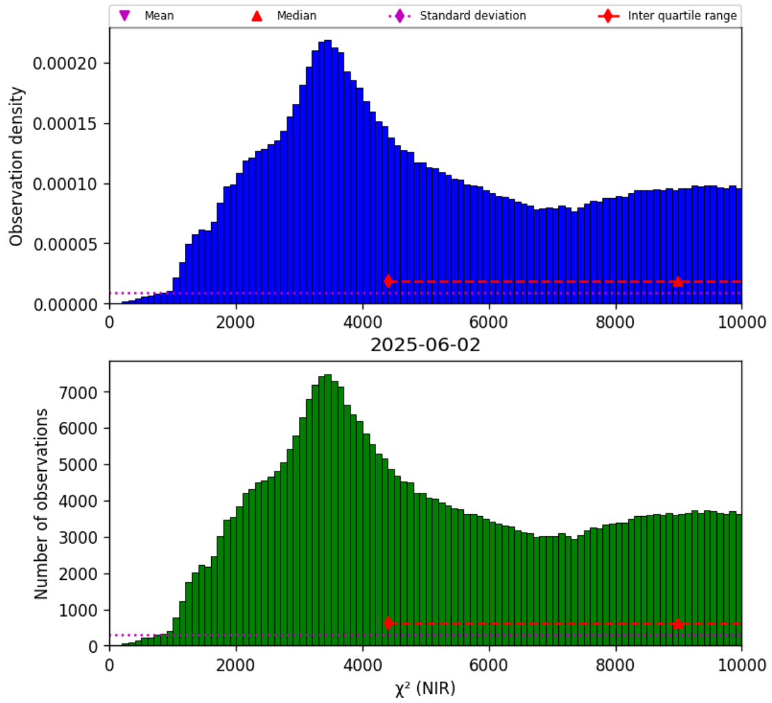
Figure 29: Histogram of “ \chi^2 (NIR)” for 2025-06-01 to 2025-06-03
