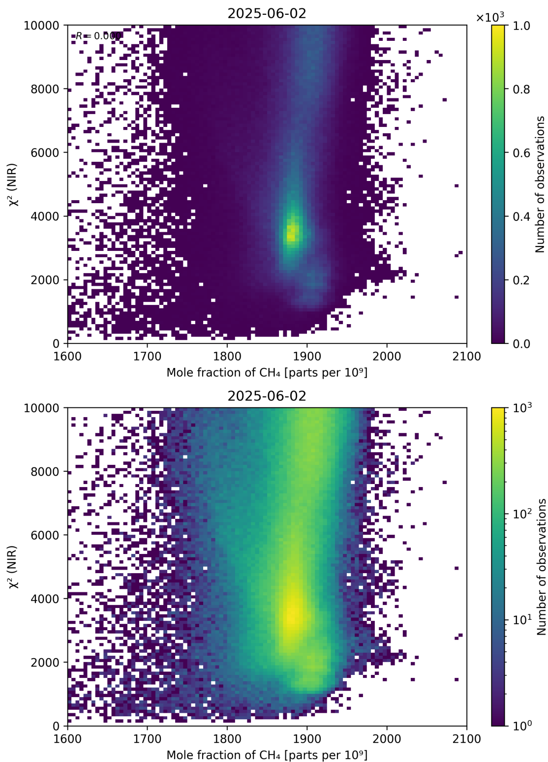
Figure 70: Scatter density plot of “Mole fraction of \text{CH}_4 ” against “ \chi^2 (NIR)” for 2025-06-01 to 2025-06-03.
