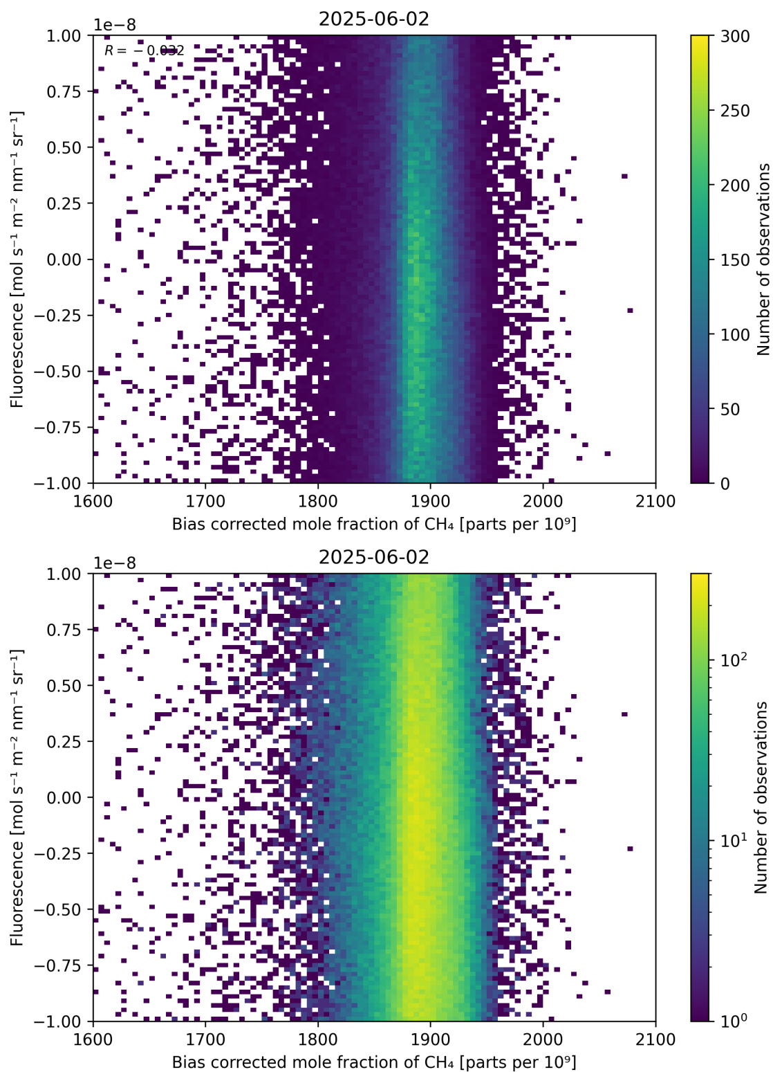
Figure 66: Scatter density plot of “Bias corrected mole fraction of \text{CH}_4 ” against “Fluorescence” for 2025-06-01 to 2025-06-03.
