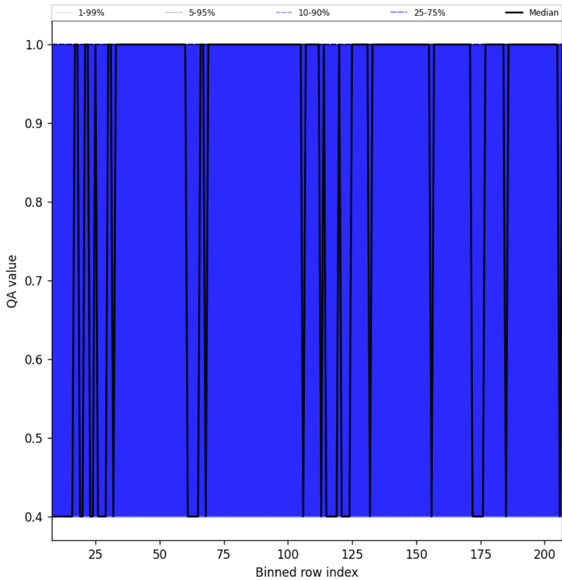
Figure 33: Along track statistics of “QA value” for 2025-06-01 to 2025-06-03
