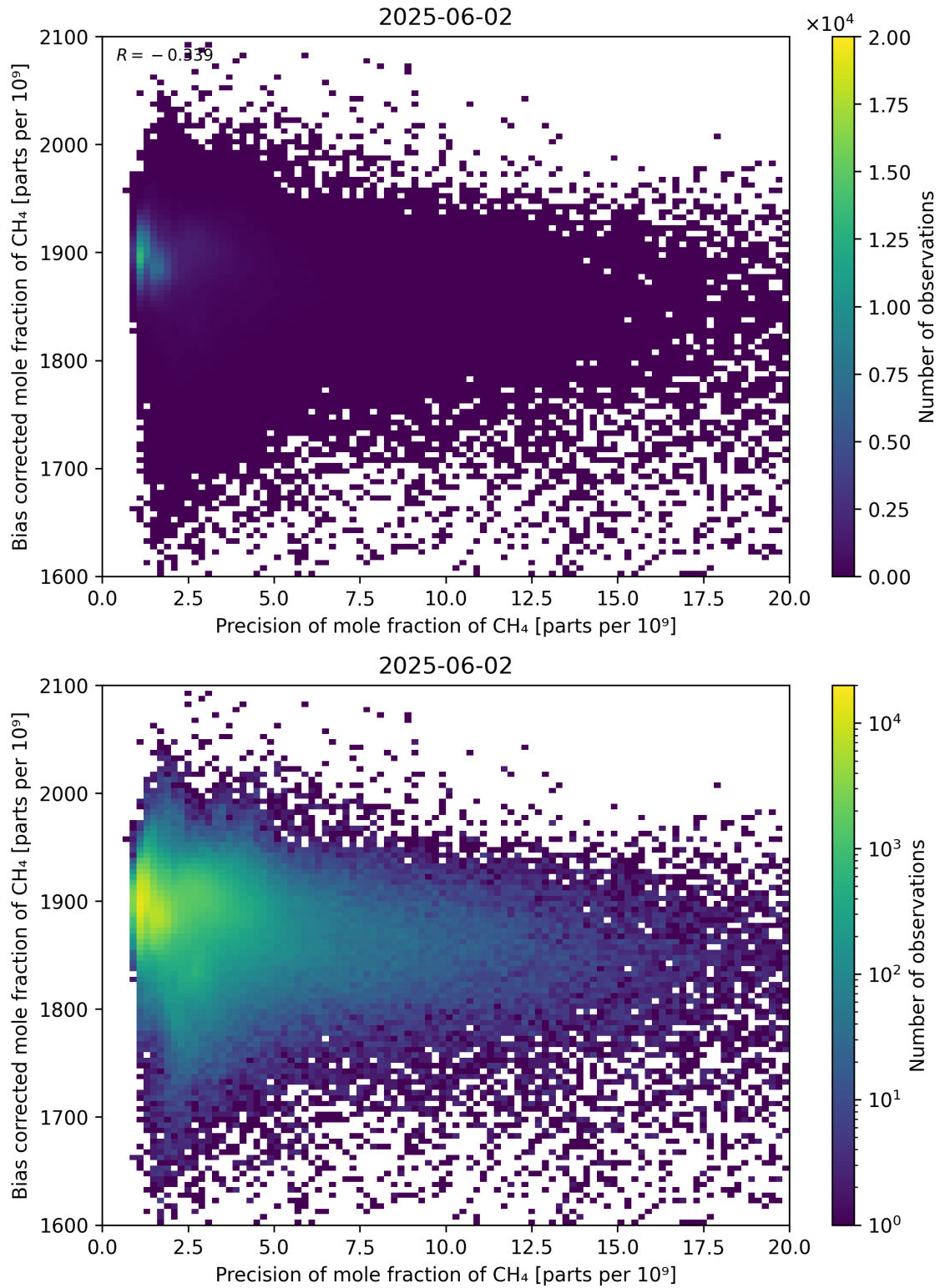
Figure 82: Scatter density plot of “Precision of mole fraction of CH 4 ” against “Bias corrected mole fraction of CH 4 ” for 2025-06-01 to 2025-06-03.
