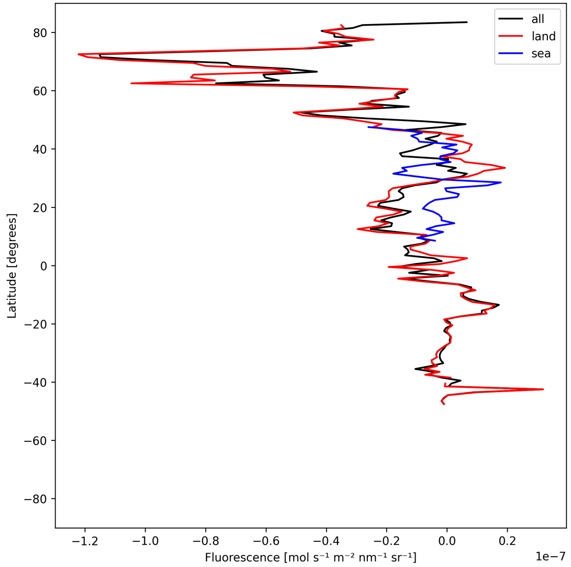
Figure 21: Zonal average of “Fluorescence” for 2025-06-01 to 2025-06-03.
