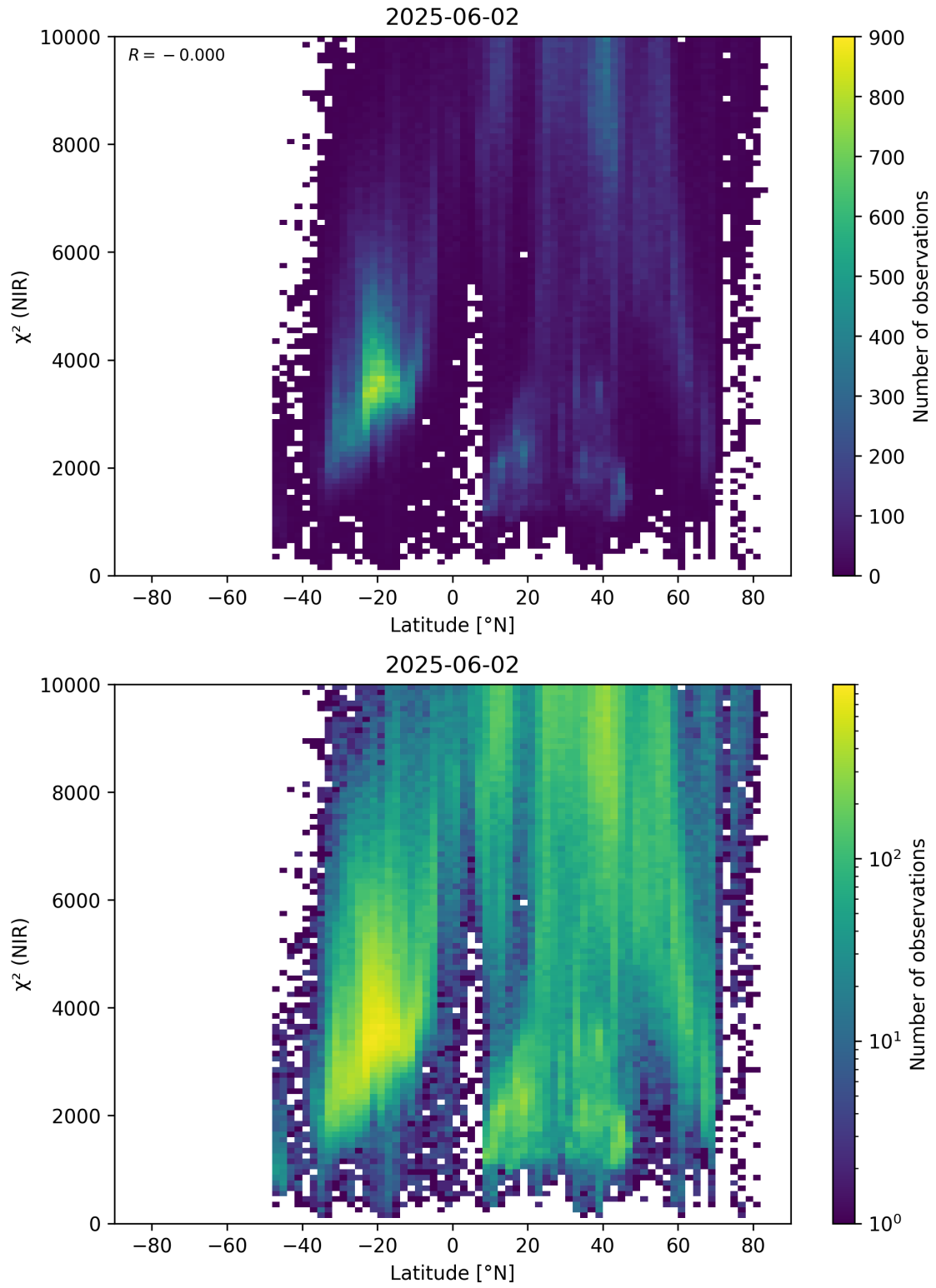
Figure 53: Scatter density plot of “Latitude” against “ \chi^2 (NIR)” for 2025-06-01 to 2025-06-03.
