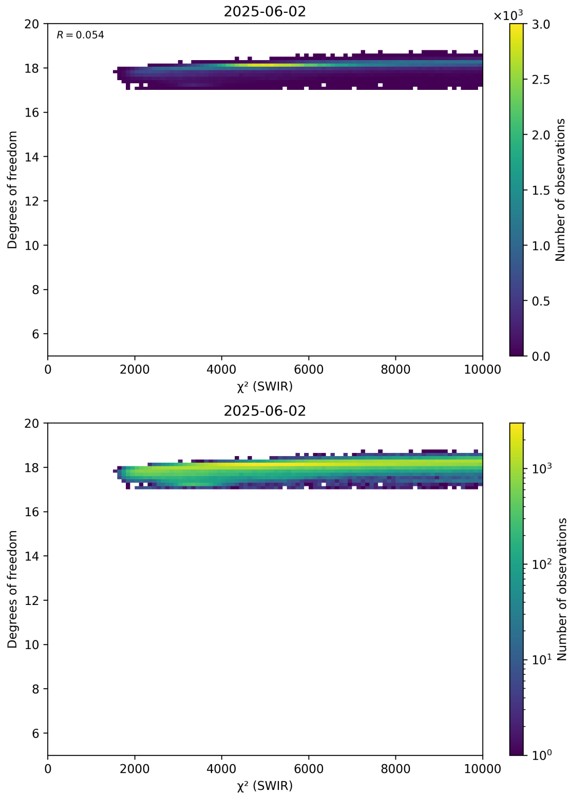
Figure 48: Scatter density plot of “ \chi^2 (SWIR)” against “Degrees of freedom” for 2025-06-01 to 2025-06-03.
