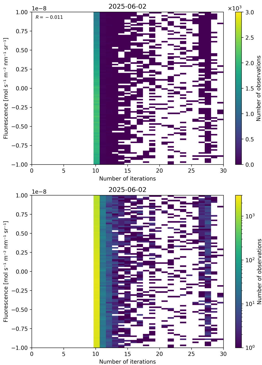
Figure 87: Scatter density plot of “Number of iterations” against “Fluorescence” for 2025-06-01 to 2025-06-03.
