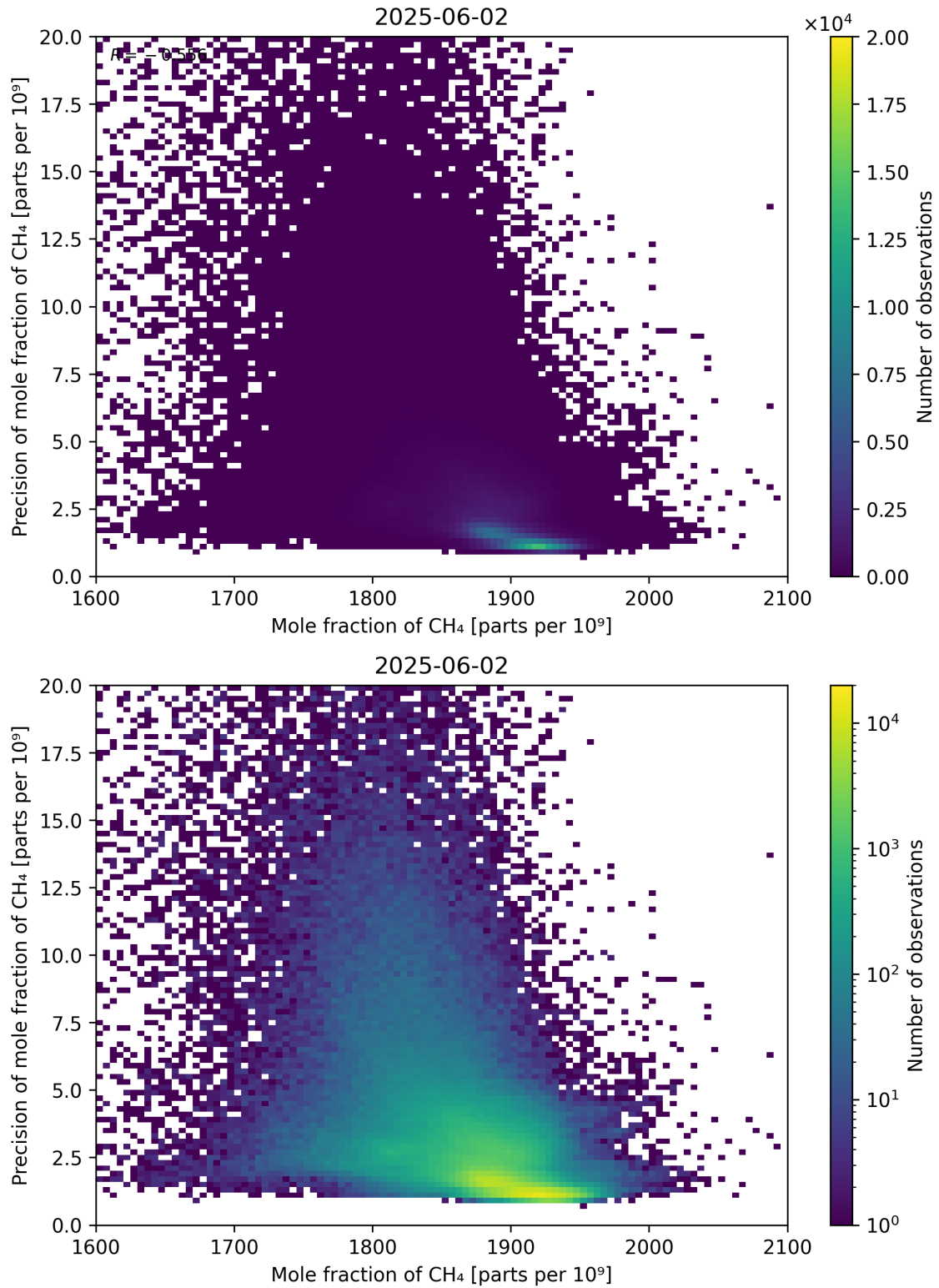
Figure 75: Scatter density plot of “Mole fraction of CH 4 ” against “Precision of mole fraction of CH 4 ” for 2025-06-01 to 2025-06-03.
