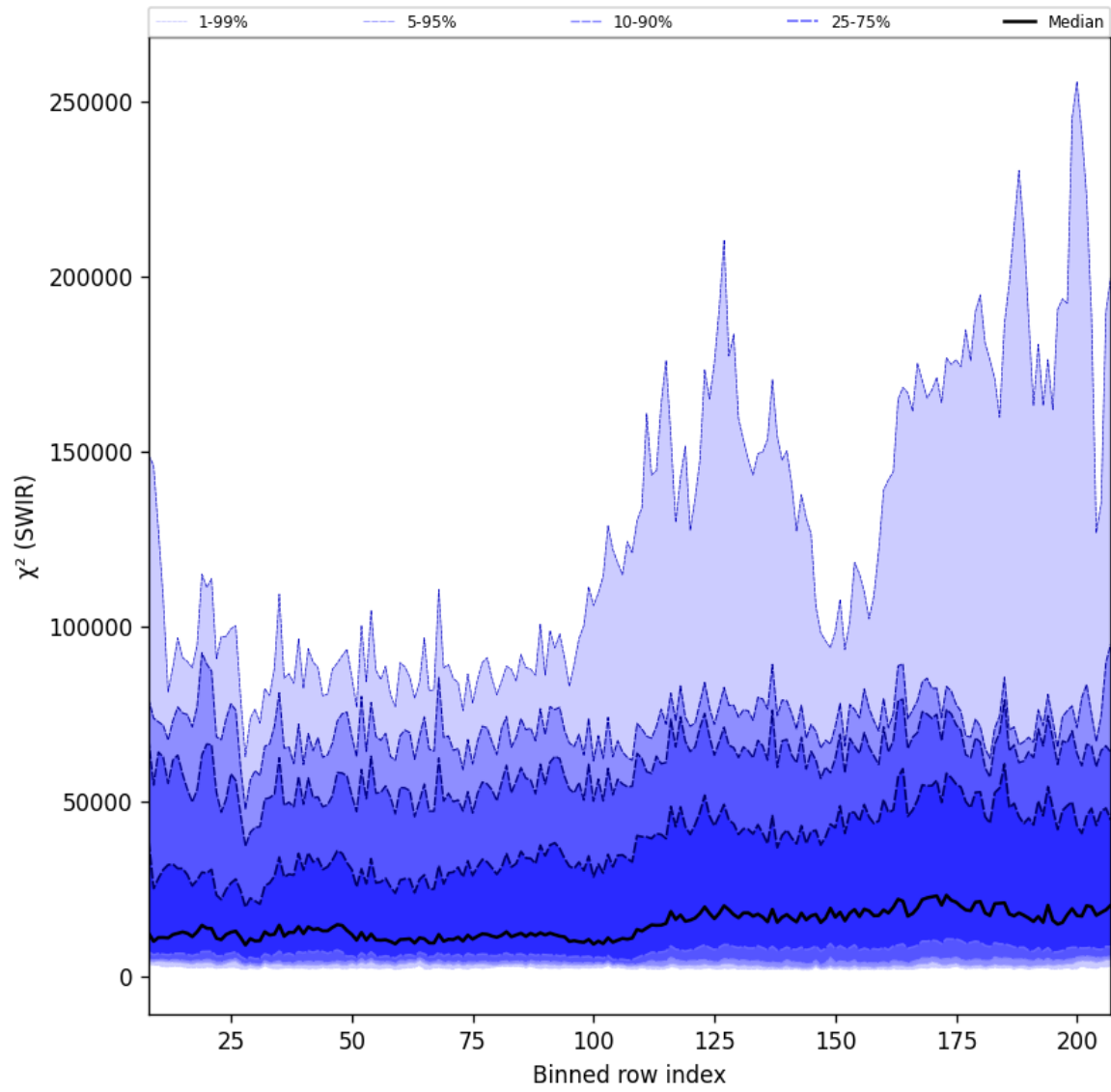
Figure 39: Along track statistics of " \chi^2 (SWIR)" for 2025-06-01 to 2025-06-03
