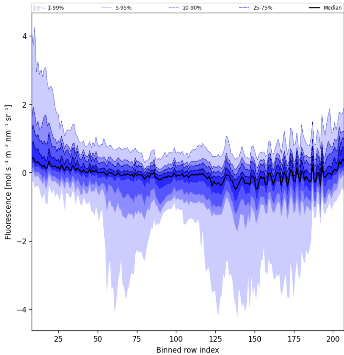
Figure 43: Along track statistics of “Fluorescence” for 2025-06-01 to 2025-06-03
