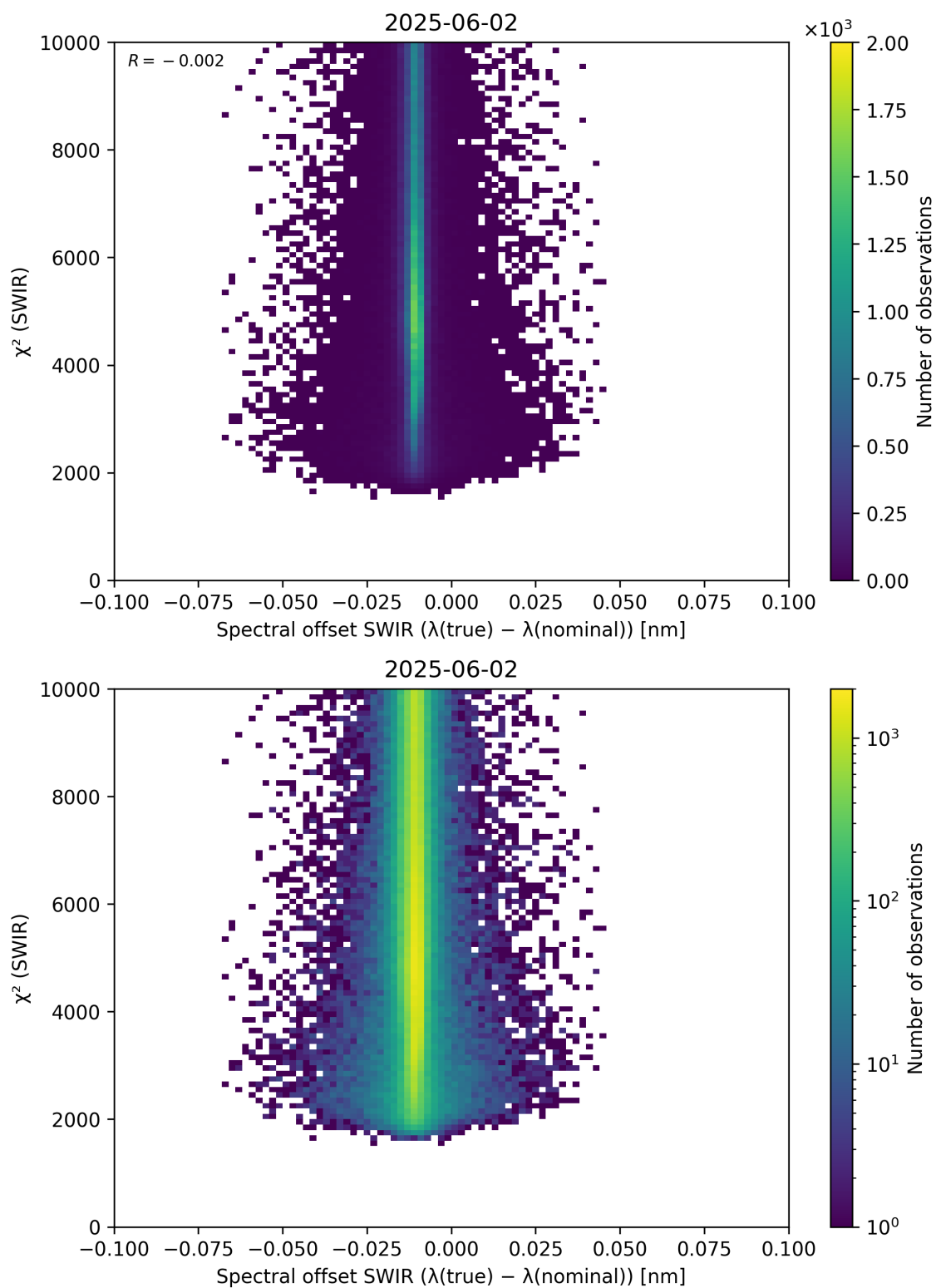
Figure 118: Scatter density plot of “Spectral offset SWIR ( \lambda_{\text{true}} - \lambda_{\text{nominal}} )” against “ \chi^2 (SWIR)” for 2025-06-01 to 2025-06-03.
