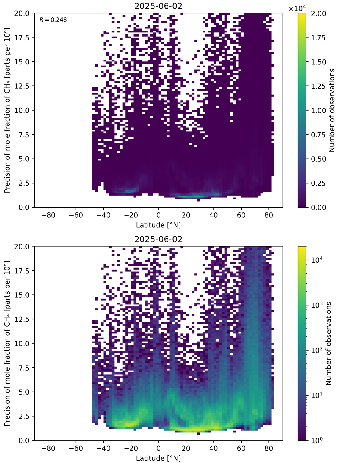
Figure 59: Scatter density plot of “Latitude” against “Precision of mole fraction of \text{CH}_4 ” for 2025-06-01 to 2025-06-03.
