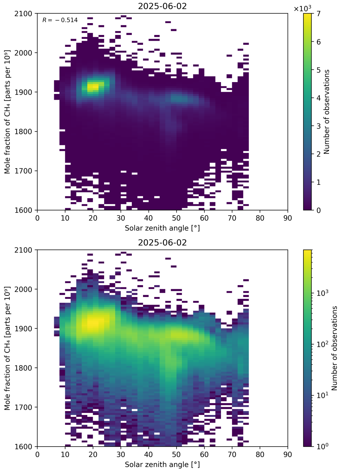
Figure 99: Scatter density plot of “Solar zenith angle” against “Mole fraction of \text{CH}_4 ” for 2025-06-01 to 2025-06-03.
