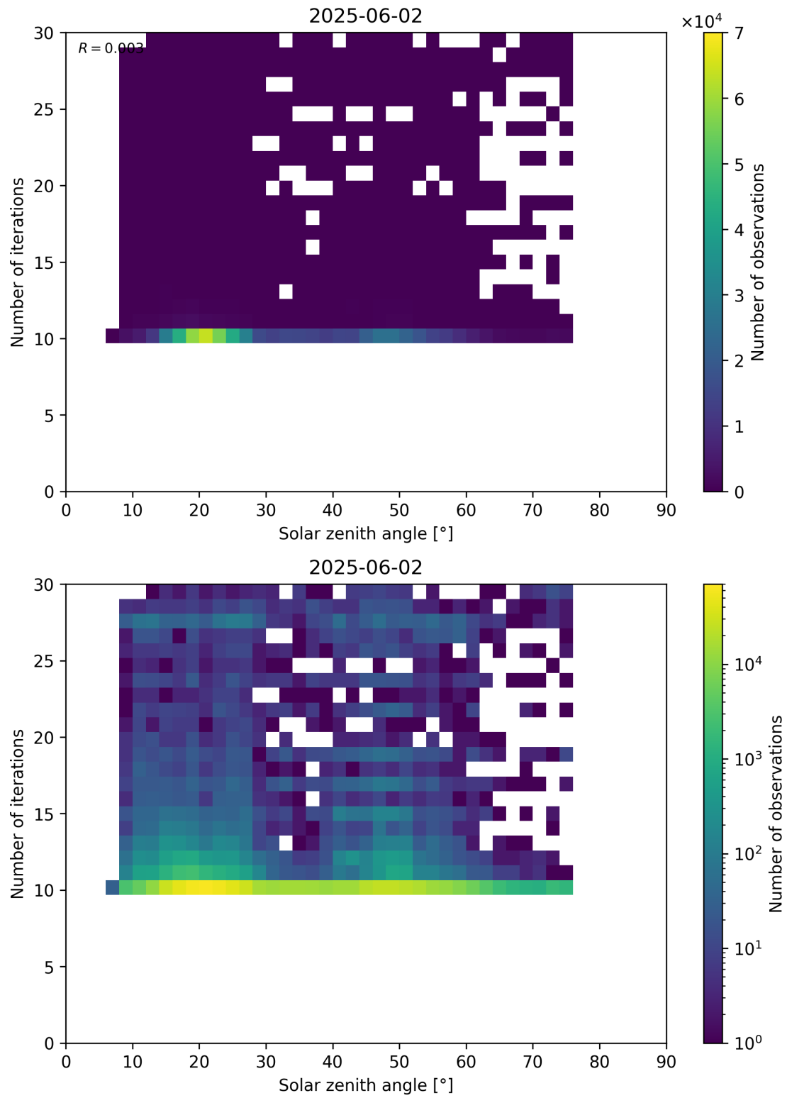
Figure 102: Scatter density plot of “Solar zenith angle” against “Number of iterations” for 2025-06-01 to 2025-06-03.
