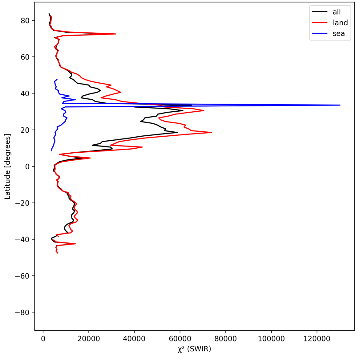
Figure 17: Zonal average of “ \chi^2 (SWIR)” for 2025-06-01 to 2025-06-03.
