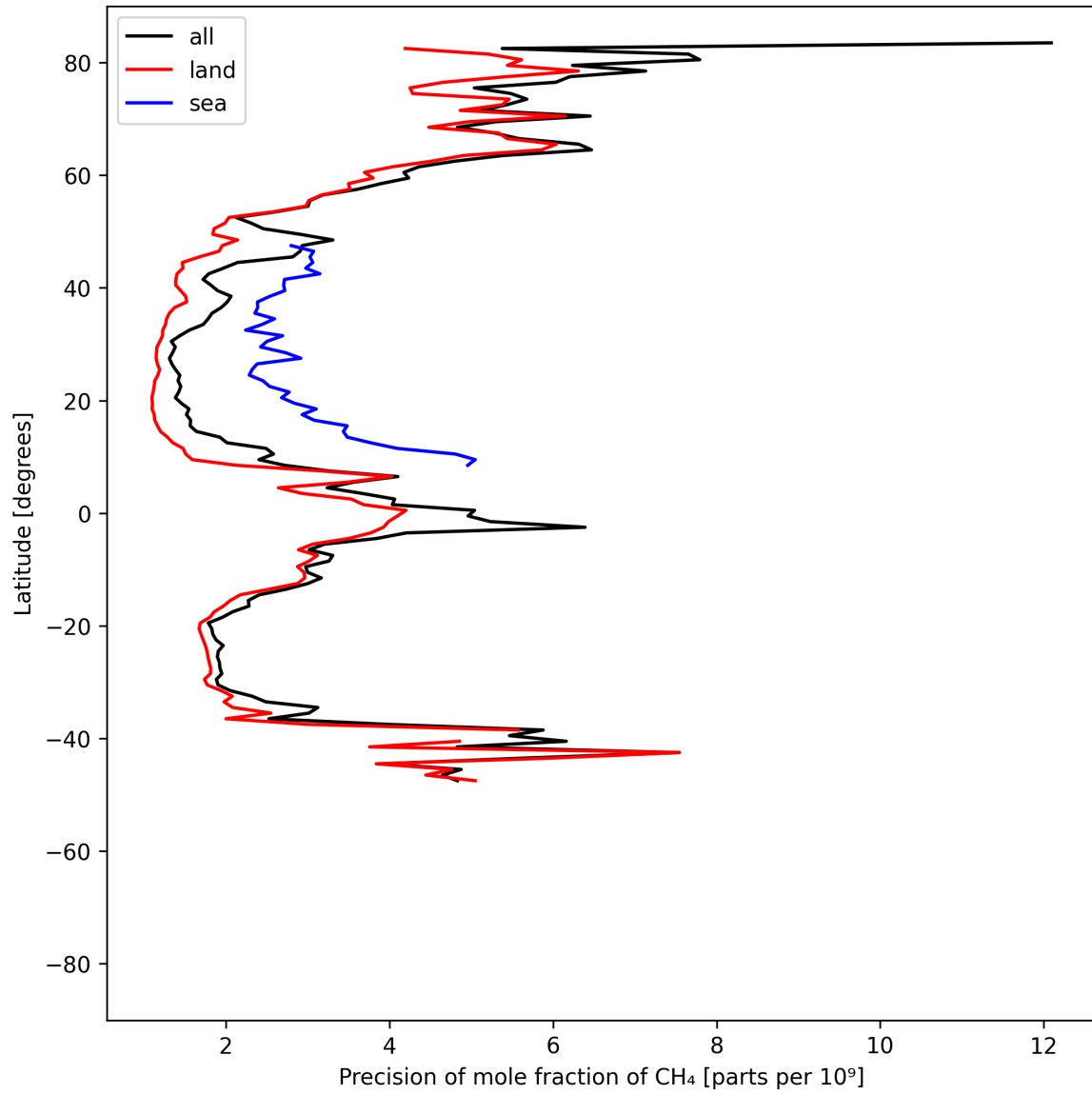
Figure 13: Zonal average of “Precision of mole fraction of CH 4 ” for 2025-06-01 to 2025-06-03.
