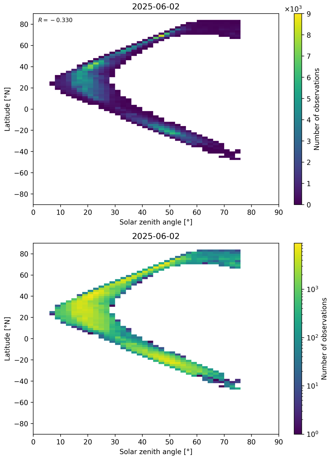
Figure 98: Scatter density plot of “Solar zenith angle” against “Latitude” for 2025-06-01 to 2025-06-03.
