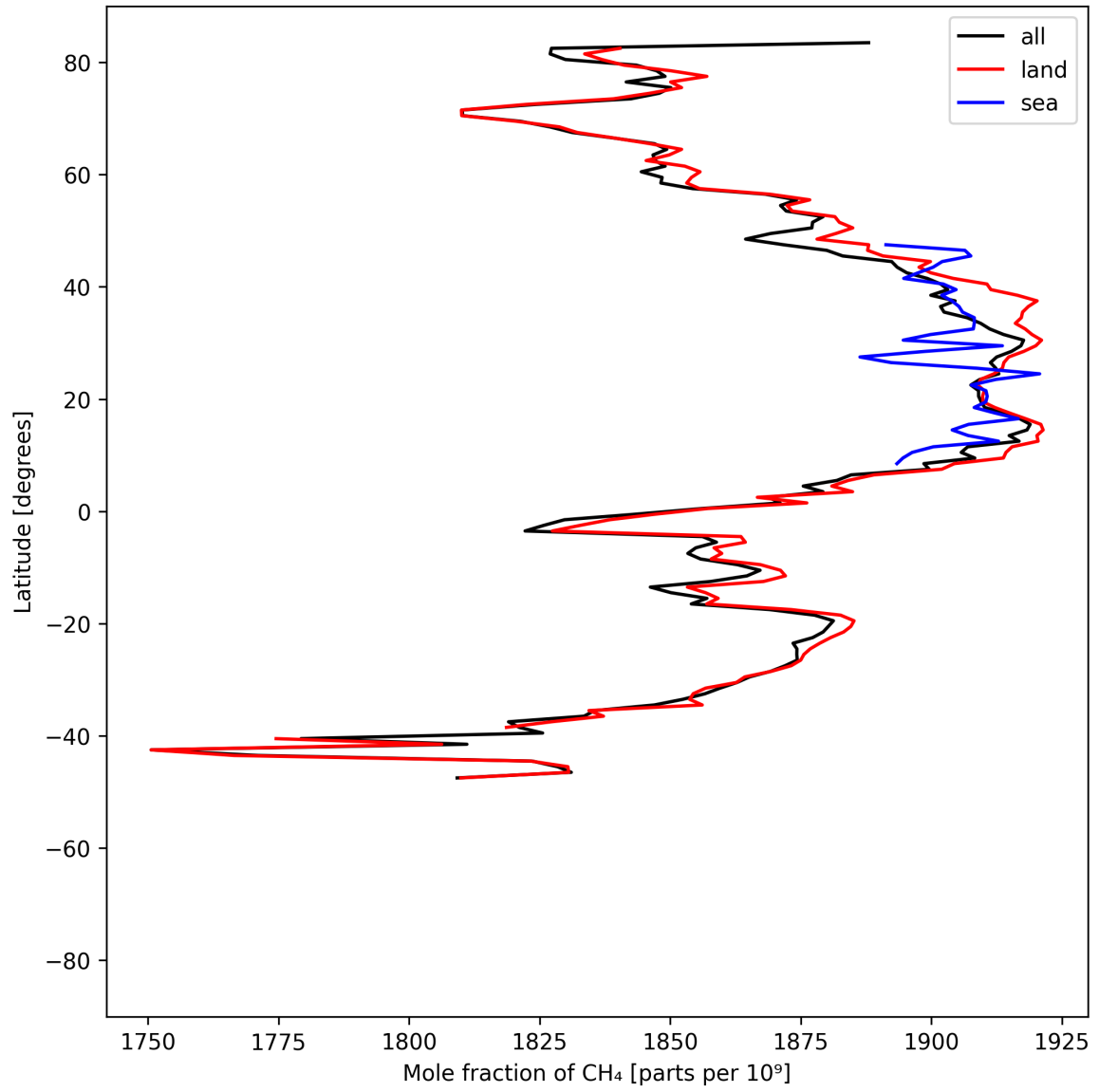
Figure 12: Zonal average of “Mole fraction of \text{CH}_4 ” for 2025-06-01 to 2025-06-03.
