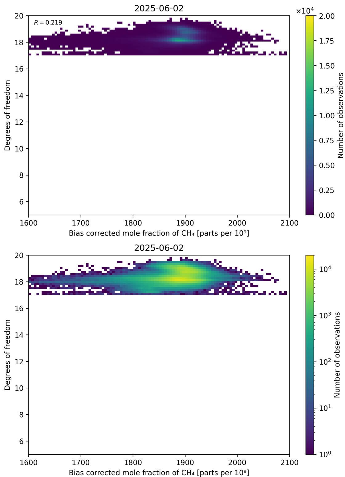
Figure 65: Scatter density plot of “Bias corrected mole fraction of CH 4 ” against “Degrees of freedom” for 2025-06-01 to 2025-06-03.
