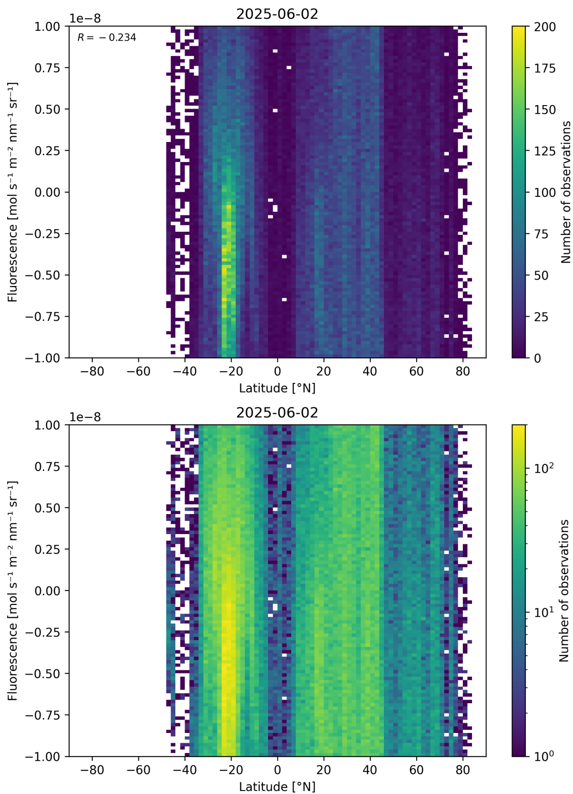
Figure 56: Scatter density plot of “Latitude” against “Fluorescence” for 2025-06-01 to 2025-06-03.
