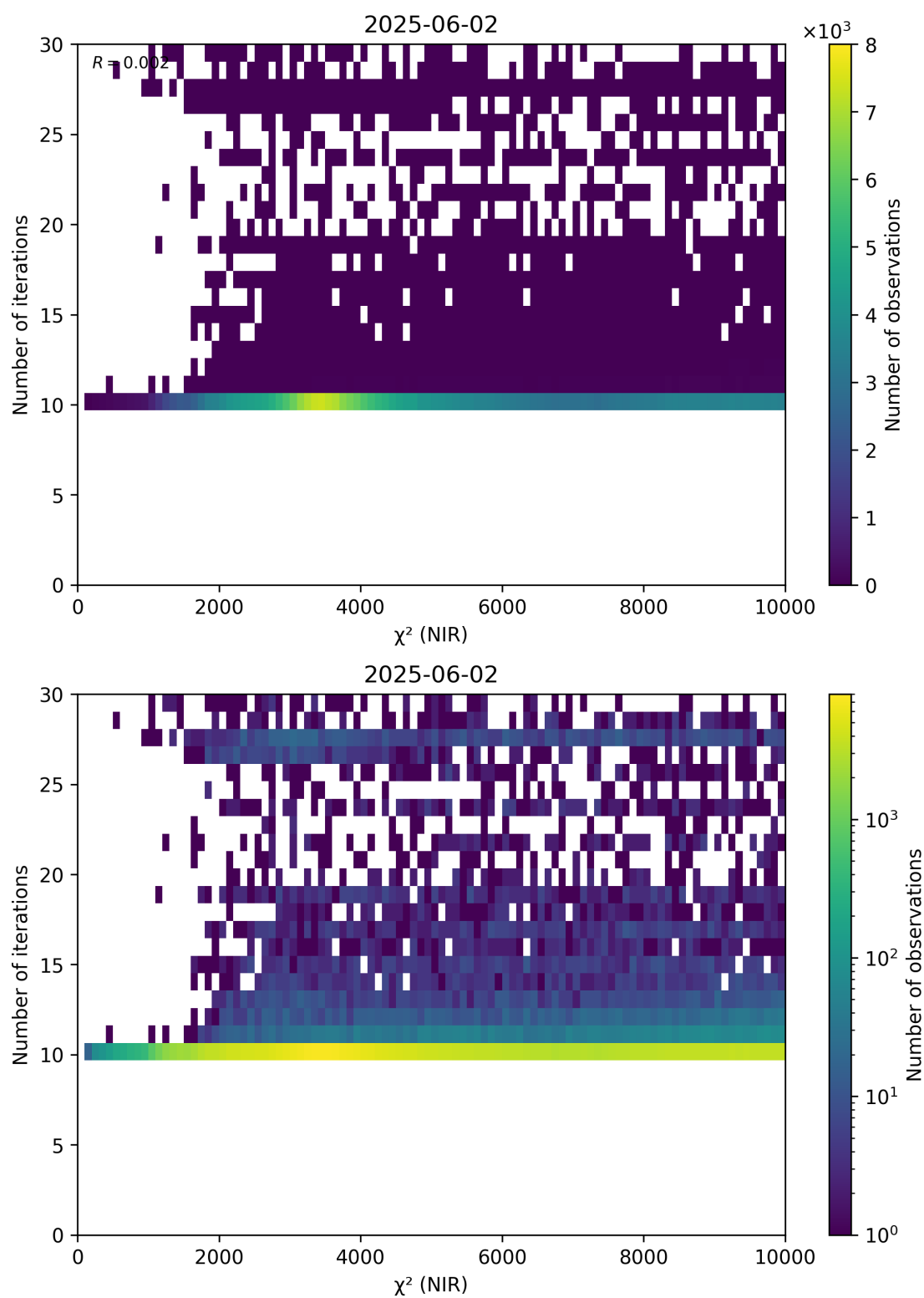
Figure 46: Scatter density plot of “ \chi^2 (NIR)” against “Number of iterations” for 2025-06-01 to 2025-06-03.
