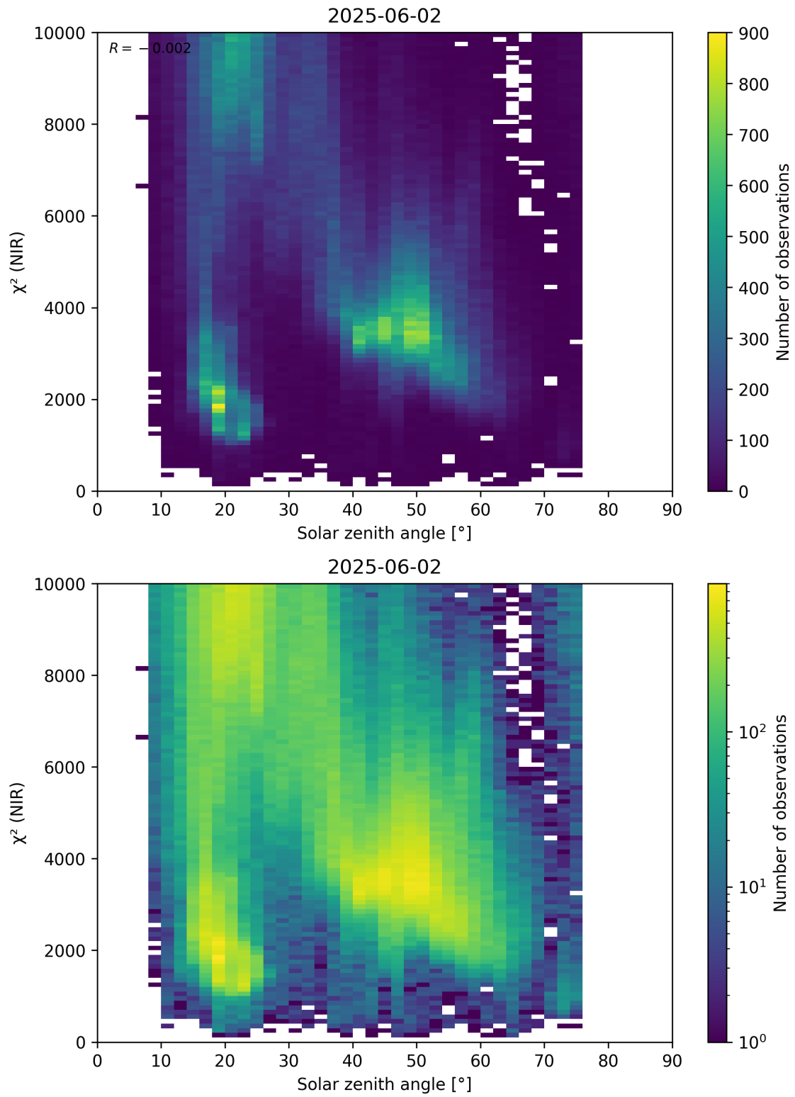
Figure 94: Scatter density plot of “Solar zenith angle” against “ \chi^2 (NIR)” for 2025-06-01 to 2025-06-03.
