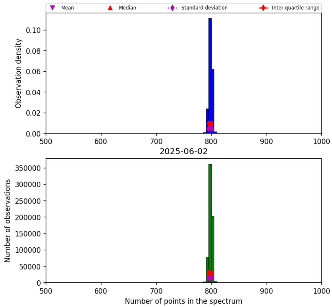
Figure 26: Histogram of “Number of points in the spectrum” for 2025-06-01 to 2025-06-03
