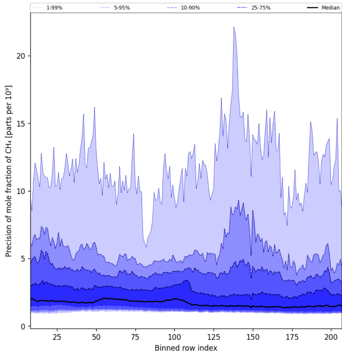
Figure 35: Along track statistics of “Precision of mole fraction of CH 4 ” for 2025-06-01 to 2025-06-03
