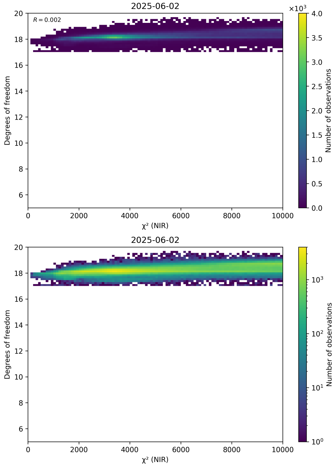
Figure 44: Scatter density plot of “ \chi^2 (NIR)” against “Degrees of freedom” for 2025-06-01 to 2025-06-03.
