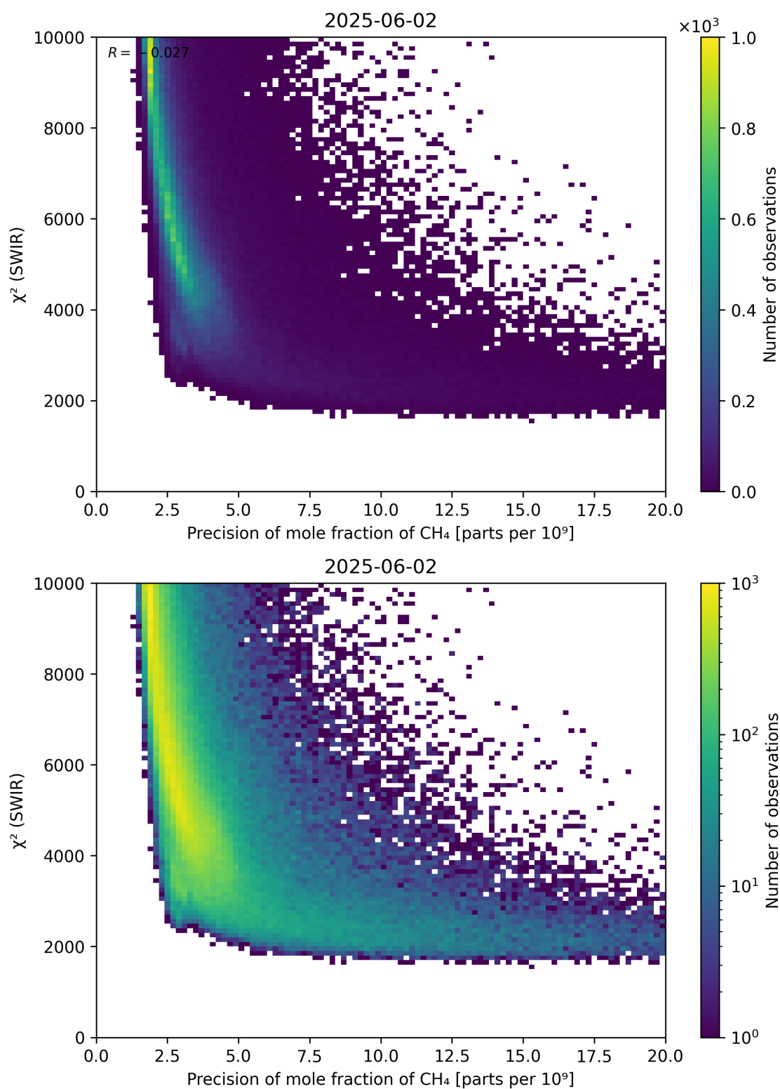
Figure 79: Scatter density plot of “Precision of mole fraction of \text{CH}_4 ” against “ \chi^2 (SWIR)” for 2025-06-01 to 2025-06-03.
