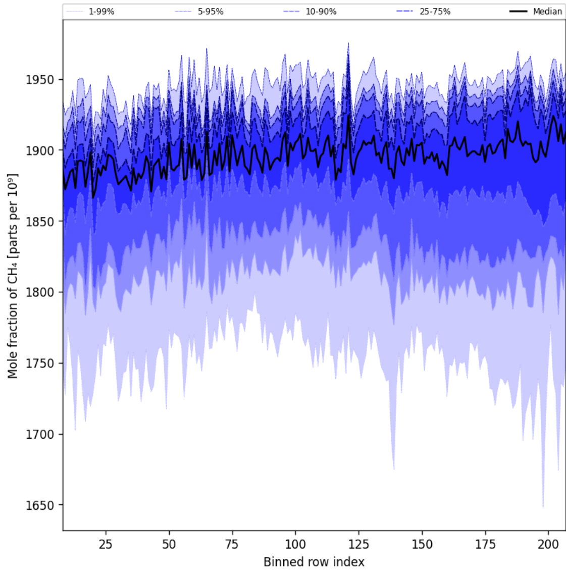
Figure 34: Along track statistics of “Mole fraction of CH 4 ” for 2025-06-01 to 2025-06-03
