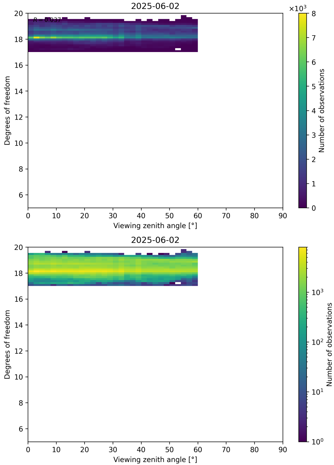
Figure 107: Scatter density plot of “Viewing zenith angle” against “Degrees of freedom” for 2025-06-01 to 2025-06-03.
