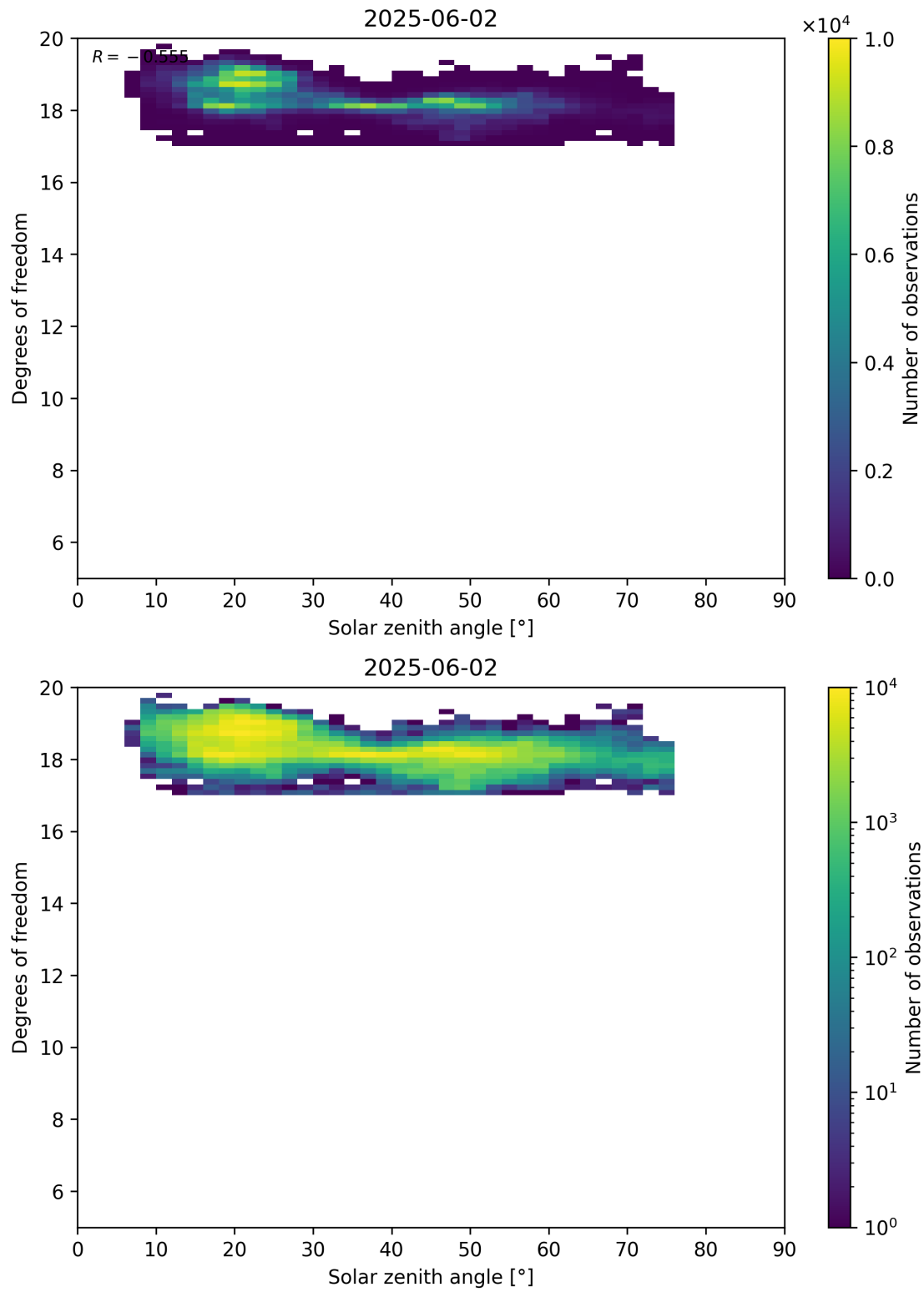
Figure 96: Scatter density plot of “Solar zenith angle” against “Degrees of freedom” for 2025-06-01 to 2025-06-03.
