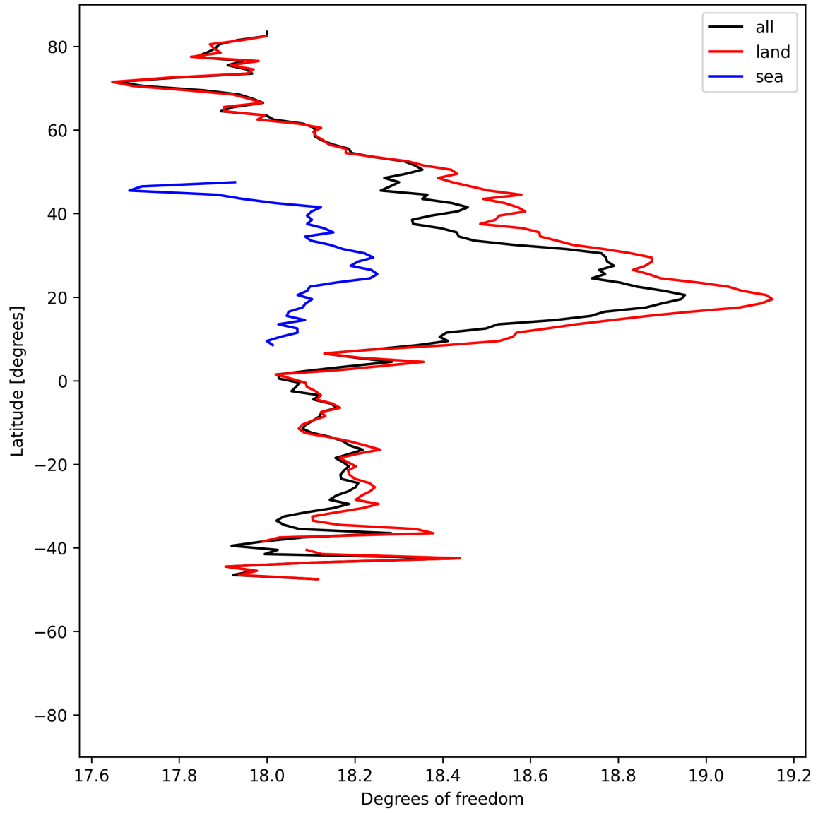
Figure 19: Zonal average of “Degrees of freedom” for 2025-06-01 to 2025-06-03.
