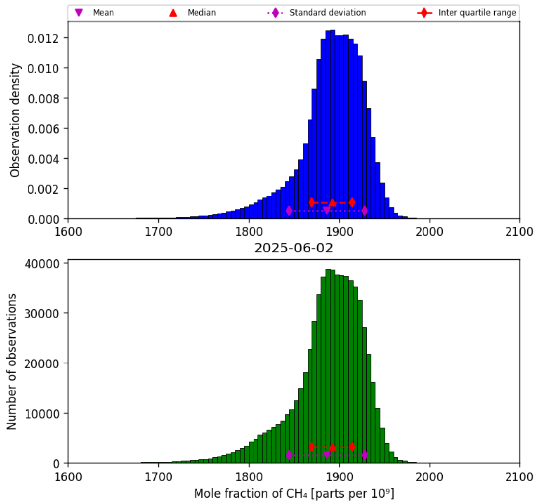
Figure 23: Histogram of “Mole fraction of CH 4 ” for 2025-06-01 to 2025-06-03
