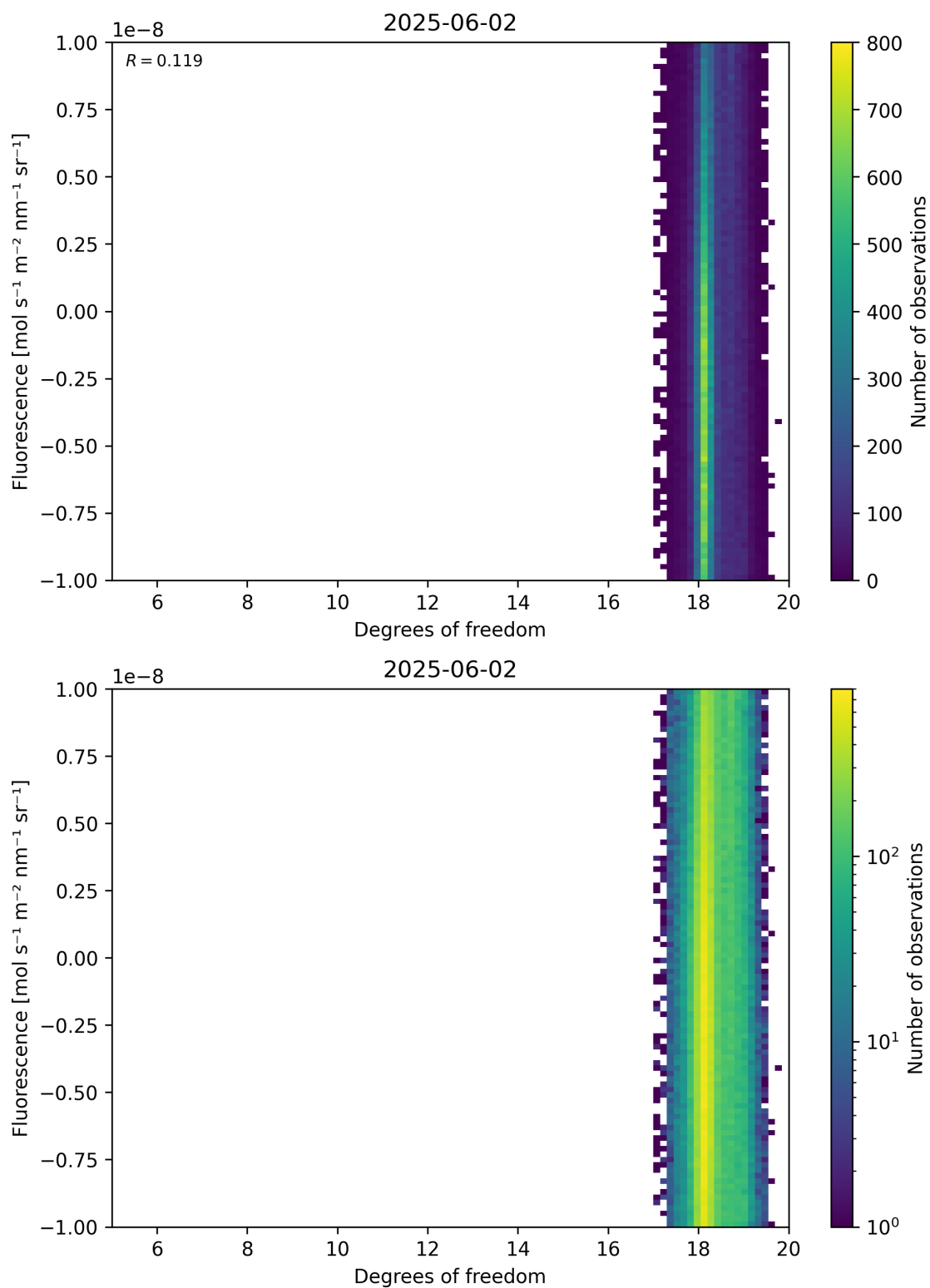
Figure 51: Scatter density plot of “Degrees of freedom” against “Fluorescence” for 2025-06-01 to 2025-06-03.
