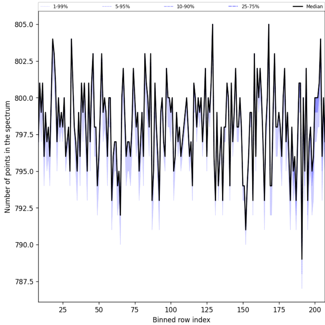
Figure 37: Along track statistics of “Number of points in the spectrum” for 2025-06-01 to 2025-06-03
