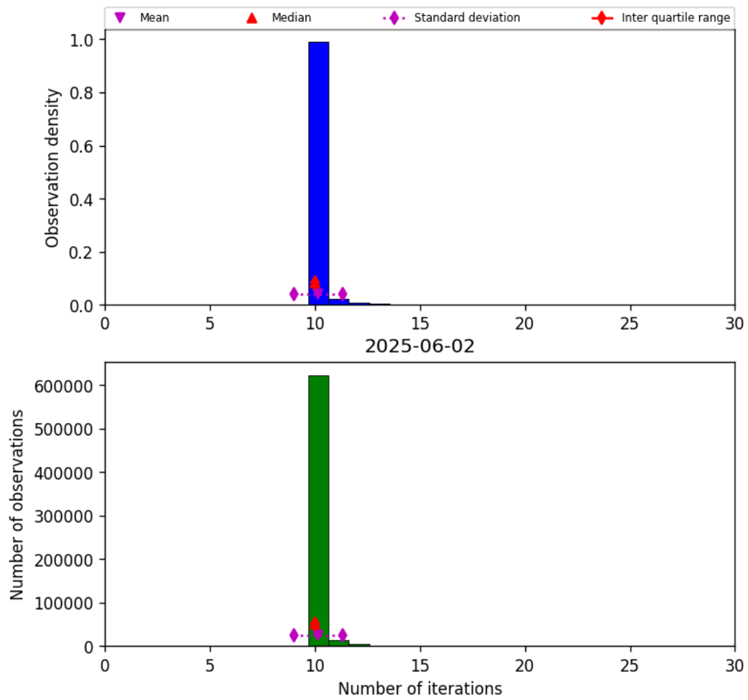
Figure 31: Histogram of “Number of iterations” for 2025-06-01 to 2025-06-03
