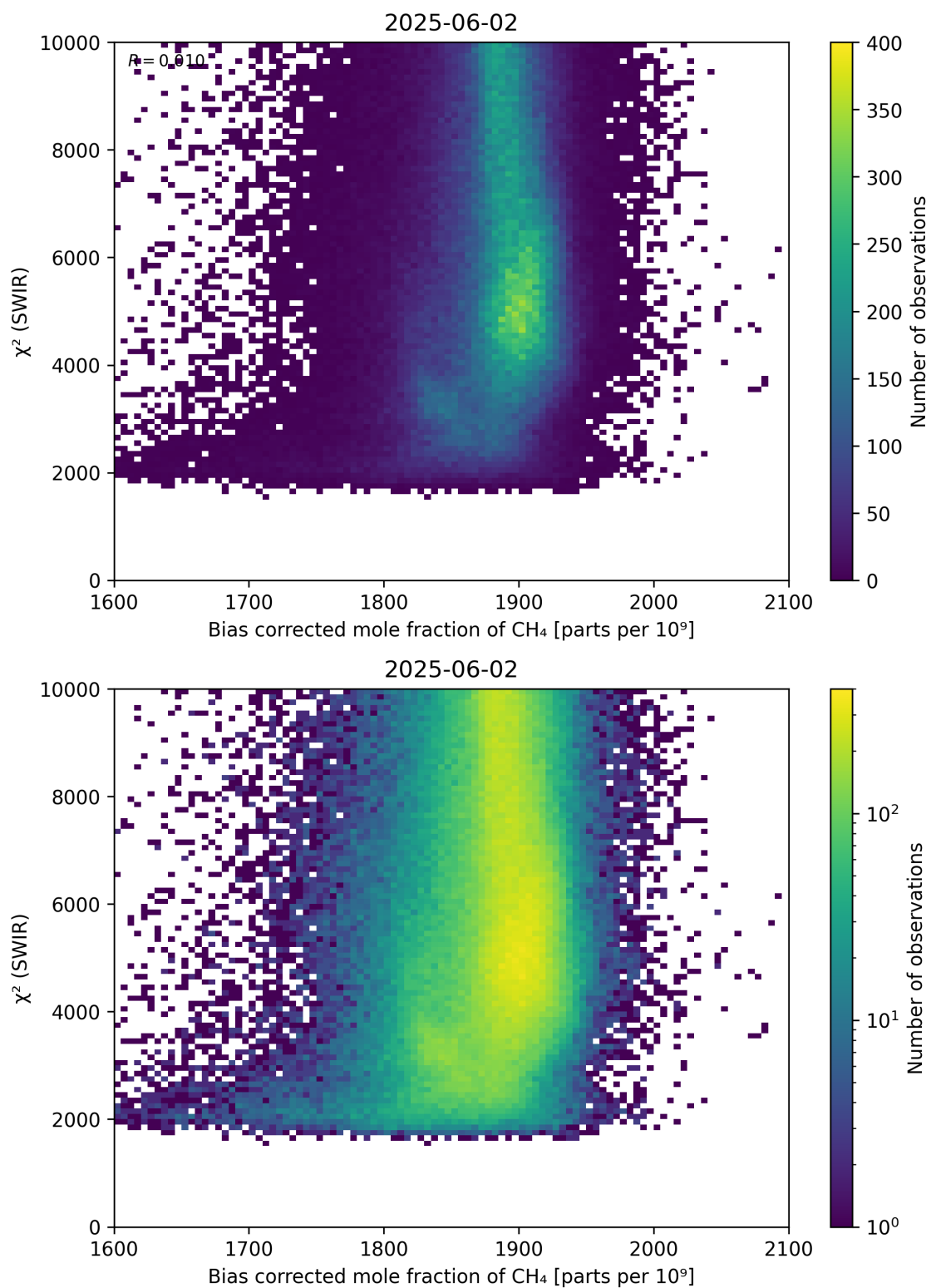
Figure 64: Scatter density plot of “Bias corrected mole fraction of \text{CH}_4 ” against “ \chi^2 (SWIR)” for 2025-06-01 to 2025-06-03.
