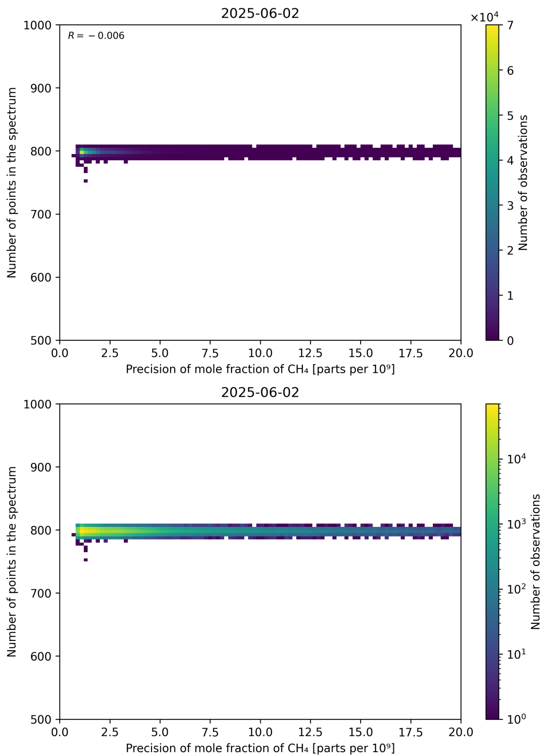
Figure 84: Scatter density plot of “Precision of mole fraction of CH 4 ” against “Number of points in the spectrum” for 2025-06-01 to 2025-06-03.
