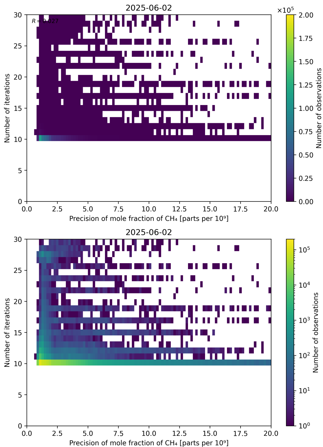
Figure 83: Scatter density plot of “Precision of mole fraction of CH 4 ” against “Number of iterations” for 2025-06-01 to 2025-06-03.
