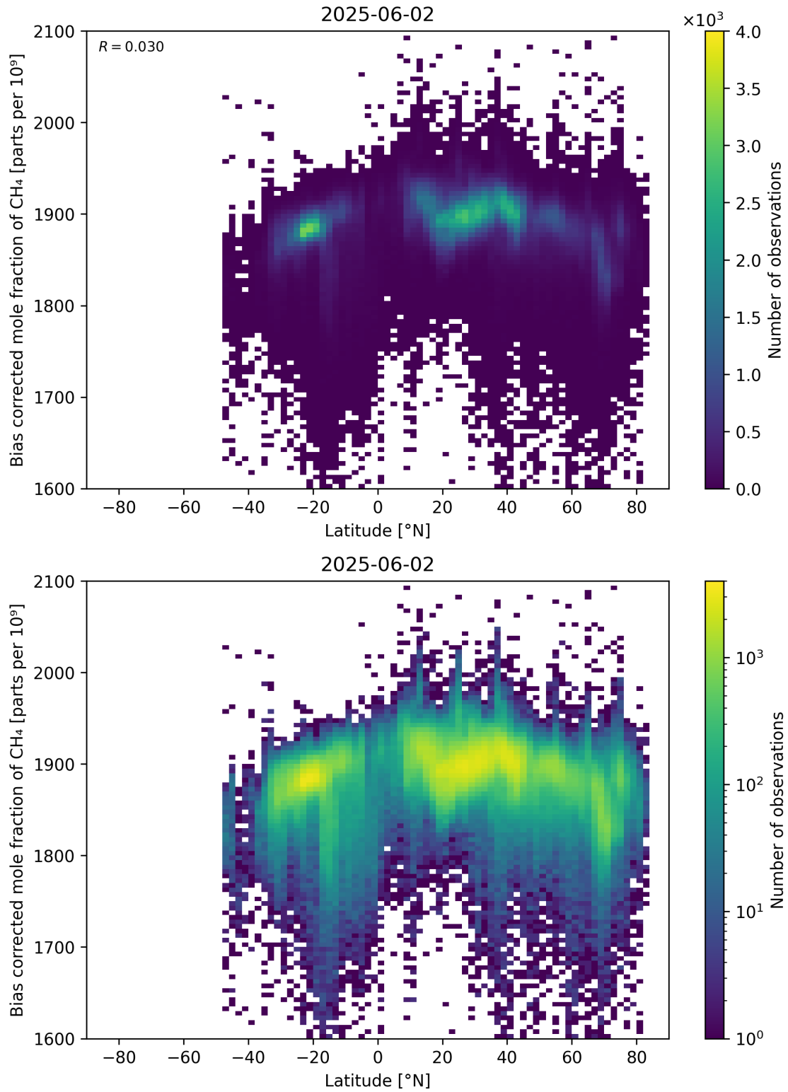
Figure 58: Scatter density plot of “Latitude” against “Bias corrected mole fraction of CH 4 ” for 2025-06-01 to 2025-06-03.
