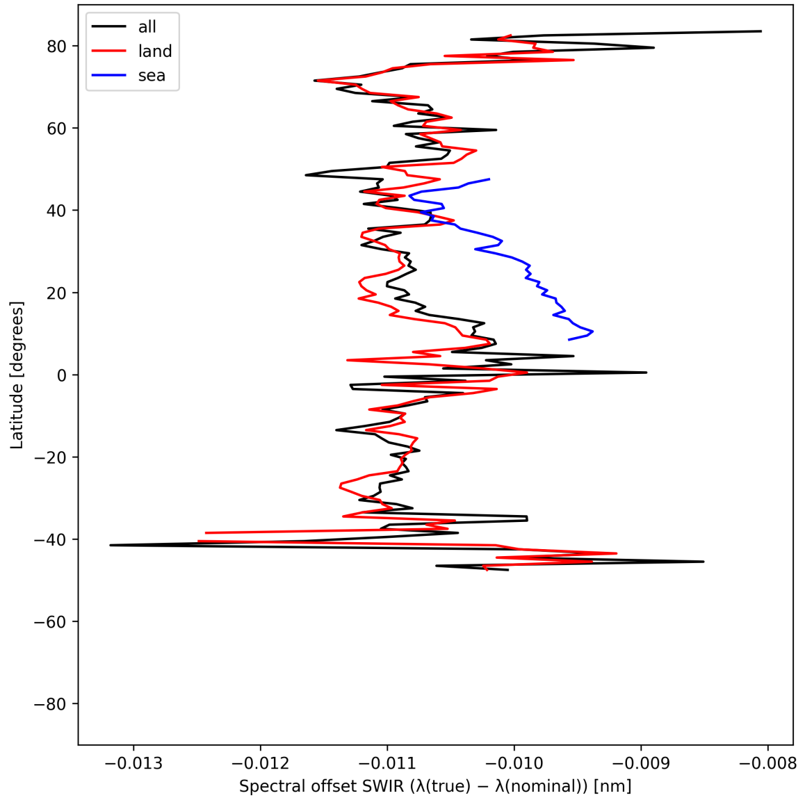
Figure 16: Zonal average of “Spectral offset SWIR ( \lambda_{\text{true}} - \lambda_{\text{nominal}} )” for 2025-06-01 to 2025-06-03.
