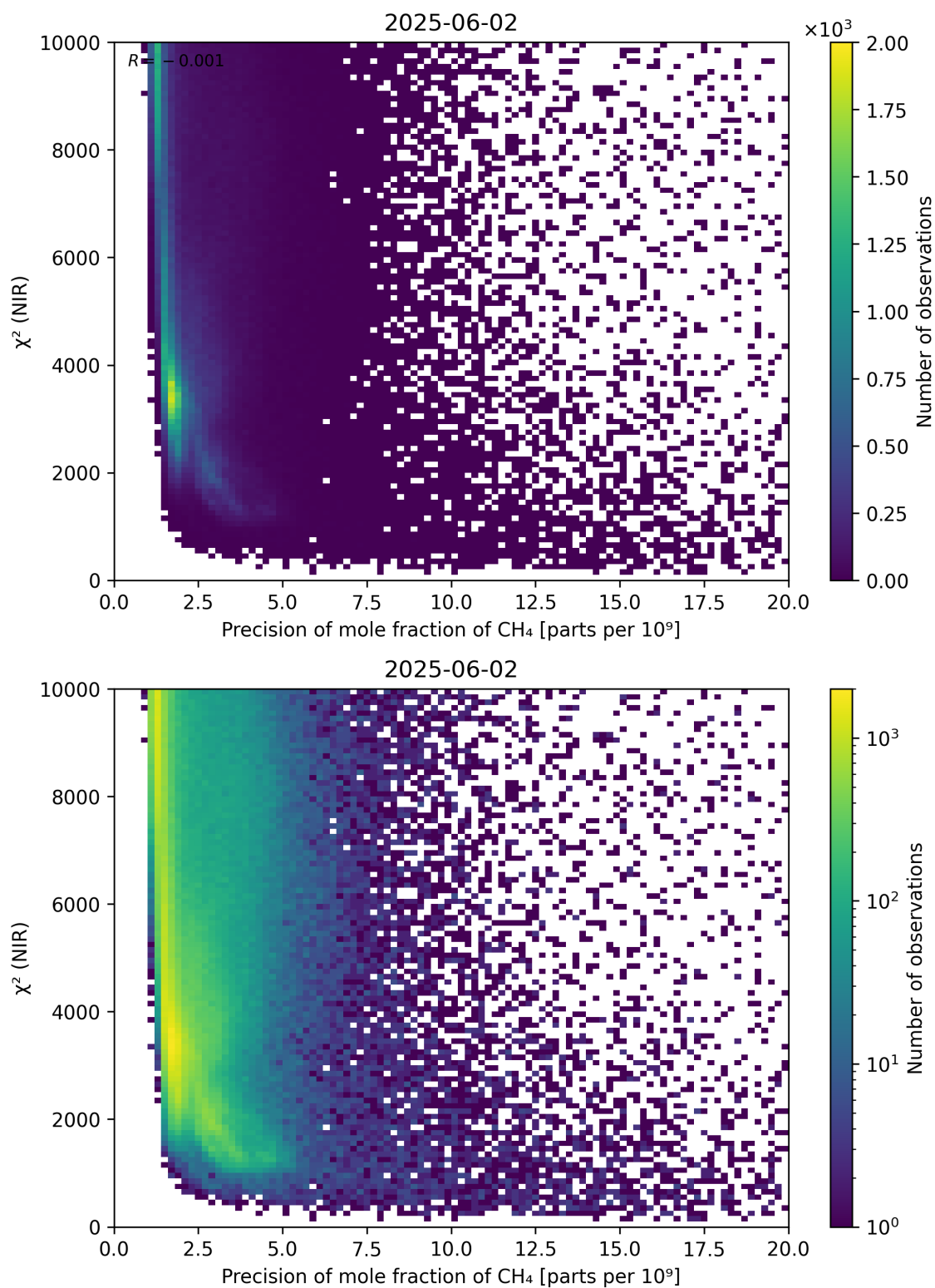
Figure 78: Scatter density plot of “Precision of mole fraction of CH 4 ” against “ \chi^2 (NIR)” for 2025-06-01 to 2025-06-03.
