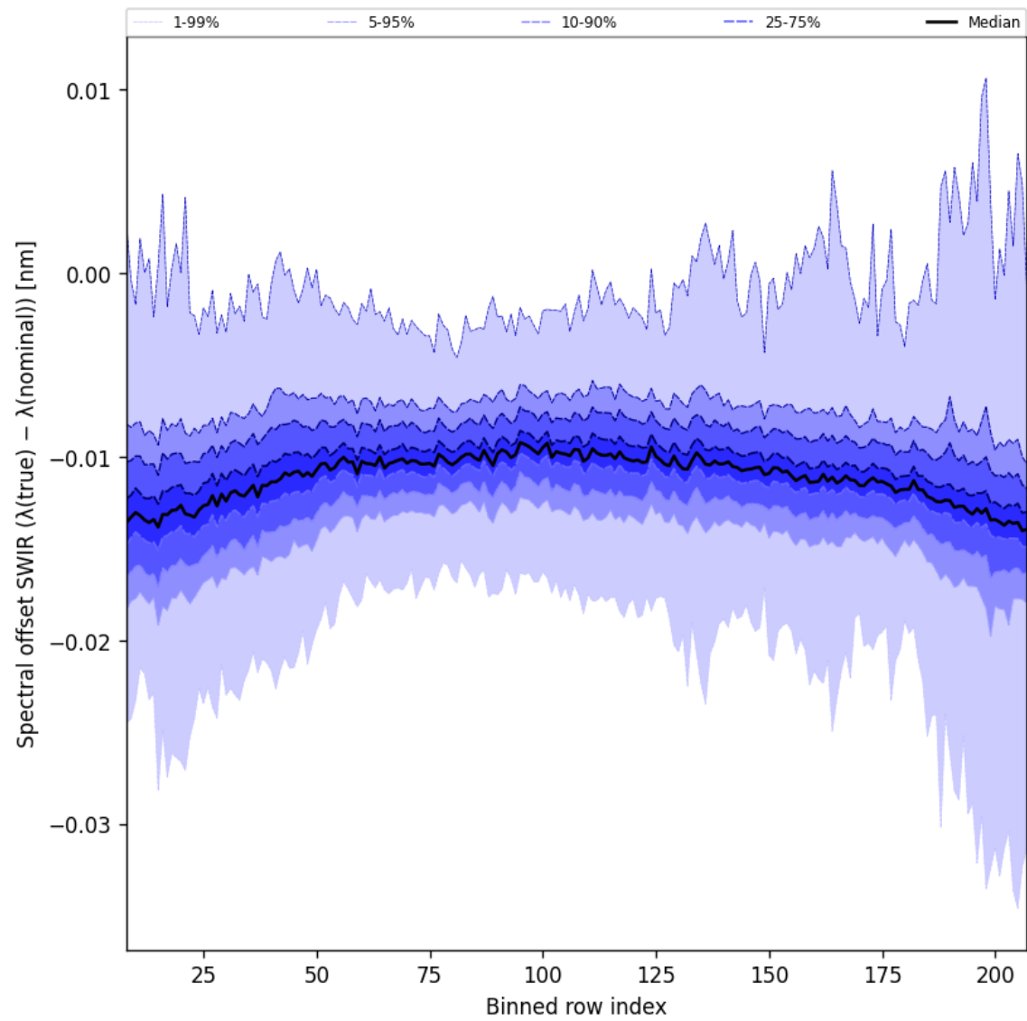
Figure 38: Along track statistics of “Spectral offset SWIR ( \lambda_{\text{true}} - \lambda_{\text{nominal}} )” for 2025-06-01 to 2025-06-03
