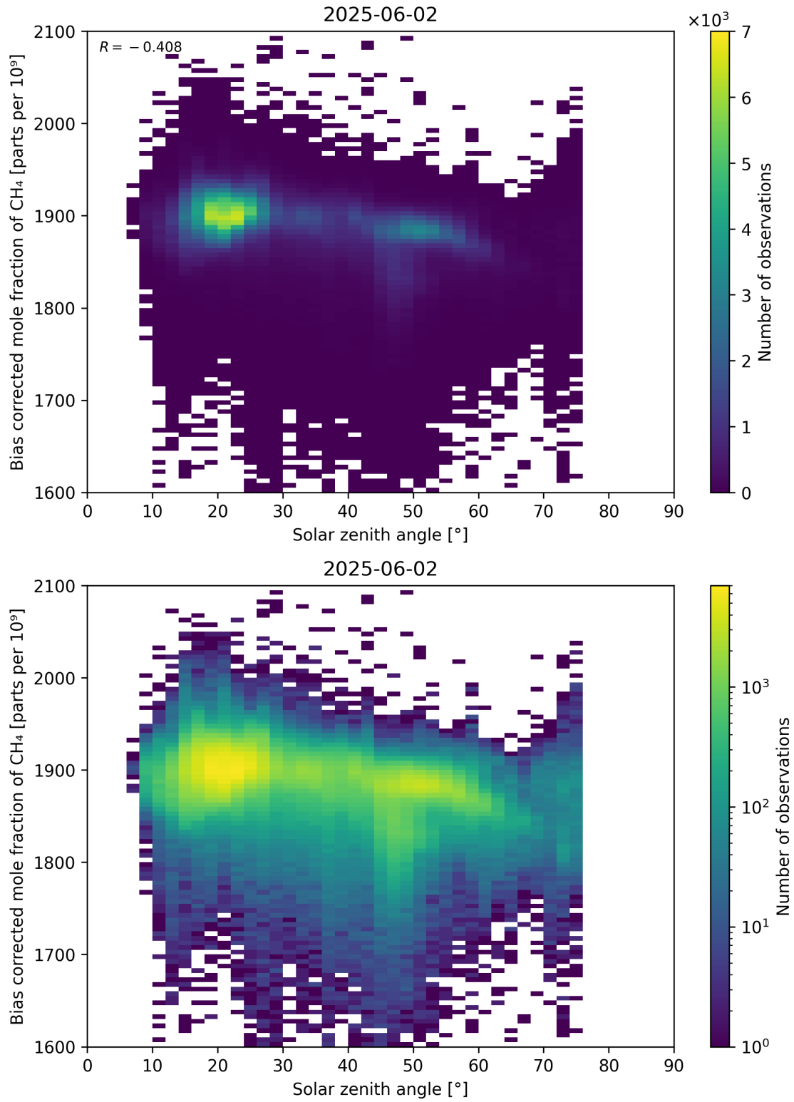
Figure 100: Scatter density plot of “Solar zenith angle” against “Bias corrected mole fraction of CH 4 ” for 2025-06-01 to 2025-06-03.
