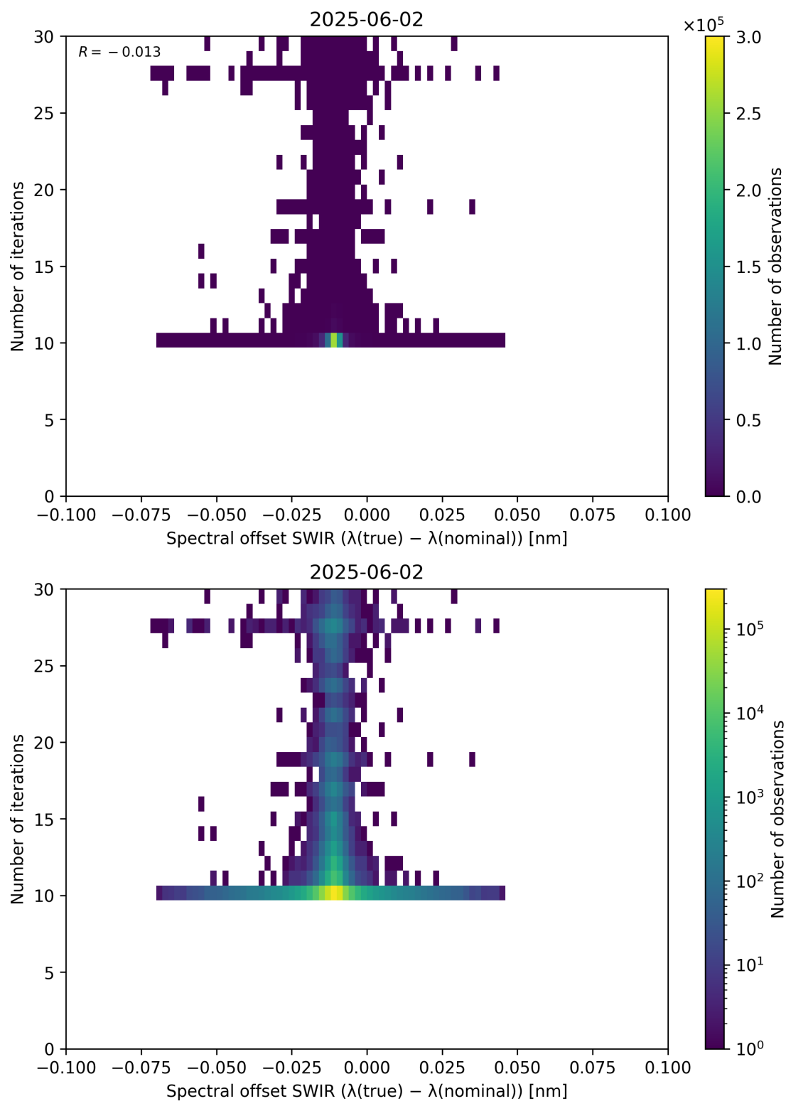
Figure 121: Scatter density plot of “Spectral offset SWIR ( \lambda_{\text{true}} - \lambda_{\text{nominal}} )” against “Number of iterations” for 2025-06-01 to 2025-06-03.
