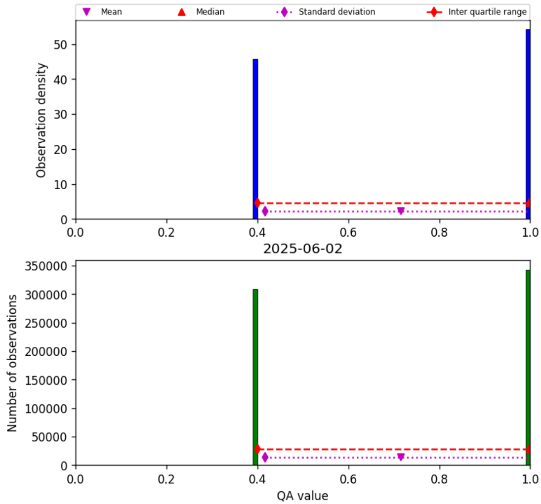
Figure 22: Histogram of “QA value” for 2025-06-01 to 2025-06-03
