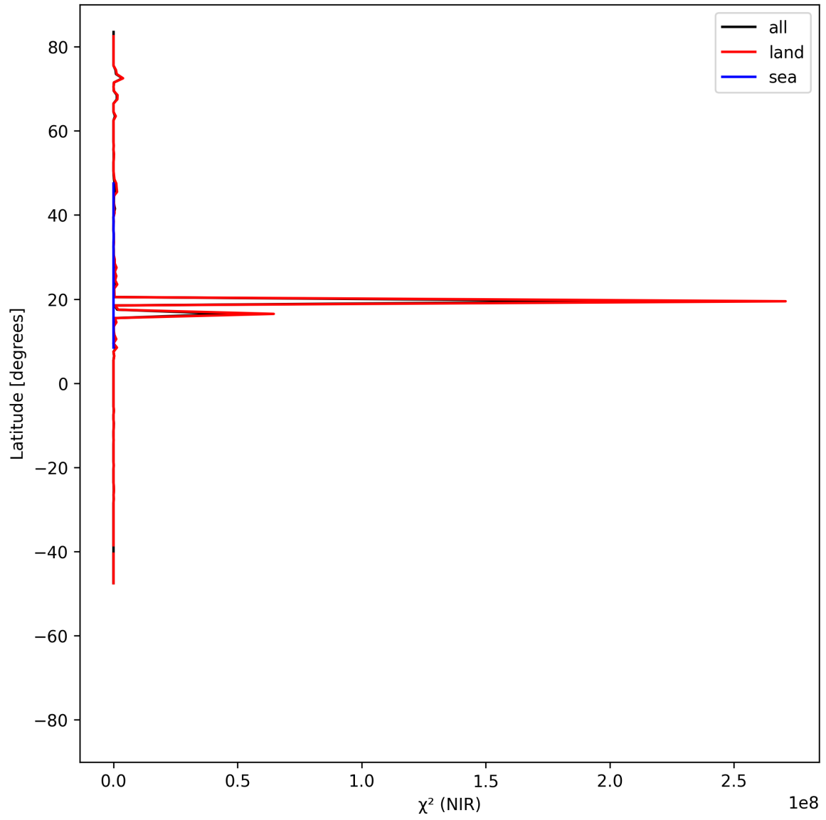
Figure 18: Zonal average of “ \chi^2 (NIR)” for 2025-06-01 to 2025-06-03.
