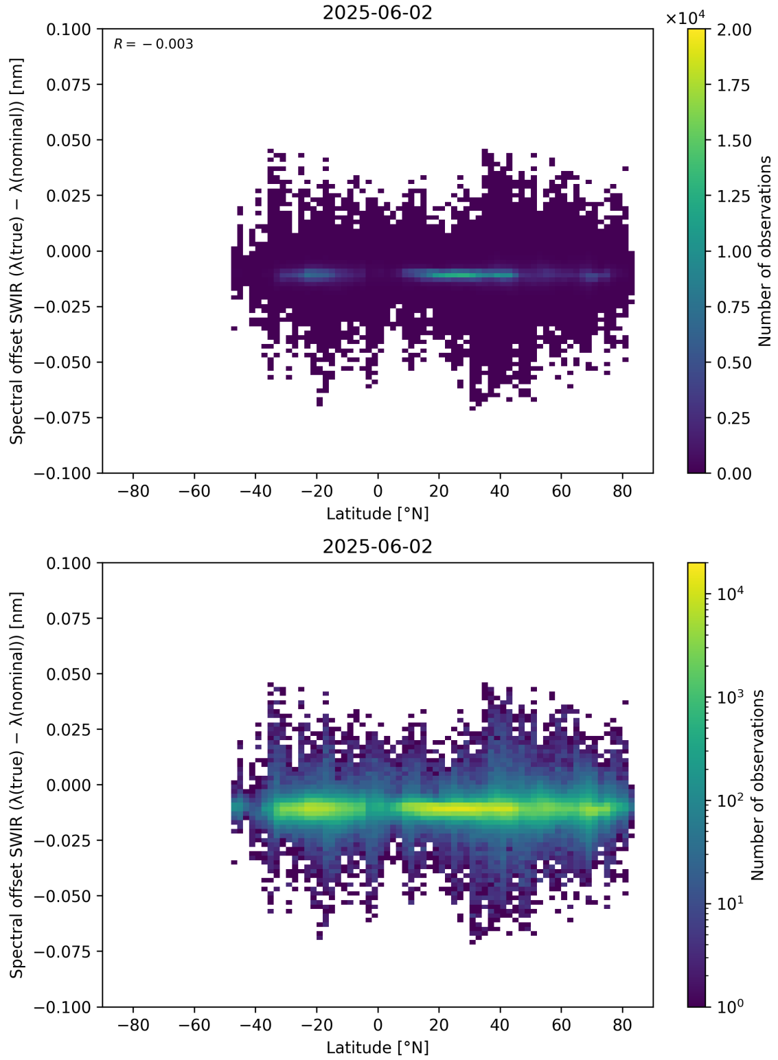
Figure 62: Scatter density plot of “Latitude” against “Spectral offset SWIR ( \lambda_{\text{true}} - \lambda_{\text{nominal}} )” for 2025-06-01 to 2025-06-03.
