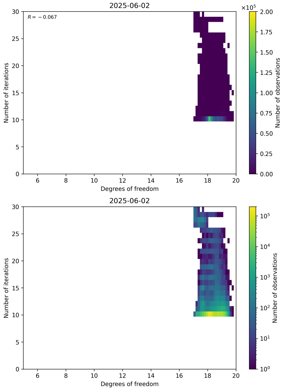
Figure 52: Scatter density plot of “Degrees of freedom” against “Number of iterations” for 2025-06-01 to 2025-06-03.
