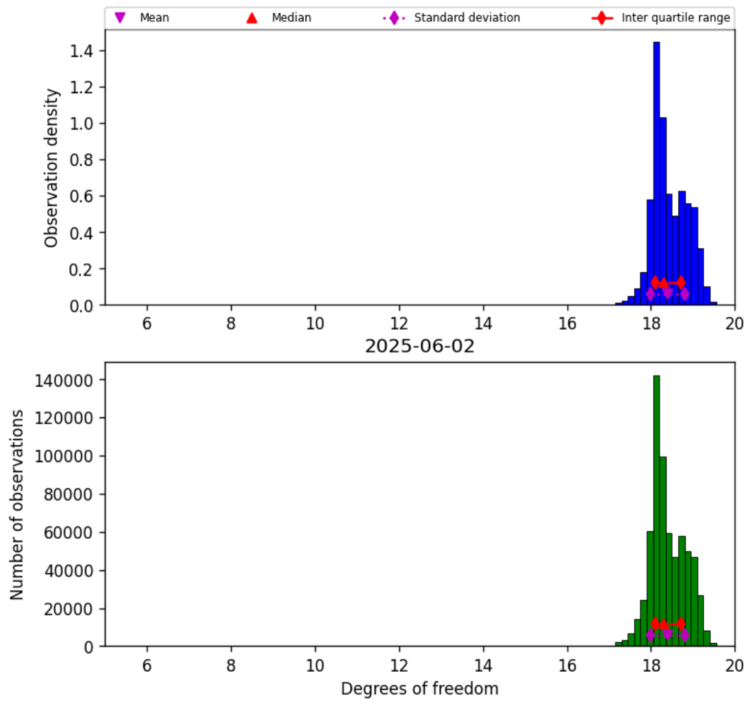
Figure 30: Histogram of “Degrees of freedom” for 2025-06-01 to 2025-06-03
