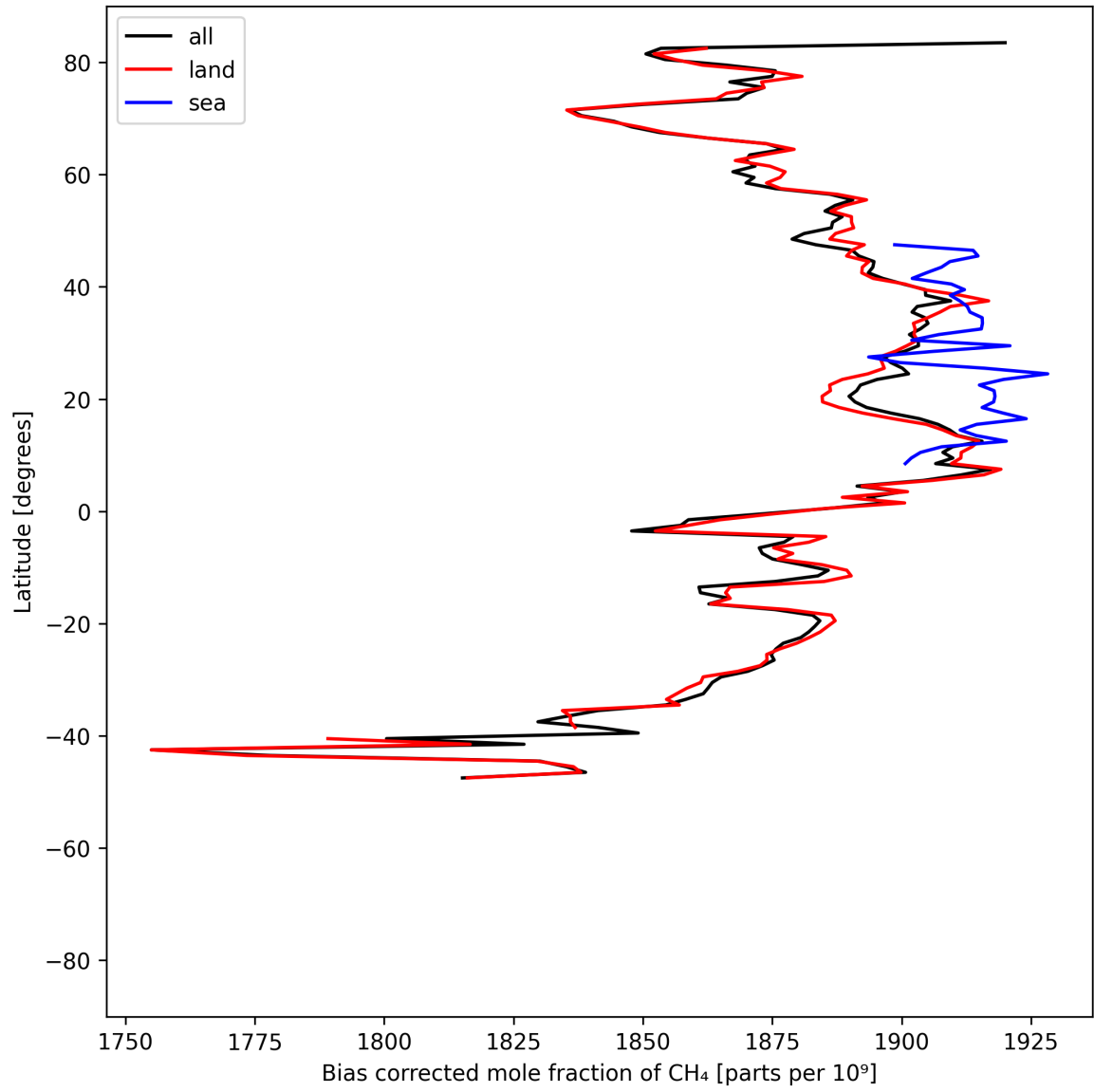
Figure 14: Zonal average of “Bias corrected mole fraction of CH 4 ” for 2025-06-01 to 2025-06-03.
