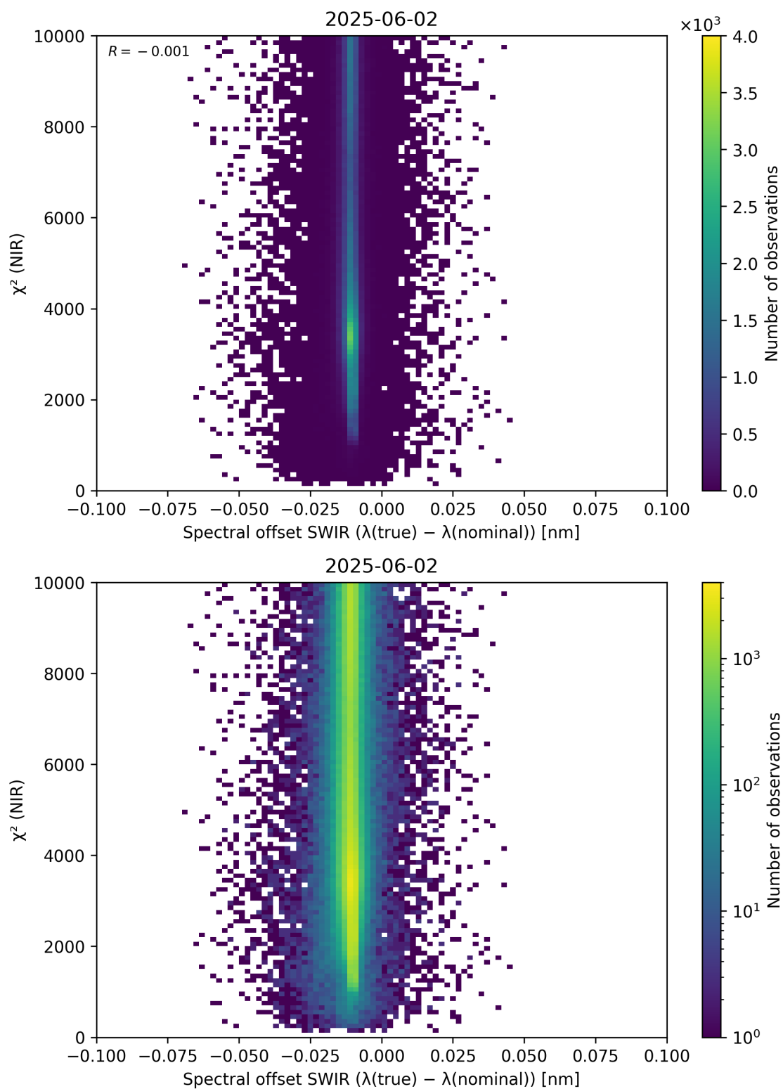
Figure 117: Scatter density plot of “Spectral offset SWIR ( \lambda_{\text{true}} - \lambda_{\text{nominal}} )” against “ \chi^2 (NIR)” for 2025-06-01 to 2025-06-03.
