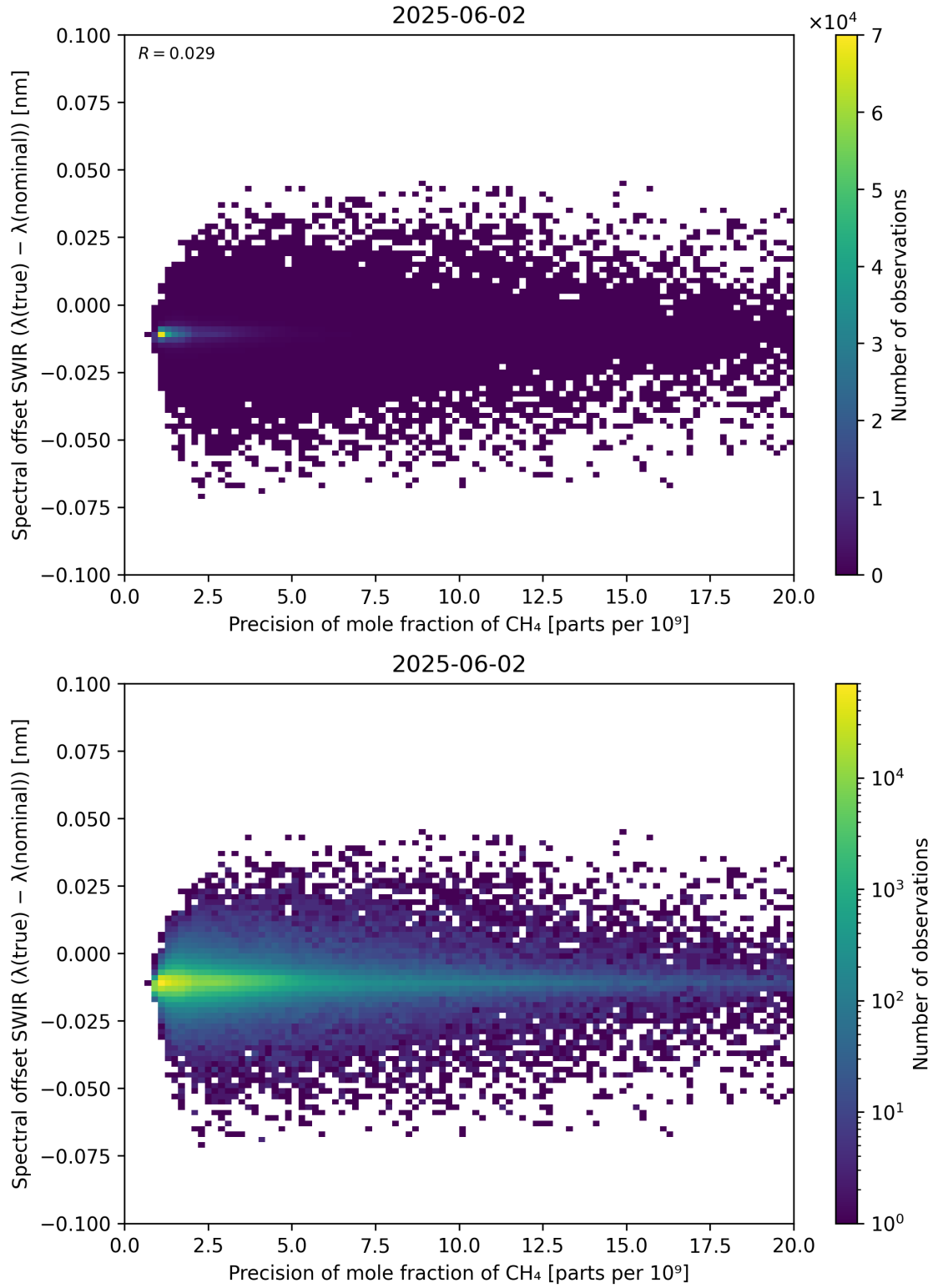
Figure 85: Scatter density plot of “Precision of mole fraction of CH 4 ” against “Spectral offset SWIR ( \lambda_{\text{true}} - \lambda_{\text{nominal}} )” for 2025-06-01 to 2025-06-03.
