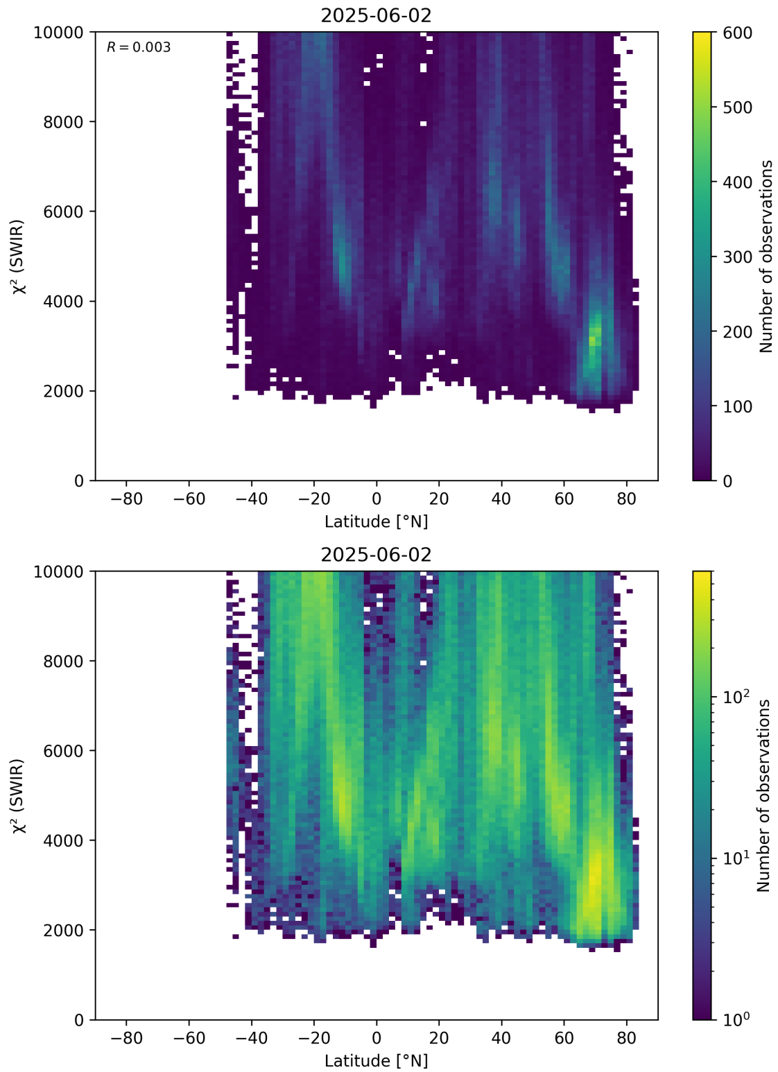
Figure 54: Scatter density plot of “Latitude” against “ \chi^2 (SWIR)” for 2025-06-01 to 2025-06-03.
