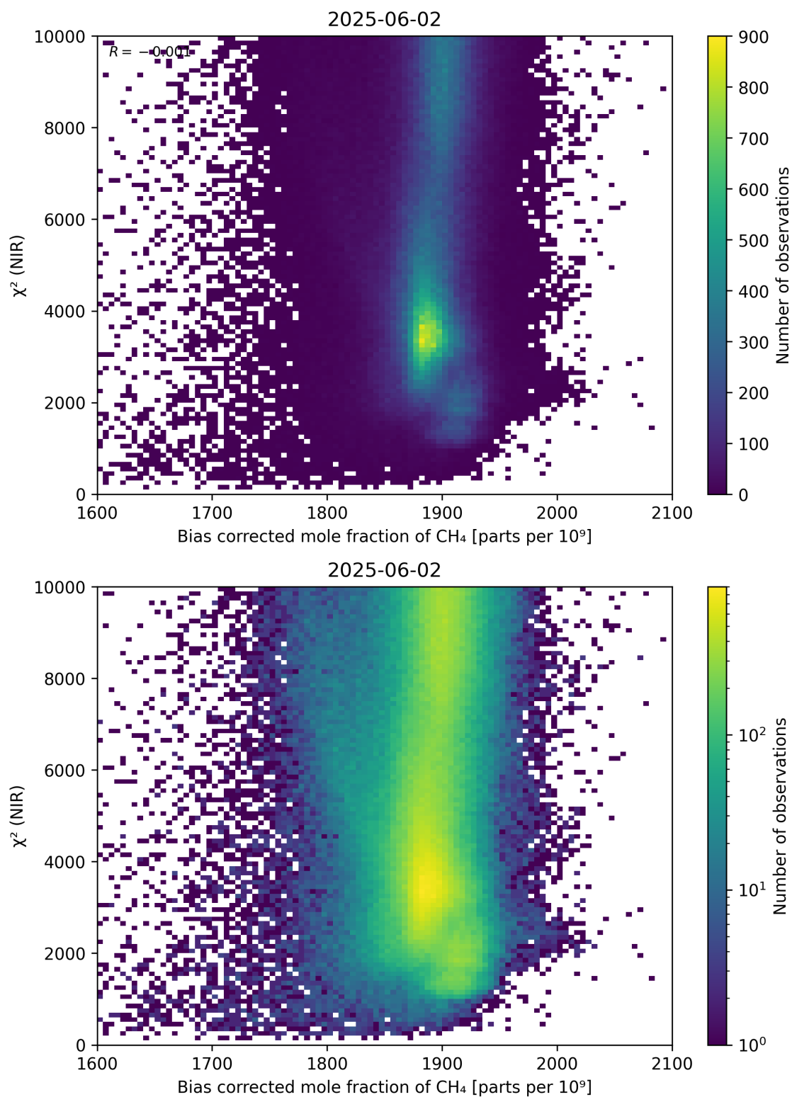
Figure 63: Scatter density plot of “Bias corrected mole fraction of \text{CH}_4 ” against “ \chi^2 (NIR)” for 2025-06-01 to 2025-06-03.
