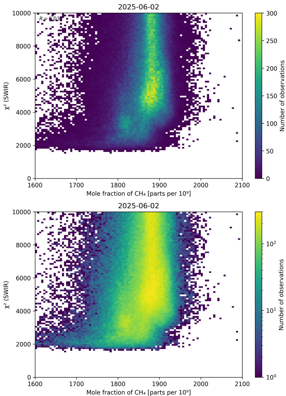
Figure 71: Scatter density plot of “Mole fraction of \text{CH}_4 ” against “ \chi^2 (SWIR)” for 2025-06-01 to 2025-06-03.
