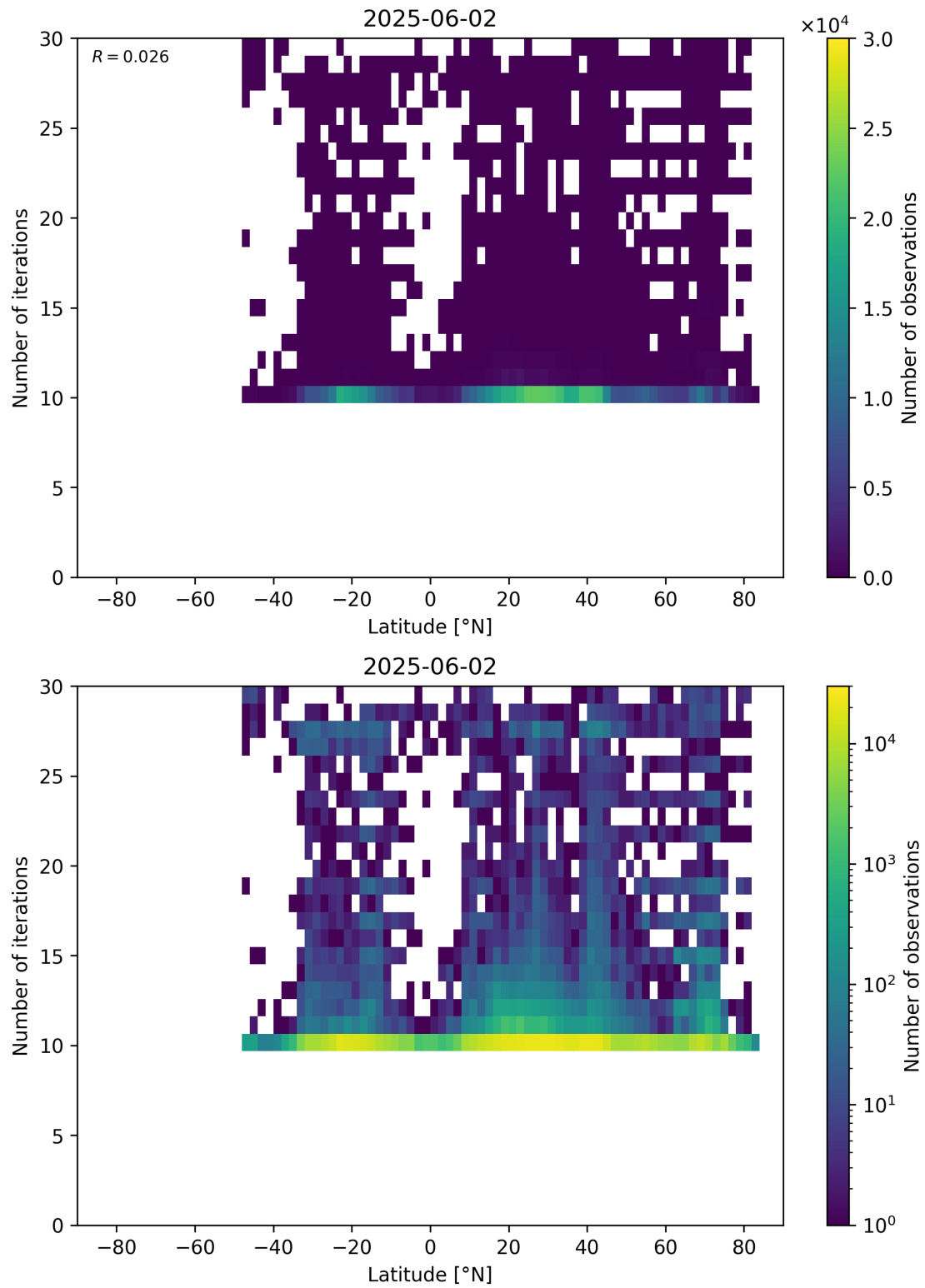
Figure 60: Scatter density plot of “Latitude” against “Number of iterations” for 2025-06-01 to 2025-06-03.
