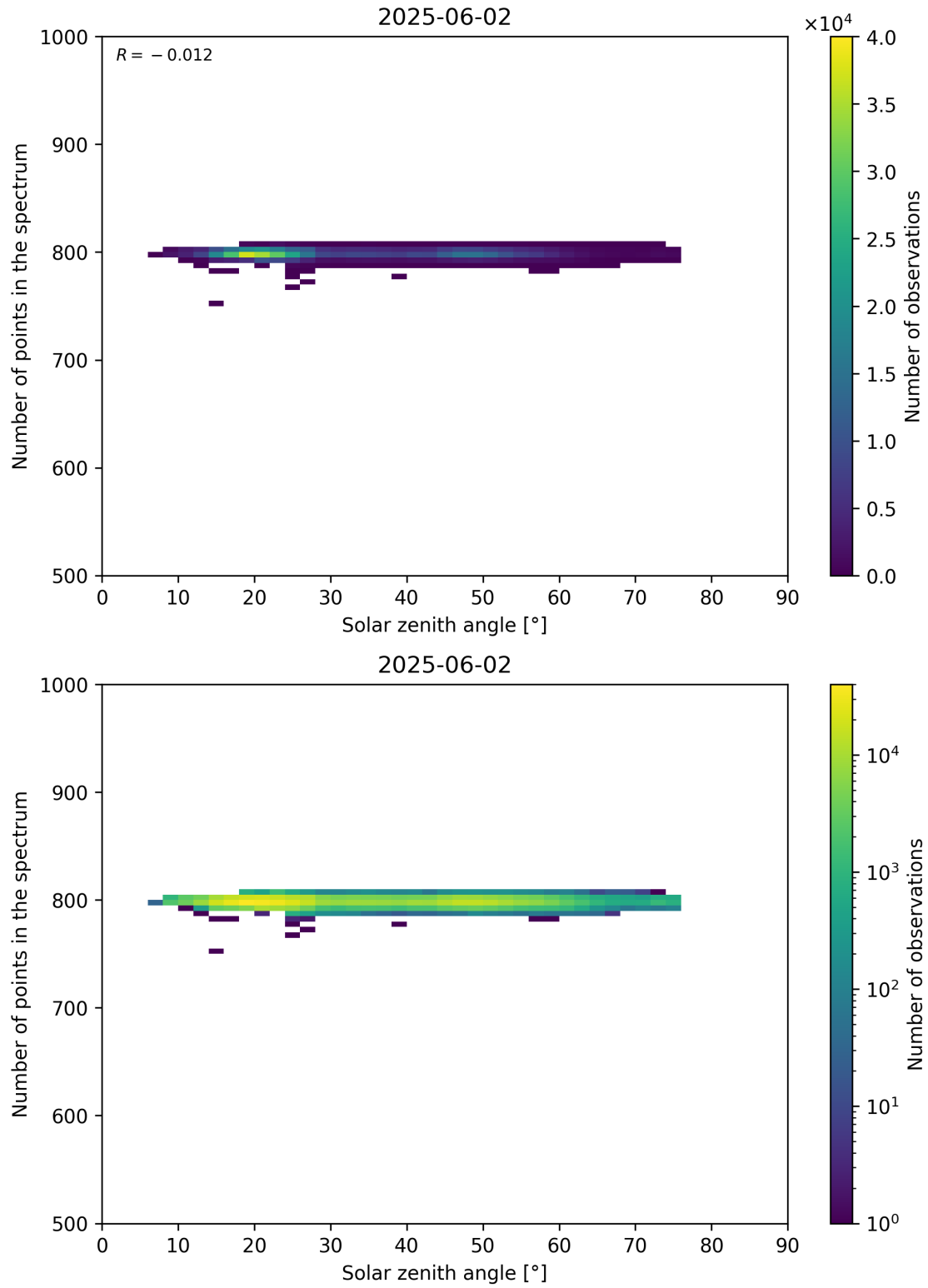
Figure 103: Scatter density plot of “Solar zenith angle” against “Number of points in the spectrum” for 2025-06-01 to 2025-06-03.
