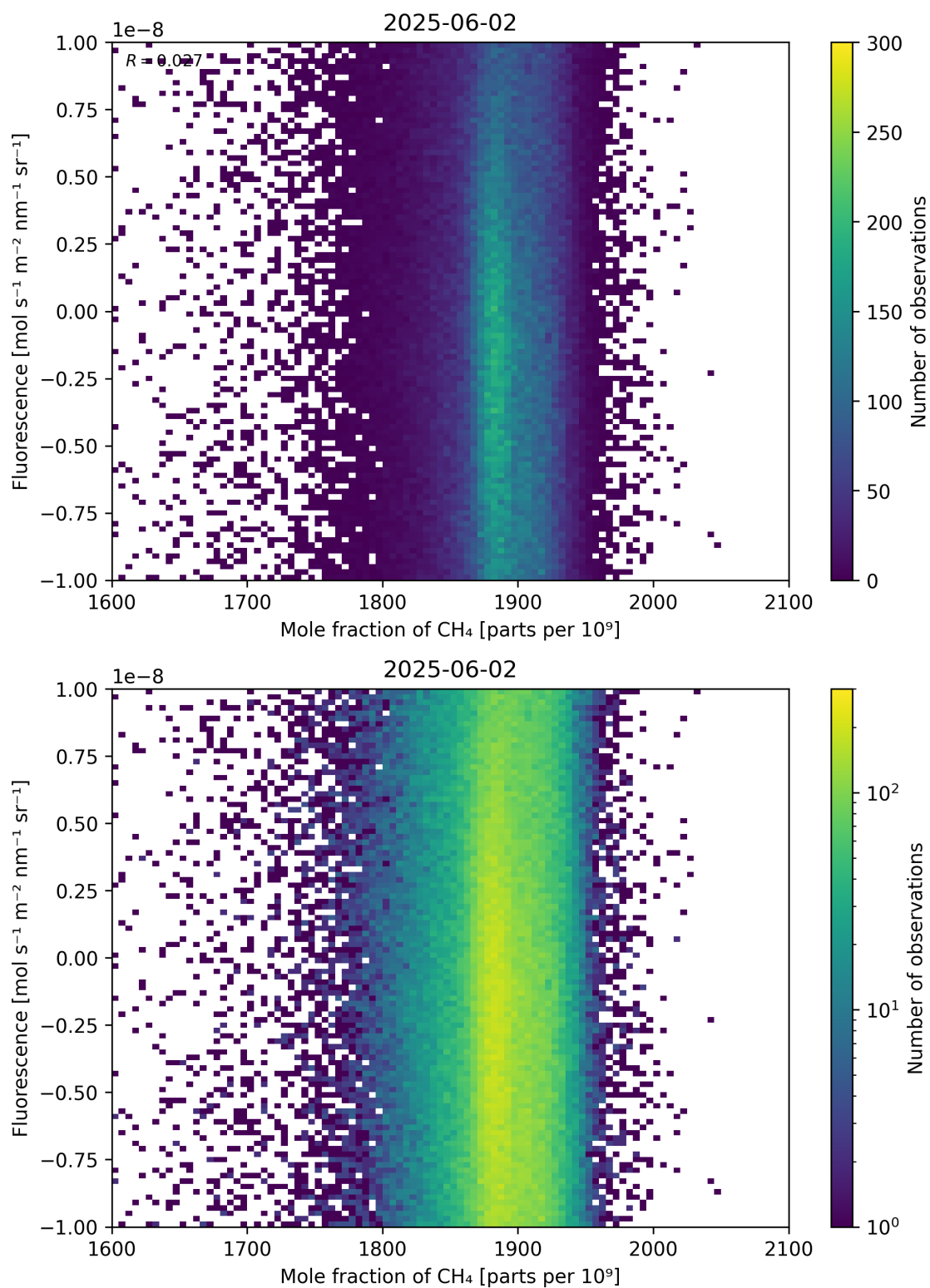
Figure 73: Scatter density plot of “Mole fraction of \text{CH}_4 ” against “Fluorescence” for 2025-06-01 to 2025-06-03.
