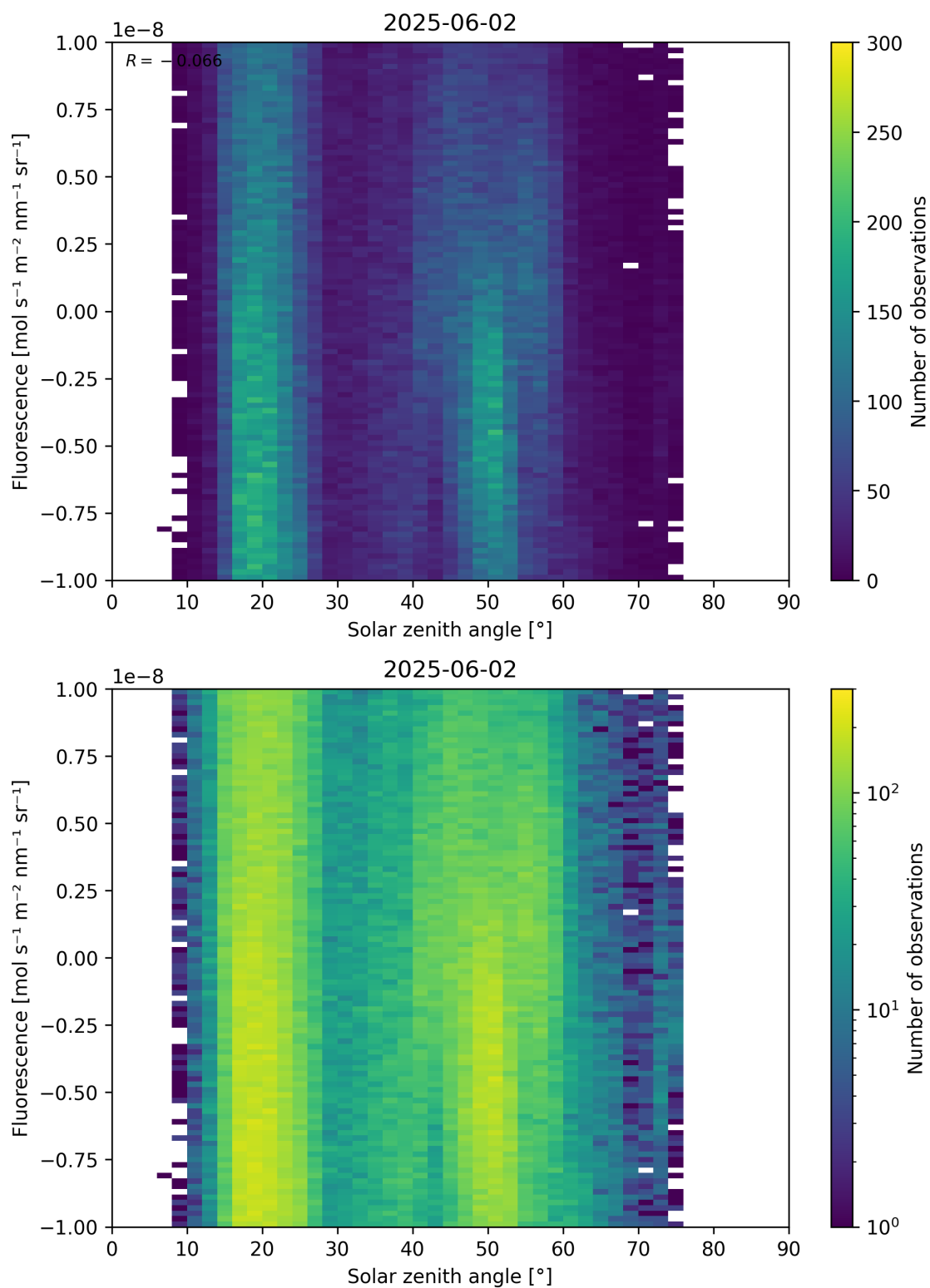
Figure 97: Scatter density plot of “Solar zenith angle” against “Fluorescence” for 2025-06-01 to 2025-06-03.
