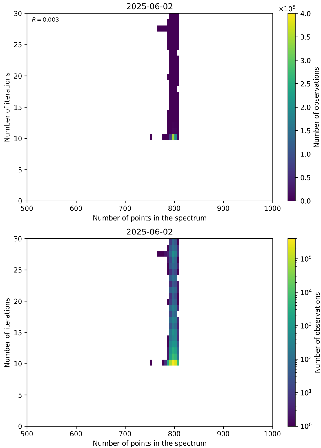
Figure 92: Scatter density plot of “Number of points in the spectrum” against “Number of iterations” for 2025-06-01 to 2025-06-03.
