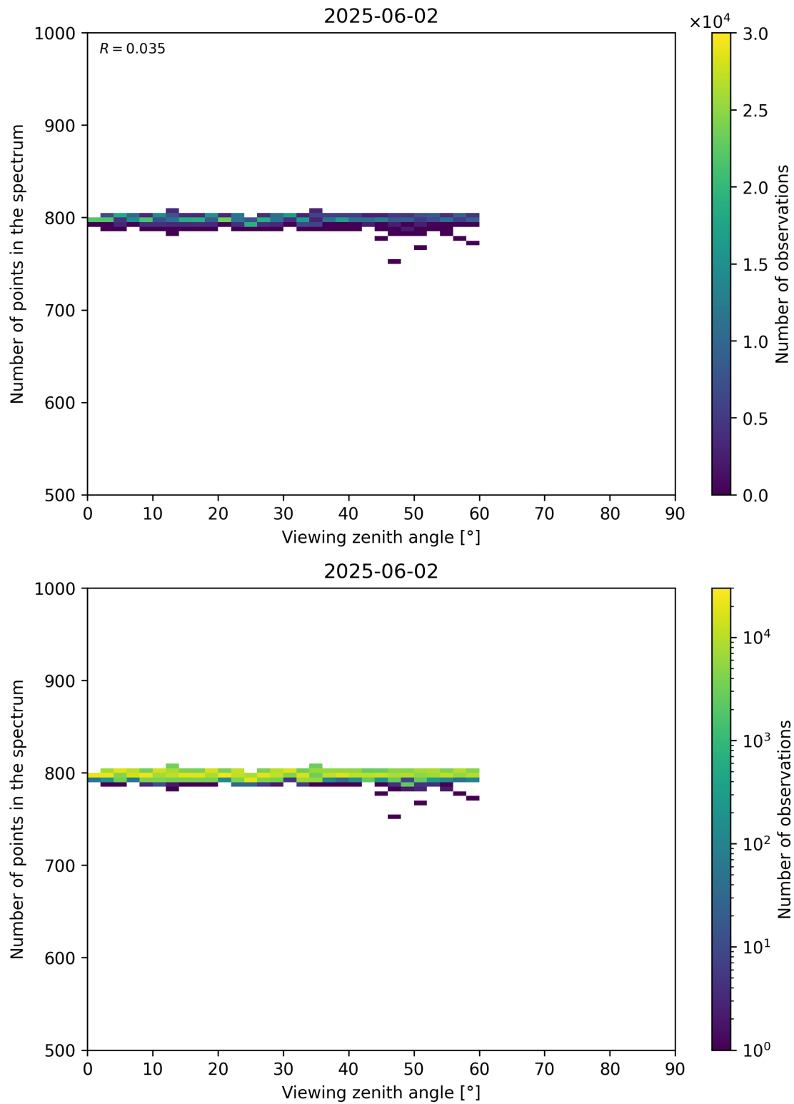
Figure 114: Scatter density plot of “Viewing zenith angle” against “Number of points in the spectrum” for 2025-06-01 to 2025-06-03.
