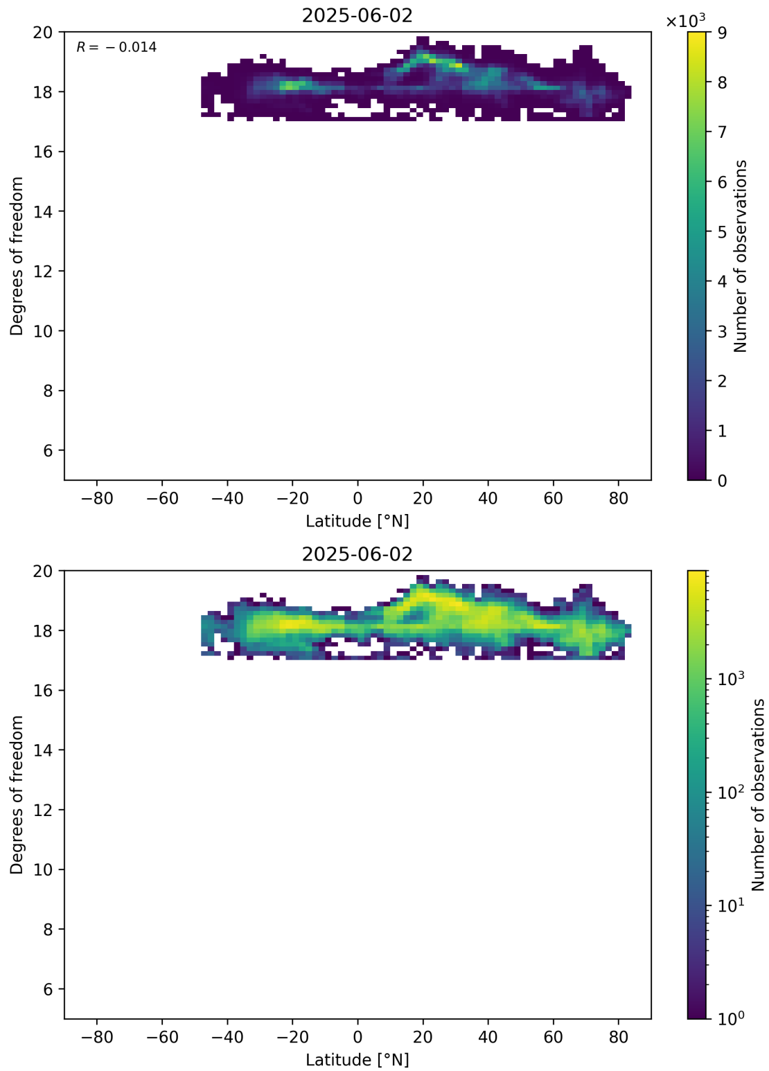
Figure 55: Scatter density plot of “Latitude” against “Degrees of freedom” for 2025-06-01 to 2025-06-03.
