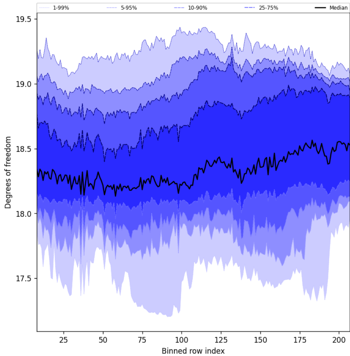
Figure 41: Along track statistics of “Degrees of freedom” for 2025-06-01 to 2025-06-03
