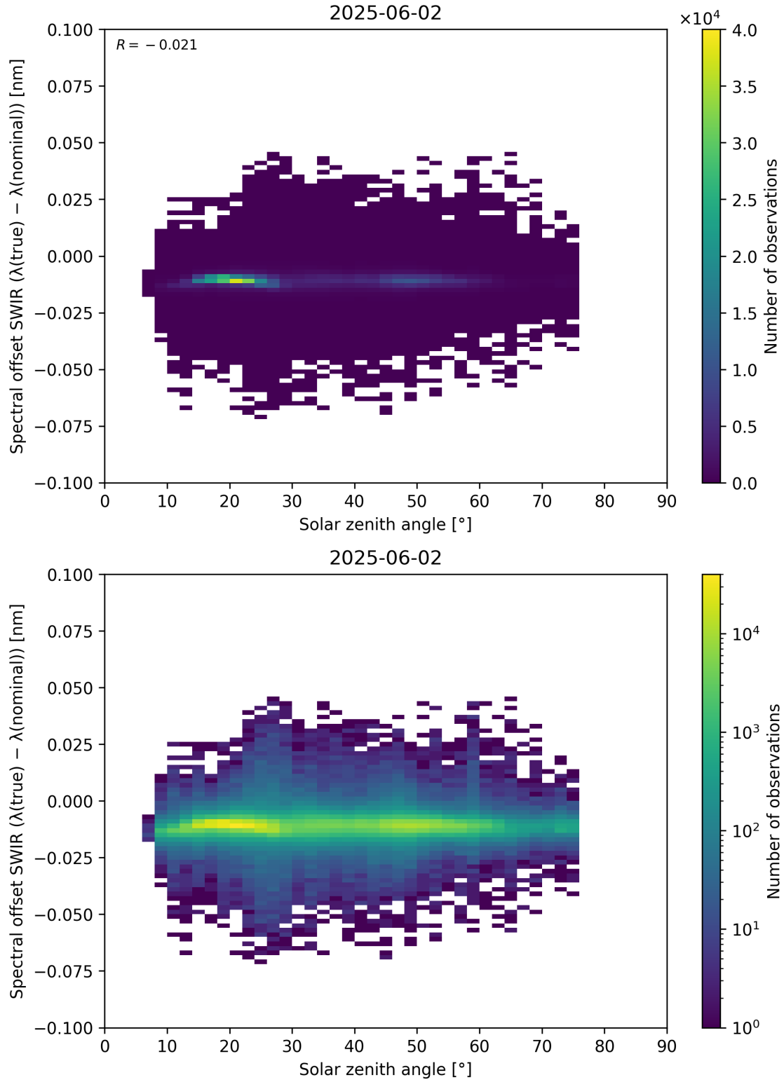
Figure 104: Scatter density plot of “Solar zenith angle” against “Spectral offset SWIR ( \lambda_{\text{true}} - \lambda_{\text{nominal}} )” for 2025-06-01 to 2025-06-03.
