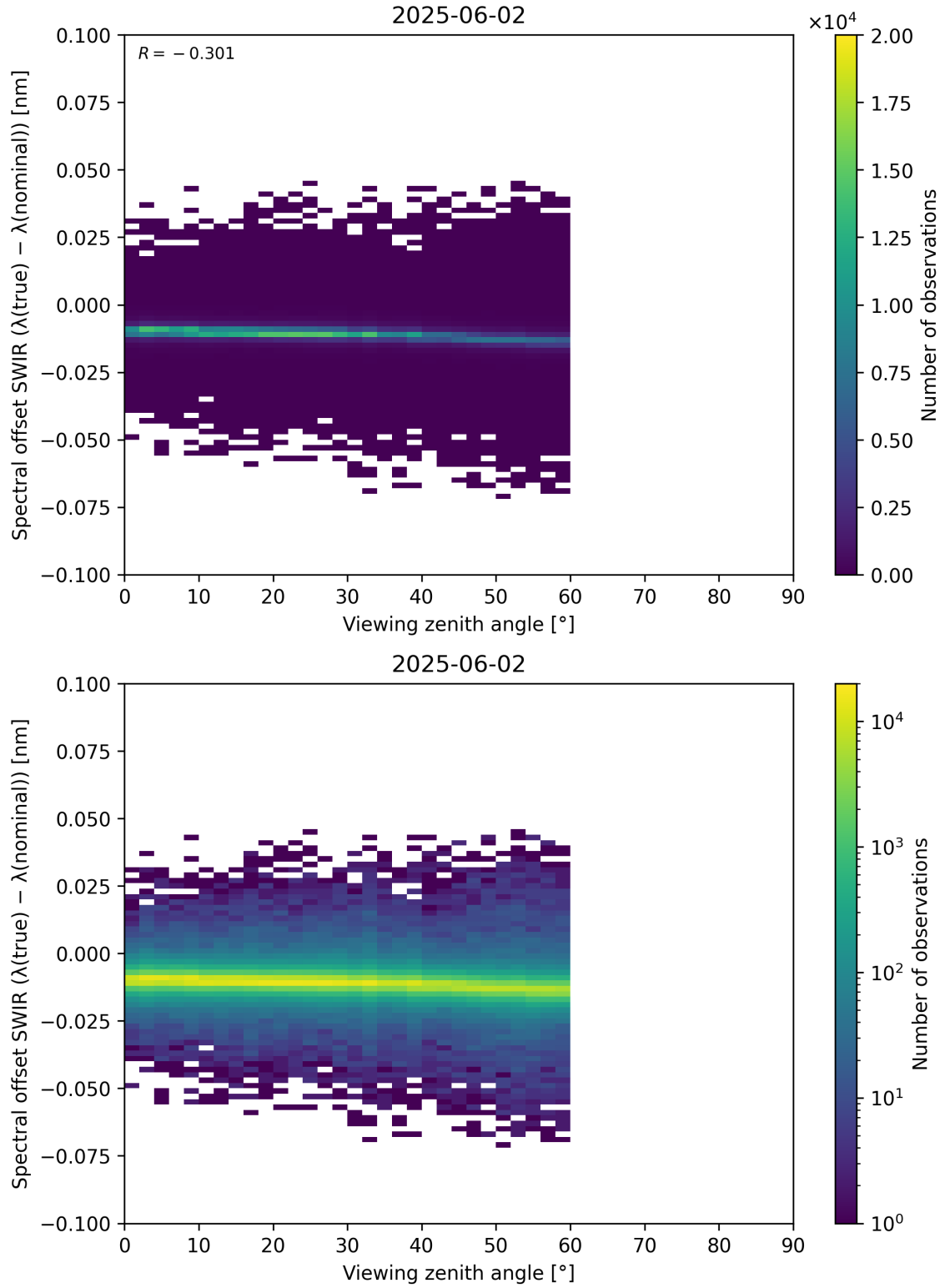
Figure 116: Scatter density plot of “Viewing zenith angle” against “Spectral offset SWIR ( \lambda_{\text{true}} - \lambda_{\text{nominal}} )” for 2025-06-01 to 2025-06-03.
