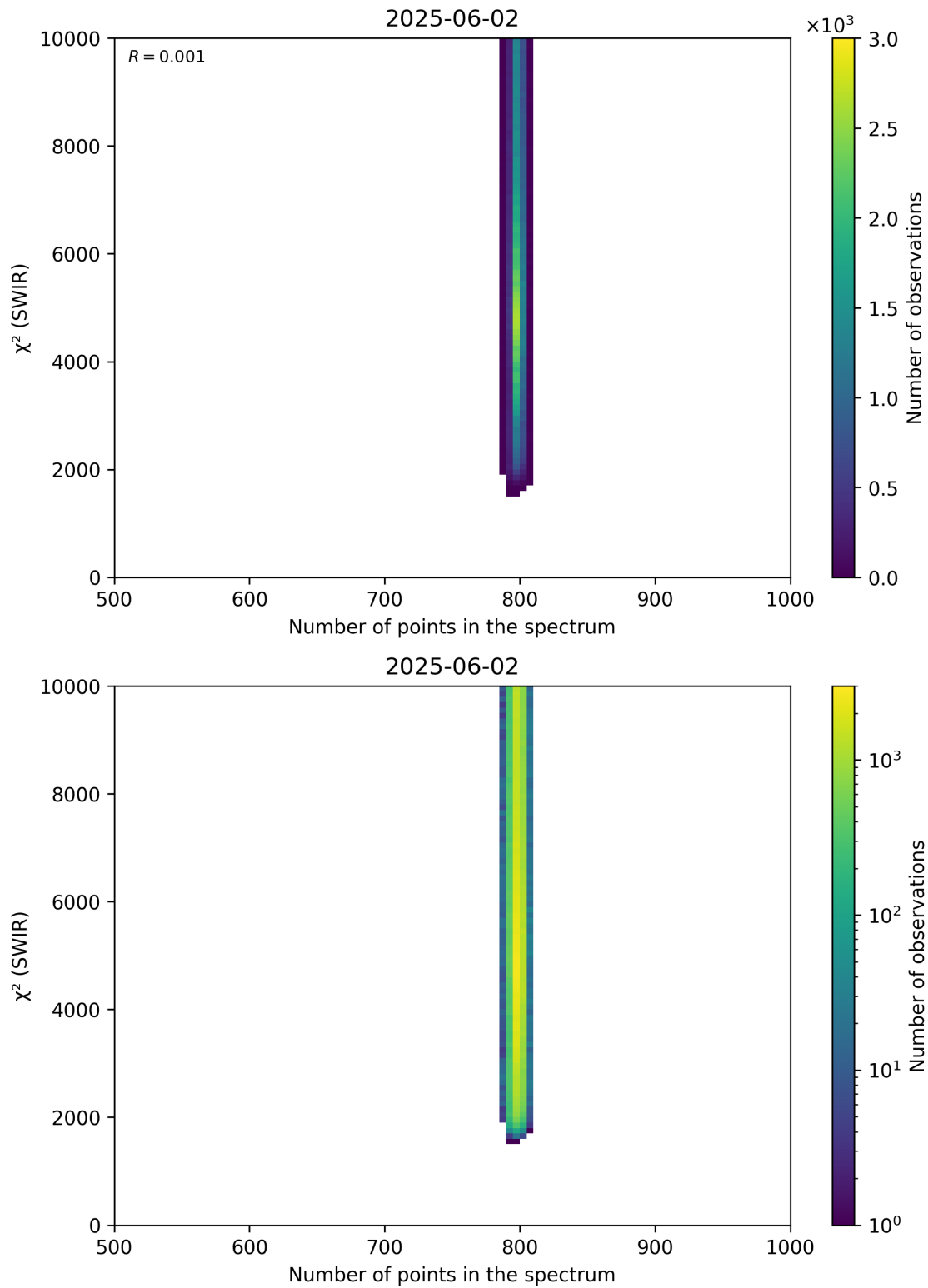
Figure 89: Scatter density plot of “Number of points in the spectrum” against “ \chi^2 (SWIR)” for 2025-06-01 to 2025-06-03.
