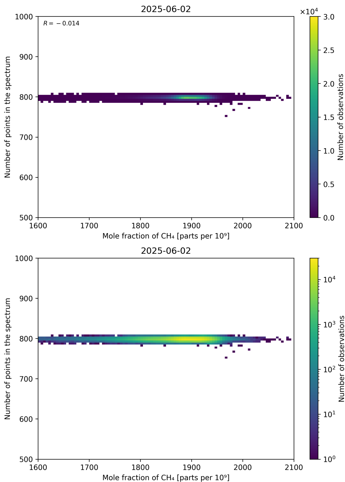
Figure 77: Scatter density plot of “Mole fraction of CH 4 ” against “Number of points in the spectrum” for 2025-06-01 to 2025-06-03.
