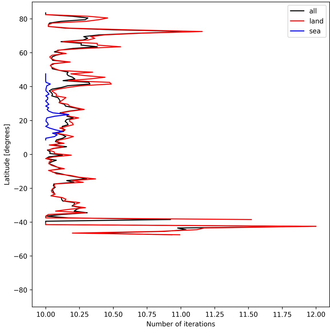
Figure 20: Zonal average of “Number of iterations” for 2025-06-01 to 2025-06-03.
