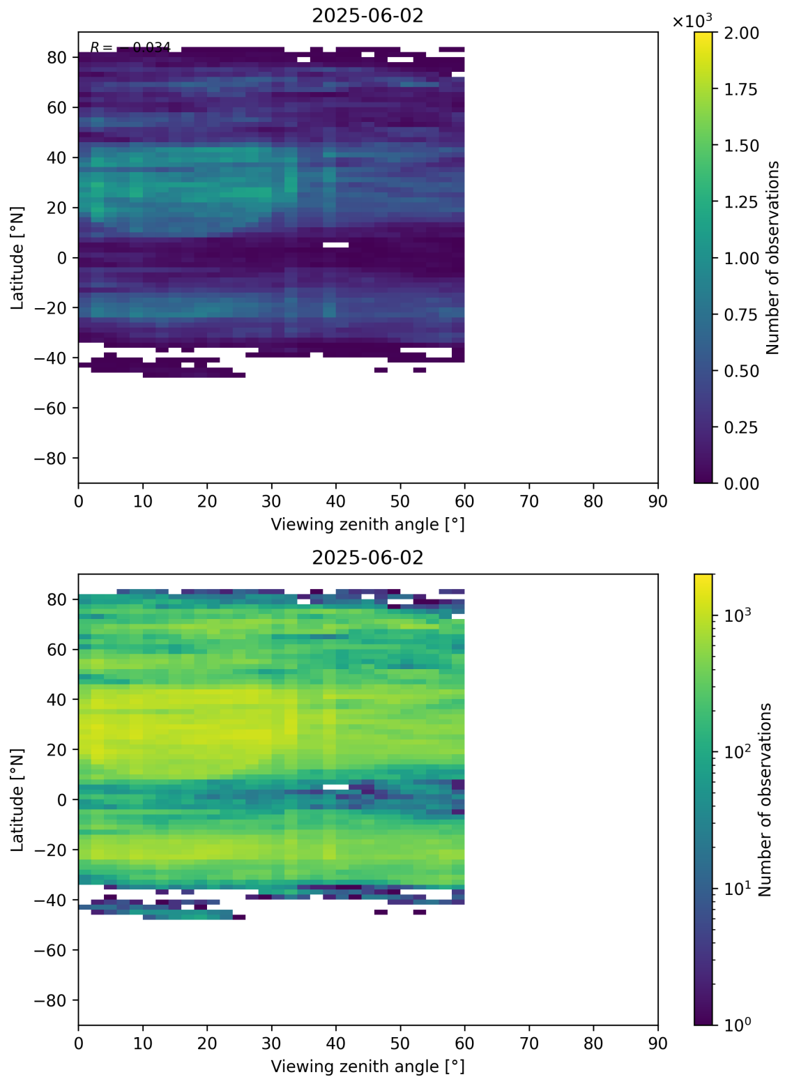
Figure 109: Scatter density plot of “Viewing zenith angle” against “Latitude” for 2025-06-01 to 2025-06-03.
