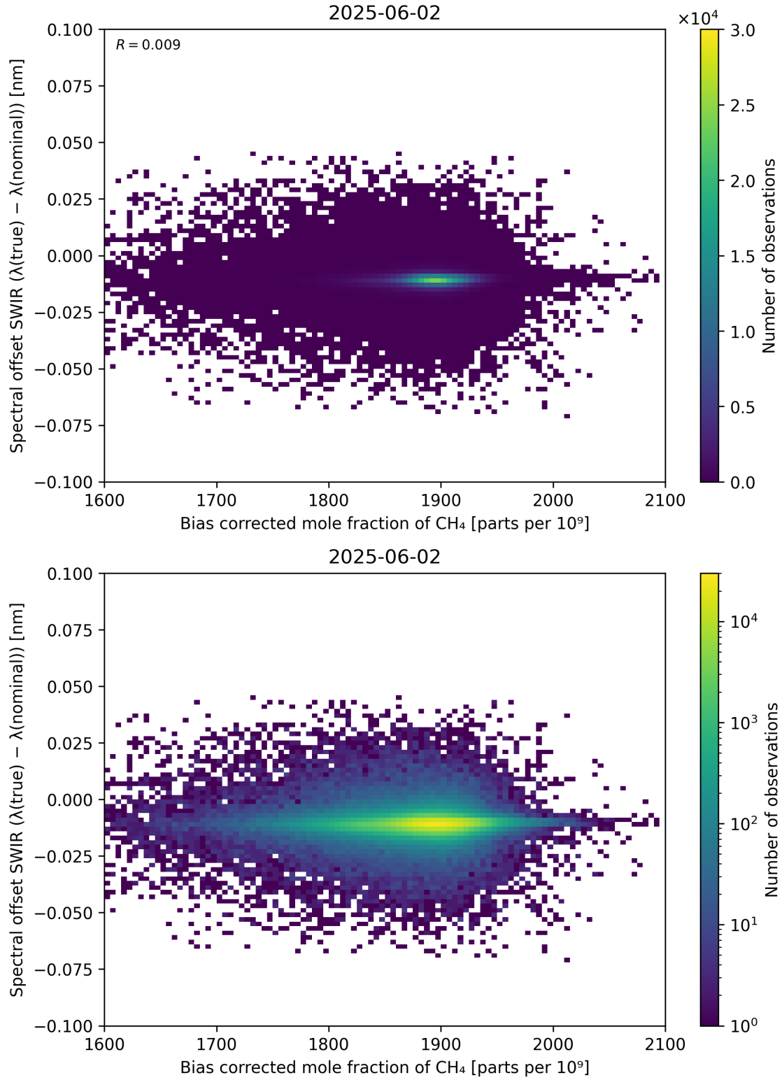
Figure 69: Scatter density plot of “Bias corrected mole fraction of \text{CH}_4 ” against “Spectral offset SWIR ( \lambda_{\text{true}} - \lambda_{\text{nominal}} )” for 2025-06-01 to 2025-06-03.
