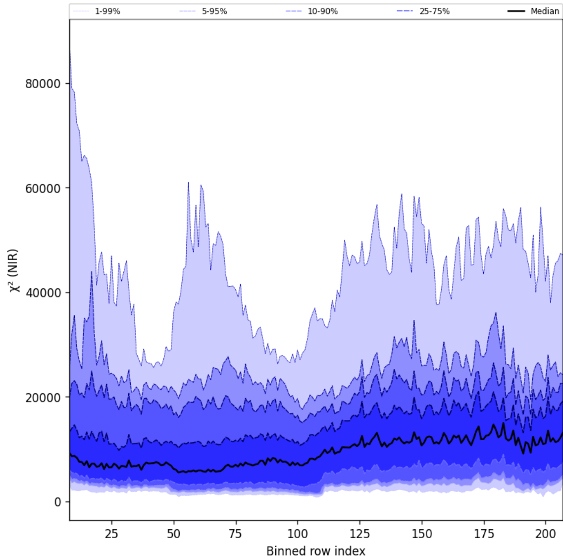
Figure 40: Along track statistics of “ \chi^2 (NIR)” for 2025-06-01 to 2025-06-03
