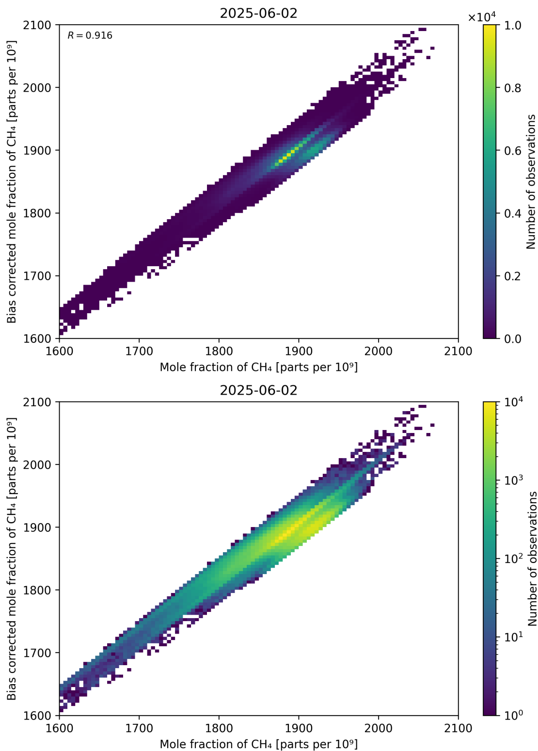
Figure 74: Scatter density plot of “Mole fraction of CH 4 ” against “Bias corrected mole fraction of CH 4 ” for 2025-06-01 to 2025-06-03.
