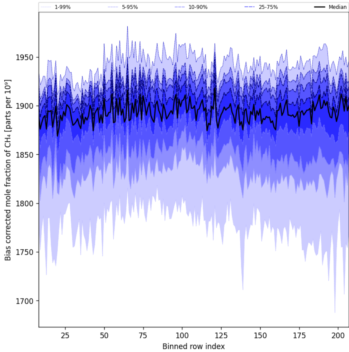
Figure 36: Along track statistics of “Bias corrected mole fraction of CH 4 ” for 2025-06-01 to 2025-06-03
