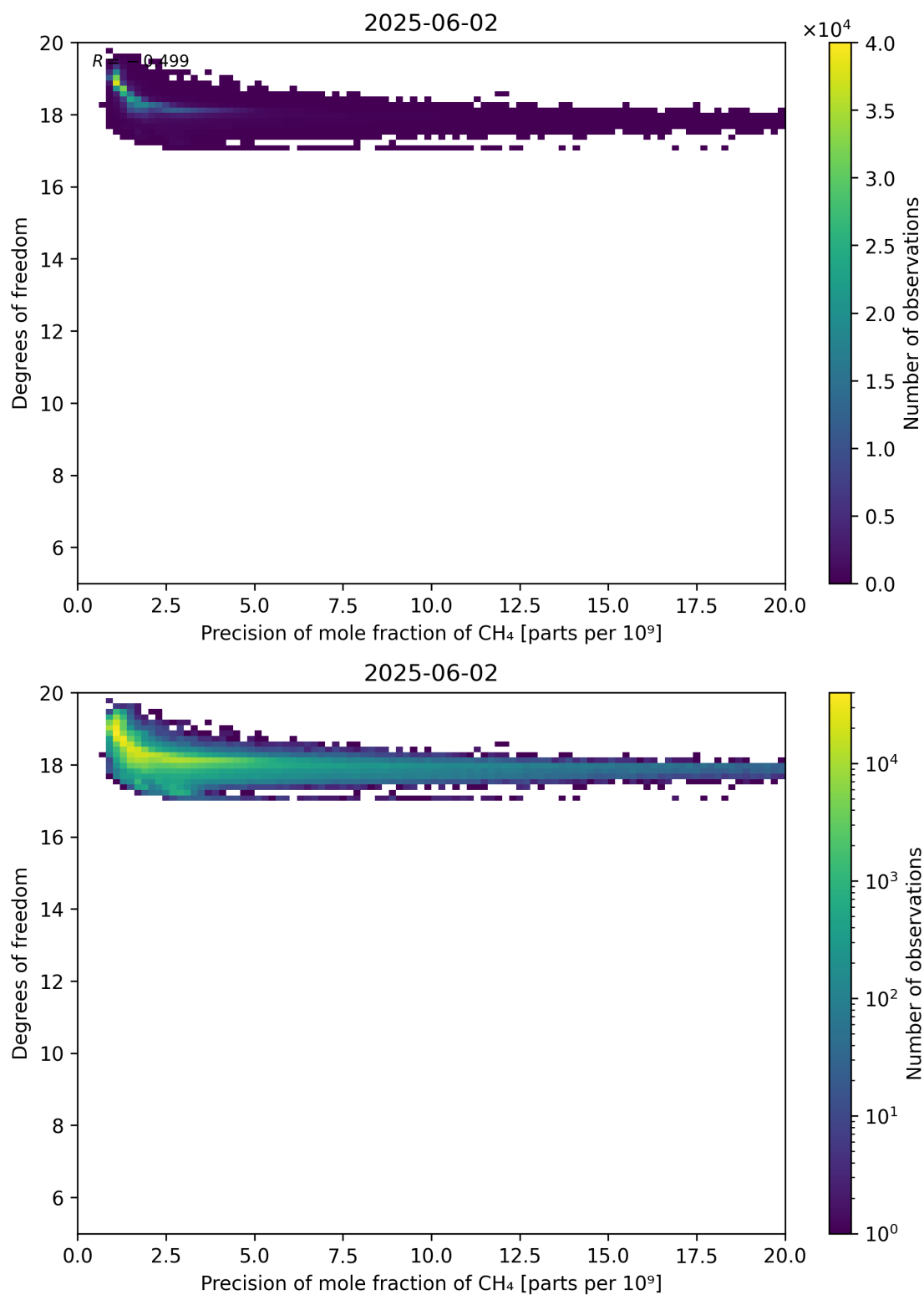
Figure 80: Scatter density plot of “Precision of mole fraction of CH 4 ” against “Degrees of freedom” for 2025-06-01 to 2025-06-03.
