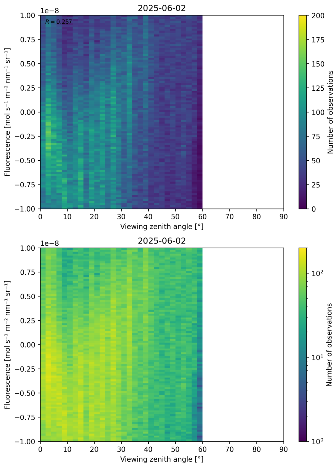
Figure 108: Scatter density plot of “Viewing zenith angle” against “Fluorescence” for 2025-06-01 to 2025-06-03.
