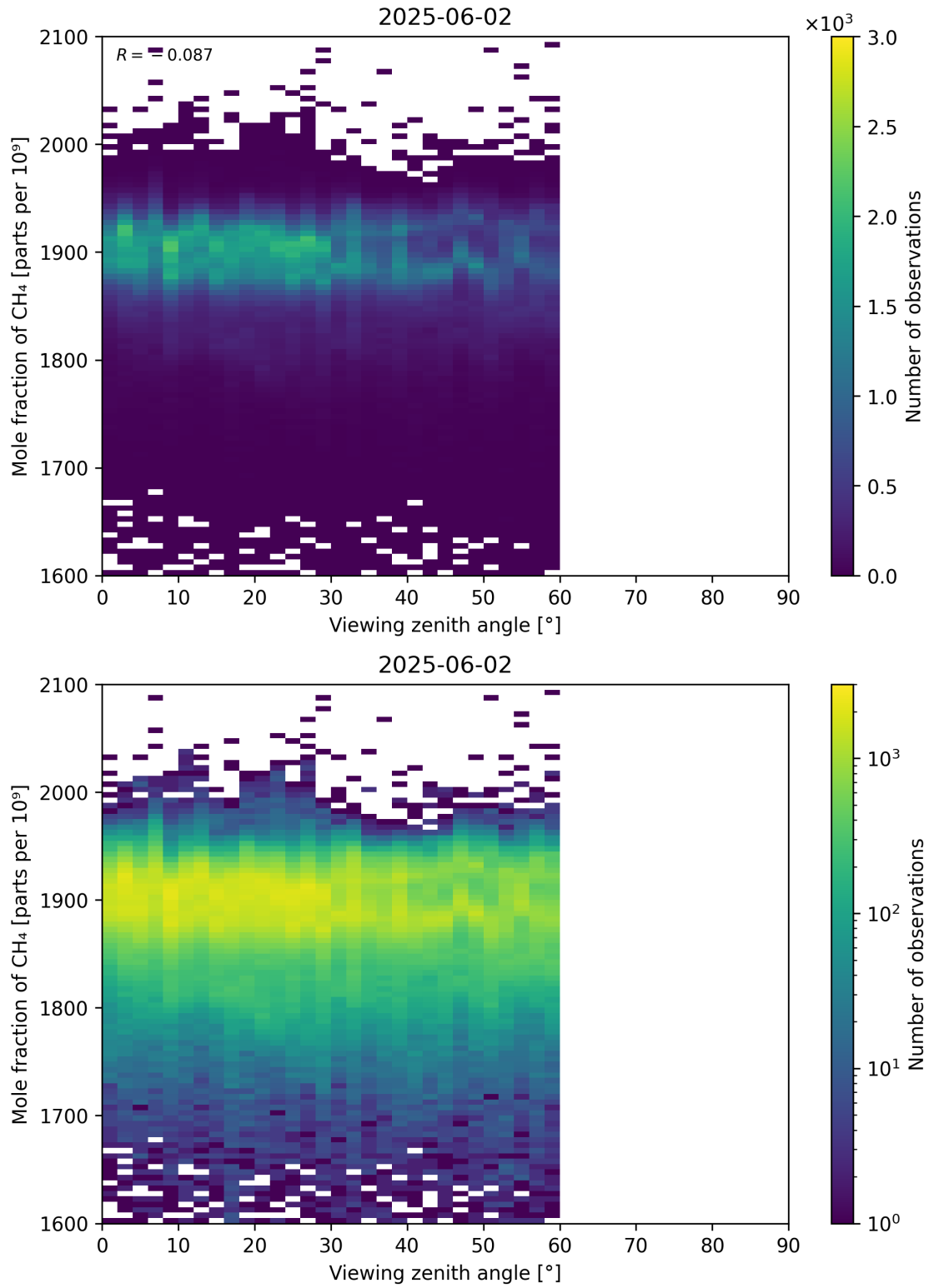
Figure 110: Scatter density plot of “Viewing zenith angle” against “Mole fraction of CH 4 ” for 2025-06-01 to 2025-06-03.
