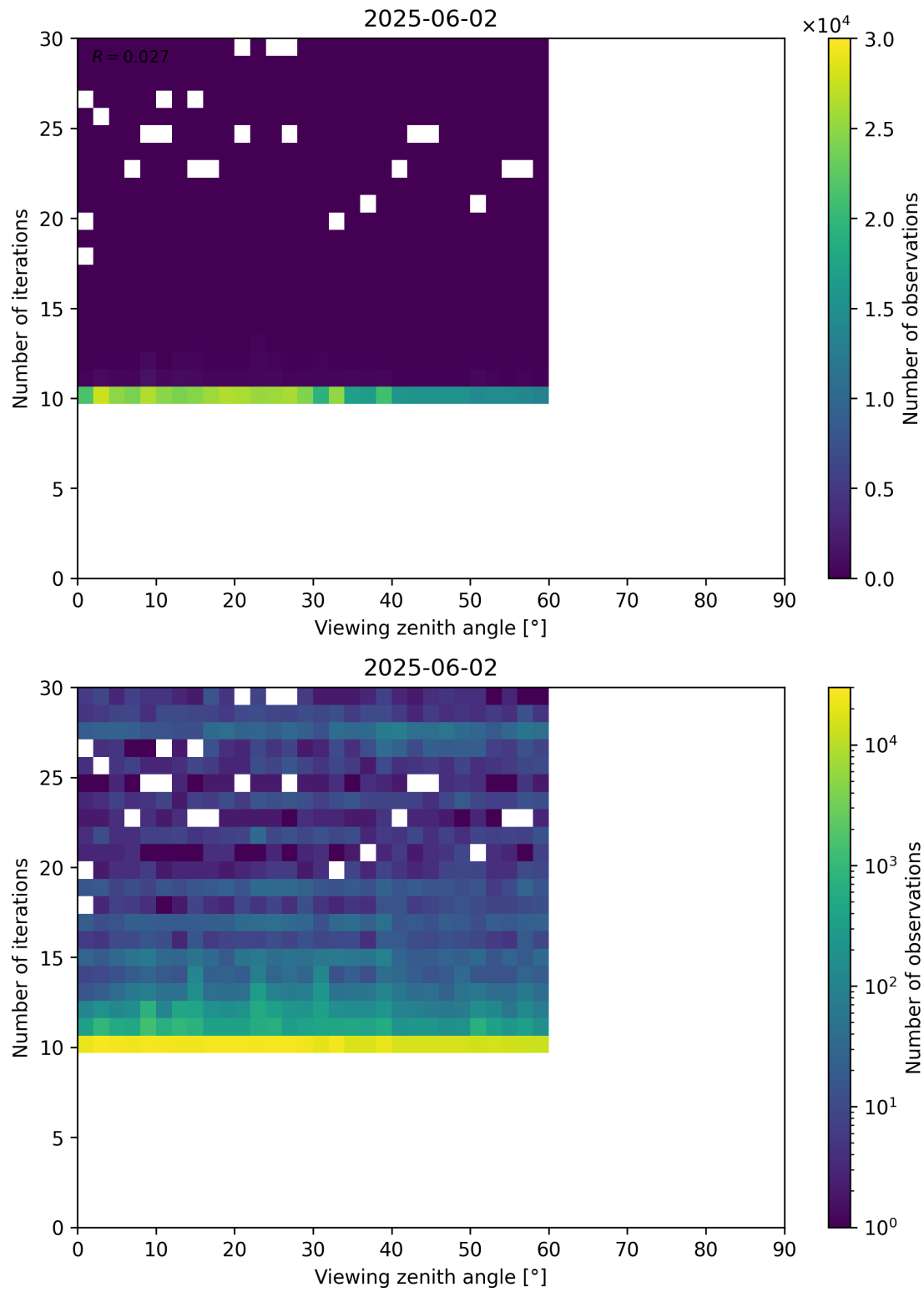
Figure 113: Scatter density plot of “Viewing zenith angle” against “Number of iterations” for 2025-06-01 to 2025-06-03.
