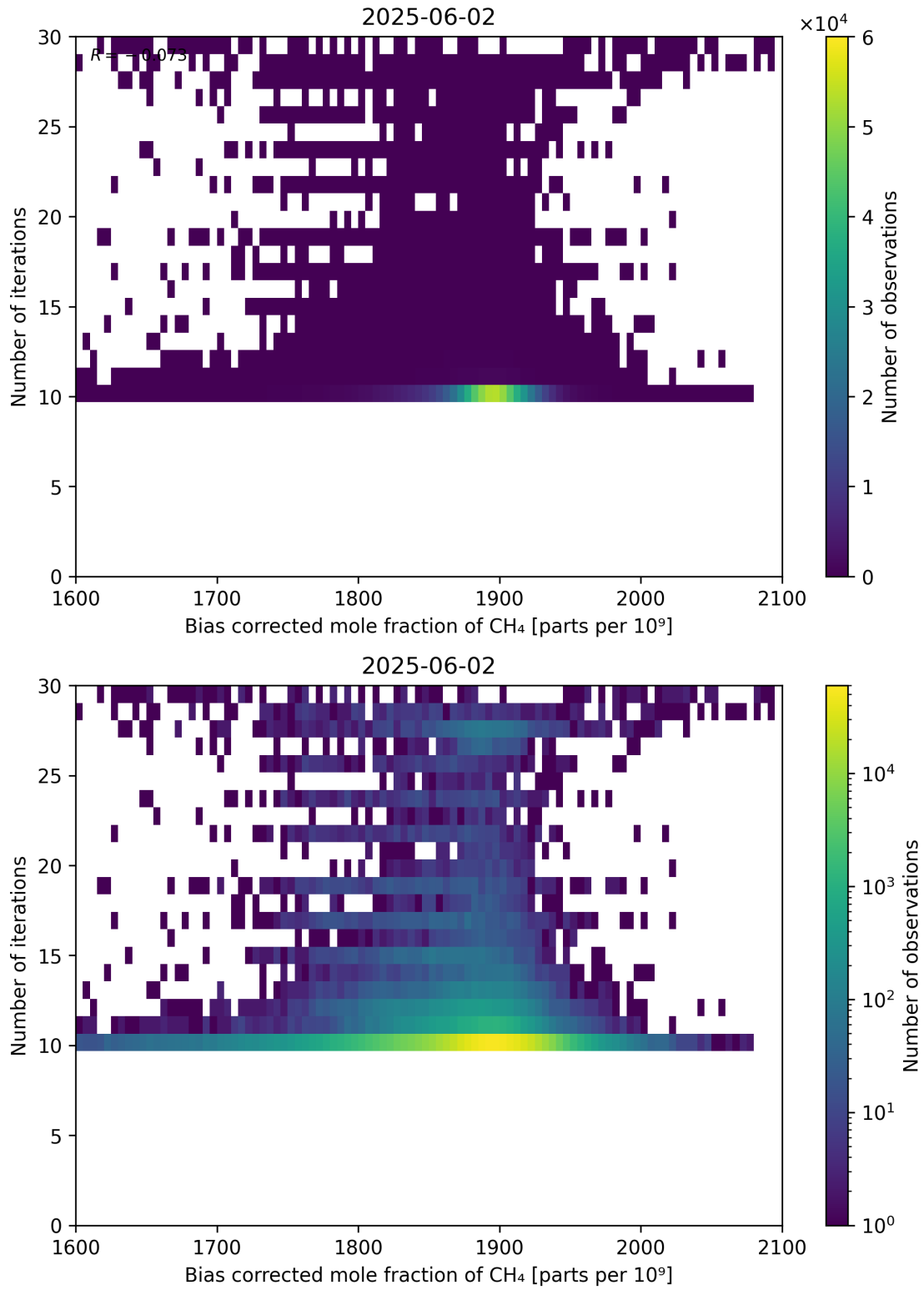
Figure 67: Scatter density plot of “Bias corrected mole fraction of CH 4 ” against “Number of iterations” for 2025-06-01 to 2025-06-03.
