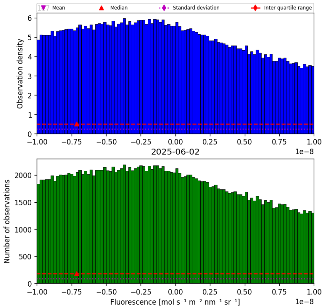
Figure 32: Histogram of “Fluorescence” for 2025-06-01 to 2025-06-03
