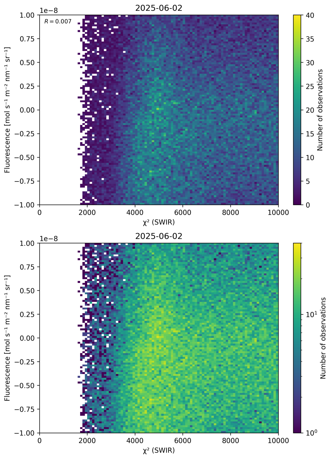
Figure 49: Scatter density plot of “ \chi^2 (SWIR)” against “Fluorescence” for 2025-06-01 to 2025-06-03.
