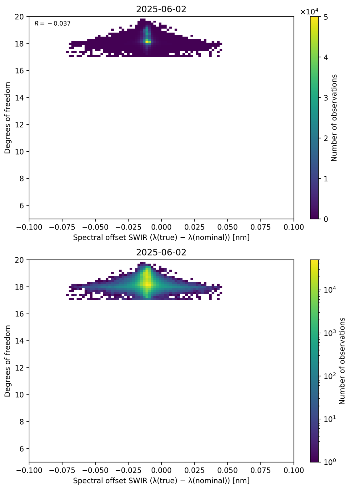
Figure 119: Scatter density plot of “Spectral offset SWIR ( \lambda_{\text{true}} - \lambda_{\text{nominal}} )” against “Degrees of freedom” for 2025-06-01 to 2025-06-03.
