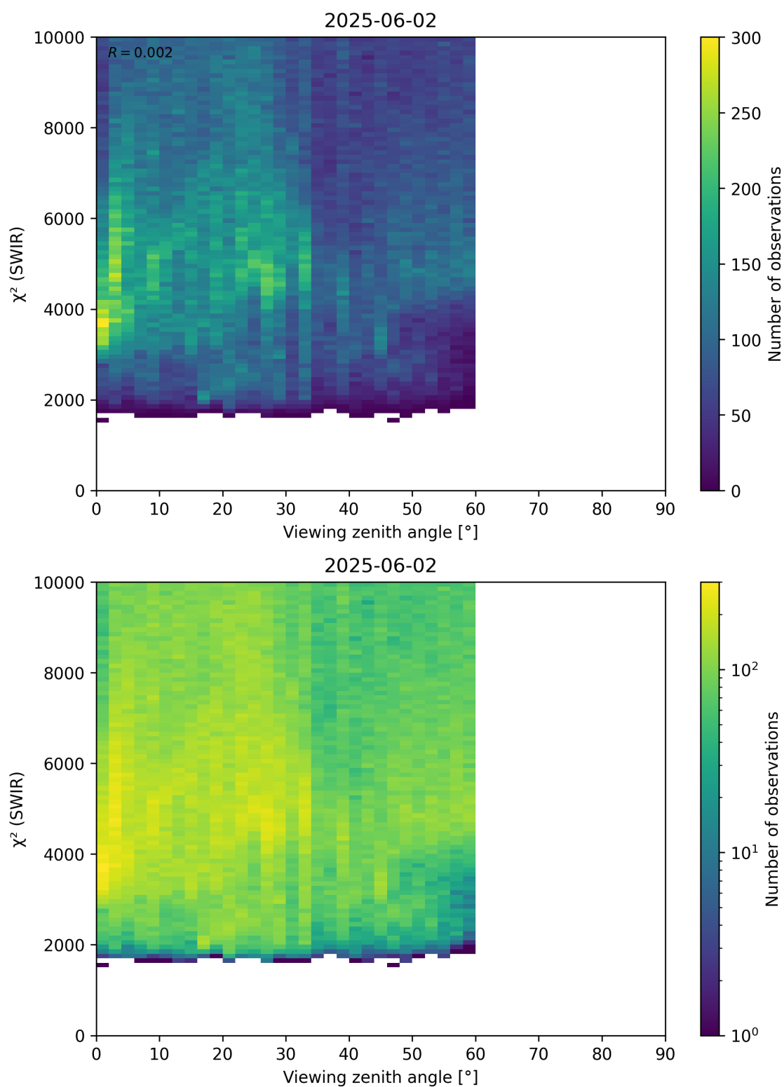
Figure 106: Scatter density plot of “Viewing zenith angle” against “ \chi^2 (SWIR)” for 2025-06-01 to 2025-06-03.
