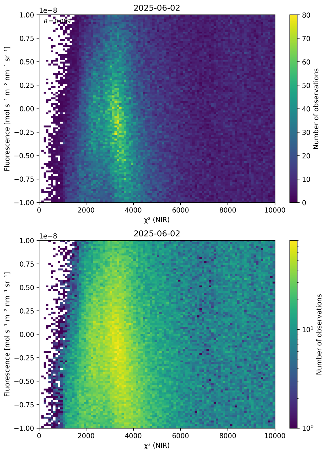
Figure 45: Scatter density plot of “ \chi^2 (NIR)” against “Fluorescence” for 2025-06-01 to 2025-06-03.
