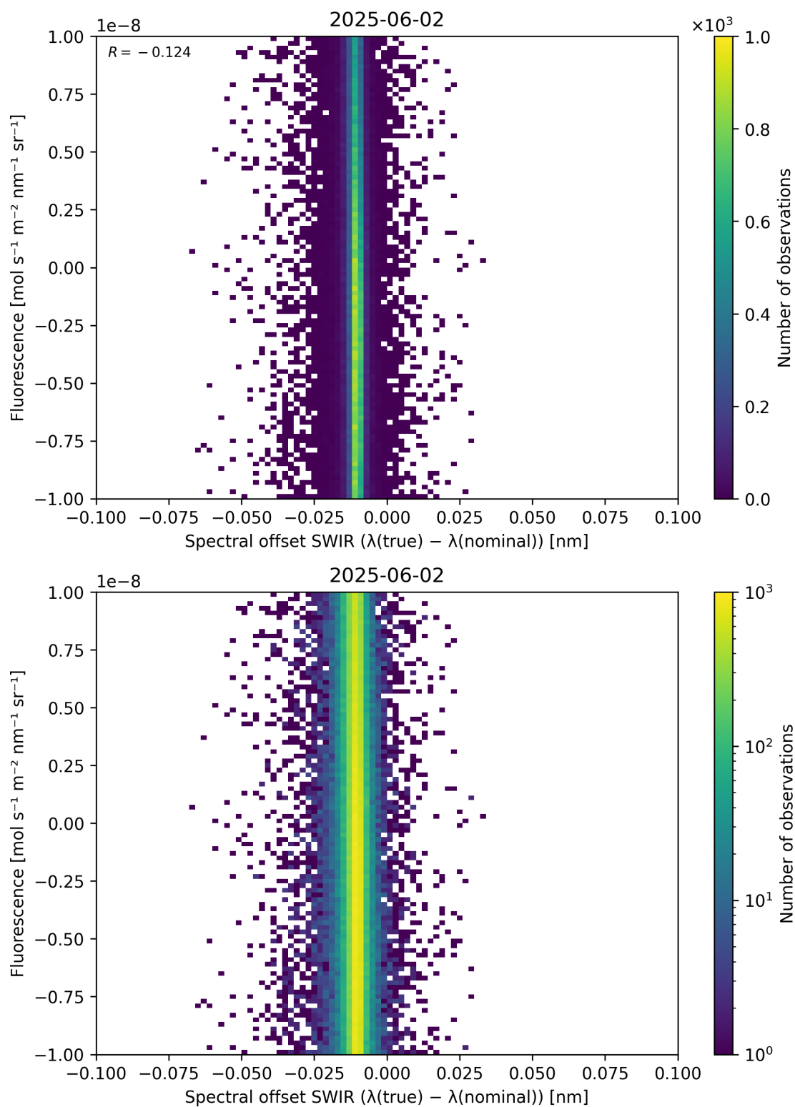
Figure 120: Scatter density plot of “Spectral offset SWIR ( \lambda_{\text{true}} - \lambda_{\text{nominal}} )” against “Fluorescence” for 2025-06-01 to 2025-06-03.
