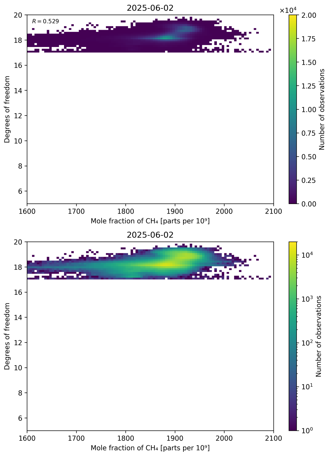
Figure 72: Scatter density plot of “Mole fraction of CH 4 ” against “Degrees of freedom” for 2025-06-01 to 2025-06-03.
