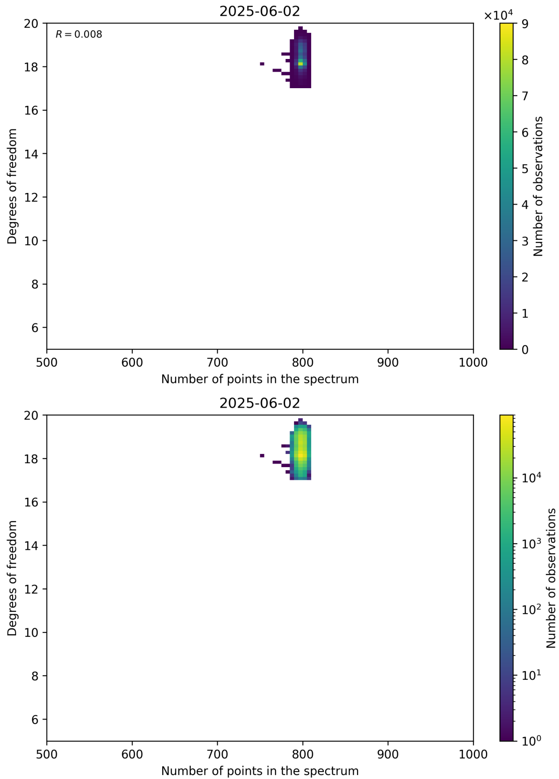
Figure 90: Scatter density plot of “Number of points in the spectrum” against “Degrees of freedom” for 2025-06-01 to 2025-06-03.
