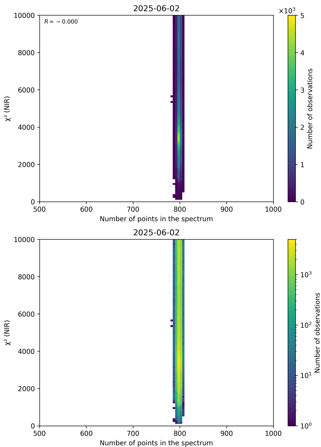
Figure 88: Scatter density plot of “Number of points in the spectrum” against “ \chi^2 (NIR)” for 2025-06-01 to 2025-06-03.
