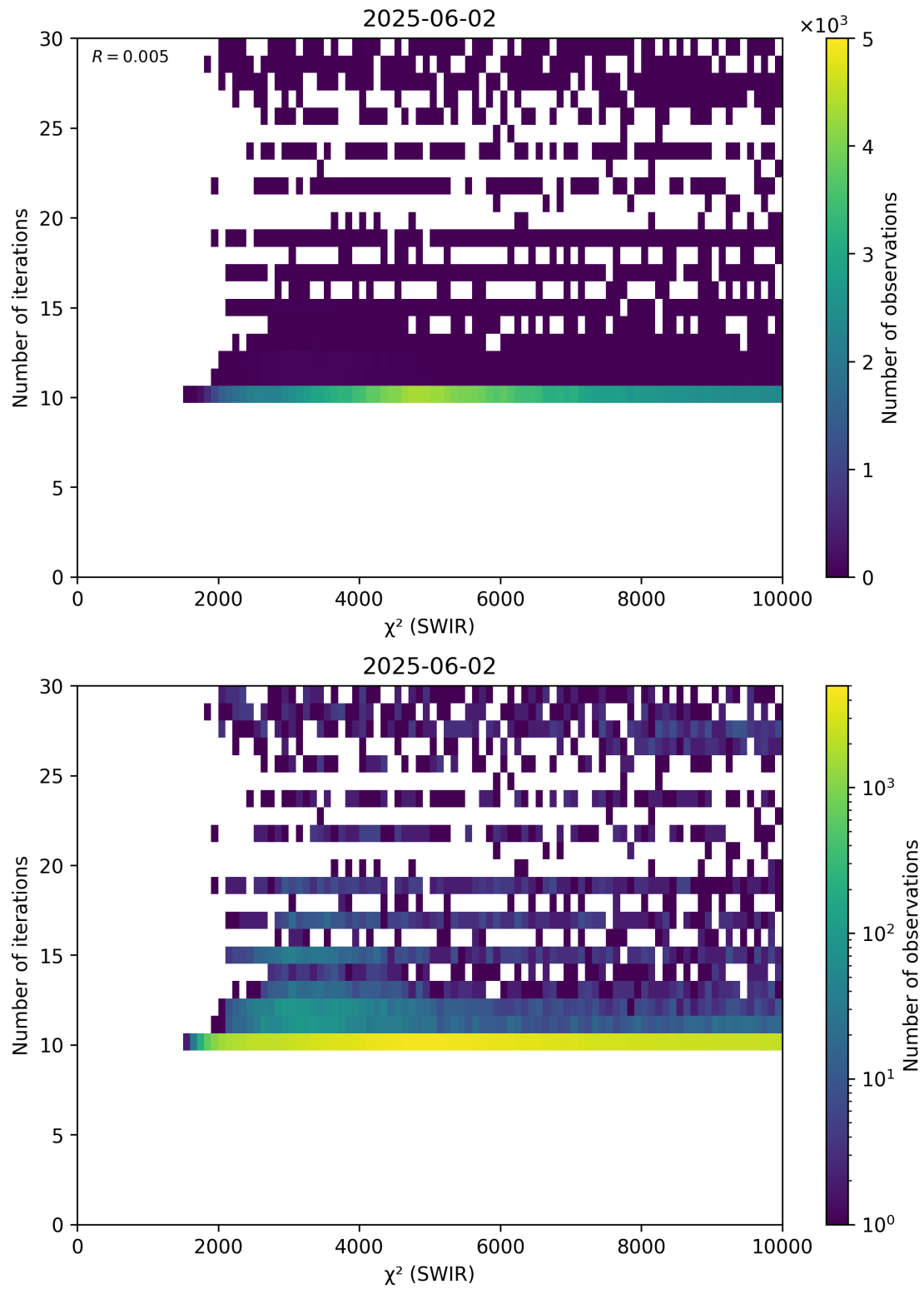
Figure 50: Scatter density plot of “ \chi^2 (SWIR)” against “Number of iterations” for 2025-06-01 to 2025-06-03.
