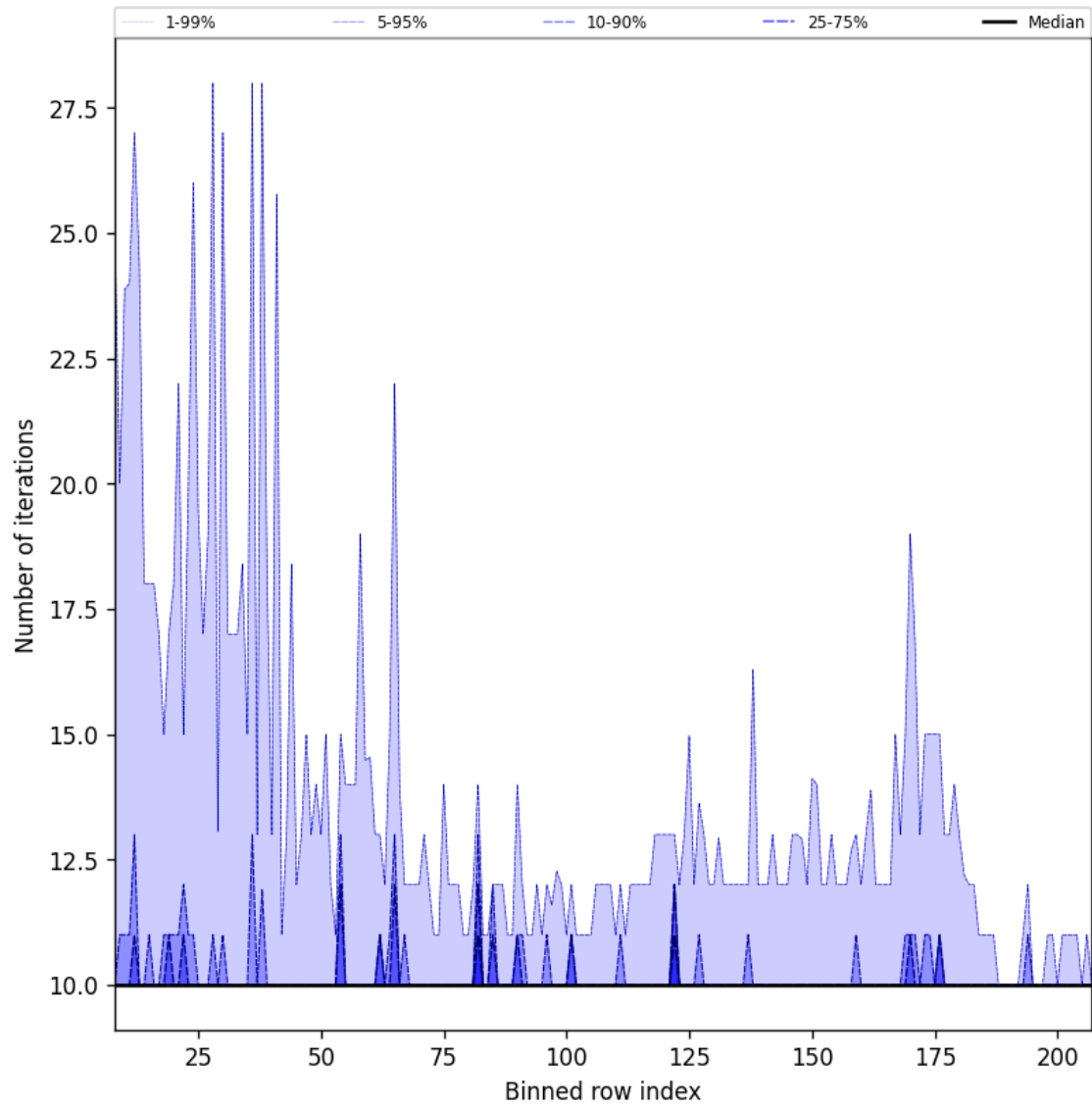
Figure 42: Along track statistics of “Number of iterations” for 2025-06-01 to 2025-06-03
