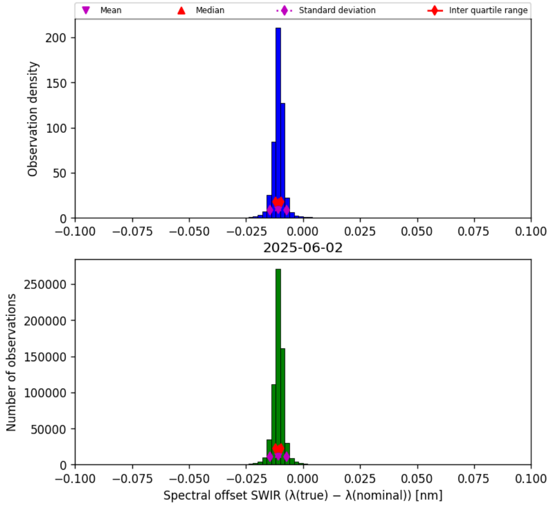
Figure 27: Histogram of “Spectral offset SWIR ( \lambda_{\text{true}} - \lambda_{\text{nominal}} )” for 2025-06-01 to 2025-06-03
