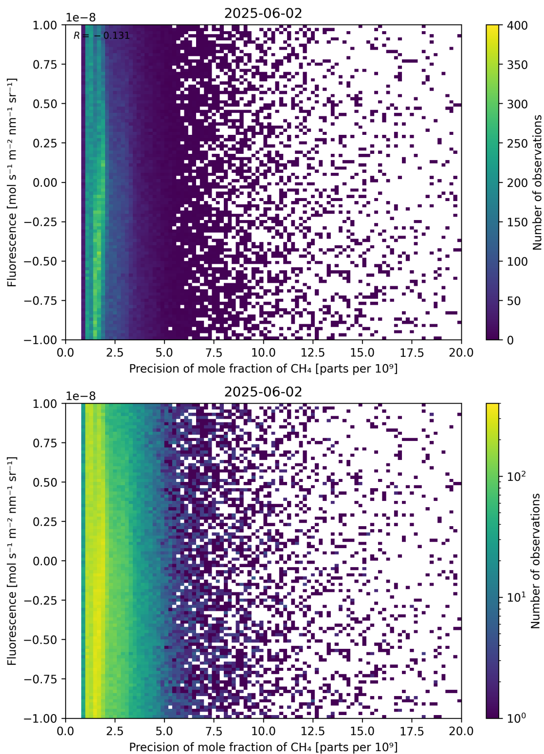
Figure 81: Scatter density plot of “Precision of mole fraction of \text{CH}_4 ” against “Fluorescence” for 2025-06-01 to 2025-06-03.
