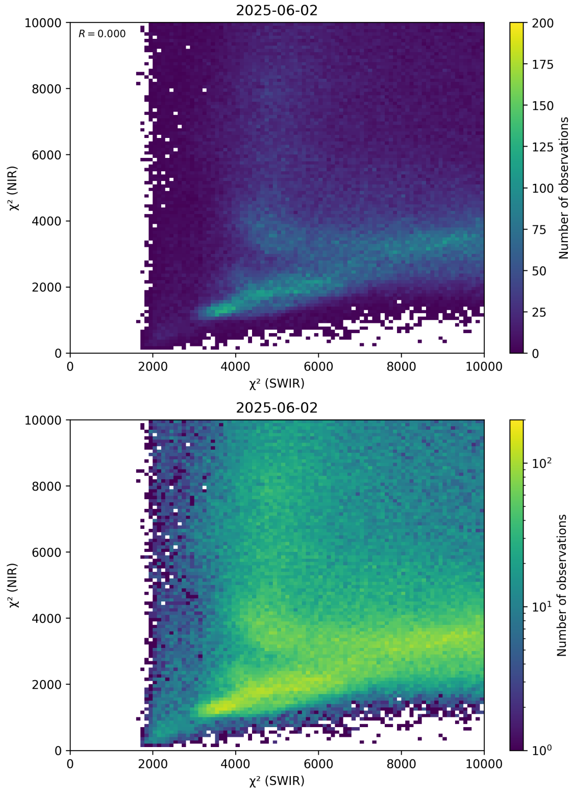
Figure 47: Scatter density plot of “ \chi^2 (SWIR)” against “ \chi^2 (NIR)” for 2025-06-01 to 2025-06-03.
