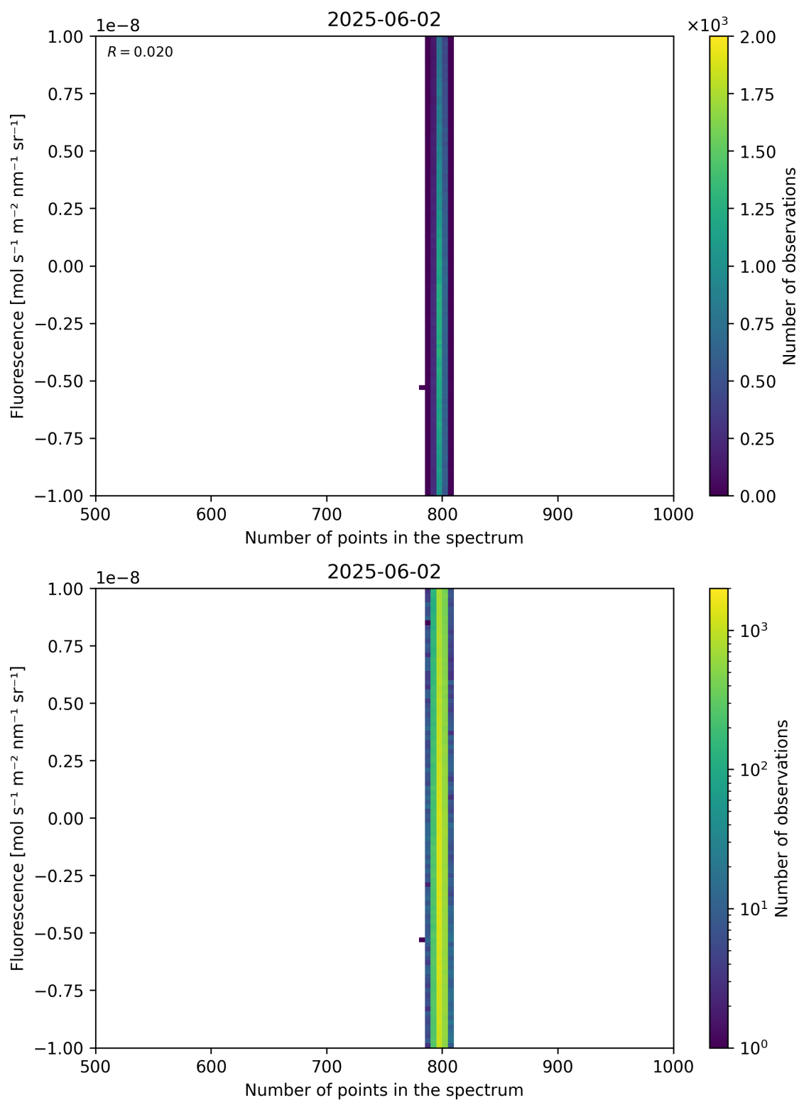
Figure 91: Scatter density plot of “Number of points in the spectrum” against “Fluorescence” for 2025-06-01 to 2025-06-03.
