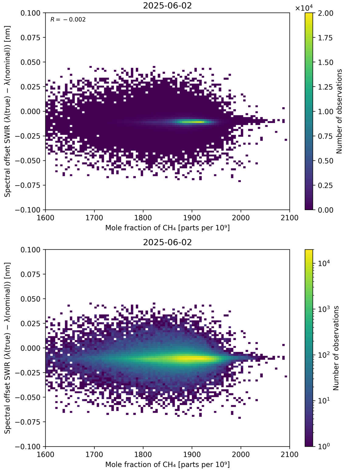
Figure 86: Scatter density plot of “Mole fraction of CH 4 ” against “Spectral offset SWIR ( \lambda_{\text{true}} - \lambda_{\text{nominal}} )” for 2025-06-01 to 2025-06-03.
