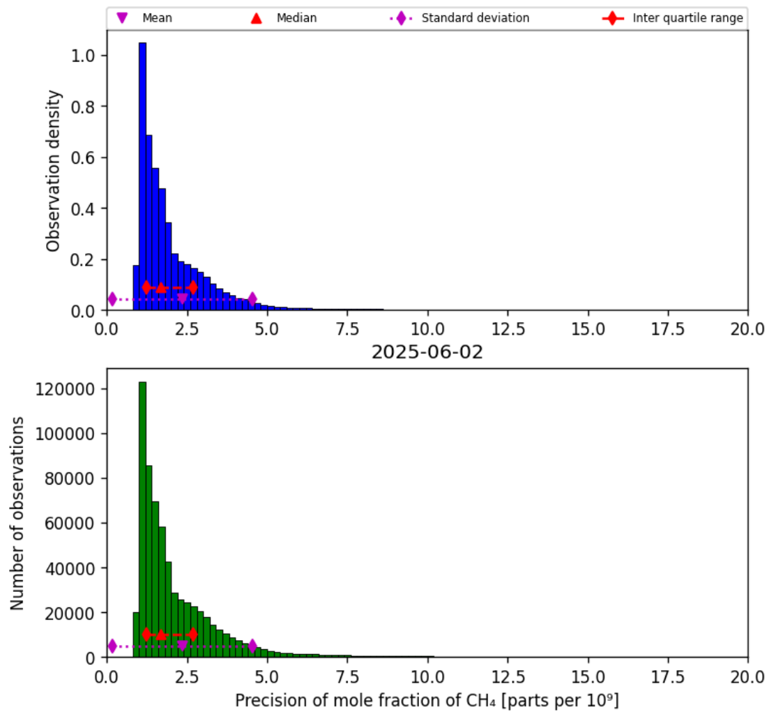
Figure 24: Histogram of “Precision of mole fraction of CH 4 ” for 2025-06-01 to 2025-06-03
