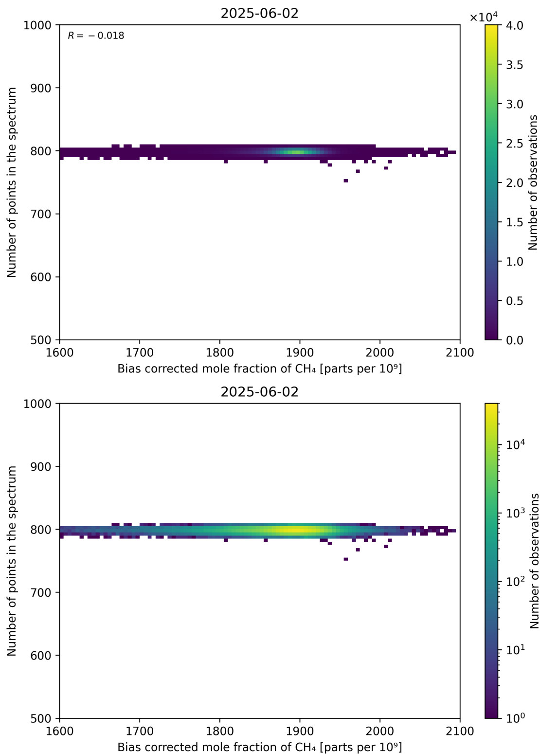
Figure 68: Scatter density plot of “Bias corrected mole fraction of CH 4 ” against “Number of points in the spectrum” for 2025-06-01 to 2025-06-03.
