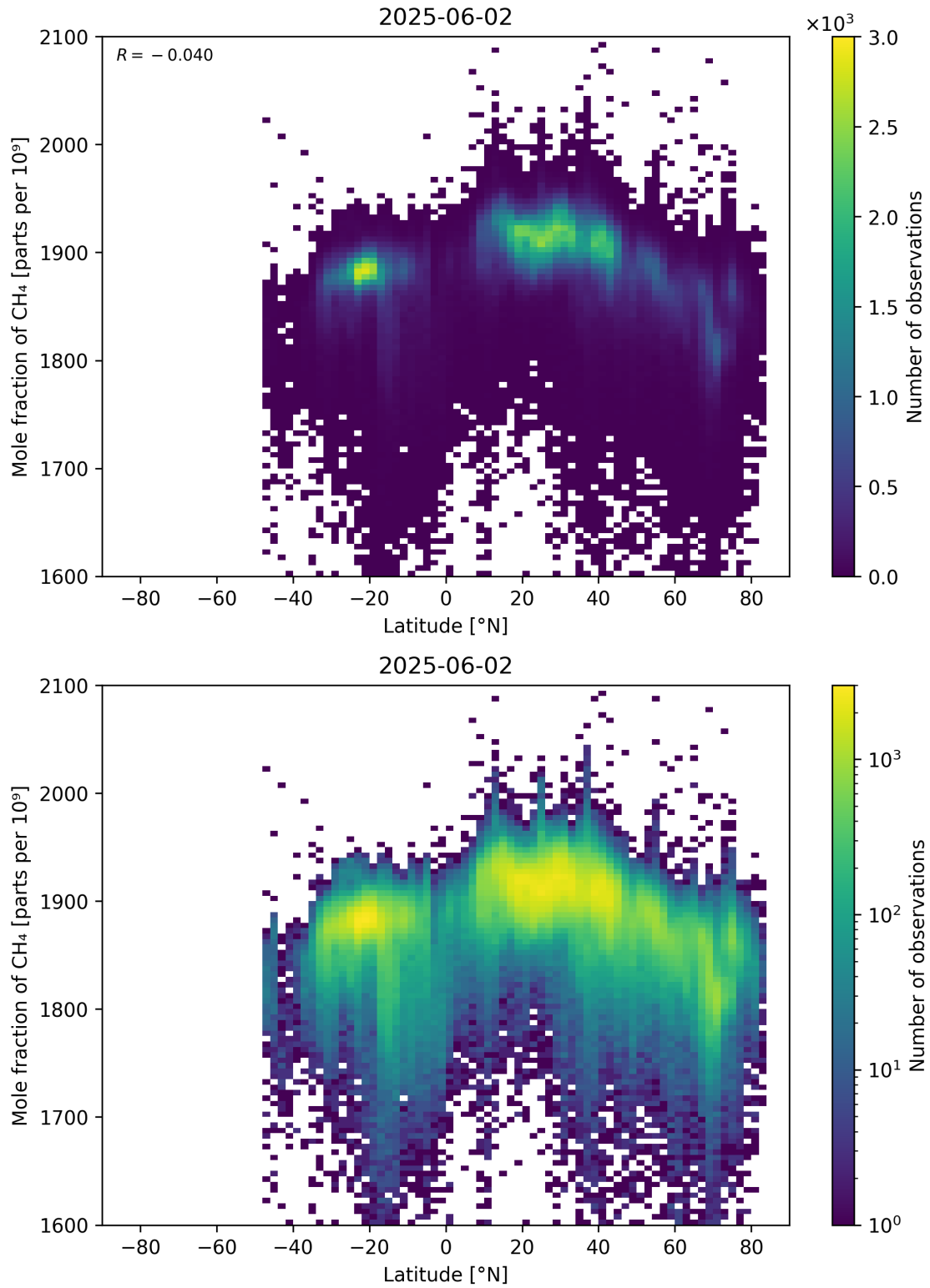
Figure 57: Scatter density plot of “Latitude” against “Mole fraction of CH 4 ” for 2025-06-01 to 2025-06-03.
