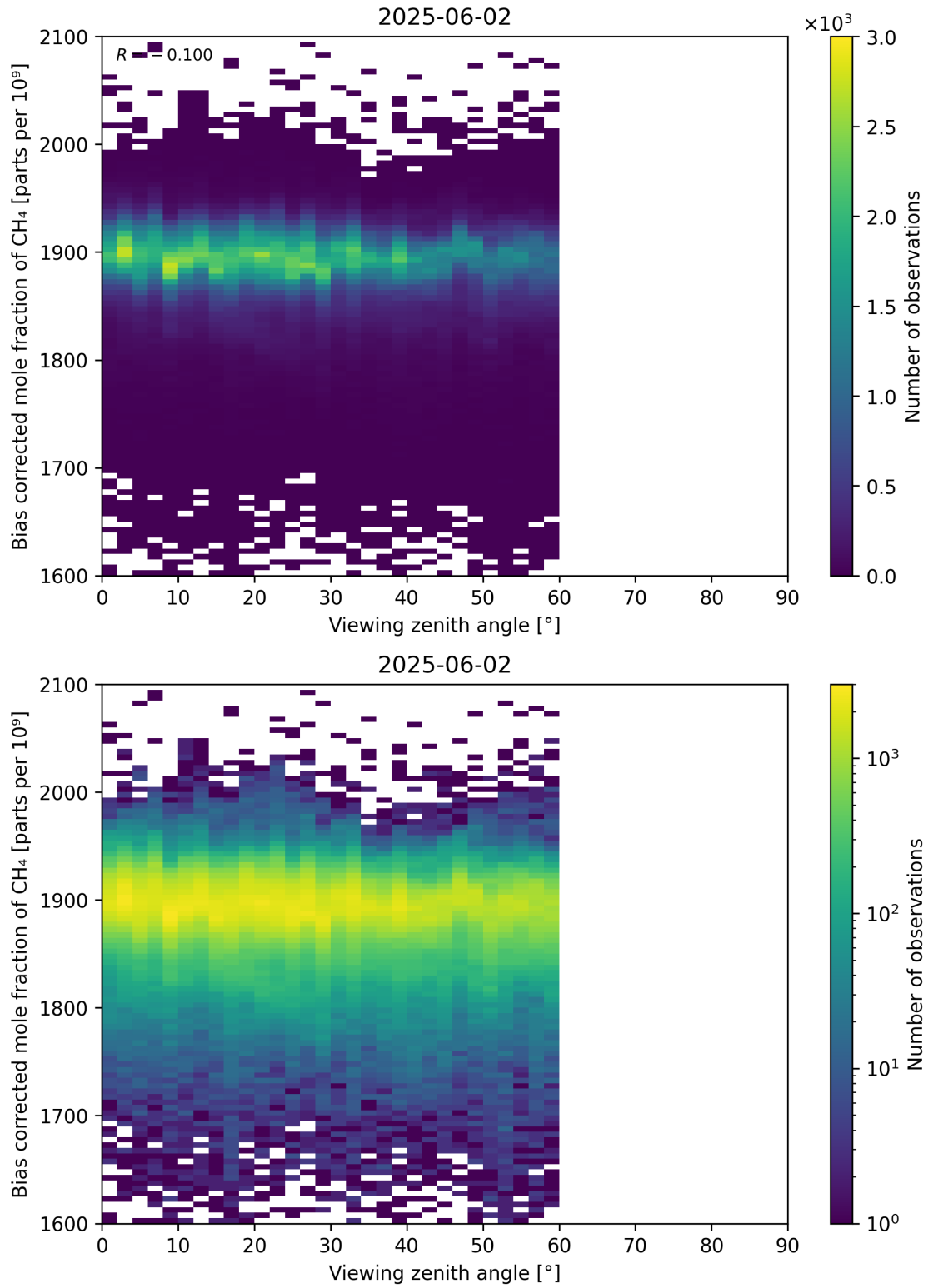
Figure 111: Scatter density plot of “Viewing zenith angle” against “Bias corrected mole fraction of CH 4 ” for 2025-06-01 to 2025-06-03.
