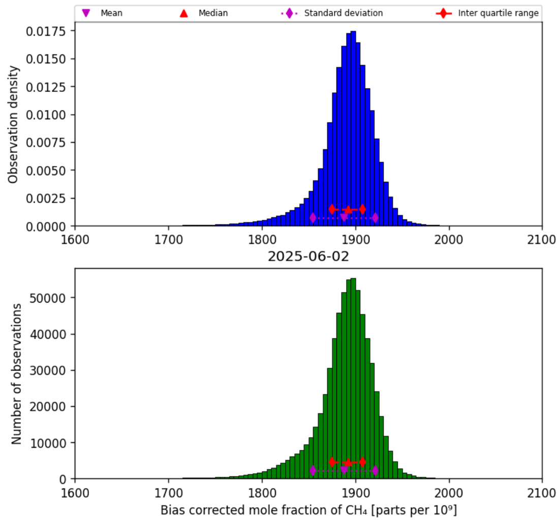
Figure 25: Histogram of “Bias corrected mole fraction of CH 4 ” for 2025-06-01 to 2025-06-03
