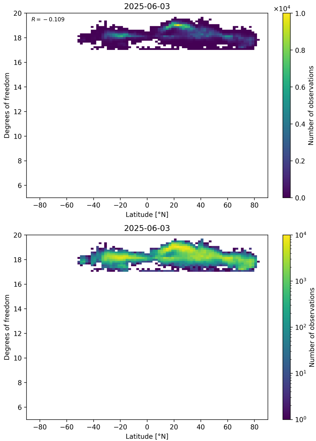
Figure 55: Scatter density plot of “Latitude” against “Degrees of freedom” for 2025-06-02 to 2025-06-04.
