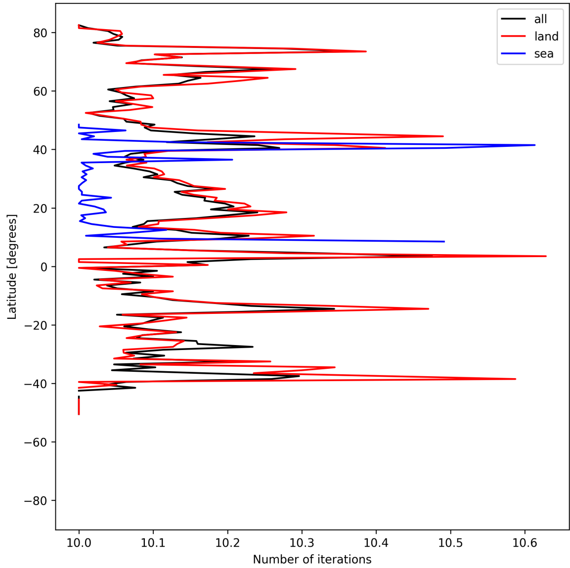
Figure 20: Zonal average of “Number of iterations” for 2025-06-02 to 2025-06-04.
