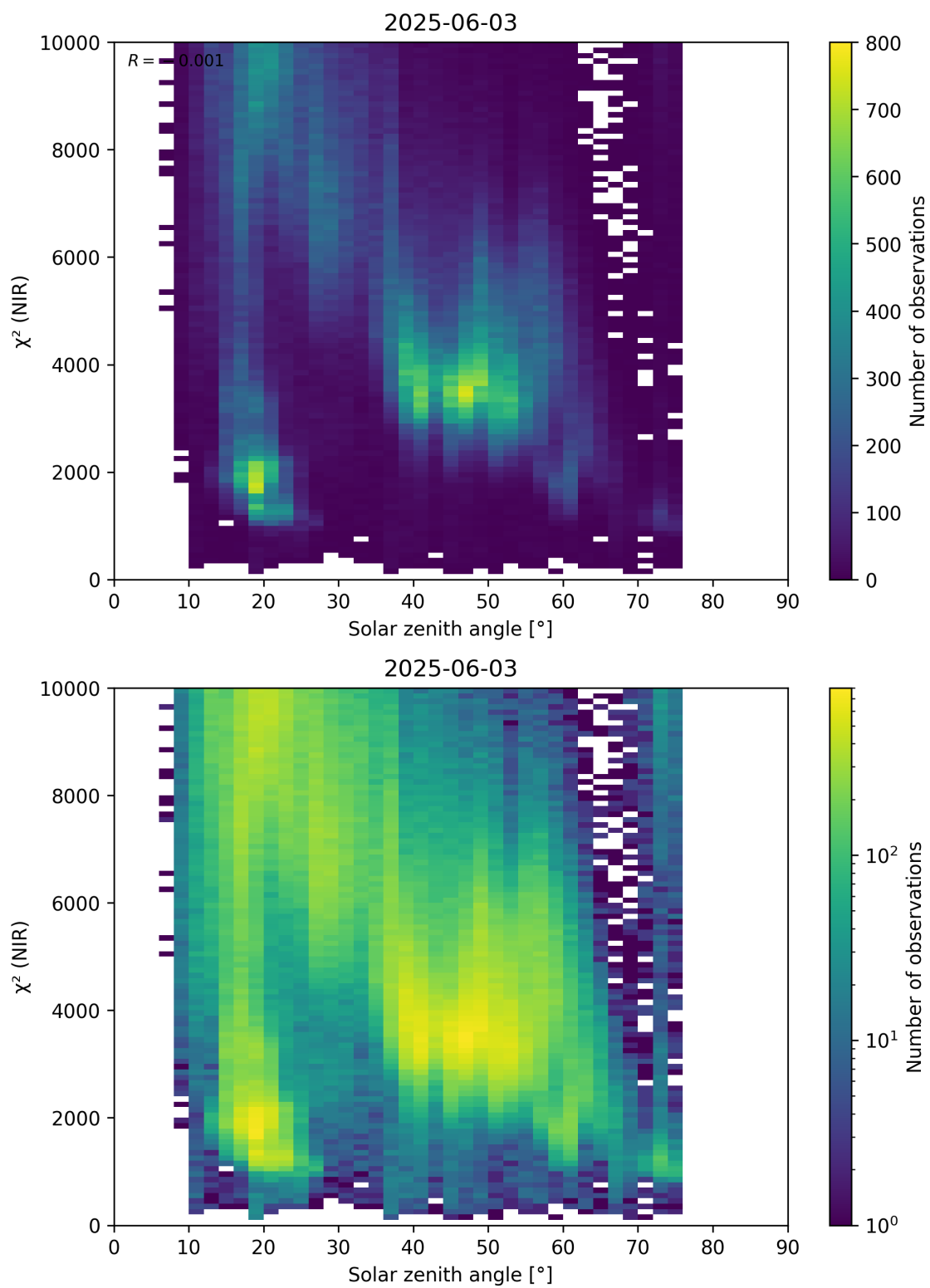
Figure 94: Scatter density plot of “Solar zenith angle” against “ \chi^2 (NIR)” for 2025-06-02 to 2025-06-04.
