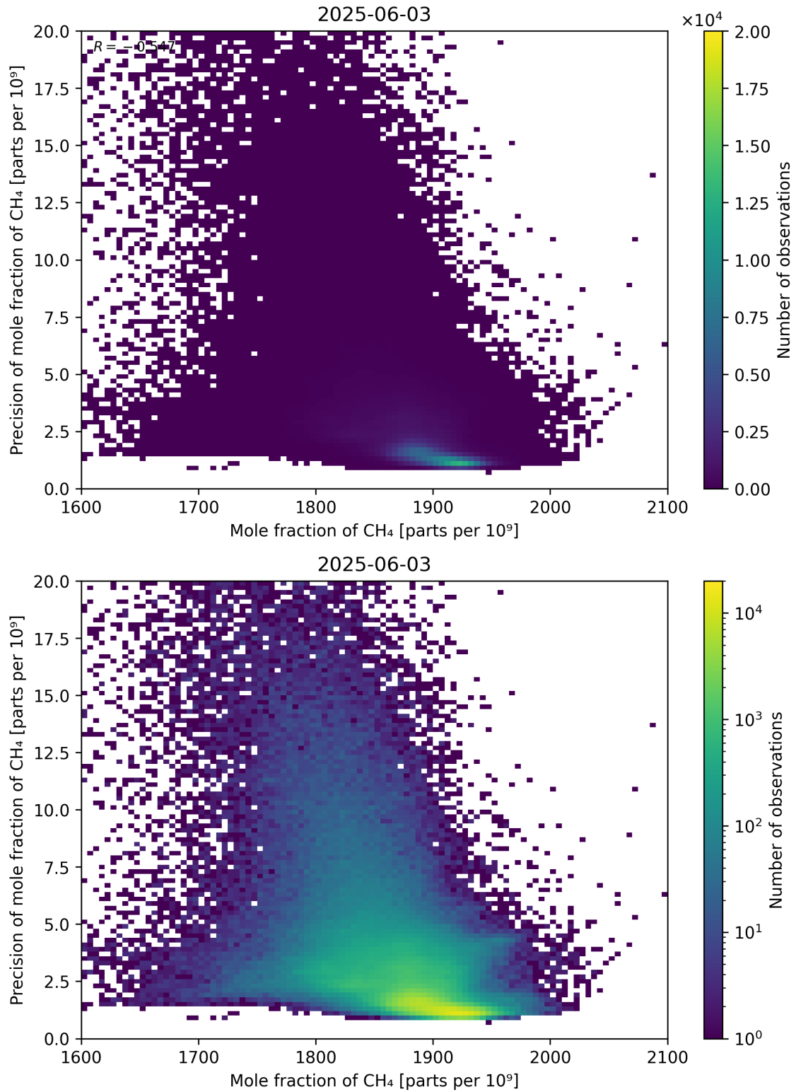
Figure 75: Scatter density plot of “Mole fraction of CH 4 ” against “Precision of mole fraction of CH 4 ” for 2025-06-02 to 2025-06-04.
