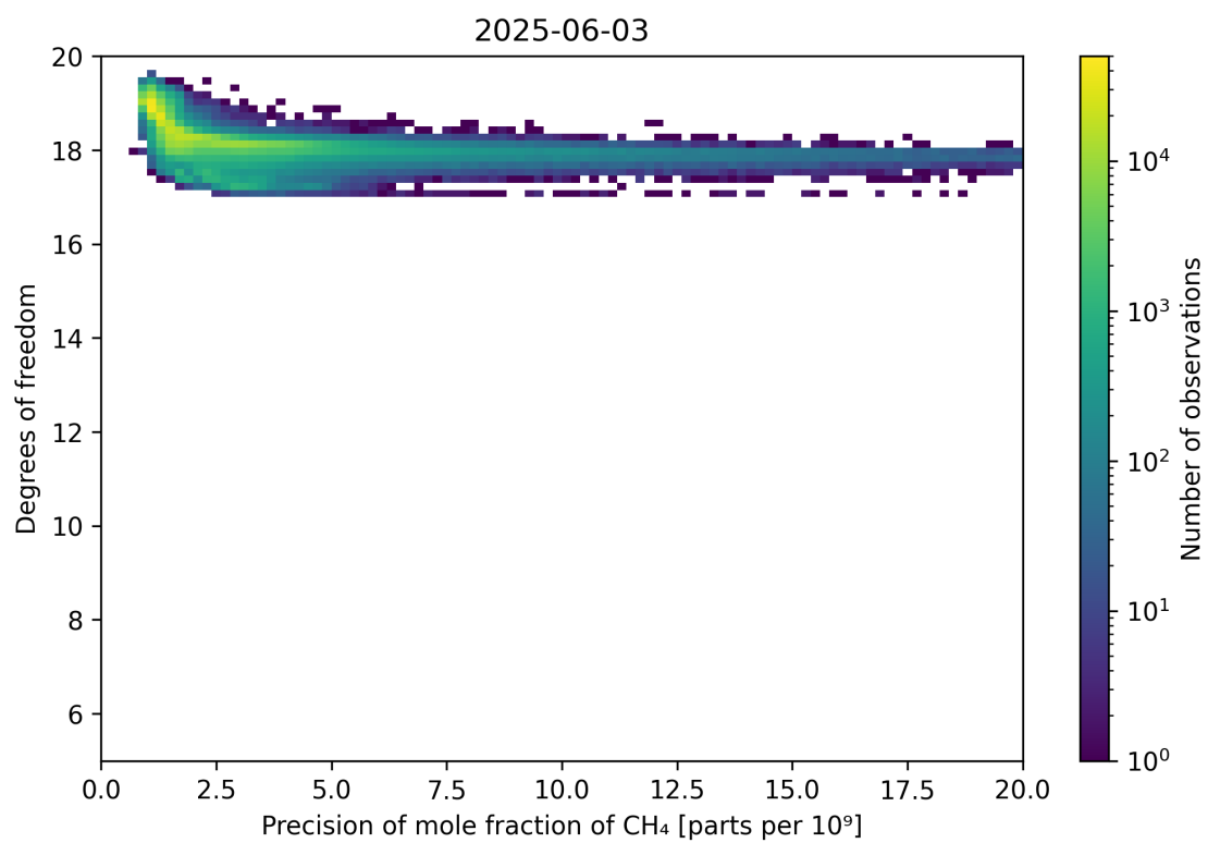
Figure 80: Scatter density plot of “Precision of mole fraction of CH 4 ” against “Degrees of freedom” for 2025-06-02 to 2025-06-04.
