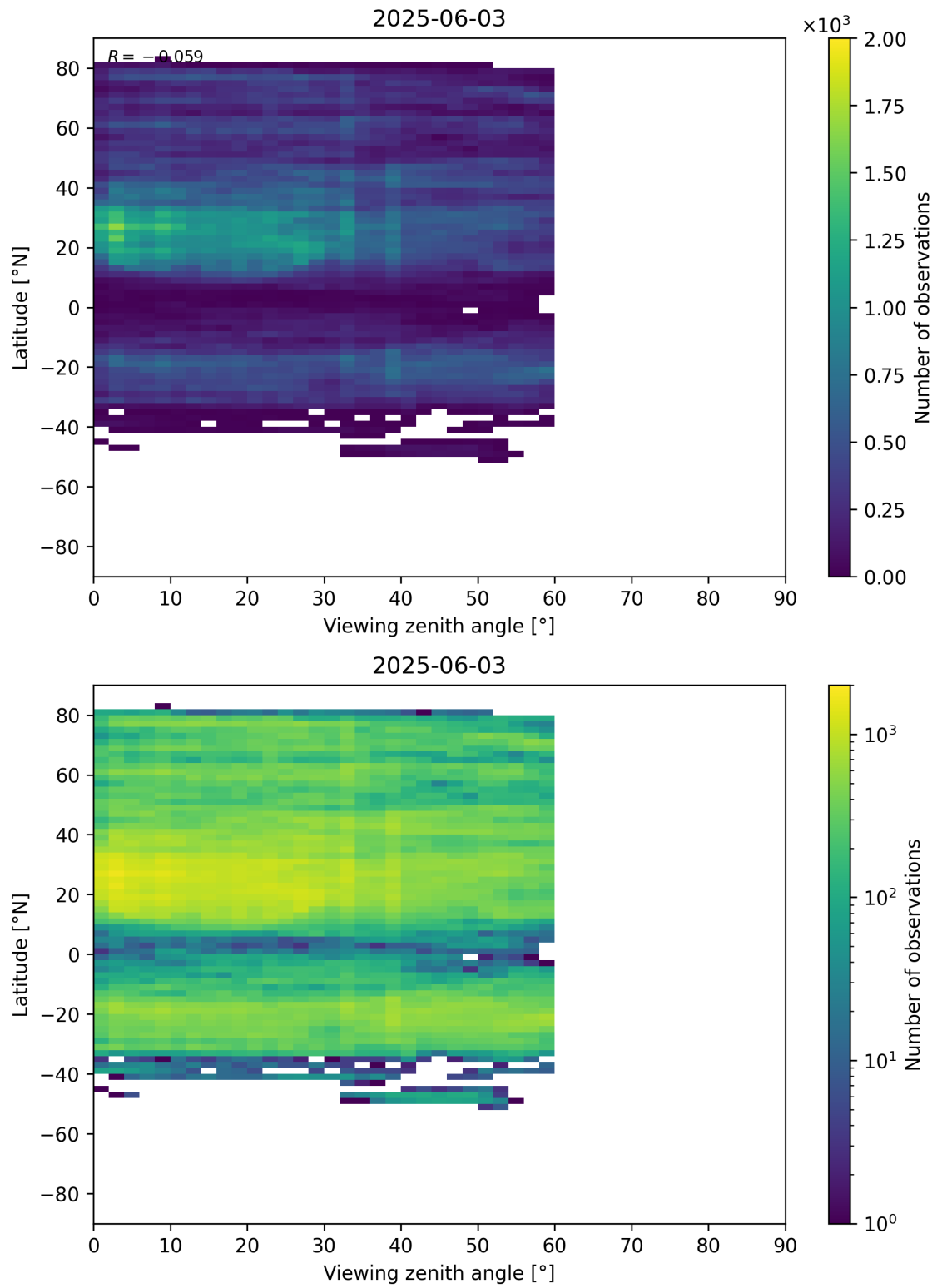
Figure 109: Scatter density plot of “Viewing zenith angle” against “Latitude” for 2025-06-02 to 2025-06-04.
