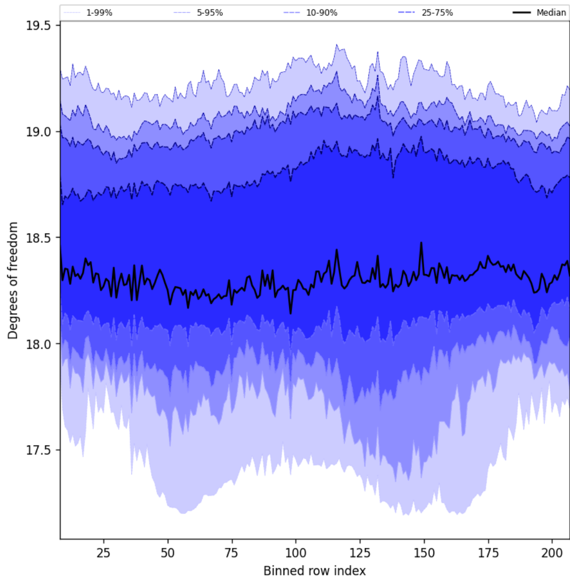
Figure 41: Along track statistics of “Degrees of freedom” for 2025-06-02 to 2025-06-04
