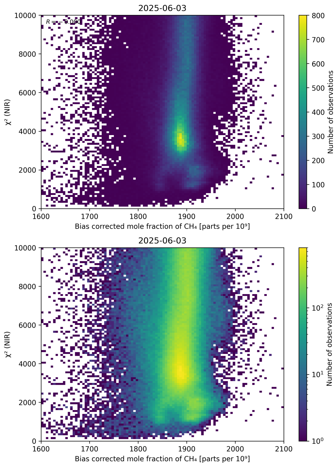
Figure 63: Scatter density plot of “Bias corrected mole fraction of \text{CH}_4 ” against “ \chi^2 (NIR)” for 2025-06-02 to 2025-06-04.
