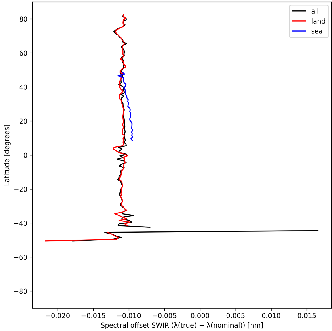
Figure 16: Zonal average of “Spectral offset SWIR ( \lambda_{\text{true}} - \lambda_{\text{nominal}} )” for 2025-06-02 to 2025-06-04.
