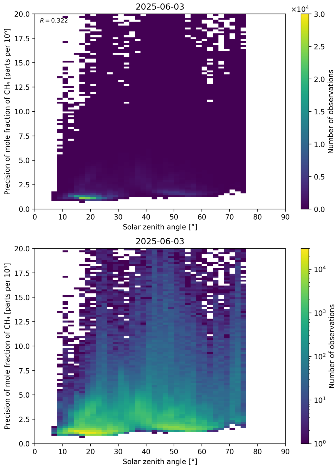
Figure 101: Scatter density plot of “Solar zenith angle” against “Precision of mole fraction of CH 4 ” for 2025-06-02 to 2025-06-04.
