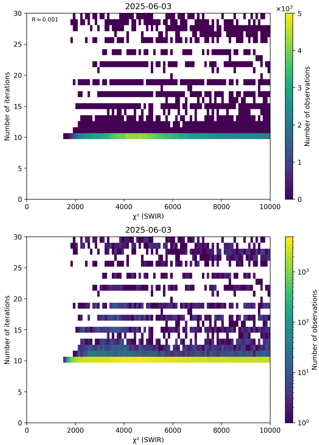
Figure 50: Scatter density plot of “ \chi^2 (SWIR)” against “Number of iterations” for 2025-06-02 to 2025-06-04.
