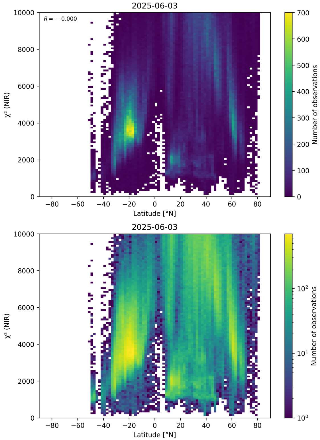
Figure 53: Scatter density plot of “Latitude” against “ \chi^2 (NIR)” for 2025-06-02 to 2025-06-04.
