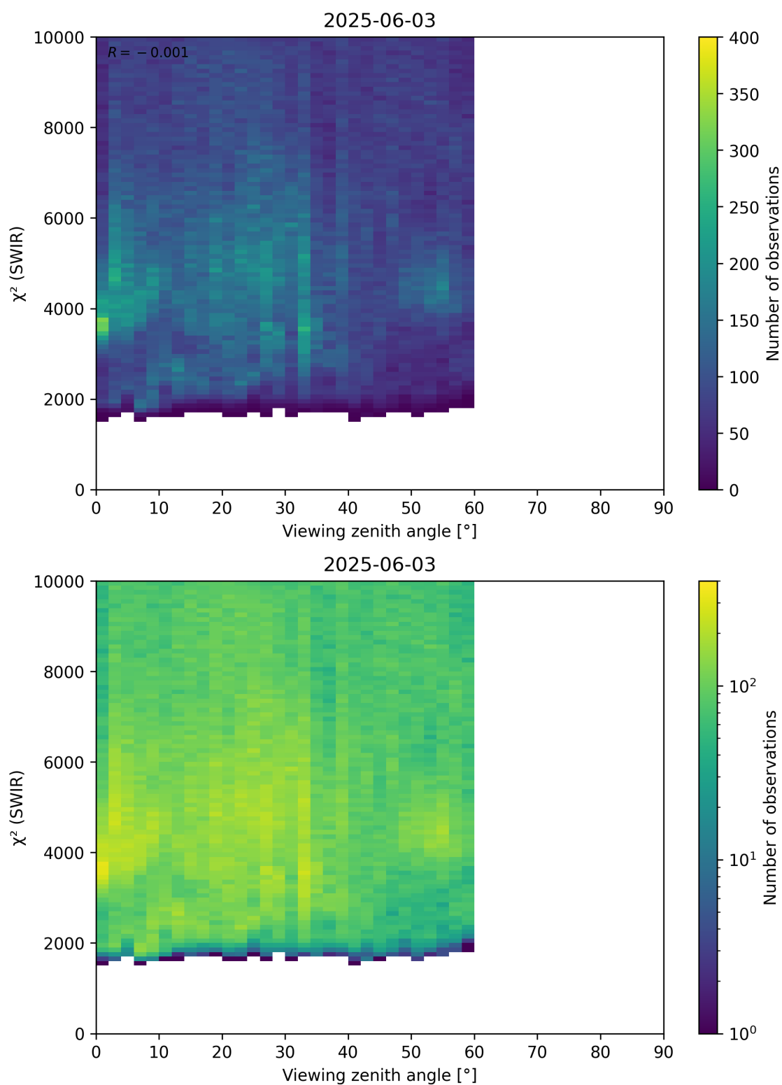
Figure 106: Scatter density plot of “Viewing zenith angle” against “ \chi^2 (SWIR)” for 2025-06-02 to 2025-06-04.
