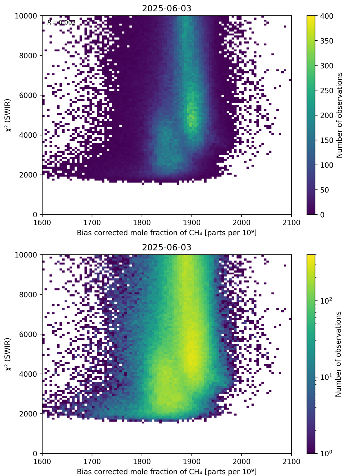
Figure 64: Scatter density plot of “Bias corrected mole fraction of \text{CH}_4 ” against “ \chi^2 (SWIR)” for 2025-06-02 to 2025-06-04.
