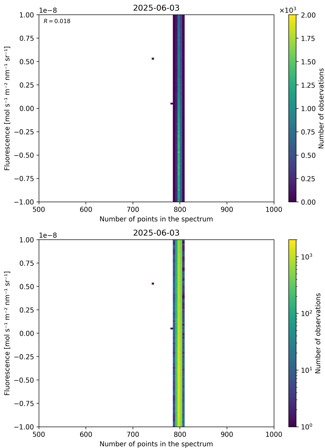
Figure 91: Scatter density plot of “Number of points in the spectrum” against “Fluorescence” for 2025-06-02 to 2025-06-04.
