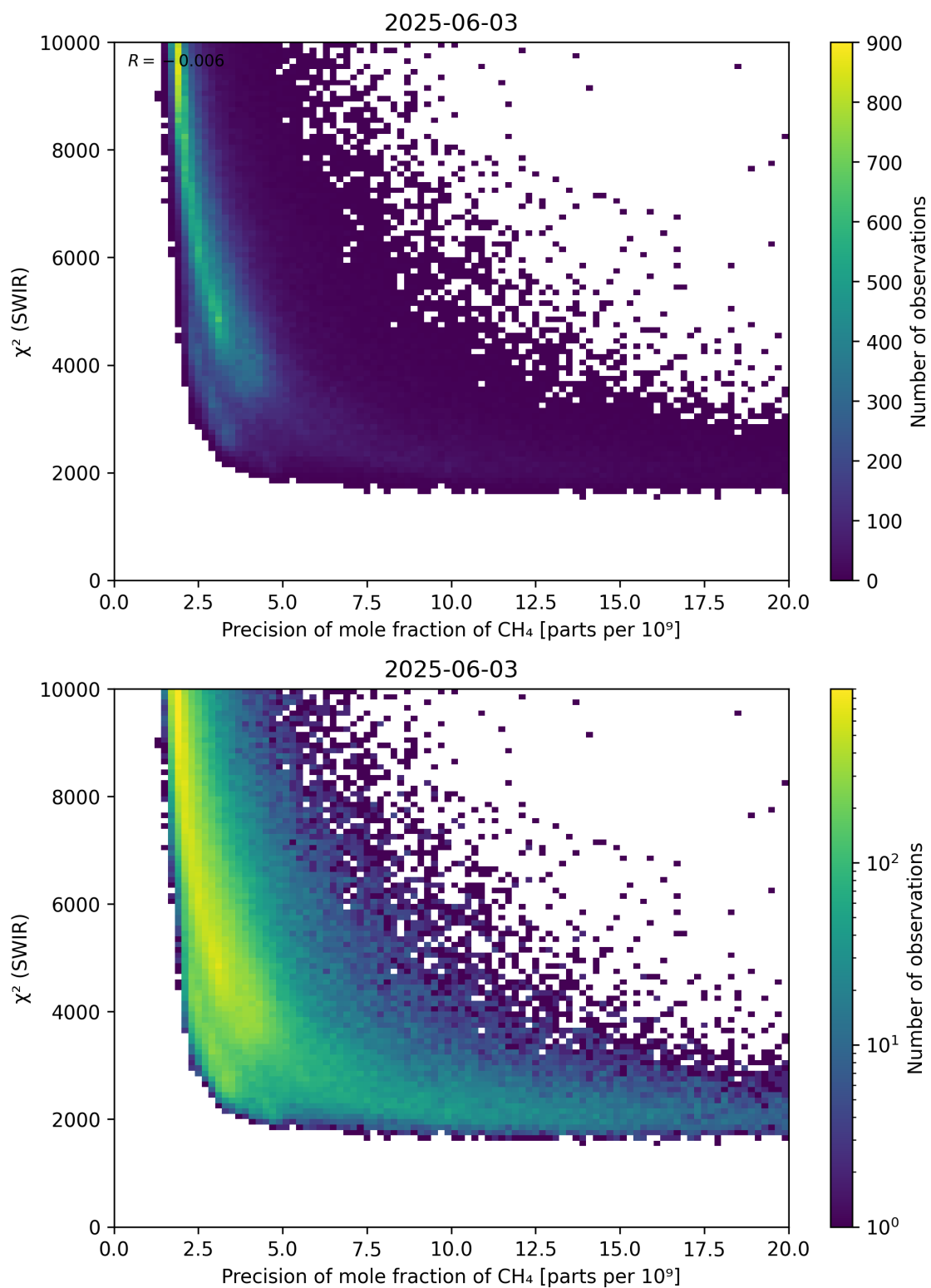
Figure 79: Scatter density plot of “Precision of mole fraction of \text{CH}_4 ” against “ \chi^2 (SWIR)” for 2025-06-02 to 2025-06-04.
