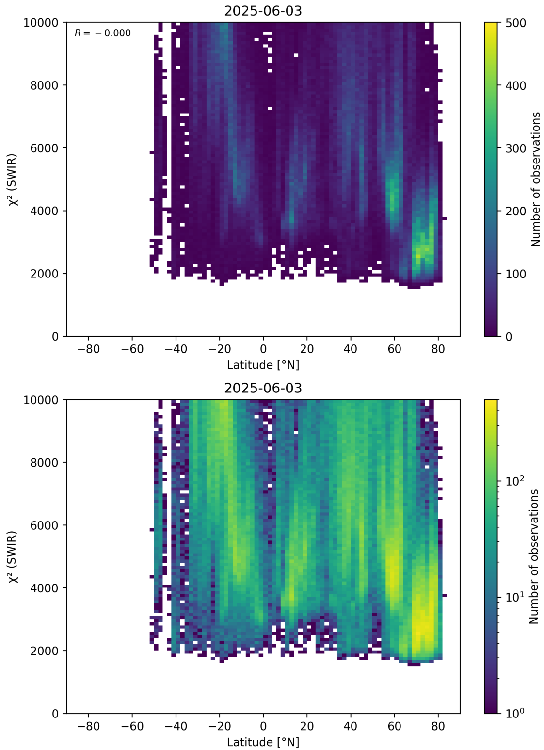
Figure 54: Scatter density plot of “Latitude” against “ \chi^2 (SWIR)” for 2025-06-02 to 2025-06-04.
