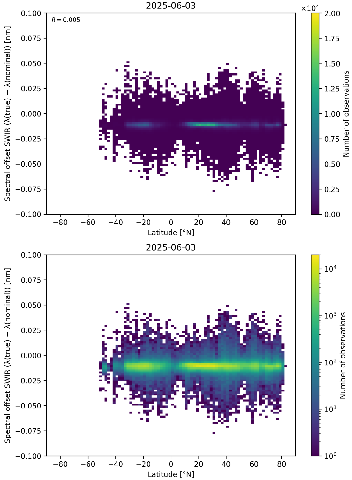
Figure 62: Scatter density plot of “Latitude” against “Spectral offset SWIR ( \lambda_{\text{true}} - \lambda_{\text{nominal}} )” for 2025-06-02 to 2025-06-04.
