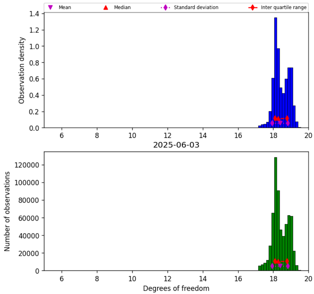
Figure 30: Histogram of “Degrees of freedom” for 2025-06-02 to 2025-06-04
