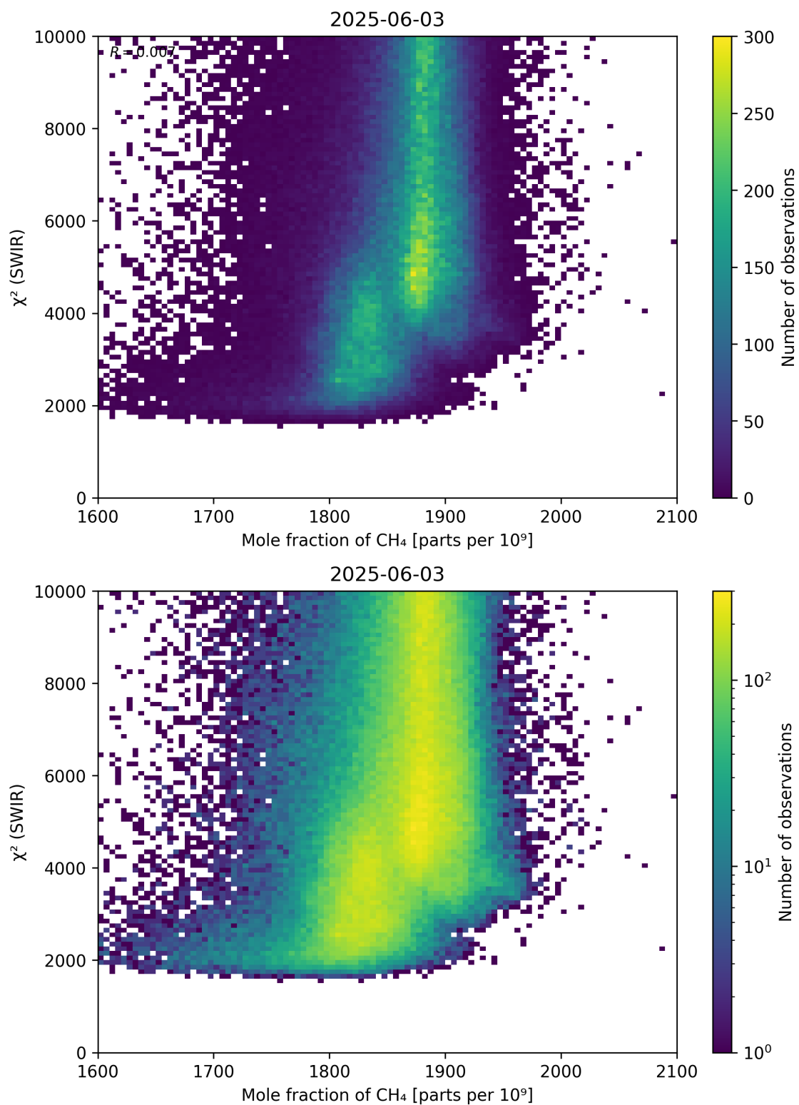
Figure 71: Scatter density plot of “Mole fraction of \text{CH}_4 ” against “ \chi^2 (SWIR)” for 2025-06-02 to 2025-06-04.
