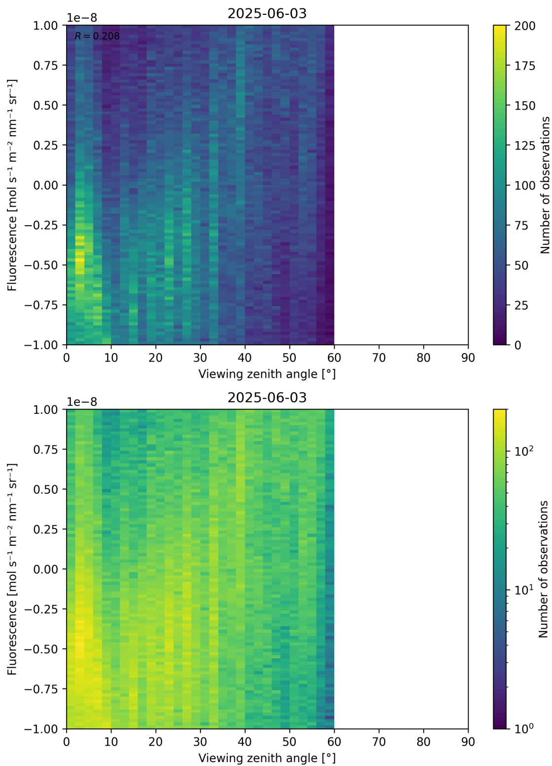
Figure 108: Scatter density plot of “Viewing zenith angle” against “Fluorescence” for 2025-06-02 to 2025-06-04.
