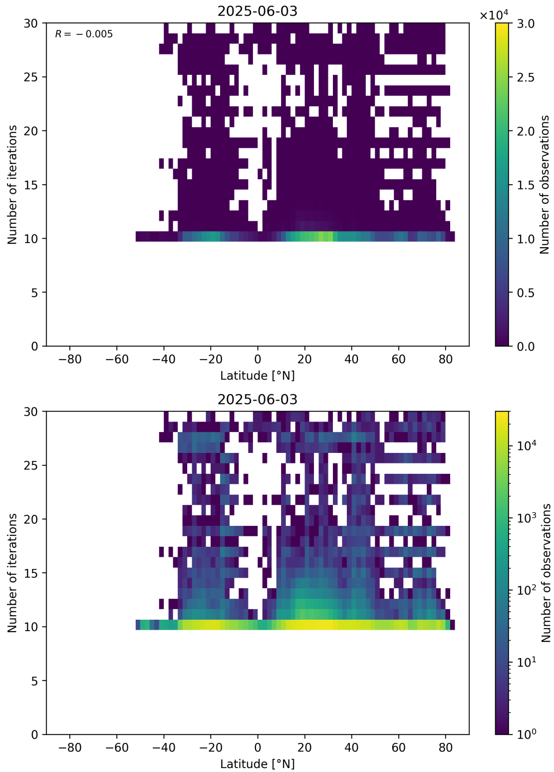
Figure 60: Scatter density plot of “Latitude” against “Number of iterations” for 2025-06-02 to 2025-06-04.
