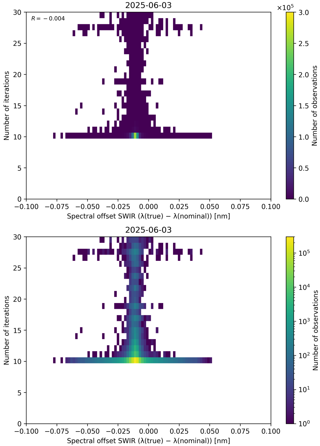
Figure 121: Scatter density plot of “Spectral offset SWIR ( \lambda_{\text{true}} - \lambda_{\text{nominal}} )” against “Number of iterations” for 2025-06-02 to 2025-06-04.
