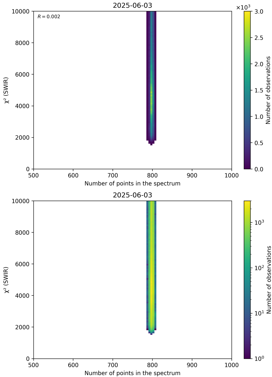
Figure 89: Scatter density plot of “Number of points in the spectrum” against “ \chi^2 (SWIR)” for 2025-06-02 to 2025-06-04.
