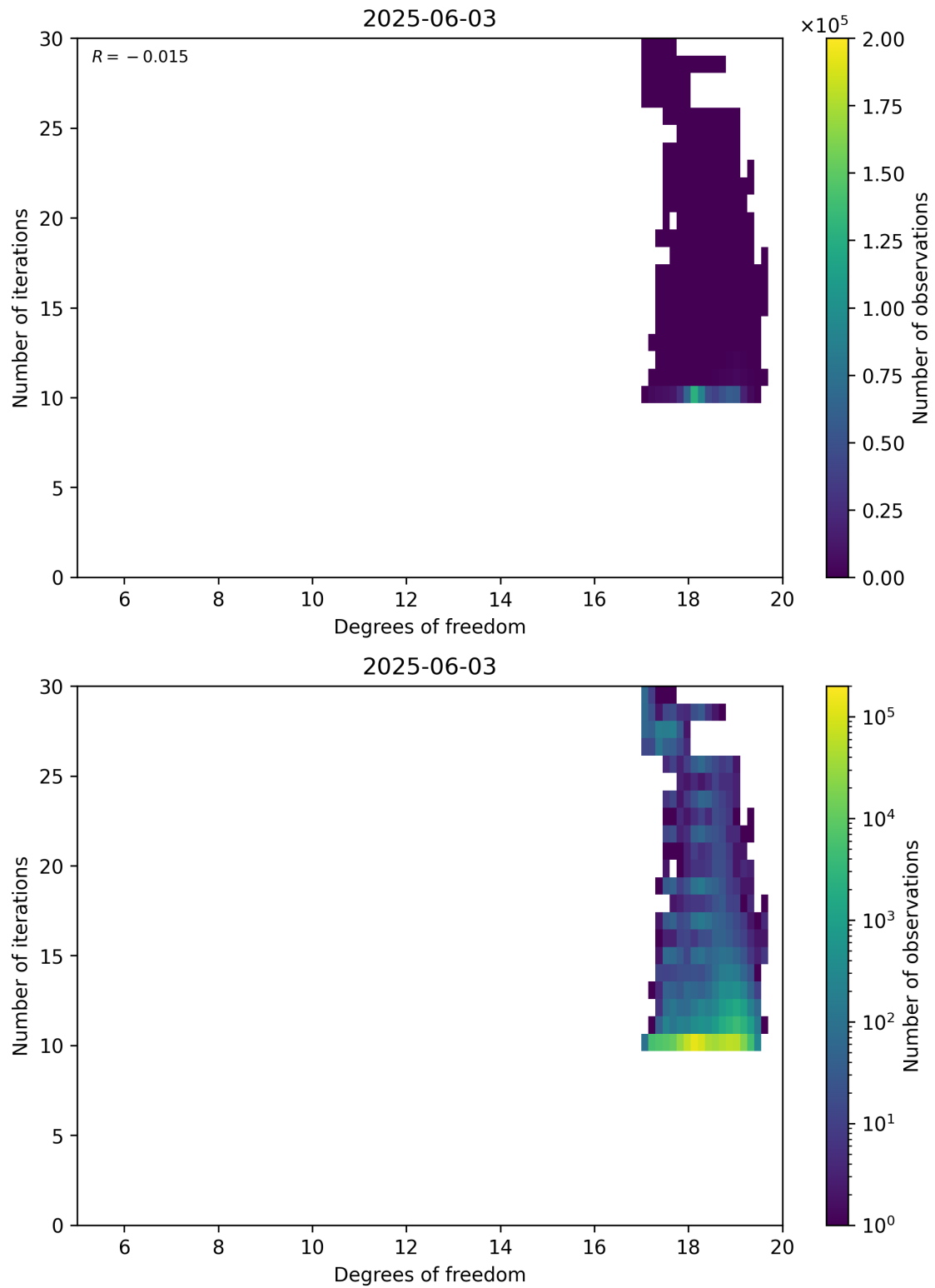
Figure 52: Scatter density plot of “Degrees of freedom” against “Number of iterations” for 2025-06-02 to 2025-06-04.
