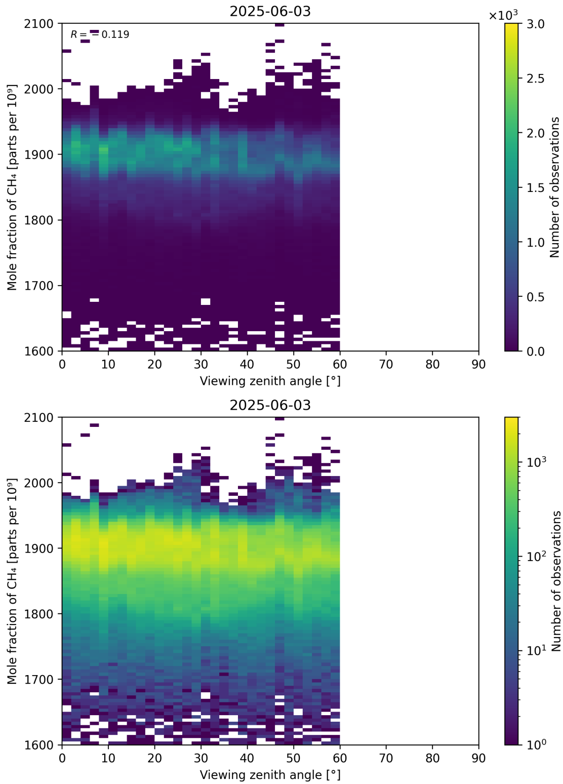
Figure 110: Scatter density plot of “Viewing zenith angle” against “Mole fraction of CH 4 ” for 2025-06-02 to 2025-06-04.
