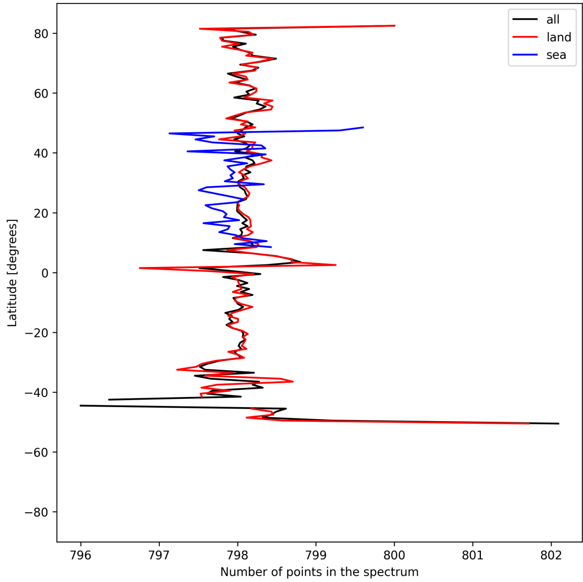
Figure 15: Zonal average of “Number of points in the spectrum” for 2025-06-02 to 2025-06-04.
