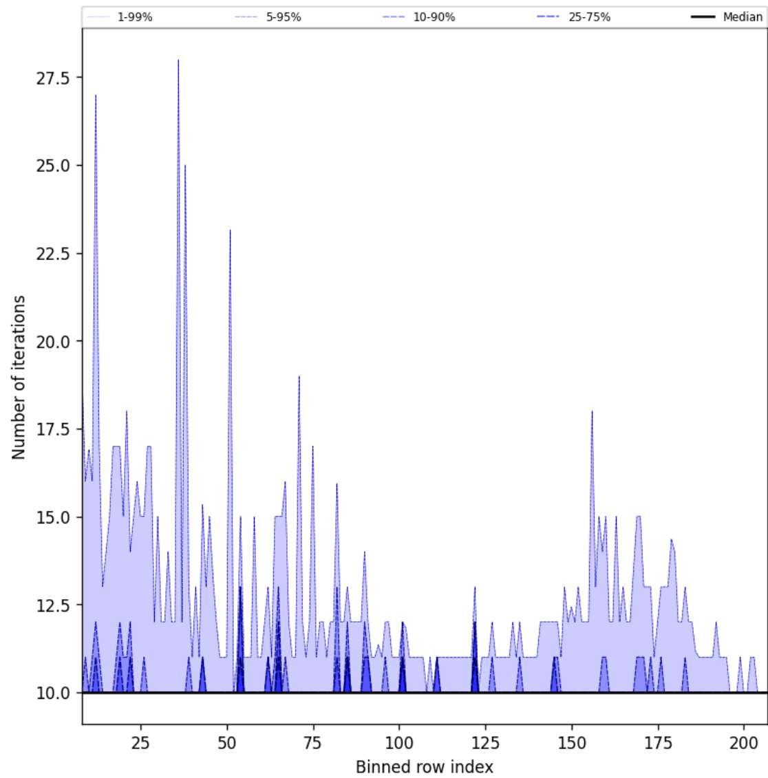
Figure 42: Along track statistics of “Number of iterations” for 2025-06-02 to 2025-06-04
