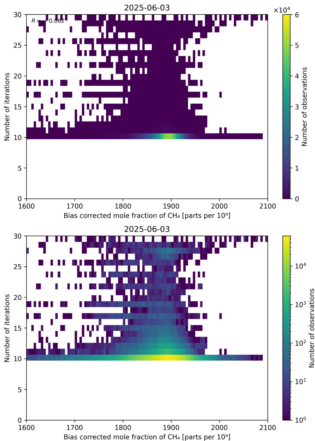
Figure 67: Scatter density plot of “Bias corrected mole fraction of \text{CH}_4 ” against “Number of iterations” for 2025-06-02 to 2025-06-04.
