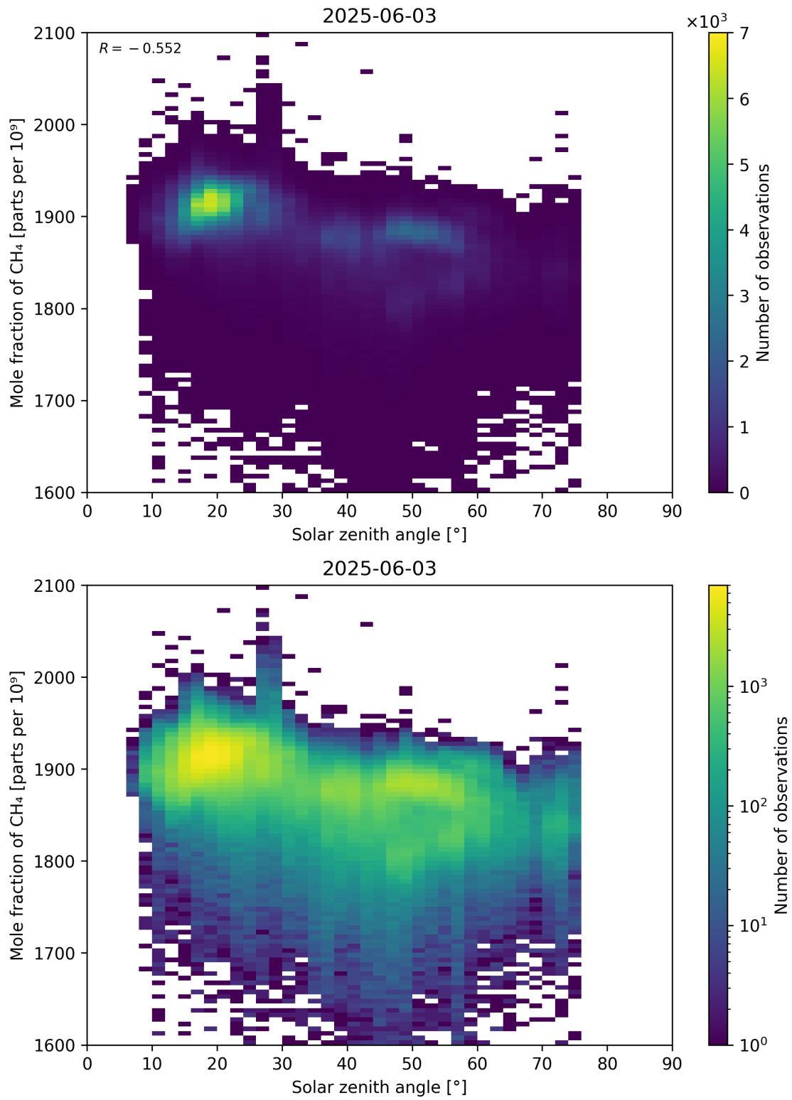
Figure 99: Scatter density plot of “Solar zenith angle” against “Mole fraction of CH 4 ” for 2025-06-02 to 2025-06-04.
