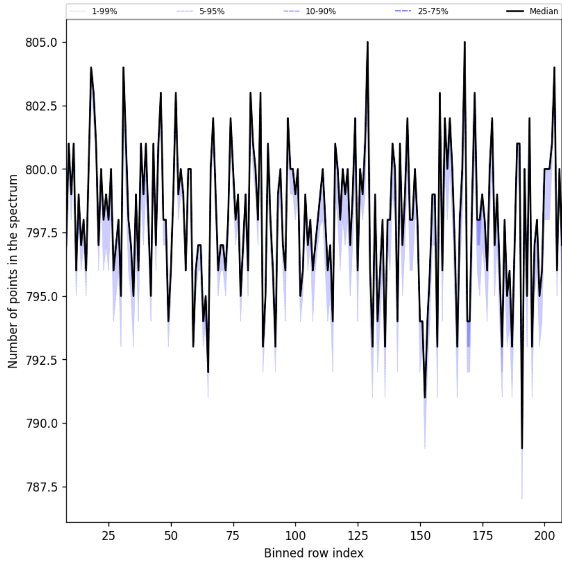
Figure 37: Along track statistics of “Number of points in the spectrum” for 2025-06-02 to 2025-06-04
