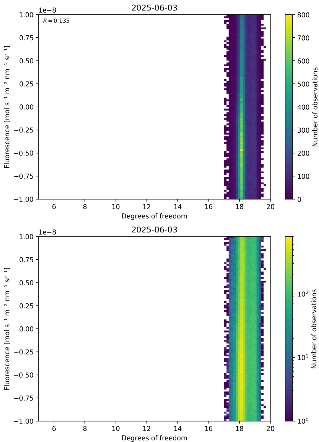
Figure 51: Scatter density plot of “Degrees of freedom” against “Fluorescence” for 2025-06-02 to 2025-06-04.
