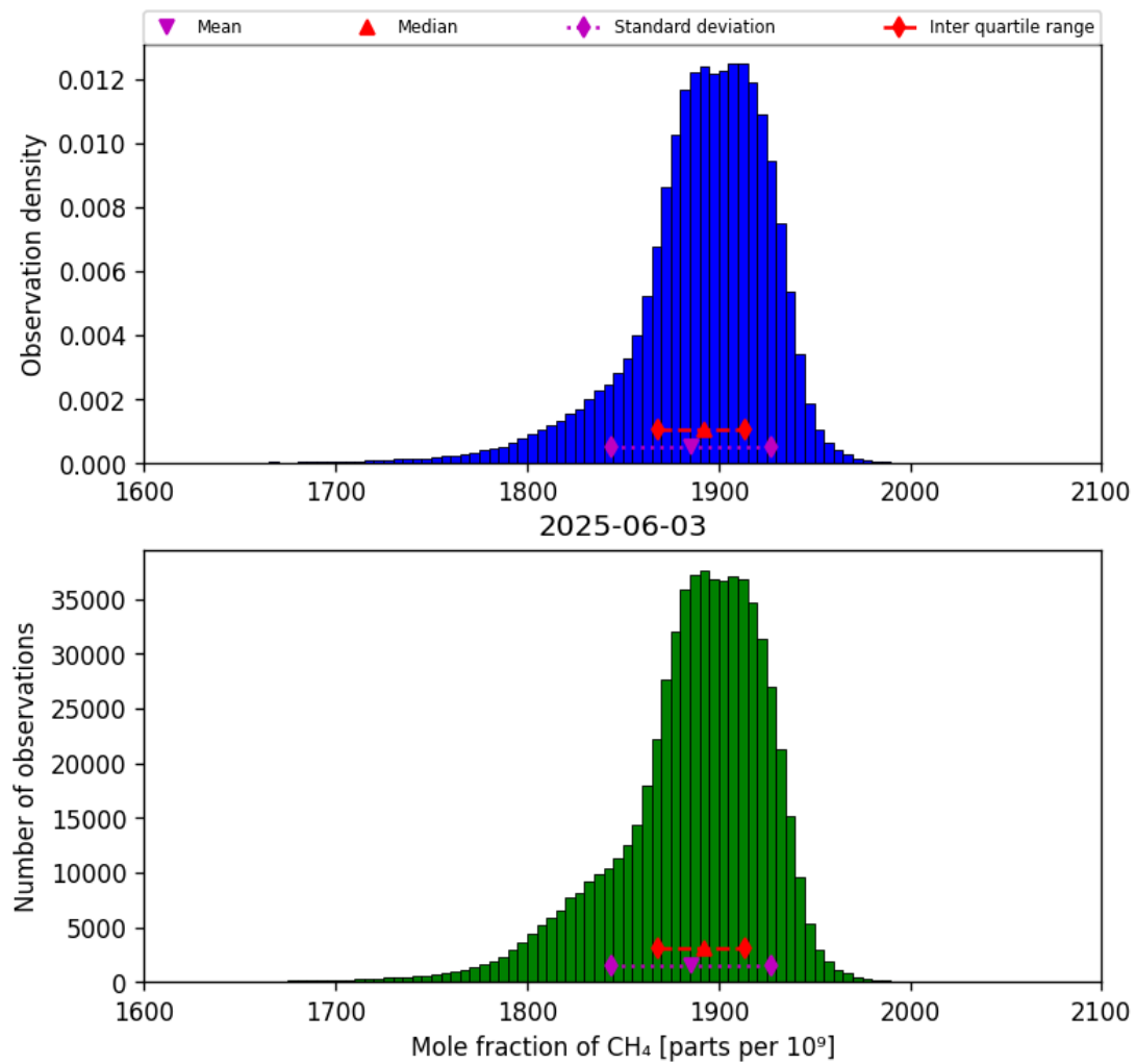
Figure 23: Histogram of “Mole fraction of CH 4 ” for 2025-06-02 to 2025-06-04
