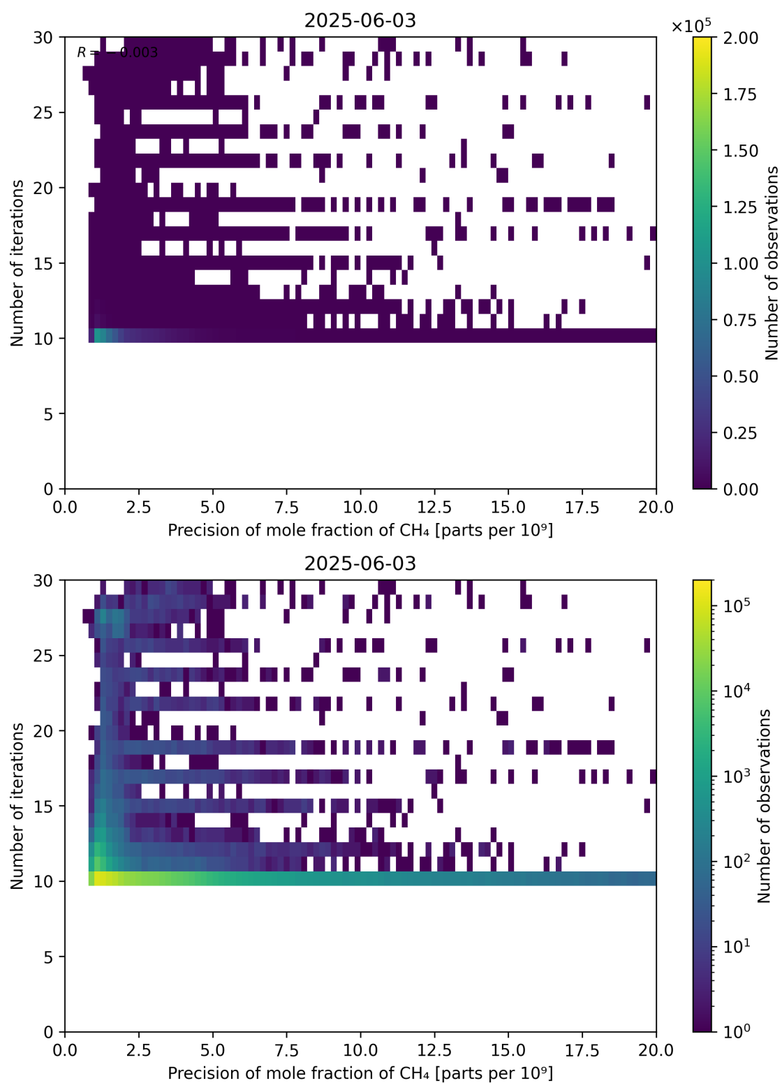
Figure 83: Scatter density plot of “Precision of mole fraction of CH 4 ” against “Number of iterations” for 2025-06-02 to 2025-06-04.
