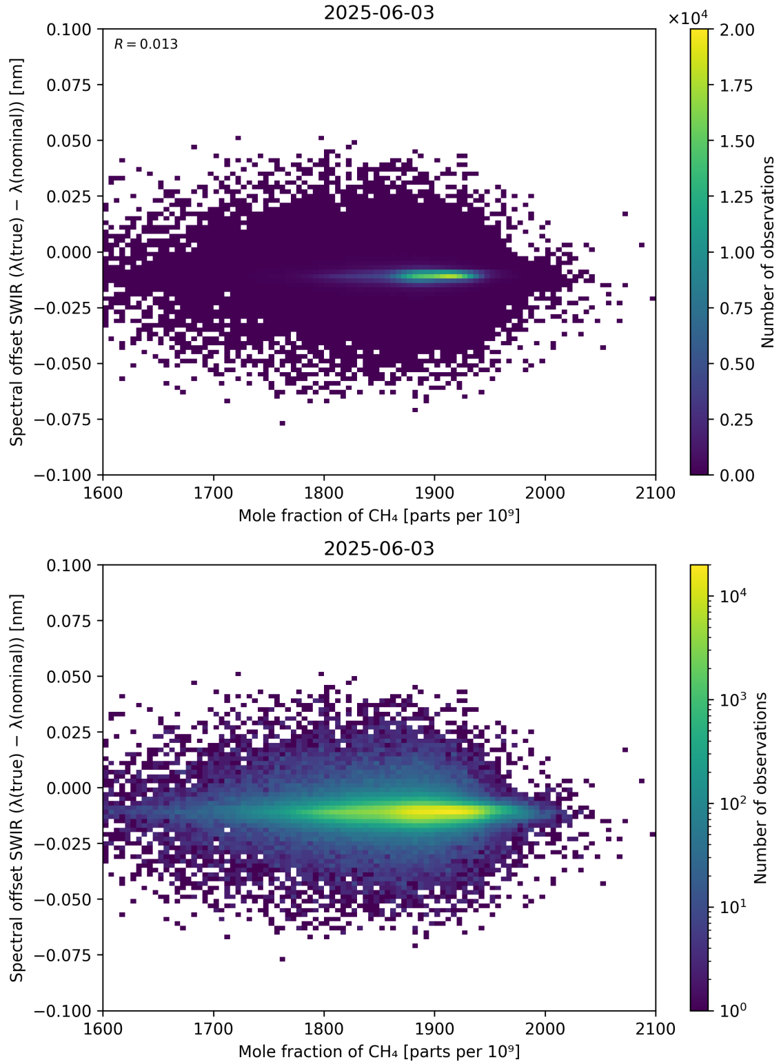
Figure 86: Scatter density plot of “Mole fraction of \text{CH}_4 ” against “Spectral offset SWIR ( \lambda_{\text{true}} - \lambda_{\text{nominal}} )” for 2025-06-02 to 2025-06-04.
