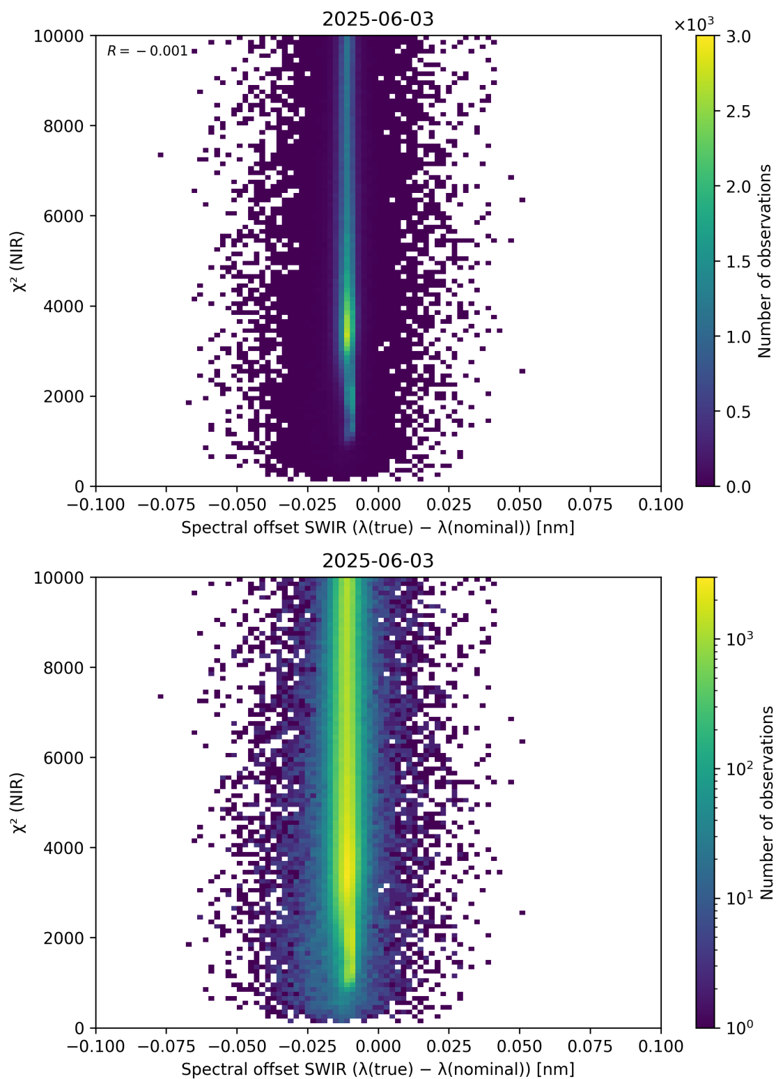
Figure 117: Scatter density plot of “Spectral offset SWIR ( \lambda_{\text{true}} - \lambda_{\text{nominal}} )” against “ \chi^2 (NIR)” for 2025-06-02 to 2025-06-04.
