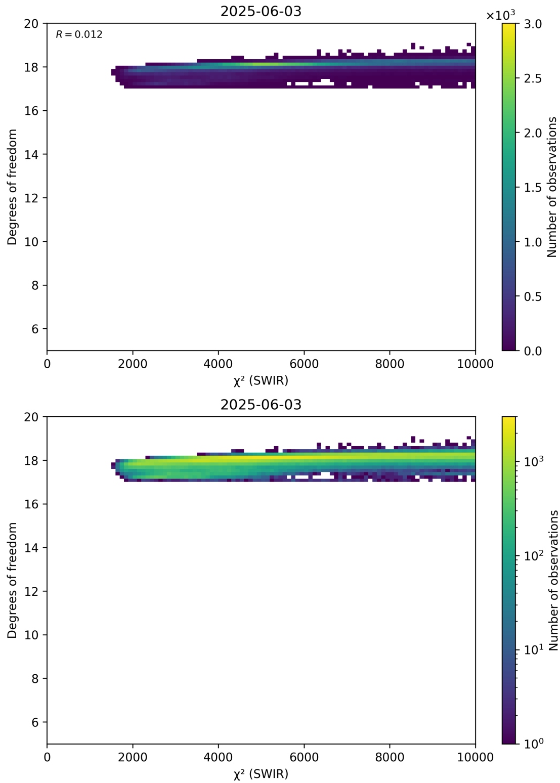
Figure 48: Scatter density plot of “ \chi^2 (SWIR)” against “Degrees of freedom” for 2025-06-02 to 2025-06-04.
