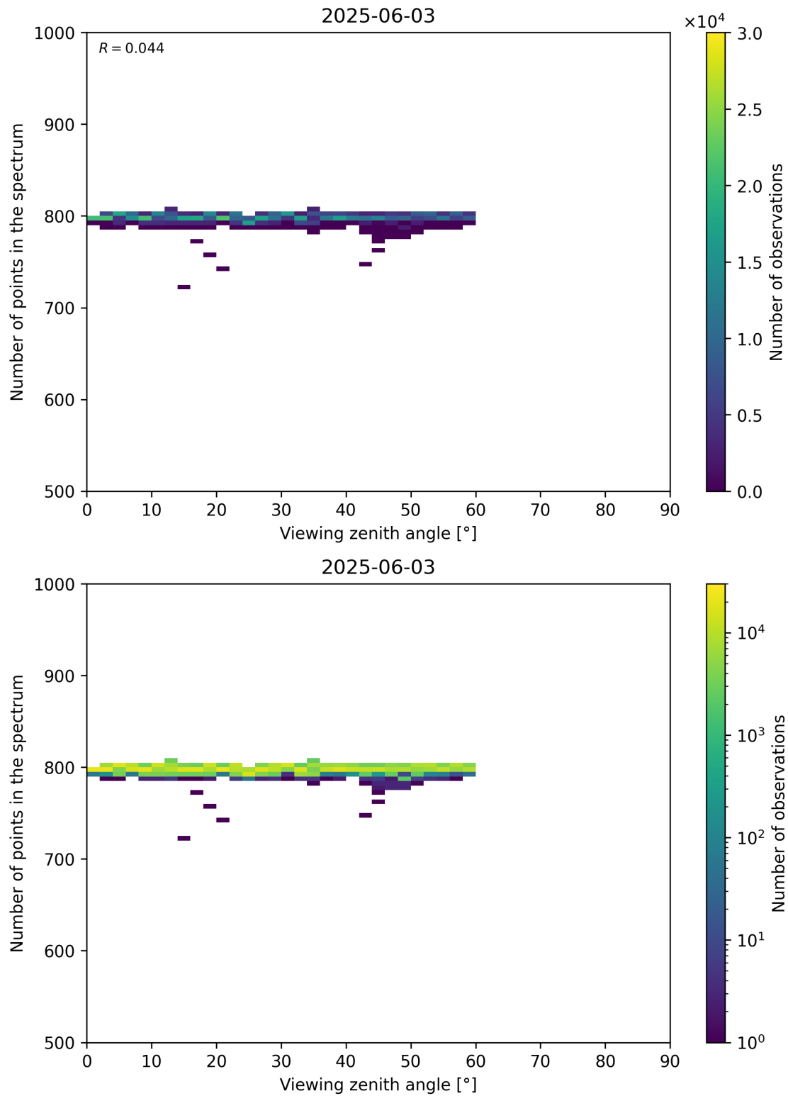
Figure 114: Scatter density plot of “Viewing zenith angle” against “Number of points in the spectrum” for 2025-06-02 to 2025-06-04.
