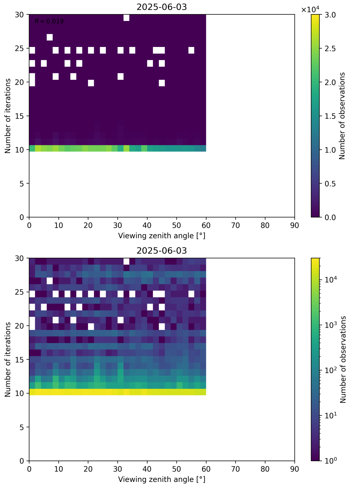
Figure 113: Scatter density plot of “Viewing zenith angle” against “Number of iterations” for 2025-06-02 to 2025-06-04.
