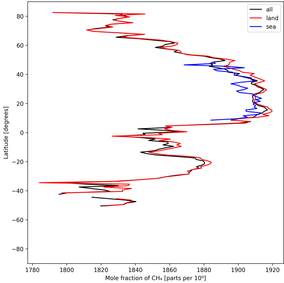
Figure 12: Zonal average of “Mole fraction of \text{CH}_4 ” for 2025-06-02 to 2025-06-04.
