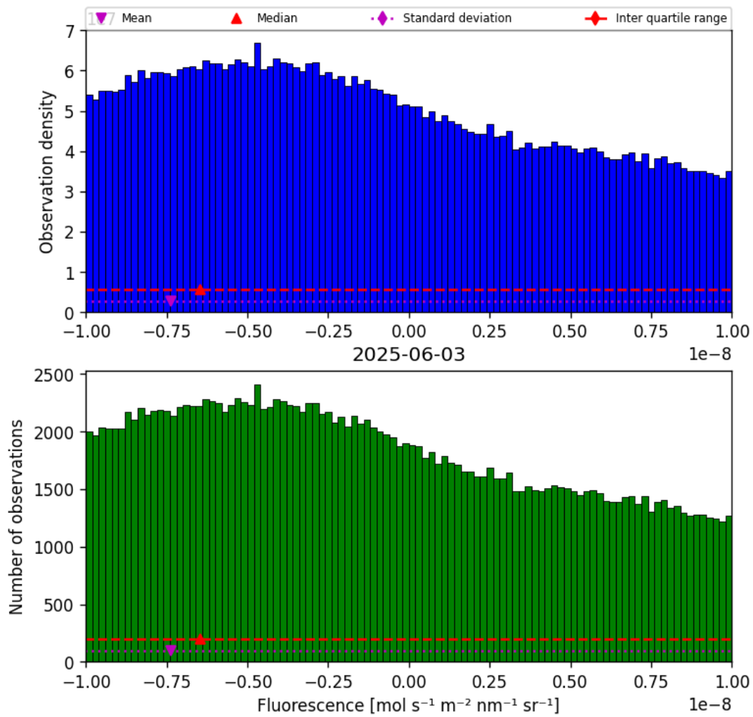
Figure 32: Histogram of “Fluorescence” for 2025-06-02 to 2025-06-04
