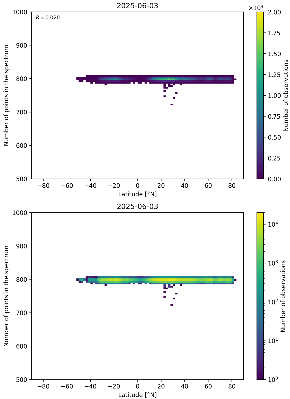
Figure 61: Scatter density plot of “Latitude” against “Number of points in the spectrum” for 2025-06-02 to 2025-06-04.
