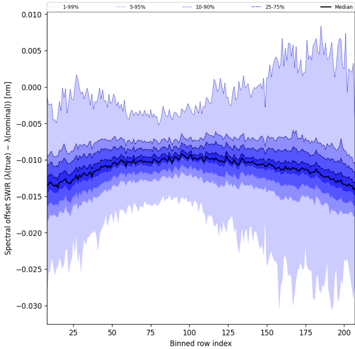
Figure 38: Along track statistics of “Spectral offset SWIR ( \lambda_{\text{true}} - \lambda_{\text{nominal}} )” for 2025-06-02 to 2025-06-04
