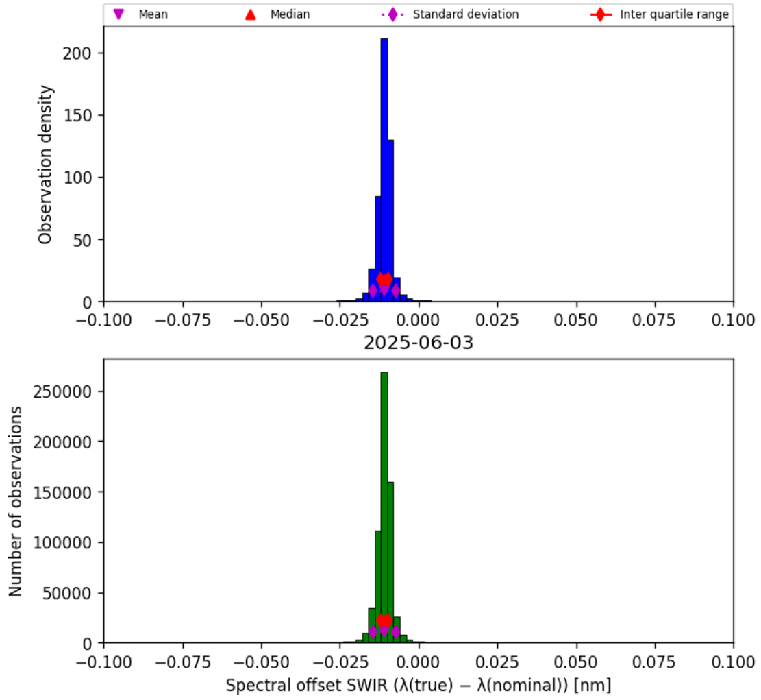
Figure 27: Histogram of “Spectral offset SWIR ( \lambda_{\text{true}} - \lambda_{\text{nominal}} )” for 2025-06-02 to 2025-06-04
