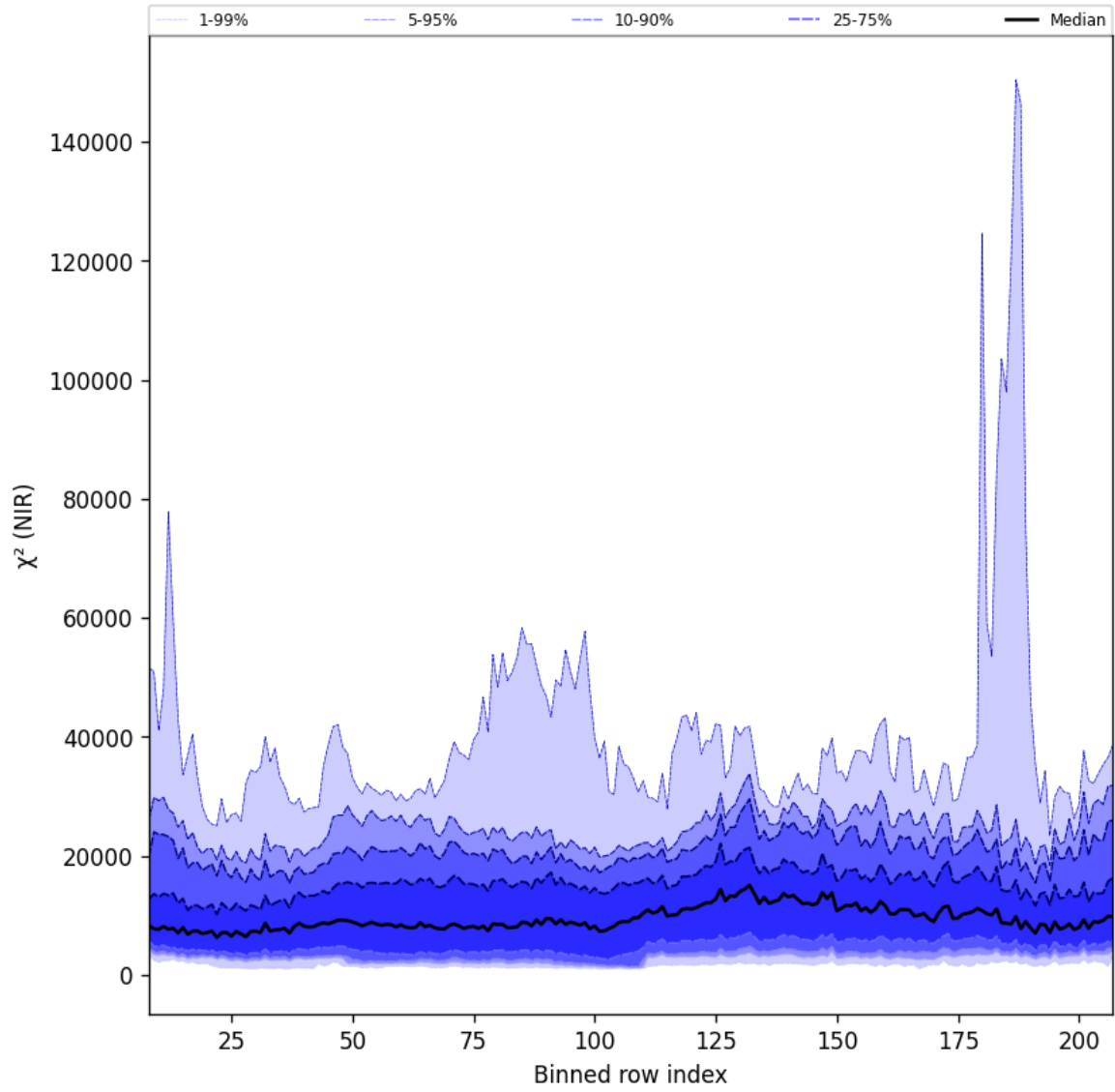
Figure 40: Along track statistics of “ \chi^2 (NIR)” for 2025-06-02 to 2025-06-04
