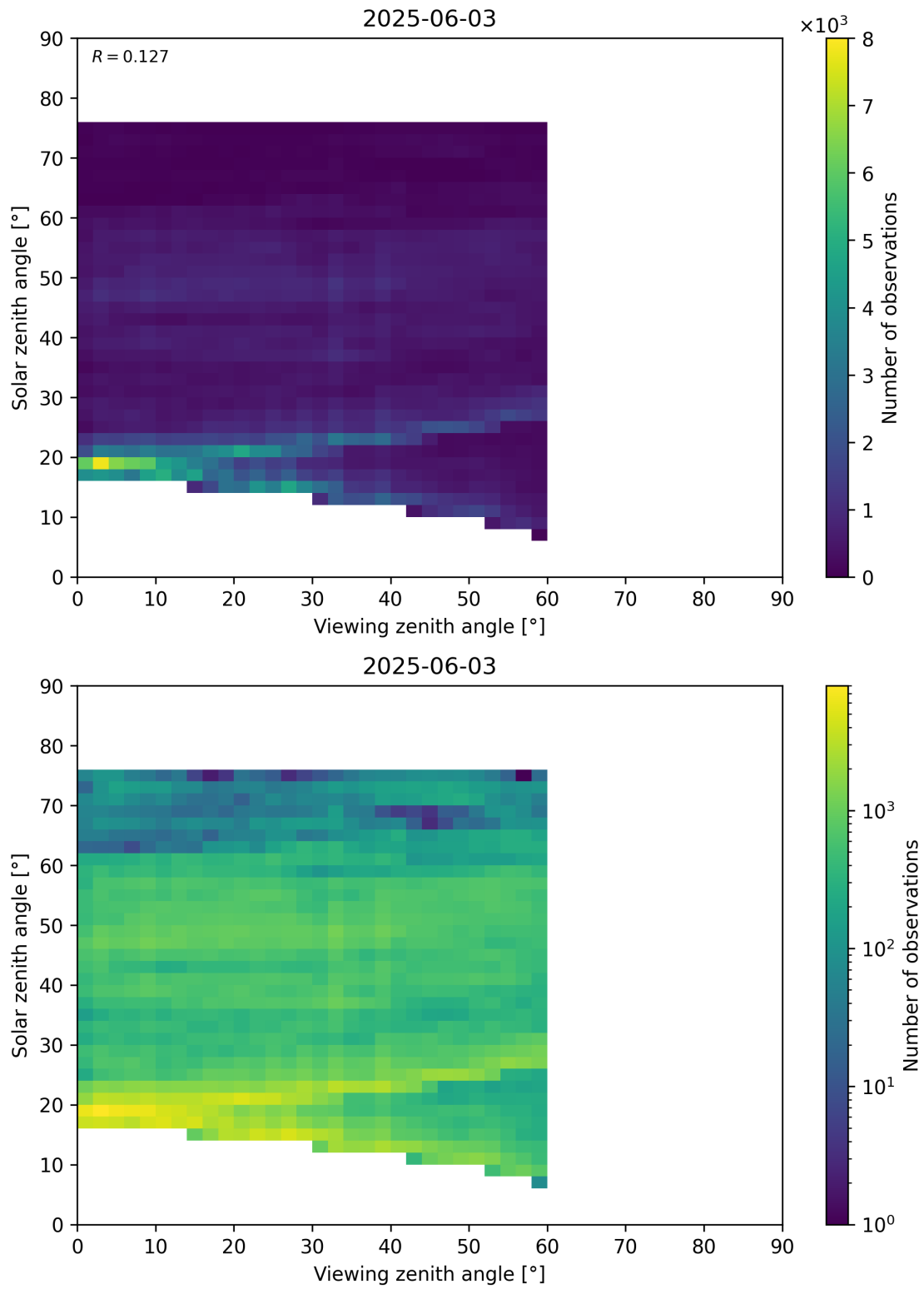
Figure 115: Scatter density plot of “Viewing zenith angle” against “Solar zenith angle” for 2025-06-02 to 2025-06-04.
