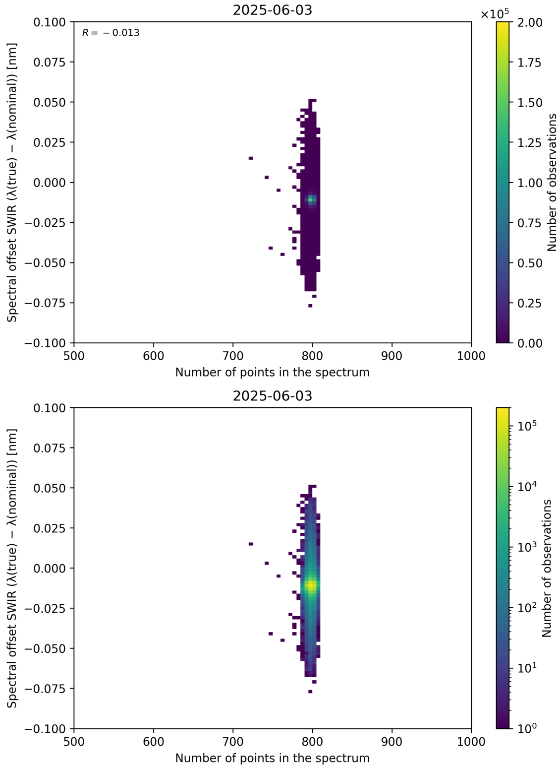
Figure 93: Scatter density plot of “Number of points in the spectrum” against “Spectral offset SWIR ( \lambda_{\text{true}} - \lambda_{\text{nominal}} )” for 2025-06-02 to 2025-06-04.
