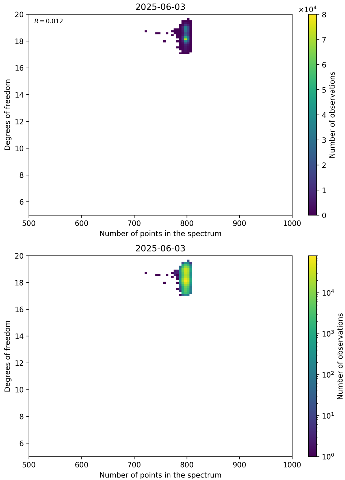
Figure 90: Scatter density plot of “Number of points in the spectrum” against “Degrees of freedom” for 2025-06-02 to 2025-06-04.
