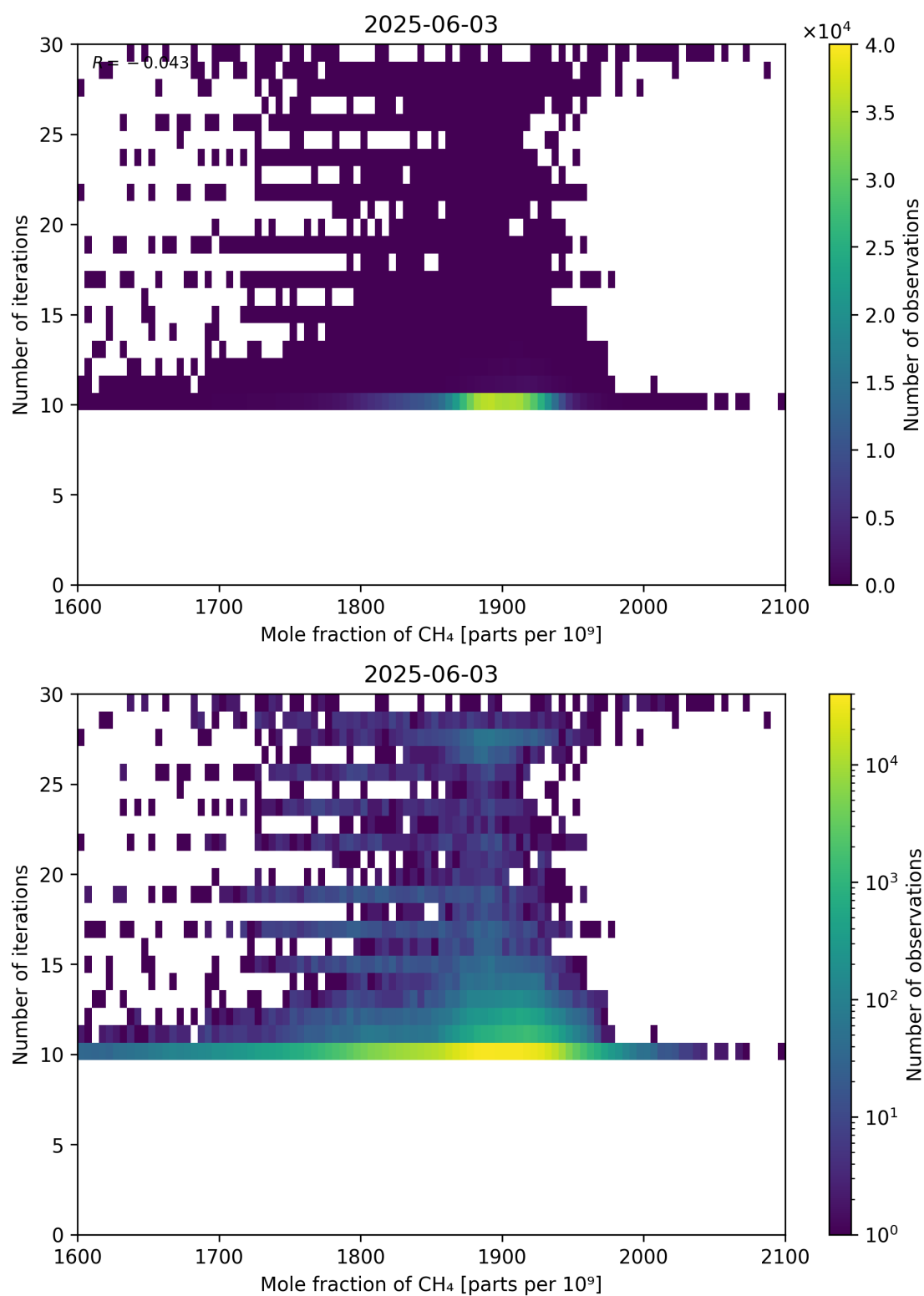
Figure 76: Scatter density plot of “Mole fraction of CH 4 ” against “Number of iterations” for 2025-06-02 to 2025-06-04.
