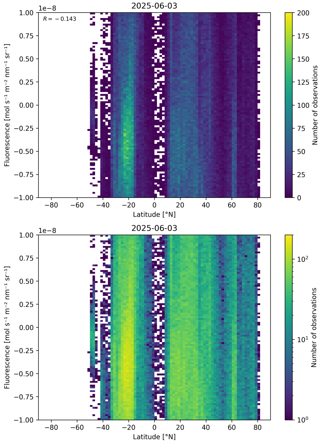
Figure 56: Scatter density plot of “Latitude” against “Fluorescence” for 2025-06-02 to 2025-06-04.
