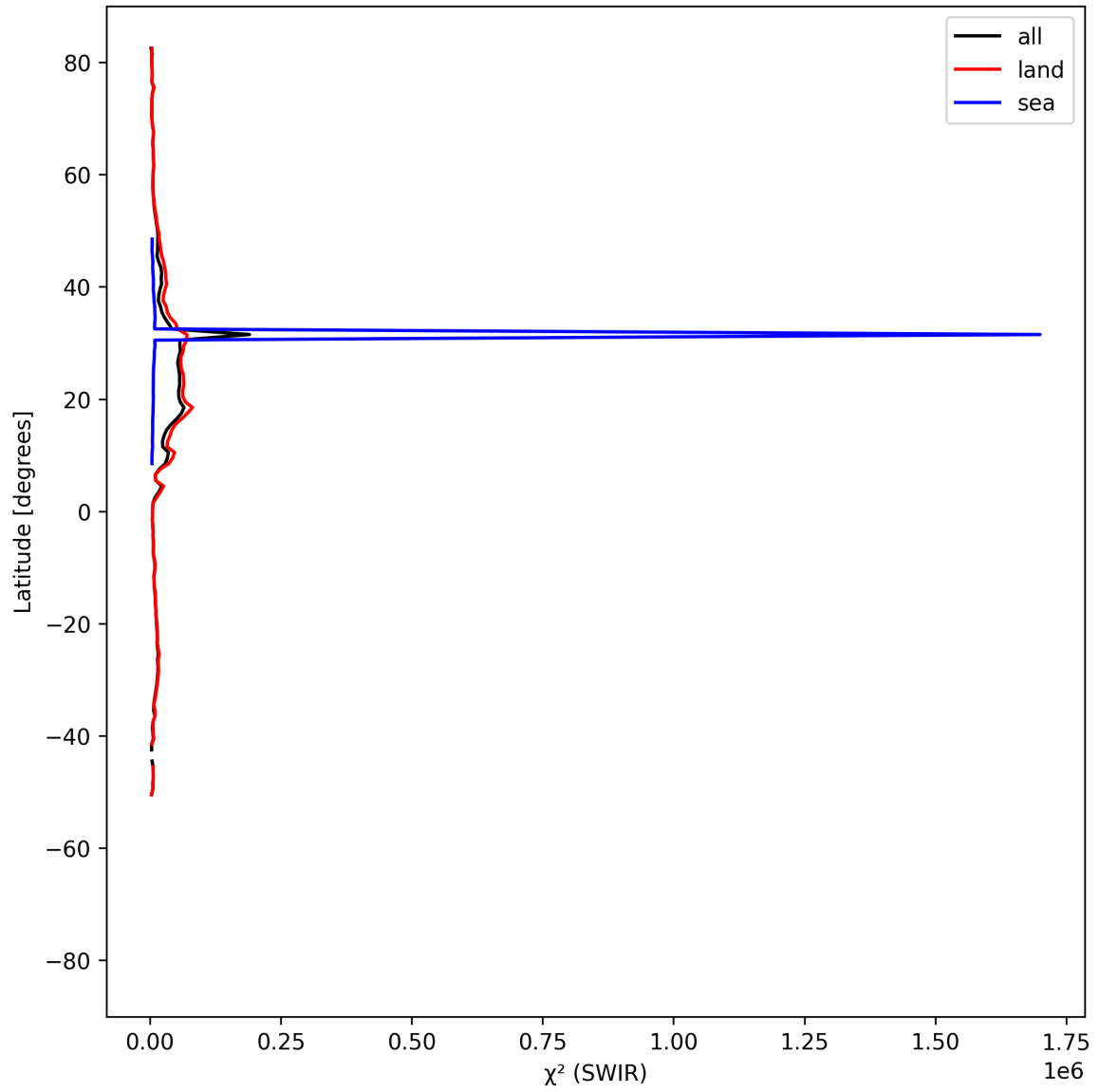
Figure 17: Zonal average of “ \chi^2 (SWIR)” for 2025-06-02 to 2025-06-04.
