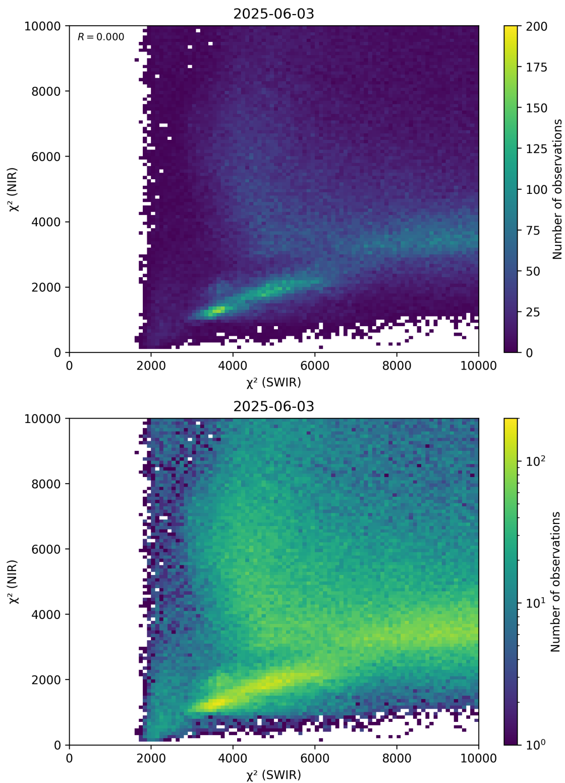
Figure 47: Scatter density plot of “ \chi^2 (SWIR)” against “ \chi^2 (NIR)” for 2025-06-02 to 2025-06-04.
