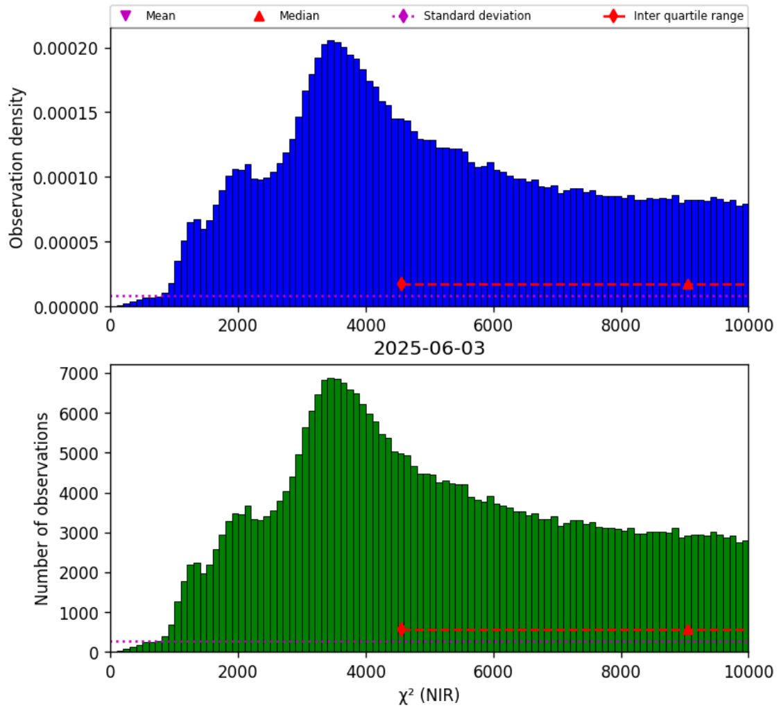
Figure 29: Histogram of " \chi^2 (NIR)" for 2025-06-02 to 2025-06-04
