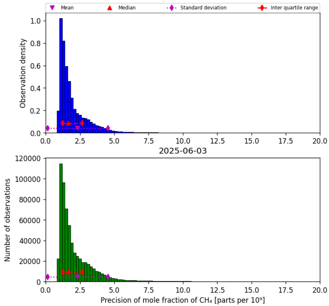
Figure 24: Histogram of “Precision of mole fraction of CH 4 ” for 2025-06-02 to 2025-06-04
