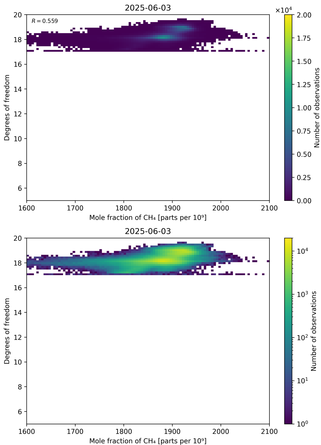
Figure 72: Scatter density plot of “Mole fraction of CH 4 ” against “Degrees of freedom” for 2025-06-02 to 2025-06-04.
