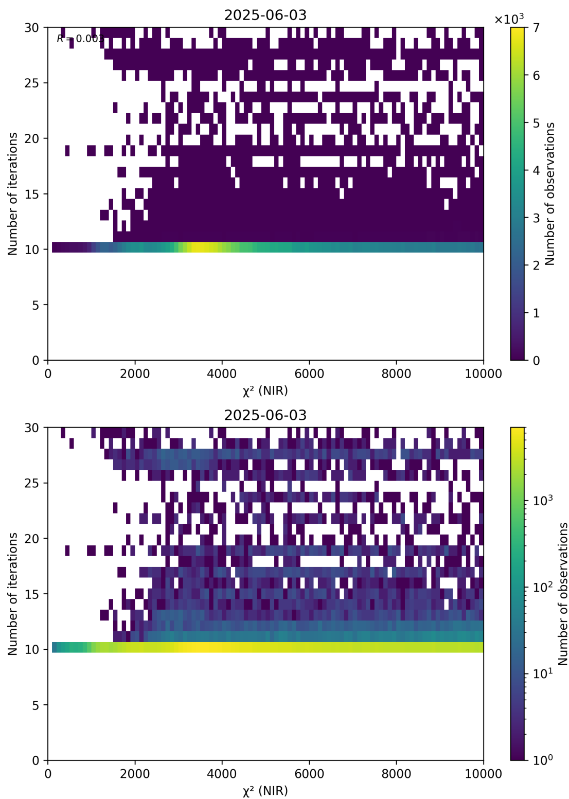
Figure 46: Scatter density plot of “ \chi^2 (NIR)” against “Number of iterations” for 2025-06-02 to 2025-06-04.
