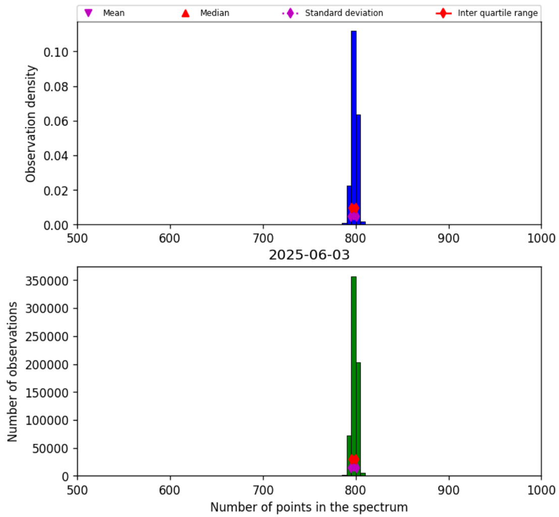
Figure 26: Histogram of “Number of points in the spectrum” for 2025-06-02 to 2025-06-04
