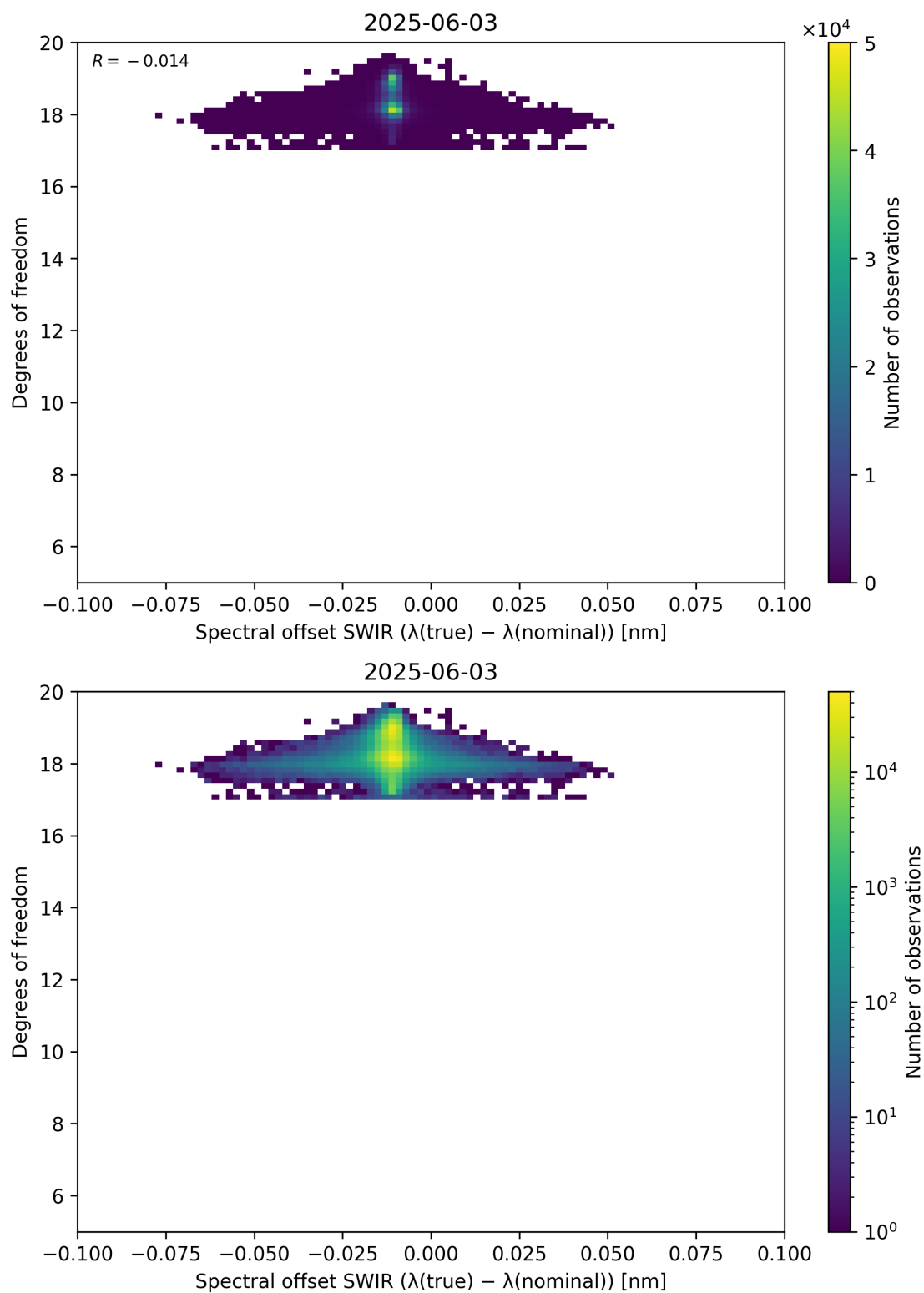
Figure 119: Scatter density plot of “Spectral offset SWIR ( \lambda_{\text{true}} - \lambda_{\text{nominal}} )” against “Degrees of freedom” for 2025-06-02 to 2025-06-04.
