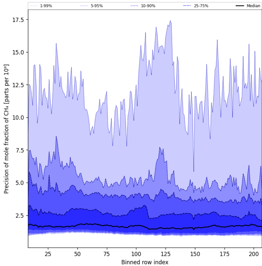
Figure 35: Along track statistics of “Precision of mole fraction of CH 4 ” for 2025-06-02 to 2025-06-04
