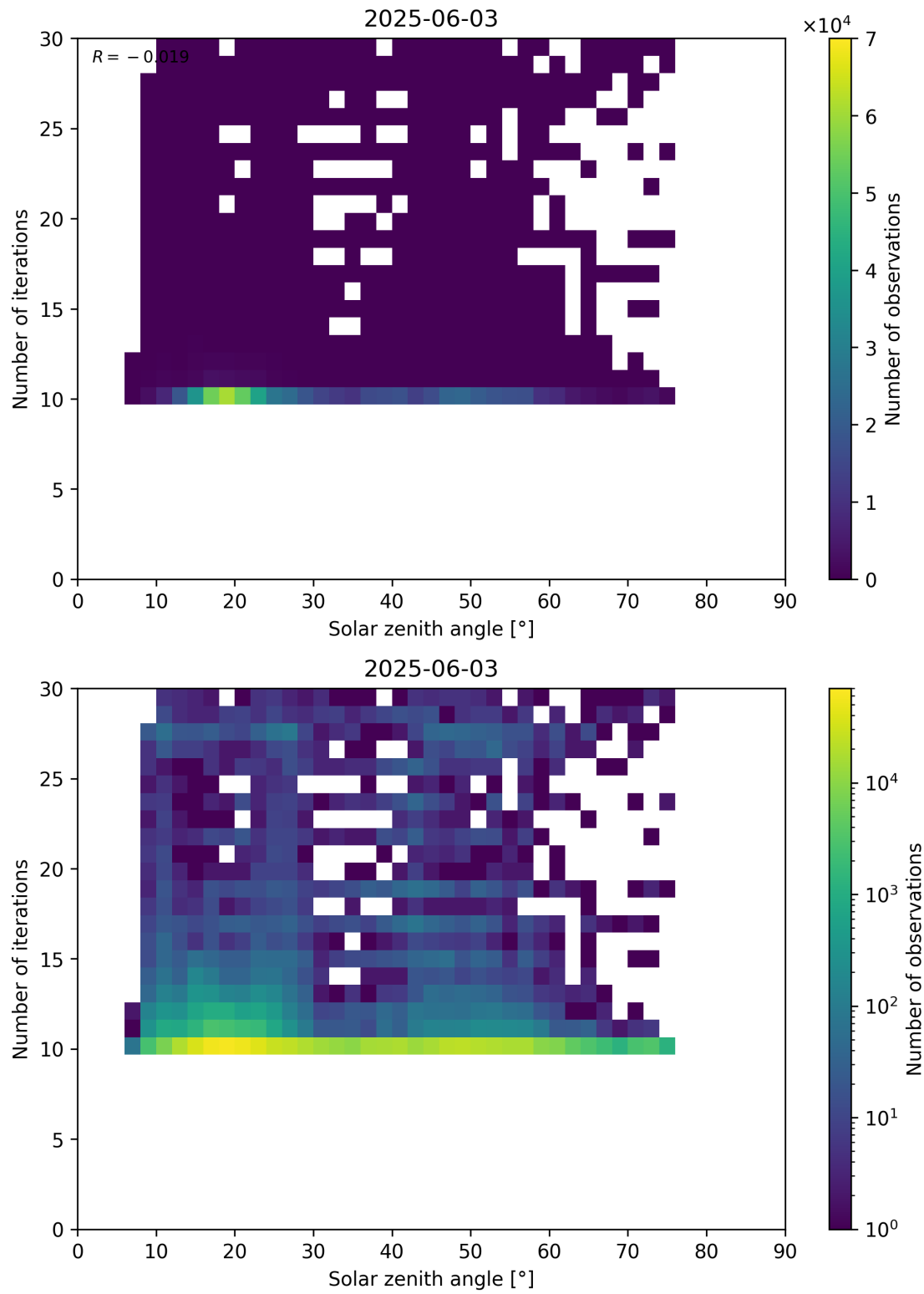
Figure 102: Scatter density plot of “Solar zenith angle” against “Number of iterations” for 2025-06-02 to 2025-06-04.
