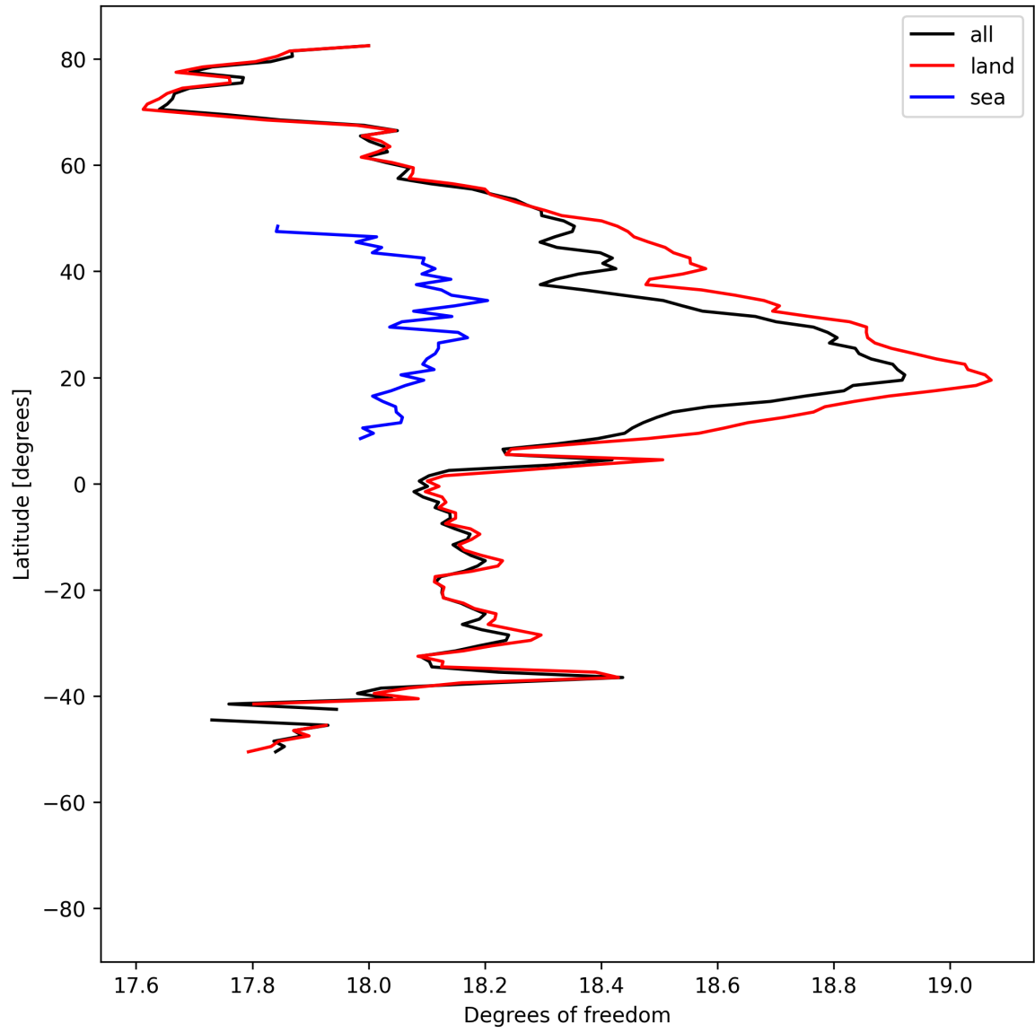
Figure 19: Zonal average of “Degrees of freedom” for 2025-06-02 to 2025-06-04.
