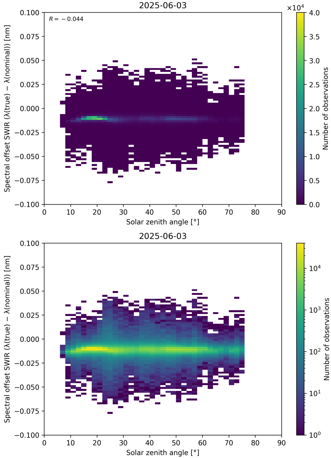
Figure 104: Scatter density plot of “Solar zenith angle” against “Spectral offset SWIR ( \lambda_{\text{true}} - \lambda_{\text{nominal}} )” for 2025-06-02 to 2025-06-04.
