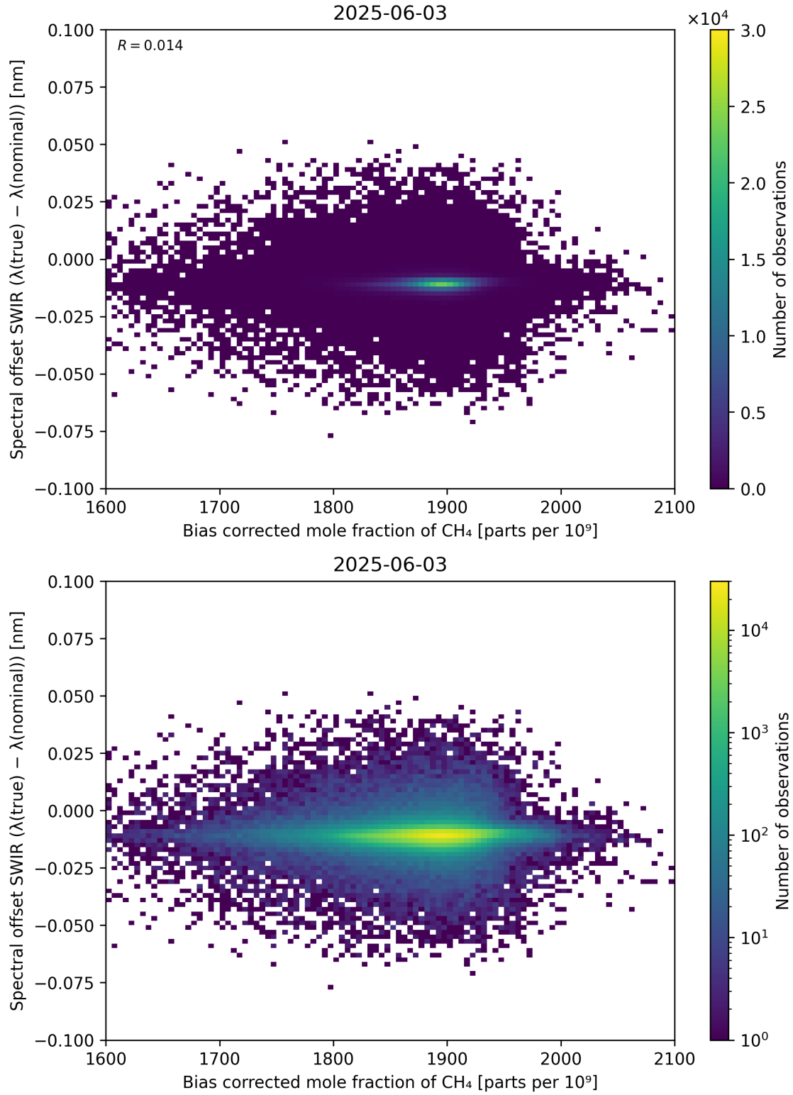
Figure 69: Scatter density plot of “Bias corrected mole fraction of \text{CH}_4 ” against “Spectral offset SWIR ( \lambda_{\text{true}} - \lambda_{\text{nominal}} )” for 2025-06-02 to 2025-06-04.
