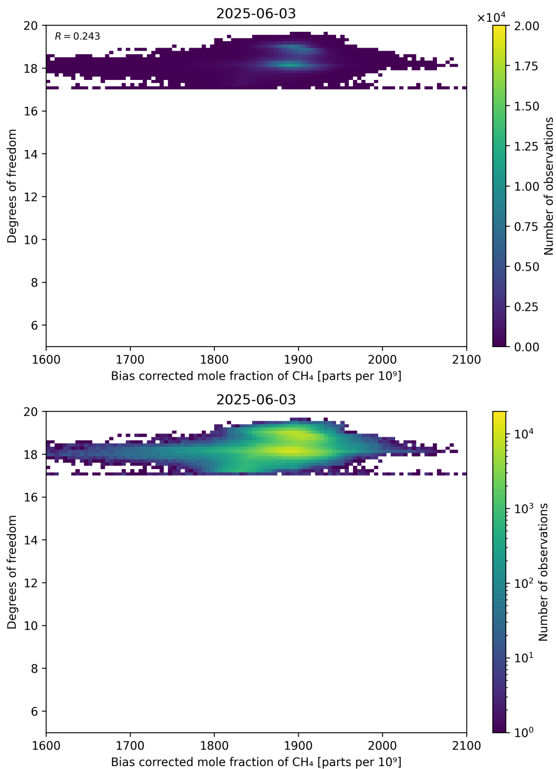
Figure 65: Scatter density plot of “Bias corrected mole fraction of CH 4 ” against “Degrees of freedom” for 2025-06-02 to 2025-06-04.
