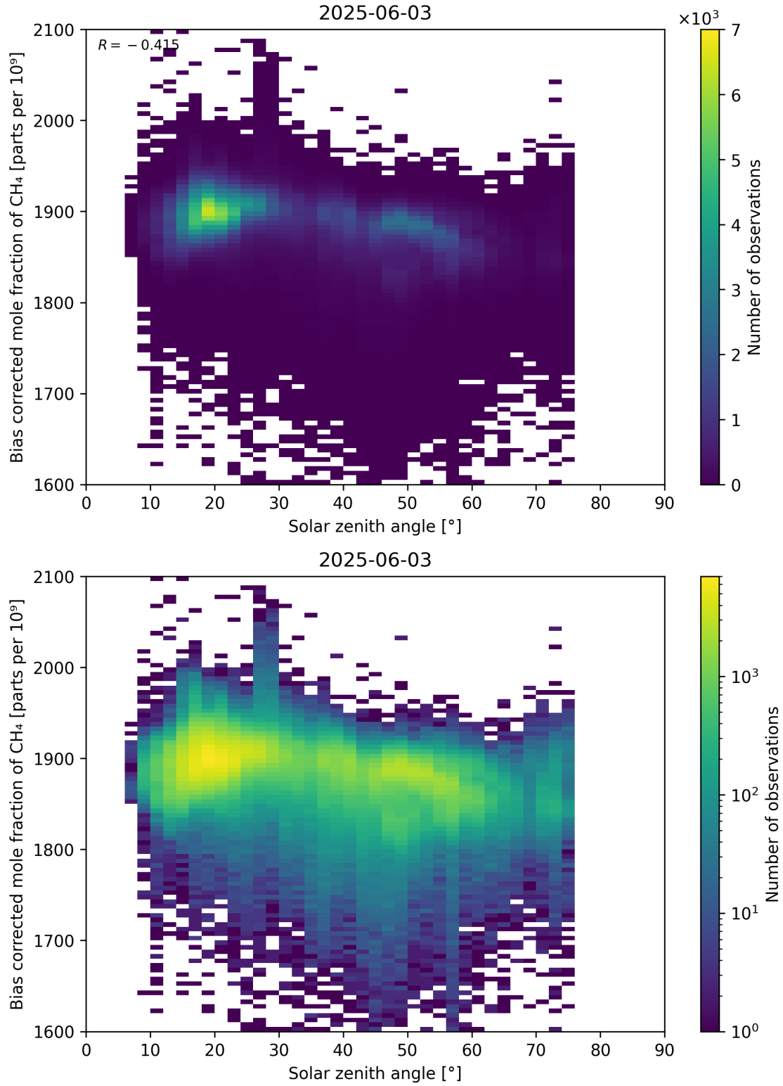
Figure 100: Scatter density plot of “Solar zenith angle” against “Bias corrected mole fraction of CH 4 ” for 2025-06-02 to 2025-06-04.
