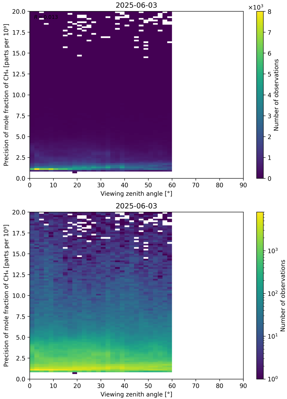
Figure 112: Scatter density plot of “Viewing zenith angle” against “Precision of mole fraction of CH 4 ” for 2025-06-02 to 2025-06-04.
