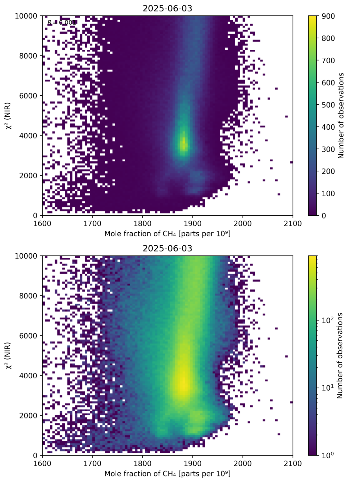
Figure 70: Scatter density plot of “Mole fraction of \text{CH}_4 ” against “ \chi^2 (NIR)” for 2025-06-02 to 2025-06-04.
