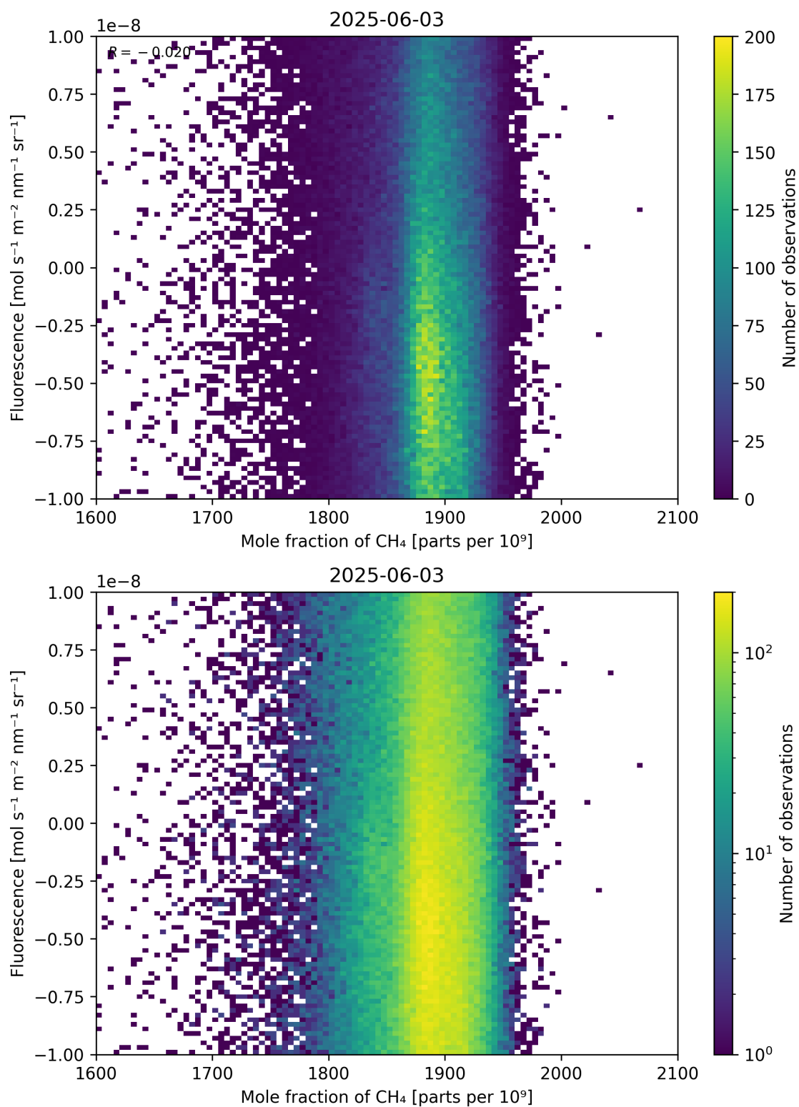
Figure 73: Scatter density plot of “Mole fraction of \text{CH}_4 ” against “Fluorescence” for 2025-06-02 to 2025-06-04.
