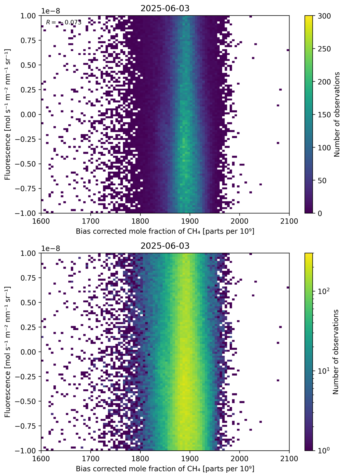
Figure 66: Scatter density plot of “Bias corrected mole fraction of \text{CH}_4 ” against “Fluorescence” for 2025-06-02 to 2025-06-04.
