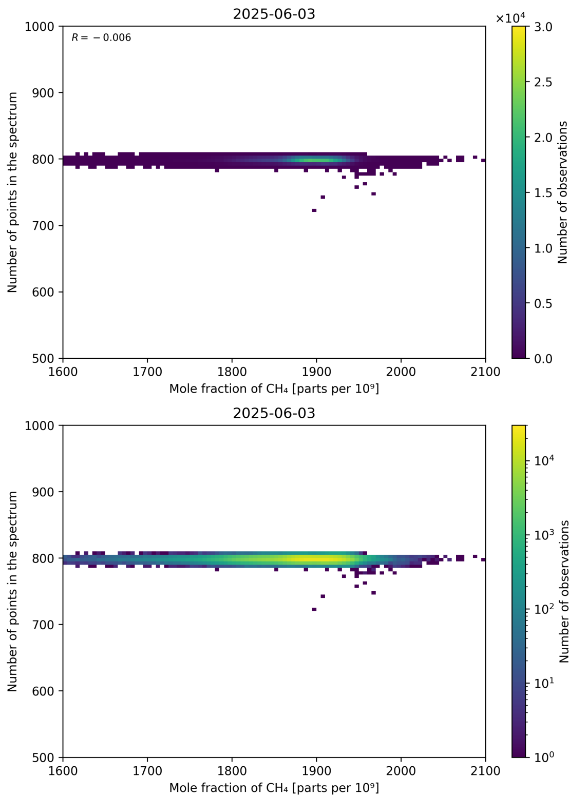
Figure 77: Scatter density plot of “Mole fraction of CH 4 ” against “Number of points in the spectrum” for 2025-06-02 to 2025-06-04.
