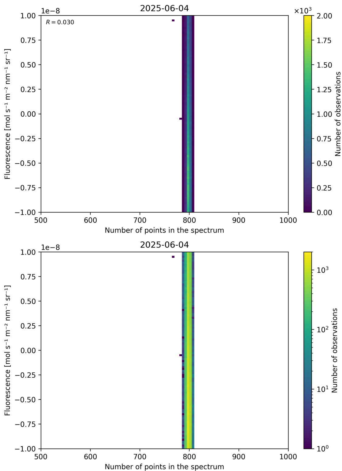
Figure 91: Scatter density plot of “Number of points in the spectrum” against “Fluorescence” for 2025-06-03 to 2025-06-05.
