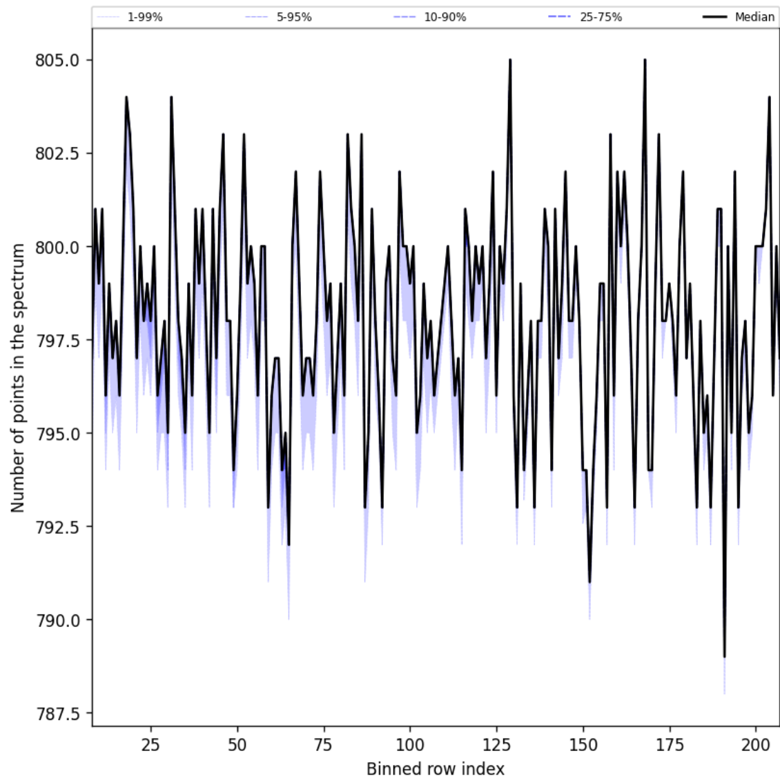
Figure 37: Along track statistics of “Number of points in the spectrum” for 2025-06-03 to 2025-06-05
