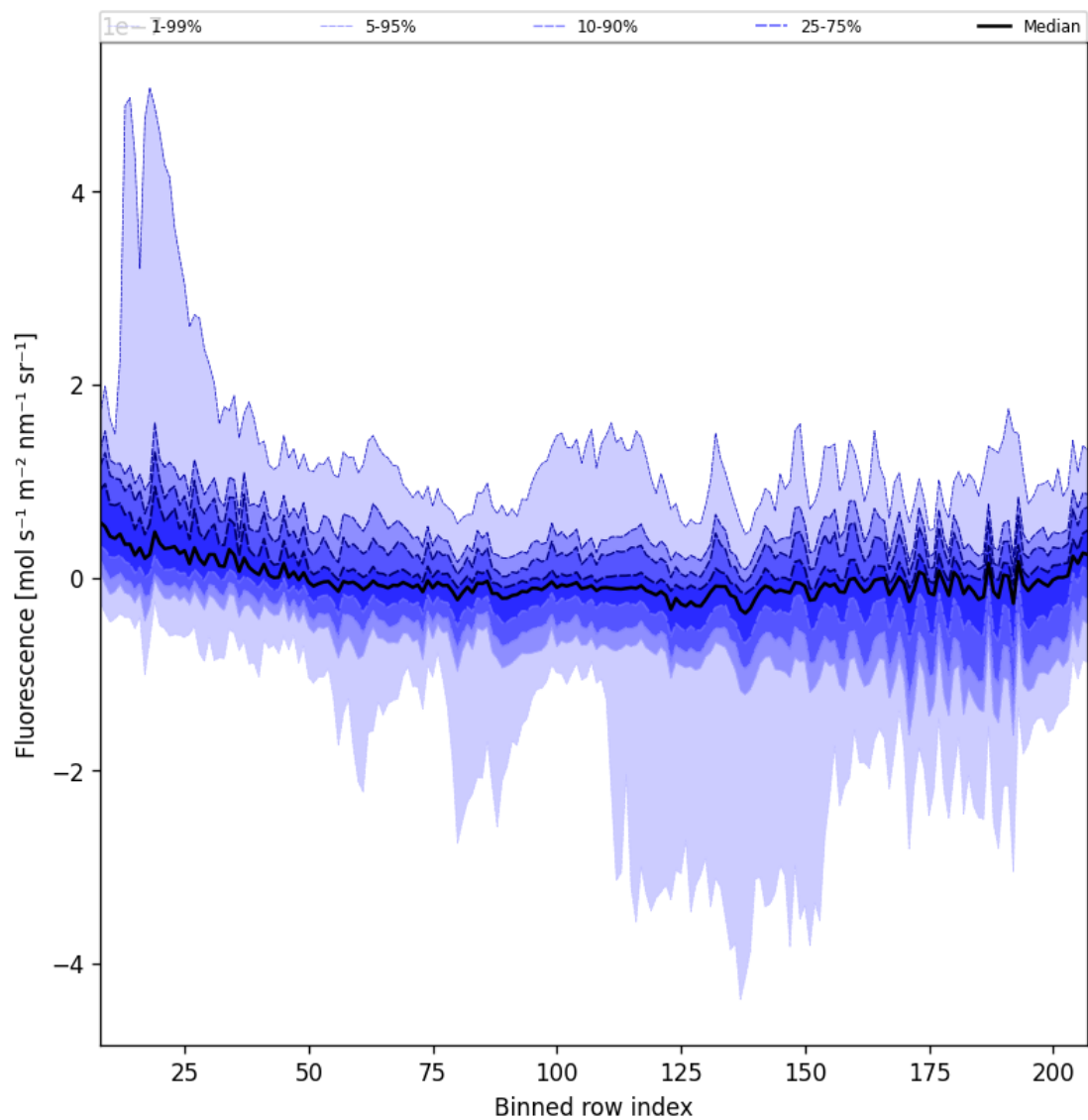
Figure 43: Along track statistics of “Fluorescence” for 2025-06-03 to 2025-06-05
