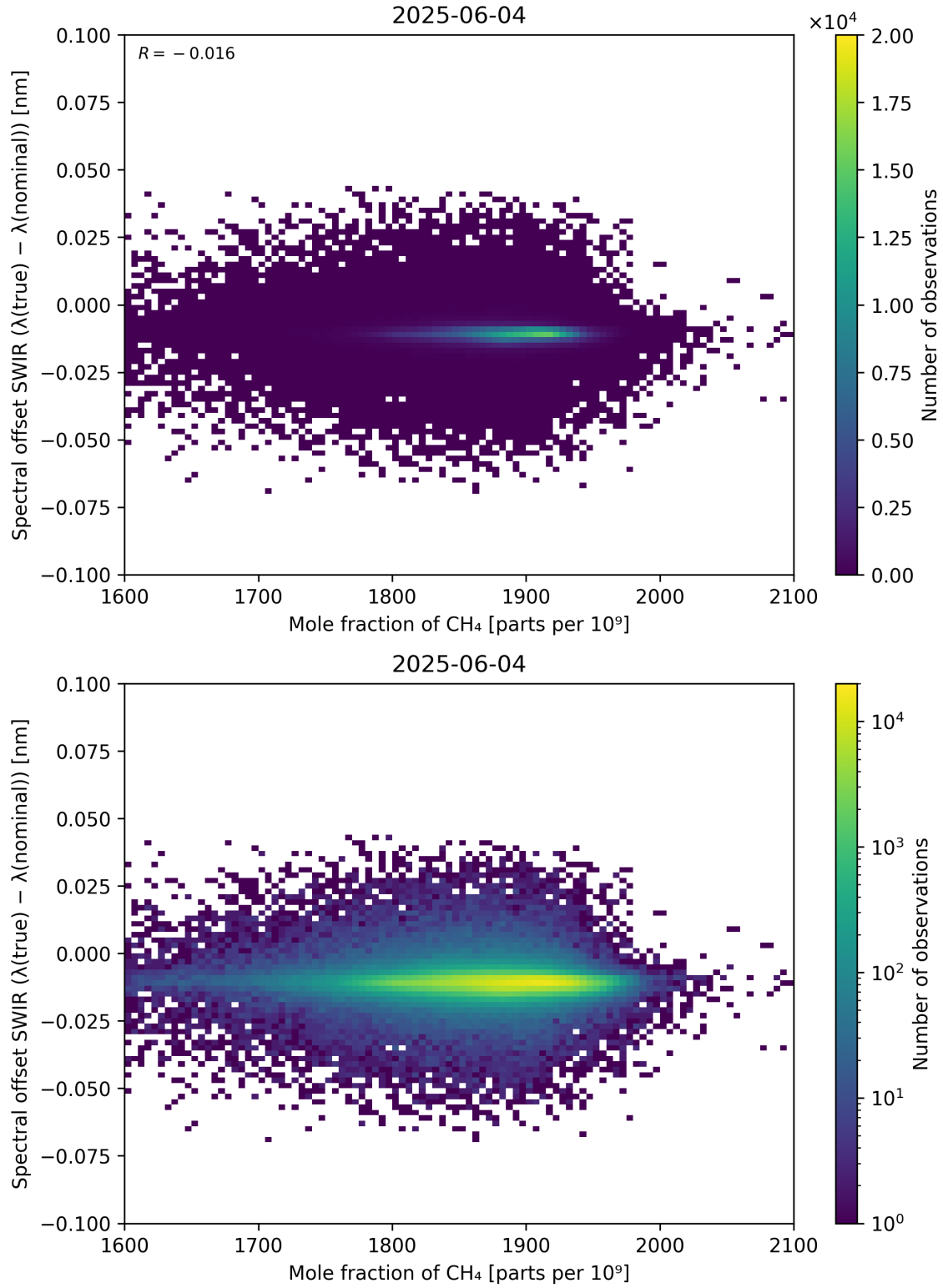
Figure 86: Scatter density plot of “Mole fraction of CH 4 ” against “Spectral offset SWIR ( \lambda_{\text{true}} - \lambda_{\text{nominal}} )” for 2025-06-03 to 2025-06-05.
