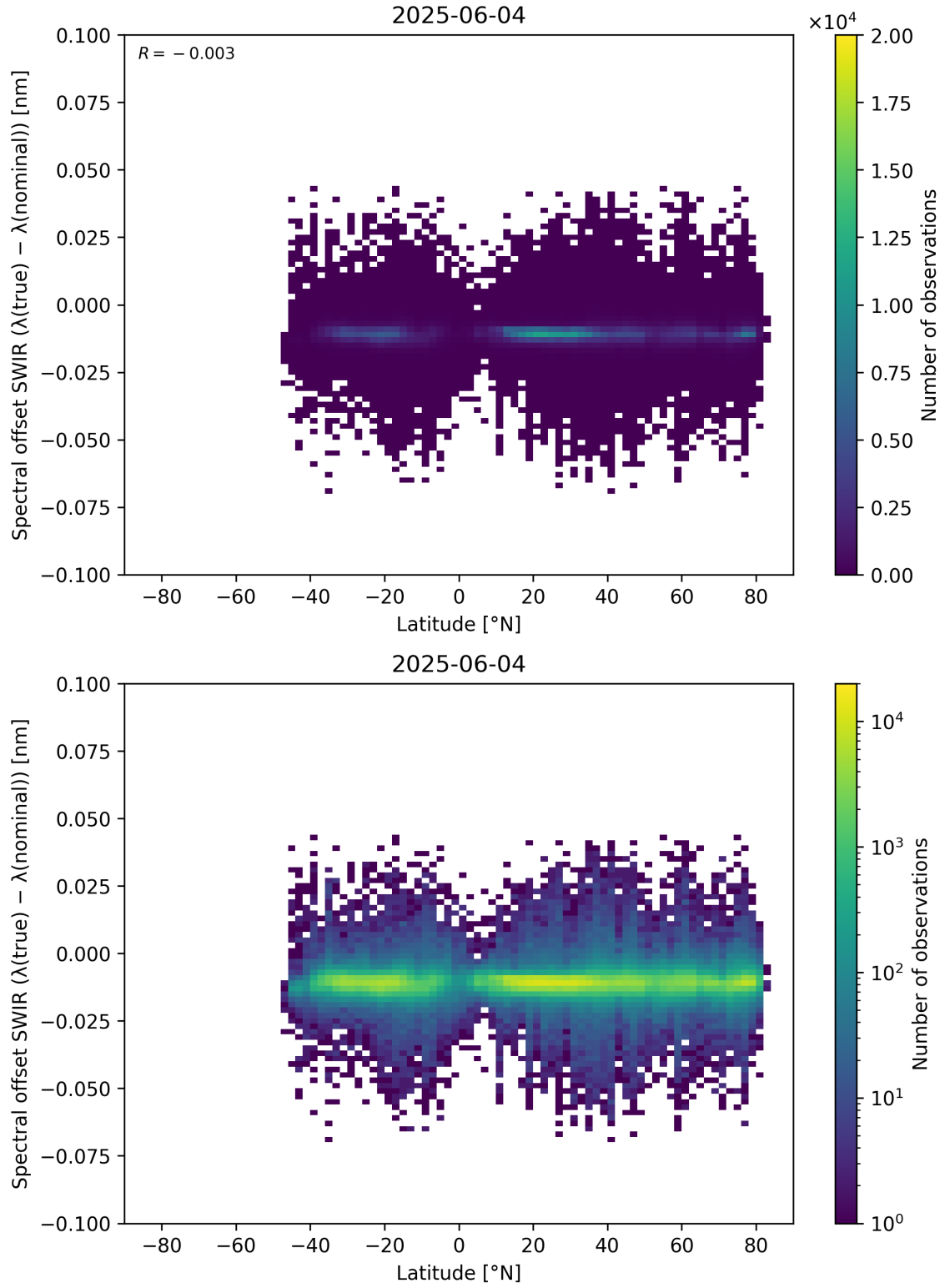
Figure 62: Scatter density plot of “Latitude” against “Spectral offset SWIR ( \lambda_{\text{true}} - \lambda_{\text{nominal}} )” for 2025-06-03 to 2025-06-05.
