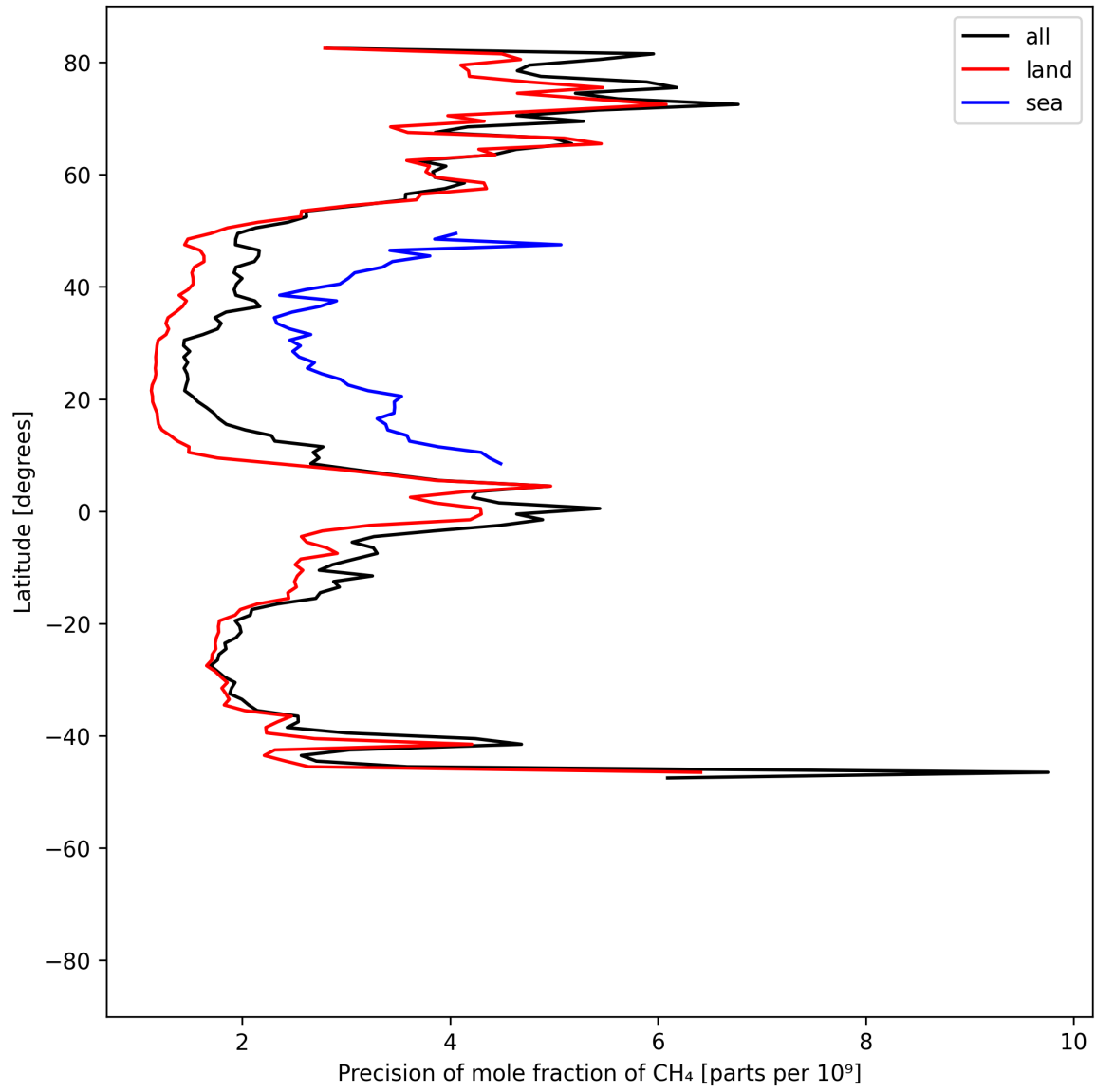
Figure 13: Zonal average of “Precision of mole fraction of CH 4 ” for 2025-06-03 to 2025-06-05.
