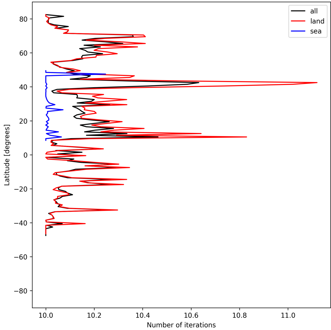
Figure 20: Zonal average of “Number of iterations” for 2025-06-03 to 2025-06-05.
