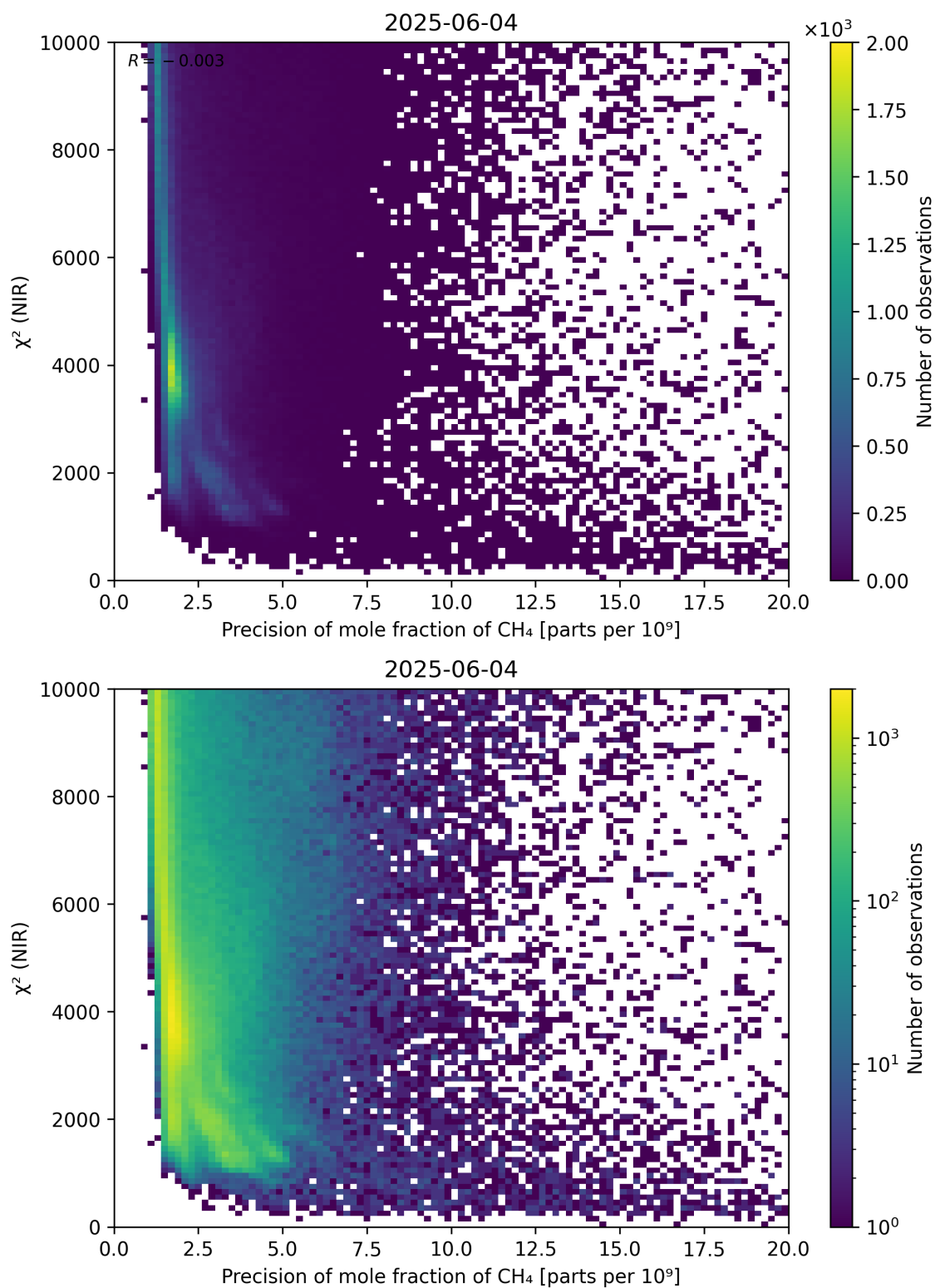
Figure 78: Scatter density plot of “Precision of mole fraction of CH 4 ” against “ \chi^2 (NIR)” for 2025-06-03 to 2025-06-05.
