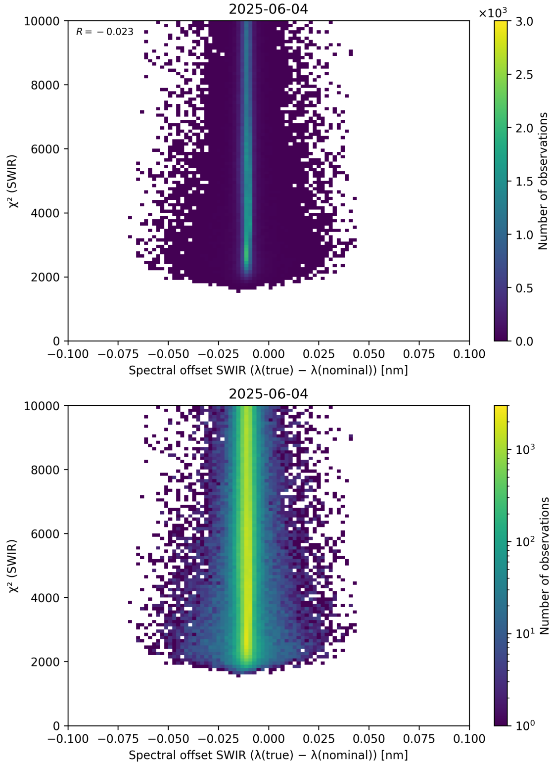
Figure 118: Scatter density plot of “Spectral offset SWIR ( \lambda_{\text{true}} - \lambda_{\text{nominal}} )” against “ \chi^2 (SWIR)” for 2025-06-03 to 2025-06-05.
