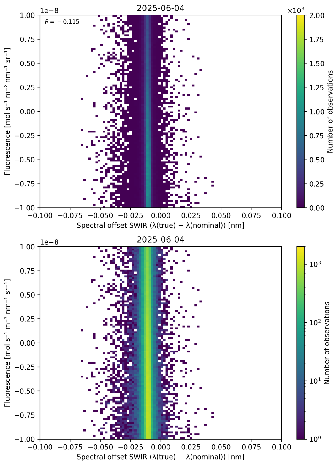
Figure 120: Scatter density plot of “Spectral offset SWIR ( \lambda_{\text{true}} - \lambda_{\text{nominal}} )” against “Fluorescence” for 2025-06-03 to 2025-06-05.
