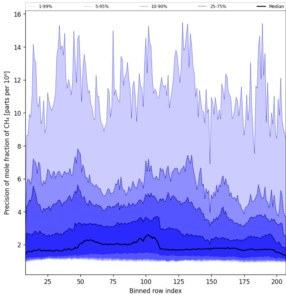
Figure 35: Along track statistics of “Precision of mole fraction of CH 4 ” for 2025-06-03 to 2025-06-05
