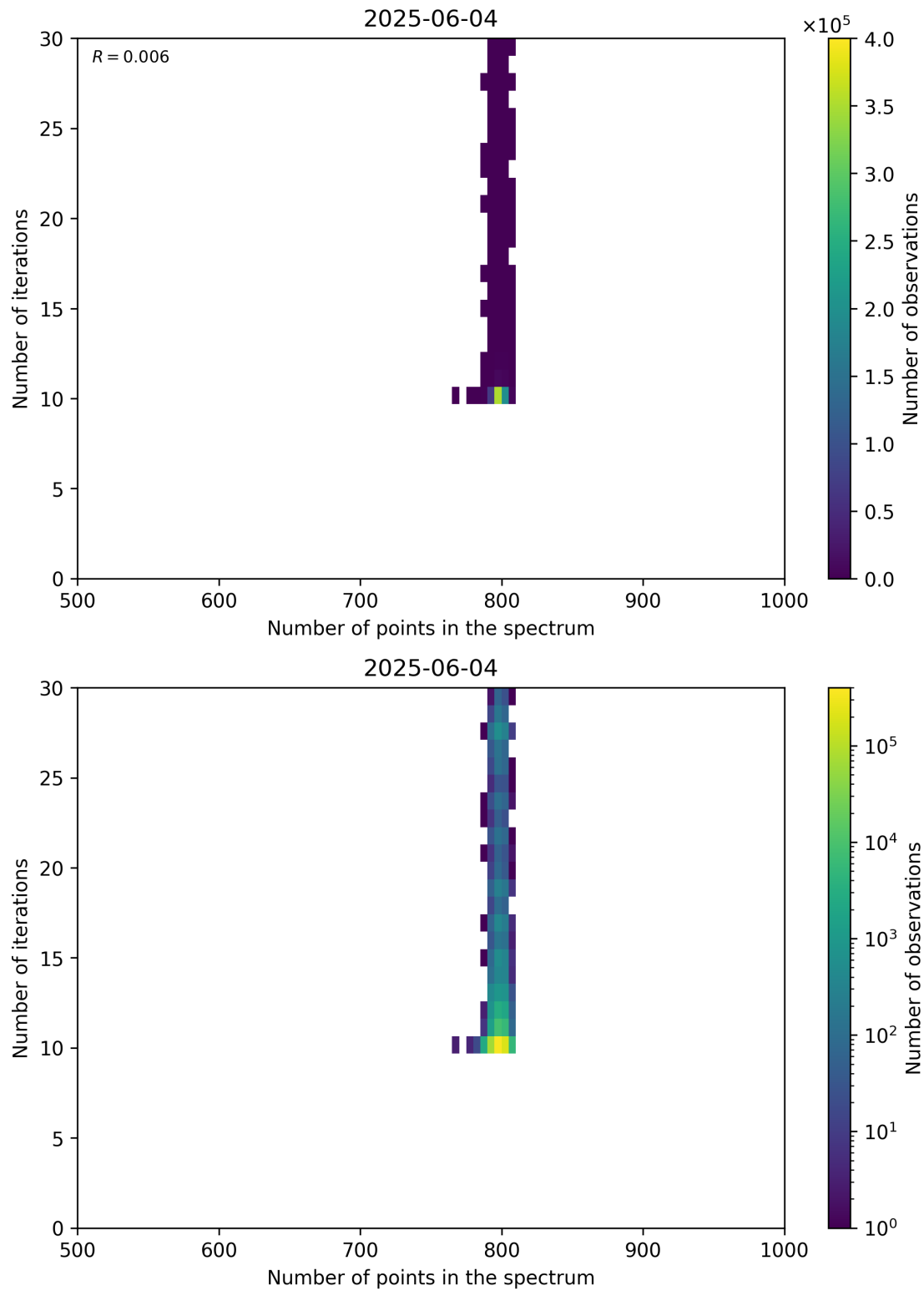
Figure 92: Scatter density plot of “Number of points in the spectrum” against “Number of iterations” for 2025-06-03 to 2025-06-05.
