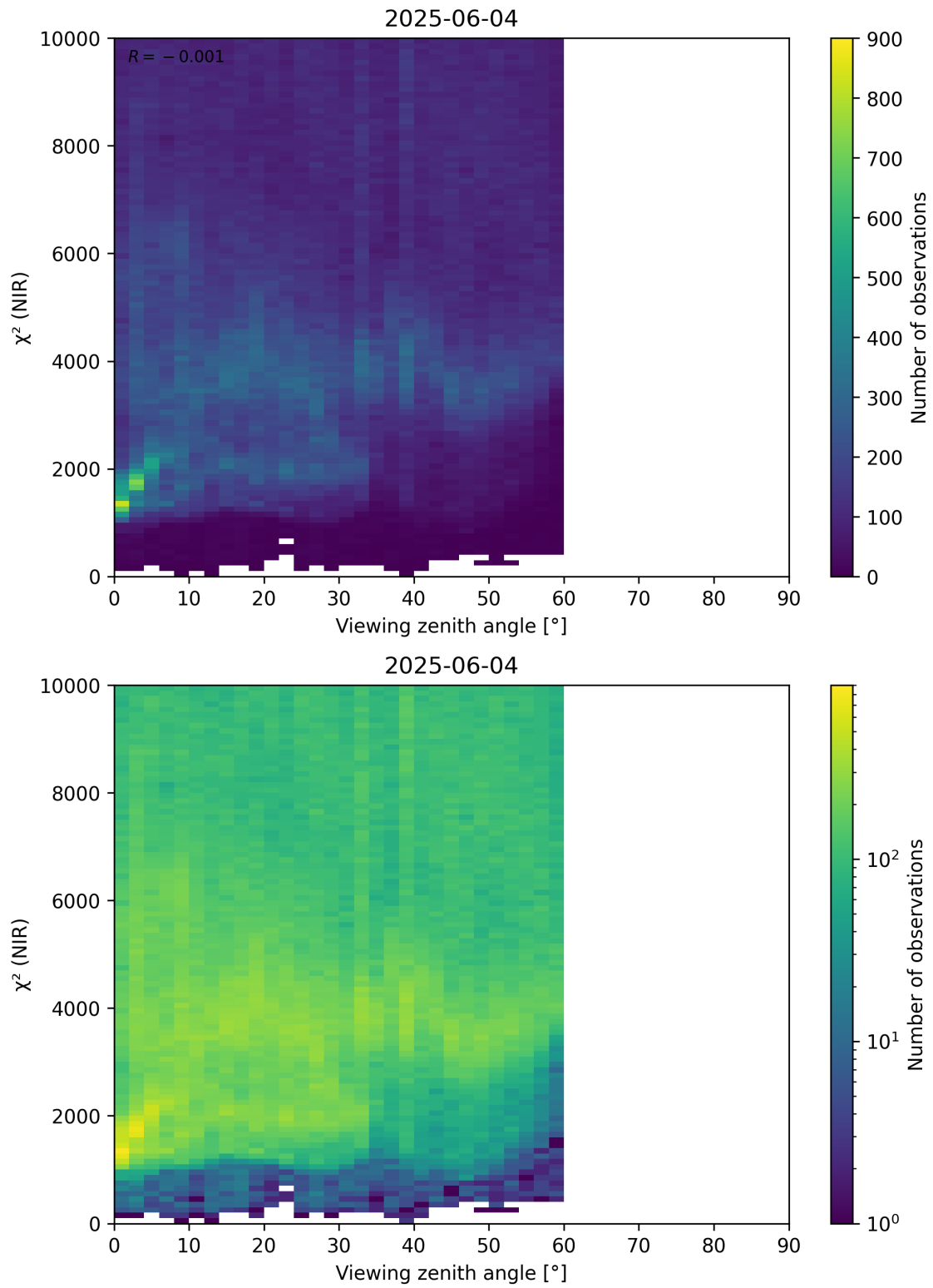
Figure 105: Scatter density plot of “Viewing zenith angle” against “ \chi^2 (NIR)” for 2025-06-03 to 2025-06-05.
