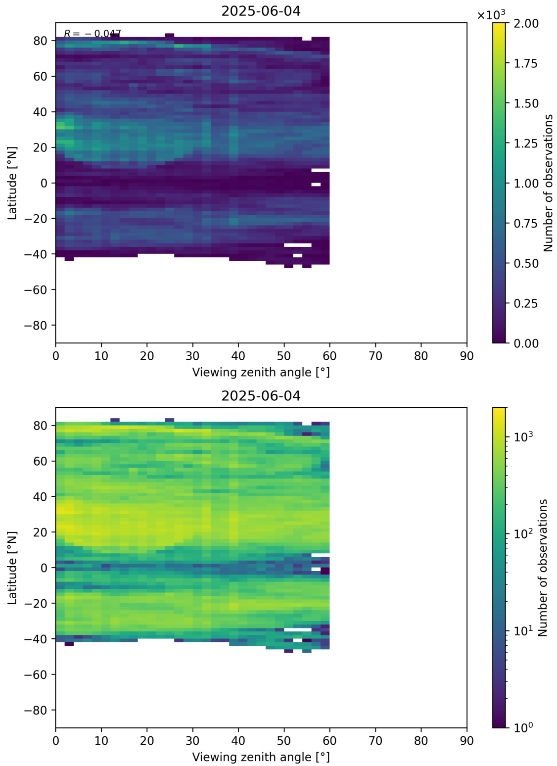
Figure 109: Scatter density plot of “Viewing zenith angle” against “Latitude” for 2025-06-03 to 2025-06-05.
