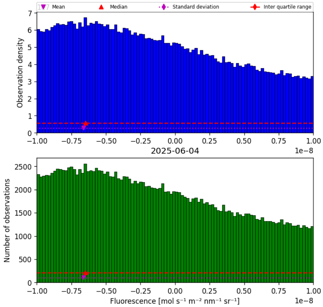
Figure 32: Histogram of “Fluorescence” for 2025-06-03 to 2025-06-05
