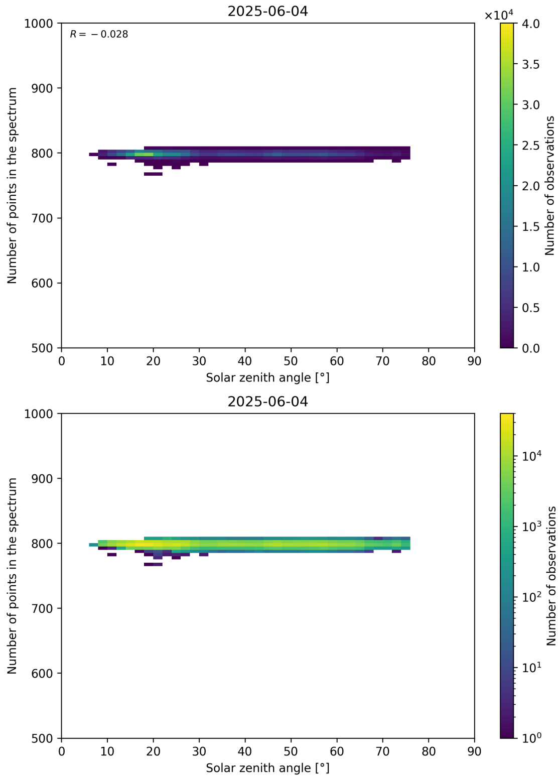
Figure 103: Scatter density plot of “Solar zenith angle” against “Number of points in the spectrum” for 2025-06-03 to 2025-06-05.
