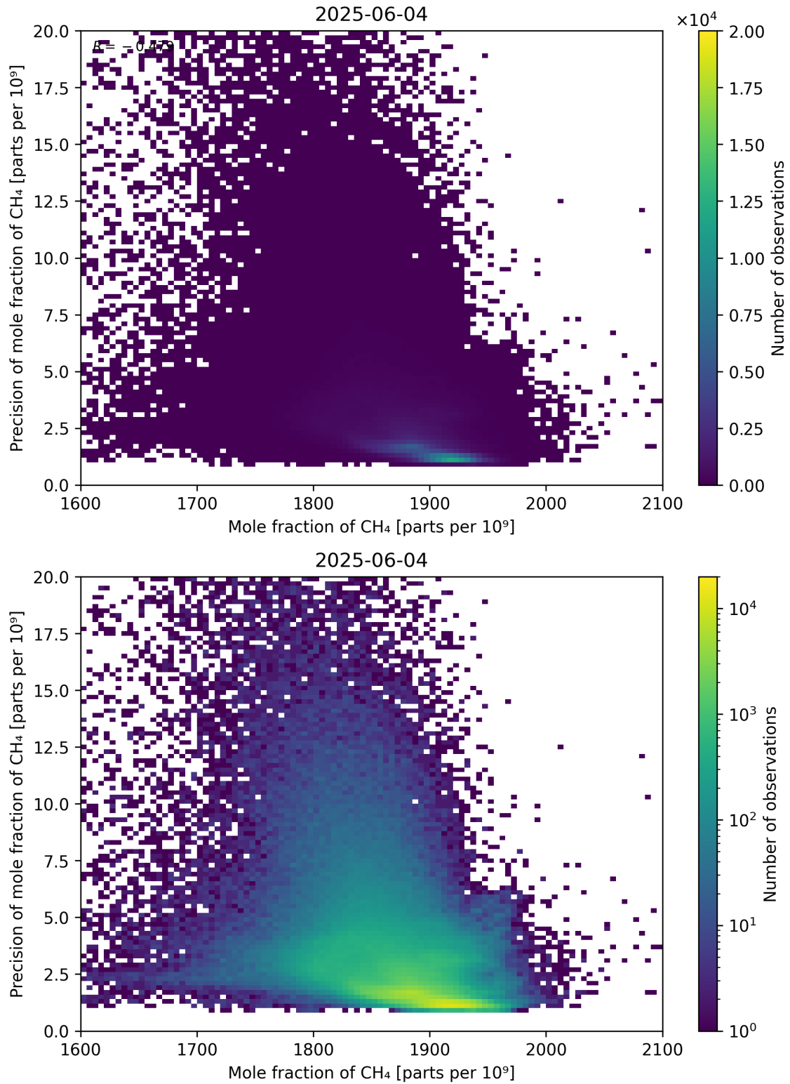
Figure 75: Scatter density plot of “Mole fraction of CH 4 ” against “Precision of mole fraction of CH 4 ” for 2025-06-03 to 2025-06-05.
