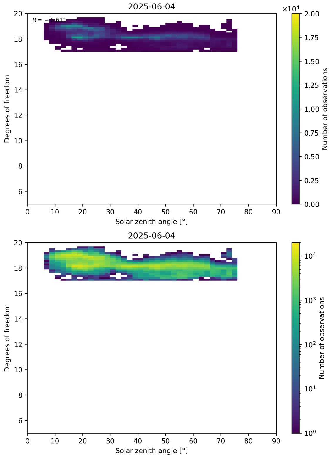
Figure 96: Scatter density plot of “Solar zenith angle” against “Degrees of freedom” for 2025-06-03 to 2025-06-05.
