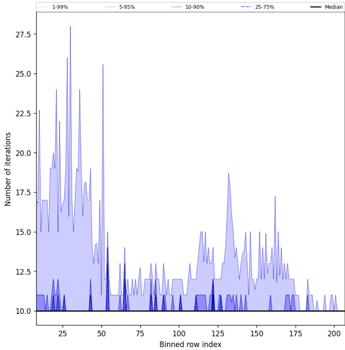
Figure 42: Along track statistics of “Number of iterations” for 2025-06-03 to 2025-06-05
