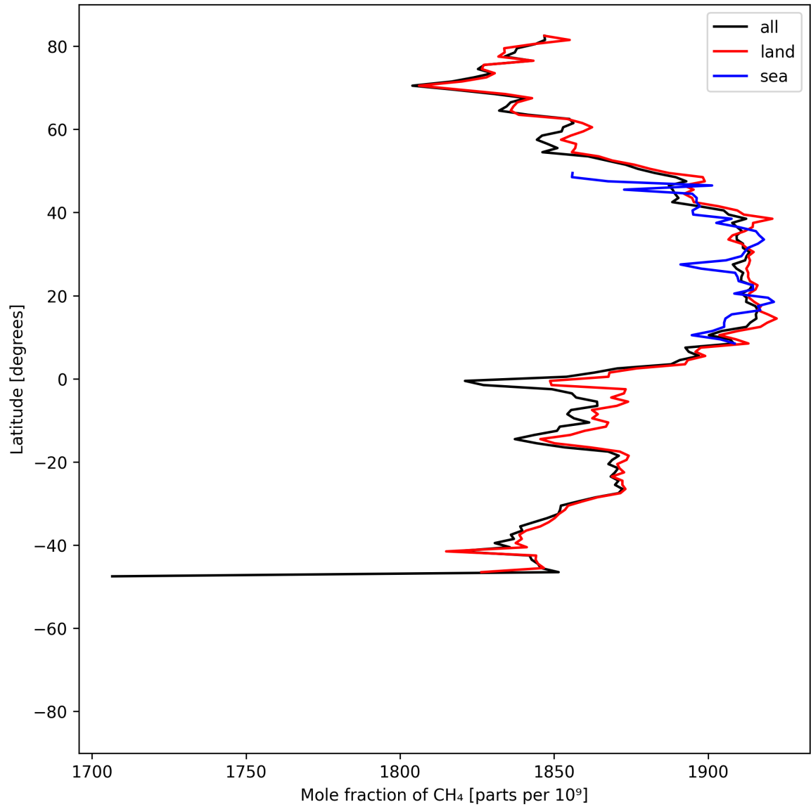
Figure 12: Zonal average of “Mole fraction of CH 4 ” for 2025-06-03 to 2025-06-05.
