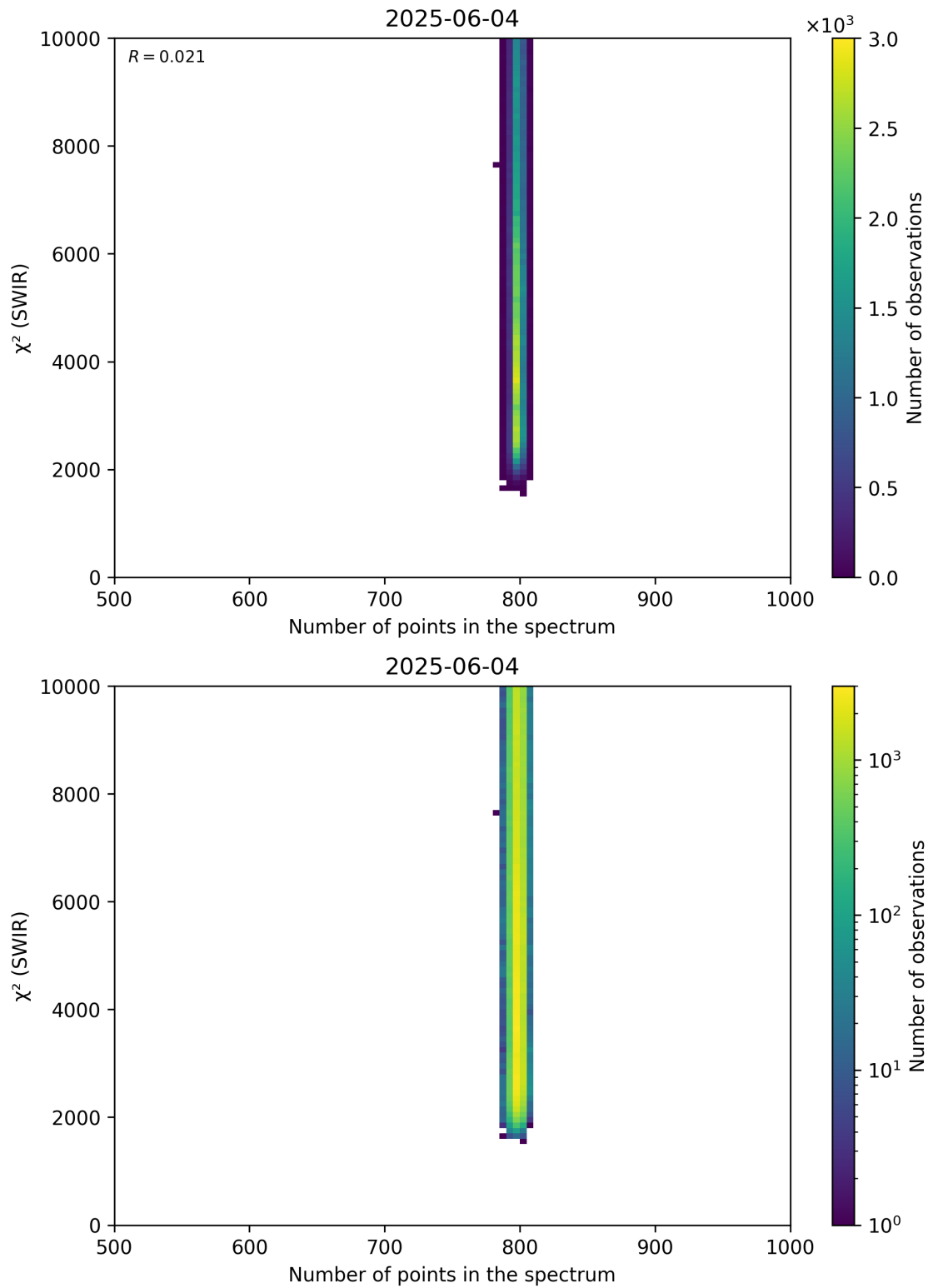
Figure 89: Scatter density plot of “Number of points in the spectrum” against “ \chi^2 (SWIR)” for 2025-06-03 to 2025-06-05.
