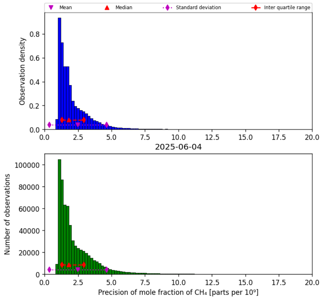
Figure 24: Histogram of “Precision of mole fraction of CH 4 ” for 2025-06-03 to 2025-06-05
