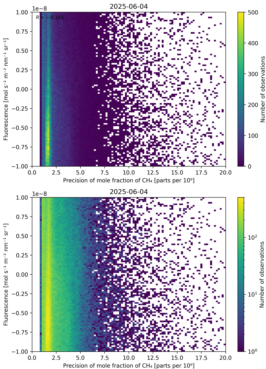
Figure 81: Scatter density plot of “Precision of mole fraction of \text{CH}_4 ” against “Fluorescence” for 2025-06-03 to 2025-06-05.
