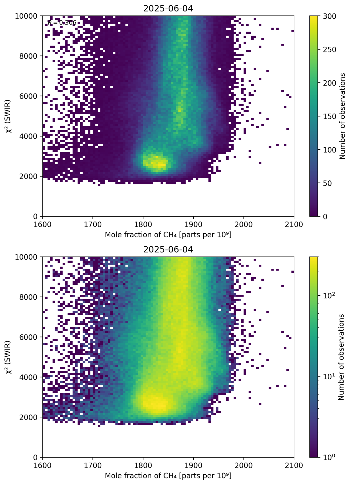
Figure 71: Scatter density plot of “Mole fraction of CH 4 ” against “ \chi^2 (SWIR)” for 2025-06-03 to 2025-06-05.
