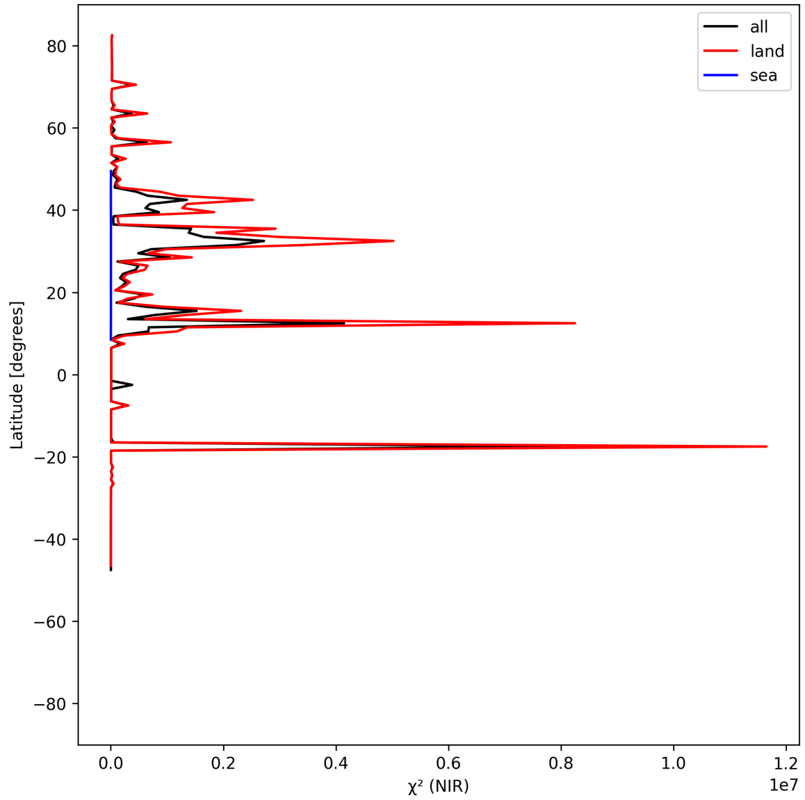
Figure 18: Zonal average of “ \chi^2 (NIR)” for 2025-06-03 to 2025-06-05.
