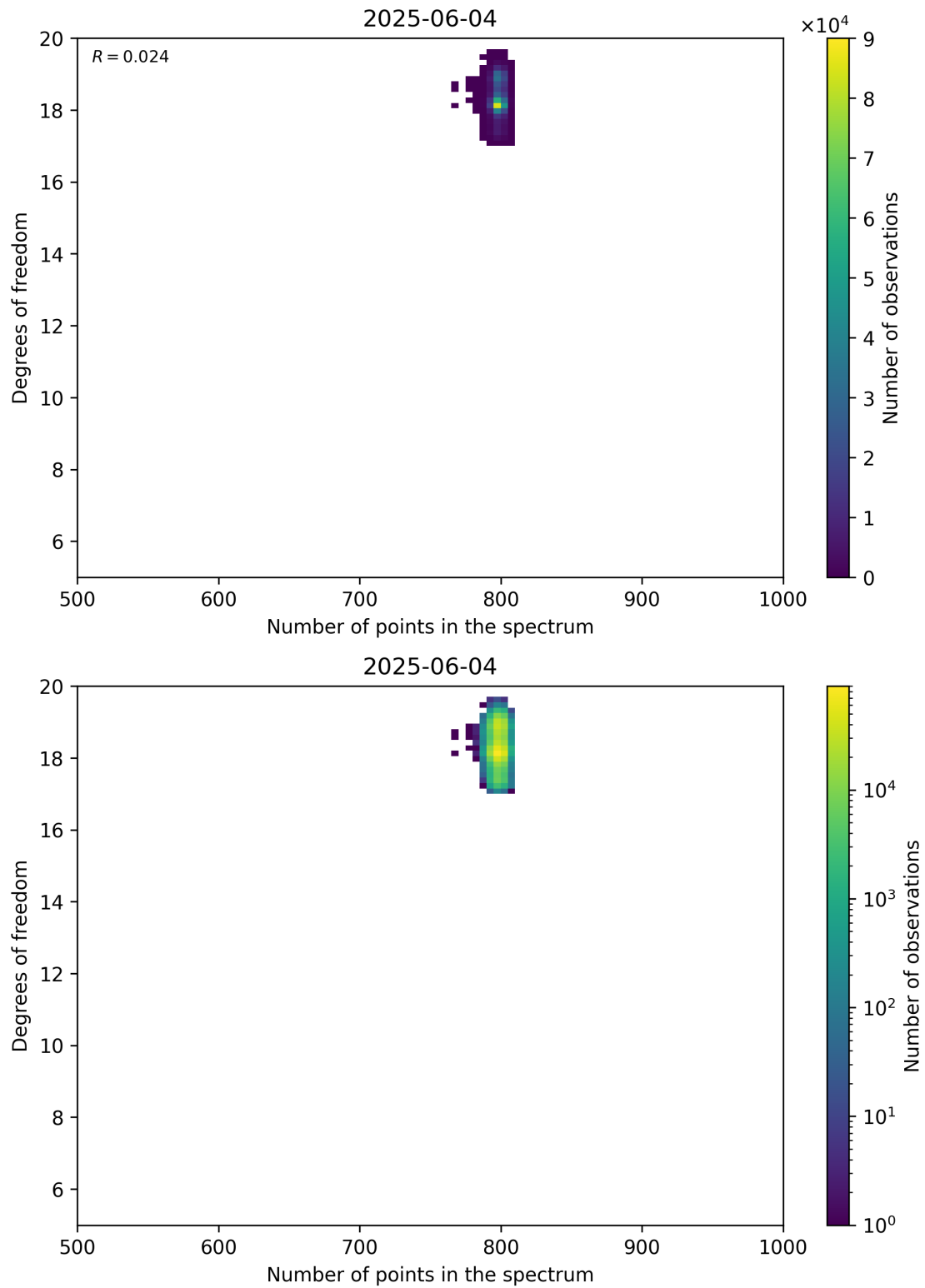
Figure 90: Scatter density plot of “Number of points in the spectrum” against “Degrees of freedom” for 2025-06-03 to 2025-06-05.
