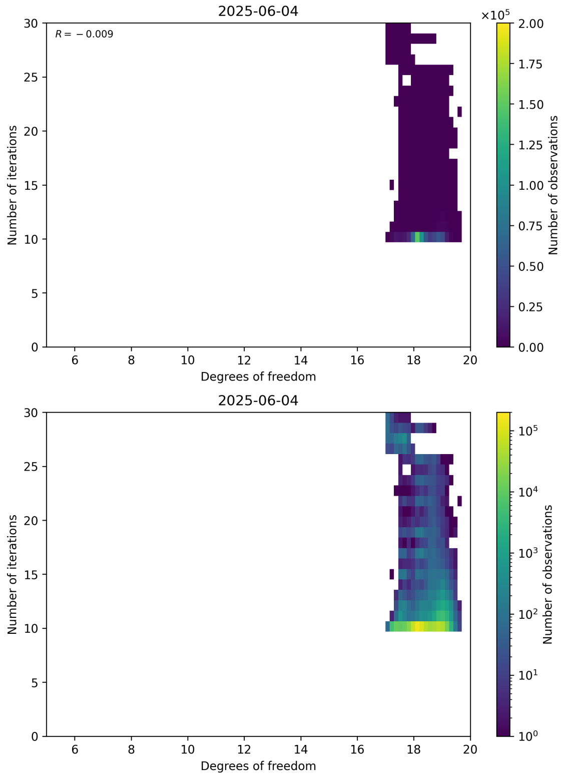
Figure 52: Scatter density plot of “Degrees of freedom” against “Number of iterations” for 2025-06-03 to 2025-06-05.
