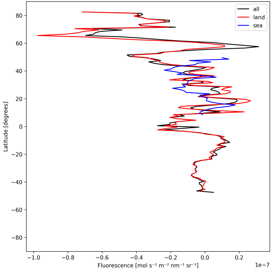
Figure 21: Zonal average of “Fluorescence” for 2025-06-03 to 2025-06-05.
