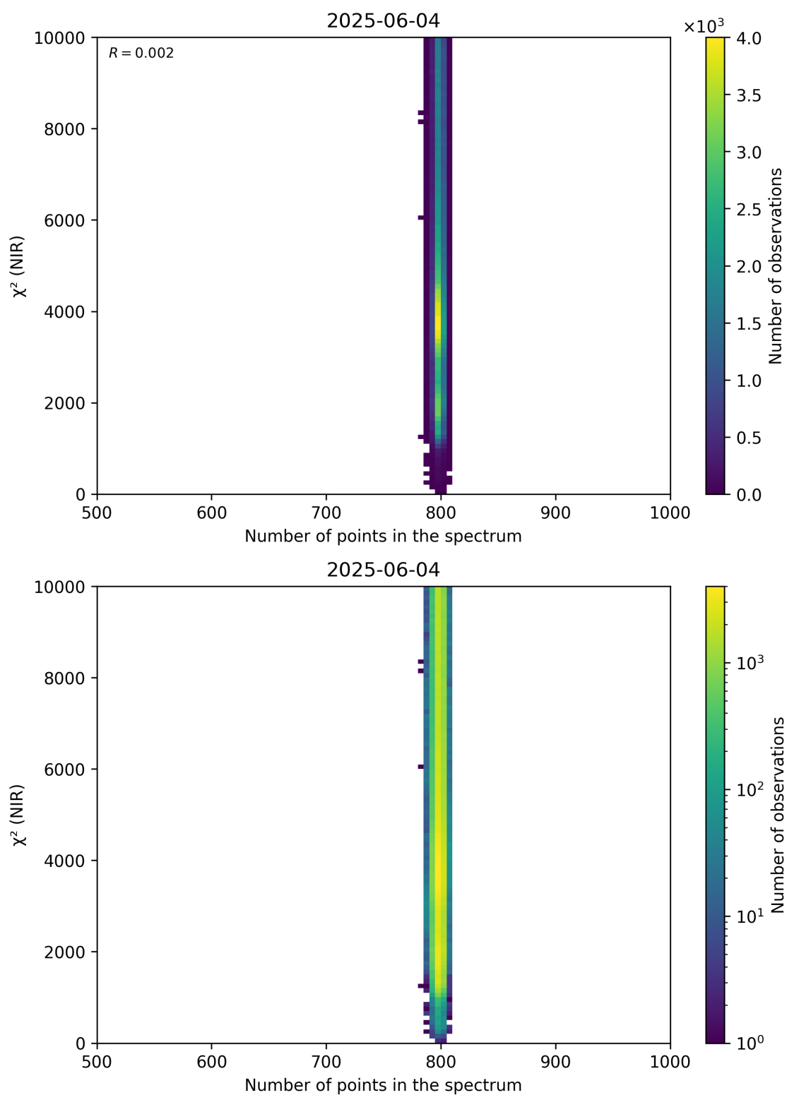
Figure 88: Scatter density plot of “Number of points in the spectrum” against “ \chi^2 (NIR)” for 2025-06-03 to 2025-06-05.
