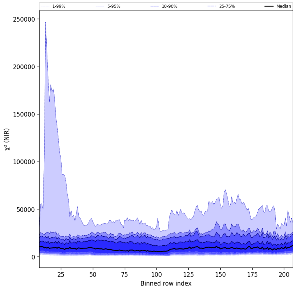
Figure 40: Along track statistics of “ \chi^2 (NIR)” for 2025-06-03 to 2025-06-05
