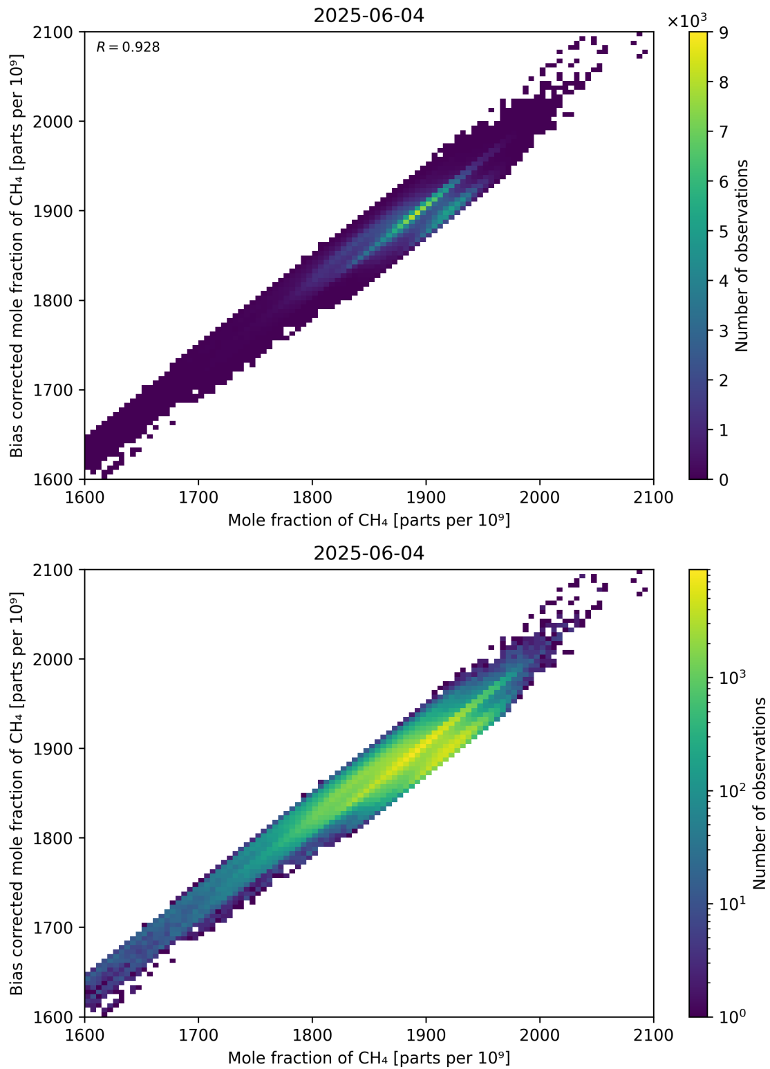
Figure 74: Scatter density plot of “Mole fraction of CH 4 ” against “Bias corrected mole fraction of CH 4 ” for 2025-06-03 to 2025-06-05.
