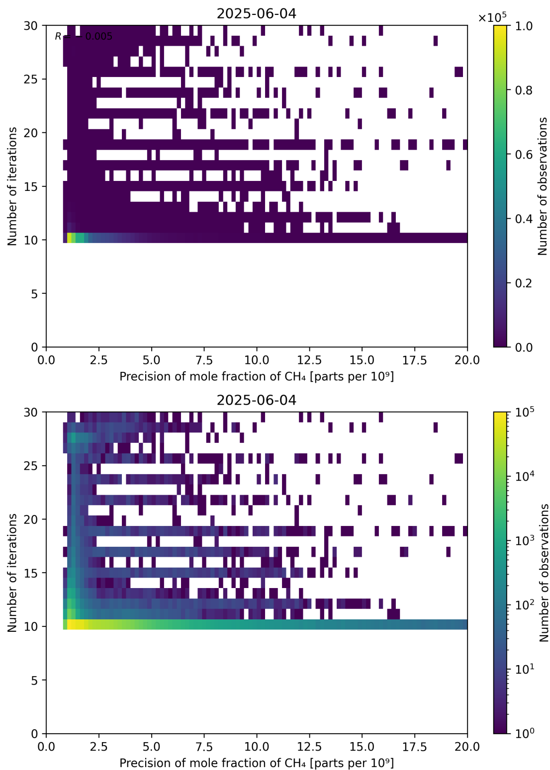
Figure 83: Scatter density plot of “Precision of mole fraction of CH 4 ” against “Number of iterations” for 2025-06-03 to 2025-06-05.
