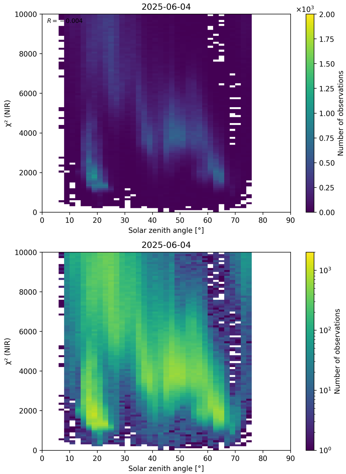
Figure 94: Scatter density plot of “Solar zenith angle” against “ \chi^2 (NIR)” for 2025-06-03 to 2025-06-05.
