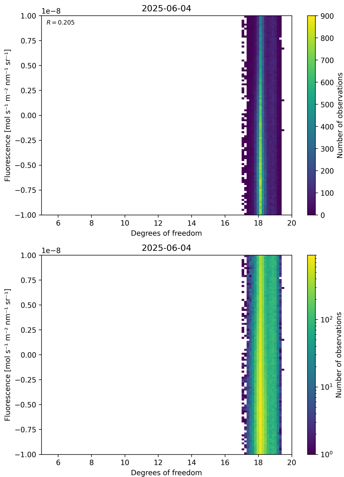
Figure 51: Scatter density plot of “Degrees of freedom” against “Fluorescence” for 2025-06-03 to 2025-06-05.
