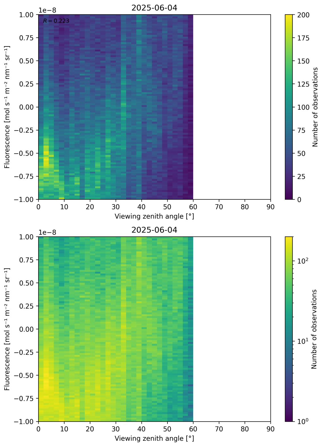
Figure 108: Scatter density plot of “Viewing zenith angle” against “Fluorescence” for 2025-06-03 to 2025-06-05.
