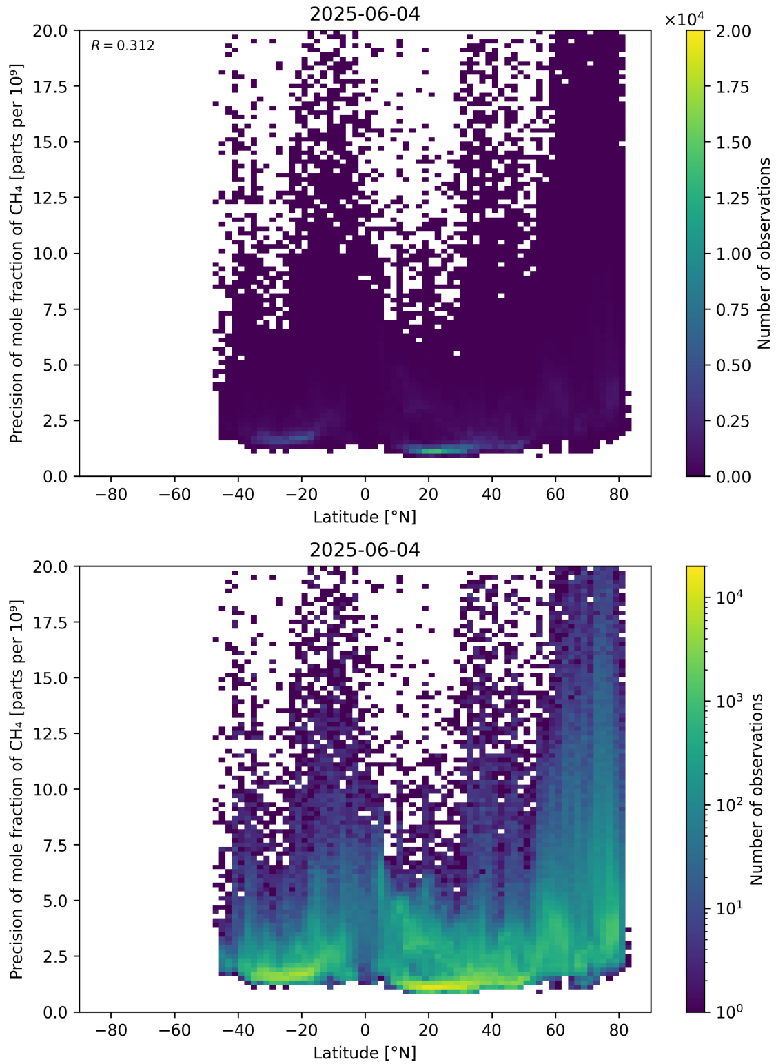
Figure 59: Scatter density plot of “Latitude” against “Precision of mole fraction of \text{CH}_4 ” for 2025-06-03 to 2025-06-05.
