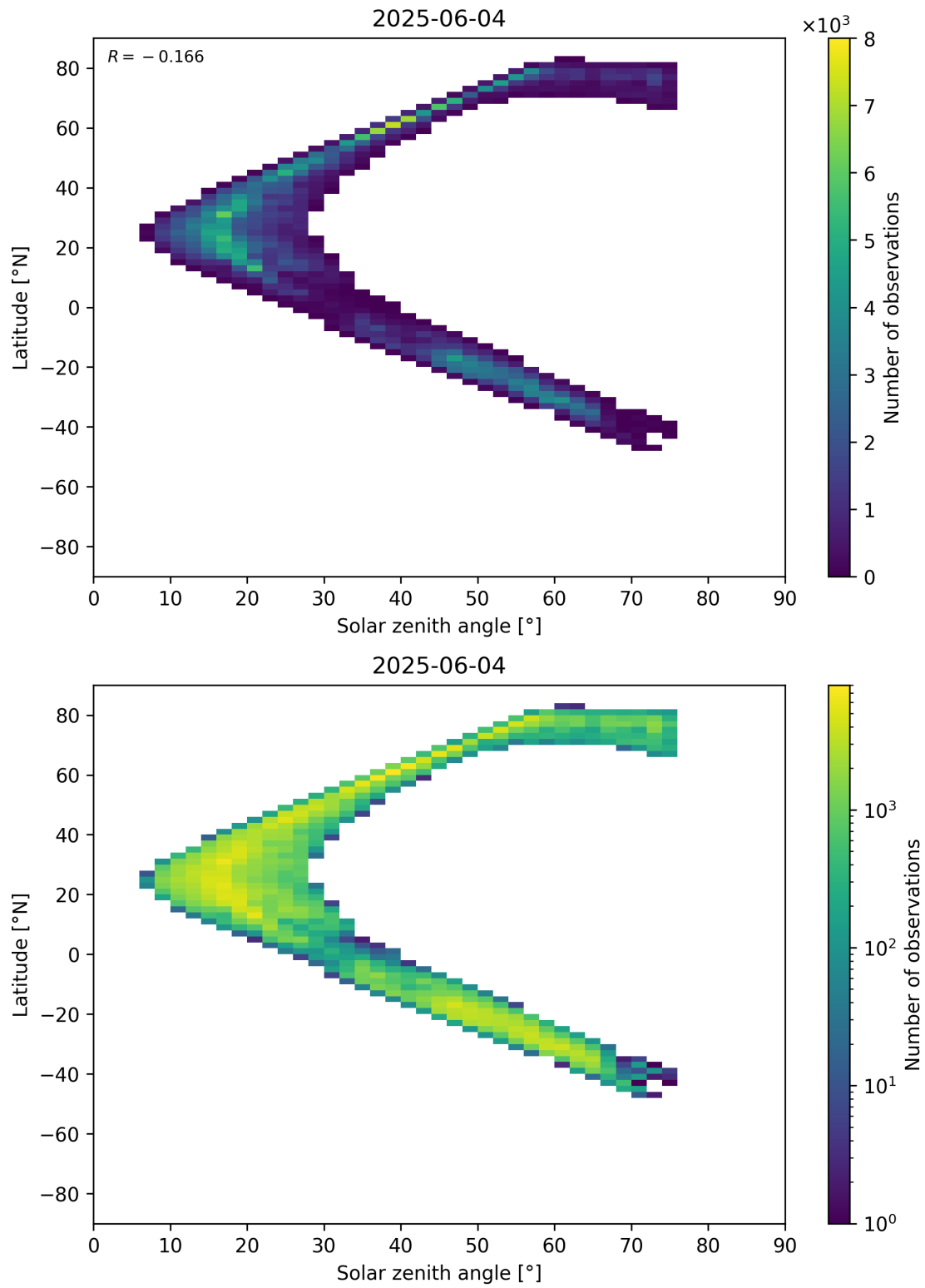
Figure 98: Scatter density plot of “Solar zenith angle” against “Latitude” for 2025-06-03 to 2025-06-05.
