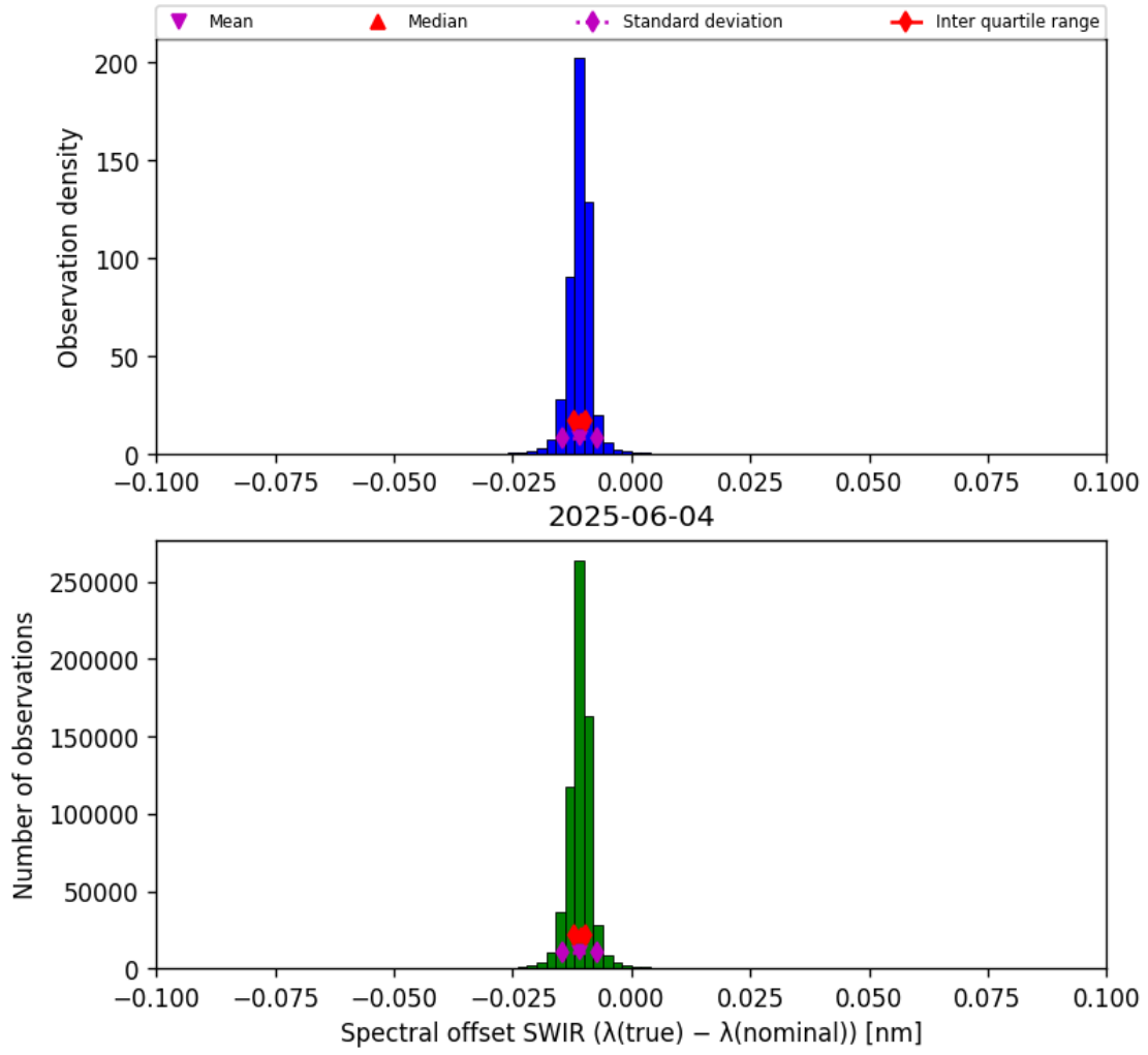
Figure 27: Histogram of “Spectral offset SWIR ( \lambda_{\text{true}} - \lambda_{\text{nominal}} )” for 2025-06-03 to 2025-06-05
