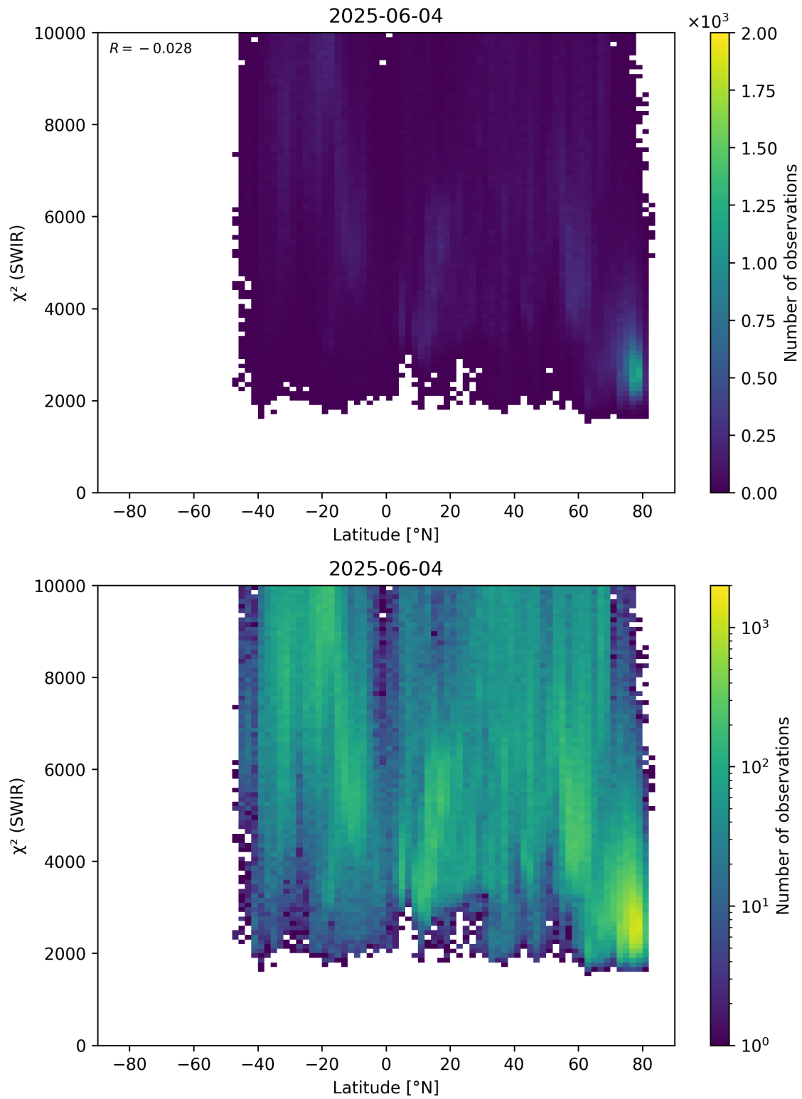
Figure 54: Scatter density plot of “Latitude” against “ \chi^2 (SWIR)” for 2025-06-03 to 2025-06-05.
