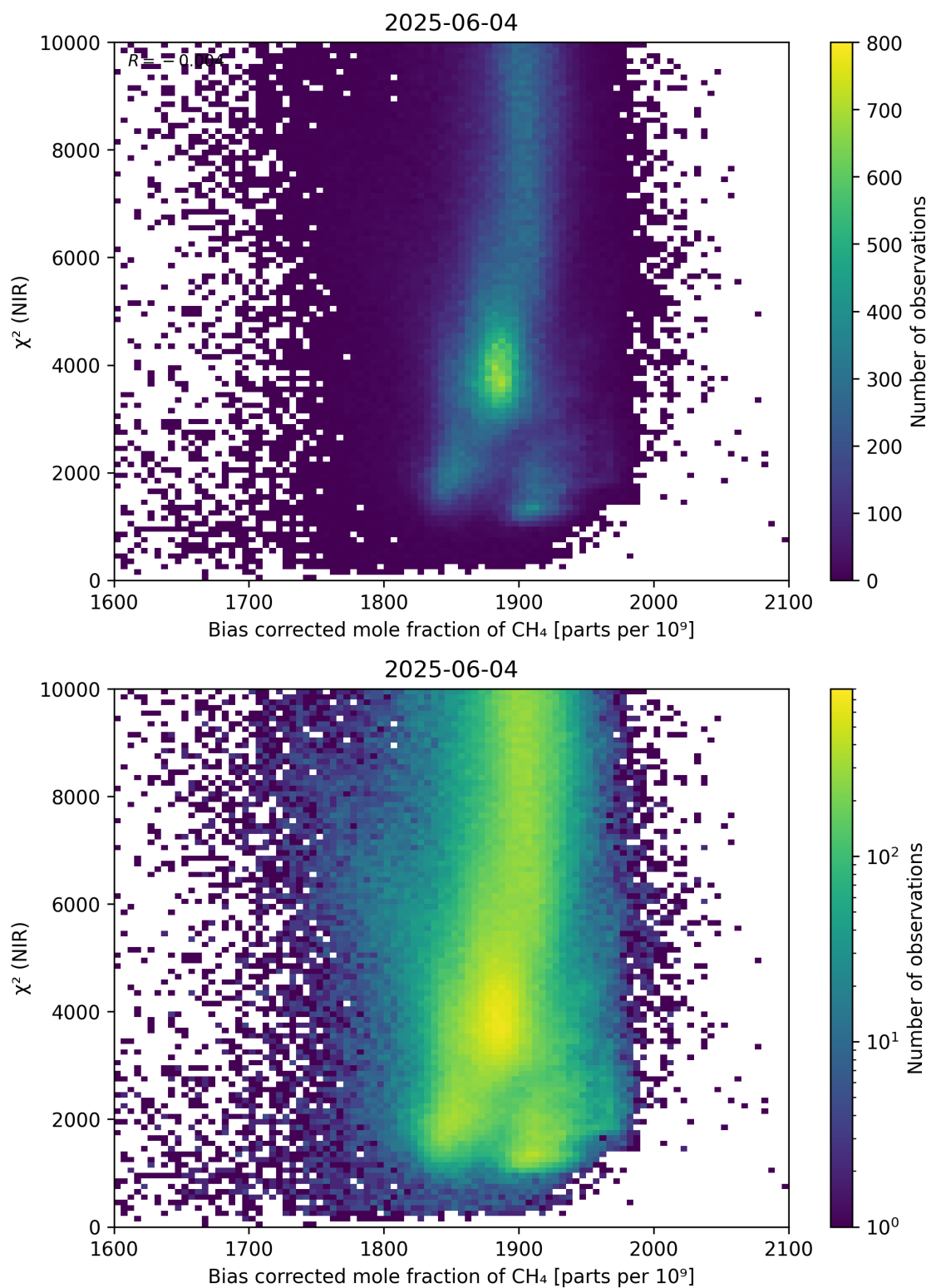
Figure 63: Scatter density plot of “Bias corrected mole fraction of \text{CH}_4 ” against “ \chi^2 (NIR)” for 2025-06-03 to 2025-06-05.
