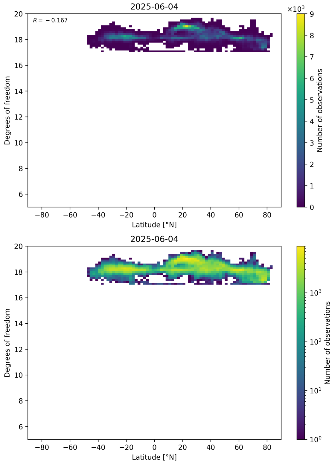
Figure 55: Scatter density plot of “Latitude” against “Degrees of freedom” for 2025-06-03 to 2025-06-05.
