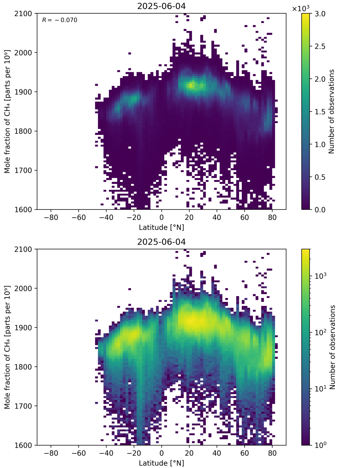
Figure 57: Scatter density plot of “Latitude” against “Mole fraction of CH 4 ” for 2025-06-03 to 2025-06-05.
