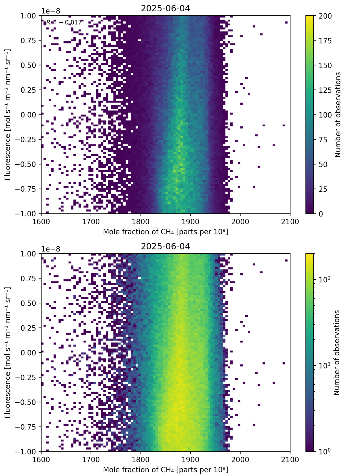
Figure 73: Scatter density plot of “Mole fraction of \text{CH}_4 ” against “Fluorescence” for 2025-06-03 to 2025-06-05.
