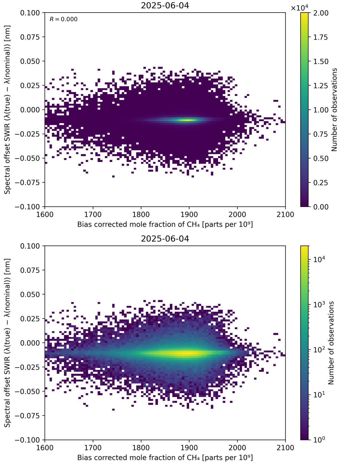
Figure 69: Scatter density plot of “Bias corrected mole fraction of \text{CH}_4 ” against “Spectral offset SWIR ( \lambda_{\text{true}} - \lambda_{\text{nominal}} )” for 2025-06-03 to 2025-06-05.
