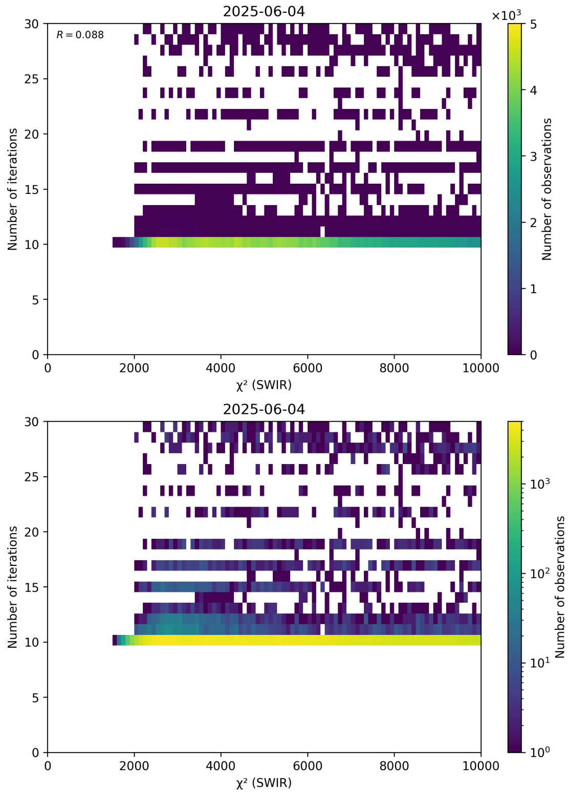
Figure 50: Scatter density plot of “ \chi^2 (SWIR)” against “Number of iterations” for 2025-06-03 to 2025-06-05.
