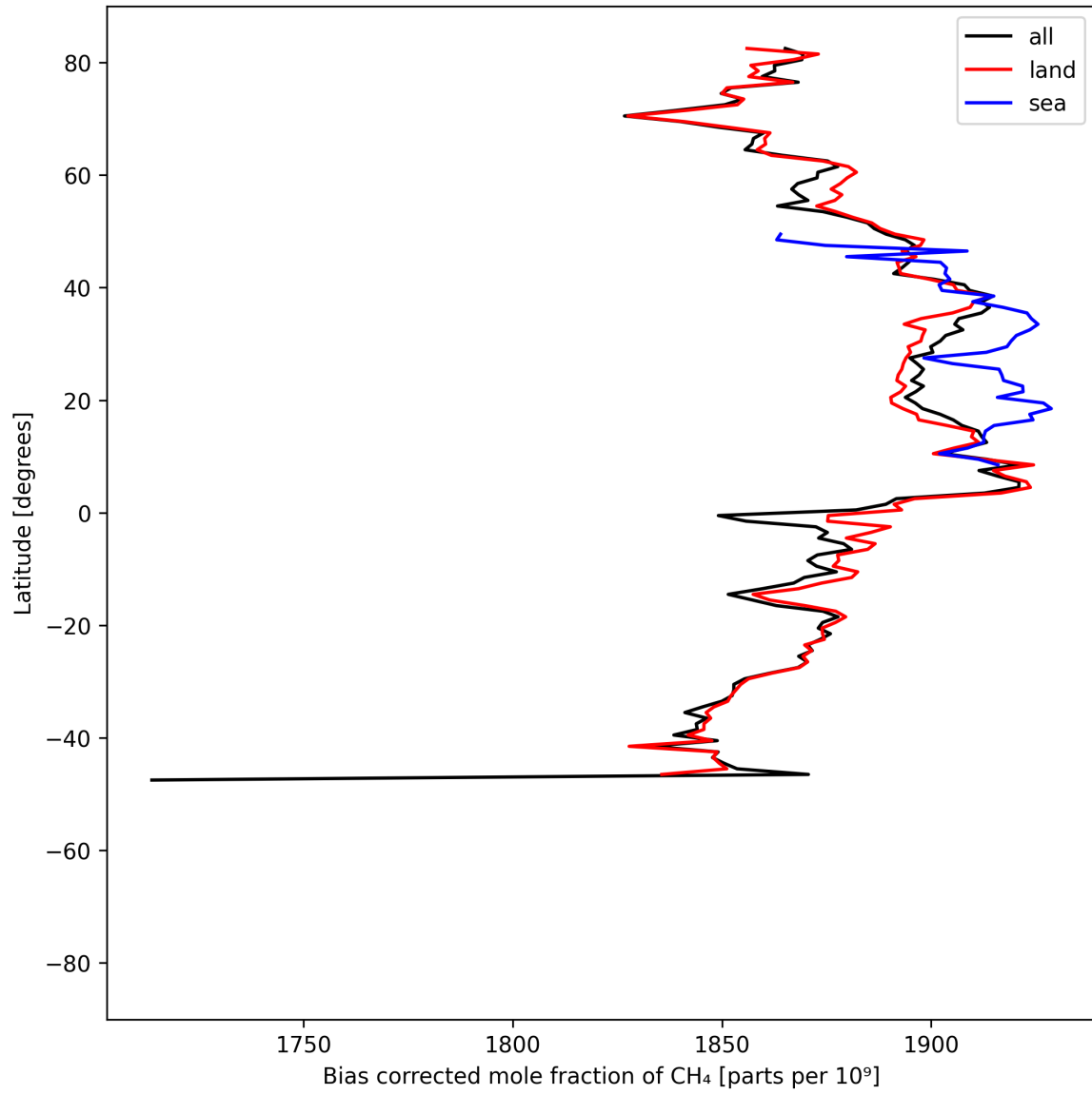
Figure 14: Zonal average of “Bias corrected mole fraction of CH 4 ” for 2025-06-03 to 2025-06-05.
