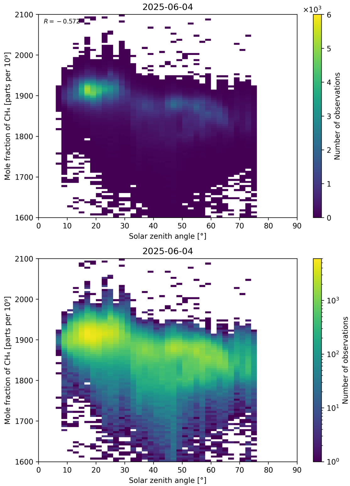
Figure 99: Scatter density plot of “Solar zenith angle” against “Mole fraction of CH 4 ” for 2025-06-03 to 2025-06-05.
