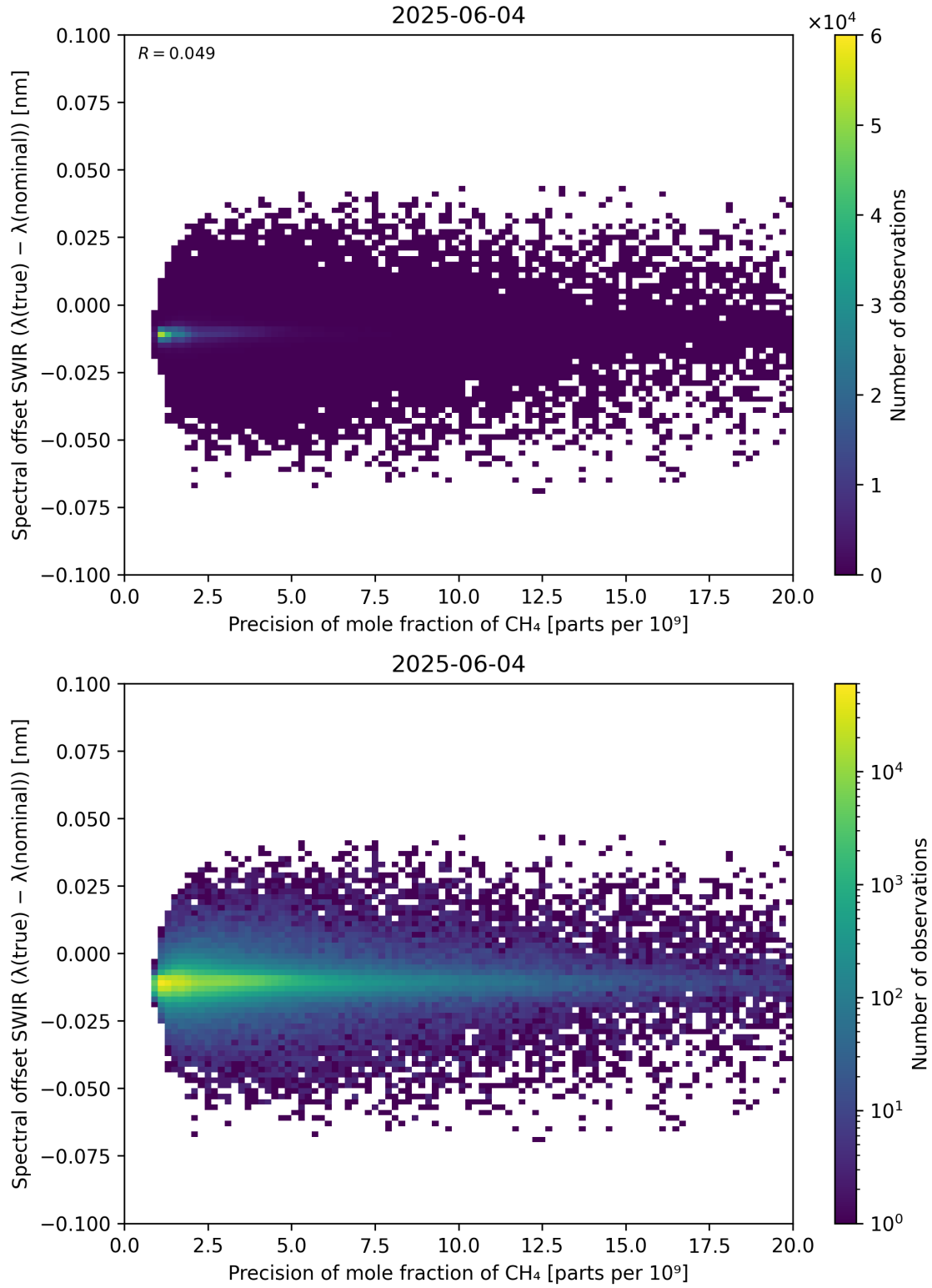
Figure 85: Scatter density plot of “Precision of mole fraction of \text{CH}_4 ” against “Spectral offset SWIR ( \lambda_{\text{true}} - \lambda_{\text{nominal}} )” for 2025-06-03 to 2025-06-05.
