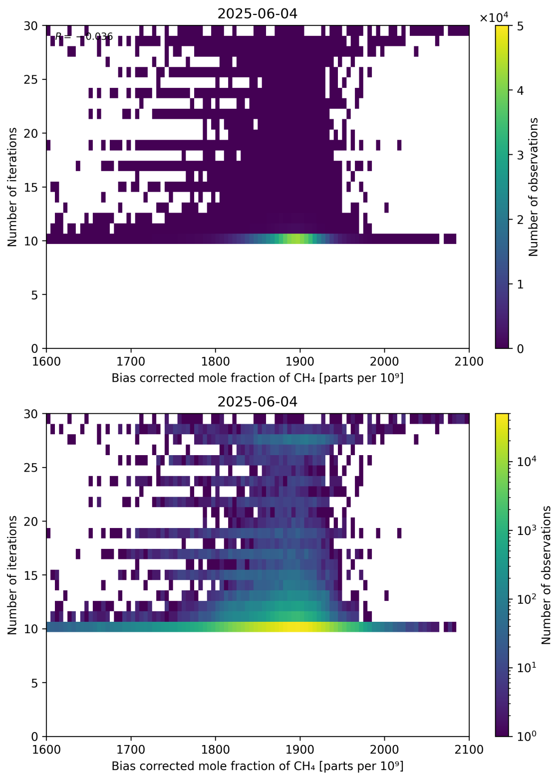
Figure 67: Scatter density plot of “Bias corrected mole fraction of CH 4 ” against “Number of iterations” for 2025-06-03 to 2025-06-05.
