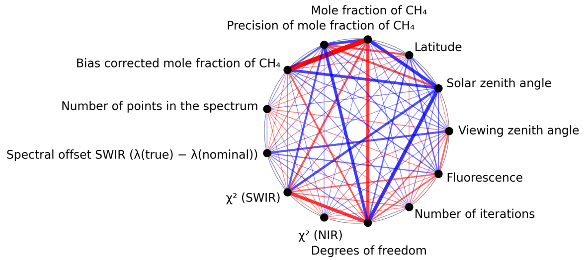
Figure 1: Map of correlation graph for 2025-06-03 to 2025-06-05.
