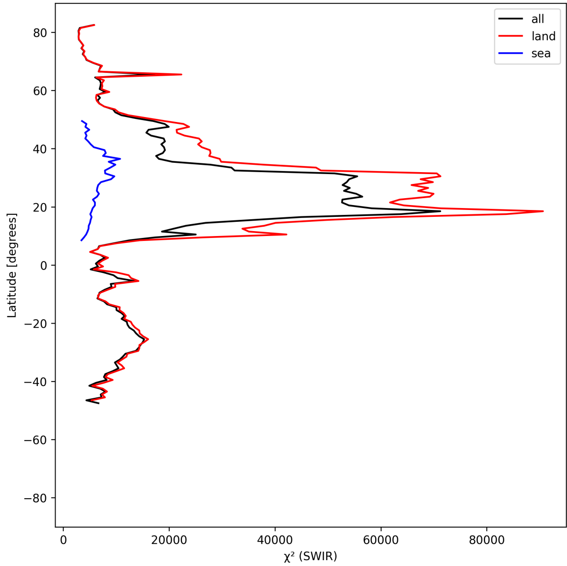
Figure 17: Zonal average of “ \chi^2 (SWIR)” for 2025-06-03 to 2025-06-05.
