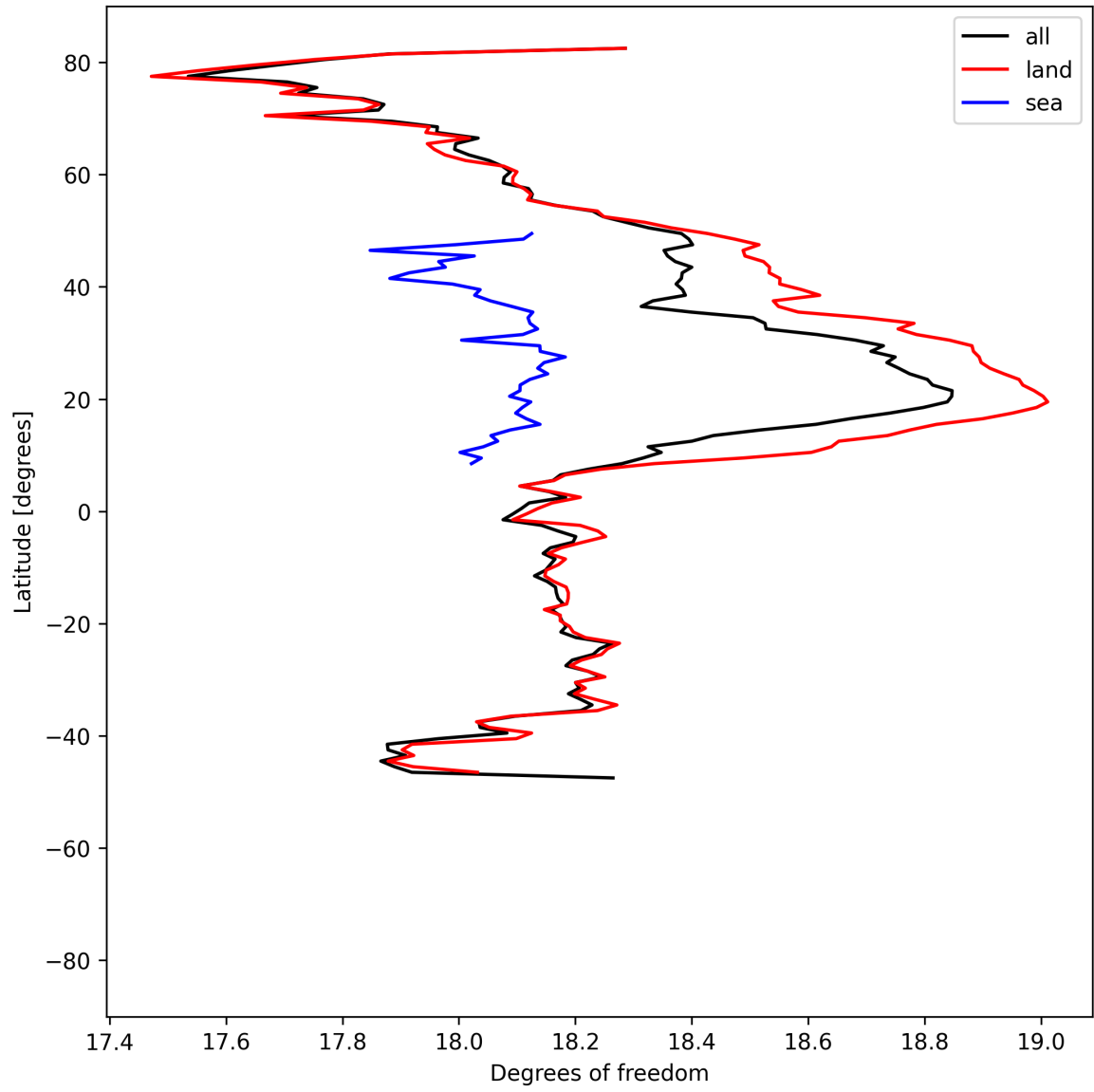
Figure 19: Zonal average of “Degrees of freedom” for 2025-06-03 to 2025-06-05.
