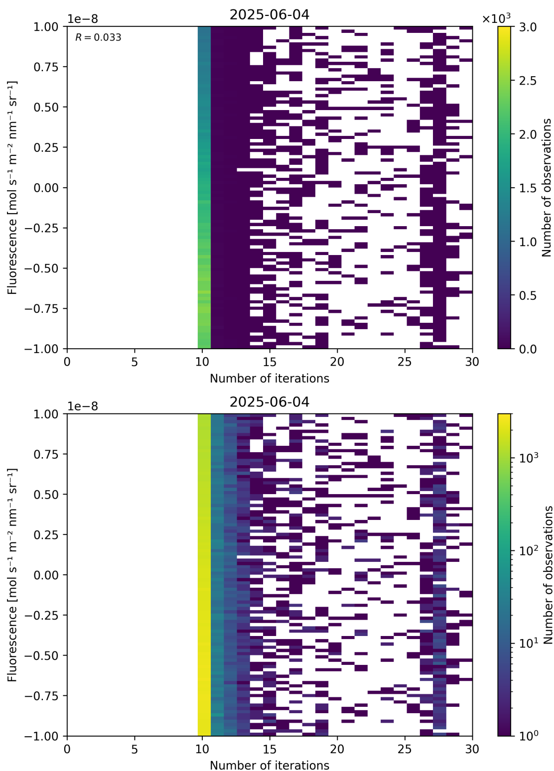
Figure 87: Scatter density plot of “Number of iterations” against “Fluorescence” for 2025-06-03 to 2025-06-05.
