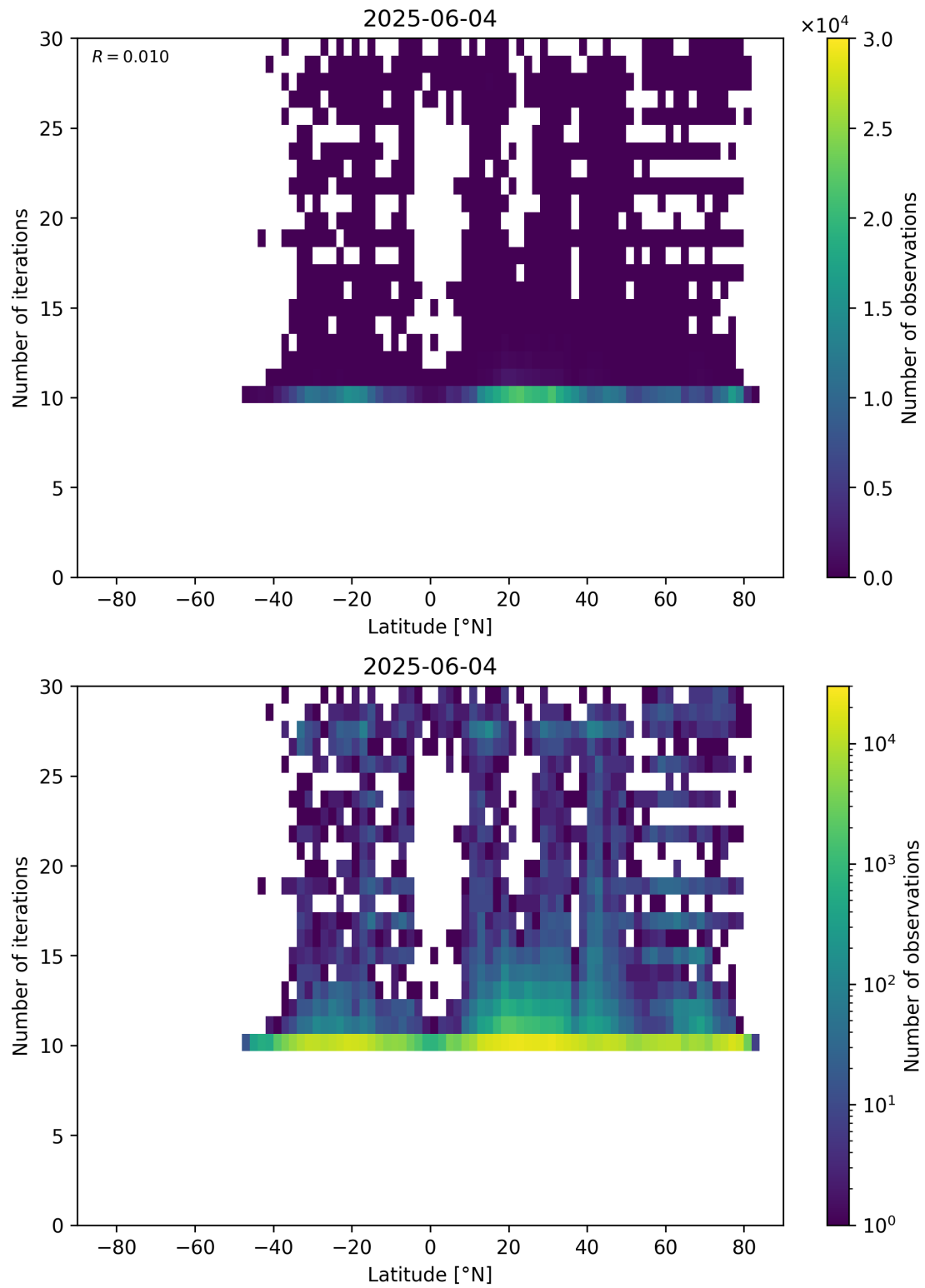
Figure 60: Scatter density plot of “Latitude” against “Number of iterations” for 2025-06-03 to 2025-06-05.
