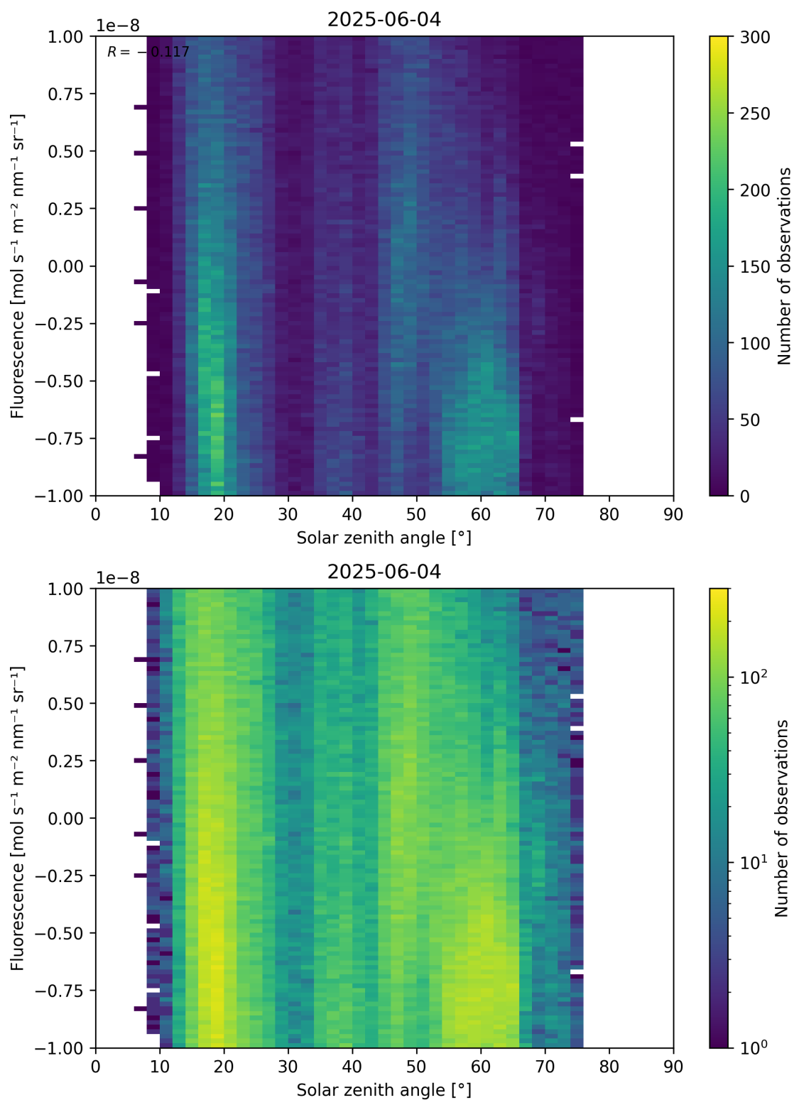
Figure 97: Scatter density plot of “Solar zenith angle” against “Fluorescence” for 2025-06-03 to 2025-06-05.
