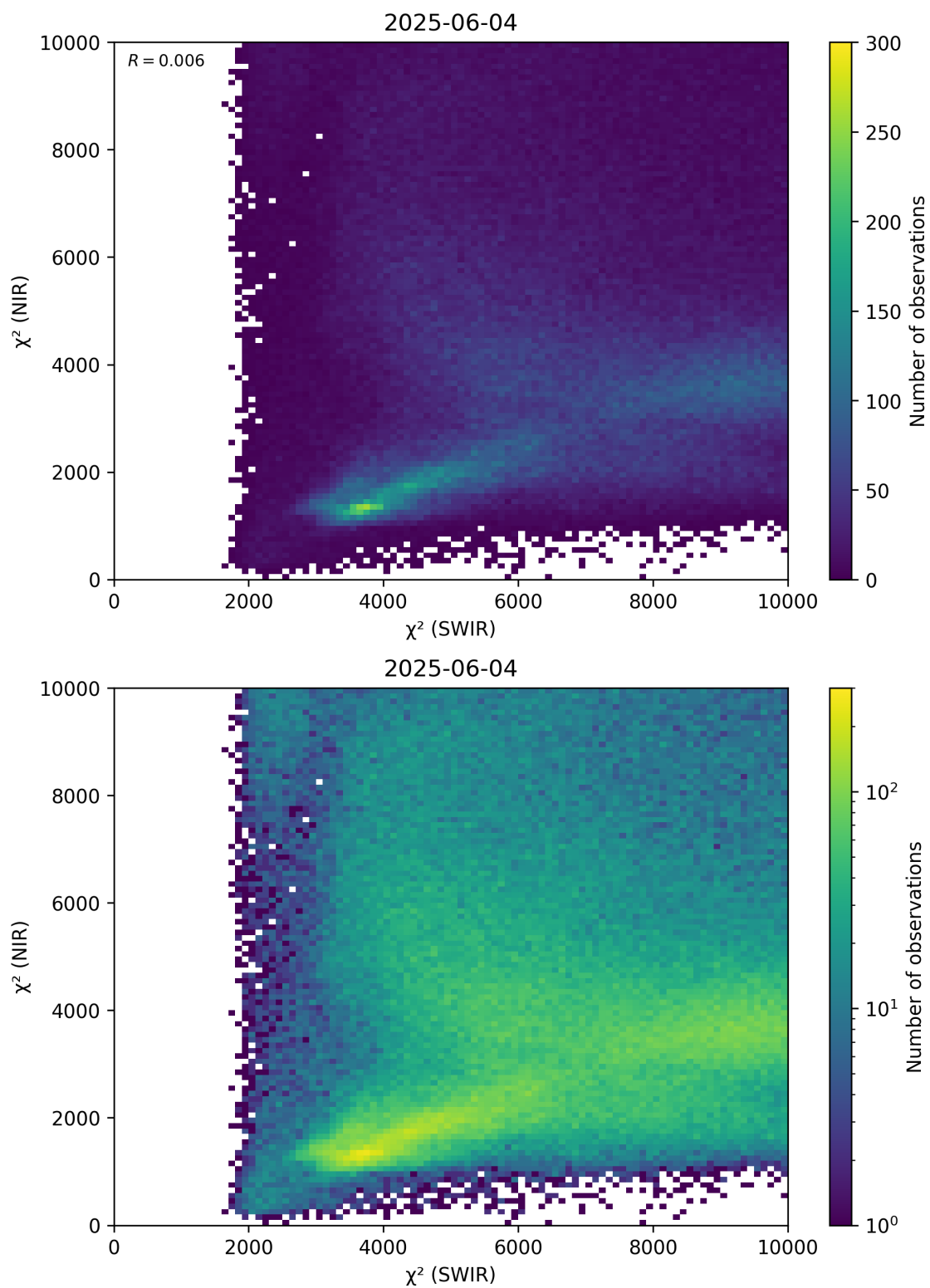
Figure 47: Scatter density plot of “ \chi^2 (SWIR)” against “ \chi^2 (NIR)” for 2025-06-03 to 2025-06-05.
