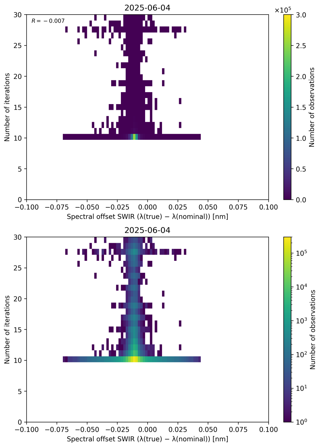
Figure 121: Scatter density plot of “Spectral offset SWIR ( \lambda_{\text{true}} - \lambda_{\text{nominal}} )” against “Number of iterations” for 2025-06-03 to 2025-06-05.
