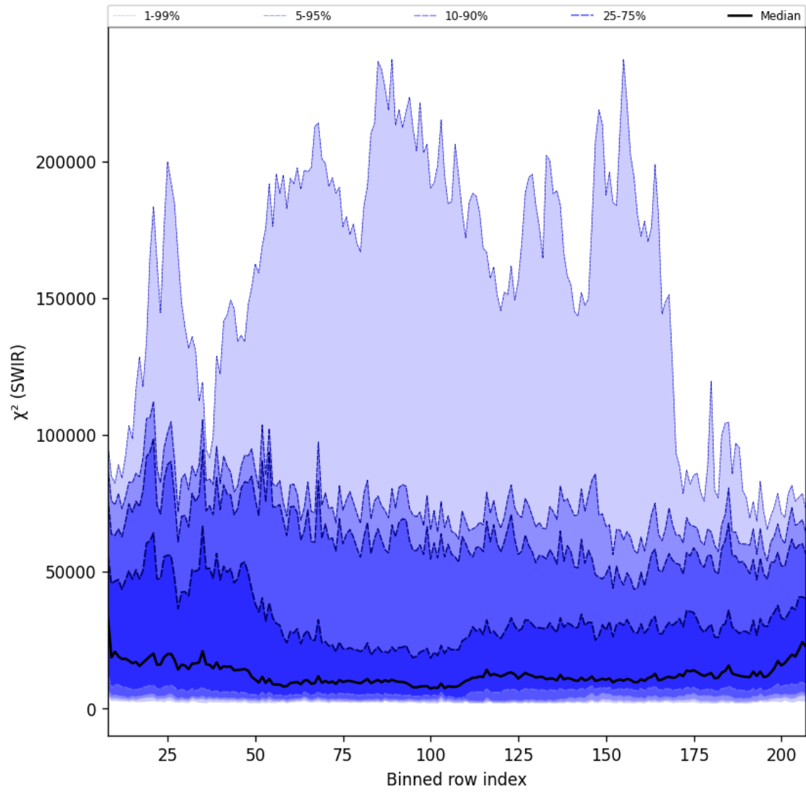
Figure 39: Along track statistics of “ \chi^2 (SWIR)” for 2025-06-03 to 2025-06-05
