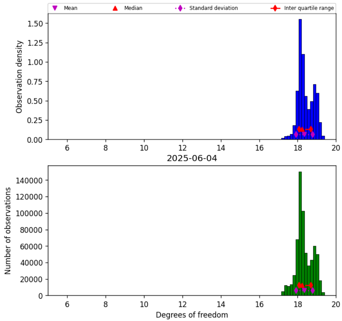
Figure 30: Histogram of “Degrees of freedom” for 2025-06-03 to 2025-06-05
