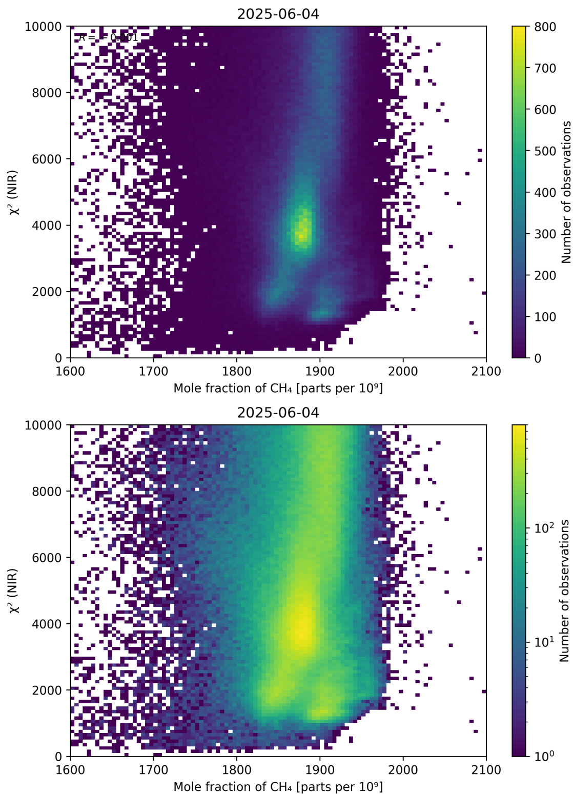
Figure 70: Scatter density plot of “Mole fraction of CH 4 ” against “ \chi^2 (NIR)” for 2025-06-03 to 2025-06-05.
