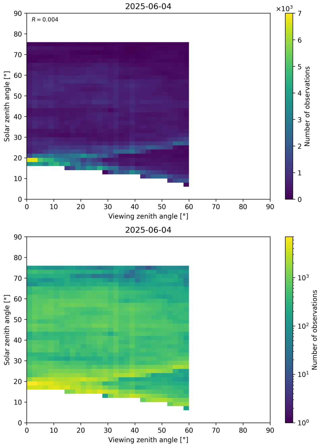
Figure 115: Scatter density plot of “Viewing zenith angle” against “Solar zenith angle” for 2025-06-03 to 2025-06-05.
