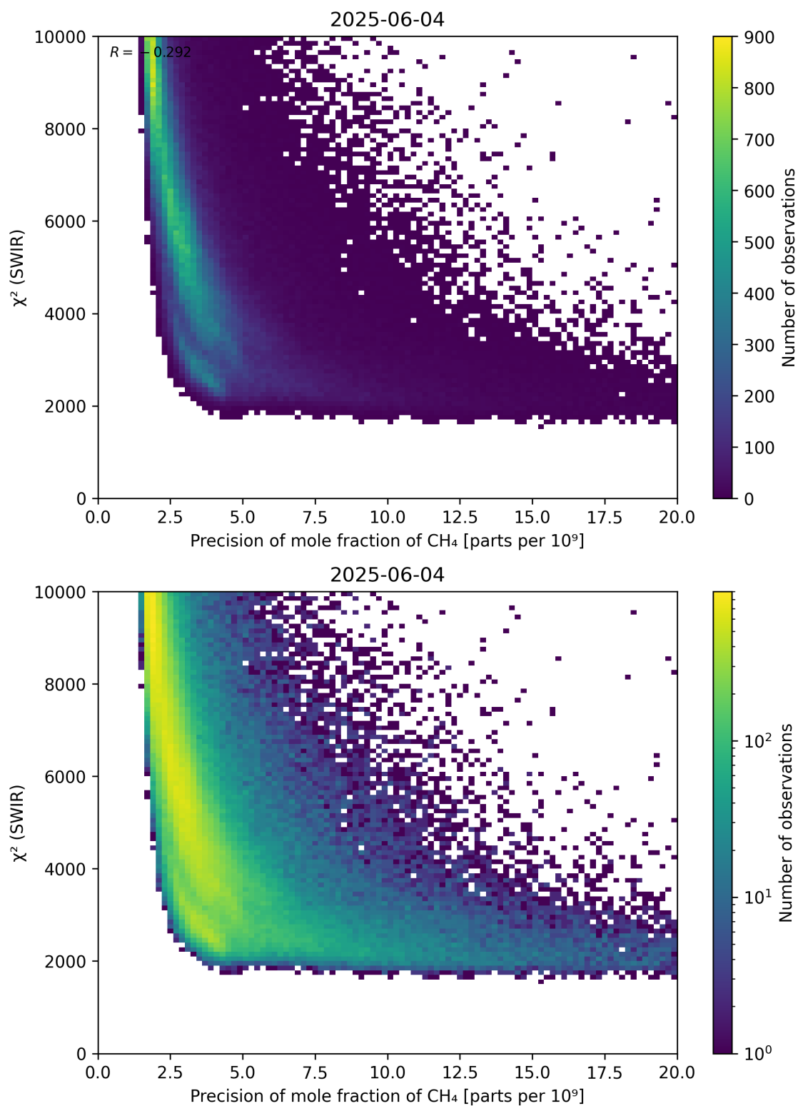
Figure 79: Scatter density plot of “Precision of mole fraction of \text{CH}_4 ” against “ \chi^2 (SWIR)” for 2025-06-03 to 2025-06-05.
