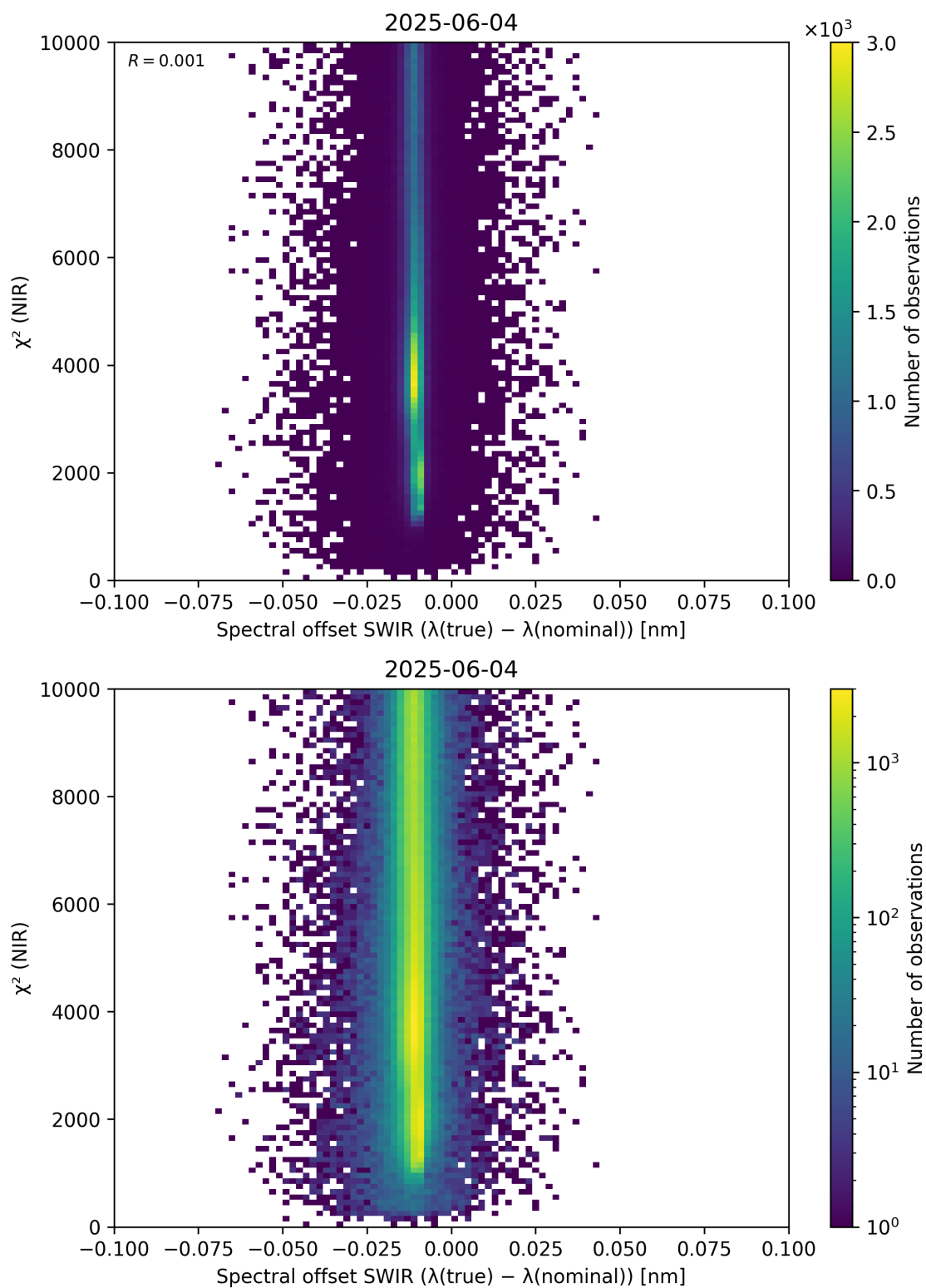
Figure 117: Scatter density plot of “Spectral offset SWIR ( \lambda_{\text{true}} - \lambda_{\text{nominal}} )” against “ \chi^2 (NIR)” for 2025-06-03 to 2025-06-05.
