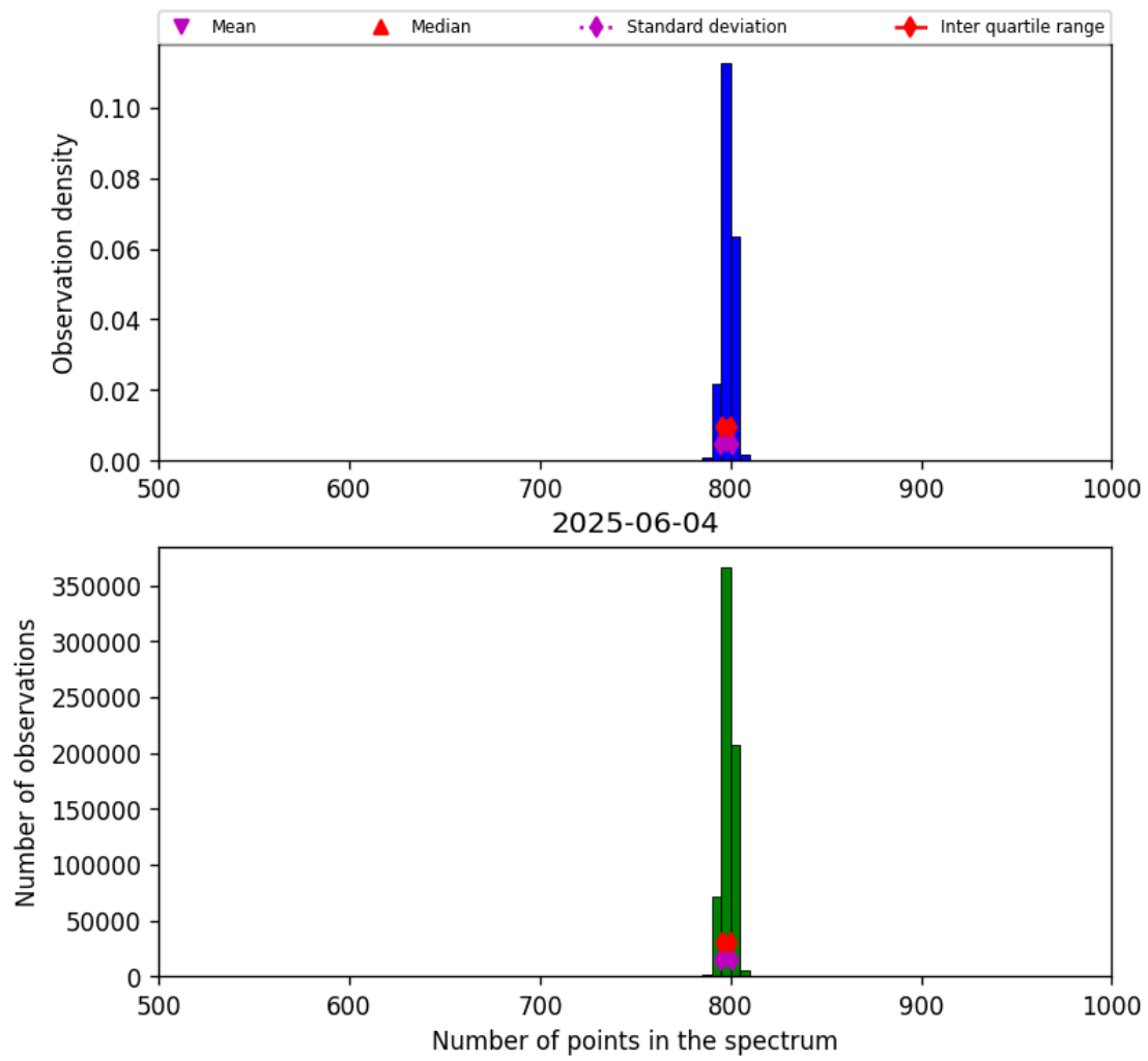
Figure 26: Histogram of “Number of points in the spectrum” for 2025-06-03 to 2025-06-05
