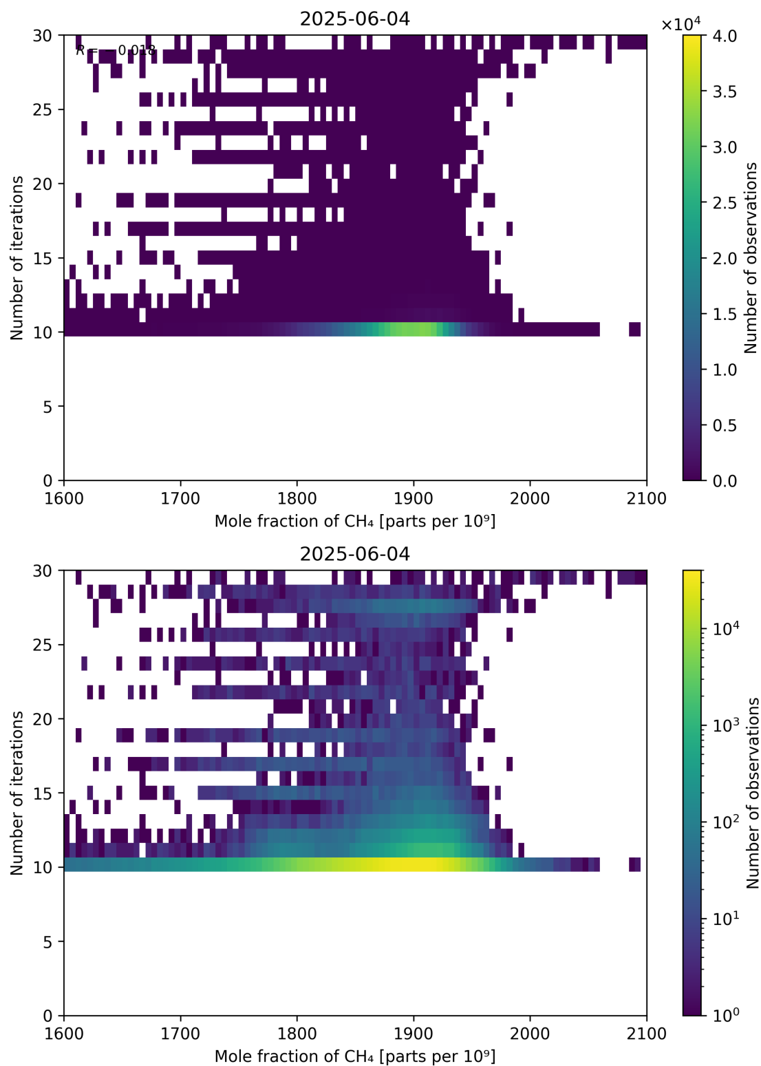
Figure 76: Scatter density plot of “Mole fraction of CH 4 ” against “Number of iterations” for 2025-06-03 to 2025-06-05.
