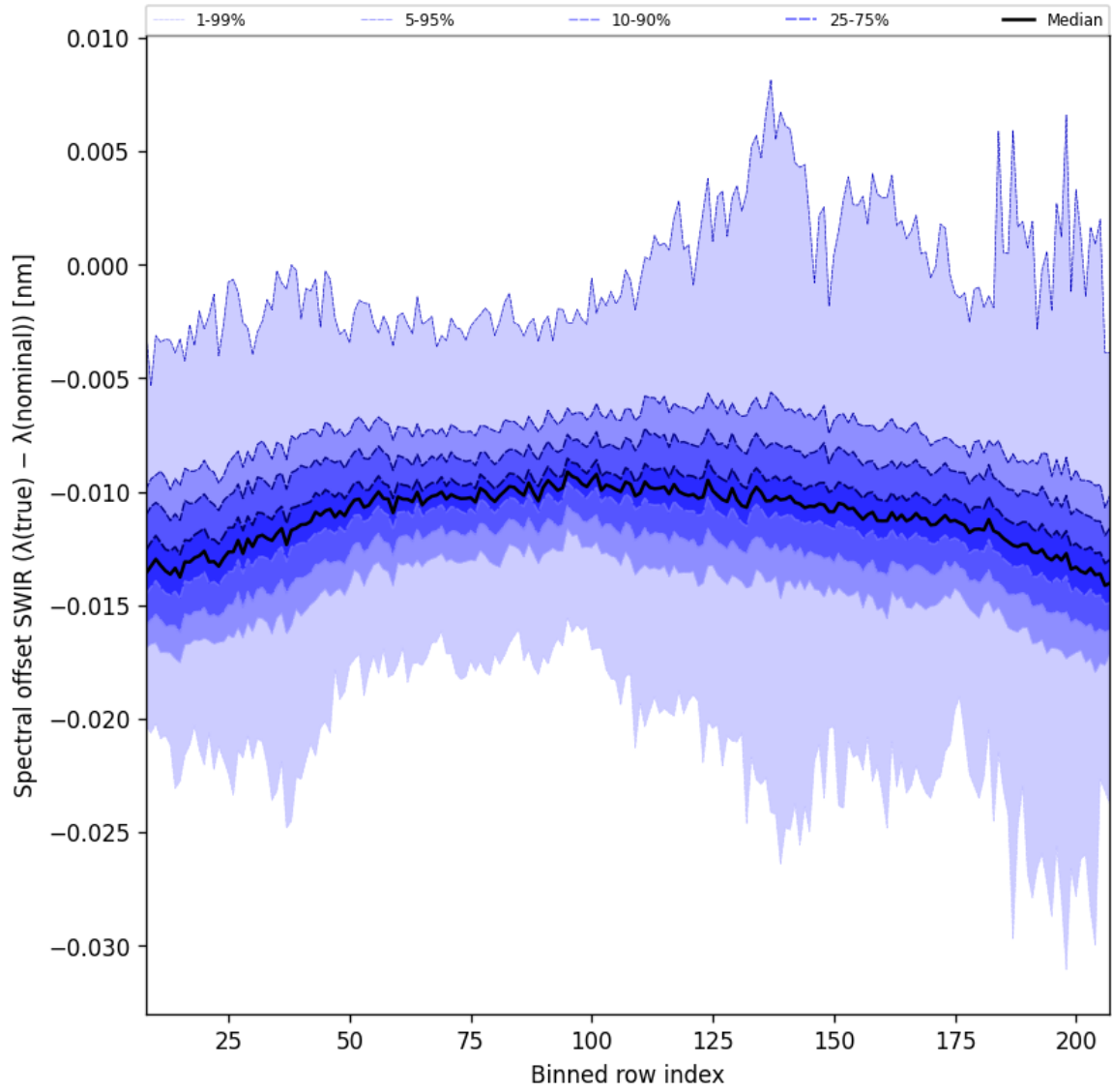
Figure 38: Along track statistics of “Spectral offset SWIR ( \lambda_{\text{true}} - \lambda_{\text{nominal}} )” for 2025-06-03 to 2025-06-05
