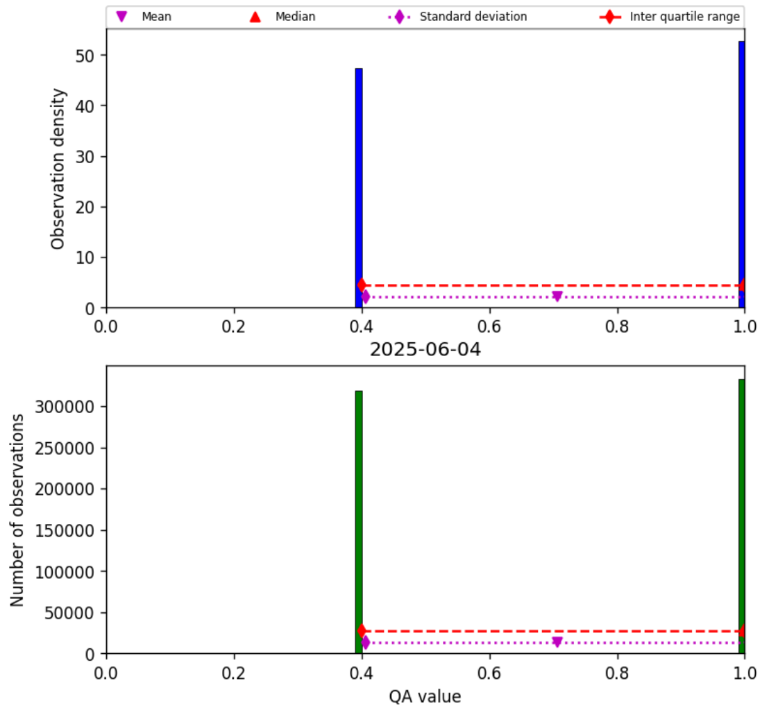
Figure 22: Histogram of “QA value” for 2025-06-03 to 2025-06-05
