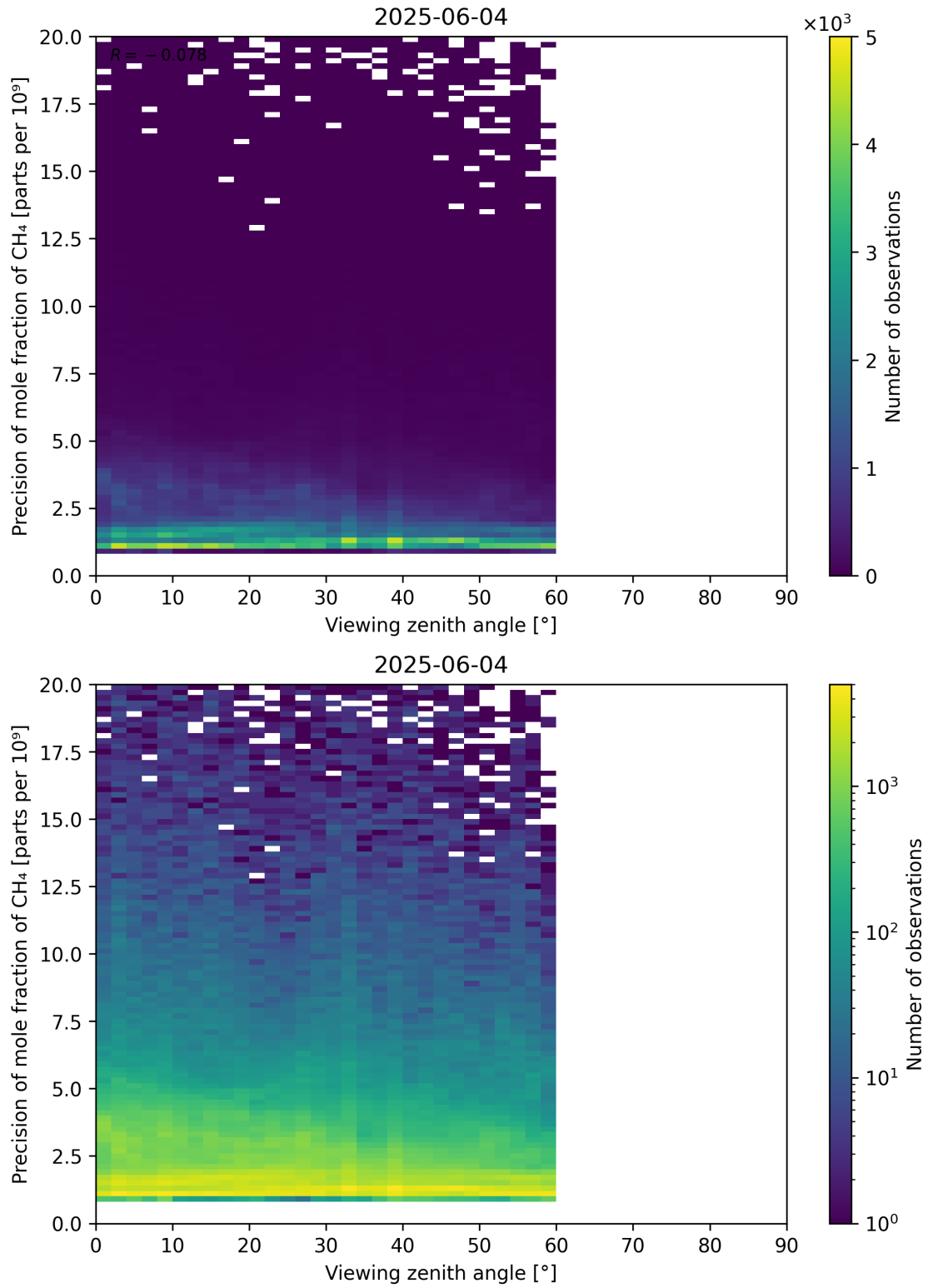
Figure 112: Scatter density plot of “Viewing zenith angle” against “Precision of mole fraction of CH 4 ” for 2025-06-03 to 2025-06-05.
