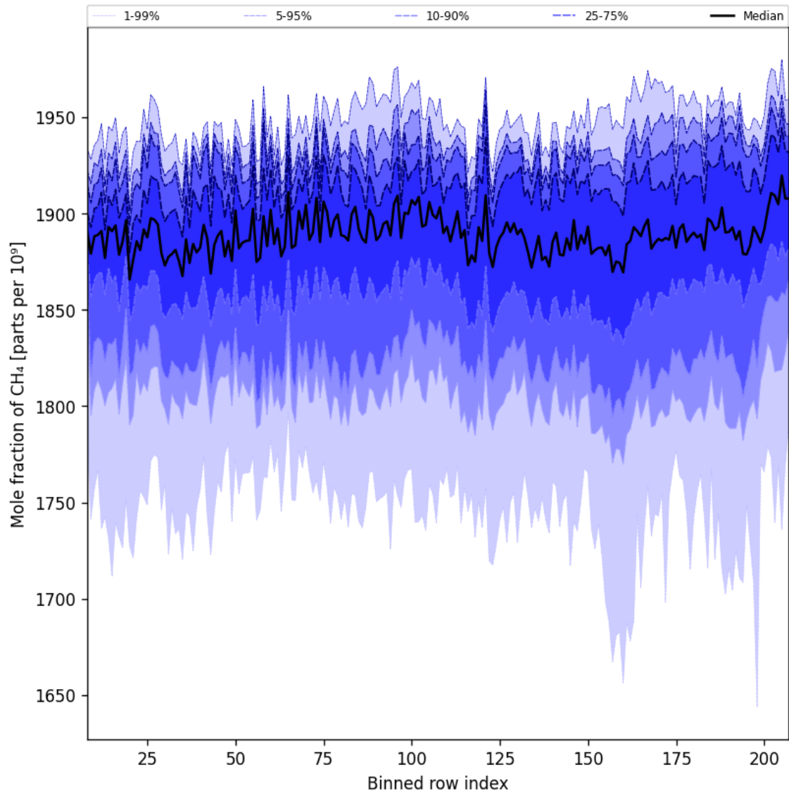
Figure 34: Along track statistics of “Mole fraction of CH 4 ” for 2025-06-03 to 2025-06-05
