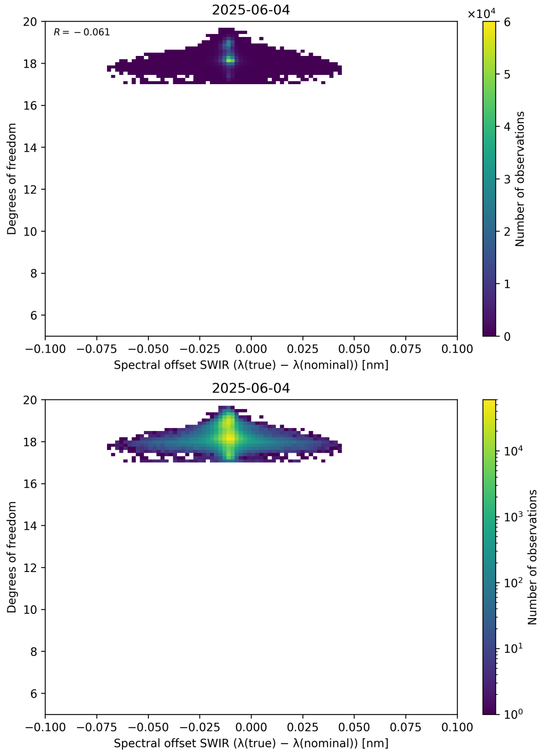
Figure 119: Scatter density plot of “Spectral offset SWIR ( \lambda_{\text{true}} - \lambda_{\text{nominal}} )” against “Degrees of freedom” for 2025-06-03 to 2025-06-05.
