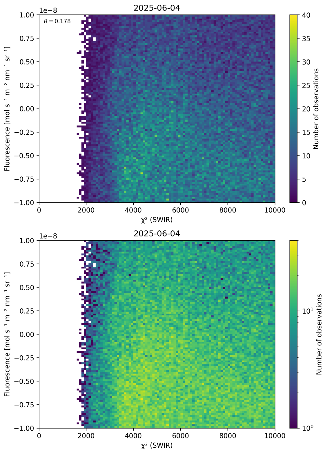
Figure 49: Scatter density plot of “ \chi^2 (SWIR)” against “Fluorescence” for 2025-06-03 to 2025-06-05.
