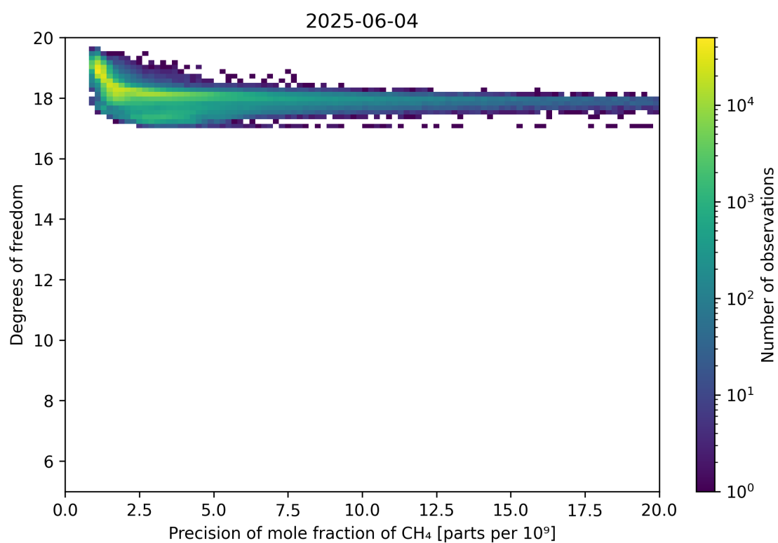
Figure 80: Scatter density plot of “Precision of mole fraction of \text{CH}_4 ” against “Degrees of freedom” for 2025-06-03 to 2025-06-05.
