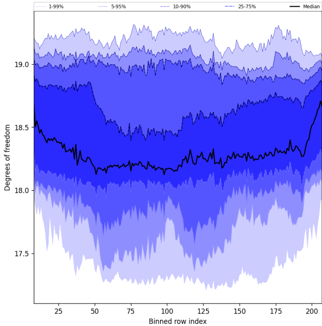
Figure 41: Along track statistics of “Degrees of freedom” for 2025-06-03 to 2025-06-05
