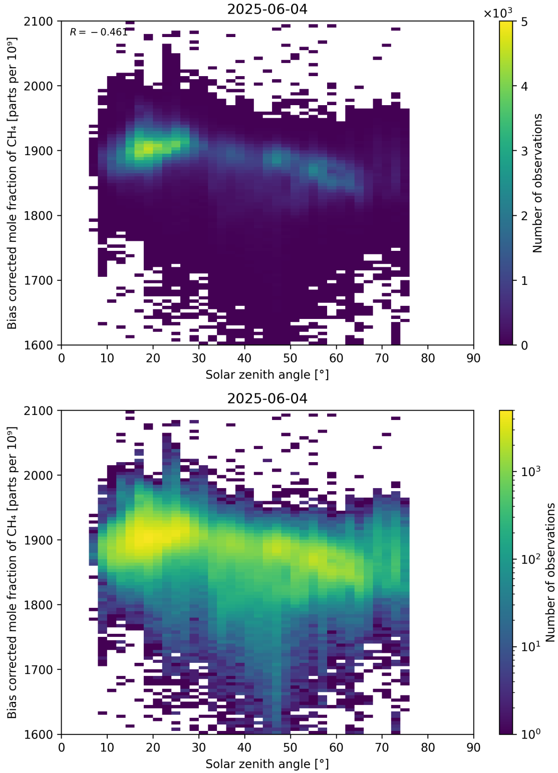
Figure 100: Scatter density plot of “Solar zenith angle” against “Bias corrected mole fraction of CH 4 ” for 2025-06-03 to 2025-06-05.
