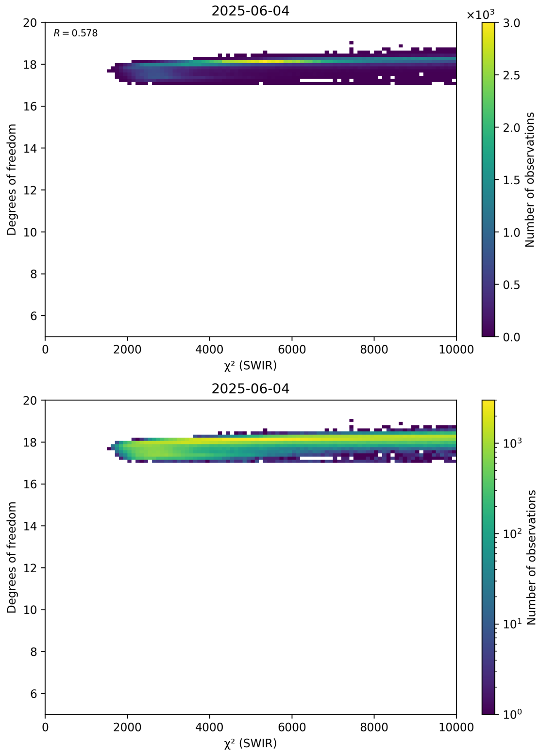
Figure 48: Scatter density plot of “ \chi^2 (SWIR)” against “Degrees of freedom” for 2025-06-03 to 2025-06-05.
