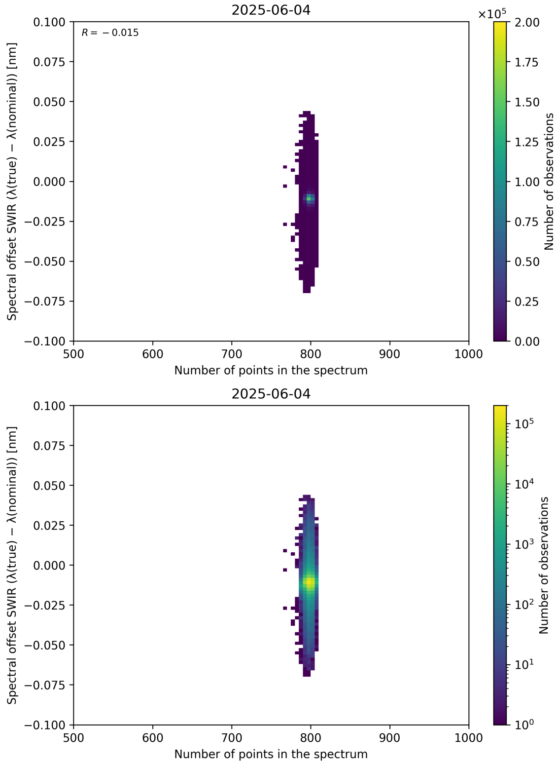
Figure 93: Scatter density plot of “Number of points in the spectrum” against “Spectral offset SWIR ( \lambda_{\text{true}} - \lambda_{\text{nominal}} )” for 2025-06-03 to 2025-06-05.
