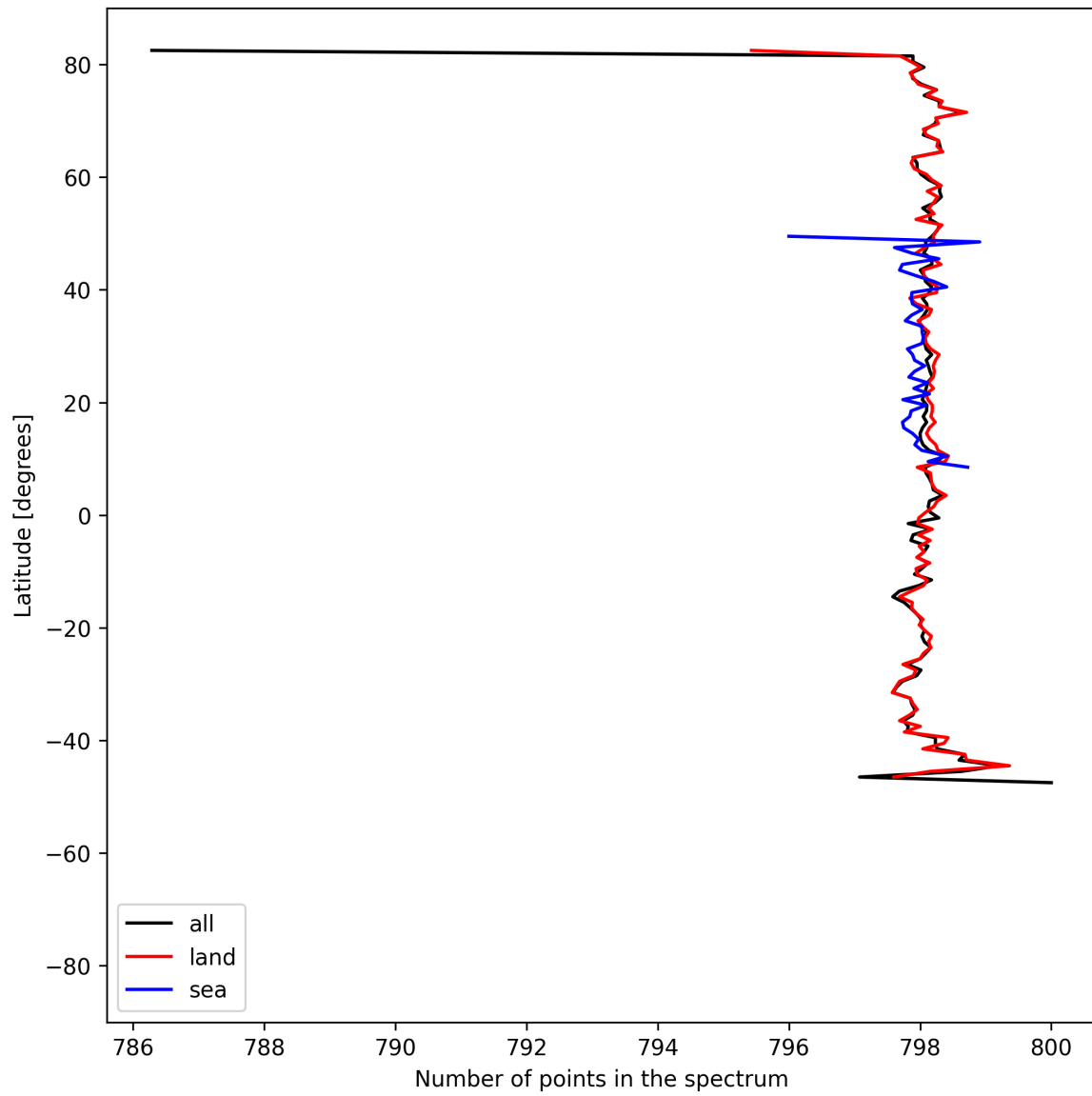
Figure 15: Zonal average of “Number of points in the spectrum” for 2025-06-03 to 2025-06-05.
