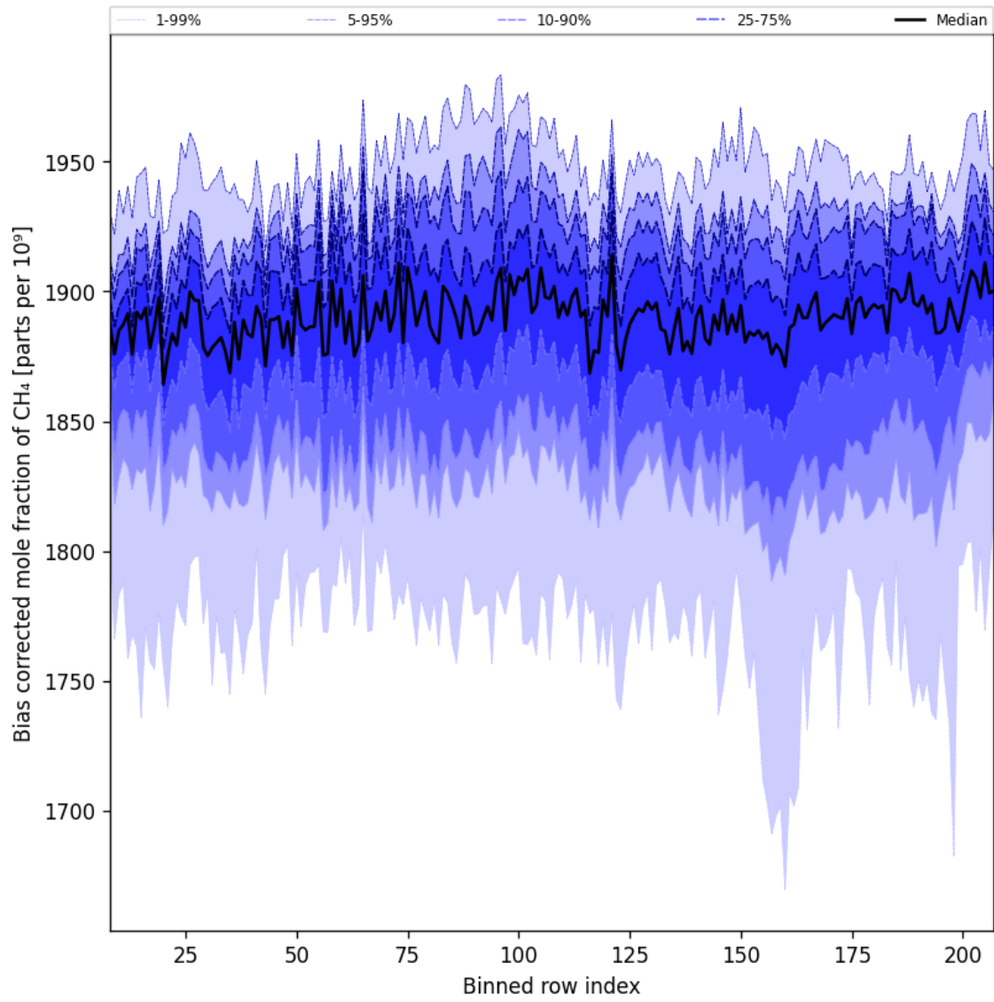
Figure 36: Along track statistics of “Bias corrected mole fraction of CH 4 ” for 2025-06-03 to 2025-06-05
