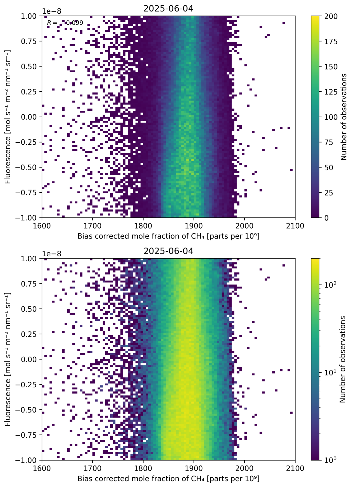
Figure 66: Scatter density plot of “Bias corrected mole fraction of CH 4 ” against “Fluorescence” for 2025-06-03 to 2025-06-05.
