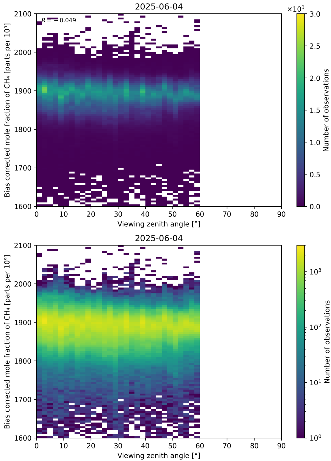
Figure 111: Scatter density plot of “Viewing zenith angle” against “Bias corrected mole fraction of CH 4 ” for 2025-06-03 to 2025-06-05.
