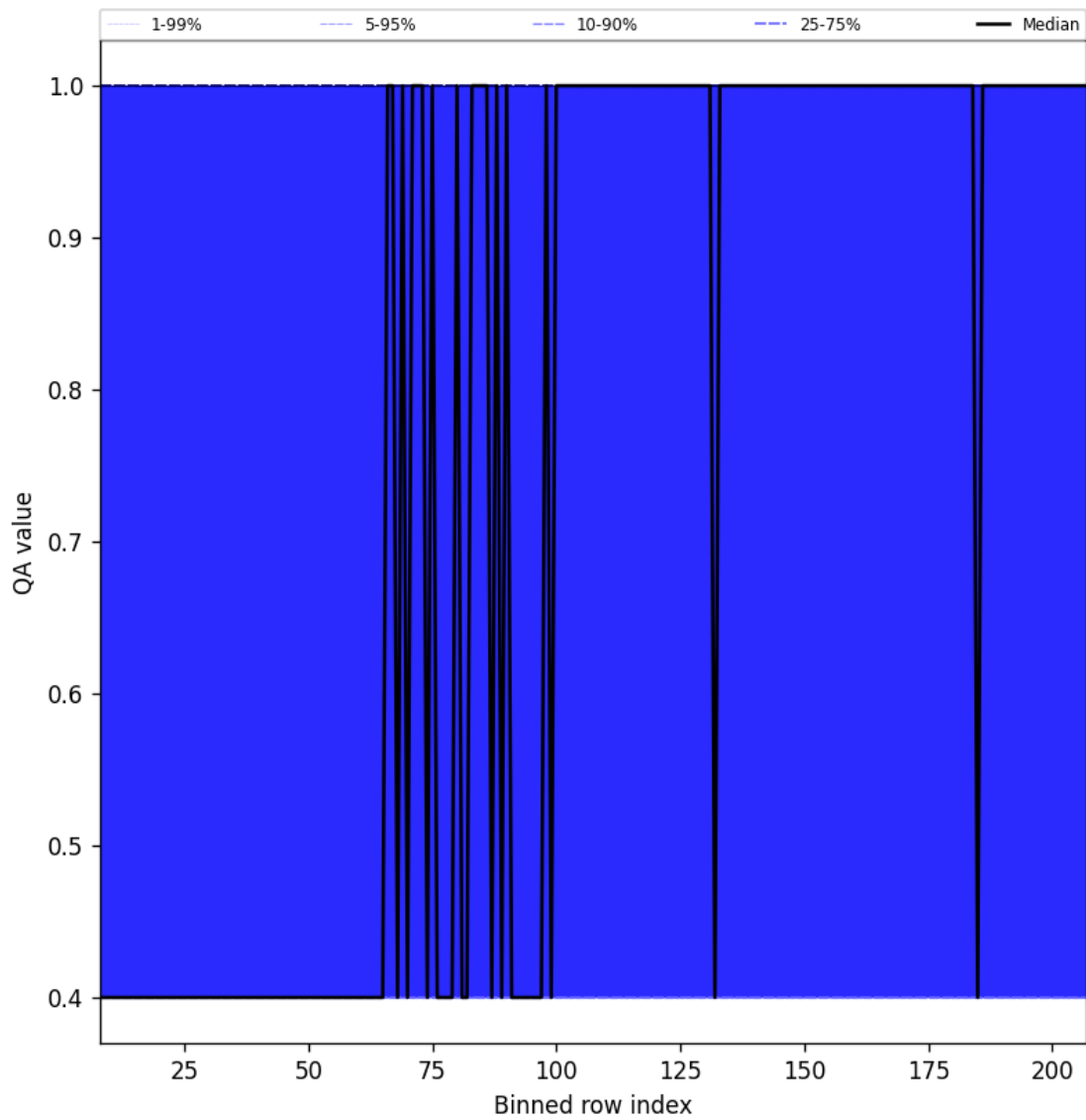
Figure 33: Along track statistics of “QA value” for 2025-06-03 to 2025-06-05
