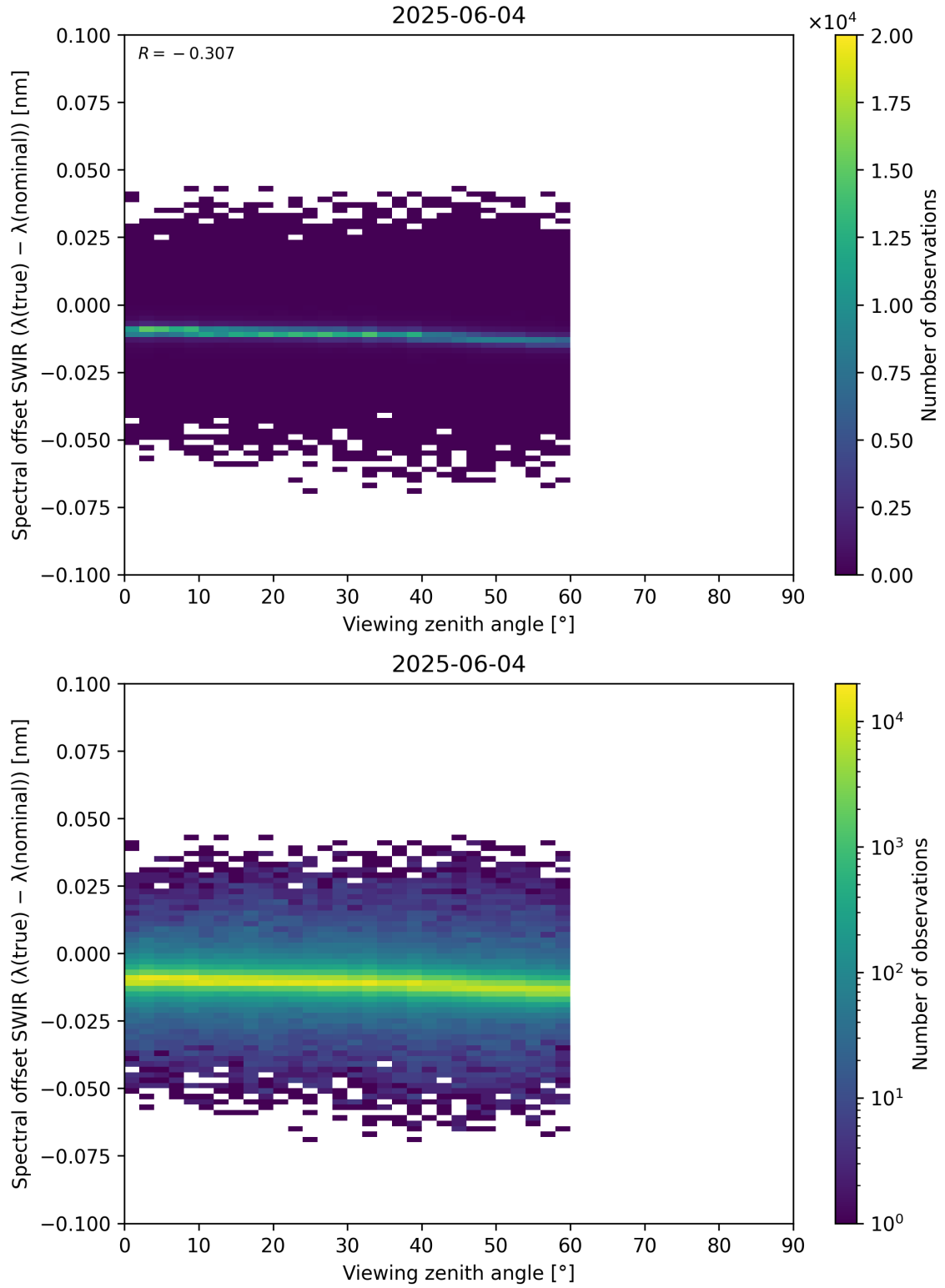
Figure 116: Scatter density plot of “Viewing zenith angle” against “Spectral offset SWIR ( \lambda_{\text{true}} - \lambda_{\text{nominal}} )” for 2025-06-03 to 2025-06-05.
