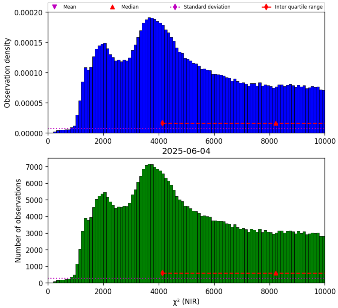
Figure 29: Histogram of " \chi^2 (NIR)" for 2025-06-03 to 2025-06-05
