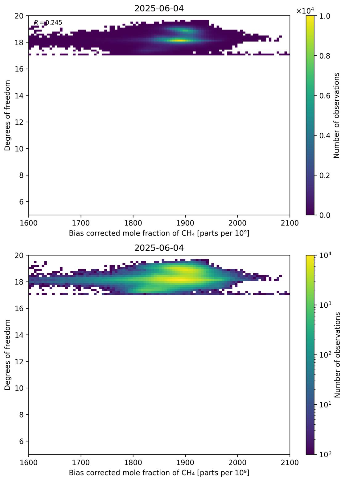
Figure 65: Scatter density plot of “Bias corrected mole fraction of CH 4 ” against “Degrees of freedom” for 2025-06-03 to 2025-06-05.
