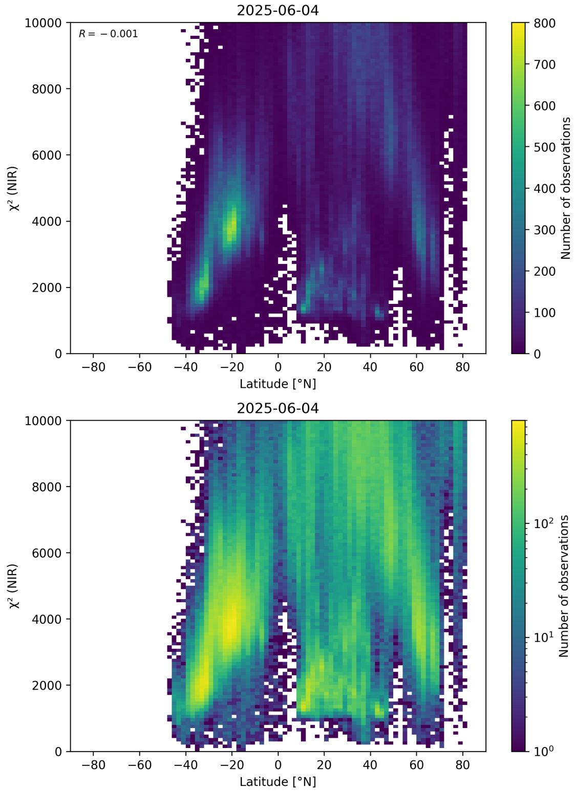
Figure 53: Scatter density plot of “Latitude” against “ \chi^2 (NIR)” for 2025-06-03 to 2025-06-05.
