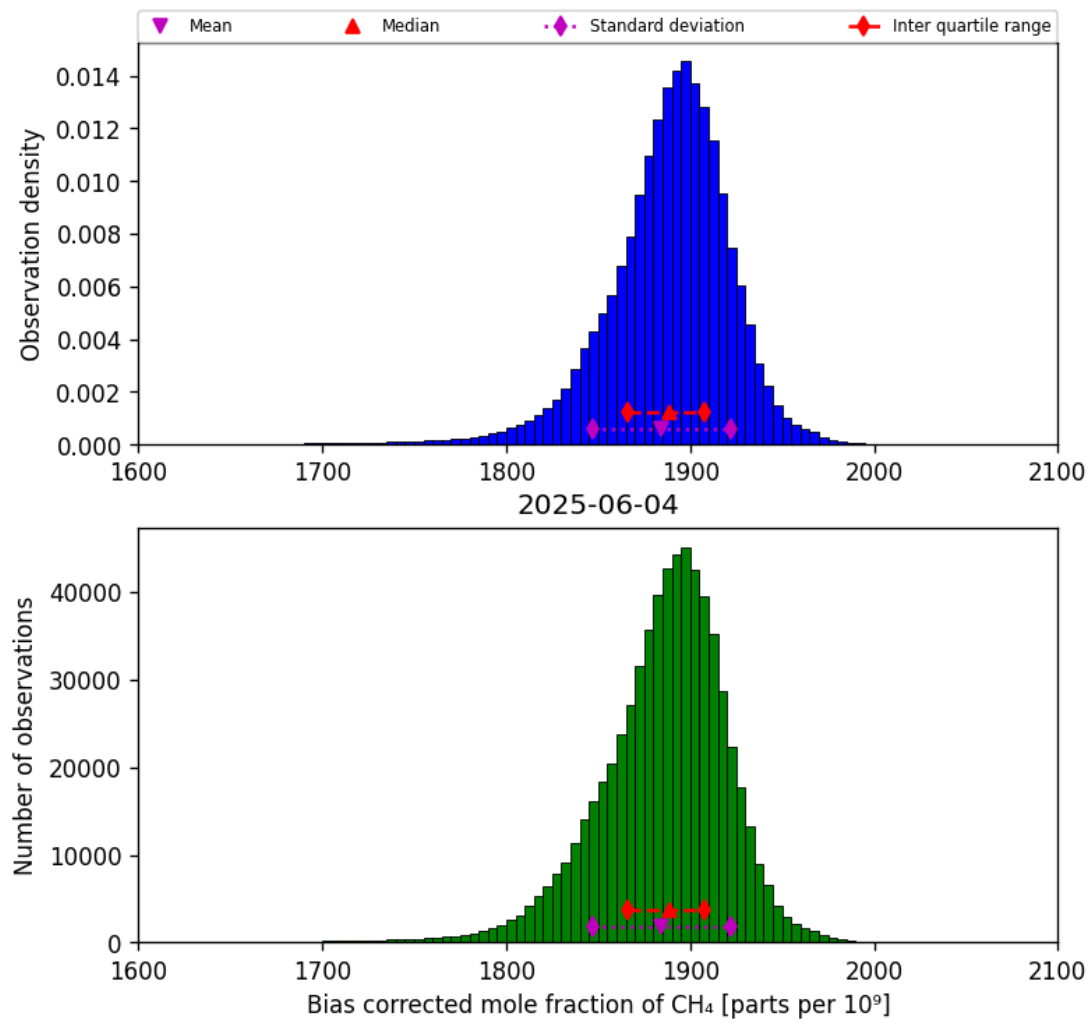
Figure 25: Histogram of “Bias corrected mole fraction of CH 4 ” for 2025-06-03 to 2025-06-05
