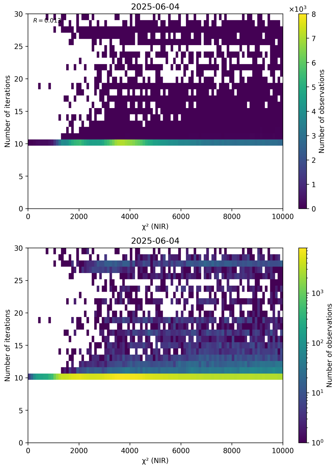
Figure 46: Scatter density plot of “ \chi^2 (NIR)” against “Number of iterations” for 2025-06-03 to 2025-06-05.
