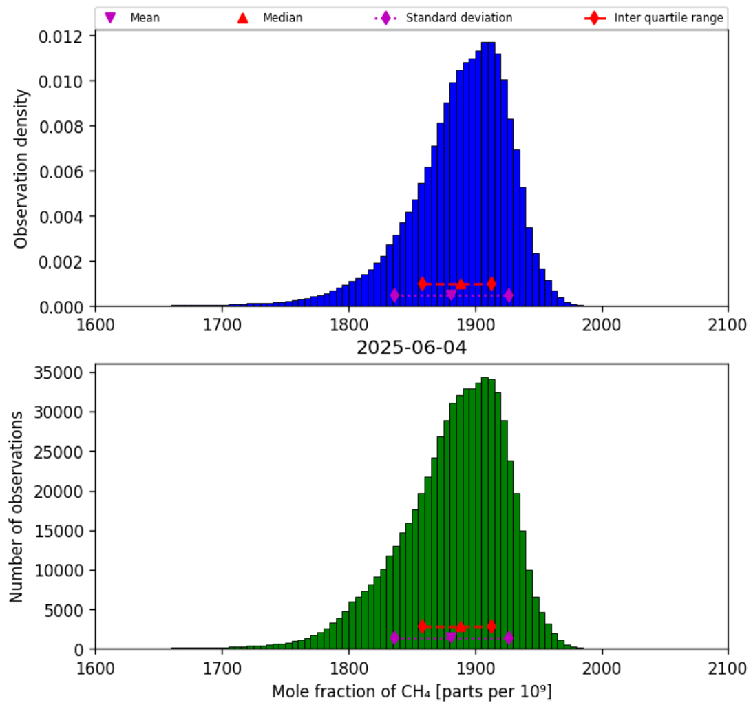
Figure 23: Histogram of “Mole fraction of CH 4 ” for 2025-06-03 to 2025-06-05
