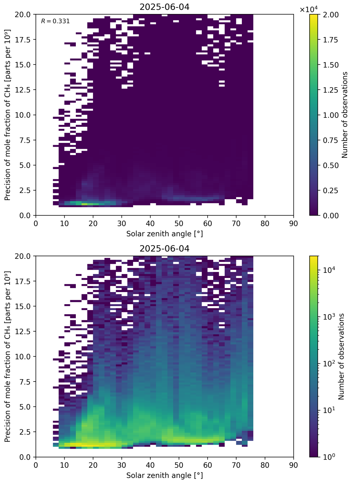
Figure 101: Scatter density plot of “Solar zenith angle” against “Precision of mole fraction of CH 4 ” for 2025-06-03 to 2025-06-05.
