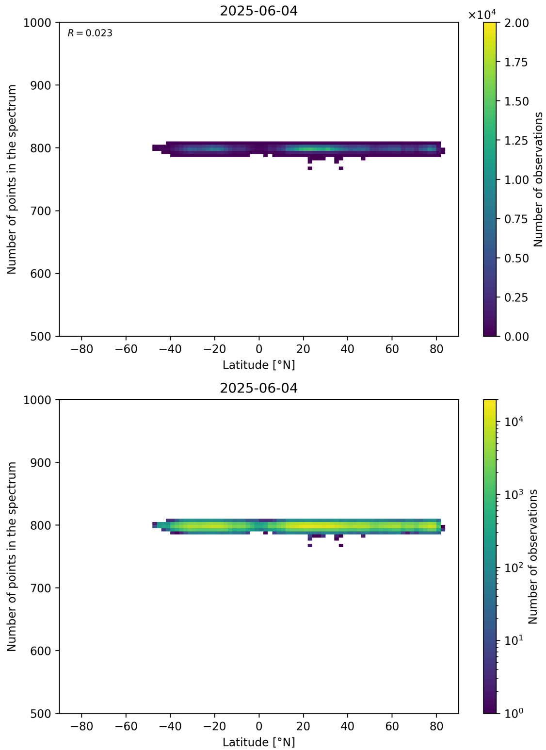
Figure 61: Scatter density plot of “Latitude” against “Number of points in the spectrum” for 2025-06-03 to 2025-06-05.
