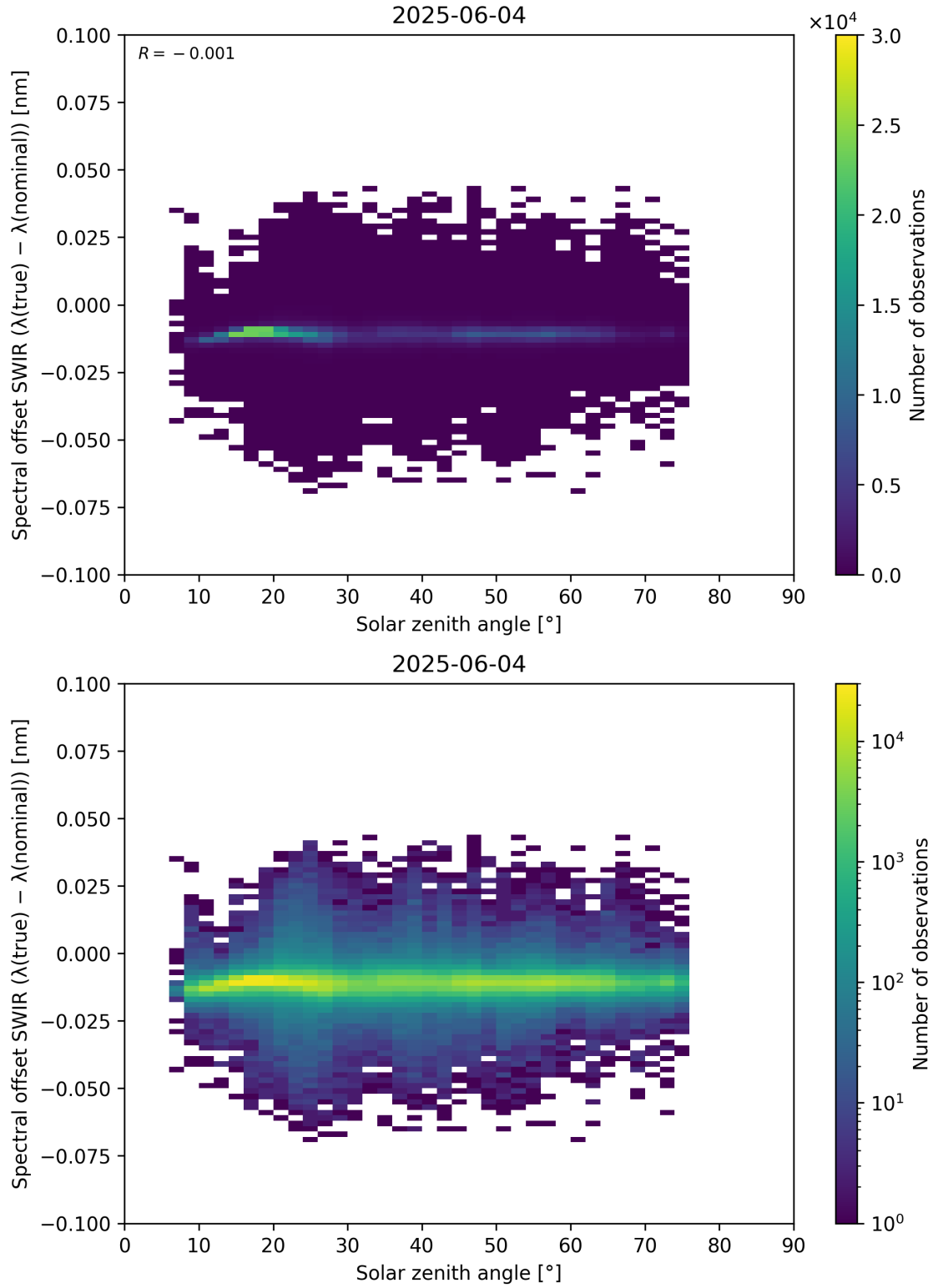
Figure 104: Scatter density plot of “Solar zenith angle” against “Spectral offset SWIR ( \lambda_{\text{true}} - \lambda_{\text{nominal}} )” for 2025-06-03 to 2025-06-05.
