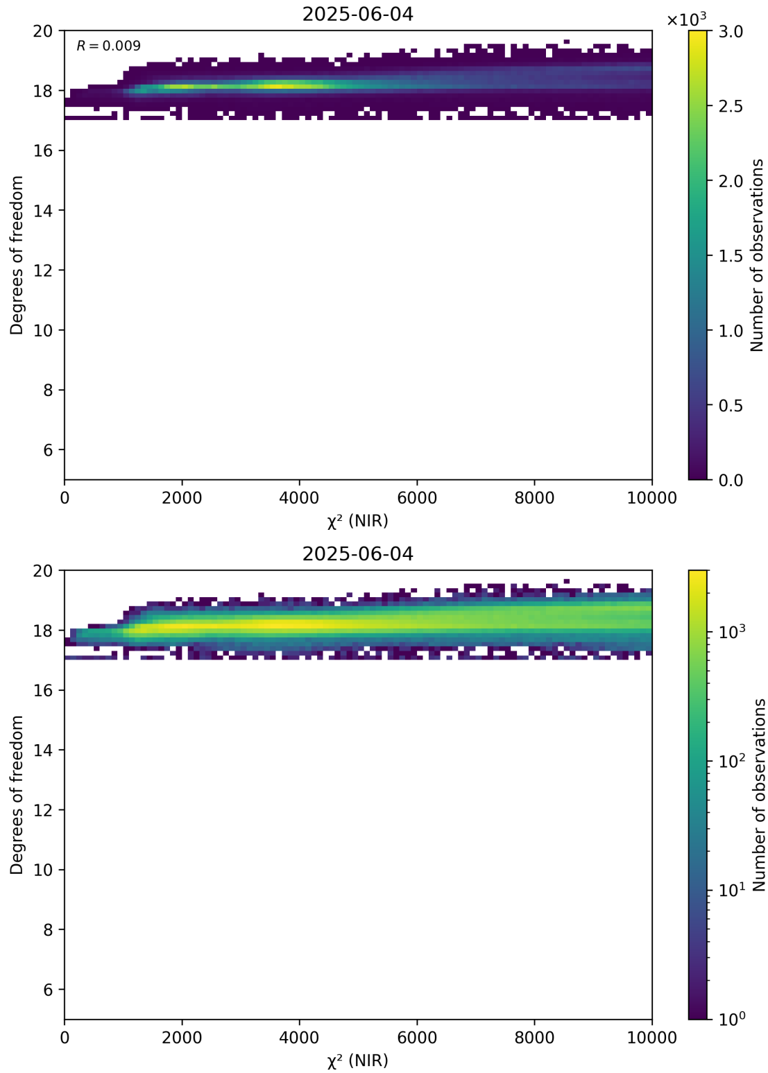
Figure 44: Scatter density plot of “ \chi^2 (NIR)” against “Degrees of freedom” for 2025-06-03 to 2025-06-05.
