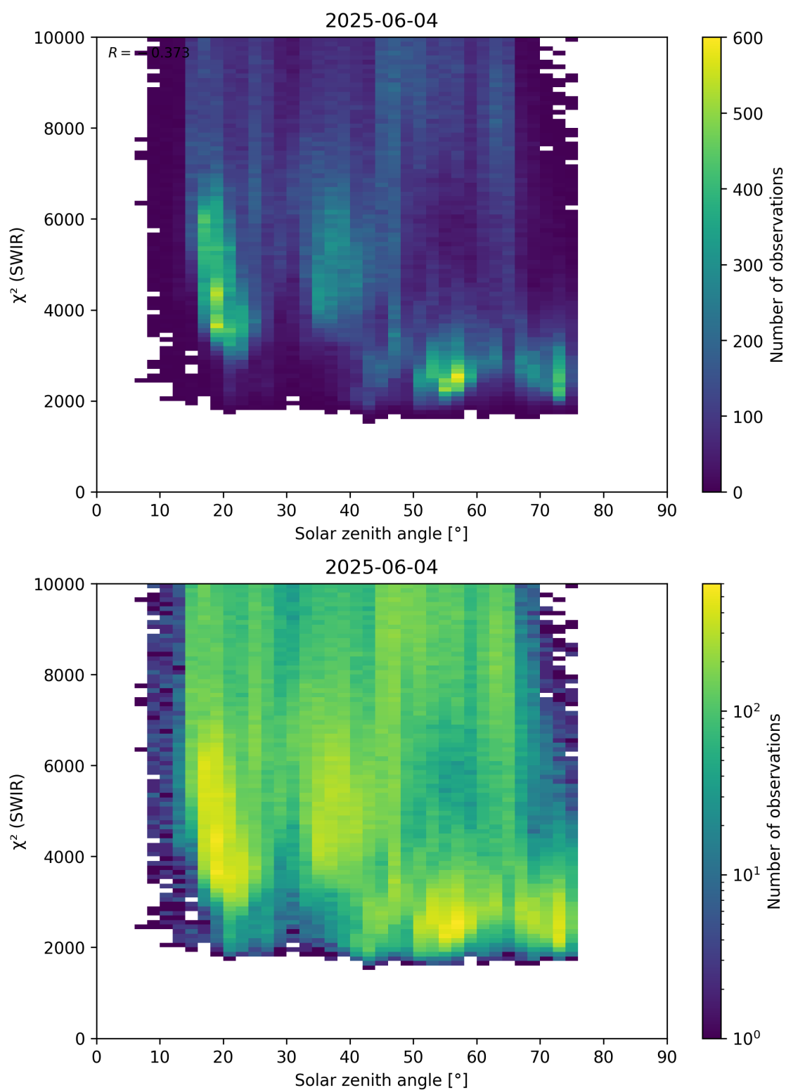
Figure 95: Scatter density plot of “Solar zenith angle” against “ \chi^2 (SWIR)” for 2025-06-03 to 2025-06-05.
