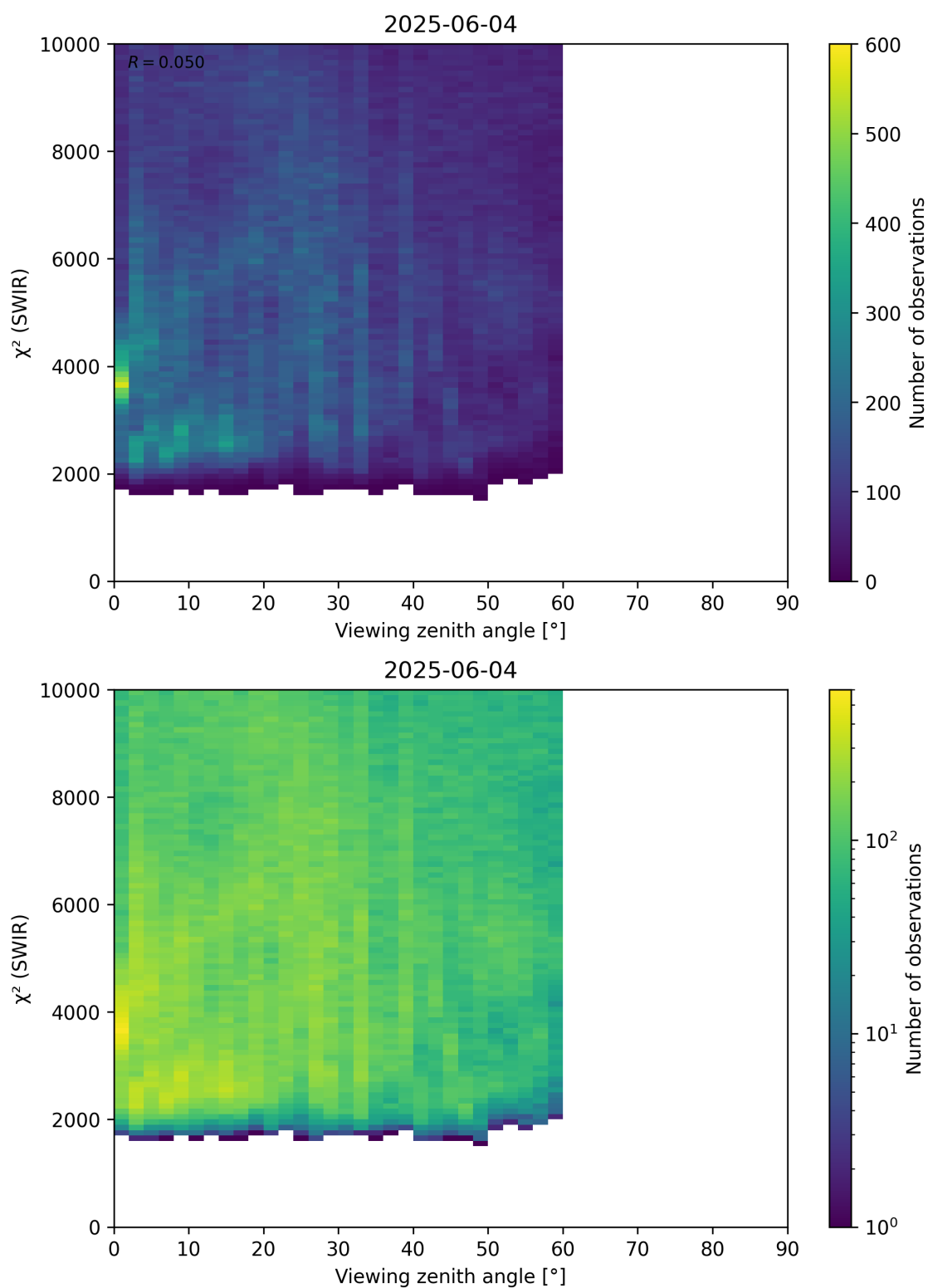
Figure 106: Scatter density plot of “Viewing zenith angle” against “ \chi^2 (SWIR)” for 2025-06-03 to 2025-06-05.
