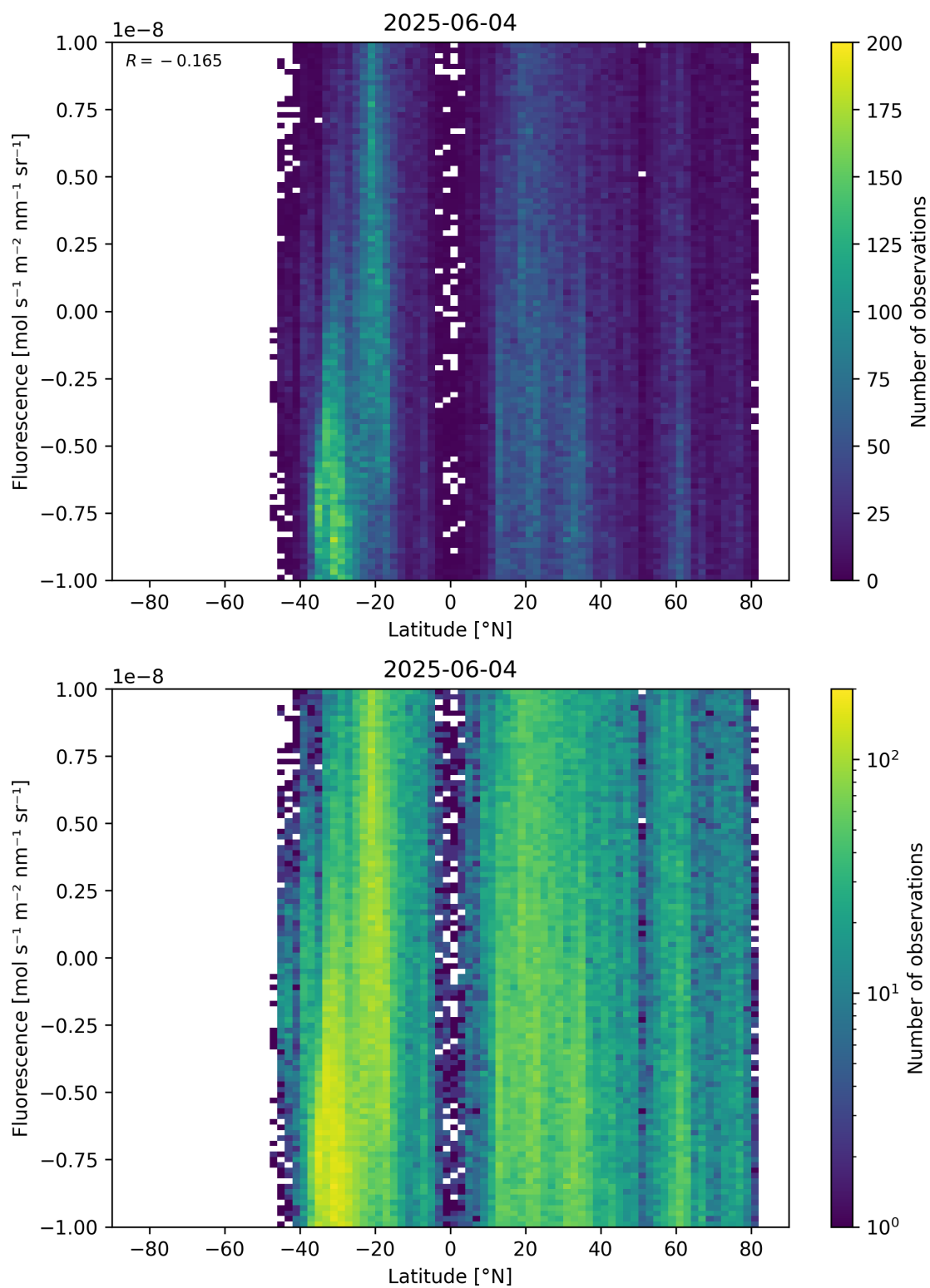
Figure 56: Scatter density plot of “Latitude” against “Fluorescence” for 2025-06-03 to 2025-06-05.
