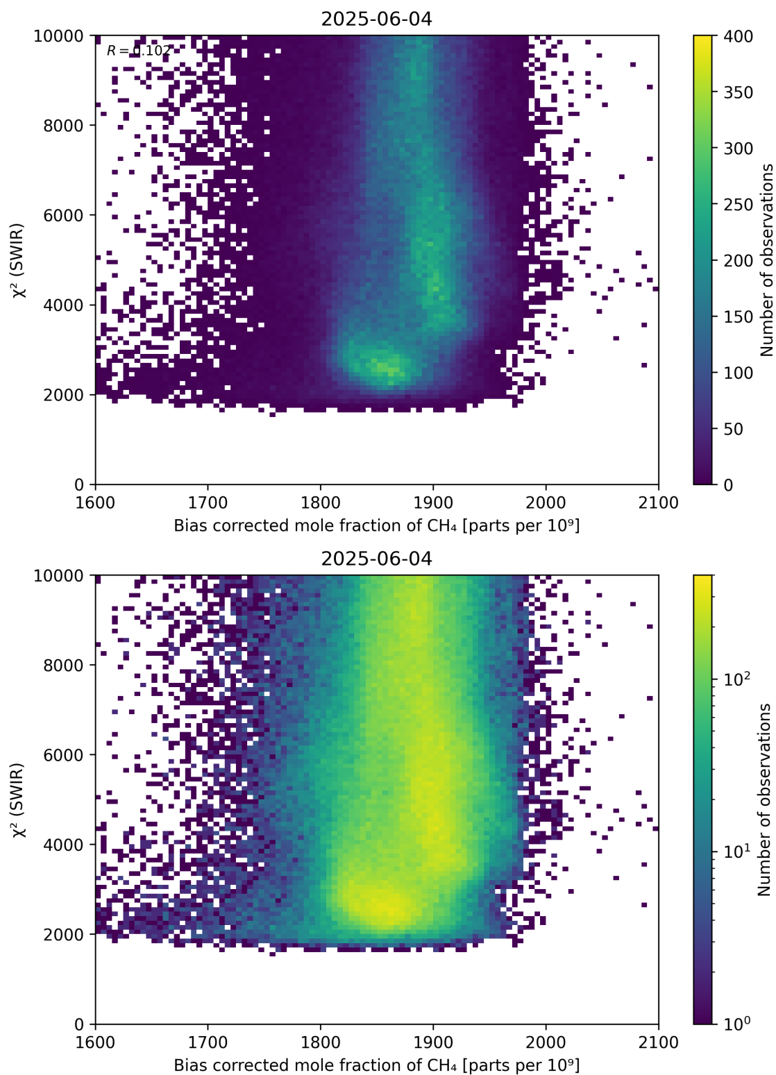
Figure 64: Scatter density plot of “Bias corrected mole fraction of \text{CH}_4 ” against “ \chi^2 (SWIR)” for 2025-06-03 to 2025-06-05.
