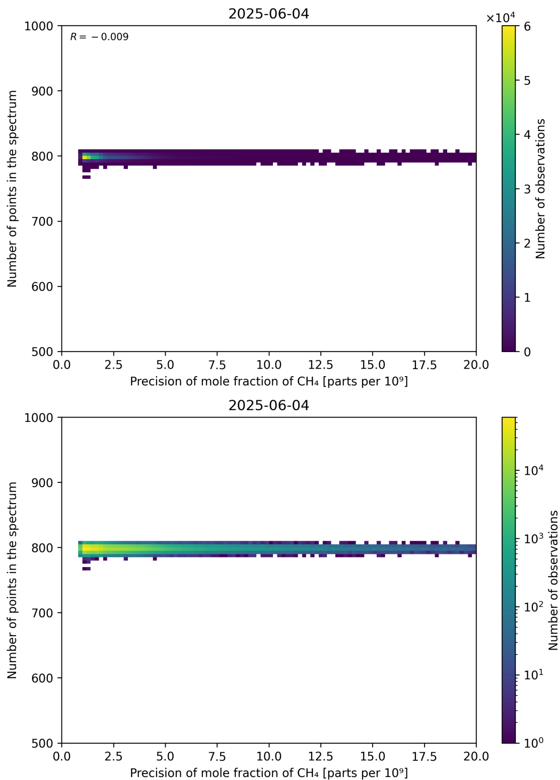
Figure 84: Scatter density plot of “Precision of mole fraction of CH 4 ” against “Number of points in the spectrum” for 2025-06-03 to 2025-06-05.
