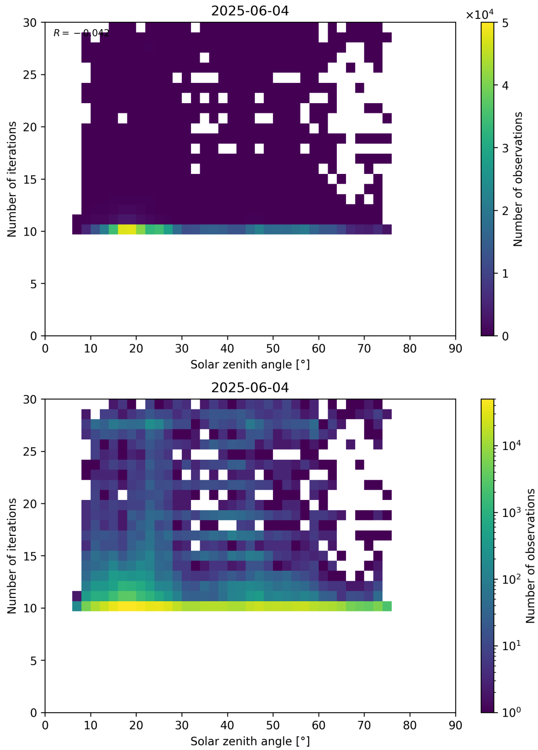
Figure 102: Scatter density plot of “Solar zenith angle” against “Number of iterations” for 2025-06-03 to 2025-06-05.
