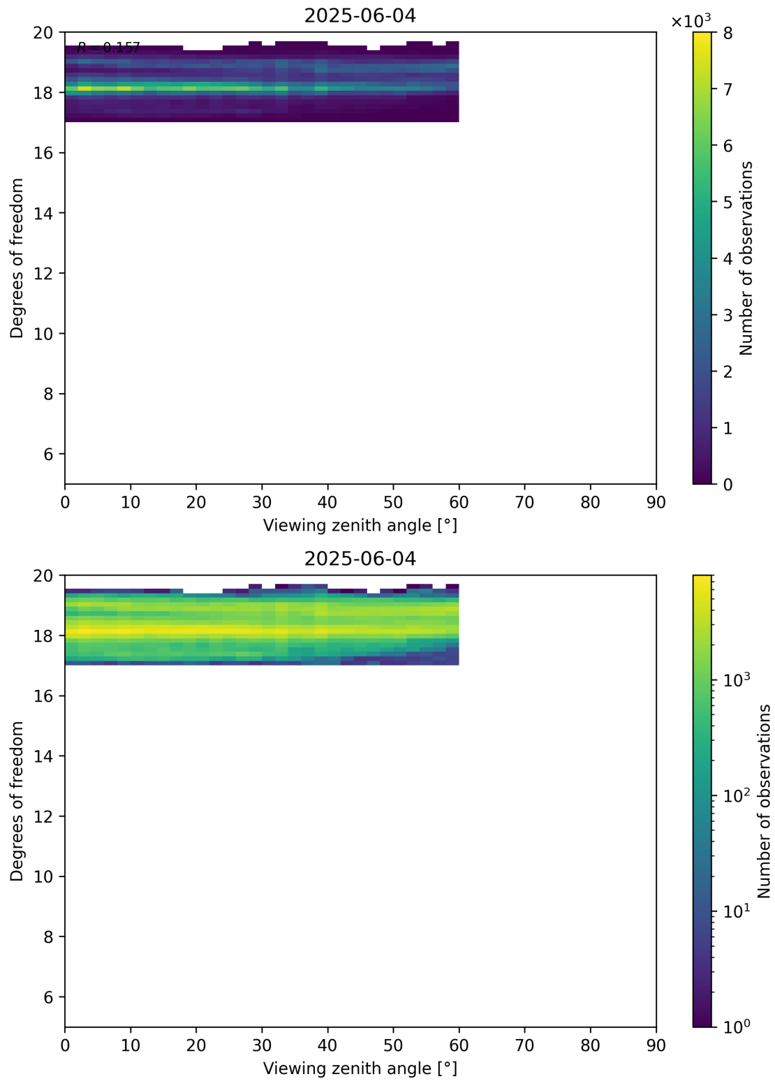
Figure 107: Scatter density plot of “Viewing zenith angle” against “Degrees of freedom” for 2025-06-03 to 2025-06-05.
