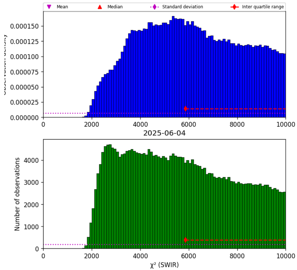
Figure 28: Histogram of “ \chi^2 (SWIR)” for 2025-06-03 to 2025-06-05
