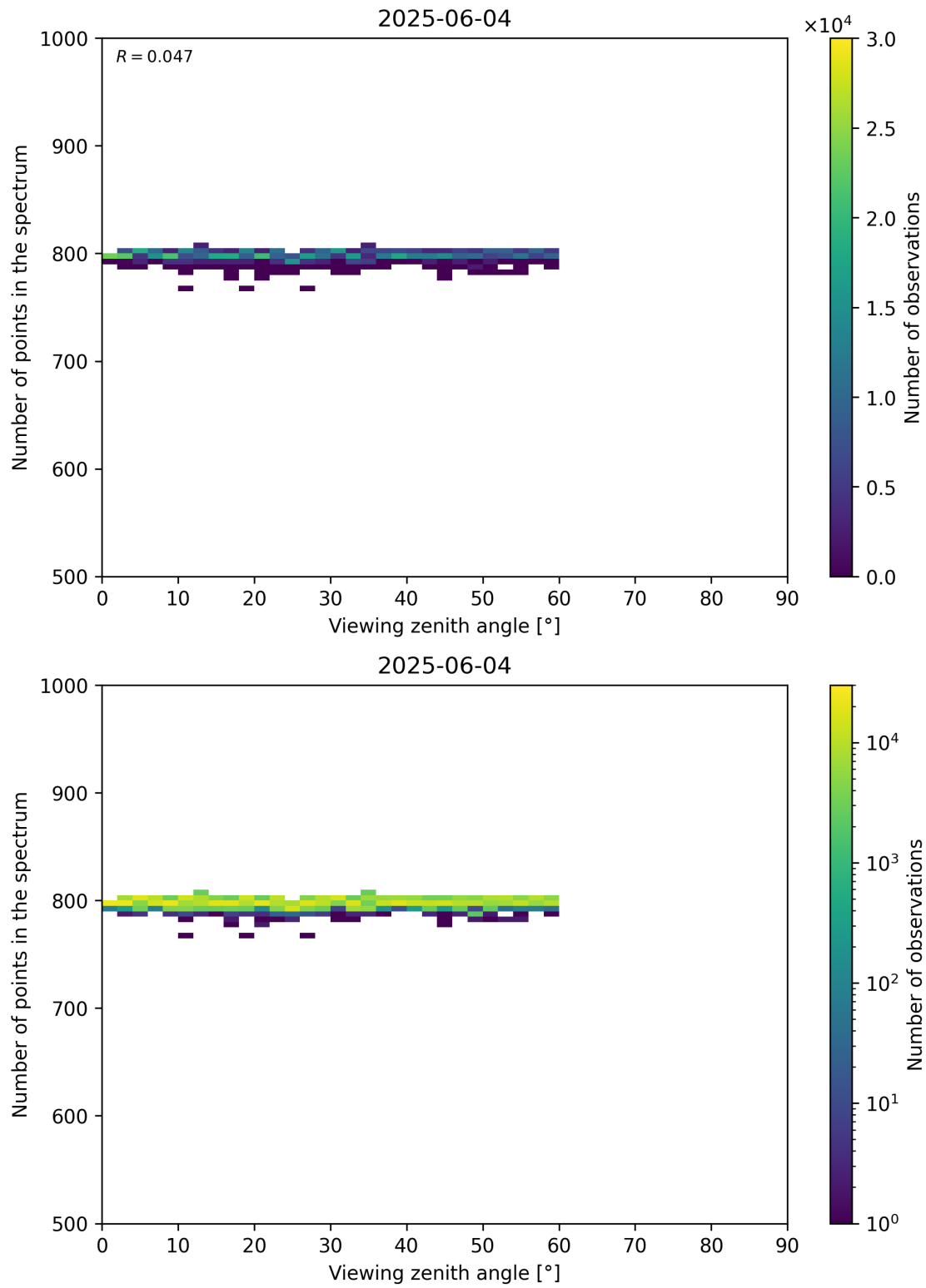
Figure 114: Scatter density plot of “Viewing zenith angle” against “Number of points in the spectrum” for 2025-06-03 to 2025-06-05.
