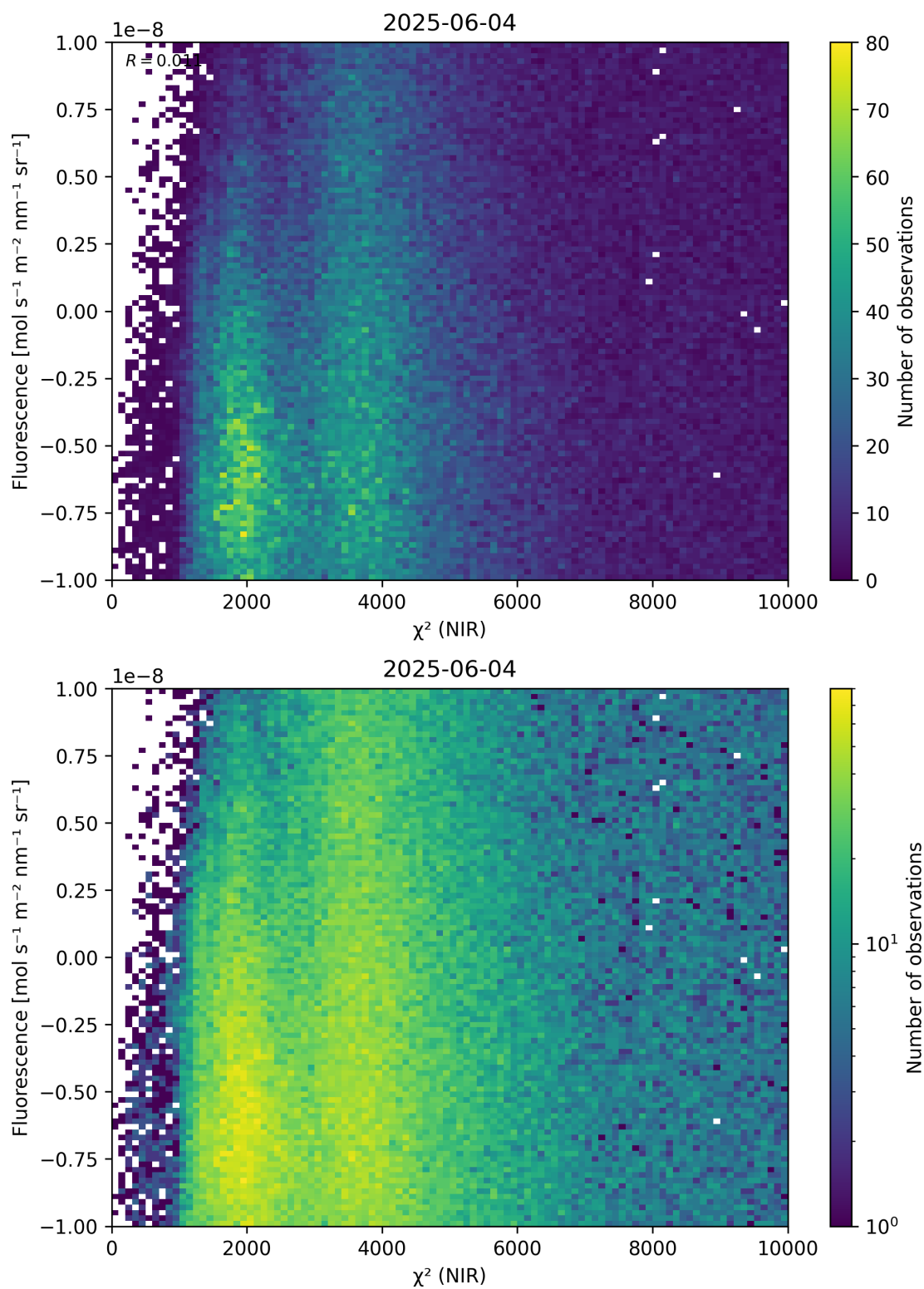
Figure 45: Scatter density plot of “ \chi^2 (NIR)” against “Fluorescence” for 2025-06-03 to 2025-06-05.
