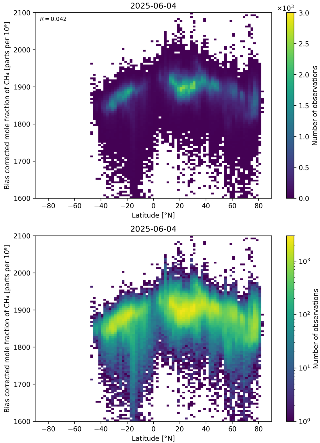
Figure 58: Scatter density plot of “Latitude” against “Bias corrected mole fraction of CH 4 ” for 2025-06-03 to 2025-06-05.
