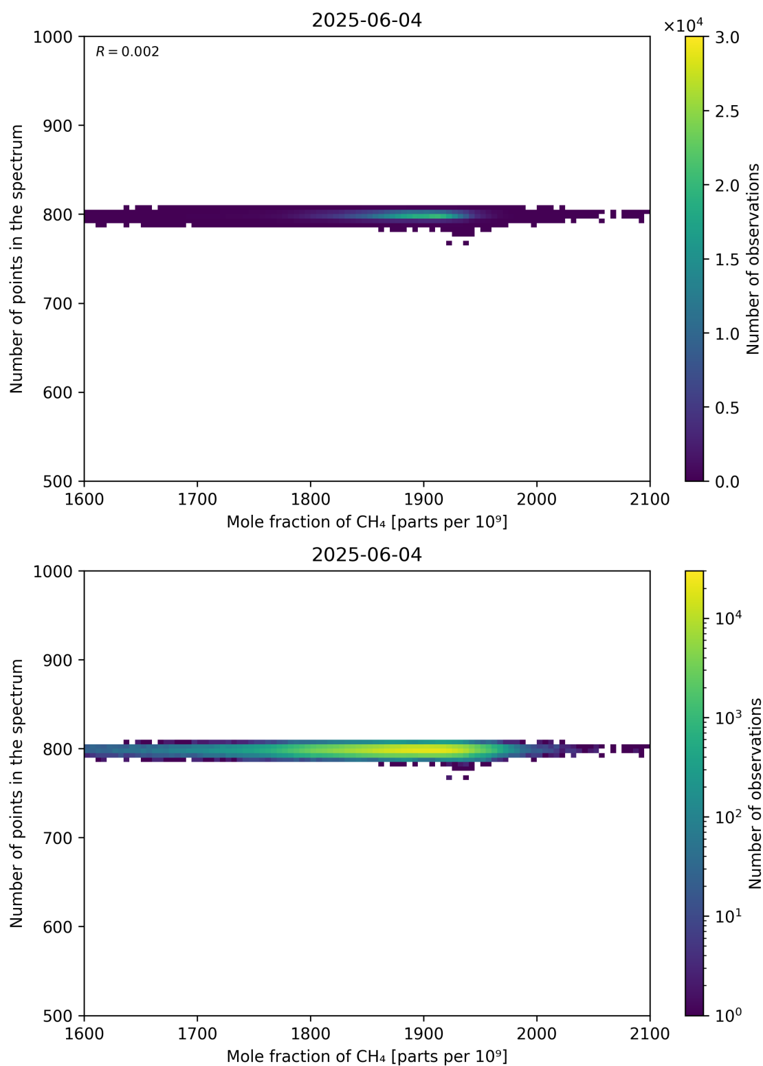
Figure 77: Scatter density plot of “Mole fraction of CH 4 ” against “Number of points in the spectrum” for 2025-06-03 to 2025-06-05.
