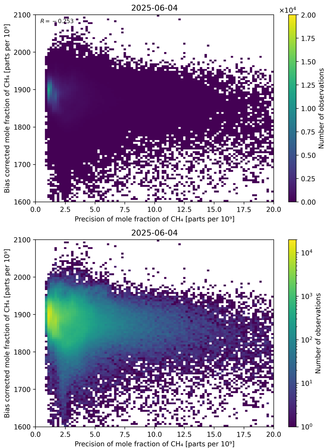
Figure 82: Scatter density plot of “Precision of mole fraction of CH 4 ” against “Bias corrected mole fraction of CH 4 ” for 2025-06-03 to 2025-06-05.
