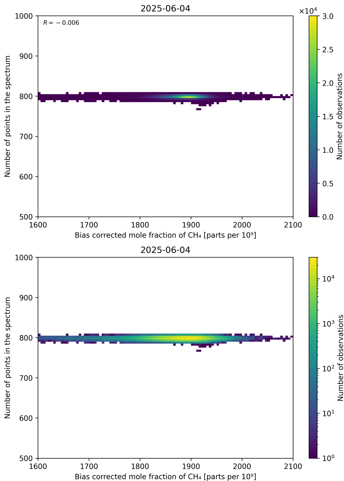
Figure 68: Scatter density plot of “Bias corrected mole fraction of CH 4 ” against “Number of points in the spectrum” for 2025-06-03 to 2025-06-05.
