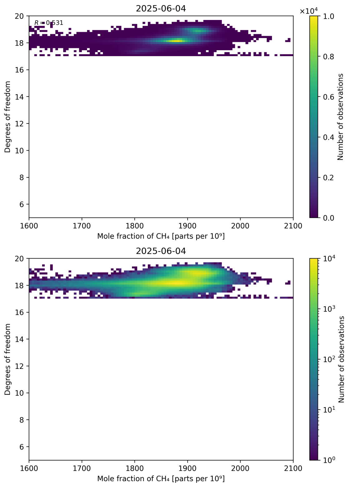
Figure 72: Scatter density plot of “Mole fraction of CH 4 ” against “Degrees of freedom” for 2025-06-03 to 2025-06-05.
