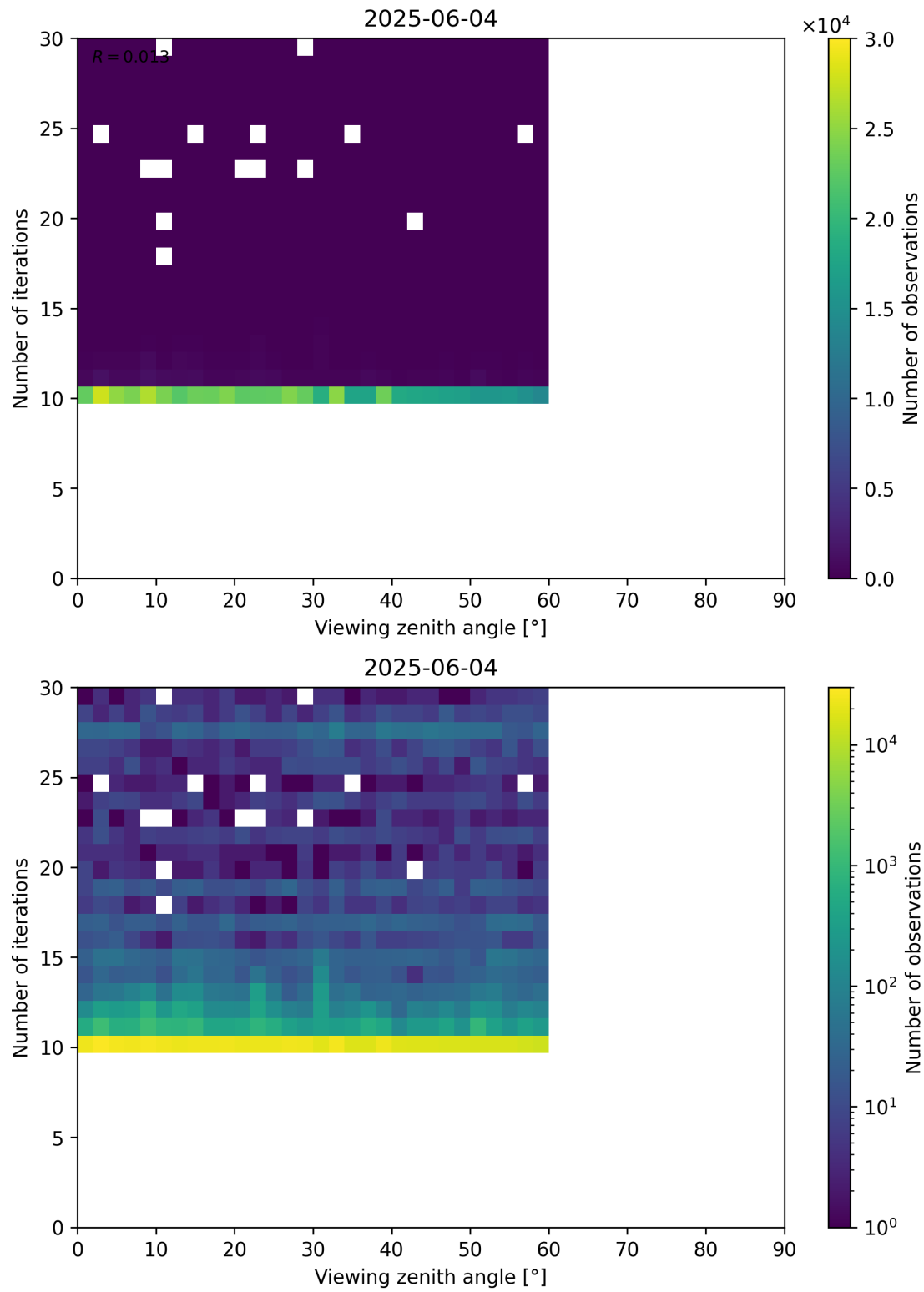
Figure 113: Scatter density plot of “Viewing zenith angle” against “Number of iterations” for 2025-06-03 to 2025-06-05.
