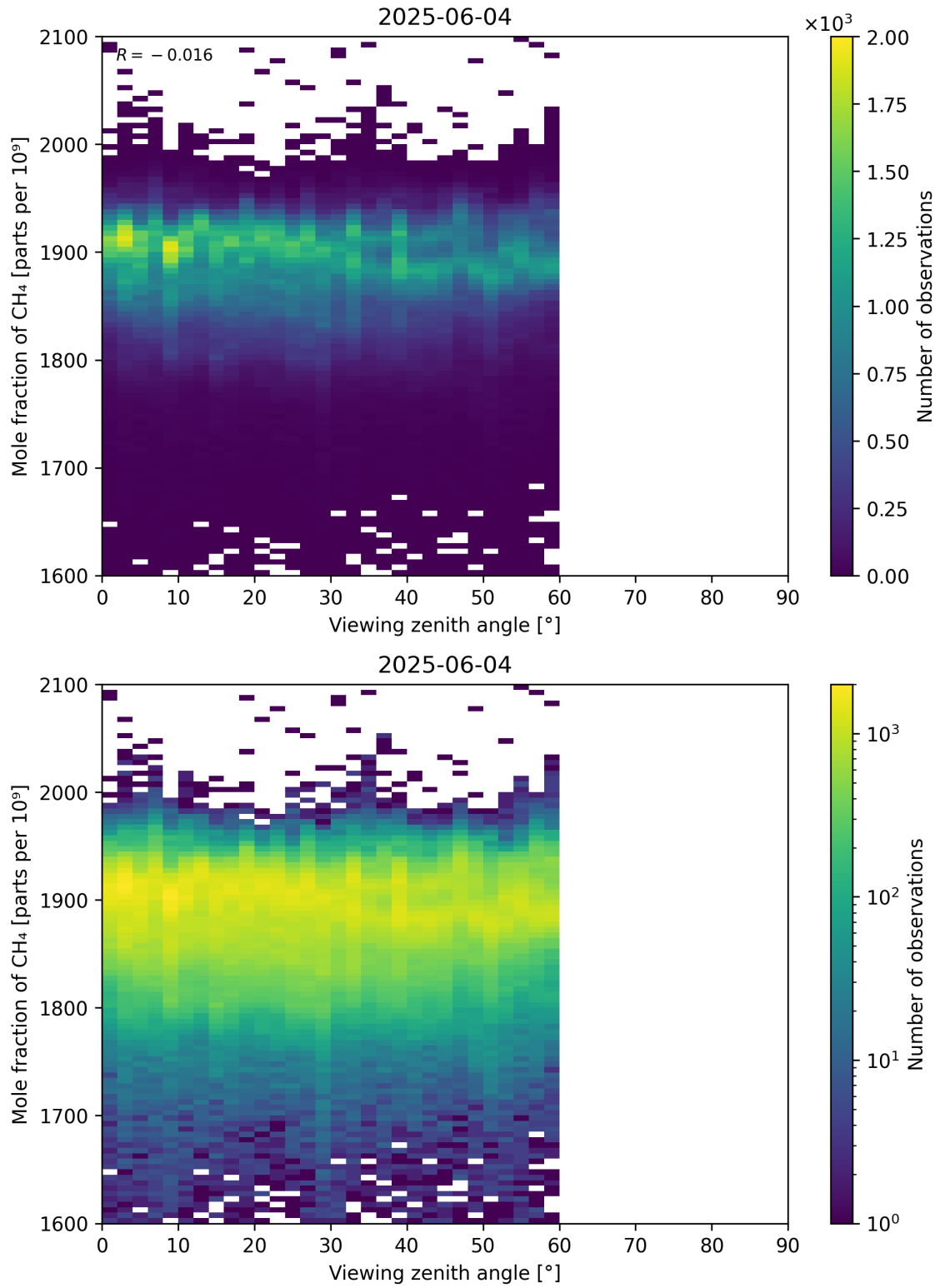
Figure 110: Scatter density plot of “Viewing zenith angle” against “Mole fraction of CH 4 ” for 2025-06-03 to 2025-06-05.
