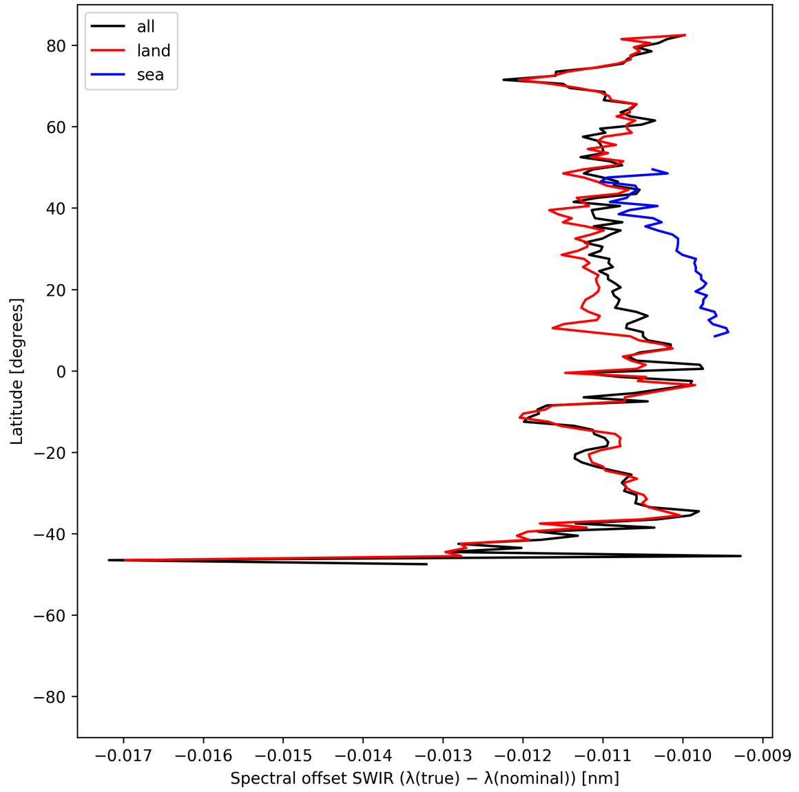
Figure 16: Zonal average of “Spectral offset SWIR ( \lambda_{\text{true}} - \lambda_{\text{nominal}} )” for 2025-06-03 to 2025-06-05.
