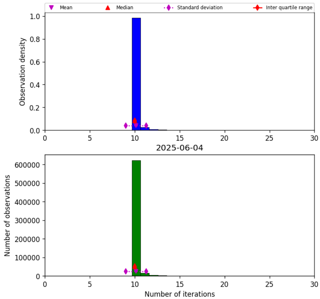
Figure 31: Histogram of “Number of iterations” for 2025-06-03 to 2025-06-05
