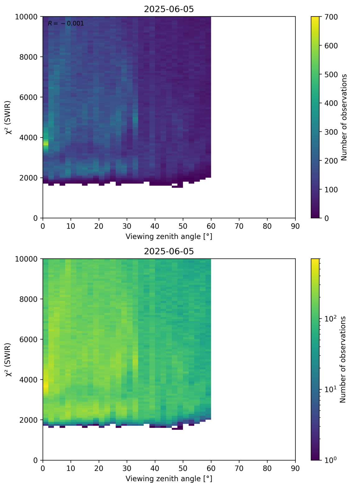
Figure 106: Scatter density plot of “Viewing zenith angle” against “ \chi^2 (SWIR)” for 2025-06-04 to 2025-06-06.
