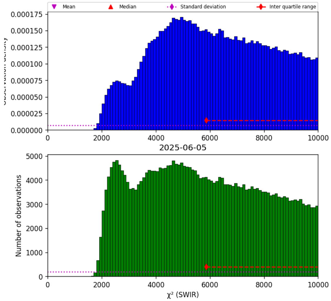
Figure 28: Histogram of “ \chi^2 (SWIR)” for 2025-06-04 to 2025-06-06
