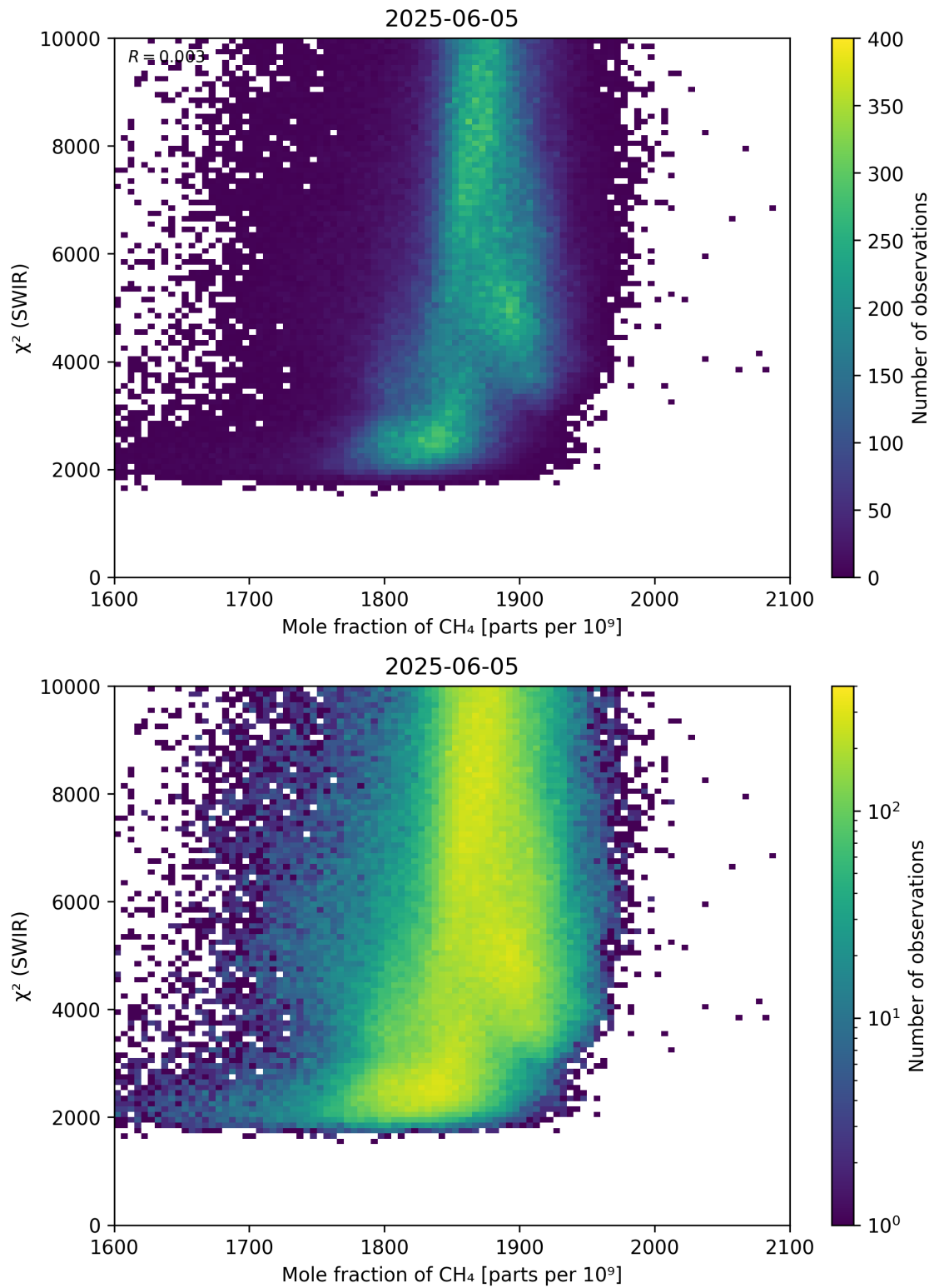
Figure 71: Scatter density plot of “Mole fraction of CH 4 ” against “ \chi^2 (SWIR)” for 2025-06-04 to 2025-06-06.
