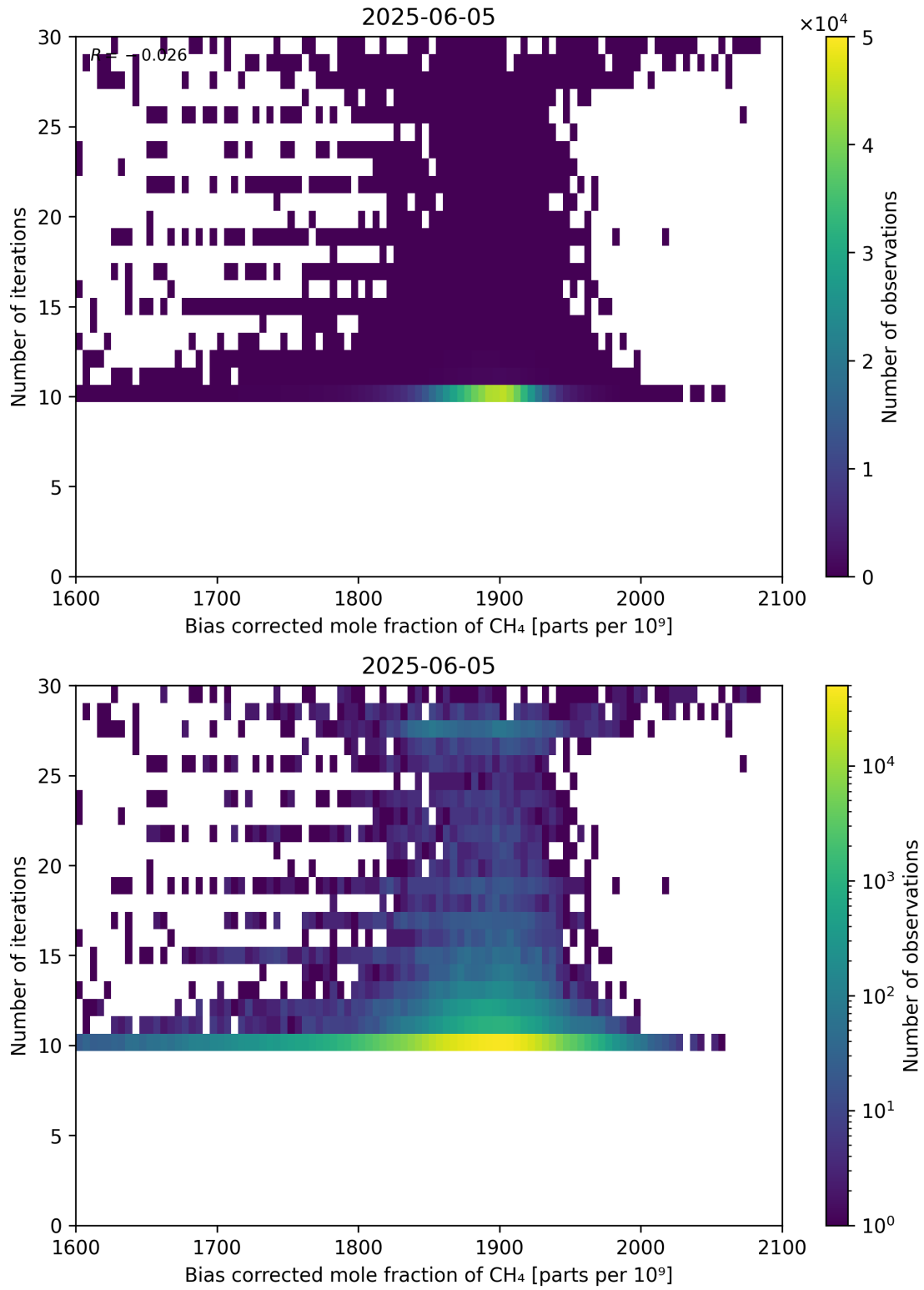
Figure 67: Scatter density plot of “Bias corrected mole fraction of CH 4 ” against “Number of iterations” for 2025-06-04 to 2025-06-06.
