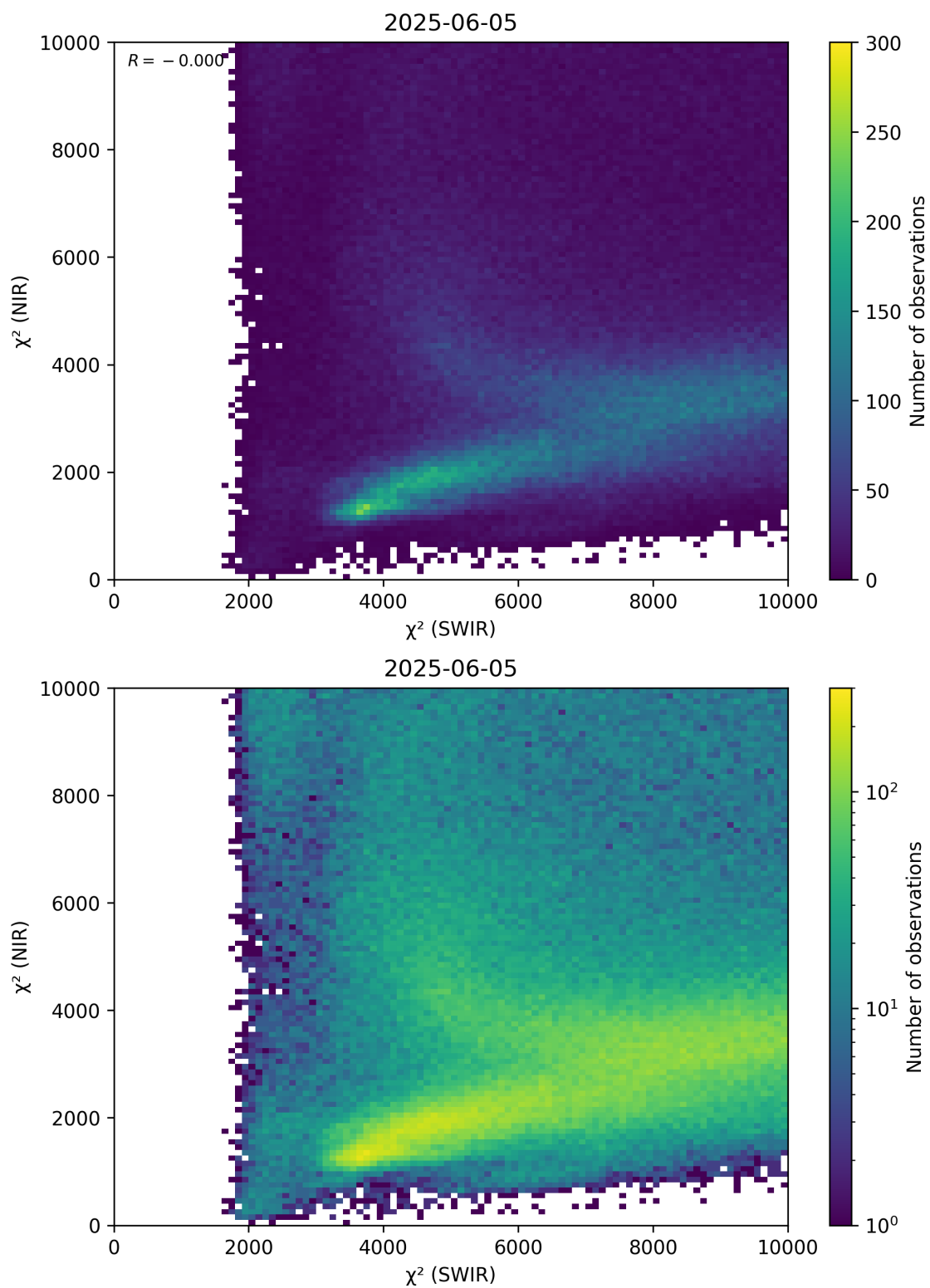
Figure 47: Scatter density plot of “ \chi^2 (SWIR)” against “ \chi^2 (NIR)” for 2025-06-04 to 2025-06-06.
