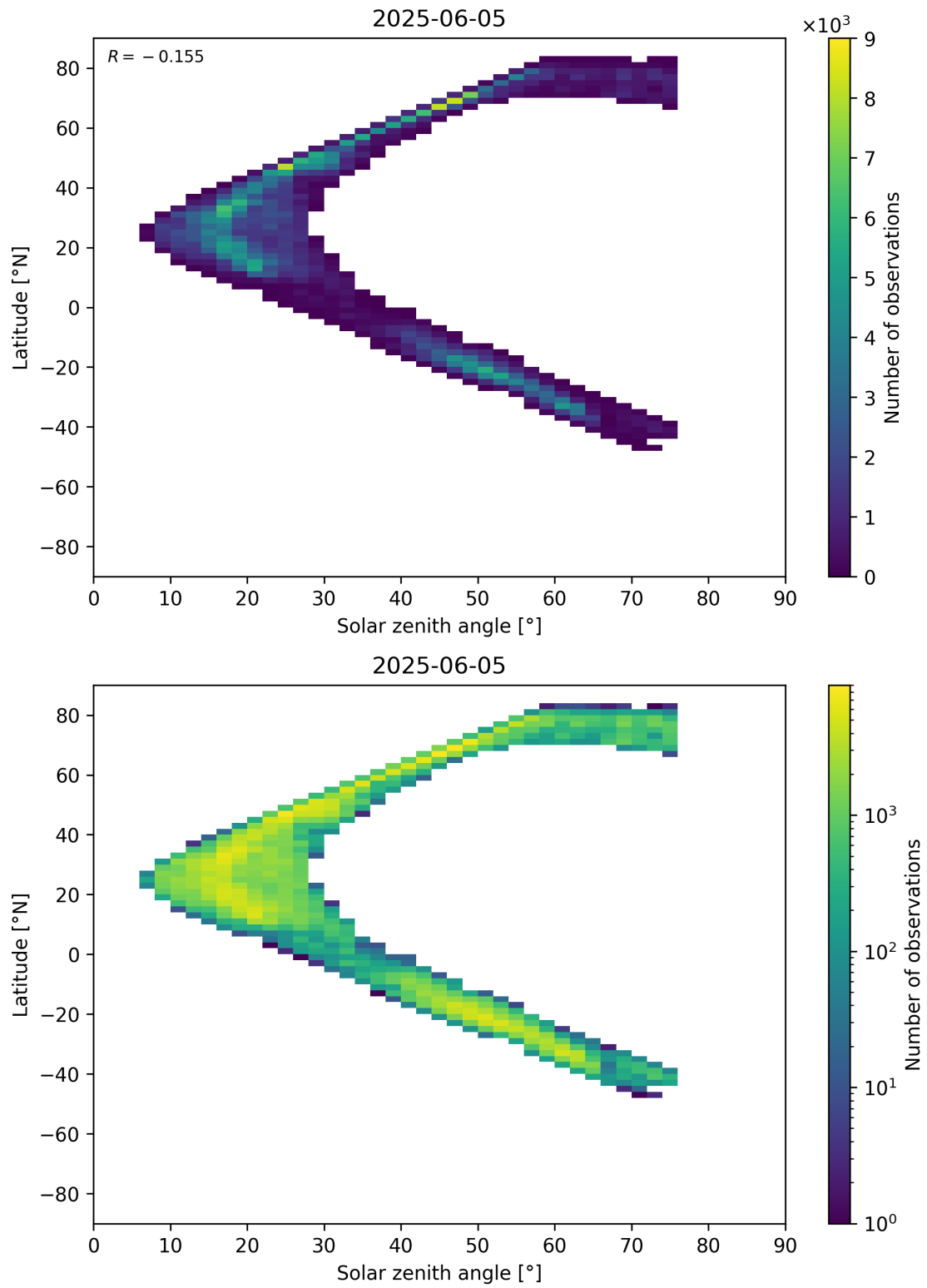
Figure 98: Scatter density plot of “Solar zenith angle” against “Latitude” for 2025-06-04 to 2025-06-06.
