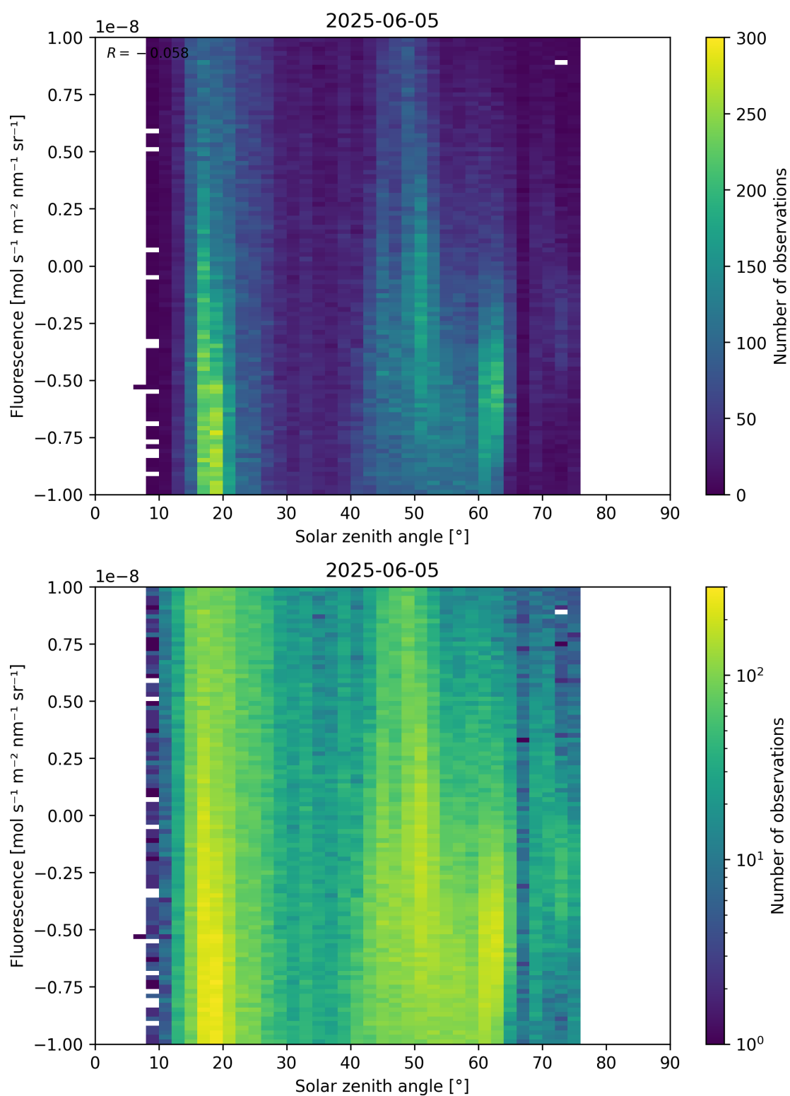
Figure 97: Scatter density plot of “Solar zenith angle” against “Fluorescence” for 2025-06-04 to 2025-06-06.
