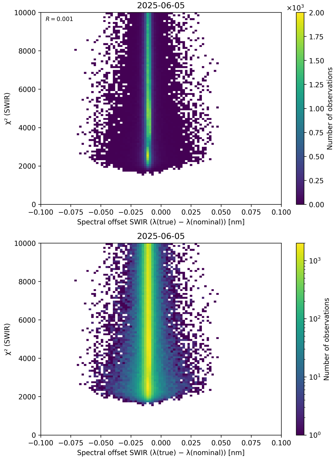
Figure 118: Scatter density plot of “Spectral offset SWIR ( \lambda_{\text{true}} - \lambda_{\text{nominal}} )” against “ \chi^2 (SWIR)” for 2025-06-04 to 2025-06-06.
