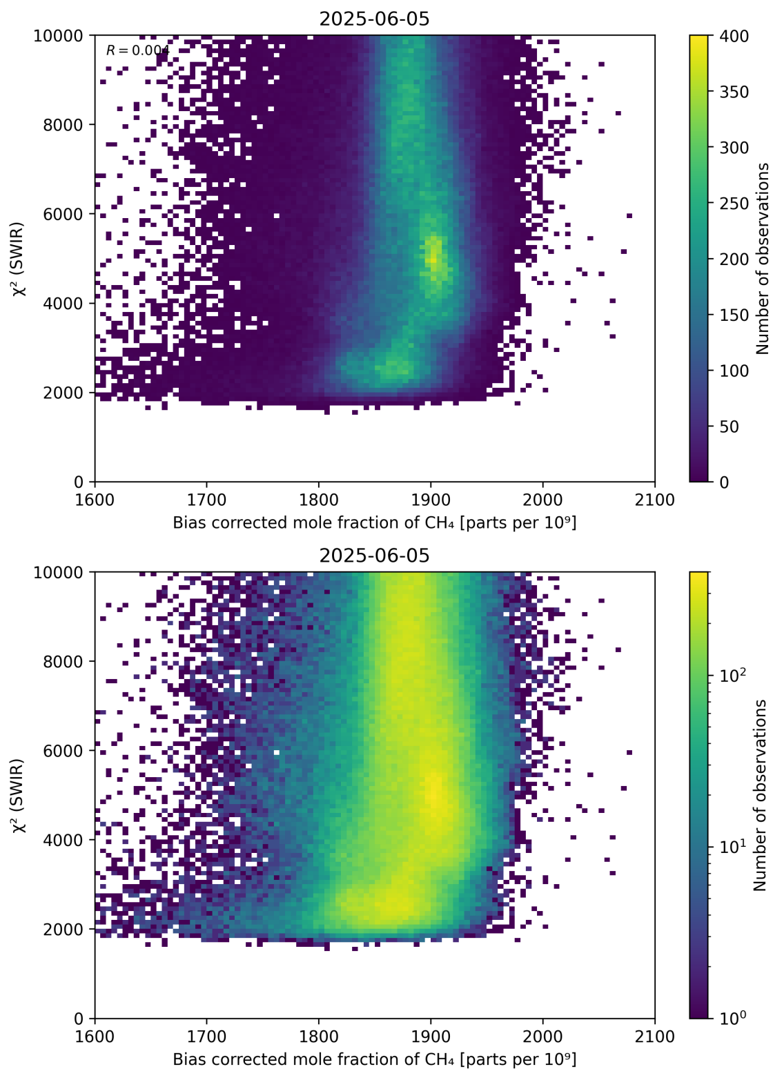
Figure 64: Scatter density plot of “Bias corrected mole fraction of \text{CH}_4 ” against “ \chi^2 (SWIR)” for 2025-06-04 to 2025-06-06.
