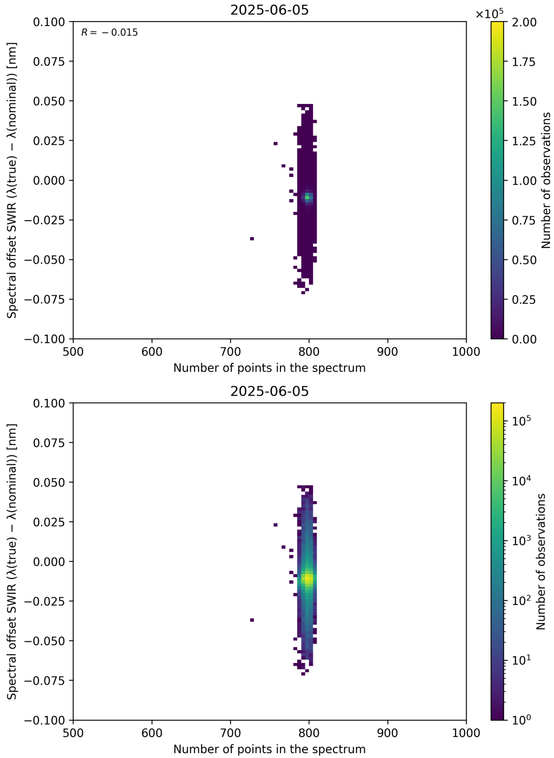
Figure 93: Scatter density plot of “Number of points in the spectrum” against “Spectral offset SWIR ( \lambda_{\text{true}} - \lambda_{\text{nominal}} )” for 2025-06-04 to 2025-06-06.
