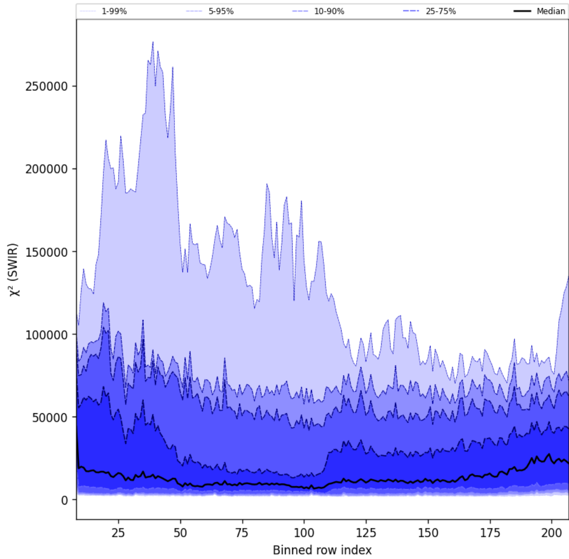
Figure 39: Along track statistics of “ \chi^2 (SWIR)” for 2025-06-04 to 2025-06-06
