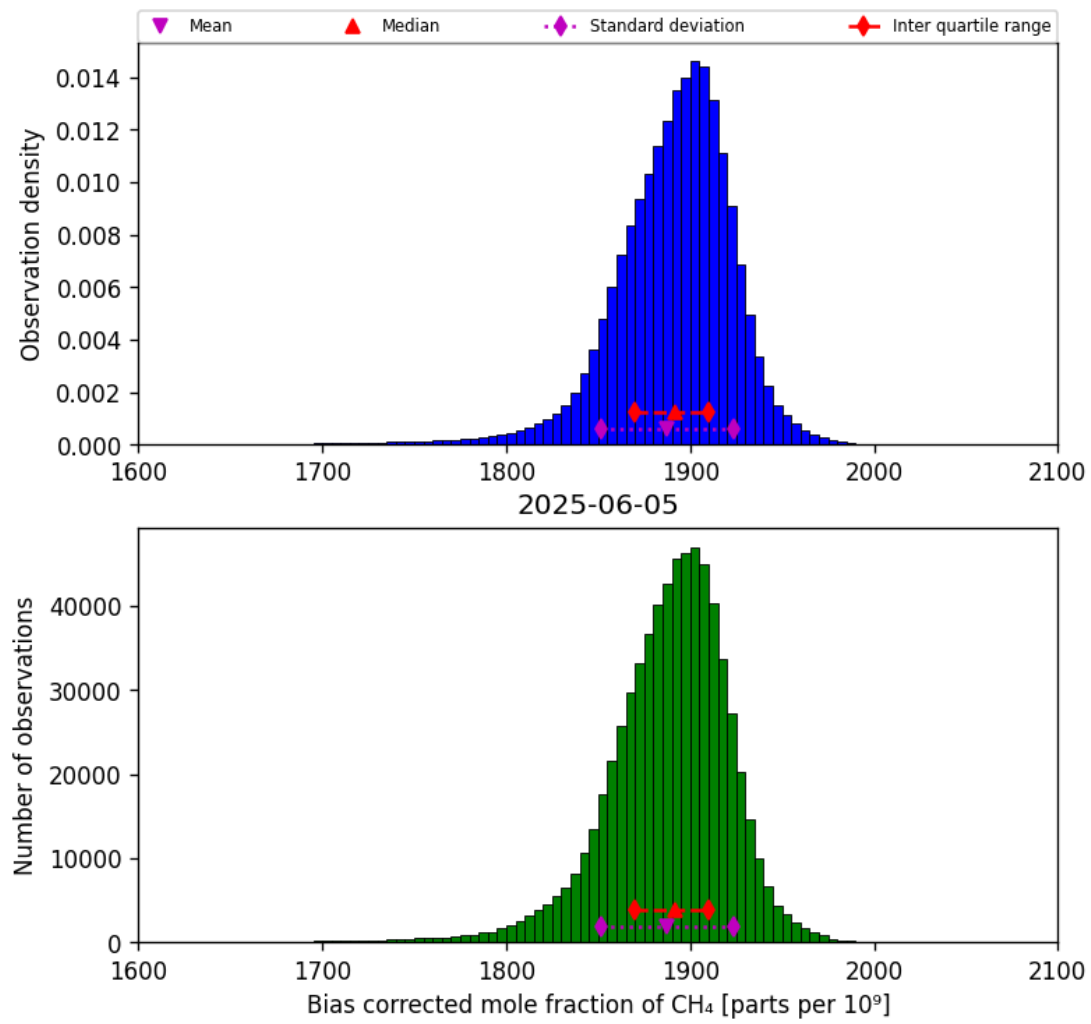
Figure 25: Histogram of “Bias corrected mole fraction of CH 4 ” for 2025-06-04 to 2025-06-06
