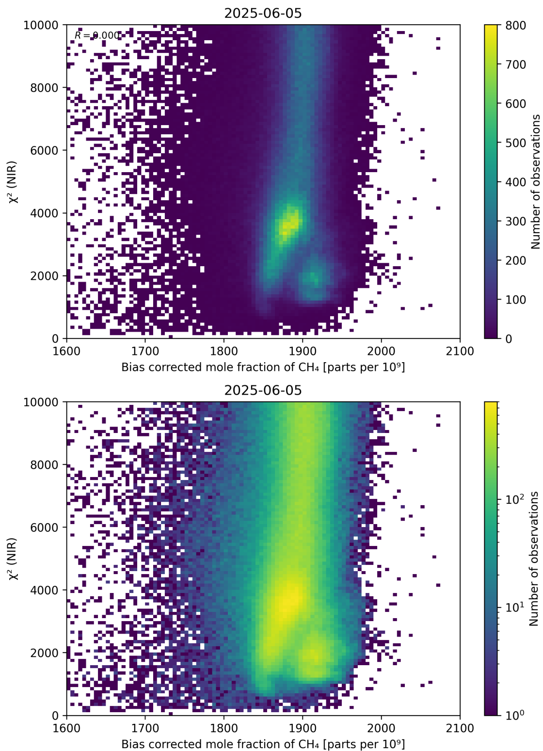
Figure 63: Scatter density plot of “Bias corrected mole fraction of \text{CH}_4 ” against “ \chi^2 (NIR)” for 2025-06-04 to 2025-06-06.
