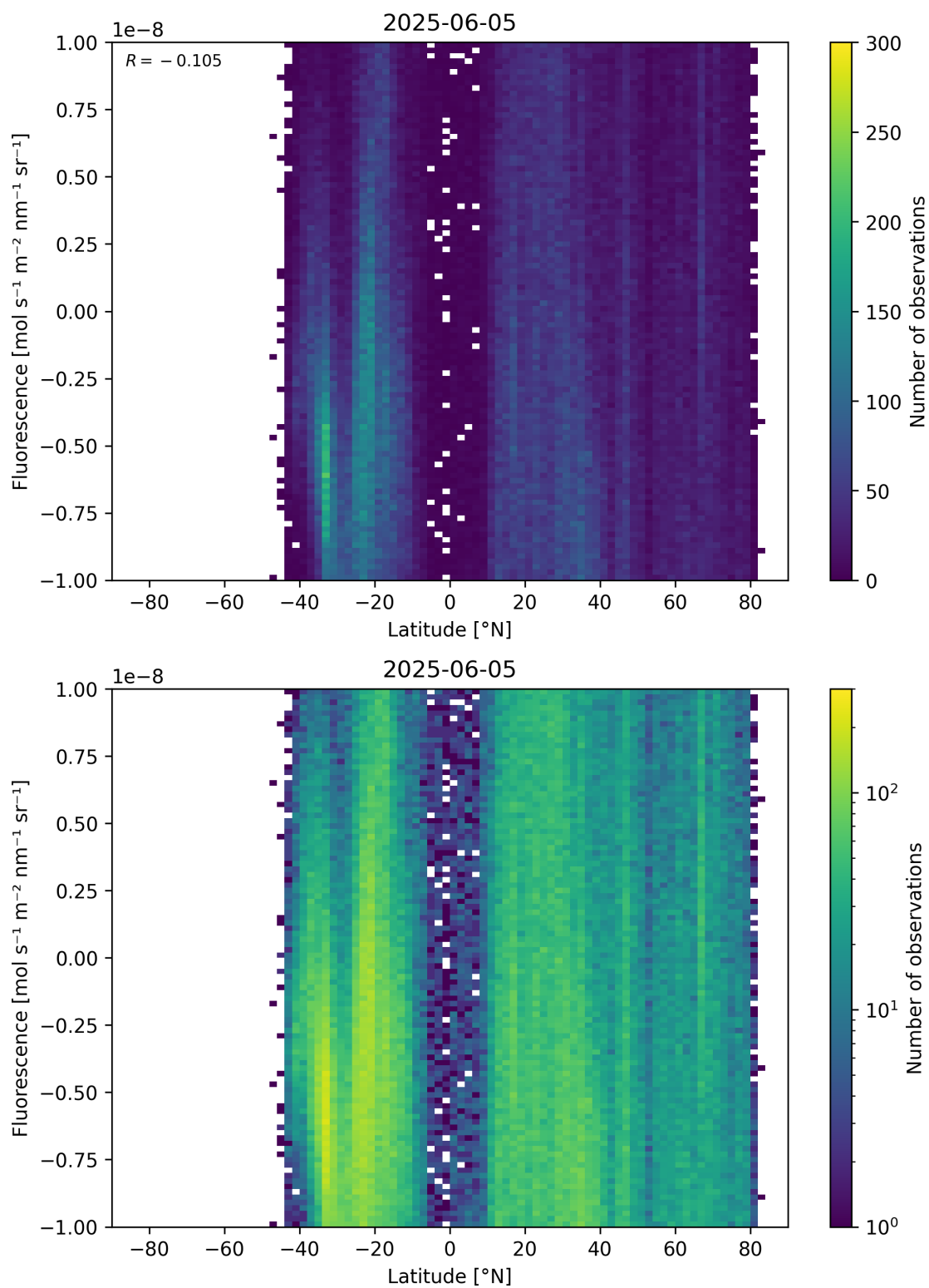
Figure 56: Scatter density plot of “Latitude” against “Fluorescence” for 2025-06-04 to 2025-06-06.
