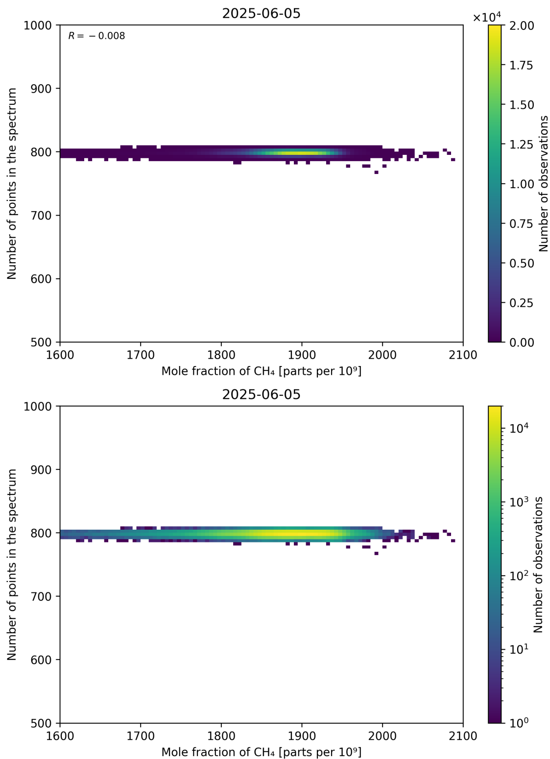
Figure 77: Scatter density plot of “Mole fraction of CH 4 ” against “Number of points in the spectrum” for 2025-06-04 to 2025-06-06.
