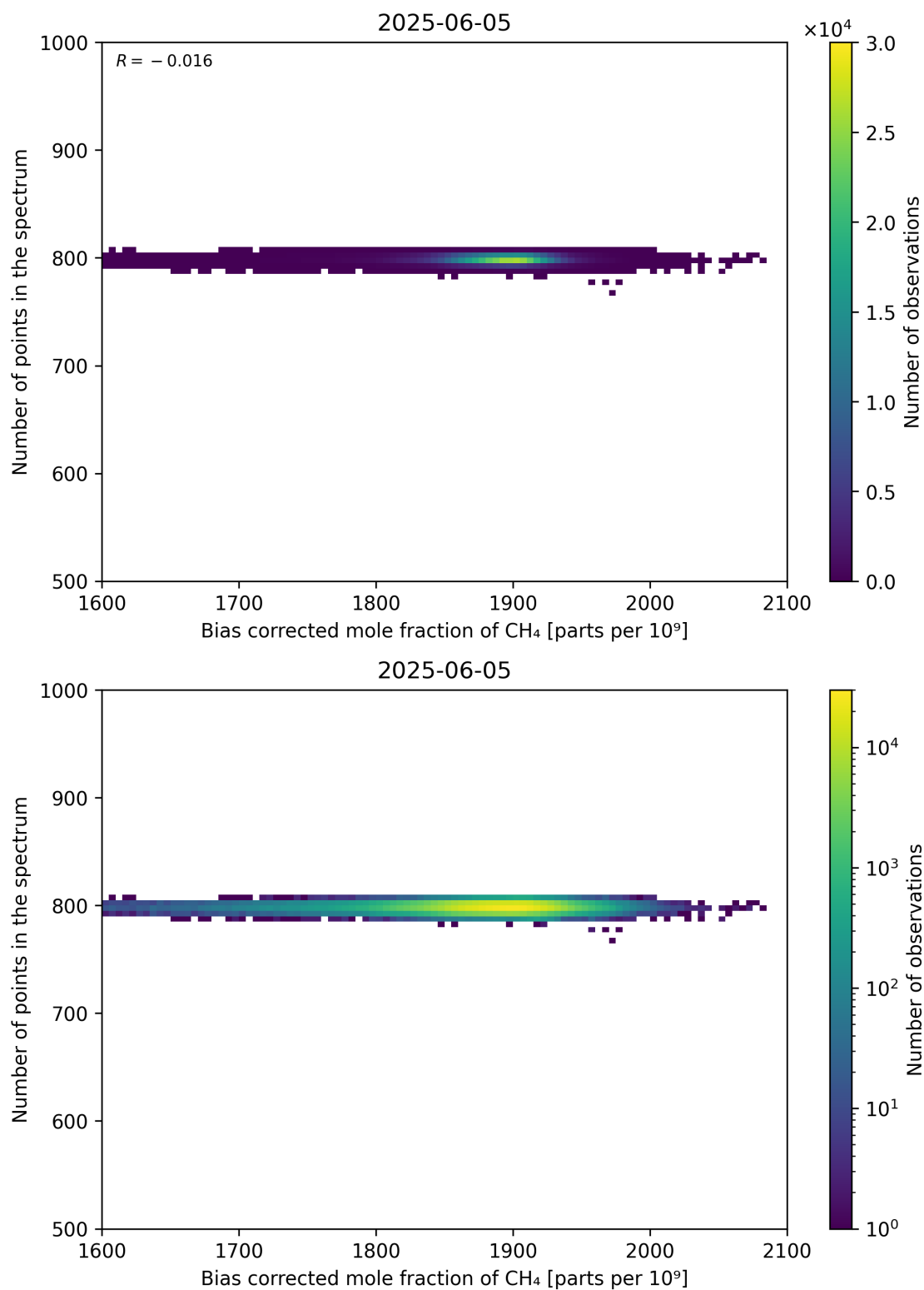
Figure 68: Scatter density plot of “Bias corrected mole fraction of CH 4 ” against “Number of points in the spectrum” for 2025-06-04 to 2025-06-06.
