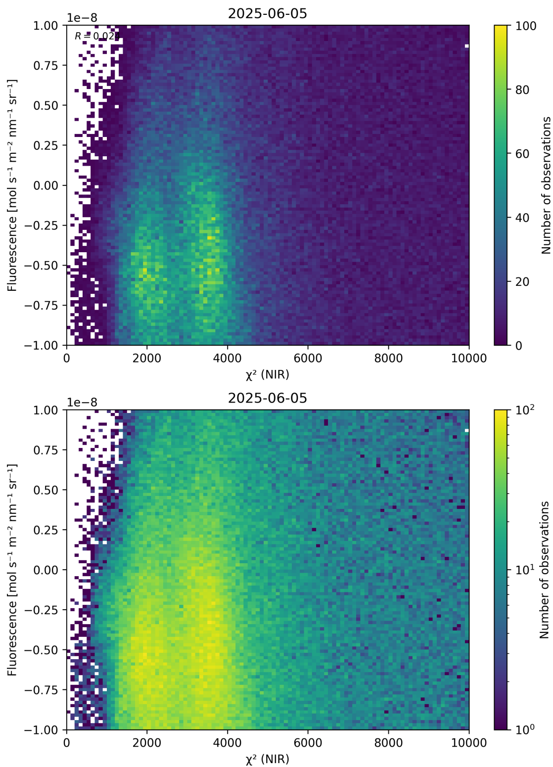
Figure 45: Scatter density plot of “ \chi^2 (NIR)” against “Fluorescence” for 2025-06-04 to 2025-06-06.
