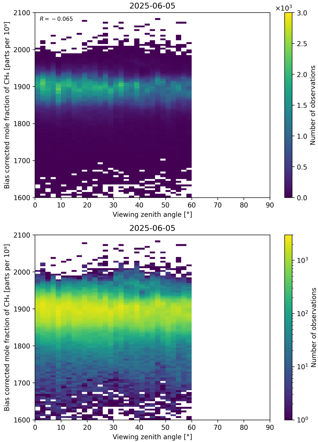
Figure 111: Scatter density plot of “Viewing zenith angle” against “Bias corrected mole fraction of CH 4 ” for 2025-06-04 to 2025-06-06.
