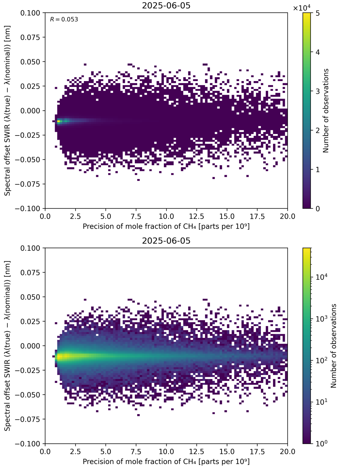
Figure 85: Scatter density plot of “Precision of mole fraction of \text{CH}_4 ” against “Spectral offset SWIR ( \lambda_{\text{true}} - \lambda_{\text{nominal}} )” for 2025-06-04 to 2025-06-06.
