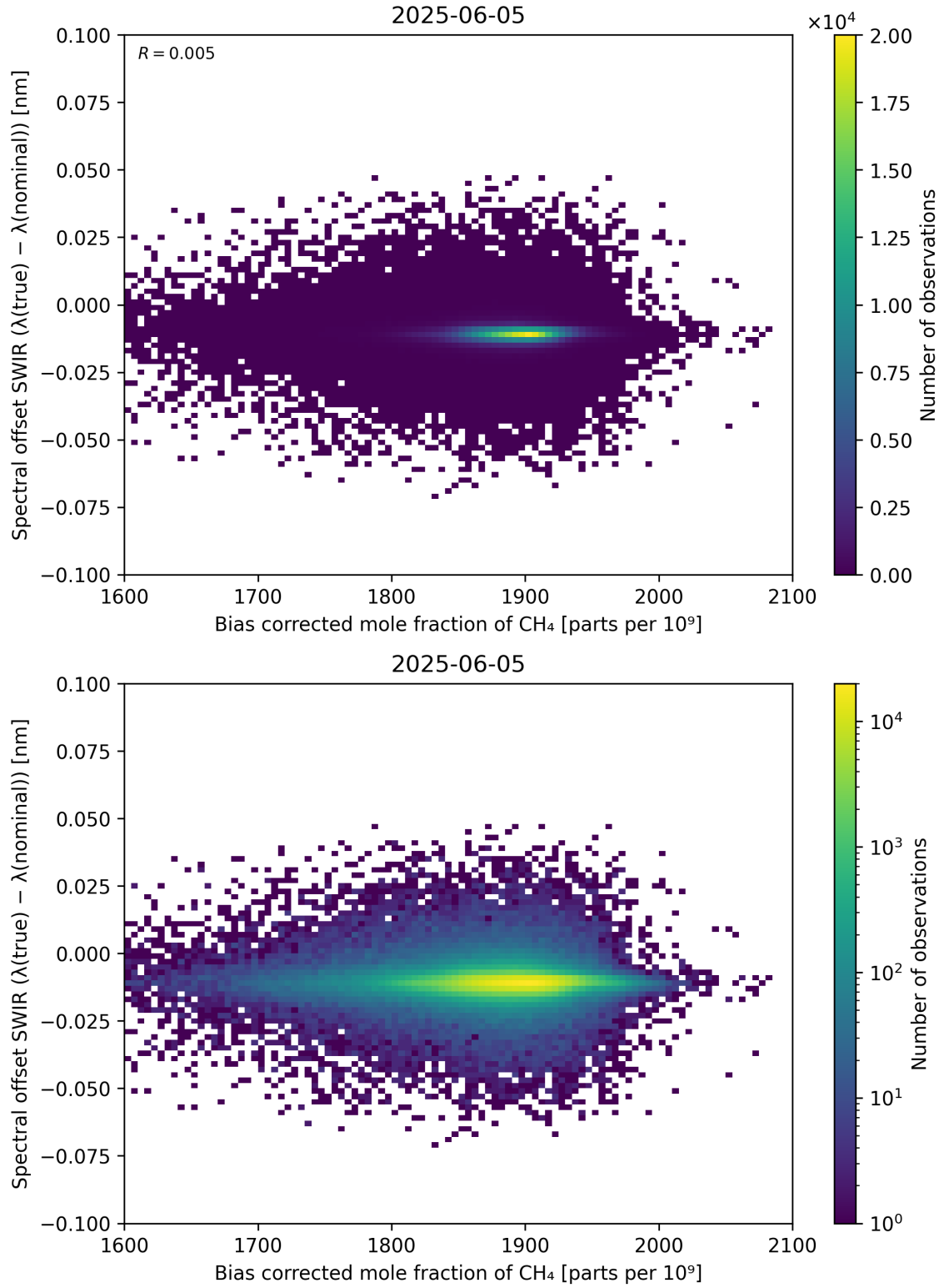
Figure 69: Scatter density plot of “Bias corrected mole fraction of \text{CH}_4 ” against “Spectral offset SWIR ( \lambda_{\text{true}} - \lambda_{\text{nominal}} )” for 2025-06-04 to 2025-06-06.
