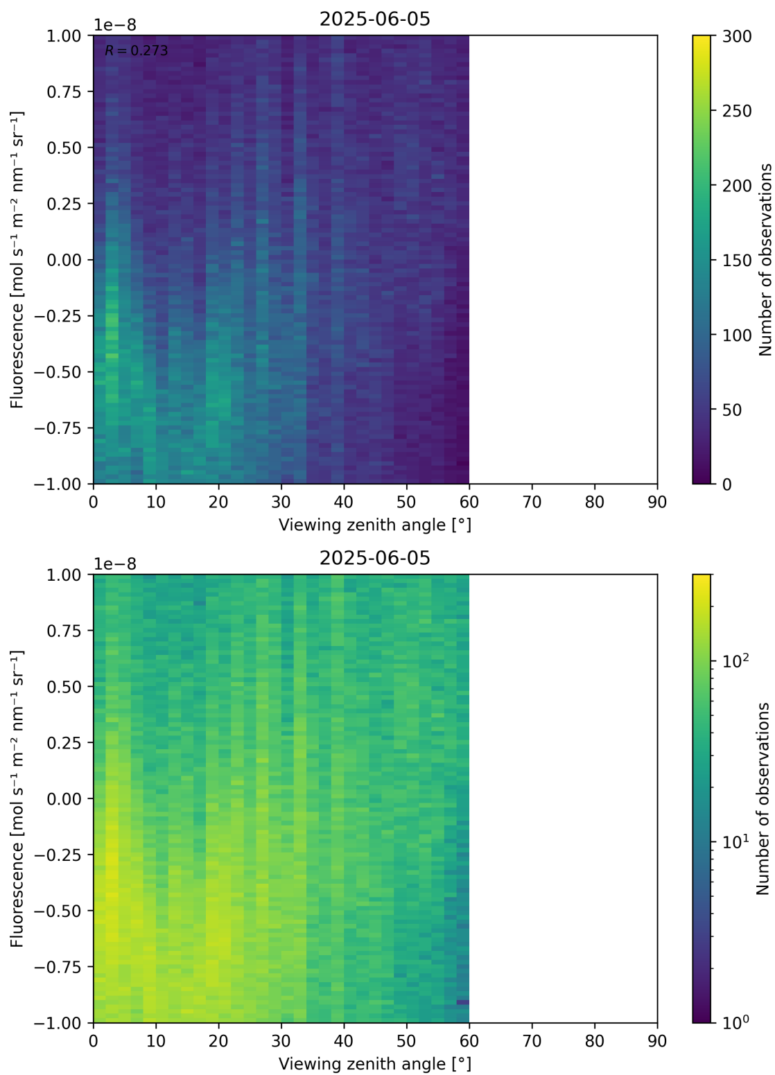
Figure 108: Scatter density plot of “Viewing zenith angle” against “Fluorescence” for 2025-06-04 to 2025-06-06.
