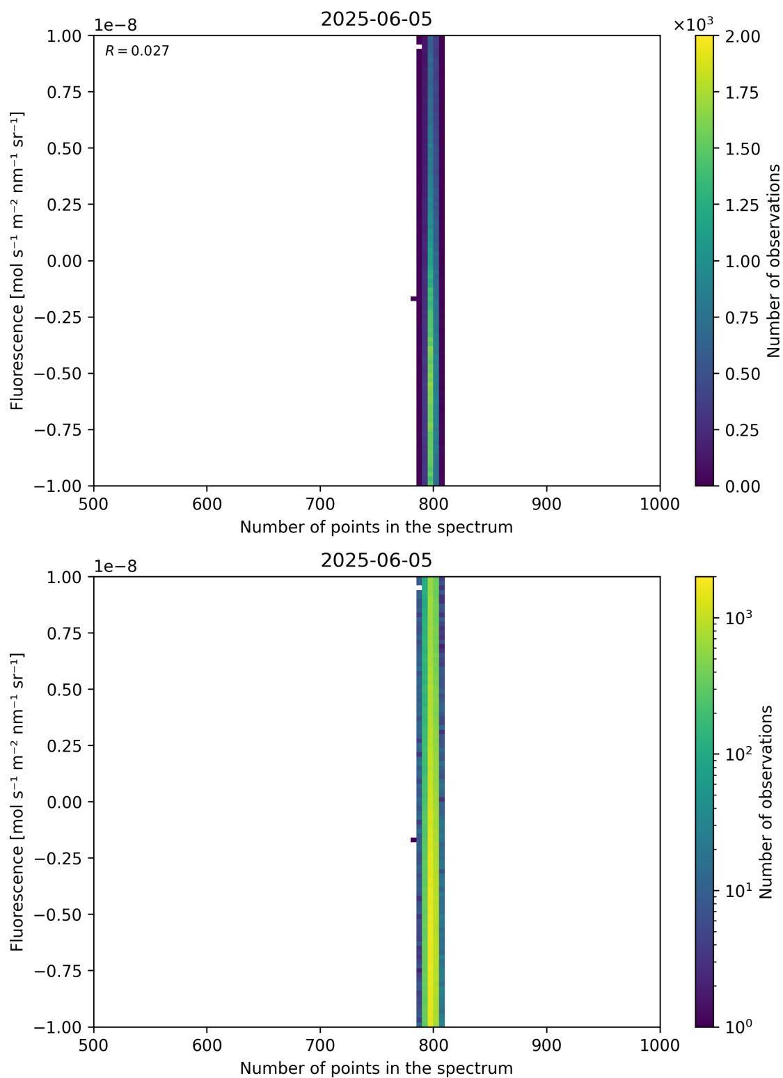
Figure 91: Scatter density plot of “Number of points in the spectrum” against “Fluorescence” for 2025-06-04 to 2025-06-06.
