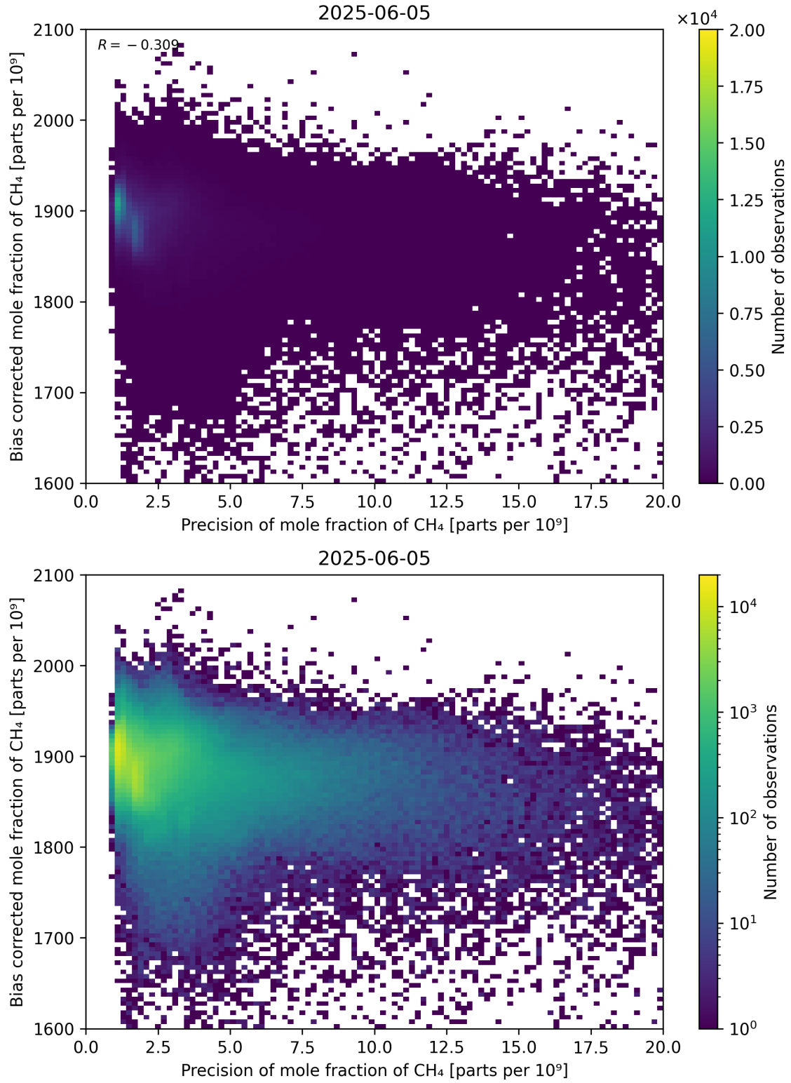
Figure 82: Scatter density plot of “Precision of mole fraction of CH 4 ” against “Bias corrected mole fraction of CH 4 ” for 2025-06-04 to 2025-06-06.
