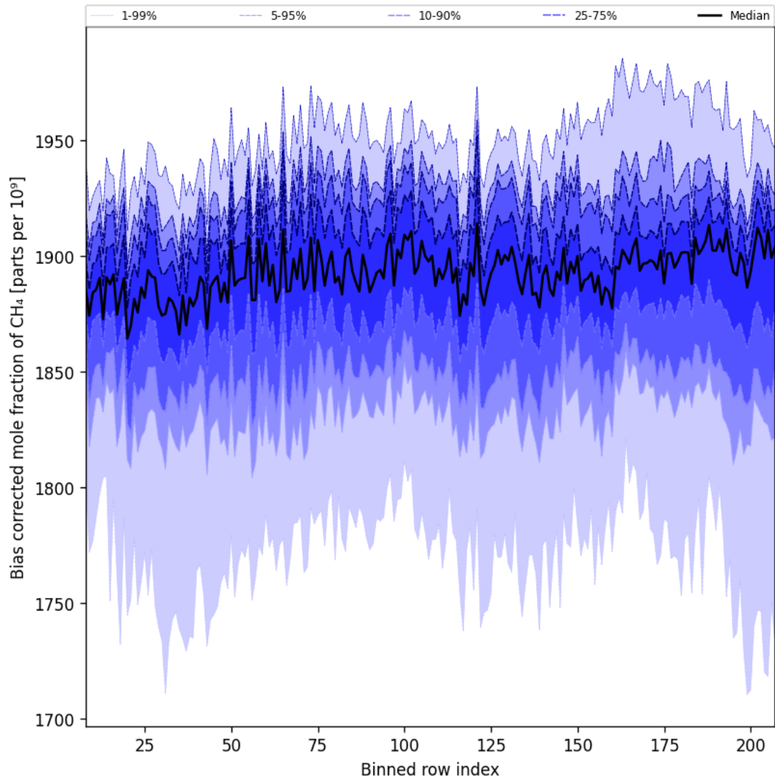
Figure 36: Along track statistics of “Bias corrected mole fraction of CH 4 ” for 2025-06-04 to 2025-06-06
