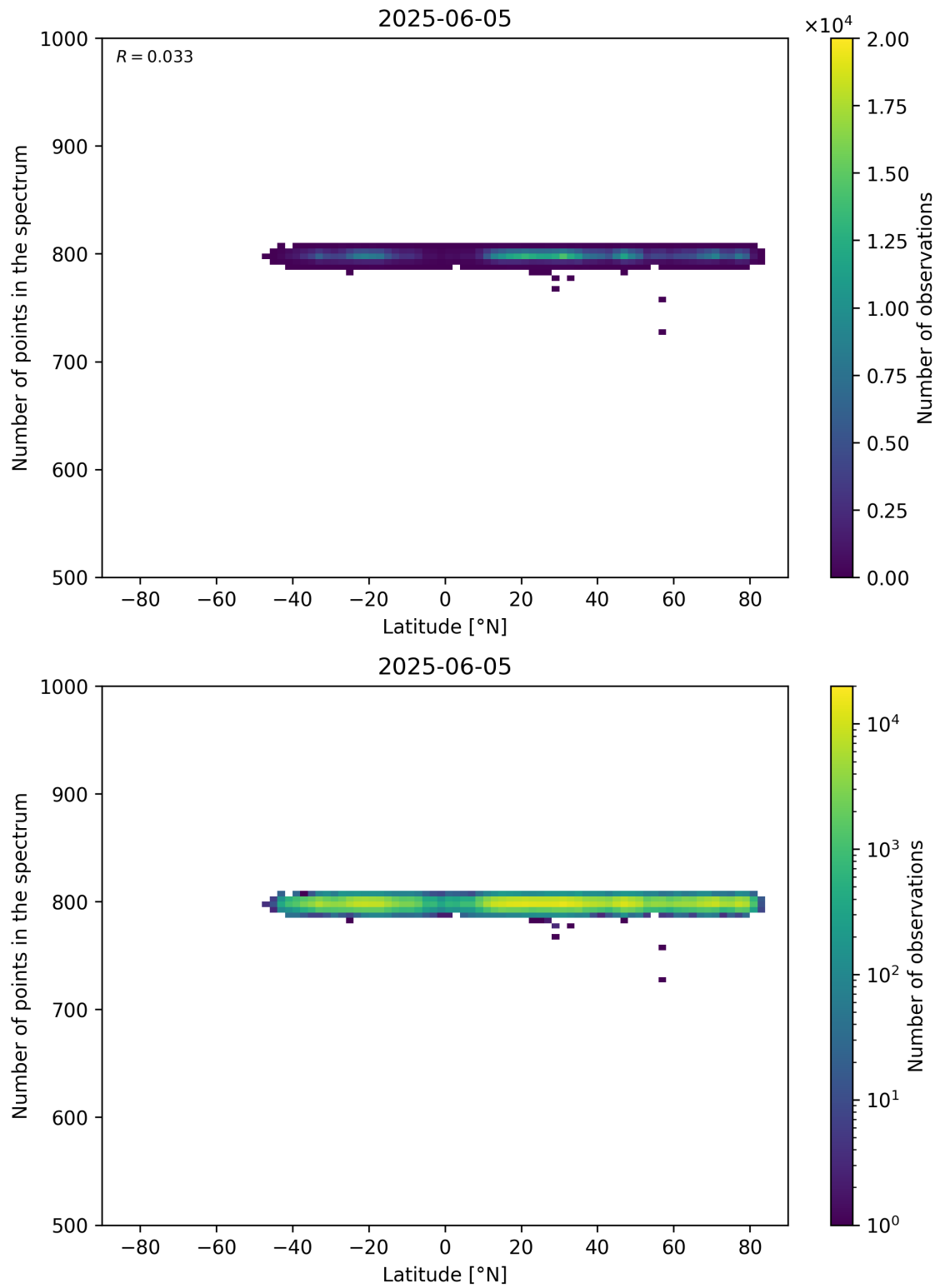
Figure 61: Scatter density plot of “Latitude” against “Number of points in the spectrum” for 2025-06-04 to 2025-06-06.
