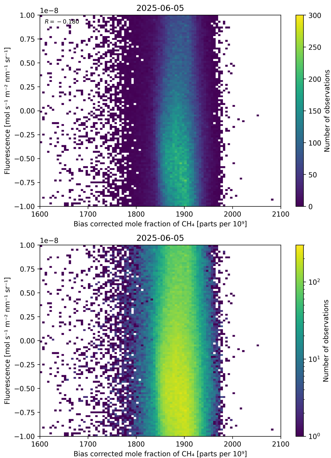
Figure 66: Scatter density plot of “Bias corrected mole fraction of CH 4 ” against “Fluorescence” for 2025-06-04 to 2025-06-06.
