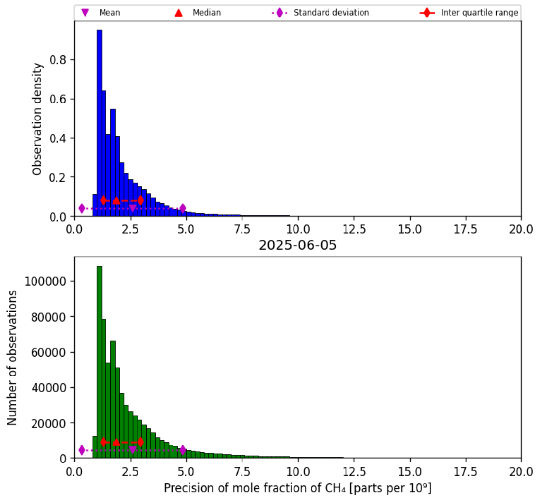
Figure 24: Histogram of “Precision of mole fraction of CH 4 ” for 2025-06-04 to 2025-06-06
