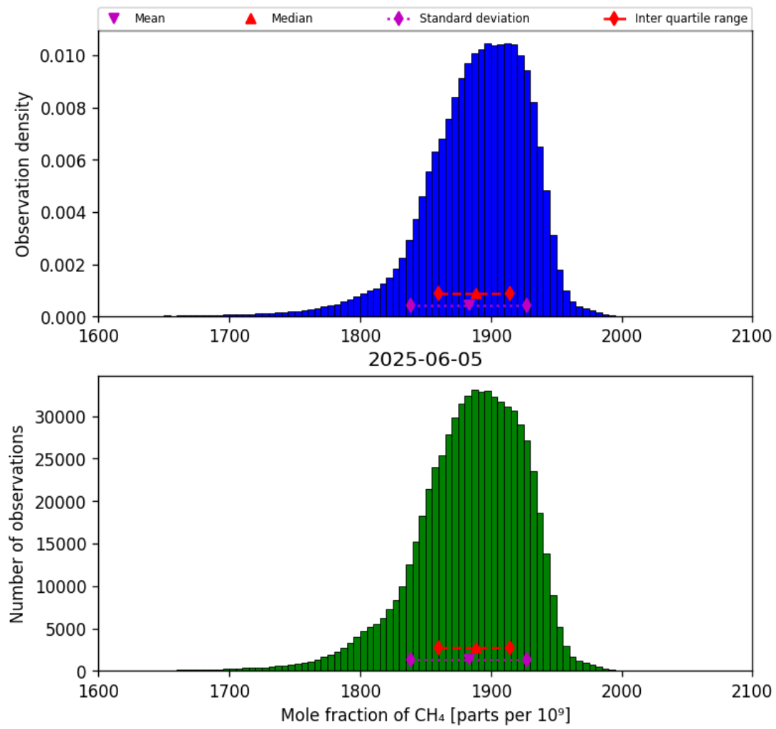
Figure 23: Histogram of “Mole fraction of CH 4 ” for 2025-06-04 to 2025-06-06
