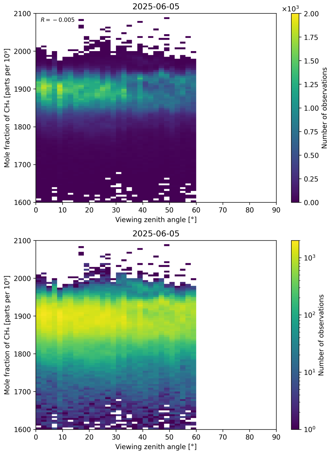
Figure 110: Scatter density plot of “Viewing zenith angle” against “Mole fraction of CH 4 ” for 2025-06-04 to 2025-06-06.
