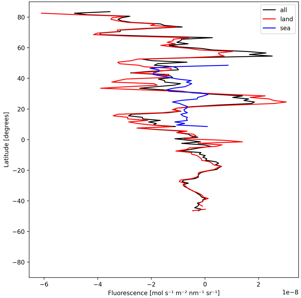
Figure 21: Zonal average of “Fluorescence” for 2025-06-04 to 2025-06-06.
