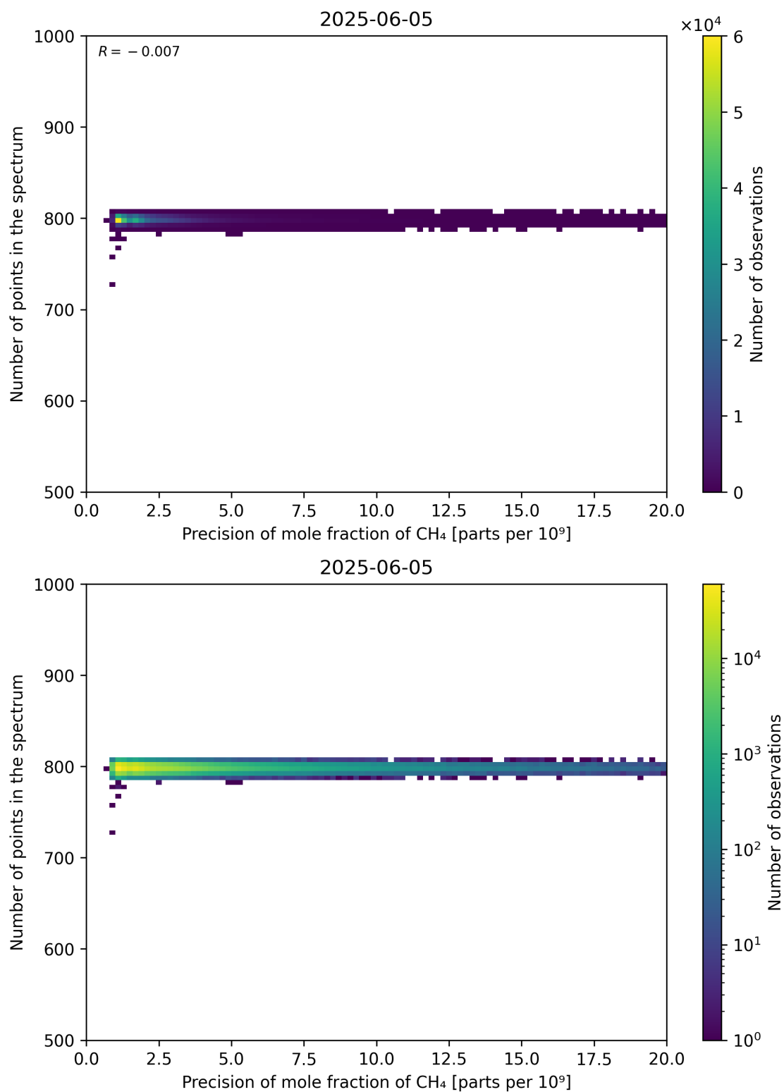
Figure 84: Scatter density plot of “Precision of mole fraction of CH 4 ” against “Number of points in the spectrum” for 2025-06-04 to 2025-06-06.
