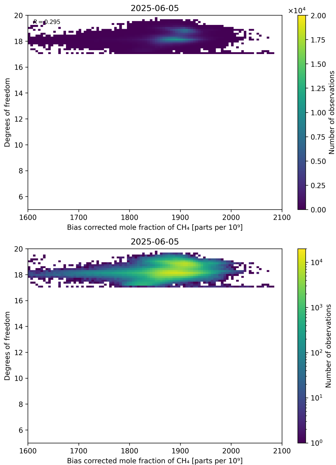
Figure 65: Scatter density plot of “Bias corrected mole fraction of CH 4 ” against “Degrees of freedom” for 2025-06-04 to 2025-06-06.
