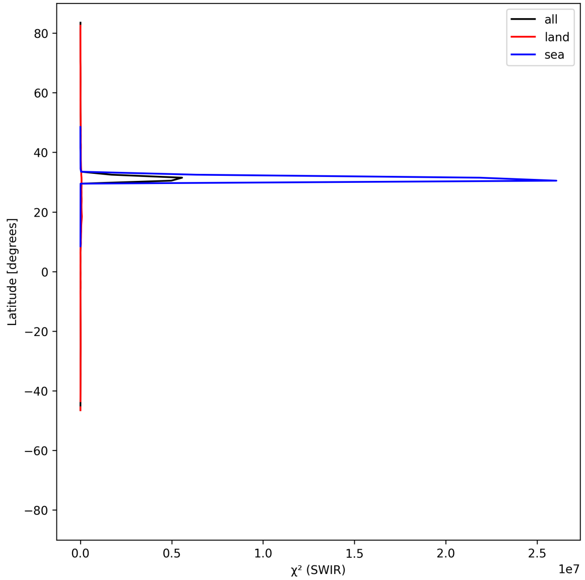
Figure 17: Zonal average of “ \chi^2 (SWIR)” for 2025-06-04 to 2025-06-06.
