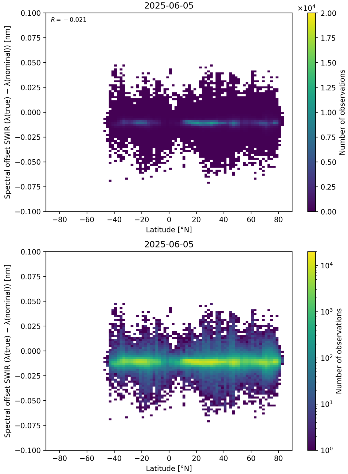
Figure 62: Scatter density plot of “Latitude” against “Spectral offset SWIR ( \lambda_{\text{true}} - \lambda_{\text{nominal}} )” for 2025-06-04 to 2025-06-06.
