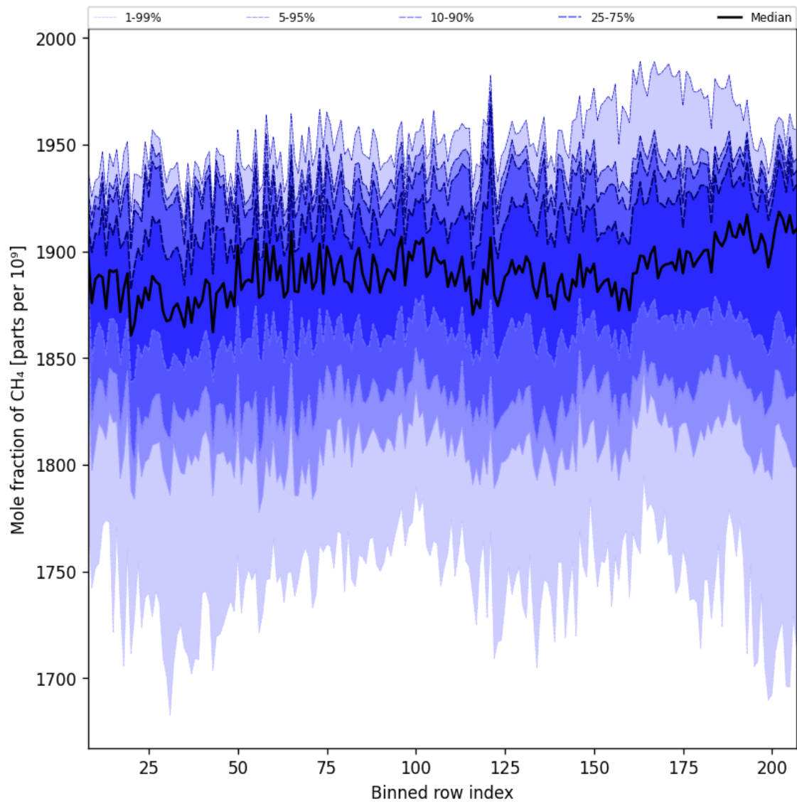
Figure 34: Along track statistics of “Mole fraction of CH 4 ” for 2025-06-04 to 2025-06-06
