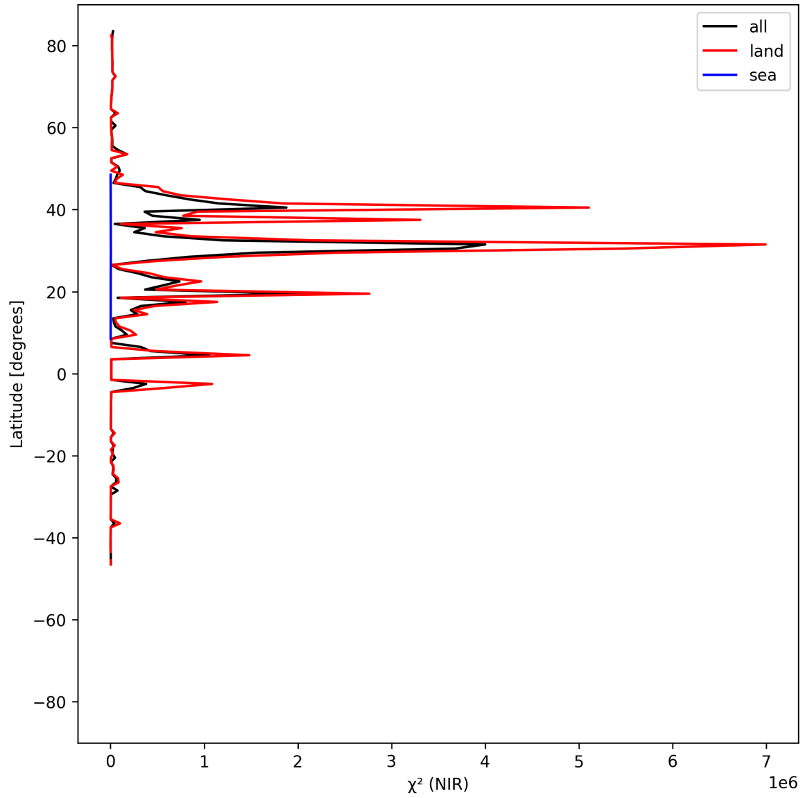
Figure 18: Zonal average of “ \chi^2 (NIR)” for 2025-06-04 to 2025-06-06.
