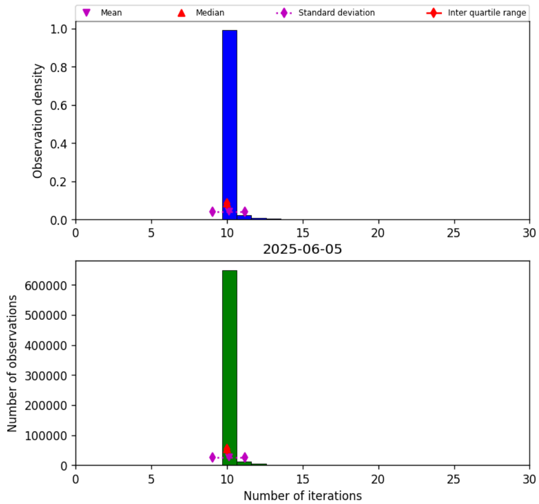
Figure 31: Histogram of “Number of iterations” for 2025-06-04 to 2025-06-06
