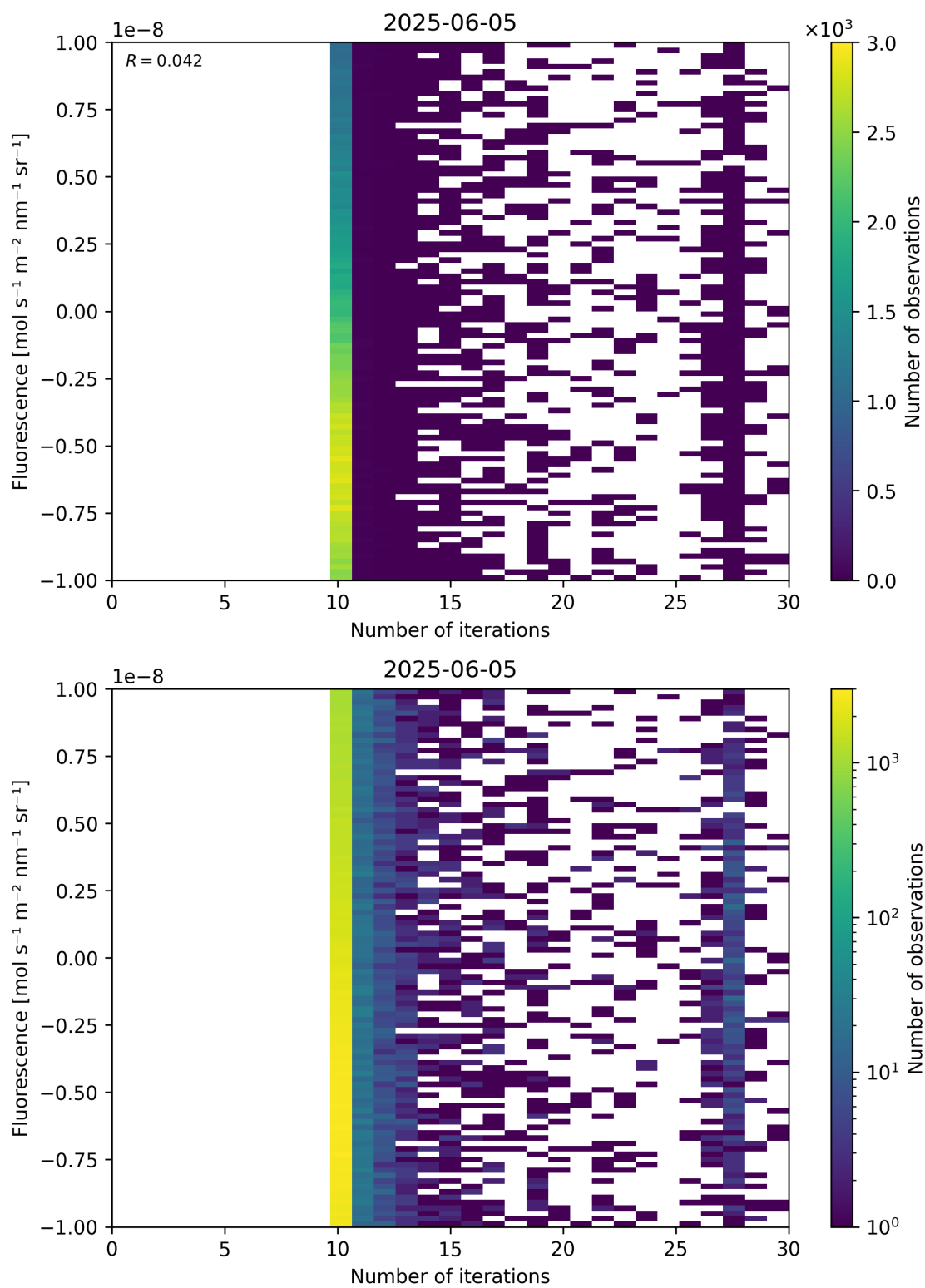
Figure 87: Scatter density plot of “Number of iterations” against “Fluorescence” for 2025-06-04 to 2025-06-06.
