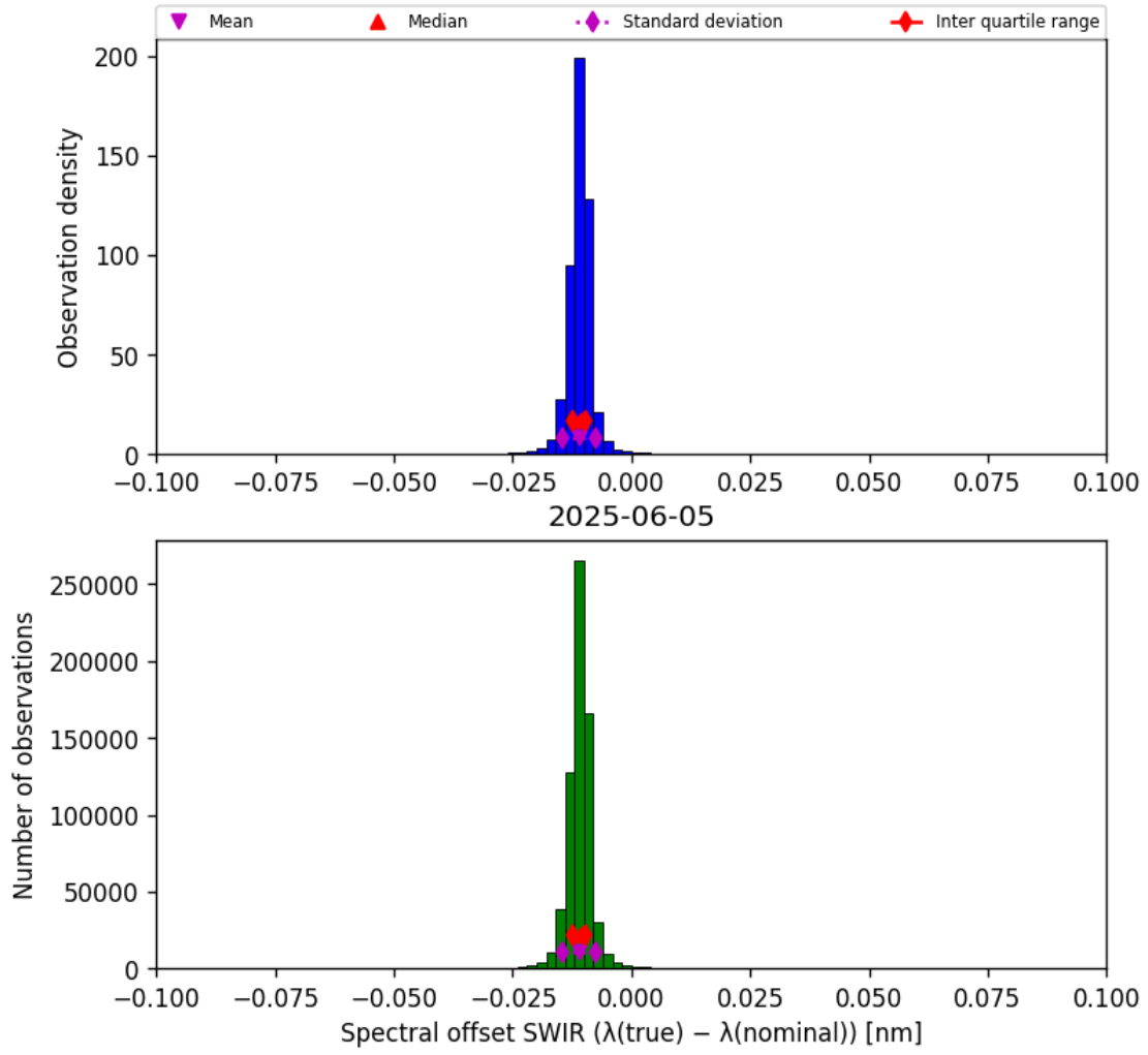
Figure 27: Histogram of “Spectral offset SWIR ( \lambda_{\text{true}} - \lambda_{\text{nominal}} )” for 2025-06-04 to 2025-06-06
