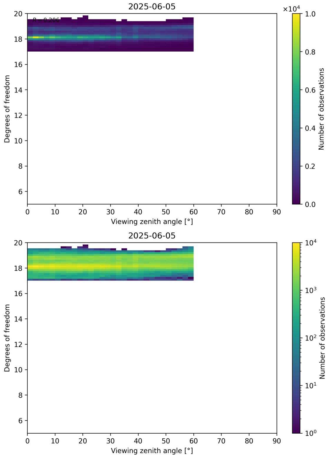
Figure 107: Scatter density plot of “Viewing zenith angle” against “Degrees of freedom” for 2025-06-04 to 2025-06-06.
