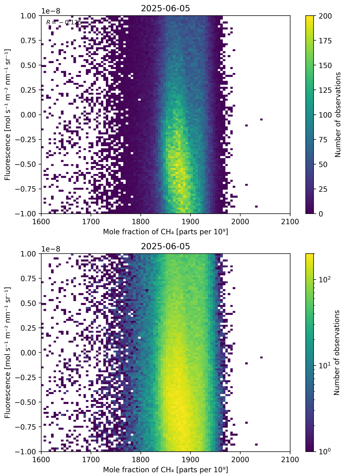
Figure 73: Scatter density plot of “Mole fraction of \text{CH}_4 ” against “Fluorescence” for 2025-06-04 to 2025-06-06.
