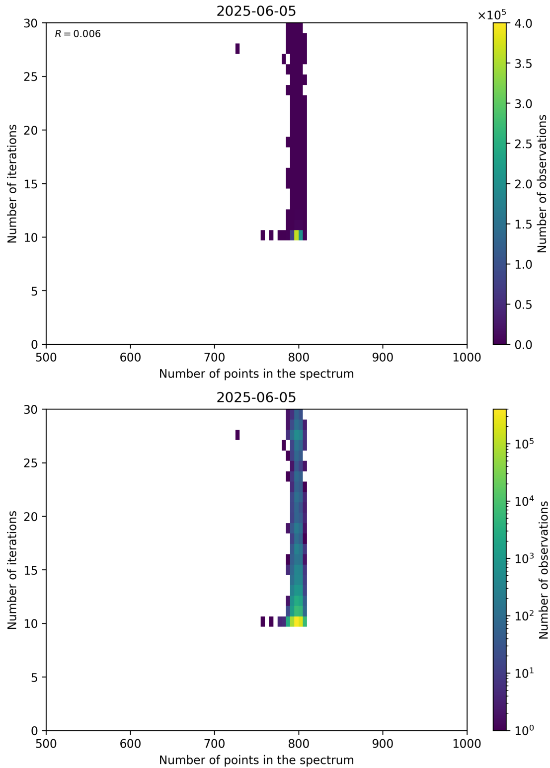
Figure 92: Scatter density plot of “Number of points in the spectrum” against “Number of iterations” for 2025-06-04 to 2025-06-06.
