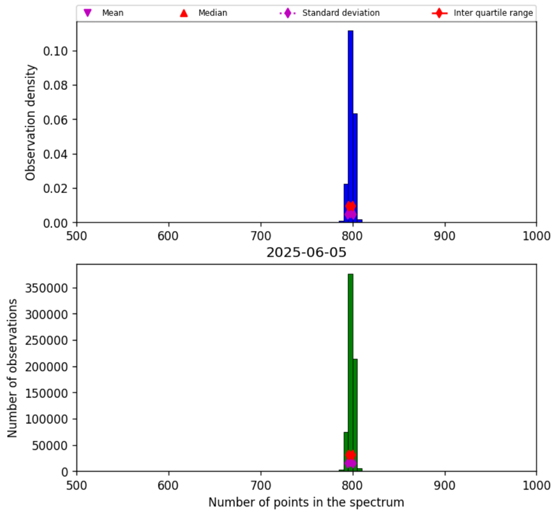
Figure 26: Histogram of “Number of points in the spectrum” for 2025-06-04 to 2025-06-06
