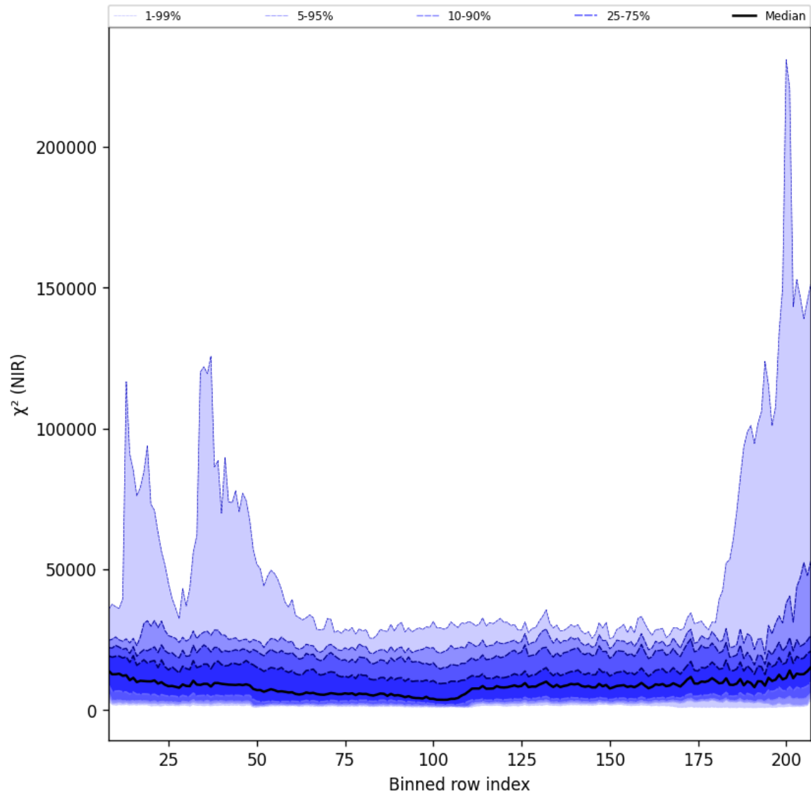
Figure 40: Along track statistics of “ \chi^2 (NIR)” for 2025-06-04 to 2025-06-06
