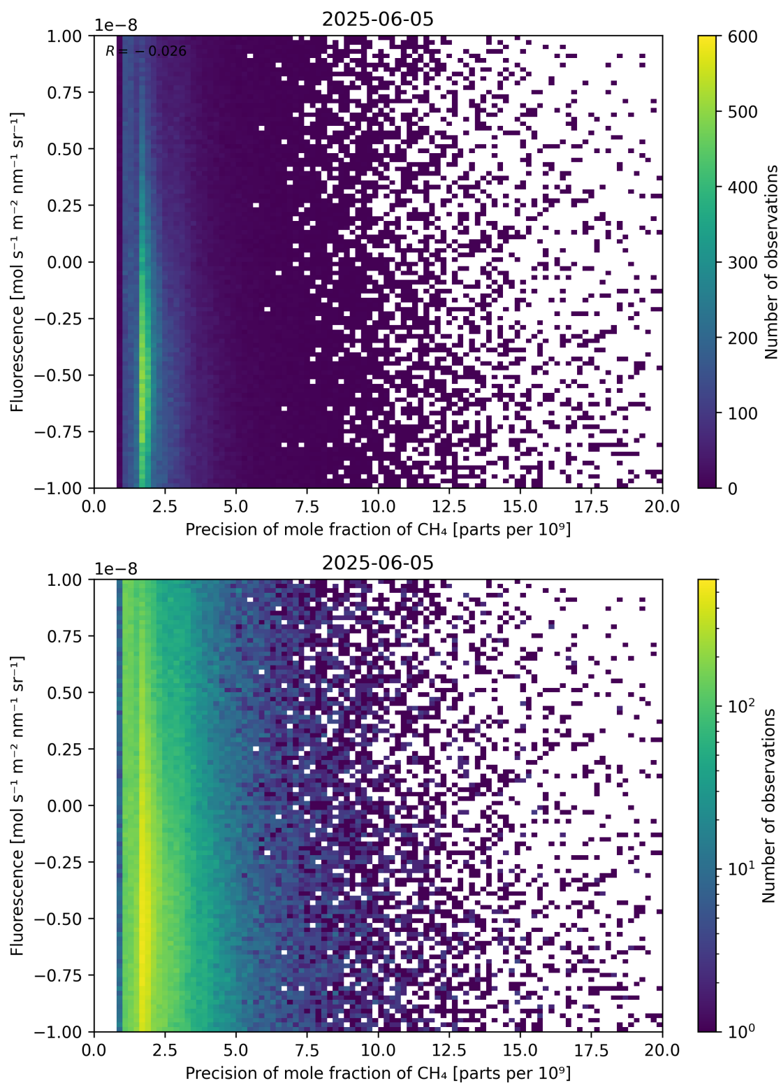
Figure 81: Scatter density plot of “Precision of mole fraction of \text{CH}_4 ” against “Fluorescence” for 2025-06-04 to 2025-06-06.
