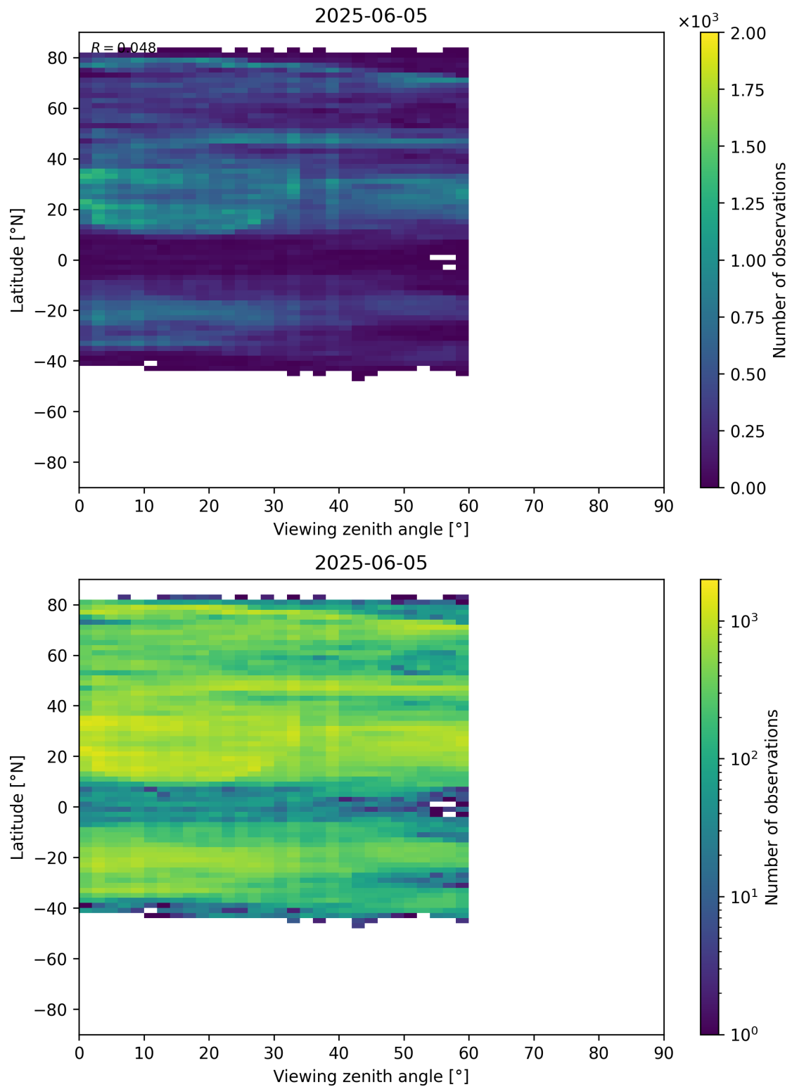
Figure 109: Scatter density plot of “Viewing zenith angle” against “Latitude” for 2025-06-04 to 2025-06-06.
