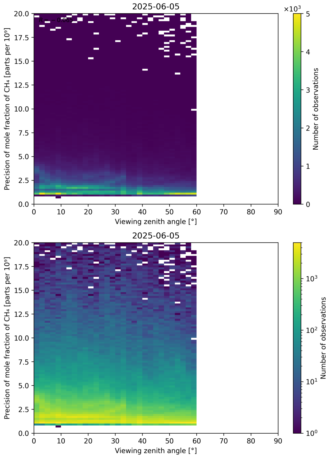
Figure 112: Scatter density plot of “Viewing zenith angle” against “Precision of mole fraction of CH 4 ” for 2025-06-04 to 2025-06-06.
