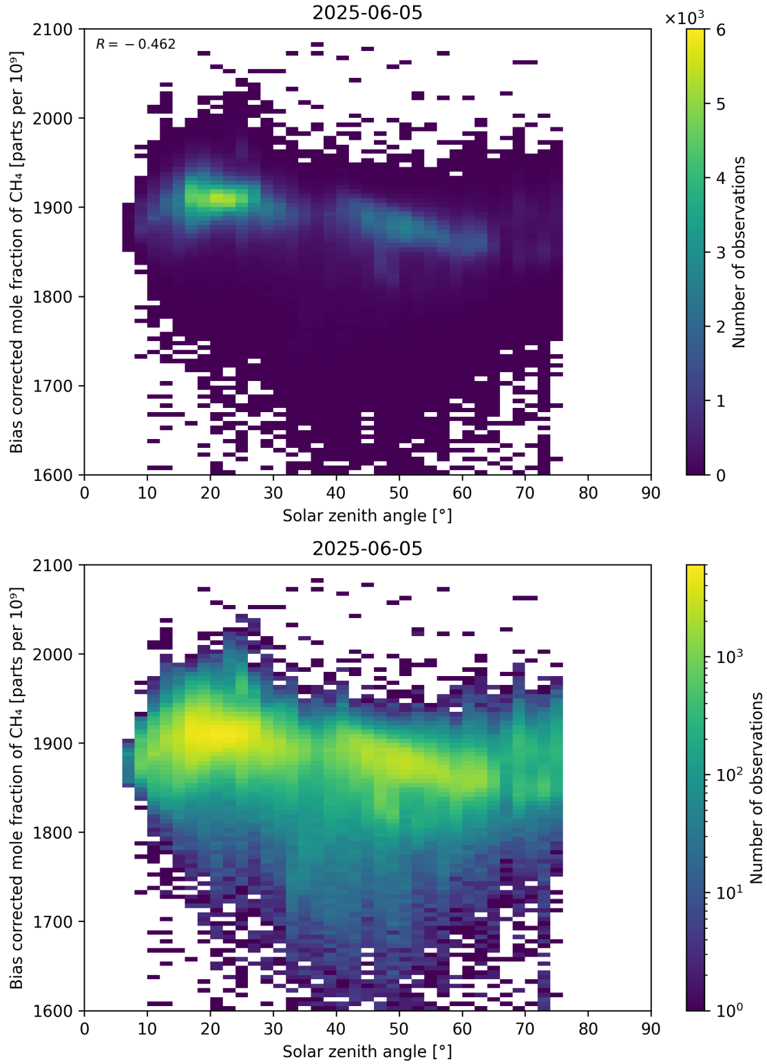
Figure 100: Scatter density plot of “Solar zenith angle” against “Bias corrected mole fraction of CH 4 ” for 2025-06-04 to 2025-06-06.
