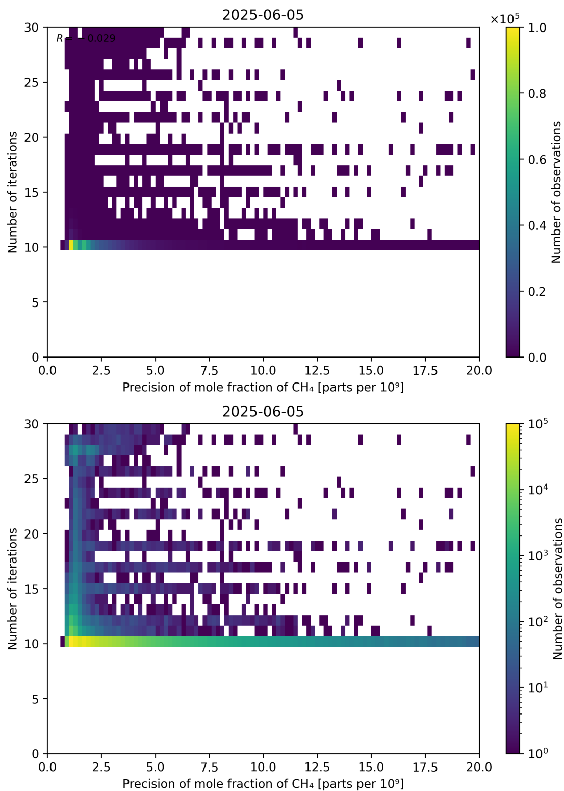
Figure 83: Scatter density plot of “Precision of mole fraction of CH 4 ” against “Number of iterations” for 2025-06-04 to 2025-06-06.
