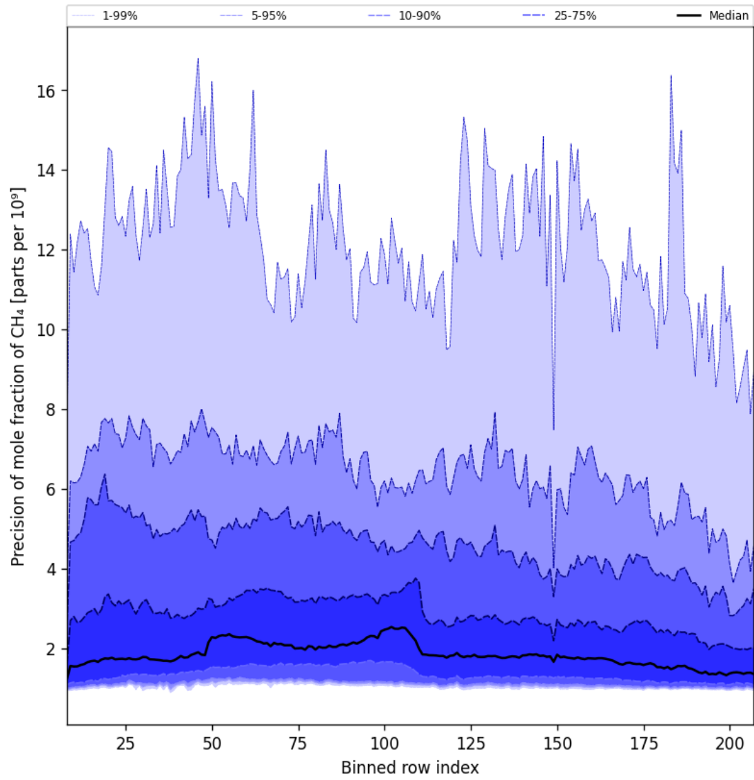
Figure 35: Along track statistics of “Precision of mole fraction of CH 4 ” for 2025-06-04 to 2025-06-06
