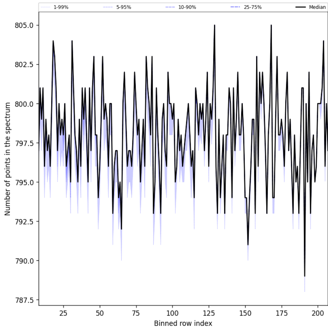
Figure 37: Along track statistics of “Number of points in the spectrum” for 2025-06-04 to 2025-06-06
