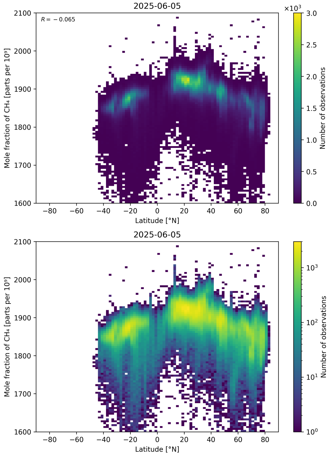
Figure 57: Scatter density plot of “Latitude” against “Mole fraction of \text{CH}_4 ” for 2025-06-04 to 2025-06-06.
