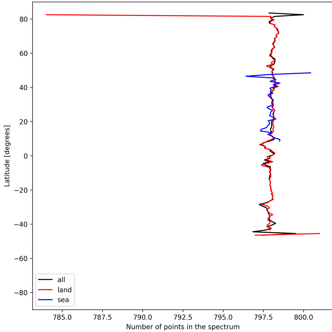
Figure 15: Zonal average of “Number of points in the spectrum” for 2025-06-04 to 2025-06-06.
