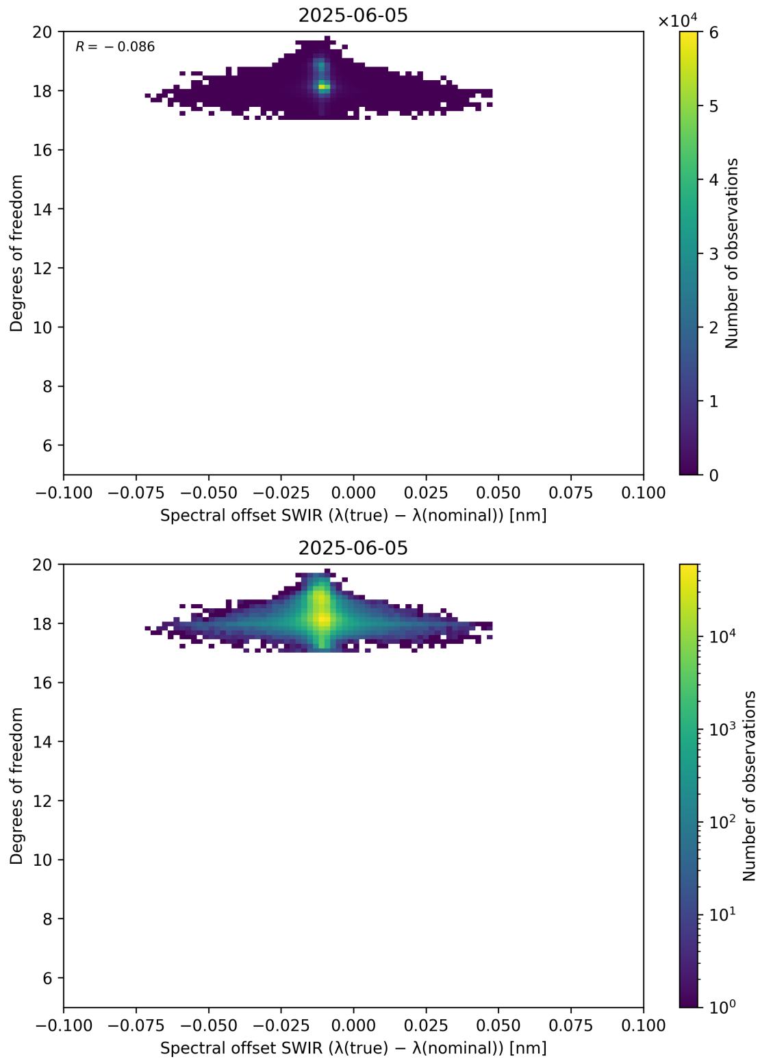
Figure 119: Scatter density plot of “Spectral offset SWIR ( \lambda_{\text{true}} - \lambda_{\text{nominal}} )” against “Degrees of freedom” for 2025-06-04 to 2025-06-06.
