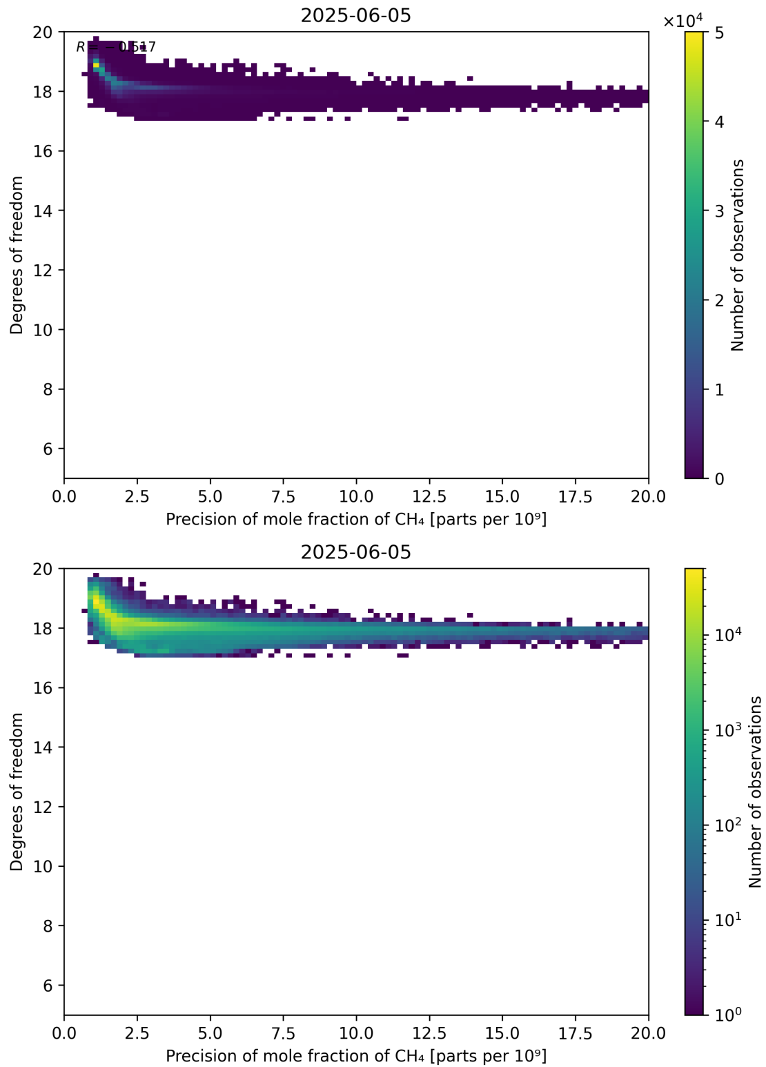
Figure 80: Scatter density plot of “Precision of mole fraction of CH 4 ” against “Degrees of freedom” for 2025-06-04 to 2025-06-06.
