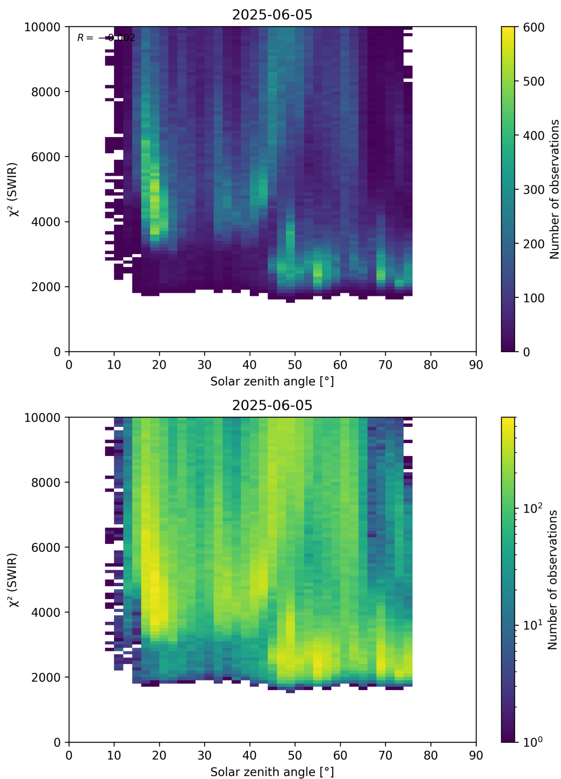
Figure 95: Scatter density plot of “Solar zenith angle” against “ \chi^2 (SWIR)” for 2025-06-04 to 2025-06-06.
