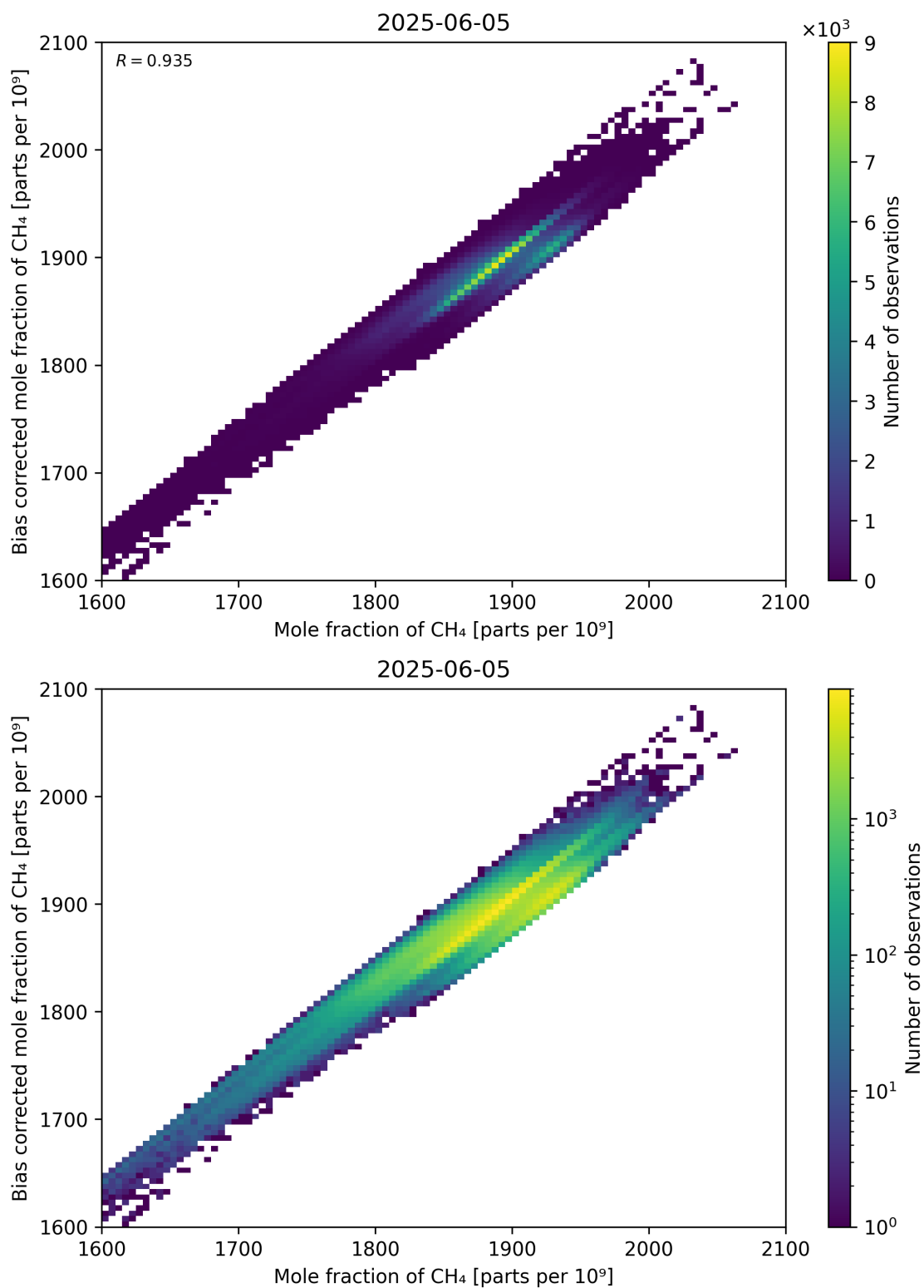
Figure 74: Scatter density plot of “Mole fraction of CH 4 ” against “Bias corrected mole fraction of CH 4 ” for 2025-06-04 to 2025-06-06.
