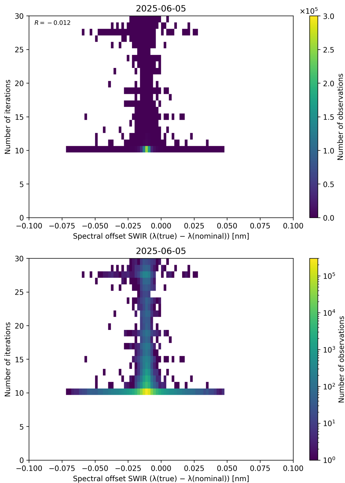
Figure 121: Scatter density plot of “Spectral offset SWIR ( \lambda_{\text{true}} - \lambda_{\text{nominal}} )” against “Number of iterations” for 2025-06-04 to 2025-06-06.
