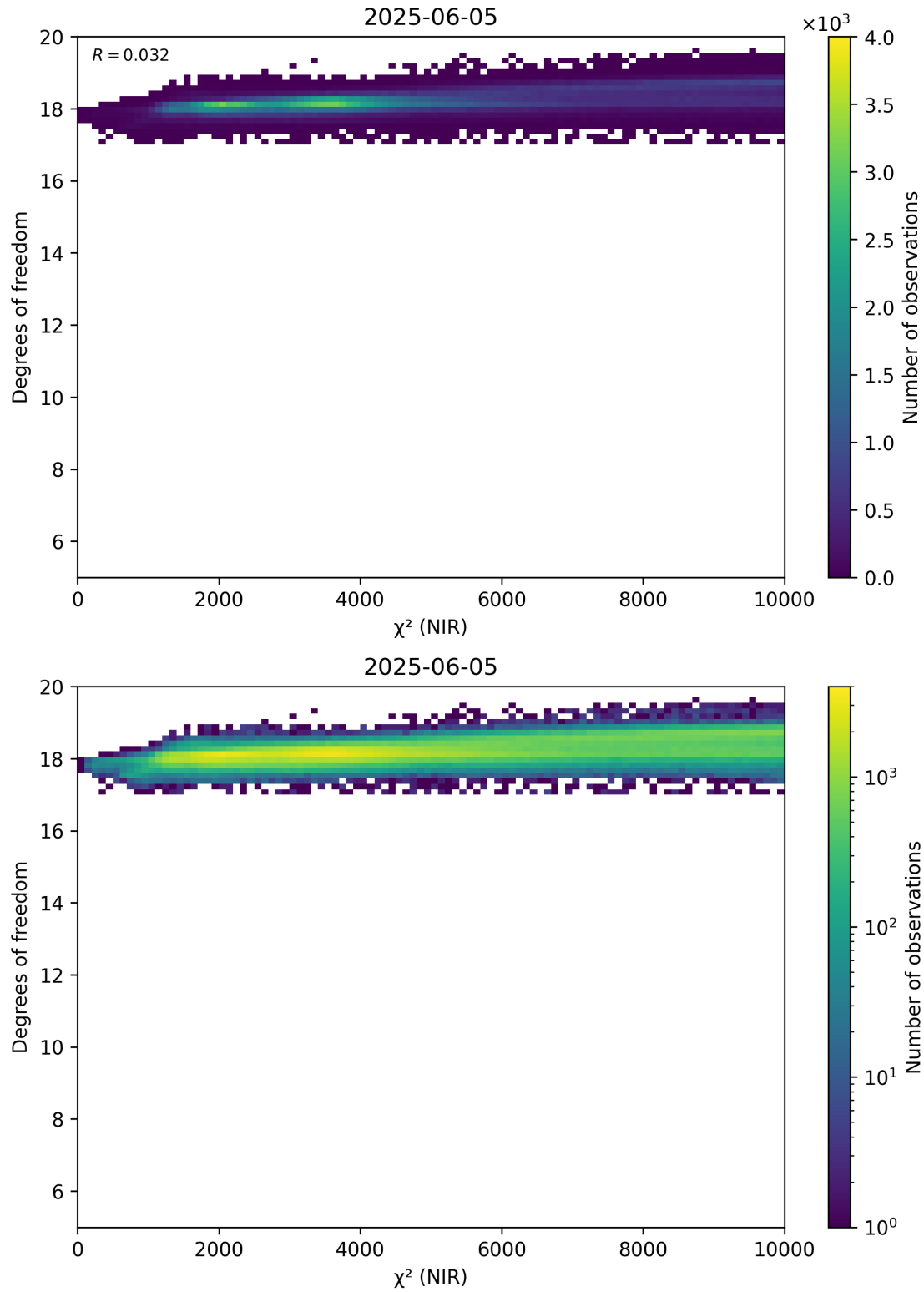
Figure 44: Scatter density plot of “ \chi^2 (NIR)” against “Degrees of freedom” for 2025-06-04 to 2025-06-06.
