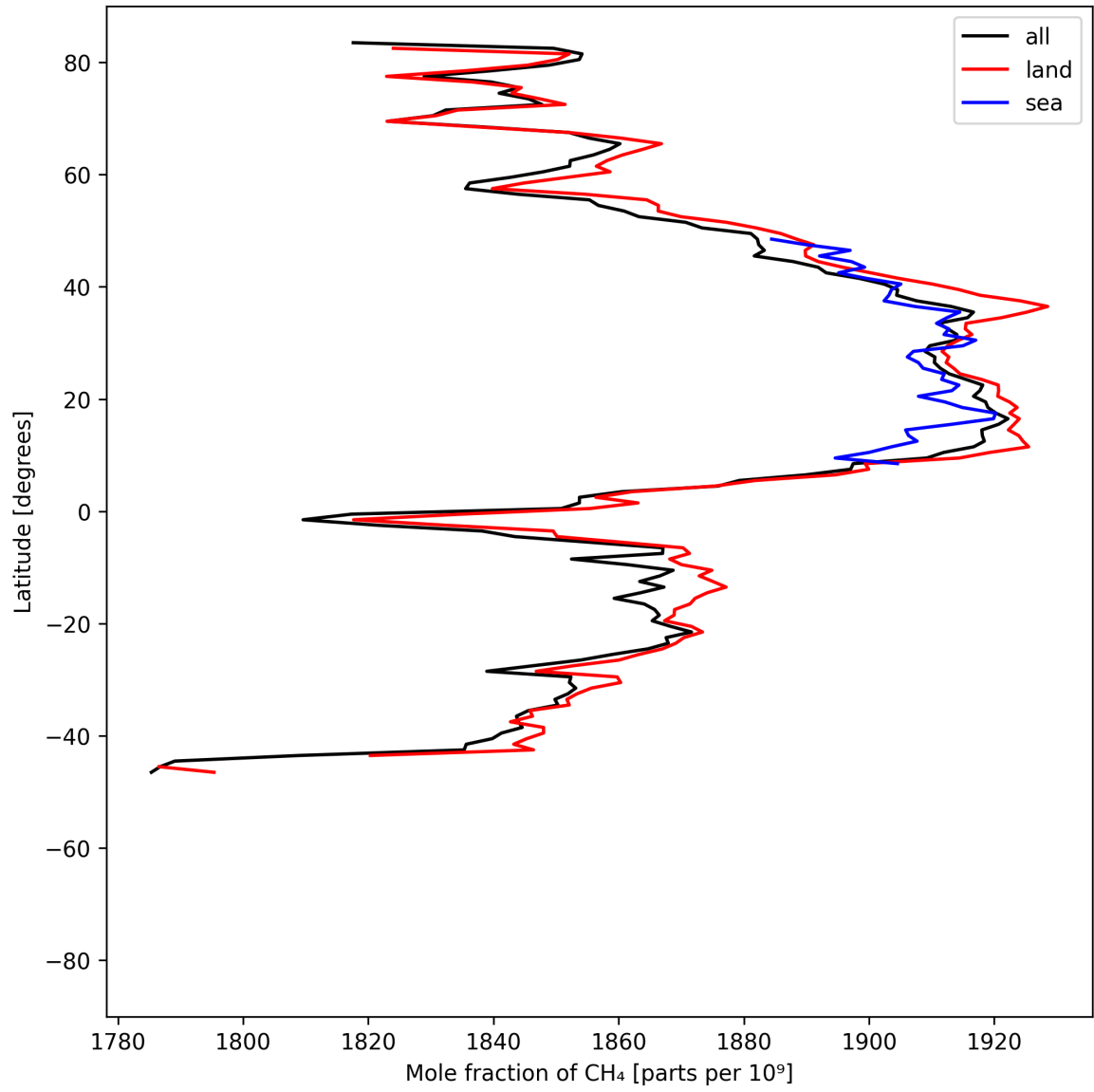
Figure 12: Zonal average of “Mole fraction of \text{CH}_4 ” for 2025-06-04 to 2025-06-06.
