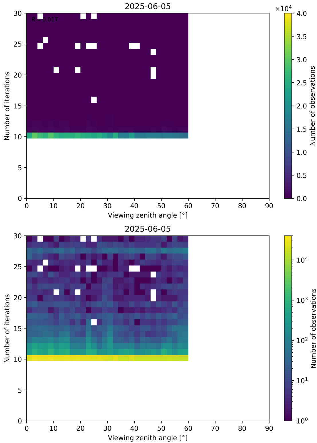
Figure 113: Scatter density plot of “Viewing zenith angle” against “Number of iterations” for 2025-06-04 to 2025-06-06.
