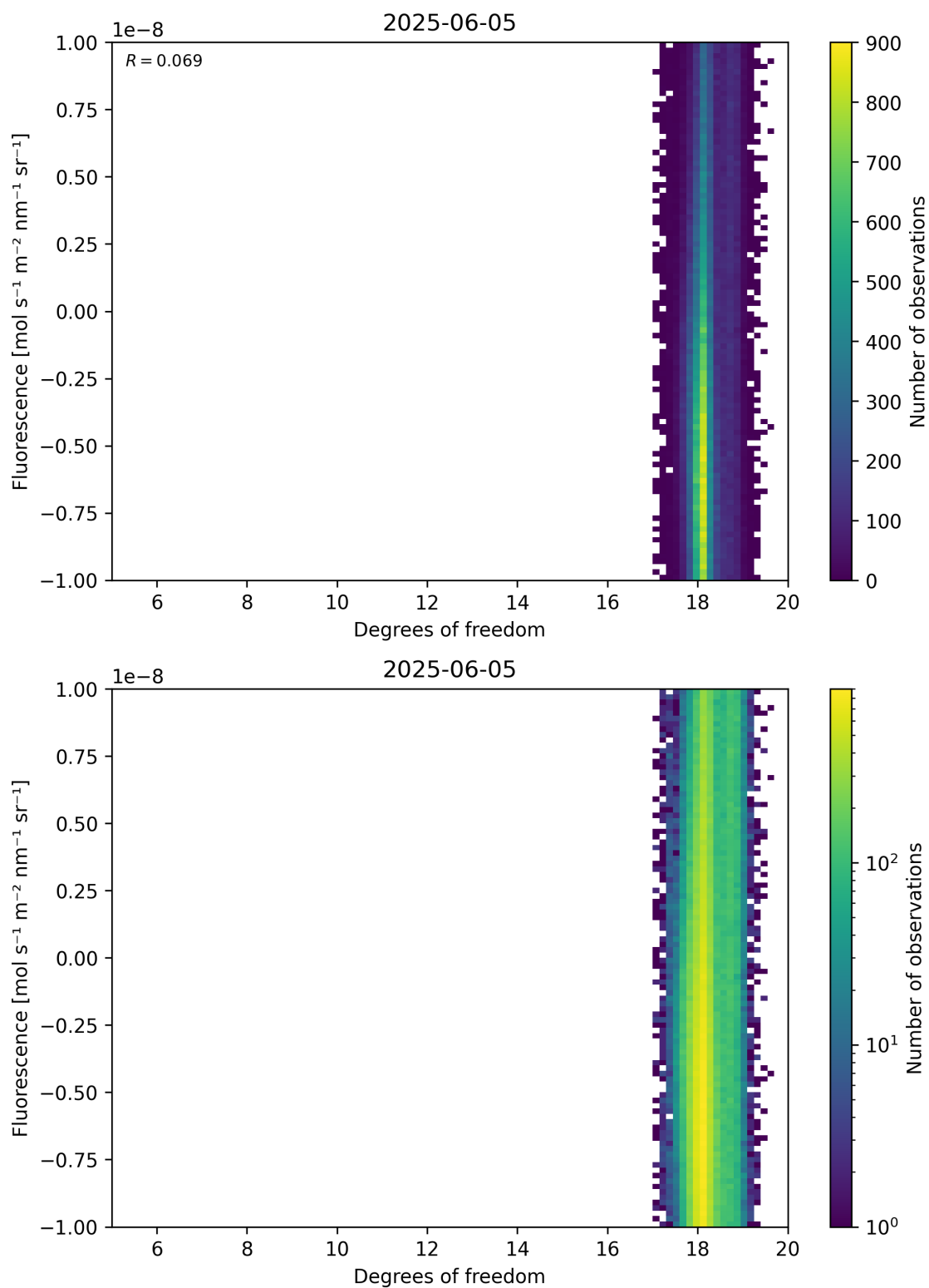
Figure 51: Scatter density plot of “Degrees of freedom” against “Fluorescence” for 2025-06-04 to 2025-06-06.
