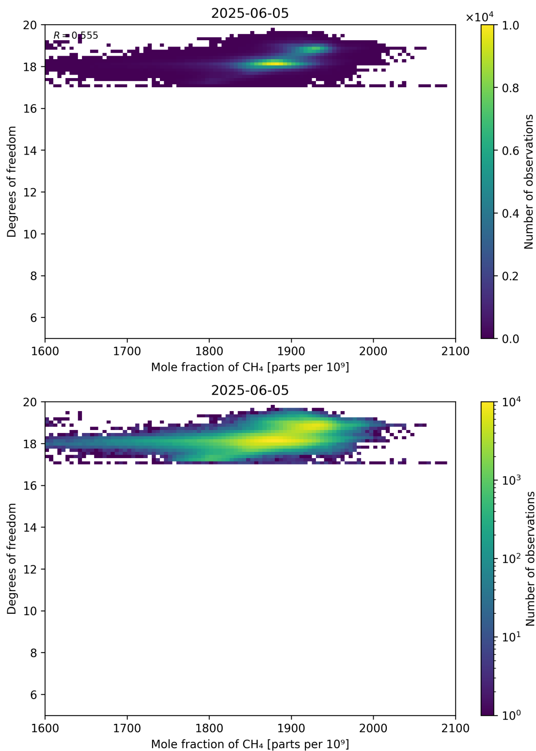
Figure 72: Scatter density plot of “Mole fraction of CH 4 ” against “Degrees of freedom” for 2025-06-04 to 2025-06-06.
