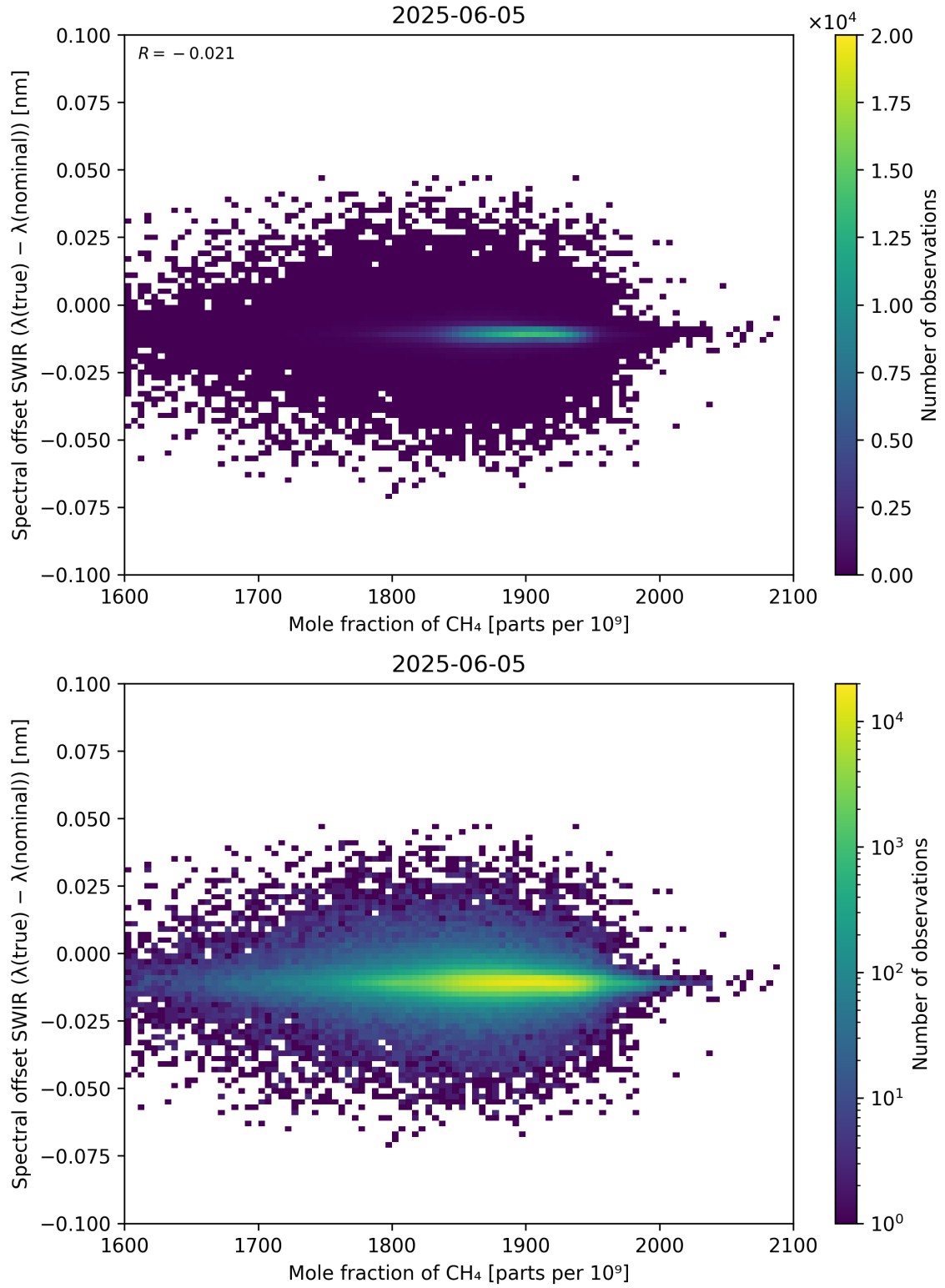
Figure 86: Scatter density plot of “Mole fraction of CH 4 ” against “Spectral offset SWIR ( \lambda_{\text{true}} - \lambda_{\text{nominal}} )” for 2025-06-04 to 2025-06-06.
