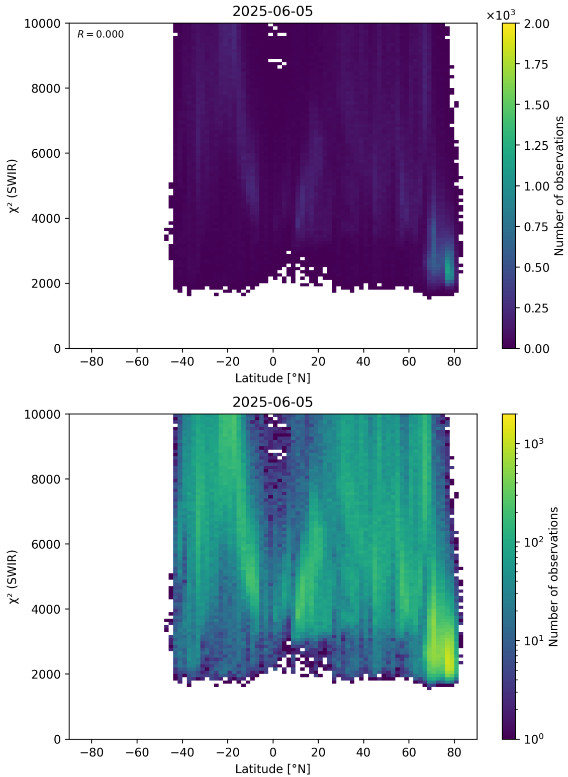
Figure 54: Scatter density plot of “Latitude” against “ \chi^2 (SWIR)” for 2025-06-04 to 2025-06-06.
