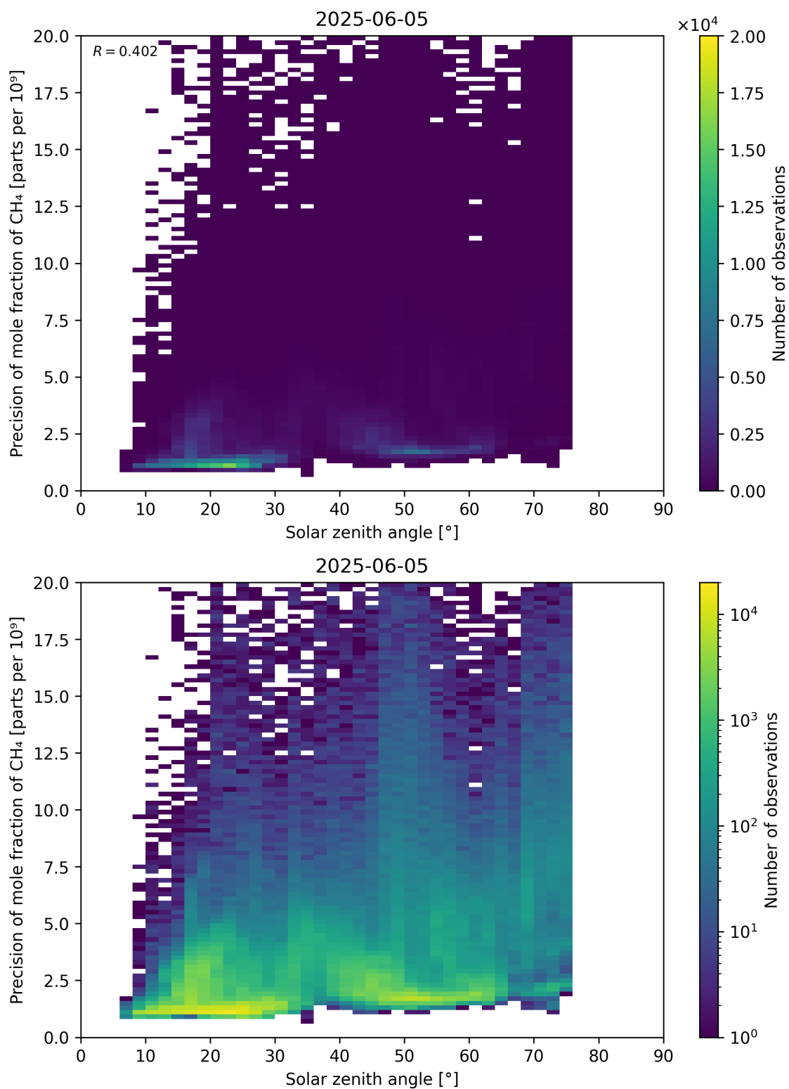
Figure 101: Scatter density plot of “Solar zenith angle” against “Precision of mole fraction of CH 4 ” for 2025-06-04 to 2025-06-06.
