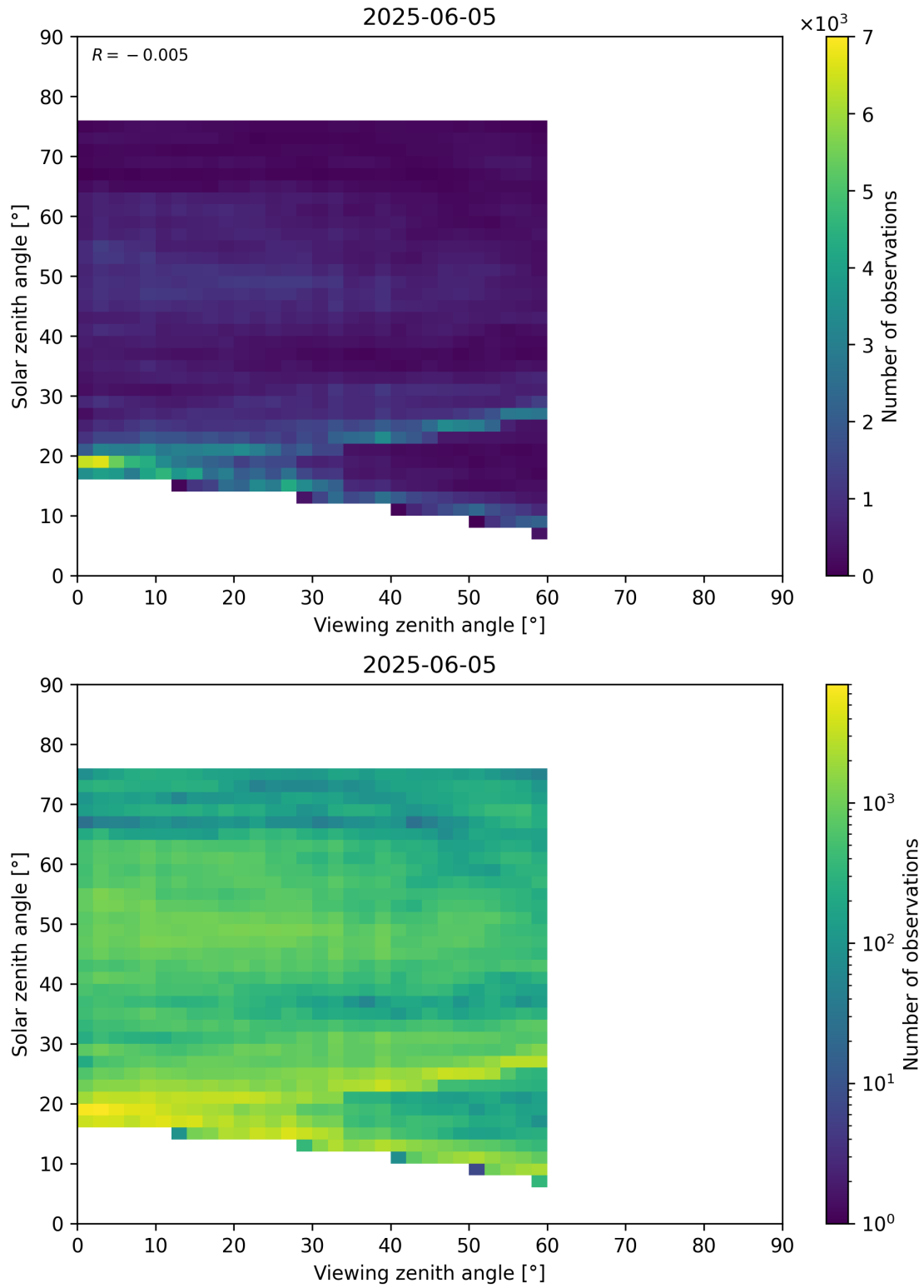
Figure 115: Scatter density plot of “Viewing zenith angle” against “Solar zenith angle” for 2025-06-04 to 2025-06-06.
