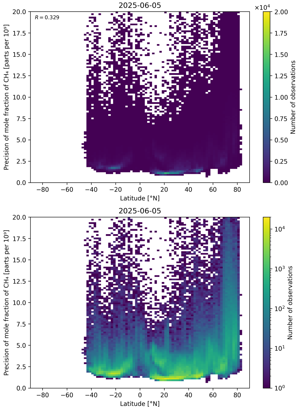
Figure 59: Scatter density plot of “Latitude” against “Precision of mole fraction of \text{CH}_4 ” for 2025-06-04 to 2025-06-06.
