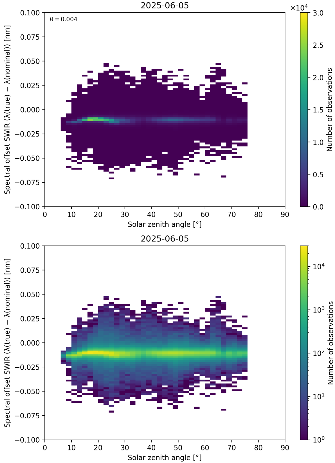
Figure 104: Scatter density plot of “Solar zenith angle” against “Spectral offset SWIR ( \lambda_{\text{true}} - \lambda_{\text{nominal}} )” for 2025-06-04 to 2025-06-06.
