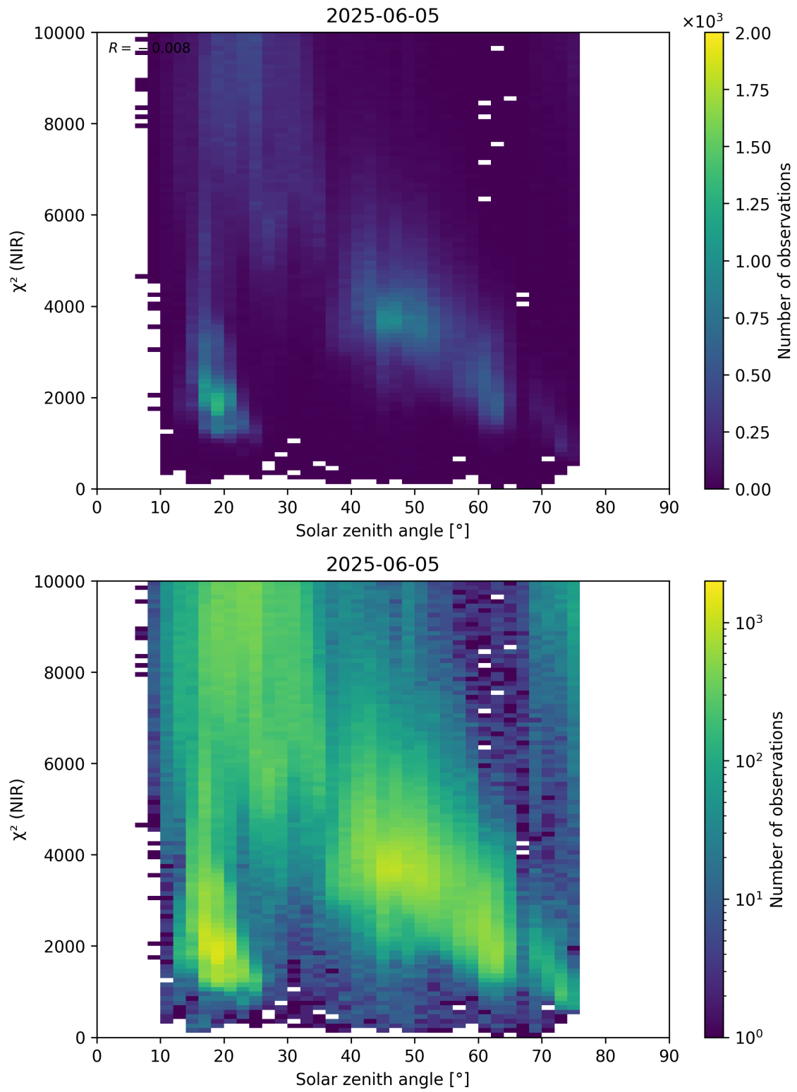
Figure 94: Scatter density plot of “Solar zenith angle” against “ \chi^2 (NIR)” for 2025-06-04 to 2025-06-06.
