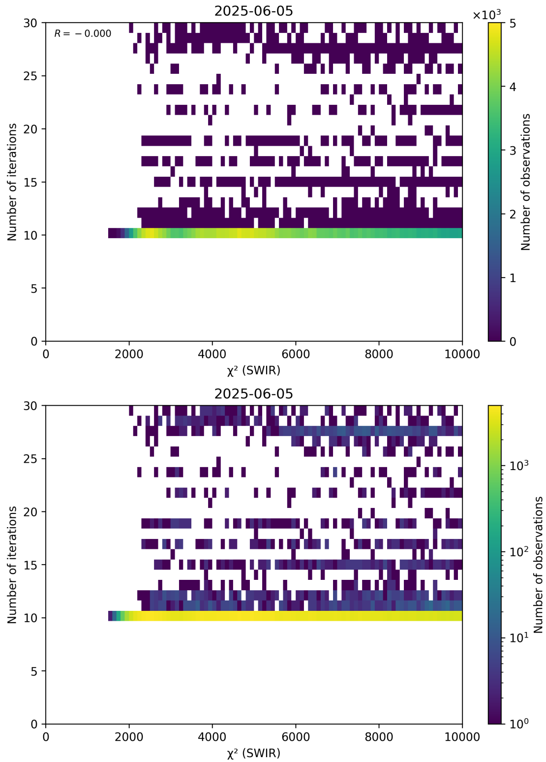
Figure 50: Scatter density plot of “ \chi^2 (SWIR)” against “Number of iterations” for 2025-06-04 to 2025-06-06.
