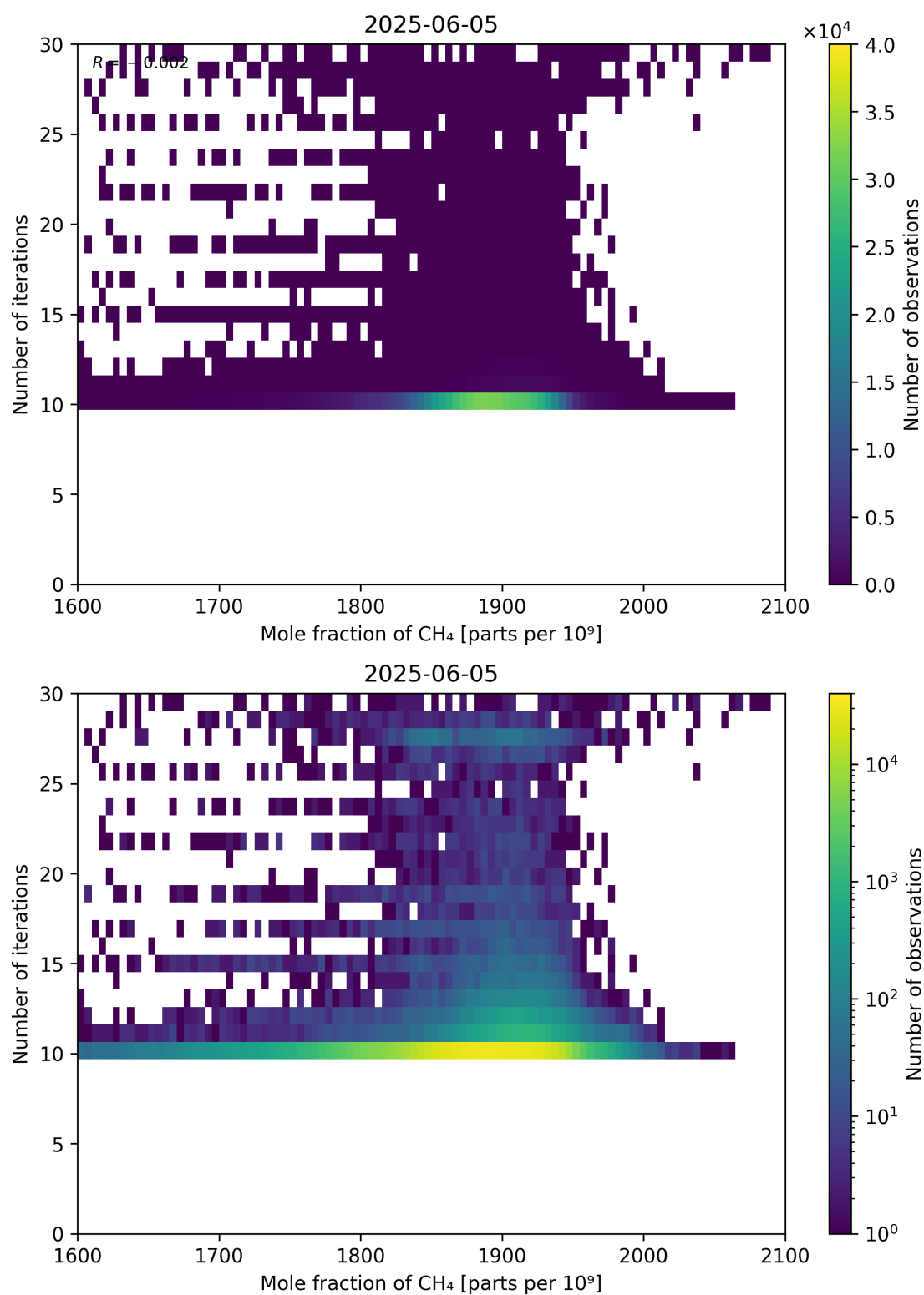
Figure 76: Scatter density plot of “Mole fraction of CH 4 ” against “Number of iterations” for 2025-06-04 to 2025-06-06.
