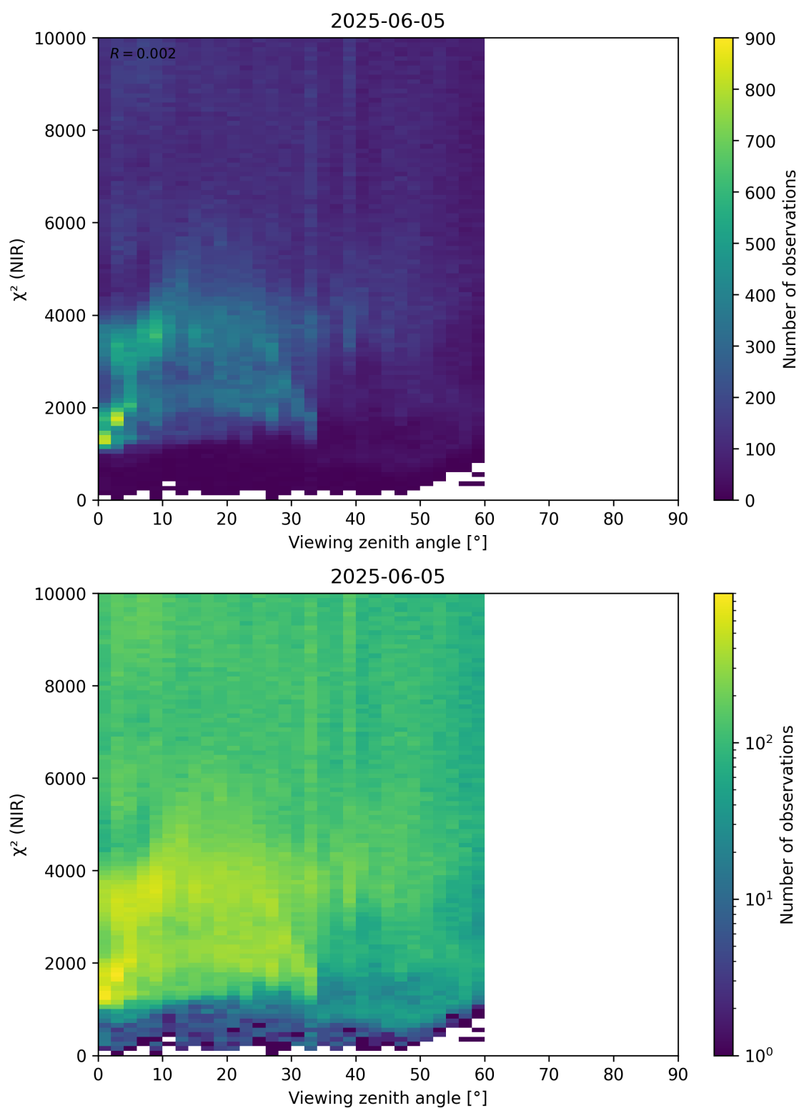
Figure 105: Scatter density plot of “Viewing zenith angle” against “ \chi^2 (NIR)” for 2025-06-04 to 2025-06-06.
