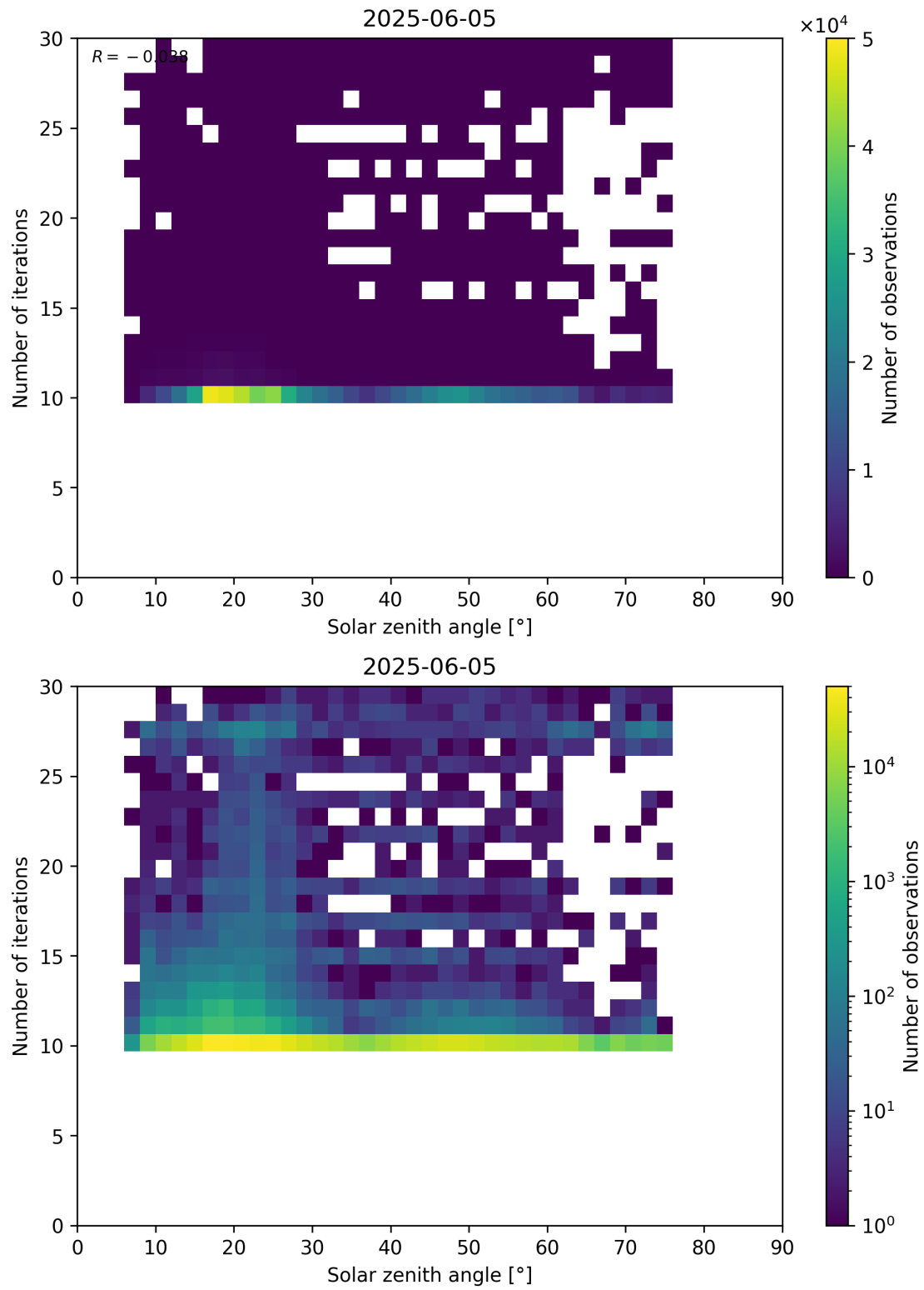
Figure 102: Scatter density plot of “Solar zenith angle” against “Number of iterations” for 2025-06-04 to 2025-06-06.
