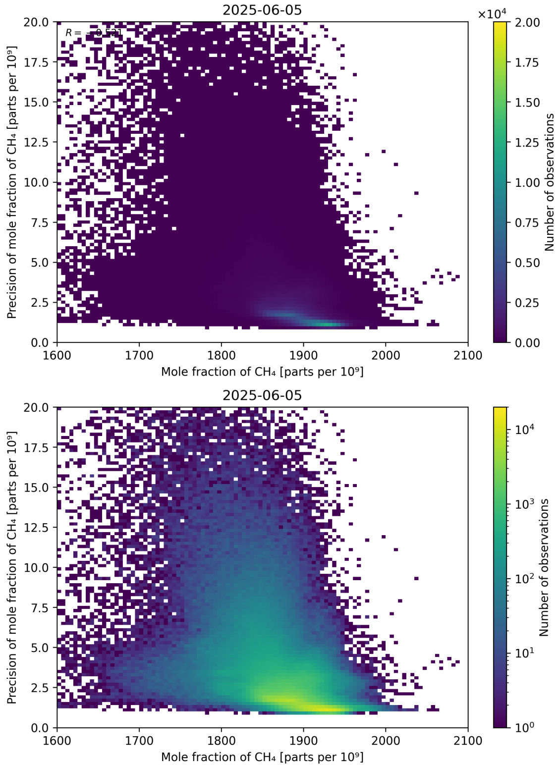
Figure 75: Scatter density plot of “Mole fraction of CH 4 ” against “Precision of mole fraction of CH 4 ” for 2025-06-04 to 2025-06-06.
