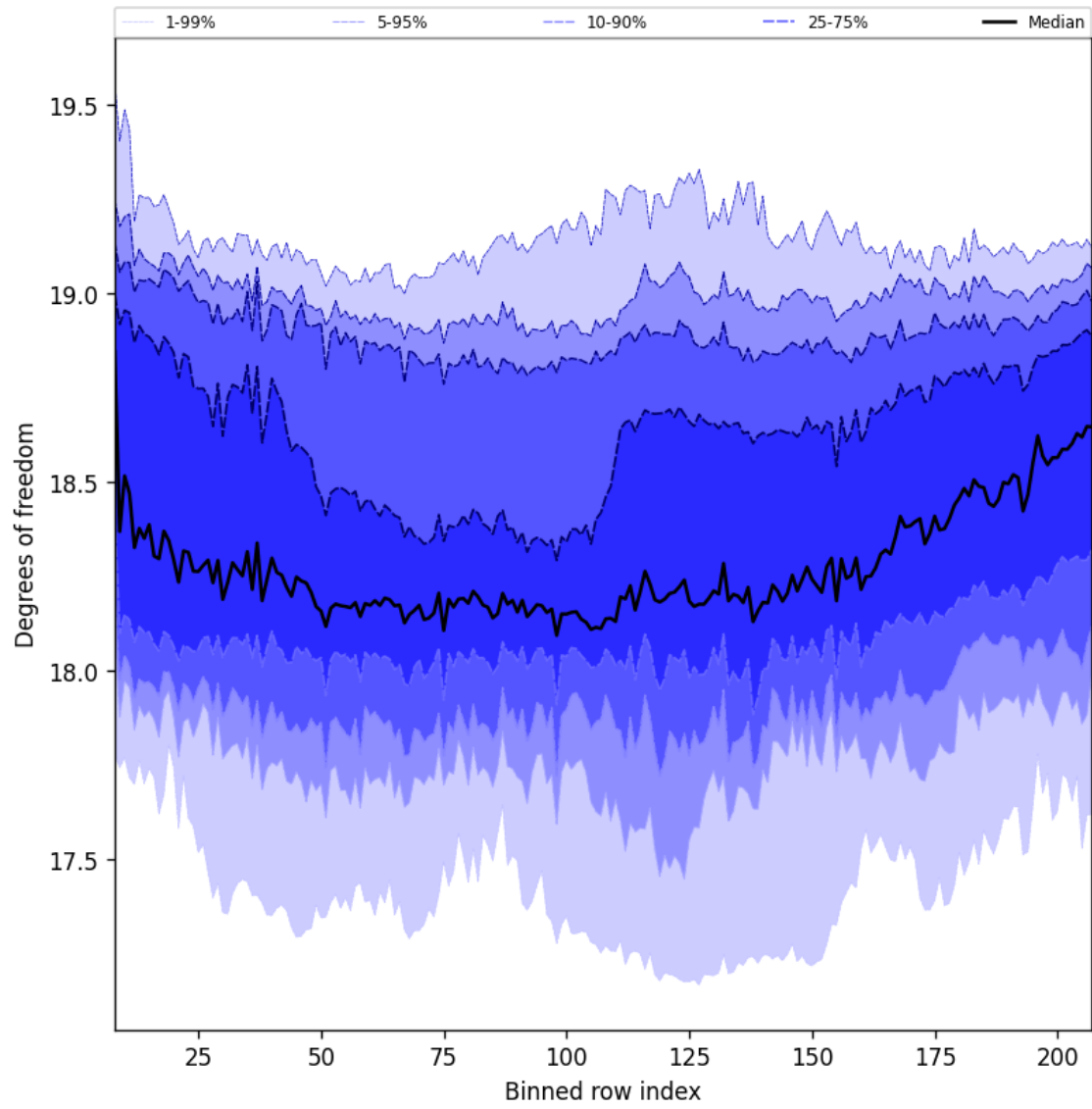
Figure 41: Along track statistics of “Degrees of freedom” for 2025-06-04 to 2025-06-06
