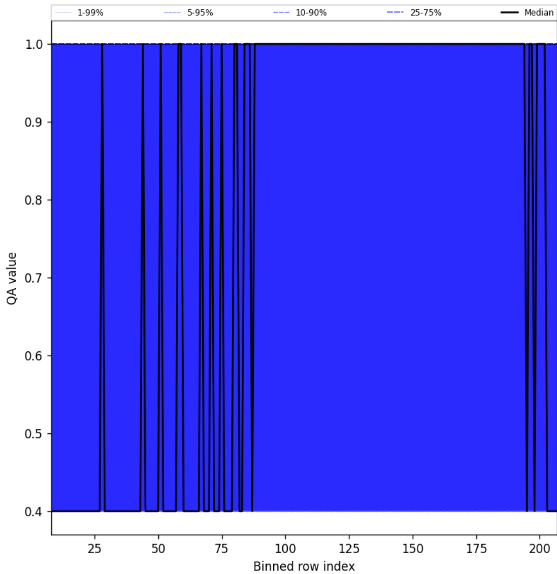
Figure 33: Along track statistics of “QA value” for 2025-06-04 to 2025-06-06
