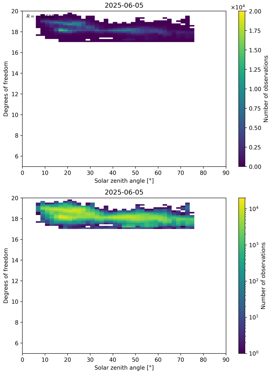
Figure 96: Scatter density plot of “Solar zenith angle” against “Degrees of freedom” for 2025-06-04 to 2025-06-06.
