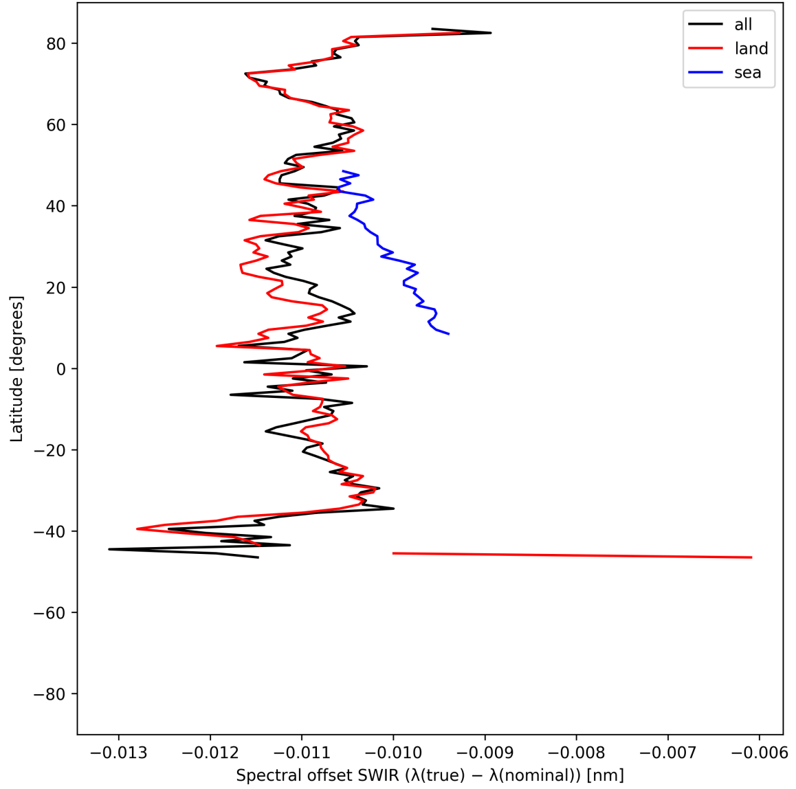
Figure 16: Zonal average of “Spectral offset SWIR ( \lambda_{\text{true}} - \lambda_{\text{nominal}} )” for 2025-06-04 to 2025-06-06.
