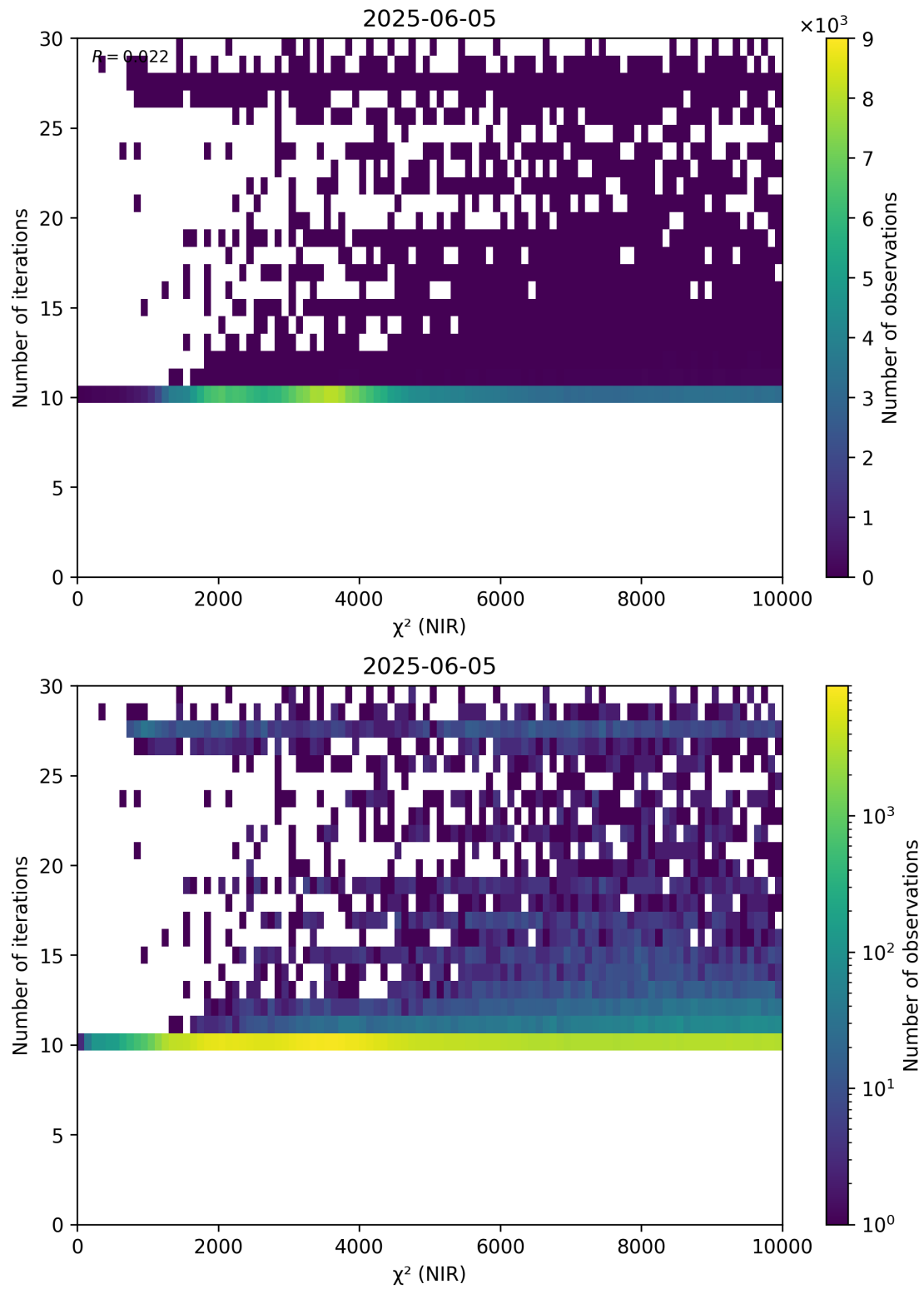
Figure 46: Scatter density plot of “ \chi^2 (NIR)” against “Number of iterations” for 2025-06-04 to 2025-06-06.
