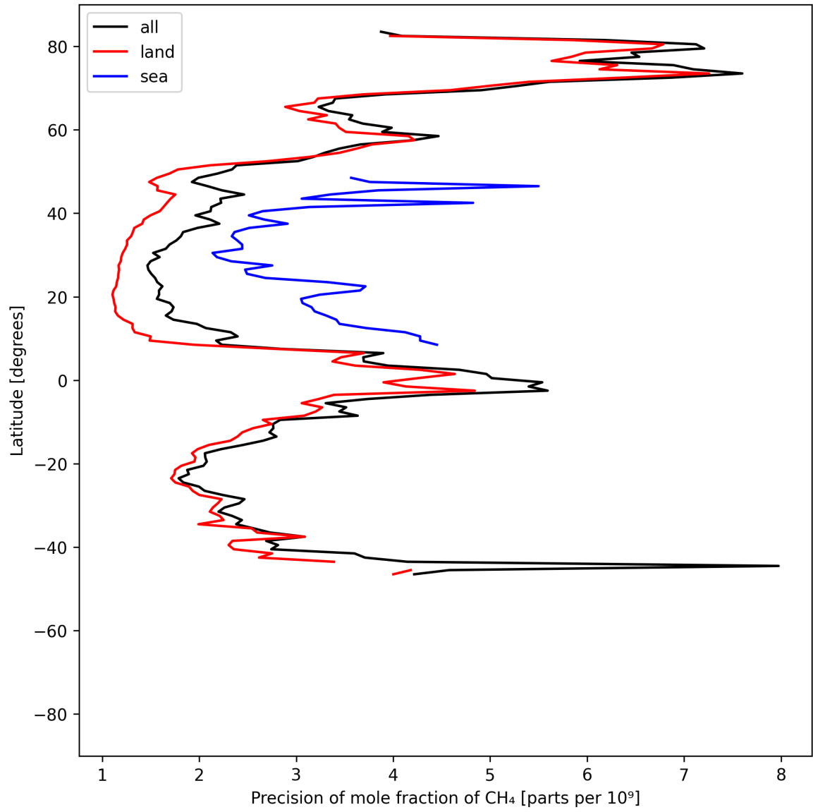
Figure 13: Zonal average of “Precision of mole fraction of CH 4 ” for 2025-06-04 to 2025-06-06.
