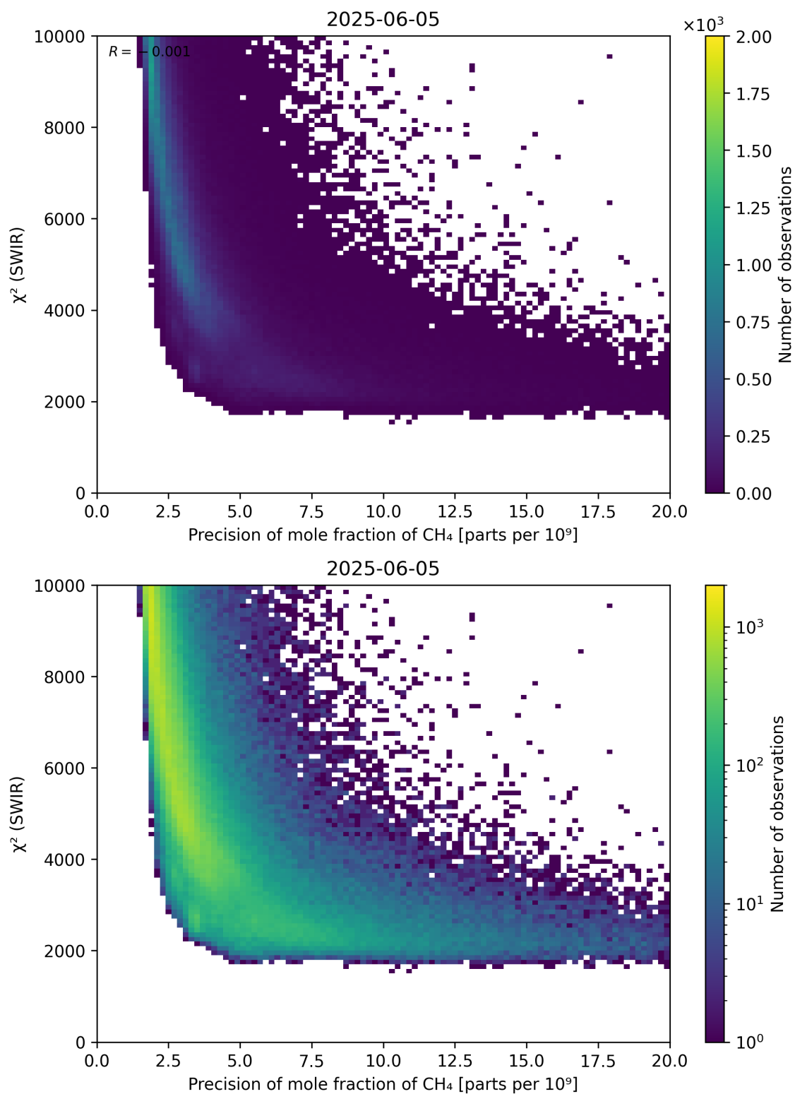
Figure 79: Scatter density plot of “Precision of mole fraction of CH 4 ” against “ \chi^2 (SWIR)” for 2025-06-04 to 2025-06-06.
