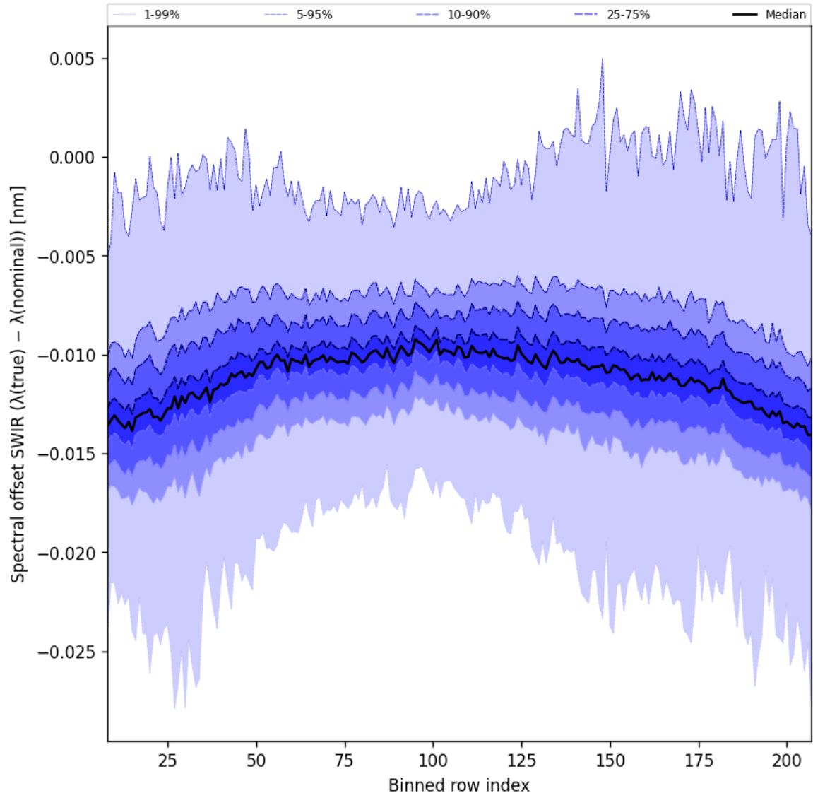
Figure 38: Along track statistics of “Spectral offset SWIR ( \lambda_{\text{true}} - \lambda_{\text{nominal}} )” for 2025-06-04 to 2025-06-06
