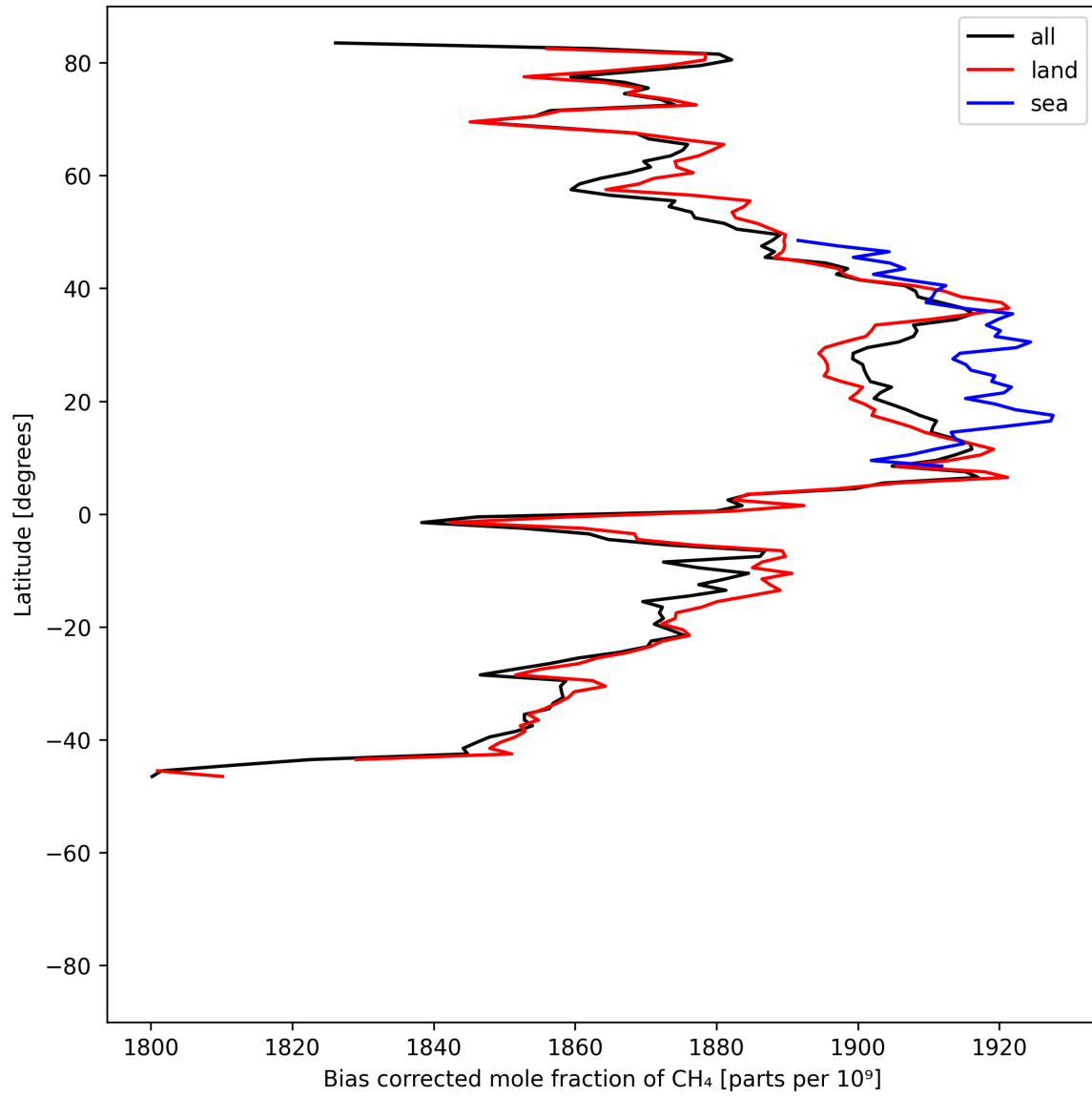
Figure 14: Zonal average of “Bias corrected mole fraction of CH 4 ” for 2025-06-04 to 2025-06-06.
