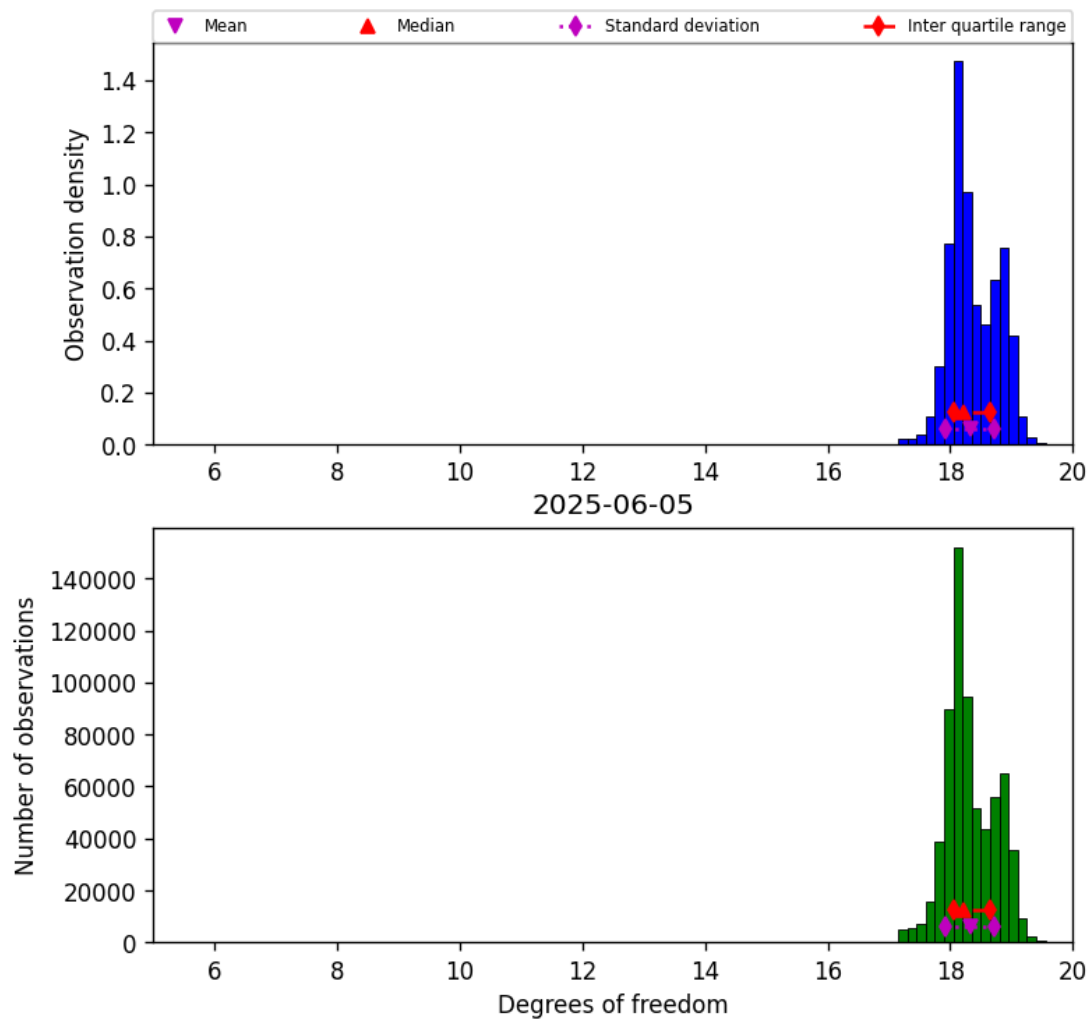
Figure 30: Histogram of “Degrees of freedom” for 2025-06-04 to 2025-06-06
