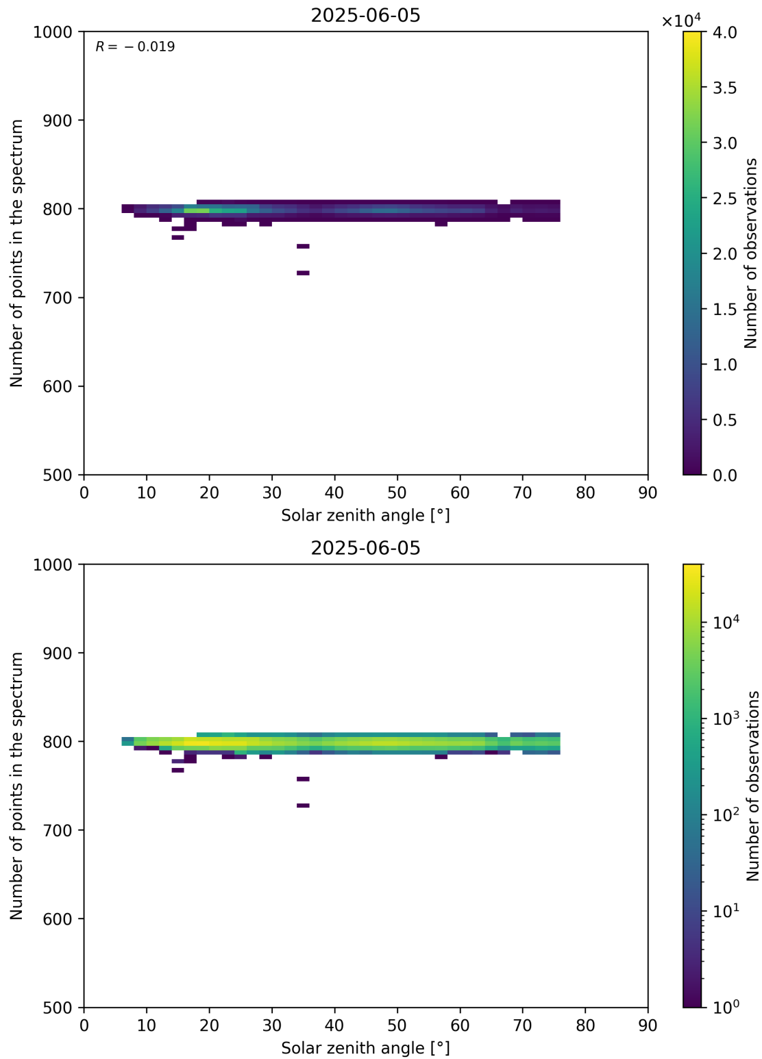
Figure 103: Scatter density plot of “Solar zenith angle” against “Number of points in the spectrum” for 2025-06-04 to 2025-06-06.
