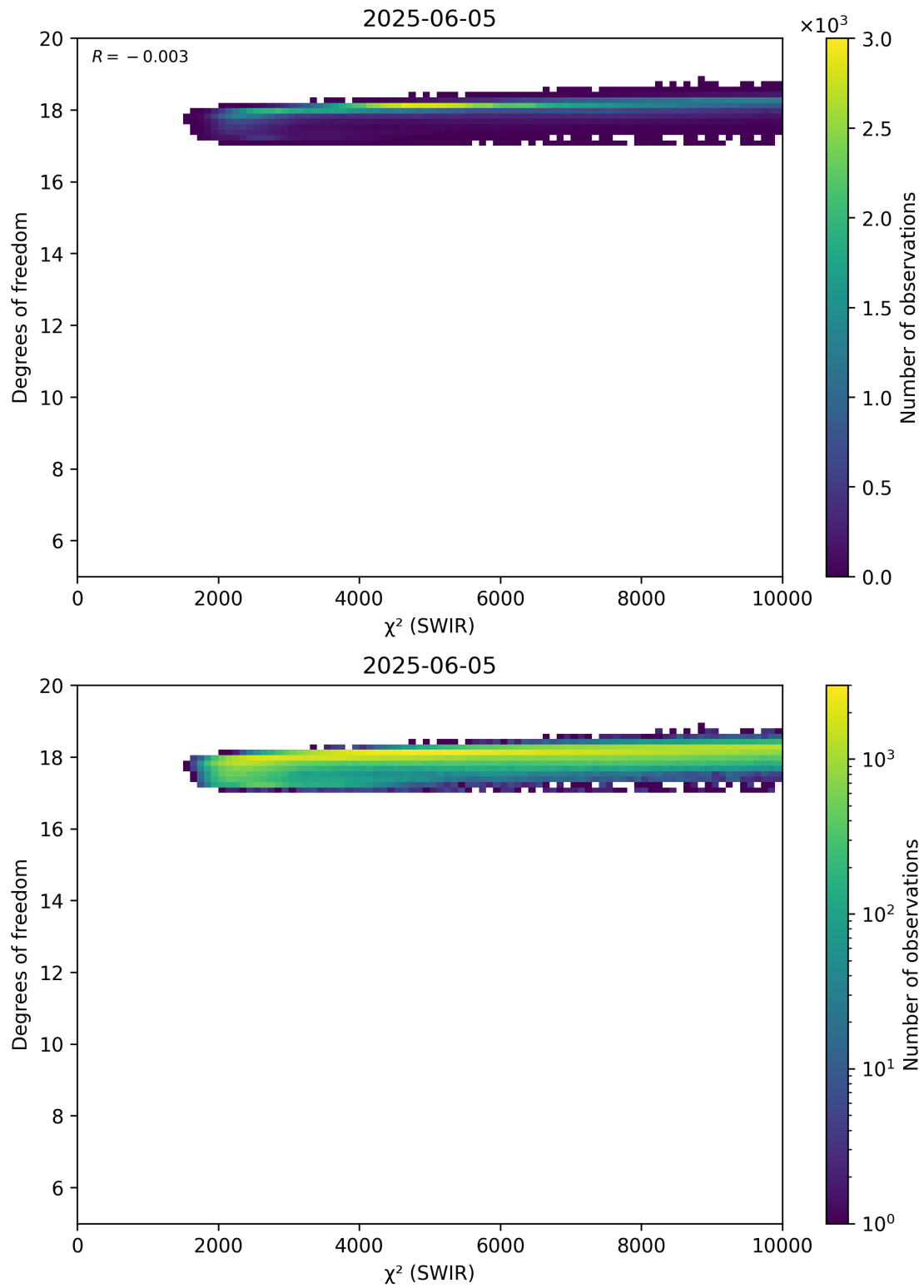
Figure 48: Scatter density plot of “ \chi^2 (SWIR)” against “Degrees of freedom” for 2025-06-04 to 2025-06-06.
