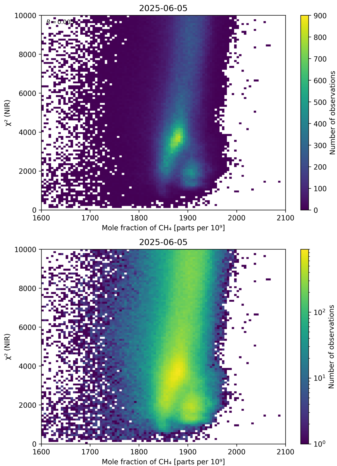
Figure 70: Scatter density plot of “Mole fraction of \text{CH}_4 ” against “ \chi^2 (NIR)” for 2025-06-04 to 2025-06-06.
