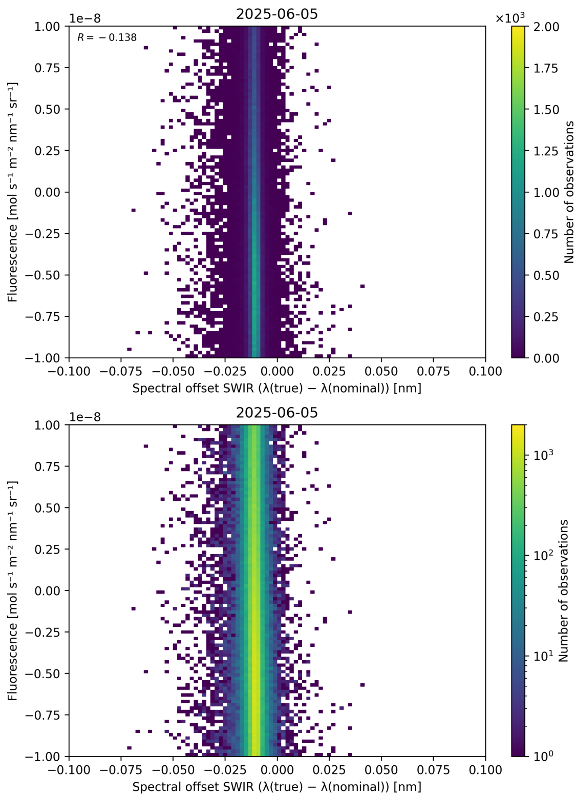
Figure 120: Scatter density plot of “Spectral offset SWIR ( \lambda_{\text{true}} - \lambda_{\text{nominal}} )” against “Fluorescence” for 2025-06-04 to 2025-06-06.
