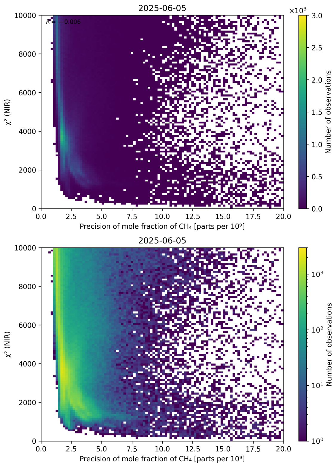
Figure 78: Scatter density plot of “Precision of mole fraction of CH 4 ” against “ \chi^2 (NIR)” for 2025-06-04 to 2025-06-06.
