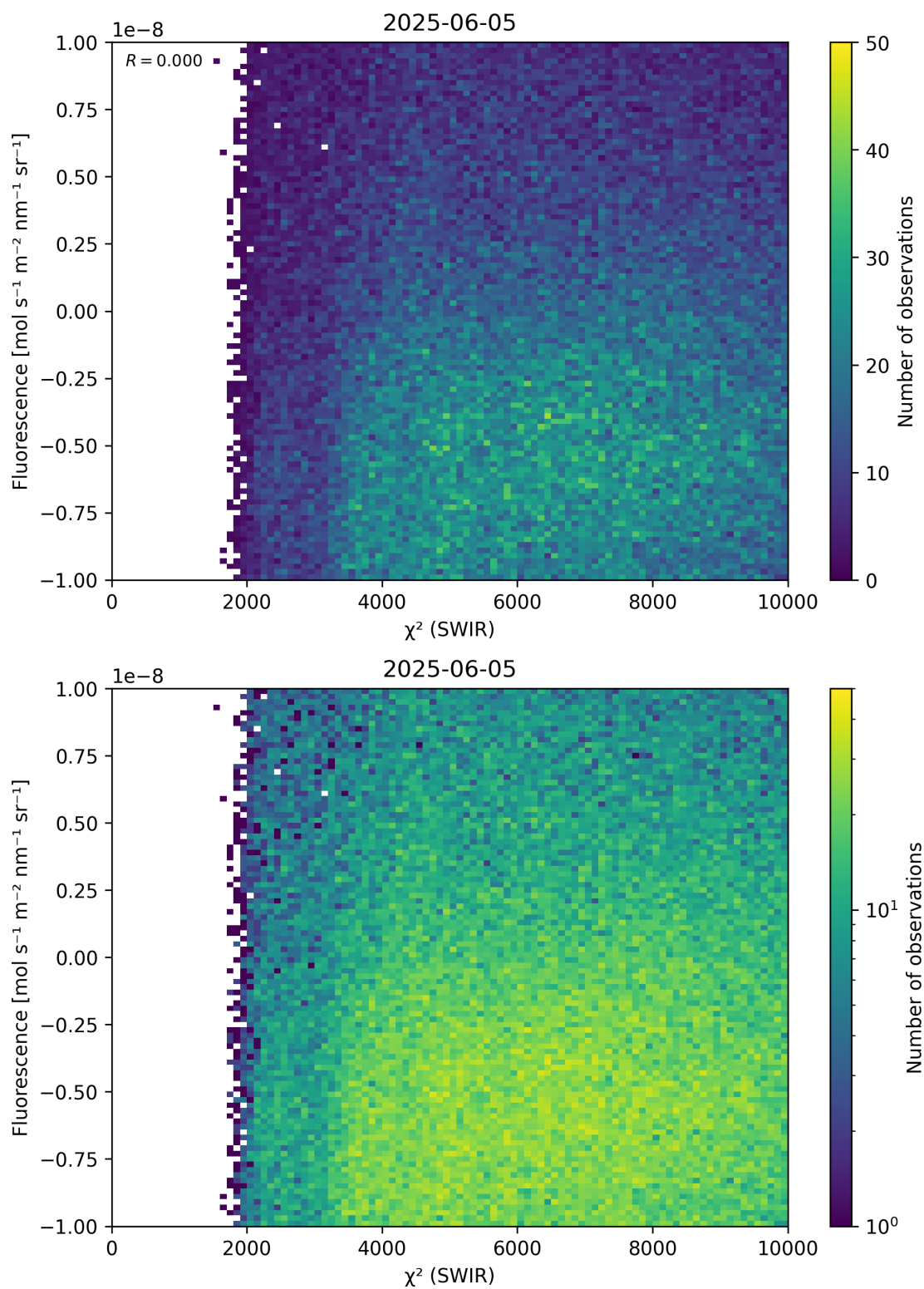
Figure 49: Scatter density plot of “ \chi^2 (SWIR)” against “Fluorescence” for 2025-06-04 to 2025-06-06.
