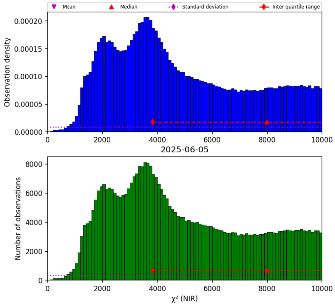
Figure 29: Histogram of “ \chi^2 (NIR)” for 2025-06-04 to 2025-06-06
