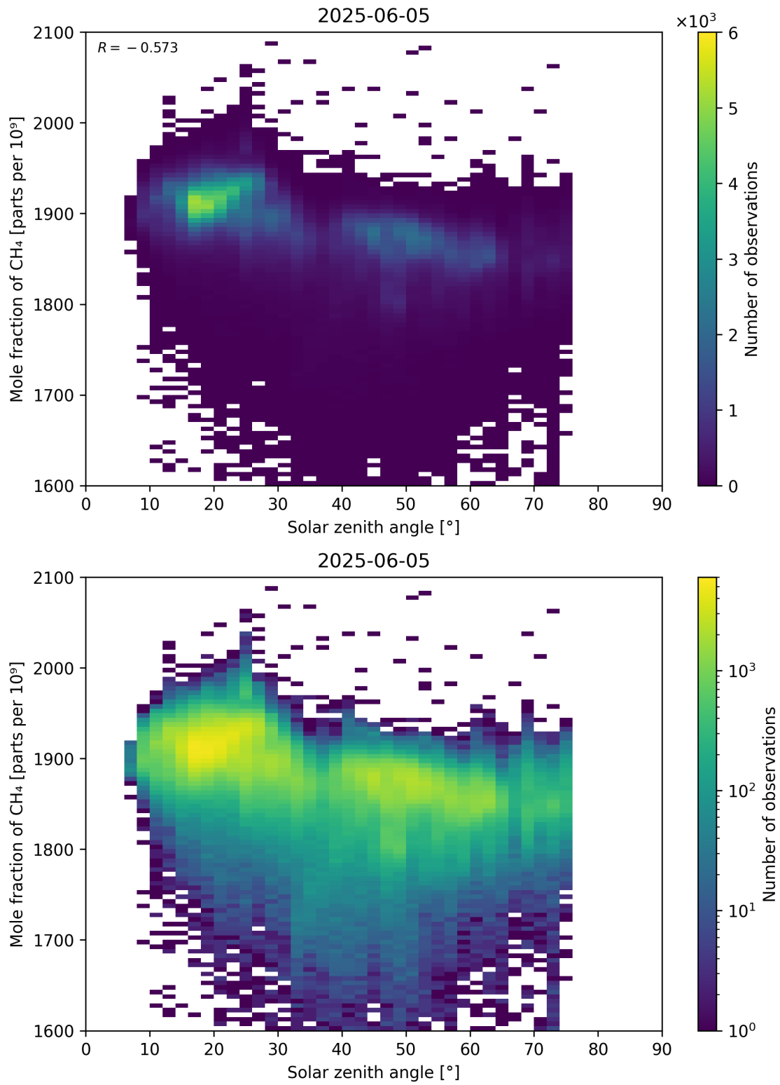
Figure 99: Scatter density plot of “Solar zenith angle” against “Mole fraction of CH 4 ” for 2025-06-04 to 2025-06-06.
