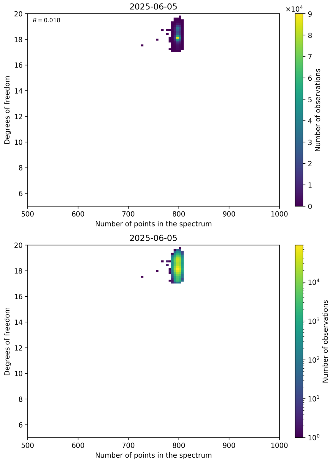
Figure 90: Scatter density plot of “Number of points in the spectrum” against “Degrees of freedom” for 2025-06-04 to 2025-06-06.
