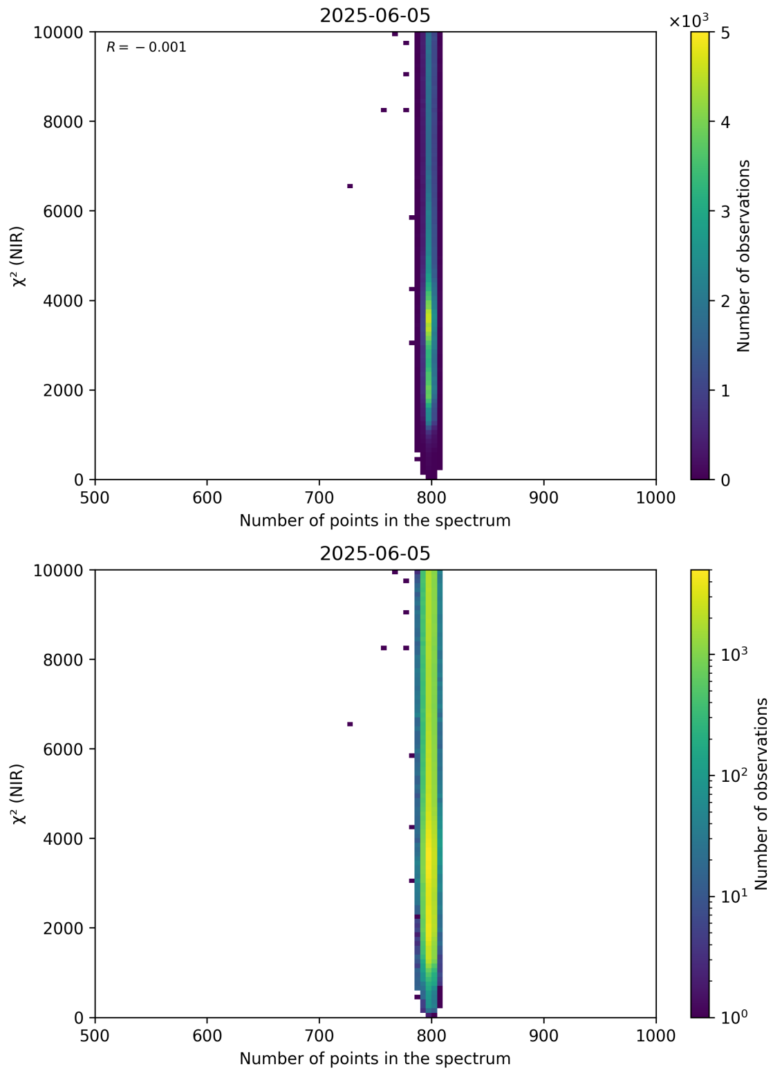
Figure 88: Scatter density plot of “Number of points in the spectrum” against “ \chi^2 (NIR)” for 2025-06-04 to 2025-06-06.
