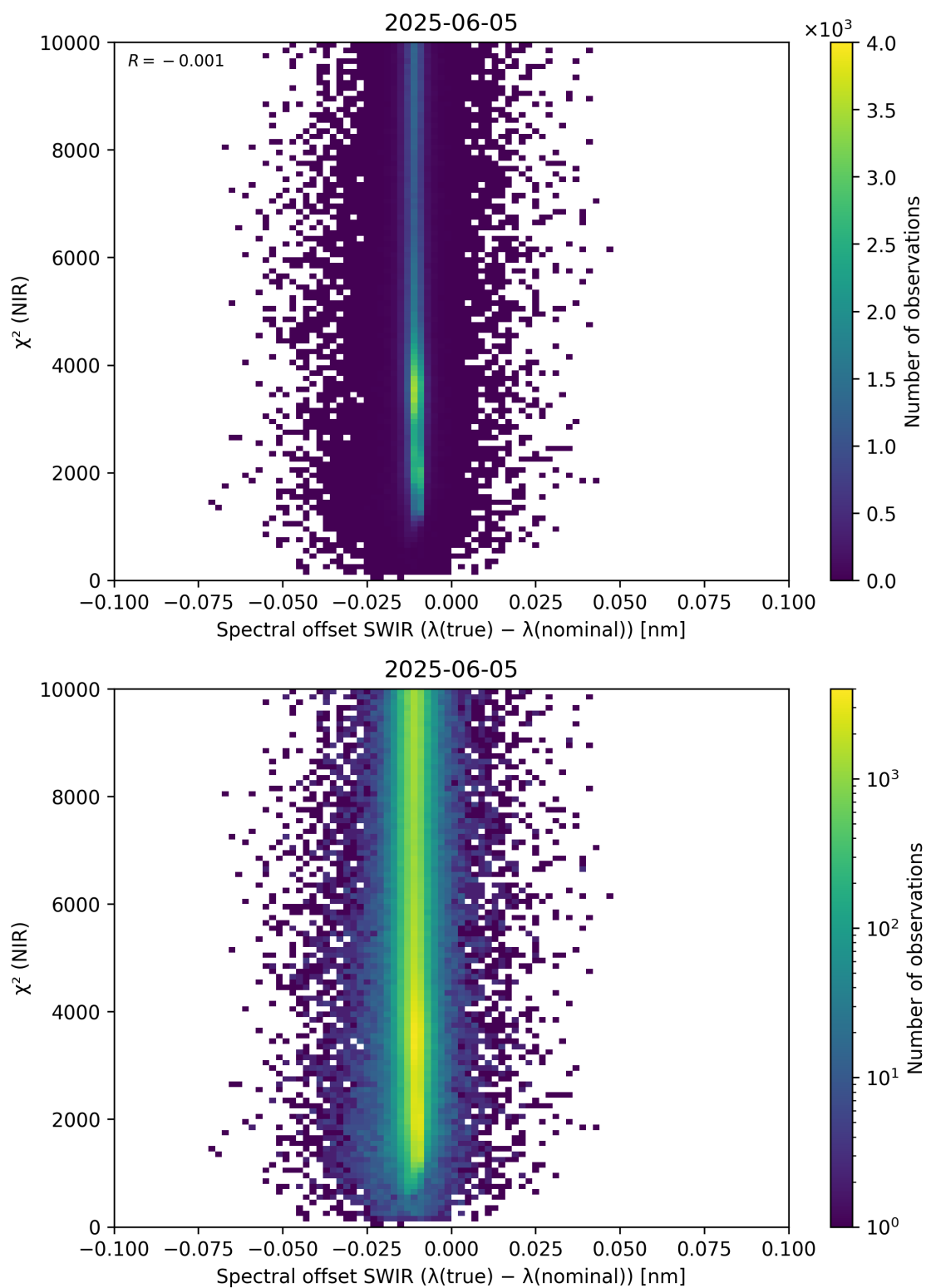
Figure 117: Scatter density plot of “Spectral offset SWIR ( \lambda_{\text{true}} - \lambda_{\text{nominal}} )” against “ \chi^2 (NIR)” for 2025-06-04 to 2025-06-06.
