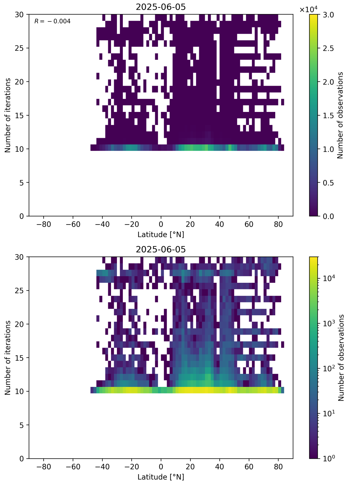
Figure 60: Scatter density plot of “Latitude” against “Number of iterations” for 2025-06-04 to 2025-06-06.
