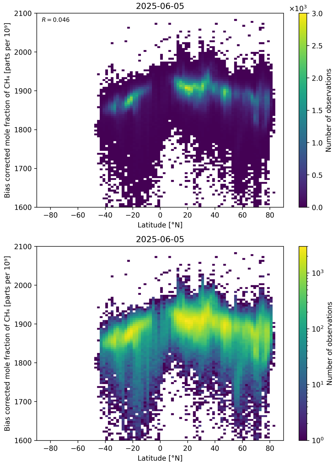
Figure 58: Scatter density plot of “Latitude” against “Bias corrected mole fraction of CH 4 ” for 2025-06-04 to 2025-06-06.
