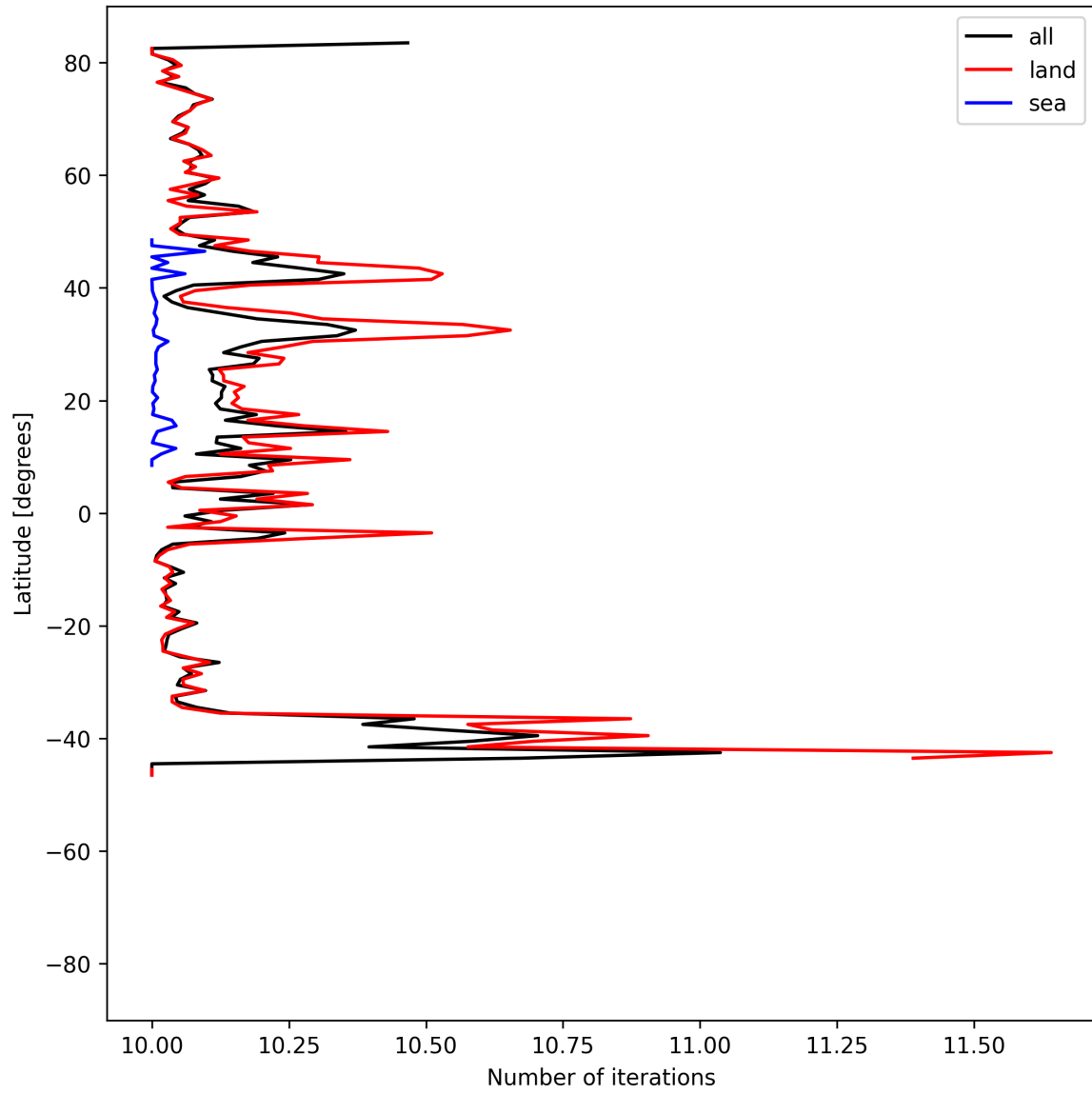
Figure 20: Zonal average of “Number of iterations” for 2025-06-04 to 2025-06-06.
