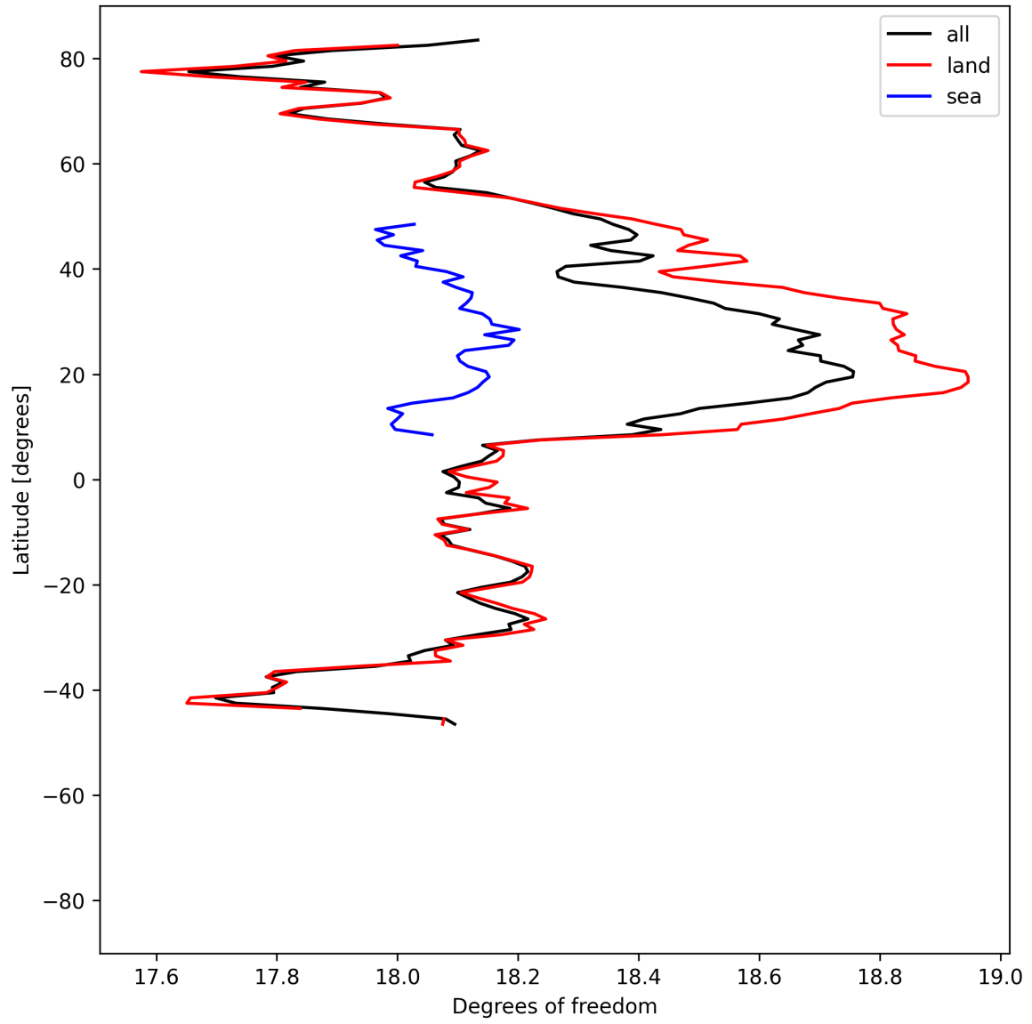
Figure 19: Zonal average of “Degrees of freedom” for 2025-06-04 to 2025-06-06.
