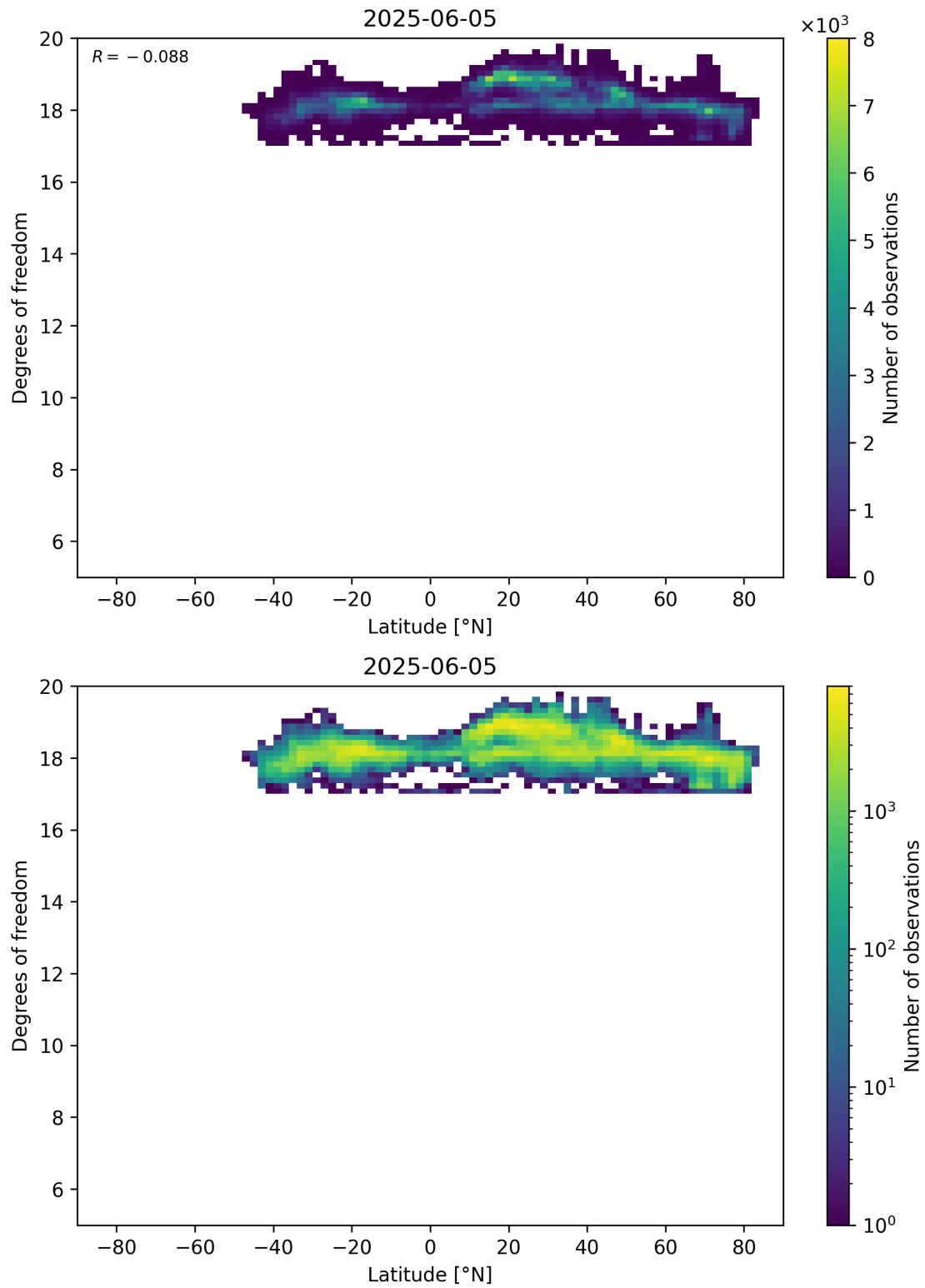
Figure 55: Scatter density plot of “Latitude” against “Degrees of freedom” for 2025-06-04 to 2025-06-06.
