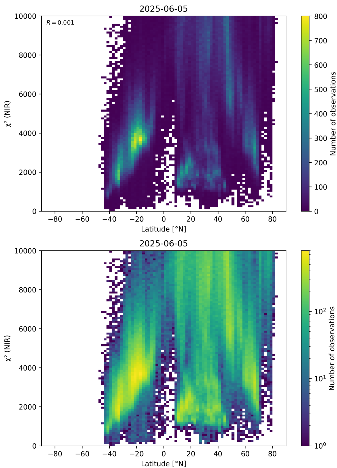
Figure 53: Scatter density plot of “Latitude” against “ \chi^2 (NIR)” for 2025-06-04 to 2025-06-06.
