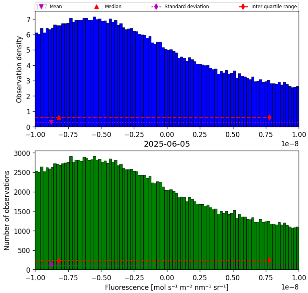
Figure 32: Histogram of “Fluorescence” for 2025-06-04 to 2025-06-06
