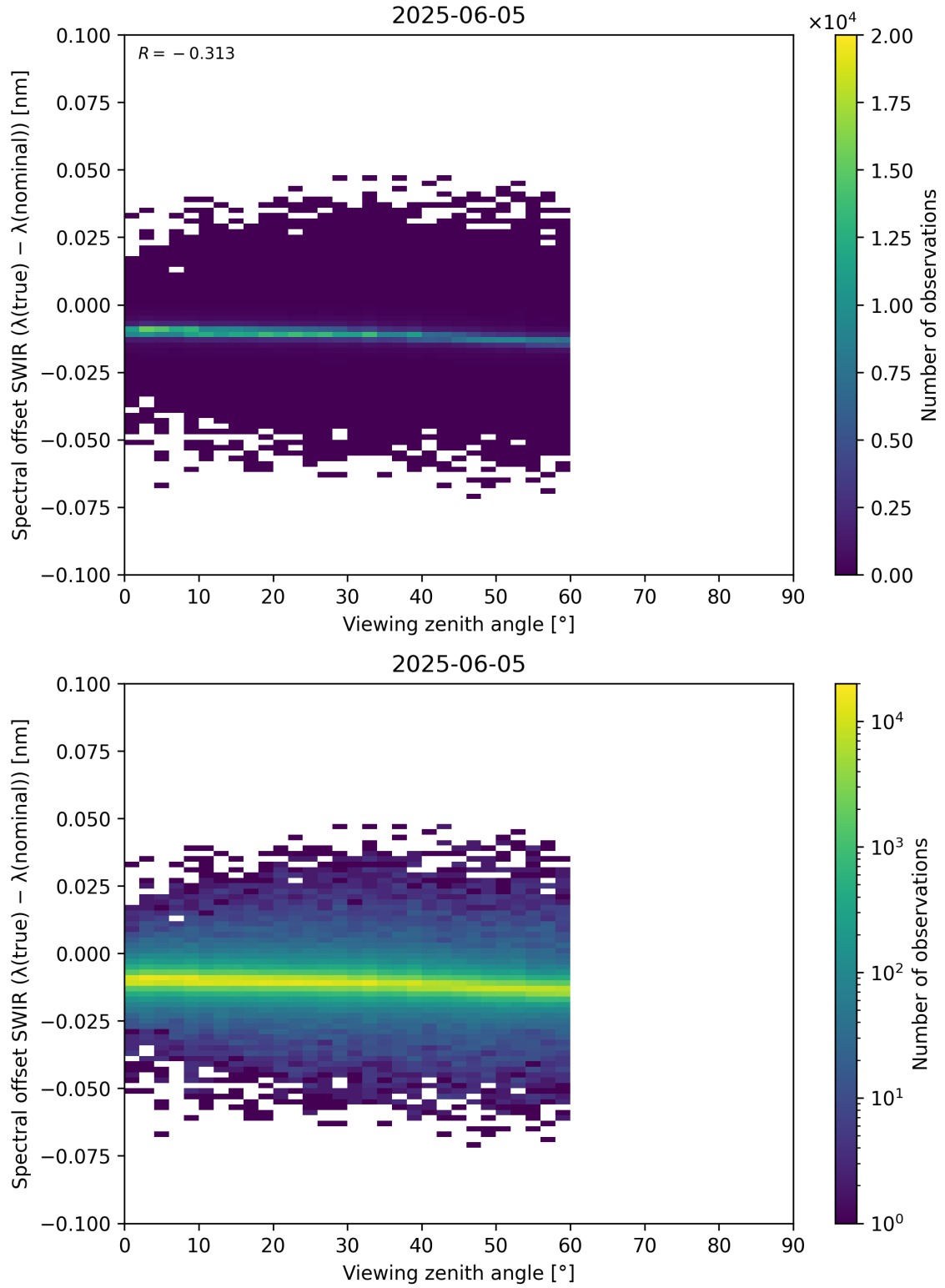
Figure 116: Scatter density plot of “Viewing zenith angle” against “Spectral offset SWIR ( \lambda_{\text{true}} - \lambda_{\text{nominal}} )” for 2025-06-04 to 2025-06-06.
