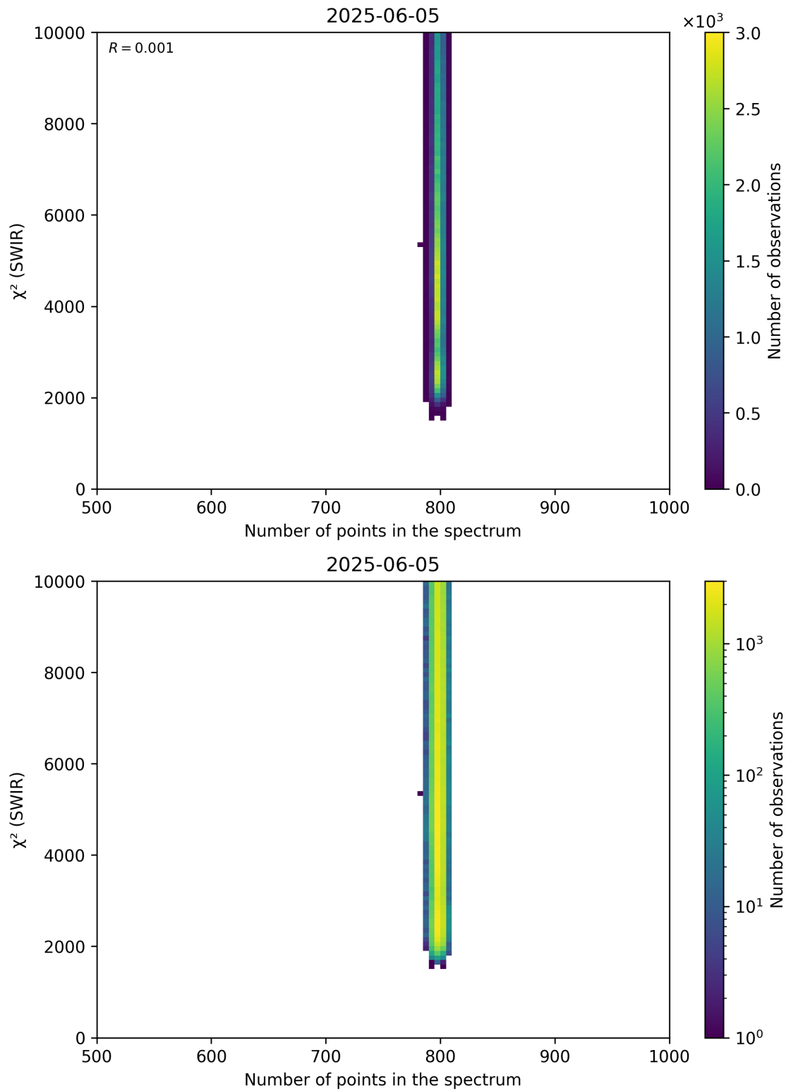
Figure 89: Scatter density plot of “Number of points in the spectrum” against “ \chi^2 (SWIR)” for 2025-06-04 to 2025-06-06.
