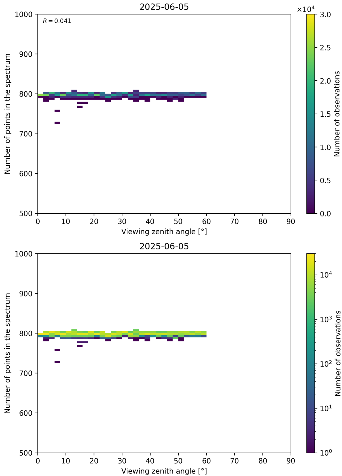
Figure 114: Scatter density plot of “Viewing zenith angle” against “Number of points in the spectrum” for 2025-06-04 to 2025-06-06.
