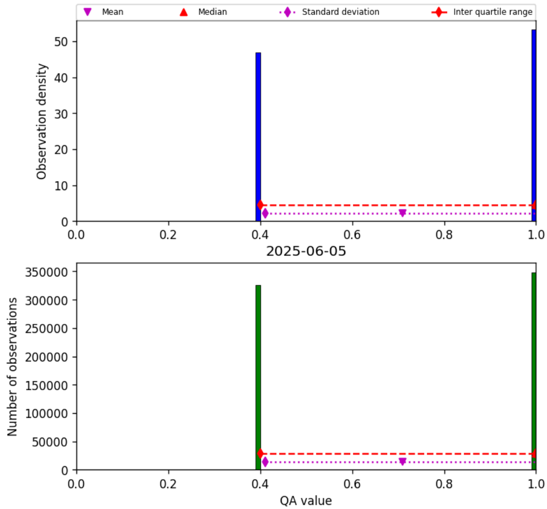
Figure 22: Histogram of “QA value” for 2025-06-04 to 2025-06-06
