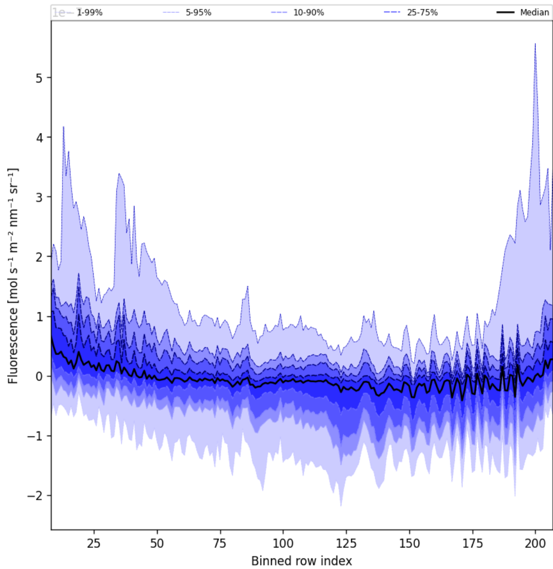
Figure 43: Along track statistics of “Fluorescence” for 2025-06-04 to 2025-06-06
