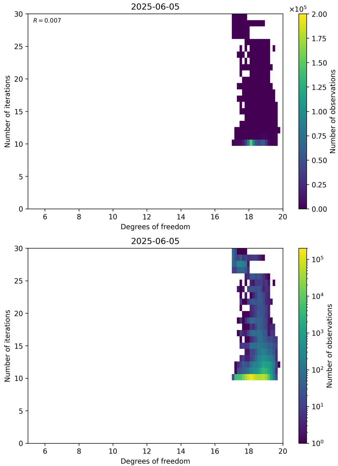
Figure 52: Scatter density plot of “Degrees of freedom” against “Number of iterations” for 2025-06-04 to 2025-06-06.
