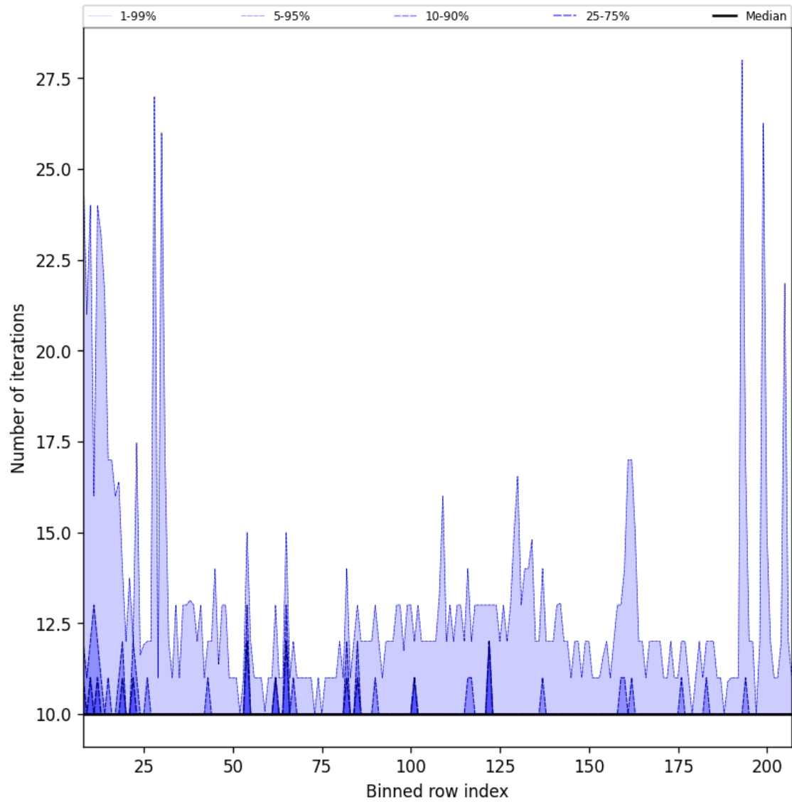
Figure 42: Along track statistics of “Number of iterations” for 2025-06-04 to 2025-06-06
