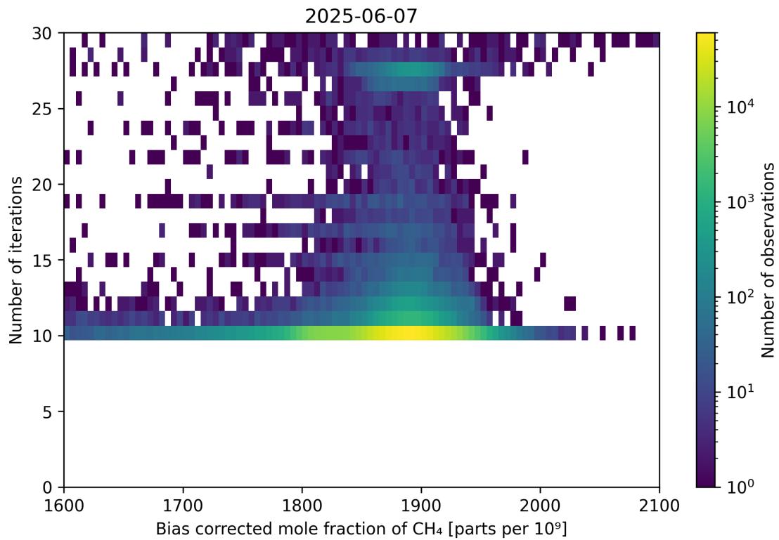
Figure 67: Scatter density plot of “Bias corrected mole fraction of CH 4 ” against “Number of iterations” for 2025-06-06 to 2025-06-08.
