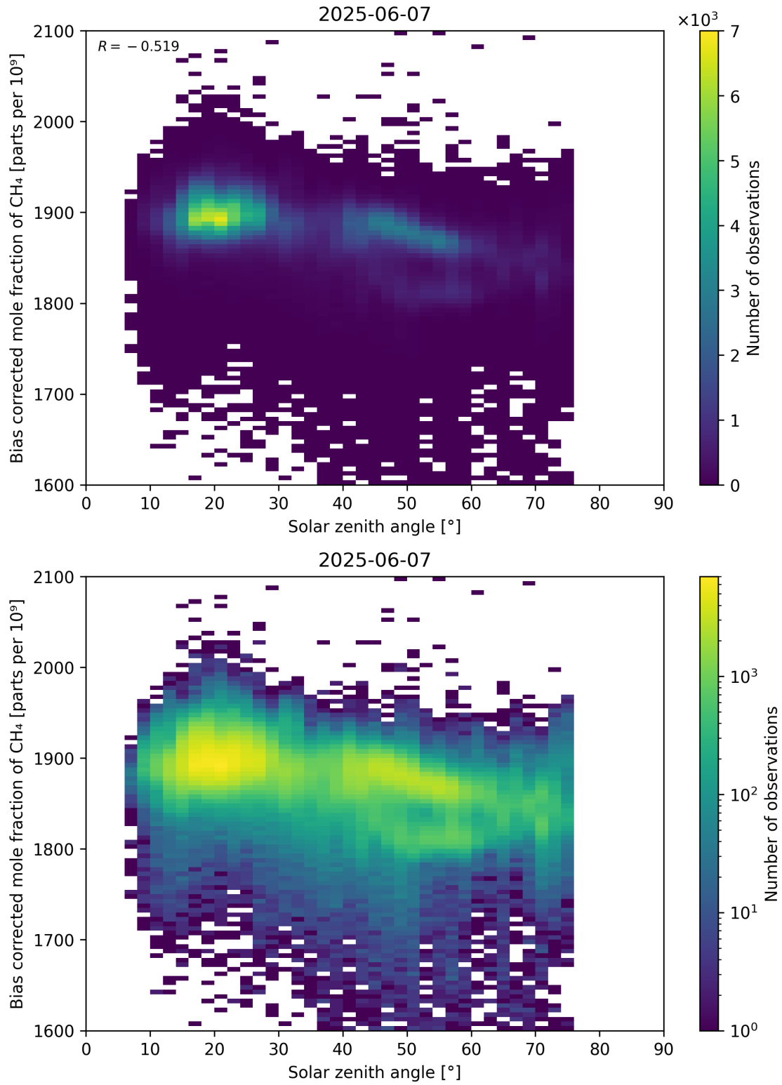
Figure 100: Scatter density plot of “Solar zenith angle” against “Bias corrected mole fraction of CH 4 ” for 2025-06-06 to 2025-06-08.
