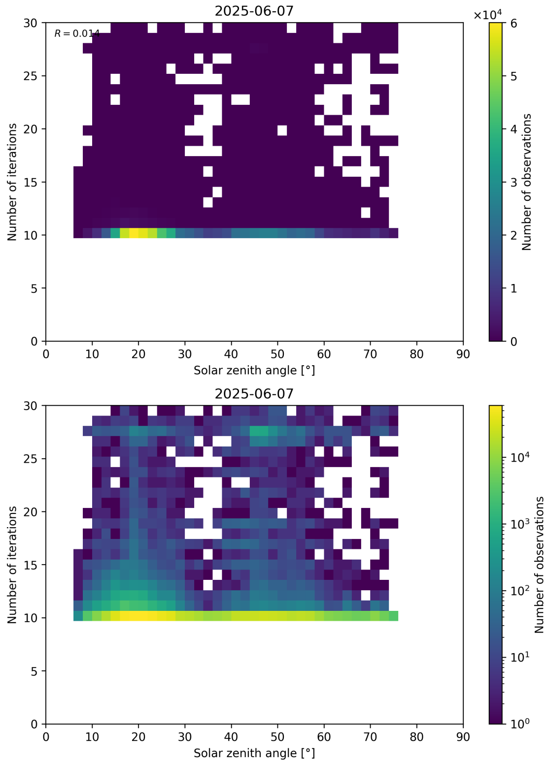
Figure 102: Scatter density plot of “Solar zenith angle” against “Number of iterations” for 2025-06-06 to 2025-06-08.
