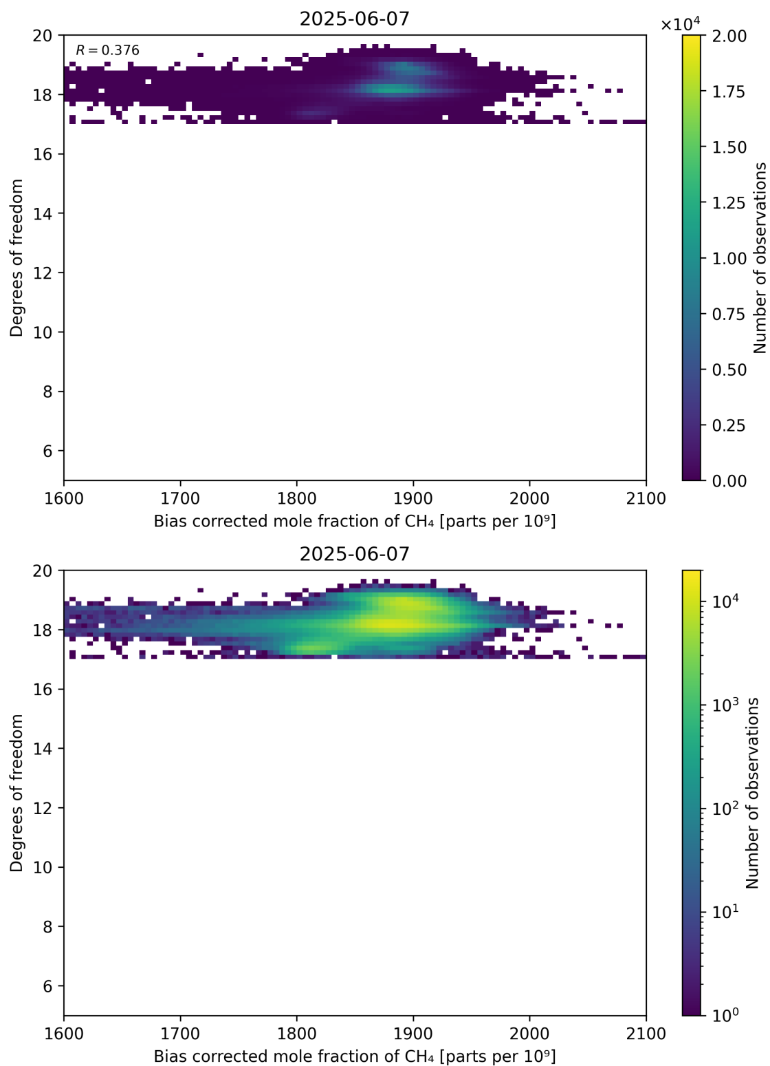
Figure 65: Scatter density plot of “Bias corrected mole fraction of CH 4 ” against “Degrees of freedom” for 2025-06-06 to 2025-06-08.
