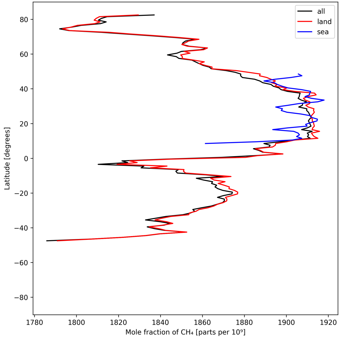
Figure 12: Zonal average of “Mole fraction of \text{CH}_4 ” for 2025-06-06 to 2025-06-08.
