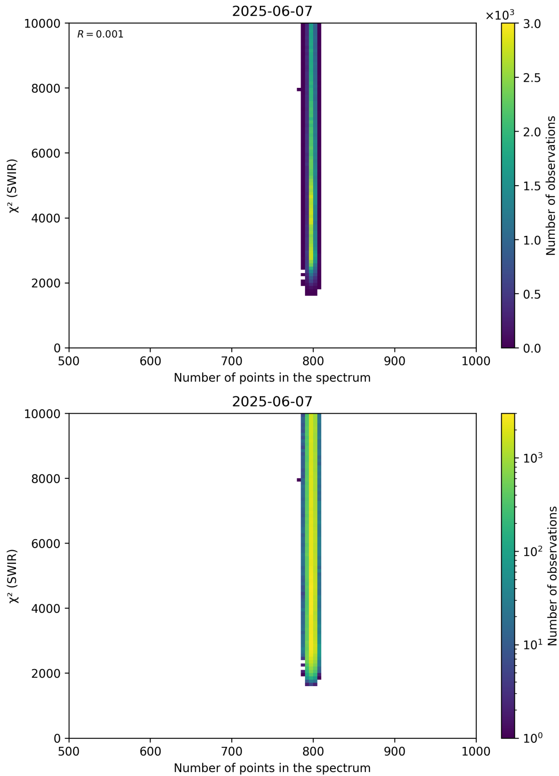
Figure 89: Scatter density plot of “Number of points in the spectrum” against “ \chi^2 (SWIR)” for 2025-06-06 to 2025-06-08.
