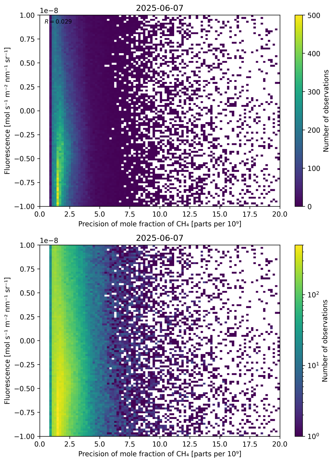
Figure 81: Scatter density plot of “Precision of mole fraction of \text{CH}_4 ” against “Fluorescence” for 2025-06-06 to 2025-06-08.
