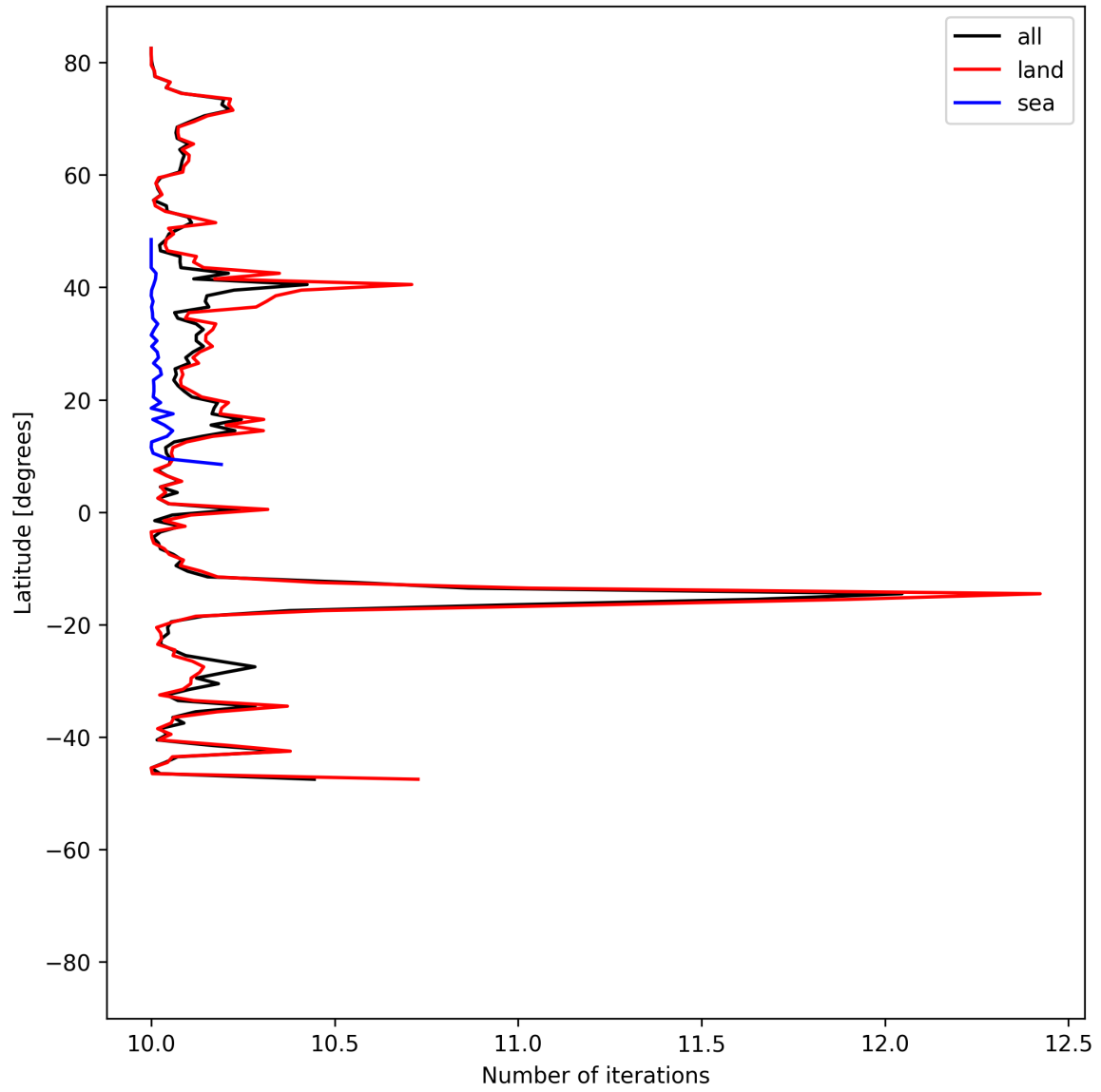
Figure 20: Zonal average of “Number of iterations” for 2025-06-06 to 2025-06-08.
