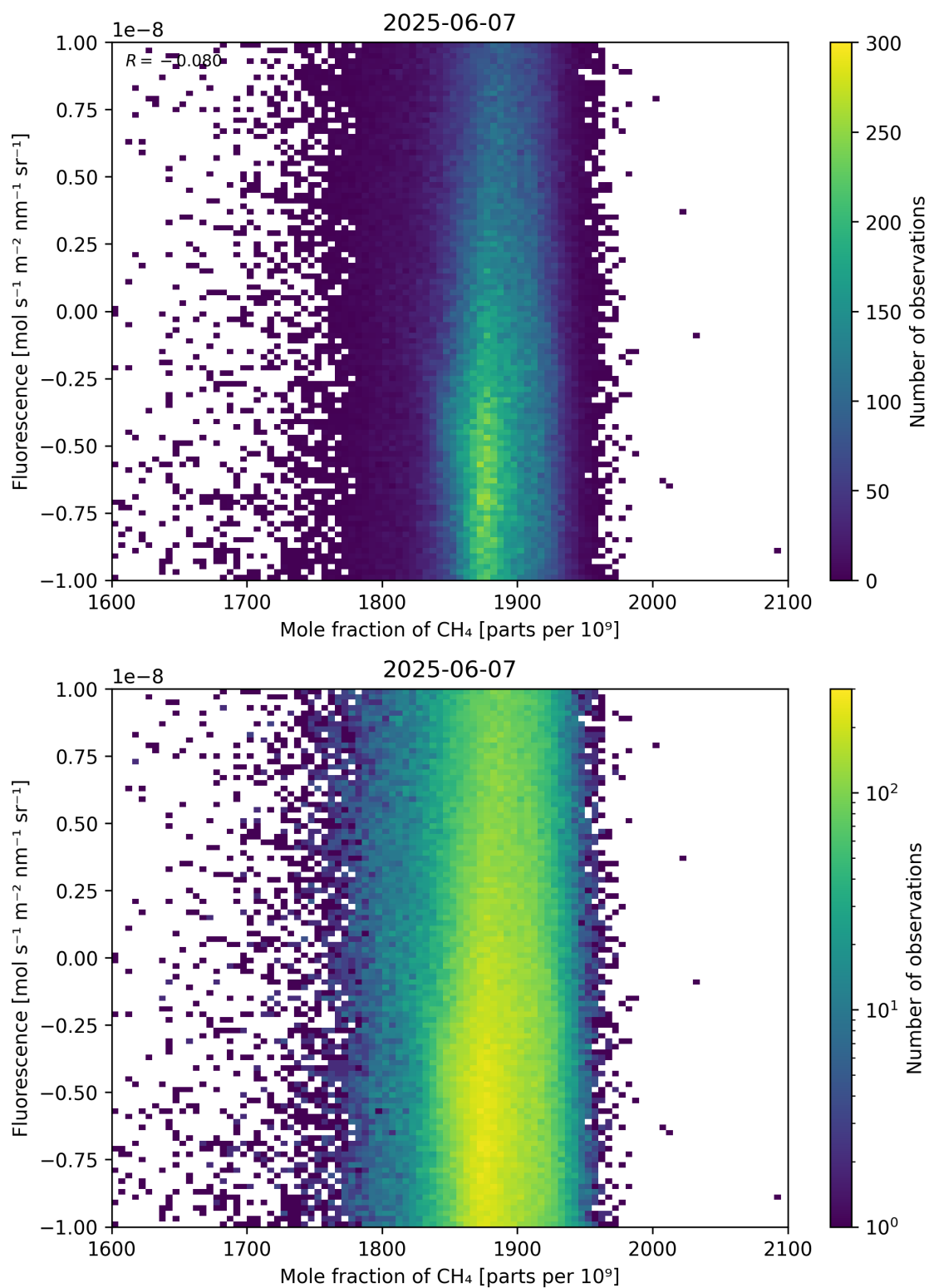
Figure 73: Scatter density plot of “Mole fraction of \text{CH}_4 ” against “Fluorescence” for 2025-06-06 to 2025-06-08.
