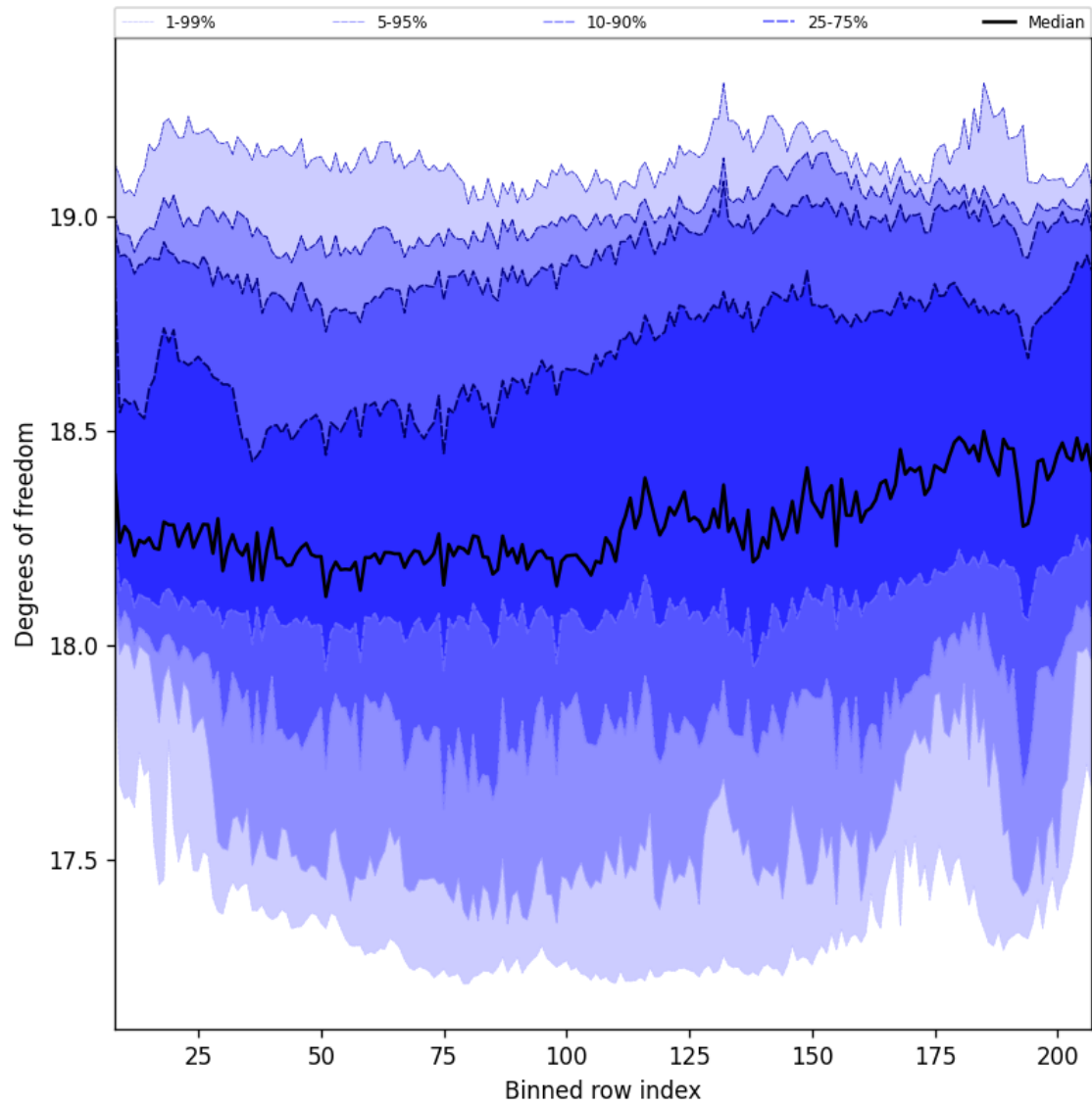
Figure 41: Along track statistics of “Degrees of freedom” for 2025-06-06 to 2025-06-08
