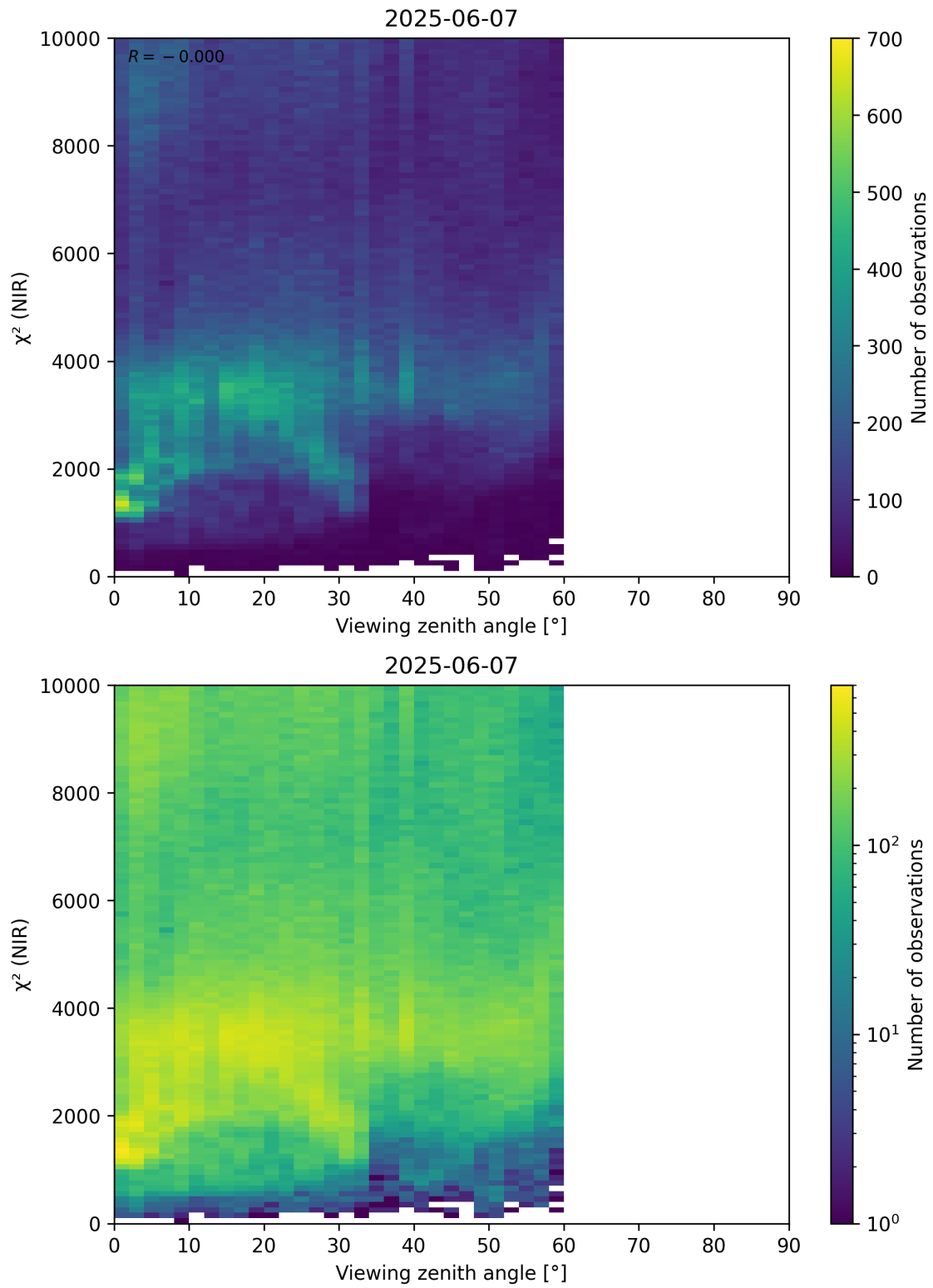
Figure 105: Scatter density plot of “Viewing zenith angle” against “ \chi^2 (NIR)” for 2025-06-06 to 2025-06-08.
