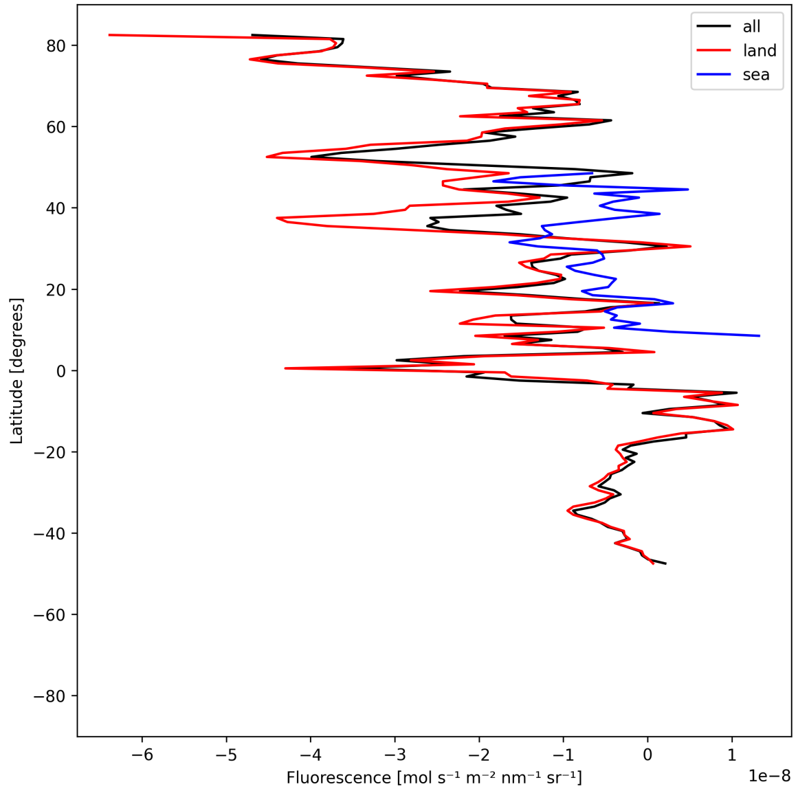
Figure 21: Zonal average of “Fluorescence” for 2025-06-06 to 2025-06-08.
