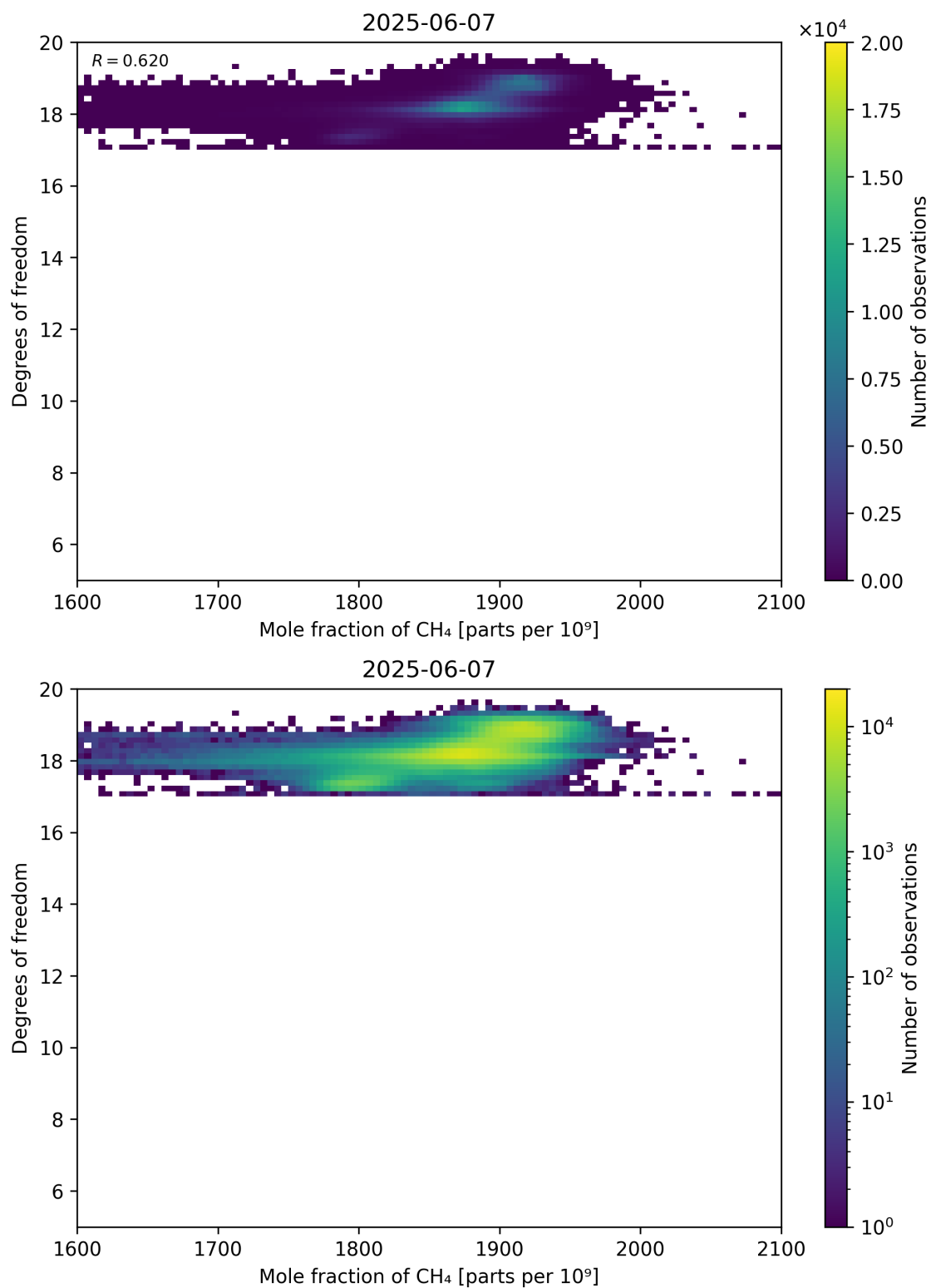
Figure 72: Scatter density plot of “Mole fraction of CH 4 ” against “Degrees of freedom” for 2025-06-06 to 2025-06-08.
