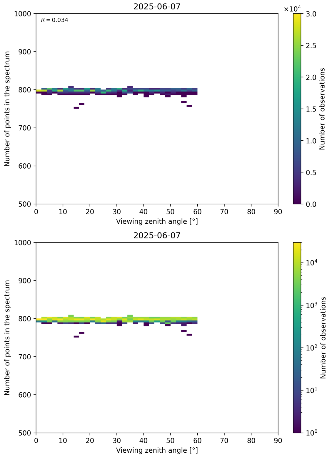
Figure 114: Scatter density plot of “Viewing zenith angle” against “Number of points in the spectrum” for 2025-06-06 to 2025-06-08.
