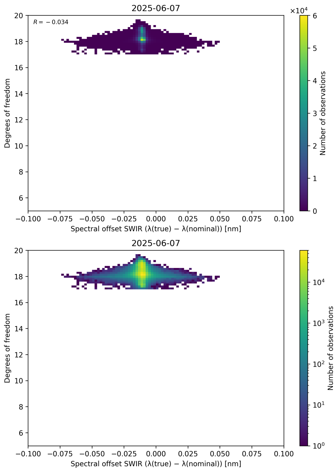
Figure 119: Scatter density plot of “Spectral offset SWIR ( \lambda_{\text{true}} - \lambda_{\text{nominal}} )” against “Degrees of freedom” for 2025-06-06 to 2025-06-08.
