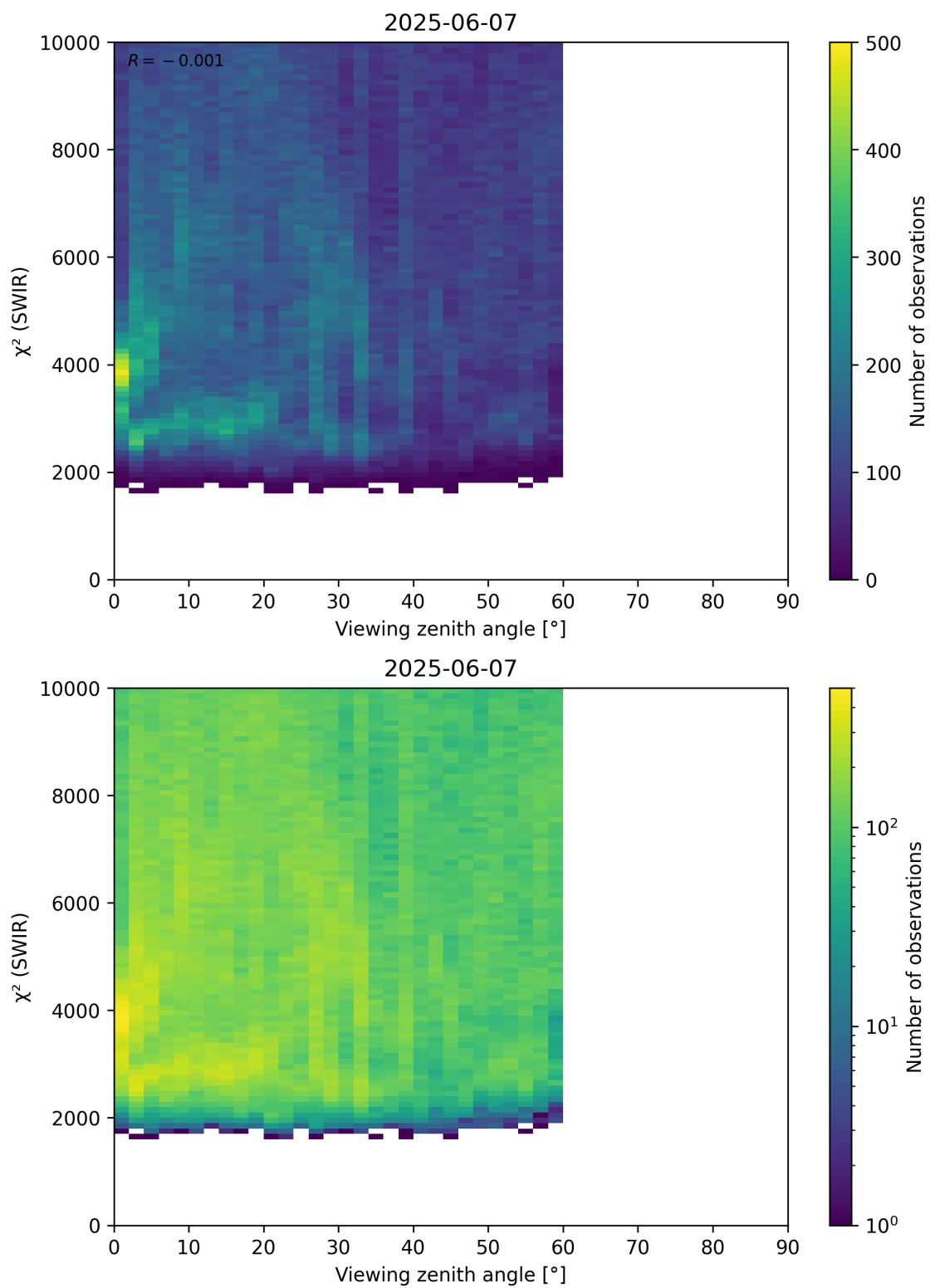
Figure 106: Scatter density plot of “Viewing zenith angle” against “ \chi^2 (SWIR)” for 2025-06-06 to 2025-06-08.
