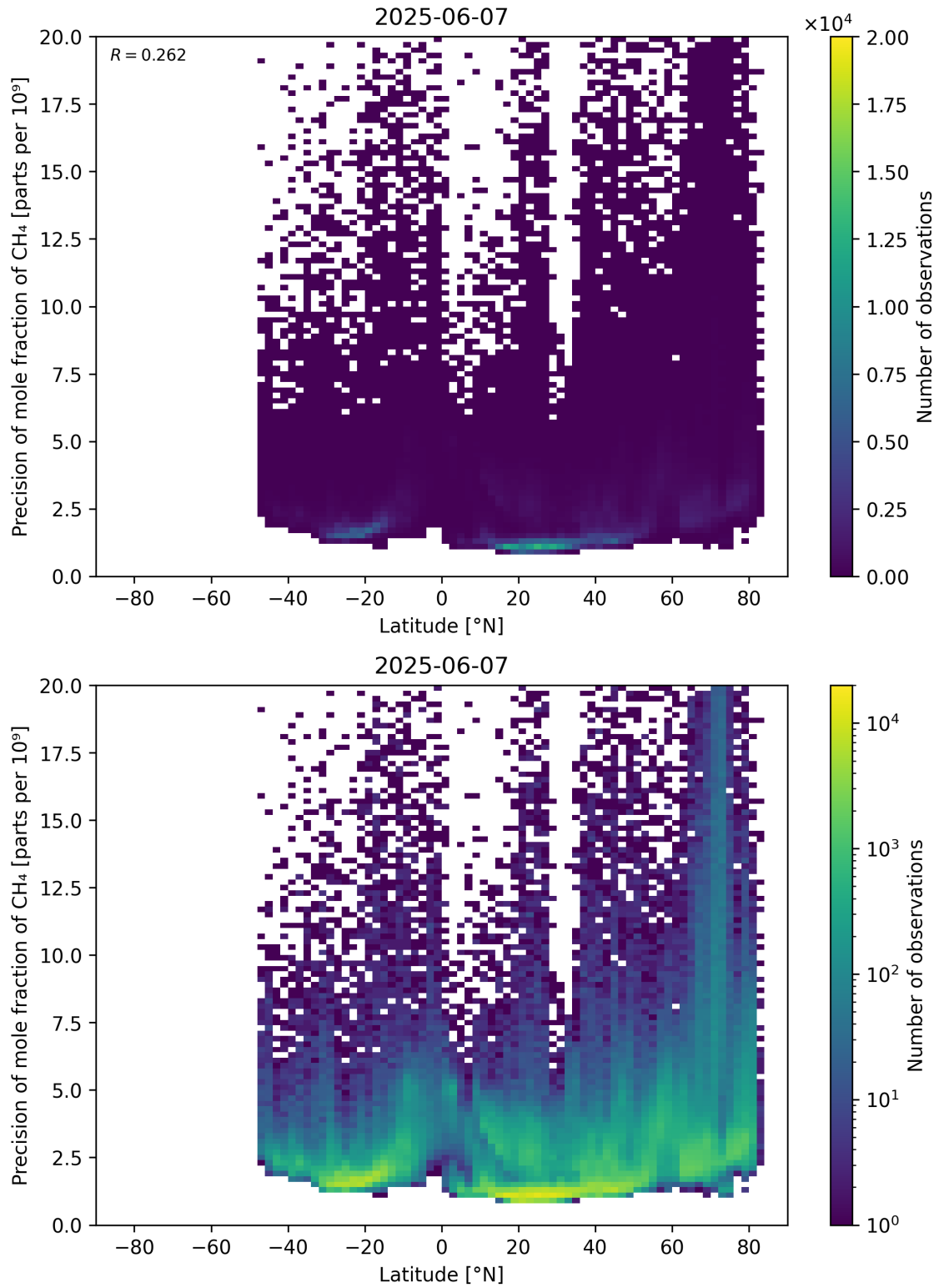
Figure 59: Scatter density plot of “Latitude” against “Precision of mole fraction of \text{CH}_4 ” for 2025-06-06 to 2025-06-08.
