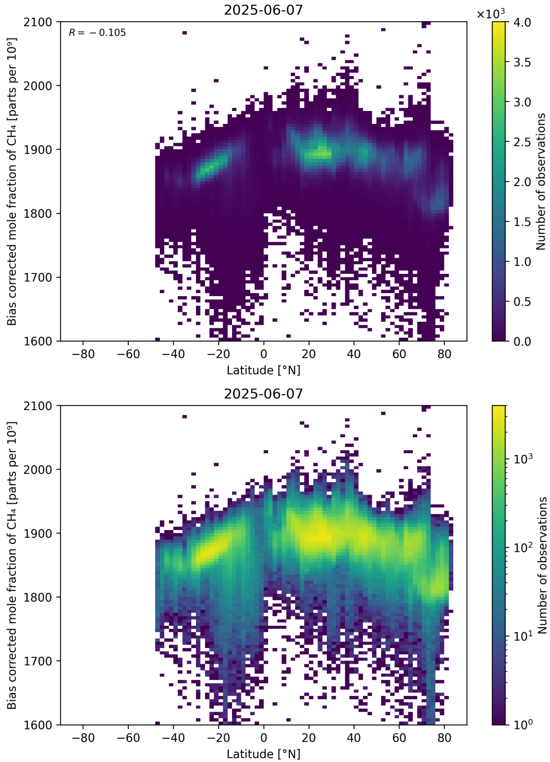
Figure 58: Scatter density plot of “Latitude” against “Bias corrected mole fraction of CH 4 ” for 2025-06-06 to 2025-06-08.
