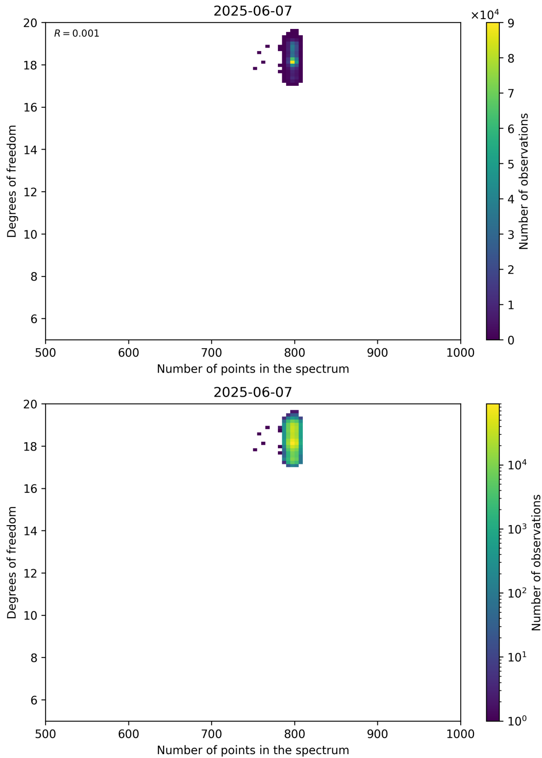
Figure 90: Scatter density plot of “Number of points in the spectrum” against “Degrees of freedom” for 2025-06-06 to 2025-06-08.
