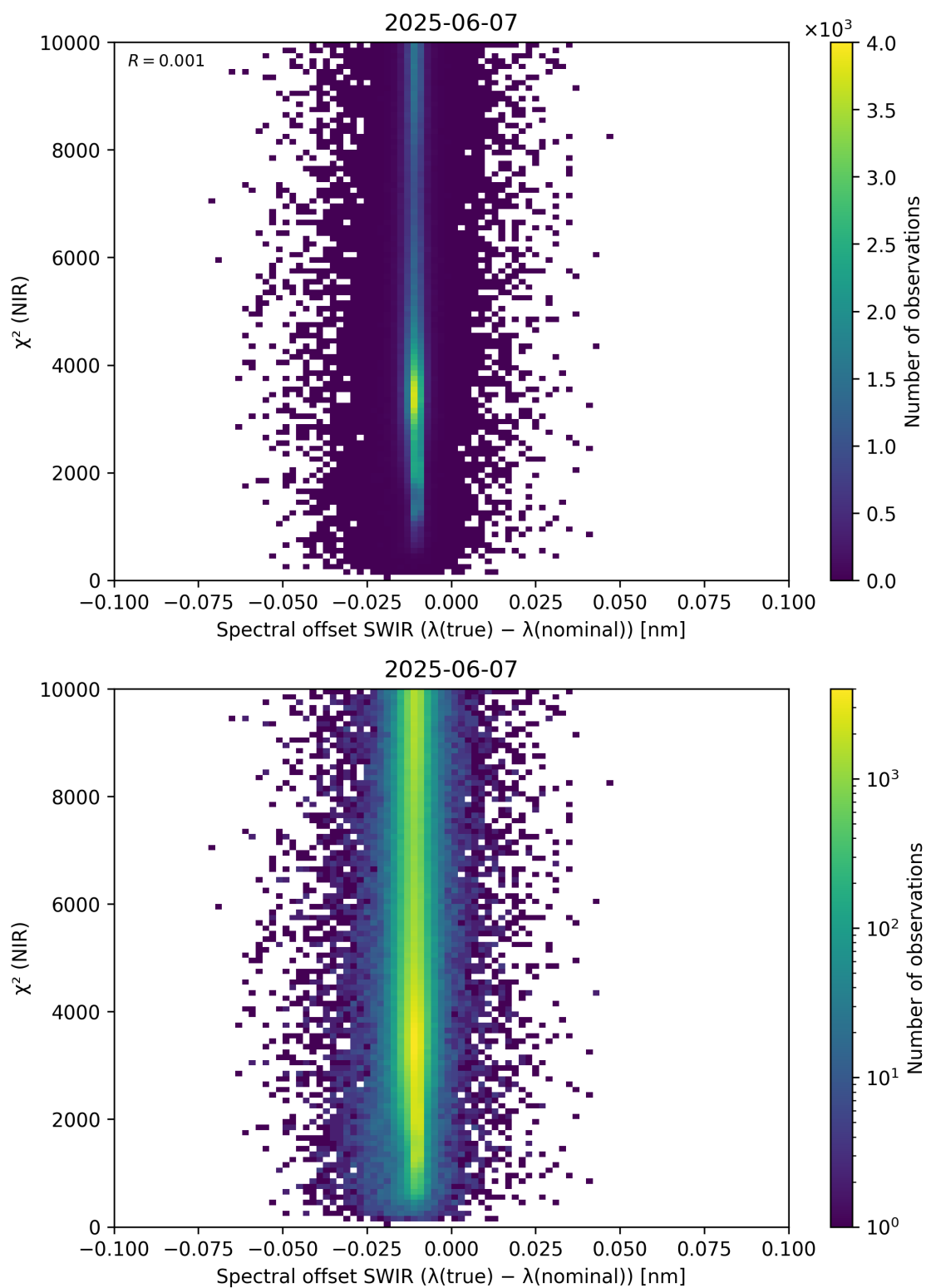
Figure 117: Scatter density plot of “Spectral offset SWIR ( \lambda_{\text{true}} - \lambda_{\text{nominal}} )” against “ \chi^2 (NIR)” for 2025-06-06 to 2025-06-08.
