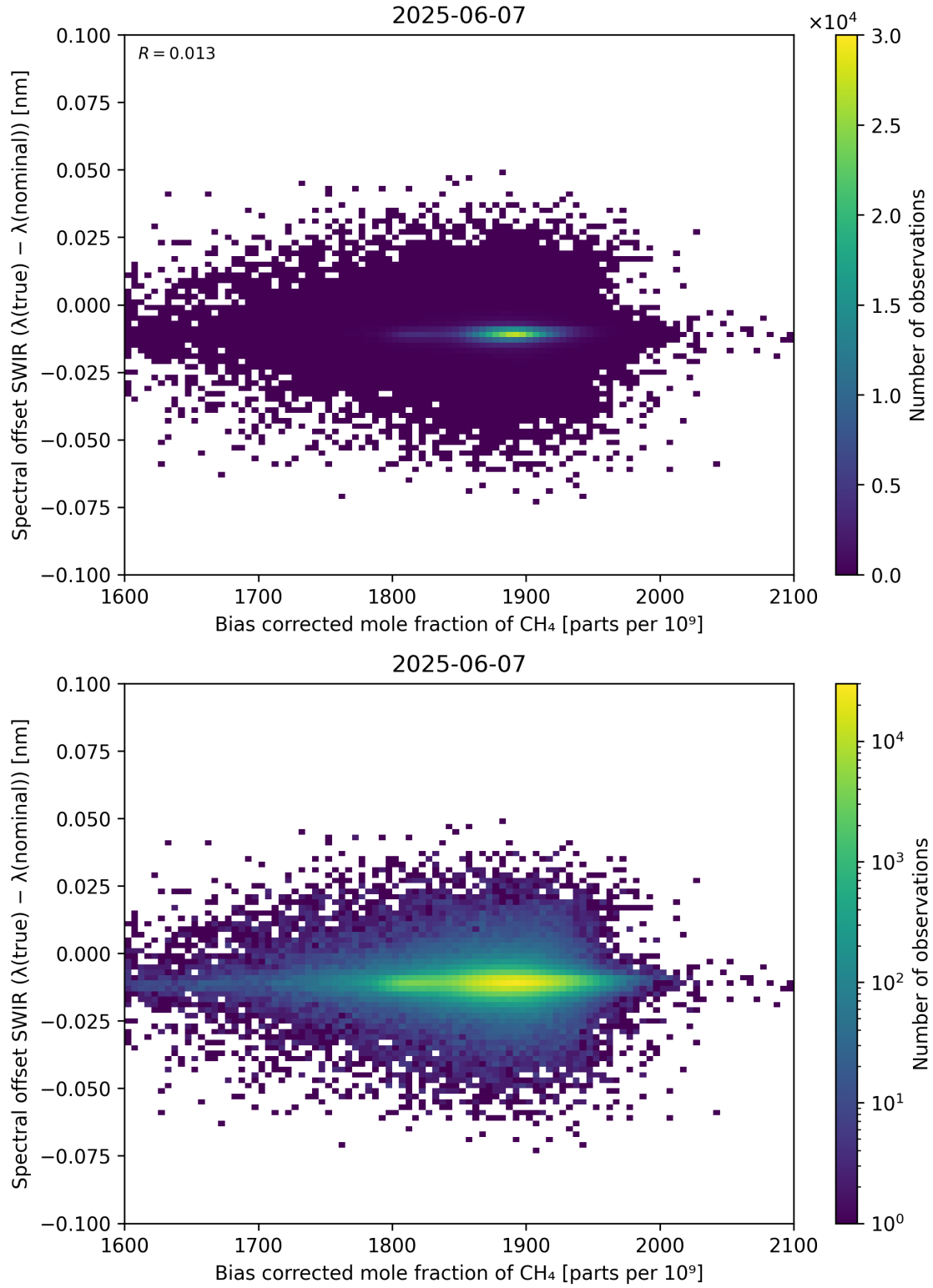
Figure 69: Scatter density plot of “Bias corrected mole fraction of CH 4 ” against “Spectral offset SWIR ( \lambda_{\text{true}} - \lambda_{\text{nominal}} )” for 2025-06-06 to 2025-06-08.
