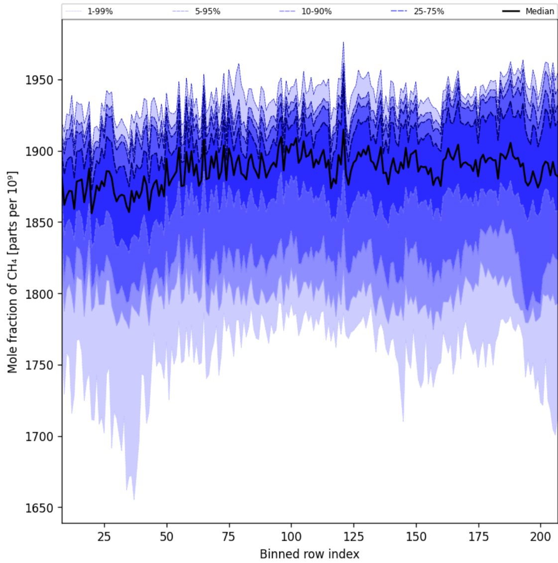
Figure 34: Along track statistics of “Mole fraction of CH 4 ” for 2025-06-06 to 2025-06-08
