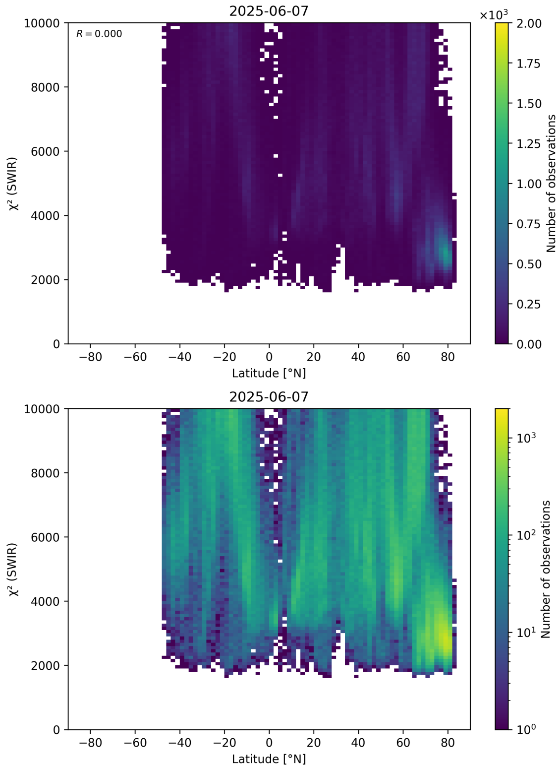
Figure 54: Scatter density plot of “Latitude” against “ \chi^2 (SWIR)” for 2025-06-06 to 2025-06-08.
