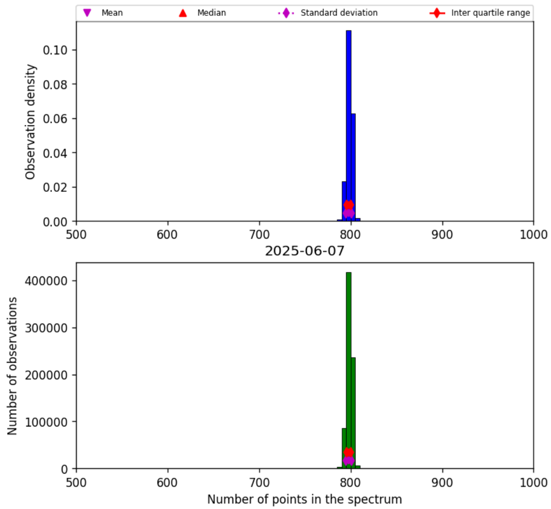
Figure 26: Histogram of “Number of points in the spectrum” for 2025-06-06 to 2025-06-08
