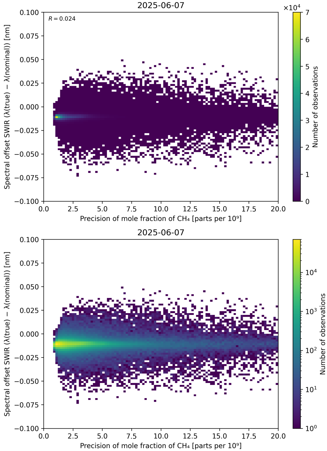
Figure 85: Scatter density plot of “Precision of mole fraction of CH 4 ” against “Spectral offset SWIR ( \lambda_{\text{true}} - \lambda_{\text{nominal}} )” for 2025-06-06 to 2025-06-08.
