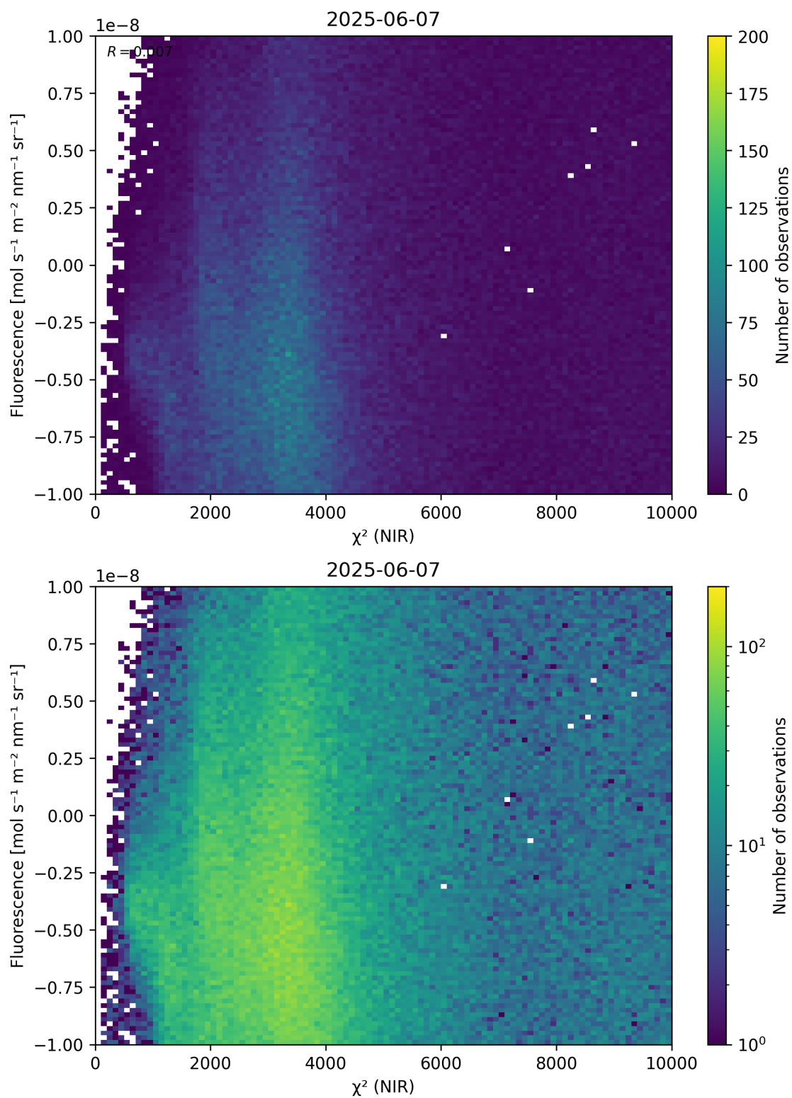
Figure 45: Scatter density plot of “ \chi^2 (NIR)” against “Fluorescence” for 2025-06-06 to 2025-06-08.
