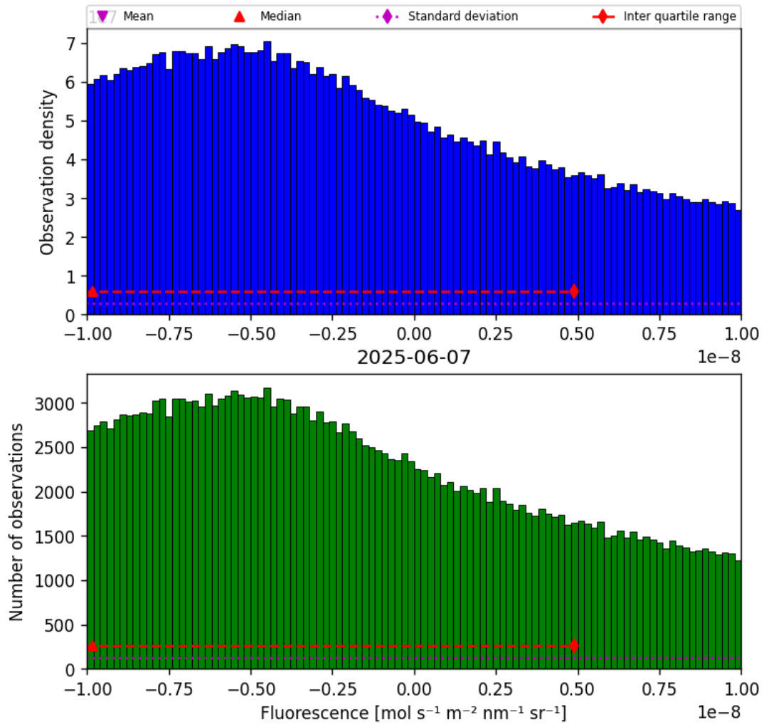
Figure 32: Histogram of “Fluorescence” for 2025-06-06 to 2025-06-08
