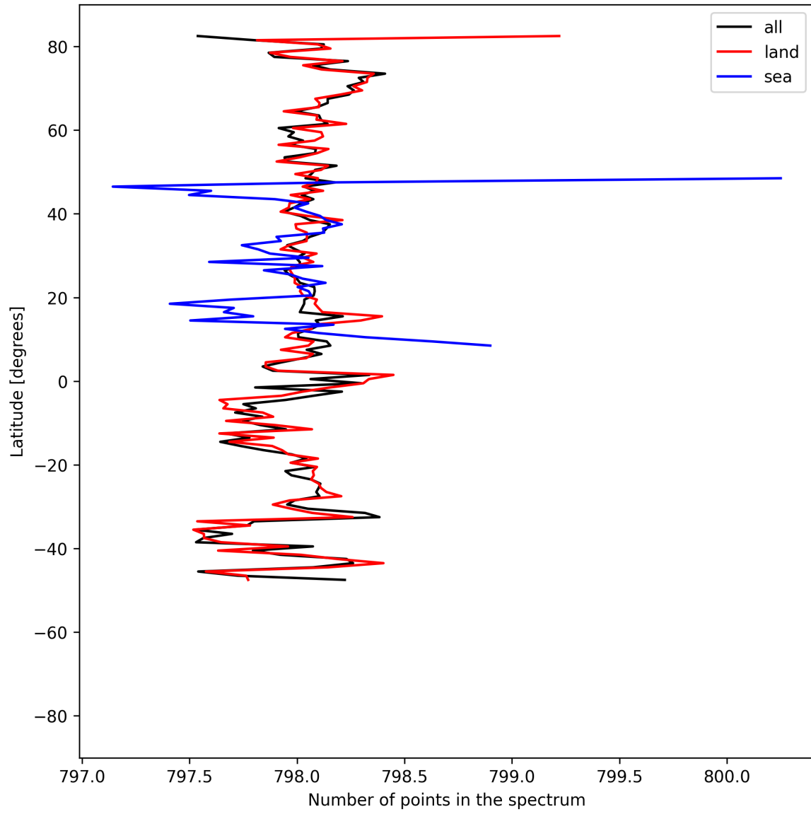
Figure 15: Zonal average of “Number of points in the spectrum” for 2025-06-06 to 2025-06-08.
