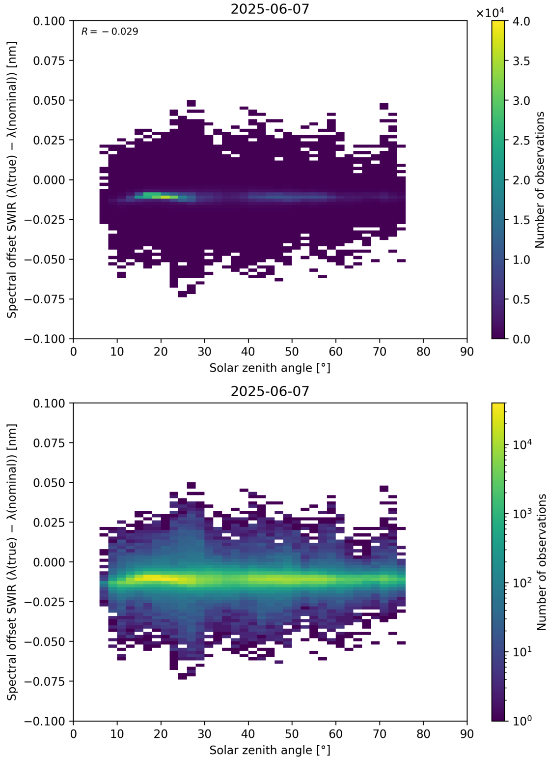
Figure 104: Scatter density plot of “Solar zenith angle” against “Spectral offset SWIR ( \lambda_{\text{true}} - \lambda_{\text{nominal}} )” for 2025-06-06 to 2025-06-08.
