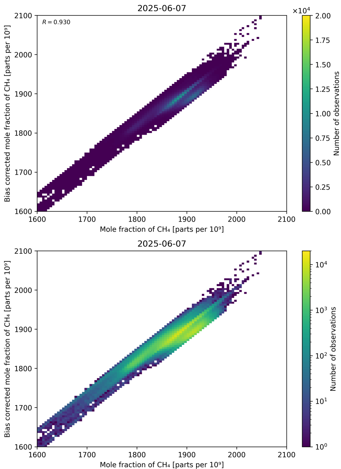
Figure 74: Scatter density plot of “Mole fraction of CH 4 ” against “Bias corrected mole fraction of CH 4 ” for 2025-06-06 to 2025-06-08.
