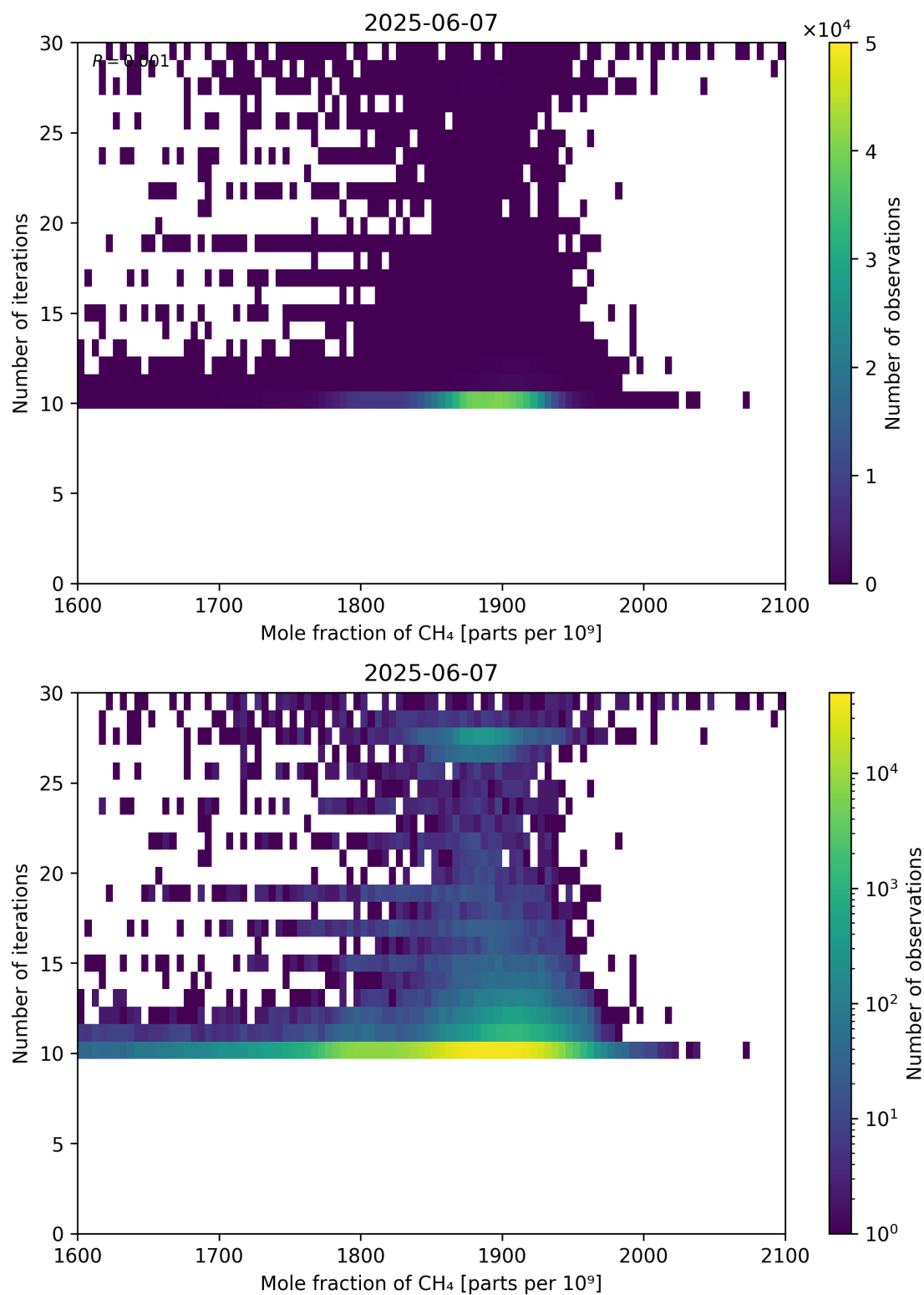
Figure 76: Scatter density plot of “Mole fraction of CH 4 ” against “Number of iterations” for 2025-06-06 to 2025-06-08.
