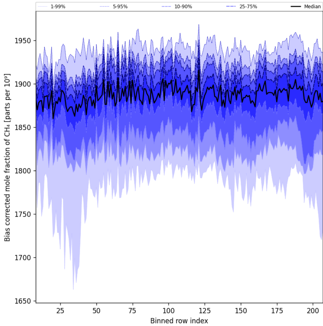
Figure 36: Along track statistics of “Bias corrected mole fraction of \text{CH}_4 ” for 2025-06-06 to 2025-06-08
