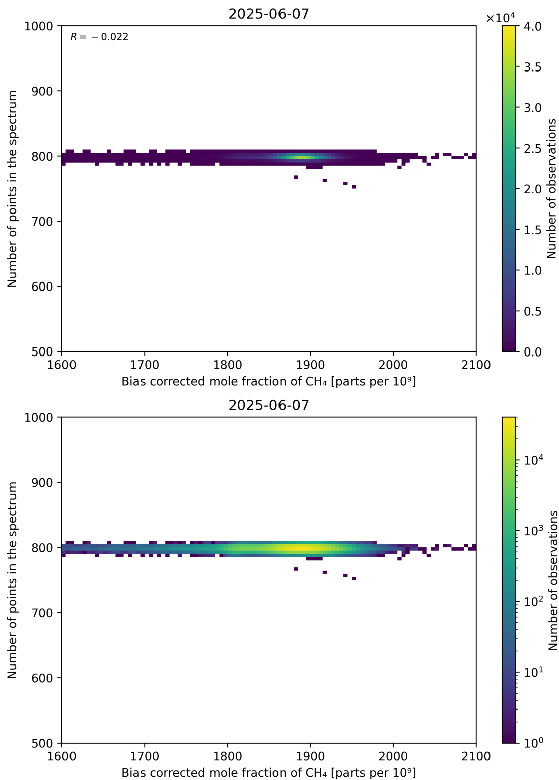
Figure 68: Scatter density plot of “Bias corrected mole fraction of CH 4 ” against “Number of points in the spectrum” for 2025-06-06 to 2025-06-08.
