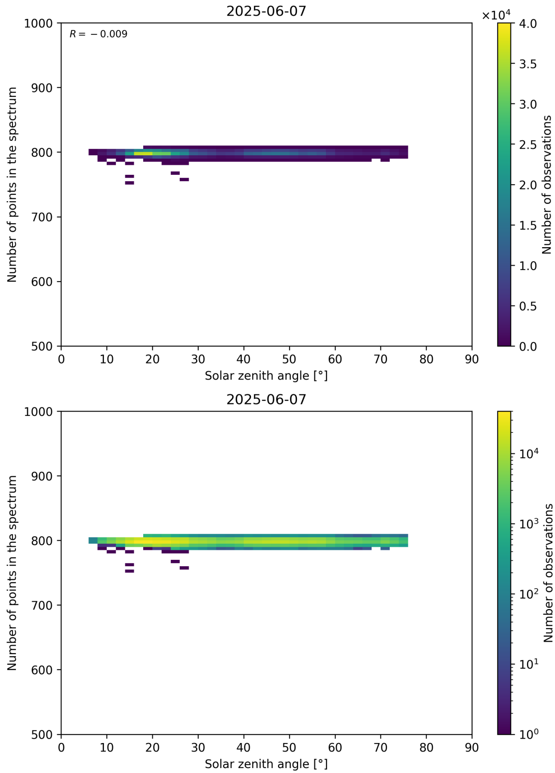
Figure 103: Scatter density plot of “Solar zenith angle” against “Number of points in the spectrum” for 2025-06-06 to 2025-06-08.
