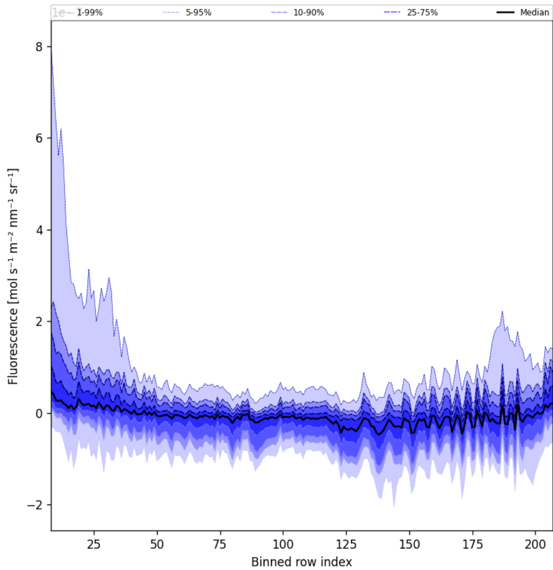
Figure 43: Along track statistics of “Fluorescence” for 2025-06-06 to 2025-06-08
