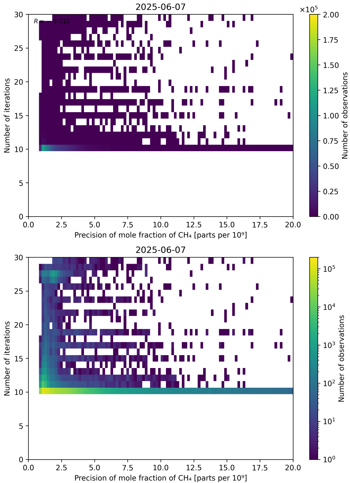
Figure 83: Scatter density plot of “Precision of mole fraction of CH 4 ” against “Number of iterations” for 2025-06-06 to 2025-06-08.
