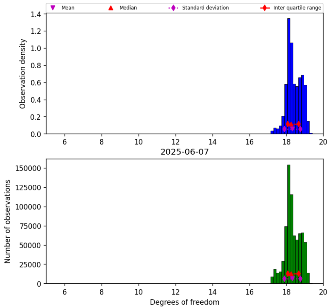
Figure 30: Histogram of “Degrees of freedom” for 2025-06-06 to 2025-06-08
