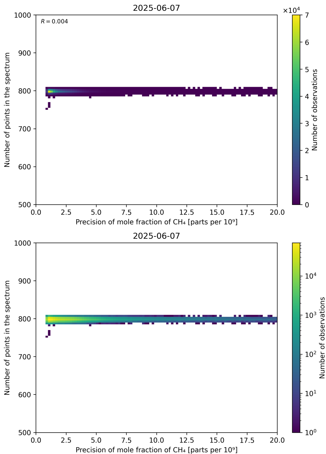
Figure 84: Scatter density plot of “Precision of mole fraction of CH 4 ” against “Number of points in the spectrum” for 2025-06-06 to 2025-06-08.
