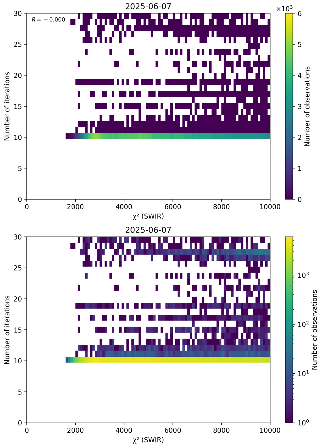
Figure 50: Scatter density plot of “ \chi^2 (SWIR)” against “Number of iterations” for 2025-06-06 to 2025-06-08.
