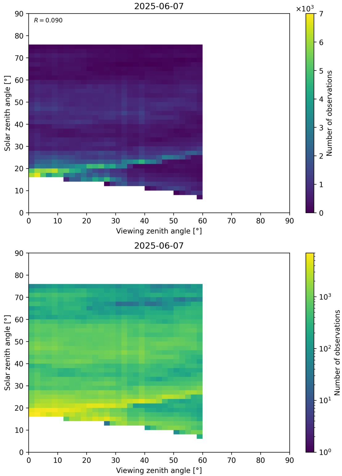
Figure 115: Scatter density plot of “Viewing zenith angle” against “Solar zenith angle” for 2025-06-06 to 2025-06-08.
