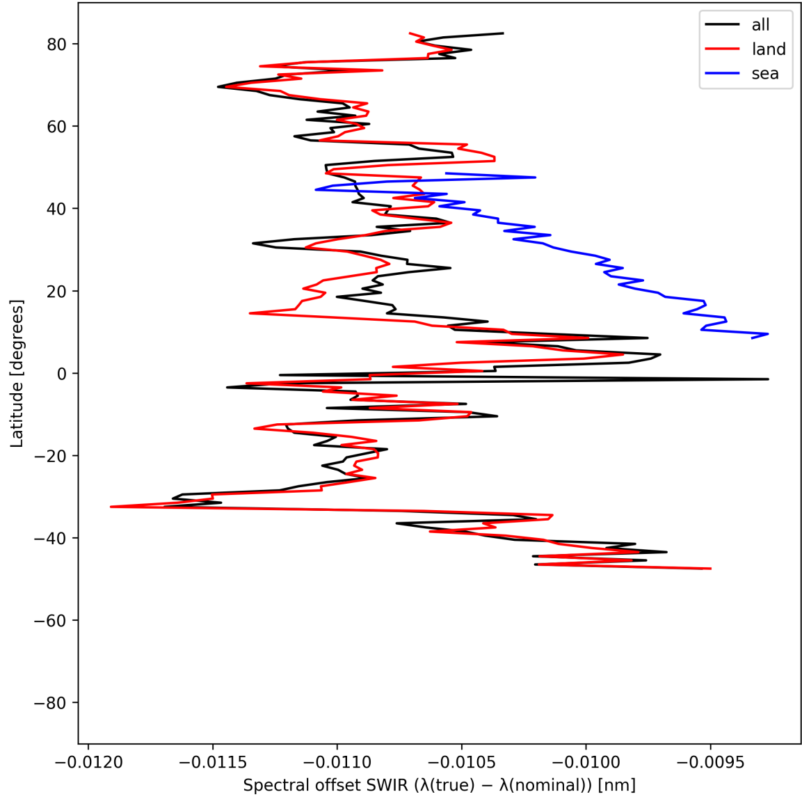
Figure 16: Zonal average of “Spectral offset SWIR ( \lambda_{\text{true}} - \lambda_{\text{nominal}} )” for 2025-06-06 to 2025-06-08.
