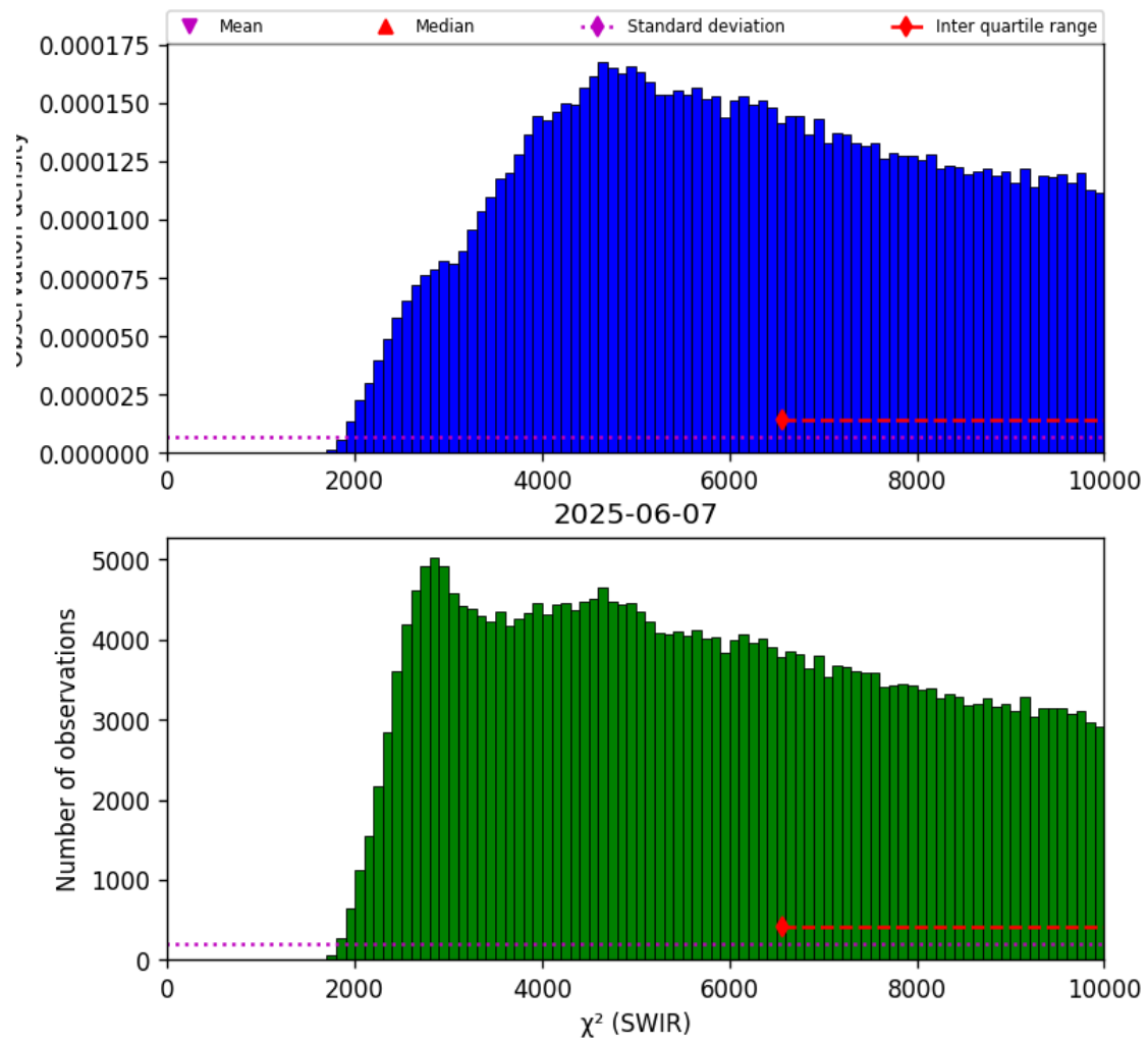
Figure 28: Histogram of “ \chi^2 (SWIR)” for 2025-06-06 to 2025-06-08
