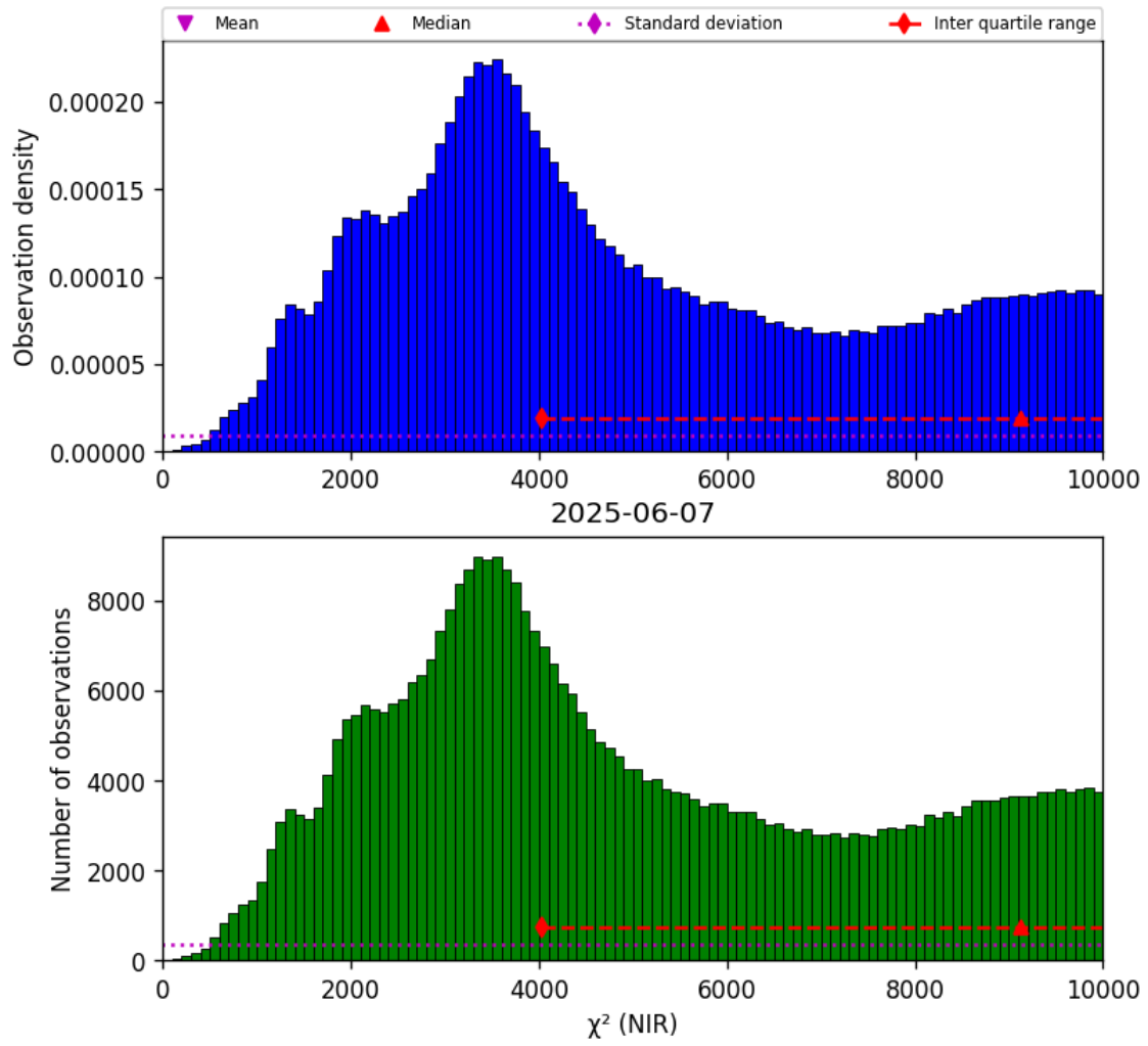
Figure 29: Histogram of “ \chi^2 (NIR)” for 2025-06-06 to 2025-06-08
