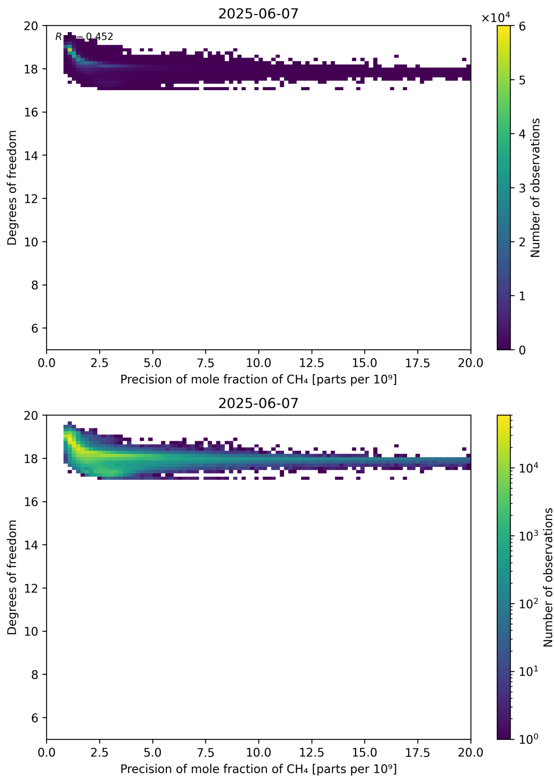
Figure 80: Scatter density plot of “Precision of mole fraction of CH 4 ” against “Degrees of freedom” for 2025-06-06 to 2025-06-08.
