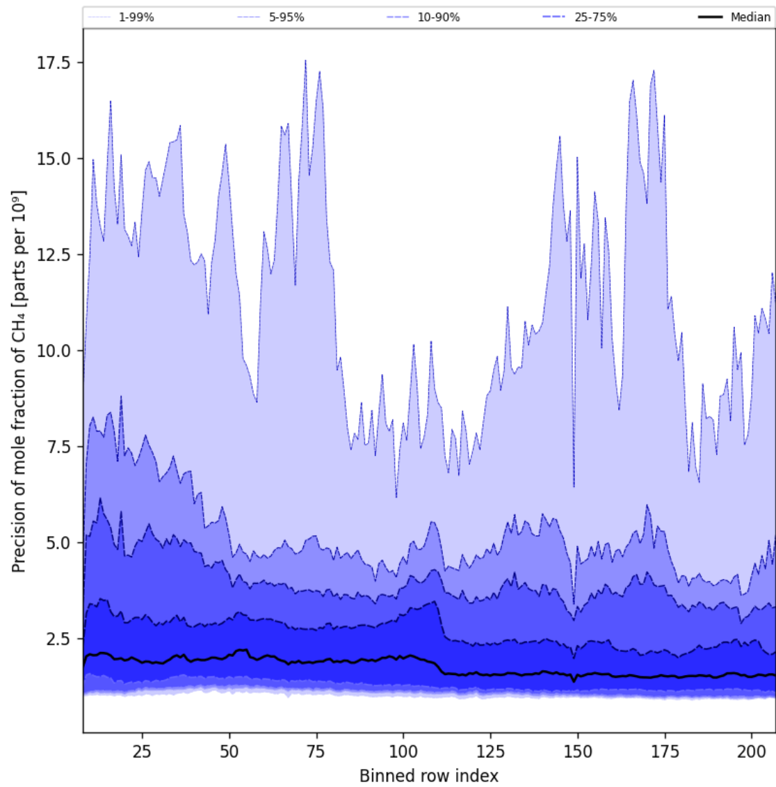
Figure 35: Along track statistics of “Precision of mole fraction of CH 4 ” for 2025-06-06 to 2025-06-08
