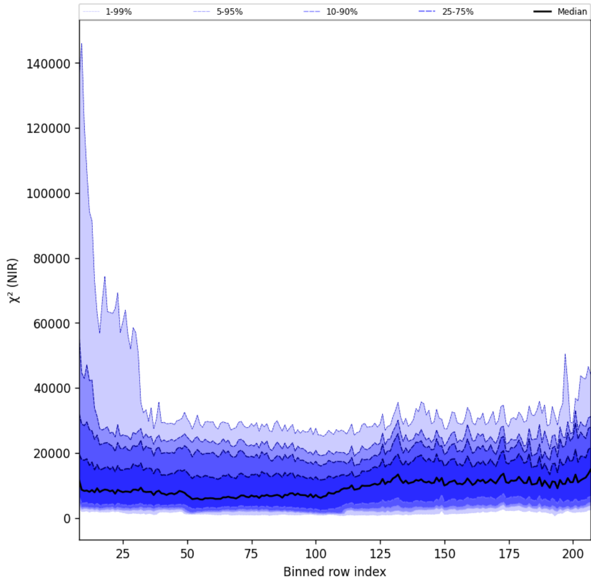
Figure 40: Along track statistics of “ \chi^2 (NIR)” for 2025-06-06 to 2025-06-08
