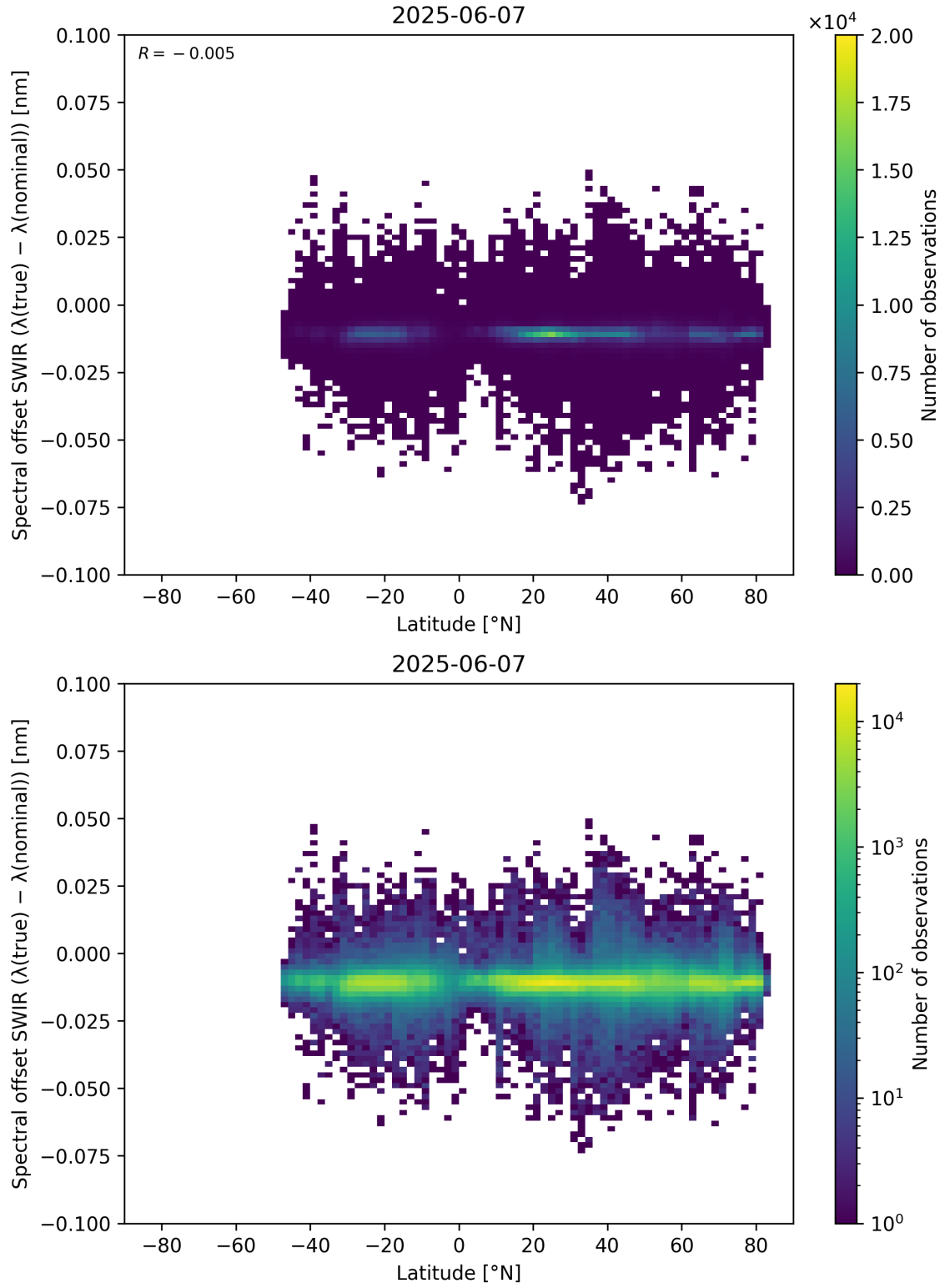
Figure 62: Scatter density plot of “Latitude” against “Spectral offset SWIR ( \lambda_{\text{true}} - \lambda_{\text{nominal}} )” for 2025-06-06 to 2025-06-08.
