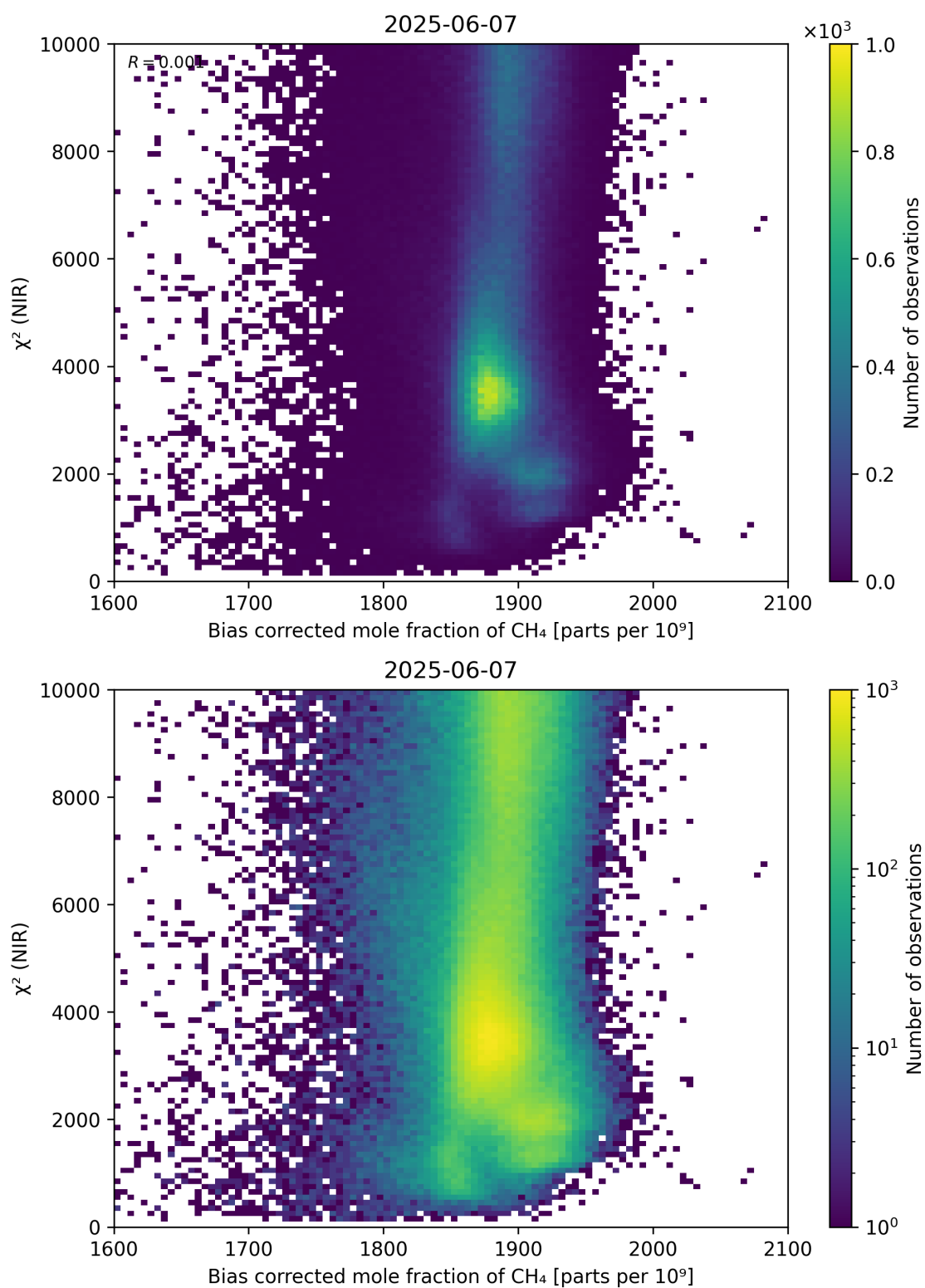
Figure 63: Scatter density plot of “Bias corrected mole fraction of \text{CH}_4 ” against “ \chi^2 (NIR)” for 2025-06-06 to 2025-06-08.
