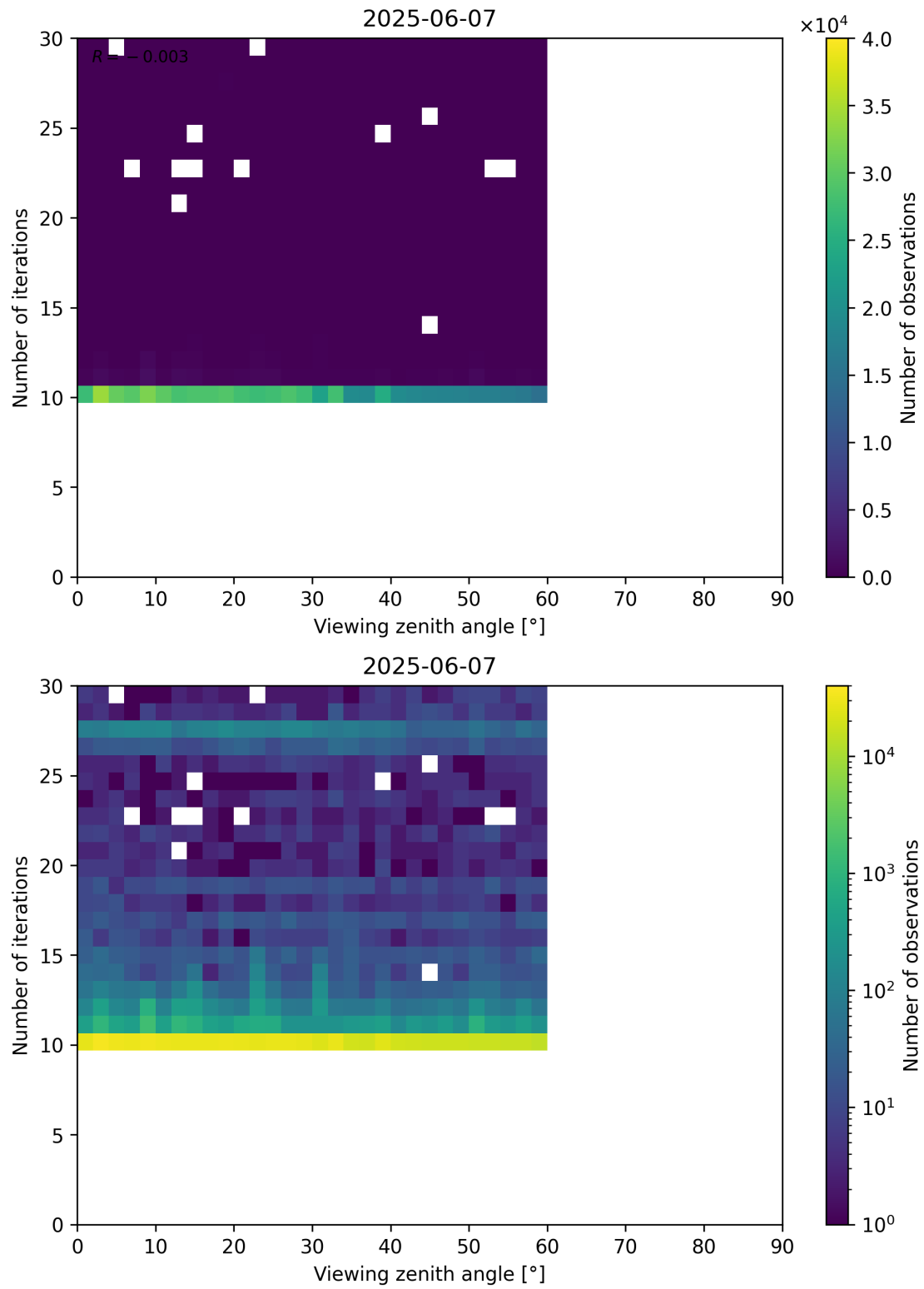
Figure 113: Scatter density plot of “Viewing zenith angle” against “Number of iterations” for 2025-06-06 to 2025-06-08.
