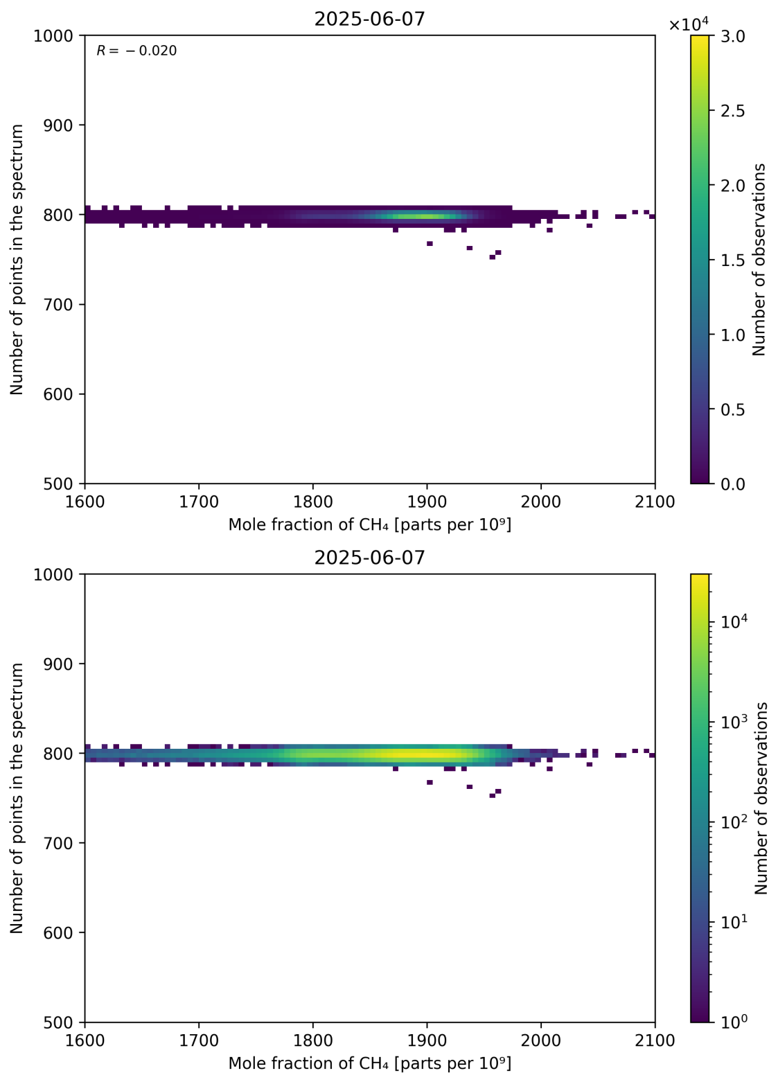
Figure 77: Scatter density plot of “Mole fraction of CH 4 ” against “Number of points in the spectrum” for 2025-06-06 to 2025-06-08.
