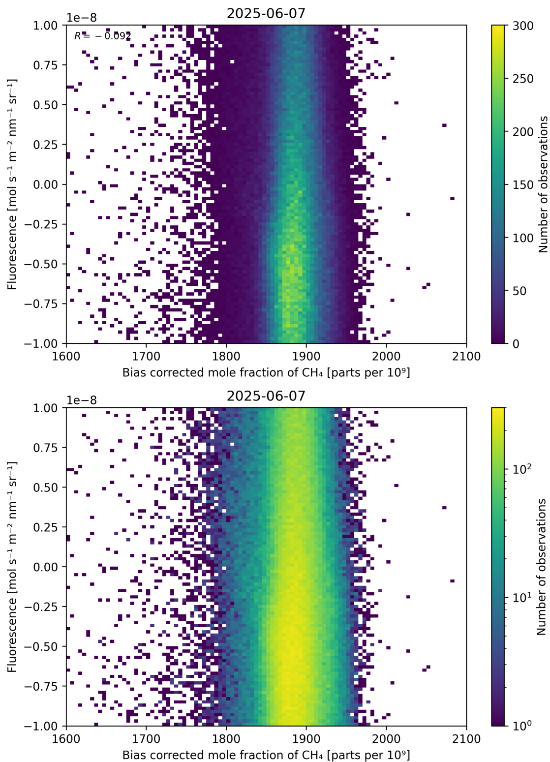
Figure 66: Scatter density plot of “Bias corrected mole fraction of \text{CH}_4 ” against “Fluorescence” for 2025-06-06 to 2025-06-08.
