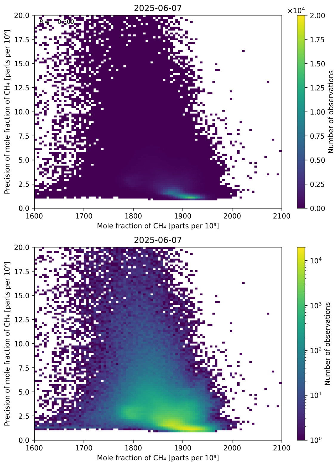
Figure 75: Scatter density plot of “Mole fraction of CH 4 ” against “Precision of mole fraction of CH 4 ” for 2025-06-06 to 2025-06-08.
