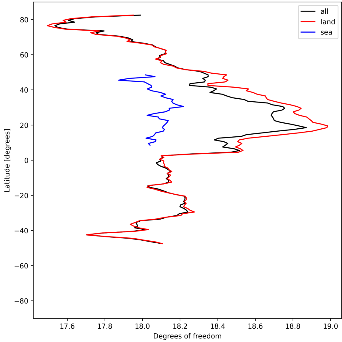
Figure 19: Zonal average of “Degrees of freedom” for 2025-06-06 to 2025-06-08.
