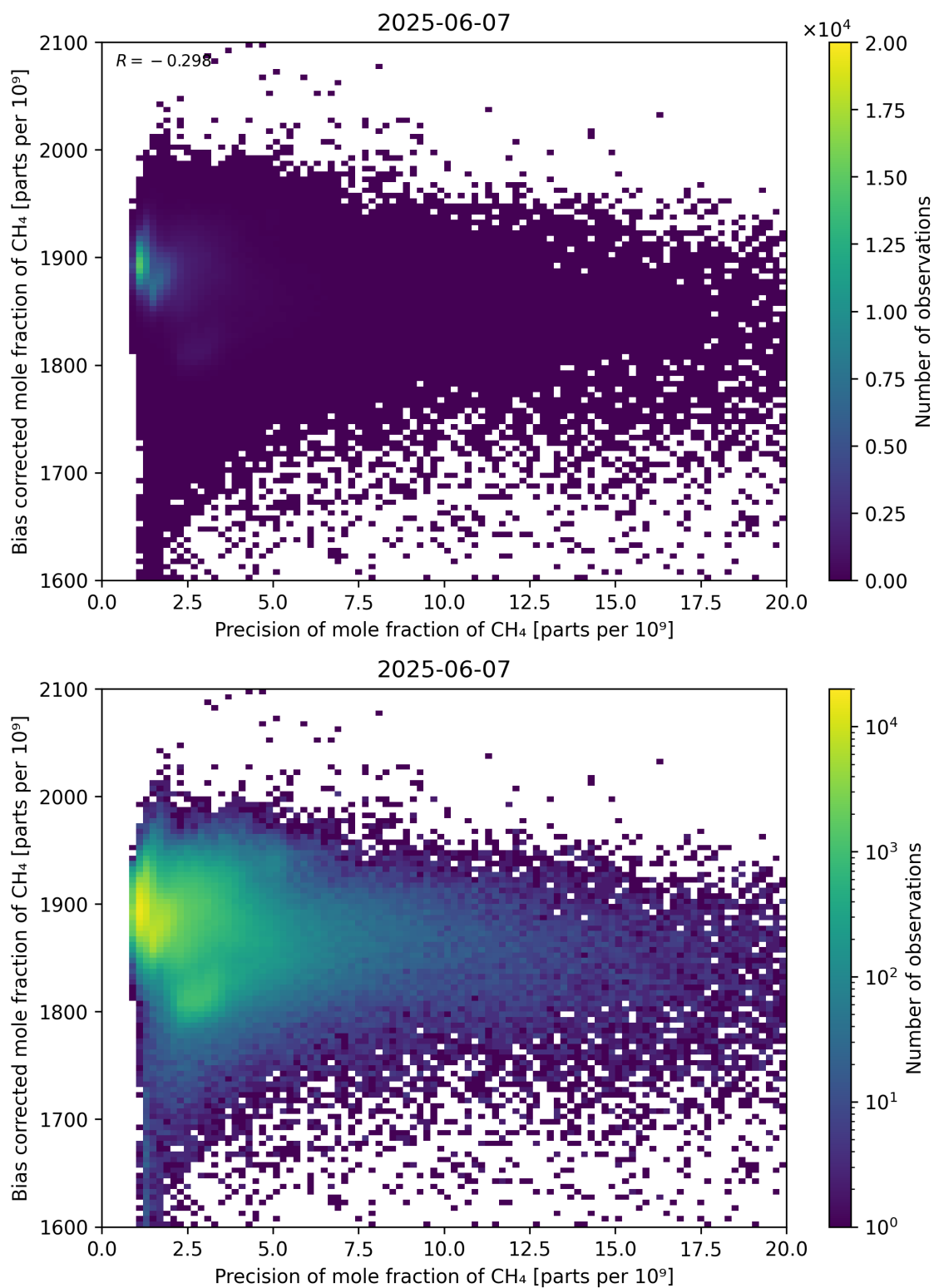
Figure 82: Scatter density plot of “Precision of mole fraction of CH 4 ” against “Bias corrected mole fraction of CH 4 ” for 2025-06-06 to 2025-06-08.
