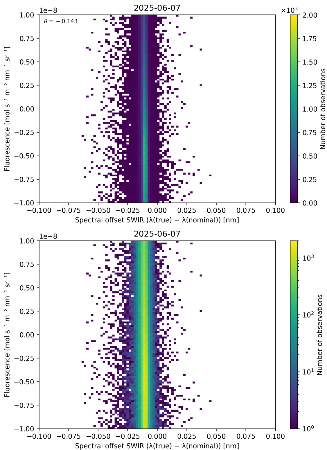
Figure 120: Scatter density plot of “Spectral offset SWIR ( \lambda_{\text{true}} - \lambda_{\text{nominal}} )” against “Fluorescence” for 2025-06-06 to 2025-06-08.
