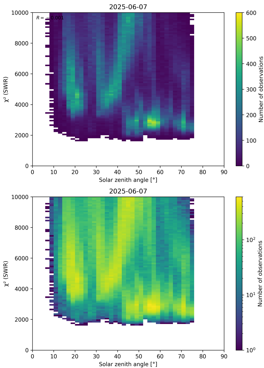
Figure 95: Scatter density plot of “Solar zenith angle” against “ \chi^2 (SWIR)” for 2025-06-06 to 2025-06-08.
