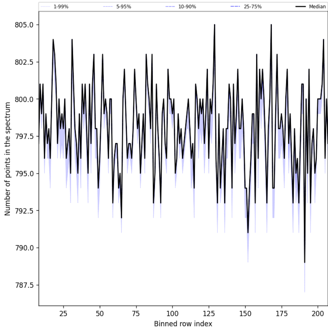
Figure 37: Along track statistics of “Number of points in the spectrum” for 2025-06-06 to 2025-06-08
