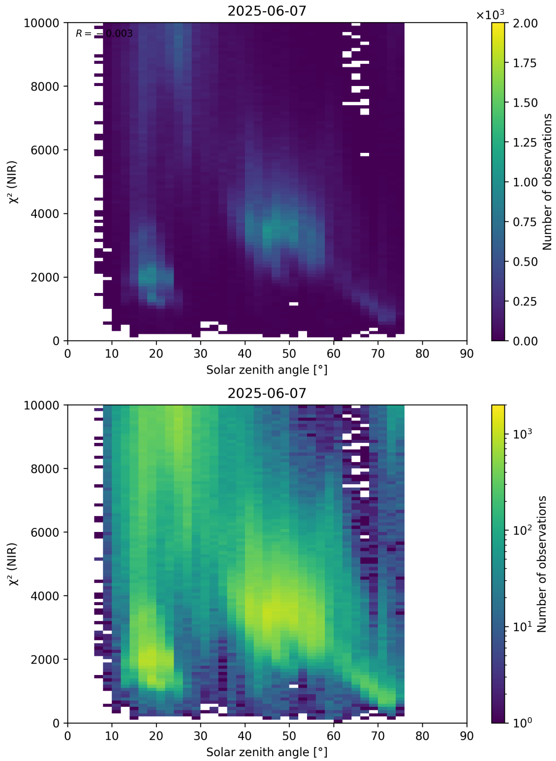
Figure 94: Scatter density plot of “Solar zenith angle” against “ \chi^2 (NIR)” for 2025-06-06 to 2025-06-08.
