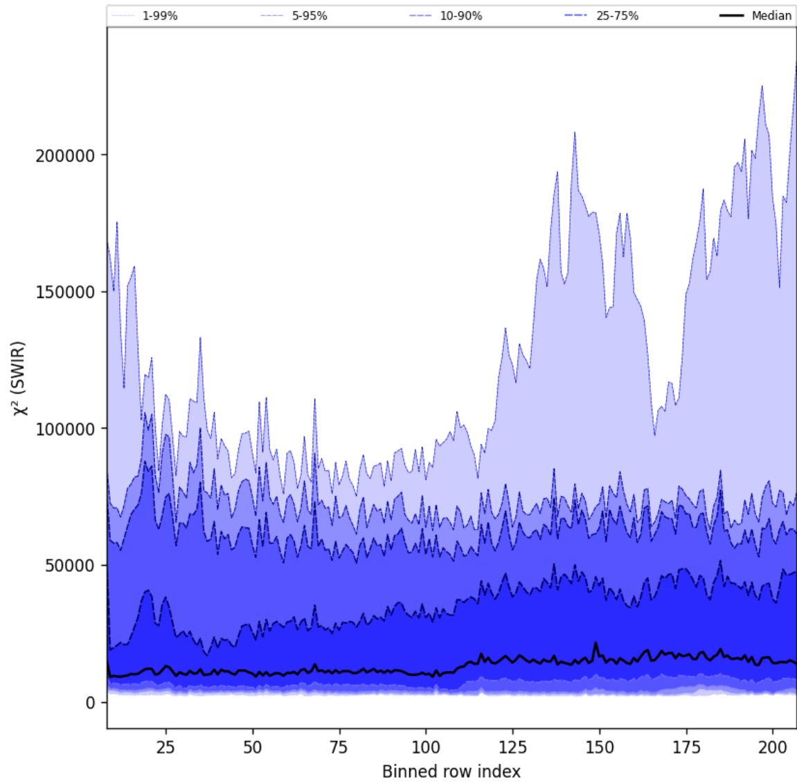
Figure 39: Along track statistics of “ \chi^2 (SWIR)” for 2025-06-06 to 2025-06-08
