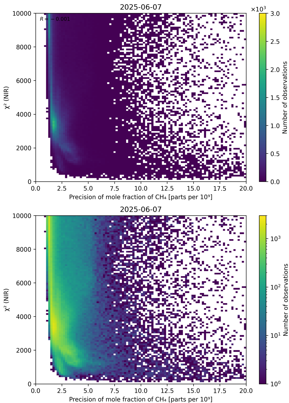
Figure 78: Scatter density plot of “Precision of mole fraction of CH 4 ” against “ \chi^2 (NIR)” for 2025-06-06 to 2025-06-08.
