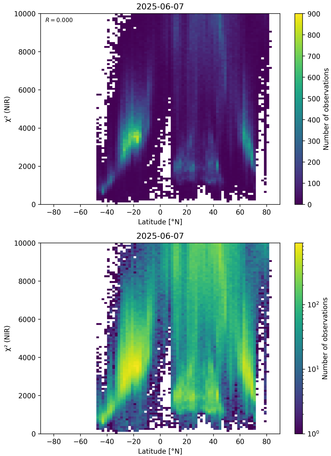
Figure 53: Scatter density plot of “Latitude” against “ \chi^2 (NIR)” for 2025-06-06 to 2025-06-08.
