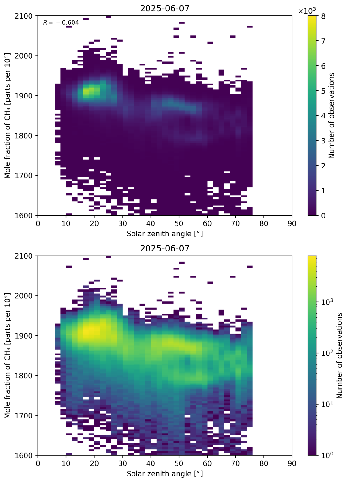
Figure 99: Scatter density plot of “Solar zenith angle” against “Mole fraction of \text{CH}_4 ” for 2025-06-06 to 2025-06-08.
