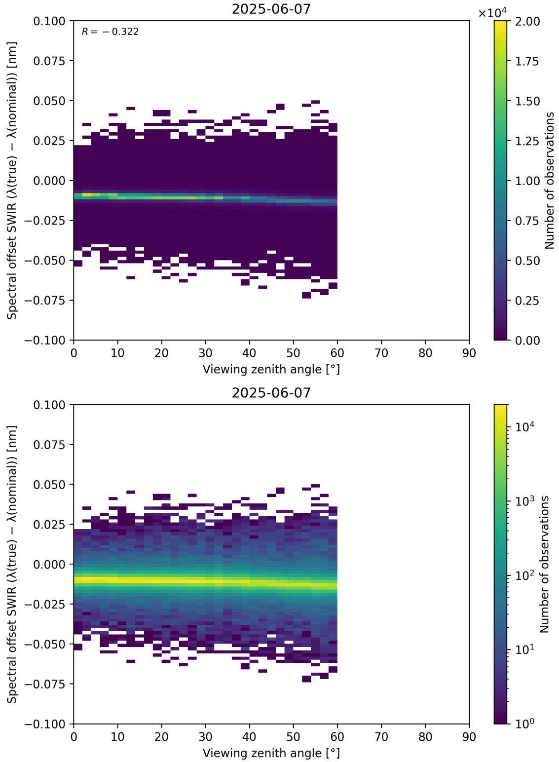
Figure 116: Scatter density plot of “Viewing zenith angle” against “Spectral offset SWIR ( \lambda_{\text{true}} - \lambda_{\text{nominal}} )” for 2025-06-06 to 2025-06-08.
