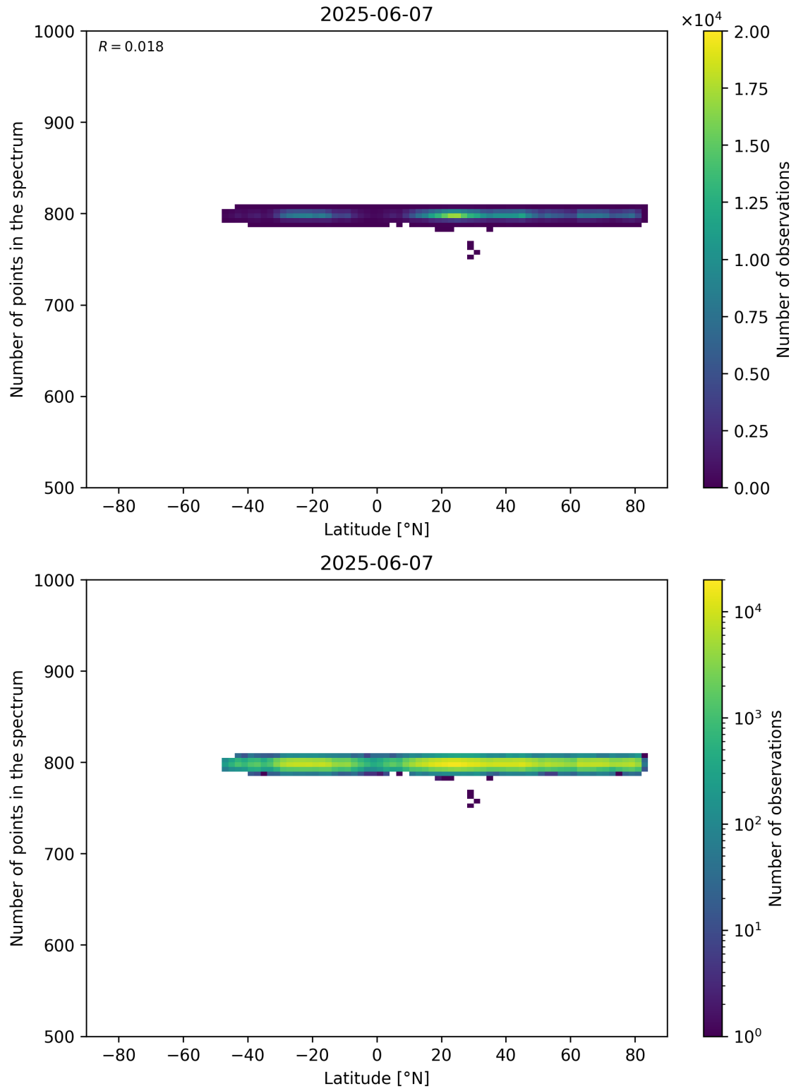
Figure 61: Scatter density plot of “Latitude” against “Number of points in the spectrum” for 2025-06-06 to 2025-06-08.
