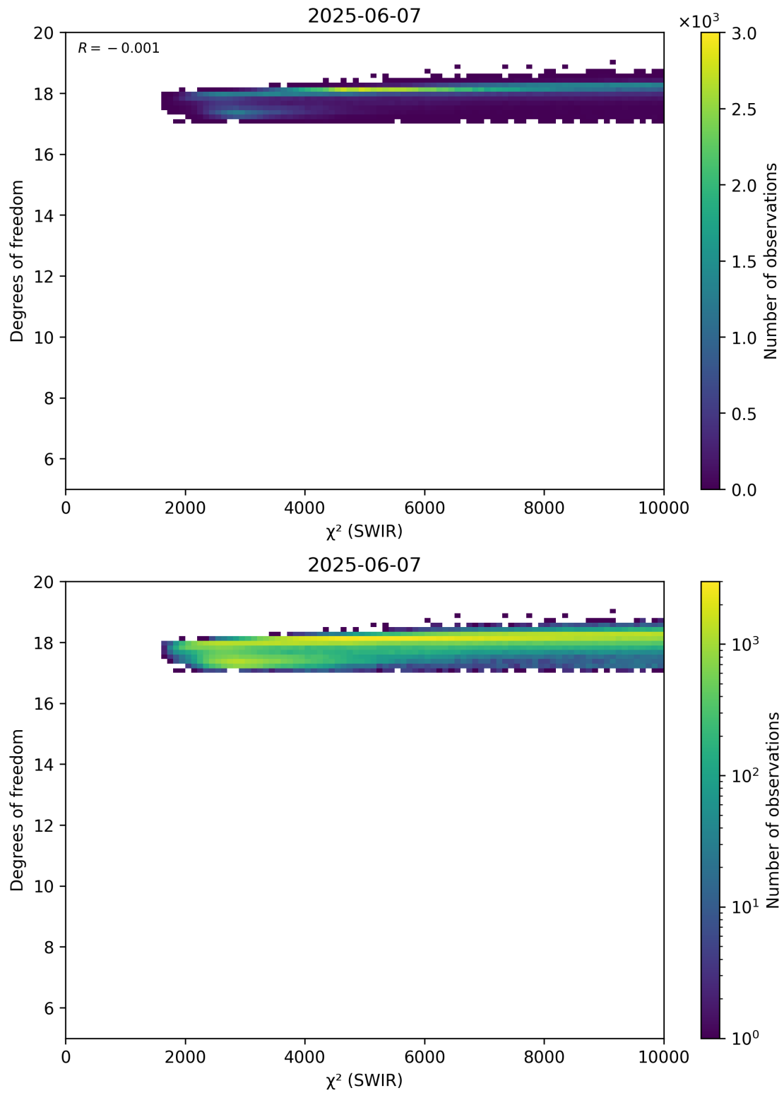
Figure 48: Scatter density plot of “ \chi^2 (SWIR)” against “Degrees of freedom” for 2025-06-06 to 2025-06-08.
