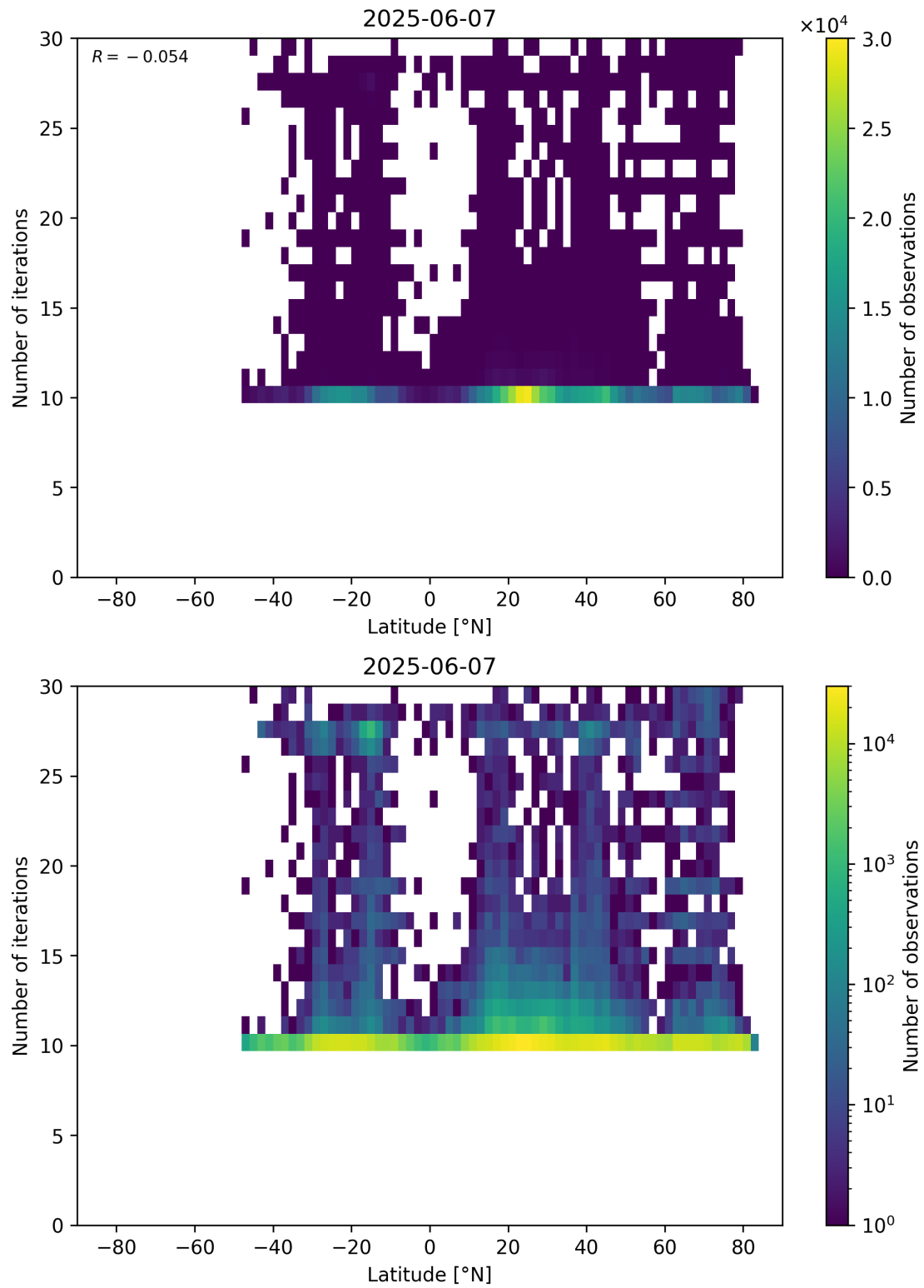
Figure 60: Scatter density plot of “Latitude” against “Number of iterations” for 2025-06-06 to 2025-06-08.
