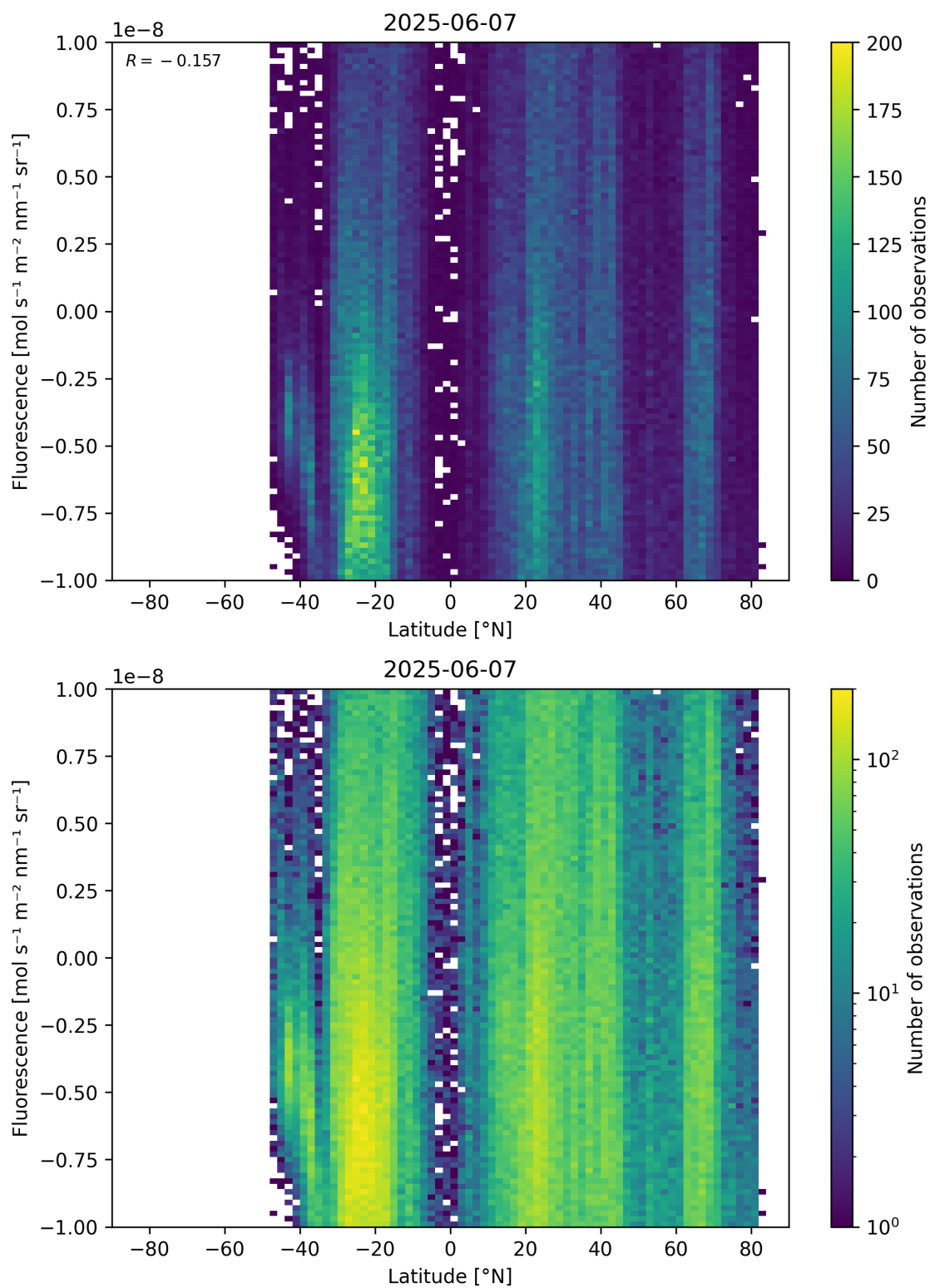
Figure 56: Scatter density plot of “Latitude” against “Fluorescence” for 2025-06-06 to 2025-06-08.
