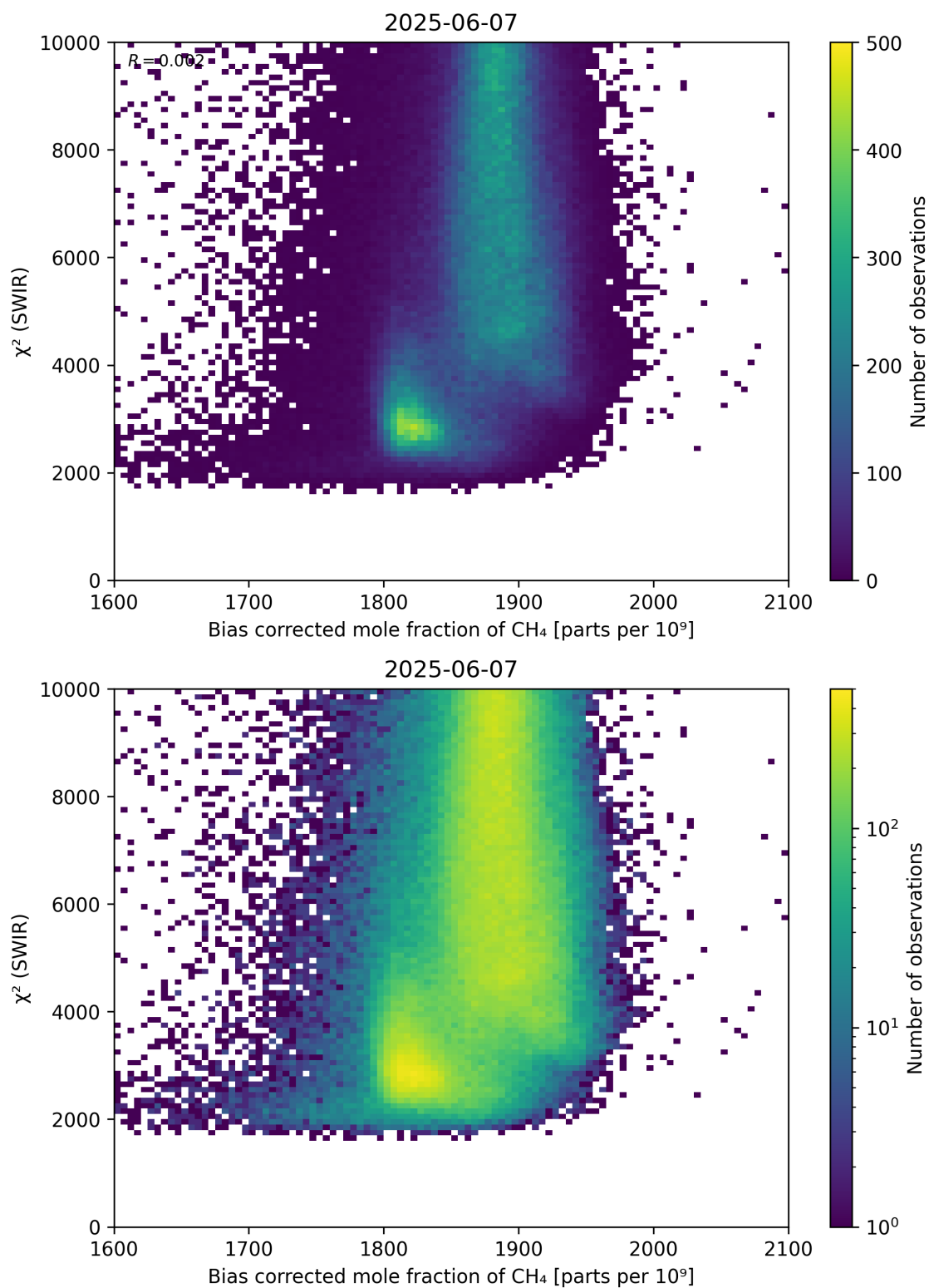
Figure 64: Scatter density plot of “Bias corrected mole fraction of \text{CH}_4 ” against “ \chi^2 (SWIR)” for 2025-06-06 to 2025-06-08.
