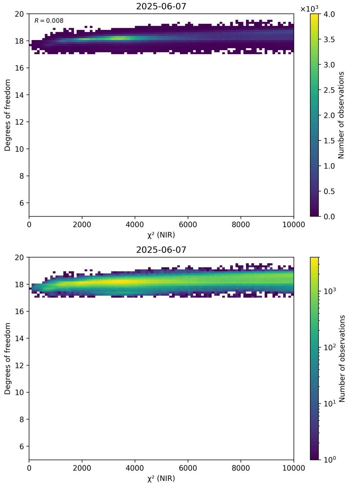
Figure 44: Scatter density plot of “ \chi^2 (NIR)” against “Degrees of freedom” for 2025-06-06 to 2025-06-08.
