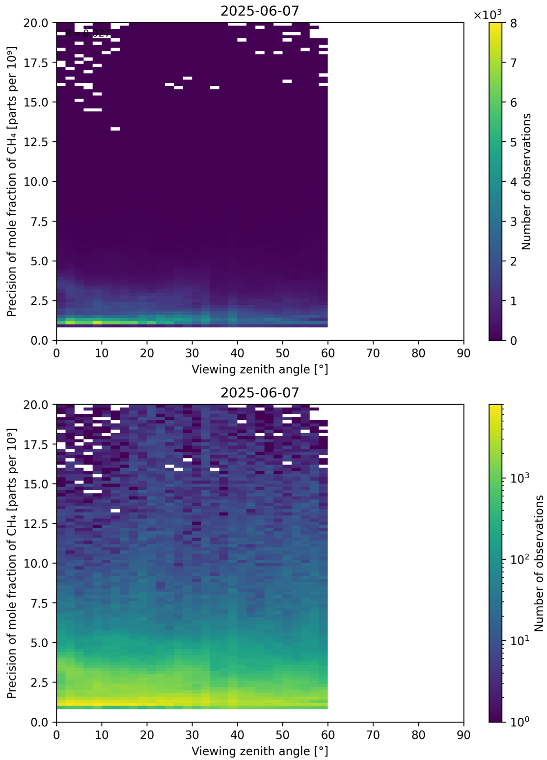
Figure 112: Scatter density plot of “Viewing zenith angle” against “Precision of mole fraction of CH 4 ” for 2025-06-06 to 2025-06-08.
