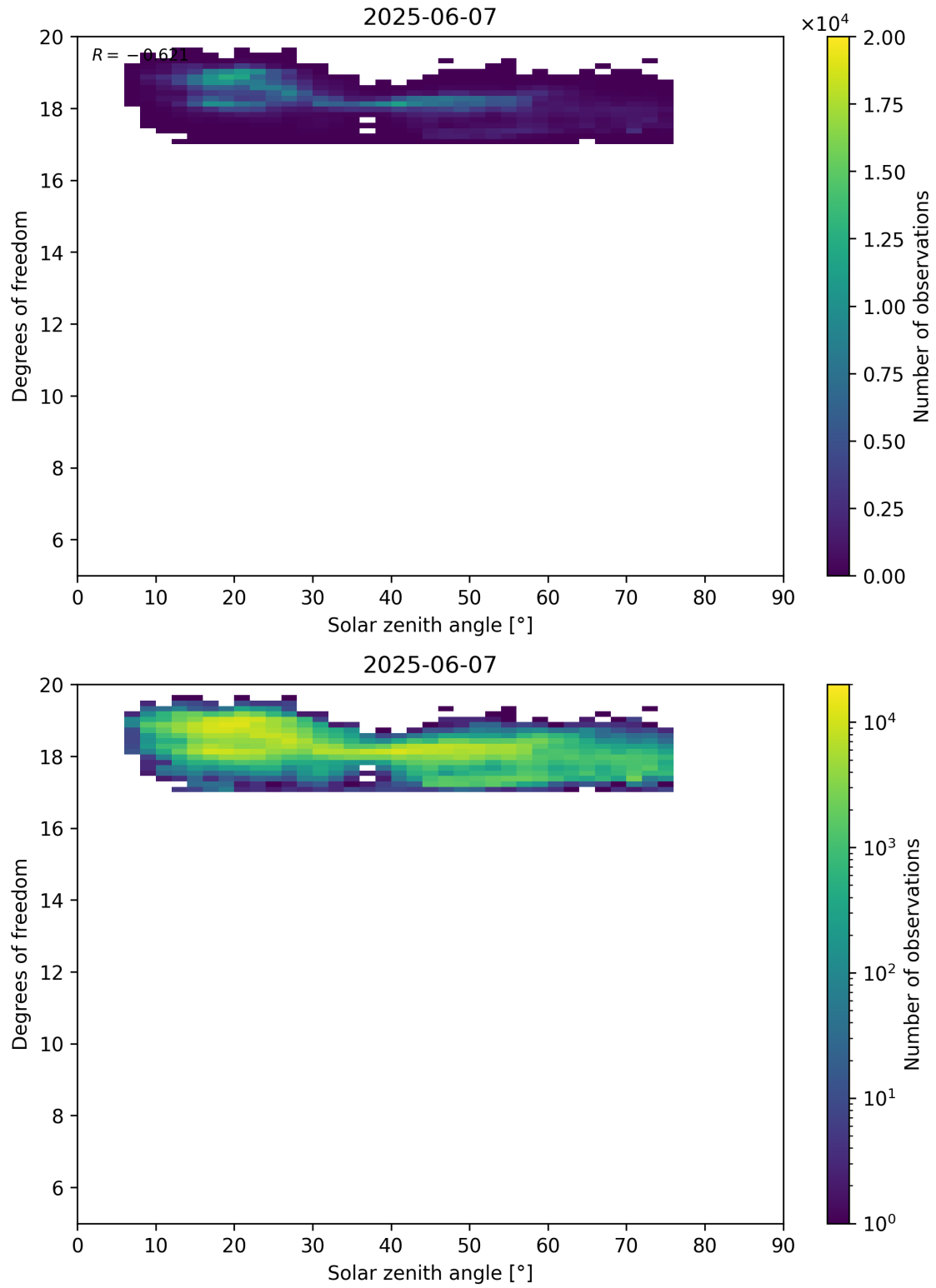
Figure 96: Scatter density plot of “Solar zenith angle” against “Degrees of freedom” for 2025-06-06 to 2025-06-08.
