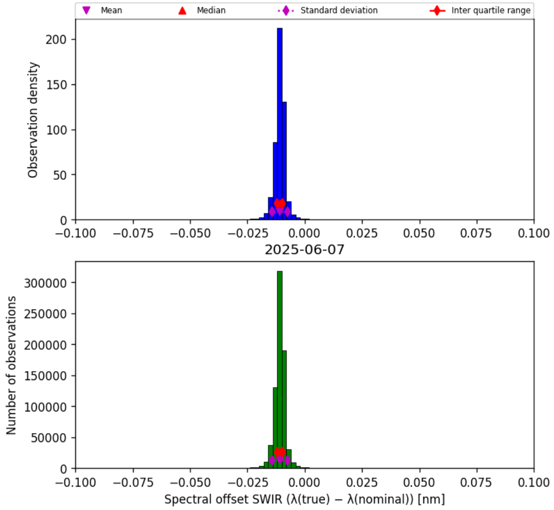
Figure 27: Histogram of “Spectral offset SWIR ( \lambda_{\text{true}} - \lambda_{\text{nominal}} )” for 2025-06-06 to 2025-06-08
