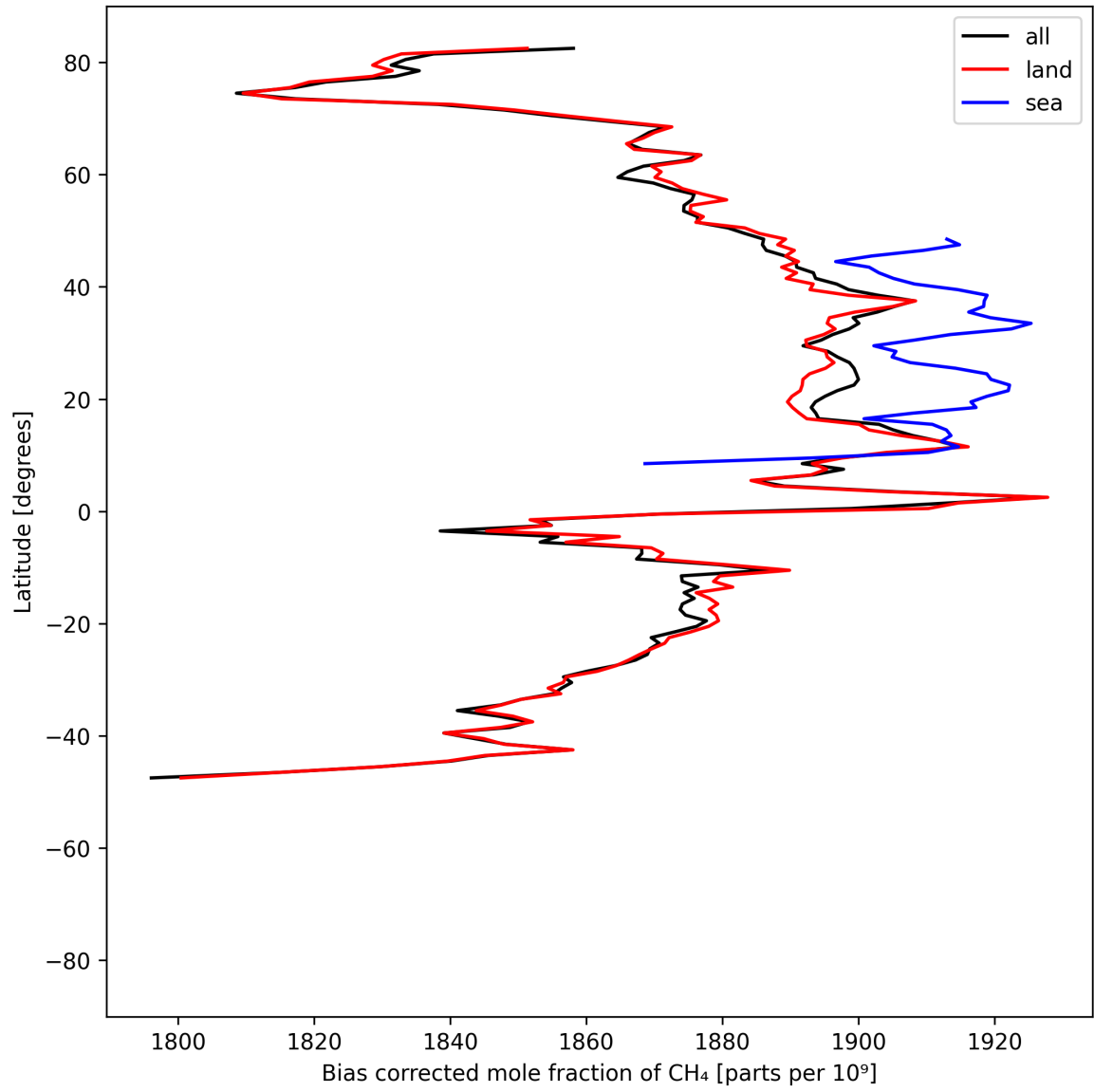
Figure 14: Zonal average of “Bias corrected mole fraction of CH 4 ” for 2025-06-06 to 2025-06-08.
