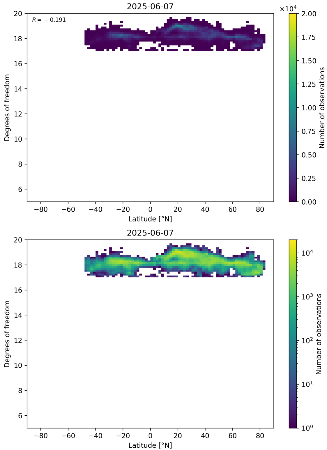
Figure 55: Scatter density plot of “Latitude” against “Degrees of freedom” for 2025-06-06 to 2025-06-08.
