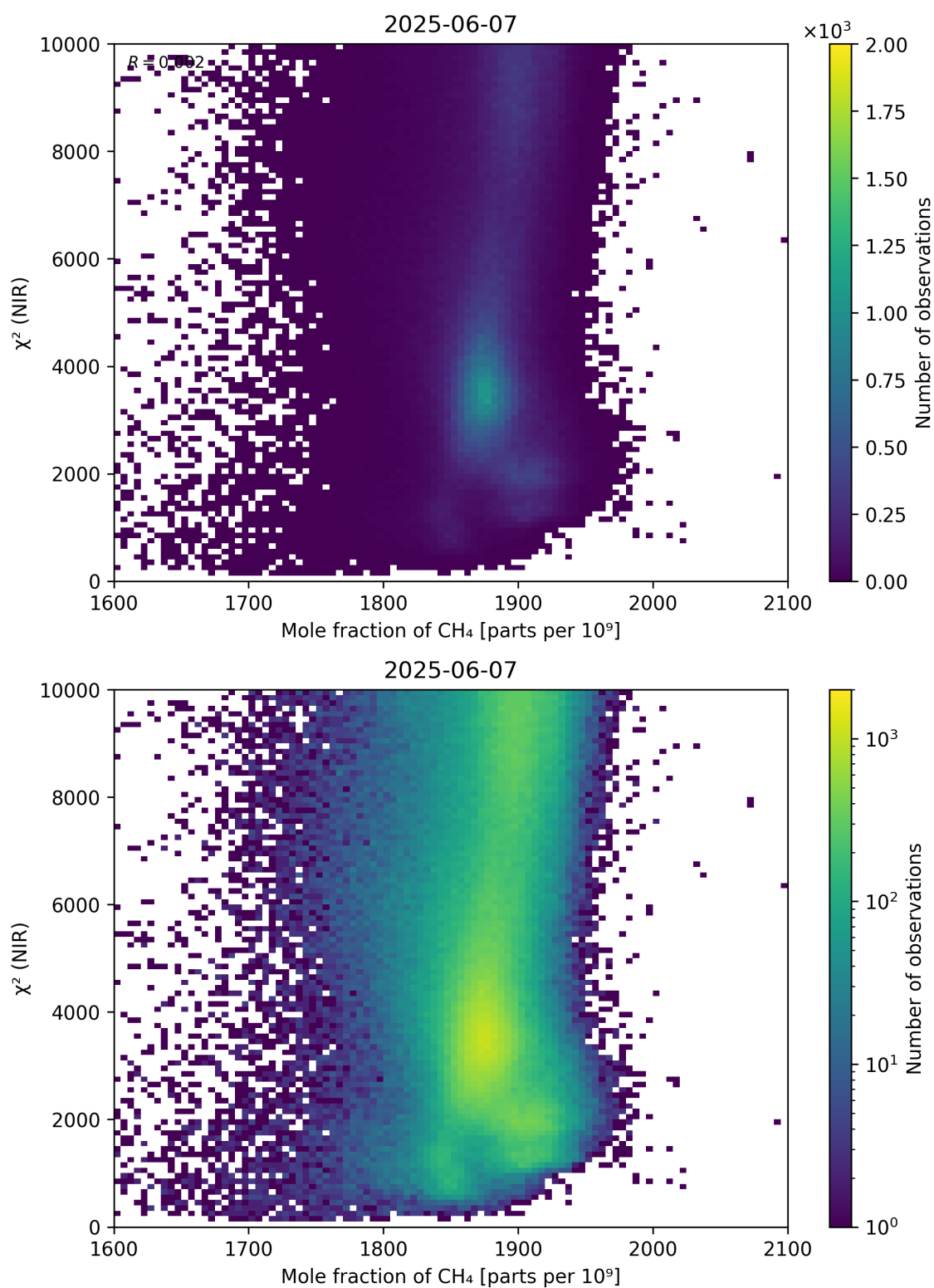
Figure 70: Scatter density plot of “Mole fraction of \text{CH}_4 ” against “ \chi^2 (NIR)” for 2025-06-06 to 2025-06-08.
