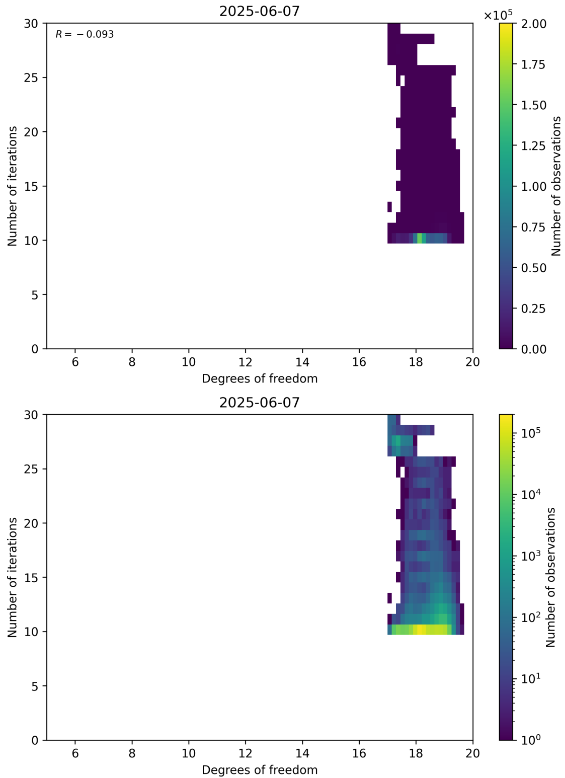
Figure 52: Scatter density plot of “Degrees of freedom” against “Number of iterations” for 2025-06-06 to 2025-06-08.
