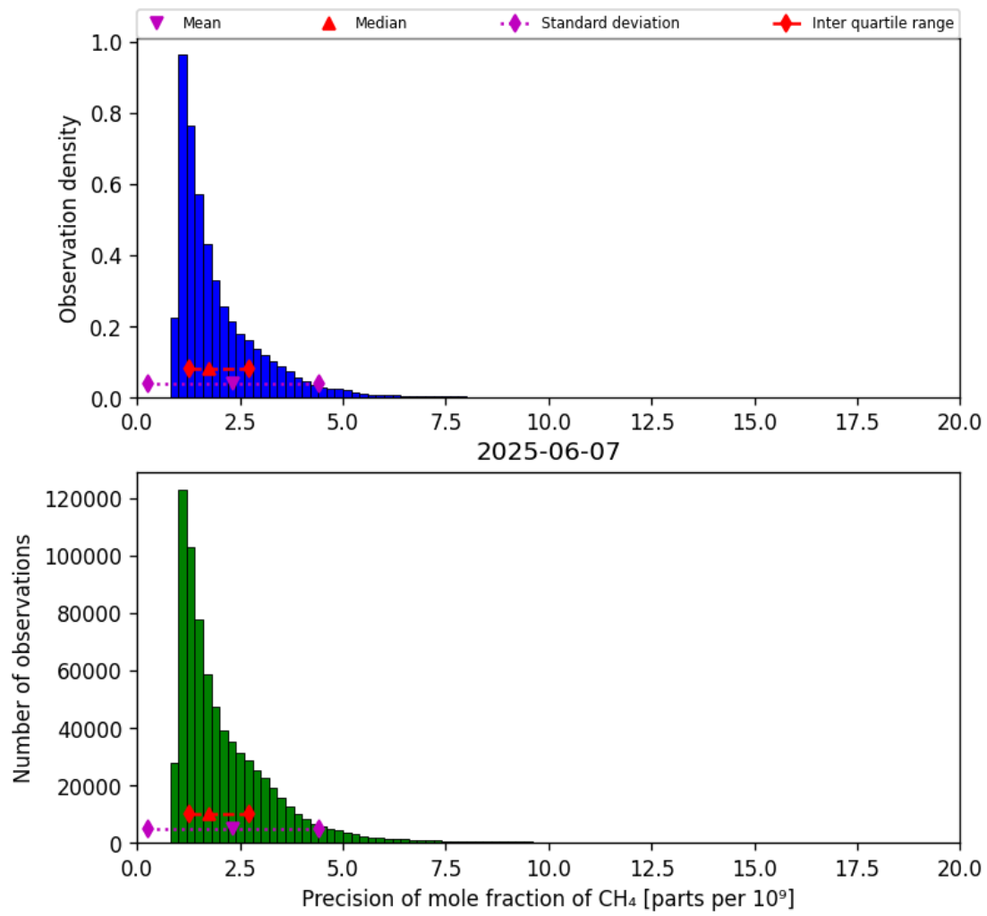
Figure 24: Histogram of “Precision of mole fraction of CH 4 ” for 2025-06-06 to 2025-06-08
