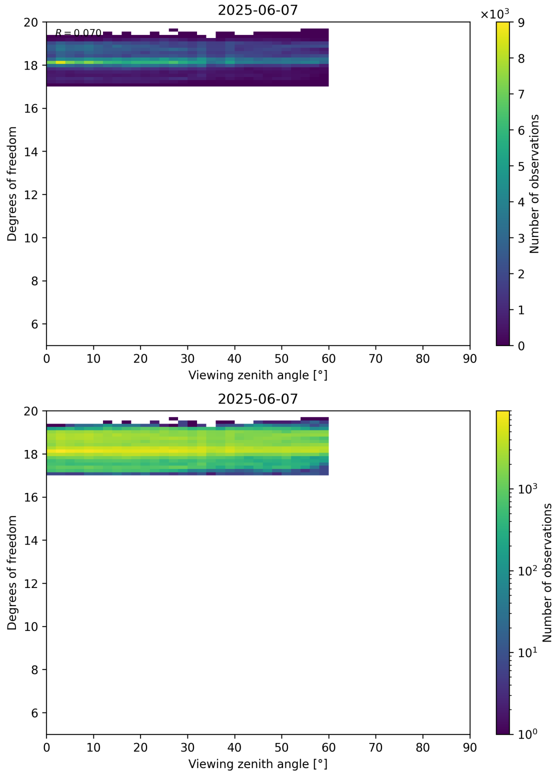
Figure 107: Scatter density plot of “Viewing zenith angle” against “Degrees of freedom” for 2025-06-06 to 2025-06-08.
