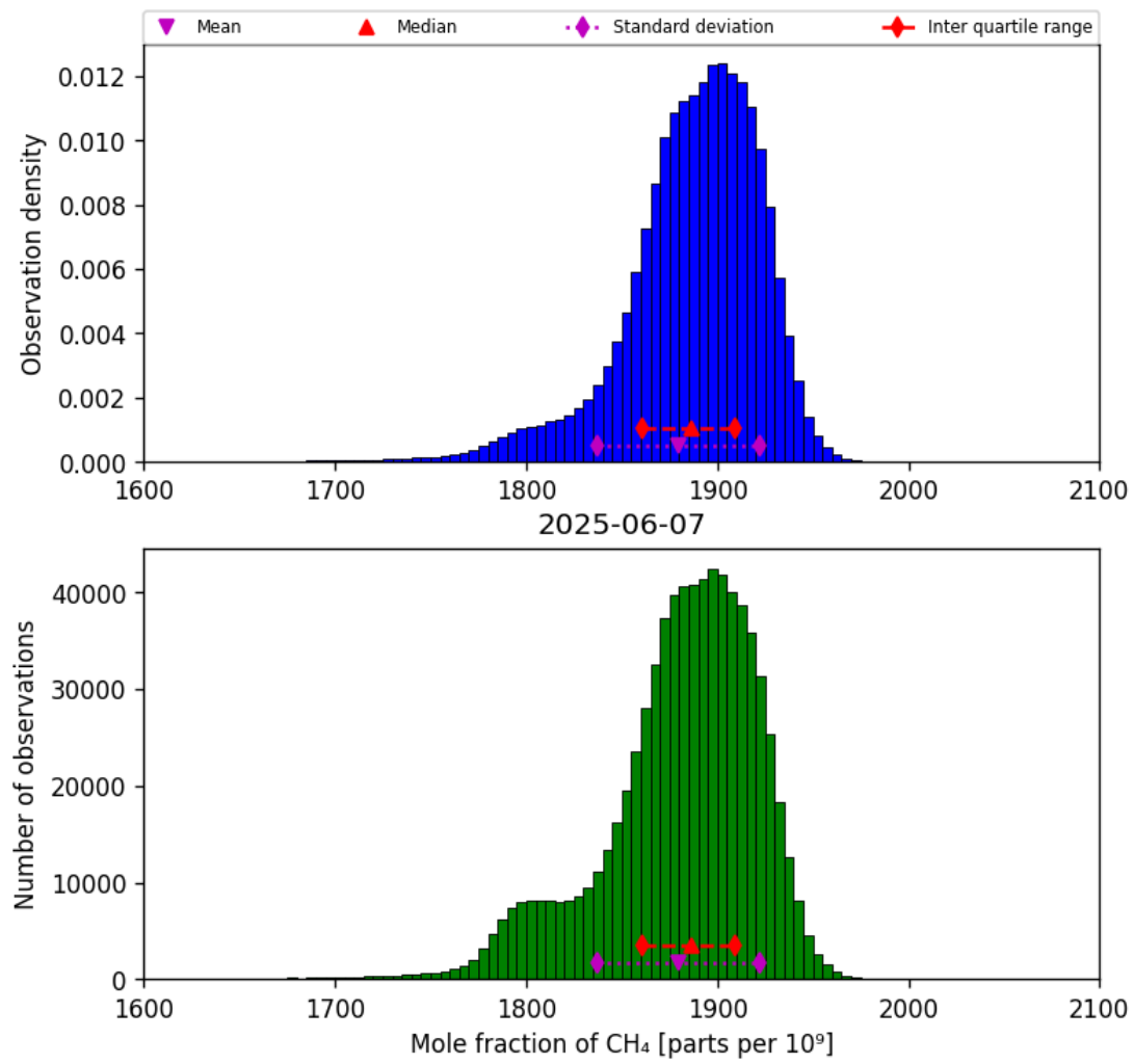
Figure 23: Histogram of “Mole fraction of CH 4 ” for 2025-06-06 to 2025-06-08
