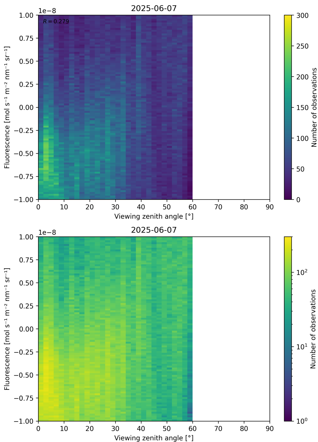
Figure 108: Scatter density plot of “Viewing zenith angle” against “Fluorescence” for 2025-06-06 to 2025-06-08.
