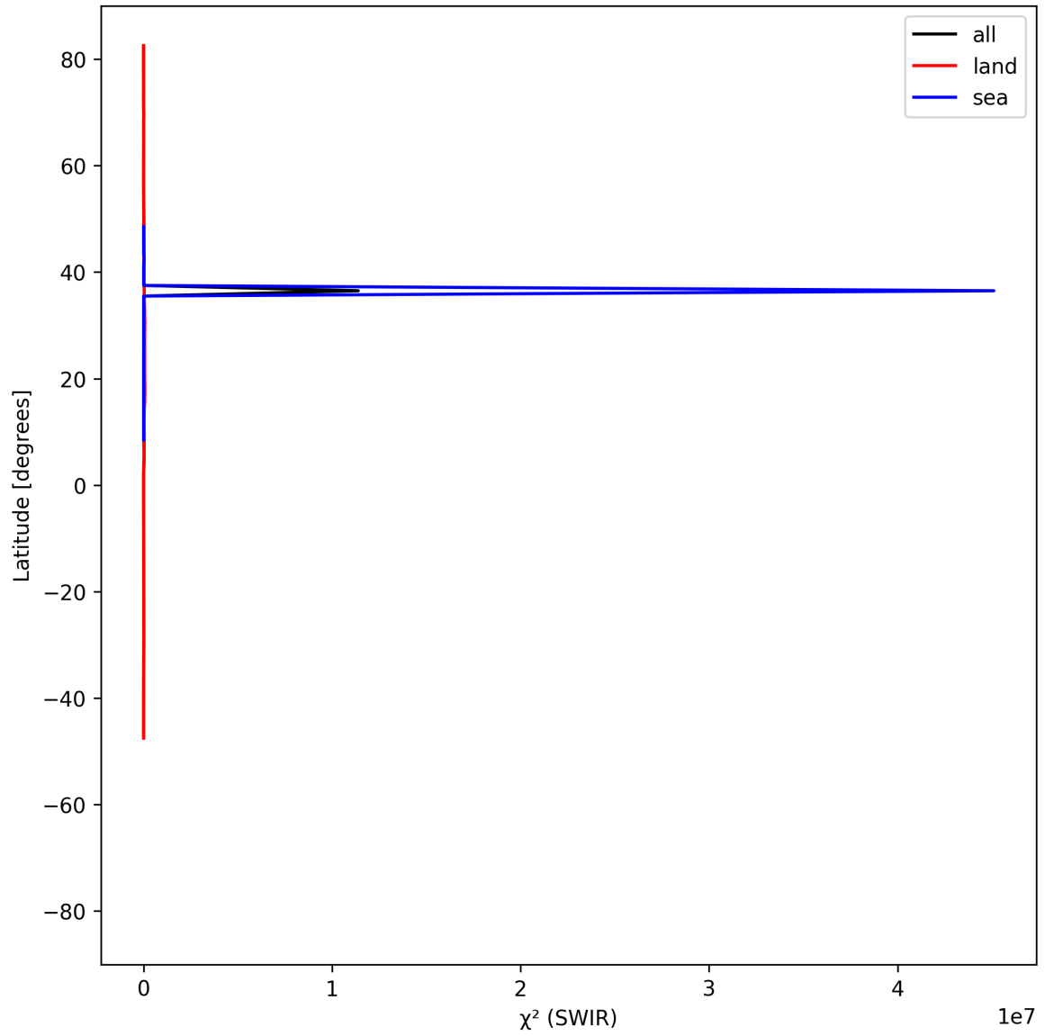
Figure 17: Zonal average of “ \chi^2 (SWIR)” for 2025-06-06 to 2025-06-08.
