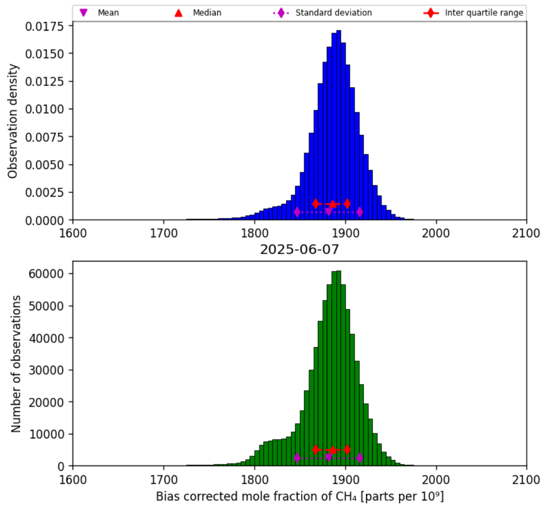
Figure 25: Histogram of “Bias corrected mole fraction of CH 4 ” for 2025-06-06 to 2025-06-08
