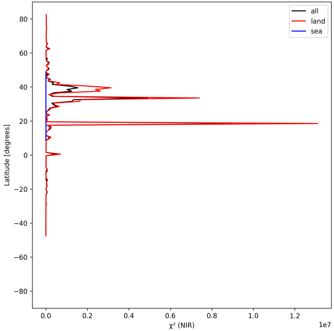
Figure 18: Zonal average of “ \chi^2 (NIR)” for 2025-06-06 to 2025-06-08.
