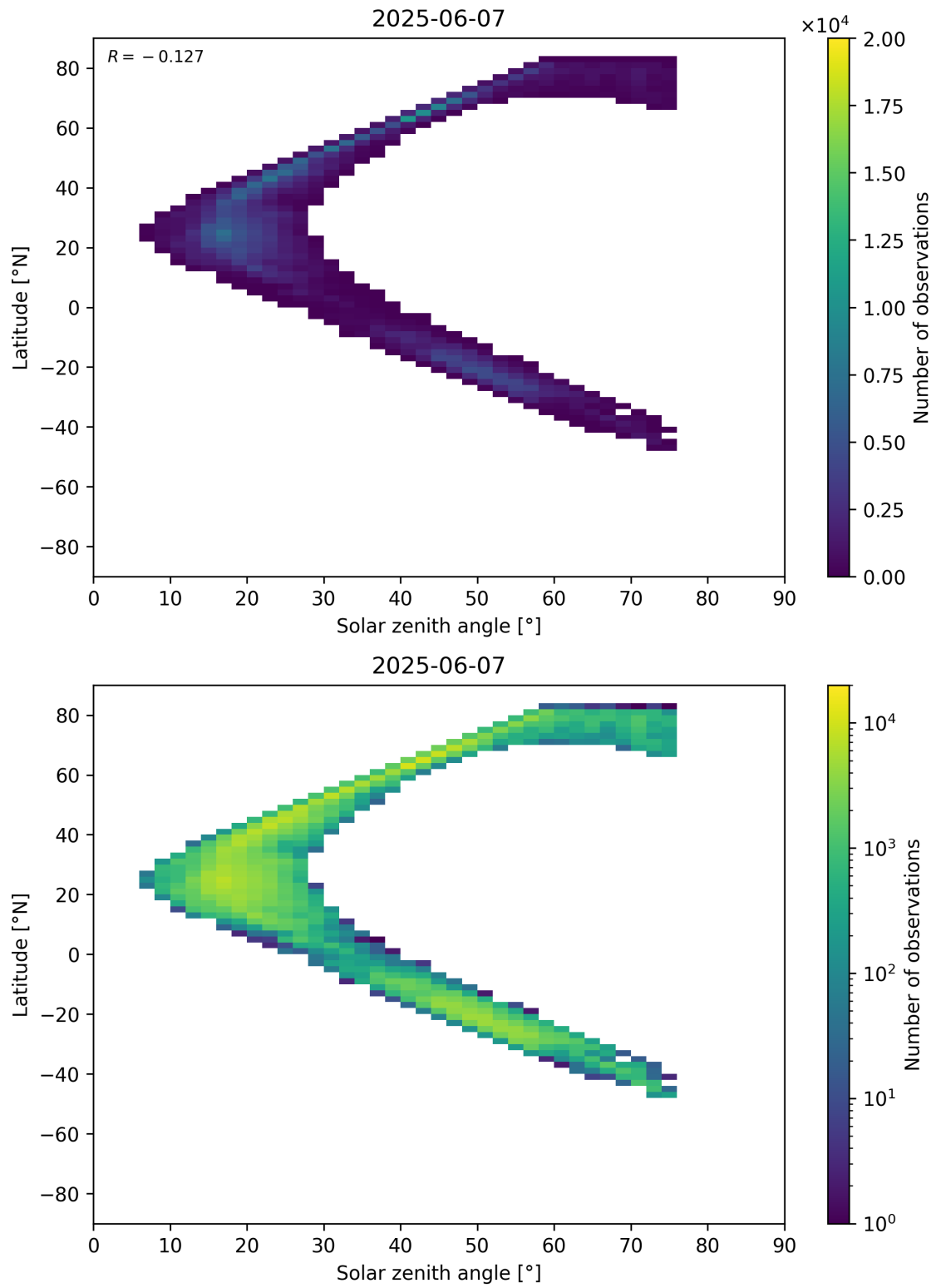
Figure 98: Scatter density plot of “Solar zenith angle” against “Latitude” for 2025-06-06 to 2025-06-08.
