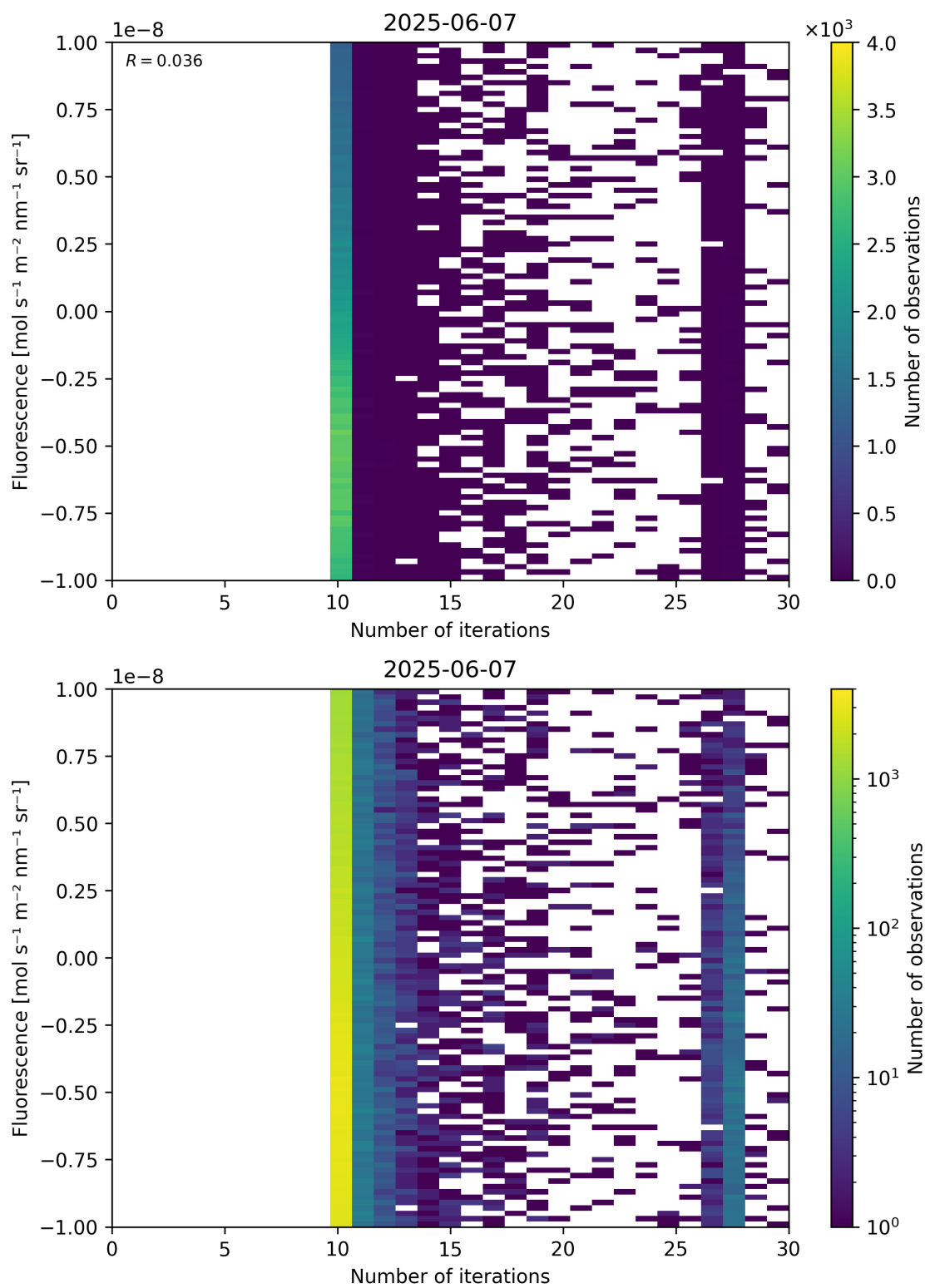
Figure 87: Scatter density plot of “Number of iterations” against “Fluorescence” for 2025-06-06 to 2025-06-08.
