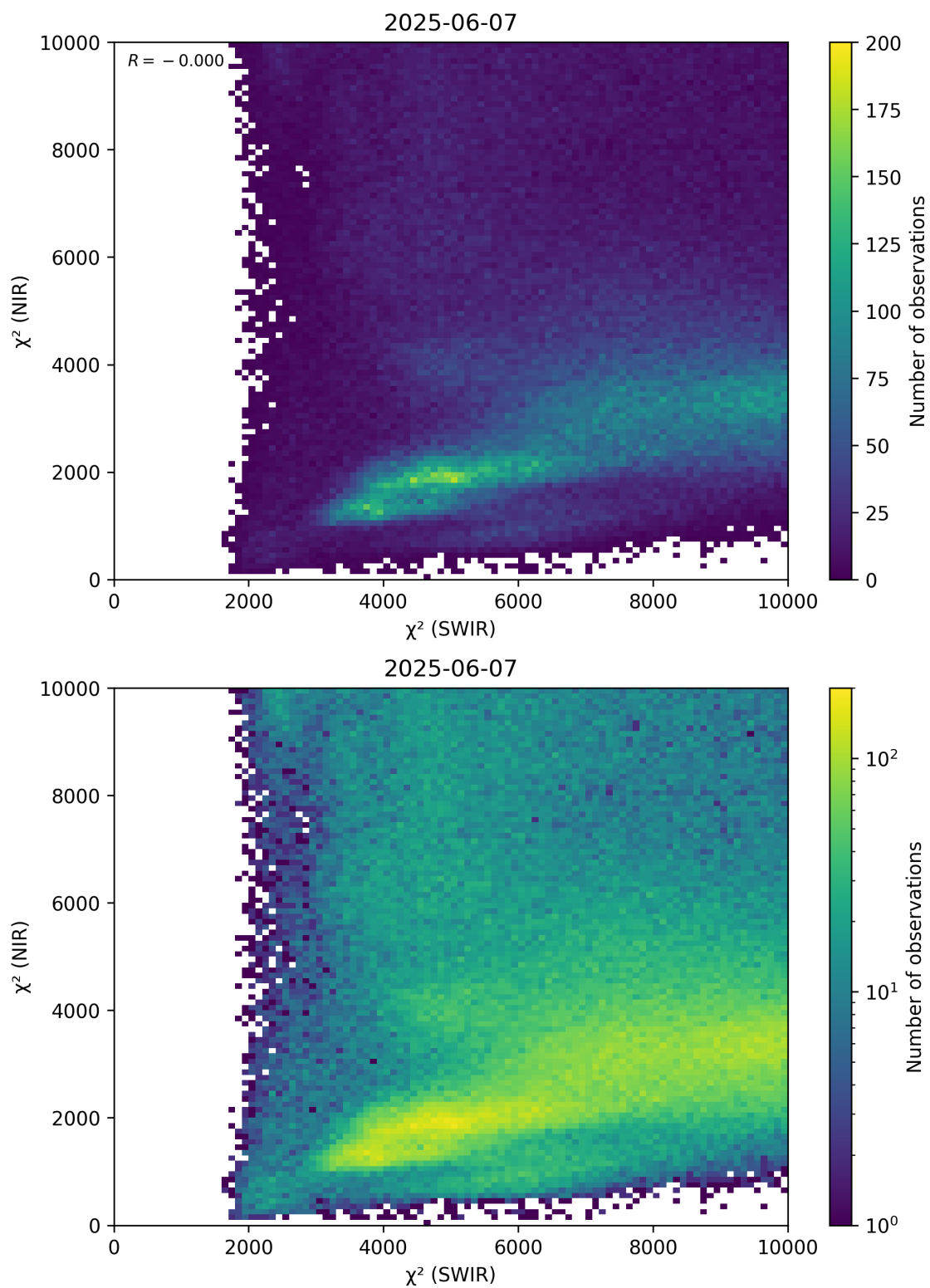
Figure 47: Scatter density plot of “ \chi^2 (SWIR)” against “ \chi^2 (NIR)” for 2025-06-06 to 2025-06-08.
