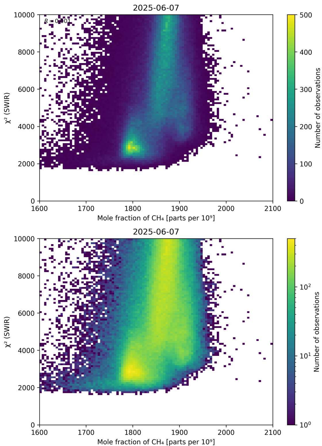
Figure 71: Scatter density plot of “Mole fraction of \text{CH}_4 ” against “ \chi^2 (SWIR)” for 2025-06-06 to 2025-06-08.
