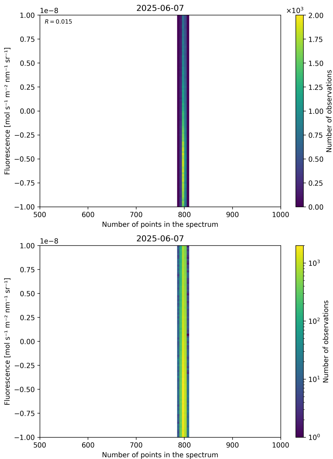
Figure 91: Scatter density plot of “Number of points in the spectrum” against “Fluorescence” for 2025-06-06 to 2025-06-08.
