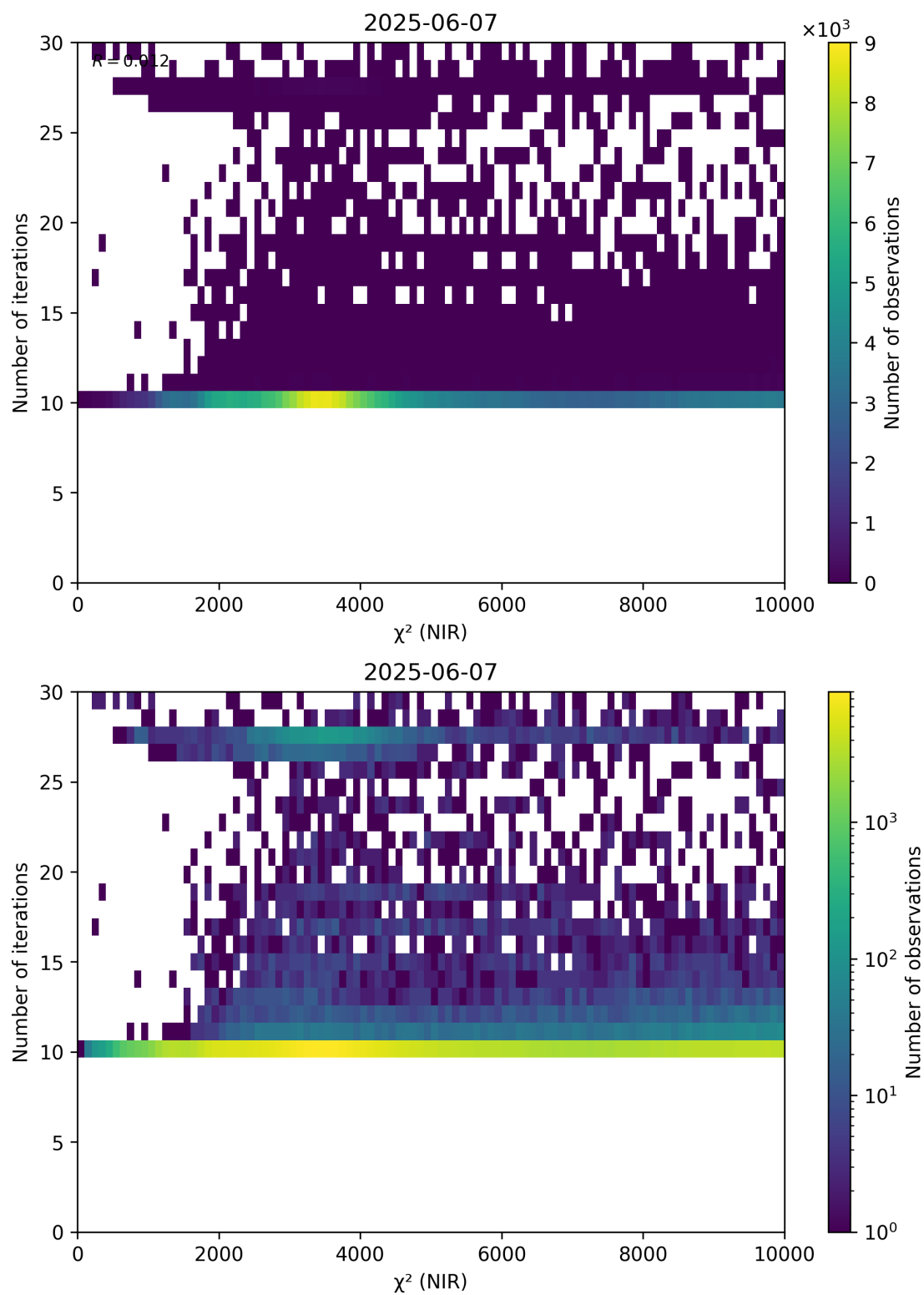
Figure 46: Scatter density plot of “ \chi^2 (NIR)” against “Number of iterations” for 2025-06-06 to 2025-06-08.
