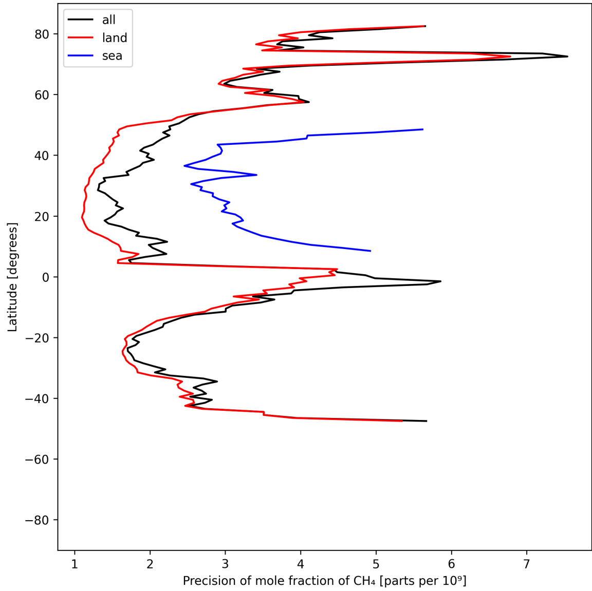
Figure 13: Zonal average of “Precision of mole fraction of CH 4 ” for 2025-06-06 to 2025-06-08.
