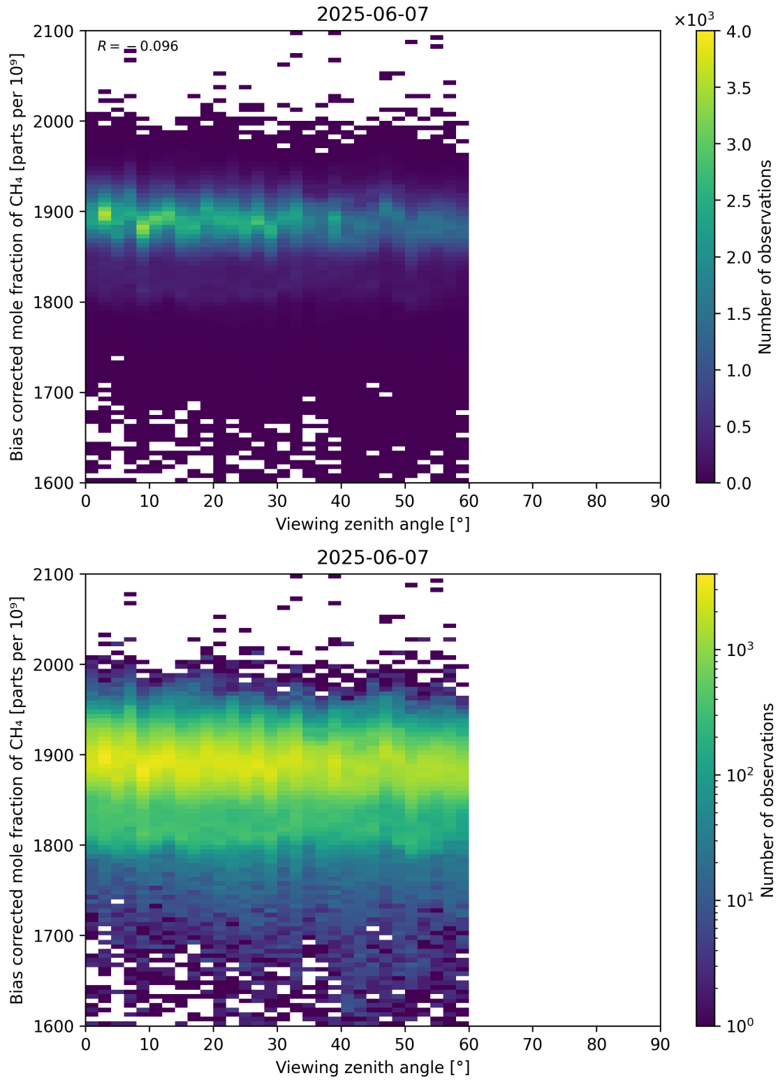
Figure 111: Scatter density plot of “Viewing zenith angle” against “Bias corrected mole fraction of CH 4 ” for 2025-06-06 to 2025-06-08.
