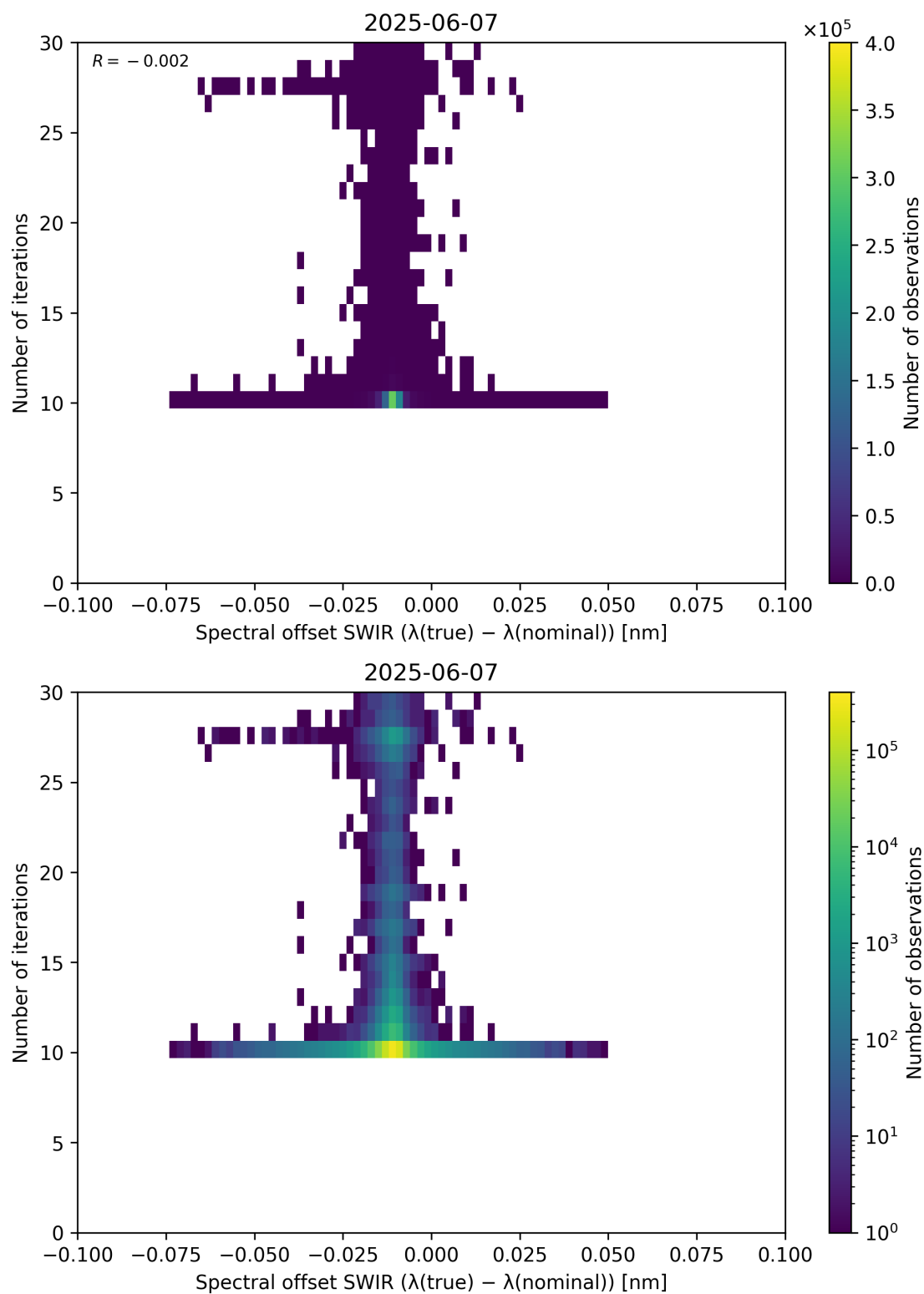
Figure 121: Scatter density plot of “Spectral offset SWIR ( \lambda_{\text{true}} - \lambda_{\text{nominal}} )” against “Number of iterations” for 2025-06-06 to 2025-06-08.
