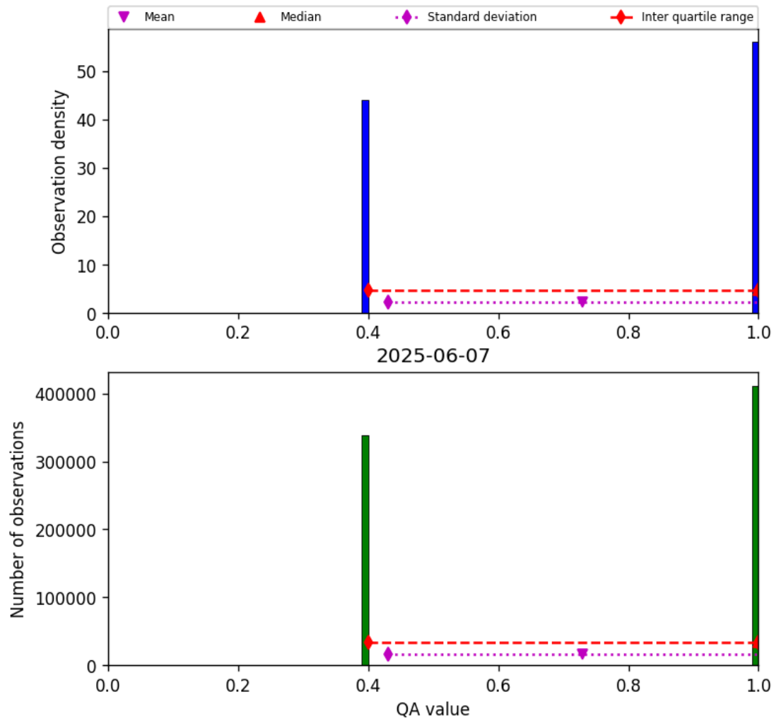
Figure 22: Histogram of “QA value” for 2025-06-06 to 2025-06-08
