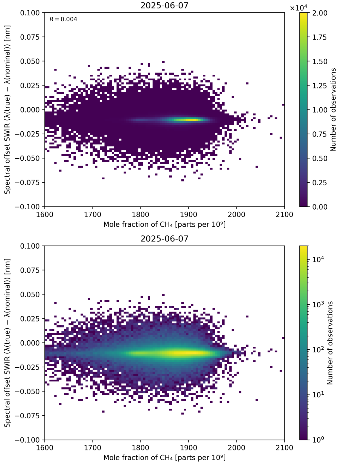
Figure 86: Scatter density plot of “Mole fraction of CH 4 ” against “Spectral offset SWIR ( \lambda_{\text{true}} - \lambda_{\text{nominal}} )” for 2025-06-06 to 2025-06-08.
