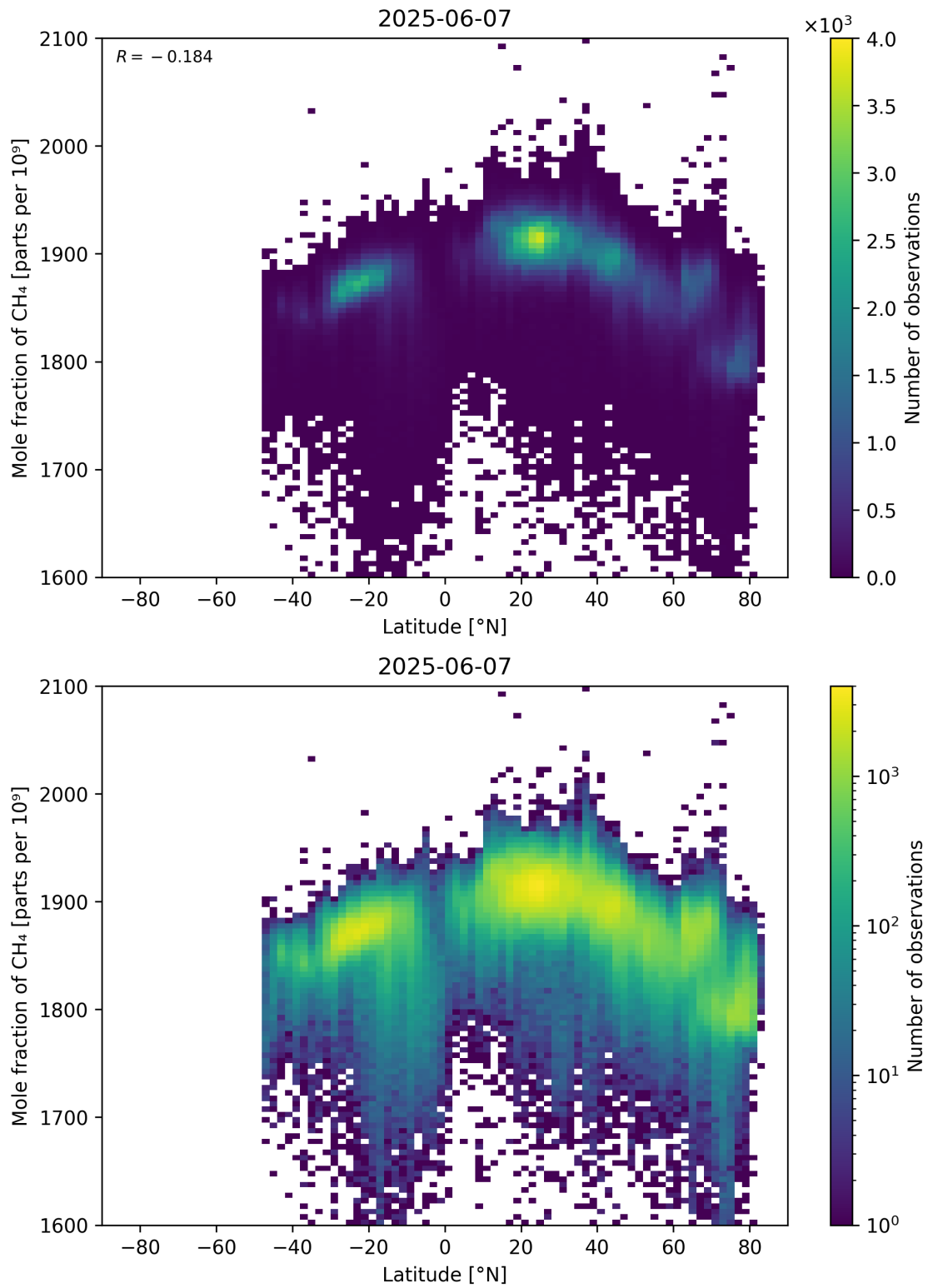
Figure 57: Scatter density plot of “Latitude” against “Mole fraction of \text{CH}_4 ” for 2025-06-06 to 2025-06-08.
