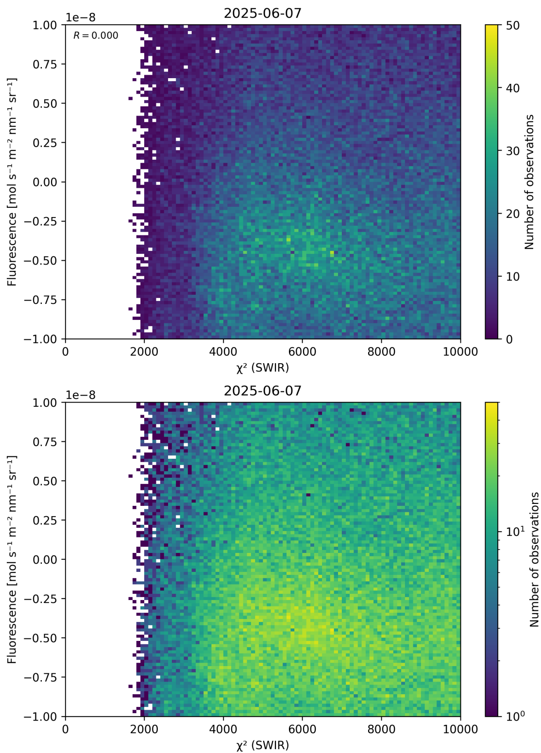
Figure 49: Scatter density plot of “ \chi^2 (SWIR)” against “Fluorescence” for 2025-06-06 to 2025-06-08.
