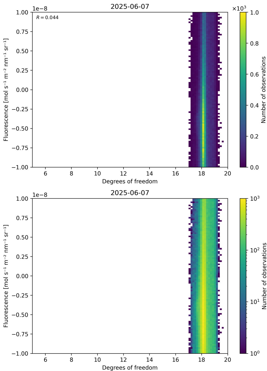
Figure 51: Scatter density plot of “Degrees of freedom” against “Fluorescence” for 2025-06-06 to 2025-06-08.
