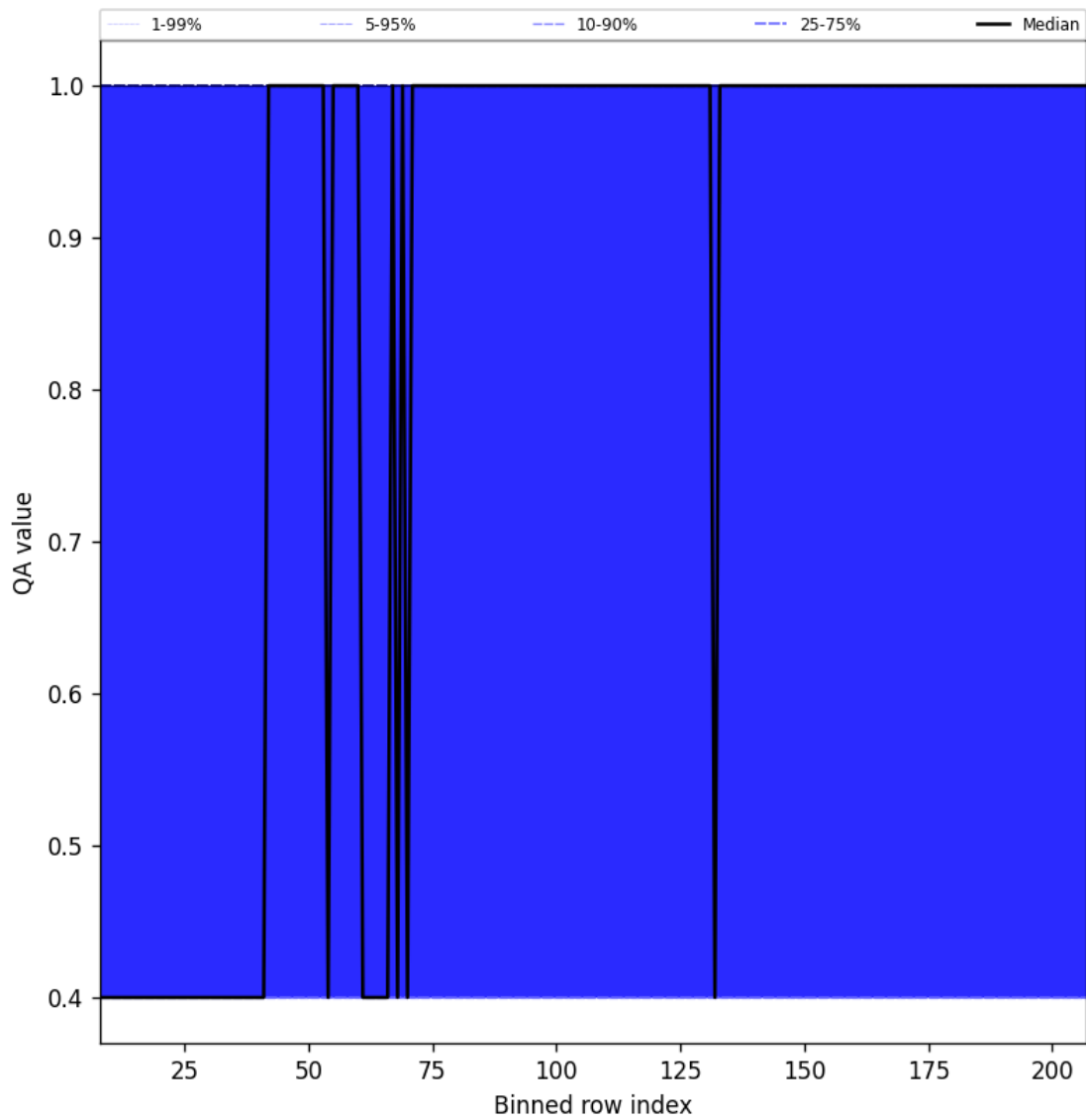
Figure 33: Along track statistics of “QA value” for 2025-06-06 to 2025-06-08
