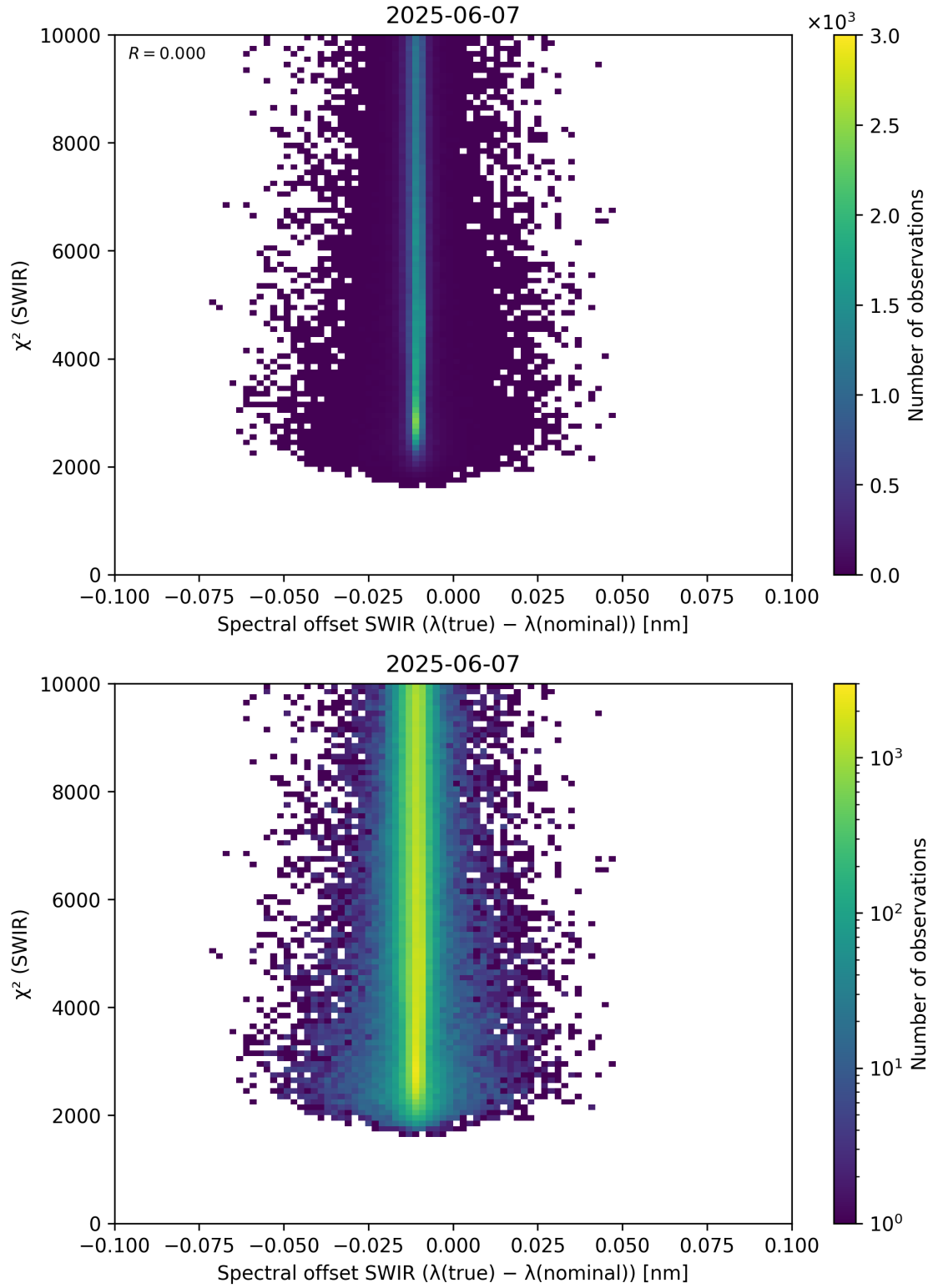
Figure 118: Scatter density plot of “Spectral offset SWIR ( \lambda_{\text{true}} - \lambda_{\text{nominal}} )” against “ \chi^2 (SWIR)” for 2025-06-06 to 2025-06-08.
