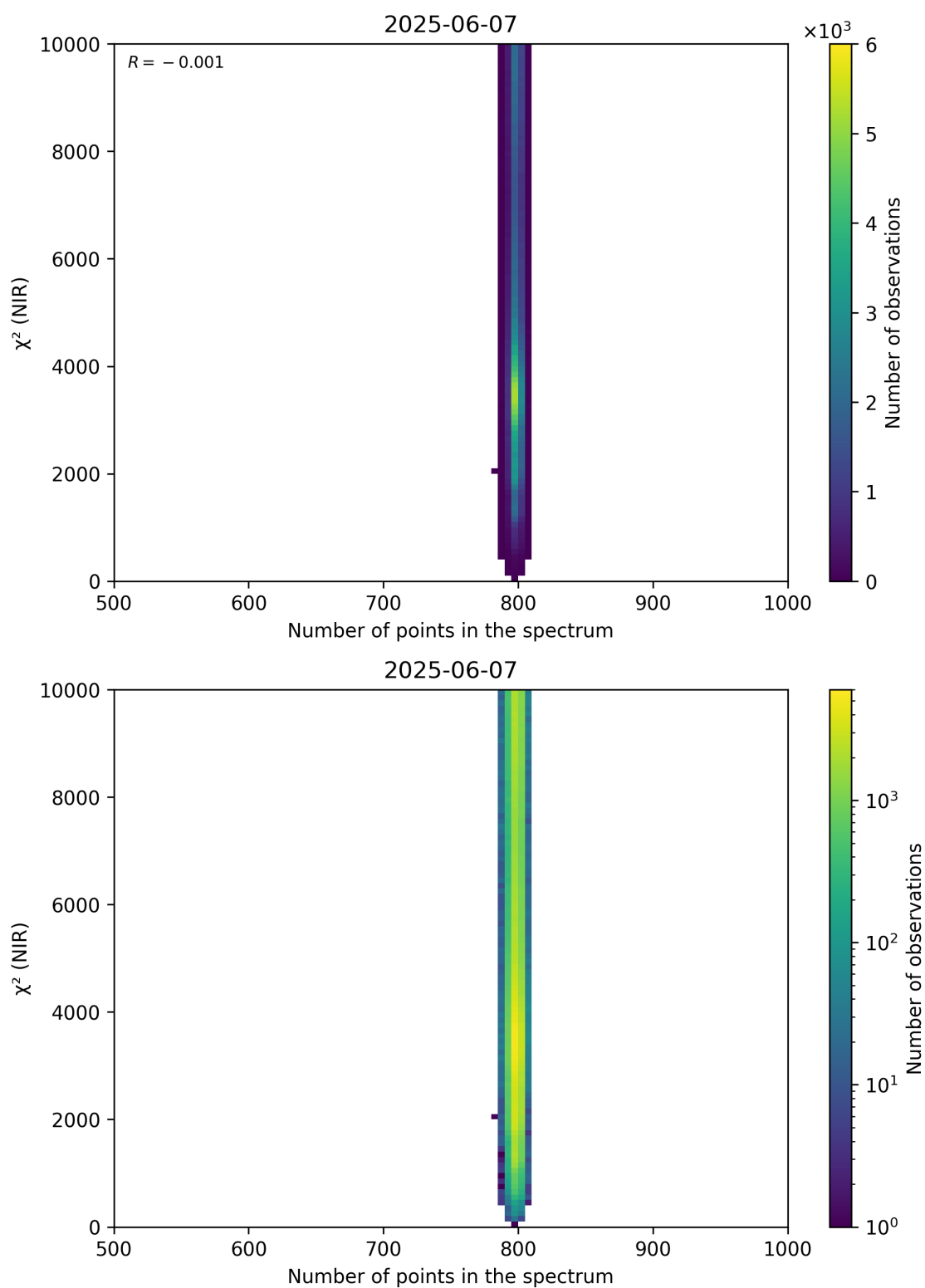
Figure 88: Scatter density plot of “Number of points in the spectrum” against “ \chi^2 (NIR)” for 2025-06-06 to 2025-06-08.
