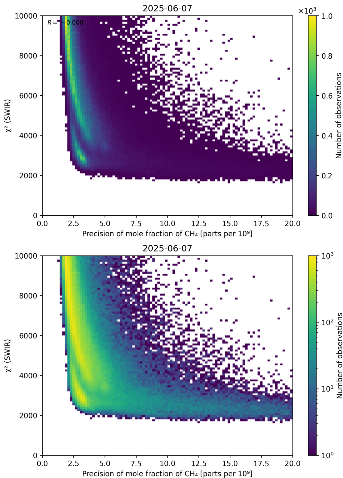
Figure 79: Scatter density plot of “Precision of mole fraction of CH 4 ” against “ \chi^2 (SWIR)” for 2025-06-06 to 2025-06-08.
