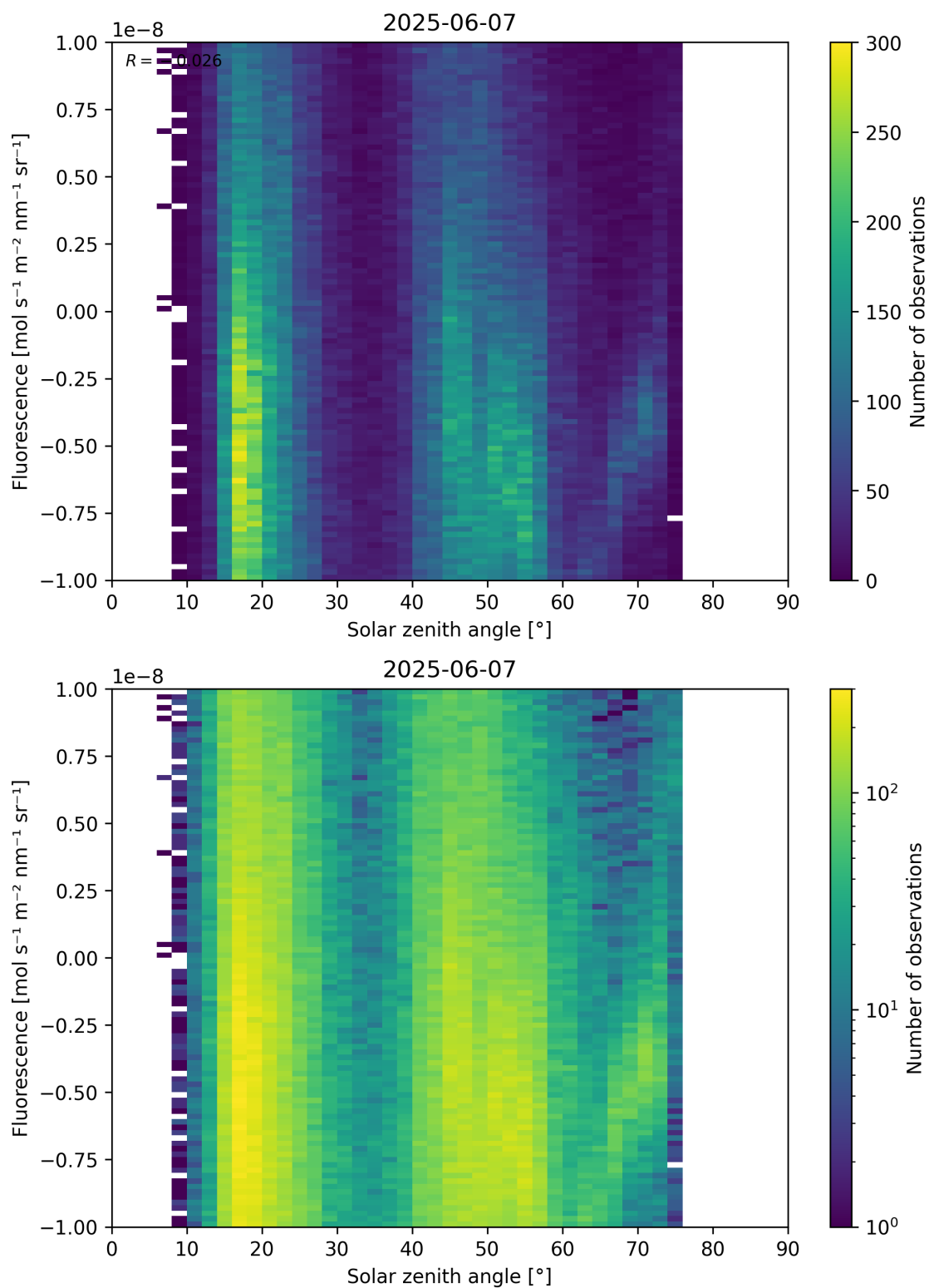
Figure 97: Scatter density plot of “Solar zenith angle” against “Fluorescence” for 2025-06-06 to 2025-06-08.
