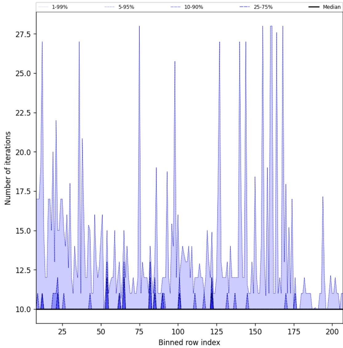
Figure 42: Along track statistics of “Number of iterations” for 2025-06-06 to 2025-06-08
