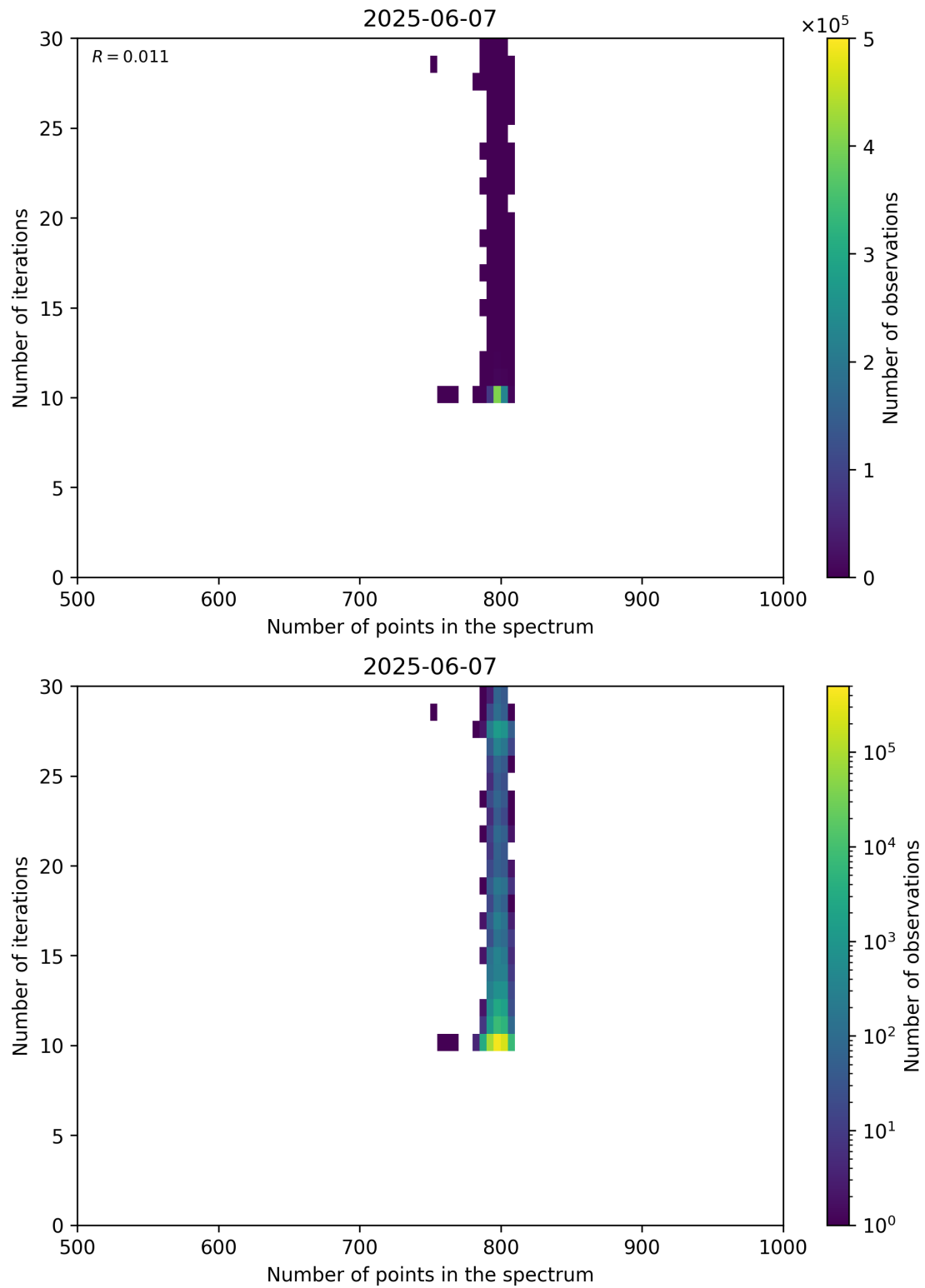
Figure 92: Scatter density plot of “Number of points in the spectrum” against “Number of iterations” for 2025-06-06 to 2025-06-08.
