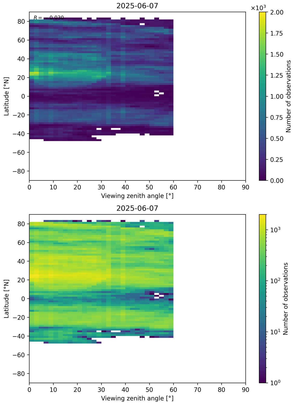
Figure 109: Scatter density plot of “Viewing zenith angle” against “Latitude” for 2025-06-06 to 2025-06-08.
