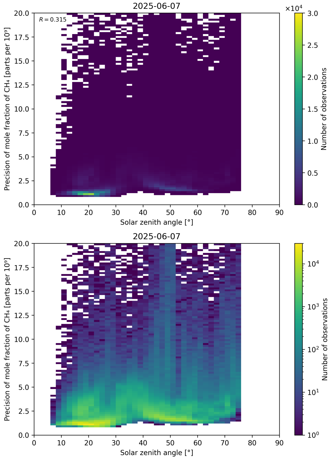
Figure 101: Scatter density plot of “Solar zenith angle” against “Precision of mole fraction of CH 4 ” for 2025-06-06 to 2025-06-08.
