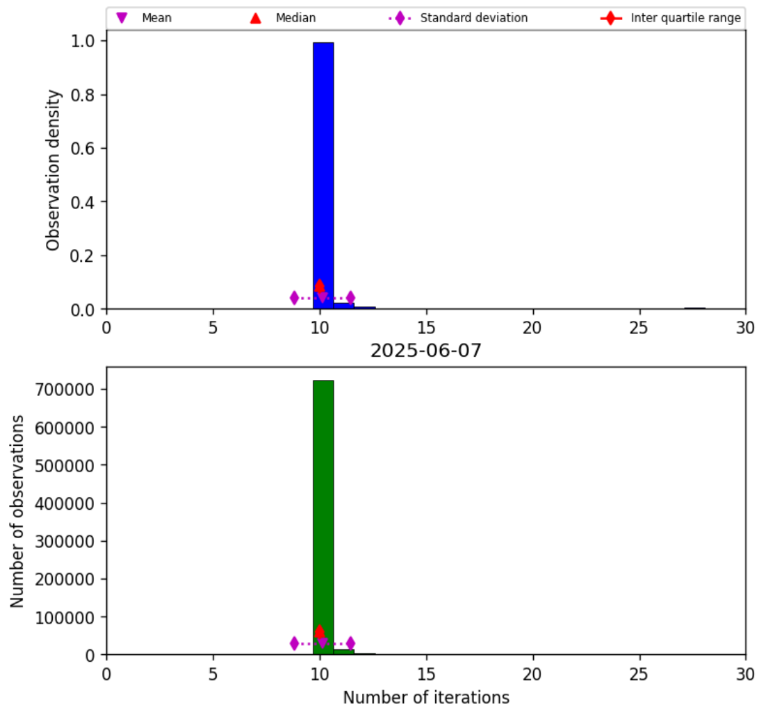
Figure 31: Histogram of “Number of iterations” for 2025-06-06 to 2025-06-08
