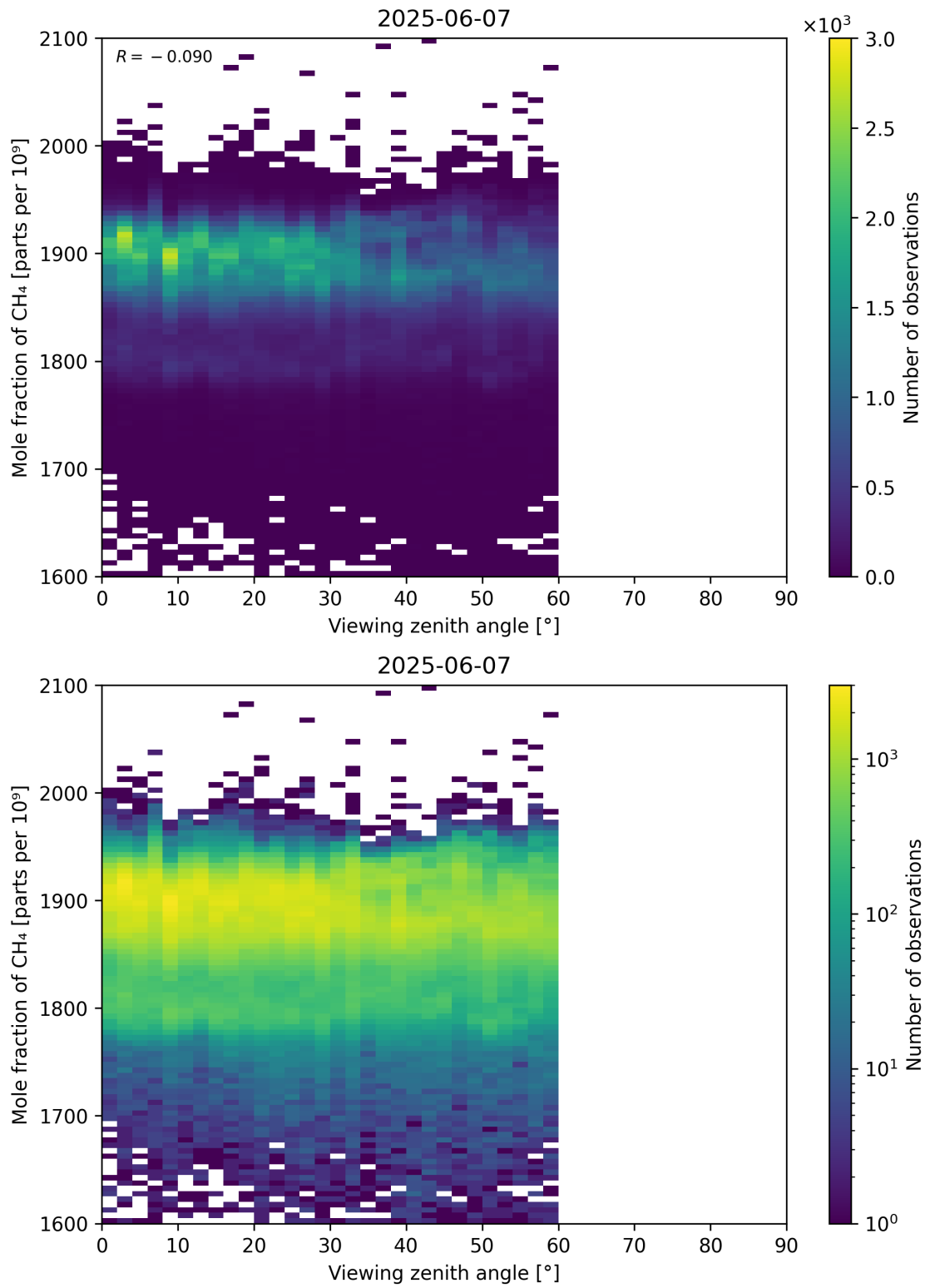
Figure 110: Scatter density plot of “Viewing zenith angle” against “Mole fraction of CH 4 ” for 2025-06-06 to 2025-06-08.
