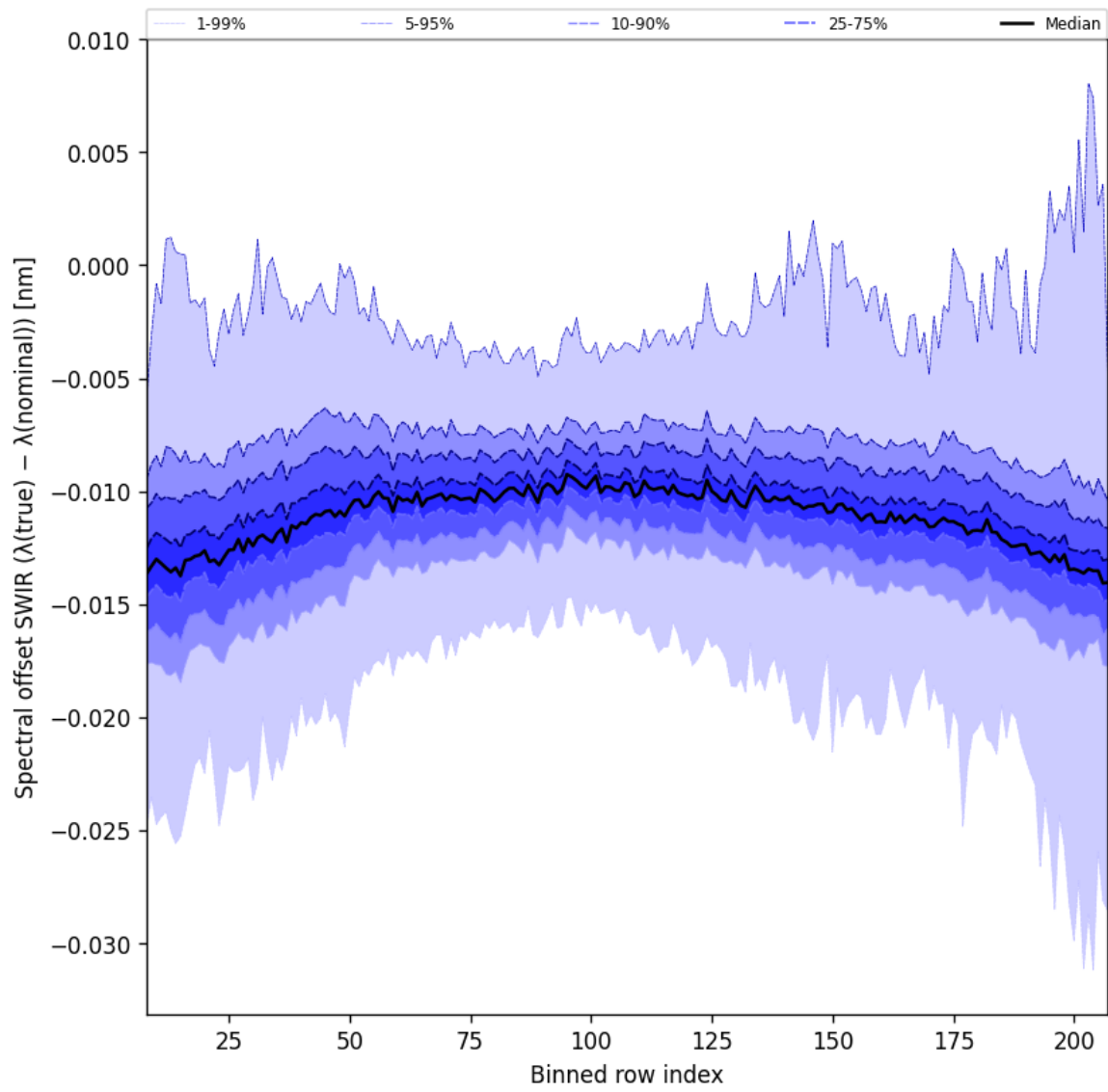
Figure 38: Along track statistics of “Spectral offset SWIR ( \lambda_{\text{true}} - \lambda_{\text{nominal}} )” for 2025-06-06 to 2025-06-08
