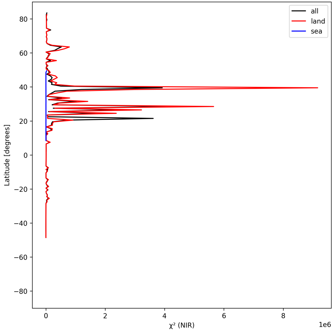
Figure 18: Zonal average of “ \chi^2 (NIR)” for 2025-06-07 to 2025-06-09.
