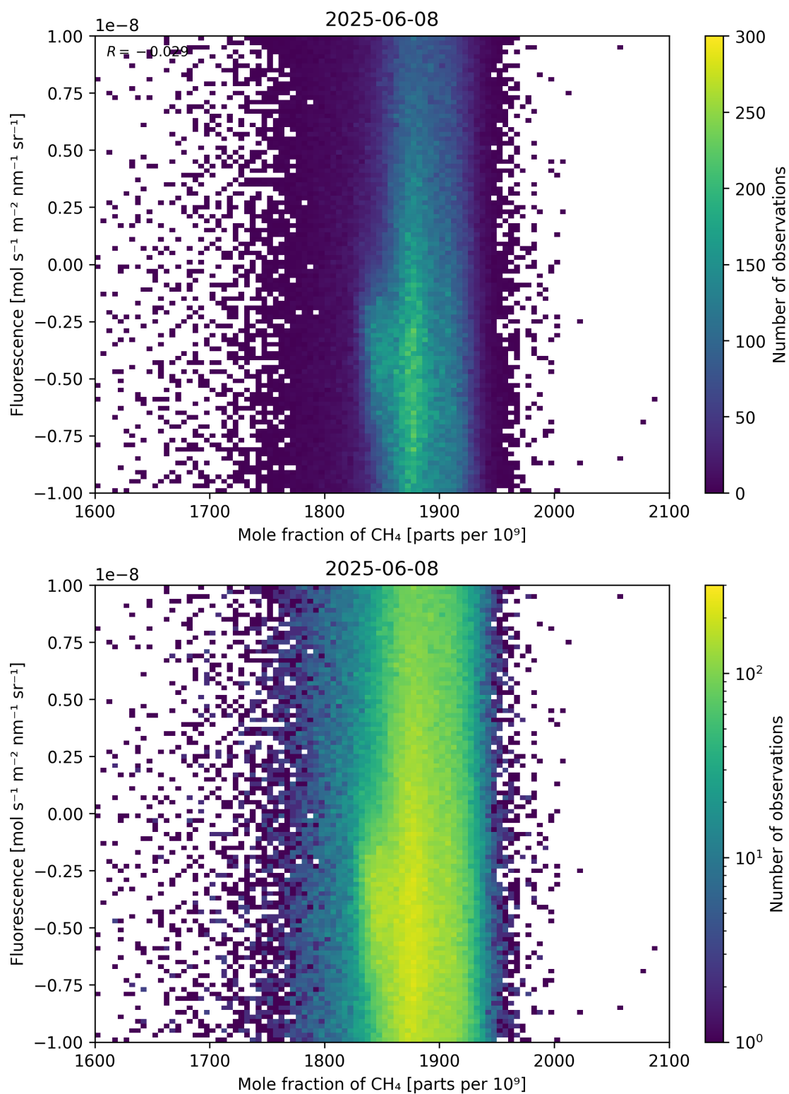
Figure 73: Scatter density plot of “Mole fraction of \text{CH}_4 ” against “Fluorescence” for 2025-06-07 to 2025-06-09.
