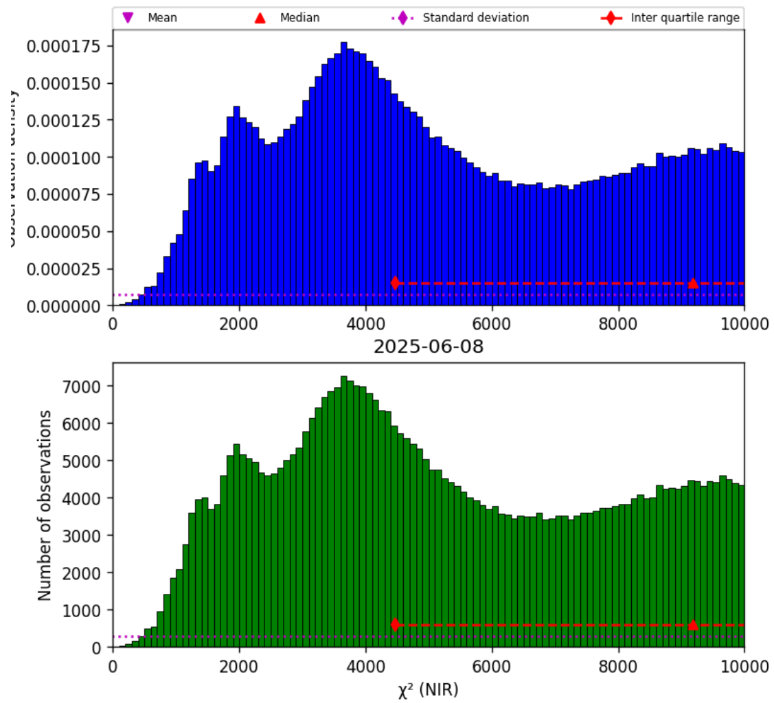
Figure 29: Histogram of “ \chi^2 (NIR)” for 2025-06-07 to 2025-06-09
