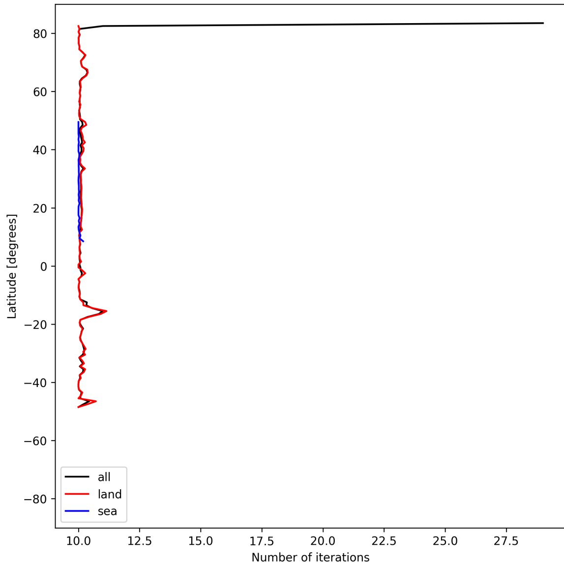
Figure 20: Zonal average of “Number of iterations” for 2025-06-07 to 2025-06-09.
