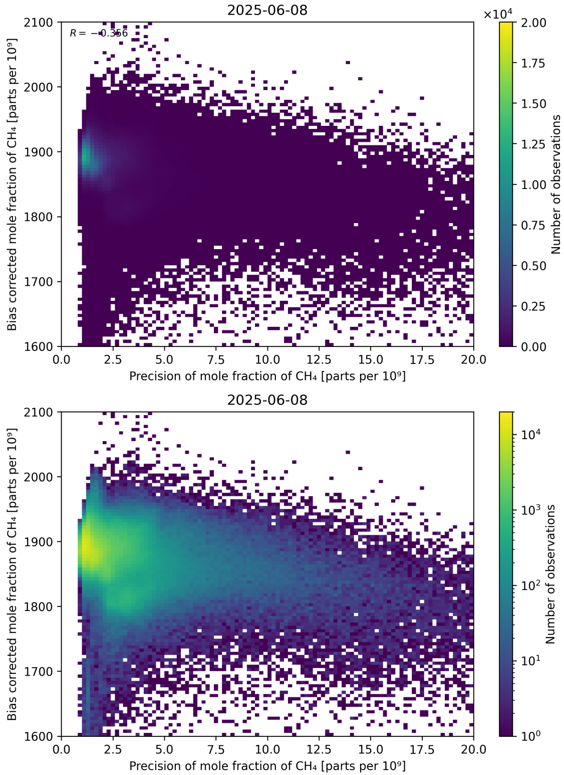
Figure 82: Scatter density plot of “Precision of mole fraction of CH 4 ” against “Bias corrected mole fraction of CH 4 ” for 2025-06-07 to 2025-06-09.
