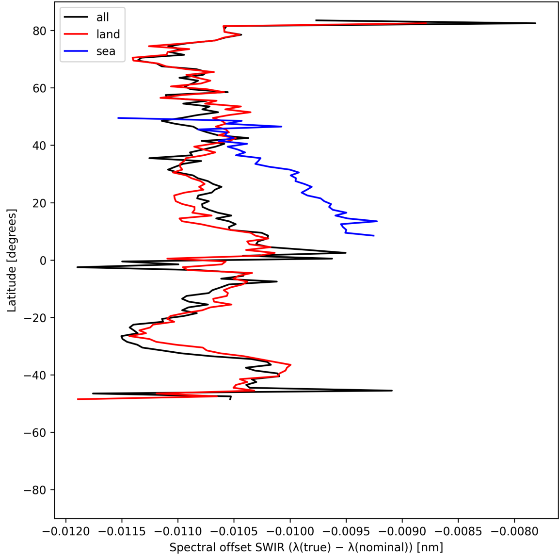
Figure 16: Zonal average of “Spectral offset SWIR ( \lambda_{\text{true}} - \lambda_{\text{nominal}} )” for 2025-06-07 to 2025-06-09.
