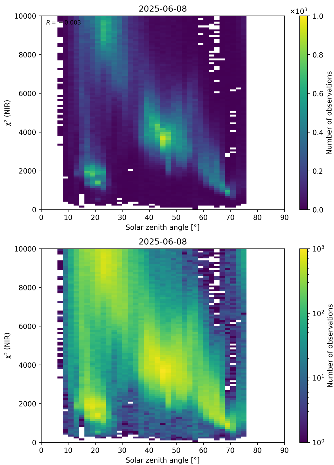
Figure 94: Scatter density plot of “Solar zenith angle” against “ \chi^2 (NIR)” for 2025-06-07 to 2025-06-09.
