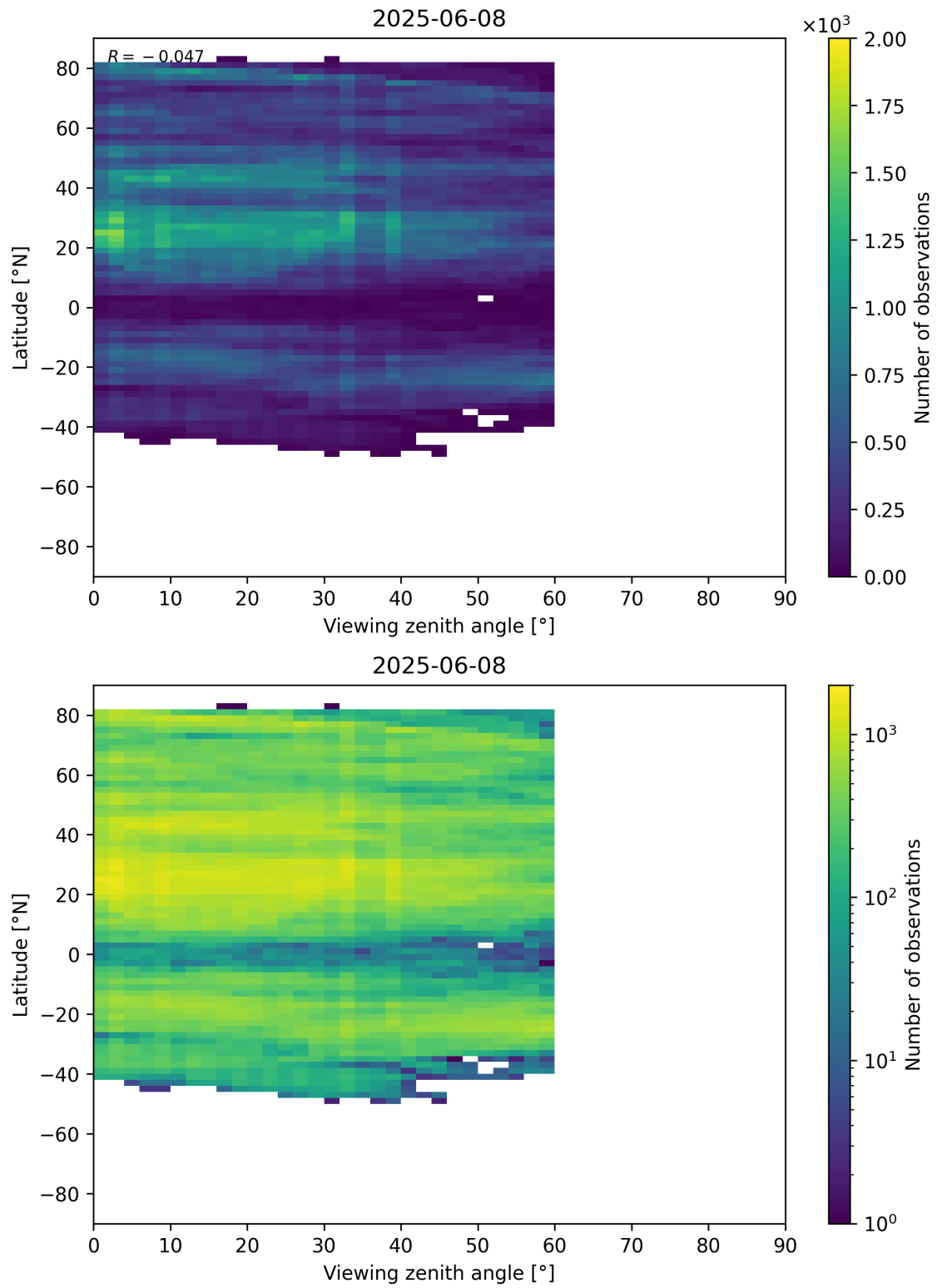
Figure 109: Scatter density plot of “Viewing zenith angle” against “Latitude” for 2025-06-07 to 2025-06-09.
