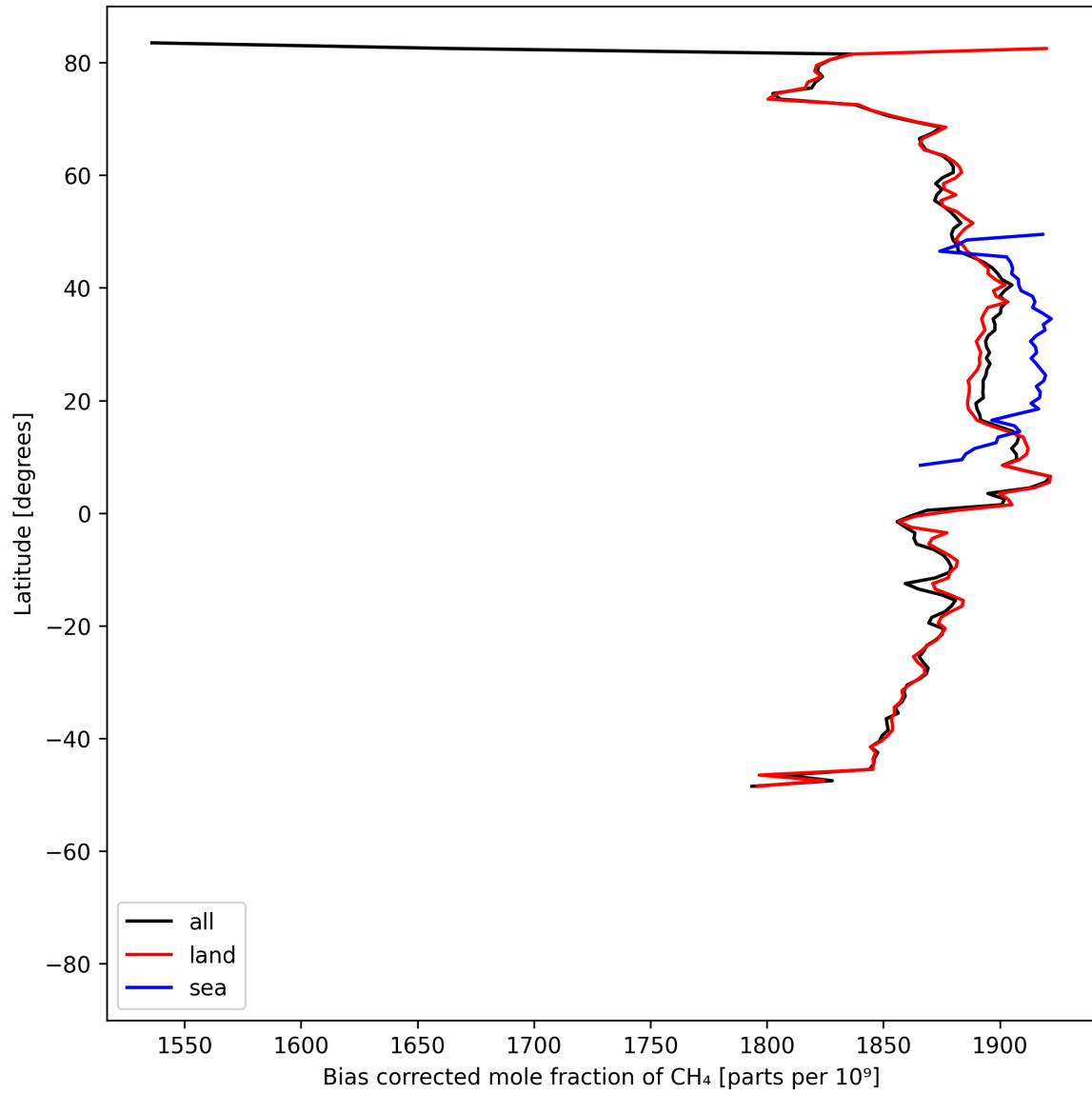
Figure 14: Zonal average of “Bias corrected mole fraction of \text{CH}_4 ” for 2025-06-07 to 2025-06-09.
