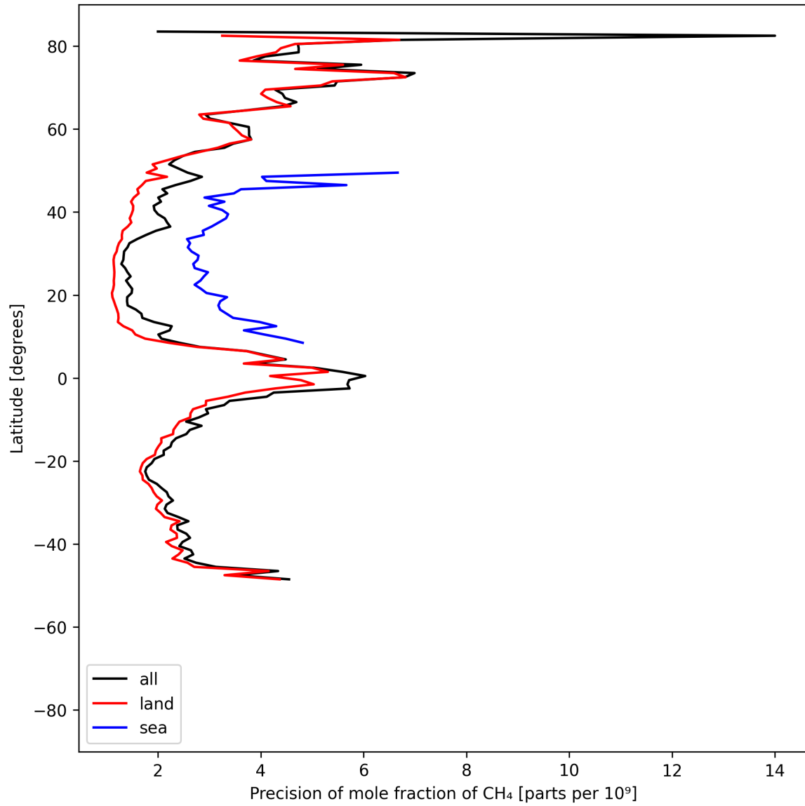
Figure 13: Zonal average of “Precision of mole fraction of \text{CH}_4 ” for 2025-06-07 to 2025-06-09.
