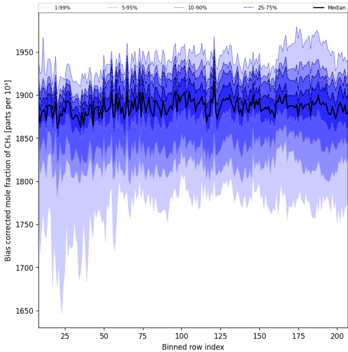
Figure 36: Along track statistics of “Bias corrected mole fraction of CH 4 ” for 2025-06-07 to 2025-06-09
