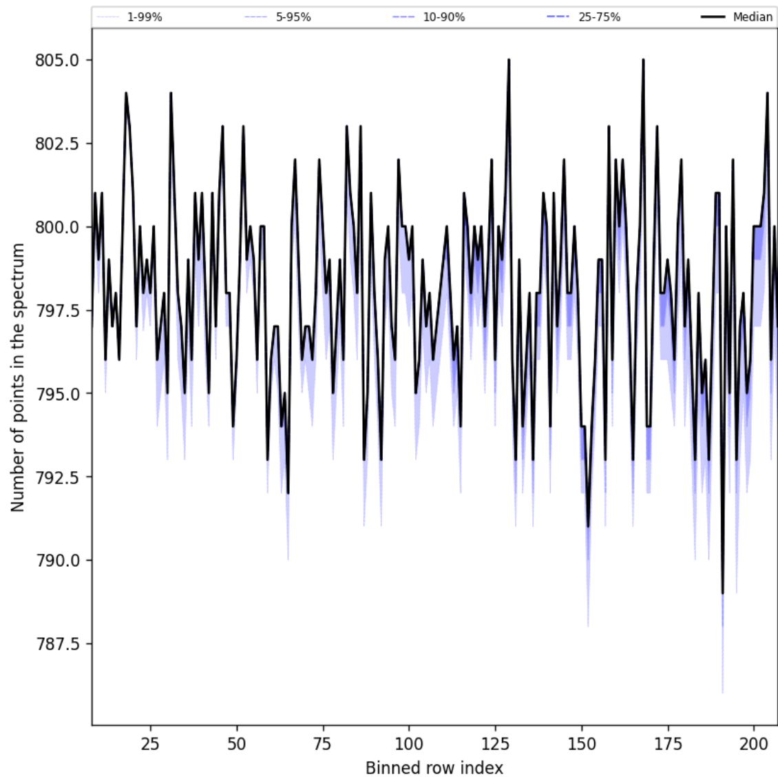
Figure 37: Along track statistics of “Number of points in the spectrum” for 2025-06-07 to 2025-06-09
