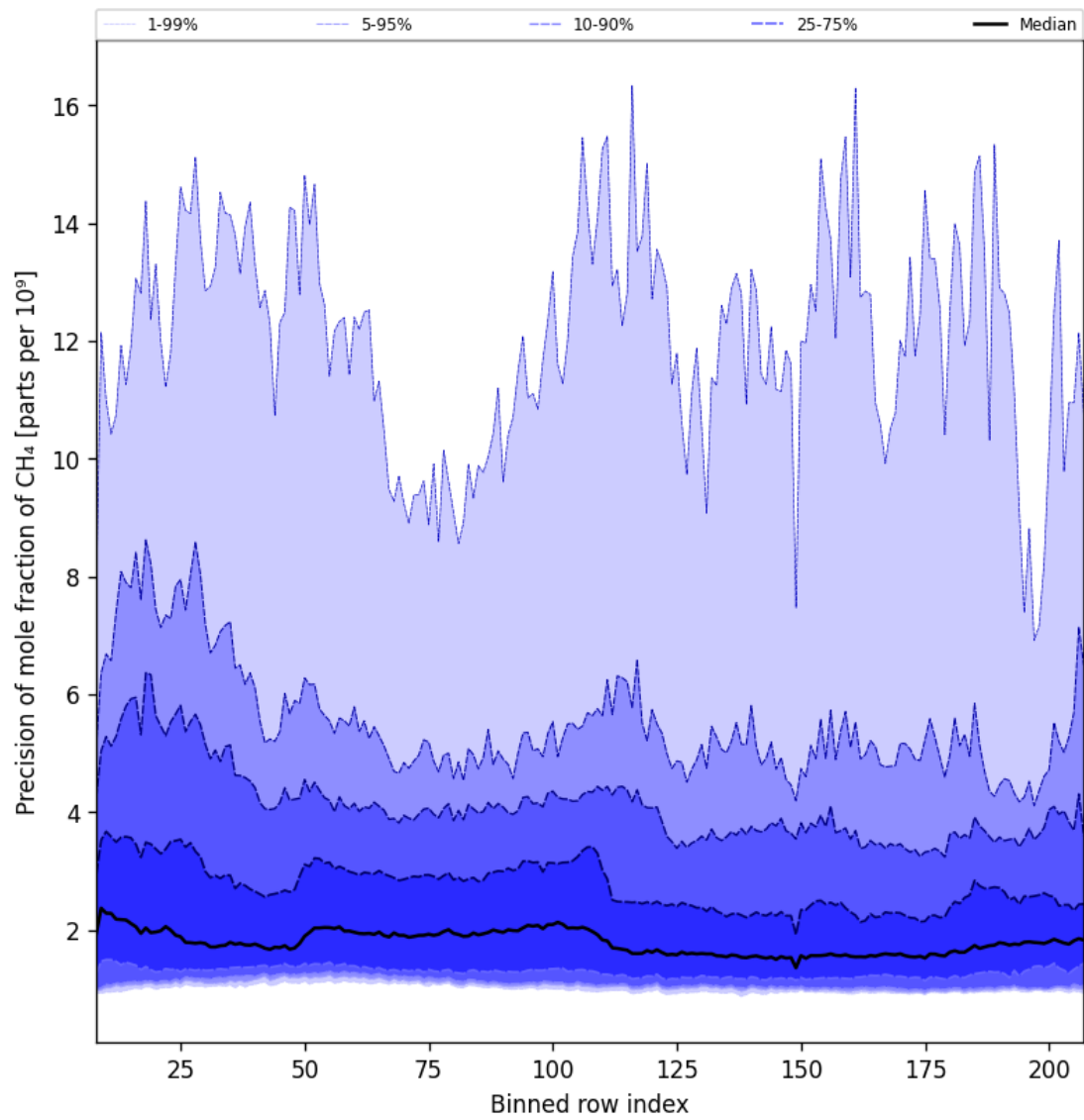
Figure 35: Along track statistics of “Precision of mole fraction of CH 4 ” for 2025-06-07 to 2025-06-09
