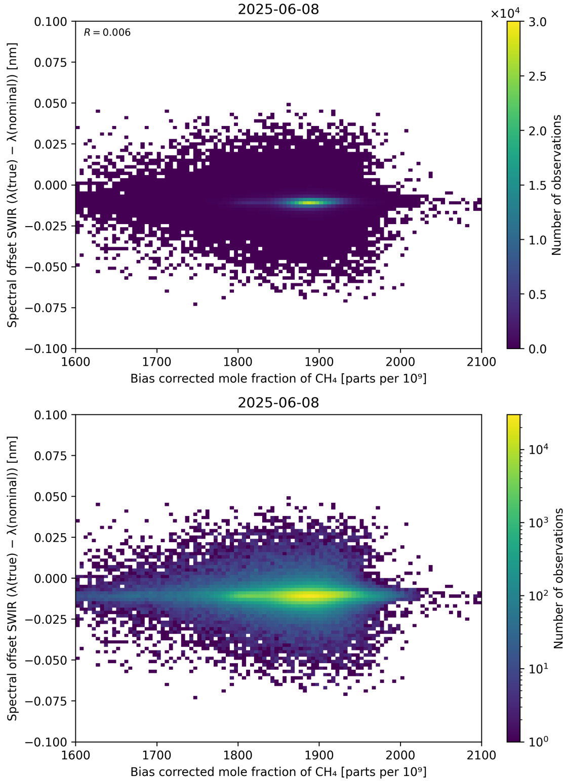
Figure 69: Scatter density plot of “Bias corrected mole fraction of \text{CH}_4 ” against “Spectral offset SWIR ( \lambda_{\text{true}} - \lambda_{\text{nominal}} )” for 2025-06-07 to 2025-06-09.
