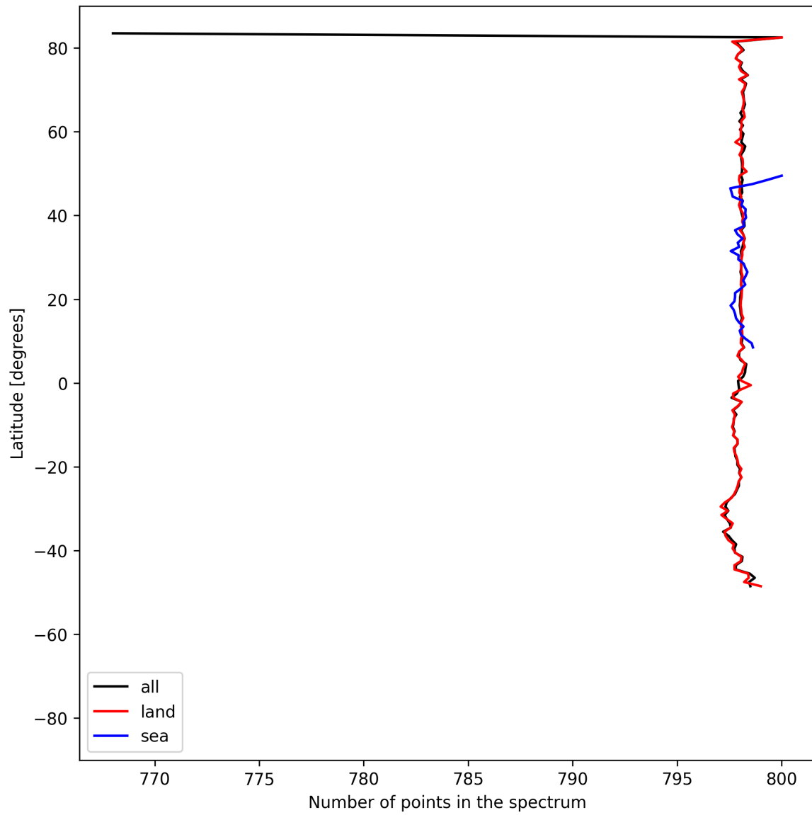
Figure 15: Zonal average of “Number of points in the spectrum” for 2025-06-07 to 2025-06-09.
