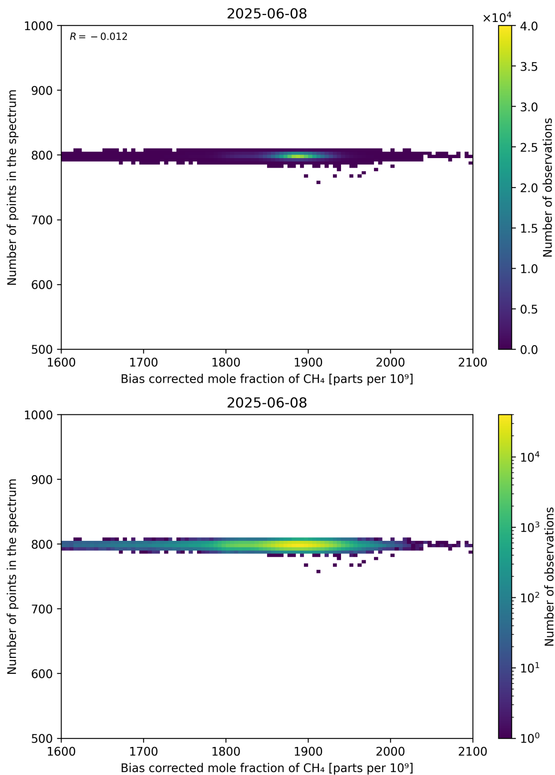
Figure 68: Scatter density plot of “Bias corrected mole fraction of CH 4 ” against “Number of points in the spectrum” for 2025-06-07 to 2025-06-09.
