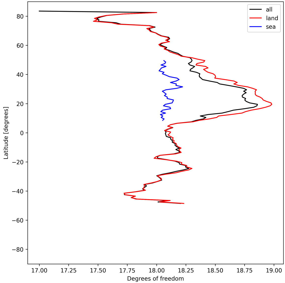
Figure 19: Zonal average of “Degrees of freedom” for 2025-06-07 to 2025-06-09.
