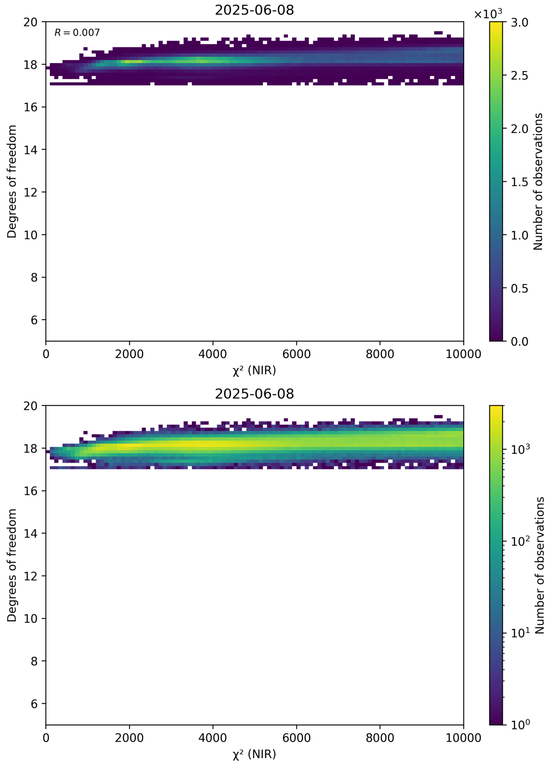
Figure 44: Scatter density plot of “ \chi^2 (NIR)” against “Degrees of freedom” for 2025-06-07 to 2025-06-09.
