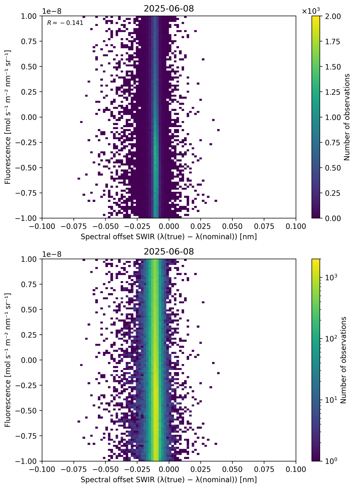
Figure 120: Scatter density plot of “Spectral offset SWIR ( \lambda_{\text{true}} - \lambda_{\text{nominal}} )” against “Fluorescence” for 2025-06-07 to 2025-06-09.
