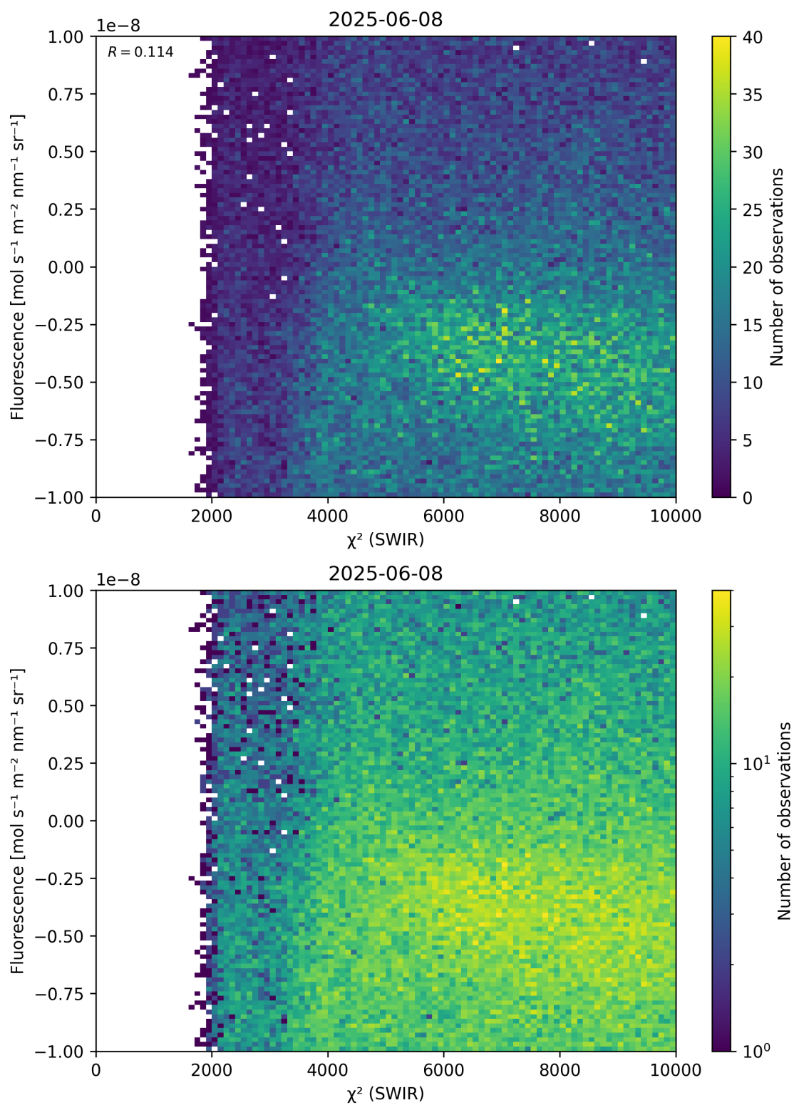
Figure 49: Scatter density plot of “ \chi^2 (SWIR)” against “Fluorescence” for 2025-06-07 to 2025-06-09.
