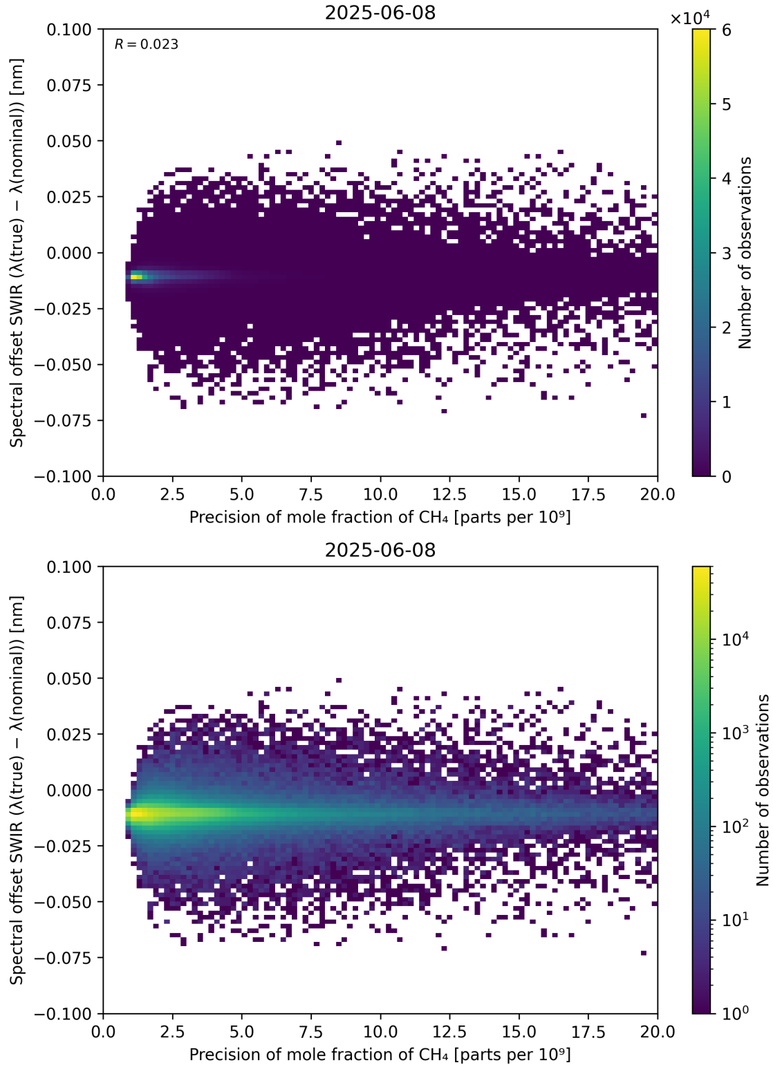
Figure 85: Scatter density plot of “Precision of mole fraction of \text{CH}_4 ” against “Spectral offset SWIR ( \lambda_{\text{true}} - \lambda_{\text{nominal}} )” for 2025-06-07 to 2025-06-09.
