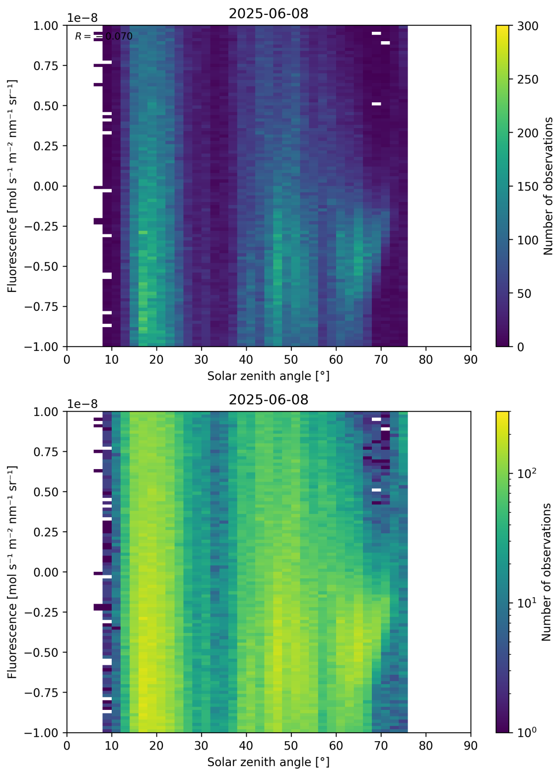
Figure 97: Scatter density plot of “Solar zenith angle” against “Fluorescence” for 2025-06-07 to 2025-06-09.
