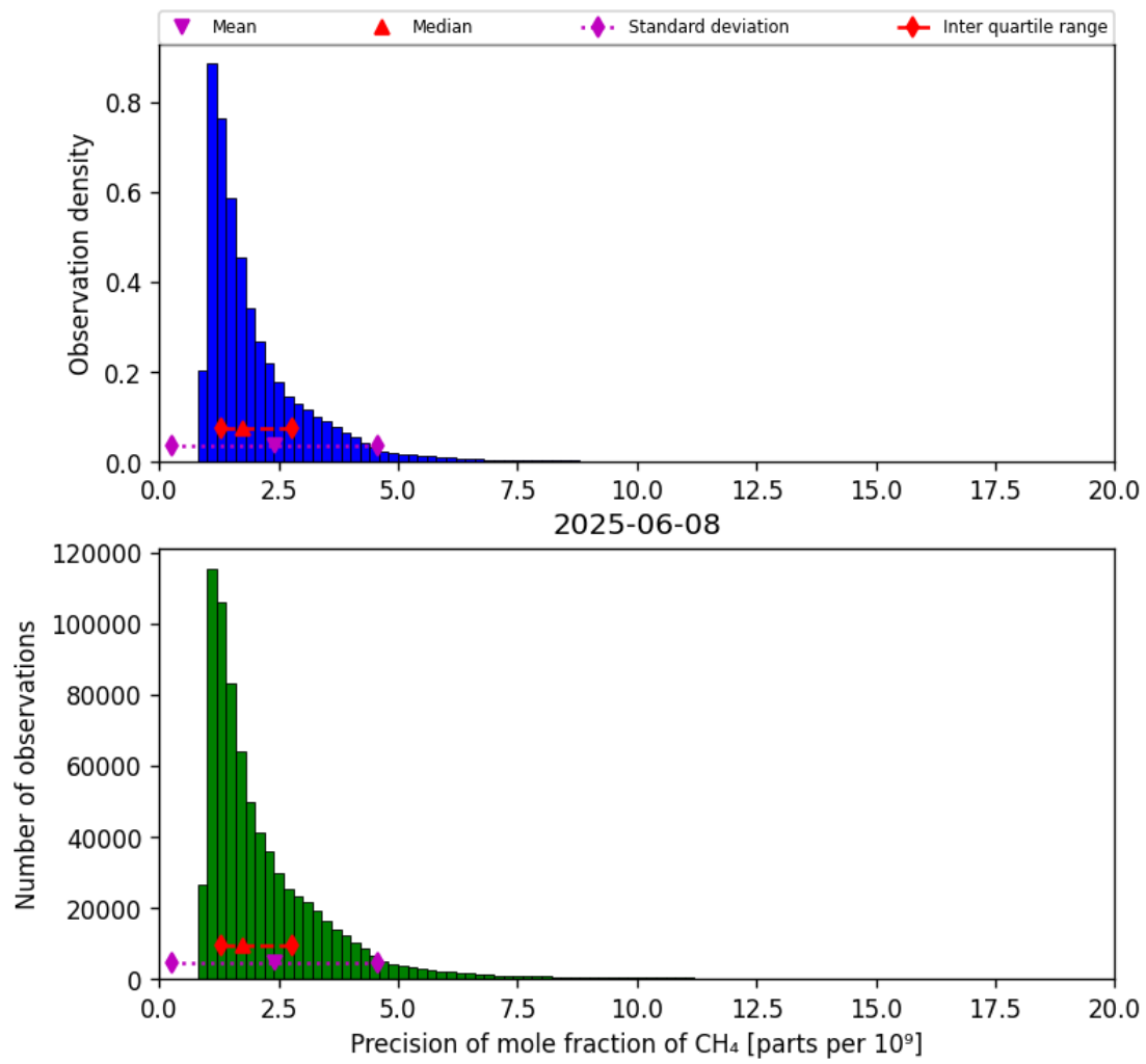
Figure 24: Histogram of “Precision of mole fraction of CH 4 ” for 2025-06-07 to 2025-06-09
