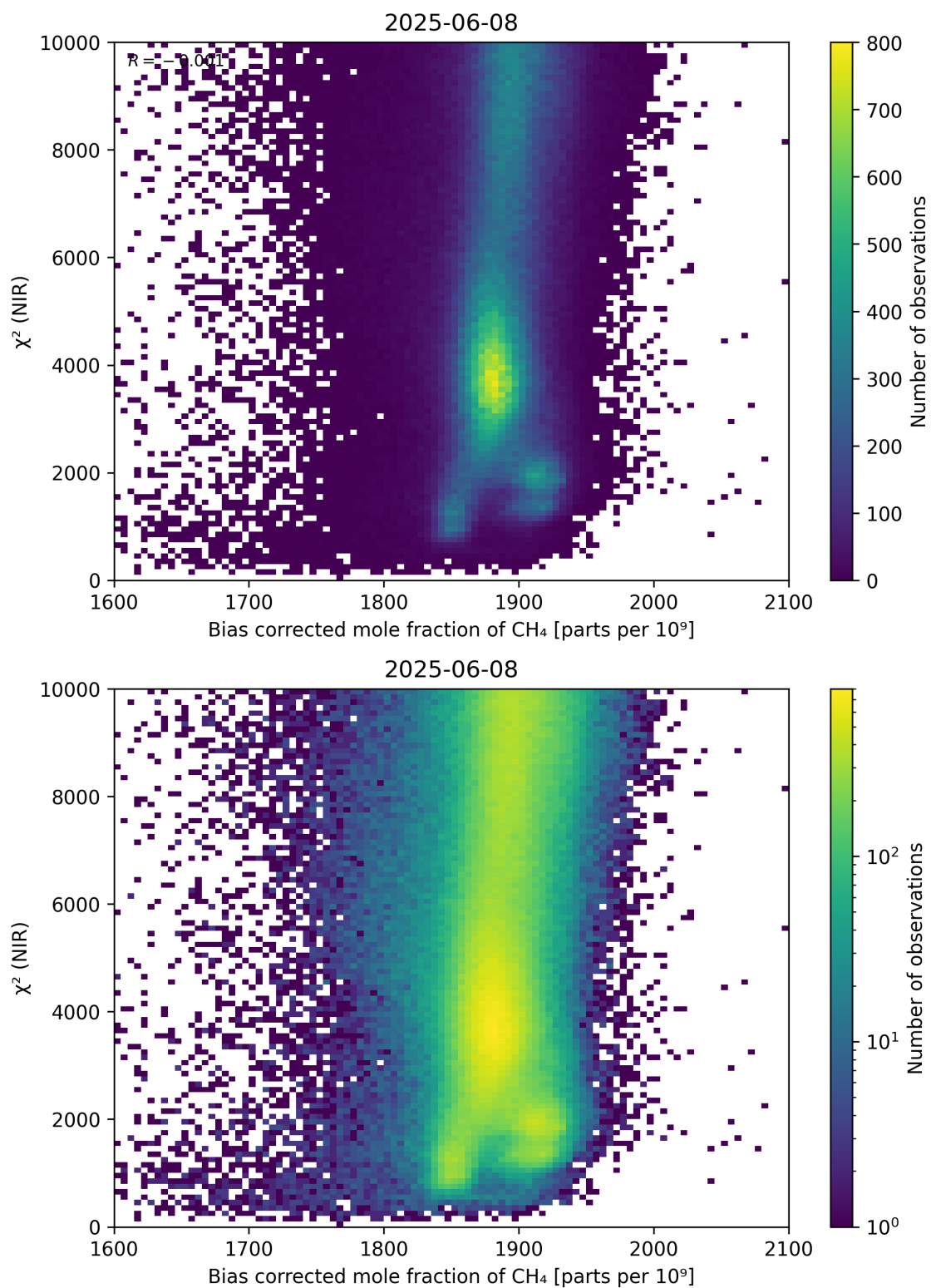
Figure 63: Scatter density plot of “Bias corrected mole fraction of \text{CH}_4 ” against “ \chi^2 (NIR)” for 2025-06-07 to 2025-06-09.
