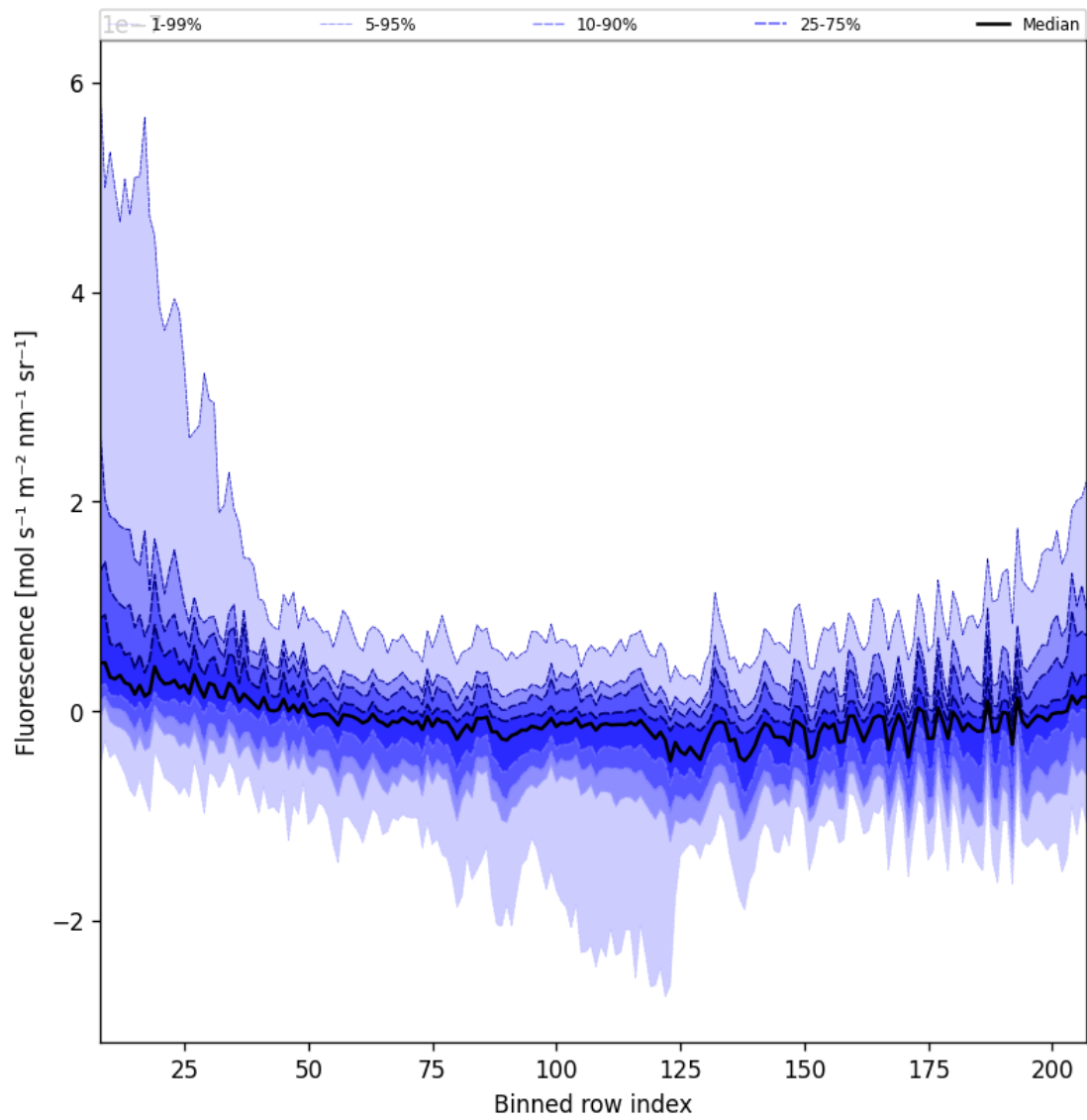
Figure 43: Along track statistics of “Fluorescence” for 2025-06-07 to 2025-06-09
