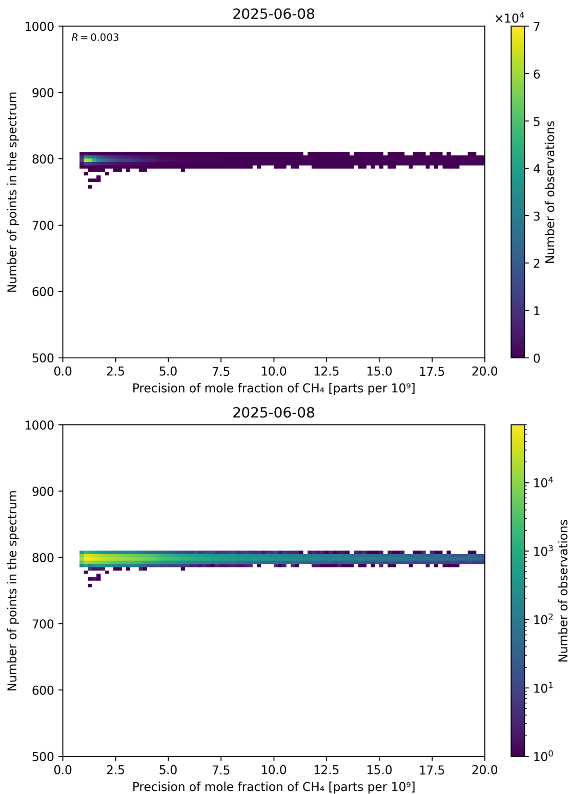
Figure 84: Scatter density plot of “Precision of mole fraction of CH 4 ” against “Number of points in the spectrum” for 2025-06-07 to 2025-06-09.
