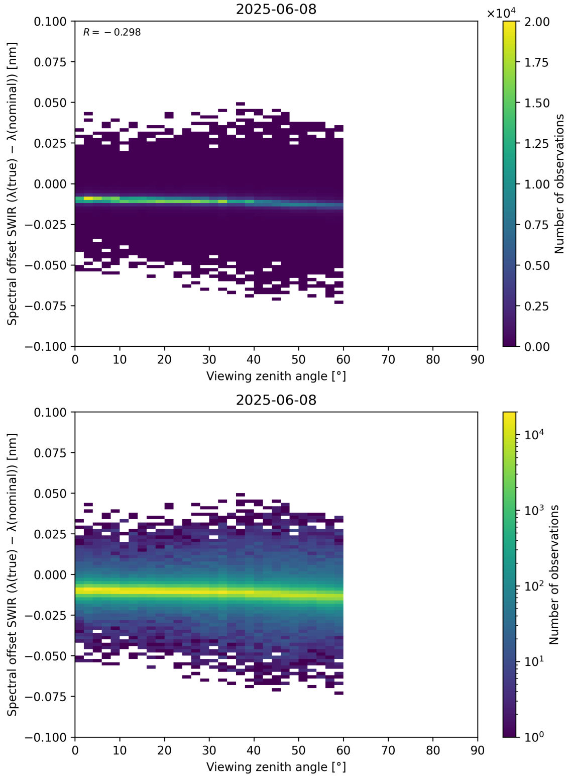
Figure 116: Scatter density plot of “Viewing zenith angle” against “Spectral offset SWIR ( \lambda_{\text{true}} - \lambda_{\text{nominal}} )” for 2025-06-07 to 2025-06-09.
