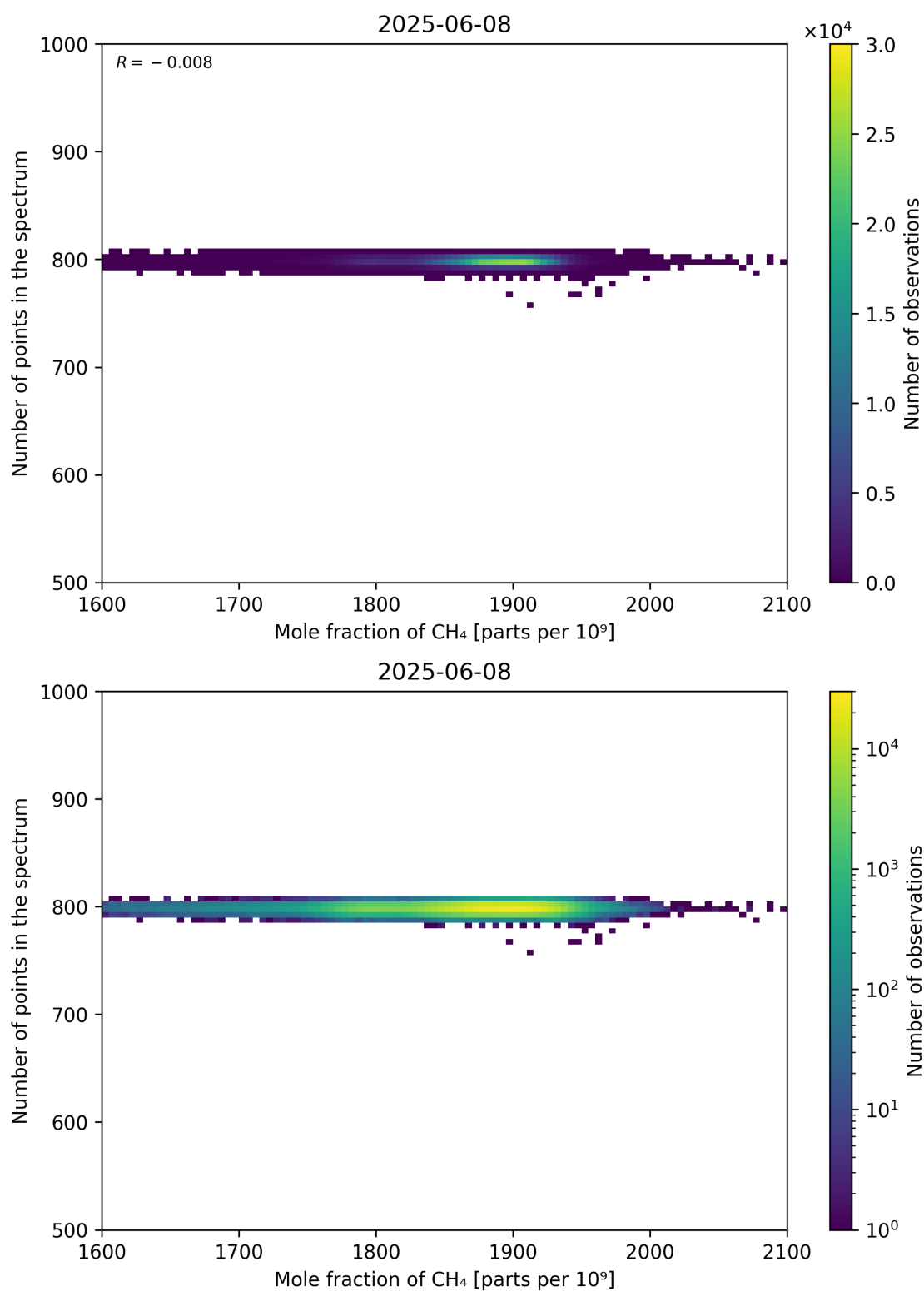
Figure 77: Scatter density plot of “Mole fraction of CH 4 ” against “Number of points in the spectrum” for 2025-06-07 to 2025-06-09.
