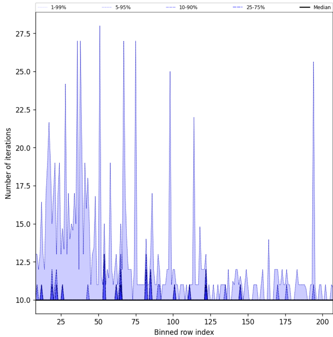
Figure 42: Along track statistics of “Number of iterations” for 2025-06-07 to 2025-06-09
