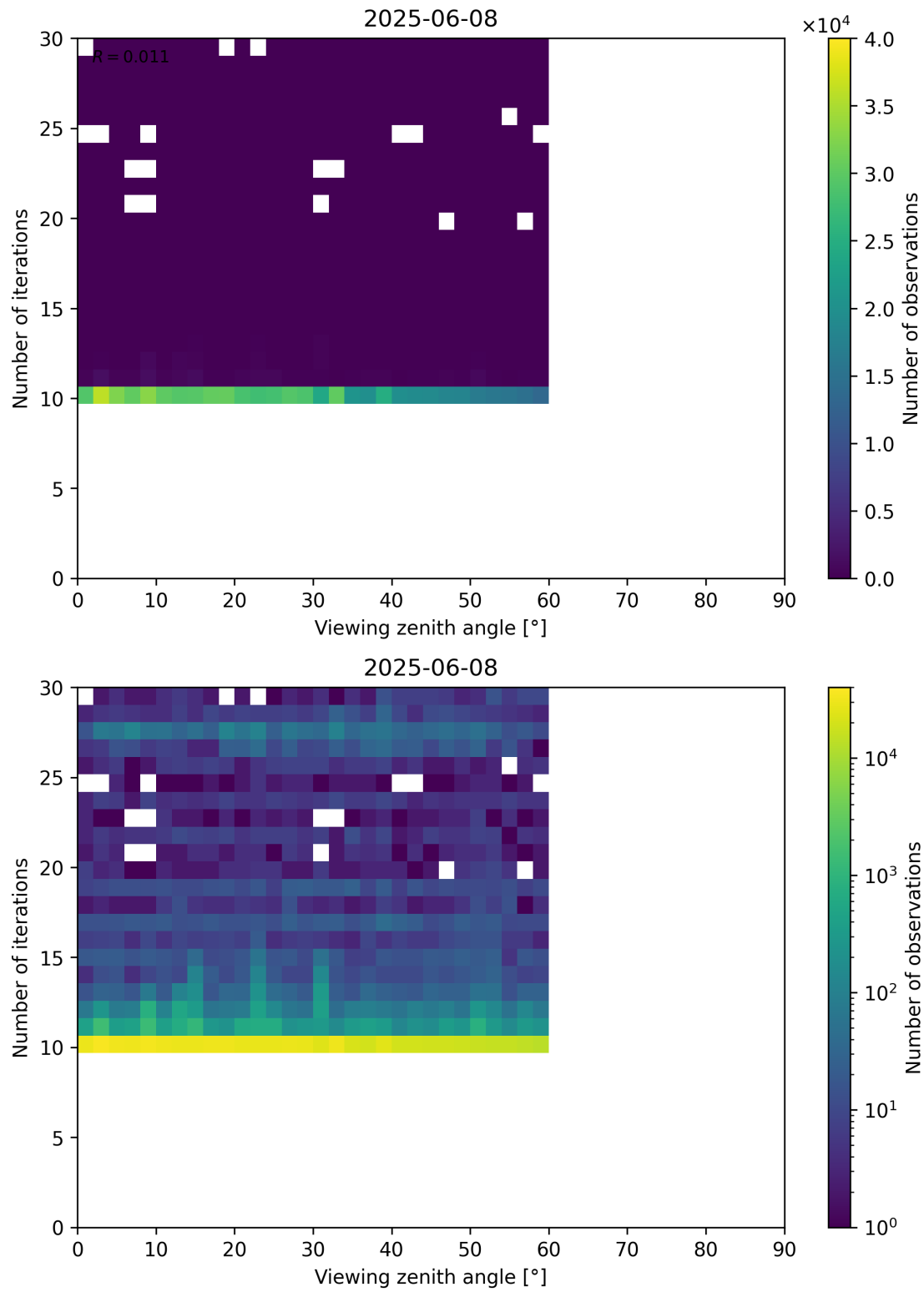
Figure 113: Scatter density plot of “Viewing zenith angle” against “Number of iterations” for 2025-06-07 to 2025-06-09.
