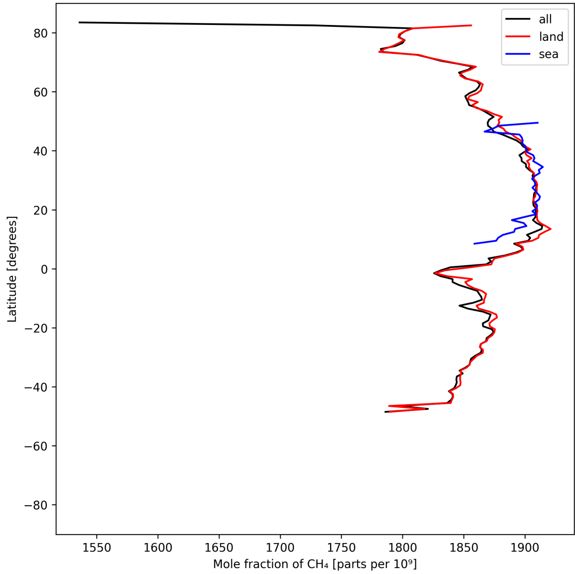
Figure 12: Zonal average of “Mole fraction of \text{CH}_4 ” for 2025-06-07 to 2025-06-09.
