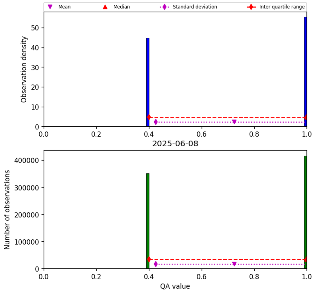
Figure 22: Histogram of “QA value” for 2025-06-07 to 2025-06-09
