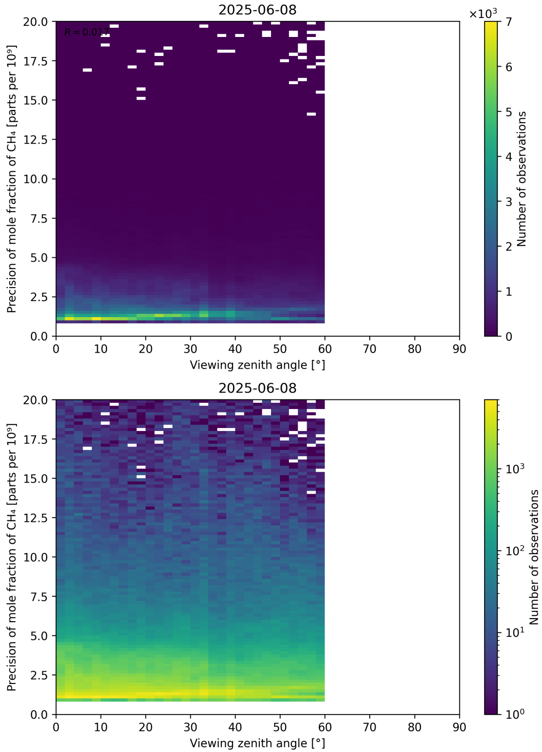
Figure 112: Scatter density plot of “Viewing zenith angle” against “Precision of mole fraction of CH 4 ” for 2025-06-07 to 2025-06-09.
