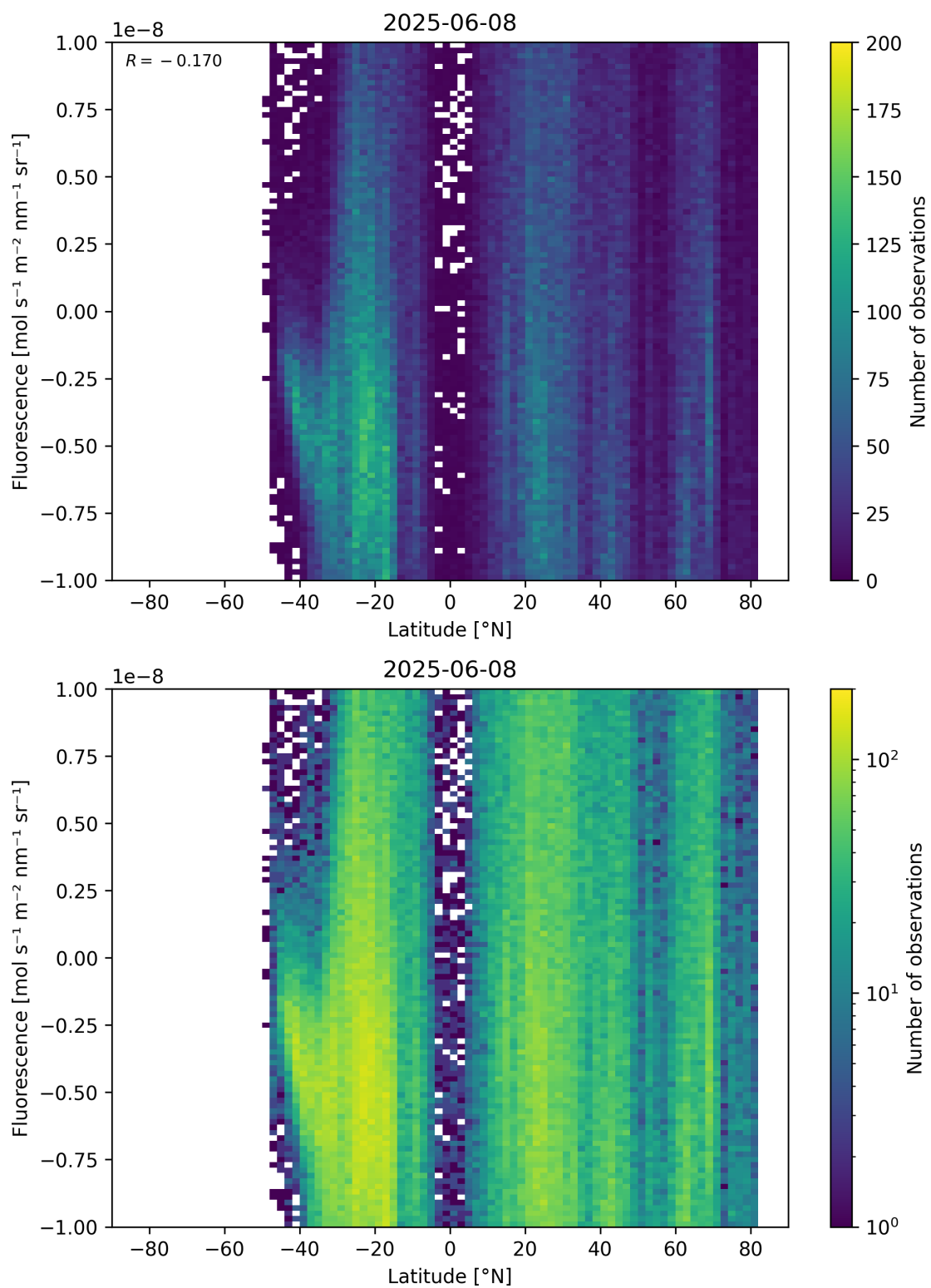
Figure 56: Scatter density plot of “Latitude” against “Fluorescence” for 2025-06-07 to 2025-06-09.
