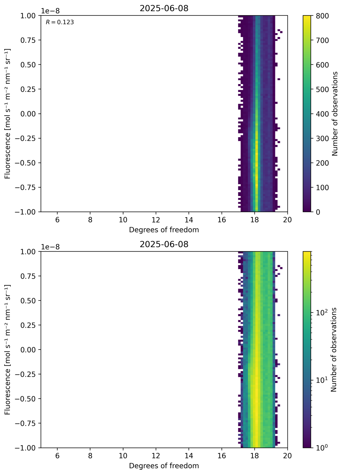
Figure 51: Scatter density plot of “Degrees of freedom” against “Fluorescence” for 2025-06-07 to 2025-06-09.
