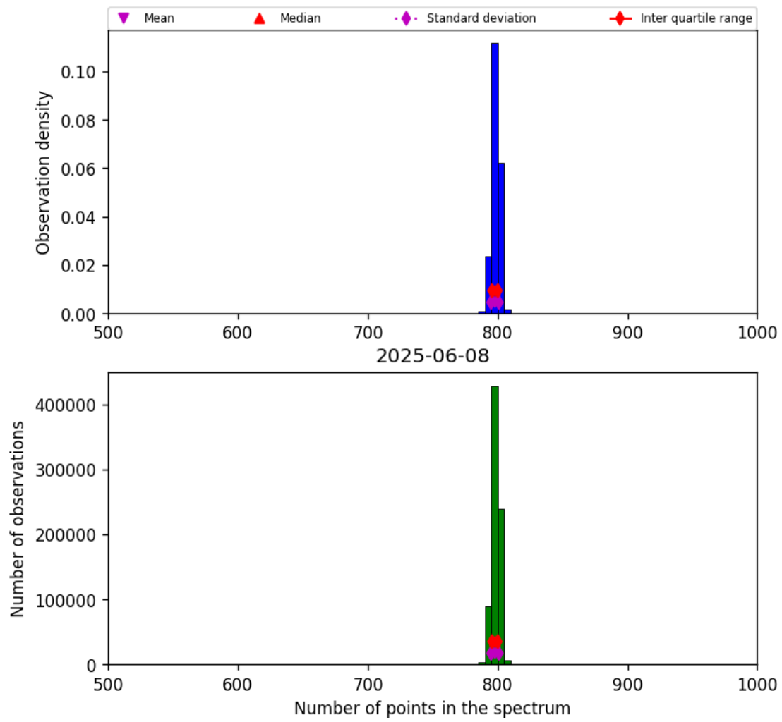
Figure 26: Histogram of “Number of points in the spectrum” for 2025-06-07 to 2025-06-09
