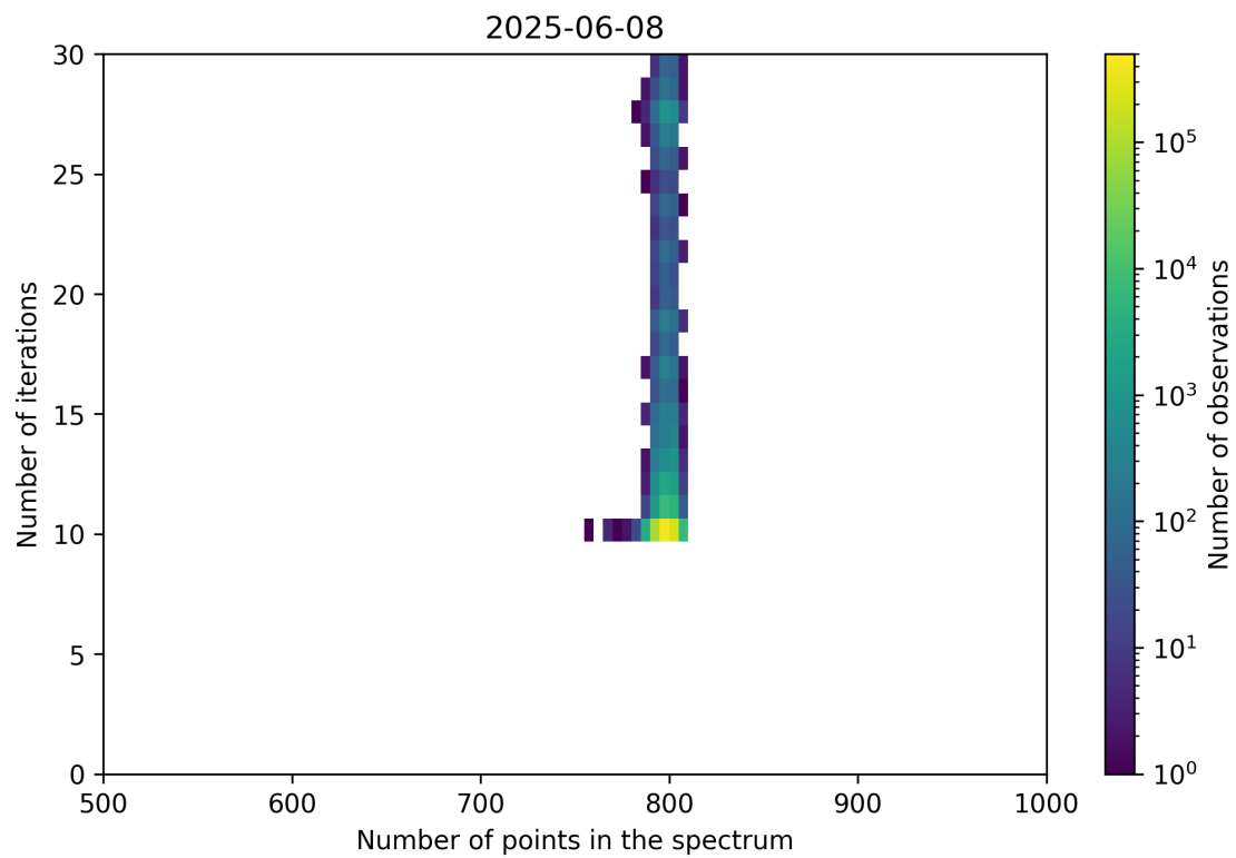
Figure 92: Scatter density plot of “Number of points in the spectrum” against “Number of iterations” for 2025-06-07 to 2025-06-09.
