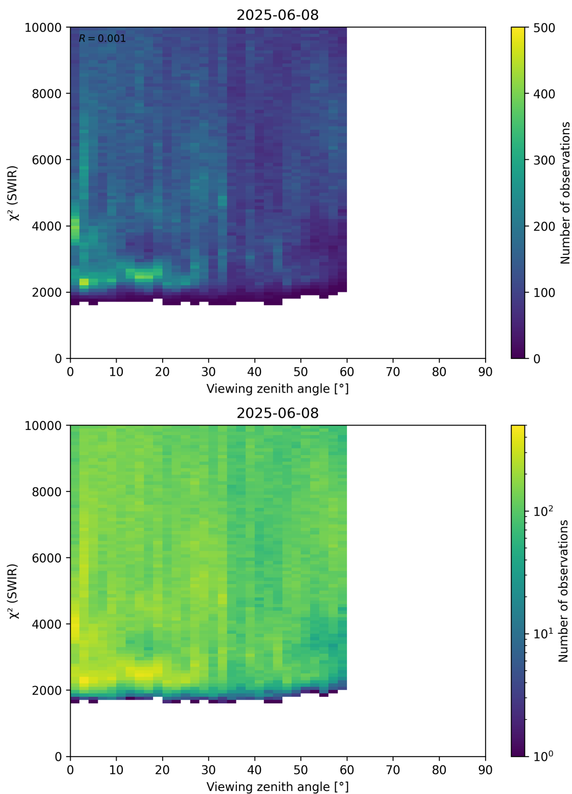
Figure 106: Scatter density plot of “Viewing zenith angle” against “ \chi^2 (SWIR)” for 2025-06-07 to 2025-06-09.
