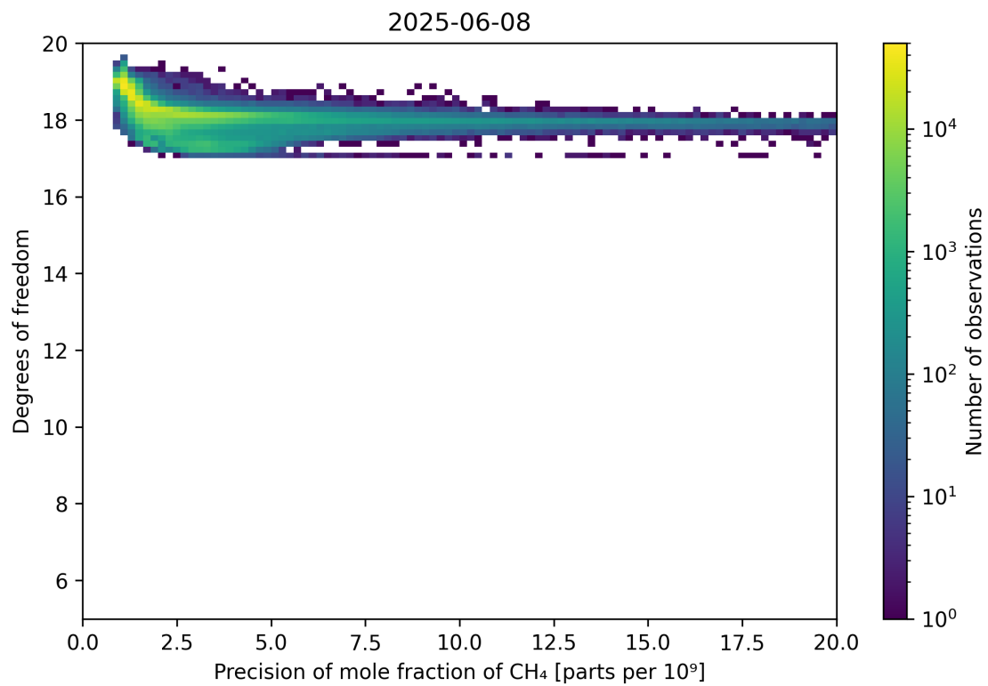
Figure 80: Scatter density plot of “Precision of mole fraction of CH 4 ” against “Degrees of freedom” for 2025-06-07 to 2025-06-09.
