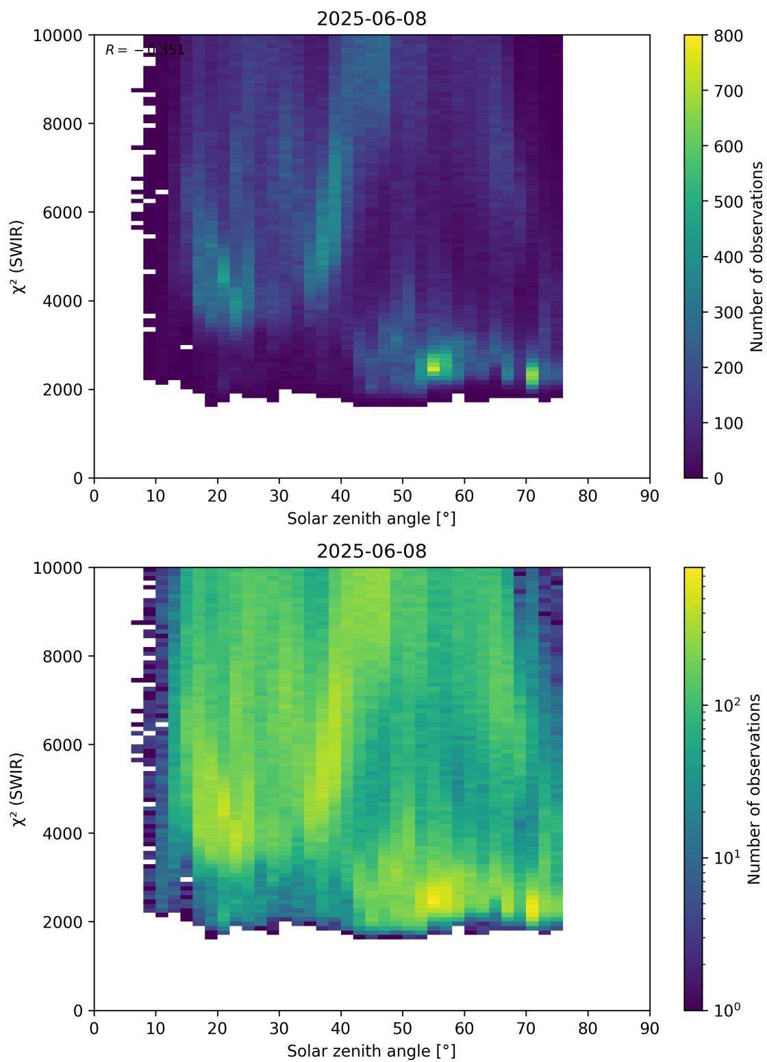
Figure 95: Scatter density plot of “Solar zenith angle” against “ \chi^2 (SWIR)” for 2025-06-07 to 2025-06-09.
