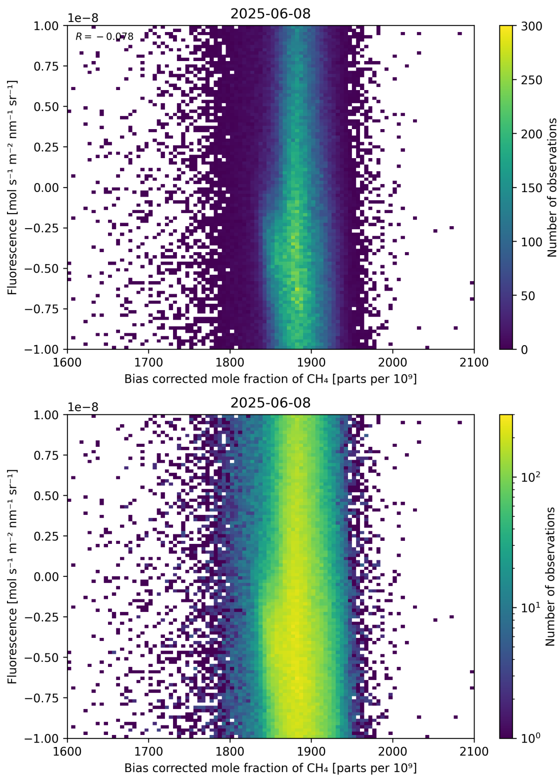
Figure 66: Scatter density plot of “Bias corrected mole fraction of \text{CH}_4 ” against “Fluorescence” for 2025-06-07 to 2025-06-09.
