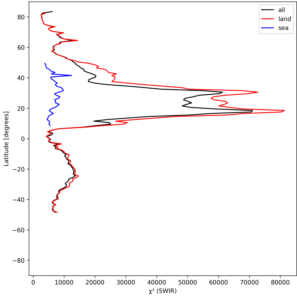
Figure 17: Zonal average of " \chi^2 (SWIR)" for 2025-06-07 to 2025-06-09.
