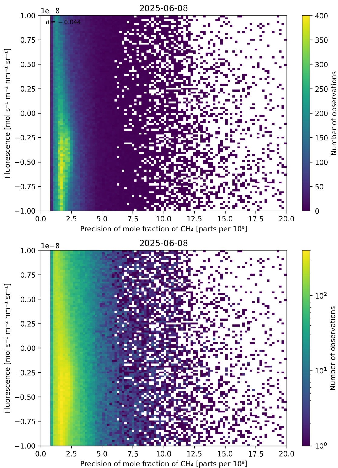
Figure 81: Scatter density plot of “Precision of mole fraction of CH 4 ” against “Fluorescence” for 2025-06-07 to 2025-06-09.
