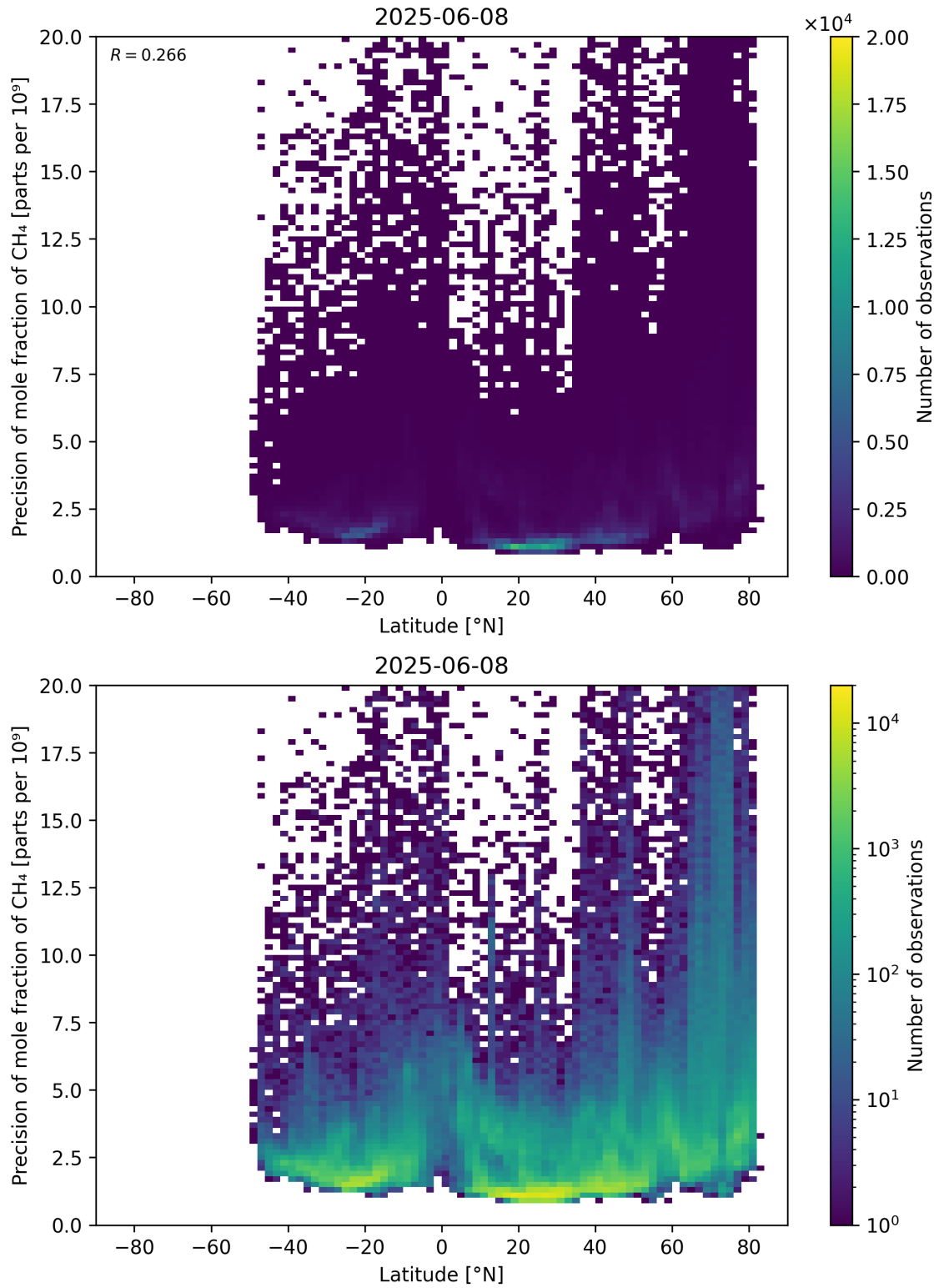
Figure 59: Scatter density plot of “Latitude” against “Precision of mole fraction of \text{CH}_4 ” for 2025-06-07 to 2025-06-09.
