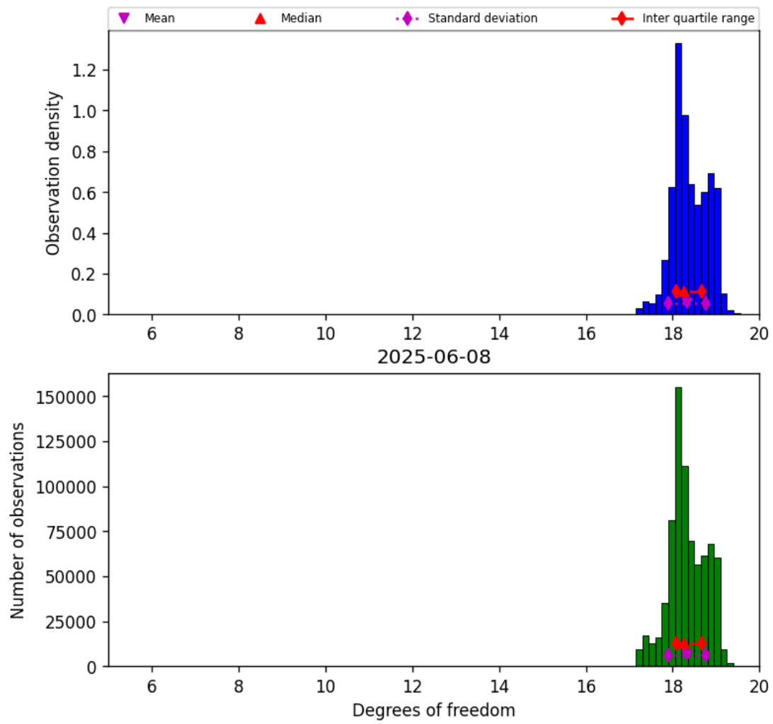
Figure 30: Histogram of “Degrees of freedom” for 2025-06-07 to 2025-06-09
