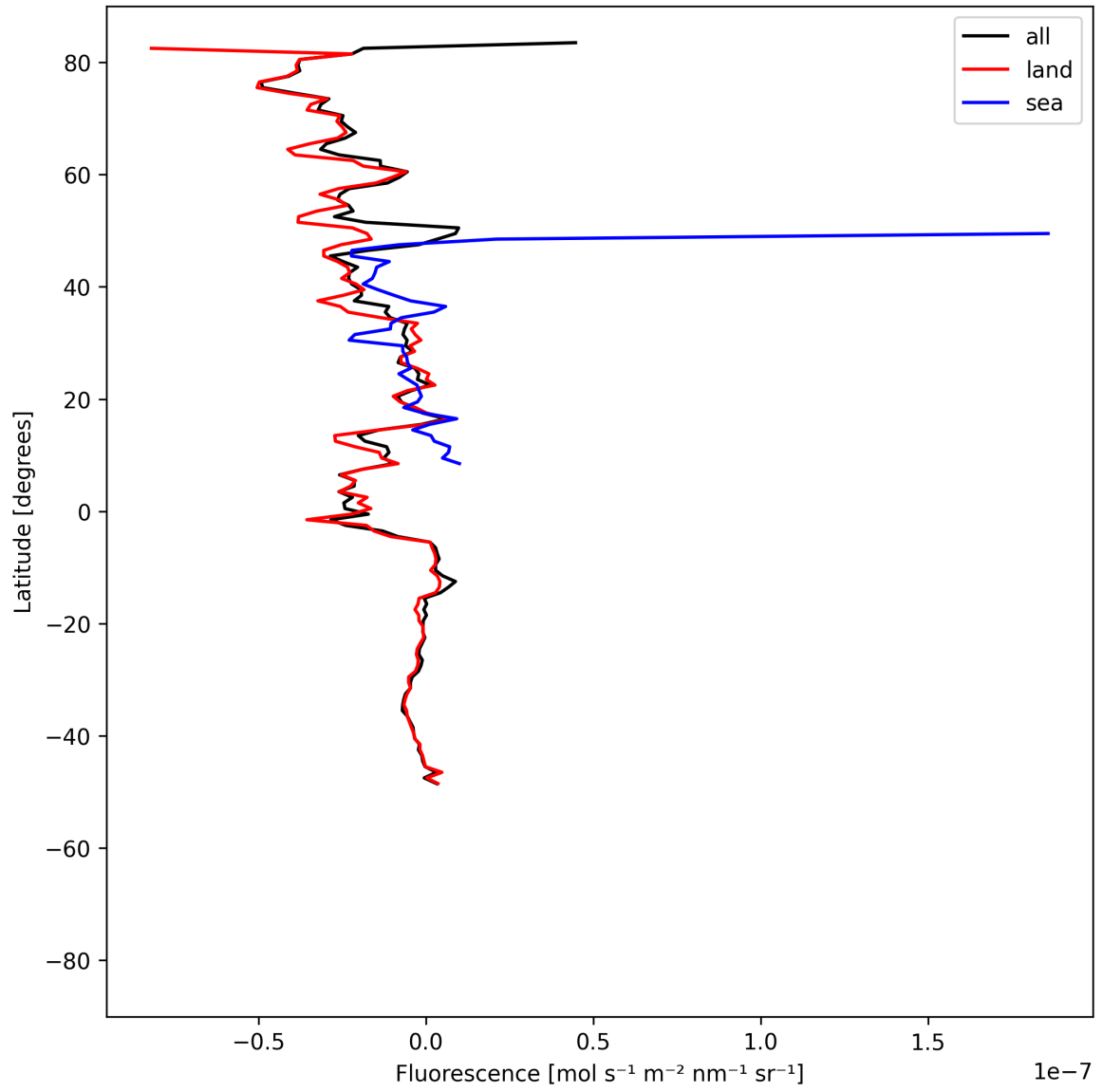
Figure 21: Zonal average of “Fluorescence” for 2025-06-07 to 2025-06-09.
