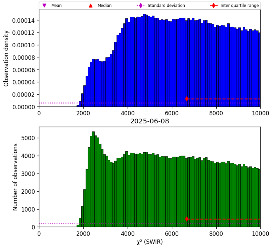
Figure 28: Histogram of “ \chi^2 (SWIR)” for 2025-06-07 to 2025-06-09
