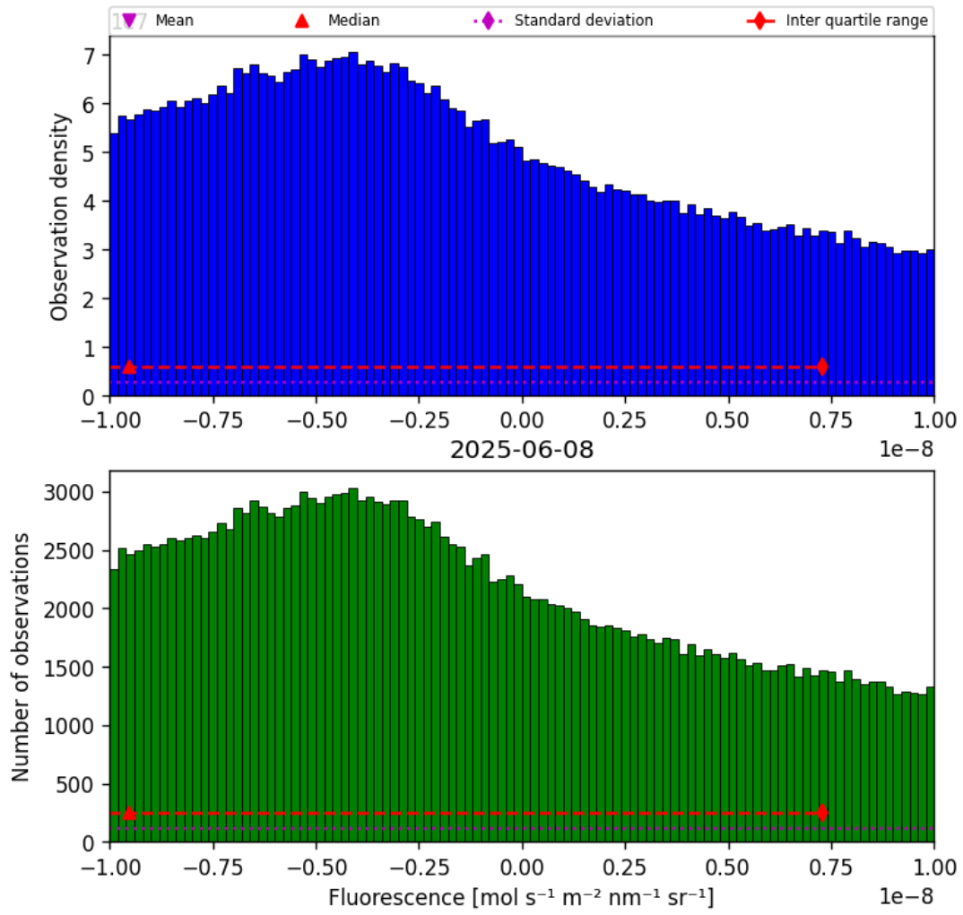
Figure 32: Histogram of “Fluorescence” for 2025-06-07 to 2025-06-09
