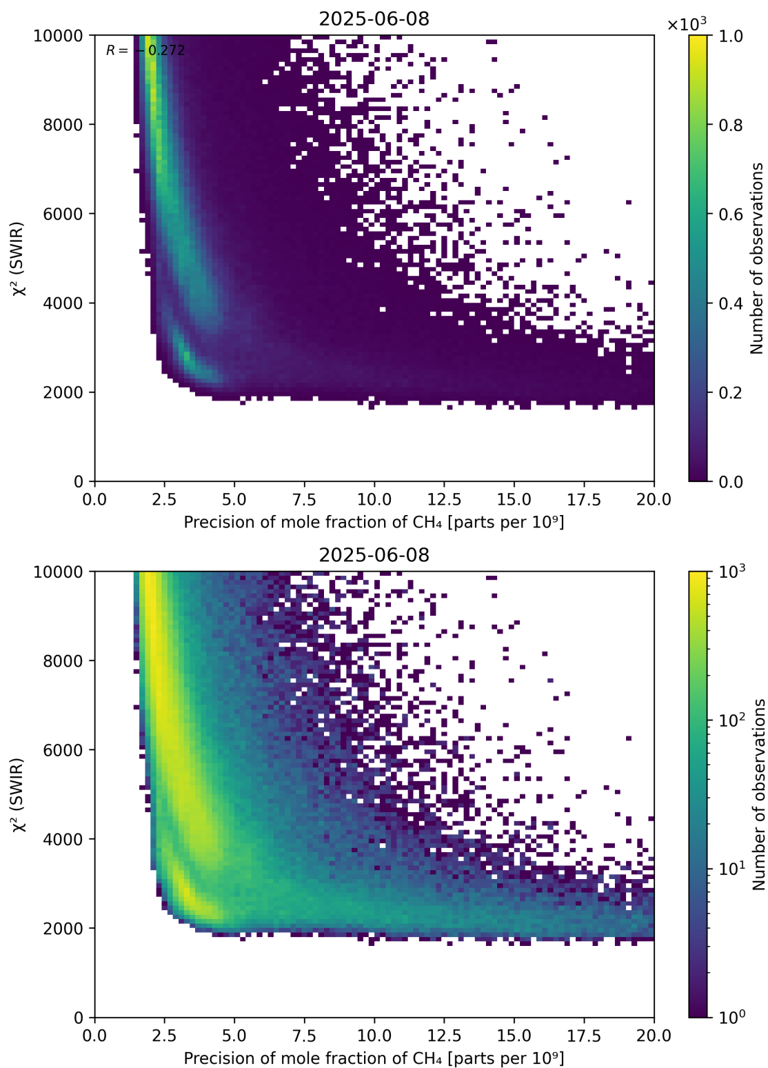
Figure 79: Scatter density plot of “Precision of mole fraction of \text{CH}_4 ” against “ \chi^2 (SWIR)” for 2025-06-07 to 2025-06-09.
