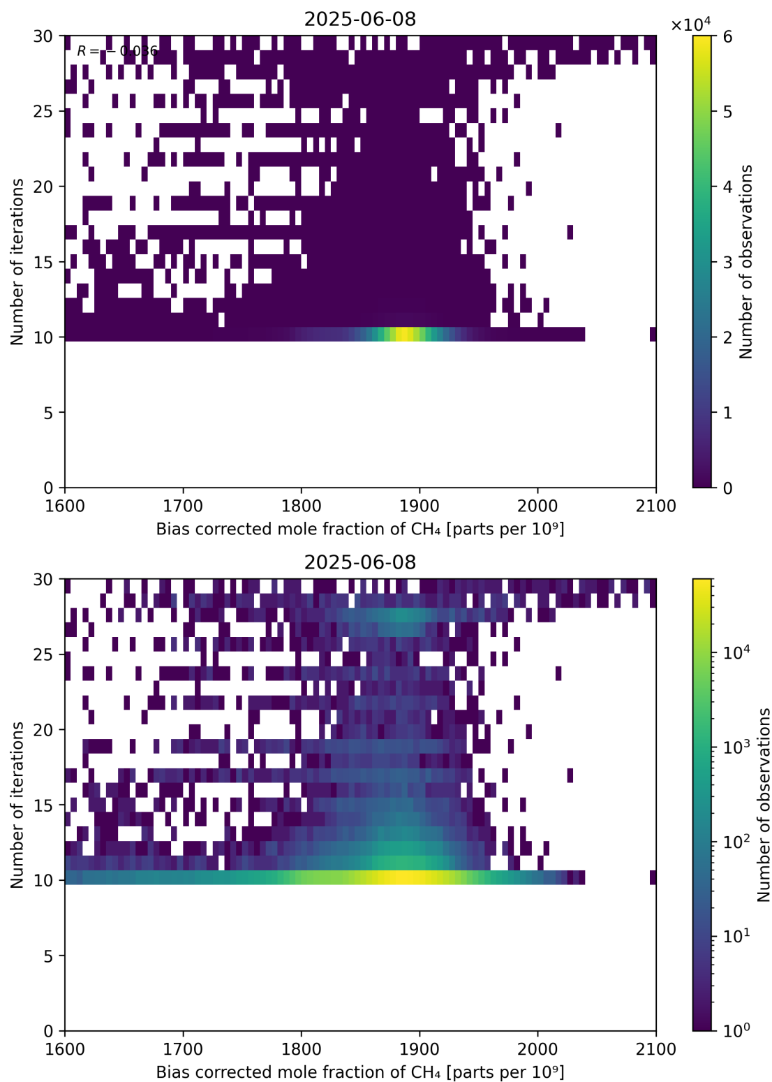
Figure 67: Scatter density plot of “Bias corrected mole fraction of CH 4 ” against “Number of iterations” for 2025-06-07 to 2025-06-09.
