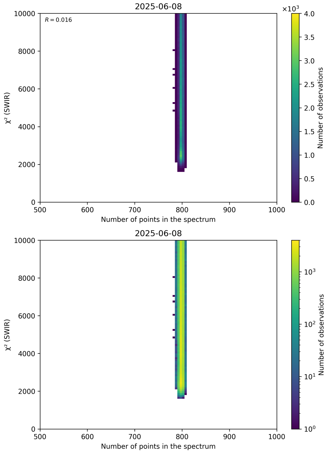
Figure 89: Scatter density plot of “Number of points in the spectrum” against “ \chi^2 (SWIR)” for 2025-06-07 to 2025-06-09.
