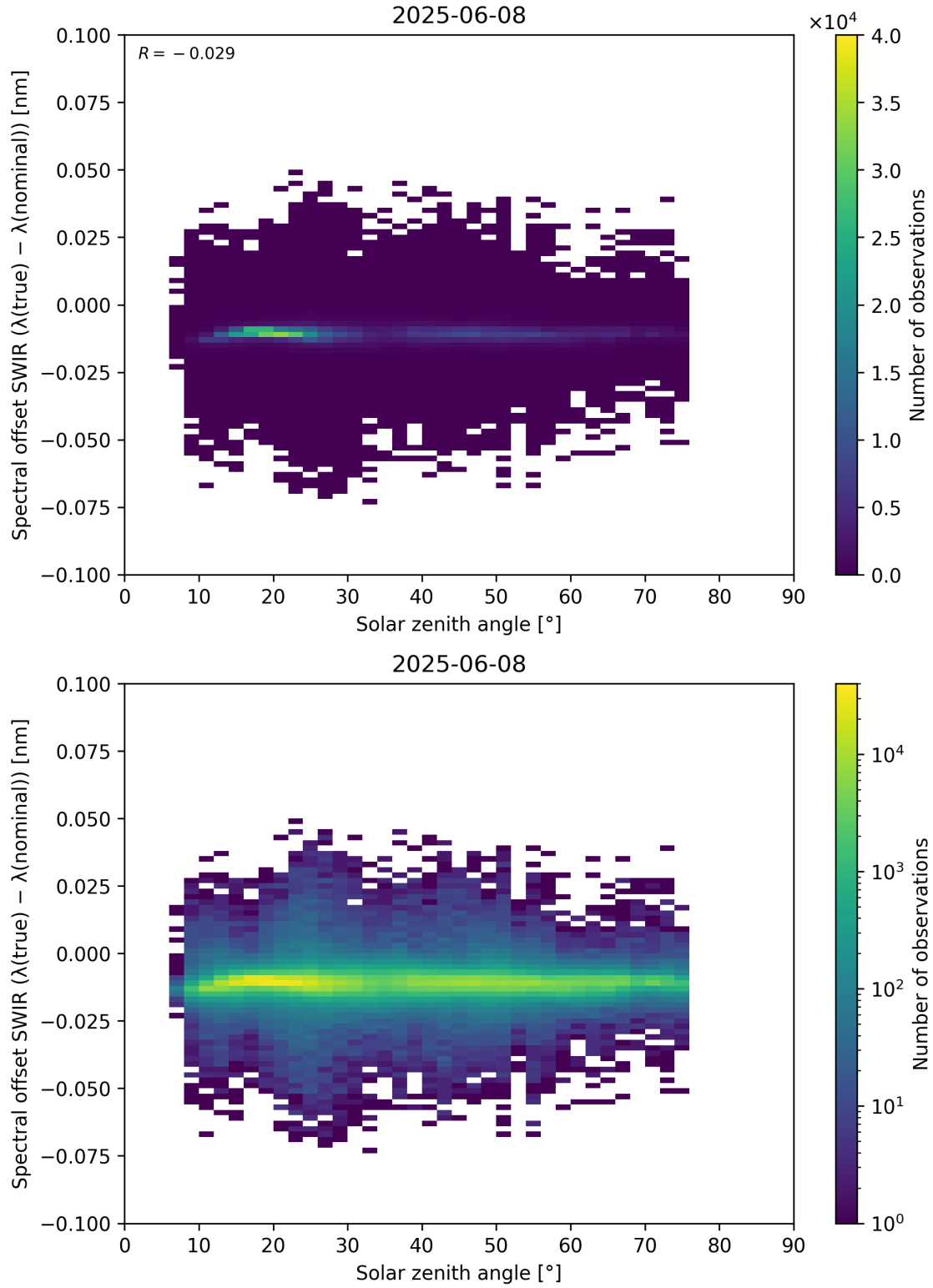
Figure 104: Scatter density plot of “Solar zenith angle” against “Spectral offset SWIR ( \lambda_{\text{true}} - \lambda_{\text{nominal}} )” for 2025-06-07 to 2025-06-09.
