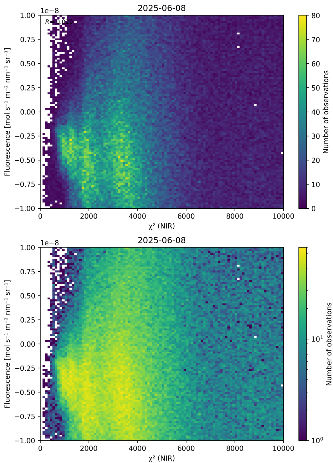
Figure 45: Scatter density plot of “ \chi^2 (NIR)” against “Fluorescence” for 2025-06-07 to 2025-06-09.
