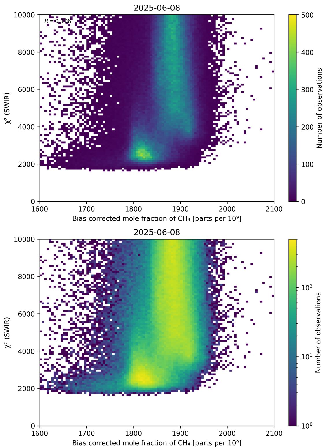
Figure 64: Scatter density plot of “Bias corrected mole fraction of CH 4 ” against “ \chi^2 (SWIR)” for 2025-06-07 to 2025-06-09.
