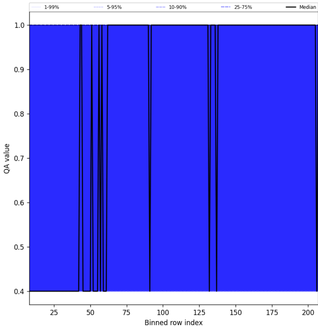
Figure 33: Along track statistics of “QA value” for 2025-06-07 to 2025-06-09
