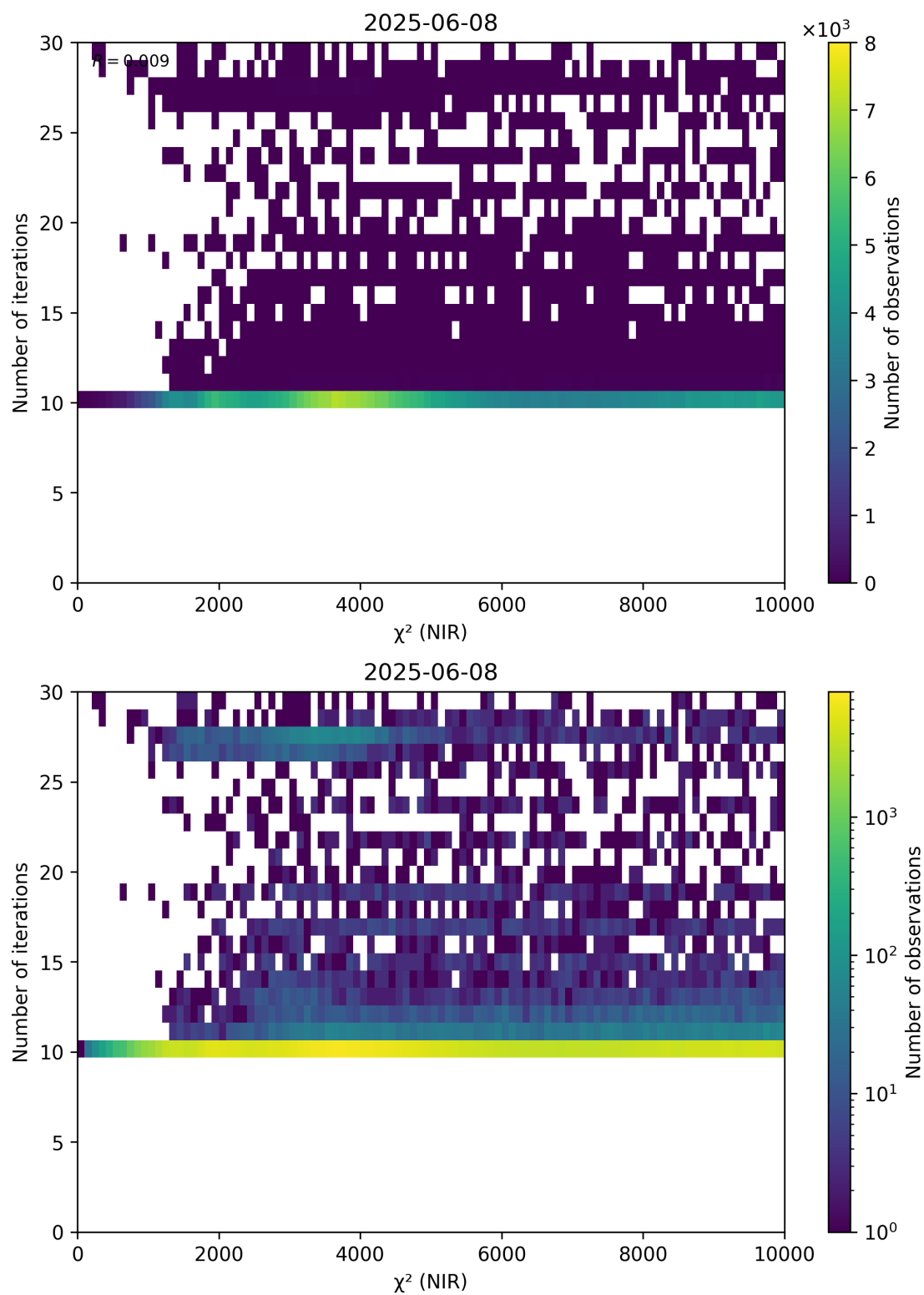
Figure 46: Scatter density plot of “ \chi^2 (NIR)” against “Number of iterations” for 2025-06-07 to 2025-06-09.
