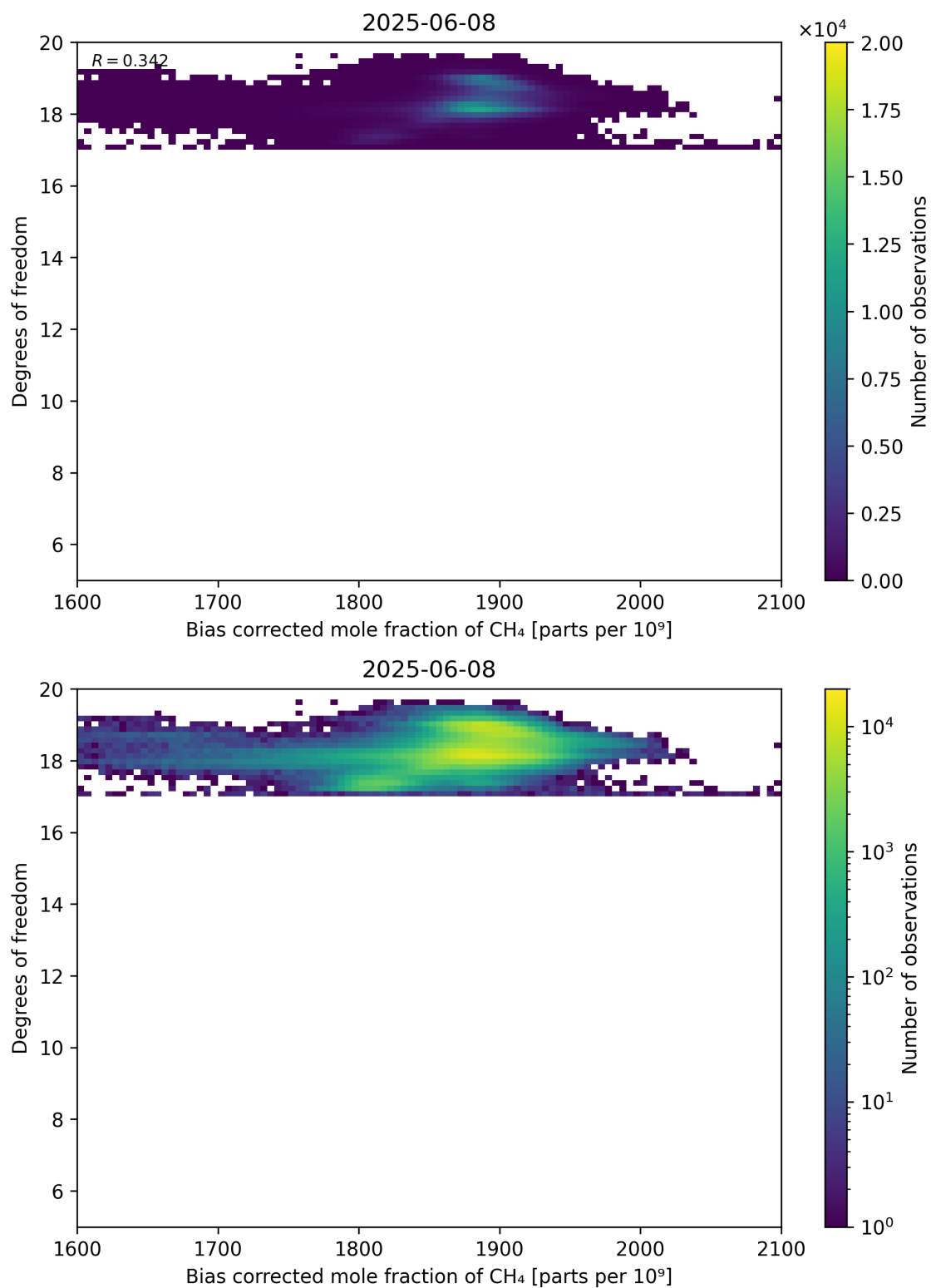
Figure 65: Scatter density plot of “Bias corrected mole fraction of CH 4 ” against “Degrees of freedom” for 2025-06-07 to 2025-06-09.
