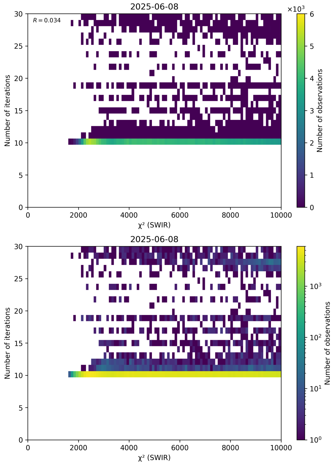
Figure 50: Scatter density plot of “ \chi^2 (SWIR)” against “Number of iterations” for 2025-06-07 to 2025-06-09.
