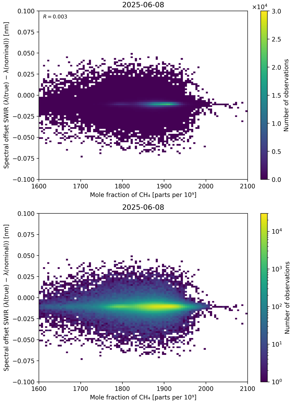
Figure 86: Scatter density plot of “Mole fraction of \text{CH}_4 ” against “Spectral offset SWIR ( \lambda_{\text{true}} - \lambda_{\text{nominal}} )” for 2025-06-07 to 2025-06-09.
