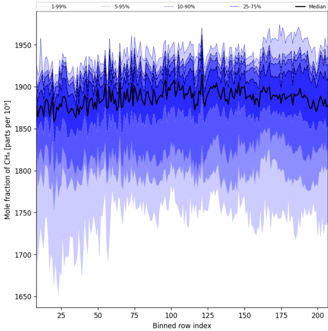
Figure 34: Along track statistics of “Mole fraction of CH 4 ” for 2025-06-07 to 2025-06-09
