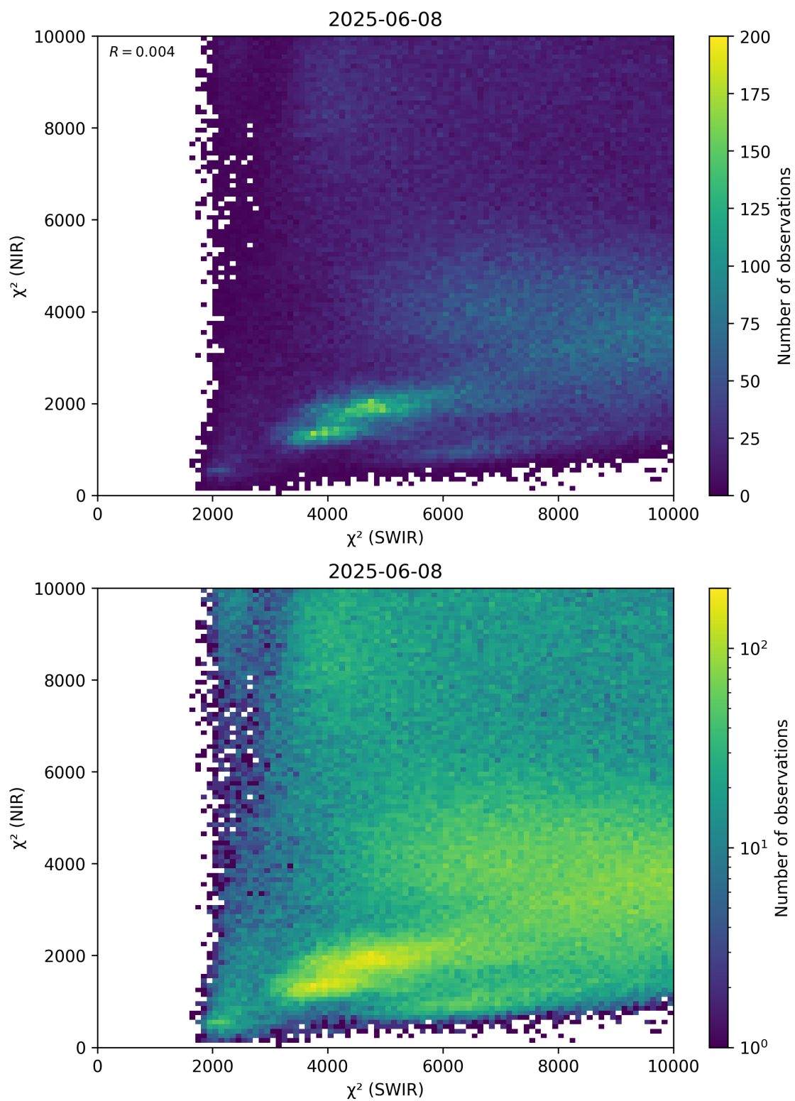
Figure 47: Scatter density plot of “ \chi^2 (SWIR)” against “ \chi^2 (NIR)” for 2025-06-07 to 2025-06-09.
