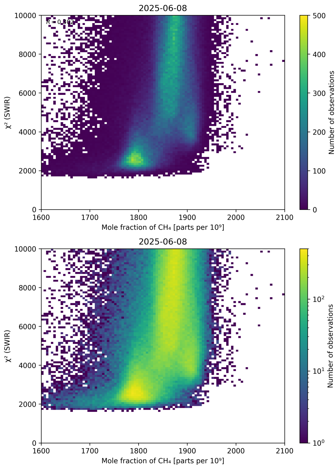
Figure 71: Scatter density plot of “Mole fraction of CH 4 ” against “ \chi^2 (SWIR)” for 2025-06-07 to 2025-06-09.
