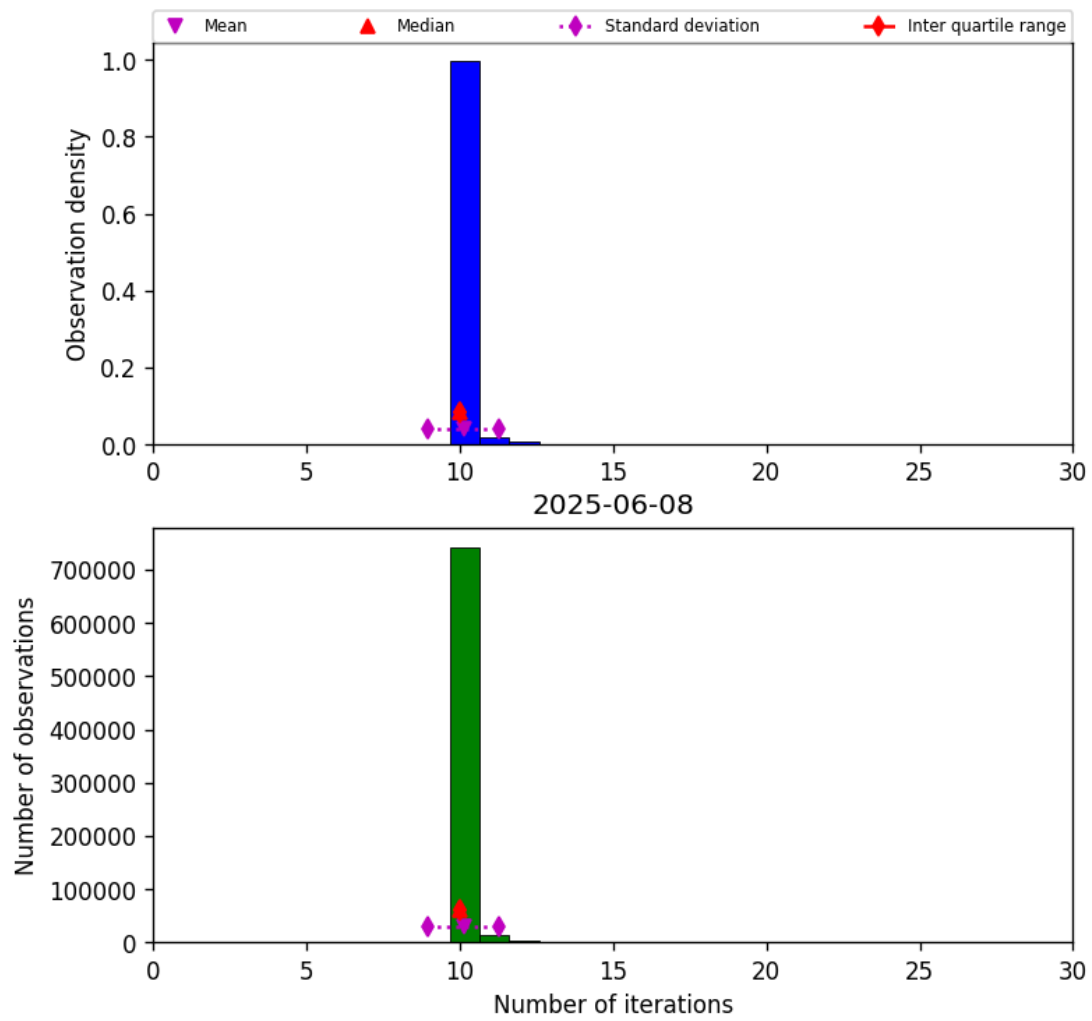
Figure 31: Histogram of “Number of iterations” for 2025-06-07 to 2025-06-09
