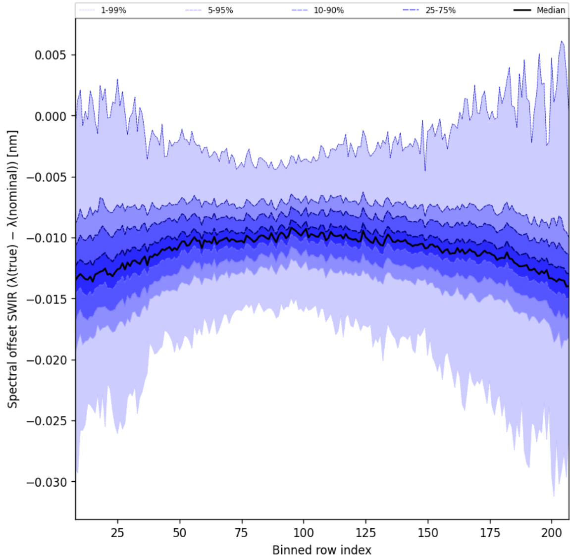
Figure 38: Along track statistics of “Spectral offset SWIR ( \lambda_{\text{true}} - \lambda_{\text{nominal}} )” for 2025-06-07 to 2025-06-09
