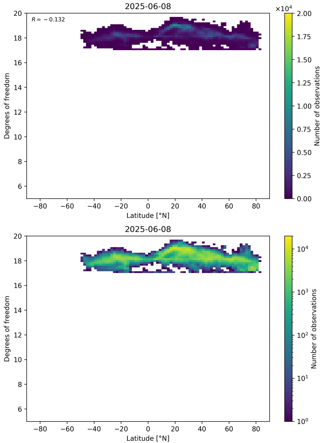
Figure 55: Scatter density plot of “Latitude” against “Degrees of freedom” for 2025-06-07 to 2025-06-09.
