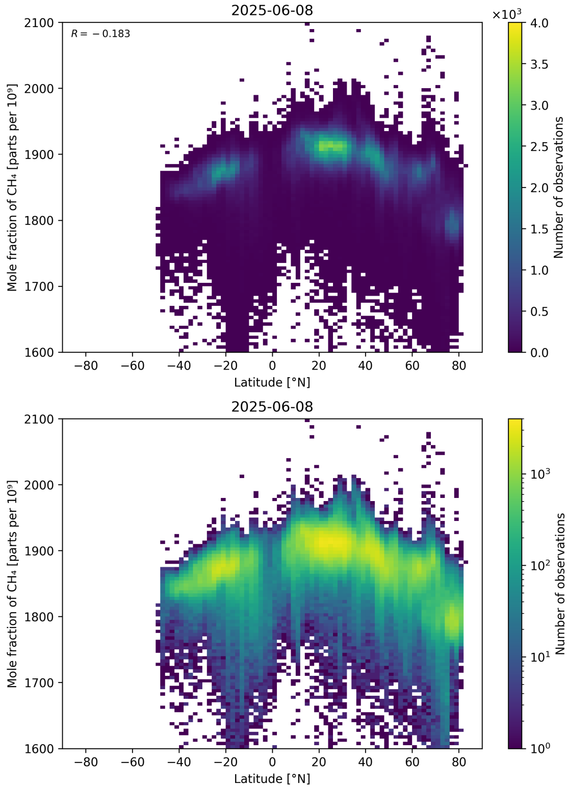
Figure 57: Scatter density plot of “Latitude” against “Mole fraction of CH 4 ” for 2025-06-07 to 2025-06-09.
