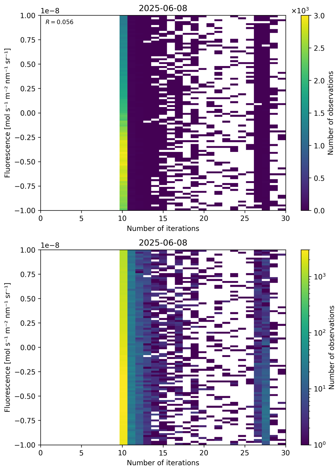
Figure 87: Scatter density plot of “Number of iterations” against “Fluorescence” for 2025-06-07 to 2025-06-09.
