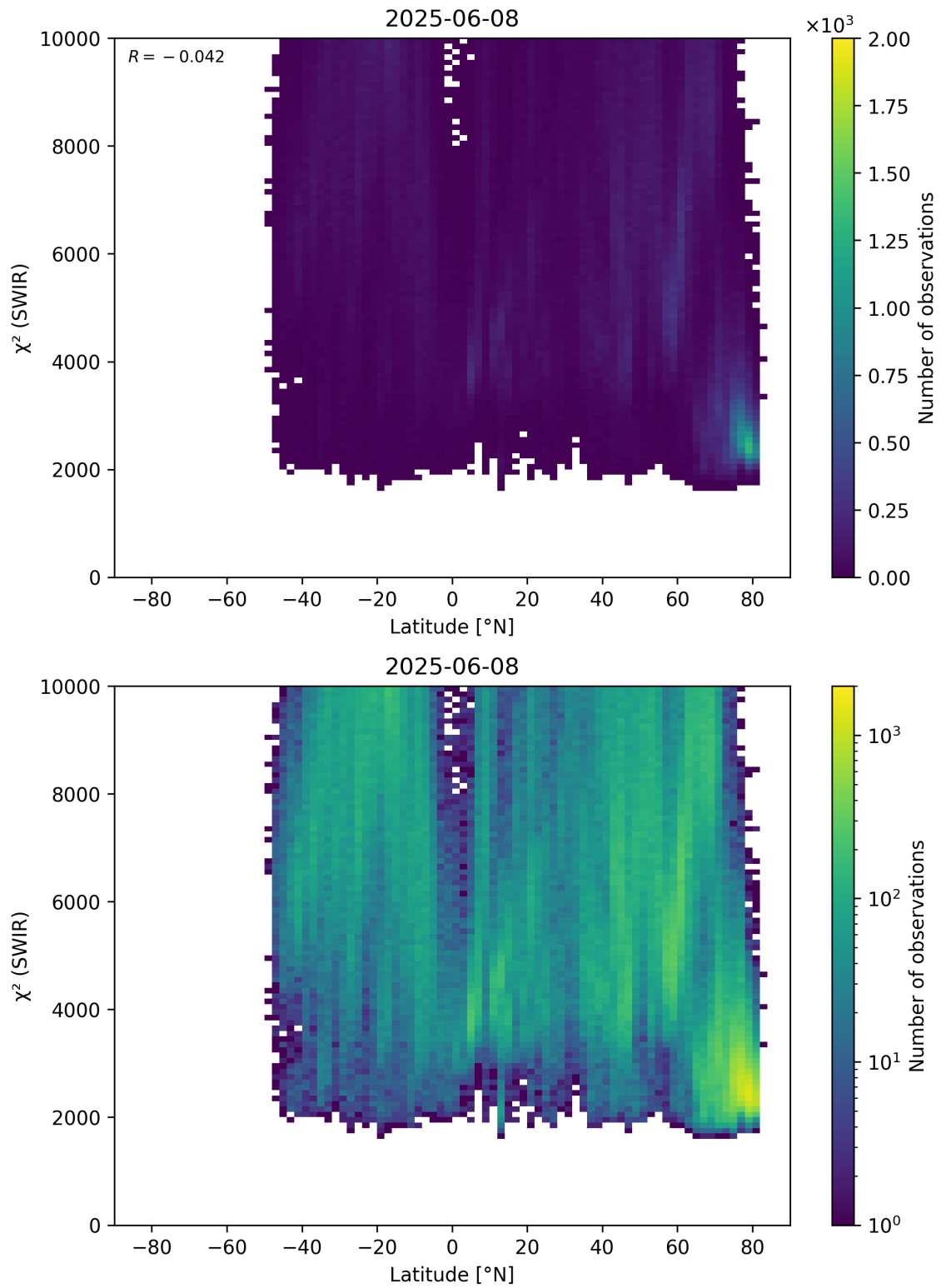
Figure 54: Scatter density plot of “Latitude” against “ \chi^2 (SWIR)” for 2025-06-07 to 2025-06-09.
