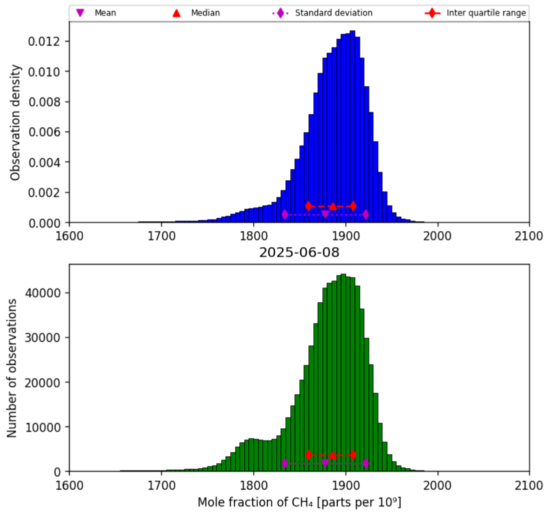
Figure 23: Histogram of “Mole fraction of CH 4 ” for 2025-06-07 to 2025-06-09
