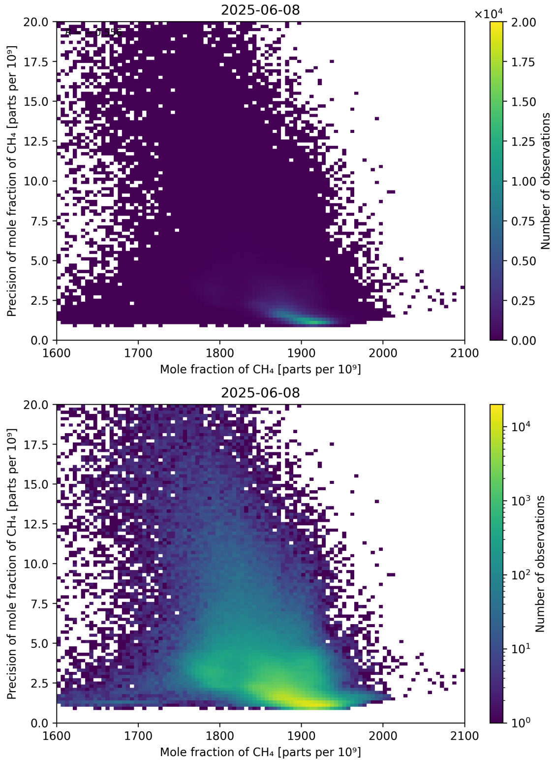
Figure 75: Scatter density plot of “Mole fraction of CH 4 ” against “Precision of mole fraction of CH 4 ” for 2025-06-07 to 2025-06-09.
