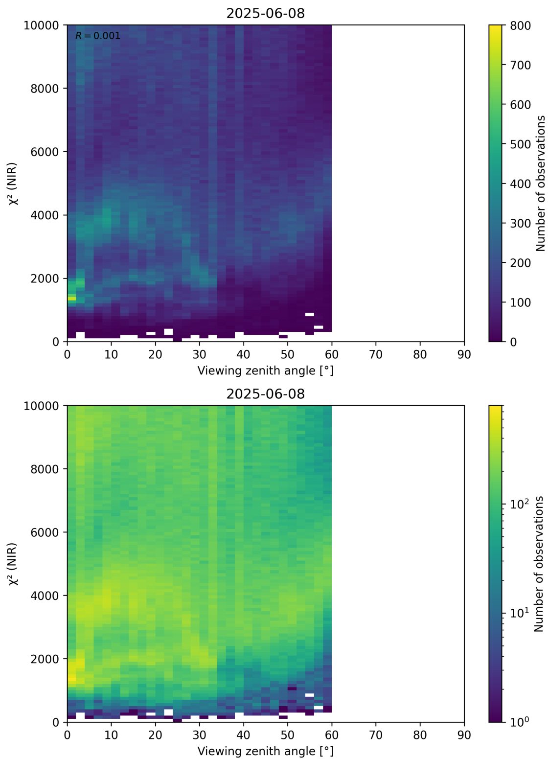
Figure 105: Scatter density plot of “Viewing zenith angle” against “ \chi^2 (NIR)” for 2025-06-07 to 2025-06-09.
