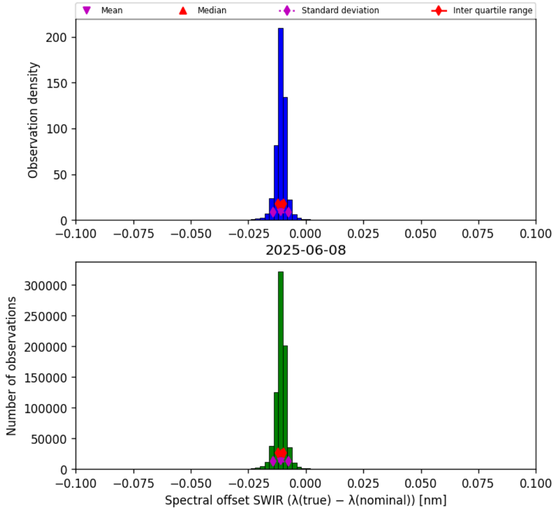
Figure 27: Histogram of “Spectral offset SWIR ( \lambda_{\text{true}} - \lambda_{\text{nominal}} )” for 2025-06-07 to 2025-06-09
