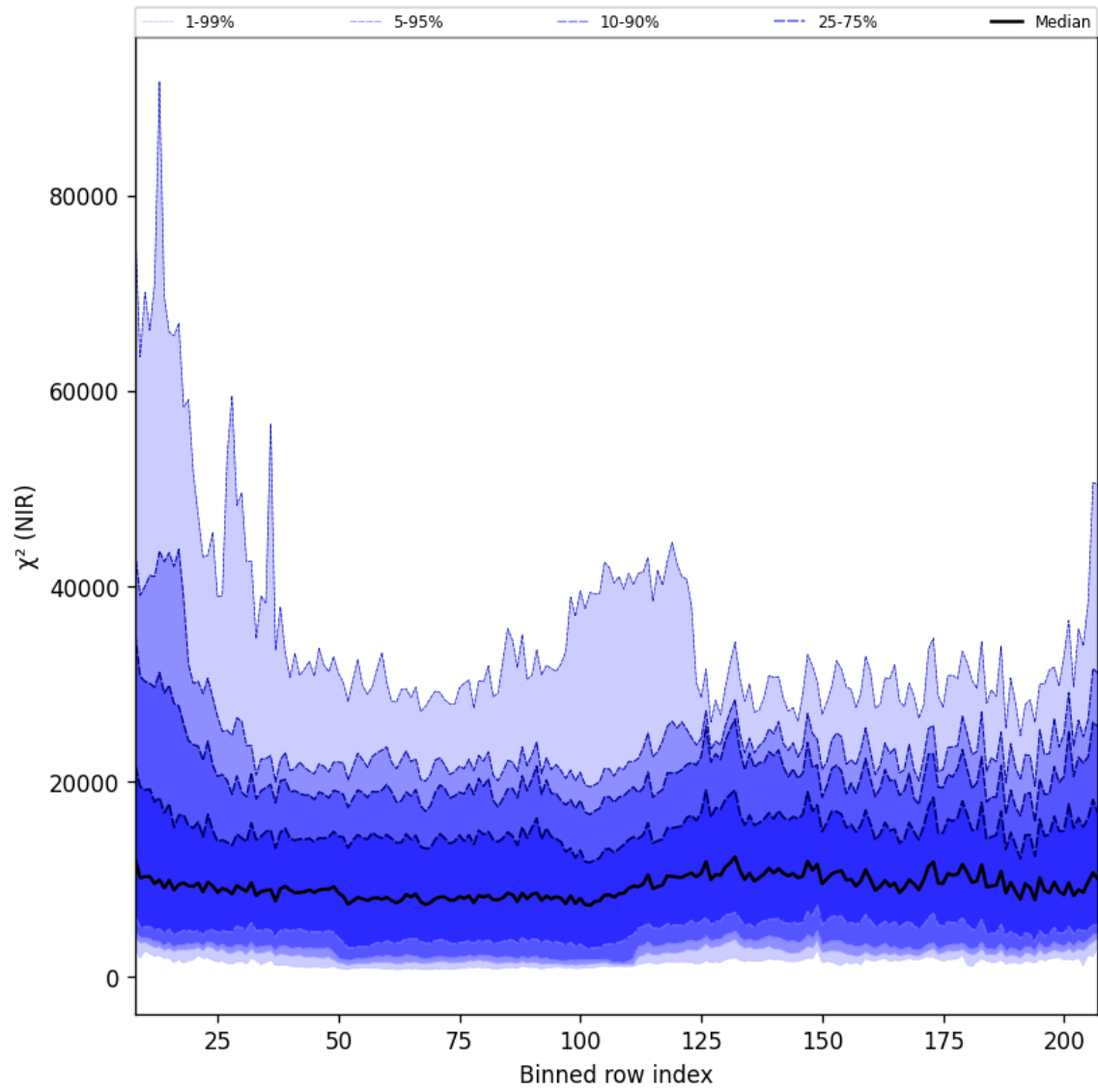
Figure 40: Along track statistics of “ \chi^2 (NIR)” for 2025-06-07 to 2025-06-09
