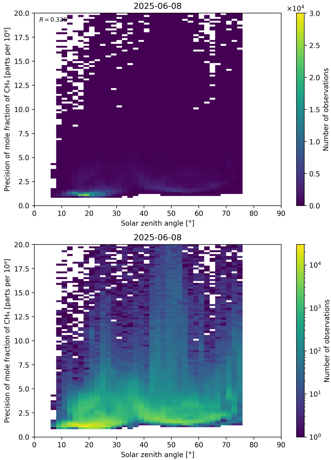
Figure 101: Scatter density plot of “Solar zenith angle” against “Precision of mole fraction of CH 4 ” for 2025-06-07 to 2025-06-09.
