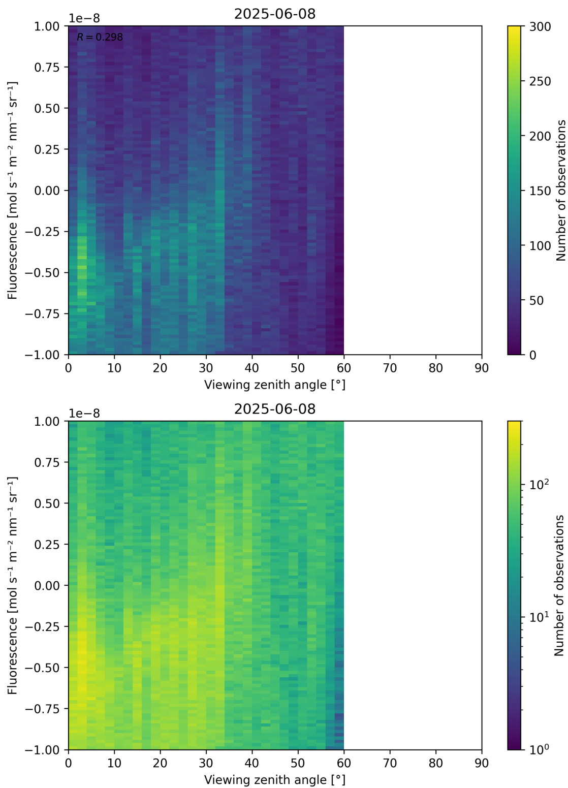
Figure 108: Scatter density plot of “Viewing zenith angle” against “Fluorescence” for 2025-06-07 to 2025-06-09.
