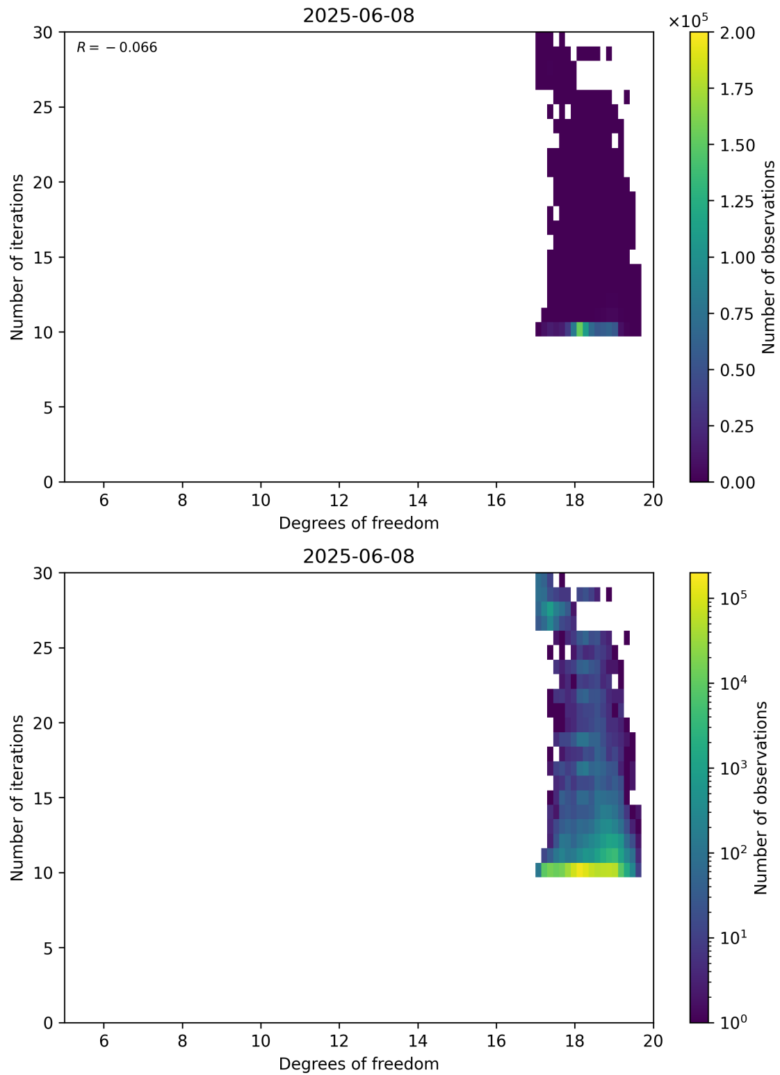
Figure 52: Scatter density plot of “Degrees of freedom” against “Number of iterations” for 2025-06-07 to 2025-06-09.
