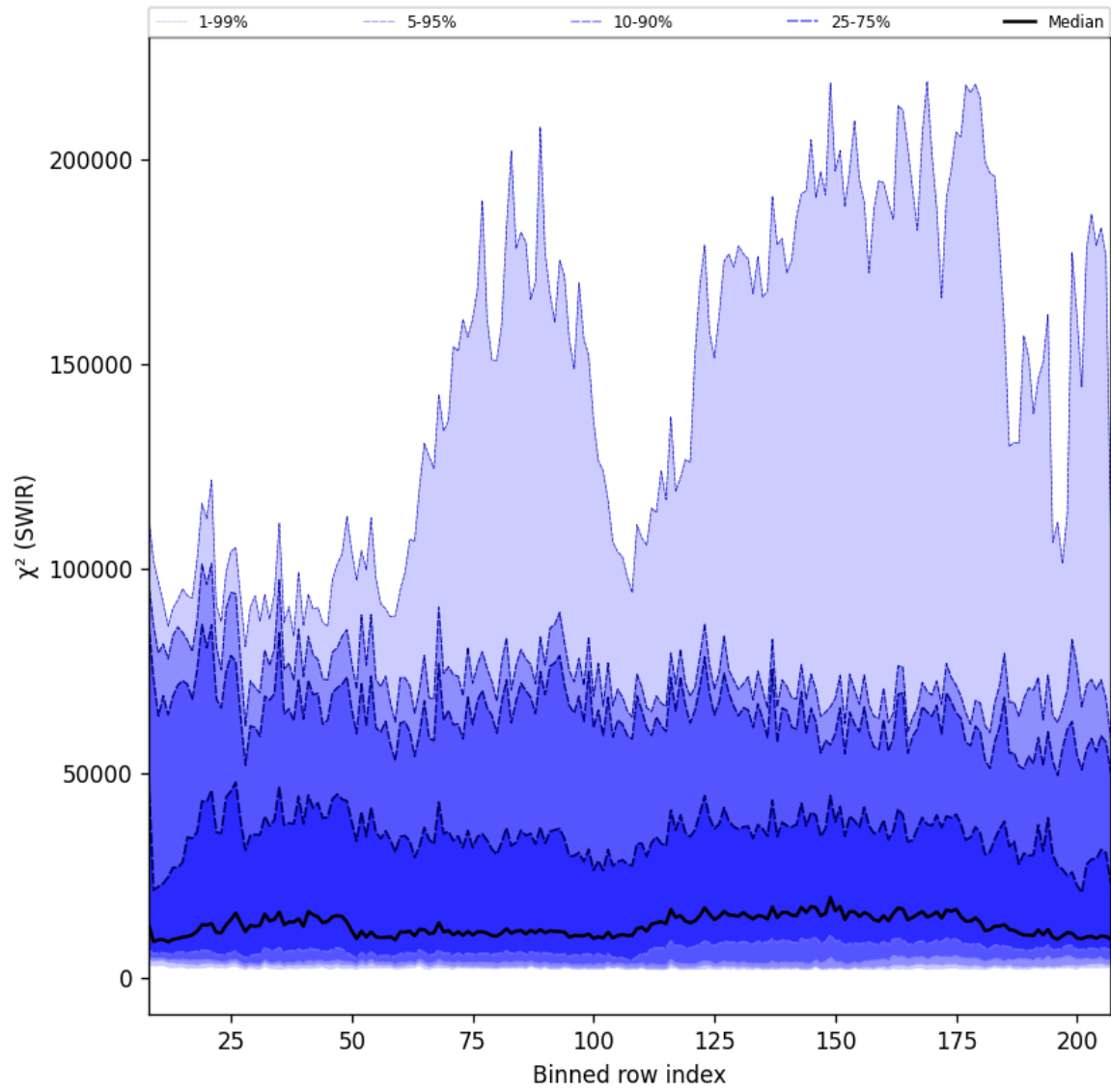
Figure 39: Along track statistics of “ \chi^2 (SWIR)” for 2025-06-07 to 2025-06-09
