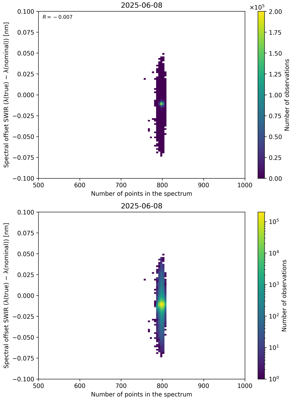
Figure 93: Scatter density plot of “Number of points in the spectrum” against “Spectral offset SWIR ( \lambda_{\text{true}} - \lambda_{\text{nominal}} )” for 2025-06-07 to 2025-06-09.
