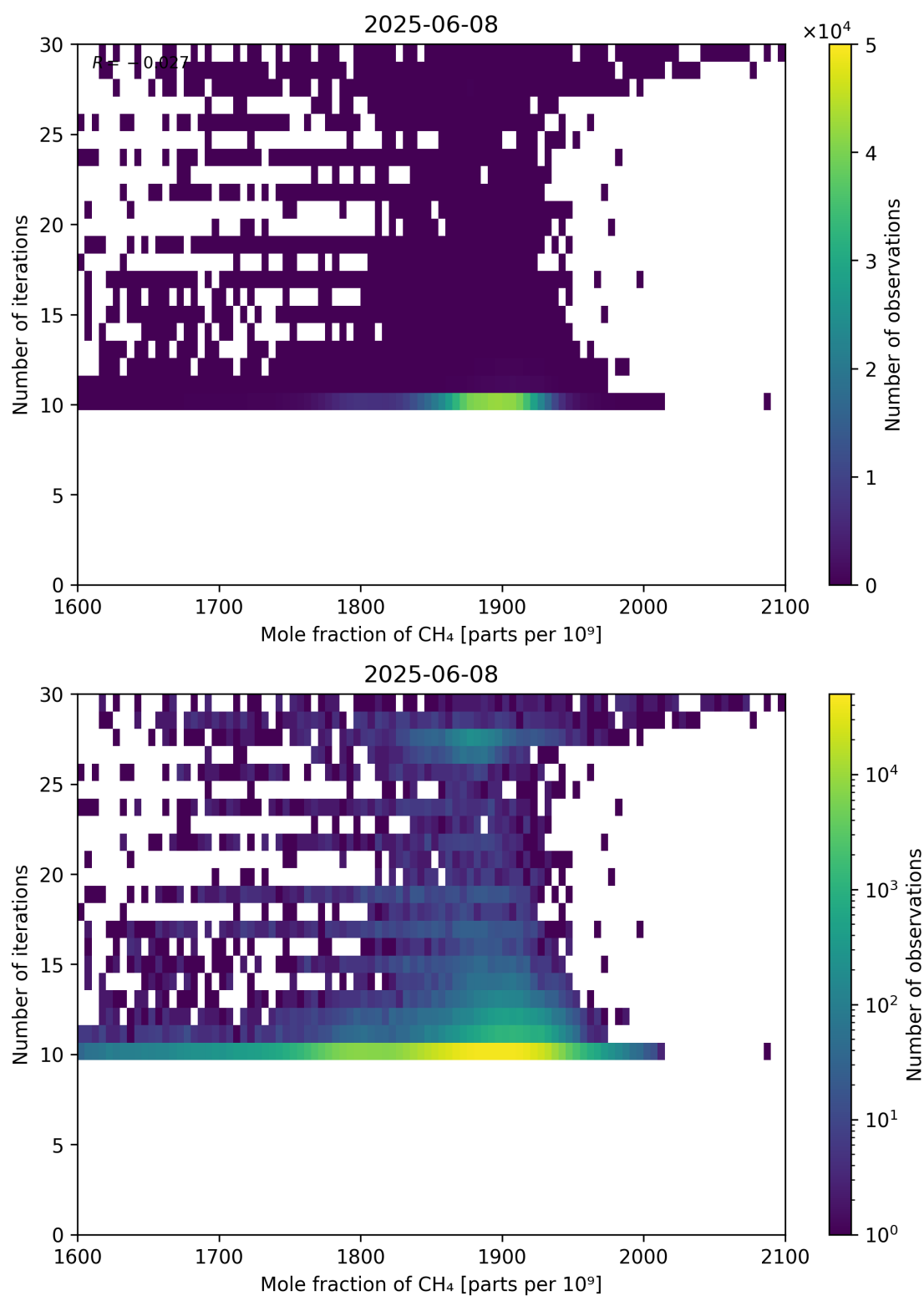
Figure 76: Scatter density plot of “Mole fraction of CH 4 ” against “Number of iterations” for 2025-06-07 to 2025-06-09.
