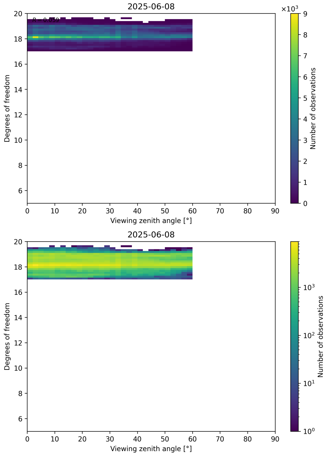
Figure 107: Scatter density plot of “Viewing zenith angle” against “Degrees of freedom” for 2025-06-07 to 2025-06-09.
