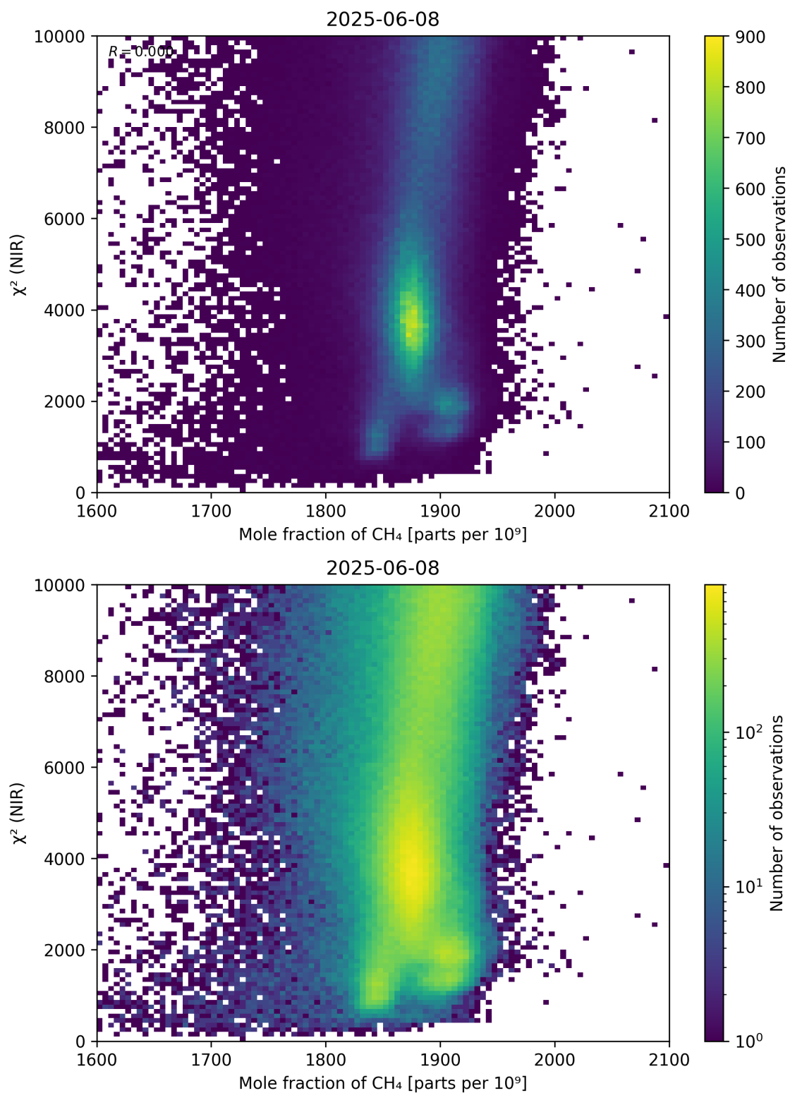
Figure 70: Scatter density plot of “Mole fraction of \text{CH}_4 ” against “ \chi^2 (NIR)” for 2025-06-07 to 2025-06-09.
