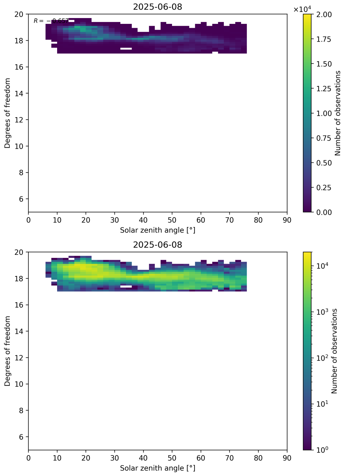
Figure 96: Scatter density plot of “Solar zenith angle” against “Degrees of freedom” for 2025-06-07 to 2025-06-09.
