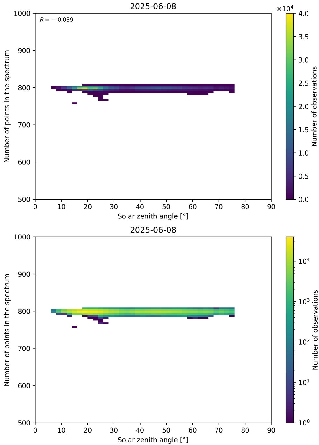
Figure 103: Scatter density plot of “Solar zenith angle” against “Number of points in the spectrum” for 2025-06-07 to 2025-06-09.
