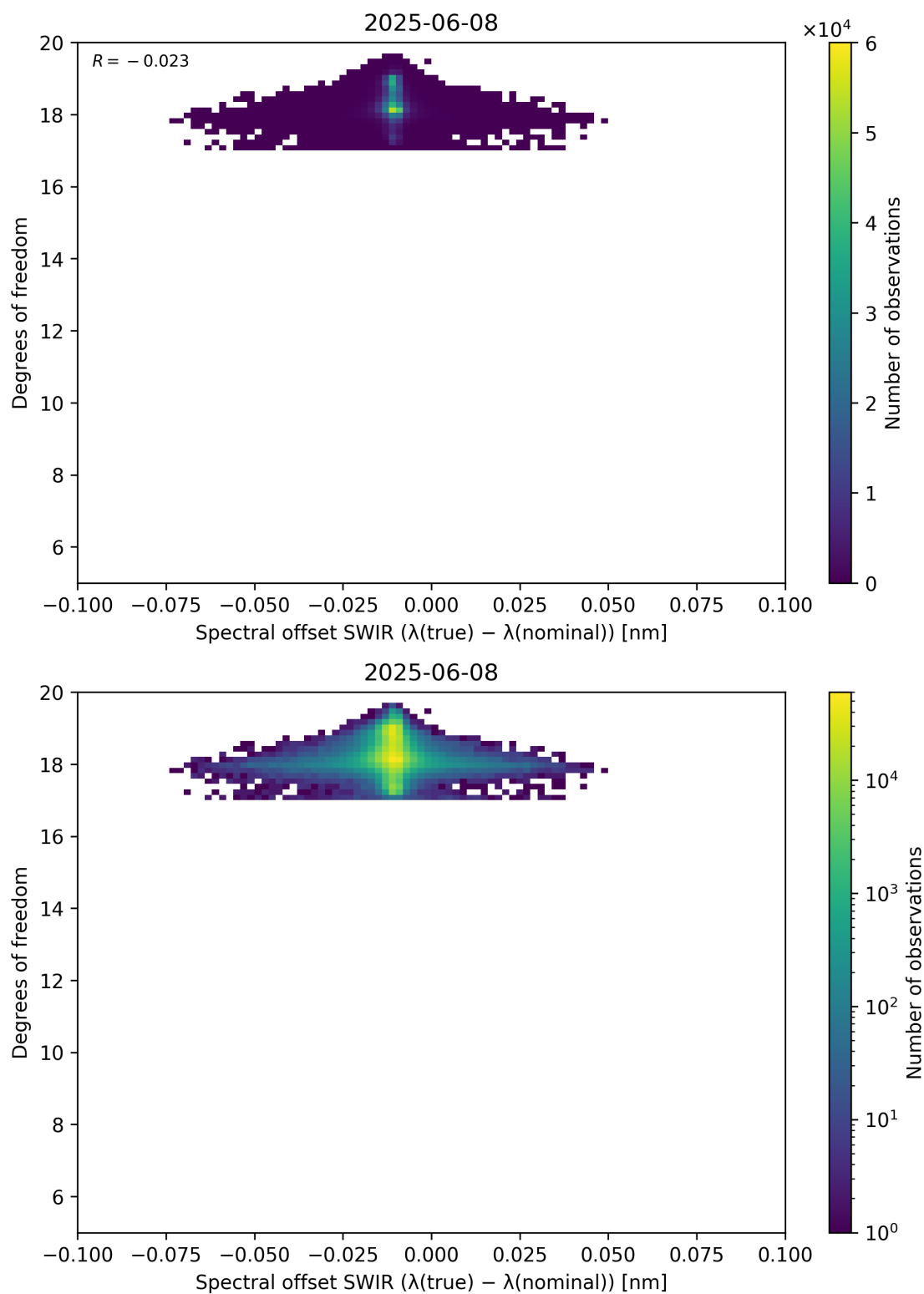
Figure 119: Scatter density plot of “Spectral offset SWIR ( \lambda_{\text{true}} - \lambda_{\text{nominal}} )” against “Degrees of freedom” for 2025-06-07 to 2025-06-09.
