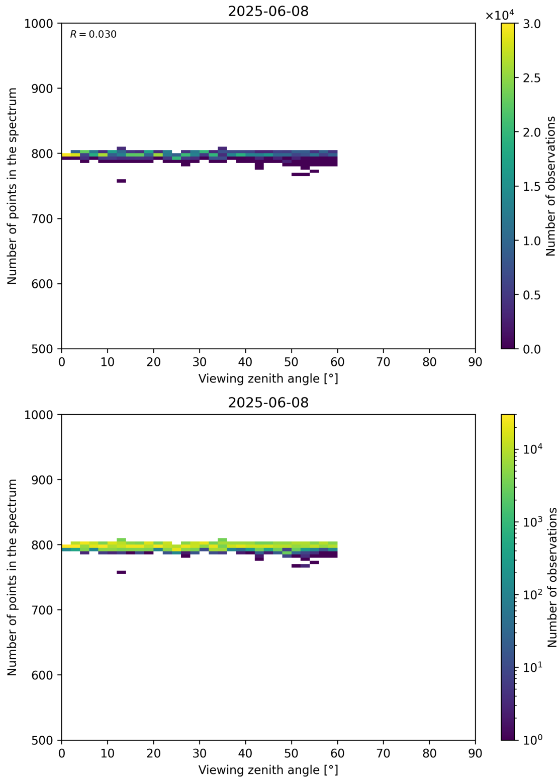
Figure 114: Scatter density plot of “Viewing zenith angle” against “Number of points in the spectrum” for 2025-06-07 to 2025-06-09.
