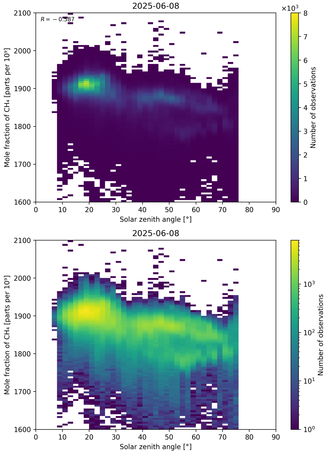
Figure 99: Scatter density plot of “Solar zenith angle” against “Mole fraction of CH 4 ” for 2025-06-07 to 2025-06-09.
