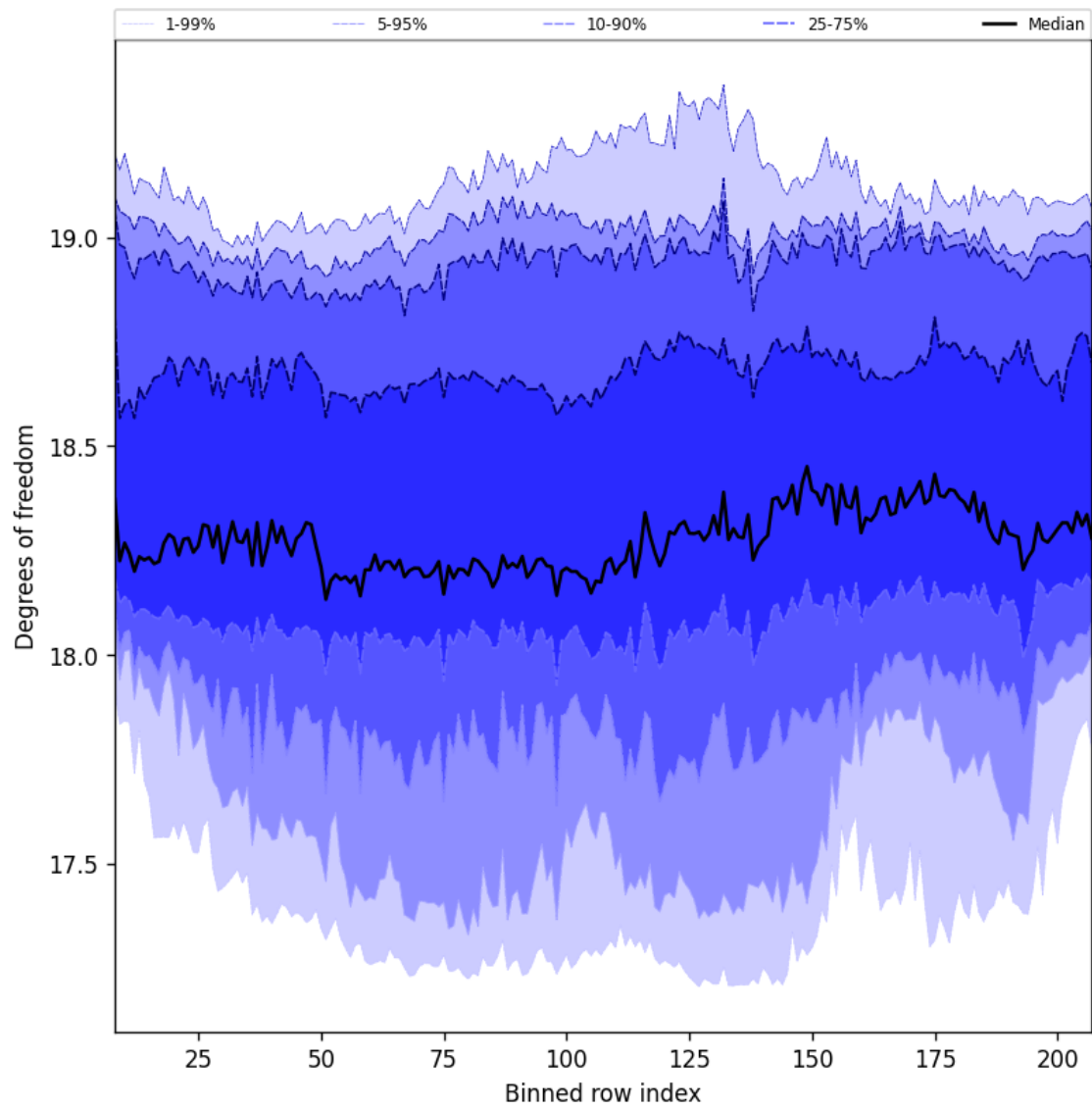
Figure 41: Along track statistics of “Degrees of freedom” for 2025-06-07 to 2025-06-09
