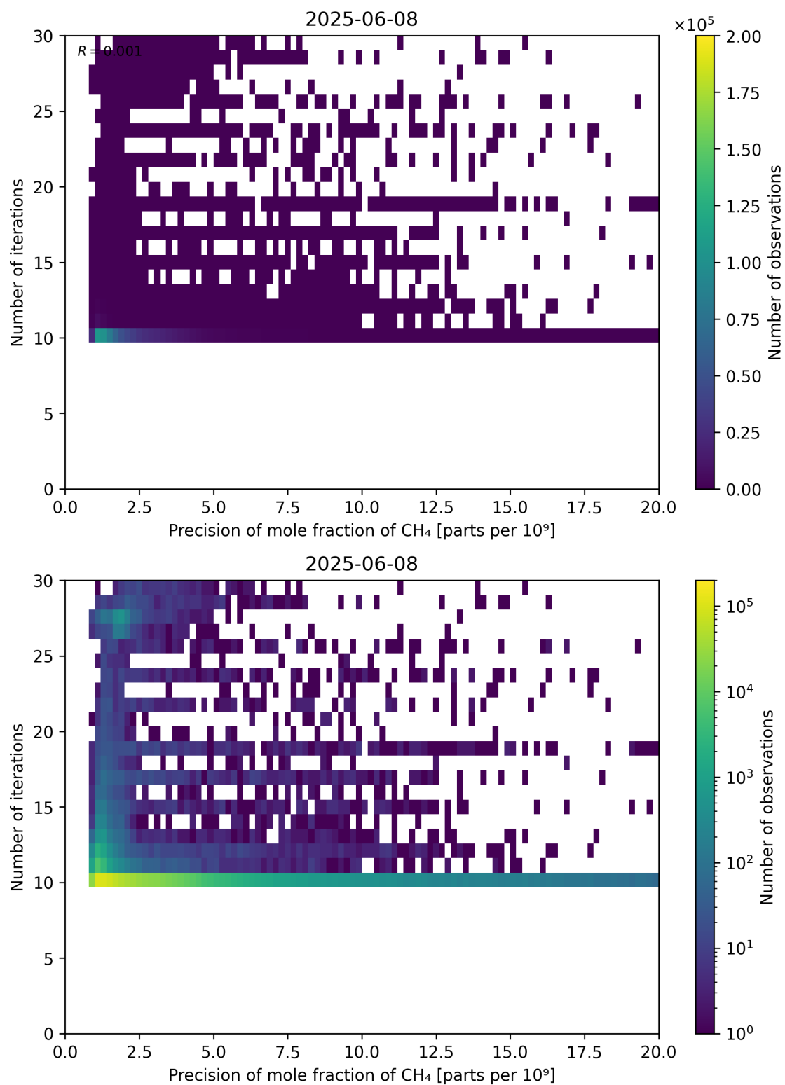
Figure 83: Scatter density plot of “Precision of mole fraction of CH 4 ” against “Number of iterations” for 2025-06-07 to 2025-06-09.
