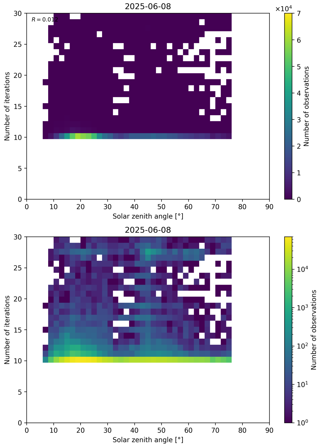
Figure 102: Scatter density plot of “Solar zenith angle” against “Number of iterations” for 2025-06-07 to 2025-06-09.
