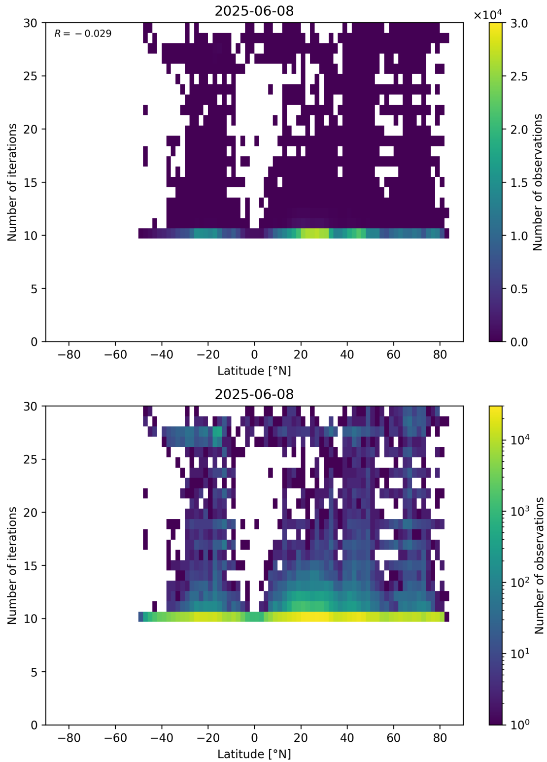
Figure 60: Scatter density plot of “Latitude” against “Number of iterations” for 2025-06-07 to 2025-06-09.
