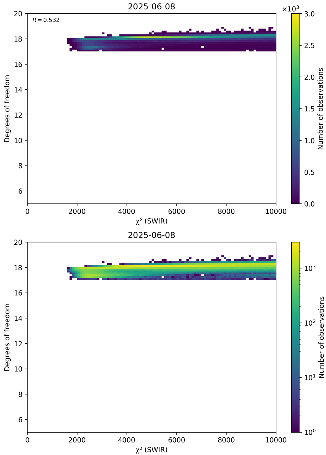
Figure 48: Scatter density plot of “ \chi^2 (SWIR)” against “Degrees of freedom” for 2025-06-07 to 2025-06-09.
