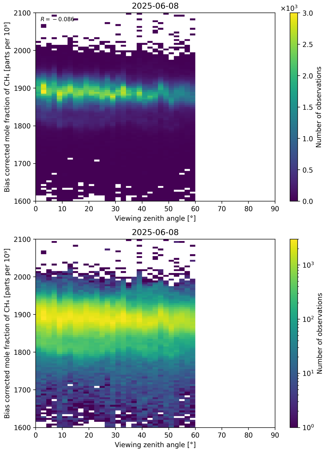
Figure 111: Scatter density plot of “Viewing zenith angle” against “Bias corrected mole fraction of CH 4 ” for 2025-06-07 to 2025-06-09.
