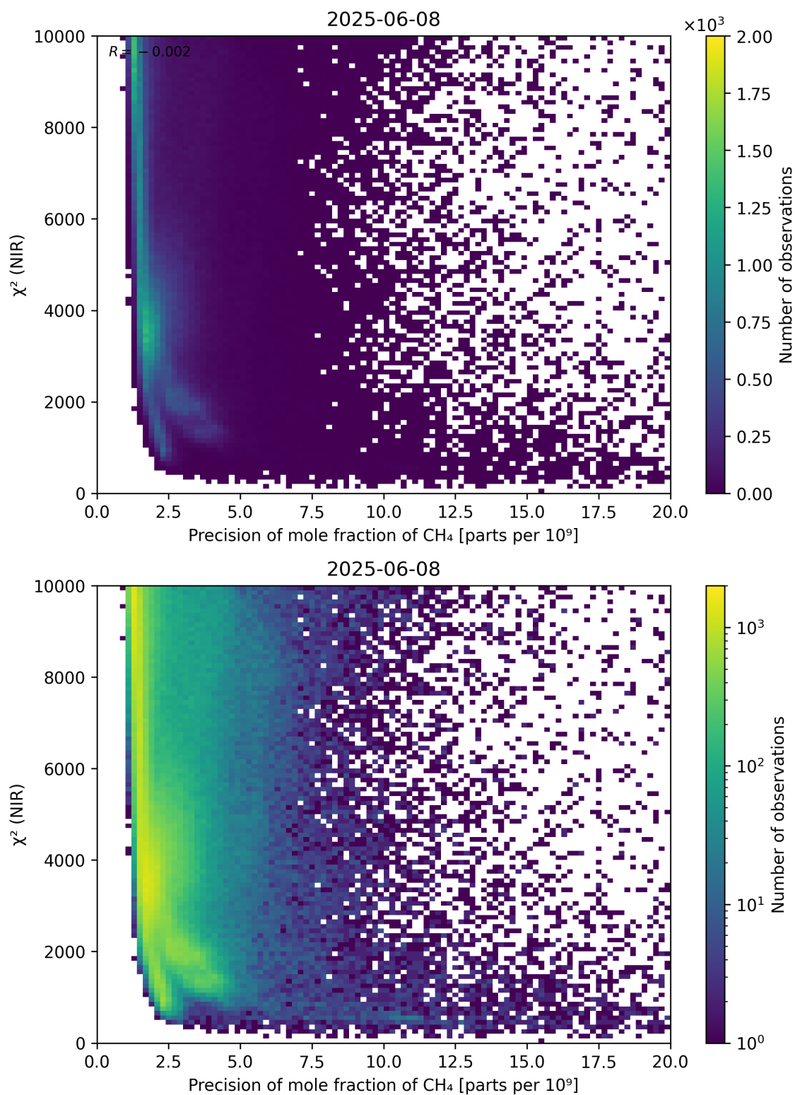
Figure 78: Scatter density plot of “Precision of mole fraction of CH 4 ” against “ \chi^2 (NIR)” for 2025-06-07 to 2025-06-09.
