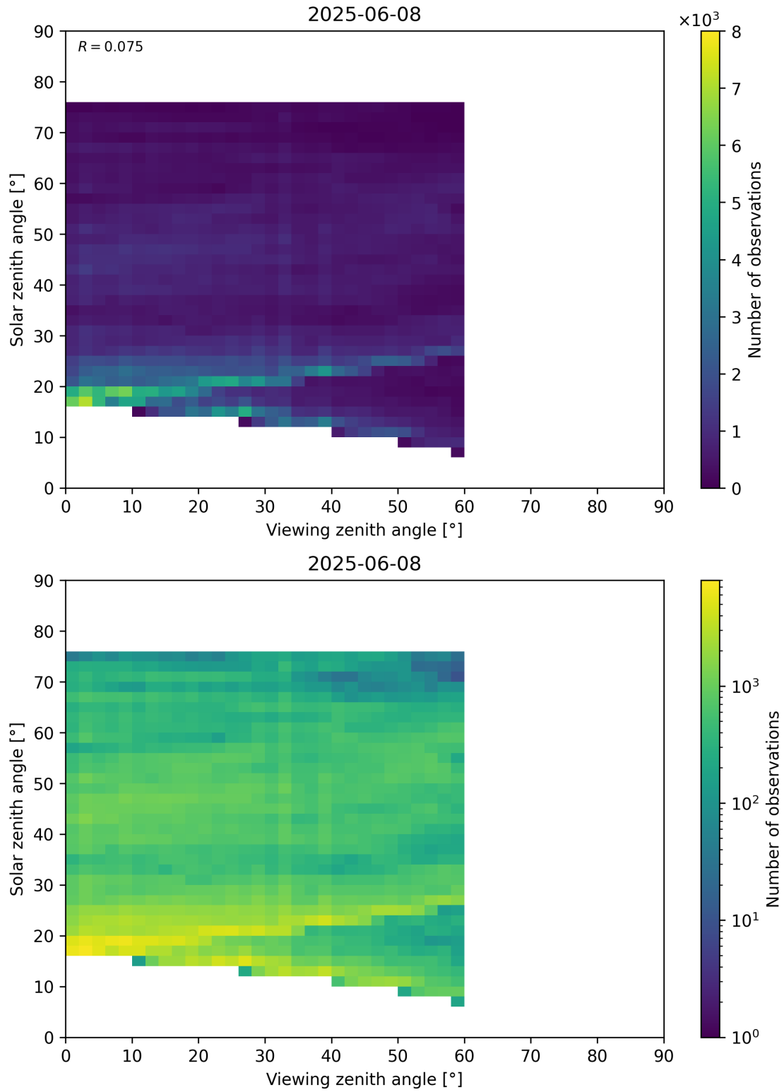
Figure 115: Scatter density plot of “Viewing zenith angle” against “Solar zenith angle” for 2025-06-07 to 2025-06-09.
