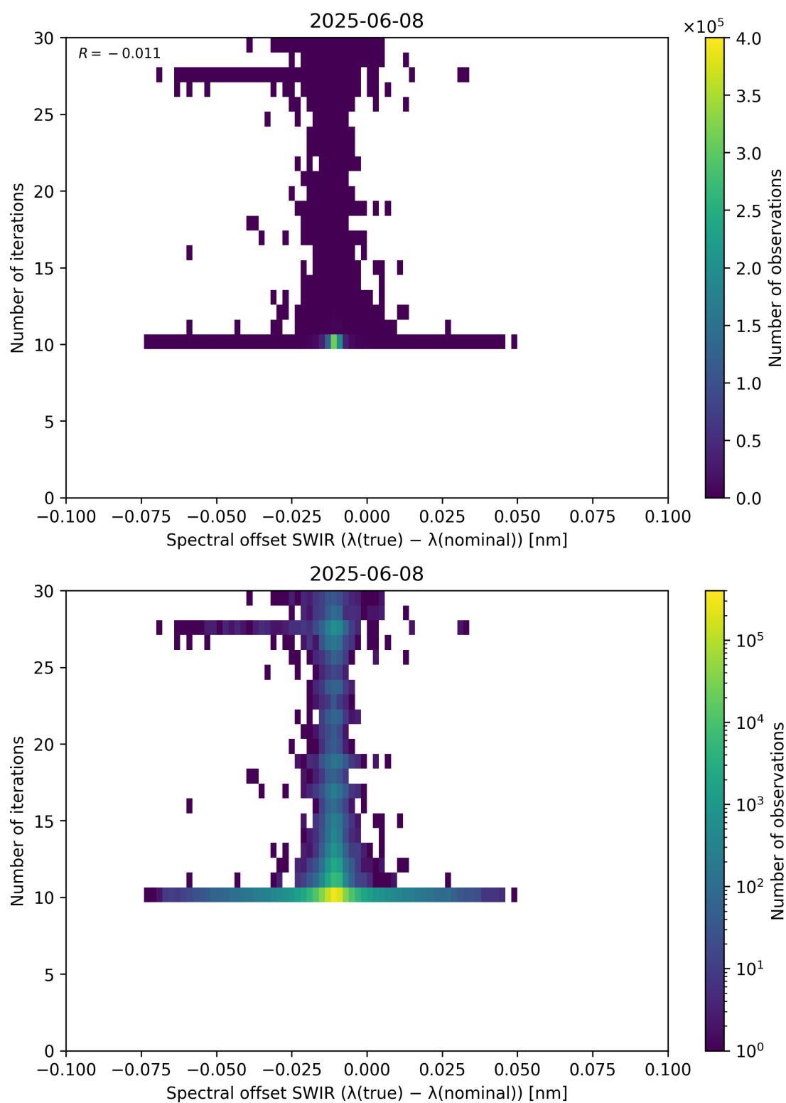
Figure 121: Scatter density plot of “Spectral offset SWIR ( \lambda_{\text{true}} - \lambda_{\text{nominal}} )” against “Number of iterations” for 2025-06-07 to 2025-06-09.
