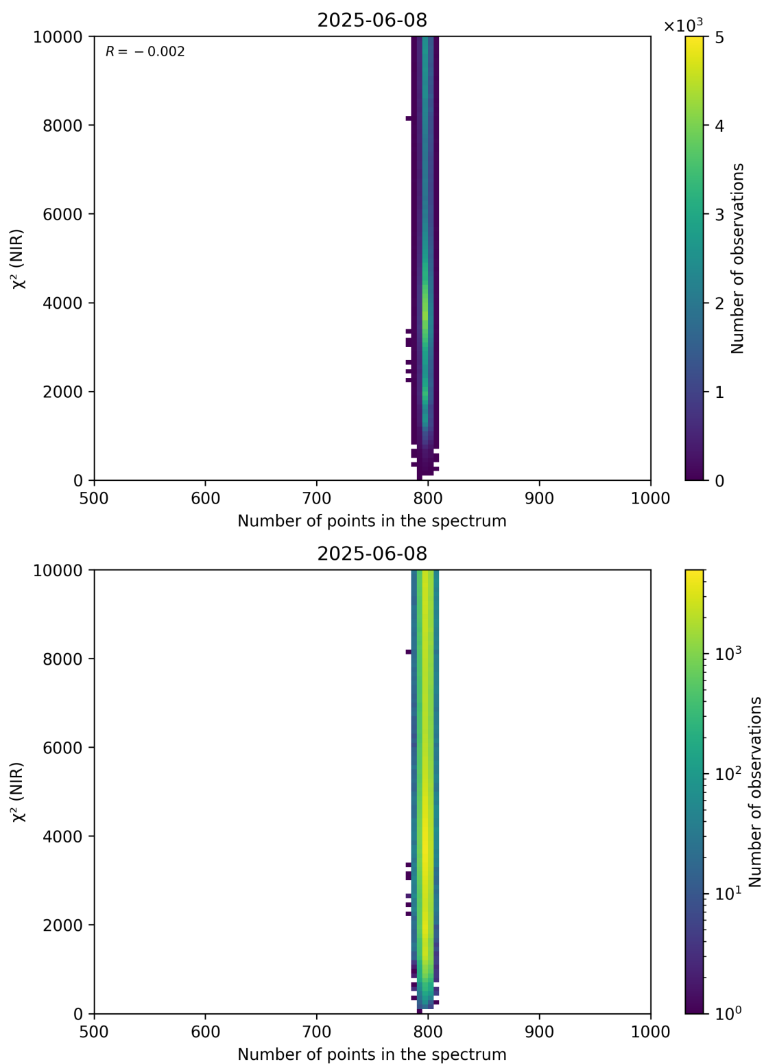
Figure 88: Scatter density plot of “Number of points in the spectrum” against “ \chi^2 (NIR)” for 2025-06-07 to 2025-06-09.
