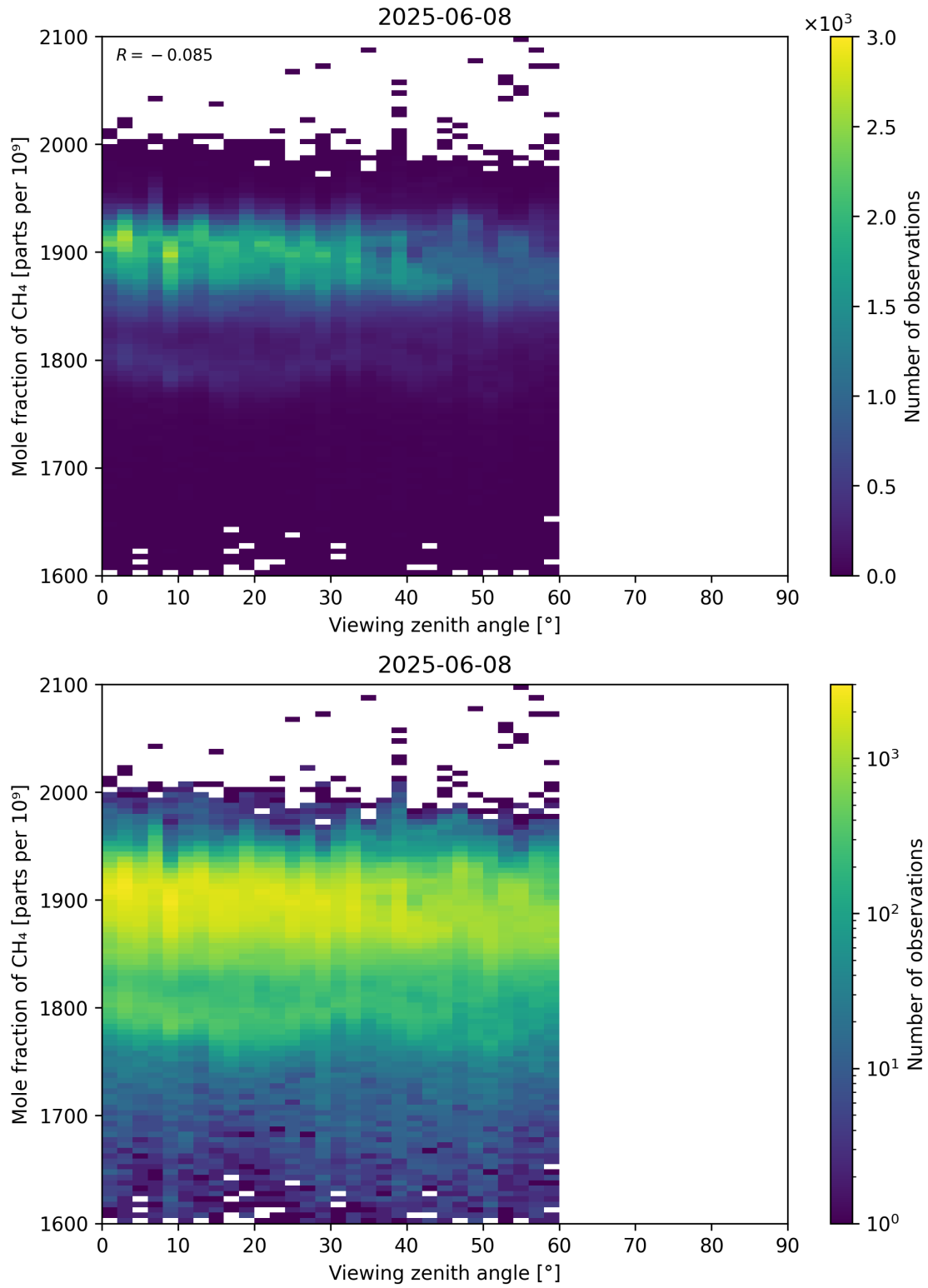
Figure 110: Scatter density plot of “Viewing zenith angle” against “Mole fraction of CH 4 ” for 2025-06-07 to 2025-06-09.
