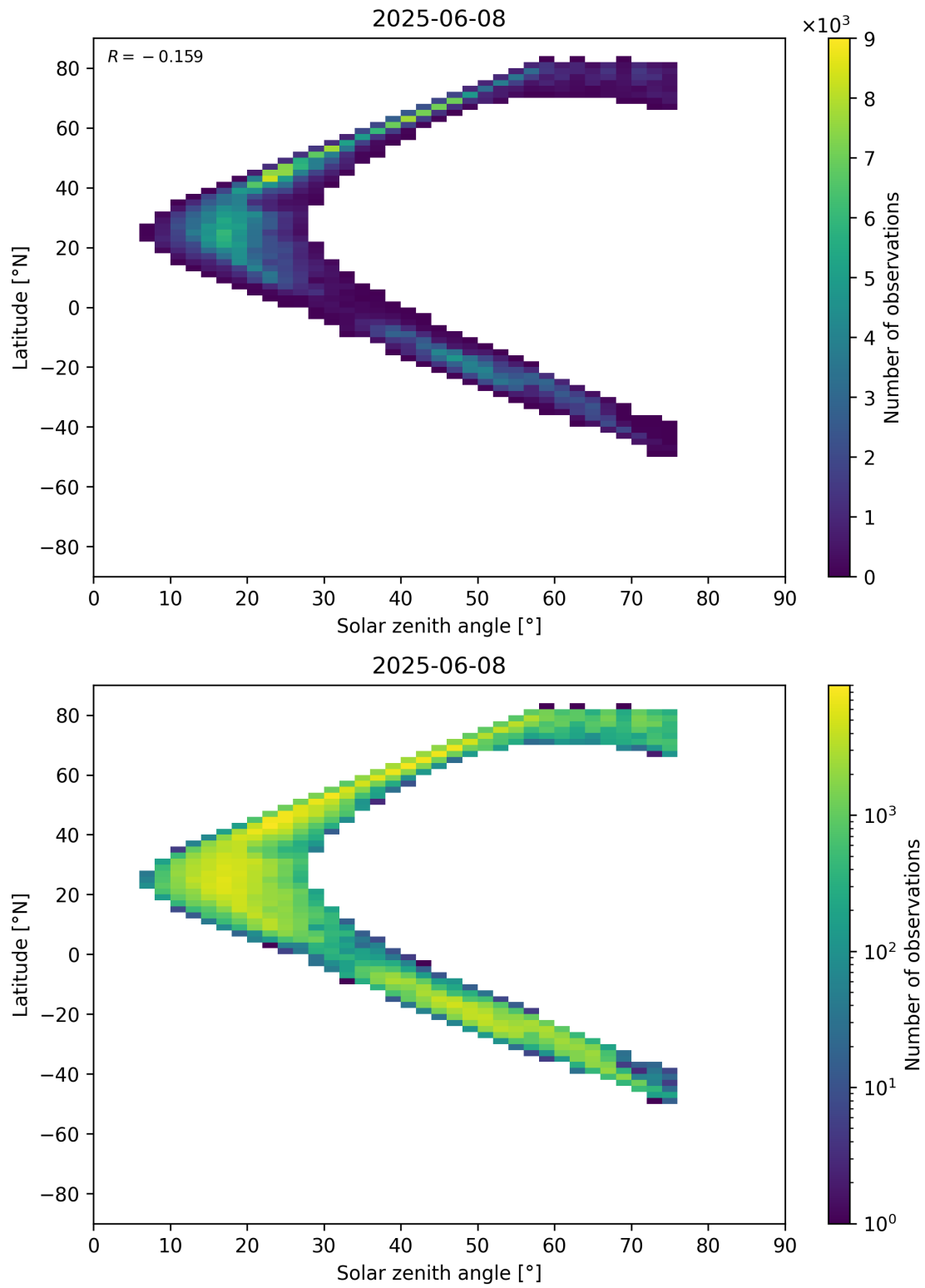
Figure 98: Scatter density plot of “Solar zenith angle” against “Latitude” for 2025-06-07 to 2025-06-09.
