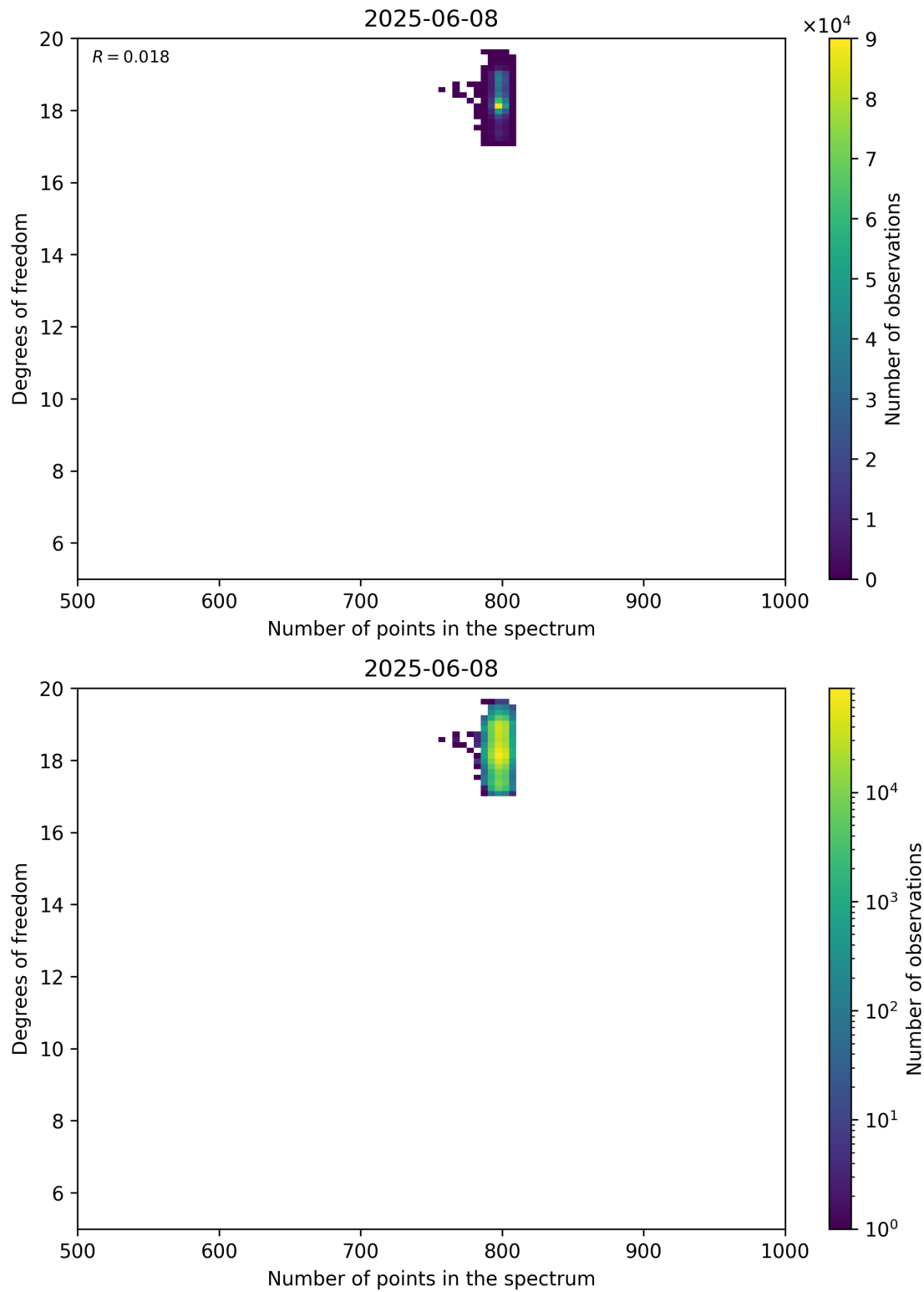
Figure 90: Scatter density plot of “Number of points in the spectrum” against “Degrees of freedom” for 2025-06-07 to 2025-06-09.
