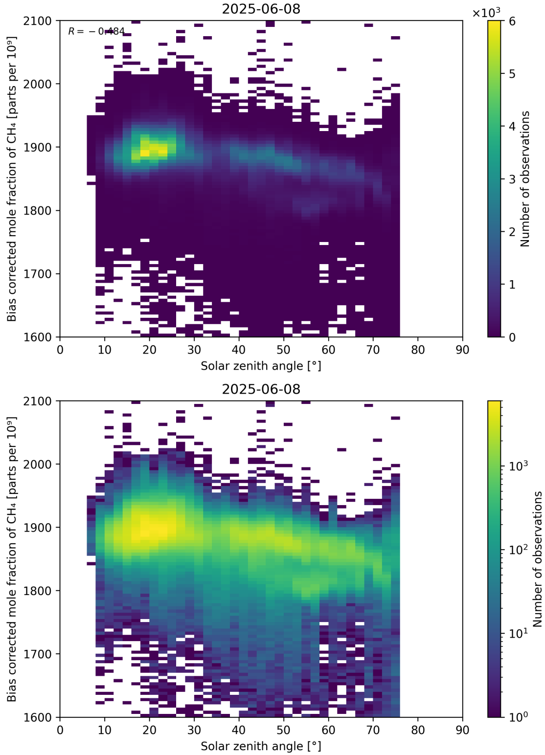
Figure 100: Scatter density plot of “Solar zenith angle” against “Bias corrected mole fraction of \text{CH}_4 ” for 2025-06-07 to 2025-06-09.
