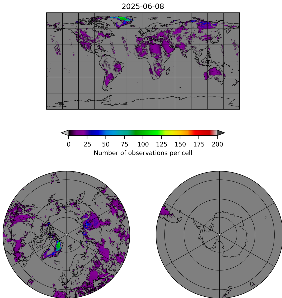
Figure 10: Map of the number of observations for 2025-06-07 to 2025-06-09
