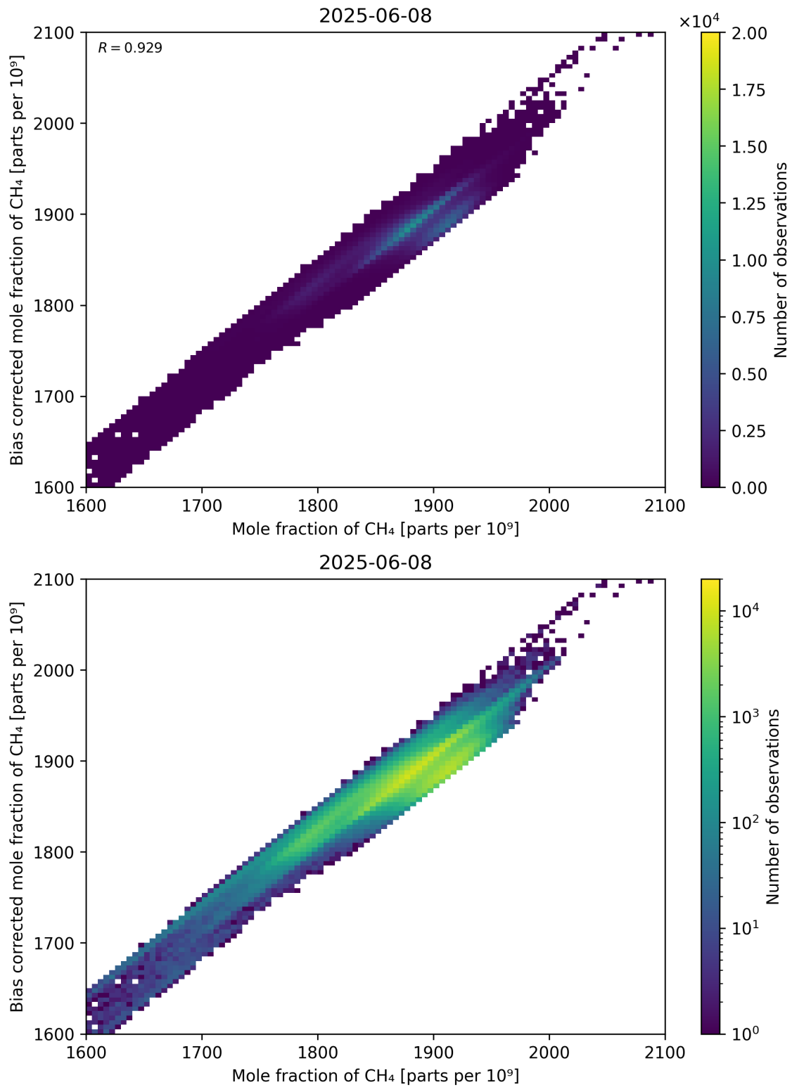
Figure 74: Scatter density plot of “Mole fraction of CH 4 ” against “Bias corrected mole fraction of CH 4 ” for 2025-06-07 to 2025-06-09.
