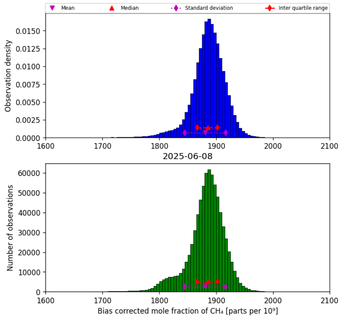
Figure 25: Histogram of “Bias corrected mole fraction of CH 4 ” for 2025-06-07 to 2025-06-09
