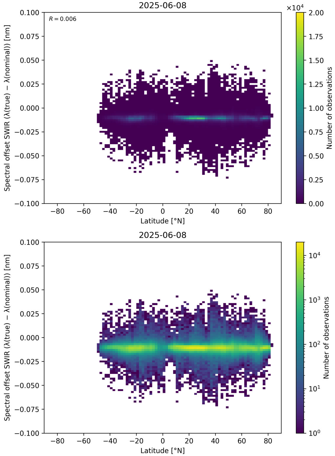
Figure 62: Scatter density plot of “Latitude” against “Spectral offset SWIR ( \lambda_{\text{true}} - \lambda_{\text{nominal}} )” for 2025-06-07 to 2025-06-09.
