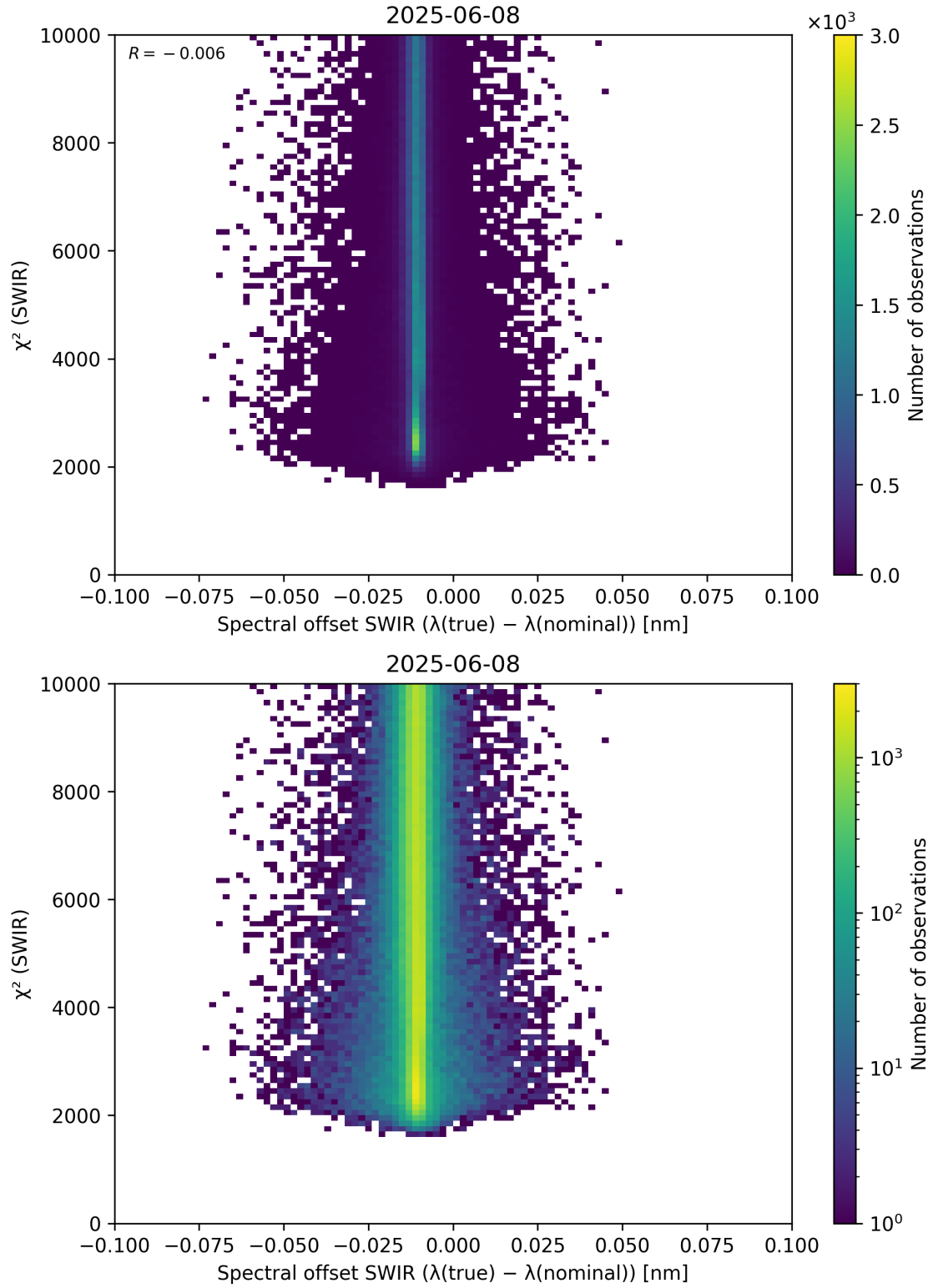
Figure 118: Scatter density plot of “Spectral offset SWIR ( \lambda_{\text{true}} - \lambda_{\text{nominal}} )” against “ \chi^2 (SWIR)” for 2025-06-07 to 2025-06-09.
