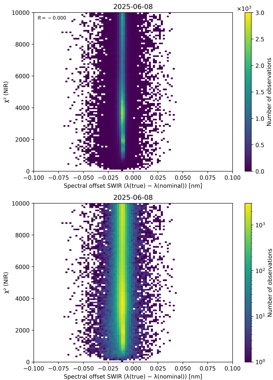
Figure 117: Scatter density plot of “Spectral offset SWIR ( \lambda_{\text{true}} - \lambda_{\text{nominal}} )” against “ \chi^2 (NIR)” for 2025-06-07 to 2025-06-09.
