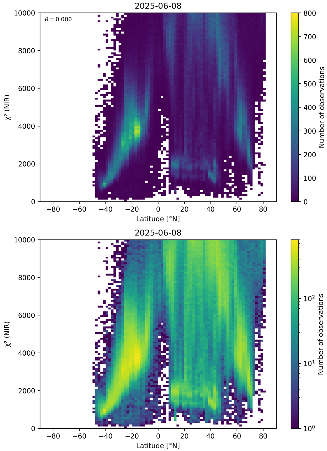
Figure 53: Scatter density plot of “Latitude” against “ \chi^2 (NIR)” for 2025-06-07 to 2025-06-09.
