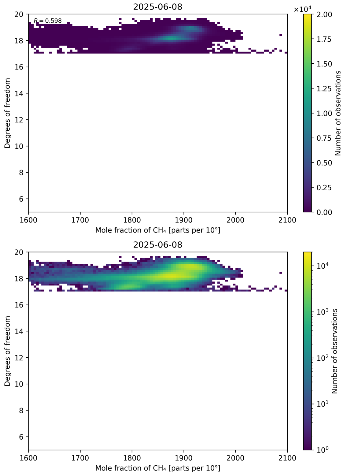
Figure 72: Scatter density plot of “Mole fraction of CH 4 ” against “Degrees of freedom” for 2025-06-07 to 2025-06-09.
