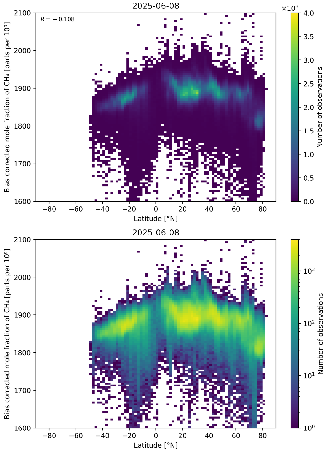
Figure 58: Scatter density plot of “Latitude” against “Bias corrected mole fraction of \text{CH}_4 ” for 2025-06-07 to 2025-06-09.
