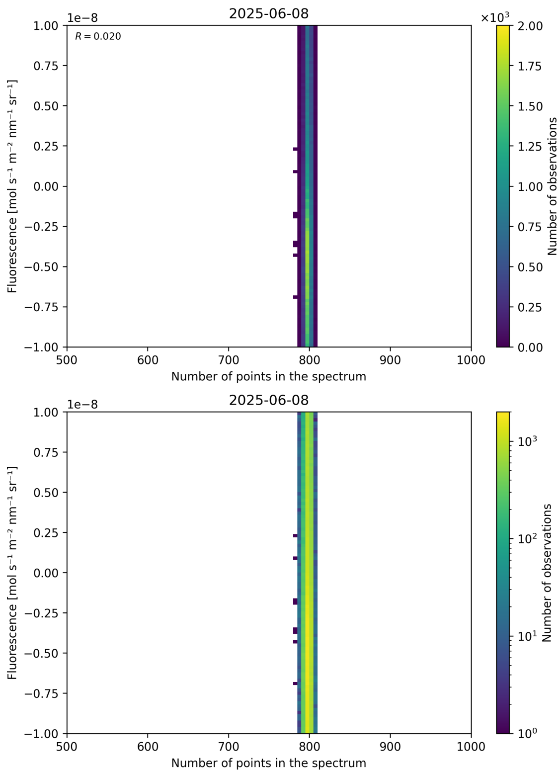
Figure 91: Scatter density plot of “Number of points in the spectrum” against “Fluorescence” for 2025-06-07 to 2025-06-09.
