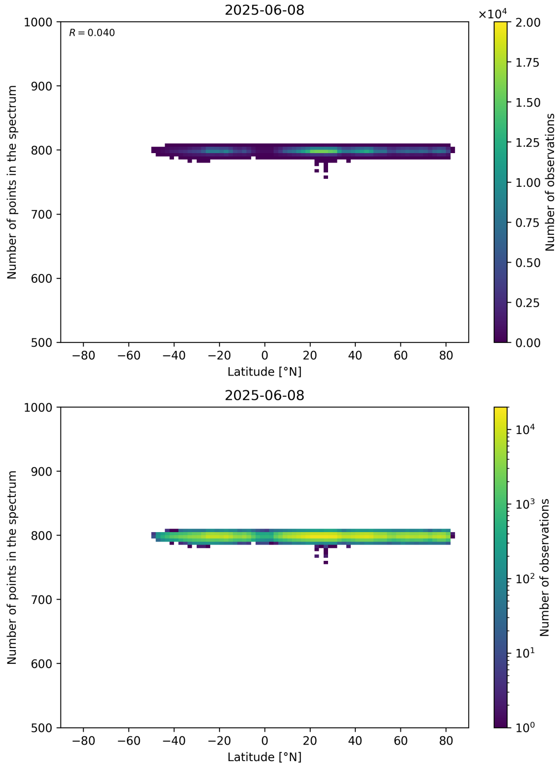
Figure 61: Scatter density plot of “Latitude” against “Number of points in the spectrum” for 2025-06-07 to 2025-06-09.
