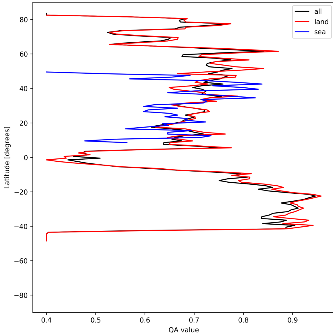
Figure 11: Zonal average of “QA value” for 2025-06-07 to 2025-06-09.
