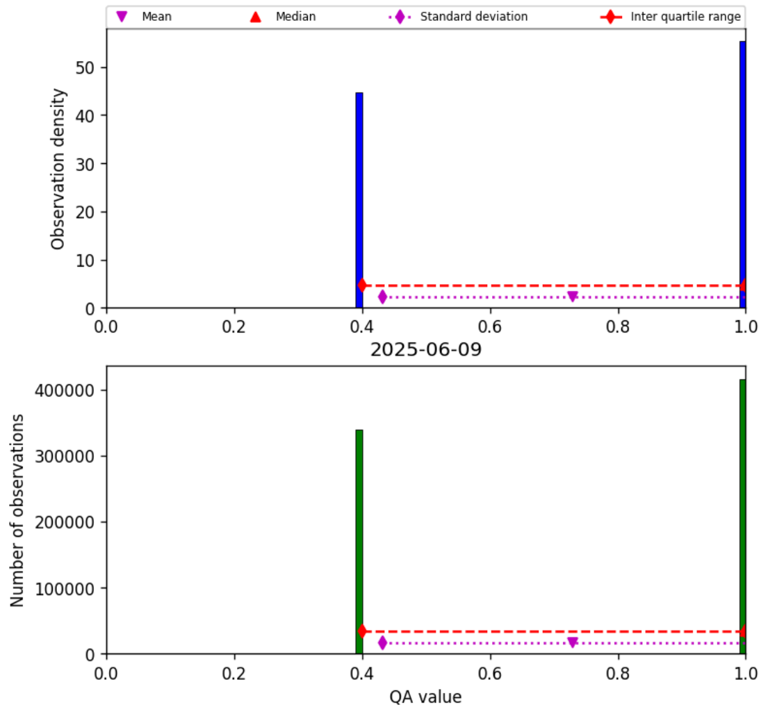
Figure 22: Histogram of “QA value” for 2025-06-08 to 2025-06-10
