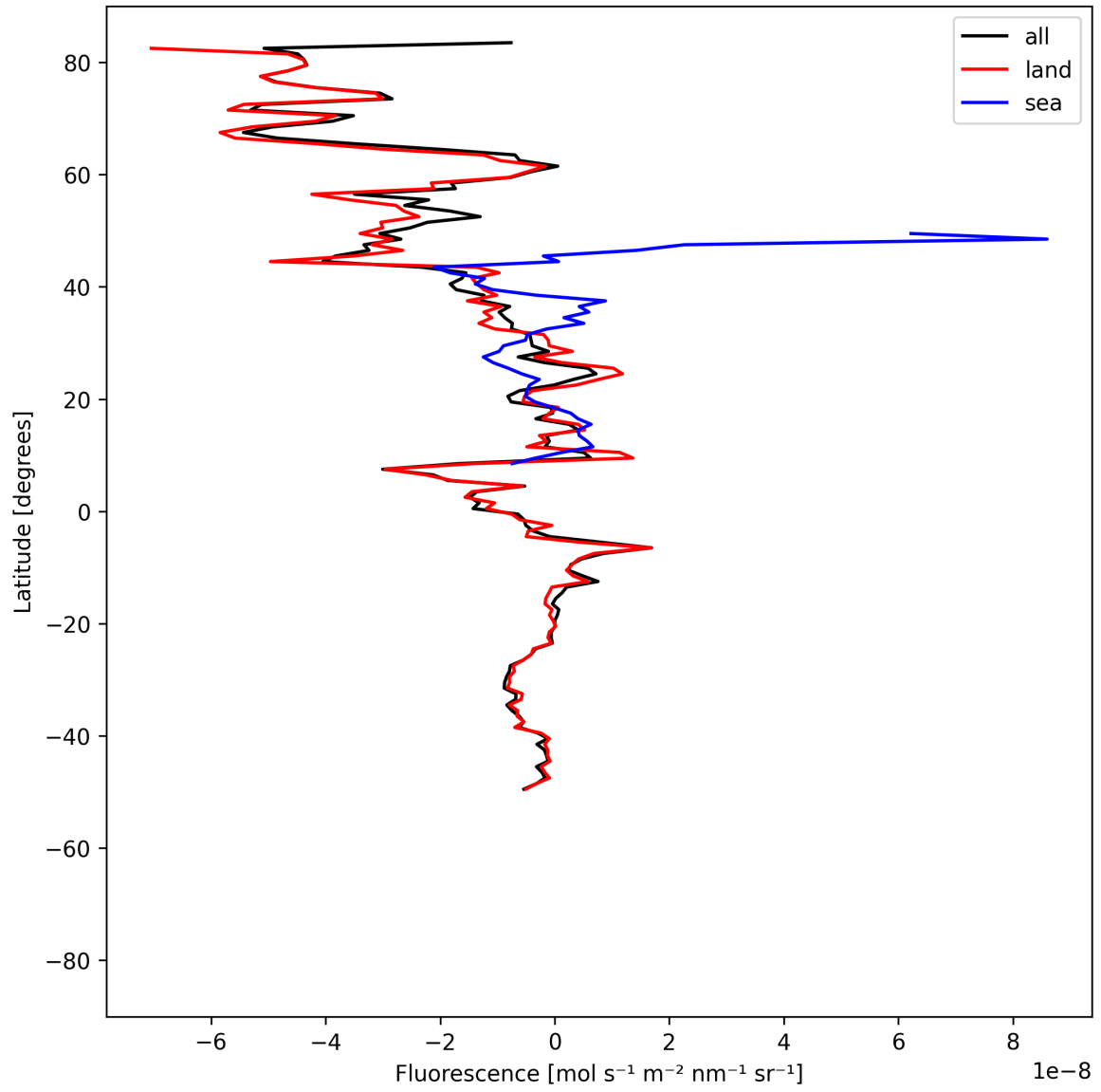
Figure 21: Zonal average of “Fluorescence” for 2025-06-08 to 2025-06-10.
