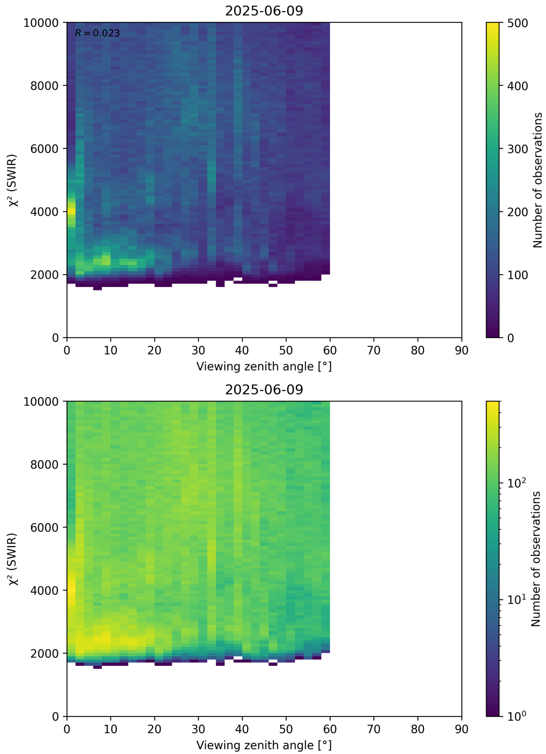
Figure 106: Scatter density plot of “Viewing zenith angle” against “ \chi^2 (SWIR)” for 2025-06-08 to 2025-06-10.
