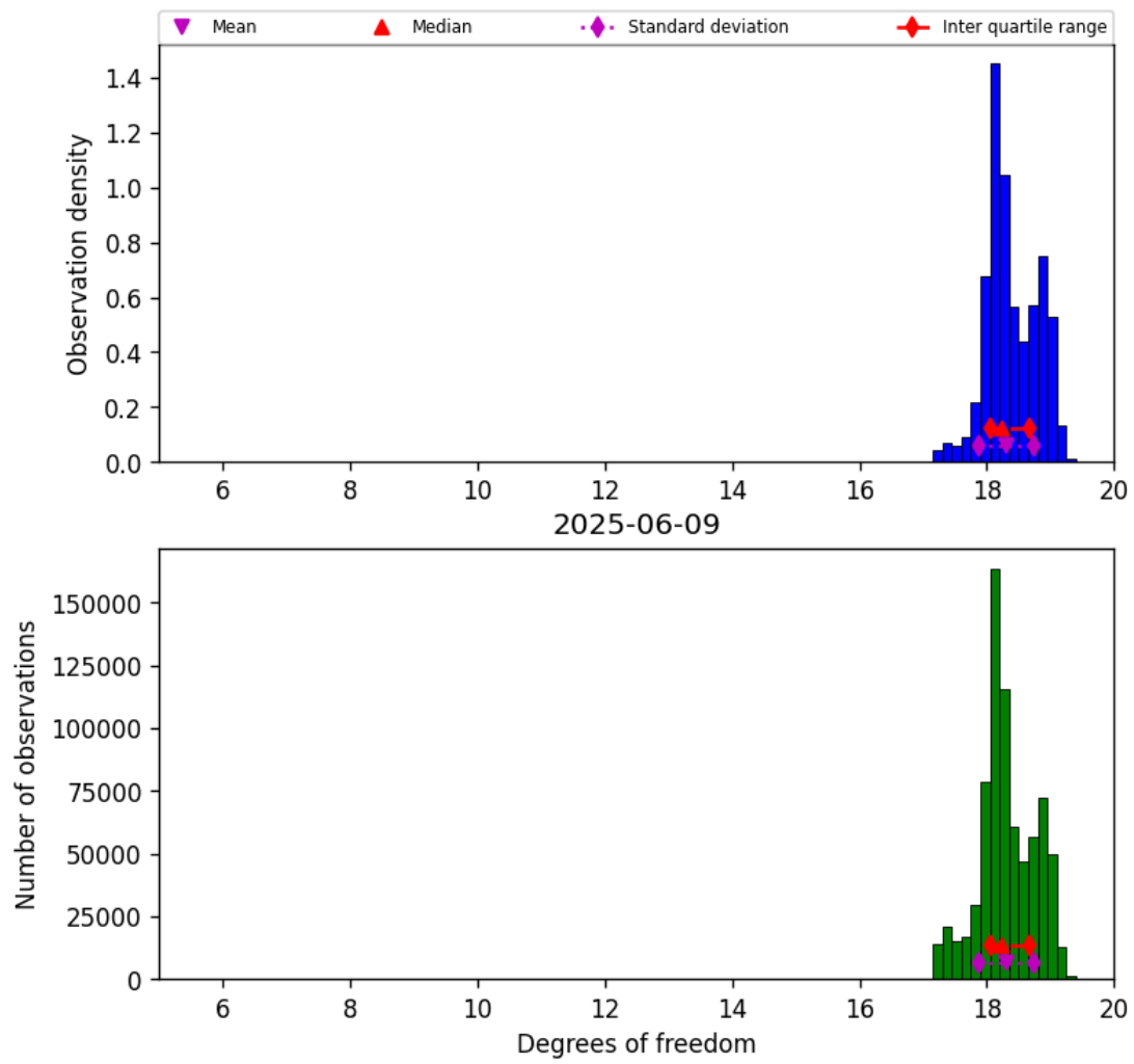
Figure 30: Histogram of “Degrees of freedom” for 2025-06-08 to 2025-06-10
