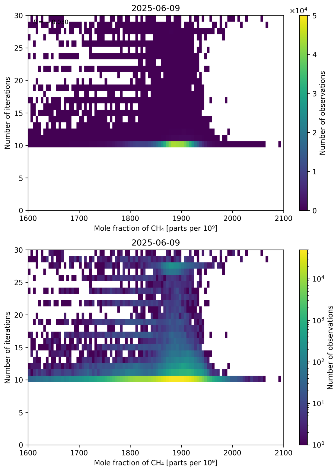
Figure 76: Scatter density plot of “Mole fraction of CH 4 ” against “Number of iterations” for 2025-06-08 to 2025-06-10.
