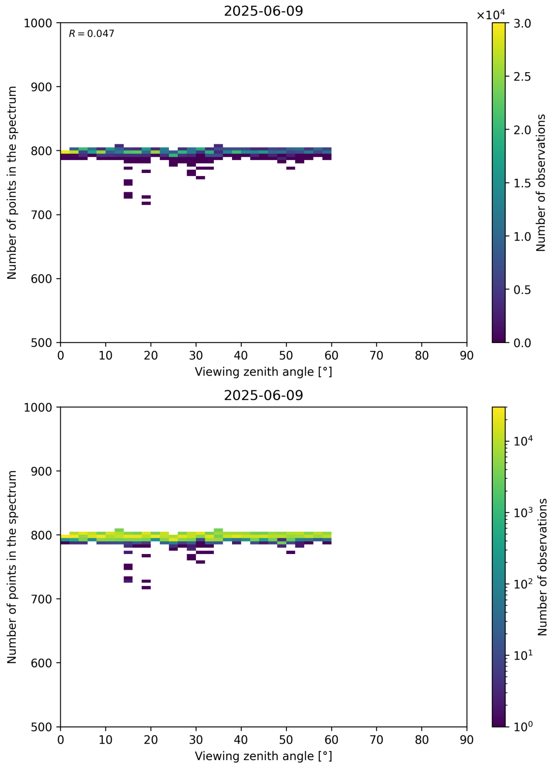
Figure 114: Scatter density plot of “Viewing zenith angle” against “Number of points in the spectrum” for 2025-06-08 to 2025-06-10.
