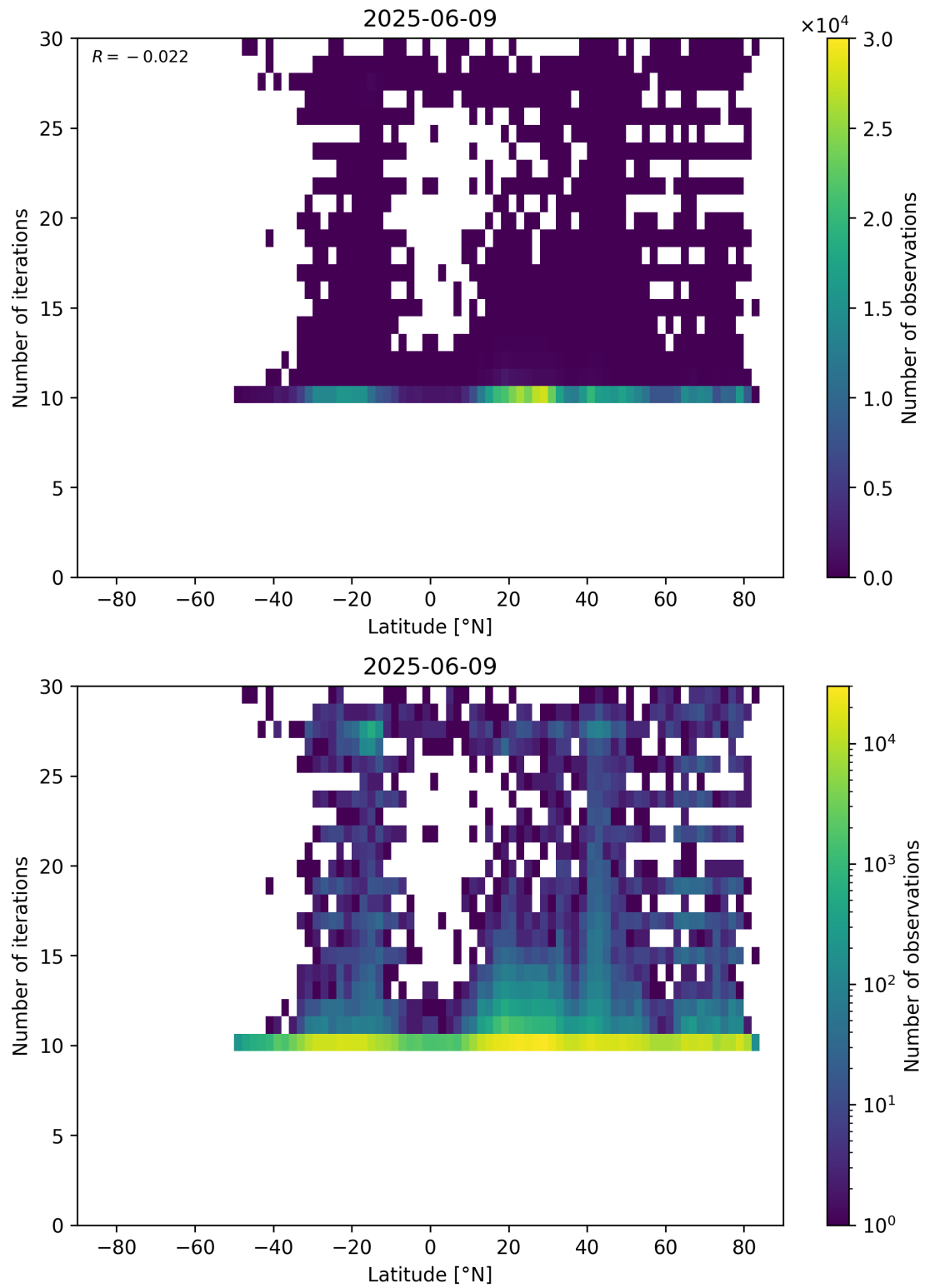
Figure 60: Scatter density plot of “Latitude” against “Number of iterations” for 2025-06-08 to 2025-06-10.
