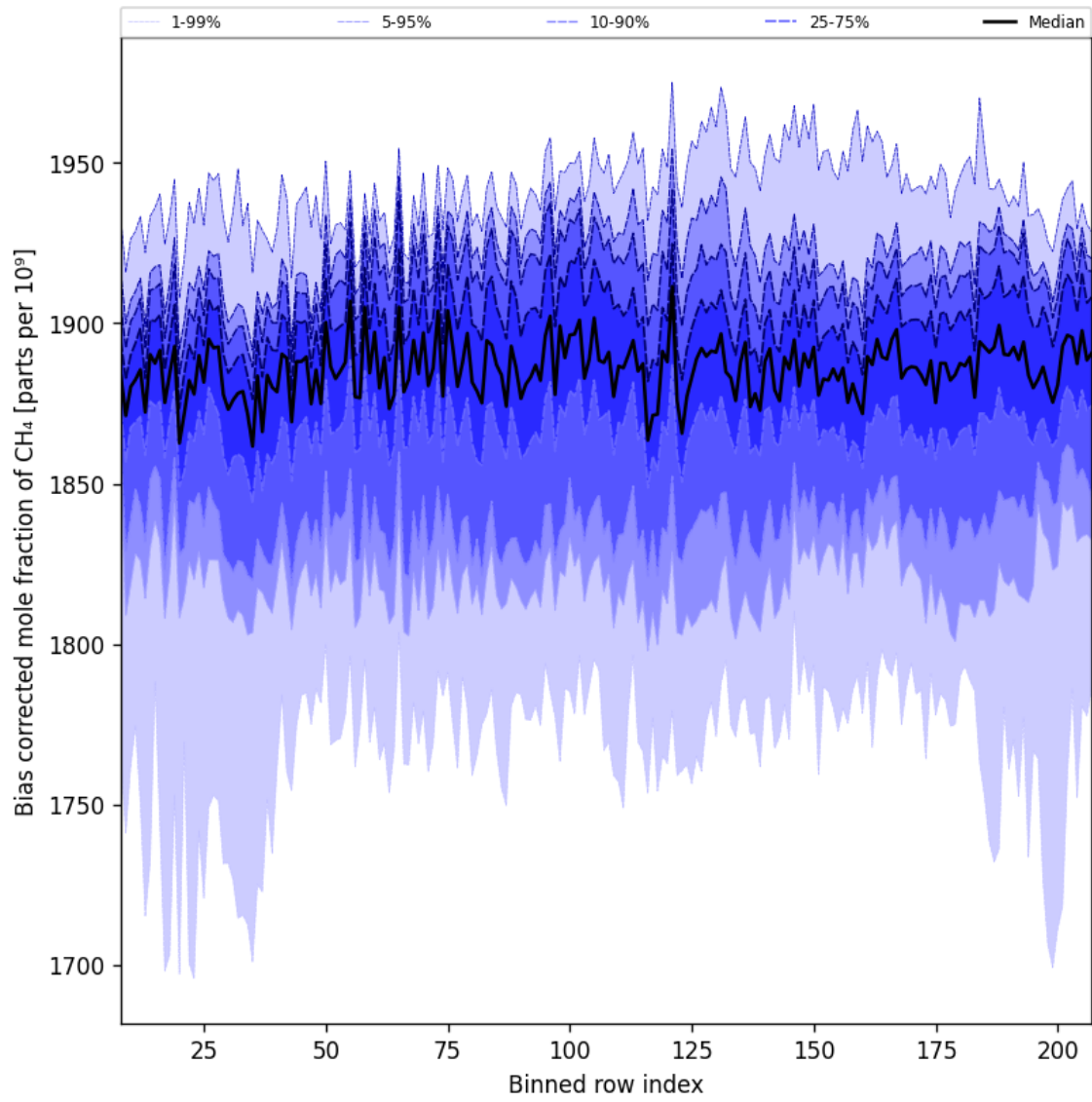
Figure 36: Along track statistics of “Bias corrected mole fraction of CH 4 ” for 2025-06-08 to 2025-06-10
