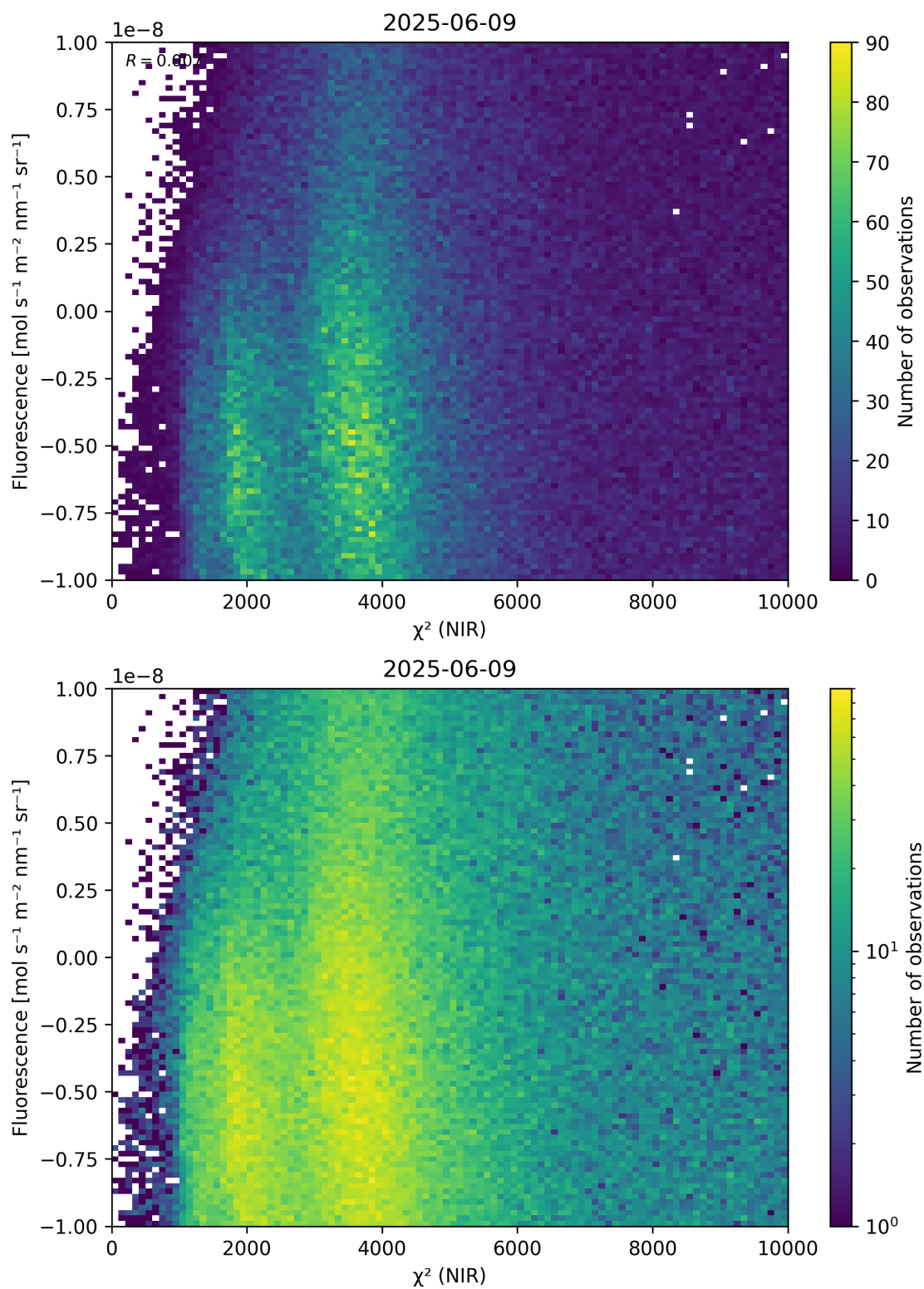
Figure 45: Scatter density plot of “ \chi^2 (NIR)” against “Fluorescence” for 2025-06-08 to 2025-06-10.
