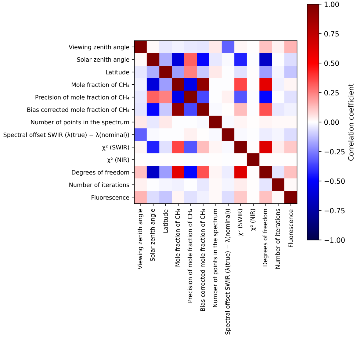
Figure 2: Map of correlation matrix for 2025-06-08 to 2025-06-10.
