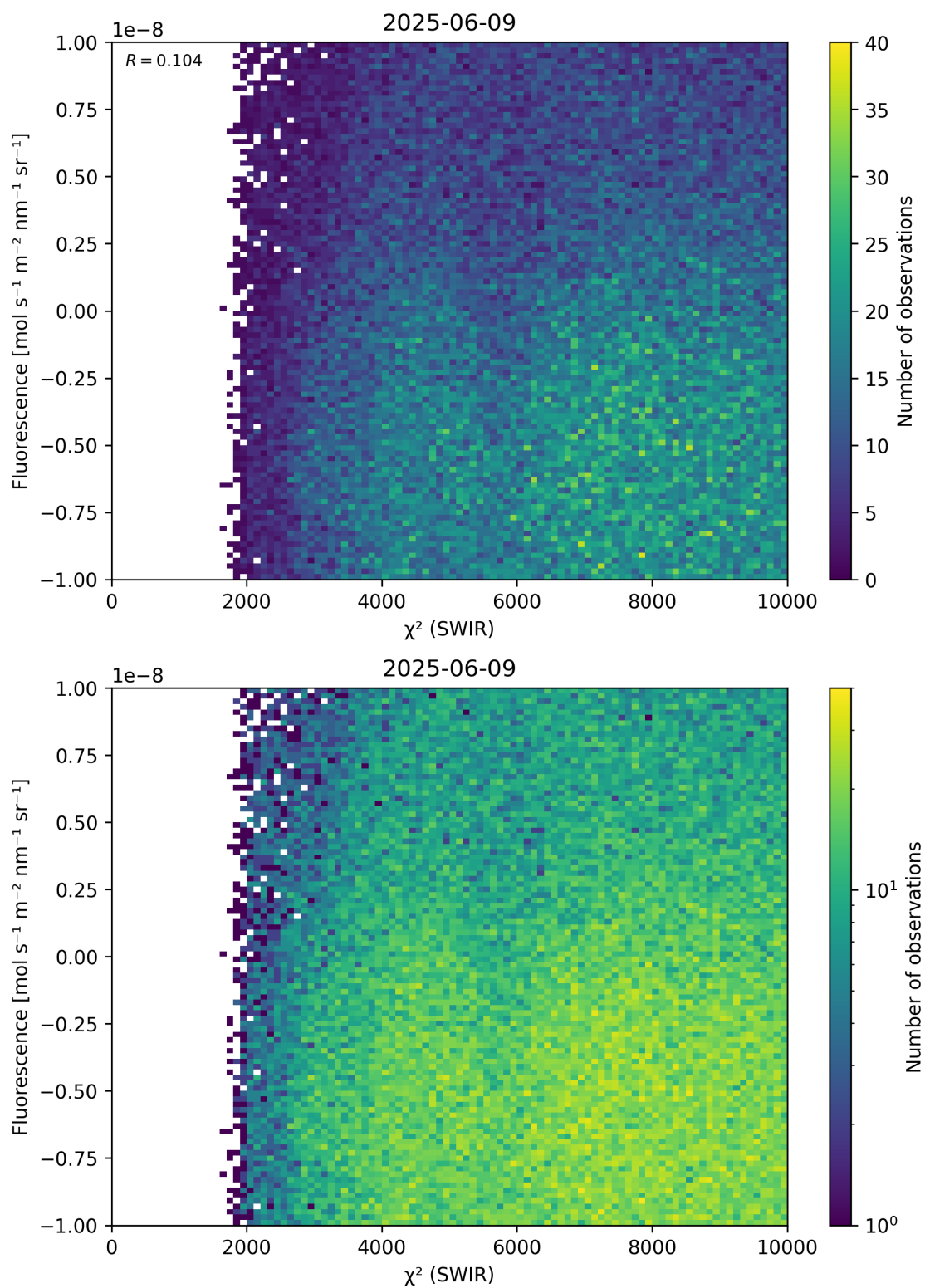
Figure 49: Scatter density plot of “ \chi^2 (SWIR)” against “Fluorescence” for 2025-06-08 to 2025-06-10.
