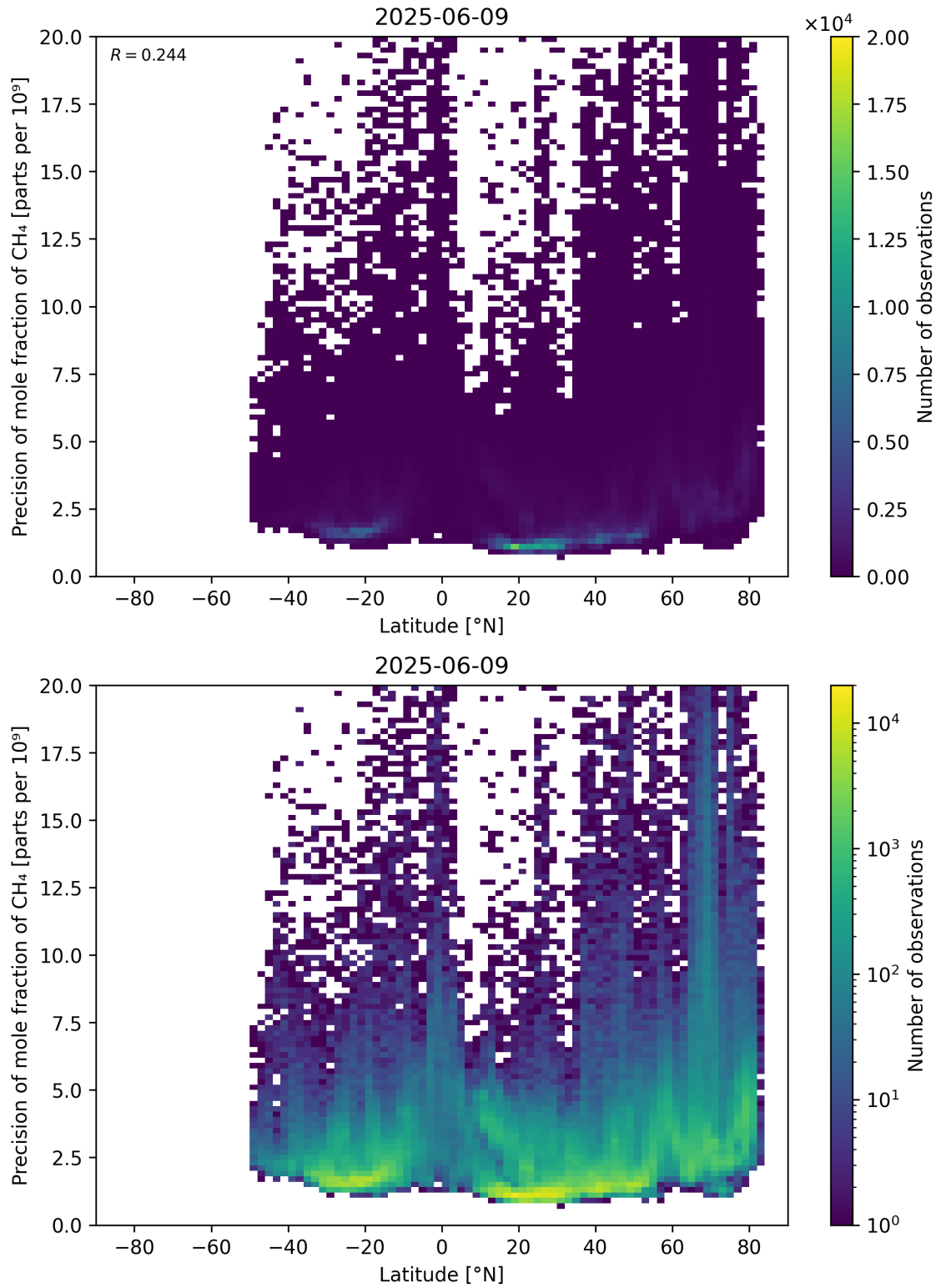
Figure 59: Scatter density plot of “Latitude” against “Precision of mole fraction of \text{CH}_4 ” for 2025-06-08 to 2025-06-10.
