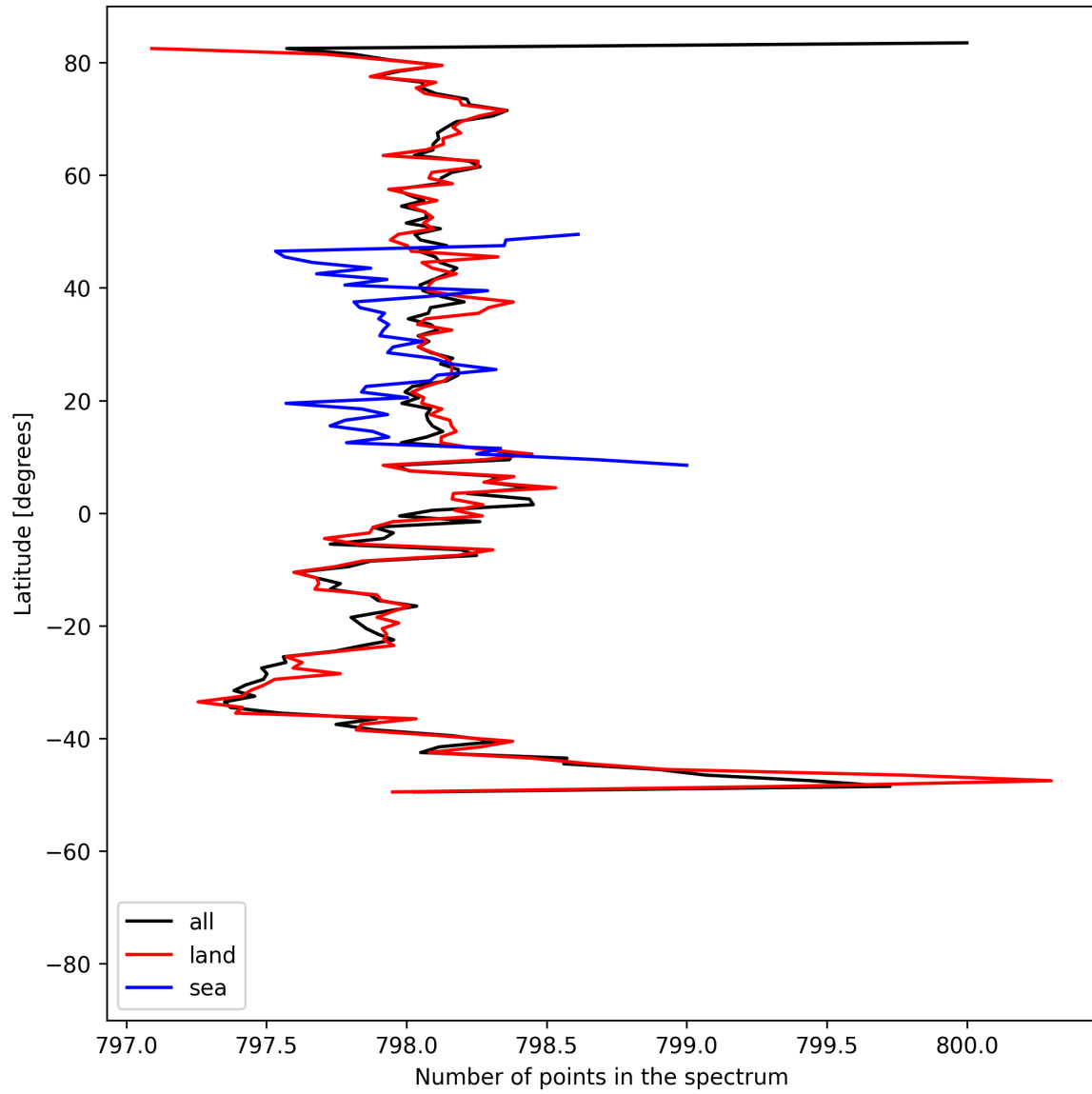
Figure 15: Zonal average of “Number of points in the spectrum” for 2025-06-08 to 2025-06-10.
