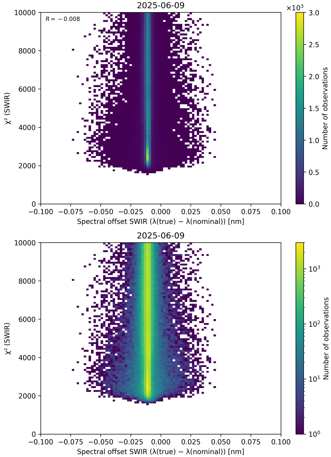
Figure 118: Scatter density plot of “Spectral offset SWIR ( \lambda_{\text{true}} - \lambda_{\text{nominal}} )” against “ \chi^2 (SWIR)” for 2025-06-08 to 2025-06-10.
