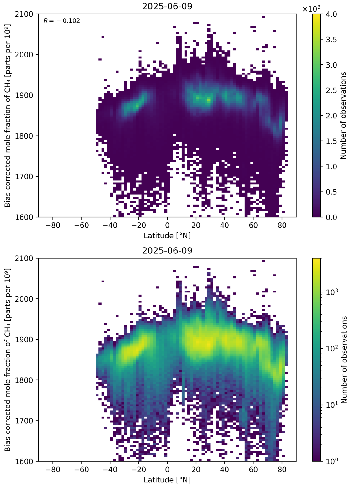
Figure 58: Scatter density plot of “Latitude” against “Bias corrected mole fraction of CH 4 ” for 2025-06-08 to 2025-06-10.
