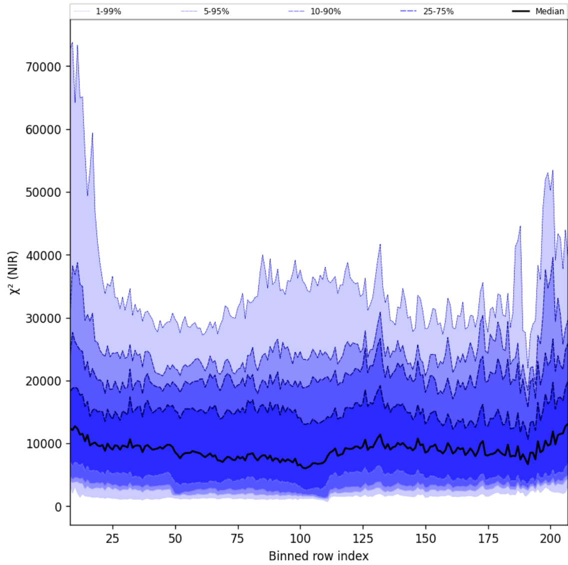
Figure 40: Along track statistics of “ \chi^2 (NIR)” for 2025-06-08 to 2025-06-10
