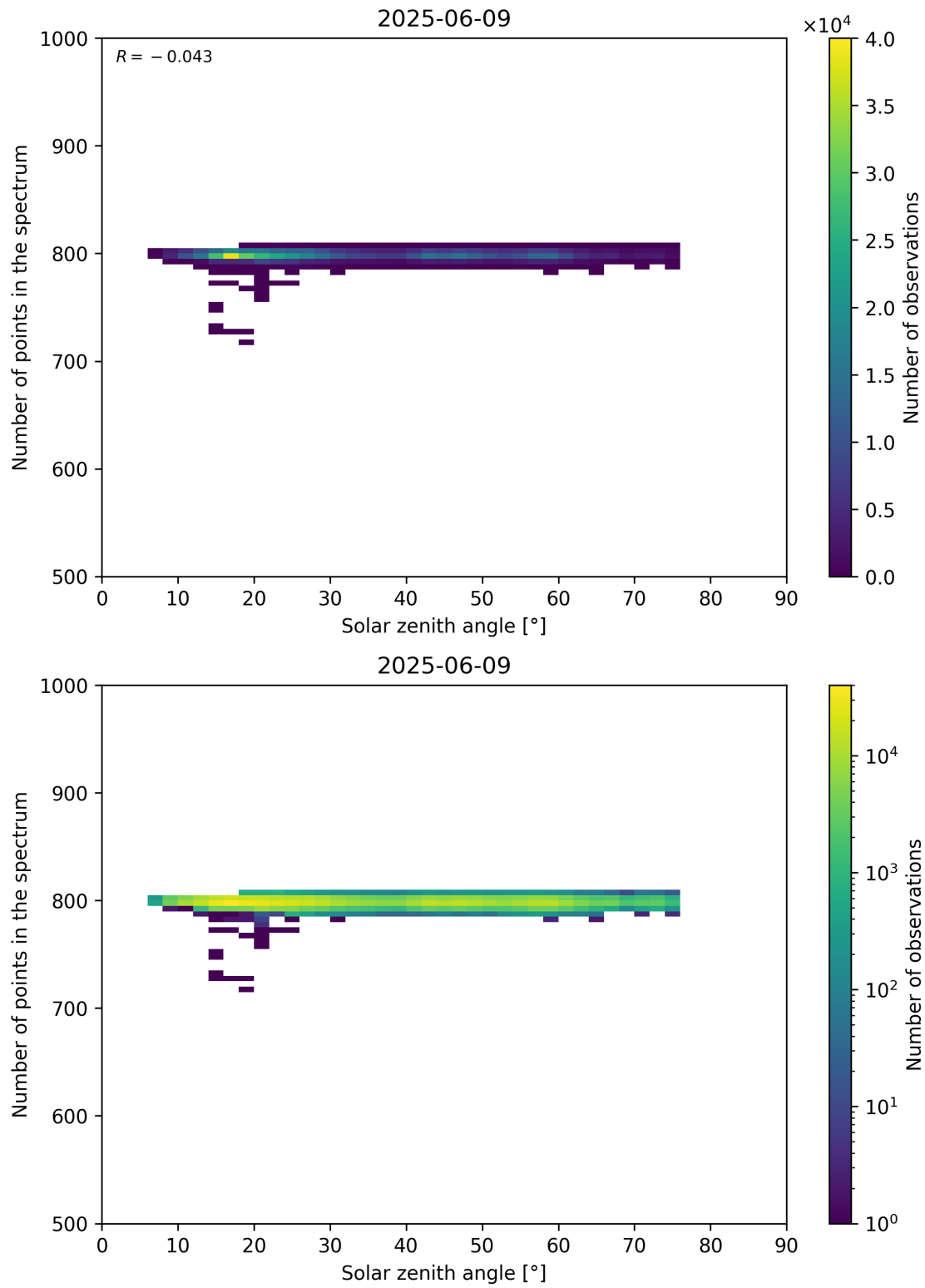
Figure 103: Scatter density plot of “Solar zenith angle” against “Number of points in the spectrum” for 2025-06-08 to 2025-06-10.
