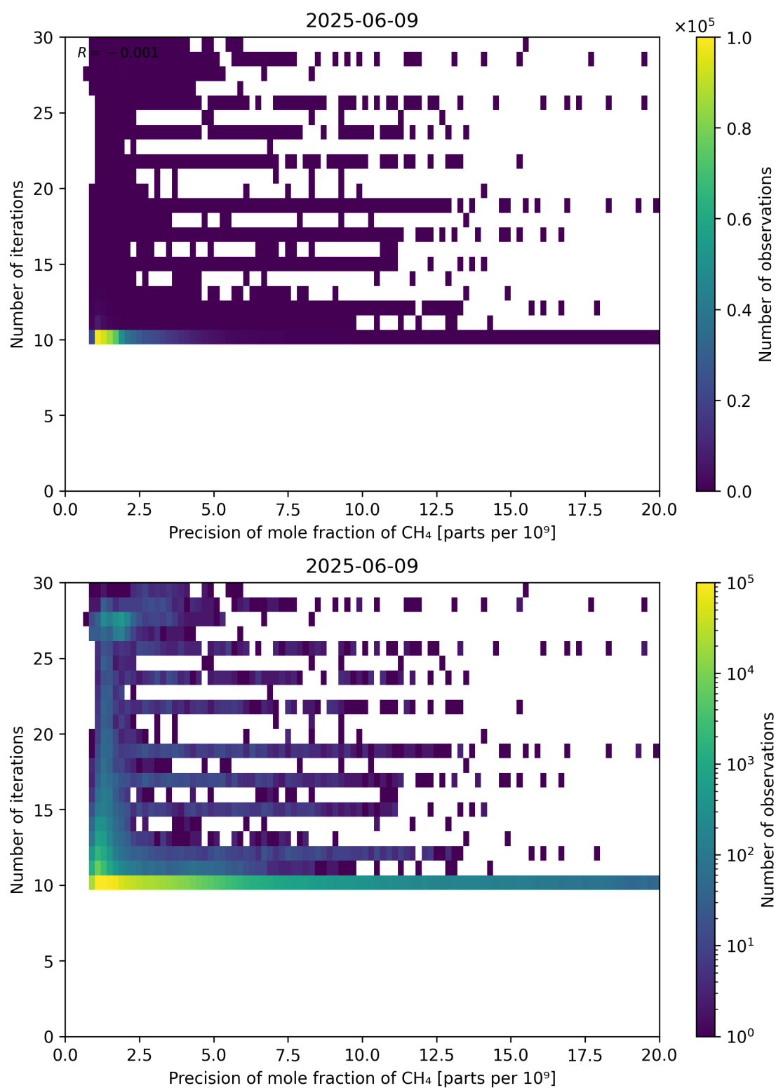
Figure 83: Scatter density plot of “Precision of mole fraction of CH 4 ” against “Number of iterations” for 2025-06-08 to 2025-06-10.
