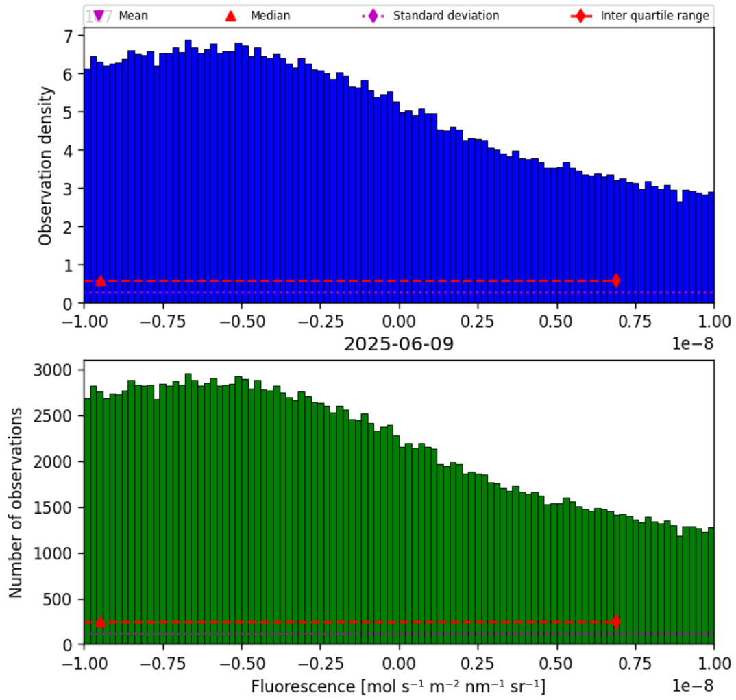
Figure 32: Histogram of “Fluorescence” for 2025-06-08 to 2025-06-10
