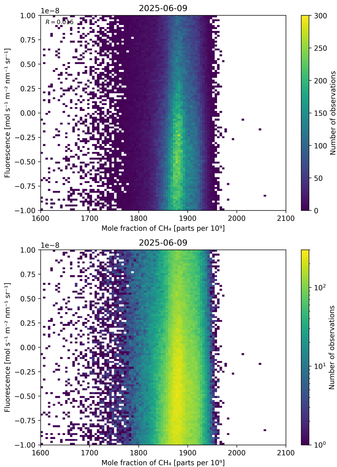
Figure 73: Scatter density plot of “Mole fraction of \text{CH}_4 ” against “Fluorescence” for 2025-06-08 to 2025-06-10.
