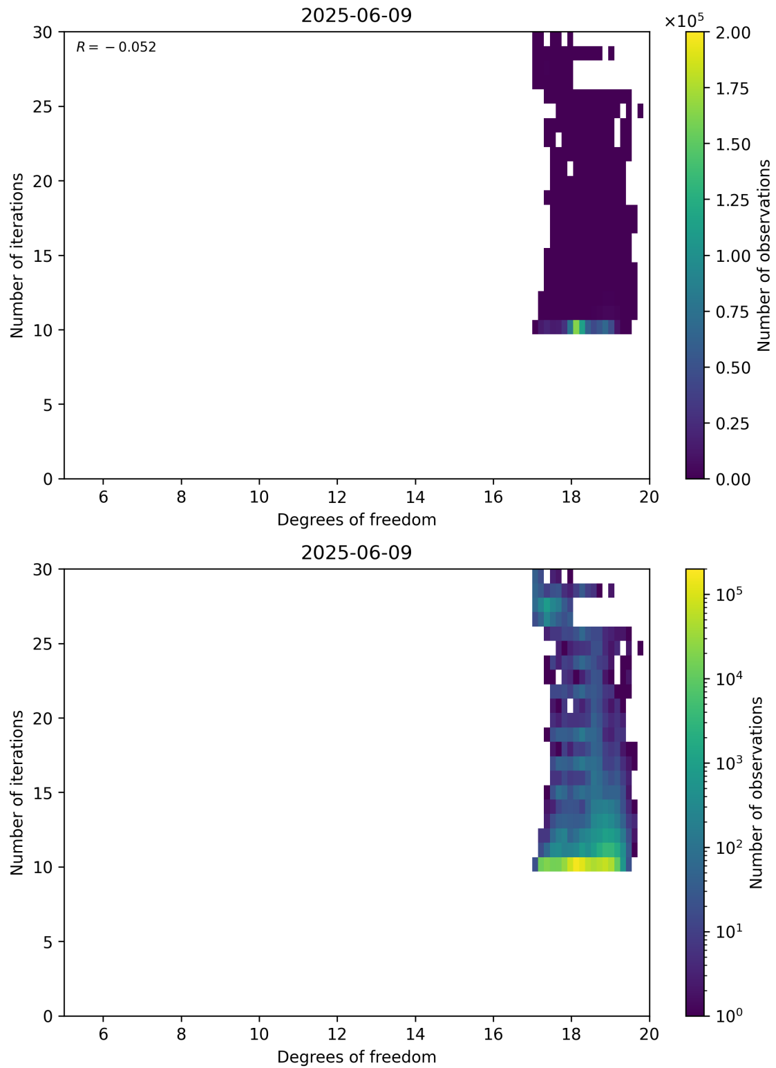
Figure 52: Scatter density plot of “Degrees of freedom” against “Number of iterations” for 2025-06-08 to 2025-06-10.
