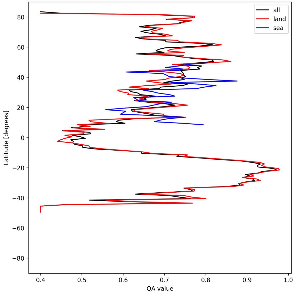
Figure 11: Zonal average of “QA value” for 2025-06-08 to 2025-06-10.
