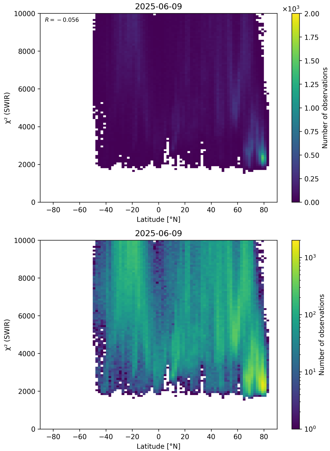
Figure 54: Scatter density plot of “Latitude” against “ \chi^2 (SWIR)” for 2025-06-08 to 2025-06-10.
