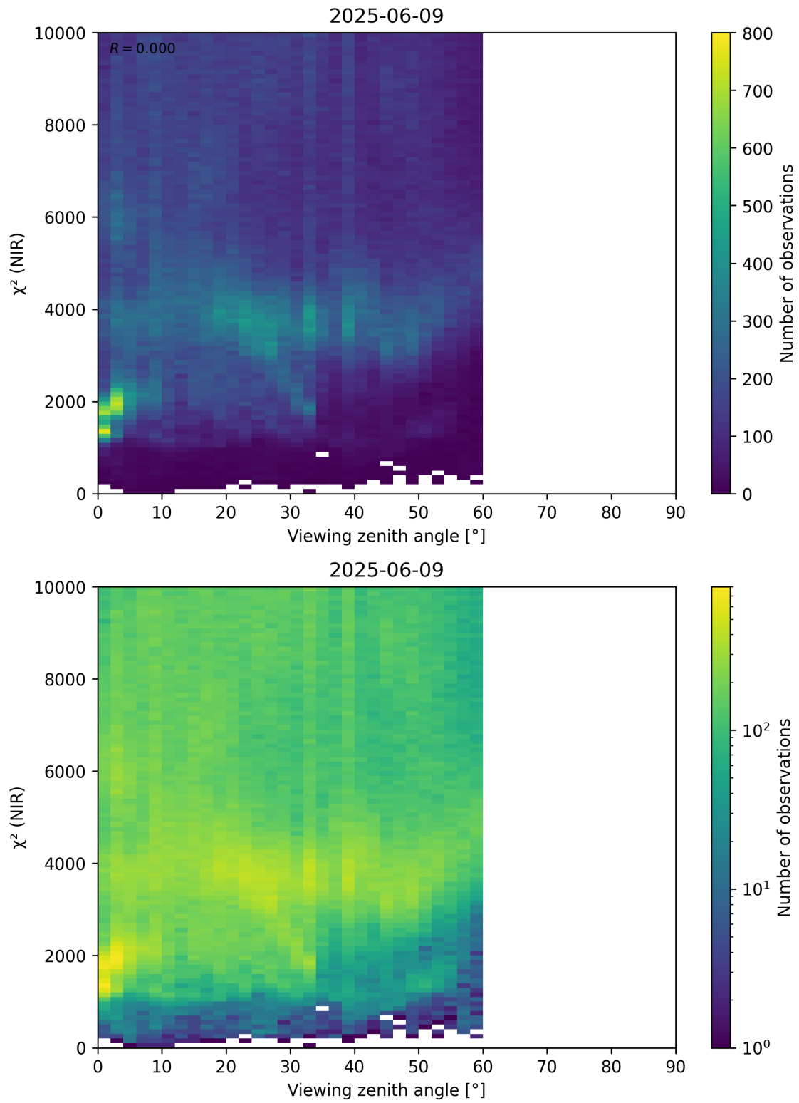
Figure 105: Scatter density plot of “Viewing zenith angle” against “ \chi^2 (NIR)” for 2025-06-08 to 2025-06-10.
