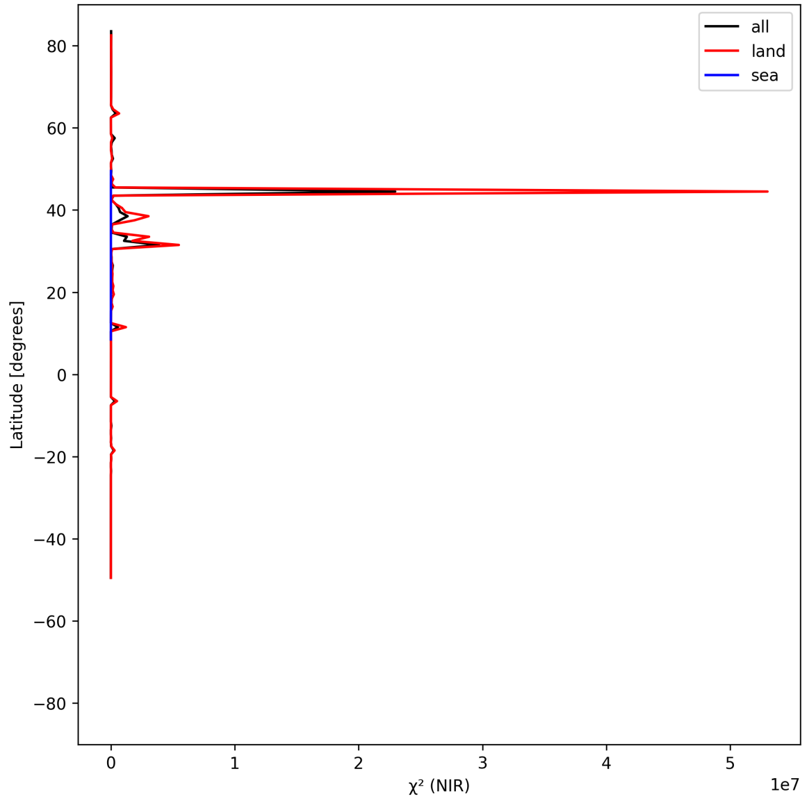
Figure 18: Zonal average of “ \chi^2 (NIR)” for 2025-06-08 to 2025-06-10.
