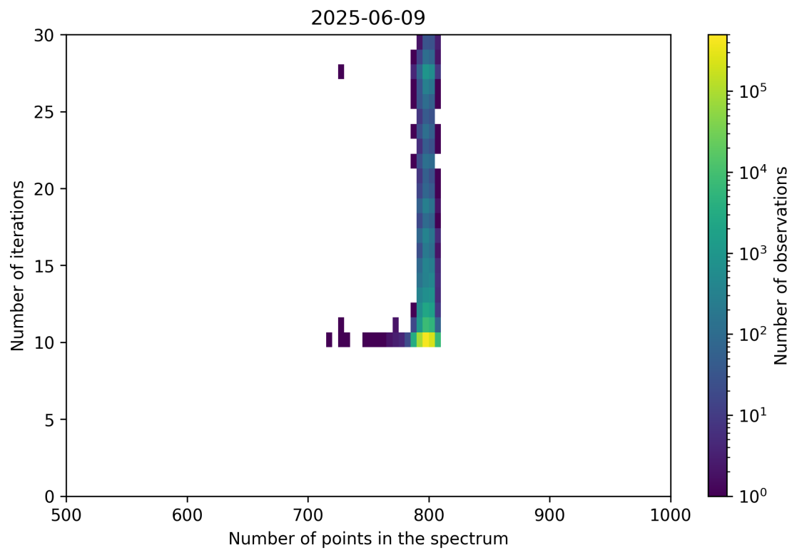
Figure 92: Scatter density plot of “Number of points in the spectrum” against “Number of iterations” for 2025-06-08 to 2025-06-10.
