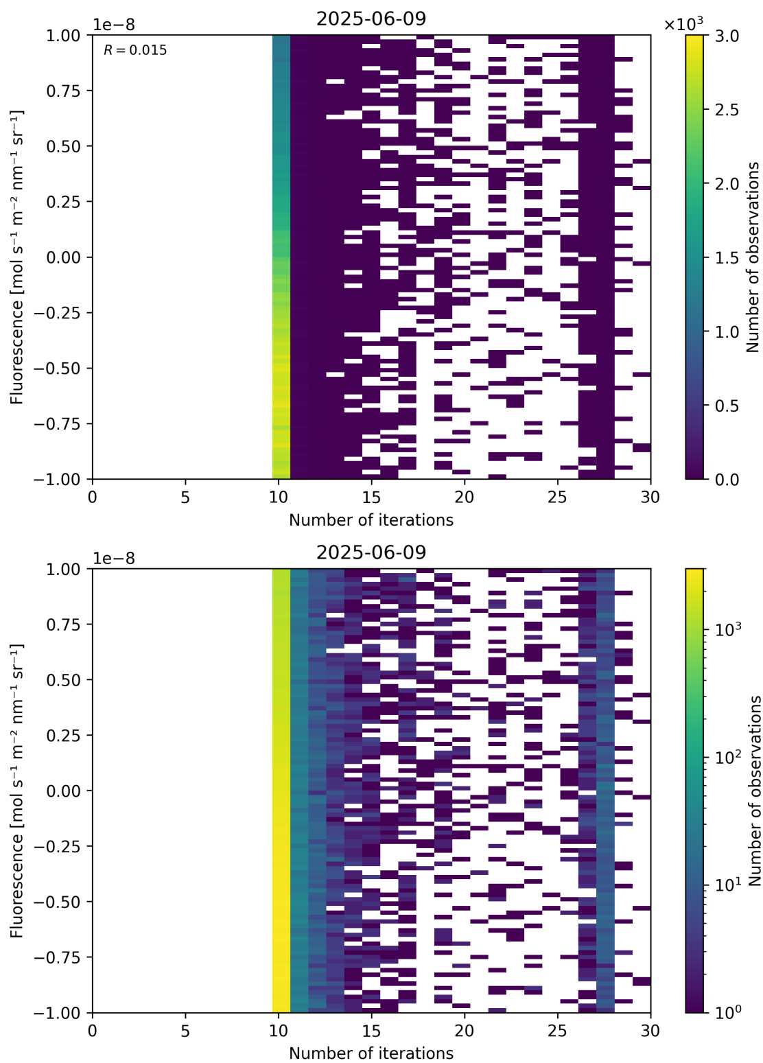
Figure 87: Scatter density plot of “Number of iterations” against “Fluorescence” for 2025-06-08 to 2025-06-10.
