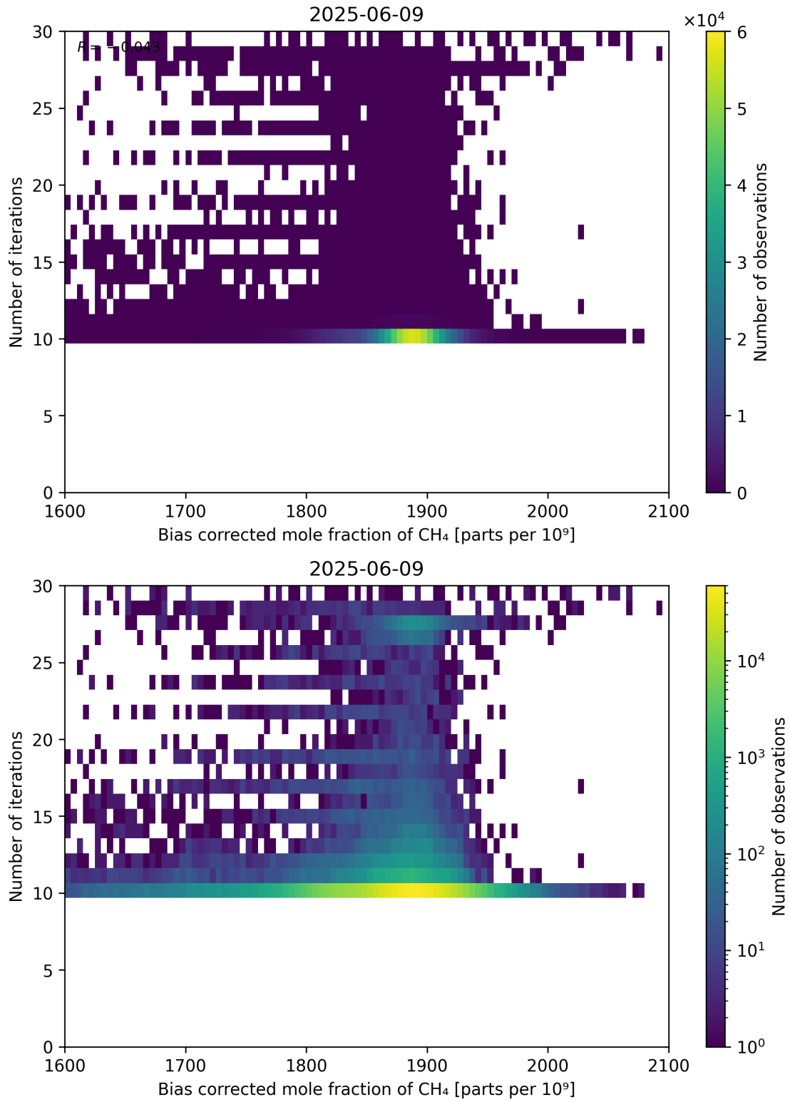
Figure 67: Scatter density plot of “Bias corrected mole fraction of CH 4 ” against “Number of iterations” for 2025-06-08 to 2025-06-10.
