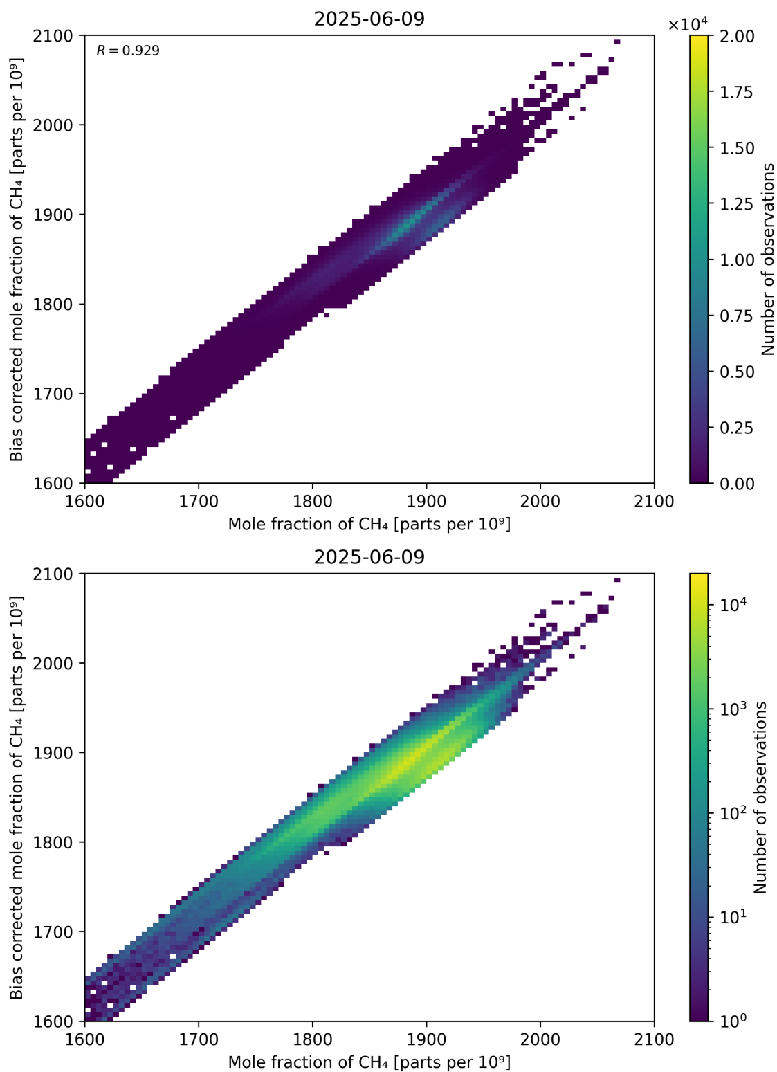
Figure 74: Scatter density plot of “Mole fraction of CH 4 ” against “Bias corrected mole fraction of CH 4 ” for 2025-06-08 to 2025-06-10.
