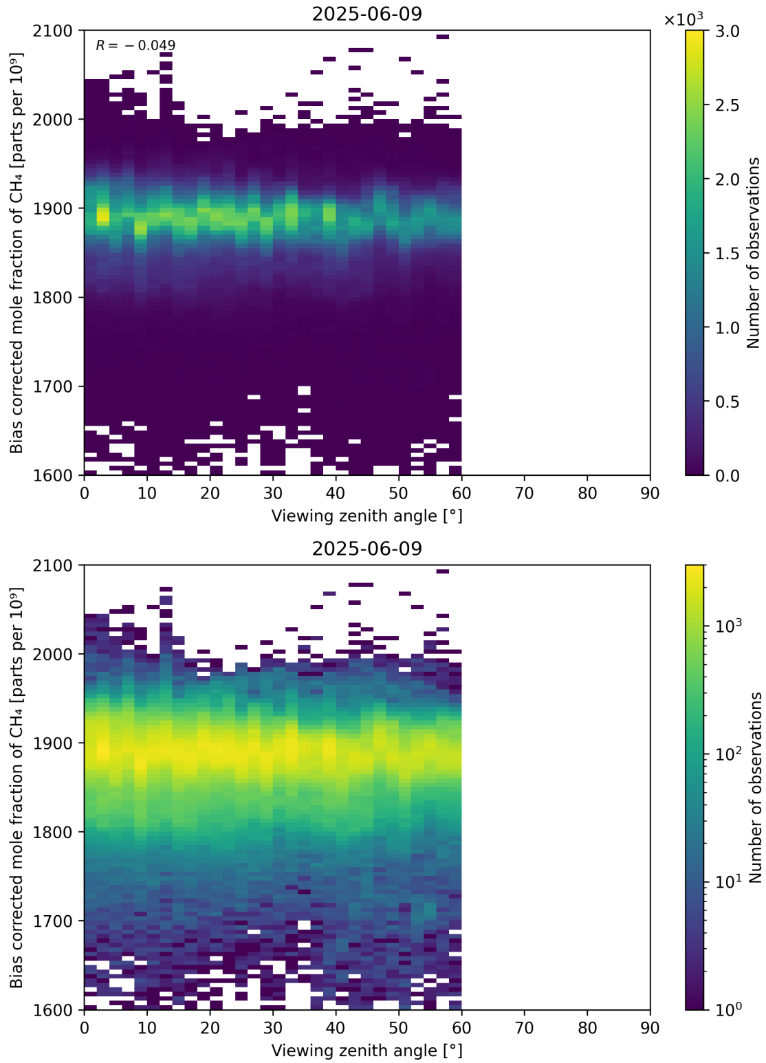
Figure 111: Scatter density plot of “Viewing zenith angle” against “Bias corrected mole fraction of CH 4 ” for 2025-06-08 to 2025-06-10.
