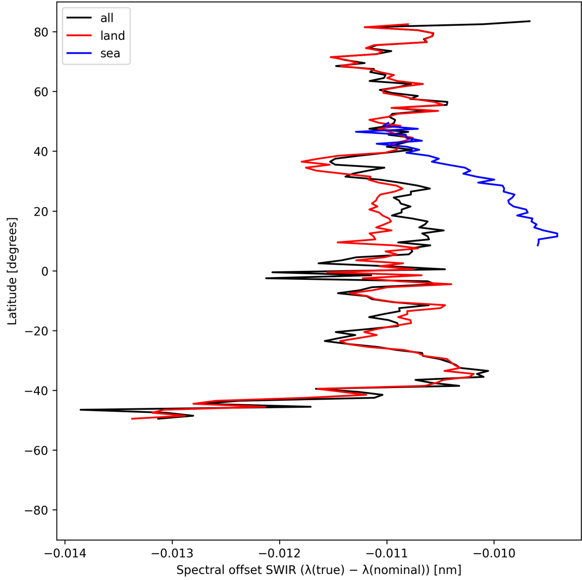
Figure 16: Zonal average of “Spectral offset SWIR ( \lambda_{\text{true}} - \lambda_{\text{nominal}} )” for 2025-06-08 to 2025-06-10.
