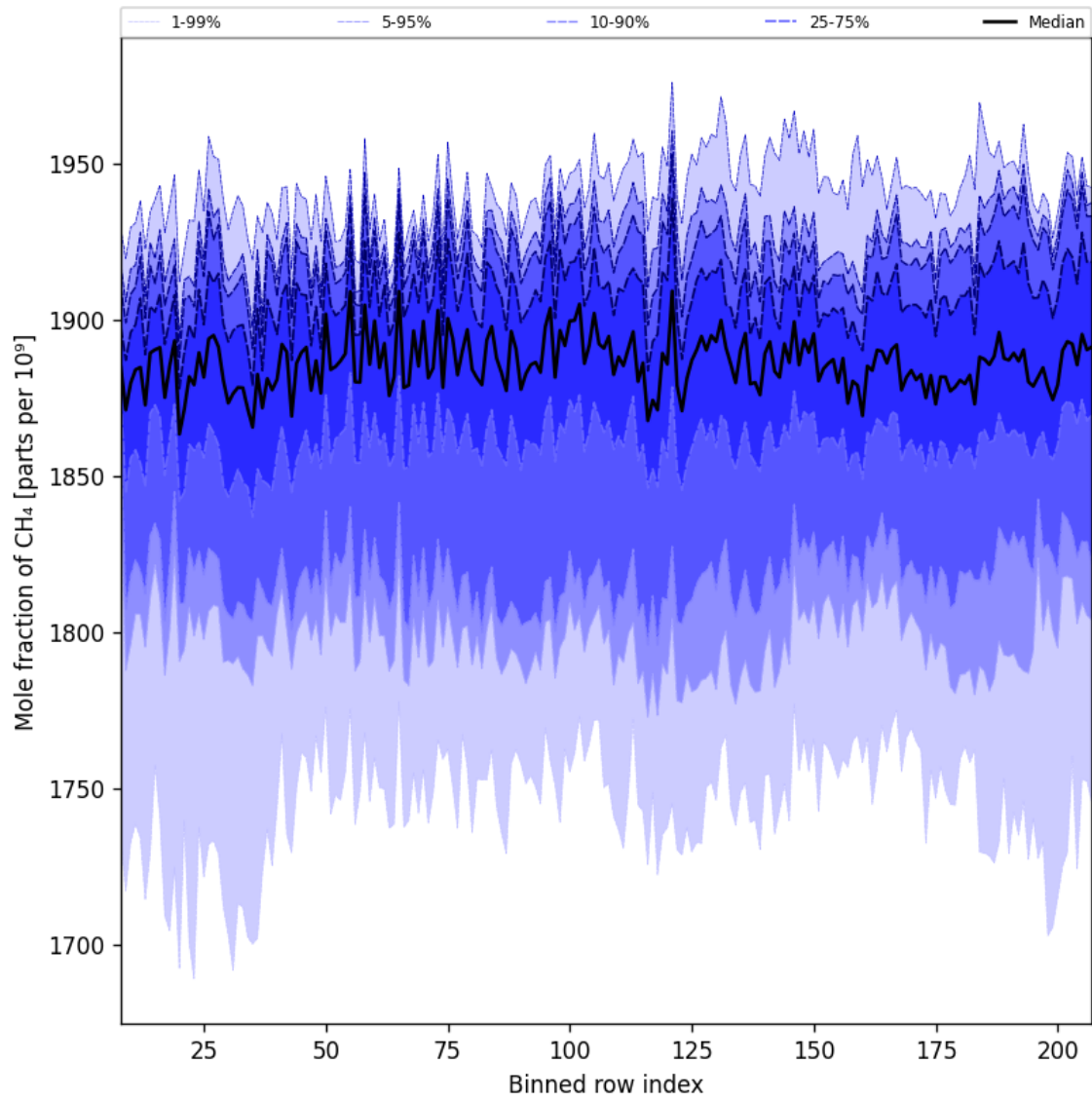
Figure 34: Along track statistics of “Mole fraction of CH 4 ” for 2025-06-08 to 2025-06-10
