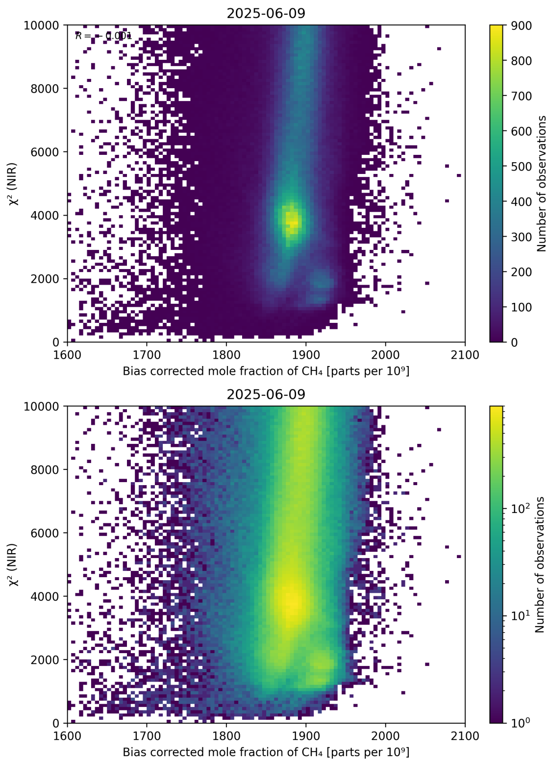
Figure 63: Scatter density plot of “Bias corrected mole fraction of CH 4 ” against “ \chi^2 (NIR)” for 2025-06-08 to 2025-06-10.
