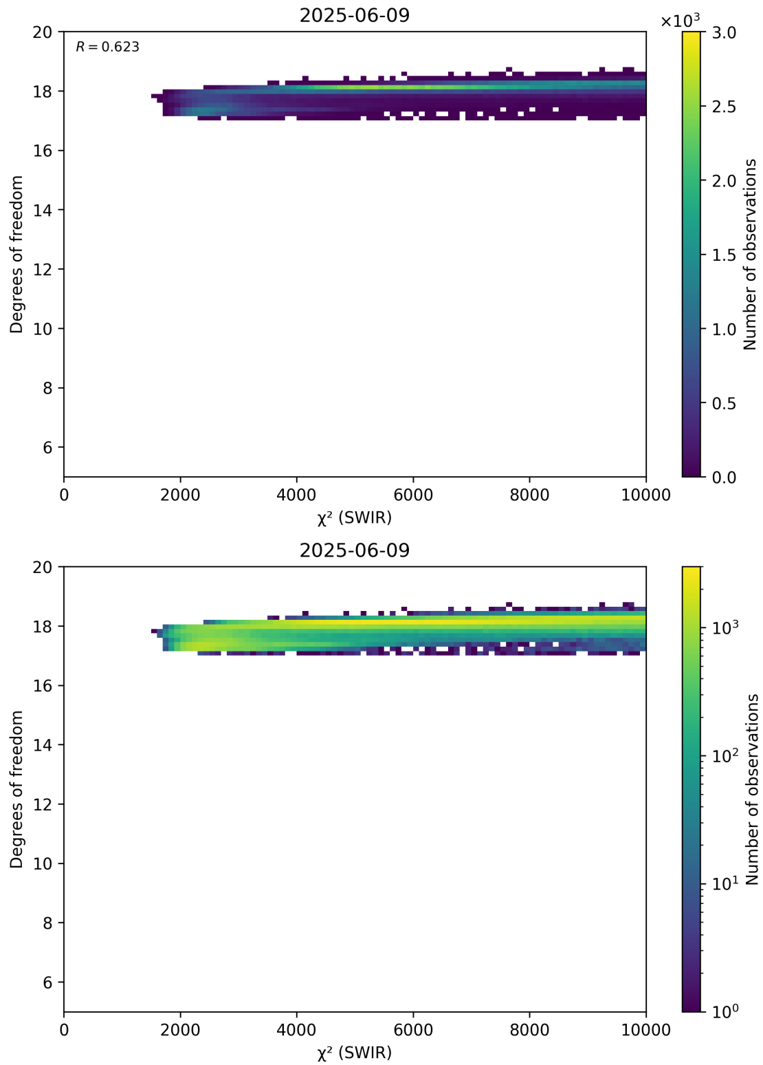
Figure 48: Scatter density plot of “ \chi^2 (SWIR)” against “Degrees of freedom” for 2025-06-08 to 2025-06-10.
