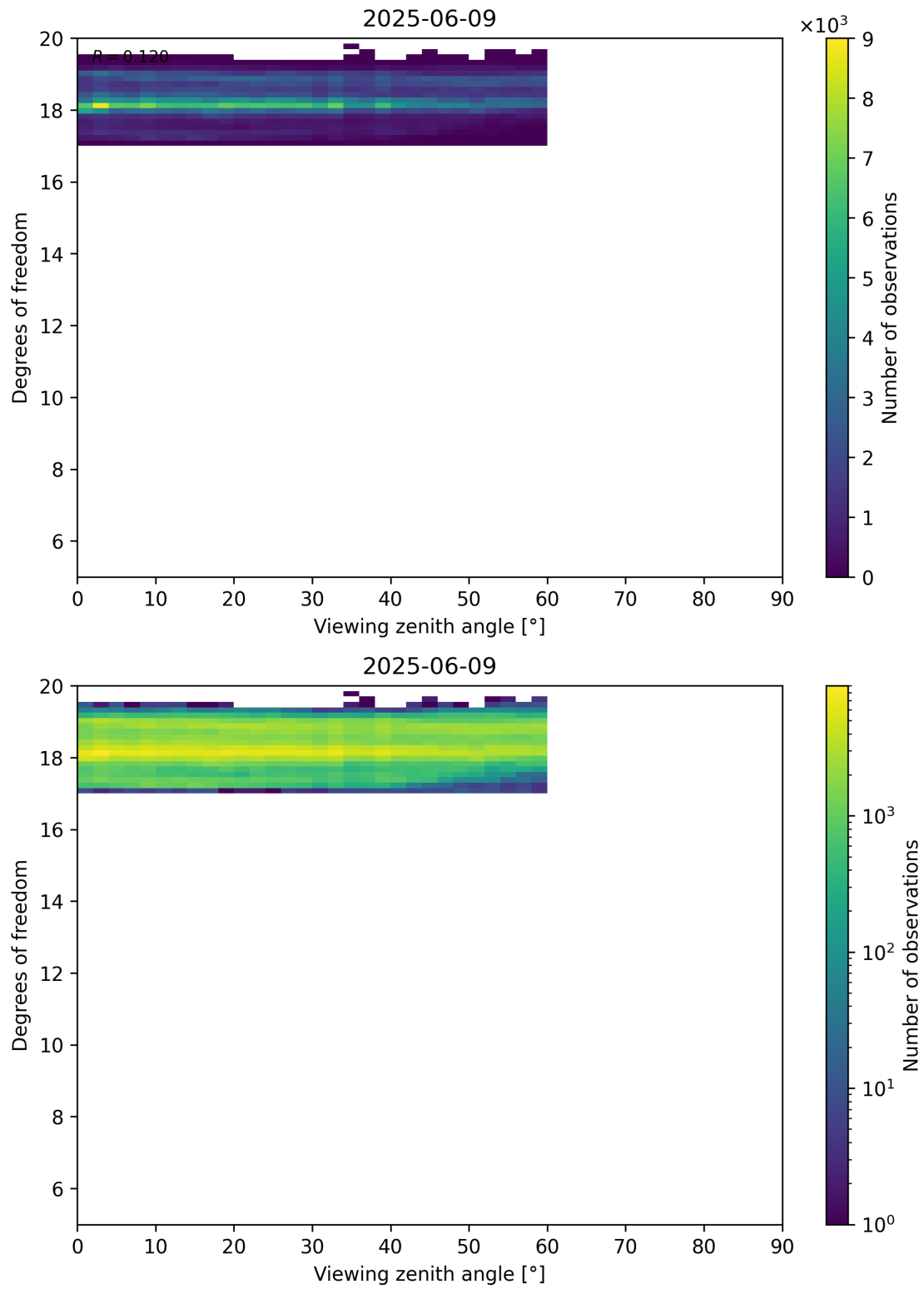
Figure 107: Scatter density plot of “Viewing zenith angle” against “Degrees of freedom” for 2025-06-08 to 2025-06-10.
