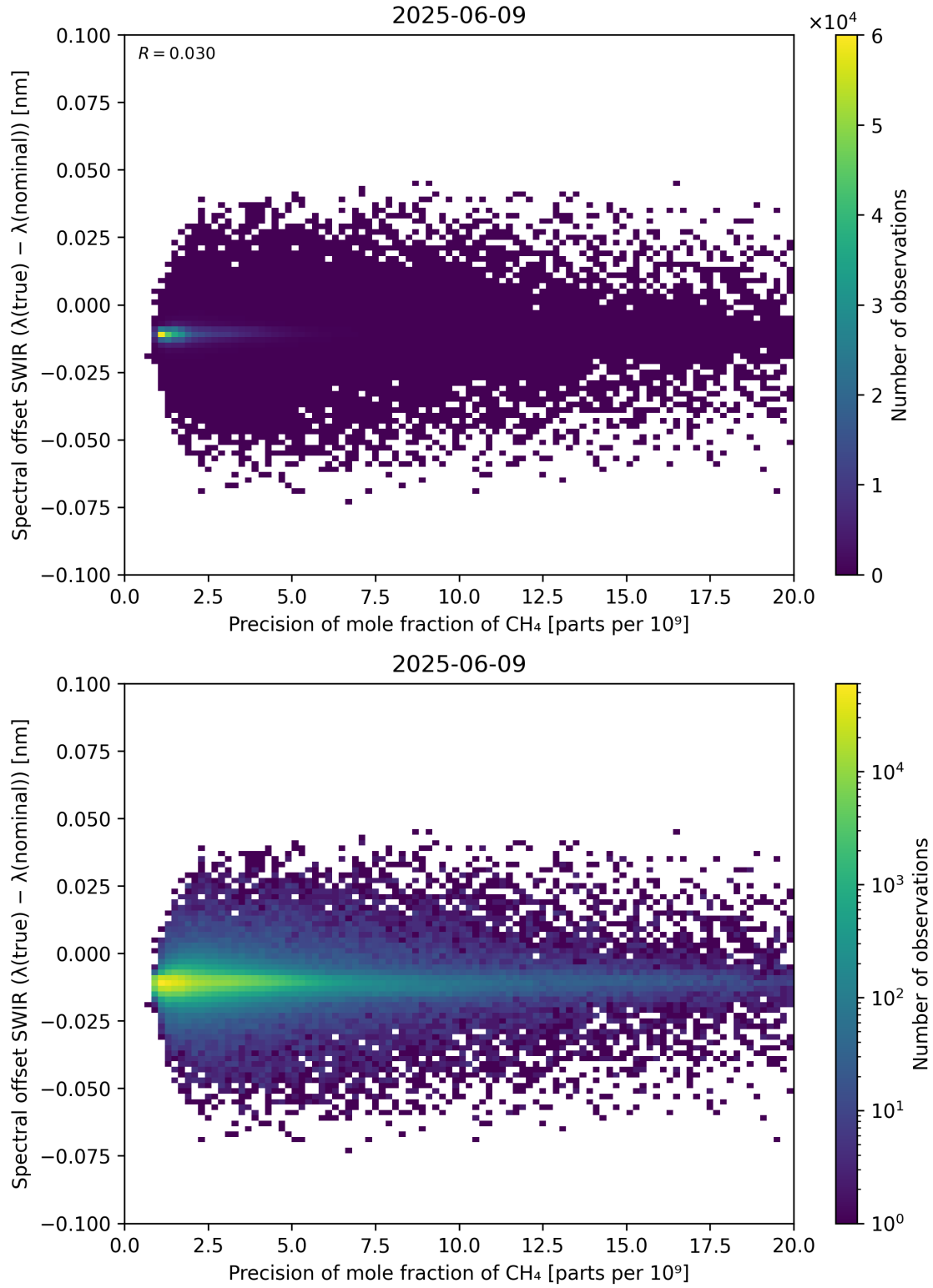
Figure 85: Scatter density plot of “Precision of mole fraction of CH 4 ” against “Spectral offset SWIR ( \lambda_{\text{true}} - \lambda_{\text{nominal}} )” for 2025-06-08 to 2025-06-10.
