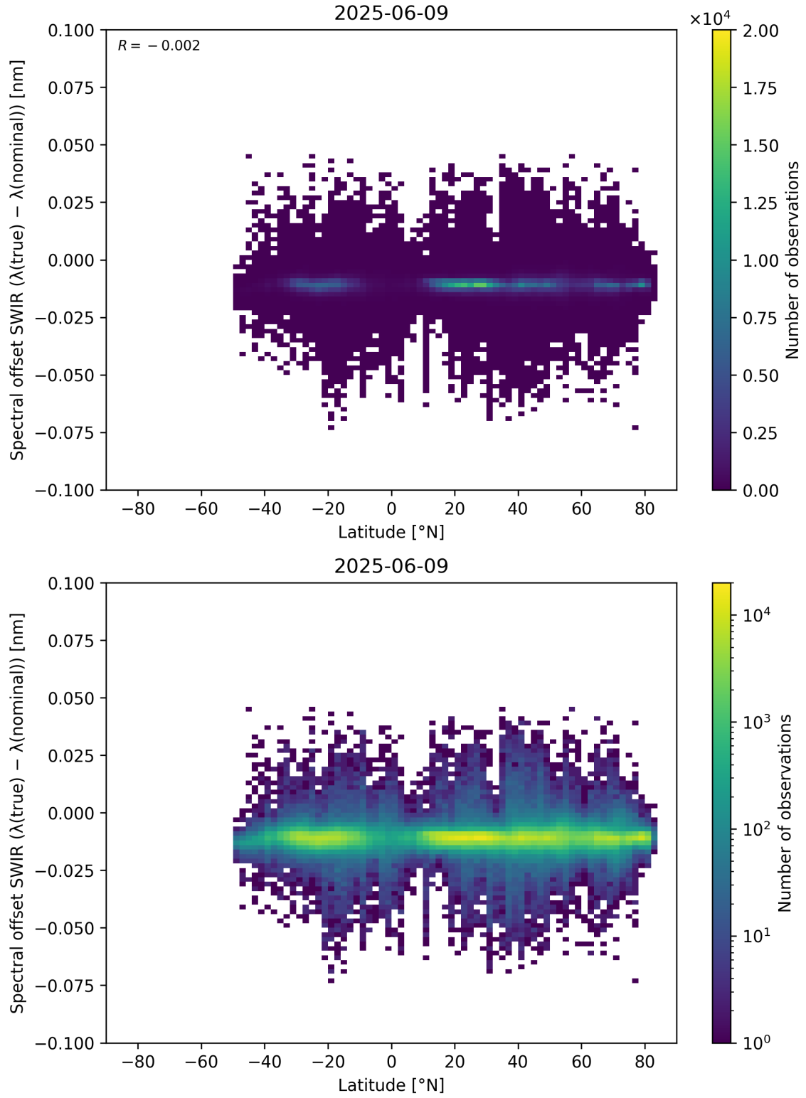
Figure 62: Scatter density plot of “Latitude” against “Spectral offset SWIR ( \lambda_{\text{true}} - \lambda_{\text{nominal}} )” for 2025-06-08 to 2025-06-10.
