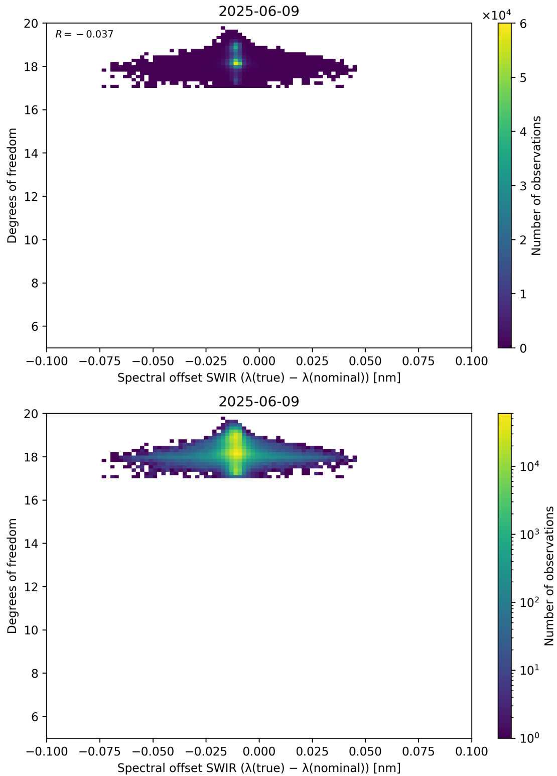
Figure 119: Scatter density plot of “Spectral offset SWIR ( \lambda_{\text{true}} - \lambda_{\text{nominal}} )” against “Degrees of freedom” for 2025-06-08 to 2025-06-10.
