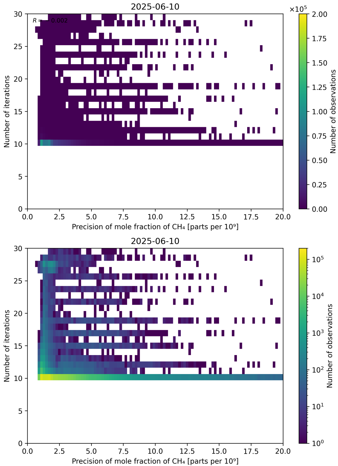
Figure 83: Scatter density plot of “Precision of mole fraction of CH 4 ” against “Number of iterations” for 2025-06-09 to 2025-06-11.
