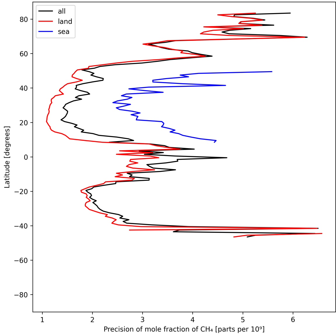
Figure 13: Zonal average of “Precision of mole fraction of CH 4 ” for 2025-06-09 to 2025-06-11.
