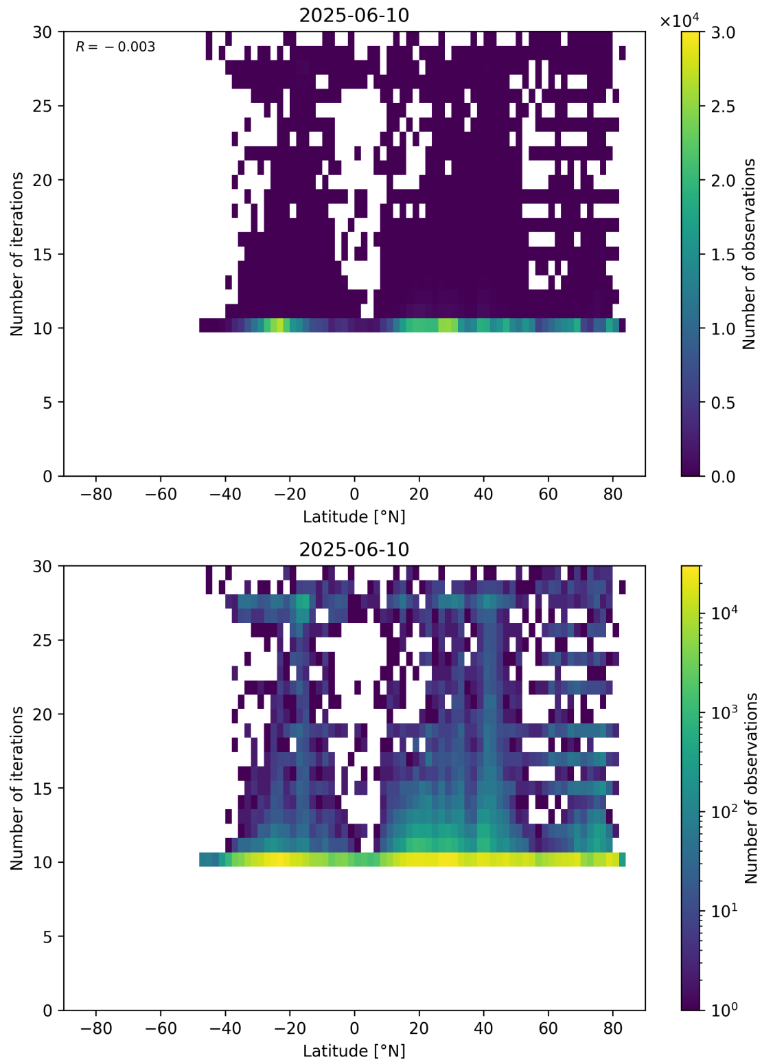
Figure 60: Scatter density plot of “Latitude” against “Number of iterations” for 2025-06-09 to 2025-06-11.
