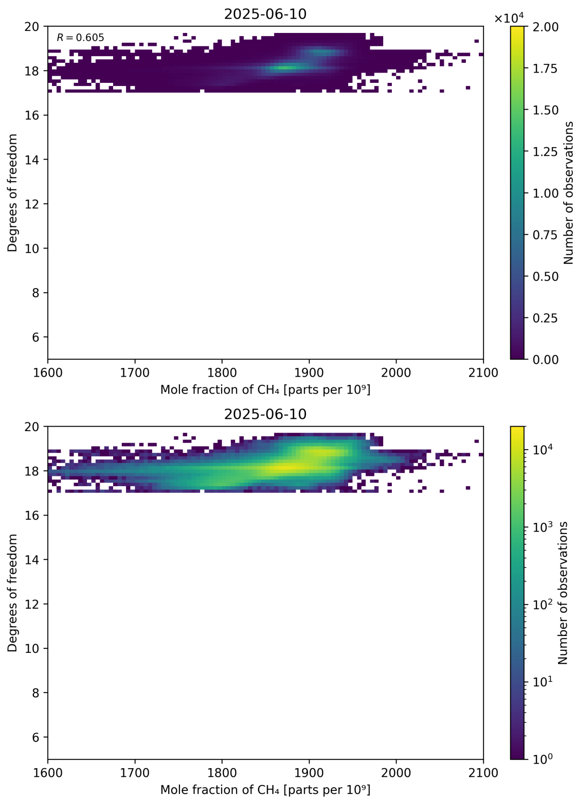
Figure 72: Scatter density plot of “Mole fraction of CH 4 ” against “Degrees of freedom” for 2025-06-09 to 2025-06-11.
