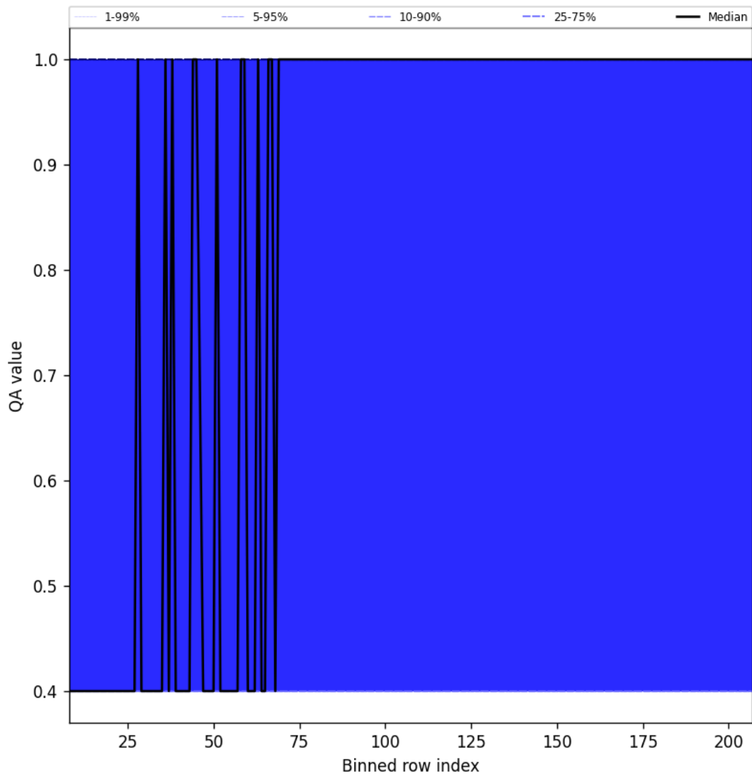
Figure 33: Along track statistics of “QA value” for 2025-06-09 to 2025-06-11
