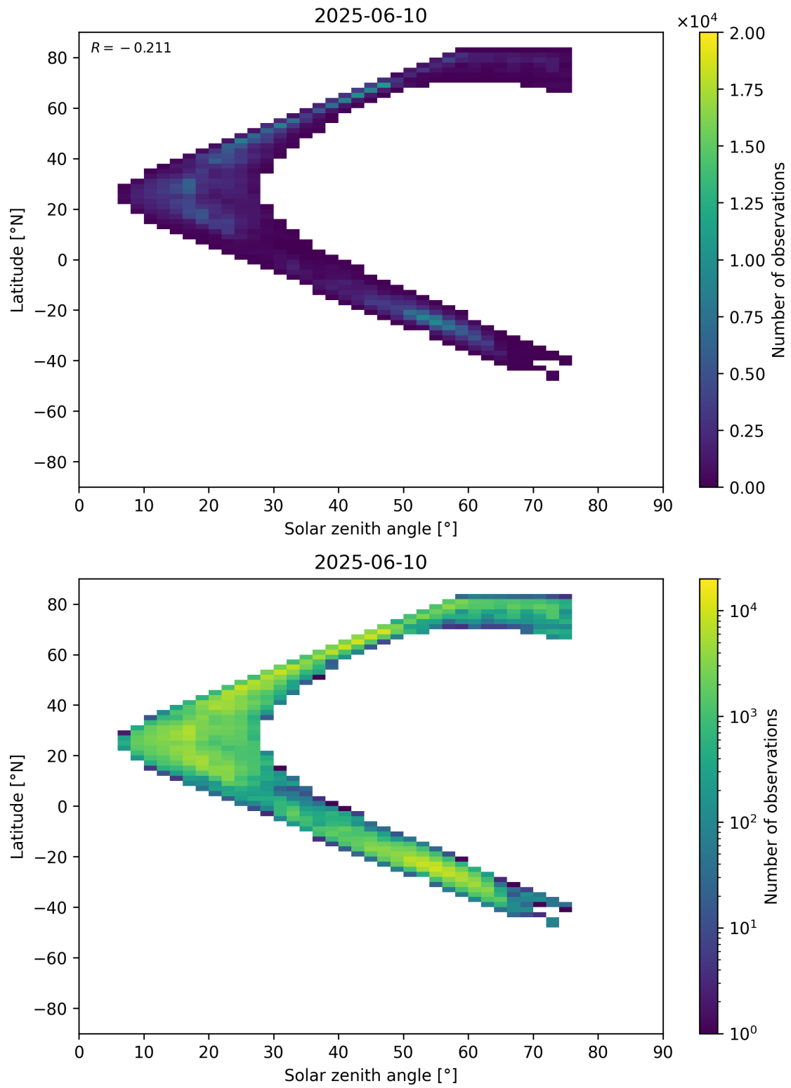
Figure 98: Scatter density plot of “Solar zenith angle” against “Latitude” for 2025-06-09 to 2025-06-11.
