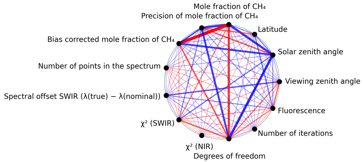
Figure 1: Map of correlation graph for 2025-06-09 to 2025-06-11.
