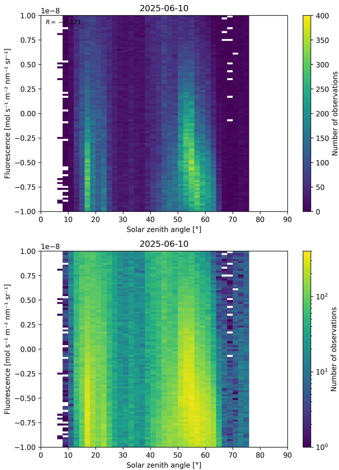
Figure 97: Scatter density plot of “Solar zenith angle” against “Fluorescence” for 2025-06-09 to 2025-06-11.
