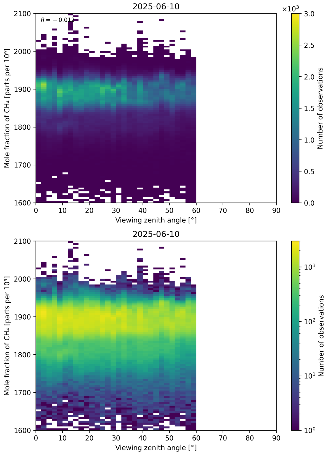
Figure 110: Scatter density plot of “Viewing zenith angle” against “Mole fraction of CH 4 ” for 2025-06-09 to 2025-06-11.
