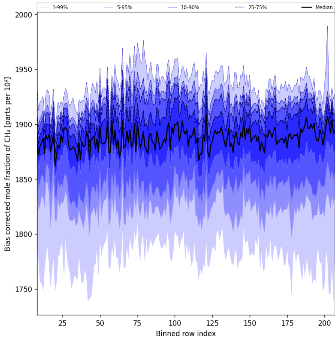
Figure 36: Along track statistics of “Bias corrected mole fraction of CH 4 ” for 2025-06-09 to 2025-06-11
