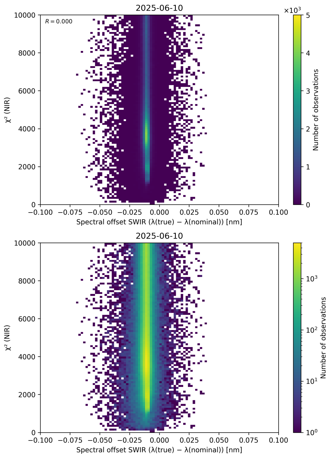
Figure 117: Scatter density plot of “Spectral offset SWIR ( \lambda_{\text{true}} - \lambda_{\text{nominal}} )” against “ \chi^2 (NIR)” for 2025-06-09 to 2025-06-11.
