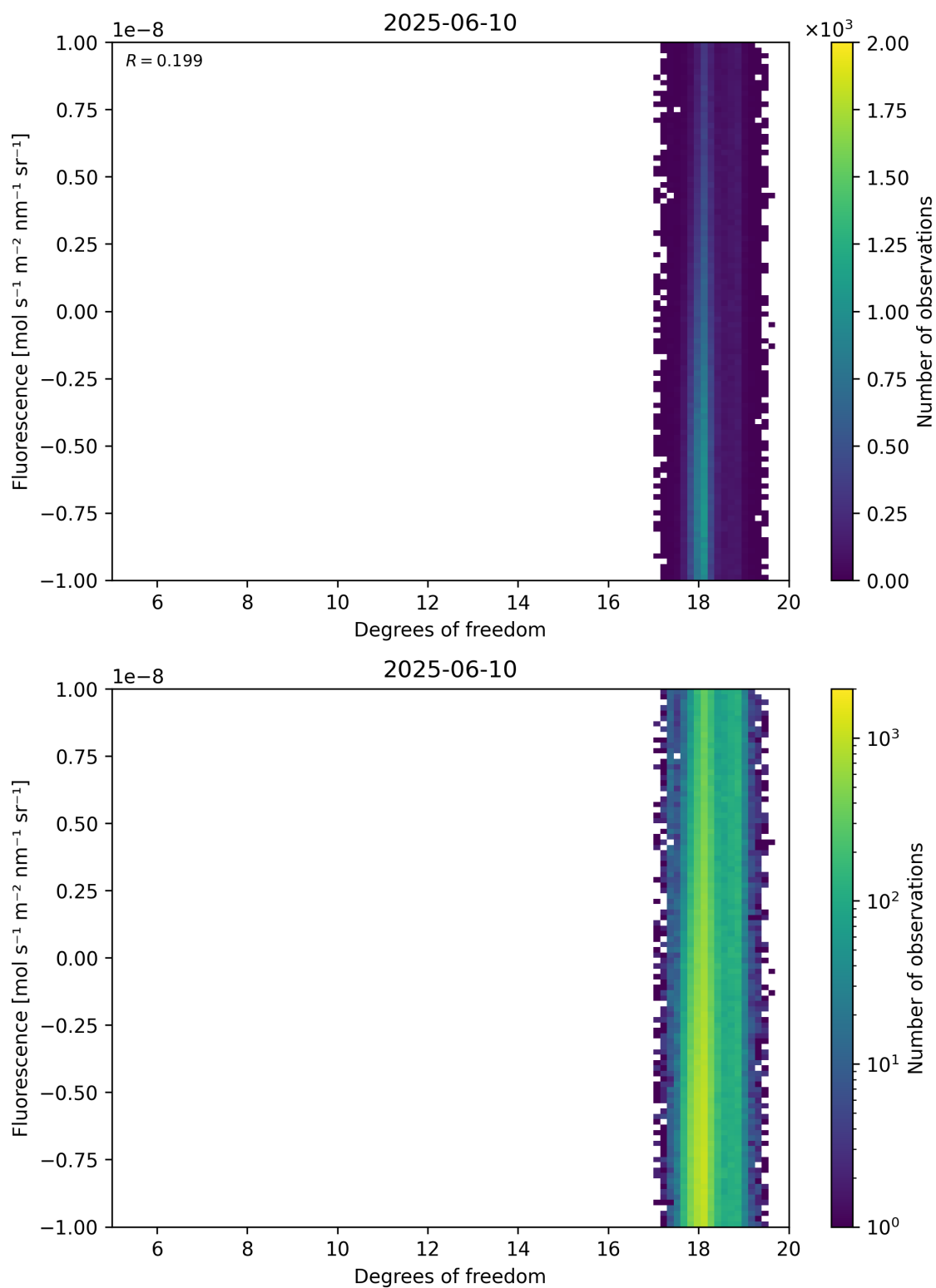
Figure 51: Scatter density plot of “Degrees of freedom” against “Fluorescence” for 2025-06-09 to 2025-06-11.
