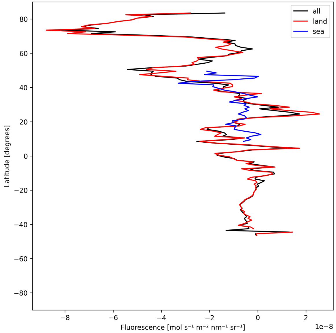
Figure 21: Zonal average of “Fluorescence” for 2025-06-09 to 2025-06-11.
