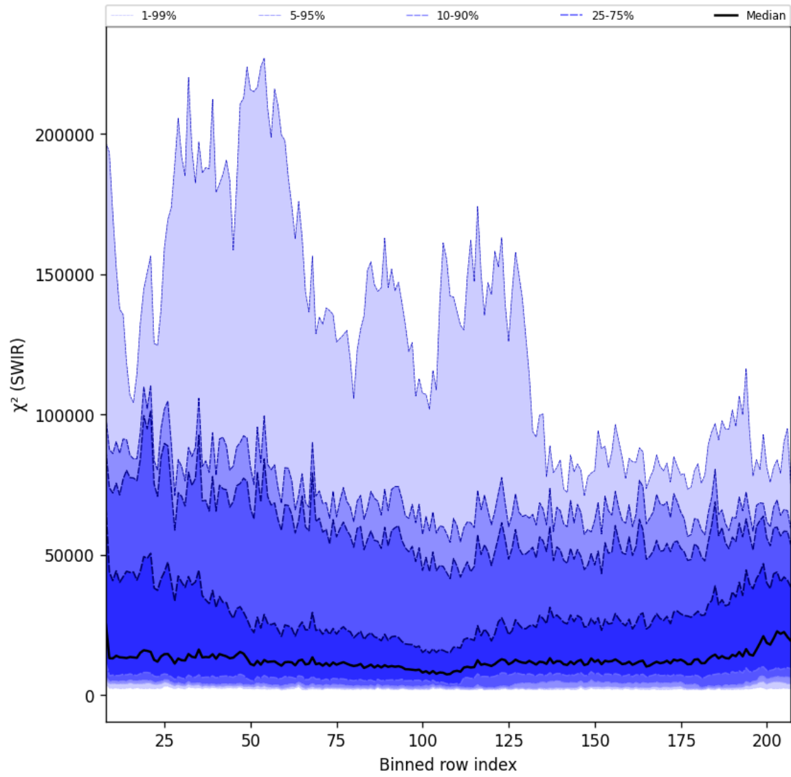
Figure 39: Along track statistics of “ \chi^2 (SWIR)” for 2025-06-09 to 2025-06-11
