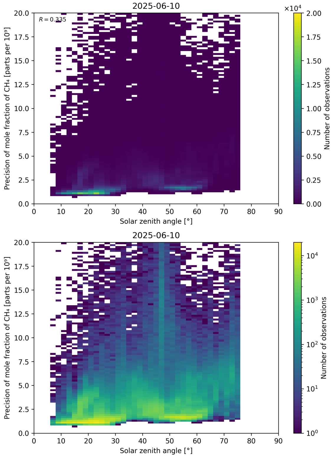
Figure 101: Scatter density plot of “Solar zenith angle” against “Precision of mole fraction of CH 4 ” for 2025-06-09 to 2025-06-11.
