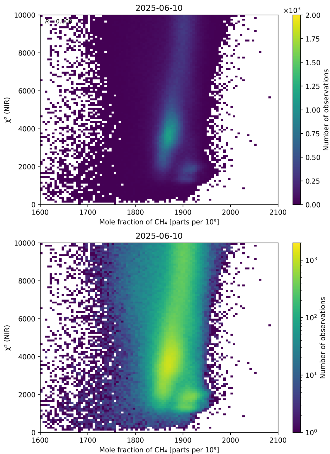
Figure 70: Scatter density plot of “Mole fraction of CH 4 ” against “ \chi^2 (NIR)” for 2025-06-09 to 2025-06-11.
