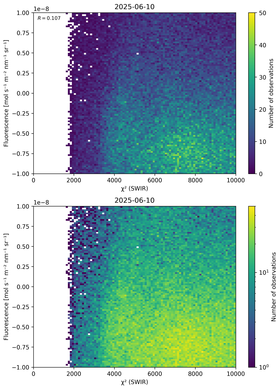
Figure 49: Scatter density plot of “ \chi^2 (SWIR)” against “Fluorescence” for 2025-06-09 to 2025-06-11.
