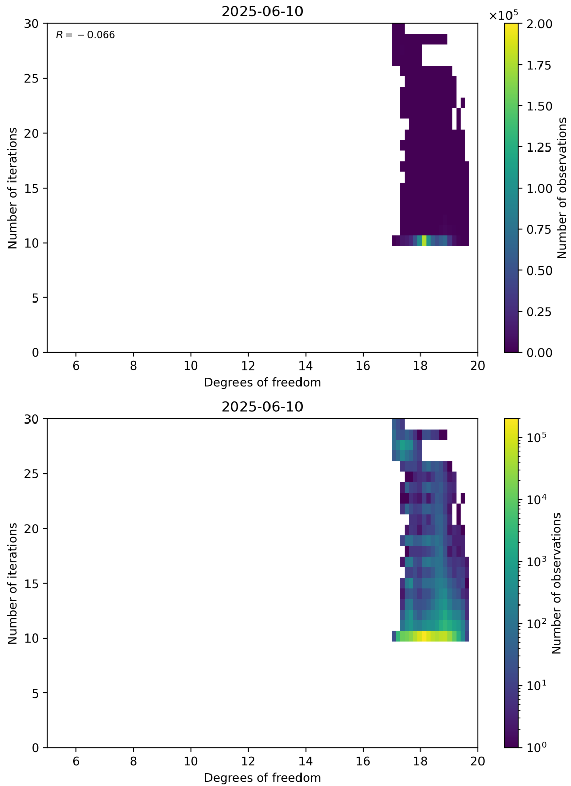
Figure 52: Scatter density plot of “Degrees of freedom” against “Number of iterations” for 2025-06-09 to 2025-06-11.
