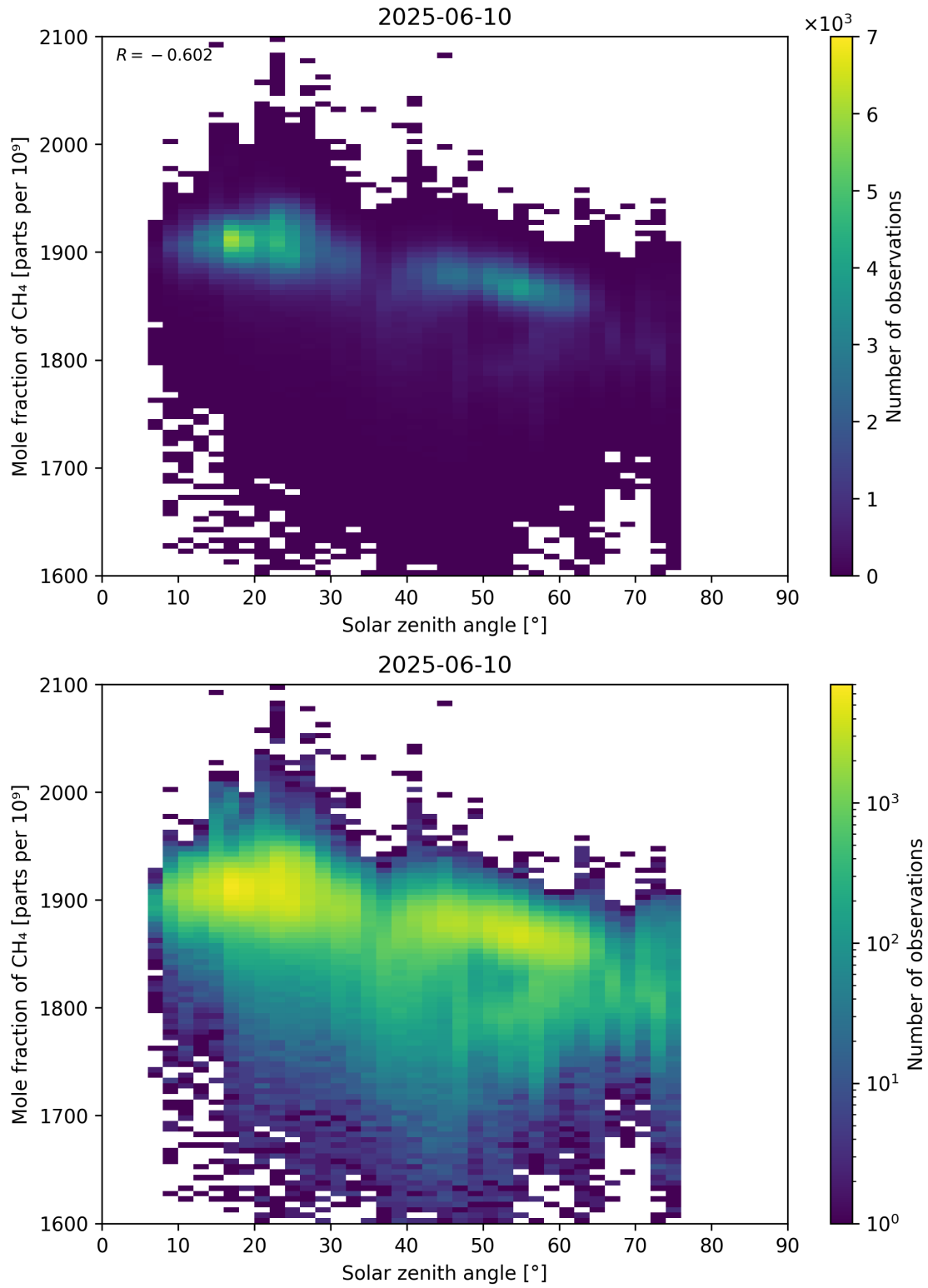
Figure 99: Scatter density plot of “Solar zenith angle” against “Mole fraction of \text{CH}_4 ” for 2025-06-09 to 2025-06-11.
