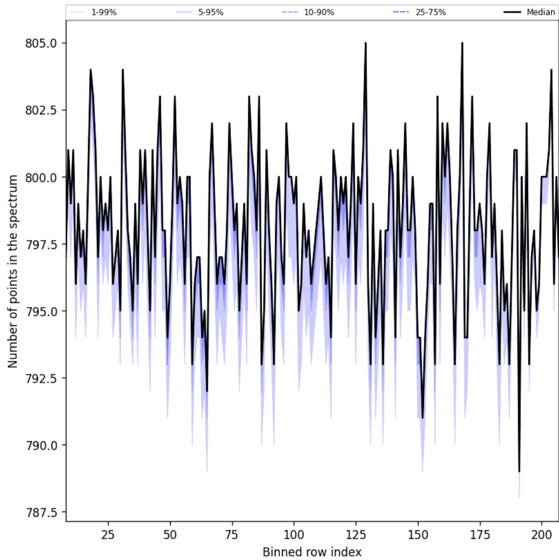
Figure 37: Along track statistics of “Number of points in the spectrum” for 2025-06-09 to 2025-06-11
