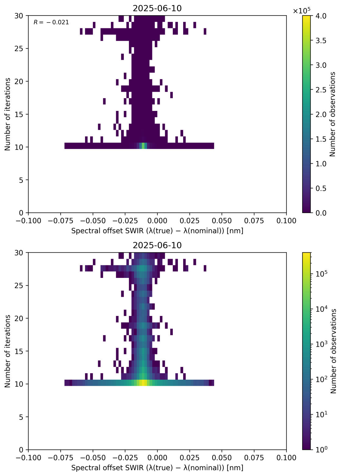
Figure 121: Scatter density plot of “Spectral offset SWIR ( \lambda_{\text{true}} - \lambda_{\text{nominal}} )” against “Number of iterations” for 2025-06-09 to 2025-06-11.
