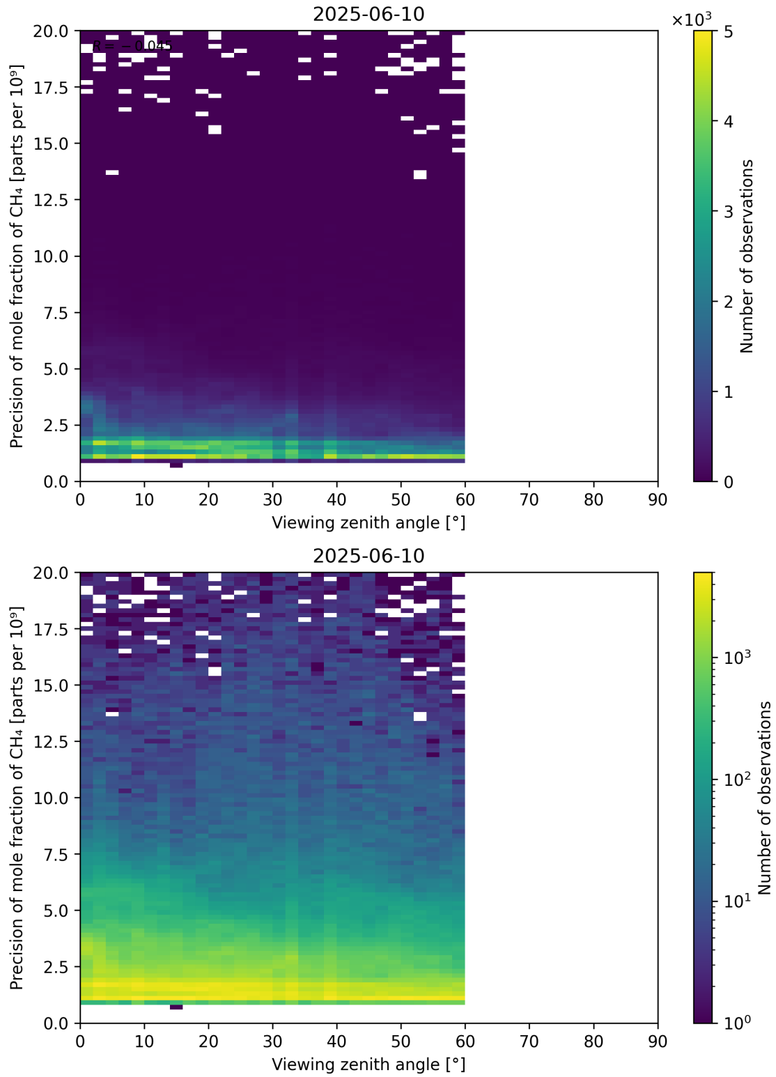
Figure 112: Scatter density plot of “Viewing zenith angle” against “Precision of mole fraction of CH 4 ” for 2025-06-09 to 2025-06-11.
