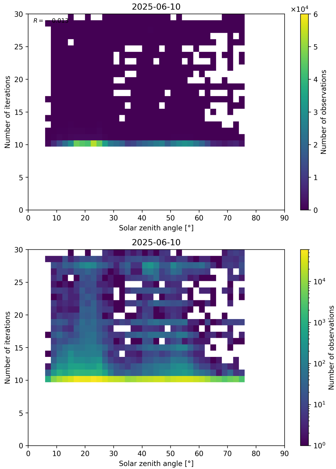
Figure 102: Scatter density plot of “Solar zenith angle” against “Number of iterations” for 2025-06-09 to 2025-06-11.
