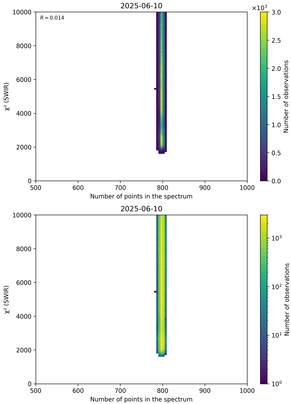
Figure 89: Scatter density plot of “Number of points in the spectrum” against “ \chi^2 (SWIR)” for 2025-06-09 to 2025-06-11.
