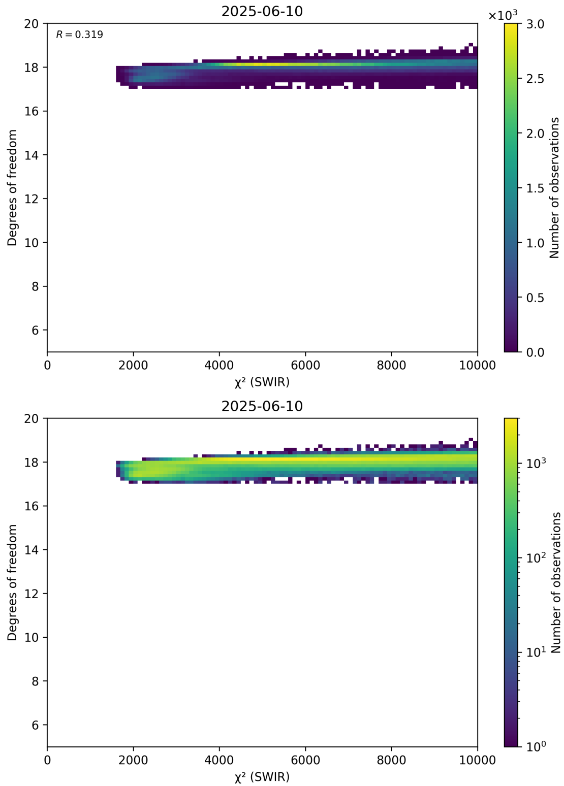
Figure 48: Scatter density plot of “ \chi^2 (SWIR)” against “Degrees of freedom” for 2025-06-09 to 2025-06-11.
