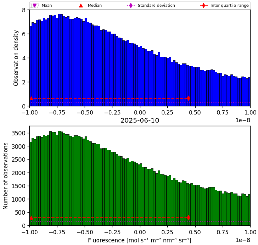
Figure 32: Histogram of “Fluorescence” for 2025-06-09 to 2025-06-11
