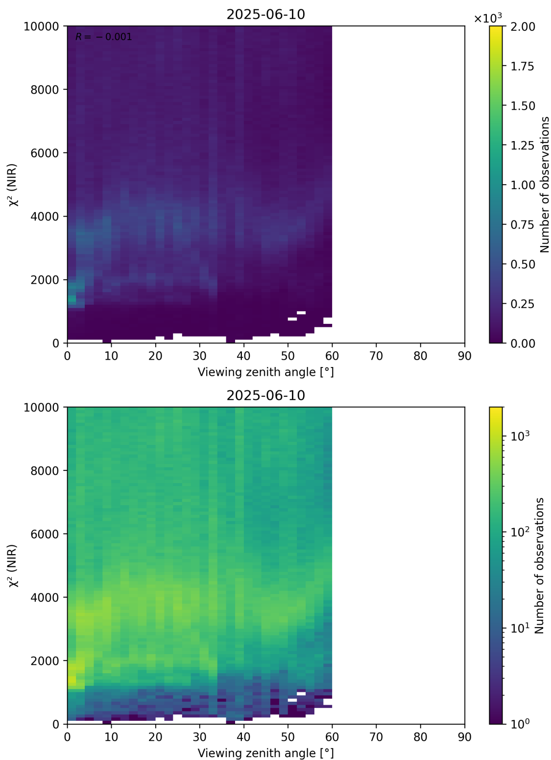
Figure 105: Scatter density plot of “Viewing zenith angle” against “ \chi^2 (NIR)” for 2025-06-09 to 2025-06-11.
