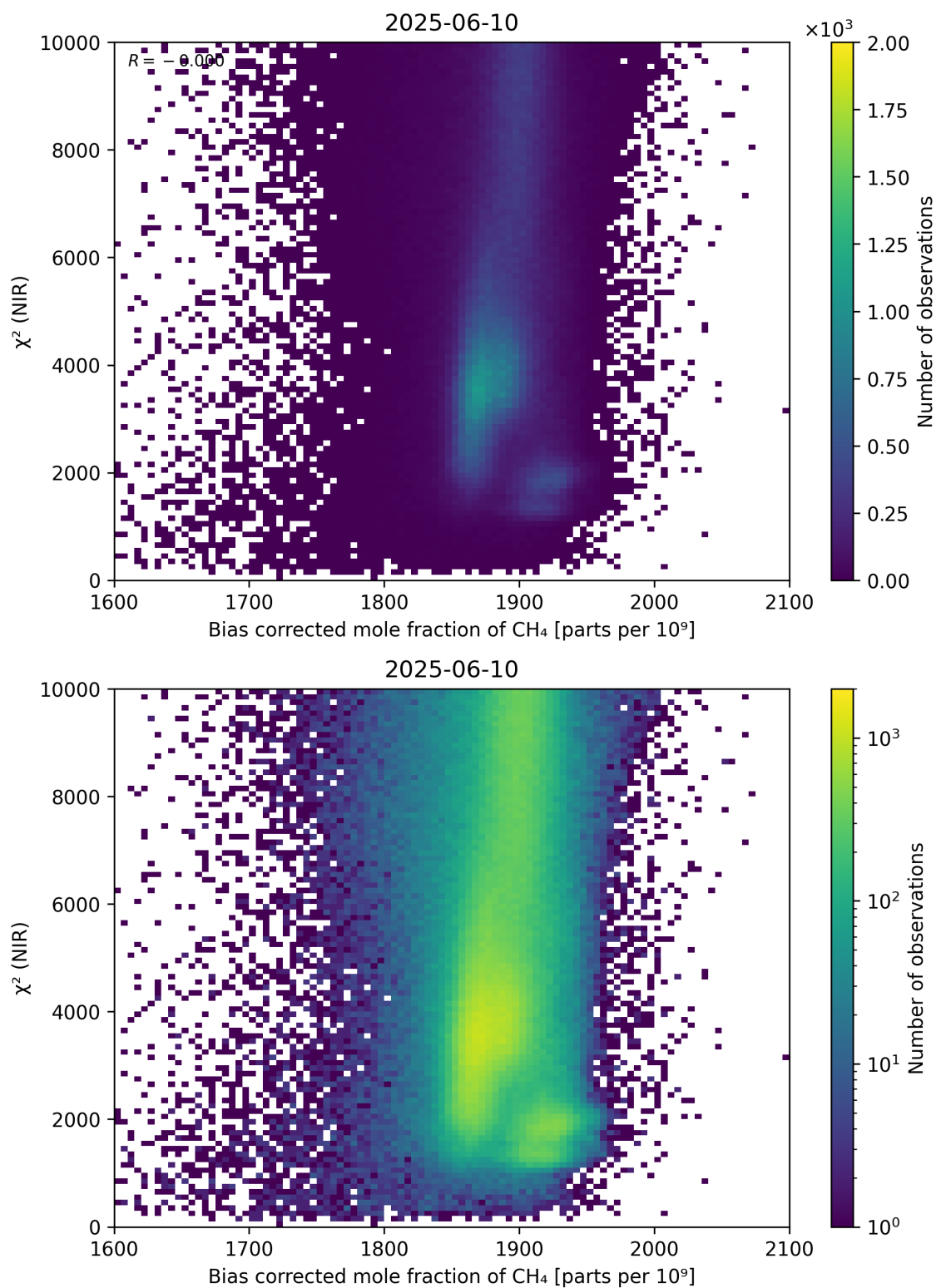
Figure 63: Scatter density plot of “Bias corrected mole fraction of CH 4 ” against “ \chi^2 (NIR)” for 2025-06-09 to 2025-06-11.
