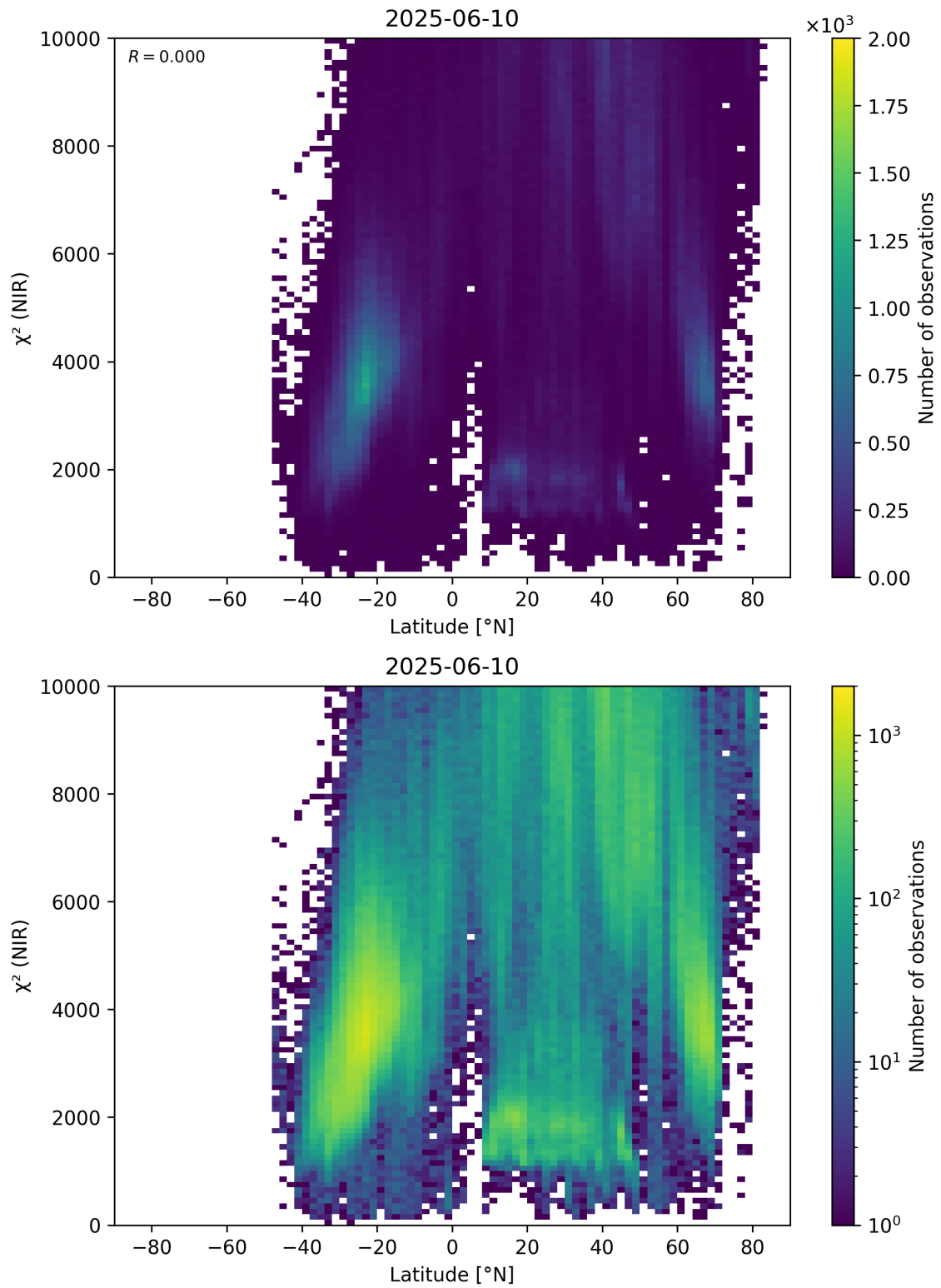
Figure 53: Scatter density plot of “Latitude” against “ \chi^2 (NIR)” for 2025-06-09 to 2025-06-11.
