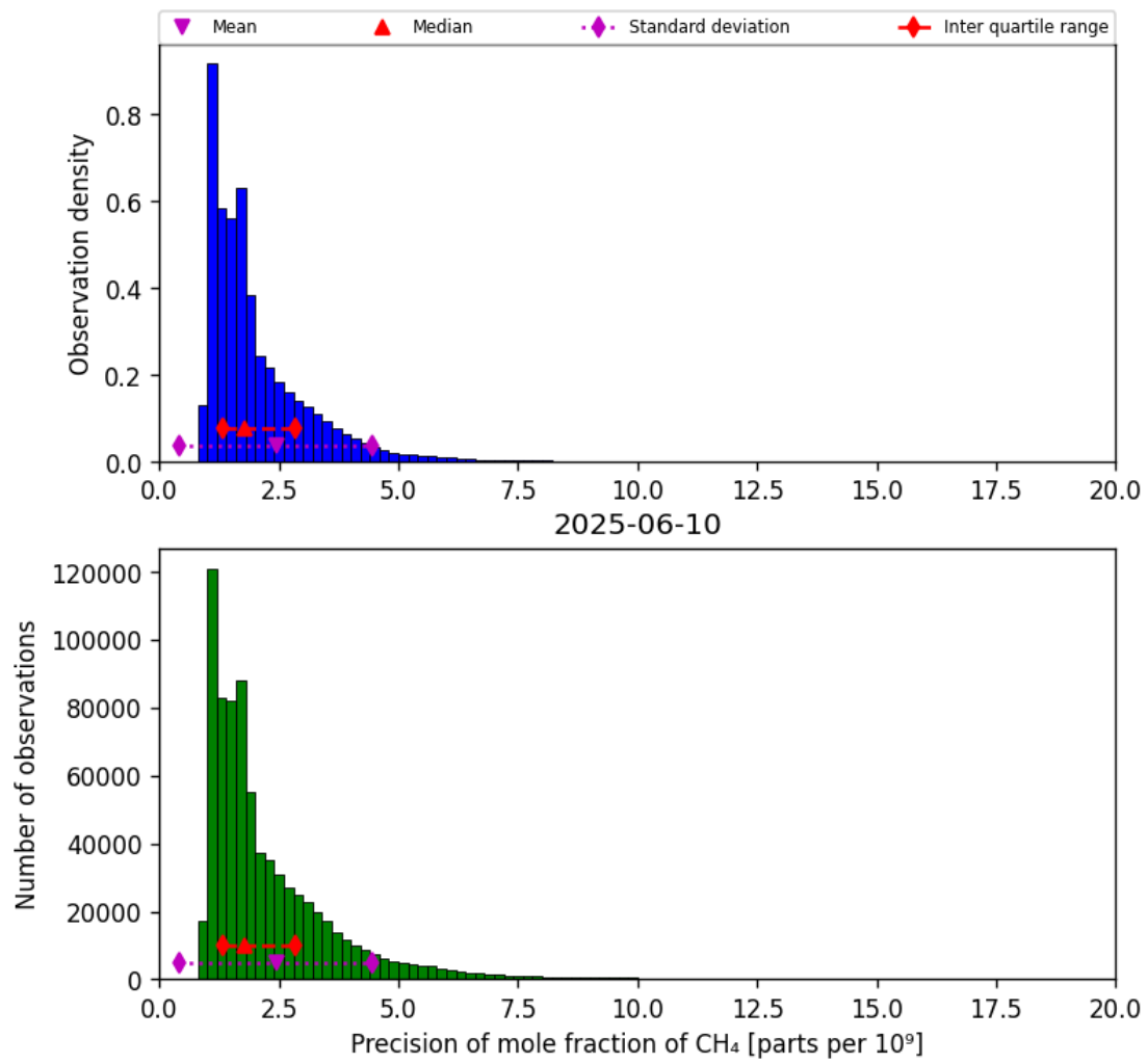
Figure 24: Histogram of “Precision of mole fraction of CH 4 ” for 2025-06-09 to 2025-06-11
