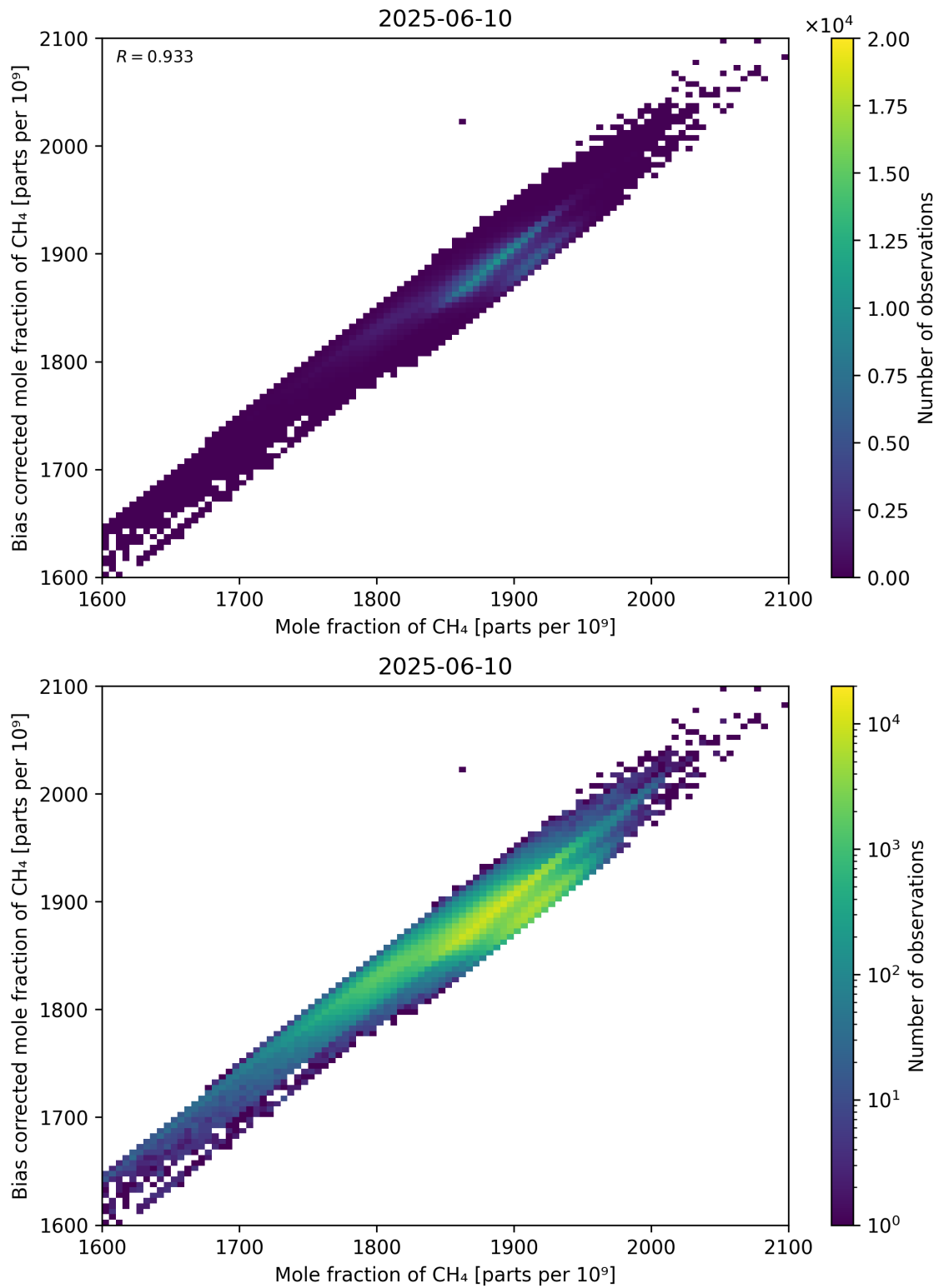
Figure 74: Scatter density plot of “Mole fraction of CH 4 ” against “Bias corrected mole fraction of CH 4 ” for 2025-06-09 to 2025-06-11.
