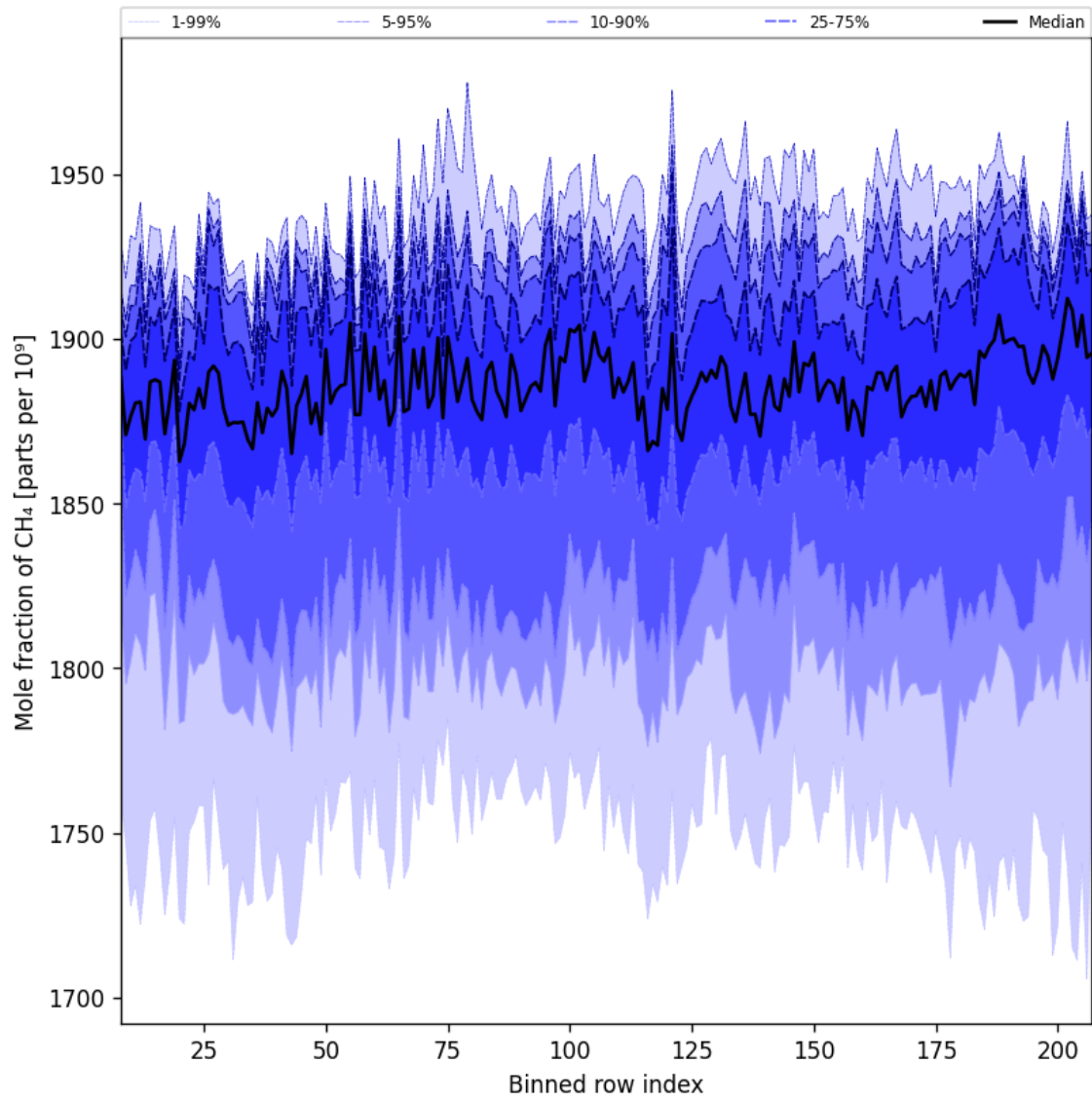
Figure 34: Along track statistics of “Mole fraction of CH 4 ” for 2025-06-09 to 2025-06-11
