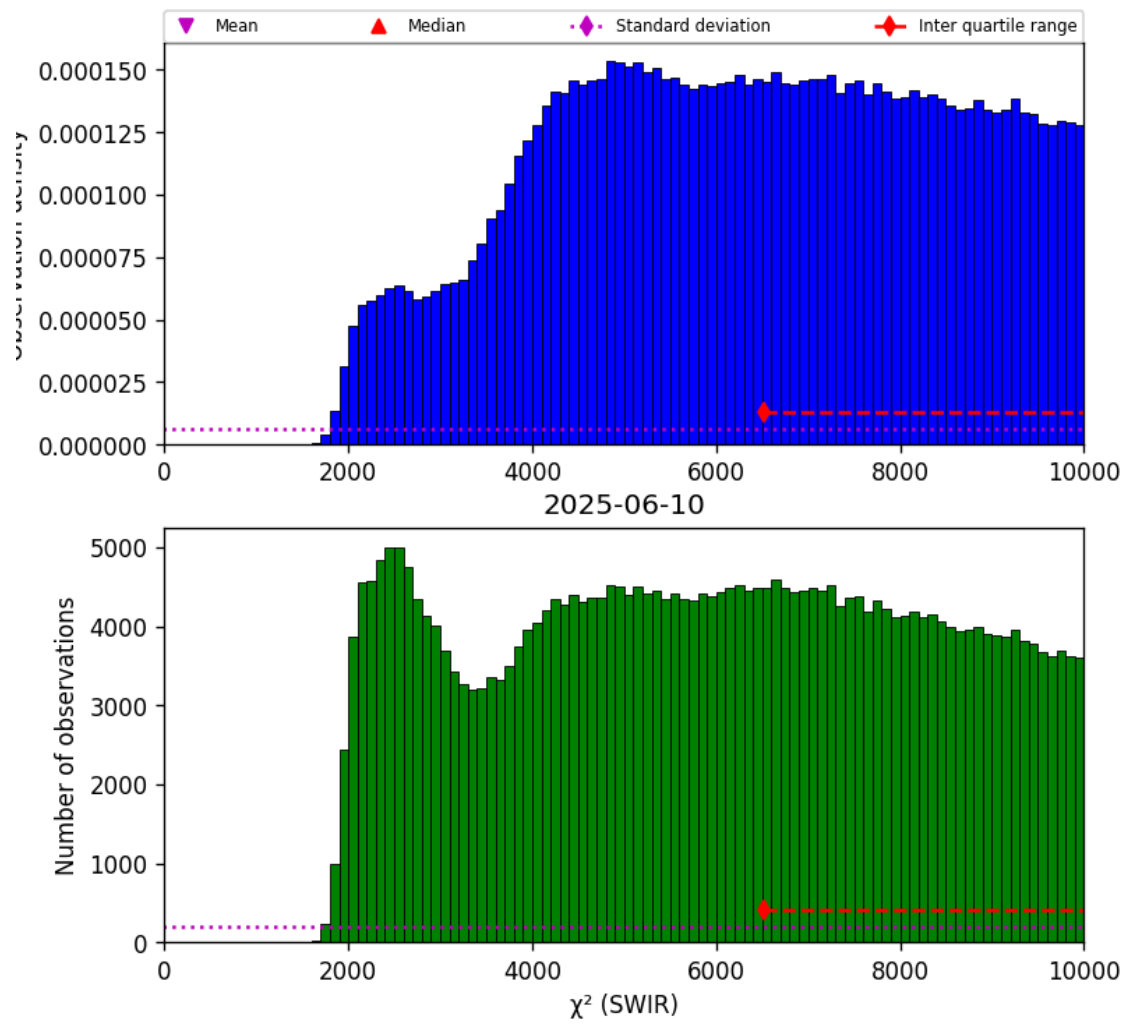
Figure 28: Histogram of “ \chi^2 (SWIR)” for 2025-06-09 to 2025-06-11
