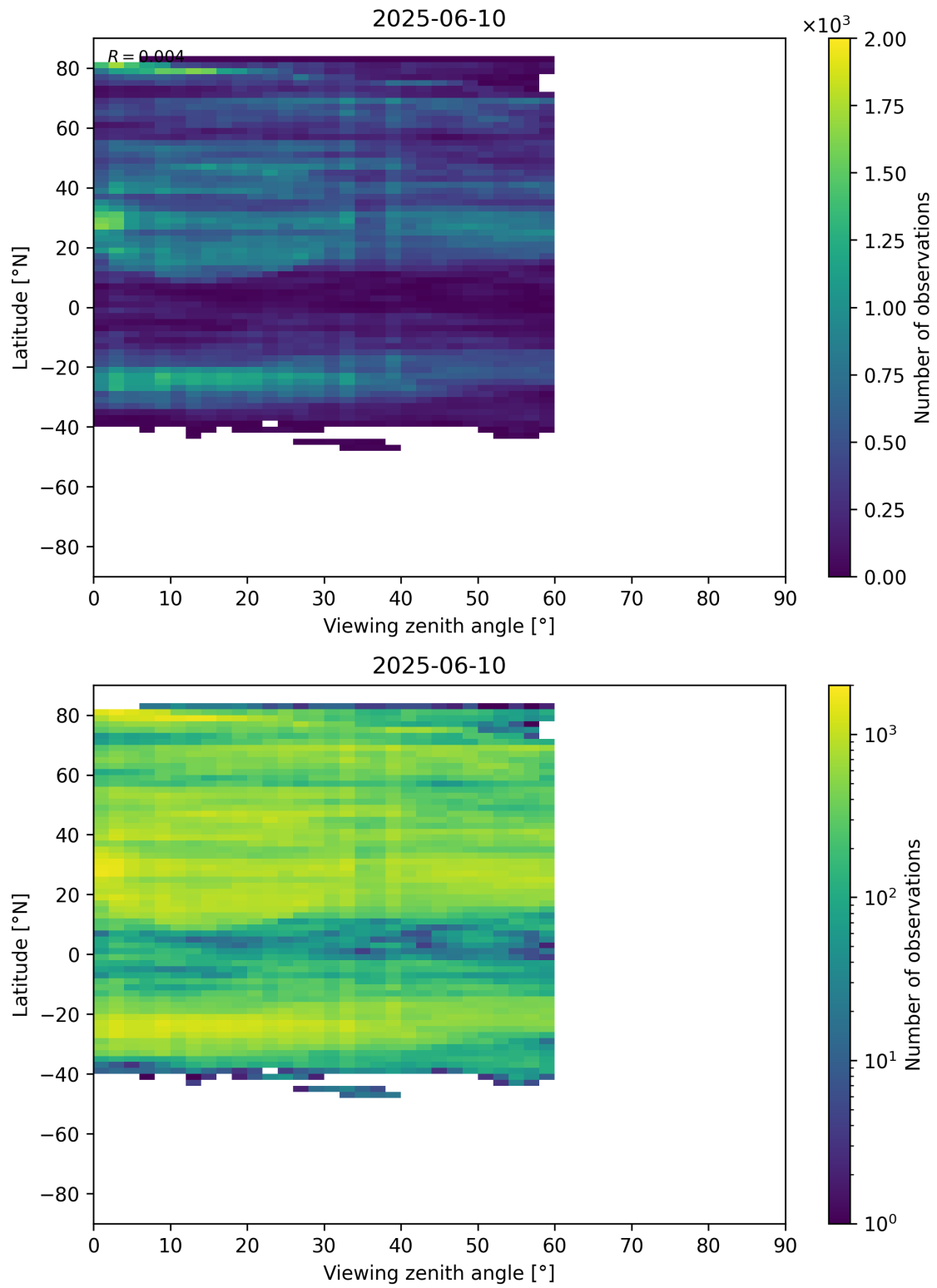
Figure 109: Scatter density plot of “Viewing zenith angle” against “Latitude” for 2025-06-09 to 2025-06-11.
