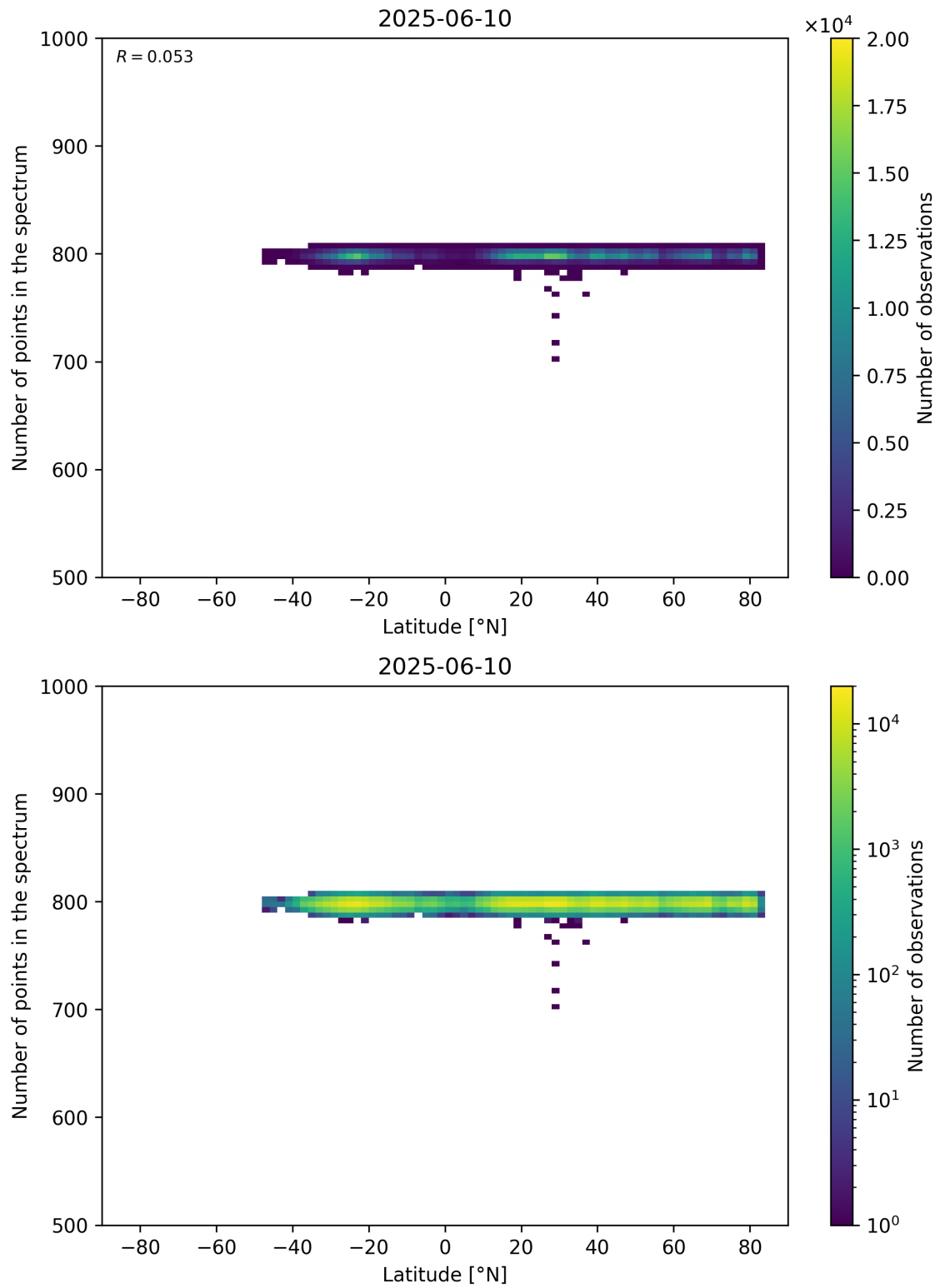
Figure 61: Scatter density plot of “Latitude” against “Number of points in the spectrum” for 2025-06-09 to 2025-06-11.
