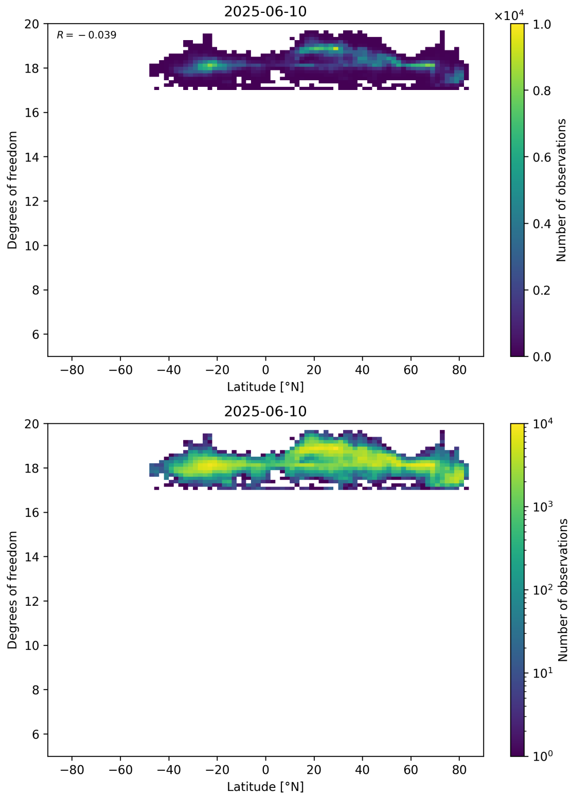
Figure 55: Scatter density plot of “Latitude” against “Degrees of freedom” for 2025-06-09 to 2025-06-11.
