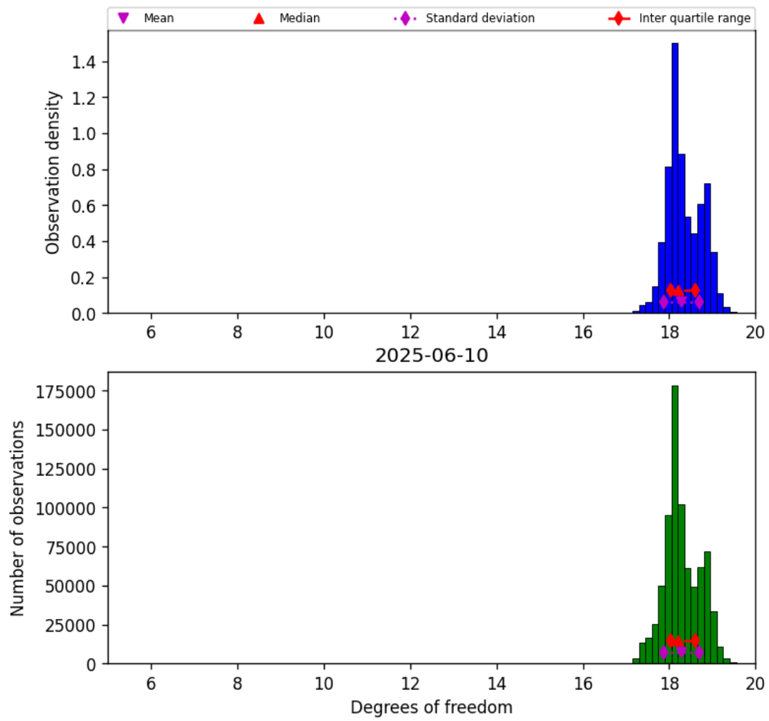
Figure 30: Histogram of “Degrees of freedom” for 2025-06-09 to 2025-06-11
