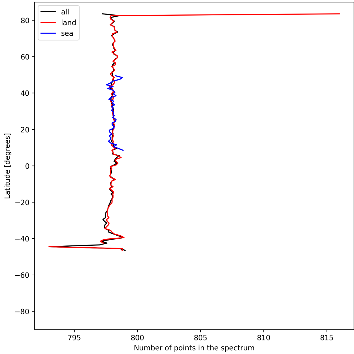
Figure 15: Zonal average of “Number of points in the spectrum” for 2025-06-09 to 2025-06-11.
