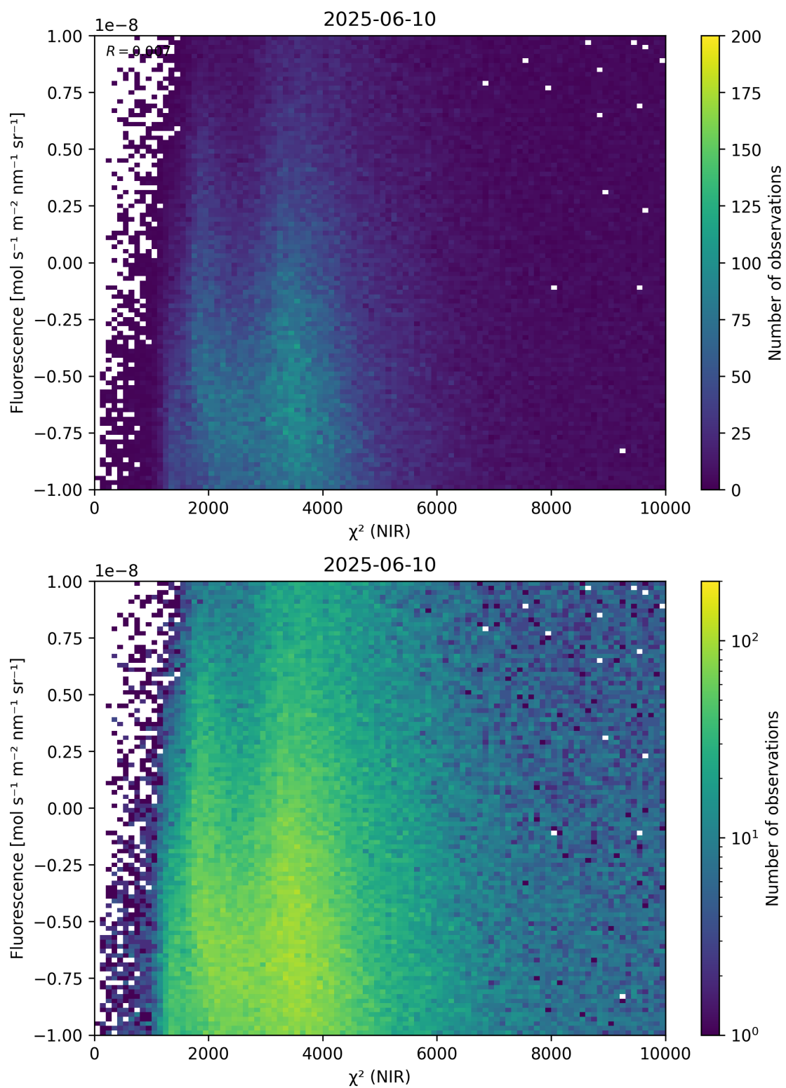
Figure 45: Scatter density plot of “ \chi^2 (NIR)” against “Fluorescence” for 2025-06-09 to 2025-06-11.
