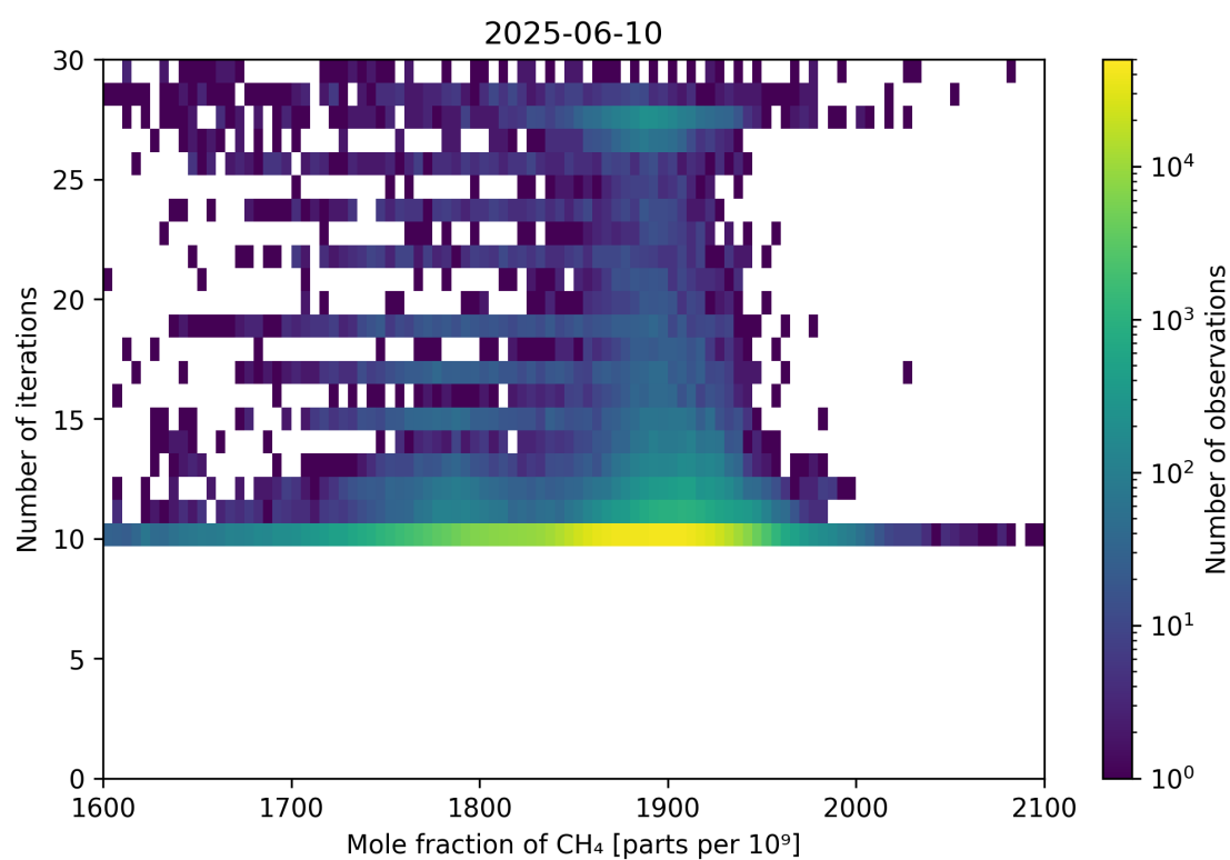
Figure 76: Scatter density plot of “Mole fraction of CH 4 ” against “Number of iterations” for 2025-06-09 to 2025-06-11.
