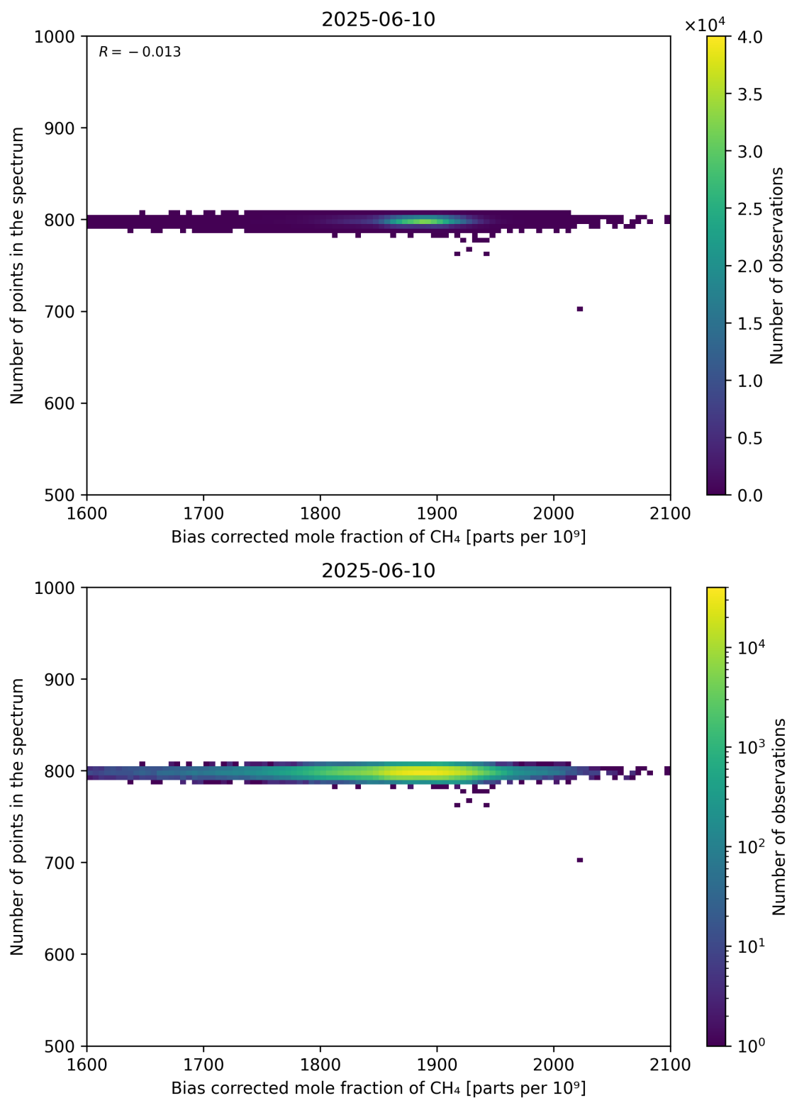
Figure 68: Scatter density plot of “Bias corrected mole fraction of CH 4 ” against “Number of points in the spectrum” for 2025-06-09 to 2025-06-11.
