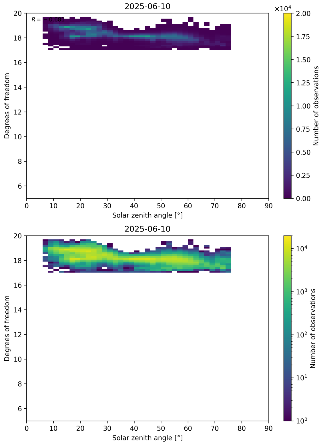
Figure 96: Scatter density plot of “Solar zenith angle” against “Degrees of freedom” for 2025-06-09 to 2025-06-11.
