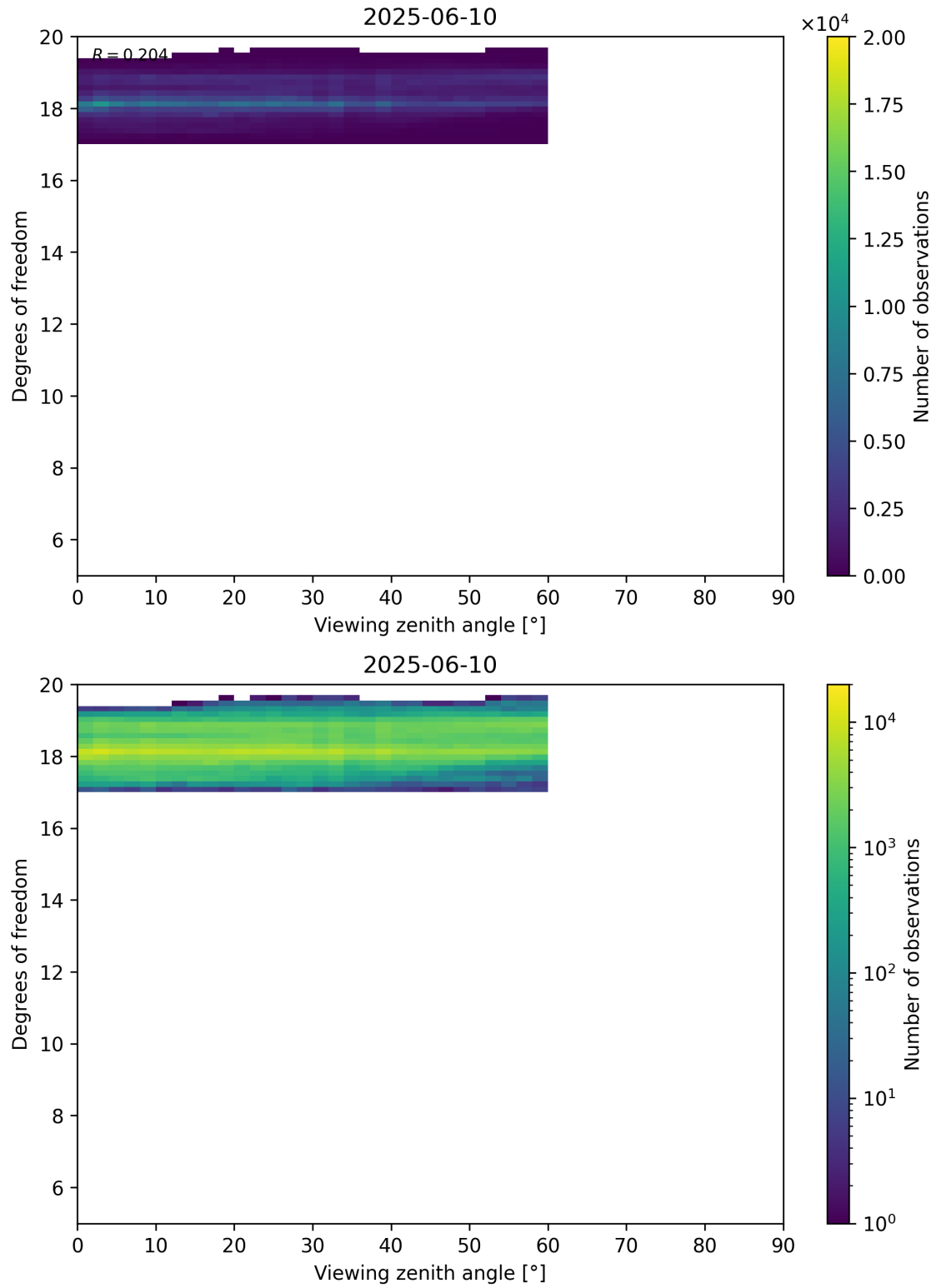
Figure 107: Scatter density plot of “Viewing zenith angle” against “Degrees of freedom” for 2025-06-09 to 2025-06-11.
