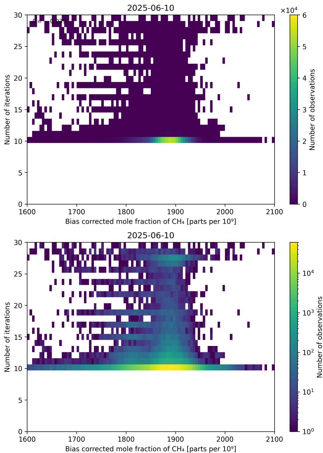
Figure 67: Scatter density plot of “Bias corrected mole fraction of CH 4 ” against “Number of iterations” for 2025-06-09 to 2025-06-11.
