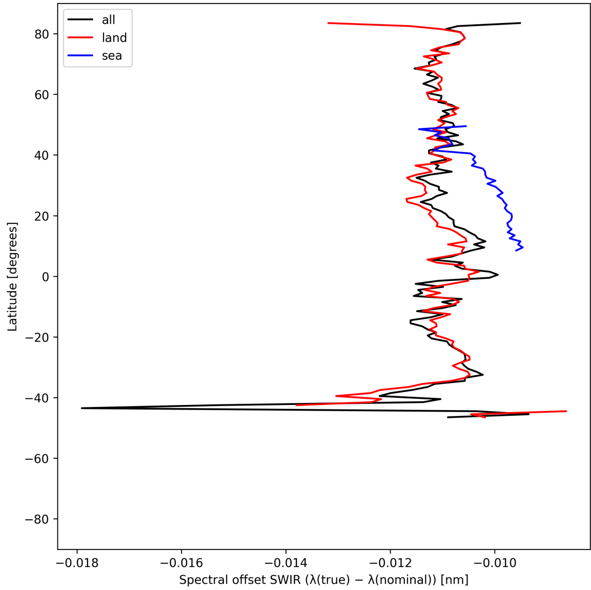
Figure 16: Zonal average of “Spectral offset SWIR ( \lambda_{\text{true}} - \lambda_{\text{nominal}} )” for 2025-06-09 to 2025-06-11.
