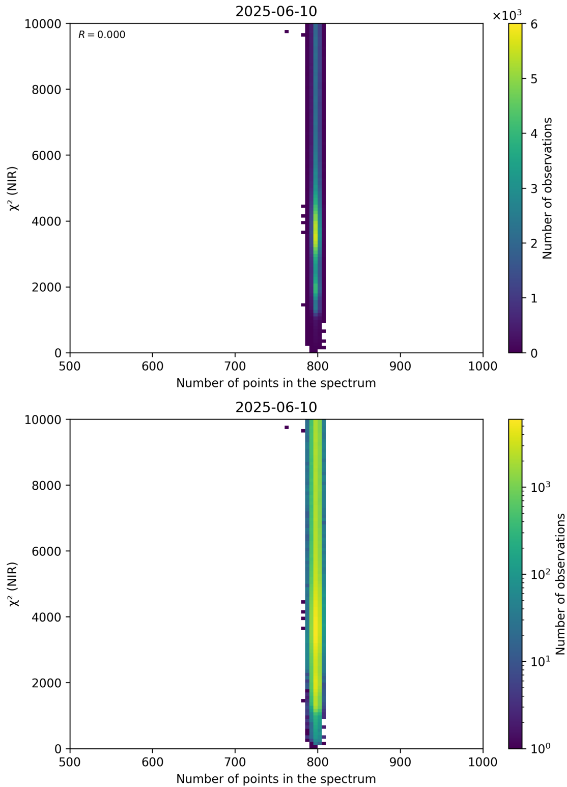
Figure 88: Scatter density plot of “Number of points in the spectrum” against “ \chi^2 (NIR)” for 2025-06-09 to 2025-06-11.
