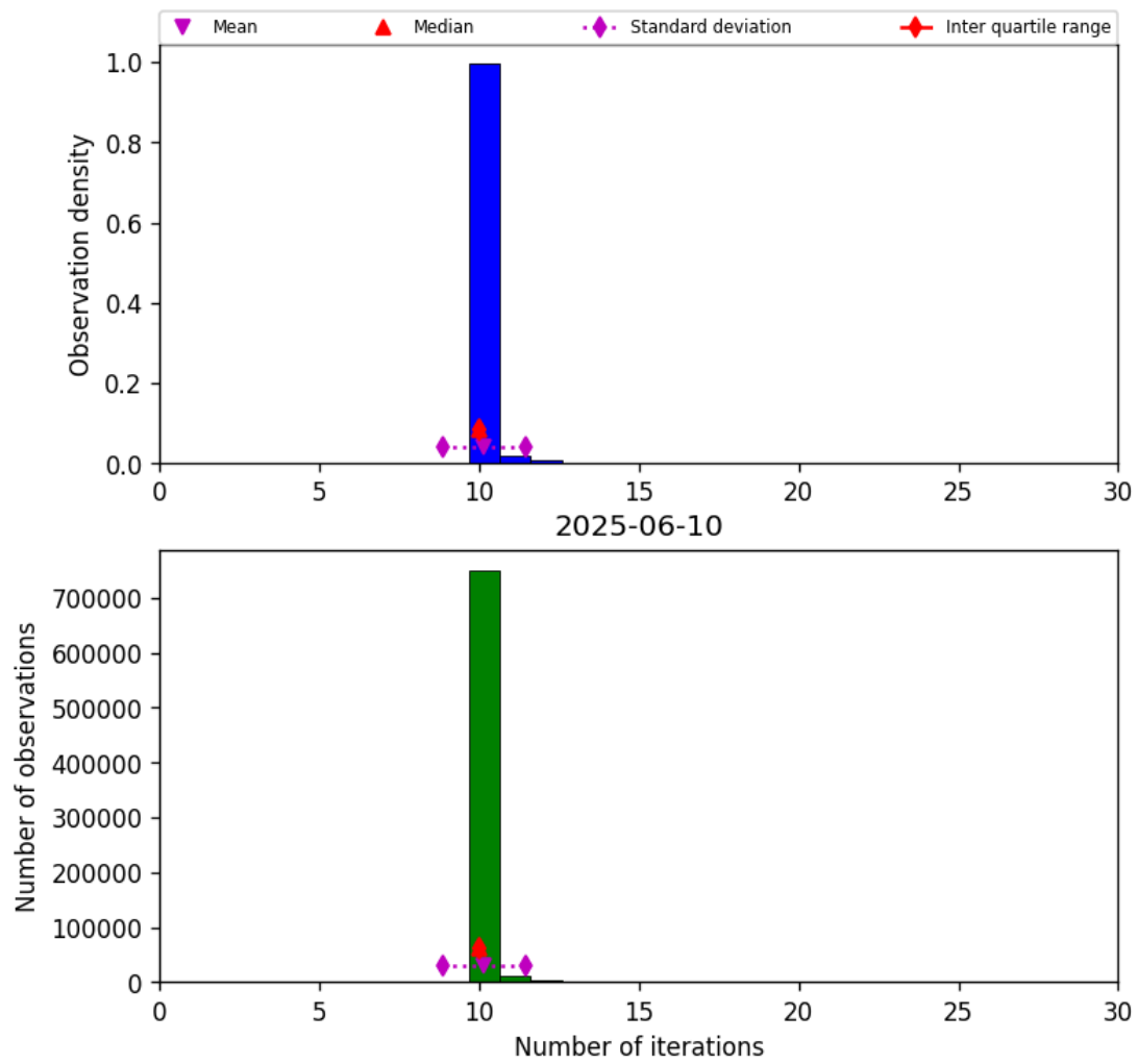
Figure 31: Histogram of “Number of iterations” for 2025-06-09 to 2025-06-11
