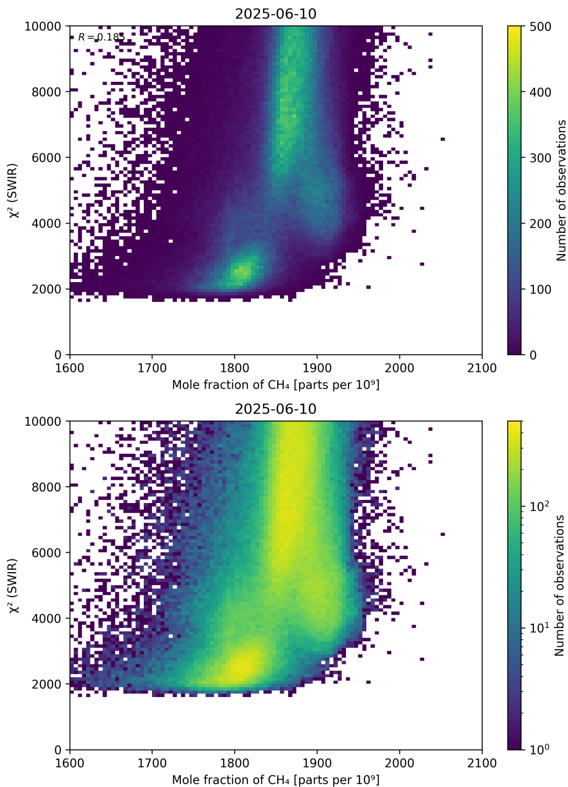
Figure 71: Scatter density plot of “Mole fraction of \text{CH}_4 ” against “ \chi^2 (SWIR)” for 2025-06-09 to 2025-06-11.
