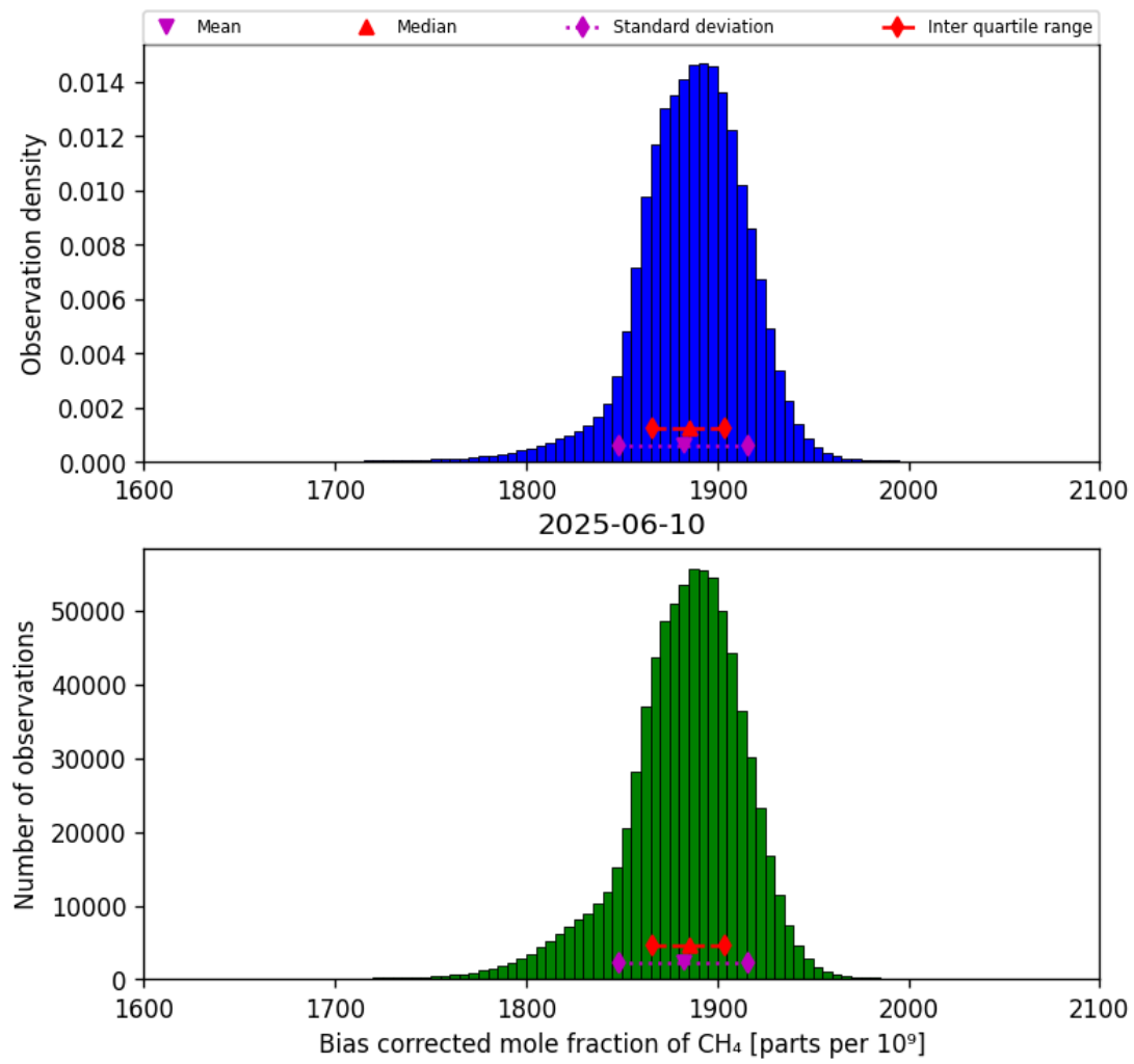
Figure 25: Histogram of “Bias corrected mole fraction of CH 4 ” for 2025-06-09 to 2025-06-11
