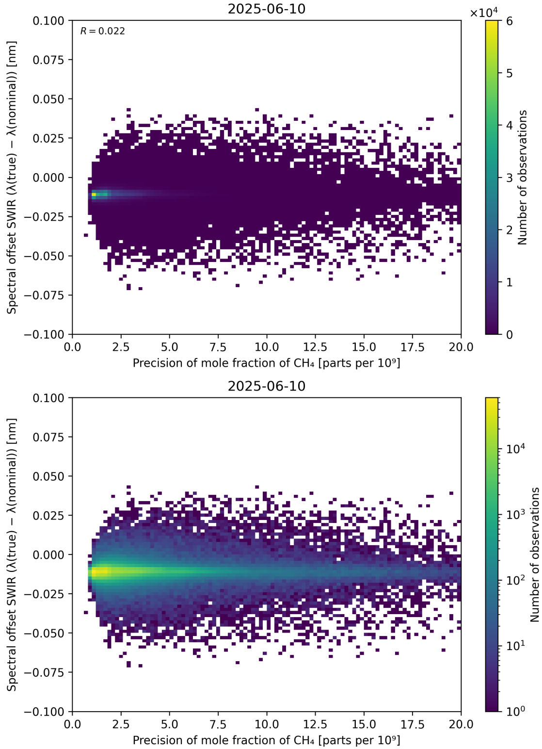
Figure 85: Scatter density plot of “Precision of mole fraction of CH 4 ” against “Spectral offset SWIR ( \lambda_{\text{true}} - \lambda_{\text{nominal}} )” for 2025-06-09 to 2025-06-11.
