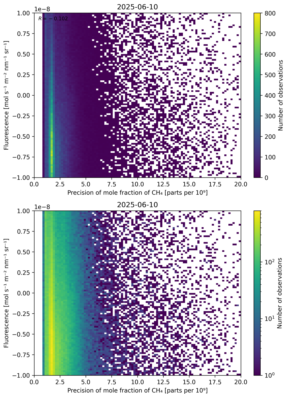
Figure 81: Scatter density plot of “Precision of mole fraction of CH 4 ” against “Fluorescence” for 2025-06-09 to 2025-06-11.
