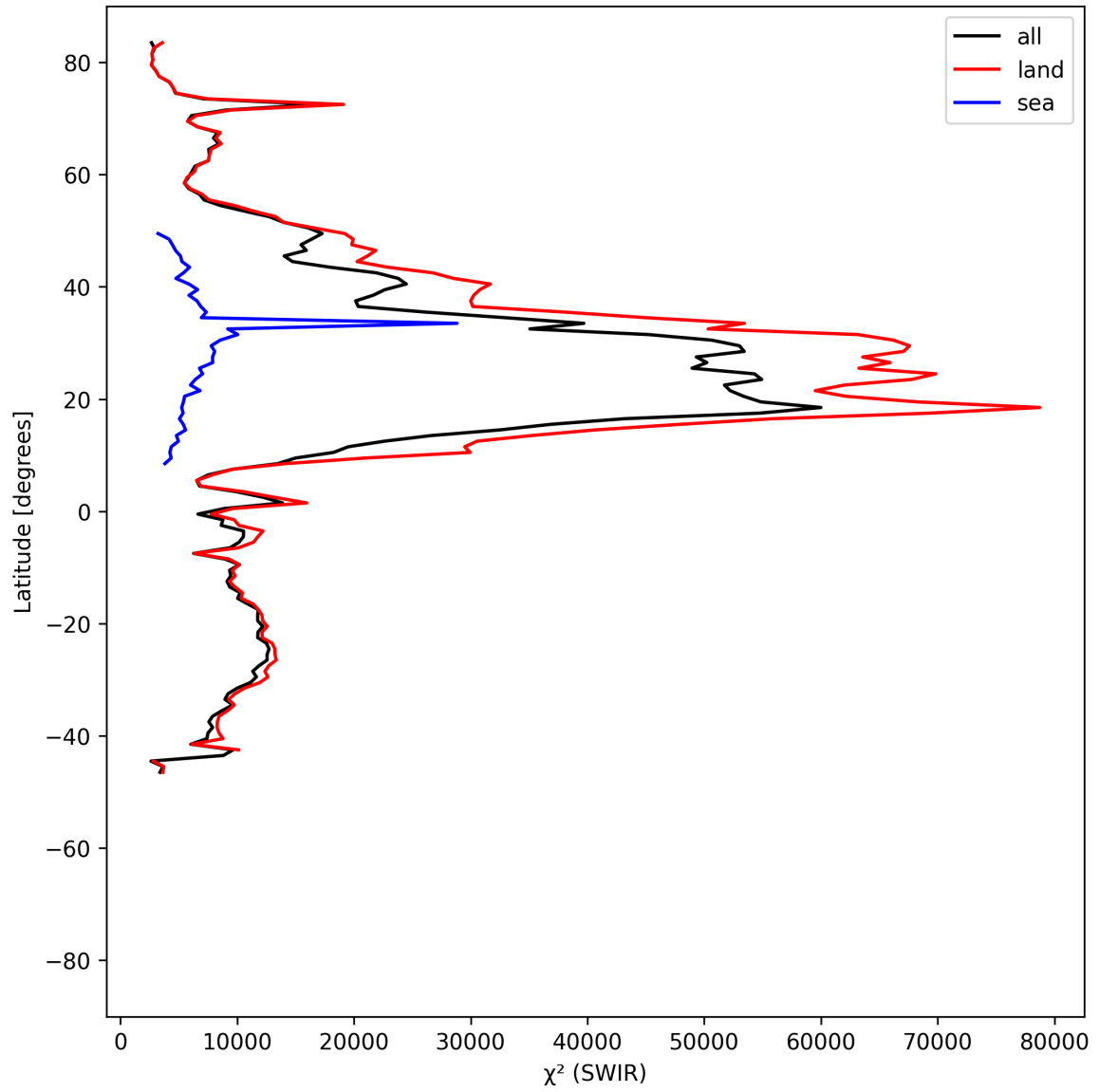
Figure 17: Zonal average of “ \chi^2 (SWIR)” for 2025-06-09 to 2025-06-11.
