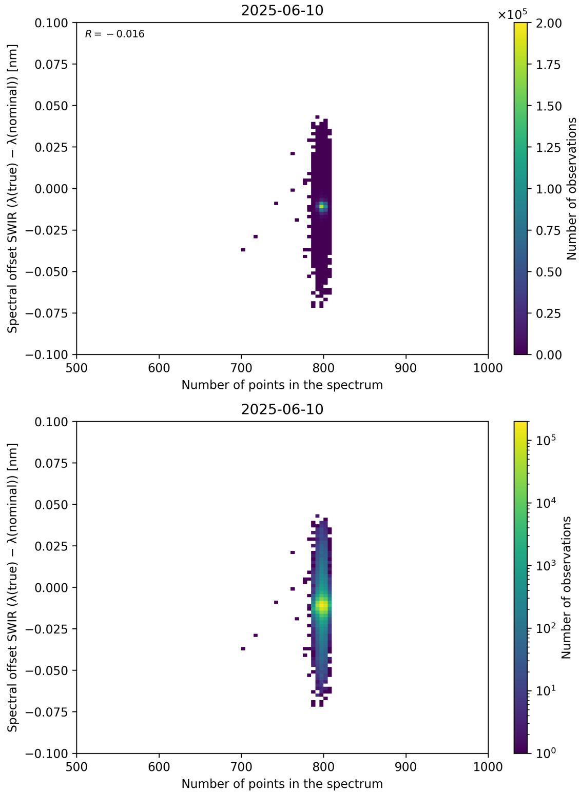
Figure 93: Scatter density plot of “Number of points in the spectrum” against “Spectral offset SWIR ( \lambda_{\text{true}} - \lambda_{\text{nominal}} )” for 2025-06-09 to 2025-06-11.
