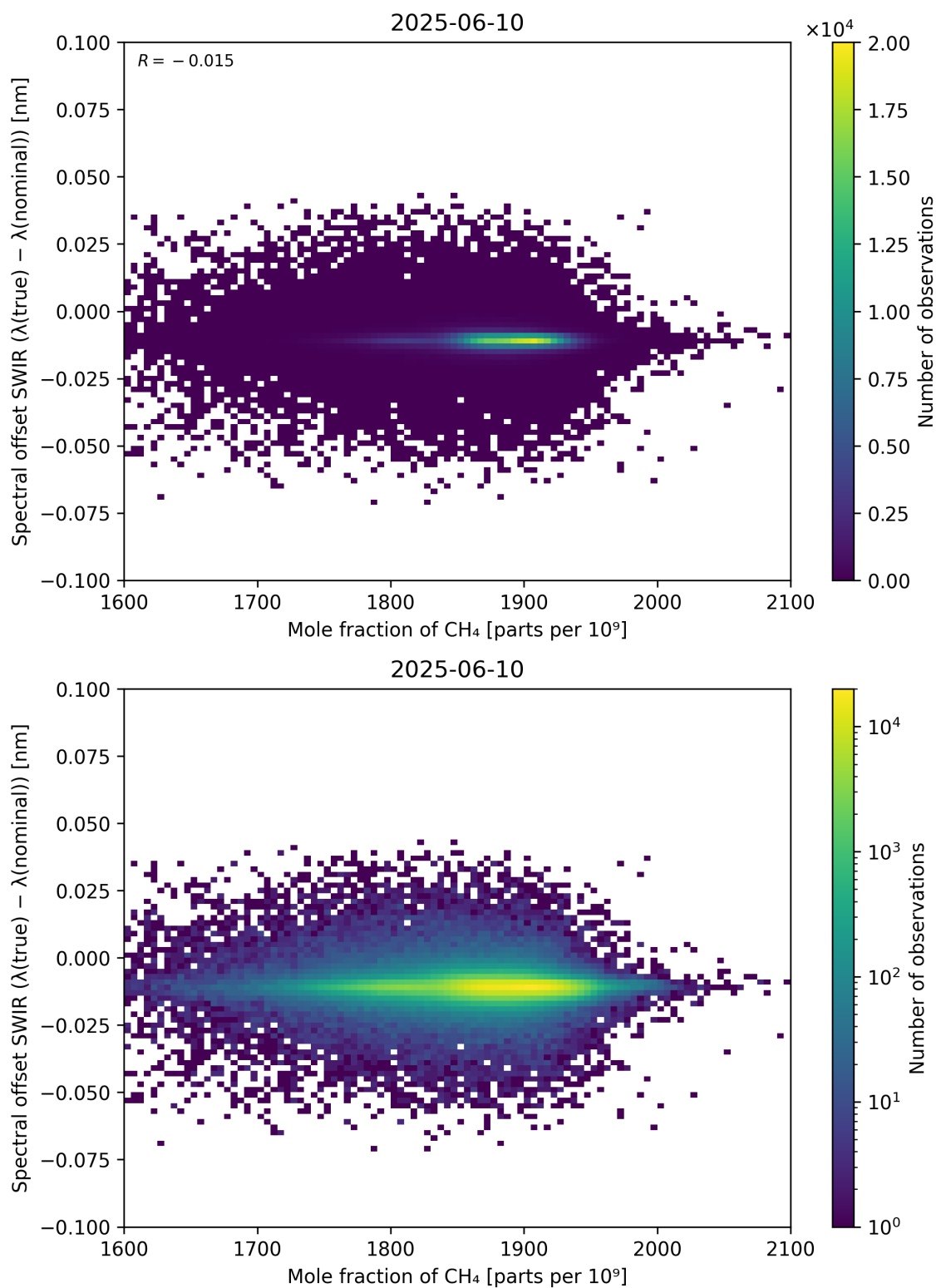
Figure 86: Scatter density plot of “Mole fraction of CH 4 ” against “Spectral offset SWIR ( \lambda_{\text{true}} - \lambda_{\text{nominal}} )” for 2025-06-09 to 2025-06-11.
