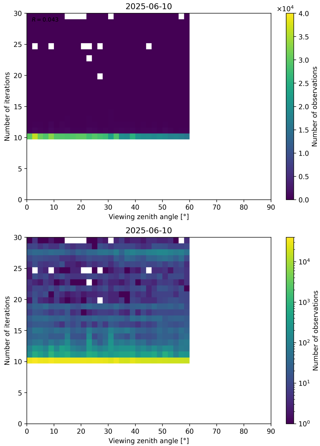
Figure 113: Scatter density plot of “Viewing zenith angle” against “Number of iterations” for 2025-06-09 to 2025-06-11.
