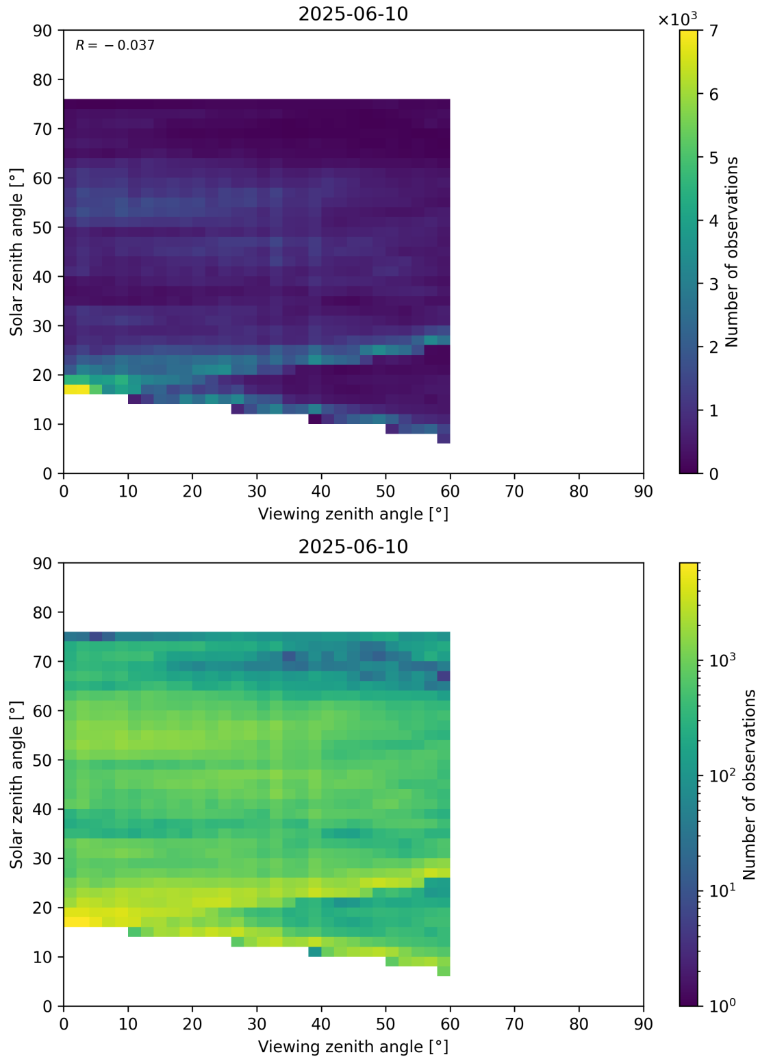
Figure 115: Scatter density plot of “Viewing zenith angle” against “Solar zenith angle” for 2025-06-09 to 2025-06-11.
