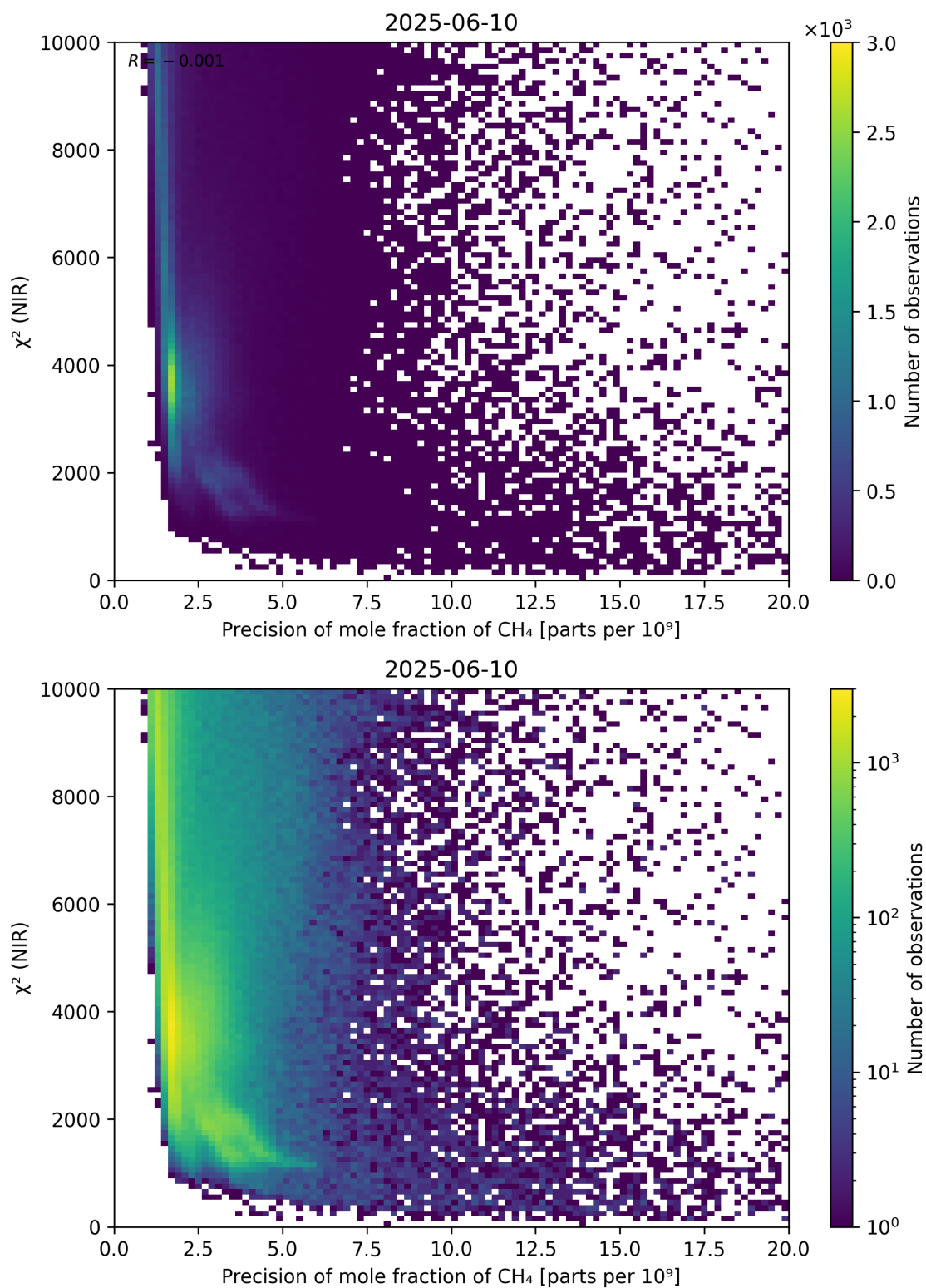
Figure 78: Scatter density plot of “Precision of mole fraction of CH 4 ” against “ \chi^2 (NIR)” for 2025-06-09 to 2025-06-11.
