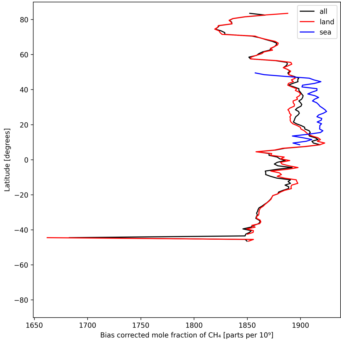
Figure 14: Zonal average of “Bias corrected mole fraction of CH 4 ” for 2025-06-09 to 2025-06-11.
