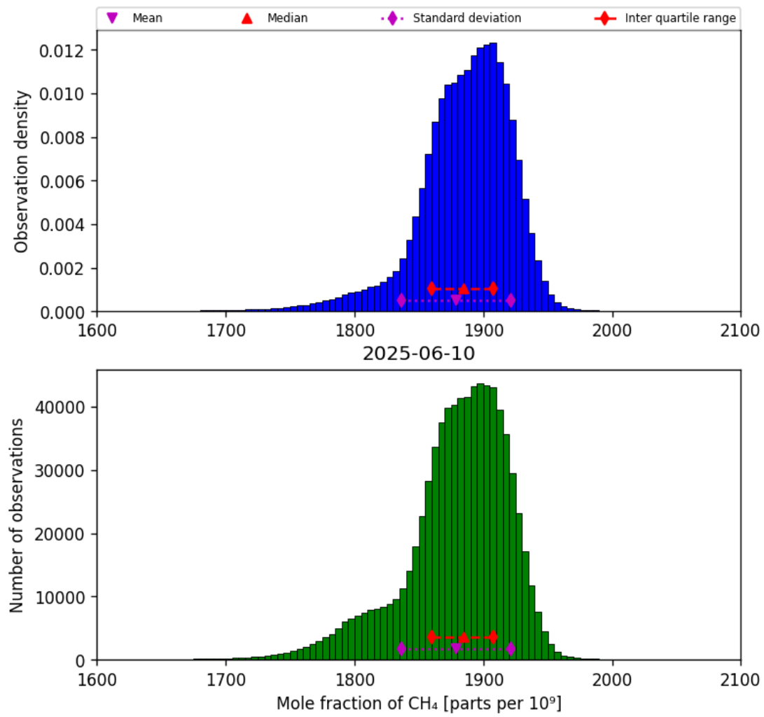
Figure 23: Histogram of “Mole fraction of CH 4 ” for 2025-06-09 to 2025-06-11
