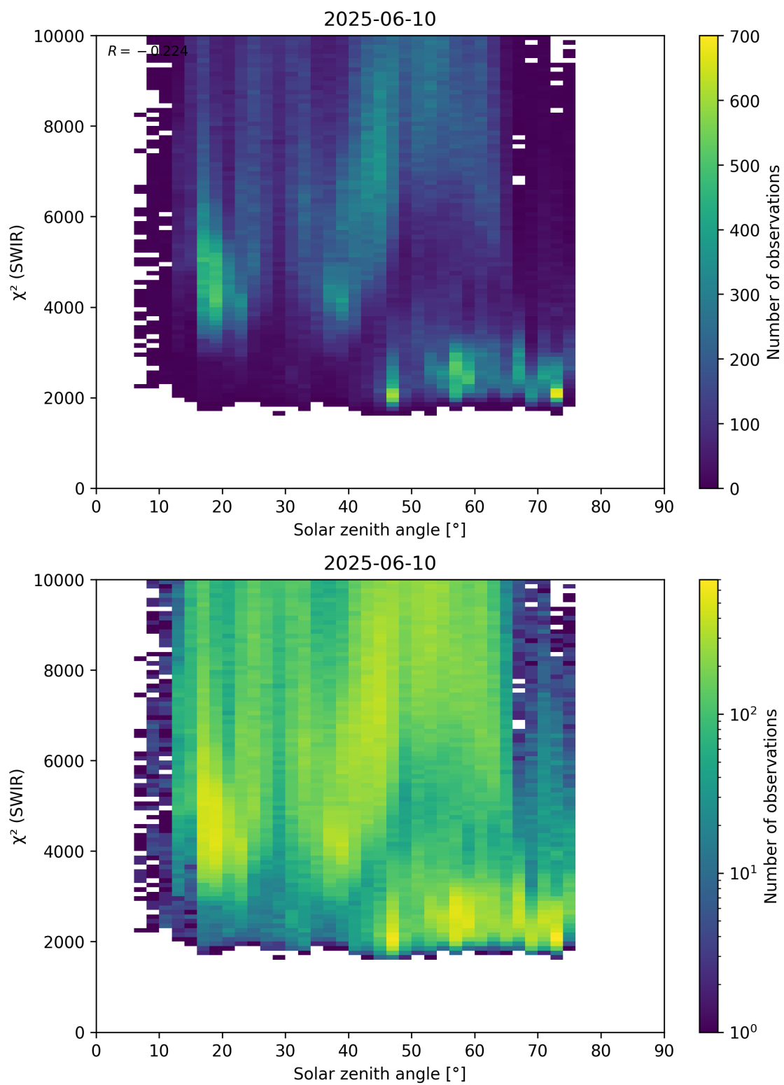
Figure 95: Scatter density plot of “Solar zenith angle” against “ \chi^2 (SWIR)” for 2025-06-09 to 2025-06-11.
