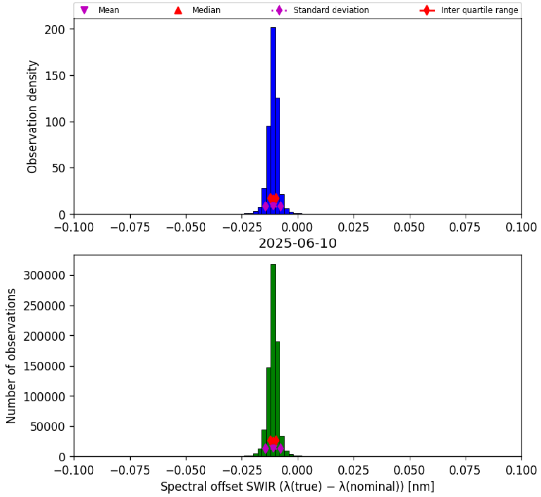
Figure 27: Histogram of “Spectral offset SWIR ( \lambda_{\text{true}} - \lambda_{\text{nominal}} )” for 2025-06-09 to 2025-06-11
