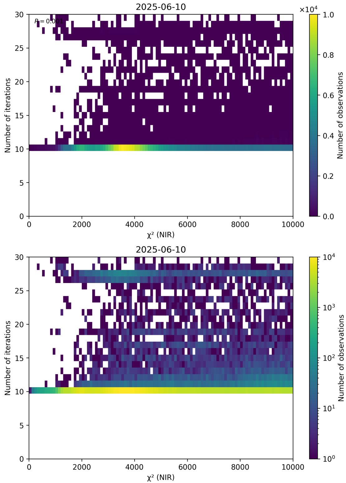
Figure 46: Scatter density plot of “ \chi^2 (NIR)” against “Number of iterations” for 2025-06-09 to 2025-06-11.
