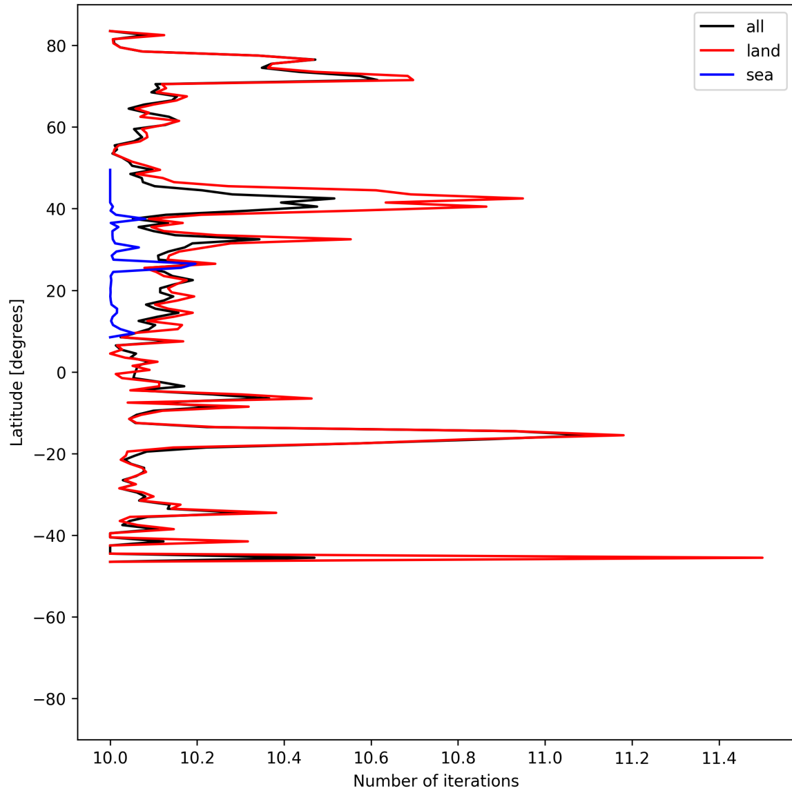
Figure 20: Zonal average of “Number of iterations” for 2025-06-09 to 2025-06-11.
