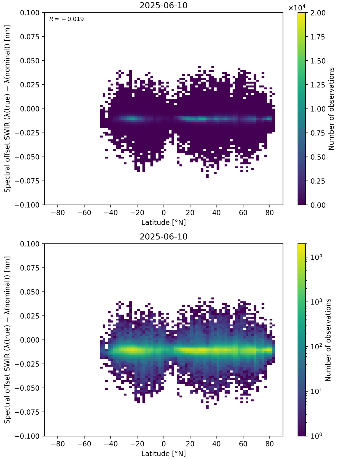
Figure 62: Scatter density plot of “Latitude” against “Spectral offset SWIR ( \lambda_{\text{true}} - \lambda_{\text{nominal}} )” for 2025-06-09 to 2025-06-11.
