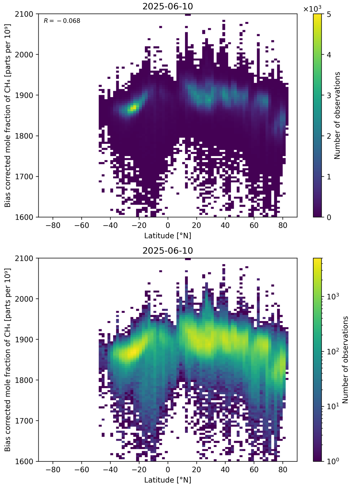
Figure 58: Scatter density plot of “Latitude” against “Bias corrected mole fraction of \text{CH}_4 ” for 2025-06-09 to 2025-06-11.
