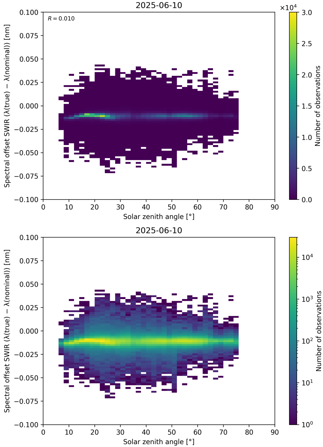
Figure 104: Scatter density plot of “Solar zenith angle” against “Spectral offset SWIR ( \lambda_{\text{true}} - \lambda_{\text{nominal}} )” for 2025-06-09 to 2025-06-11.
