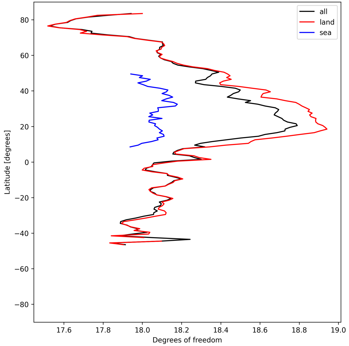
Figure 19: Zonal average of “Degrees of freedom” for 2025-06-09 to 2025-06-11.
