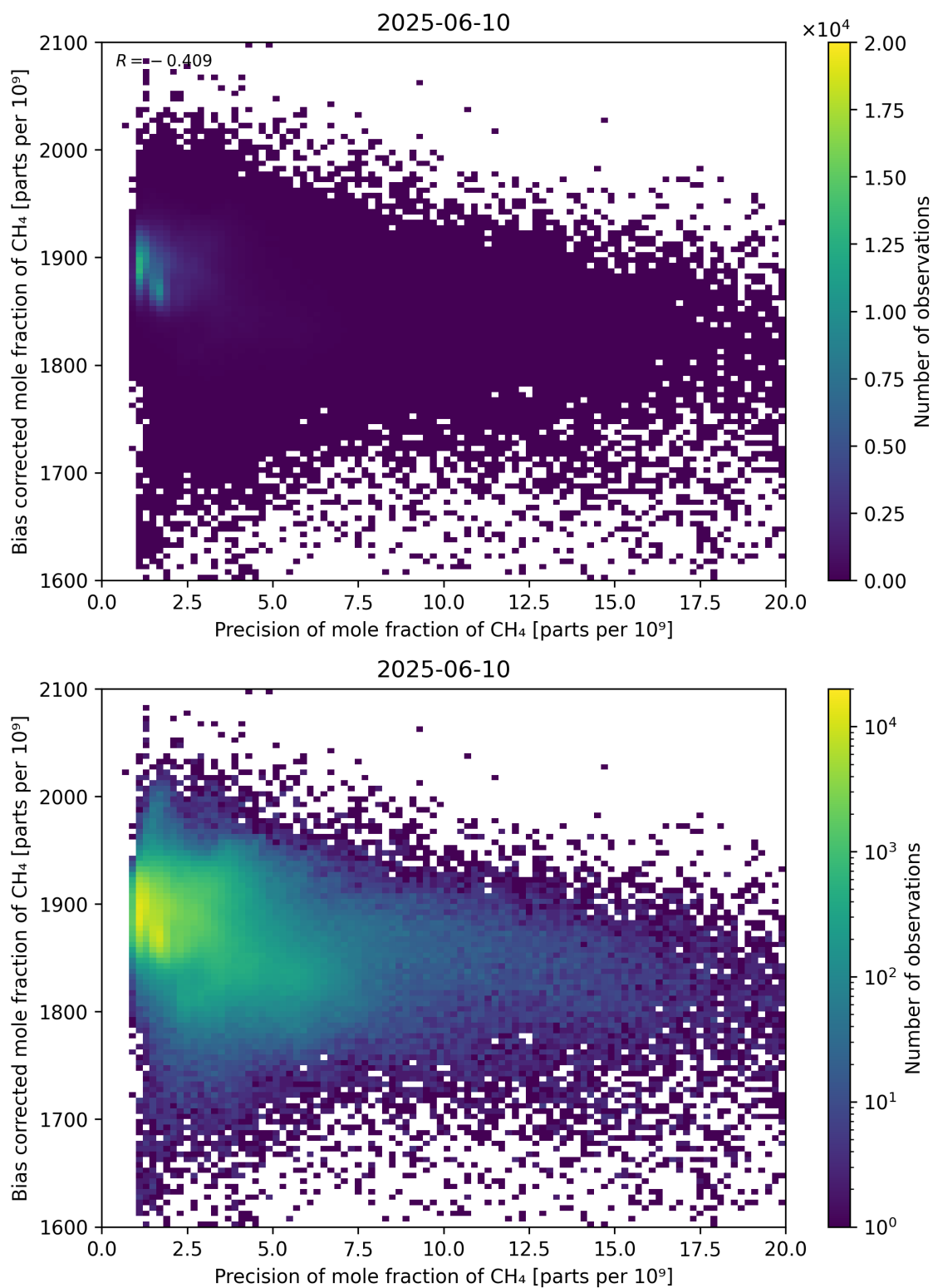
Figure 82: Scatter density plot of “Precision of mole fraction of CH 4 ” against “Bias corrected mole fraction of CH 4 ” for 2025-06-09 to 2025-06-11.
