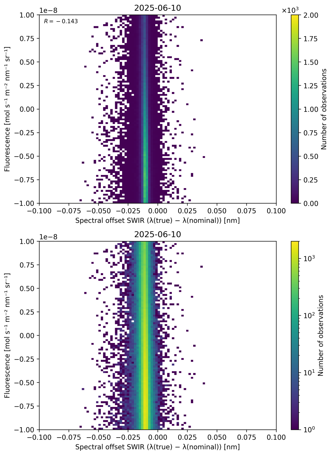
Figure 120: Scatter density plot of “Spectral offset SWIR ( \lambda_{\text{true}} - \lambda_{\text{nominal}} )” against “Fluorescence” for 2025-06-09 to 2025-06-11.
