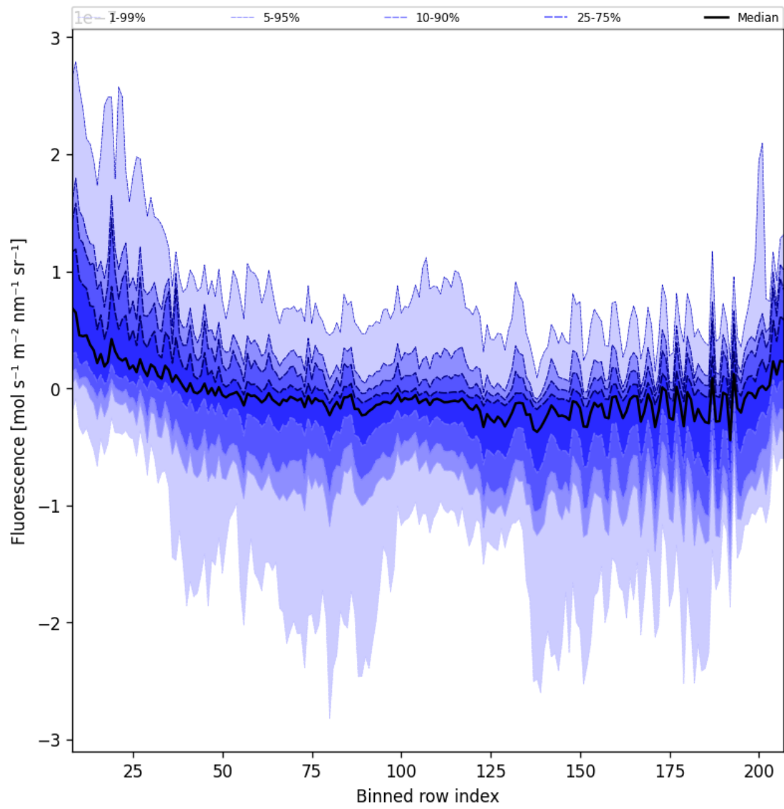
Figure 43: Along track statistics of “Fluorescence” for 2025-06-09 to 2025-06-11
