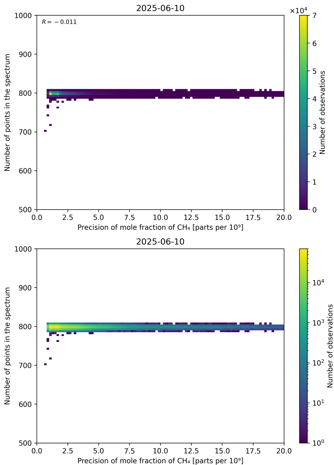
Figure 84: Scatter density plot of “Precision of mole fraction of CH 4 ” against “Number of points in the spectrum” for 2025-06-09 to 2025-06-11.
