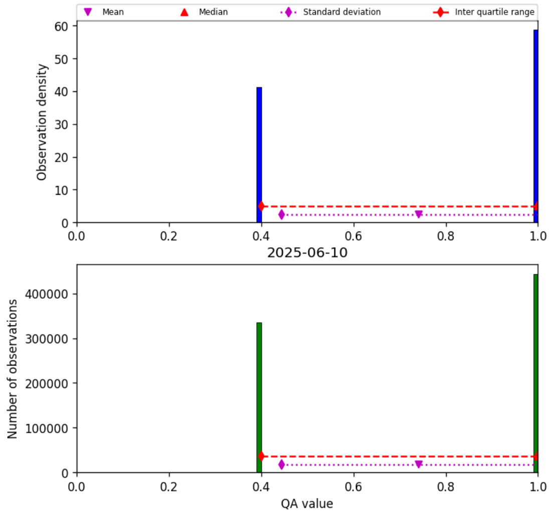
Figure 22: Histogram of “QA value” for 2025-06-09 to 2025-06-11
