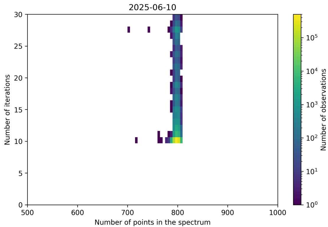
Figure 92: Scatter density plot of “Number of points in the spectrum” against “Number of iterations” for 2025-06-09 to 2025-06-11.
