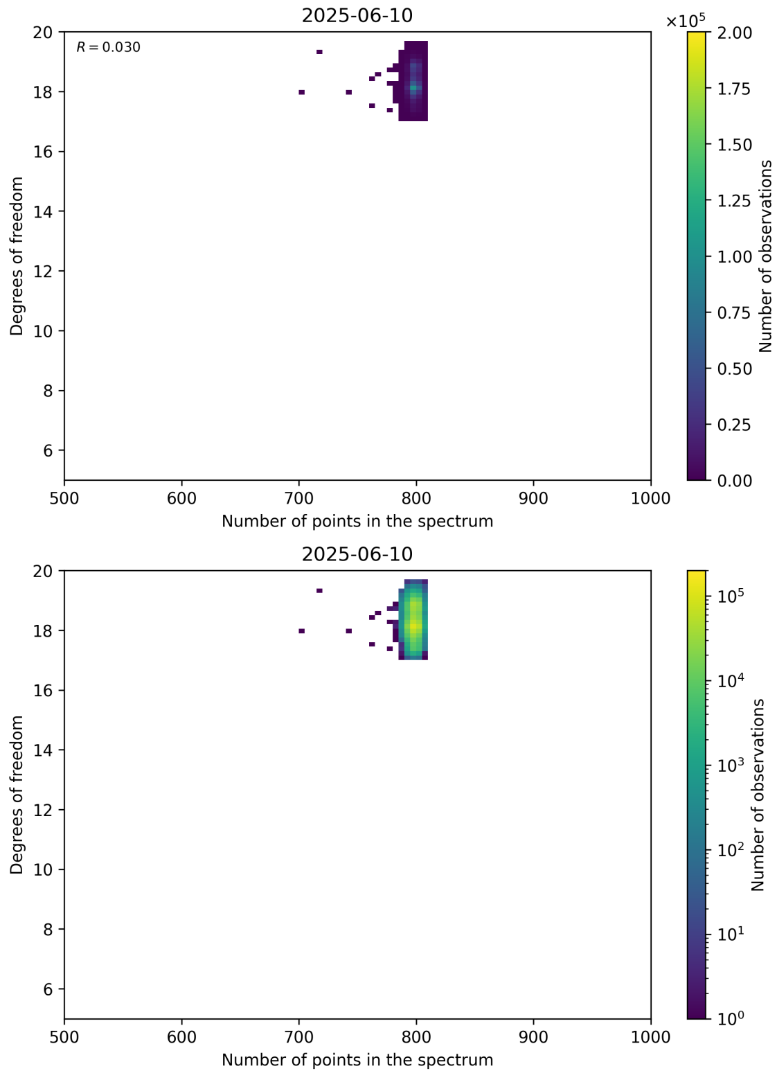
Figure 90: Scatter density plot of “Number of points in the spectrum” against “Degrees of freedom” for 2025-06-09 to 2025-06-11.
