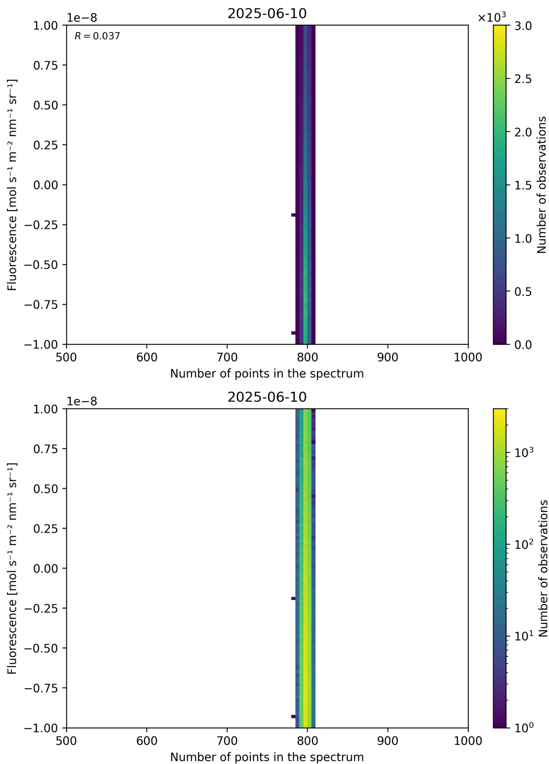
Figure 91: Scatter density plot of “Number of points in the spectrum” against “Fluorescence” for 2025-06-09 to 2025-06-11.
