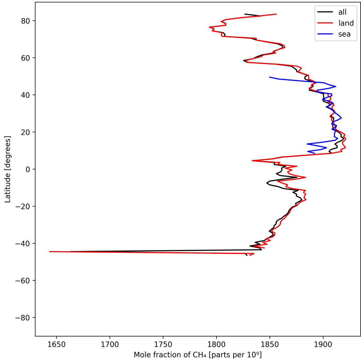
Figure 12: Zonal average of “Mole fraction of \text{CH}_4 ” for 2025-06-09 to 2025-06-11.
