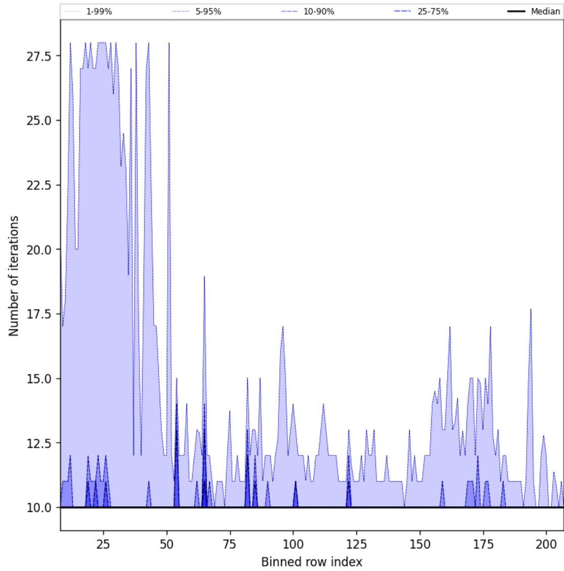
Figure 42: Along track statistics of “Number of iterations” for 2025-06-09 to 2025-06-11
