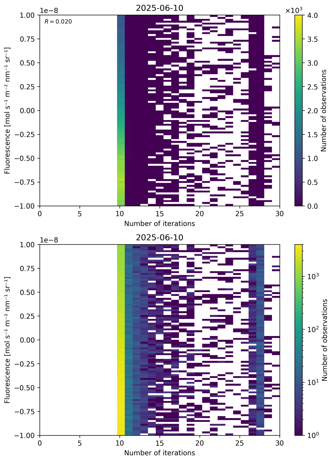
Figure 87: Scatter density plot of “Number of iterations” against “Fluorescence” for 2025-06-09 to 2025-06-11.
