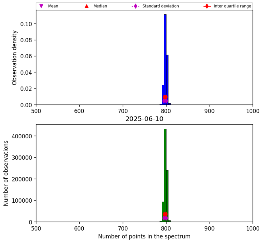
Figure 26: Histogram of “Number of points in the spectrum” for 2025-06-09 to 2025-06-11
