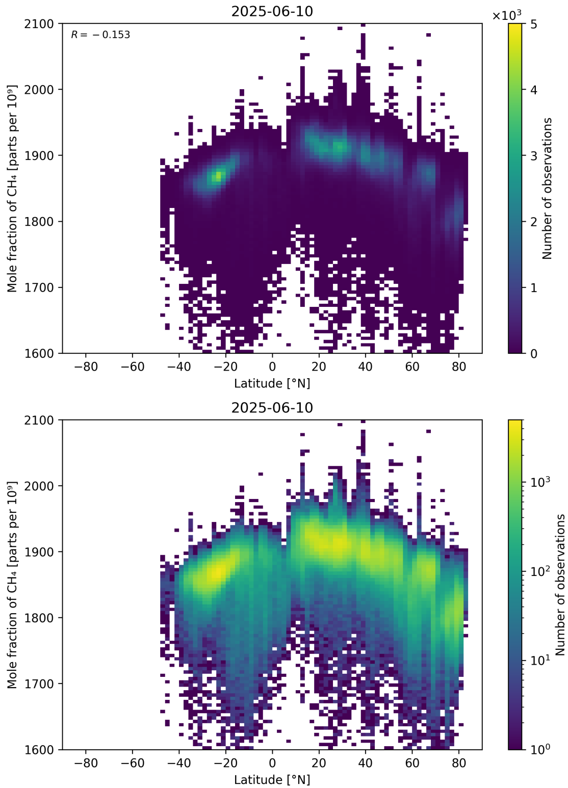
Figure 57: Scatter density plot of “Latitude” against “Mole fraction of CH 4 ” for 2025-06-09 to 2025-06-11.
