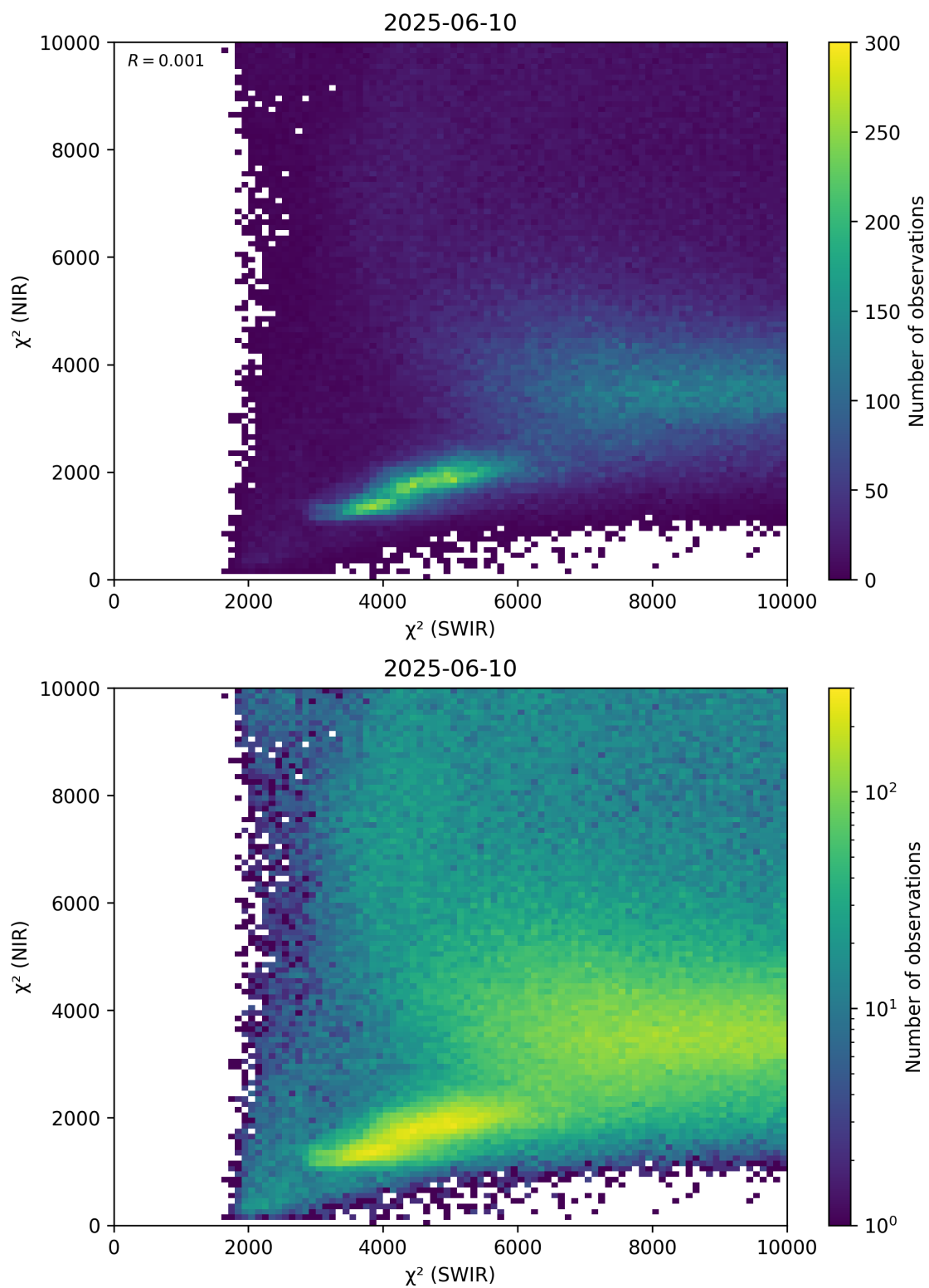
Figure 47: Scatter density plot of “ \chi^2 (SWIR)” against “ \chi^2 (NIR)” for 2025-06-09 to 2025-06-11.
