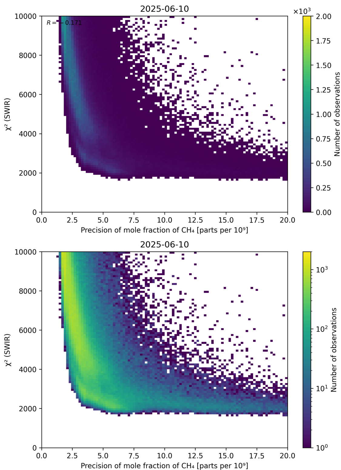
Figure 79: Scatter density plot of “Precision of mole fraction of \text{CH}_4 ” against “ \chi^2 (SWIR)” for 2025-06-09 to 2025-06-11.
