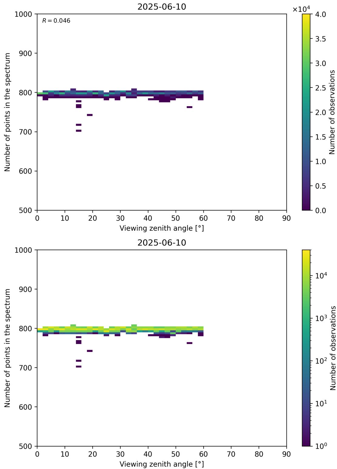
Figure 114: Scatter density plot of “Viewing zenith angle” against “Number of points in the spectrum” for 2025-06-09 to 2025-06-11.
