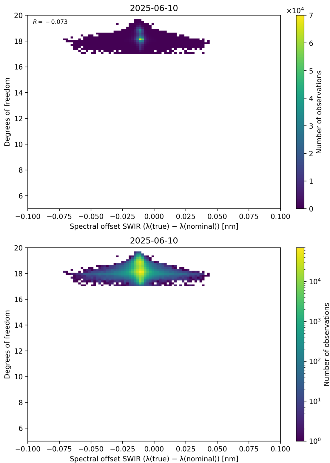
Figure 119: Scatter density plot of “Spectral offset SWIR ( \lambda_{\text{true}} - \lambda_{\text{nominal}} )” against “Degrees of freedom” for 2025-06-09 to 2025-06-11.
