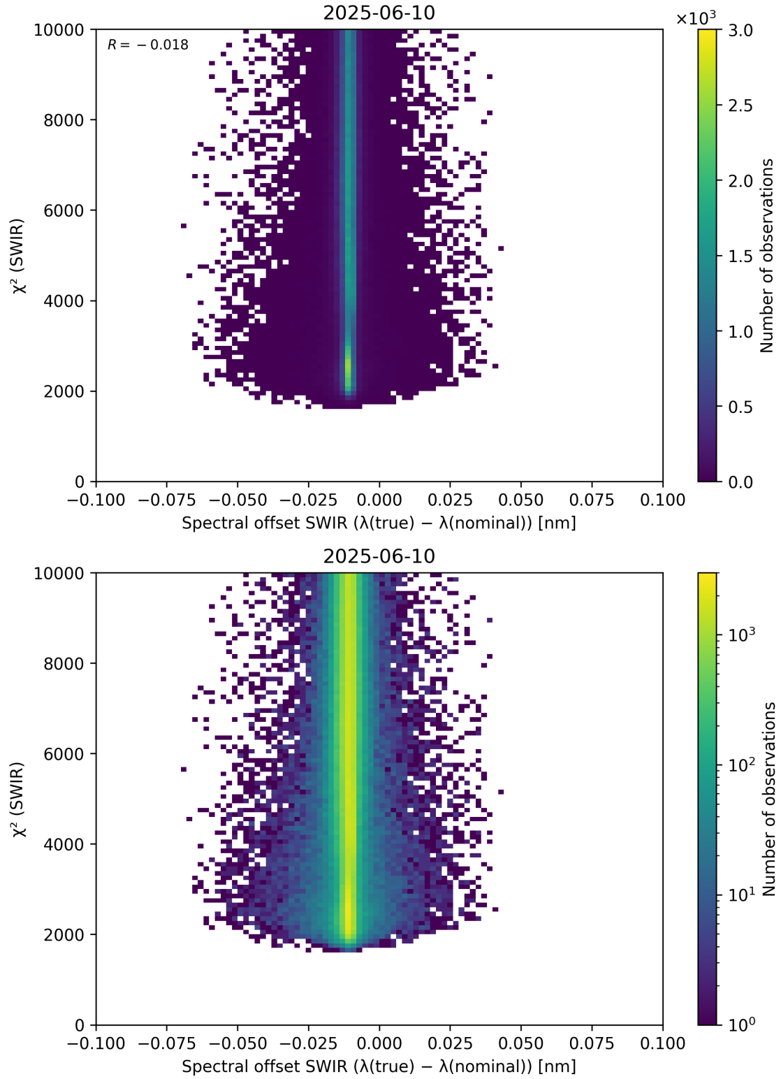
Figure 118: Scatter density plot of “Spectral offset SWIR ( \lambda_{\text{true}} - \lambda_{\text{nominal}} )” against “ \chi^2 (SWIR)” for 2025-06-09 to 2025-06-11.
