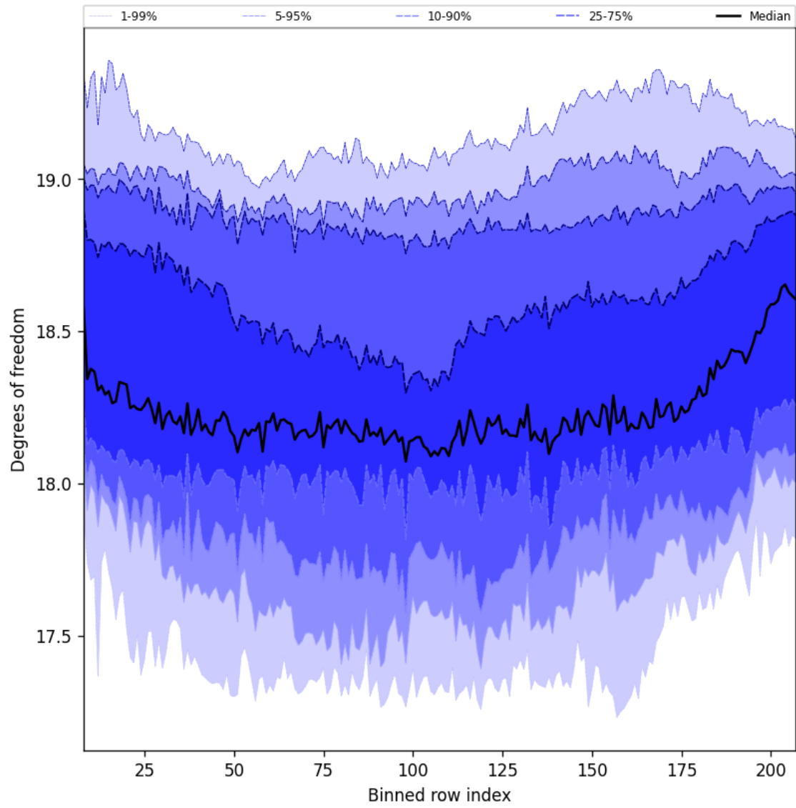
Figure 41: Along track statistics of “Degrees of freedom” for 2025-06-09 to 2025-06-11
