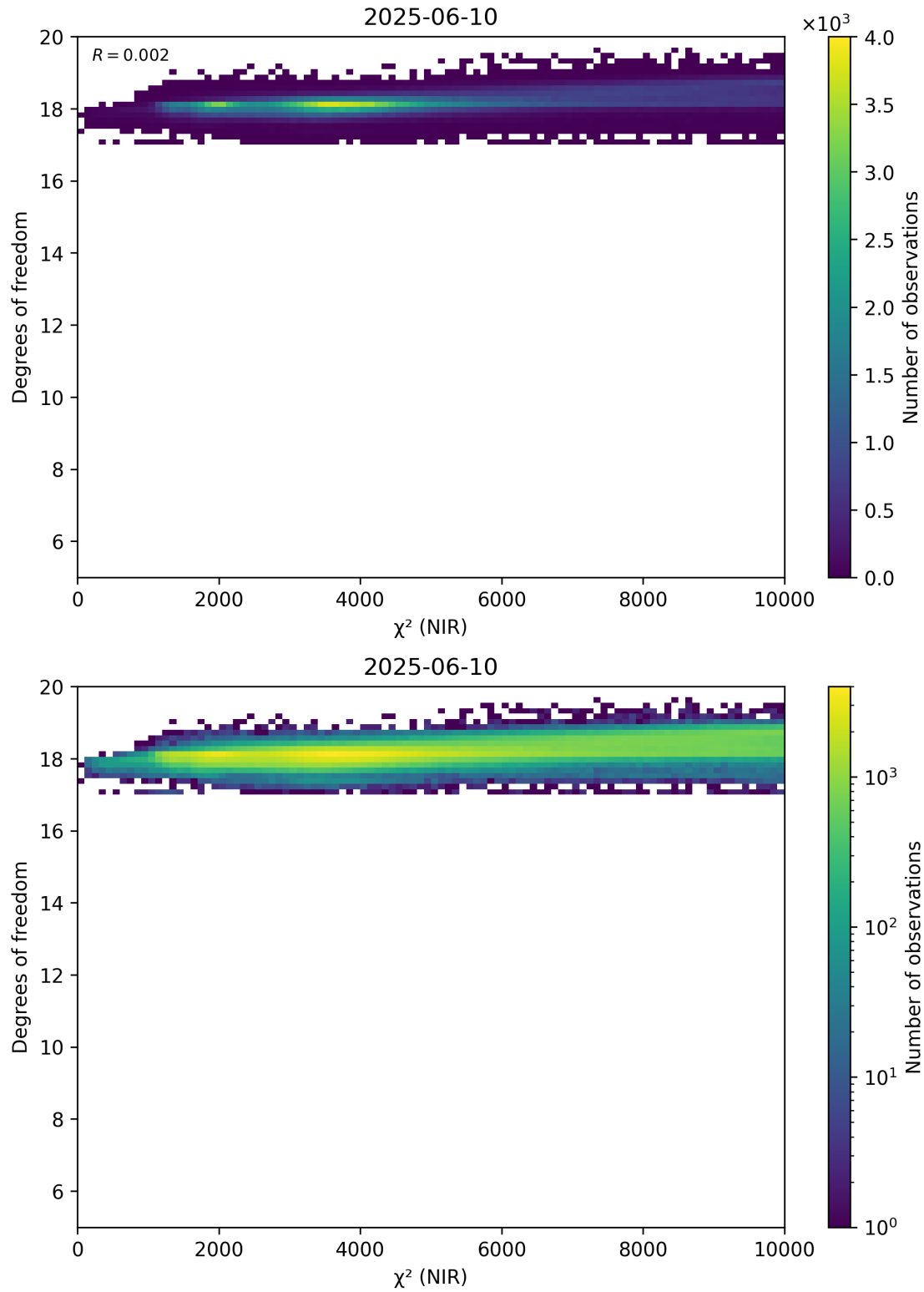
Figure 44: Scatter density plot of “ \chi^2 (NIR)” against “Degrees of freedom” for 2025-06-09 to 2025-06-11.
