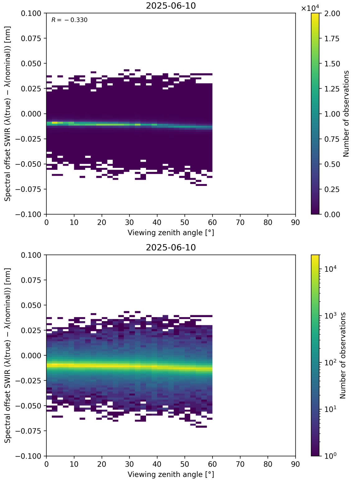
Figure 116: Scatter density plot of “Viewing zenith angle” against “Spectral offset SWIR ( \lambda_{\text{true}} - \lambda_{\text{nominal}} )” for 2025-06-09 to 2025-06-11.
