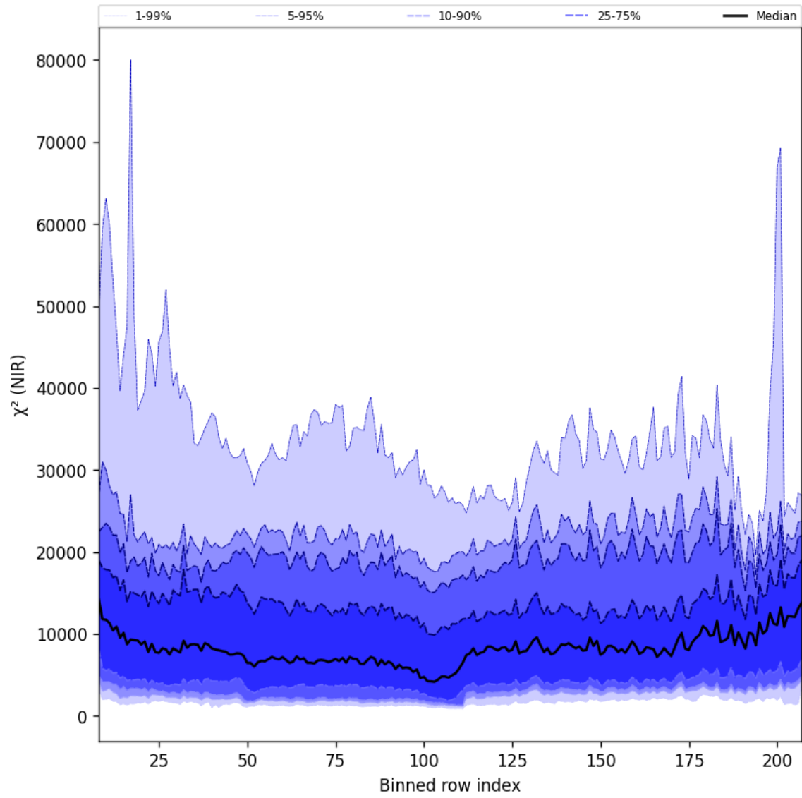
Figure 40: Along track statistics of “ \chi^2 (NIR)” for 2025-06-09 to 2025-06-11
