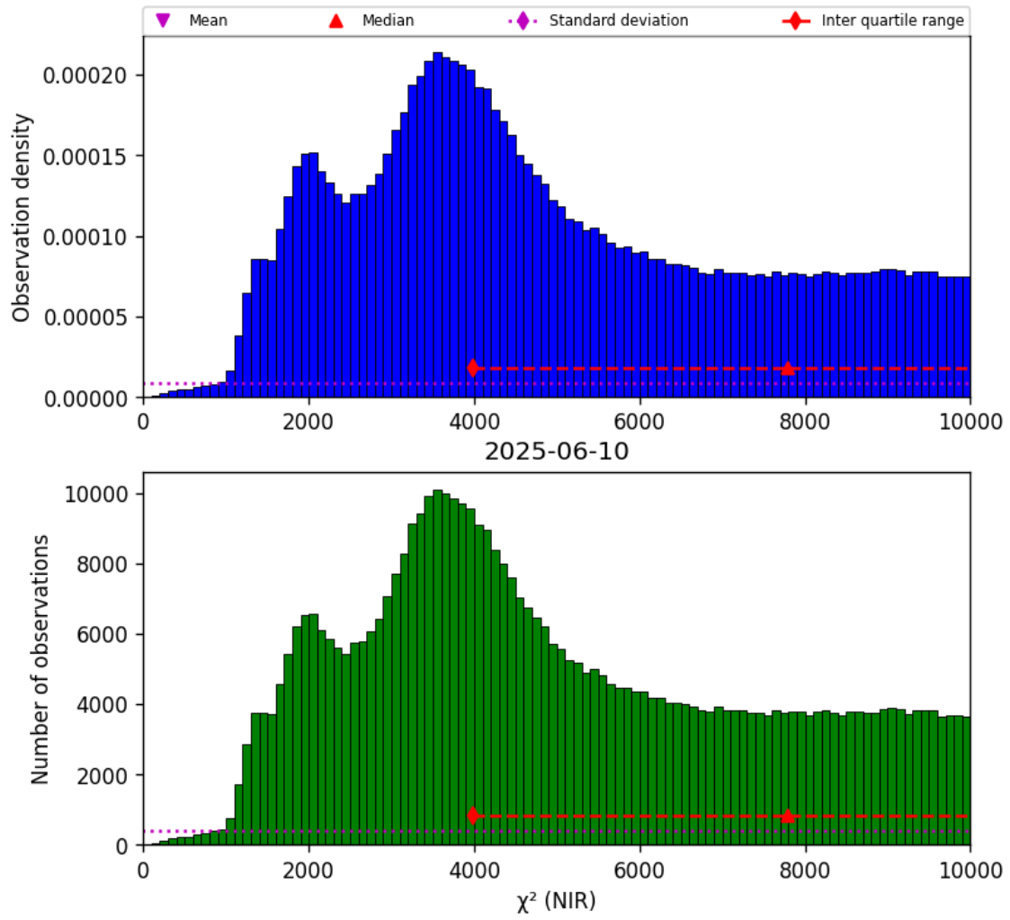
Figure 29: Histogram of " \chi^2 (NIR)" for 2025-06-09 to 2025-06-11
