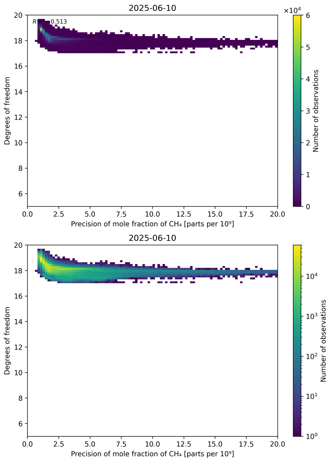
Figure 80: Scatter density plot of “Precision of mole fraction of CH 4 ” against “Degrees of freedom” for 2025-06-09 to 2025-06-11.
