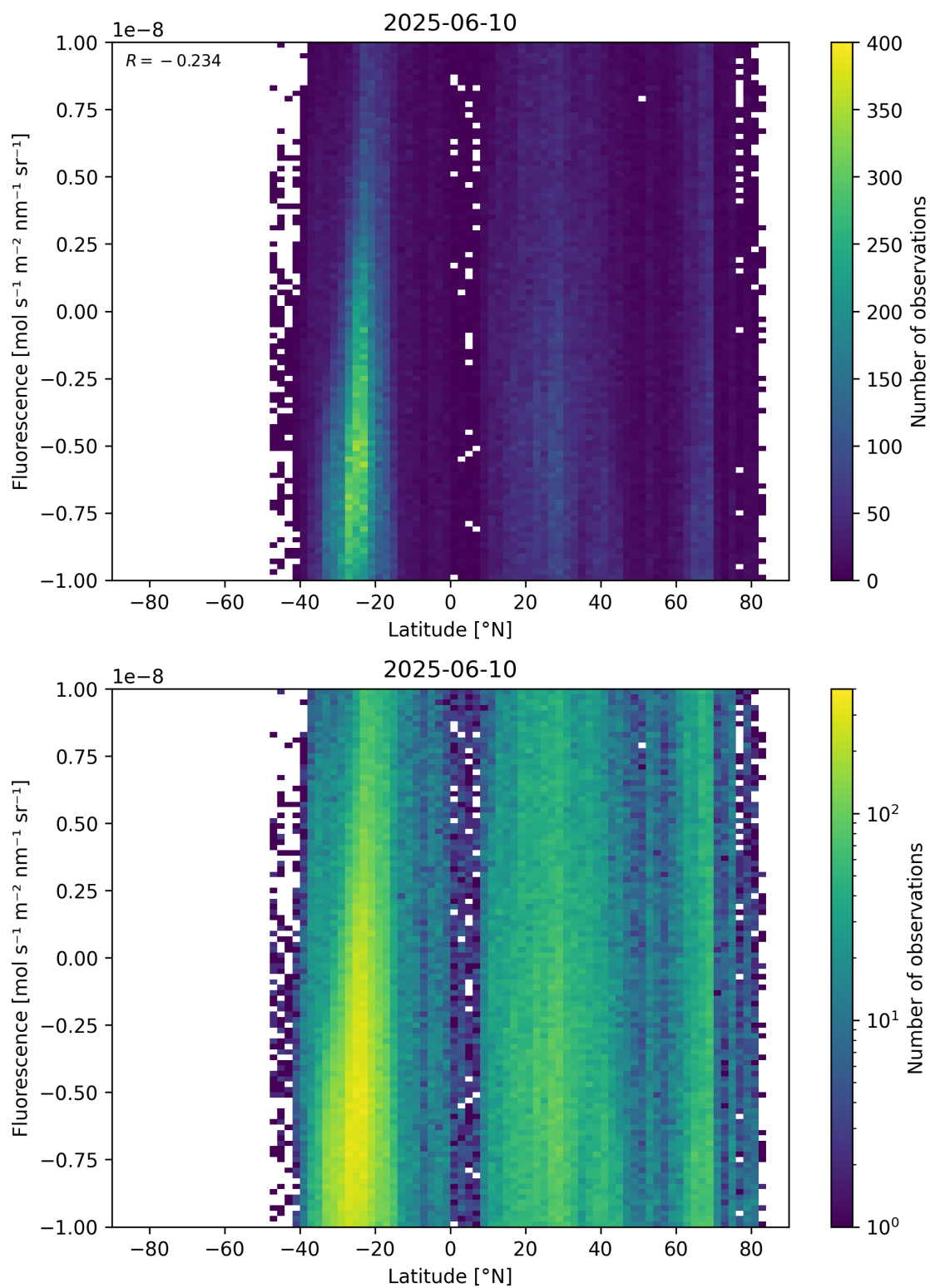
Figure 56: Scatter density plot of “Latitude” against “Fluorescence” for 2025-06-09 to 2025-06-11.
