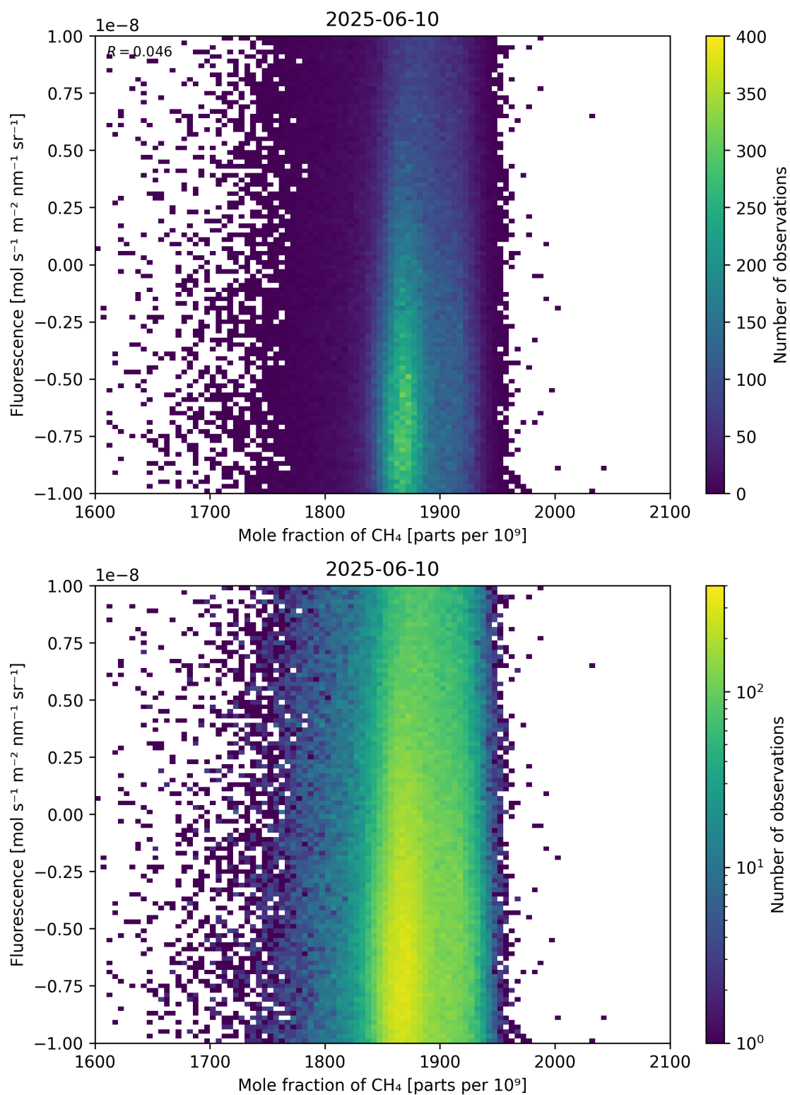
Figure 73: Scatter density plot of “Mole fraction of \text{CH}_4 ” against “Fluorescence” for 2025-06-09 to 2025-06-11.
