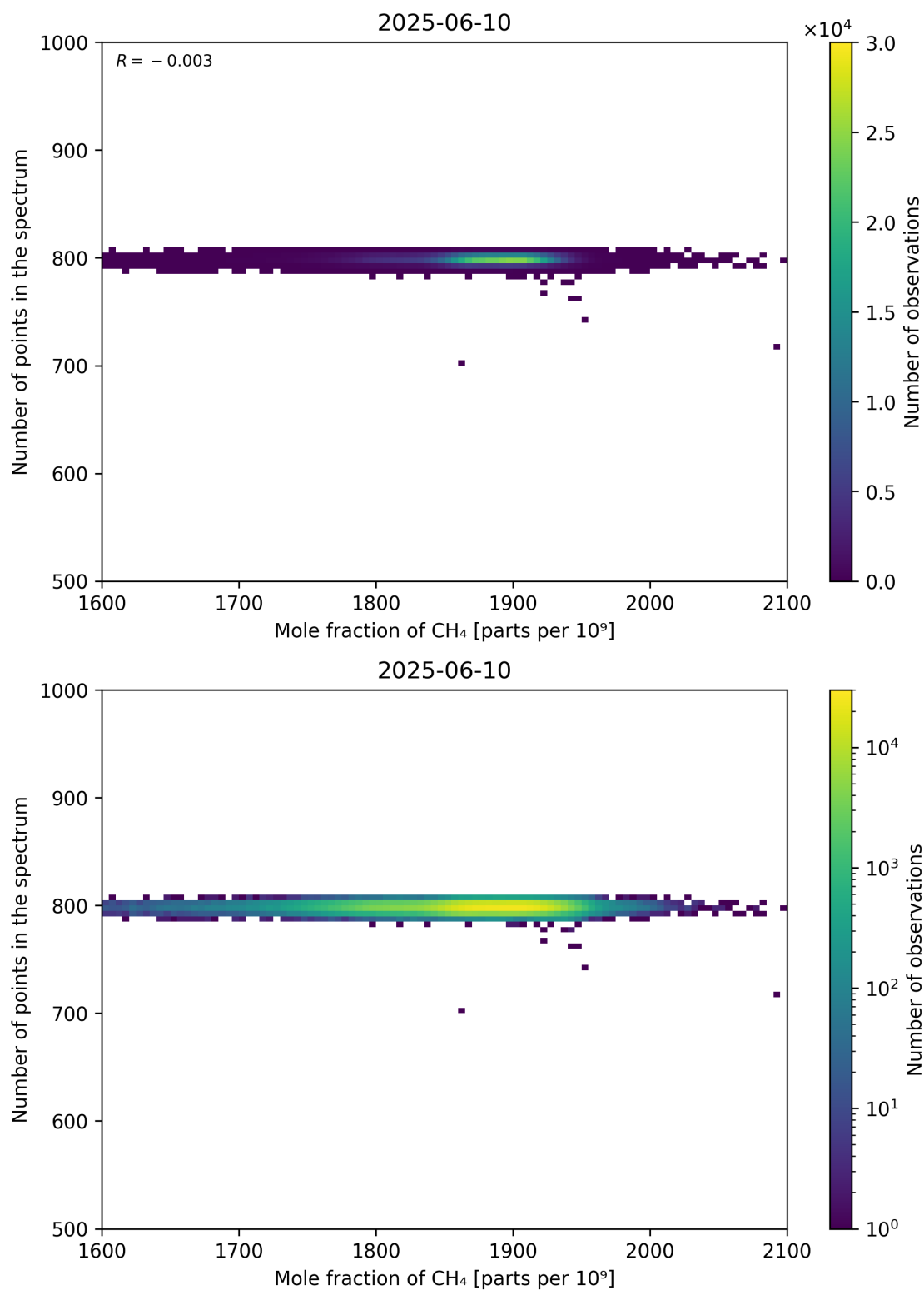
Figure 77: Scatter density plot of “Mole fraction of CH 4 ” against “Number of points in the spectrum” for 2025-06-09 to 2025-06-11.
