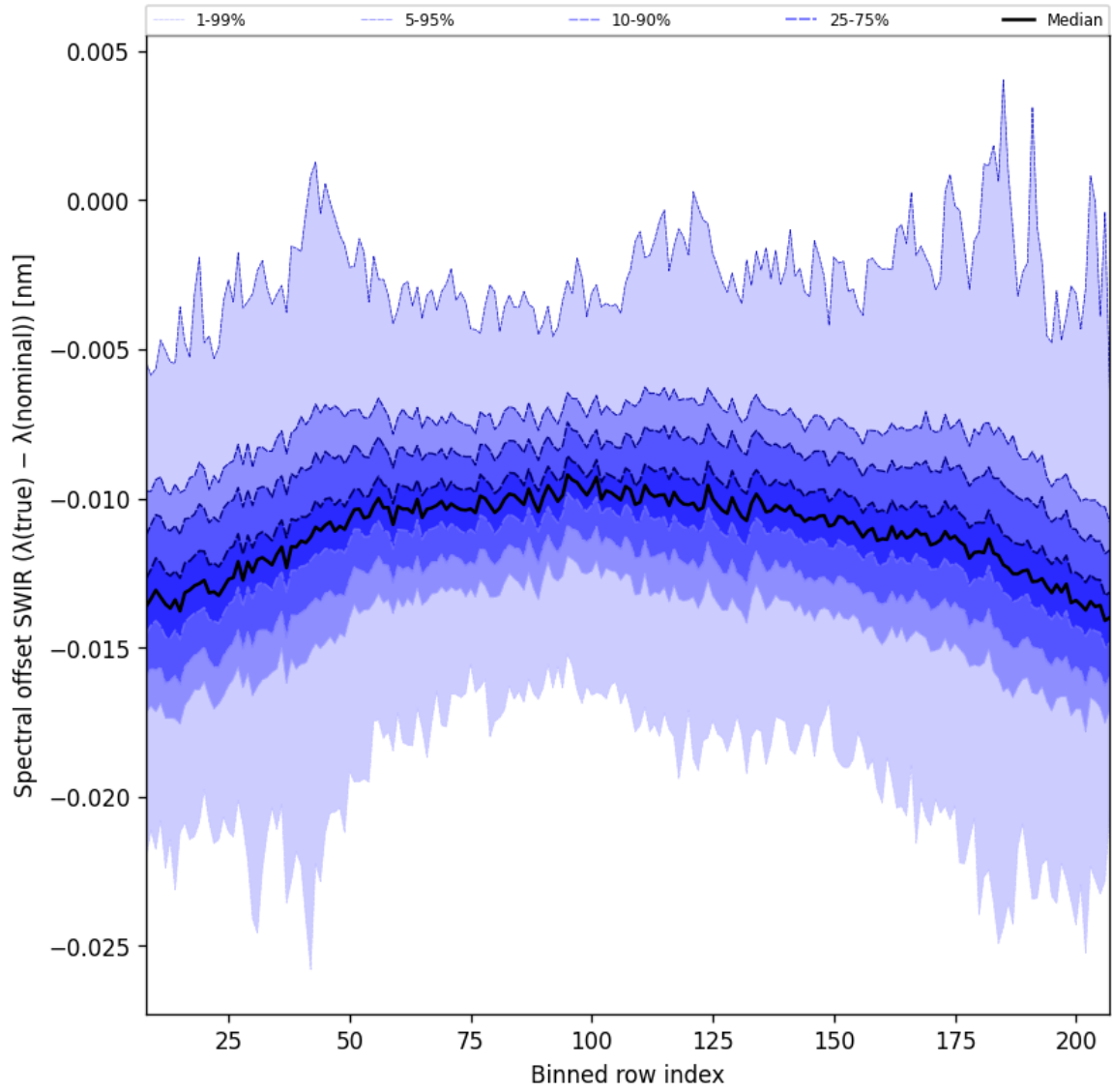
Figure 38: Along track statistics of “Spectral offset SWIR ( \lambda_{\text{true}} - \lambda_{\text{nominal}} )” for 2025-06-09 to 2025-06-11
