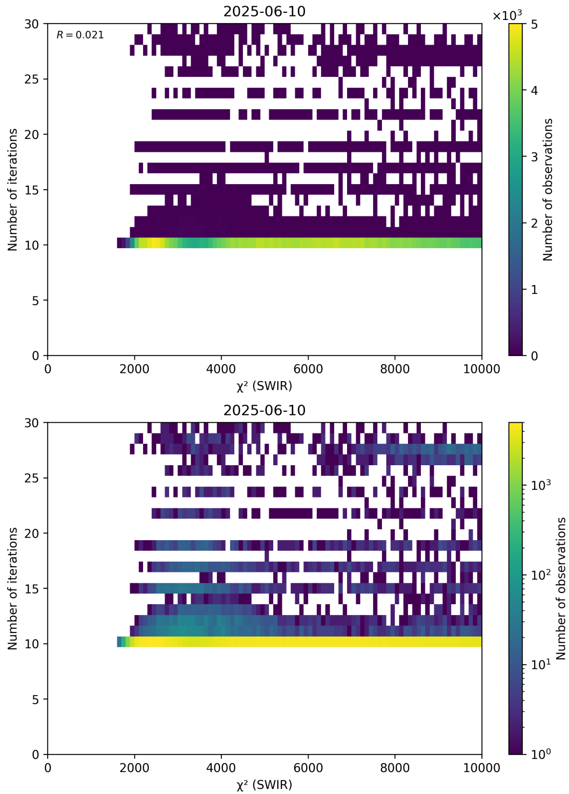
Figure 50: Scatter density plot of “ \chi^2 (SWIR)” against “Number of iterations” for 2025-06-09 to 2025-06-11.
