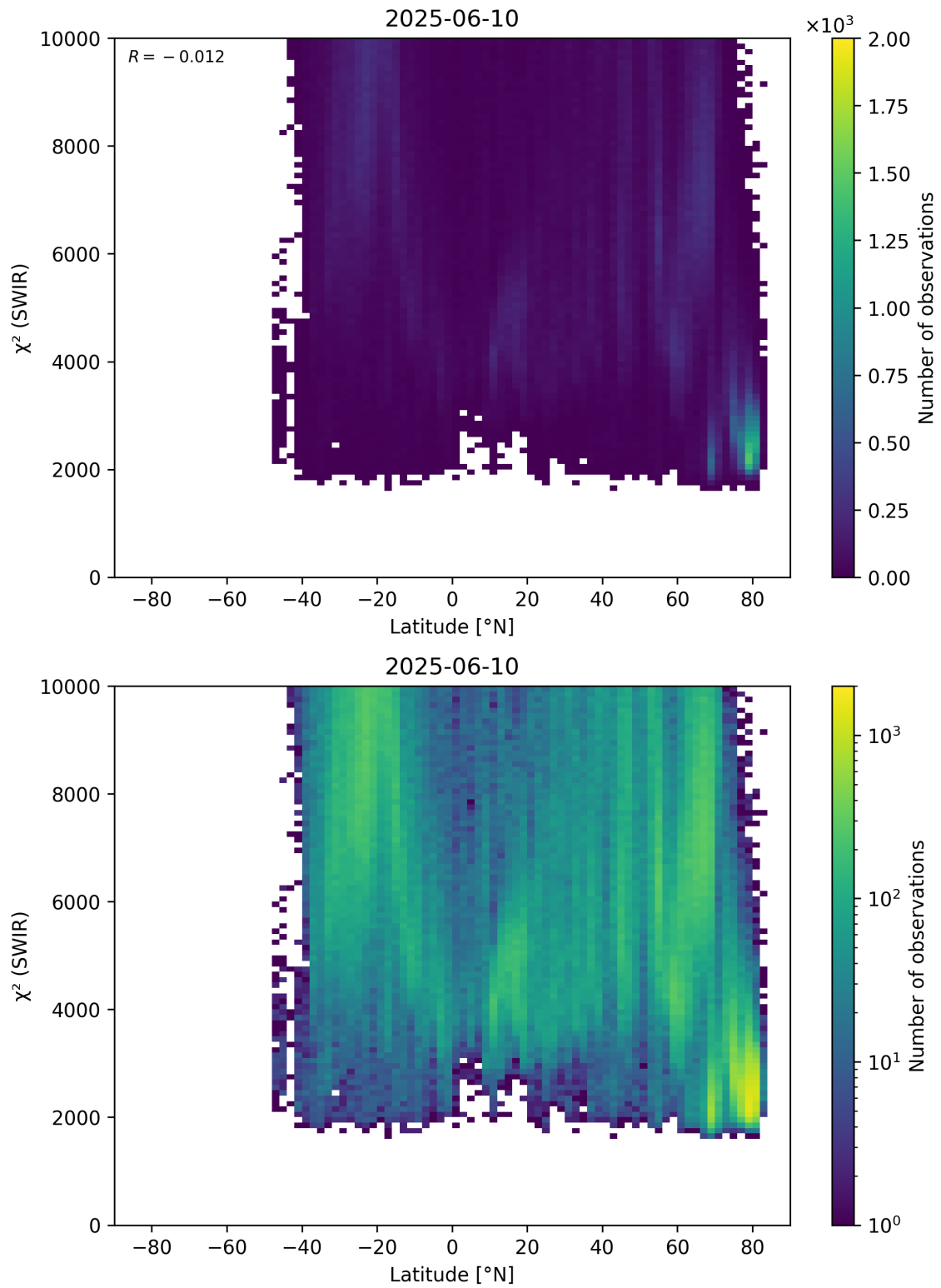
Figure 54: Scatter density plot of “Latitude” against “ \chi^2 (SWIR)” for 2025-06-09 to 2025-06-11.
