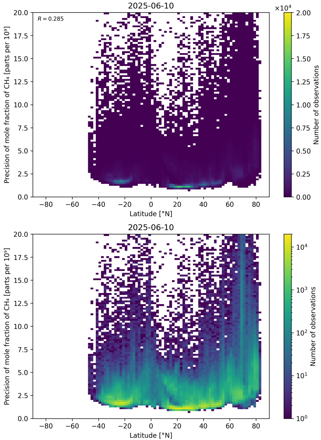
Figure 59: Scatter density plot of “Latitude” against “Precision of mole fraction of \text{CH}_4 ” for 2025-06-09 to 2025-06-11.
