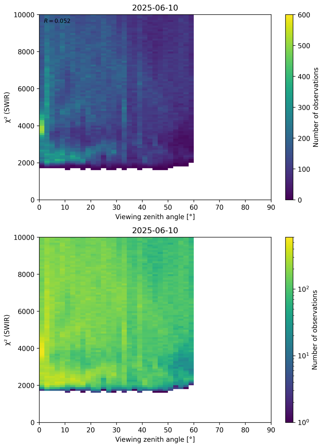
Figure 106: Scatter density plot of “Viewing zenith angle” against “ \chi^2 (SWIR)” for 2025-06-09 to 2025-06-11.
