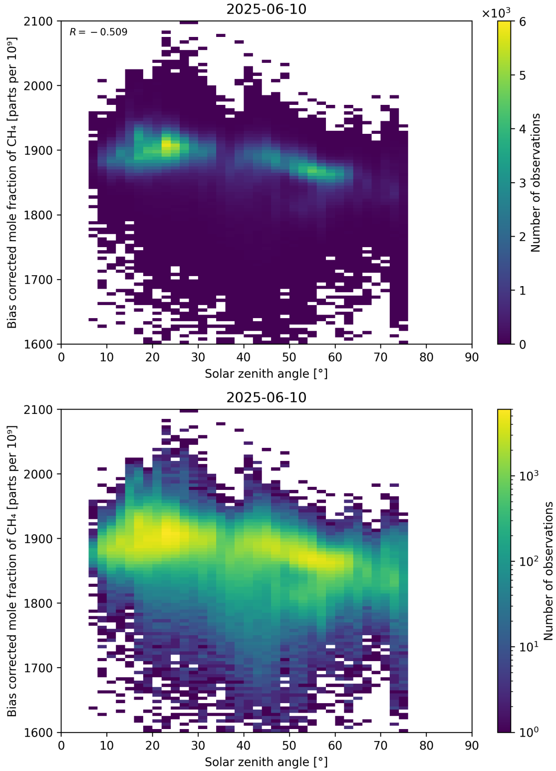
Figure 100: Scatter density plot of “Solar zenith angle” against “Bias corrected mole fraction of CH 4 ” for 2025-06-09 to 2025-06-11.
