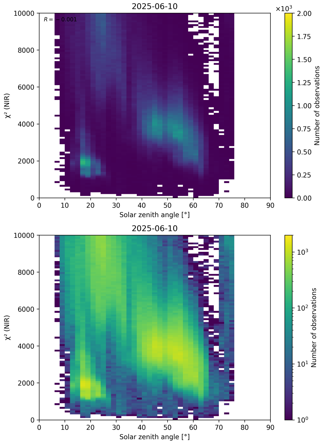
Figure 94: Scatter density plot of “Solar zenith angle” against “ \chi^2 (NIR)” for 2025-06-09 to 2025-06-11.
