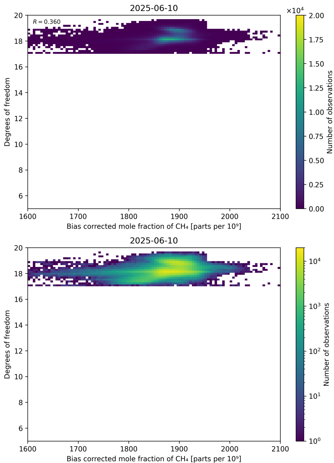
Figure 65: Scatter density plot of “Bias corrected mole fraction of CH 4 ” against “Degrees of freedom” for 2025-06-09 to 2025-06-11.
