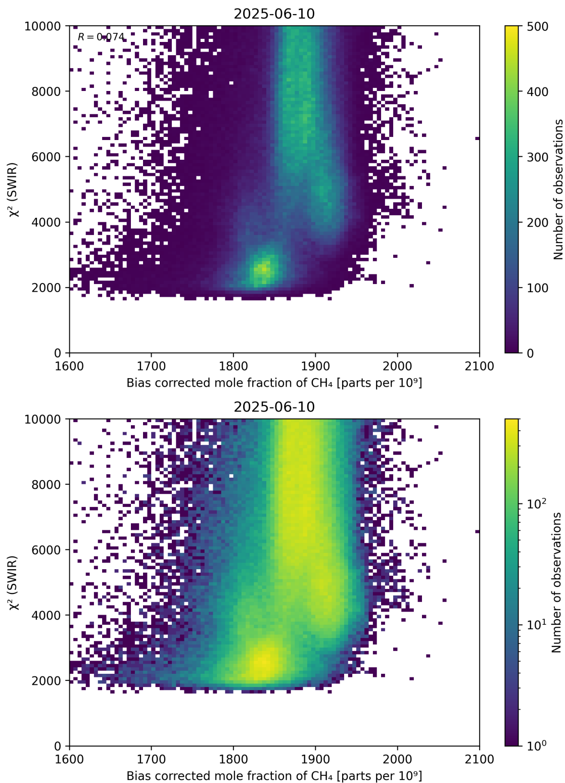
Figure 64: Scatter density plot of “Bias corrected mole fraction of \text{CH}_4 ” against “ \chi^2 (SWIR)” for 2025-06-09 to 2025-06-11.
