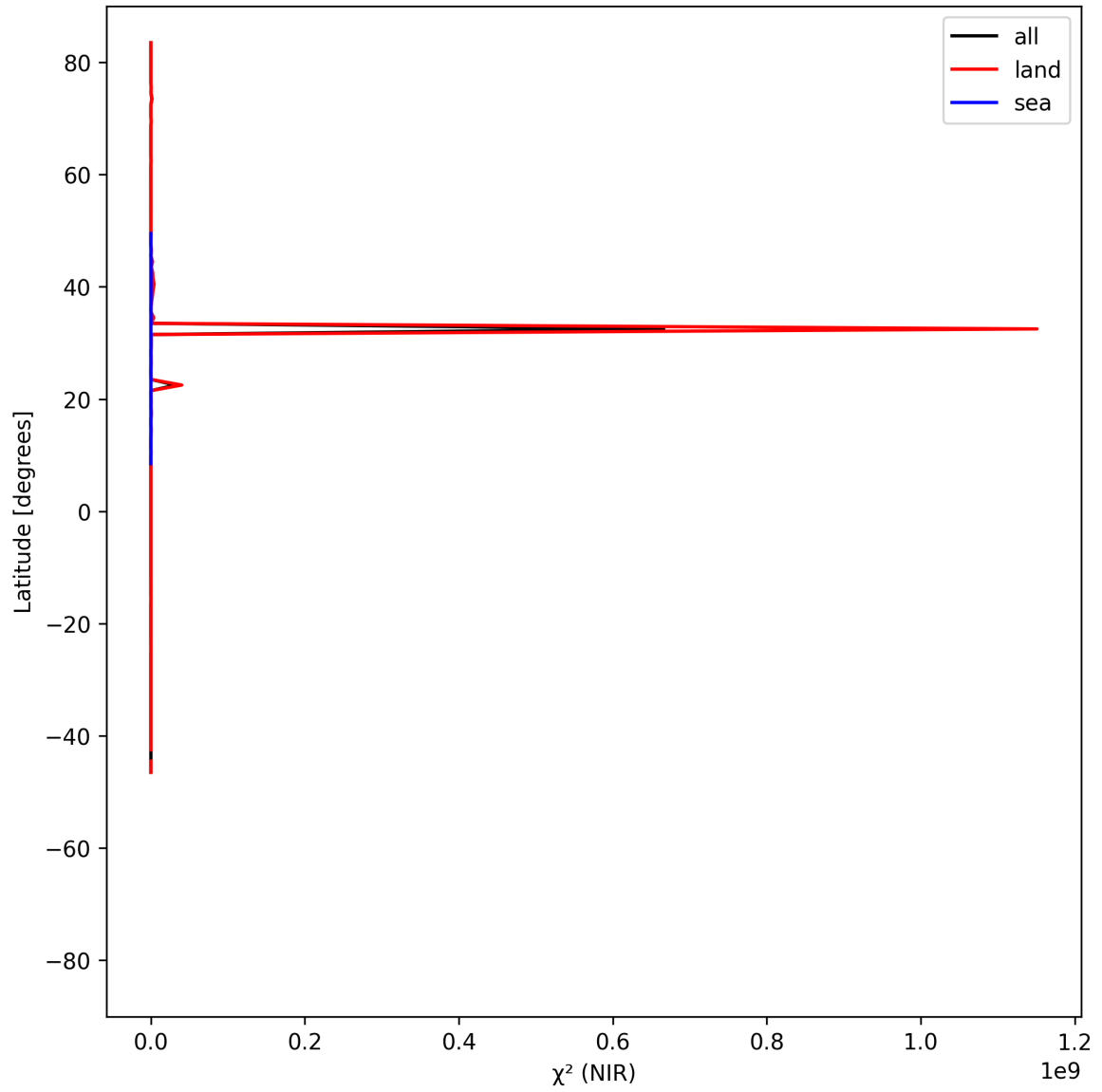
Figure 18: Zonal average of “ \chi^2 (NIR)” for 2025-06-09 to 2025-06-11.
