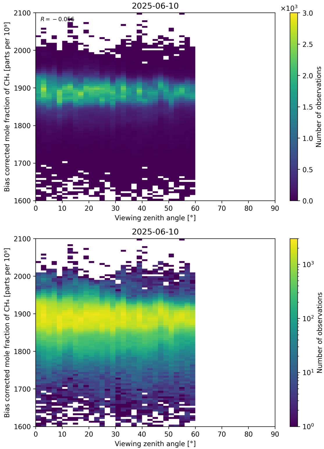
Figure 111: Scatter density plot of “Viewing zenith angle” against “Bias corrected mole fraction of CH 4 ” for 2025-06-09 to 2025-06-11.
