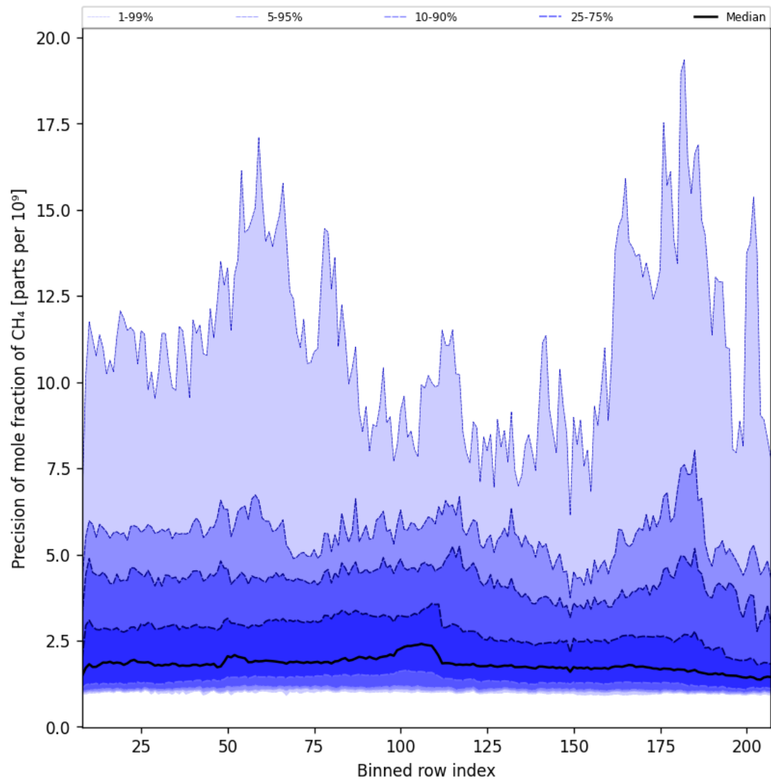
Figure 35: Along track statistics of “Precision of mole fraction of CH 4 ” for 2025-06-09 to 2025-06-11
