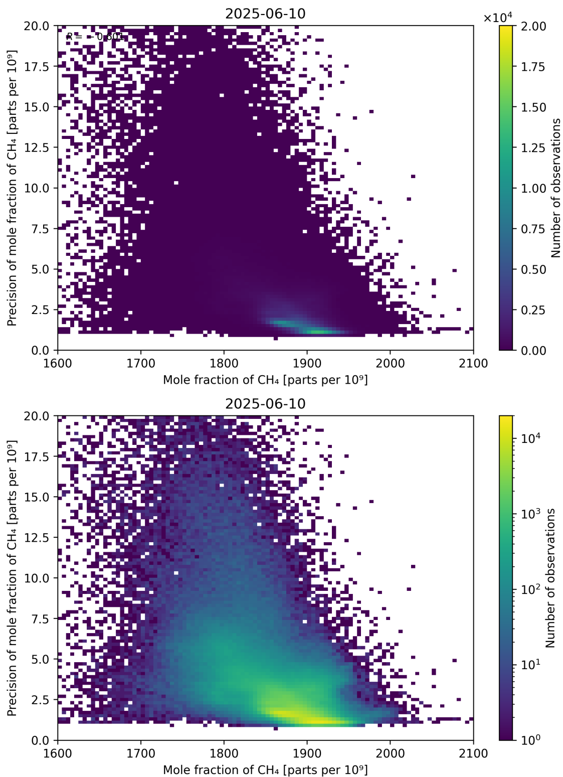
Figure 75: Scatter density plot of “Mole fraction of CH 4 ” against “Precision of mole fraction of CH 4 ” for 2025-06-09 to 2025-06-11.
