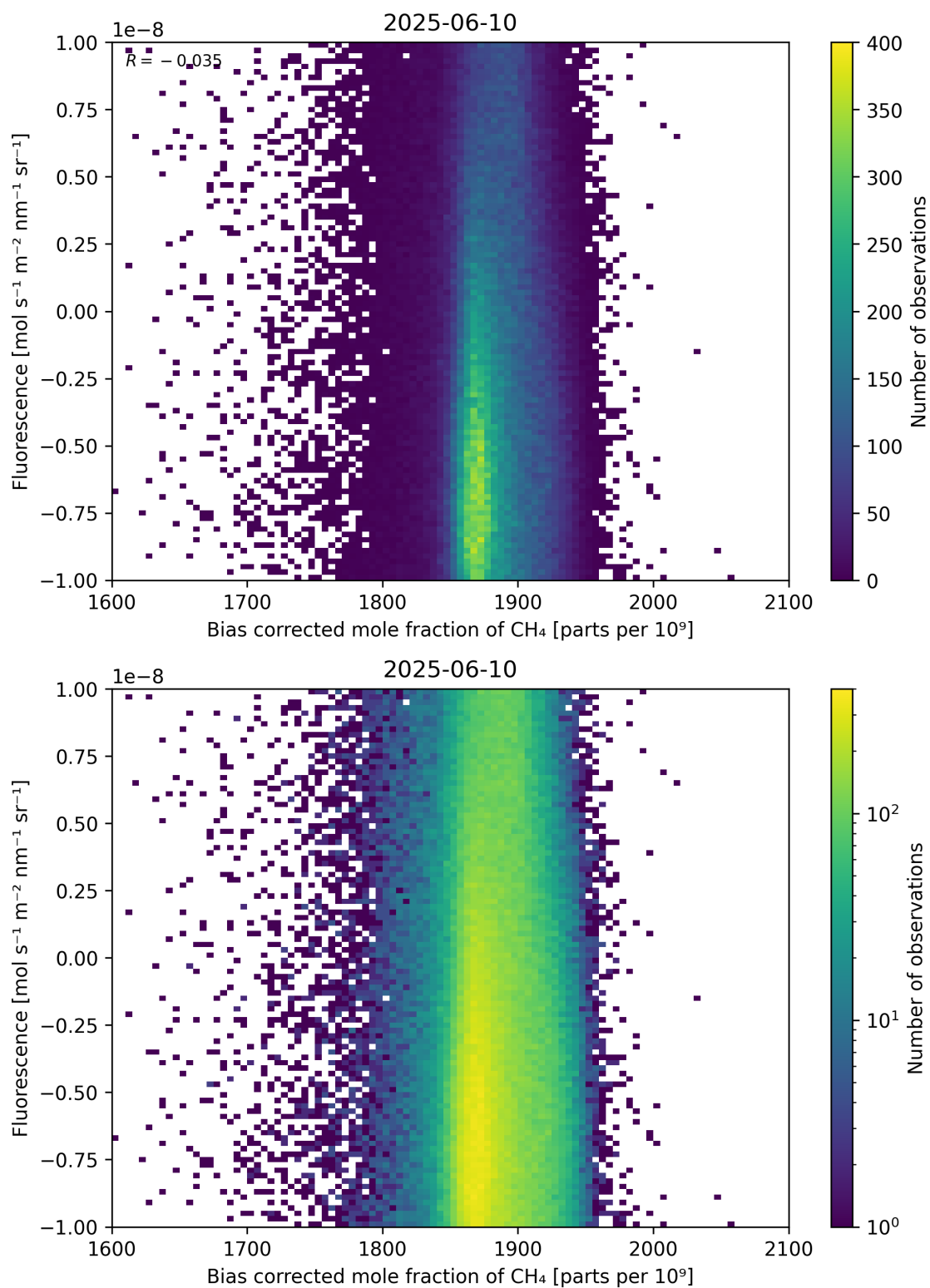
Figure 66: Scatter density plot of “Bias corrected mole fraction of \text{CH}_4 ” against “Fluorescence” for 2025-06-09 to 2025-06-11.
