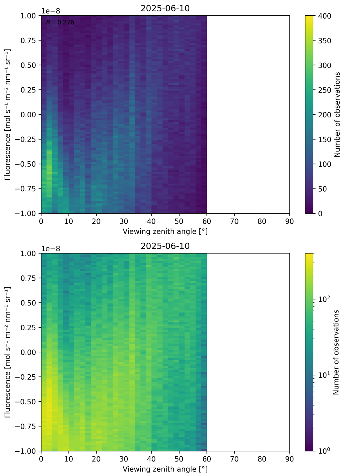
Figure 108: Scatter density plot of “Viewing zenith angle” against “Fluorescence” for 2025-06-09 to 2025-06-11.
