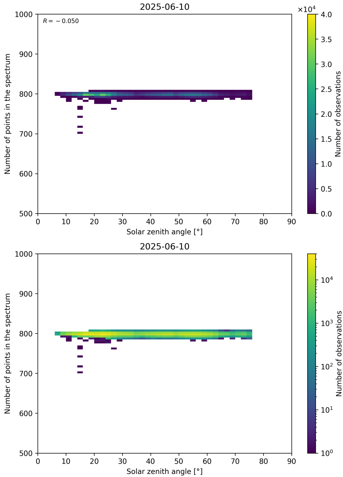
Figure 103: Scatter density plot of “Solar zenith angle” against “Number of points in the spectrum” for 2025-06-09 to 2025-06-11.
