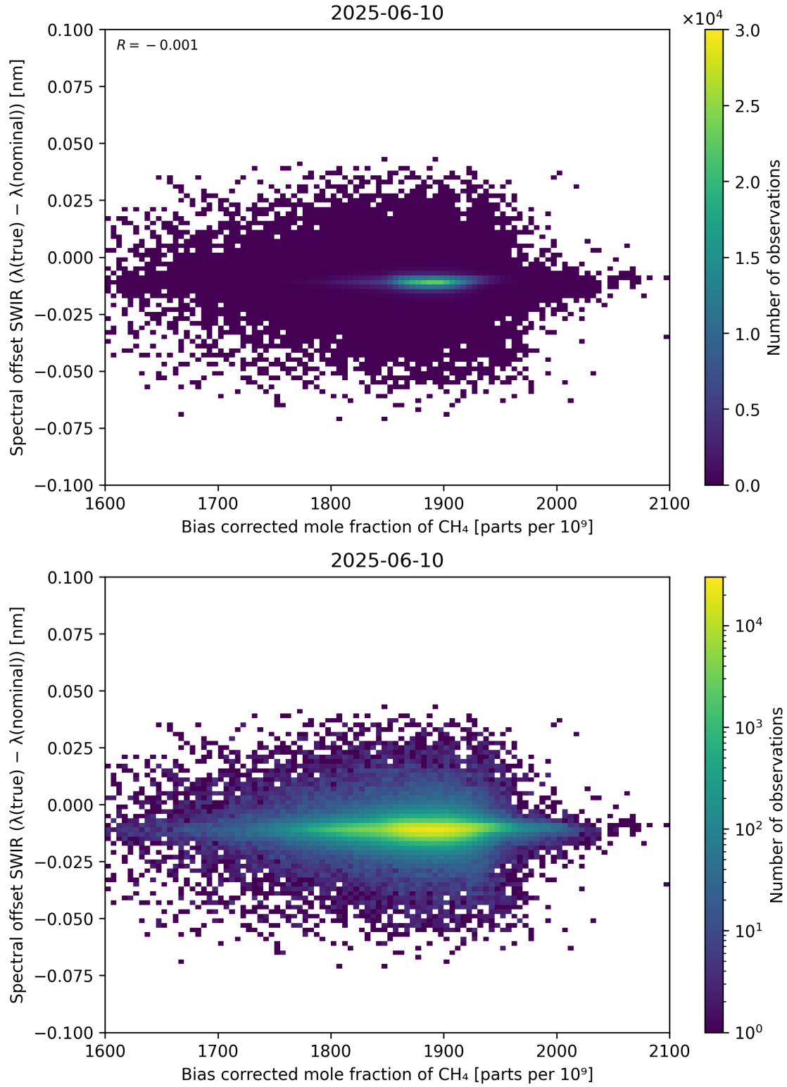
Figure 69: Scatter density plot of “Bias corrected mole fraction of CH 4 ” against “Spectral offset SWIR ( \lambda_{\text{true}} - \lambda_{\text{nominal}} )” for 2025-06-09 to 2025-06-11.
