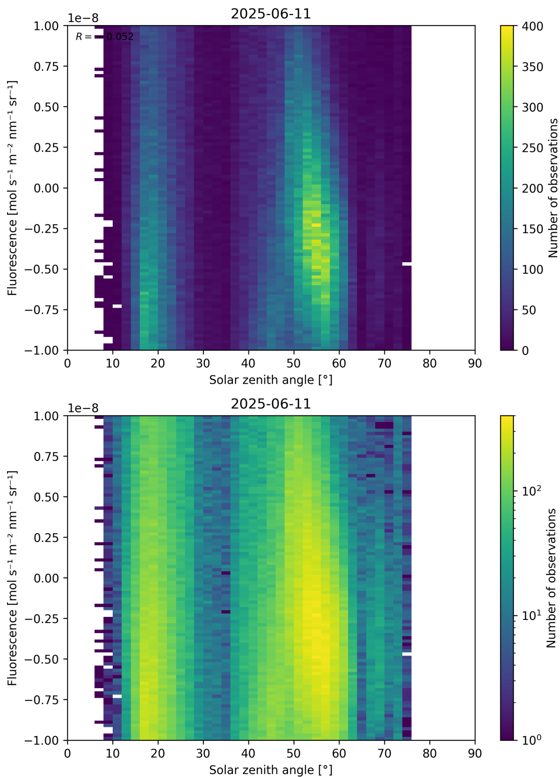
Figure 97: Scatter density plot of “Solar zenith angle” against “Fluorescence” for 2025-06-11 to 2025-06-12.
