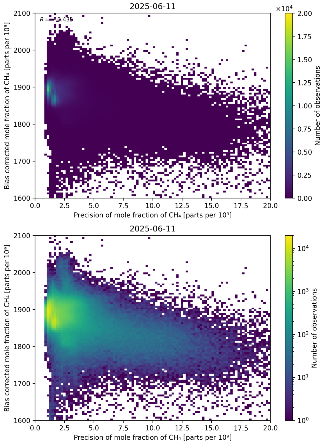
Figure 82: Scatter density plot of “Precision of mole fraction of CH 4 ” against “Bias corrected mole fraction of CH 4 ” for 2025-06-11 to 2025-06-12.
