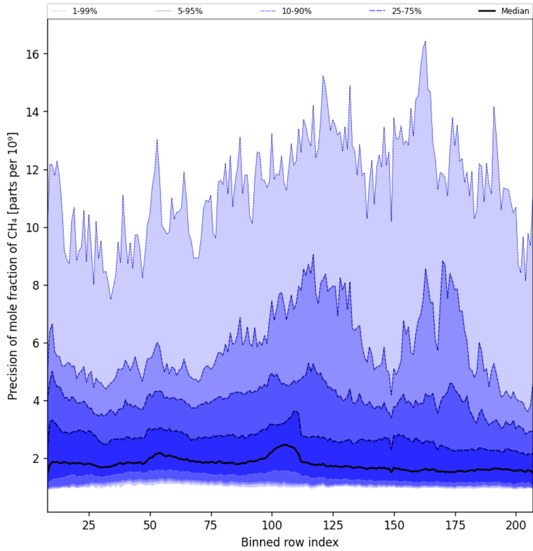
Figure 35: Along track statistics of “Precision of mole fraction of CH 4 ” for 2025-06-11 to 2025-06-12
