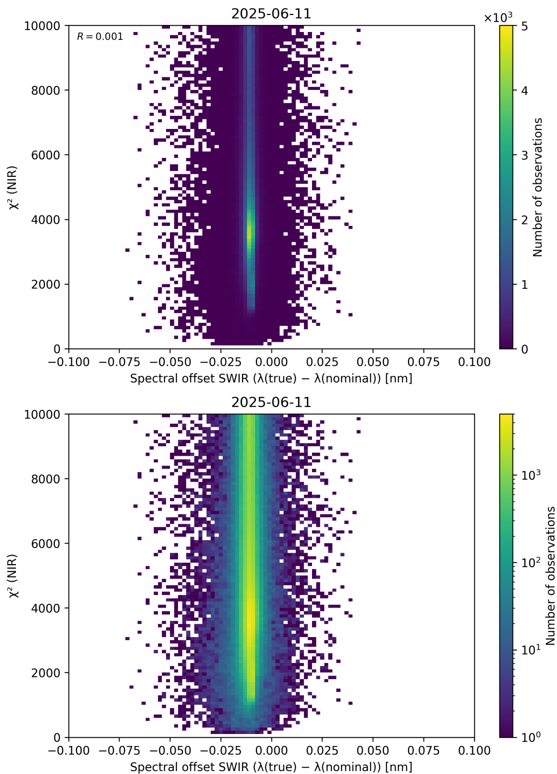
Figure 117: Scatter density plot of “Spectral offset SWIR ( \lambda_{\text{true}} - \lambda_{\text{nominal}} )” against “ \chi^2 (NIR)” for 2025-06-11 to 2025-06-12.
