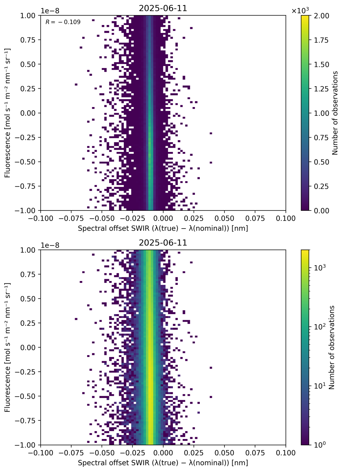
Figure 120: Scatter density plot of “Spectral offset SWIR ( \lambda_{\text{true}} - \lambda_{\text{nominal}} )” against “Fluorescence” for 2025-06-11 to 2025-06-12.
