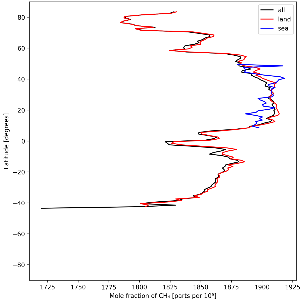
Figure 12: Zonal average of “Mole fraction of \text{CH}_4 ” for 2025-06-11 to 2025-06-12.
