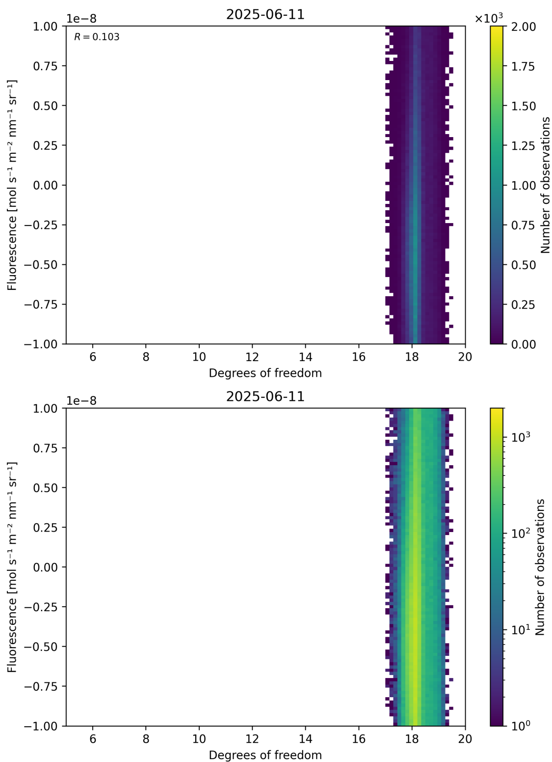
Figure 51: Scatter density plot of “Degrees of freedom” against “Fluorescence” for 2025-06-11 to 2025-06-12.
