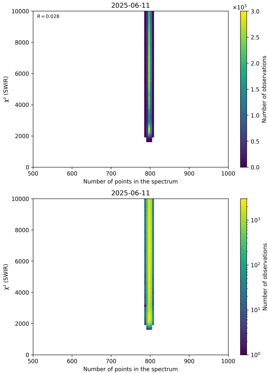
Figure 89: Scatter density plot of “Number of points in the spectrum” against “ \chi^2 (SWIR)” for 2025-06-11 to 2025-06-12.
