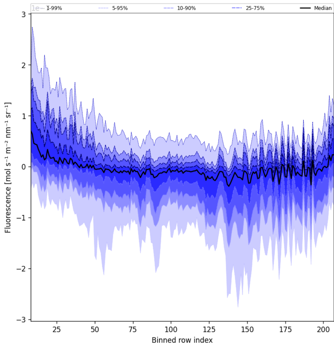
Figure 43: Along track statistics of “Fluorescence” for 2025-06-11 to 2025-06-12
