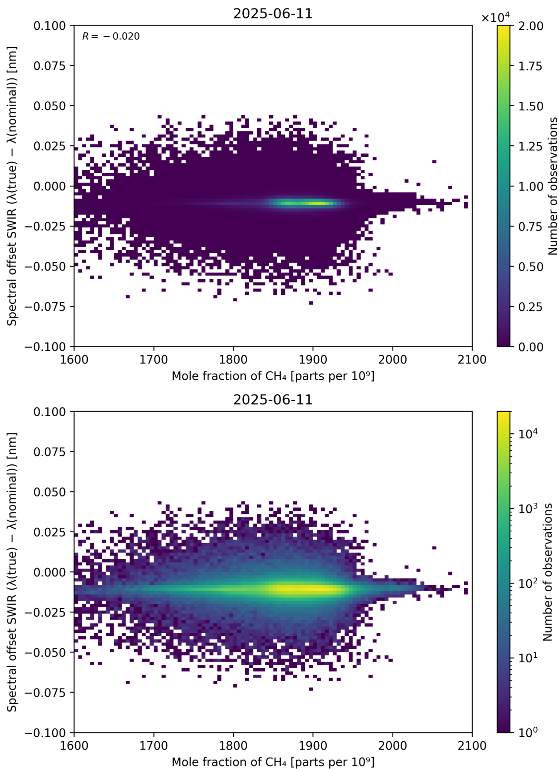
Figure 86: Scatter density plot of “Mole fraction of \text{CH}_4 ” against “Spectral offset SWIR ( \lambda_{\text{true}} - \lambda_{\text{nominal}} )” for 2025-06-11 to 2025-06-12.
