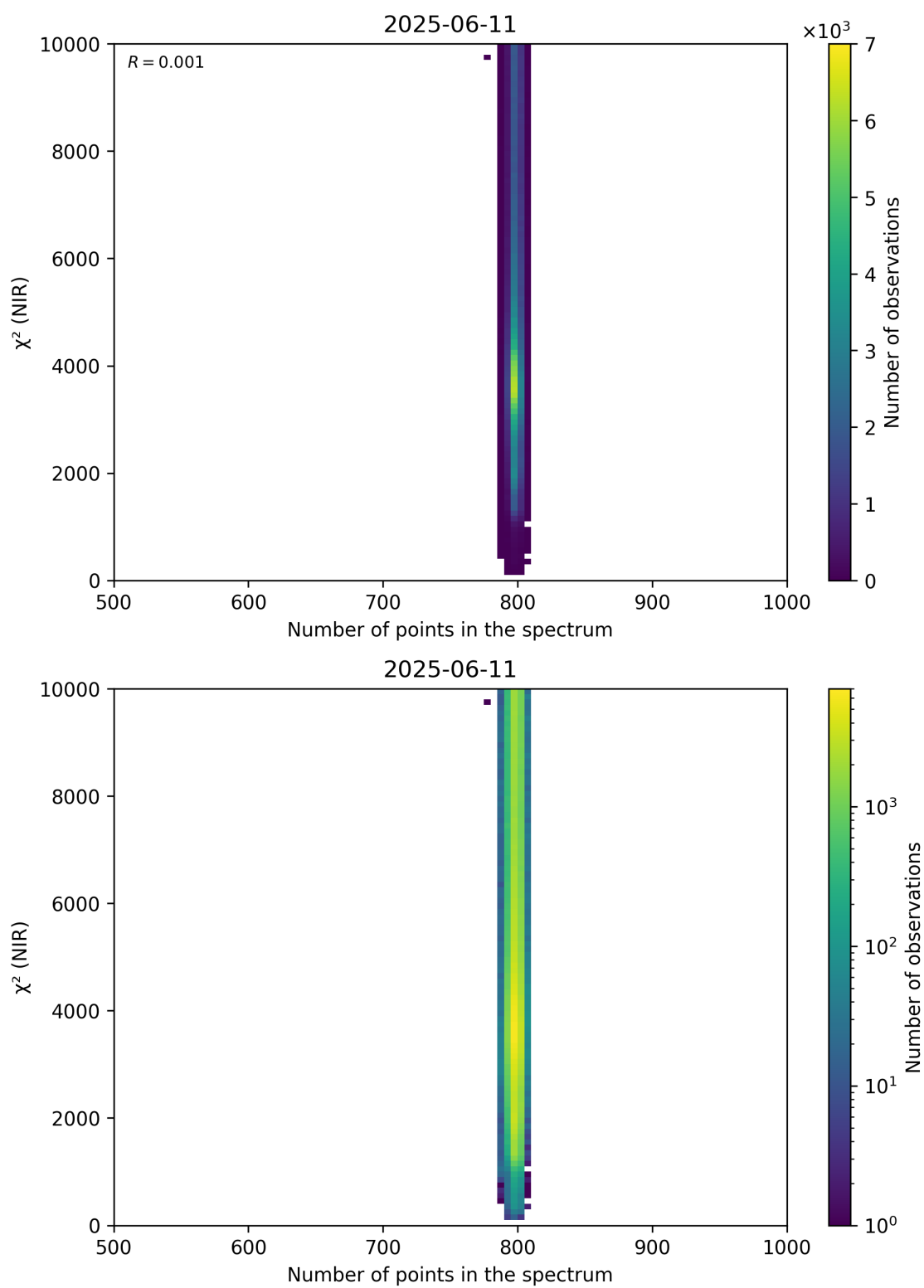
Figure 88: Scatter density plot of “Number of points in the spectrum” against “ \chi^2 (NIR)” for 2025-06-11 to 2025-06-12.
