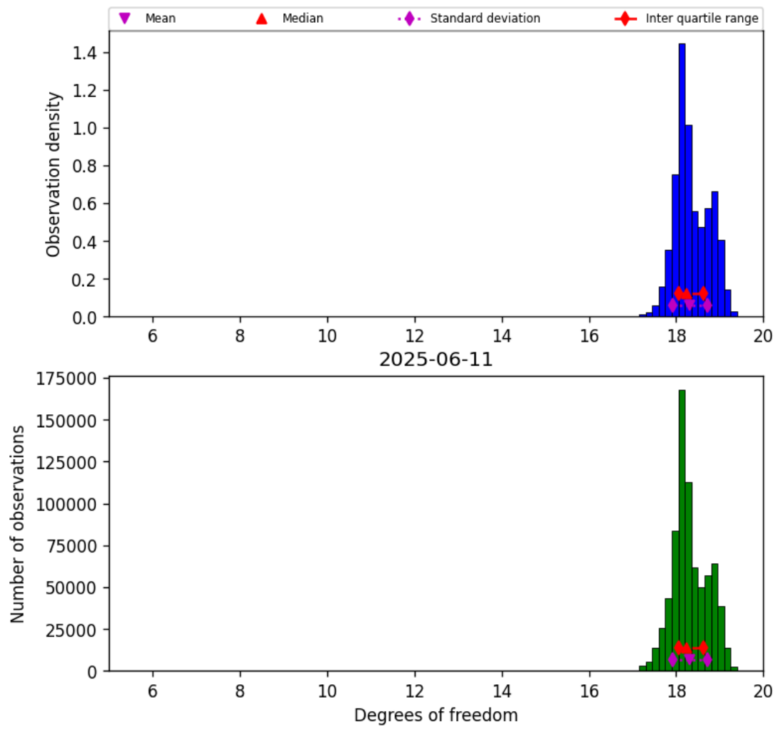
Figure 30: Histogram of “Degrees of freedom” for 2025-06-11 to 2025-06-12
