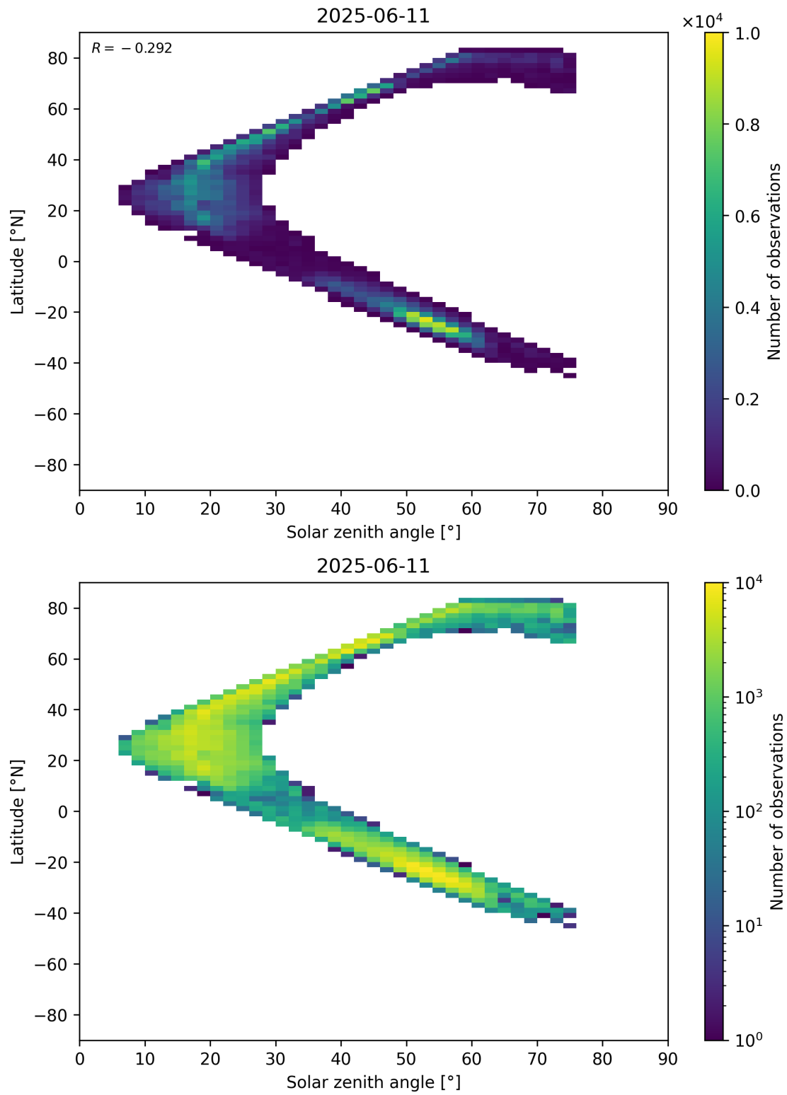
Figure 98: Scatter density plot of “Solar zenith angle” against “Latitude” for 2025-06-11 to 2025-06-12.
