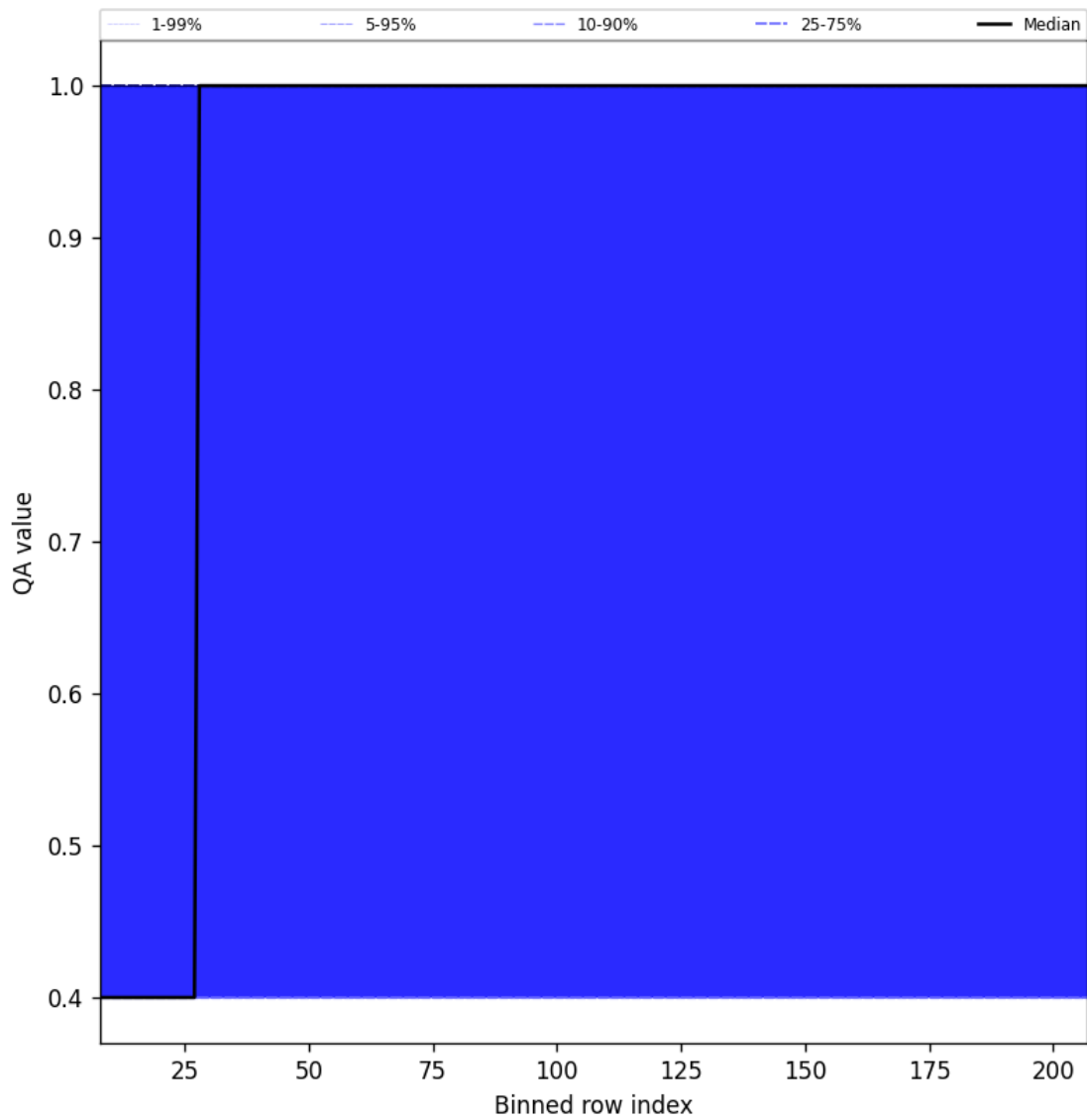
Figure 33: Along track statistics of “QA value” for 2025-06-11 to 2025-06-12
