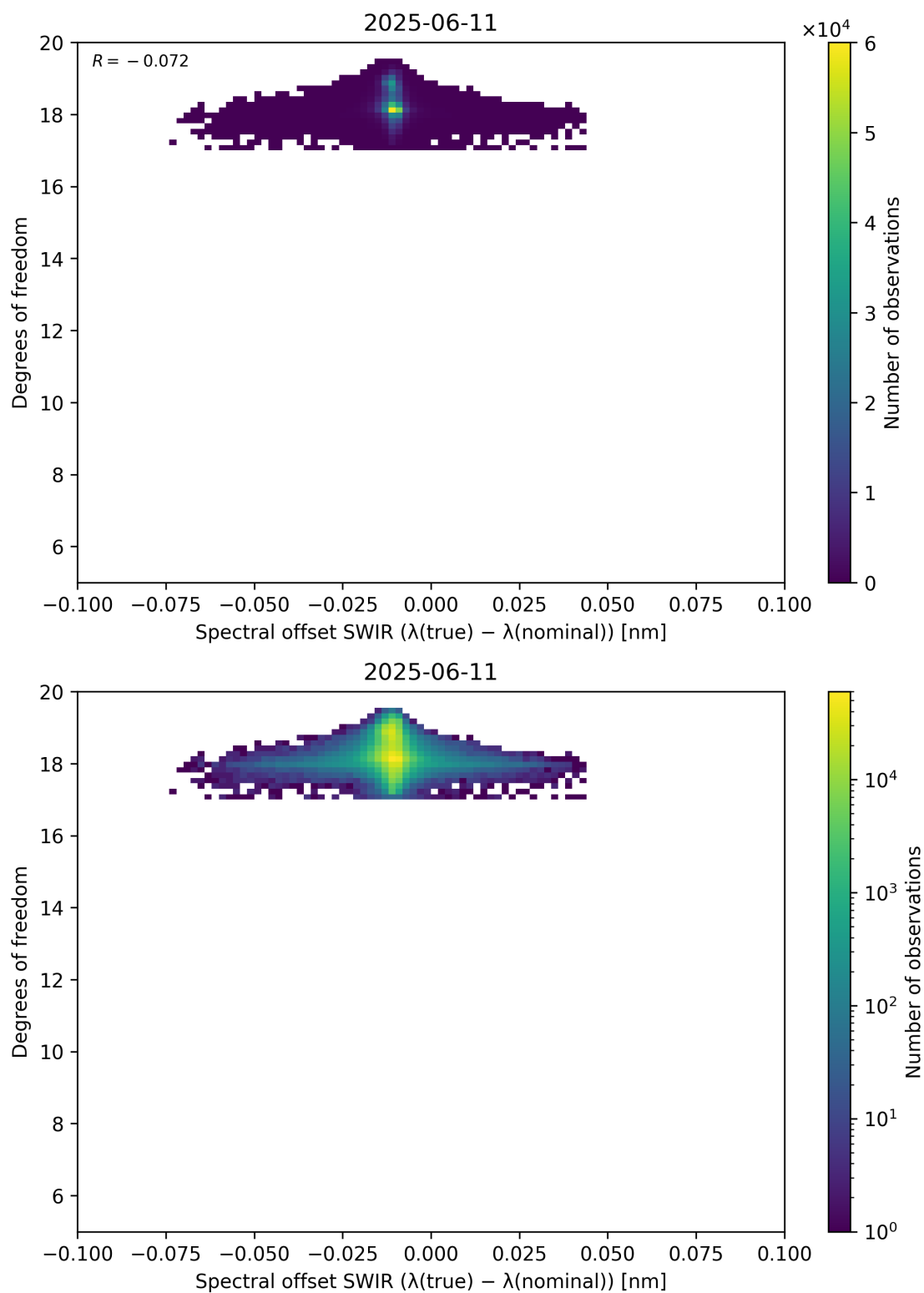
Figure 119: Scatter density plot of “Spectral offset SWIR ( \lambda_{\text{true}} - \lambda_{\text{nominal}} )” against “Degrees of freedom” for 2025-06-11 to 2025-06-12.
