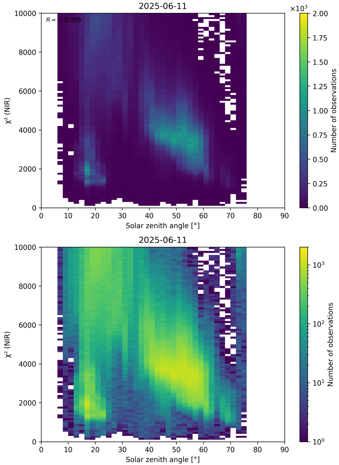
Figure 94: Scatter density plot of “Solar zenith angle” against “ \chi^2 (NIR)” for 2025-06-11 to 2025-06-12.
