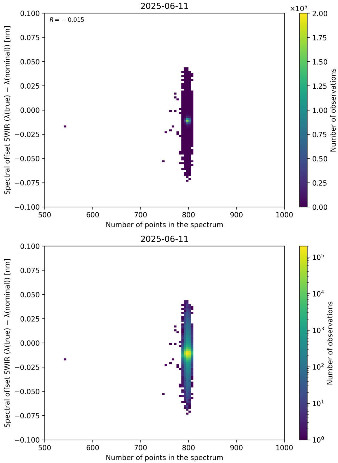
Figure 93: Scatter density plot of “Number of points in the spectrum” against “Spectral offset SWIR ( \lambda_{\text{true}} - \lambda_{\text{nominal}} )” for 2025-06-11 to 2025-06-12.
