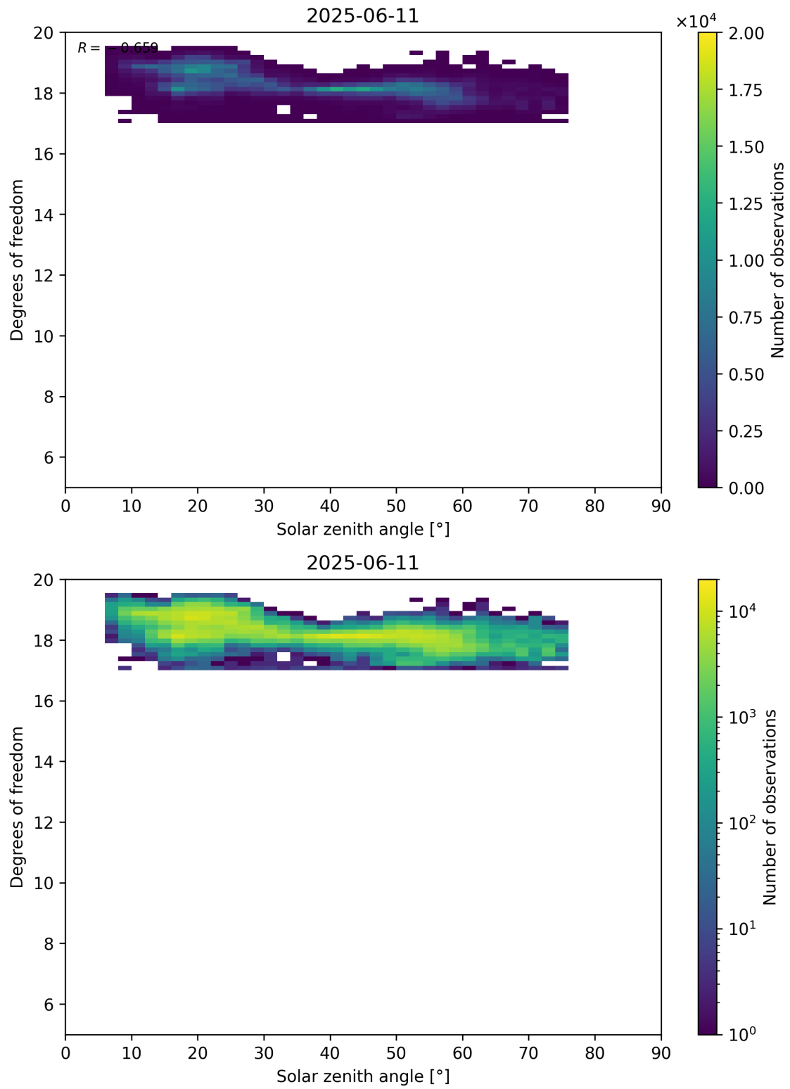
Figure 96: Scatter density plot of “Solar zenith angle” against “Degrees of freedom” for 2025-06-11 to 2025-06-12.
