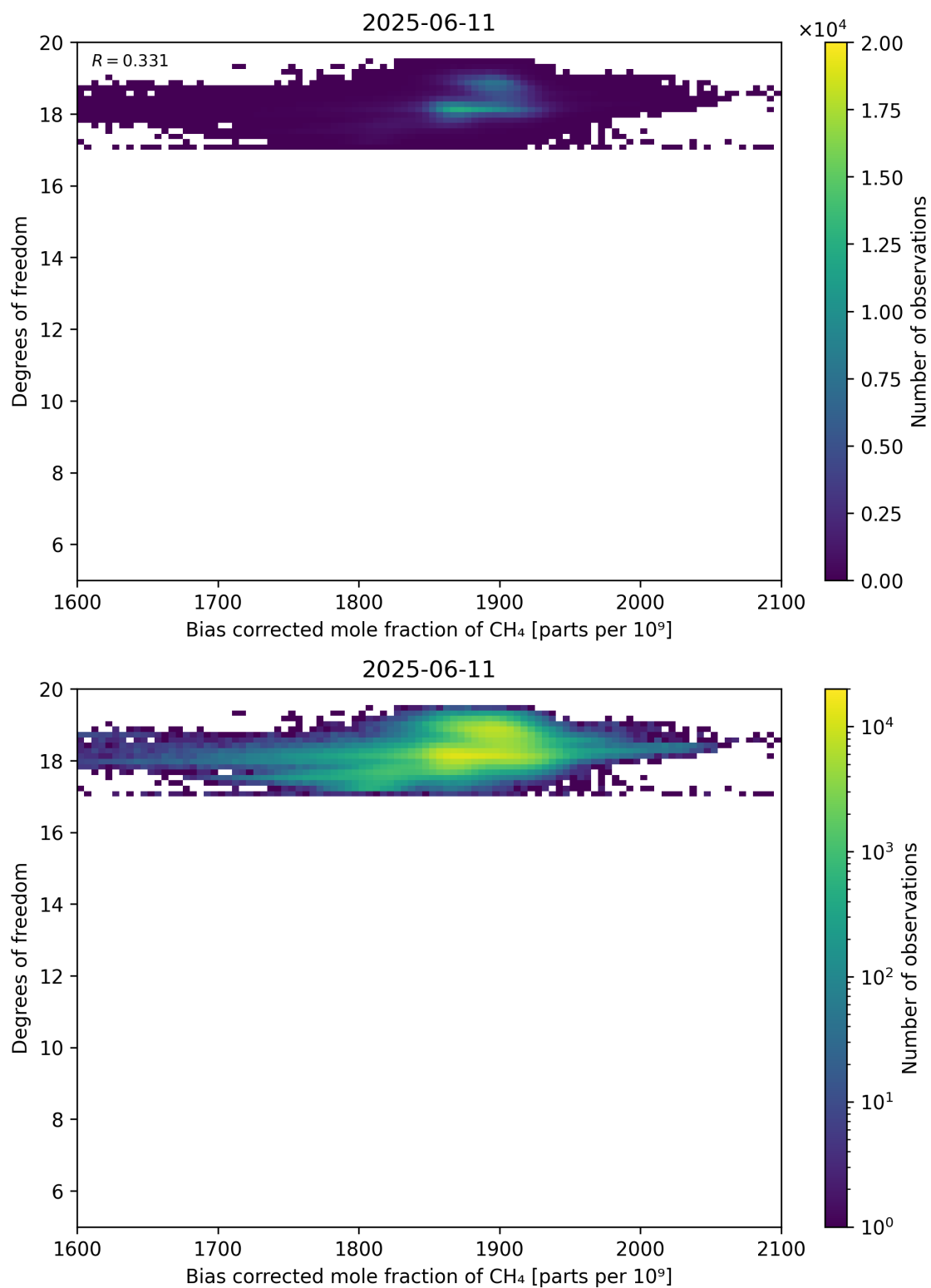
Figure 65: Scatter density plot of “Bias corrected mole fraction of CH 4 ” against “Degrees of freedom” for 2025-06-11 to 2025-06-12.
