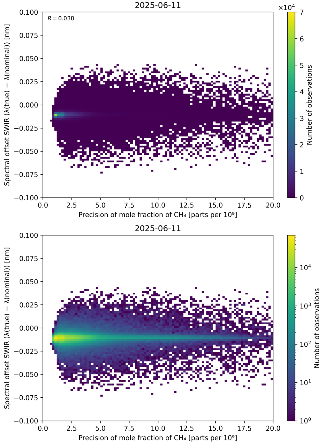
Figure 85: Scatter density plot of “Precision of mole fraction of \text{CH}_4 ” against “Spectral offset SWIR ( \lambda_{\text{true}} - \lambda_{\text{nominal}} )” for 2025-06-11 to 2025-06-12.
