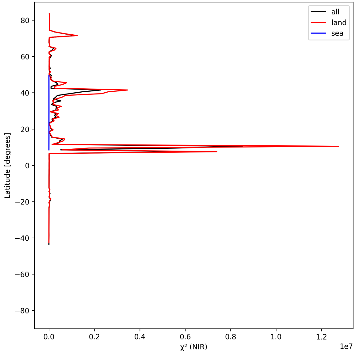
Figure 18: Zonal average of “ \chi^2 (NIR)” for 2025-06-11 to 2025-06-12.
