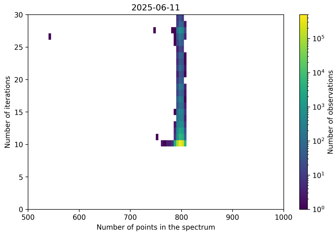
Figure 92: Scatter density plot of “Number of points in the spectrum” against “Number of iterations” for 2025-06-11 to 2025-06-12.
