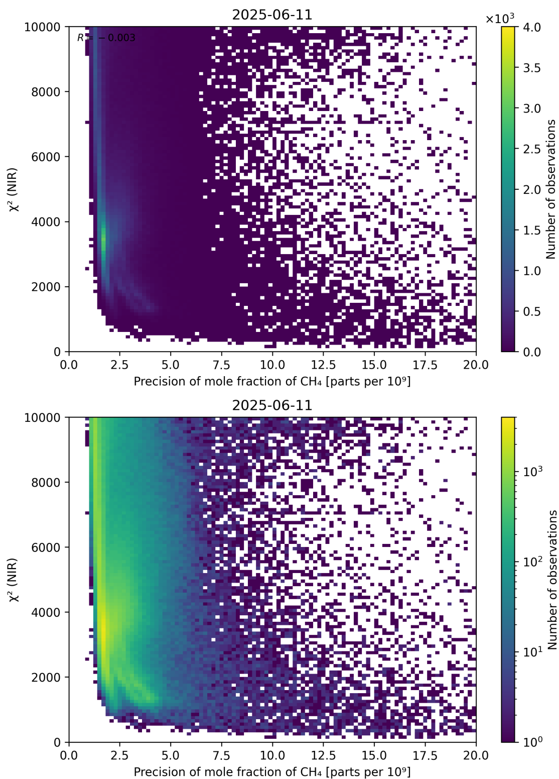
Figure 78: Scatter density plot of “Precision of mole fraction of \text{CH}_4 ” against “ \chi^2 (NIR)” for 2025-06-11 to 2025-06-12.
