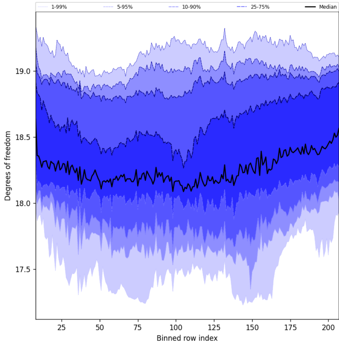
Figure 41: Along track statistics of “Degrees of freedom” for 2025-06-11 to 2025-06-12
