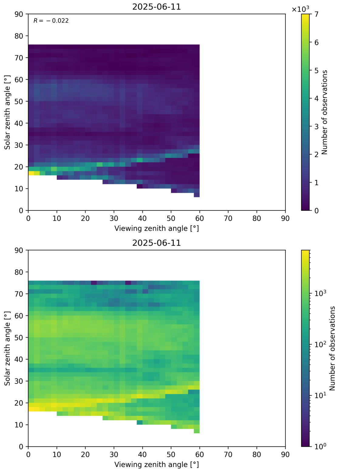
Figure 115: Scatter density plot of “Viewing zenith angle” against “Solar zenith angle” for 2025-06-11 to 2025-06-12.
