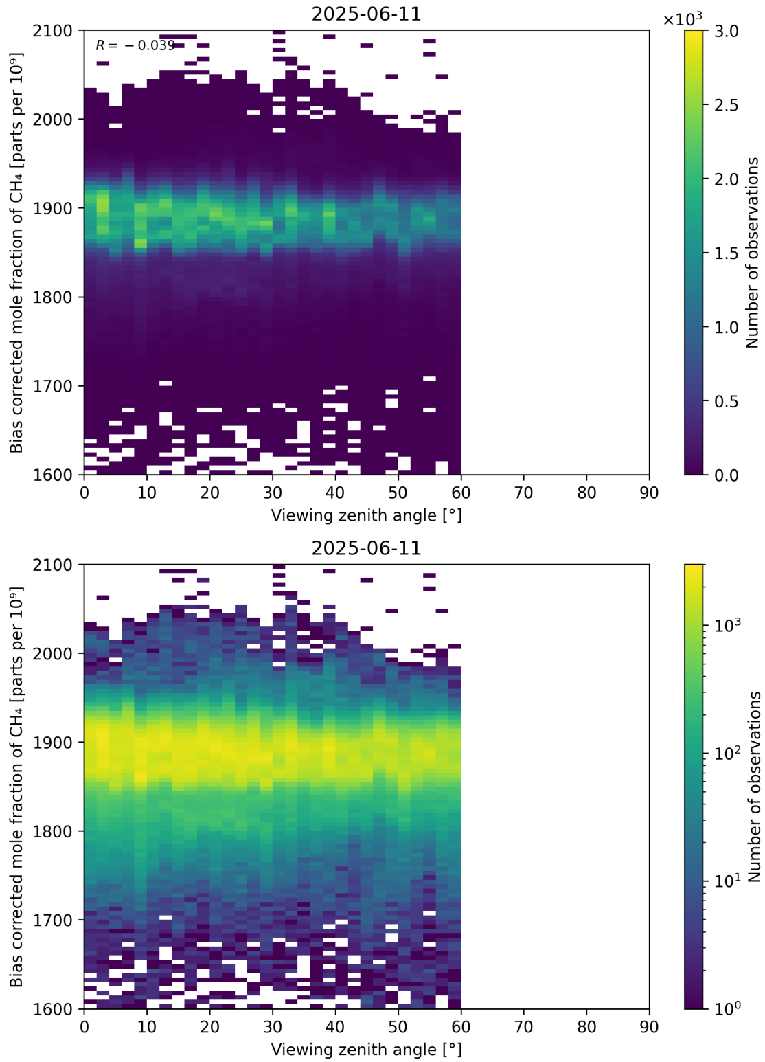
Figure 111: Scatter density plot of “Viewing zenith angle” against “Bias corrected mole fraction of CH 4 ” for 2025-06-11 to 2025-06-12.
