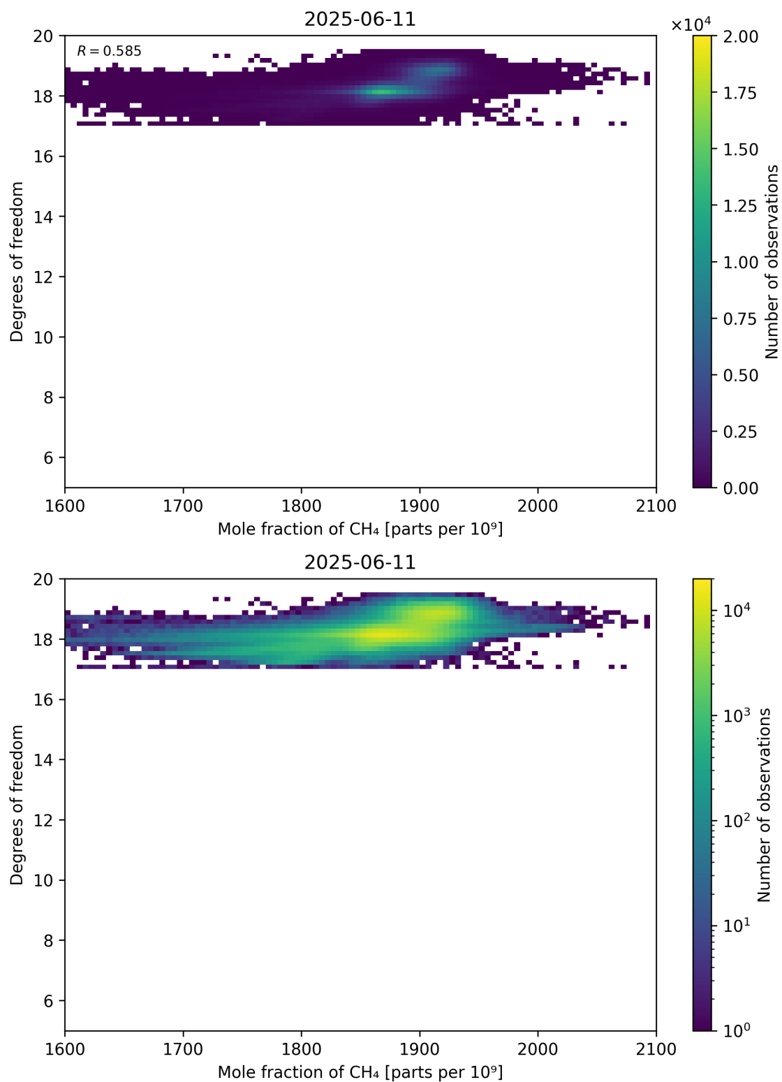
Figure 72: Scatter density plot of “Mole fraction of CH 4 ” against “Degrees of freedom” for 2025-06-11 to 2025-06-12.
