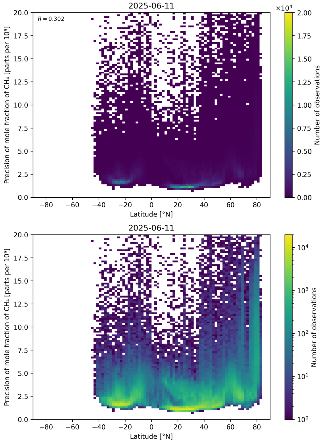
Figure 59: Scatter density plot of “Latitude” against “Precision of mole fraction of \text{CH}_4 ” for 2025-06-11 to 2025-06-12.
