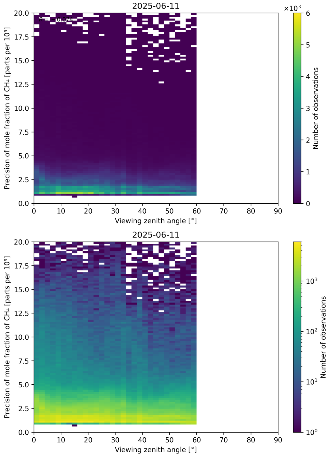
Figure 112: Scatter density plot of “Viewing zenith angle” against “Precision of mole fraction of CH 4 ” for 2025-06-11 to 2025-06-12.
