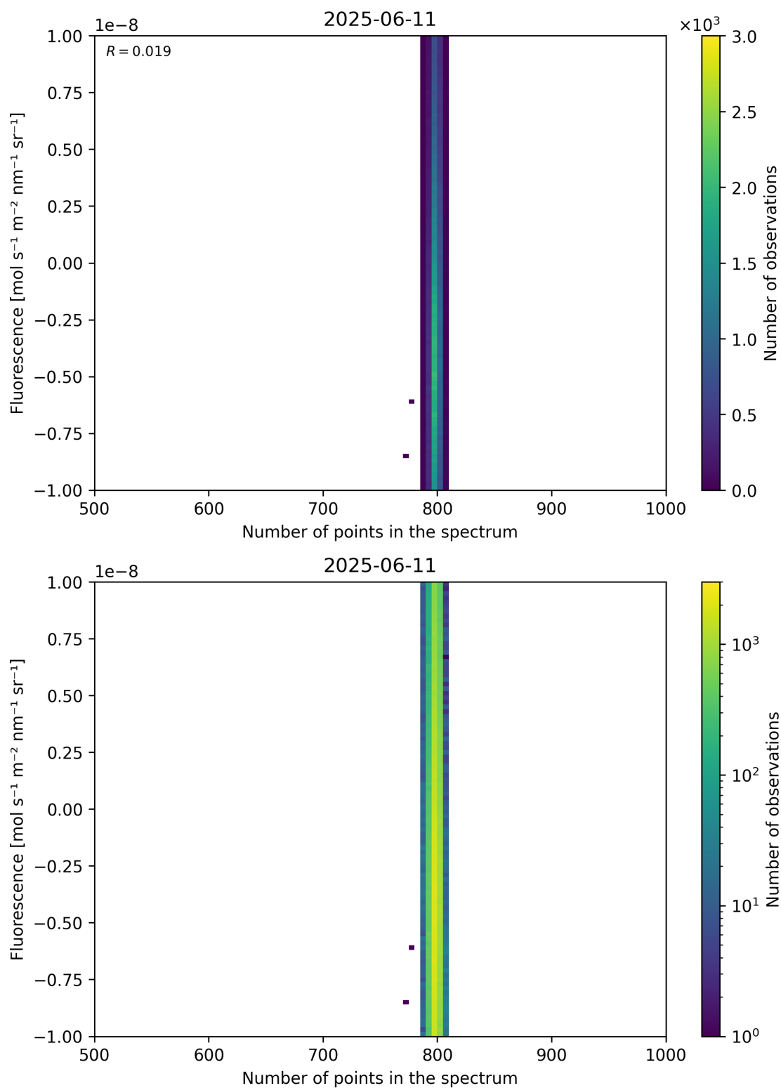
Figure 91: Scatter density plot of “Number of points in the spectrum” against “Fluorescence” for 2025-06-11 to 2025-06-12.
