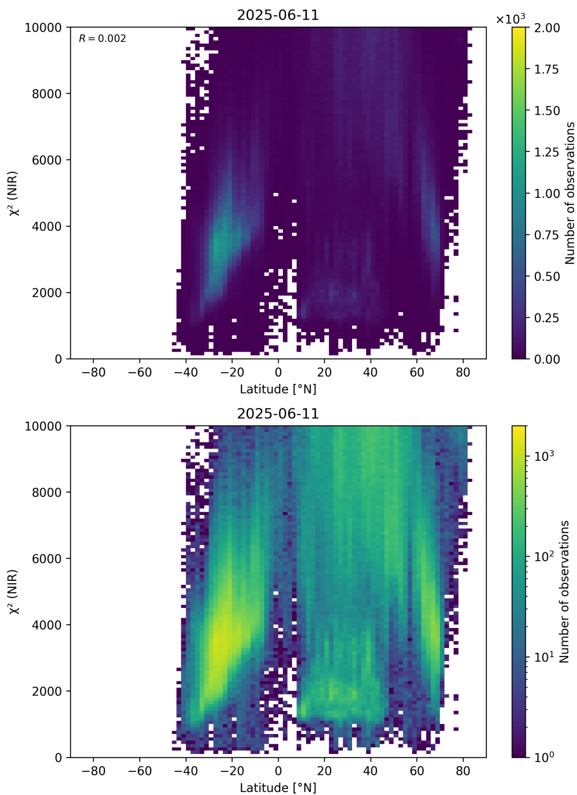
Figure 53: Scatter density plot of “Latitude” against “ \chi^2 (NIR)” for 2025-06-11 to 2025-06-12.
