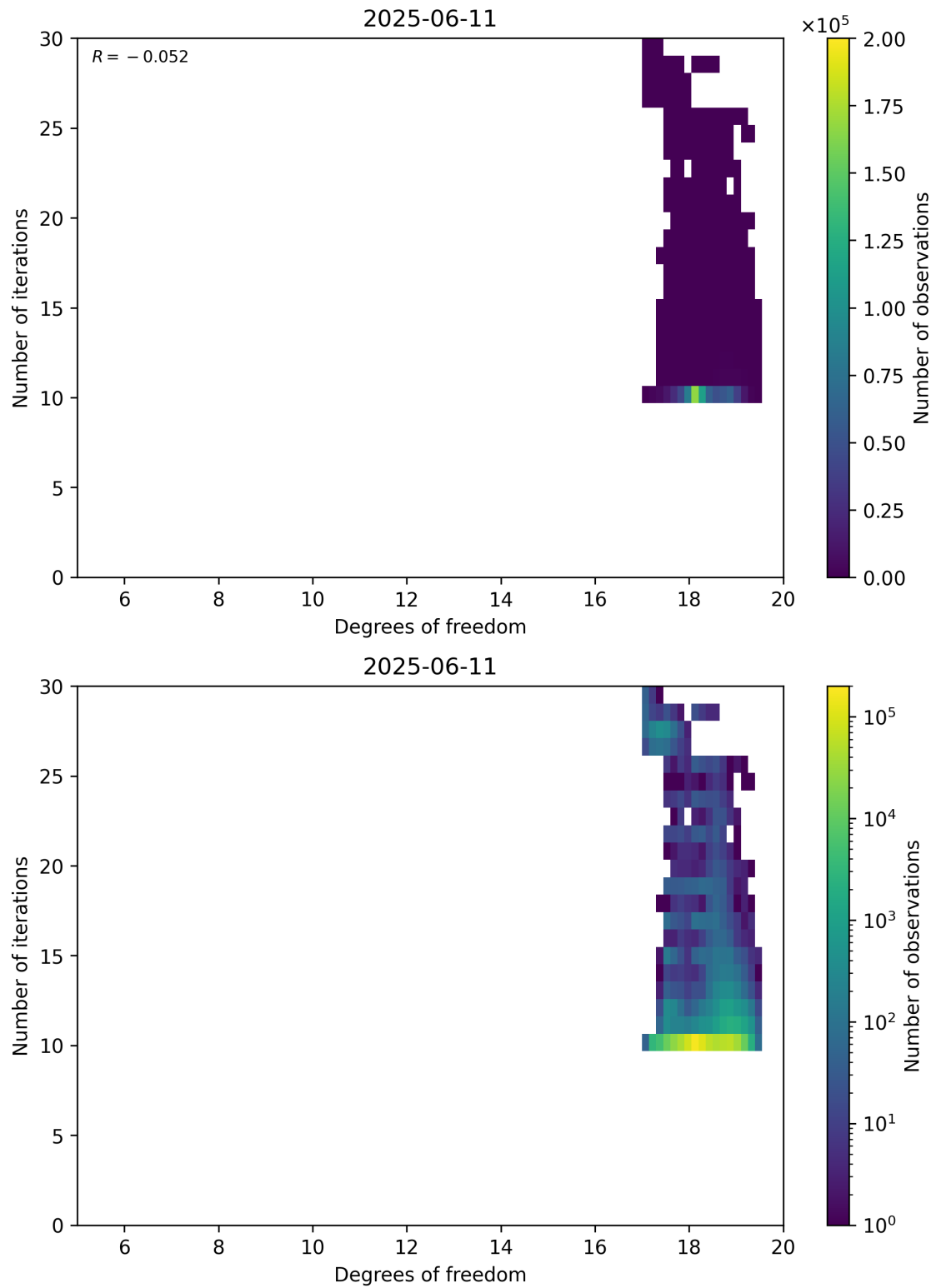
Figure 52: Scatter density plot of “Degrees of freedom” against “Number of iterations” for 2025-06-11 to 2025-06-12.
