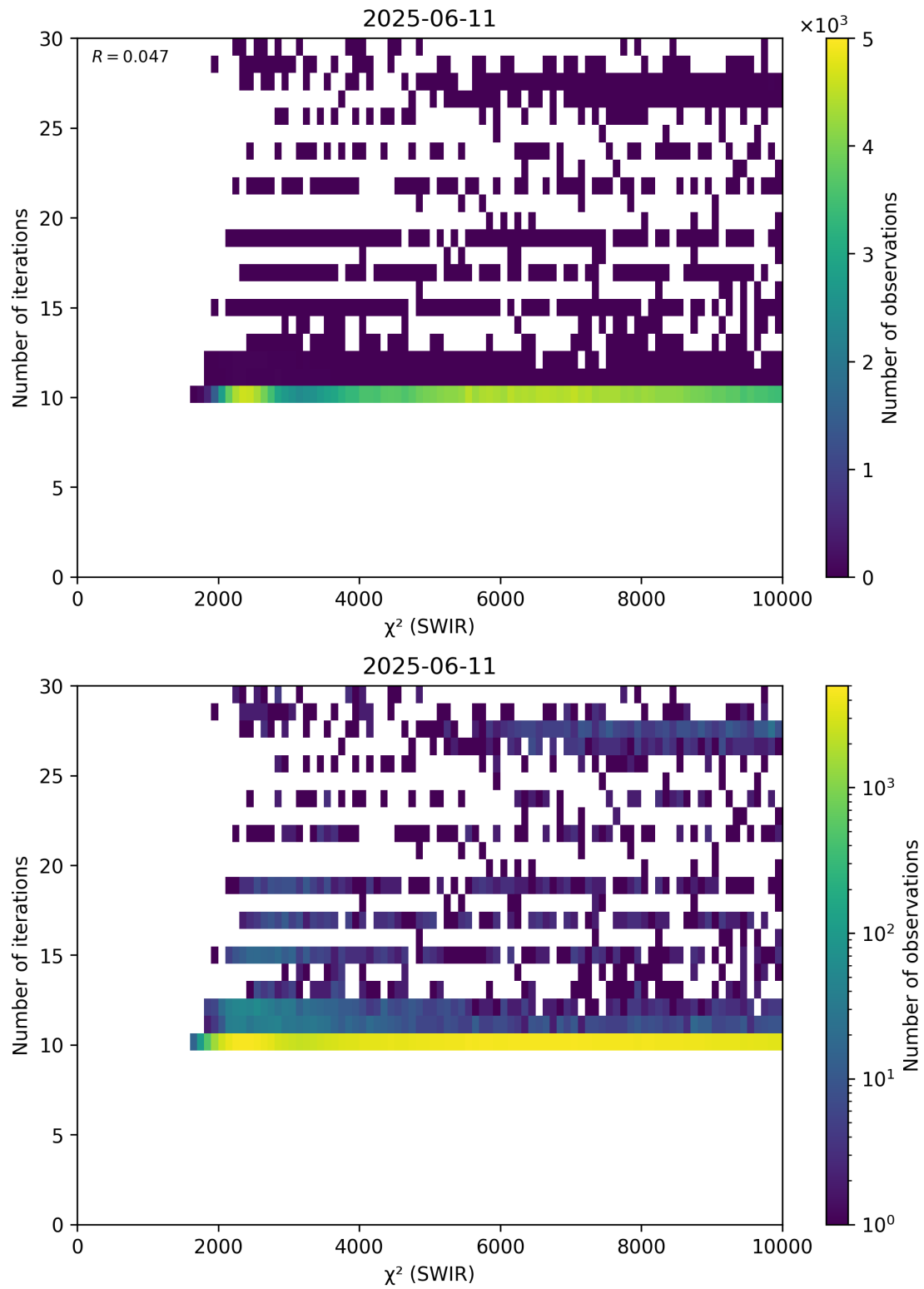
Figure 50: Scatter density plot of “ \chi^2 (SWIR)” against “Number of iterations” for 2025-06-11 to 2025-06-12.
