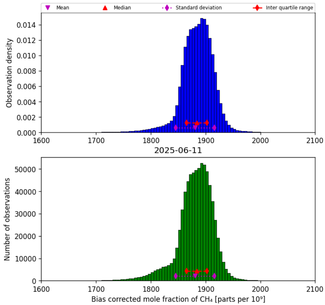
Figure 25: Histogram of “Bias corrected mole fraction of CH 4 ” for 2025-06-11 to 2025-06-12
