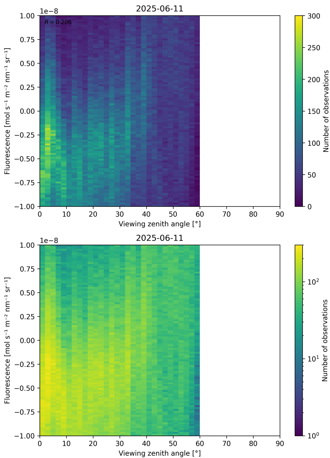
Figure 108: Scatter density plot of “Viewing zenith angle” against “Fluorescence” for 2025-06-11 to 2025-06-12.
