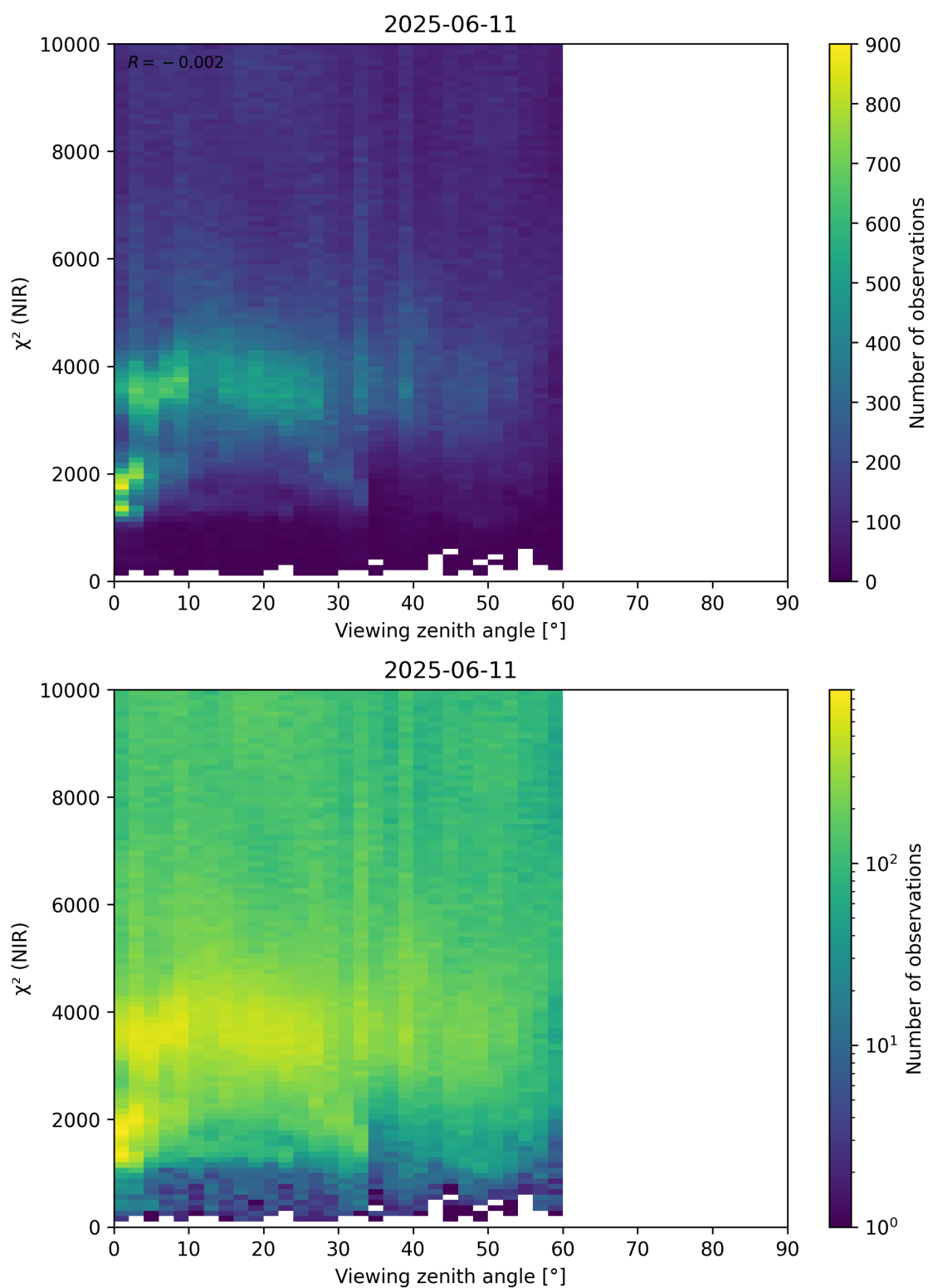
Figure 105: Scatter density plot of “Viewing zenith angle” against “ \chi^2 (NIR)” for 2025-06-11 to 2025-06-12.
