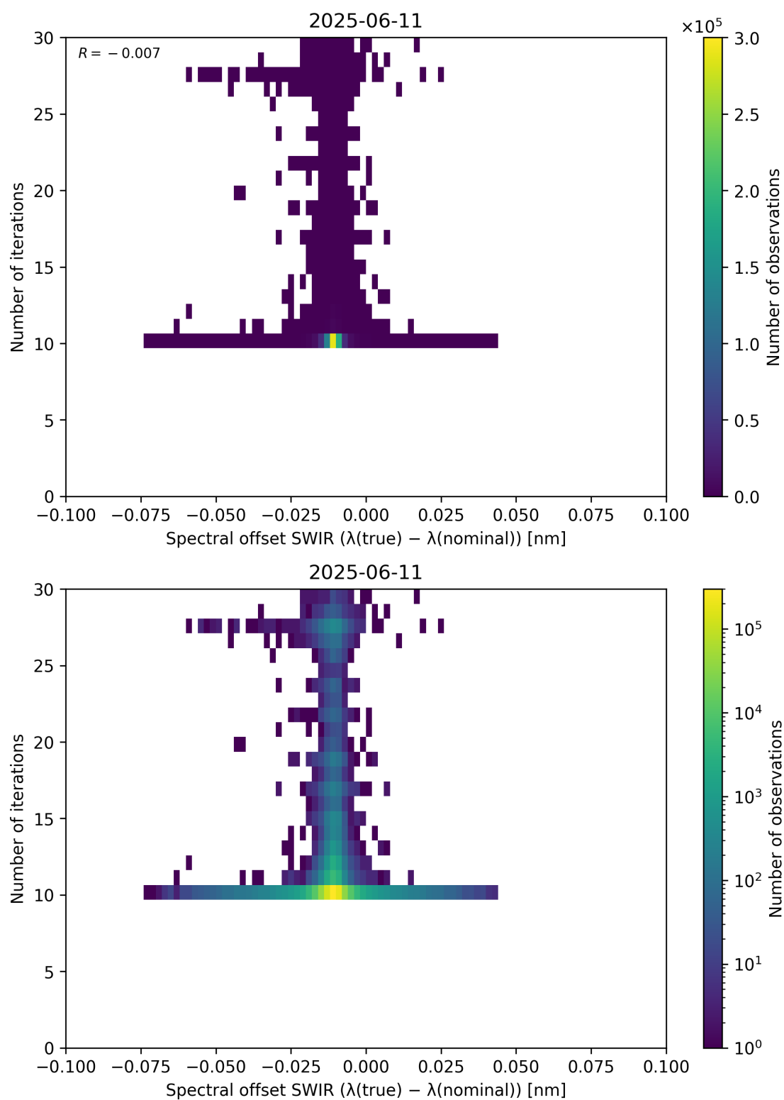
Figure 121: Scatter density plot of “Spectral offset SWIR ( \lambda_{\text{true}} - \lambda_{\text{nominal}} )” against “Number of iterations” for 2025-06-11 to 2025-06-12.
