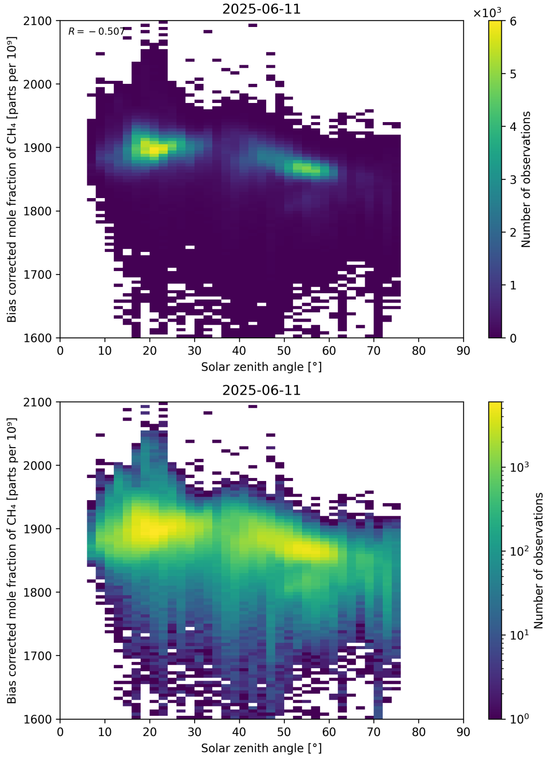
Figure 100: Scatter density plot of “Solar zenith angle” against “Bias corrected mole fraction of CH 4 ” for 2025-06-11 to 2025-06-12.
