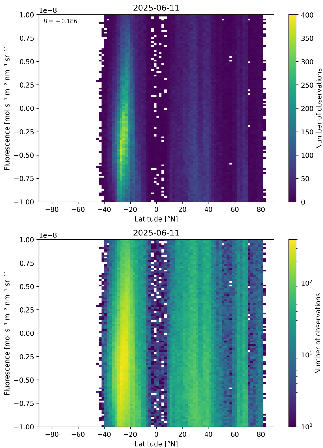
Figure 56: Scatter density plot of “Latitude” against “Fluorescence” for 2025-06-11 to 2025-06-12.
