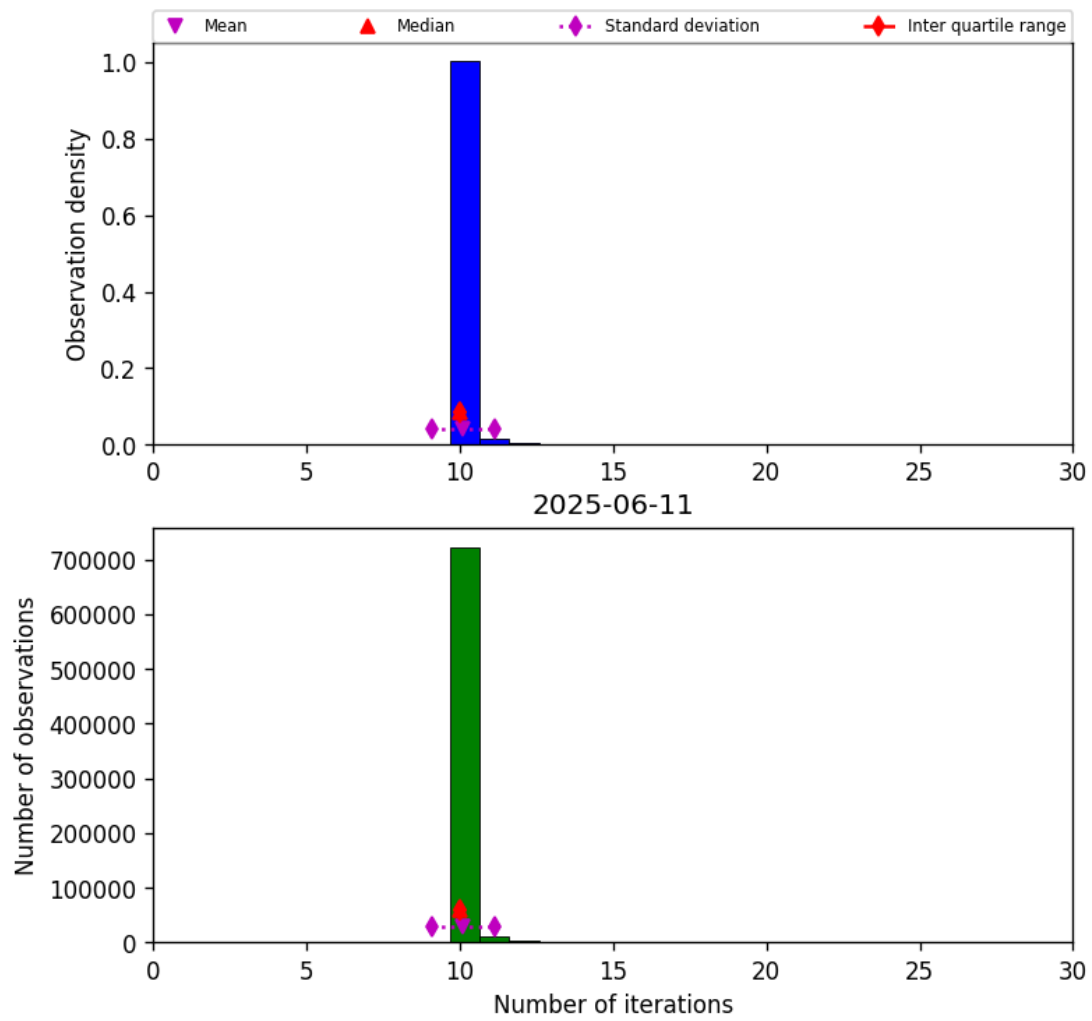
Figure 31: Histogram of “Number of iterations” for 2025-06-11 to 2025-06-12
