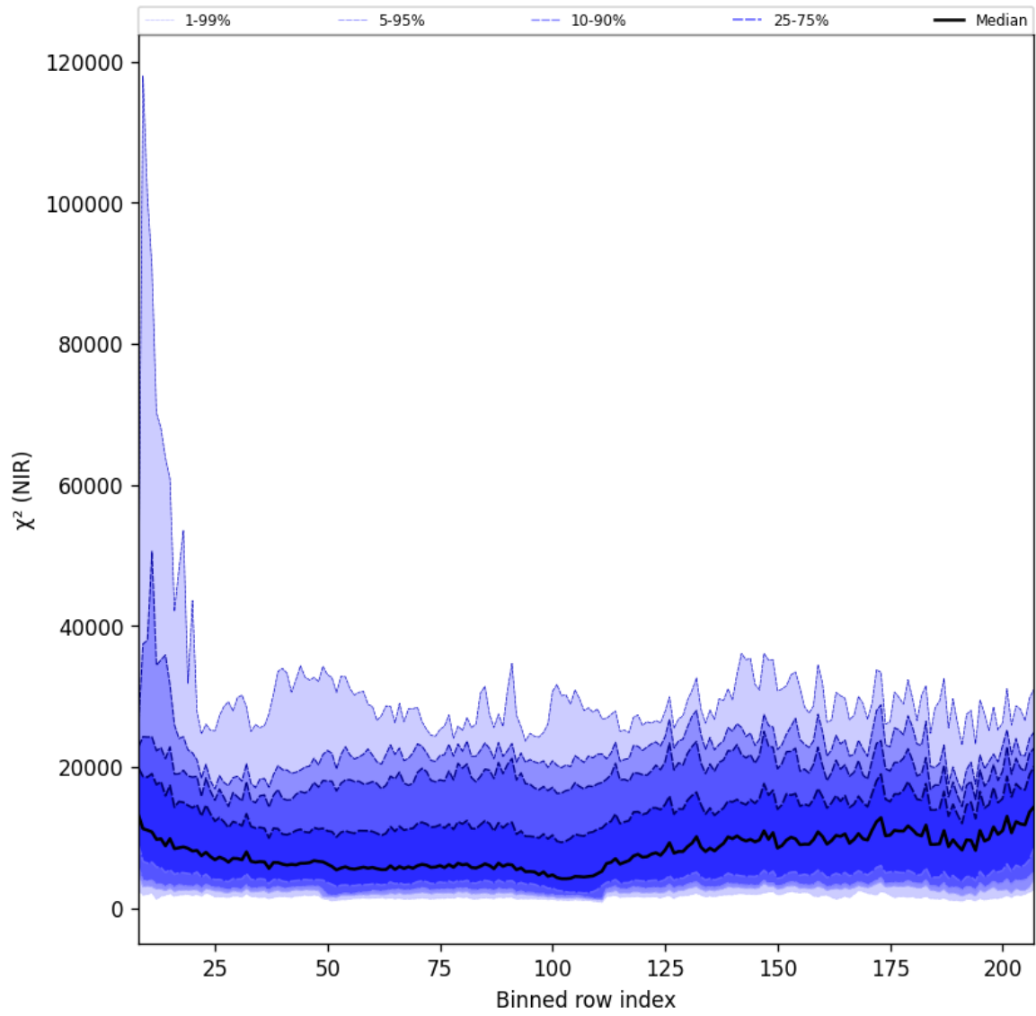
Figure 40: Along track statistics of “ \chi^2 (NIR)” for 2025-06-11 to 2025-06-12
