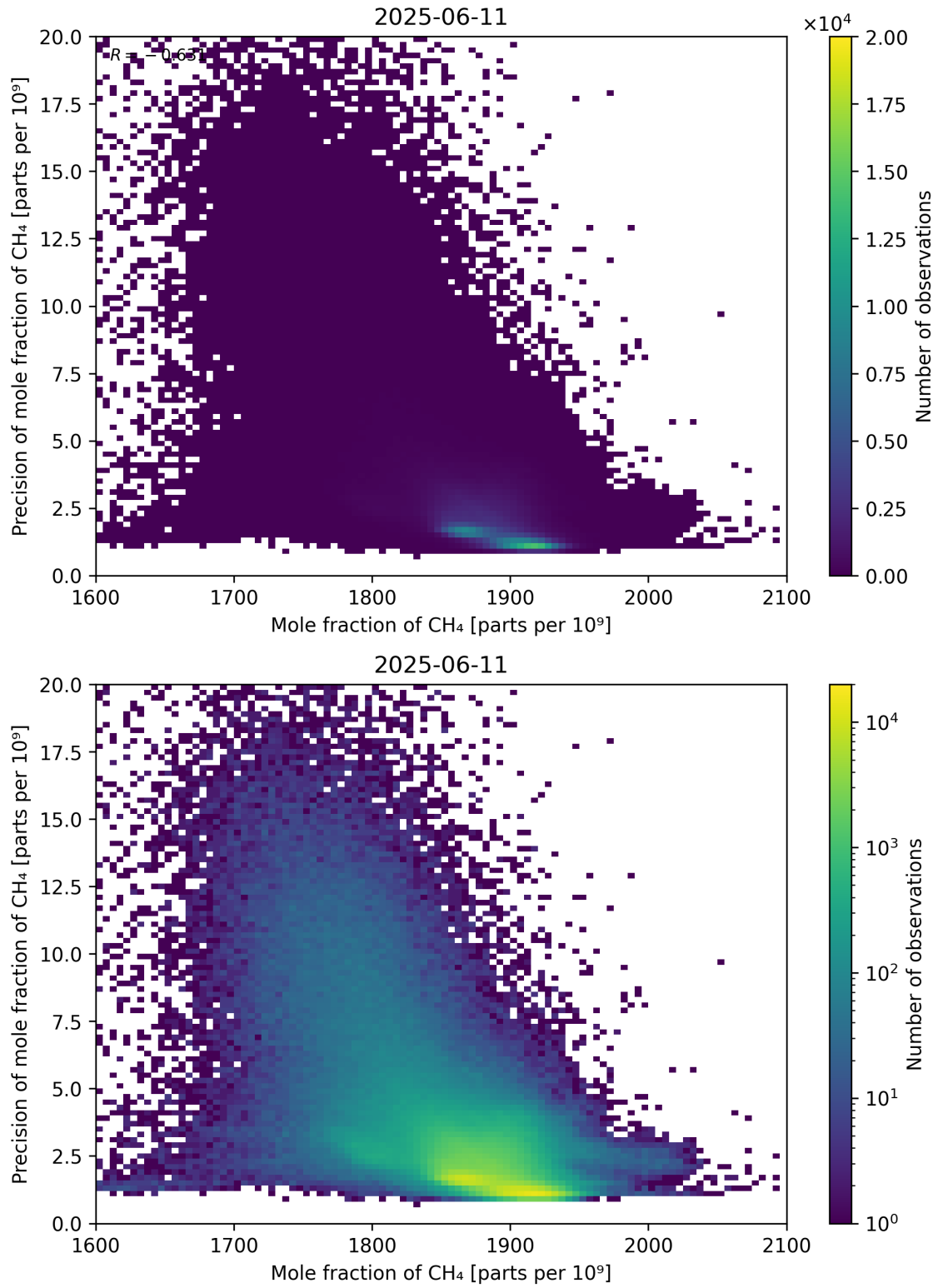
Figure 75: Scatter density plot of “Mole fraction of CH 4 ” against “Precision of mole fraction of CH 4 ” for 2025-06-11 to 2025-06-12.
