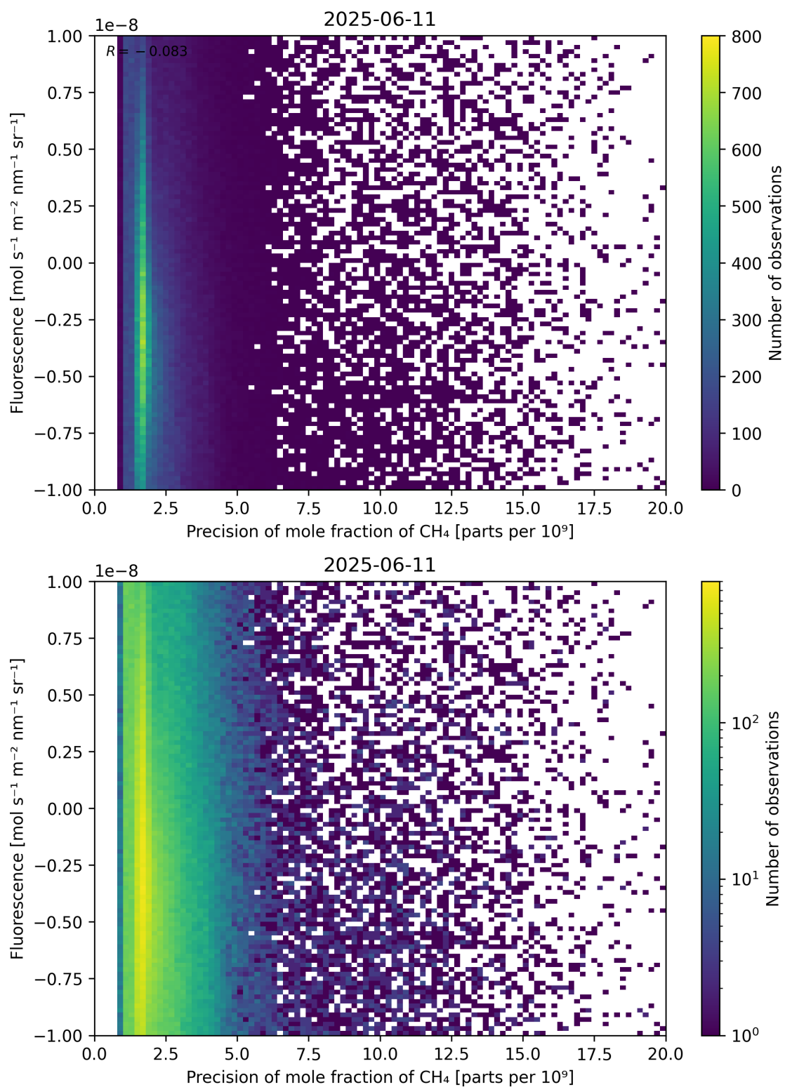
Figure 81: Scatter density plot of “Precision of mole fraction of CH 4 ” against “Fluorescence” for 2025-06-11 to 2025-06-12.
