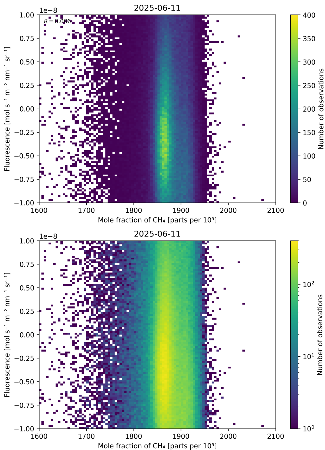
Figure 73: Scatter density plot of “Mole fraction of \text{CH}_4 ” against “Fluorescence” for 2025-06-11 to 2025-06-12.
