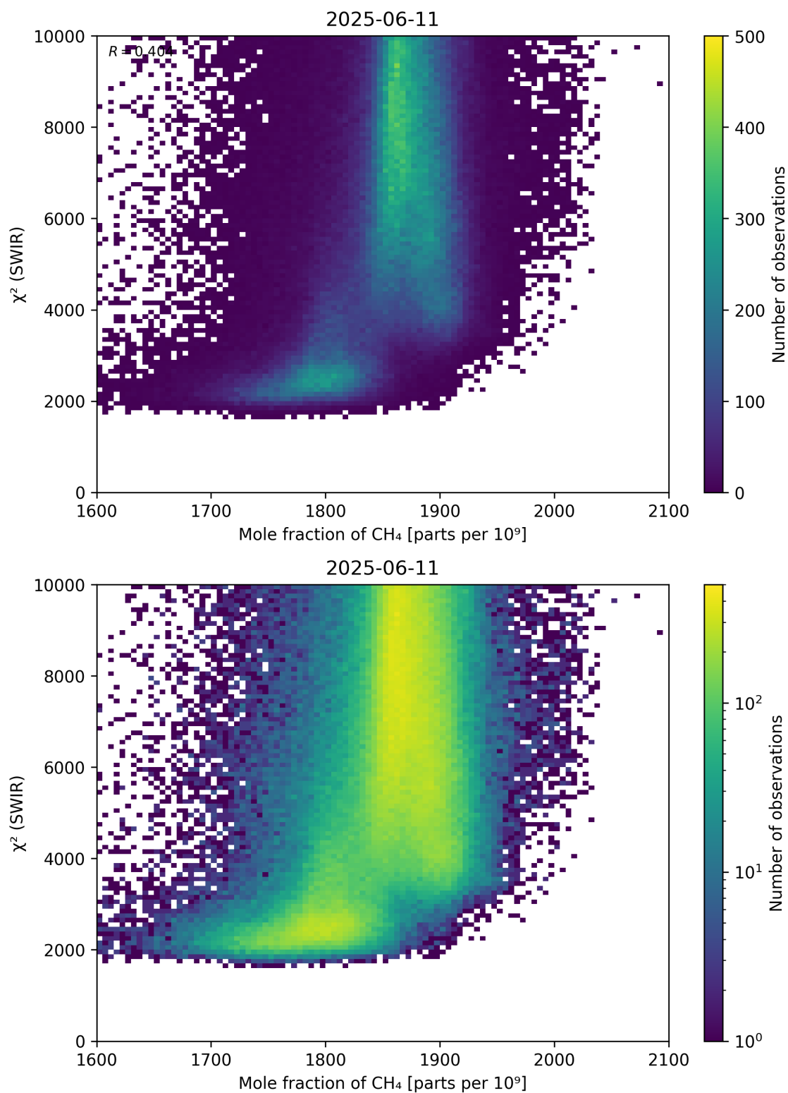
Figure 71: Scatter density plot of “Mole fraction of \text{CH}_4 ” against “ \chi^2 (SWIR)” for 2025-06-11 to 2025-06-12.
