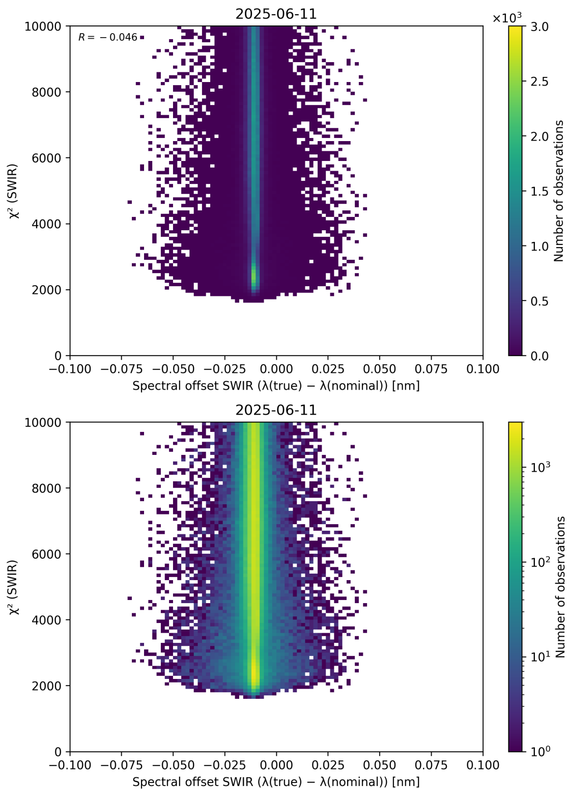
Figure 118: Scatter density plot of “Spectral offset SWIR ( \lambda_{\text{true}} - \lambda_{\text{nominal}} )” against “ \chi^2 (SWIR)” for 2025-06-11 to 2025-06-12.
