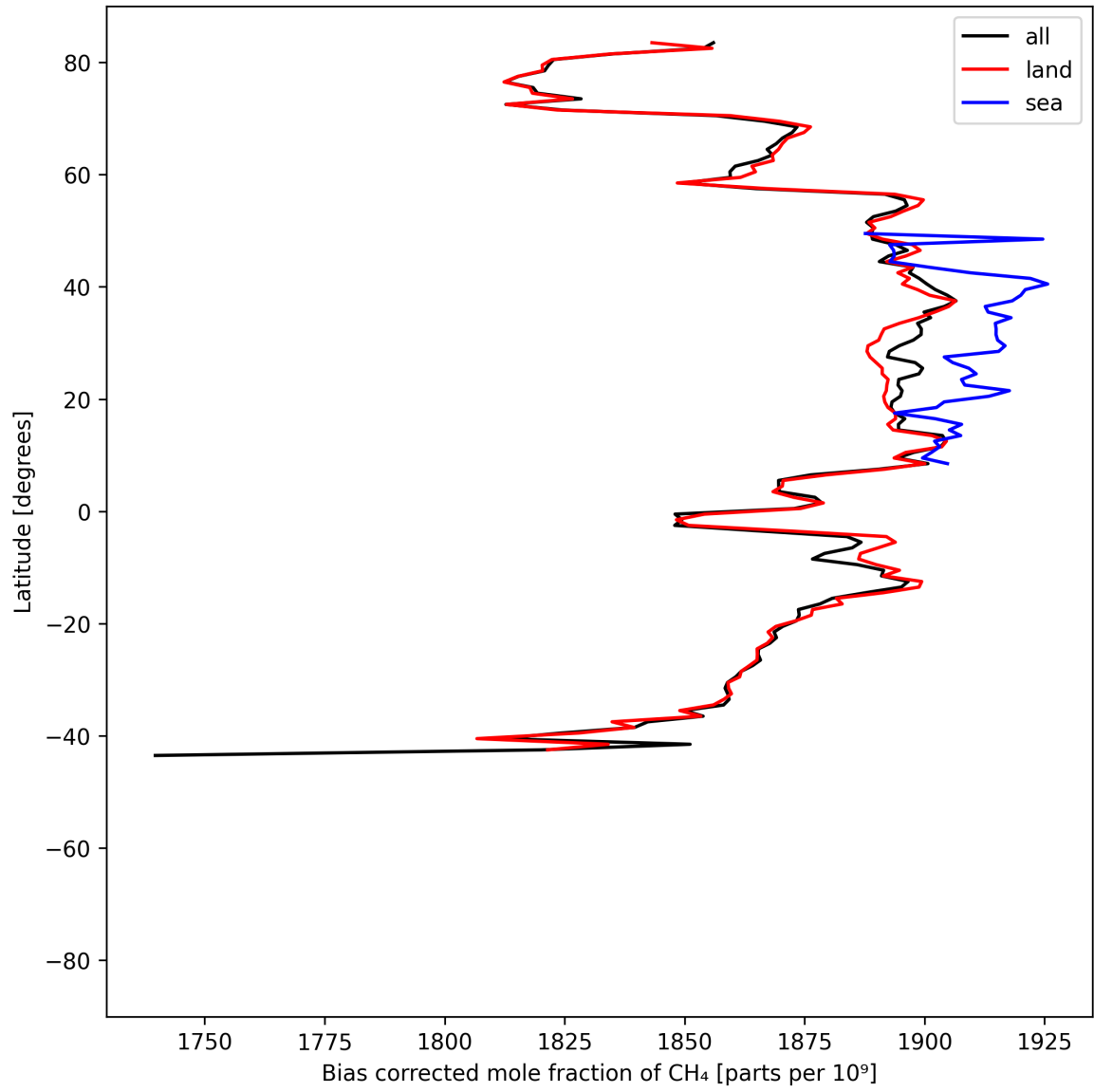
Figure 14: Zonal average of “Bias corrected mole fraction of CH 4 ” for 2025-06-11 to 2025-06-12.
