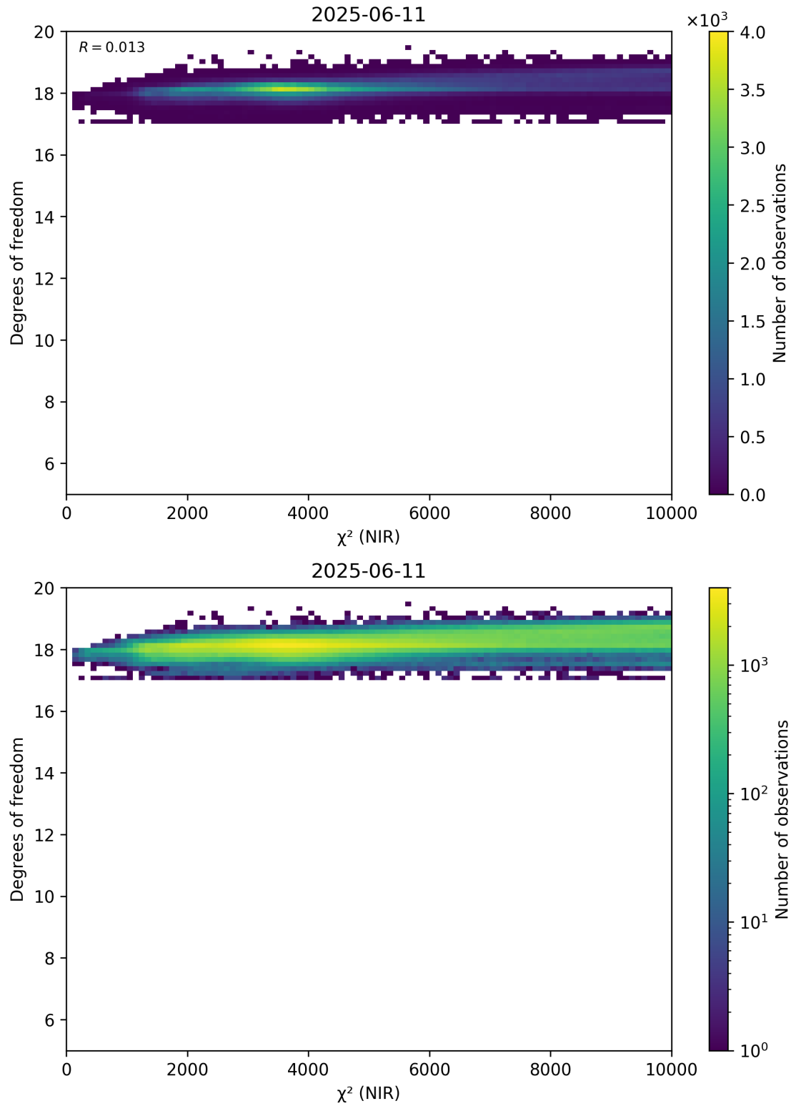
Figure 44: Scatter density plot of “ \chi^2 (NIR)” against “Degrees of freedom” for 2025-06-11 to 2025-06-12.
