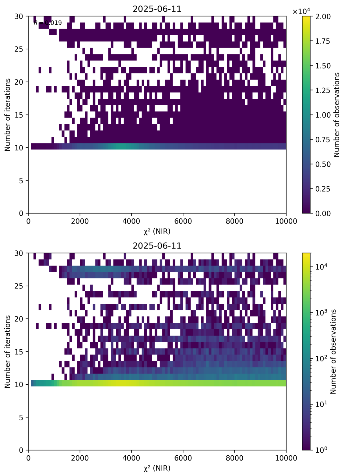
Figure 46: Scatter density plot of “ \chi^2 (NIR)” against “Number of iterations” for 2025-06-11 to 2025-06-12.
