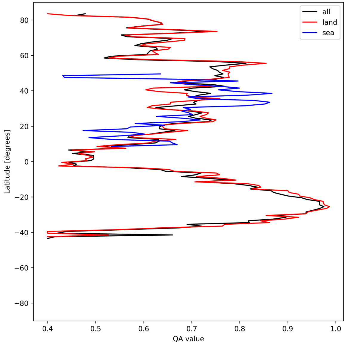
Figure 11: Zonal average of “QA value” for 2025-06-11 to 2025-06-12.
