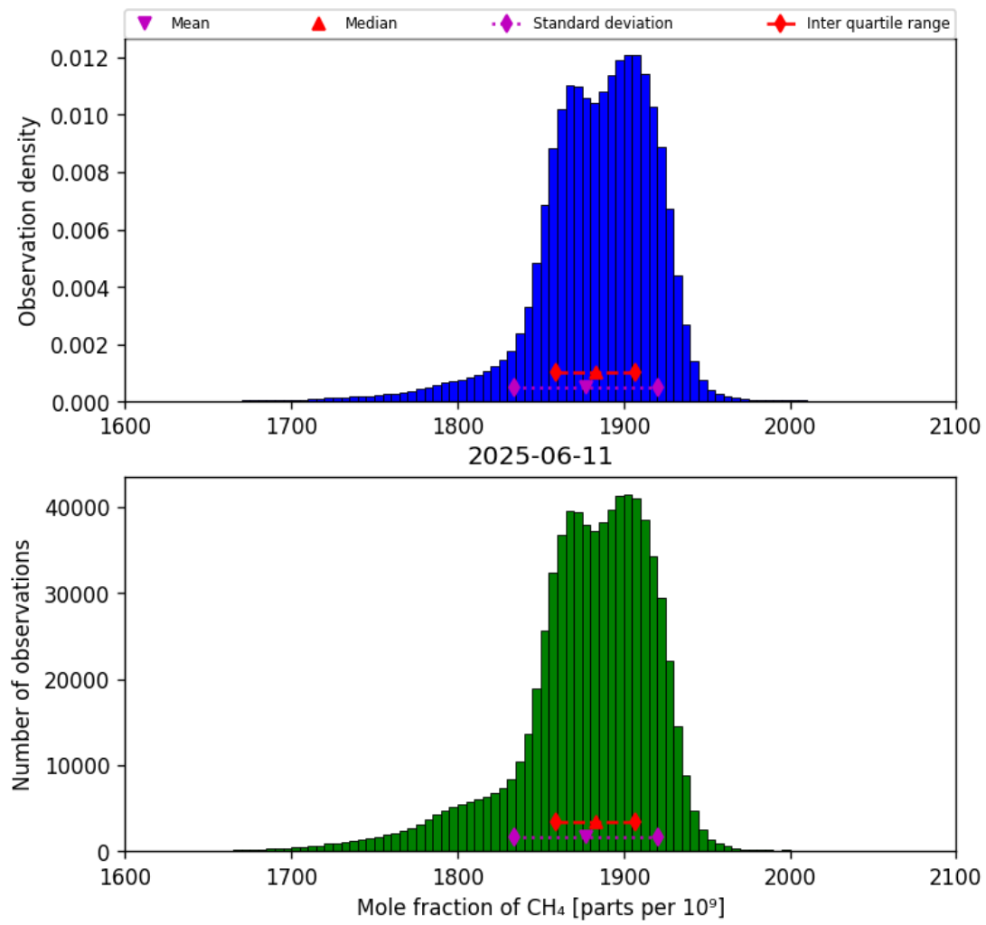
Figure 23: Histogram of “Mole fraction of CH 4 ” for 2025-06-11 to 2025-06-12
