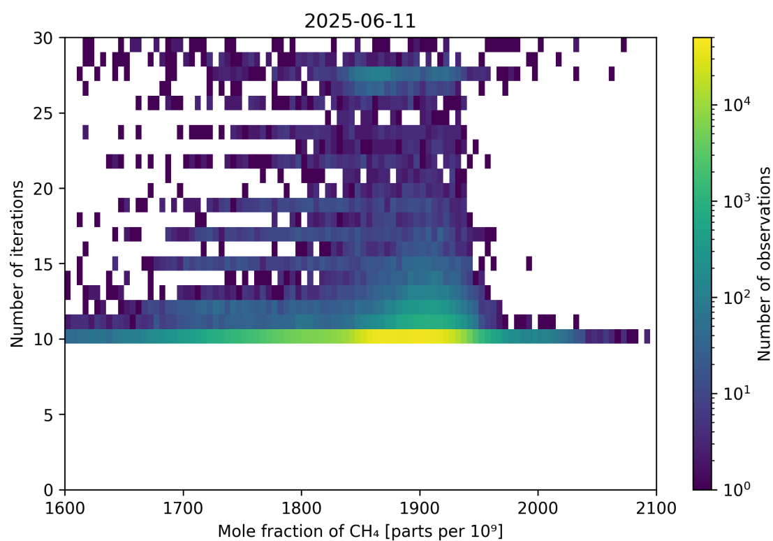
Figure 76: Scatter density plot of “Mole fraction of CH 4 ” against “Number of iterations” for 2025-06-11 to 2025-06-12.
