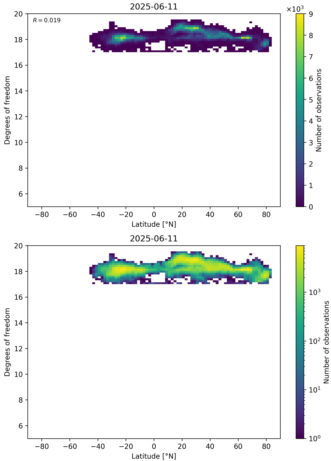
Figure 55: Scatter density plot of “Latitude” against “Degrees of freedom” for 2025-06-11 to 2025-06-12.
