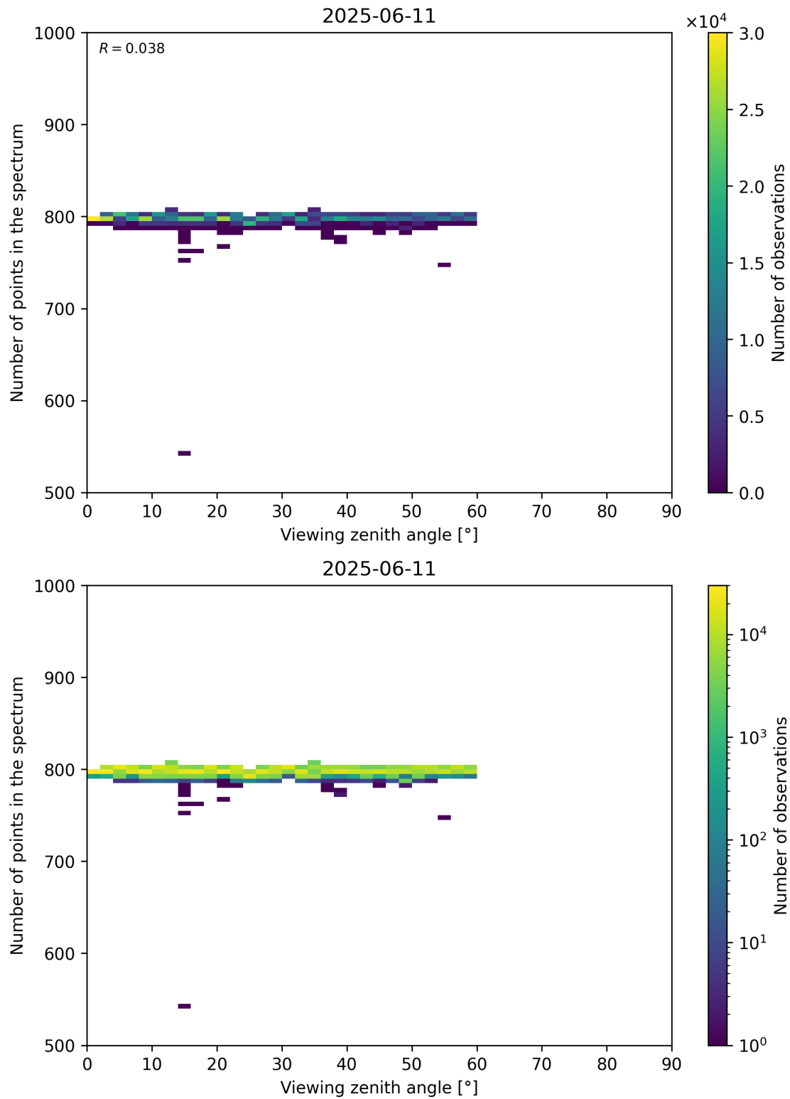
Figure 114: Scatter density plot of “Viewing zenith angle” against “Number of points in the spectrum” for 2025-06-11 to 2025-06-12.
