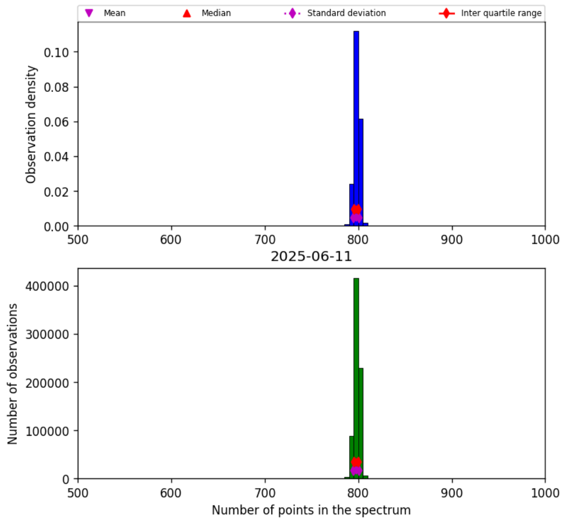
Figure 26: Histogram of “Number of points in the spectrum” for 2025-06-11 to 2025-06-12
