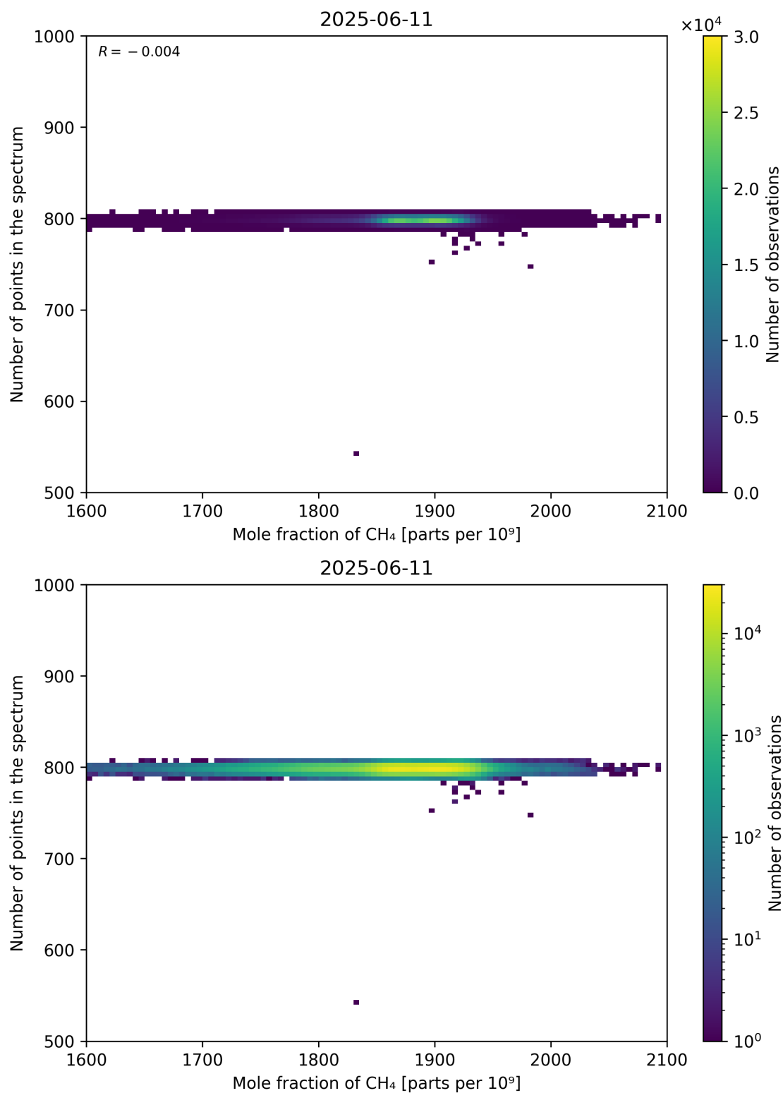
Figure 77: Scatter density plot of “Mole fraction of CH 4 ” against “Number of points in the spectrum” for 2025-06-11 to 2025-06-12.
