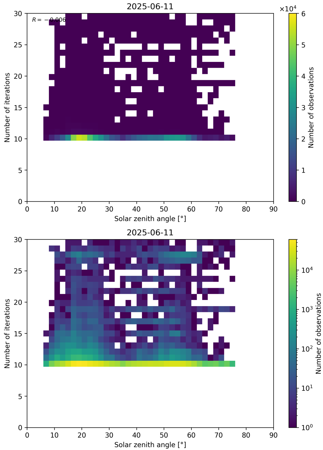
Figure 102: Scatter density plot of “Solar zenith angle” against “Number of iterations” for 2025-06-11 to 2025-06-12.
