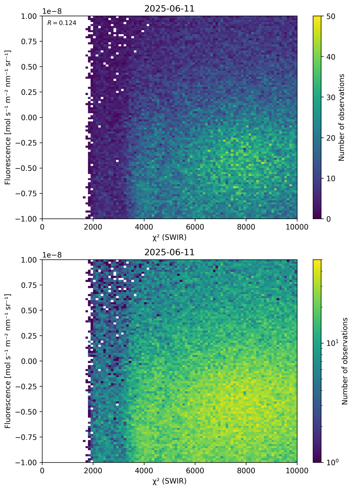
Figure 49: Scatter density plot of “ \chi^2 (SWIR)” against “Fluorescence” for 2025-06-11 to 2025-06-12.
