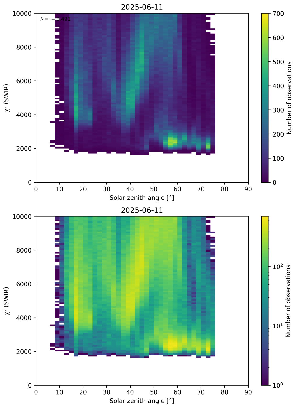
Figure 95: Scatter density plot of “Solar zenith angle” against “ \chi^2 (SWIR)” for 2025-06-11 to 2025-06-12.
