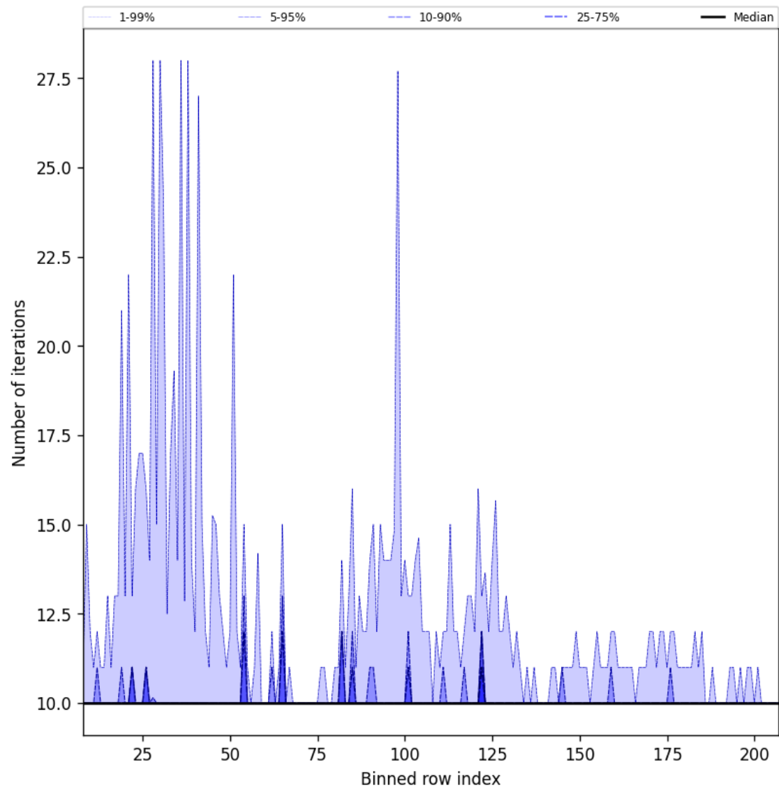
Figure 42: Along track statistics of “Number of iterations” for 2025-06-11 to 2025-06-12
