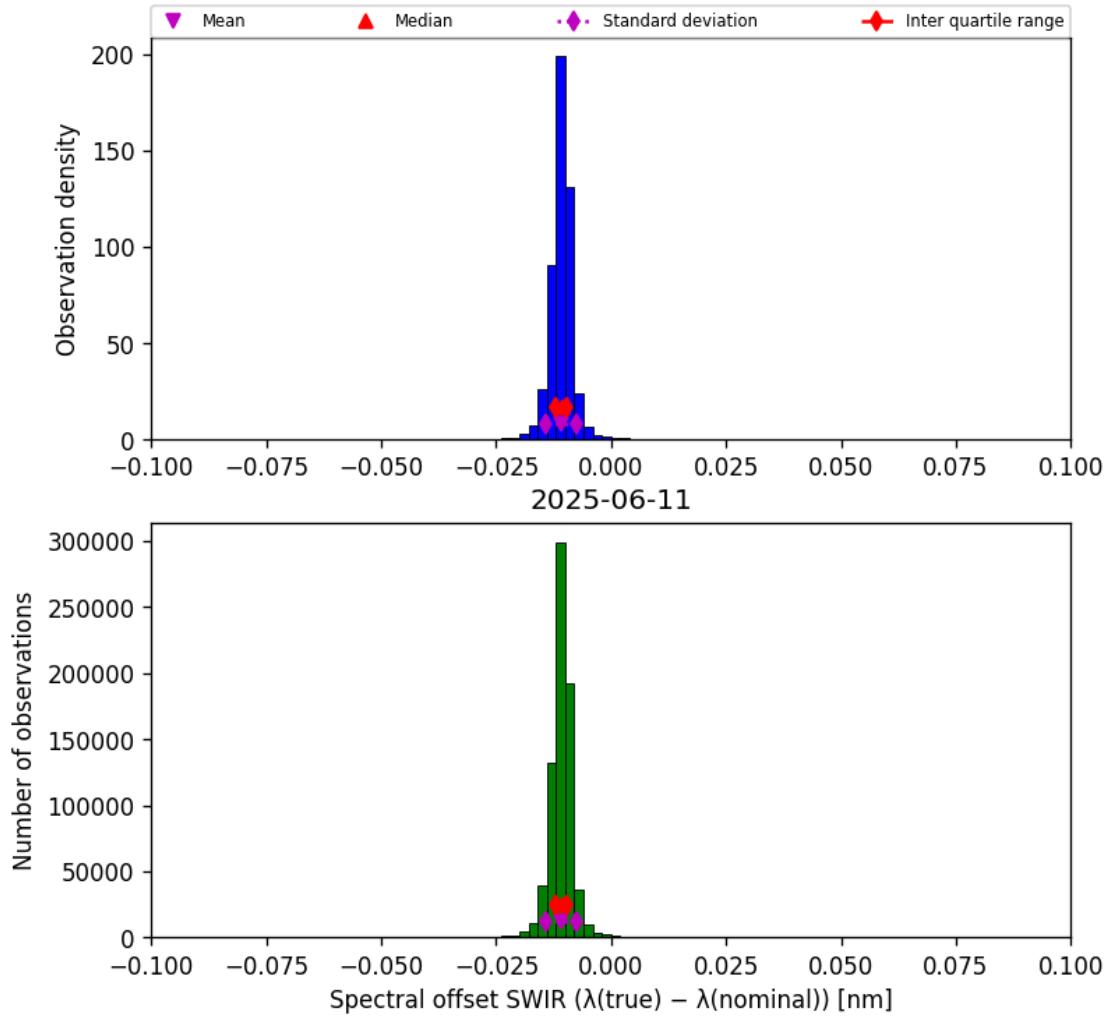
Figure 27: Histogram of “Spectral offset SWIR ( \lambda_{\text{true}} - \lambda_{\text{nominal}} )” for 2025-06-11 to 2025-06-12
