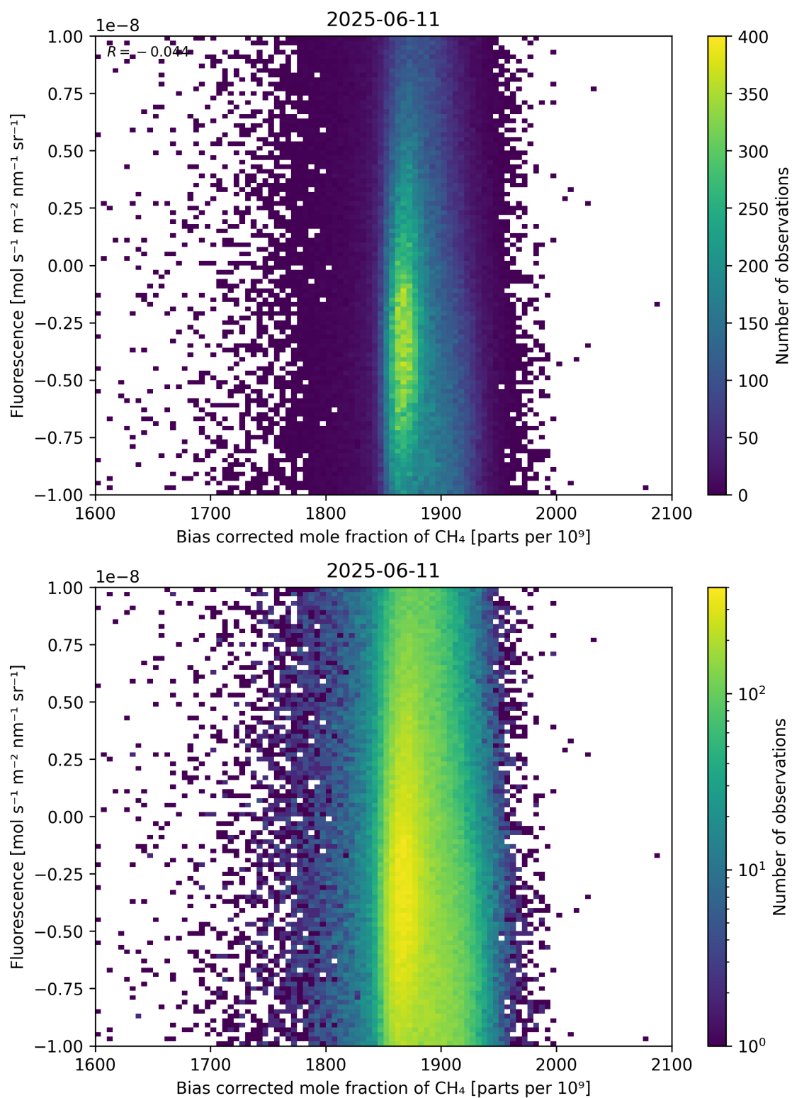
Figure 66: Scatter density plot of “Bias corrected mole fraction of \text{CH}_4 ” against “Fluorescence” for 2025-06-11 to 2025-06-12.
