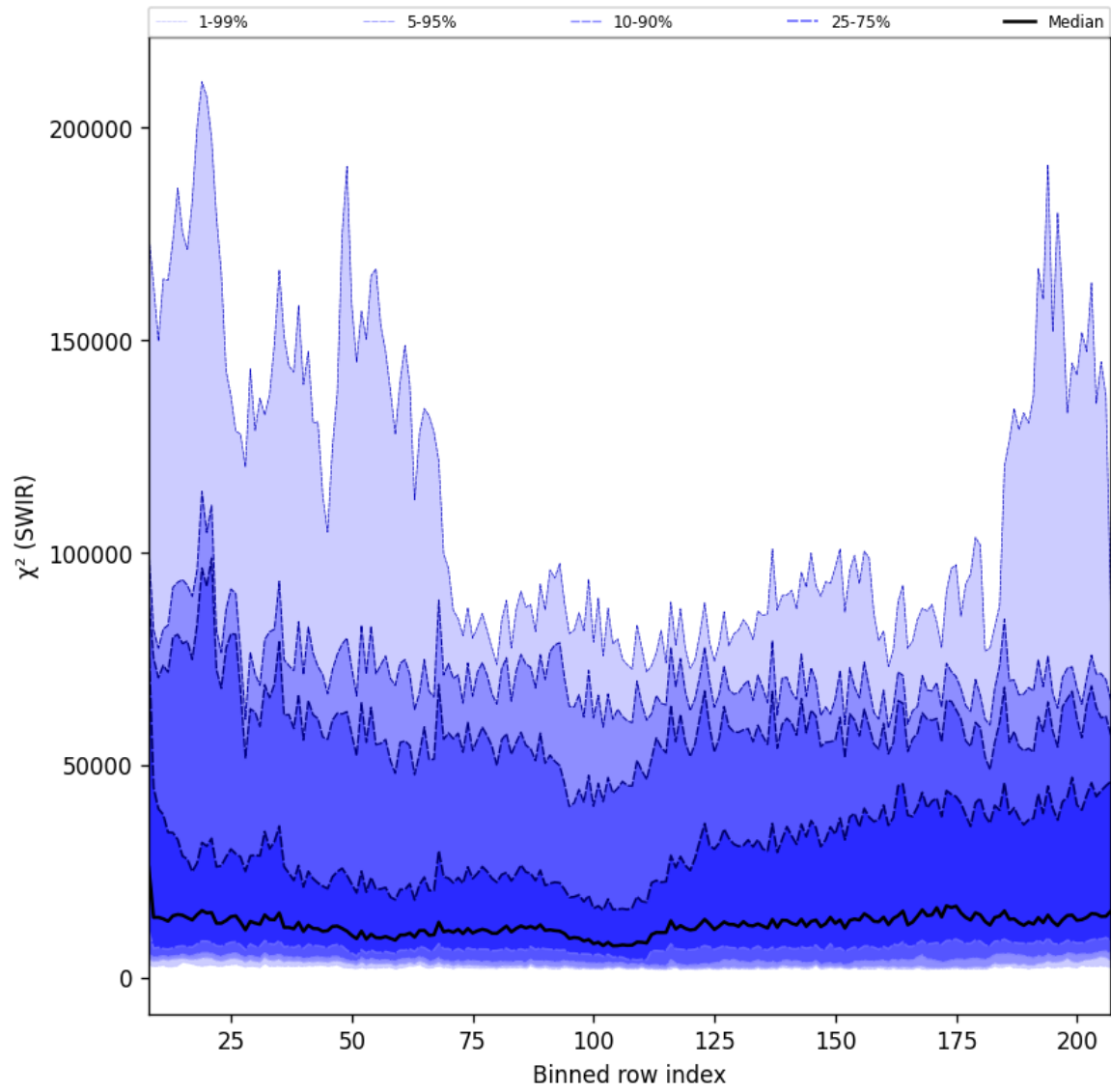
Figure 39: Along track statistics of " \chi^2 (SWIR)" for 2025-06-11 to 2025-06-12
