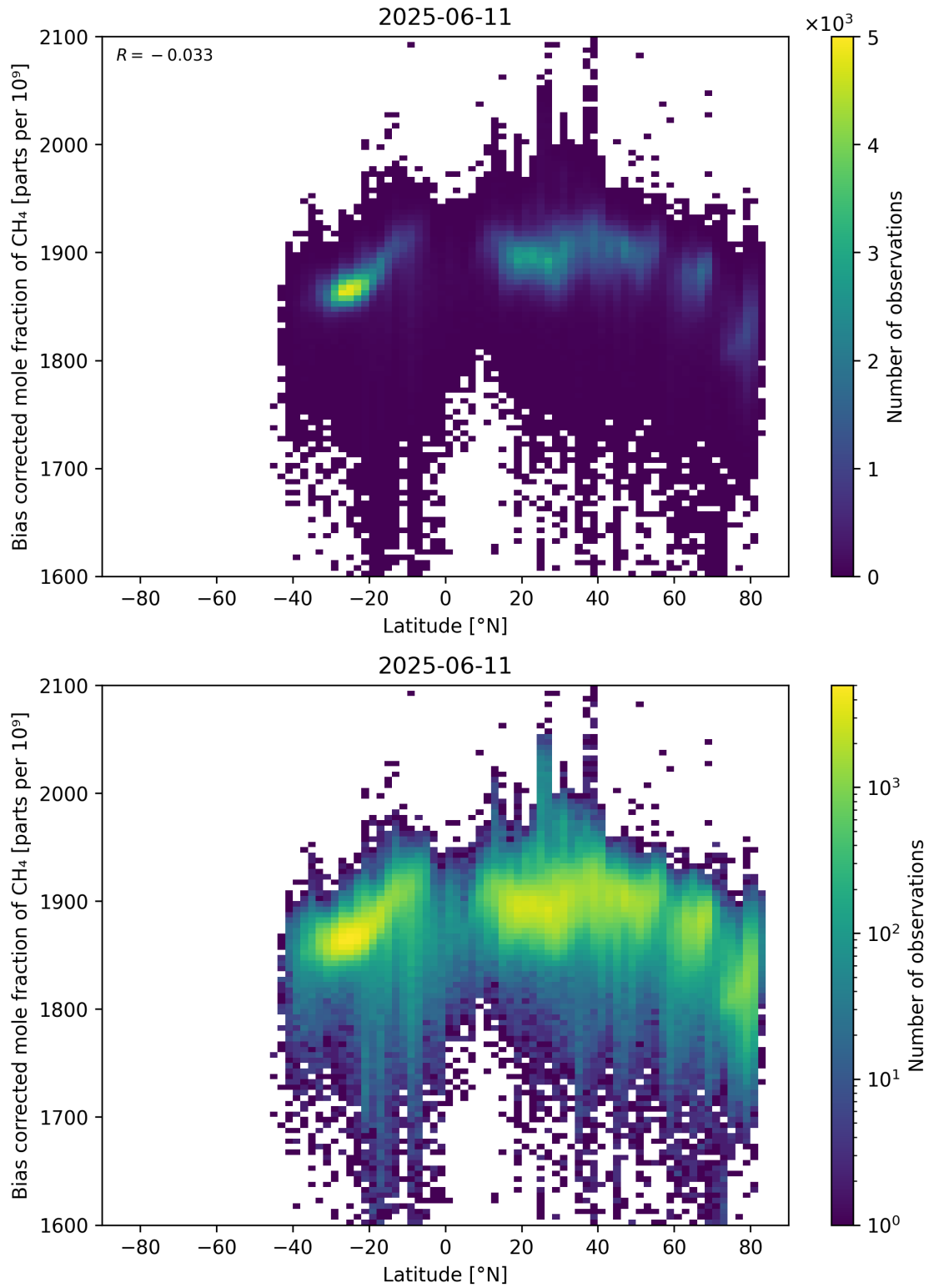
Figure 58: Scatter density plot of “Latitude” against “Bias corrected mole fraction of \text{CH}_4 ” for 2025-06-11 to 2025-06-12.
