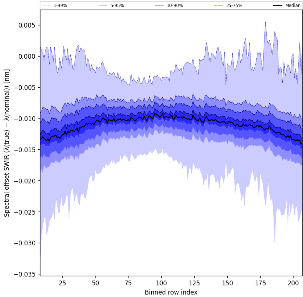
Figure 38: Along track statistics of “Spectral offset SWIR ( \lambda_{\text{true}} - \lambda_{\text{nominal}} )” for 2025-06-11 to 2025-06-12
