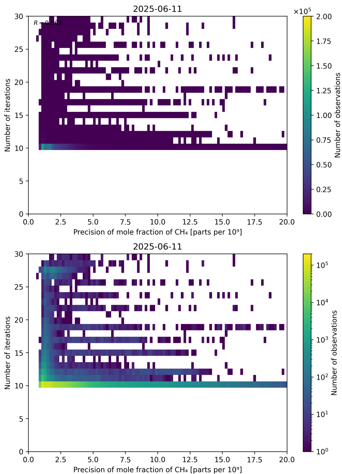
Figure 83: Scatter density plot of “Precision of mole fraction of CH 4 ” against “Number of iterations” for 2025-06-11 to 2025-06-12.
