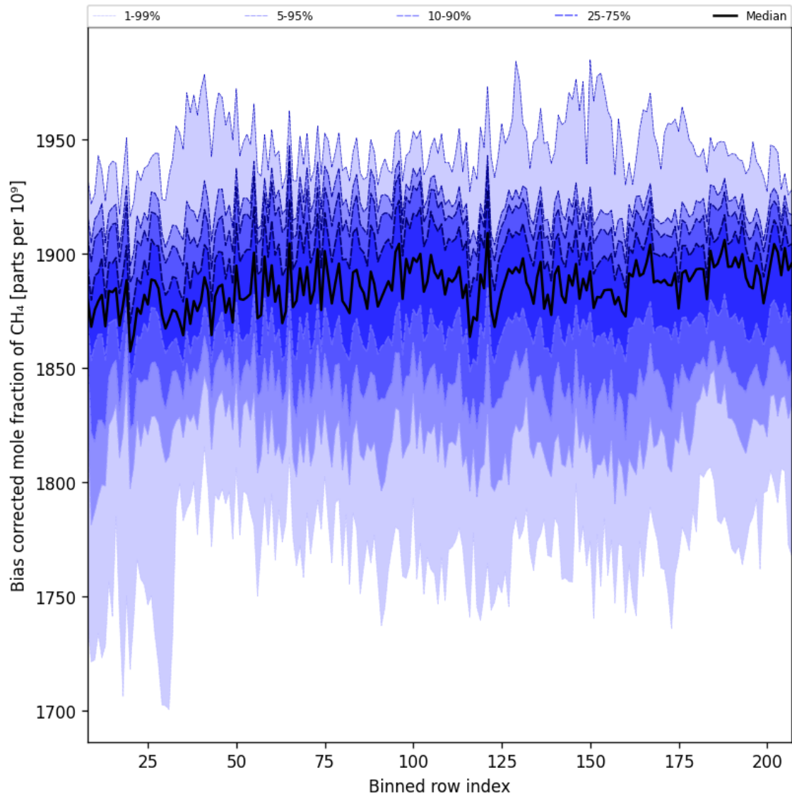
Figure 36: Along track statistics of “Bias corrected mole fraction of CH 4 ” for 2025-06-11 to 2025-06-12
