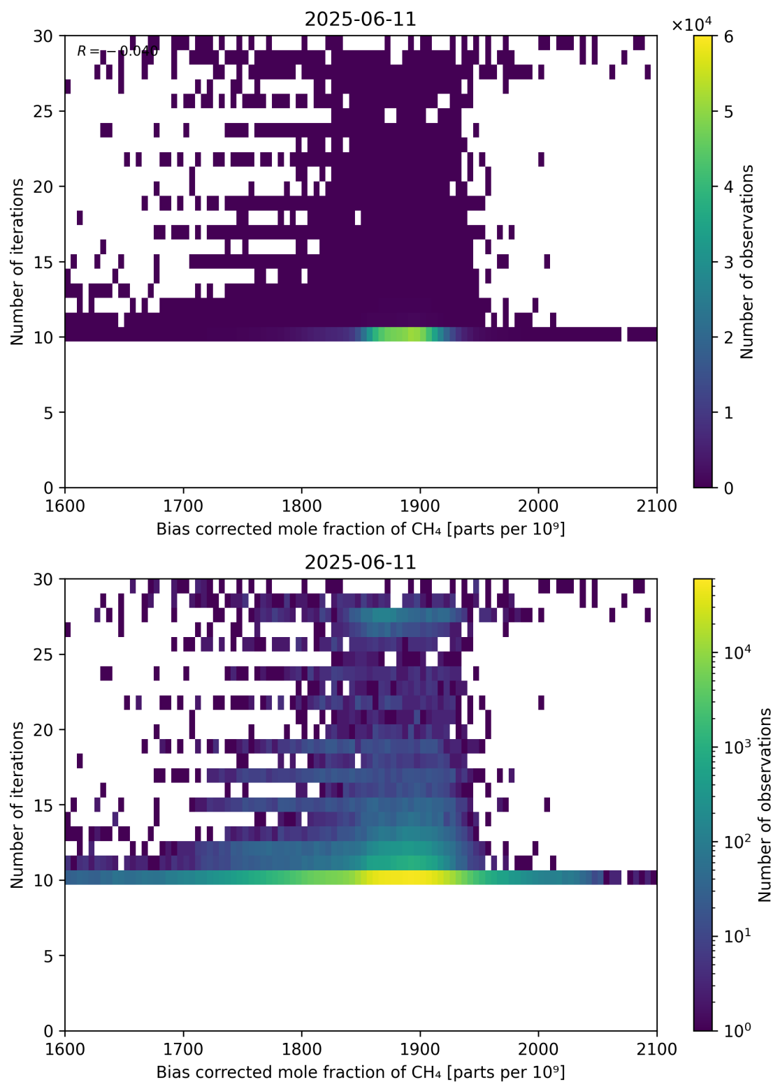
Figure 67: Scatter density plot of “Bias corrected mole fraction of CH 4 ” against “Number of iterations” for 2025-06-11 to 2025-06-12.
