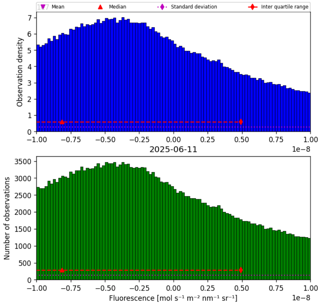
Figure 32: Histogram of “Fluorescence” for 2025-06-11 to 2025-06-12
