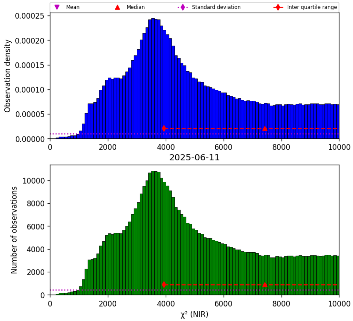
Figure 29: Histogram of " \chi^2 (NIR)" for 2025-06-11 to 2025-06-12
