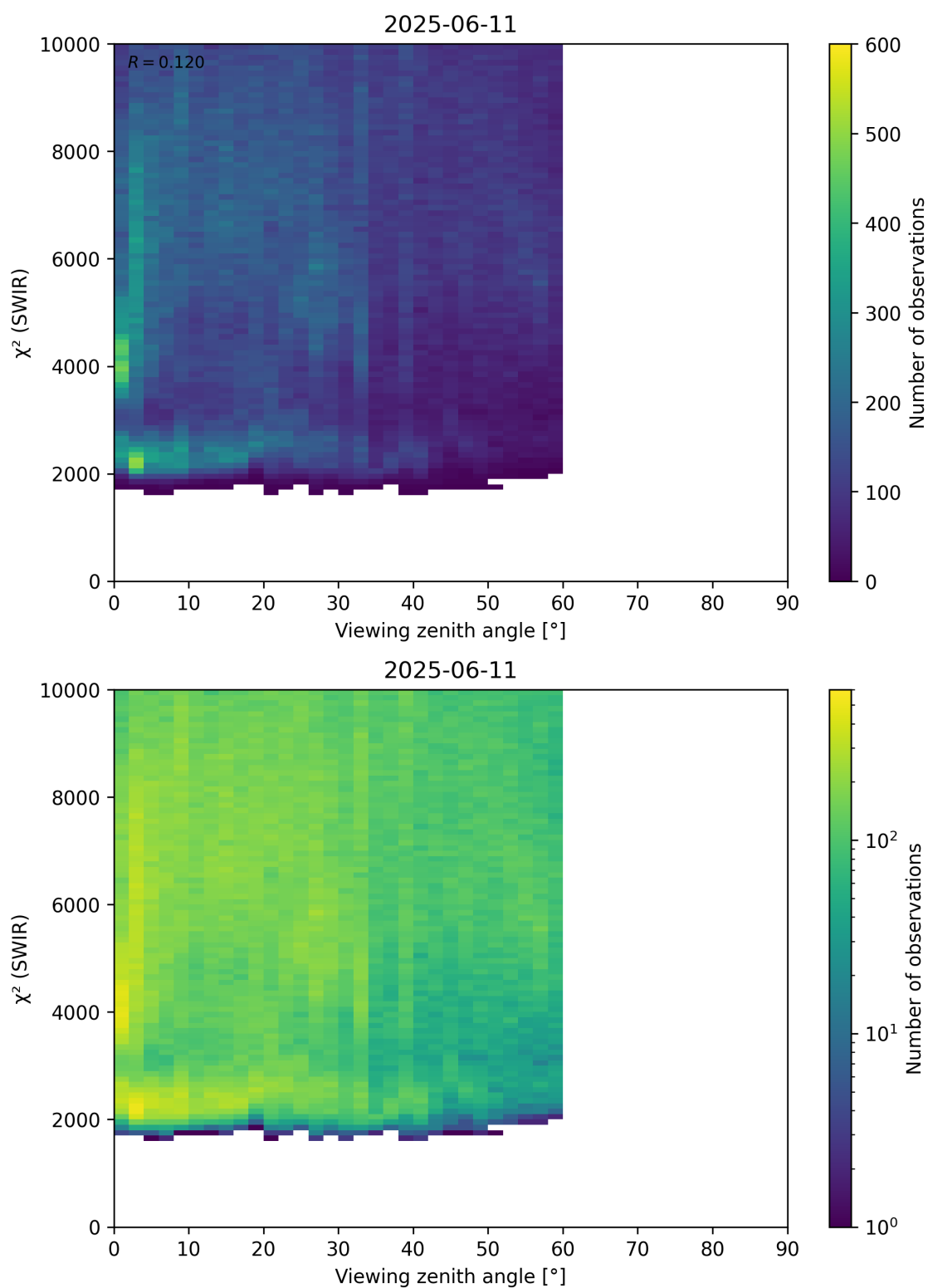
Figure 106: Scatter density plot of “Viewing zenith angle” against “ \chi^2 (SWIR)” for 2025-06-11 to 2025-06-12.
