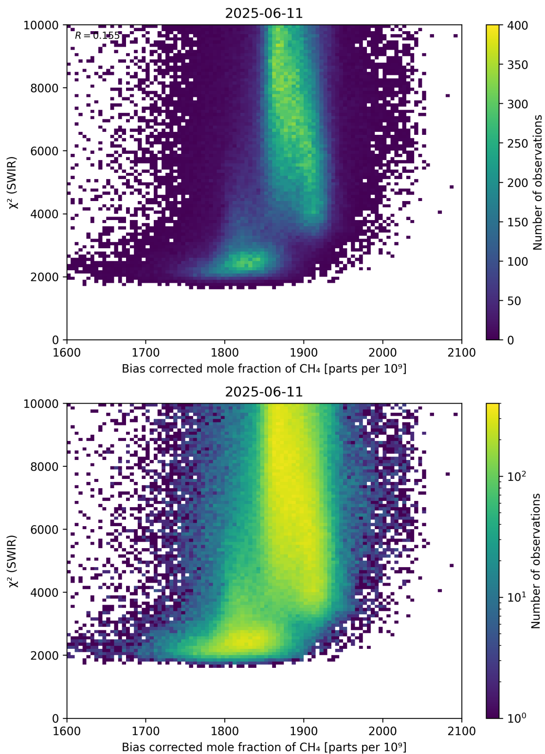
Figure 64: Scatter density plot of “Bias corrected mole fraction of \text{CH}_4 ” against “ \chi^2 (SWIR)” for 2025-06-11 to 2025-06-12.
