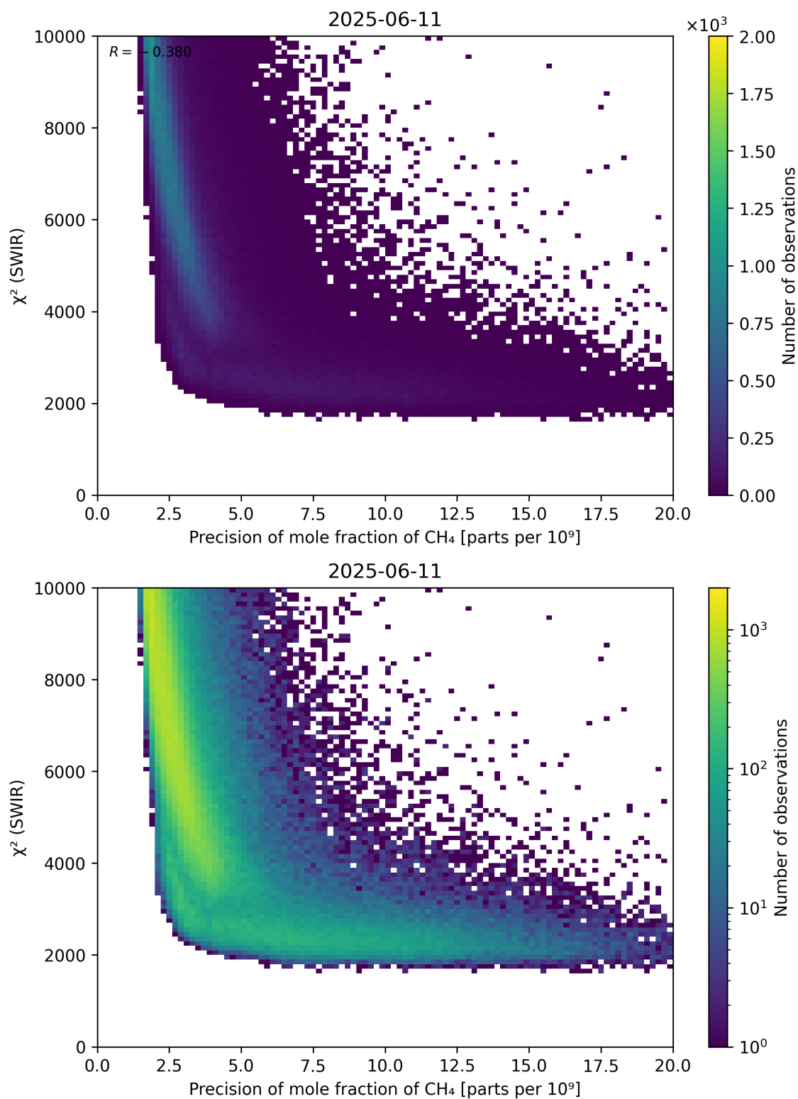
Figure 79: Scatter density plot of “Precision of mole fraction of \text{CH}_4 ” against “ \chi^2 (SWIR)” for 2025-06-11 to 2025-06-12.
