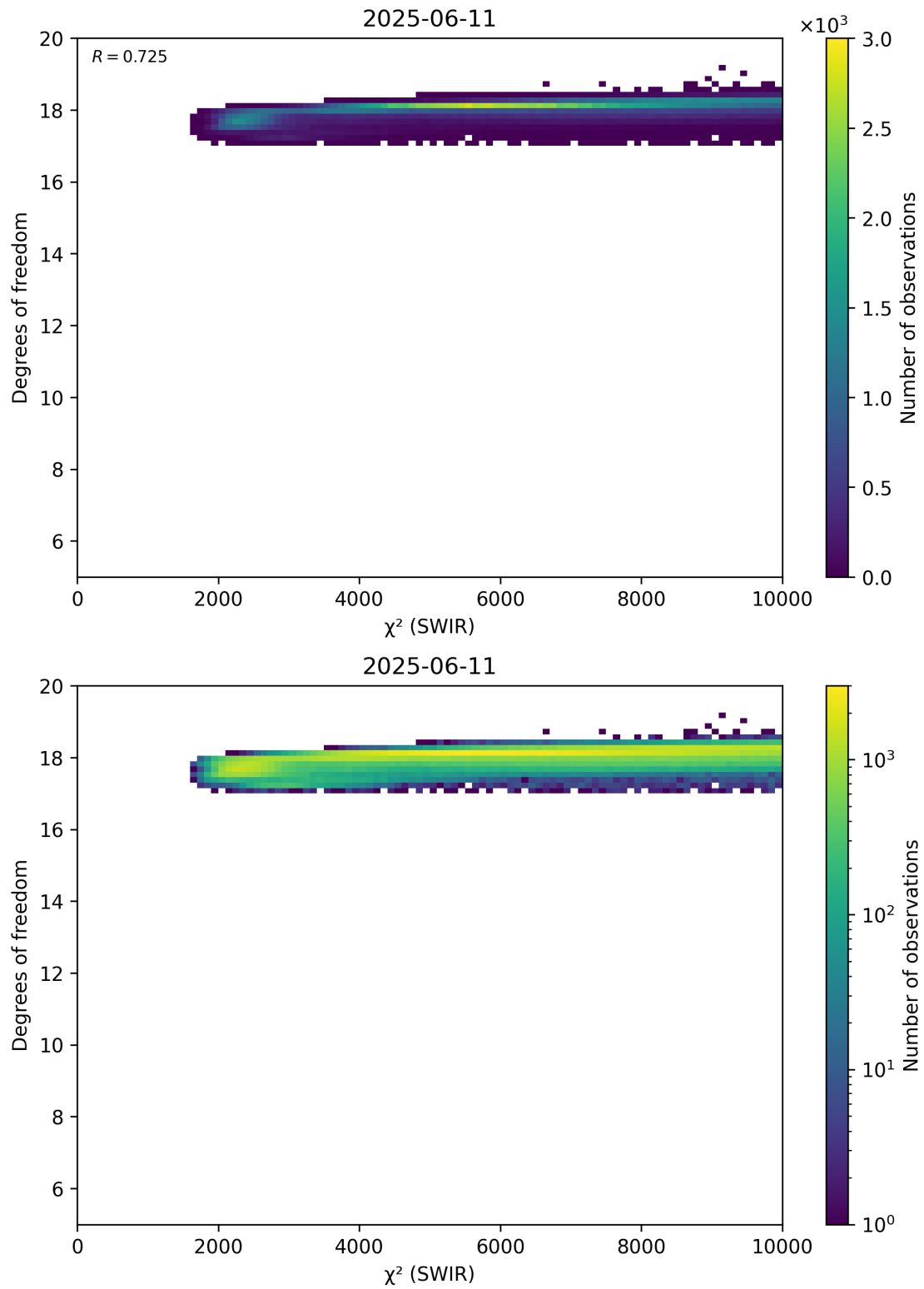
Figure 48: Scatter density plot of “ \chi^2 (SWIR)” against “Degrees of freedom” for 2025-06-11 to 2025-06-12.
