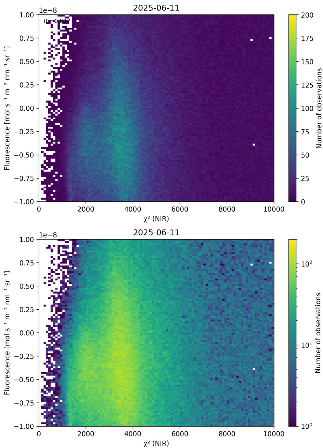
Figure 45: Scatter density plot of “ \chi^2 (NIR)” against “Fluorescence” for 2025-06-11 to 2025-06-12.
