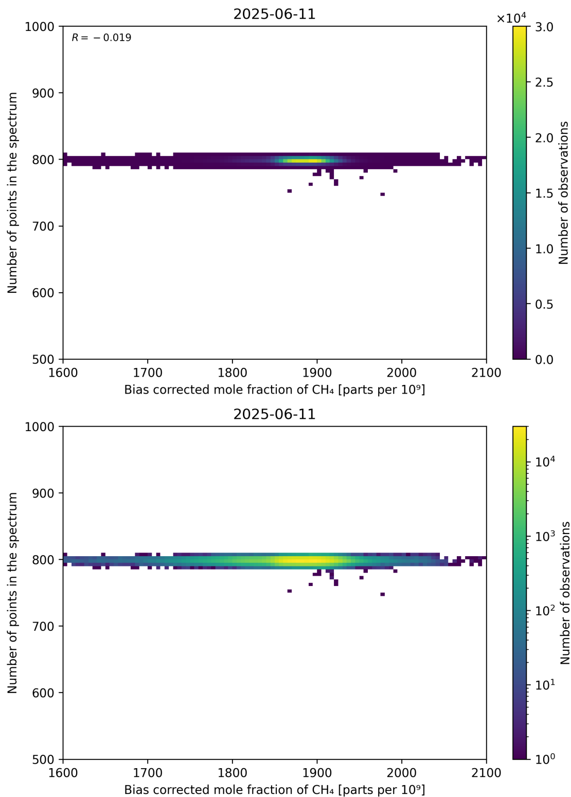
Figure 68: Scatter density plot of “Bias corrected mole fraction of CH 4 ” against “Number of points in the spectrum” for 2025-06-11 to 2025-06-12.
