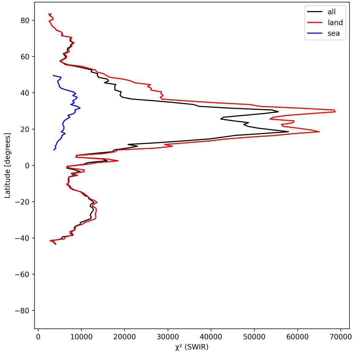
Figure 17: Zonal average of “ \chi^2 (SWIR)” for 2025-06-11 to 2025-06-12.
