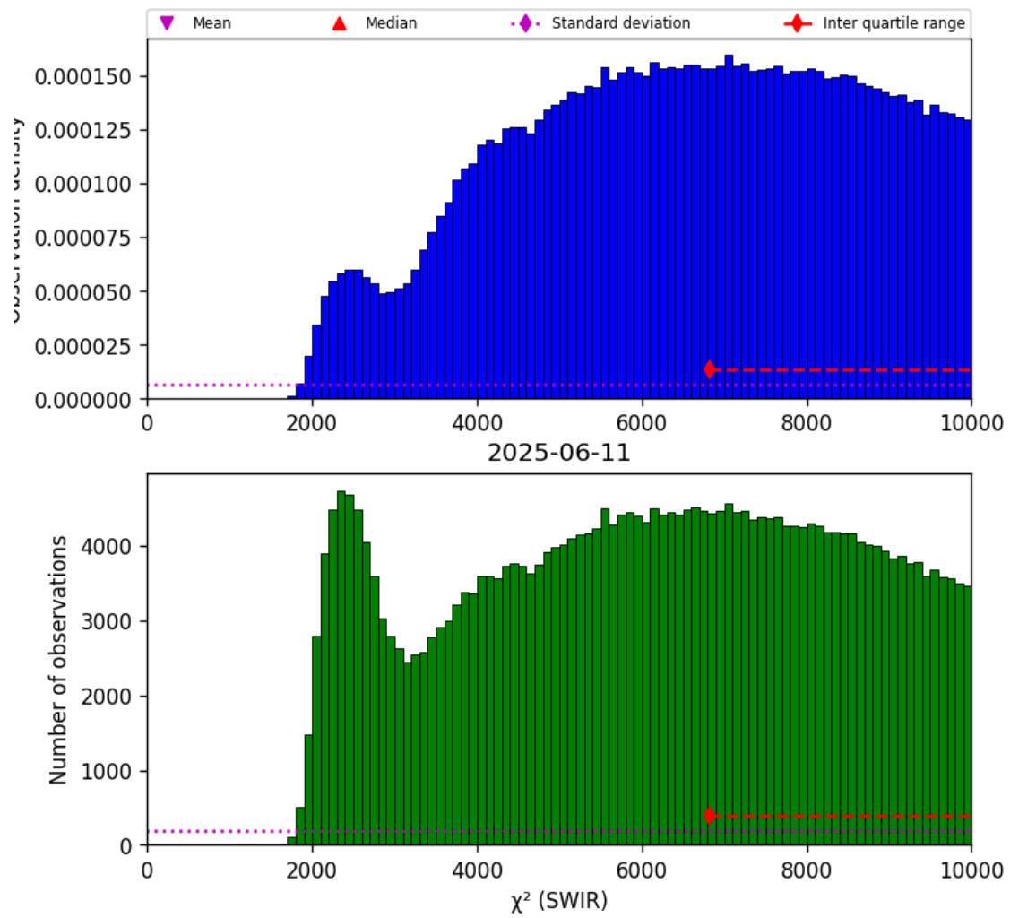
Figure 28: Histogram of “ \chi^2 (SWIR)” for 2025-06-11 to 2025-06-12
