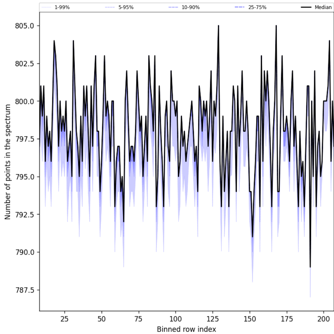
Figure 37: Along track statistics of “Number of points in the spectrum” for 2025-06-11 to 2025-06-12
