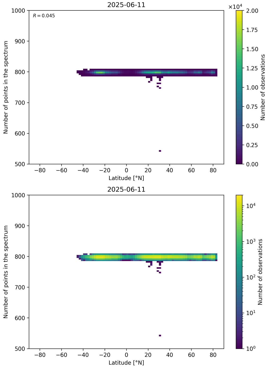
Figure 61: Scatter density plot of “Latitude” against “Number of points in the spectrum” for 2025-06-11 to 2025-06-12.
