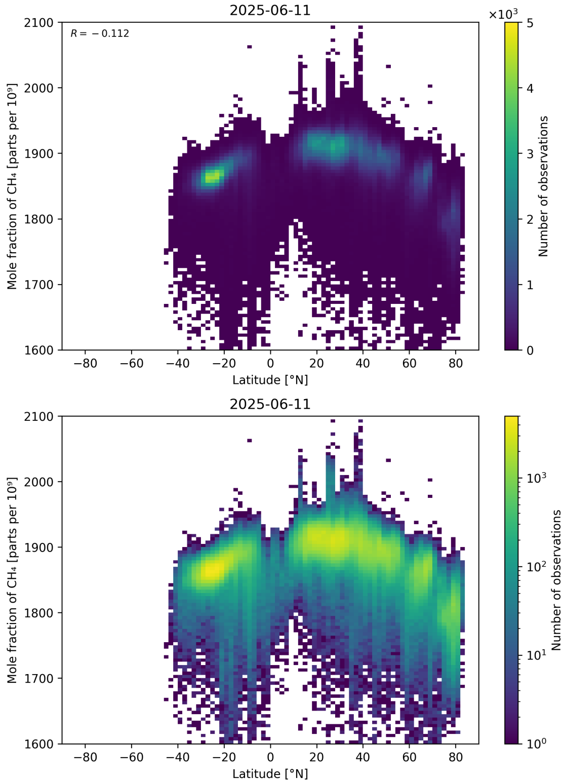
Figure 57: Scatter density plot of “Latitude” against “Mole fraction of \text{CH}_4 ” for 2025-06-11 to 2025-06-12.
