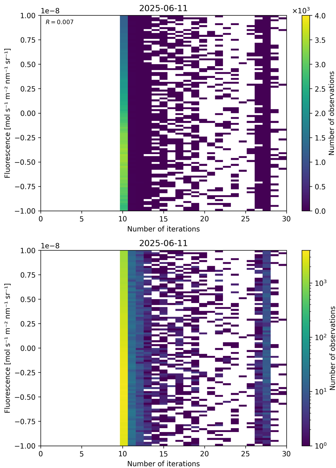
Figure 87: Scatter density plot of “Number of iterations” against “Fluorescence” for 2025-06-11 to 2025-06-12.
