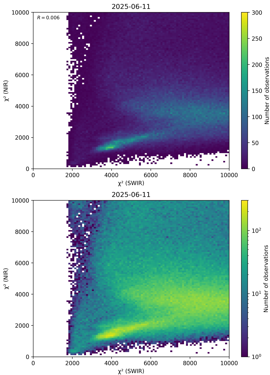
Figure 47: Scatter density plot of “ \chi^2 (SWIR)” against “ \chi^2 (NIR)” for 2025-06-11 to 2025-06-12.
