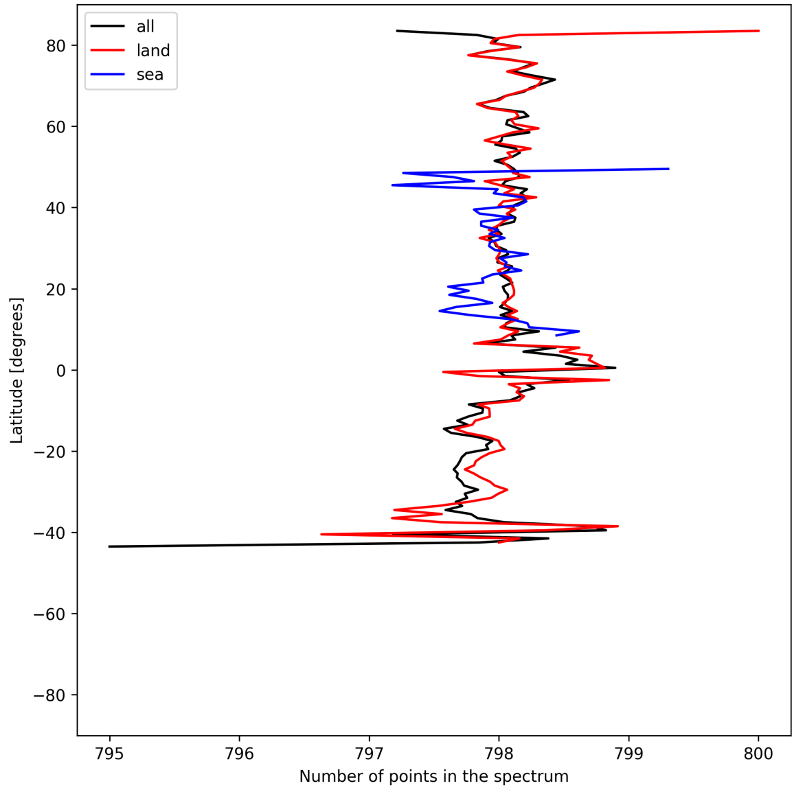
Figure 15: Zonal average of “Number of points in the spectrum” for 2025-06-11 to 2025-06-12.
