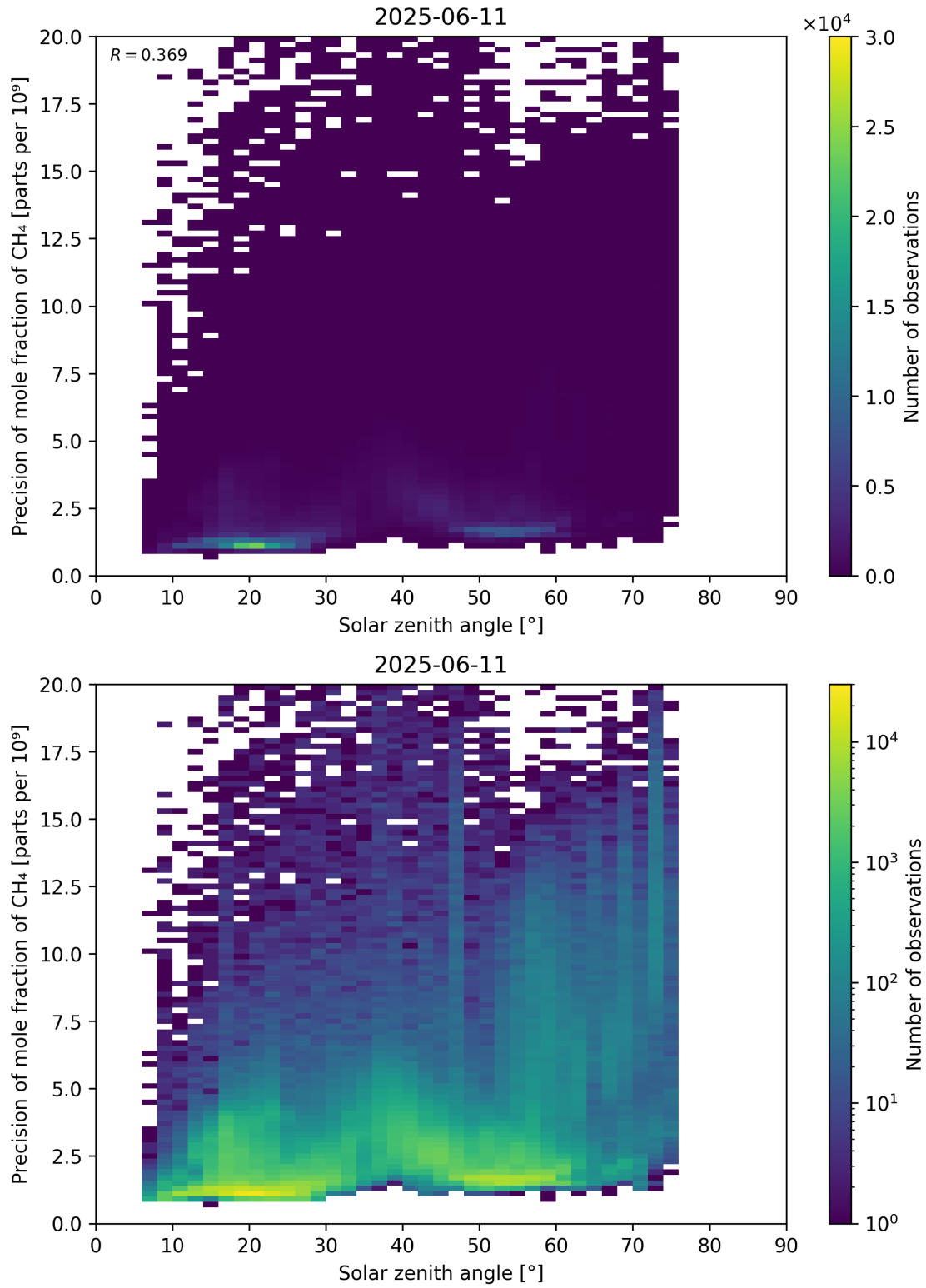
Figure 101: Scatter density plot of “Solar zenith angle” against “Precision of mole fraction of CH 4 ” for 2025-06-11 to 2025-06-12.
