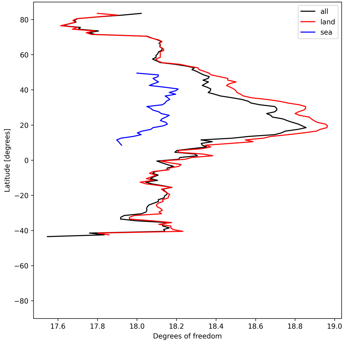
Figure 19: Zonal average of “Degrees of freedom” for 2025-06-11 to 2025-06-12.
