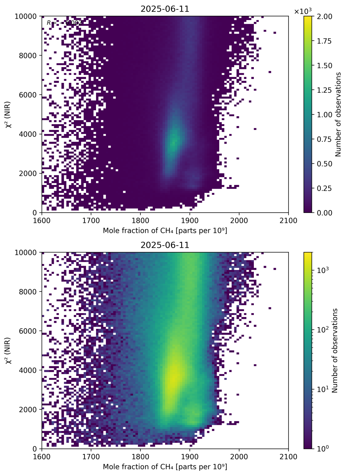
Figure 70: Scatter density plot of “Mole fraction of \text{CH}_4 ” against “ \chi^2 (NIR)” for 2025-06-11 to 2025-06-12.
