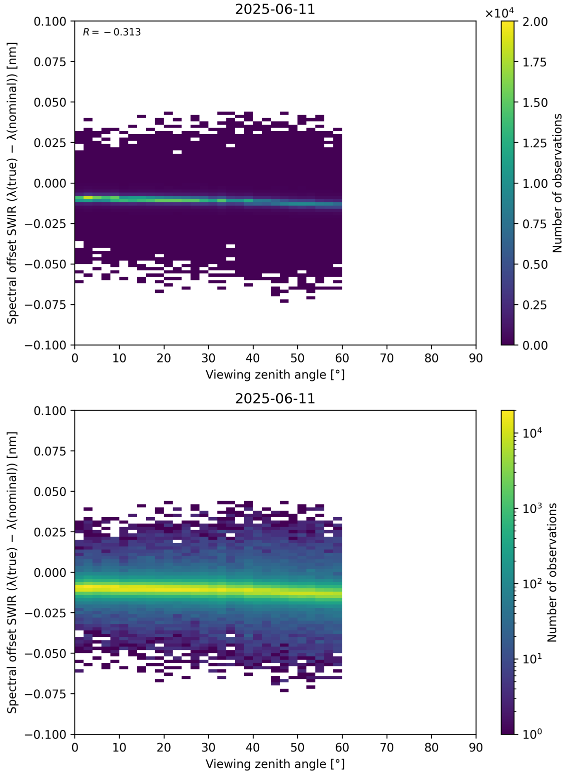
Figure 116: Scatter density plot of “Viewing zenith angle” against “Spectral offset SWIR ( \lambda_{\text{true}} - \lambda_{\text{nominal}} )” for 2025-06-11 to 2025-06-12.
