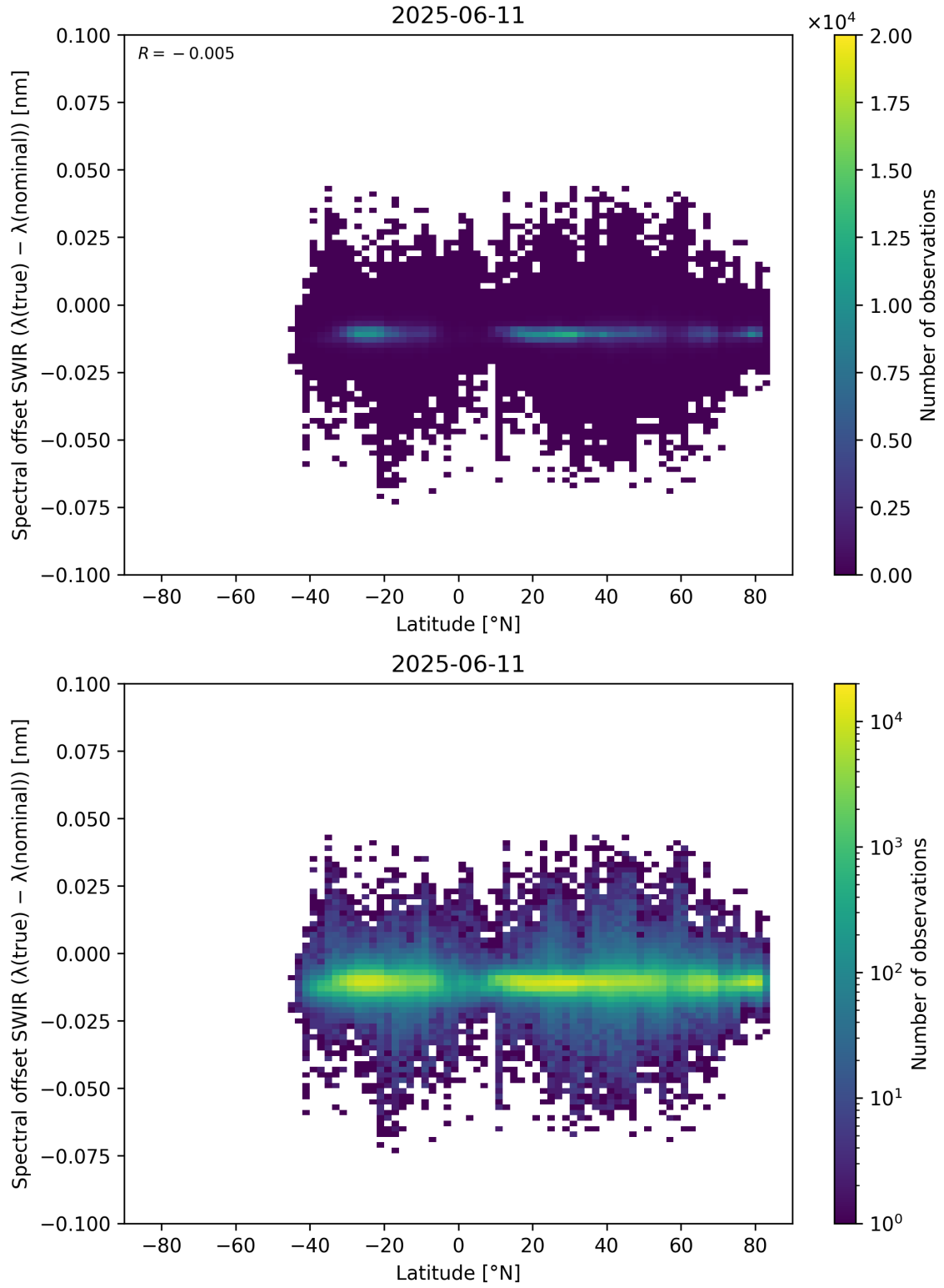
Figure 62: Scatter density plot of “Latitude” against “Spectral offset SWIR ( \lambda_{\text{true}} - \lambda_{\text{nominal}} )” for 2025-06-11 to 2025-06-12.
