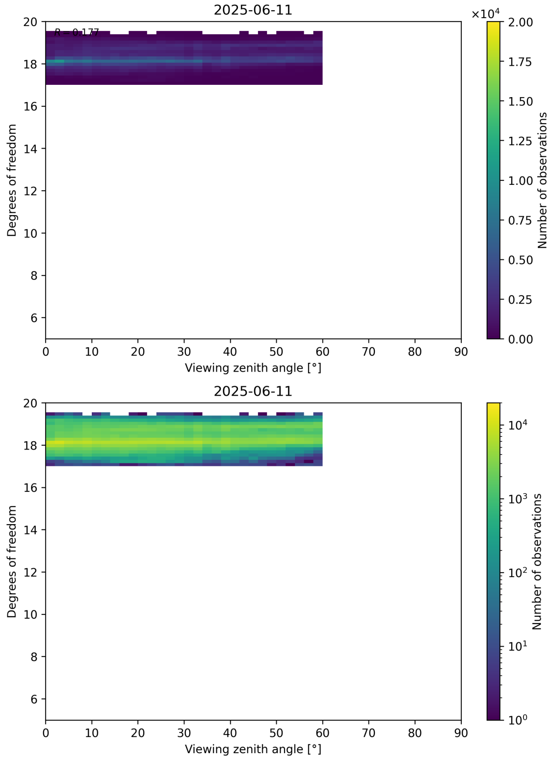
Figure 107: Scatter density plot of “Viewing zenith angle” against “Degrees of freedom” for 2025-06-11 to 2025-06-12.
