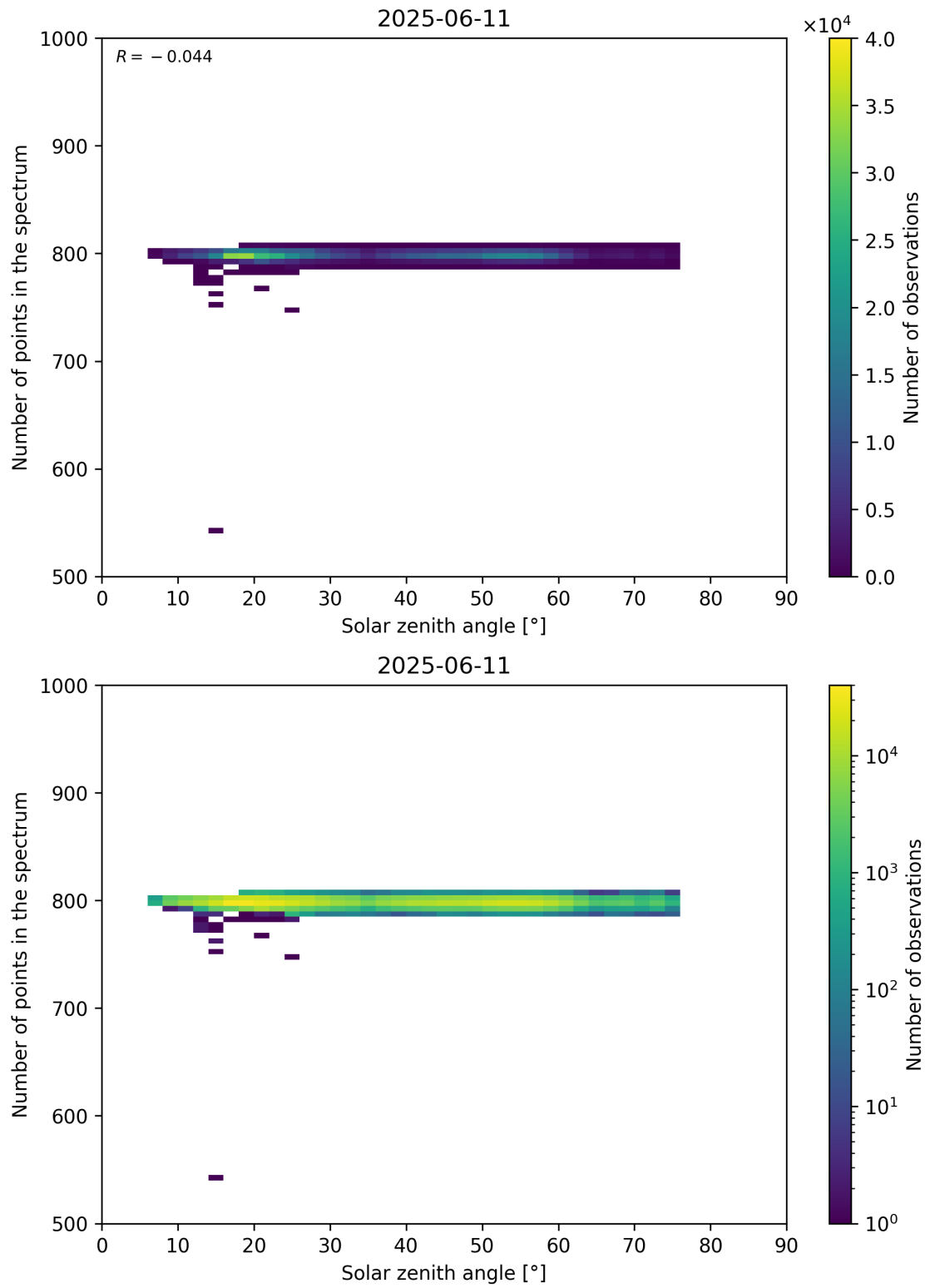
Figure 103: Scatter density plot of “Solar zenith angle” against “Number of points in the spectrum” for 2025-06-11 to 2025-06-12.
