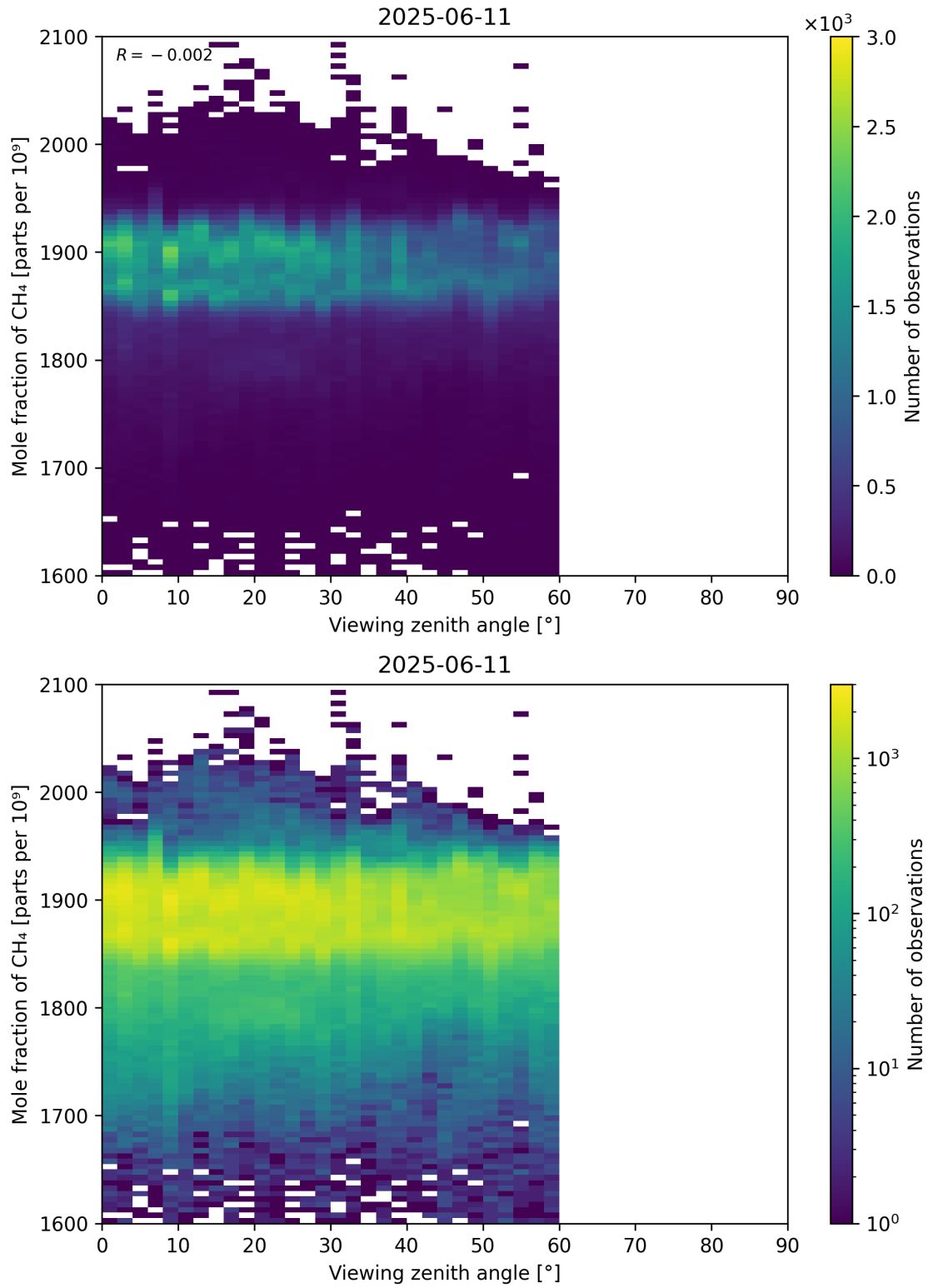
Figure 110: Scatter density plot of “Viewing zenith angle” against “Mole fraction of CH 4 ” for 2025-06-11 to 2025-06-12.
