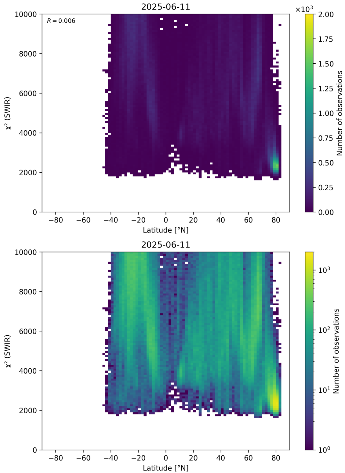
Figure 54: Scatter density plot of “Latitude” against “ \chi^2 (SWIR)” for 2025-06-11 to 2025-06-12.
