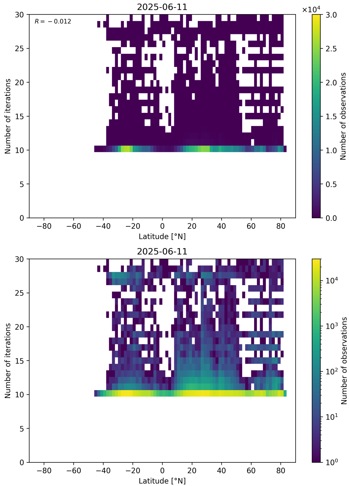
Figure 60: Scatter density plot of “Latitude” against “Number of iterations” for 2025-06-11 to 2025-06-12.
