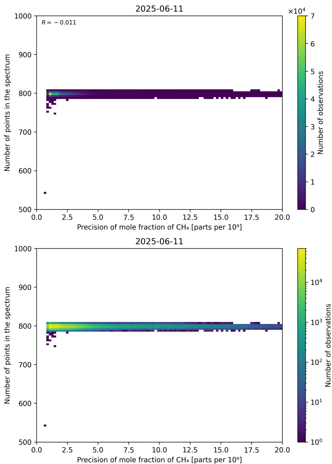
Figure 84: Scatter density plot of “Precision of mole fraction of CH 4 ” against “Number of points in the spectrum” for 2025-06-11 to 2025-06-12.
