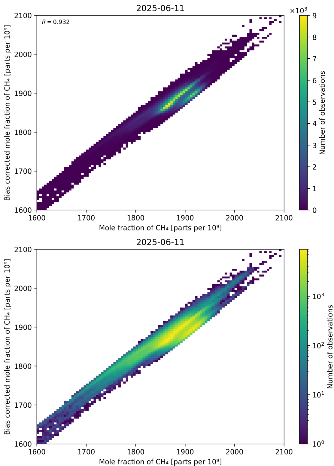
Figure 74: Scatter density plot of “Mole fraction of CH 4 ” against “Bias corrected mole fraction of CH 4 ” for 2025-06-11 to 2025-06-12.
