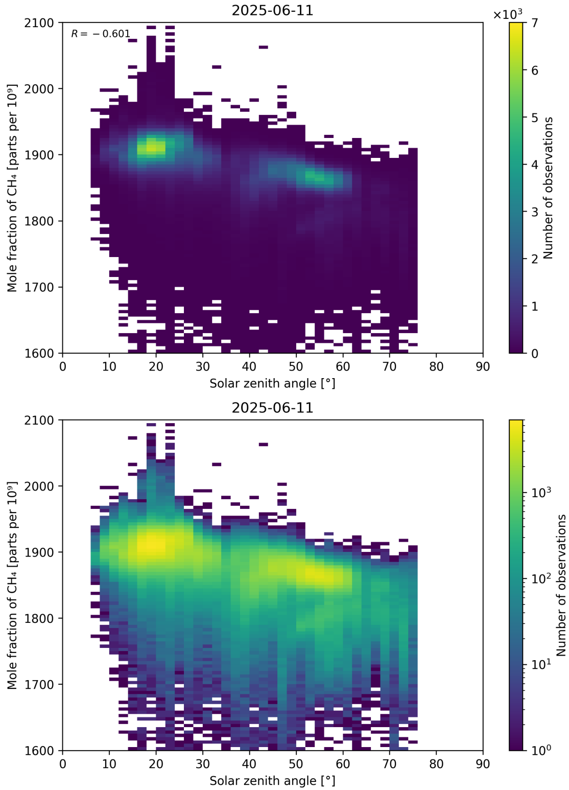
Figure 99: Scatter density plot of “Solar zenith angle” against “Mole fraction of \text{CH}_4 ” for 2025-06-11 to 2025-06-12.
