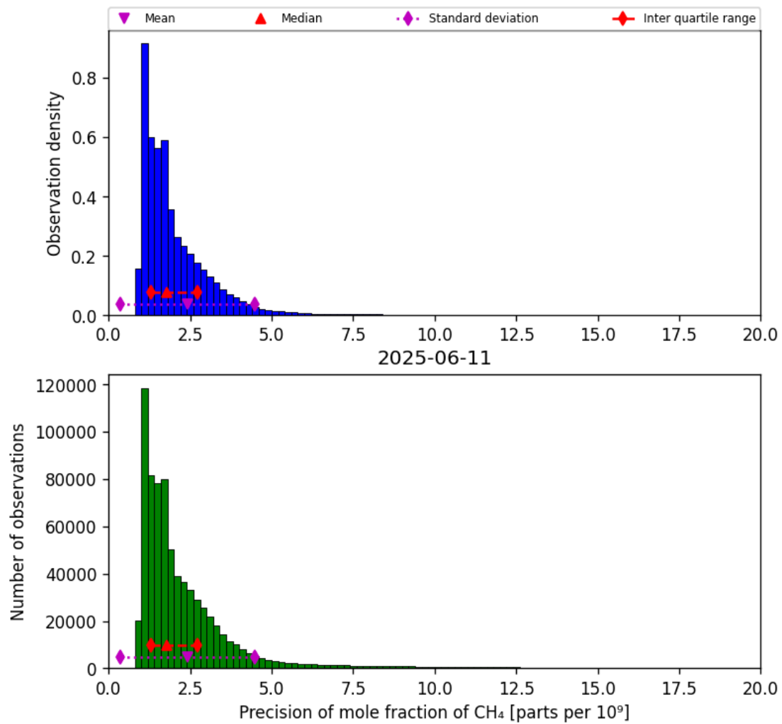
Figure 24: Histogram of “Precision of mole fraction of CH 4 ” for 2025-06-11 to 2025-06-12
