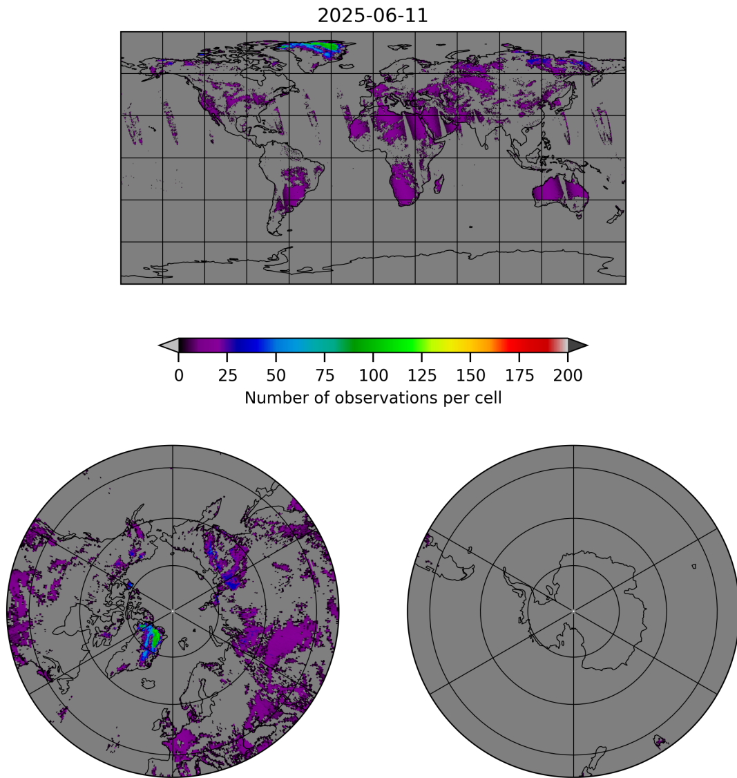
Figure 10: Map of the number of observations for 2025-06-11 to 2025-06-12
