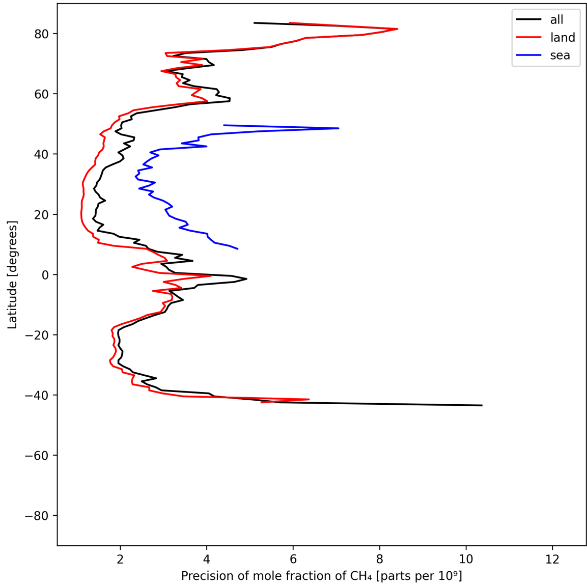
Figure 13: Zonal average of “Precision of mole fraction of CH 4 ” for 2025-06-11 to 2025-06-12.
