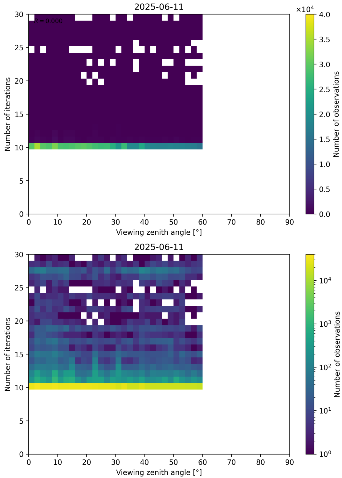
Figure 113: Scatter density plot of “Viewing zenith angle” against “Number of iterations” for 2025-06-11 to 2025-06-12.
