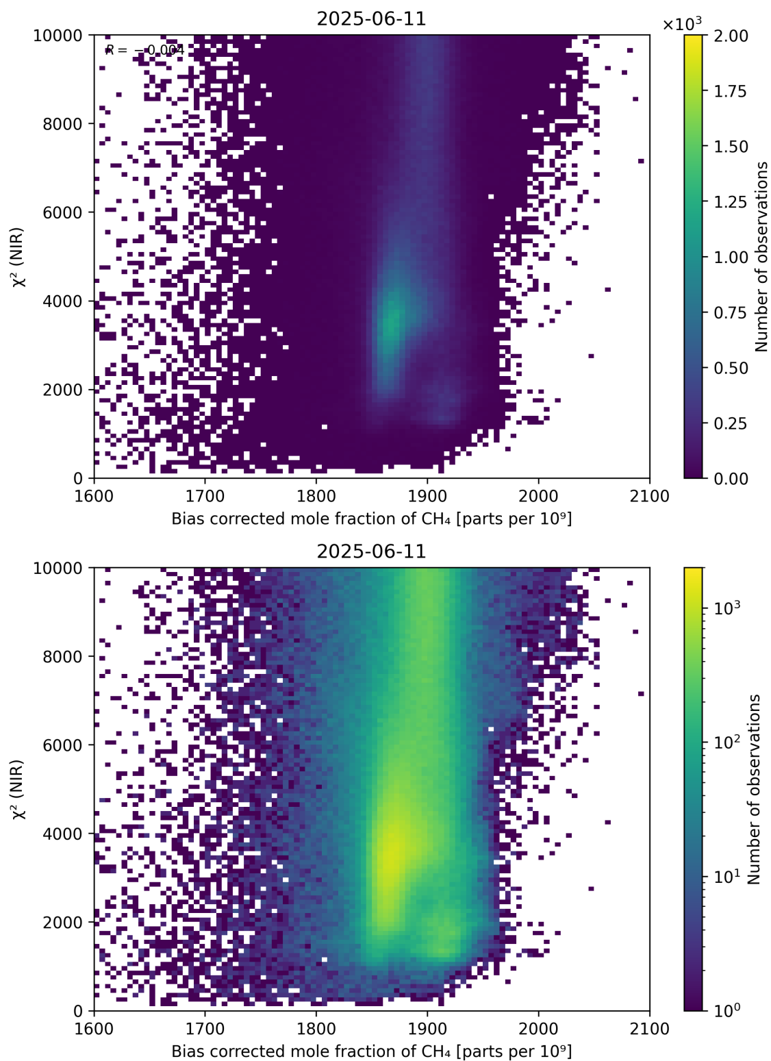
Figure 63: Scatter density plot of “Bias corrected mole fraction of \text{CH}_4 ” against “ \chi^2 (NIR)” for 2025-06-11 to 2025-06-12.
