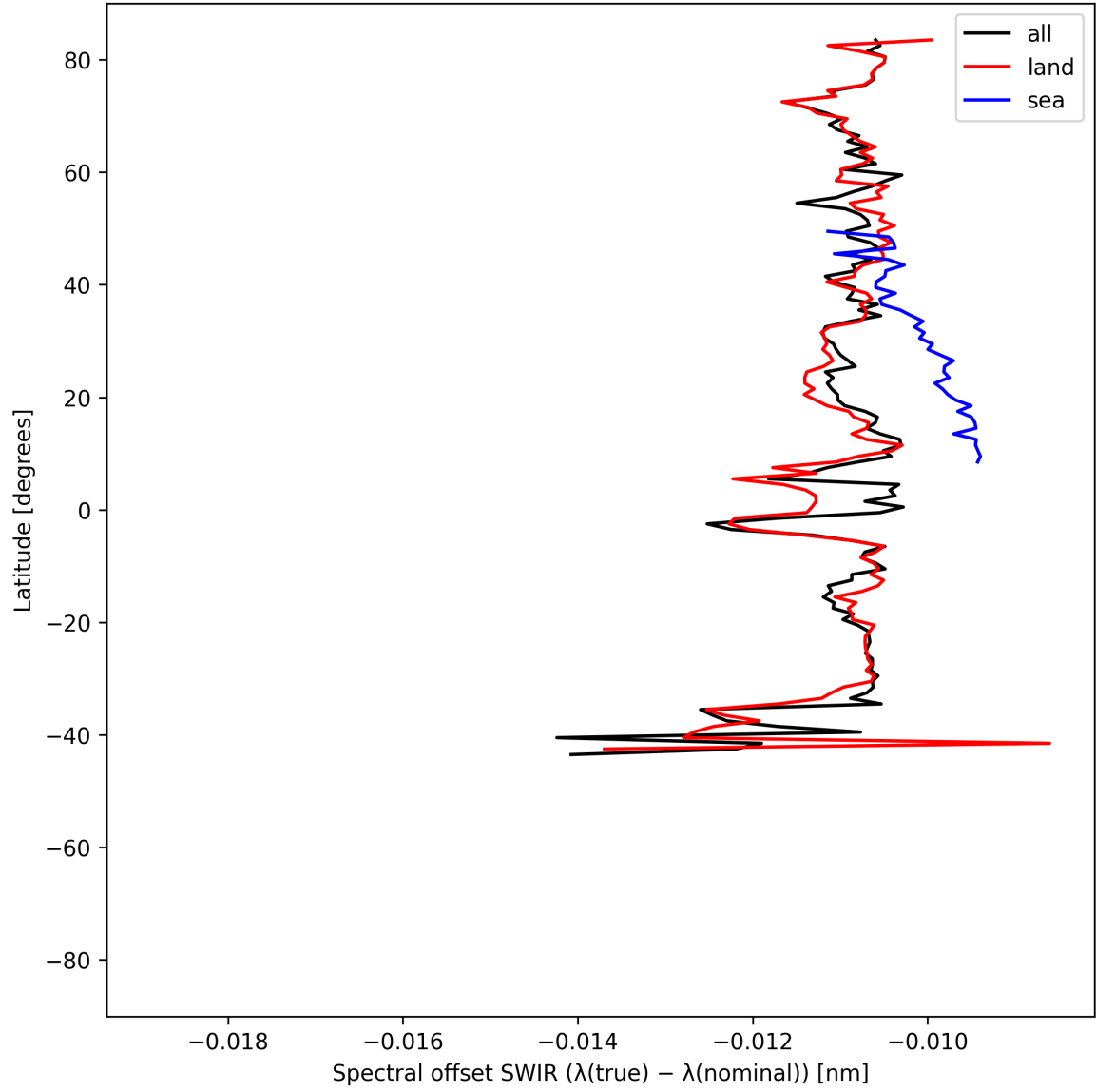
Figure 16: Zonal average of “Spectral offset SWIR ( \lambda_{\text{true}} - \lambda_{\text{nominal}} )” for 2025-06-11 to 2025-06-12.
