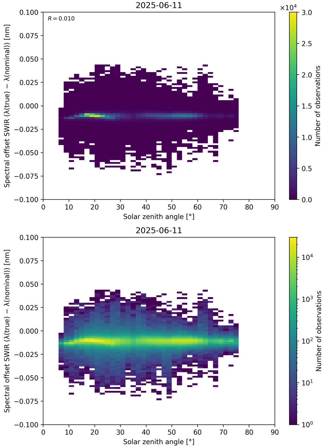
Figure 104: Scatter density plot of “Solar zenith angle” against “Spectral offset SWIR ( \lambda_{\text{true}} - \lambda_{\text{nominal}} )” for 2025-06-11 to 2025-06-12.
