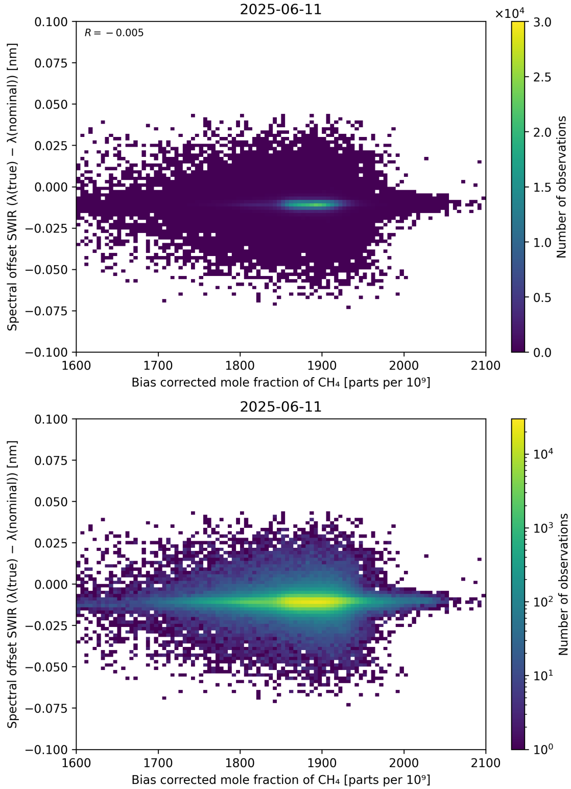
Figure 69: Scatter density plot of “Bias corrected mole fraction of CH 4 ” against “Spectral offset SWIR ( \lambda_{\text{true}} - \lambda_{\text{nominal}} )” for 2025-06-11 to 2025-06-12.
