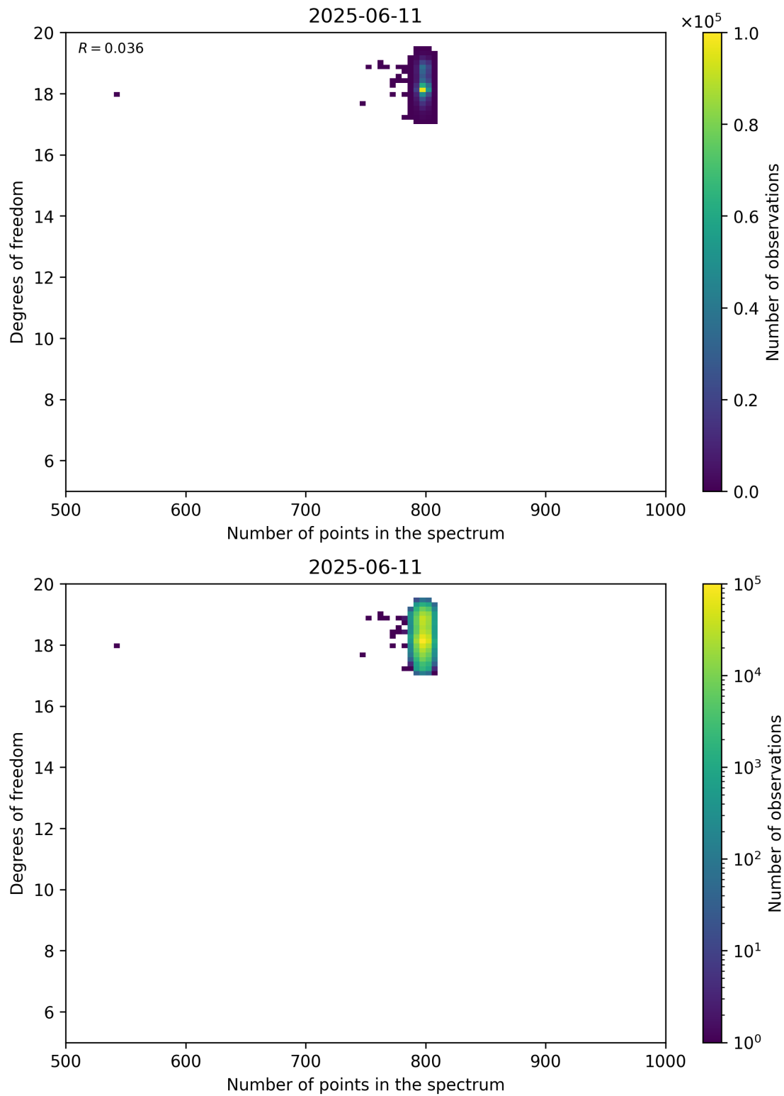
Figure 90: Scatter density plot of “Number of points in the spectrum” against “Degrees of freedom” for 2025-06-11 to 2025-06-12.
