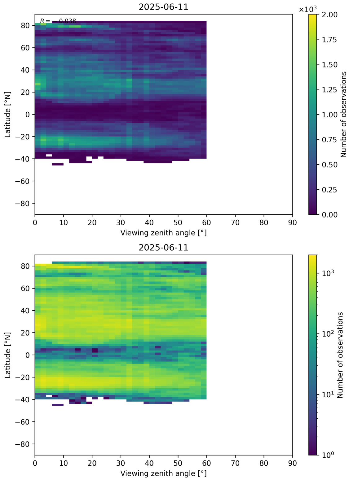
Figure 109: Scatter density plot of “Viewing zenith angle” against “Latitude” for 2025-06-11 to 2025-06-12.
