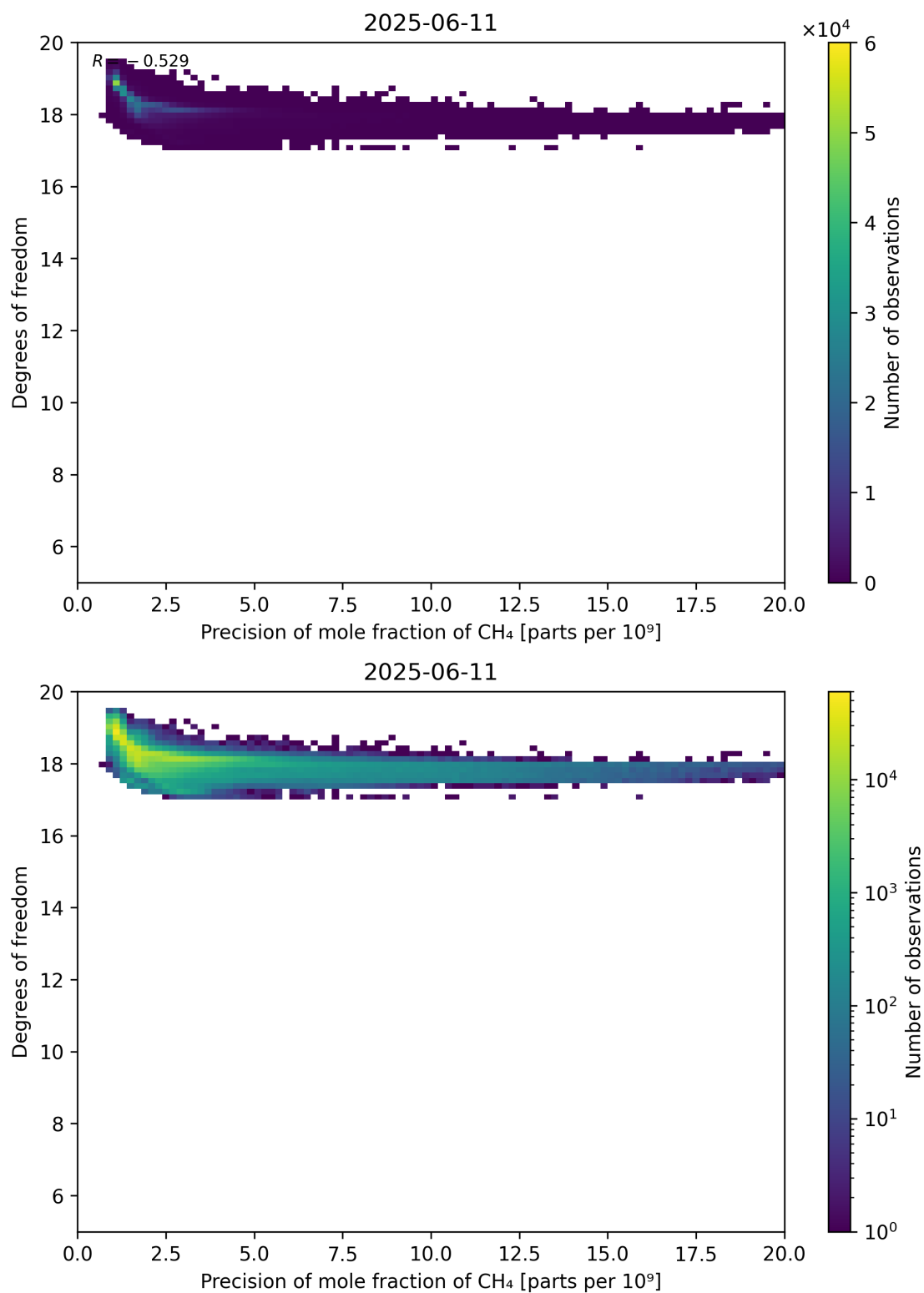
Figure 80: Scatter density plot of “Precision of mole fraction of CH 4 ” against “Degrees of freedom” for 2025-06-11 to 2025-06-12.
