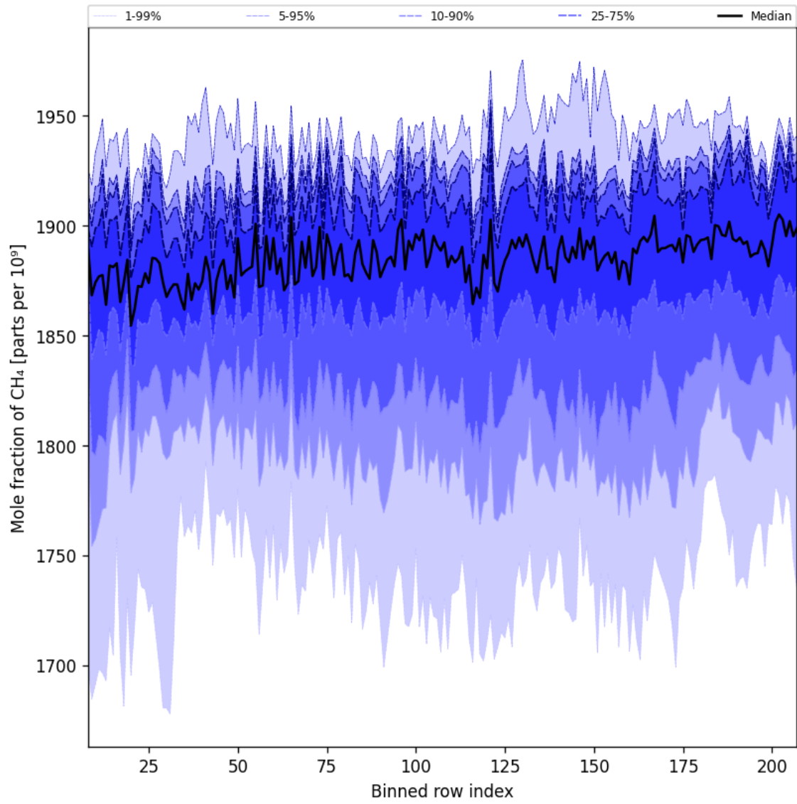
Figure 34: Along track statistics of “Mole fraction of CH 4 ” for 2025-06-11 to 2025-06-12
