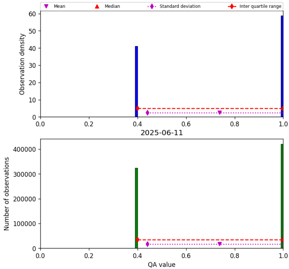
Figure 22: Histogram of “QA value” for 2025-06-11 to 2025-06-12
