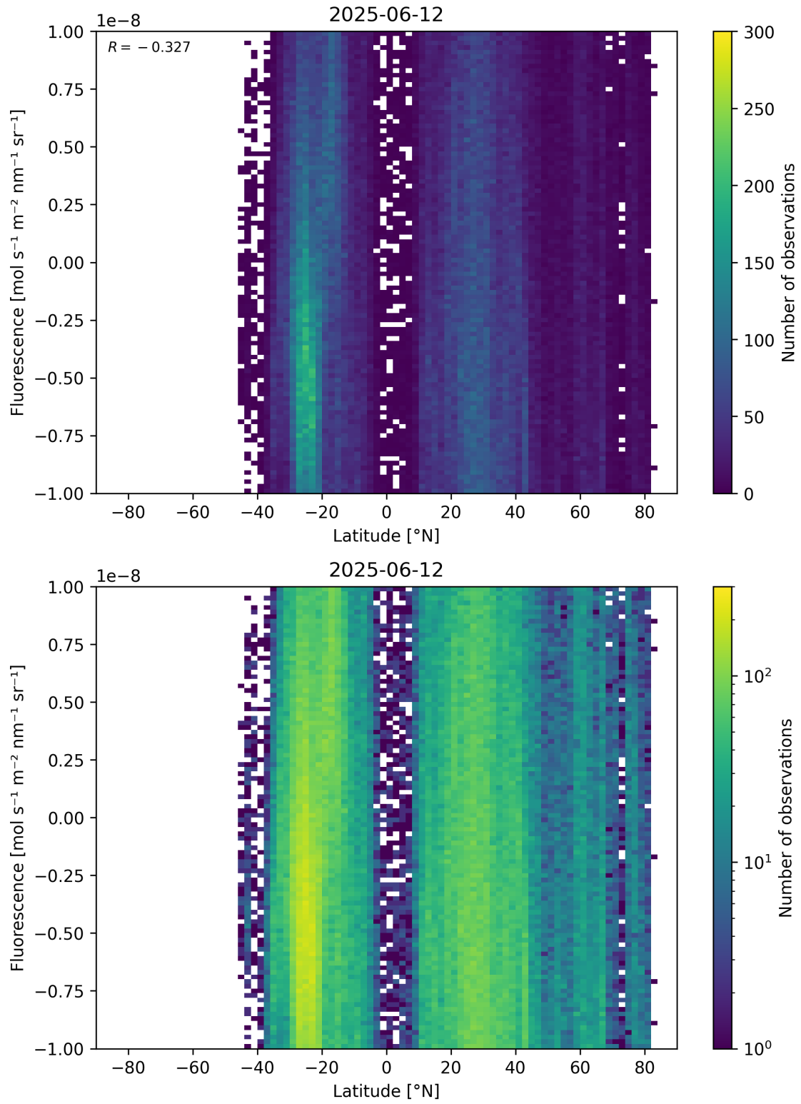
Figure 56: Scatter density plot of “Latitude” against “Fluorescence” for 2025-06-11 to 2025-06-13.
