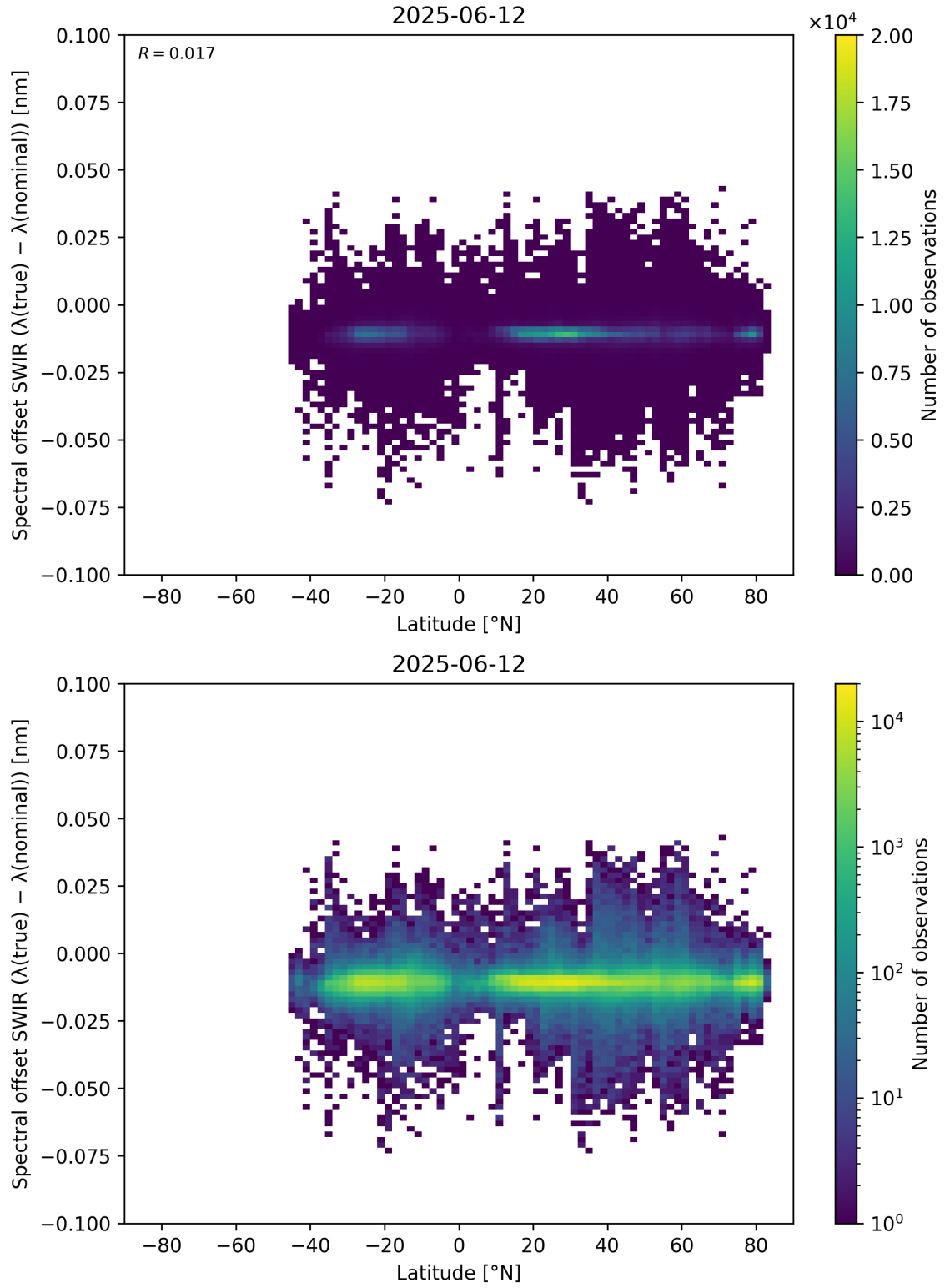
Figure 62: Scatter density plot of “Latitude” against “Spectral offset SWIR ( \lambda_{\text{true}} - \lambda_{\text{nominal}} )” for 2025-06-11 to 2025-06-13.
