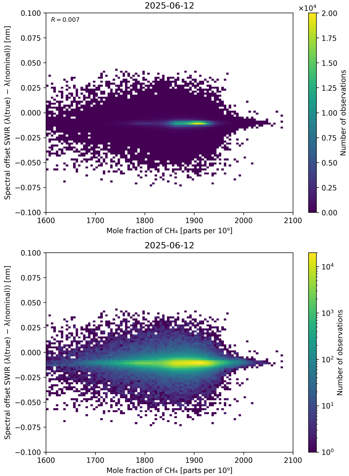
Figure 86: Scatter density plot of “Mole fraction of CH 4 ” against “Spectral offset SWIR ( \lambda_{\text{true}} - \lambda_{\text{nominal}} )” for 2025-06-11 to 2025-06-13.
