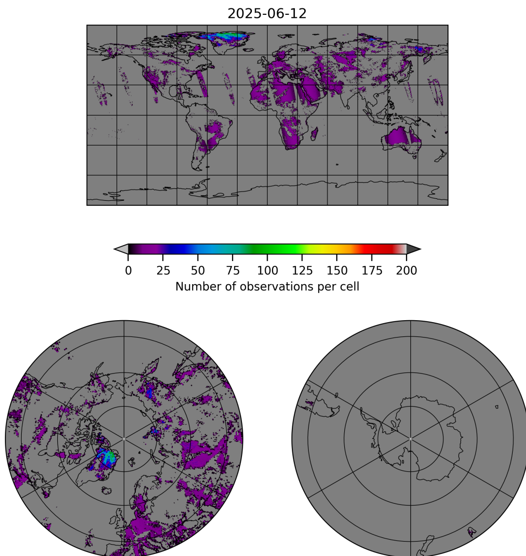
Figure 10: Map of the number of observations for 2025-06-11 to 2025-06-13
