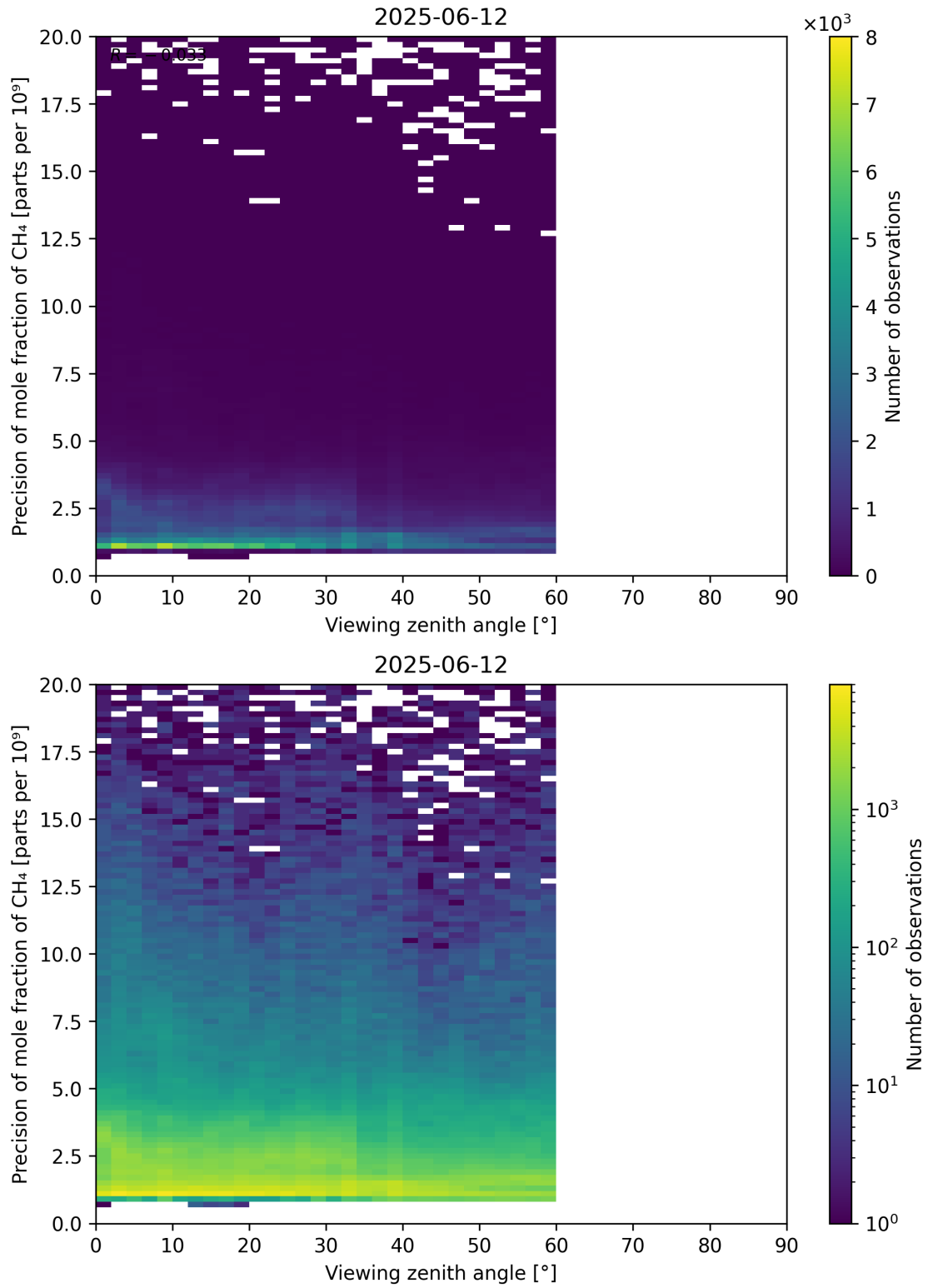
Figure 112: Scatter density plot of “Viewing zenith angle” against “Precision of mole fraction of CH 4 ” for 2025-06-11 to 2025-06-13.
