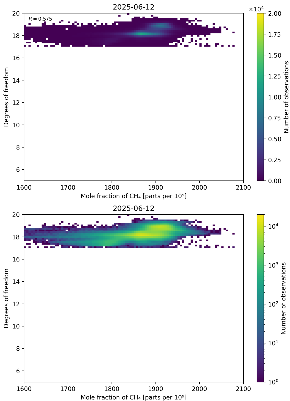
Figure 72: Scatter density plot of “Mole fraction of CH 4 ” against “Degrees of freedom” for 2025-06-11 to 2025-06-13.
