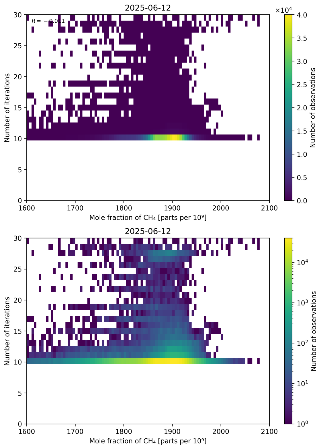
Figure 76: Scatter density plot of “Mole fraction of CH 4 ” against “Number of iterations” for 2025-06-11 to 2025-06-13.
