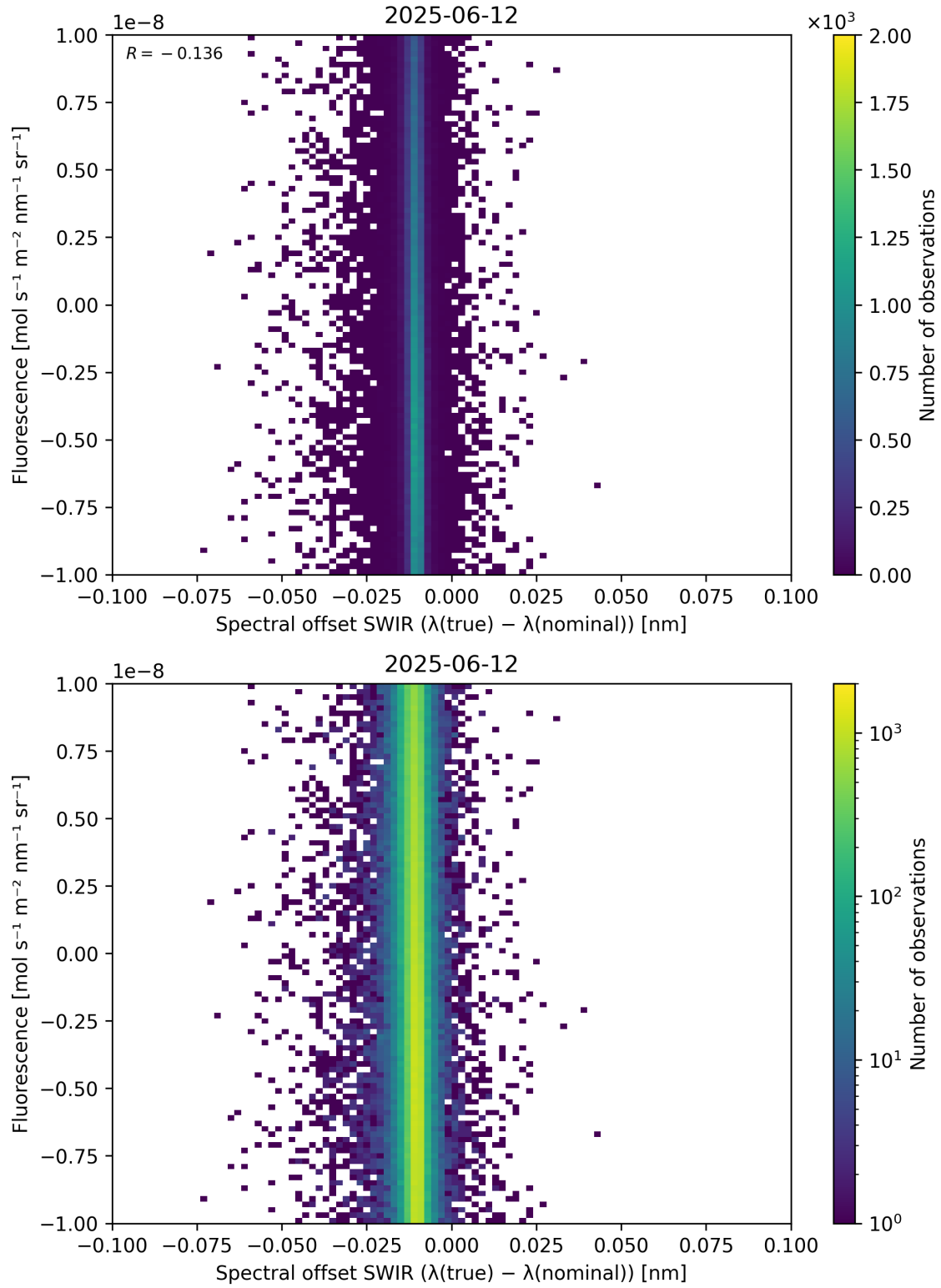
Figure 120: Scatter density plot of “Spectral offset SWIR ( \lambda_{\text{true}} - \lambda_{\text{nominal}} )” against “Fluorescence” for 2025-06-11 to 2025-06-13.
