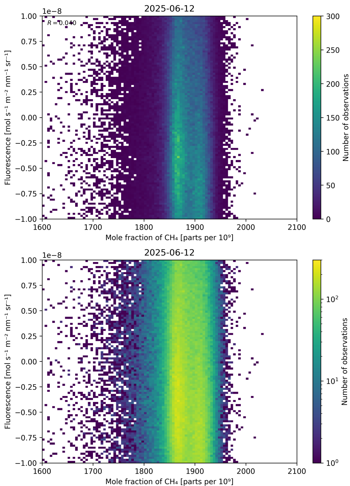
Figure 73: Scatter density plot of “Mole fraction of \text{CH}_4 ” against “Fluorescence” for 2025-06-11 to 2025-06-13.
