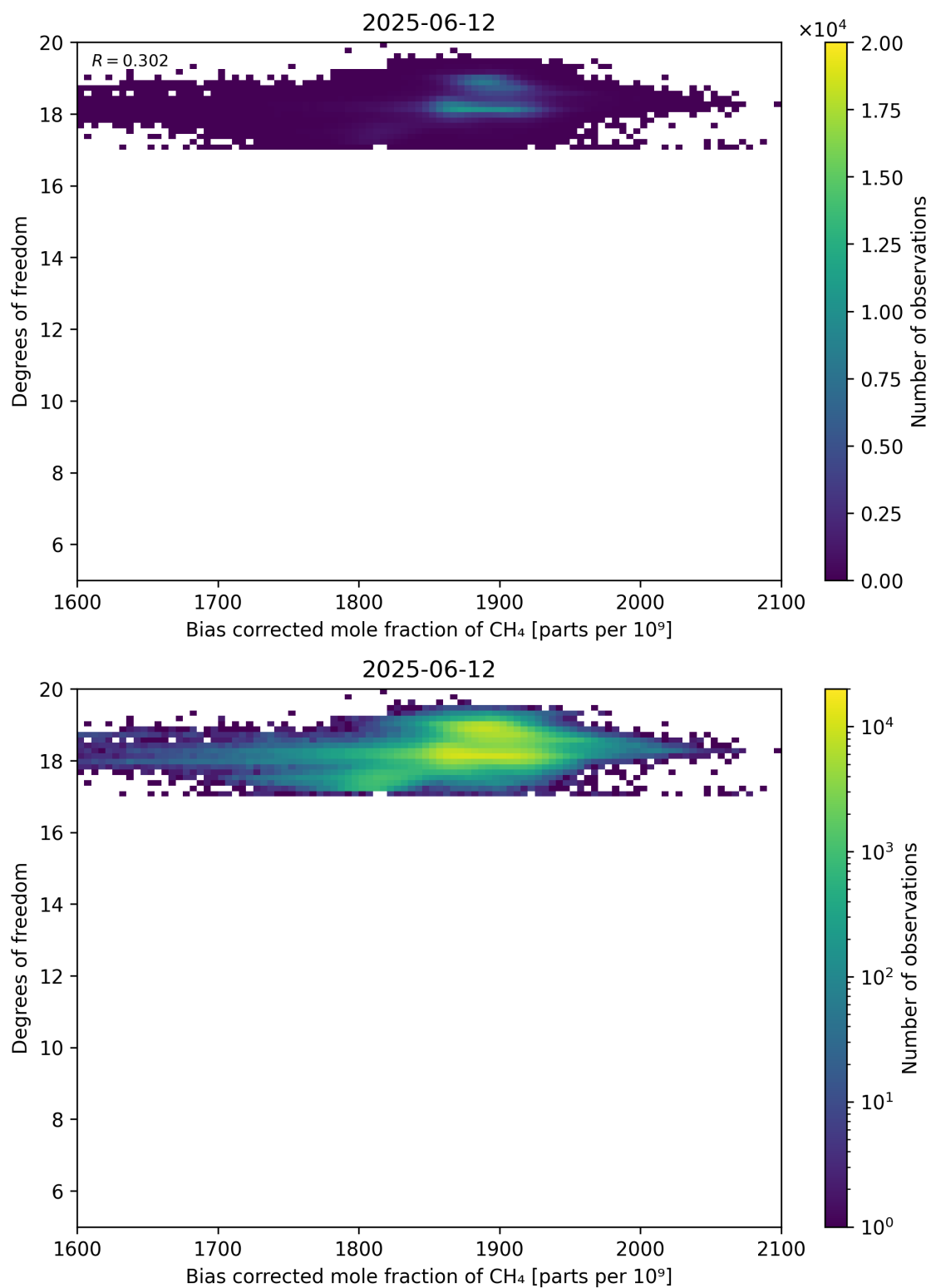
Figure 65: Scatter density plot of “Bias corrected mole fraction of CH 4 ” against “Degrees of freedom” for 2025-06-11 to 2025-06-13.
