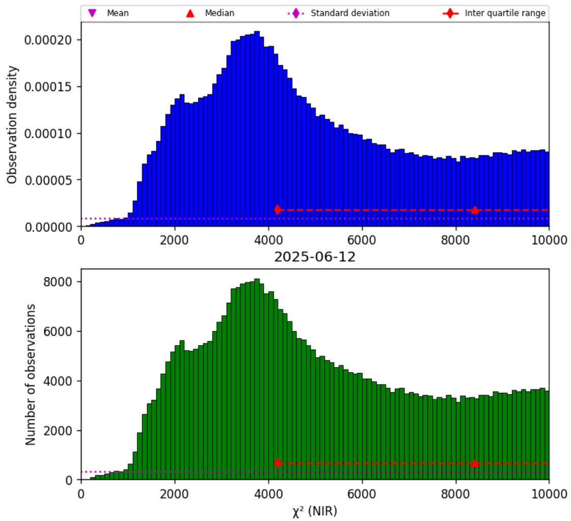
Figure 29: Histogram of " \chi^2 (NIR)" for 2025-06-11 to 2025-06-13
