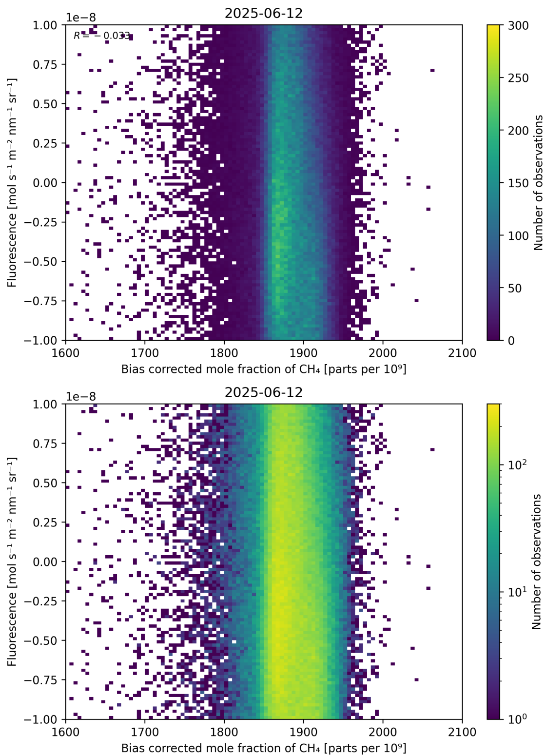
Figure 66: Scatter density plot of “Bias corrected mole fraction of \text{CH}_4 ” against “Fluorescence” for 2025-06-11 to 2025-06-13.
