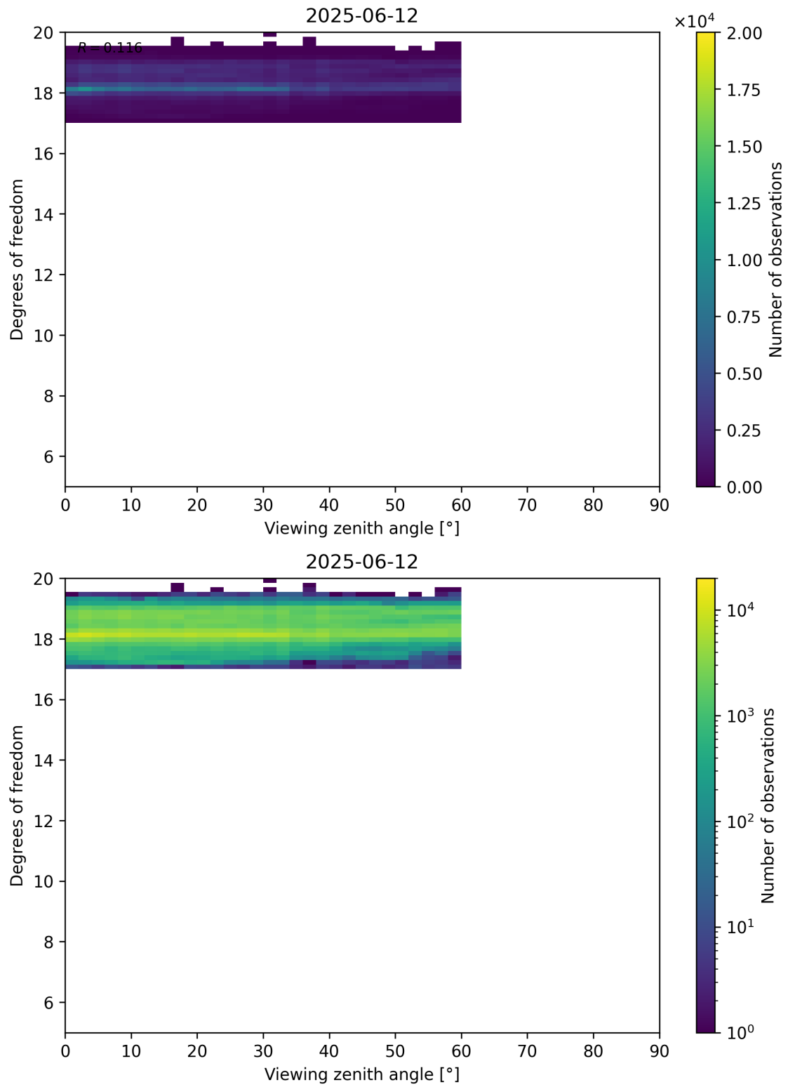
Figure 107: Scatter density plot of “Viewing zenith angle” against “Degrees of freedom” for 2025-06-11 to 2025-06-13.
