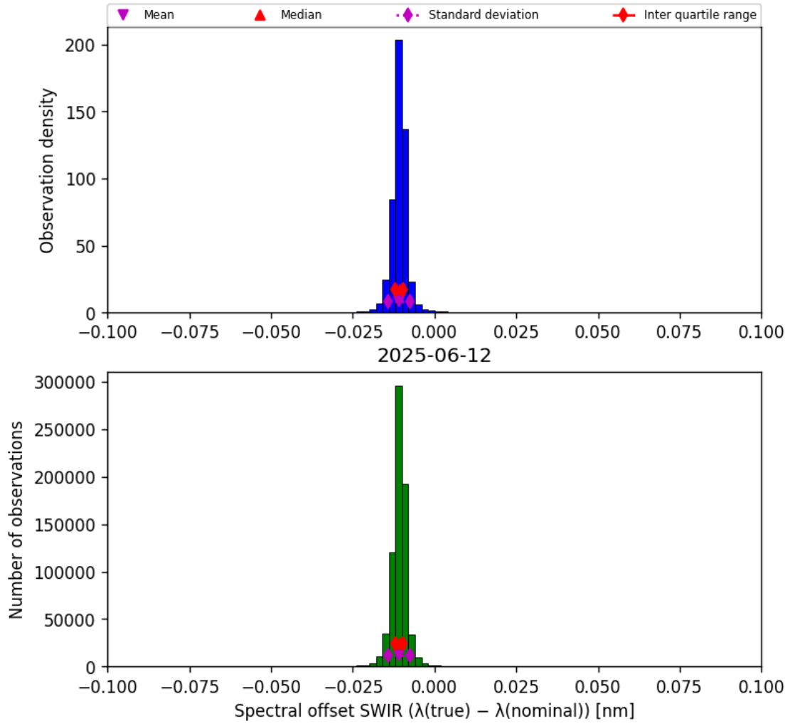
Figure 27: Histogram of “Spectral offset SWIR ( \lambda_{\text{true}} - \lambda_{\text{nominal}} )” for 2025-06-11 to 2025-06-13
