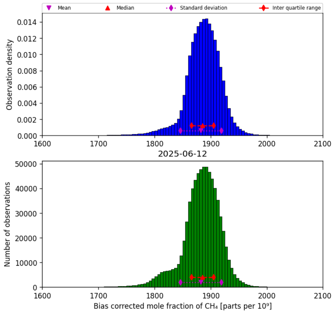
Figure 25: Histogram of “Bias corrected mole fraction of CH 4 ” for 2025-06-11 to 2025-06-13
