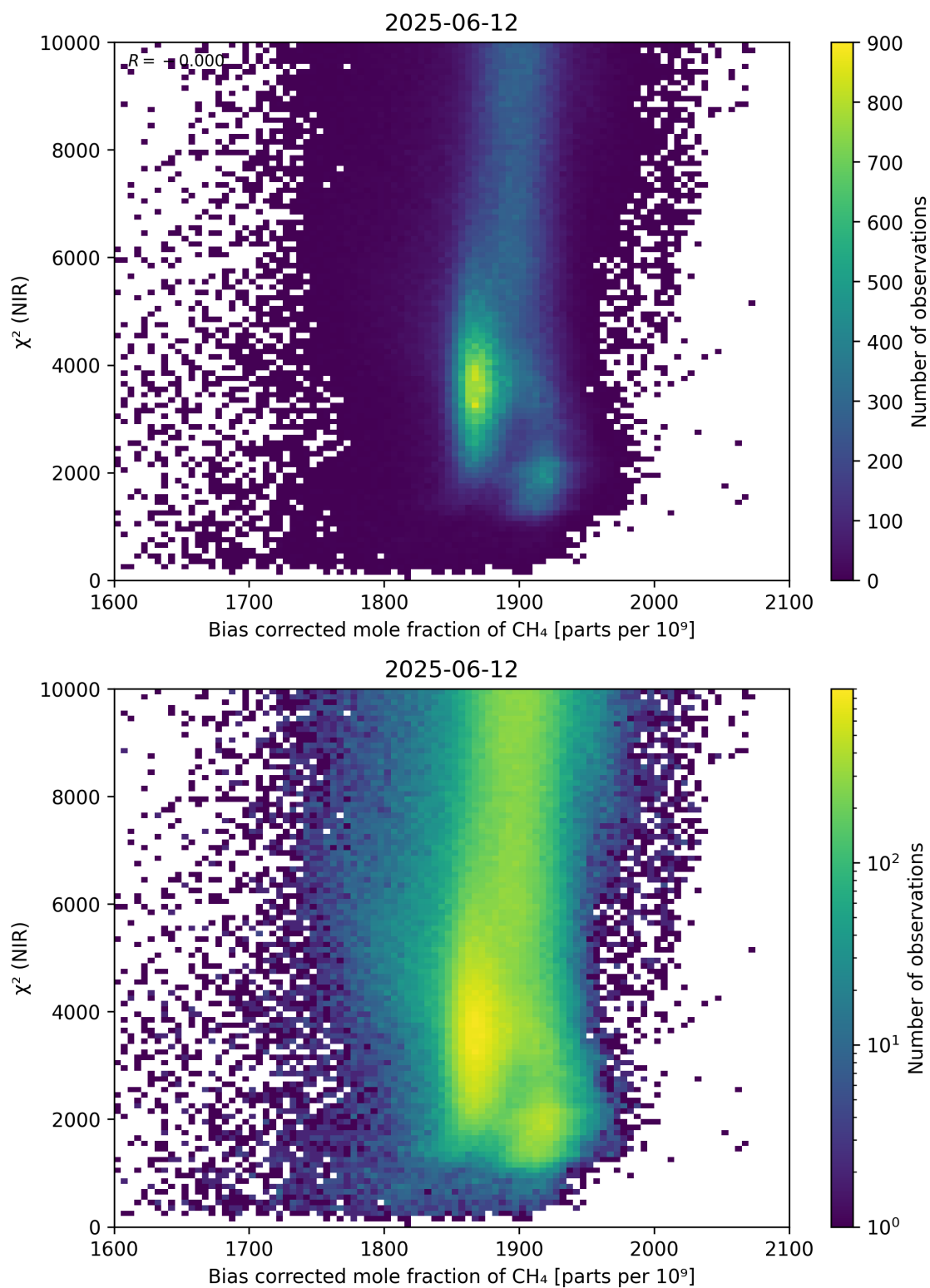
Figure 63: Scatter density plot of “Bias corrected mole fraction of \text{CH}_4 ” against “ \chi^2 (NIR)” for 2025-06-11 to 2025-06-13.
