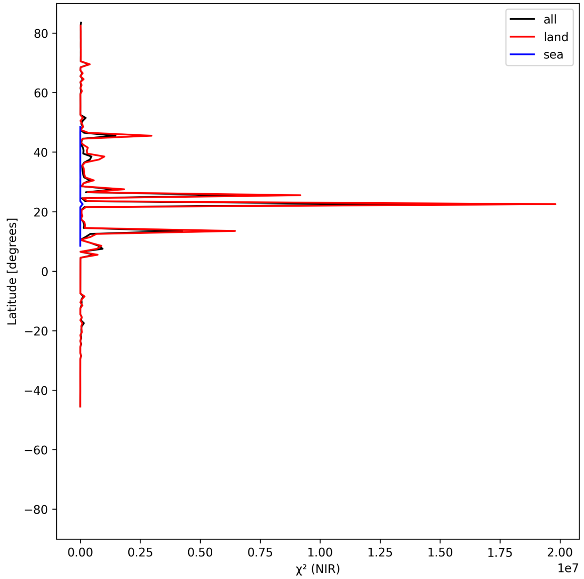
Figure 18: Zonal average of “ \chi^2 (NIR)” for 2025-06-11 to 2025-06-13.
