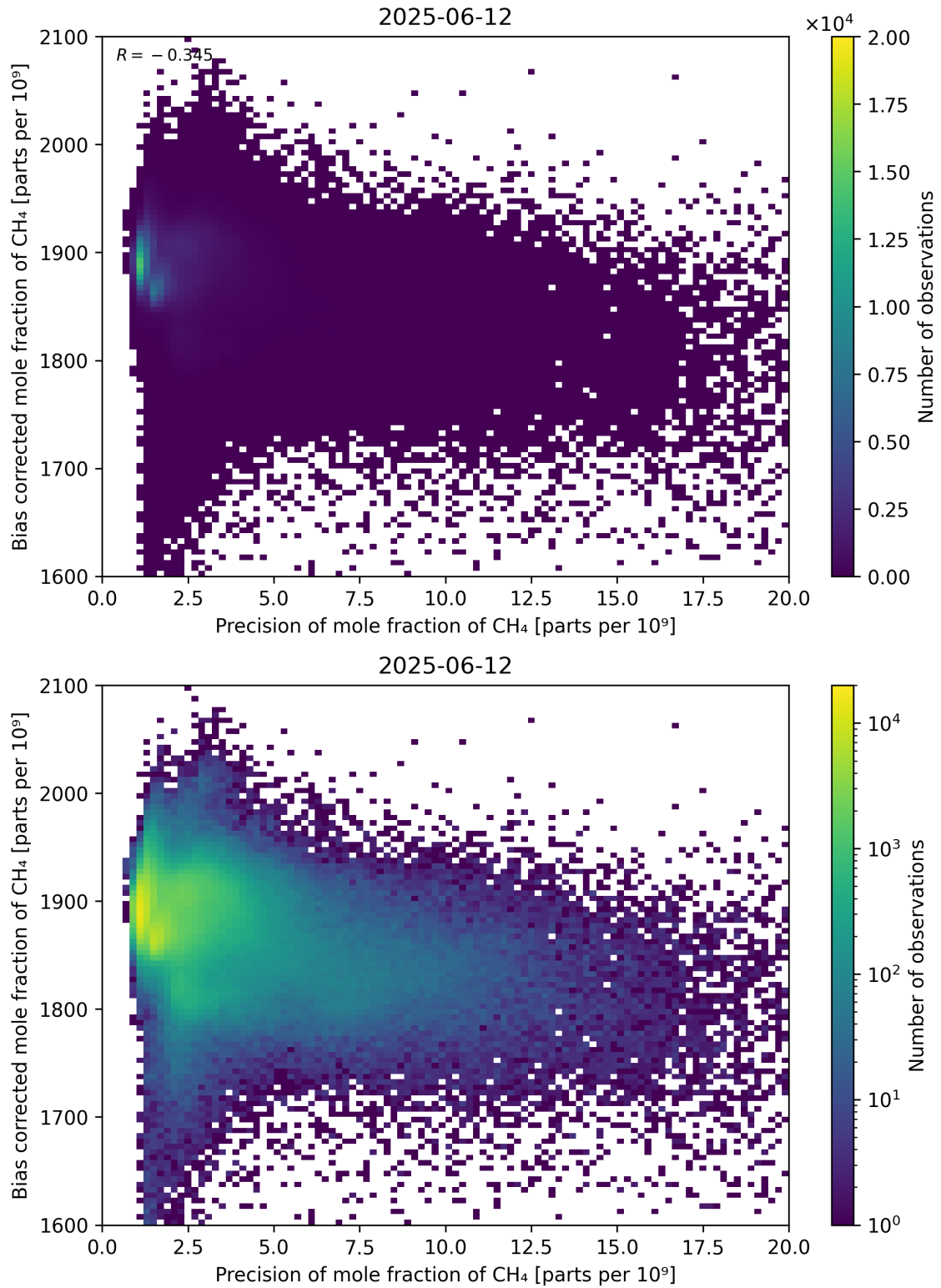
Figure 82: Scatter density plot of “Precision of mole fraction of CH 4 ” against “Bias corrected mole fraction of CH 4 ” for 2025-06-11 to 2025-06-13.
