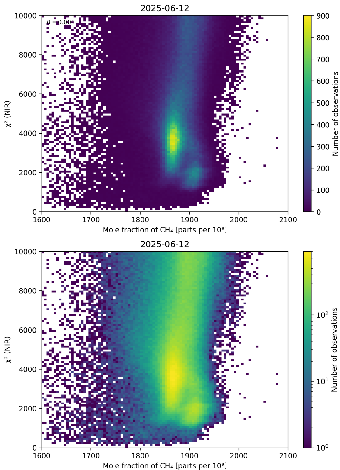
Figure 70: Scatter density plot of “Mole fraction of \text{CH}_4 ” against “ \chi^2 (NIR)” for 2025-06-11 to 2025-06-13.
