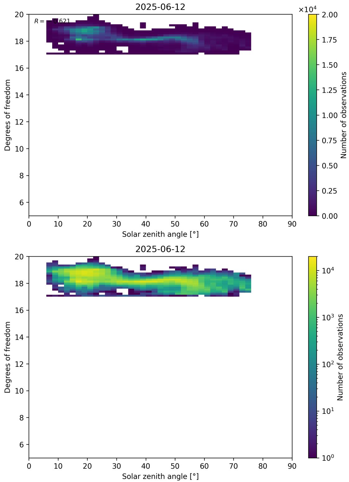
Figure 96: Scatter density plot of “Solar zenith angle” against “Degrees of freedom” for 2025-06-11 to 2025-06-13.
