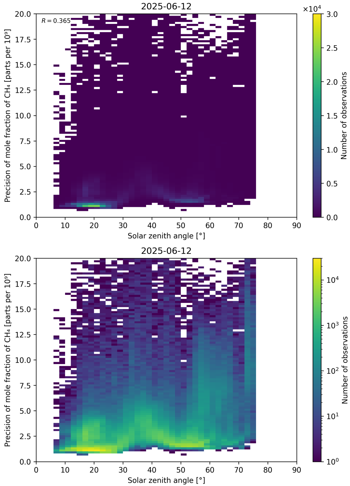
Figure 101: Scatter density plot of “Solar zenith angle” against “Precision of mole fraction of CH 4 ” for 2025-06-11 to 2025-06-13.
