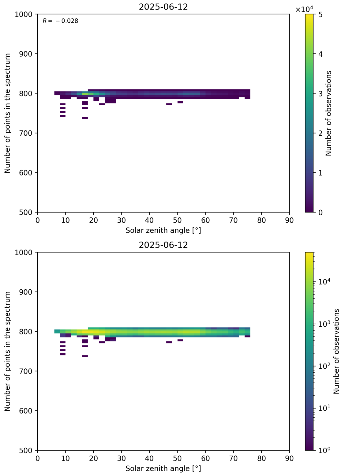
Figure 103: Scatter density plot of “Solar zenith angle” against “Number of points in the spectrum” for 2025-06-11 to 2025-06-13.
