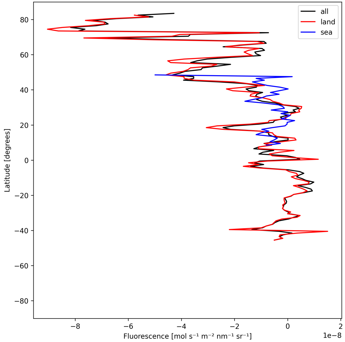
Figure 21: Zonal average of “Fluorescence” for 2025-06-11 to 2025-06-13.
