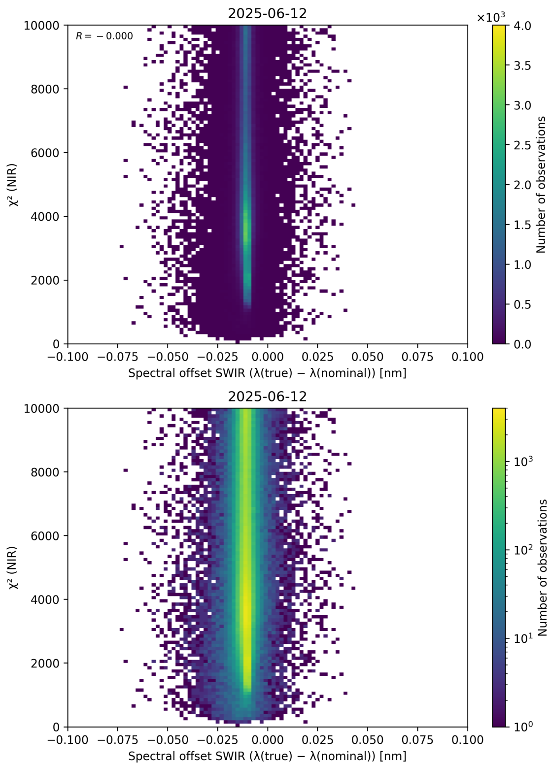
Figure 117: Scatter density plot of “Spectral offset SWIR ( \lambda_{\text{true}} - \lambda_{\text{nominal}} )” against “ \chi^2 (NIR)” for 2025-06-11 to 2025-06-13.
