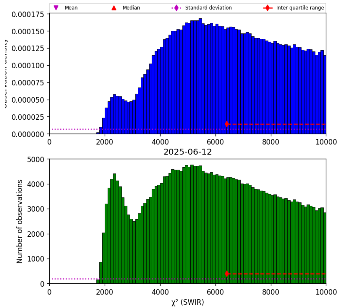
Figure 28: Histogram of “ \chi^2 (SWIR)” for 2025-06-11 to 2025-06-13
