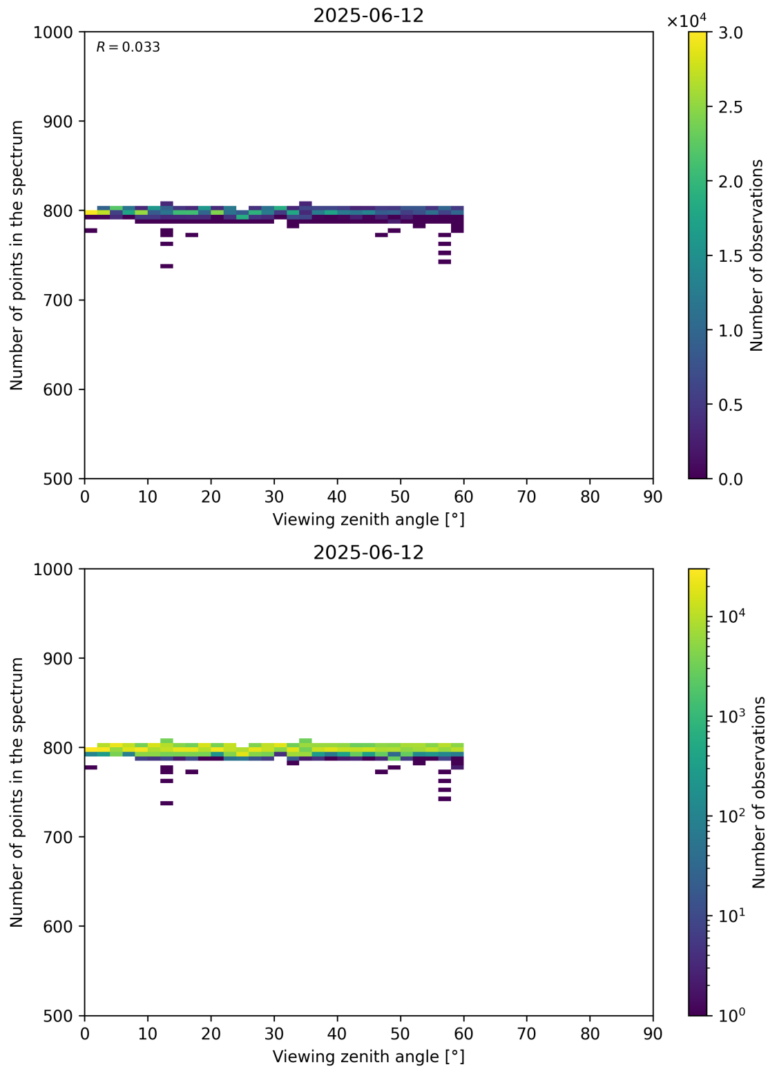
Figure 114: Scatter density plot of “Viewing zenith angle” against “Number of points in the spectrum” for 2025-06-11 to 2025-06-13.
