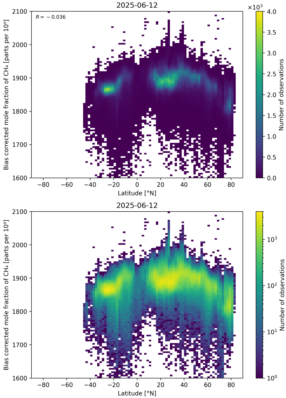
Figure 58: Scatter density plot of “Latitude” against “Bias corrected mole fraction of CH 4 ” for 2025-06-11 to 2025-06-13.
