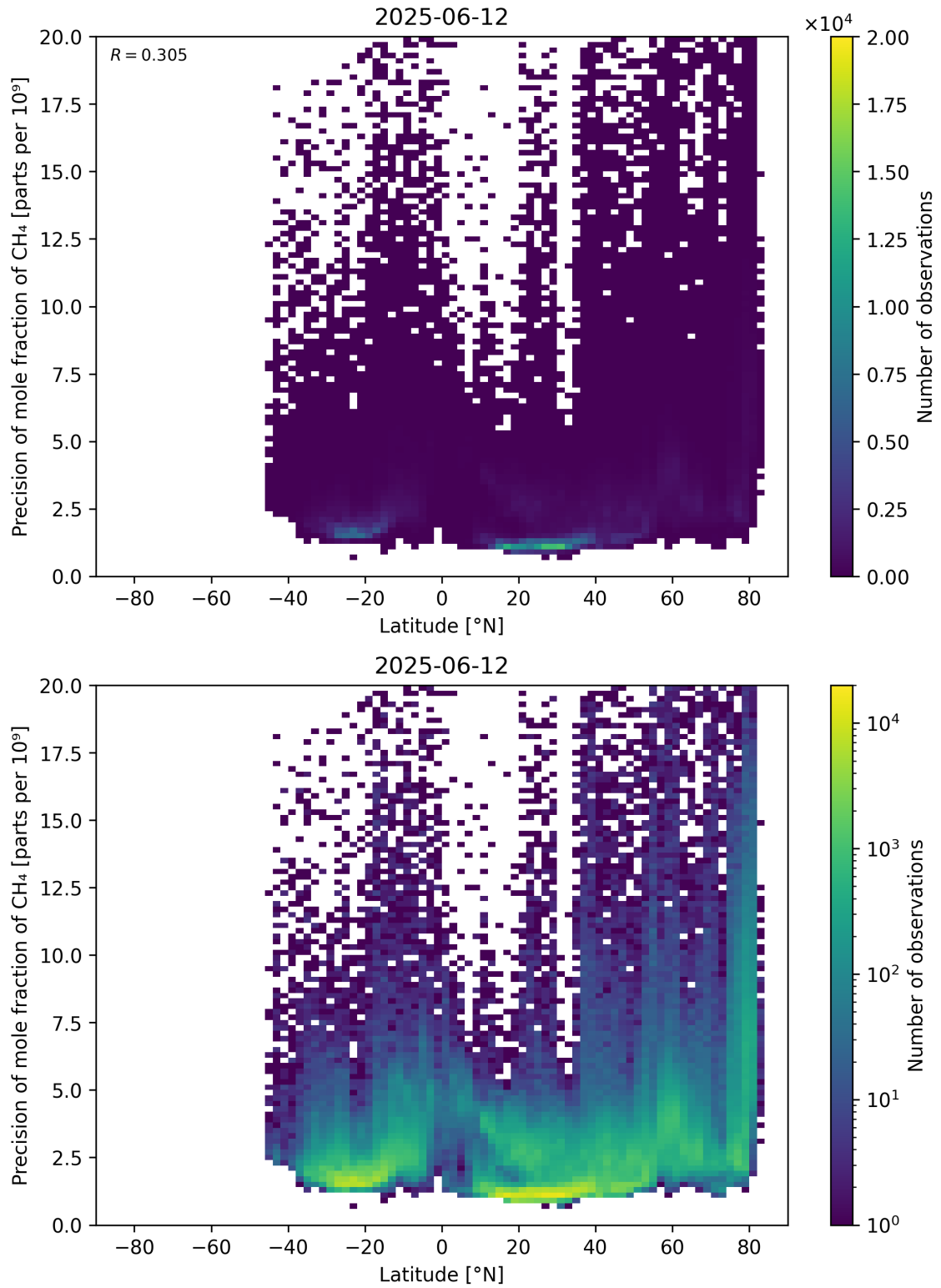
Figure 59: Scatter density plot of “Latitude” against “Precision of mole fraction of \text{CH}_4 ” for 2025-06-11 to 2025-06-13.
