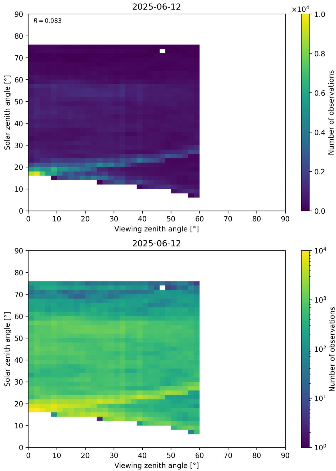
Figure 115: Scatter density plot of “Viewing zenith angle” against “Solar zenith angle” for 2025-06-11 to 2025-06-13.
