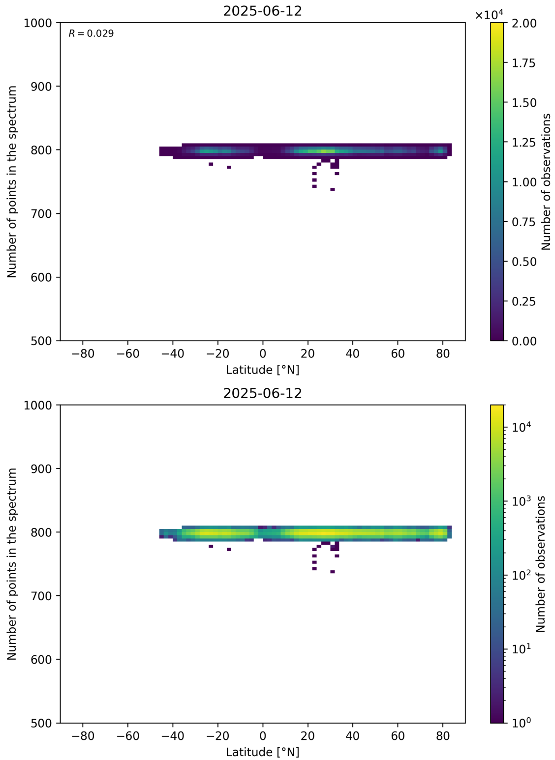
Figure 61: Scatter density plot of “Latitude” against “Number of points in the spectrum” for 2025-06-11 to 2025-06-13.
