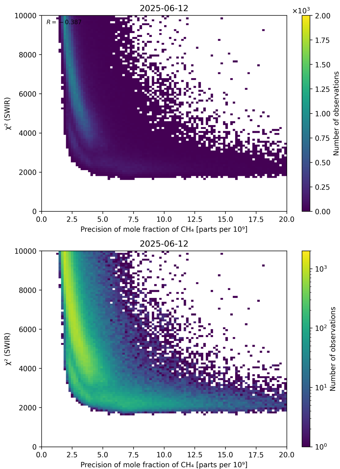
Figure 79: Scatter density plot of “Precision of mole fraction of \text{CH}_4 ” against “ \chi^2 (SWIR)” for 2025-06-11 to 2025-06-13.
