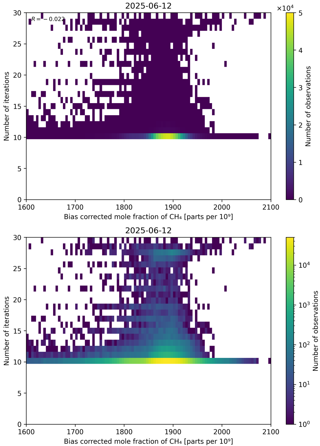
Figure 67: Scatter density plot of “Bias corrected mole fraction of CH 4 ” against “Number of iterations” for 2025-06-11 to 2025-06-13.
