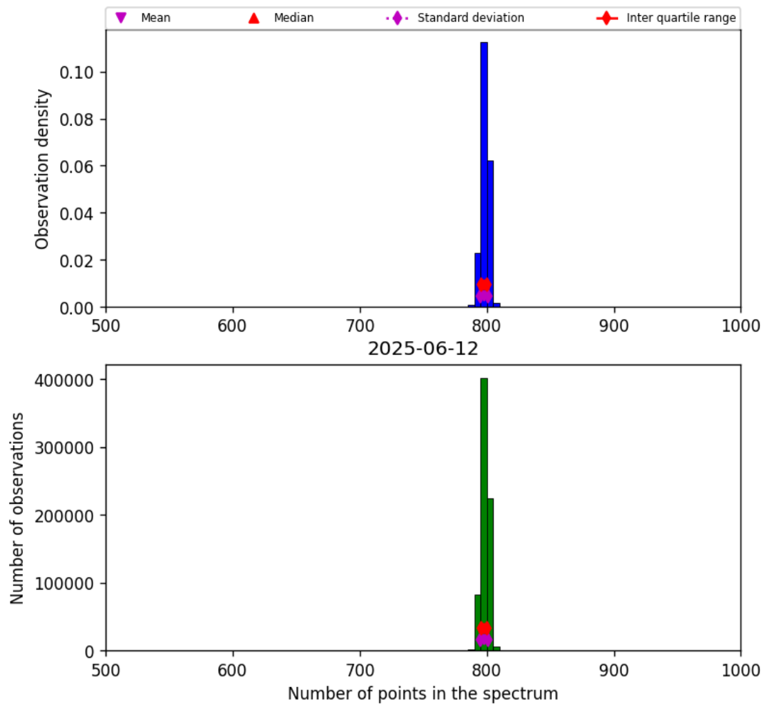
Figure 26: Histogram of “Number of points in the spectrum” for 2025-06-11 to 2025-06-13
