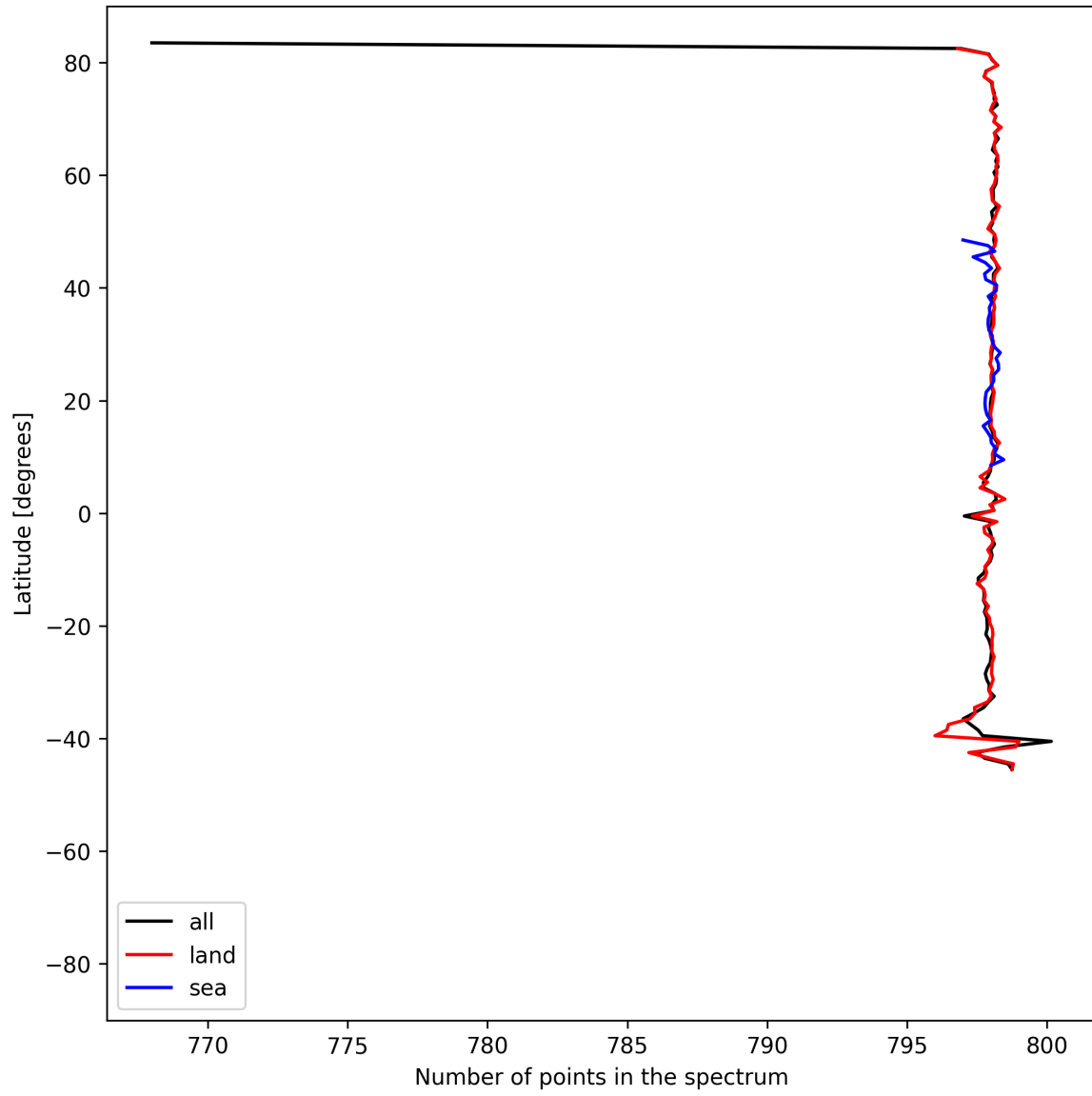
Figure 15: Zonal average of “Number of points in the spectrum” for 2025-06-11 to 2025-06-13.
