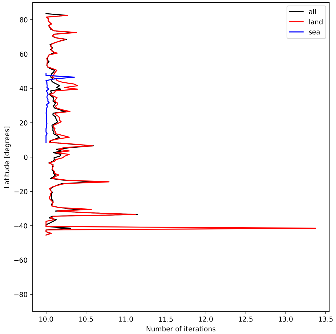
Figure 20: Zonal average of “Number of iterations” for 2025-06-11 to 2025-06-13.
