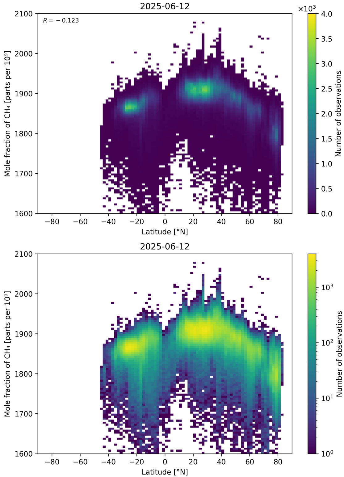
Figure 57: Scatter density plot of “Latitude” against “Mole fraction of CH 4 ” for 2025-06-11 to 2025-06-13.
