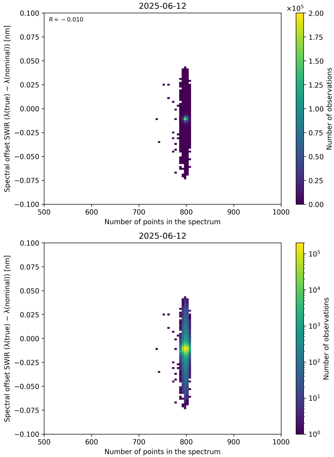
Figure 93: Scatter density plot of “Number of points in the spectrum” against “Spectral offset SWIR ( \lambda_{\text{true}} - \lambda_{\text{nominal}} )” for 2025-06-11 to 2025-06-13.
