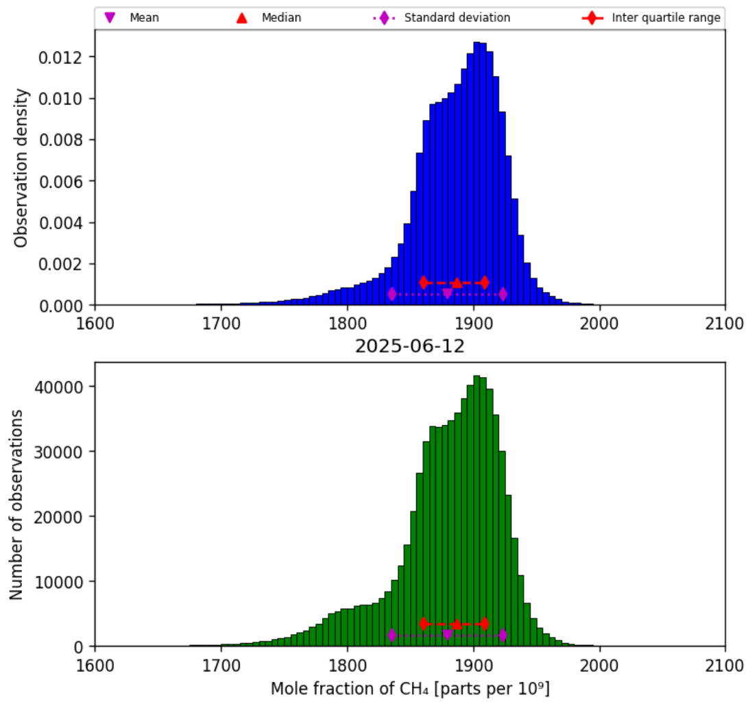
Figure 23: Histogram of “Mole fraction of CH 4 ” for 2025-06-11 to 2025-06-13
