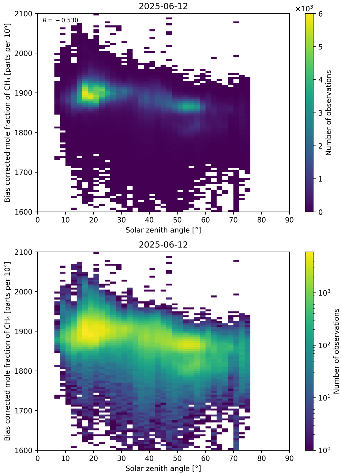
Figure 100: Scatter density plot of “Solar zenith angle” against “Bias corrected mole fraction of CH 4 ” for 2025-06-11 to 2025-06-13.
