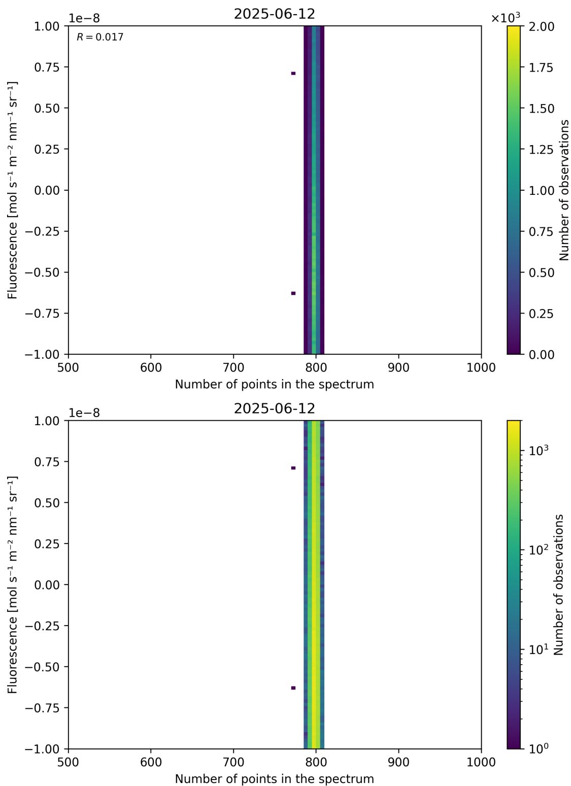
Figure 91: Scatter density plot of “Number of points in the spectrum” against “Fluorescence” for 2025-06-11 to 2025-06-13.
