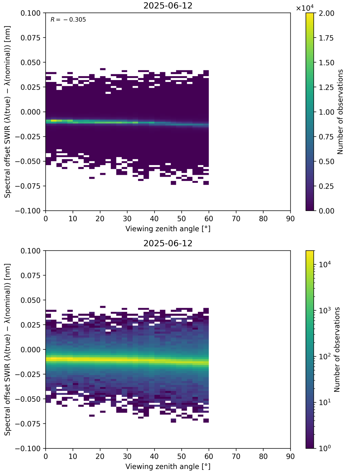
Figure 116: Scatter density plot of “Viewing zenith angle” against “Spectral offset SWIR ( \lambda_{\text{true}} - \lambda_{\text{nominal}} )” for 2025-06-11 to 2025-06-13.
