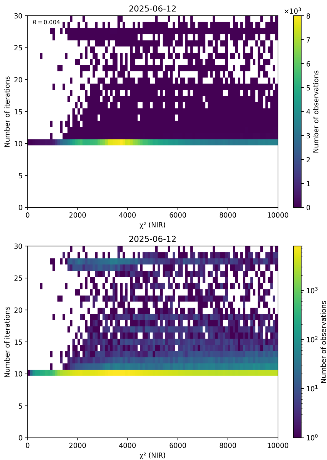
Figure 46: Scatter density plot of “ \chi^2 (NIR)” against “Number of iterations” for 2025-06-11 to 2025-06-13.
