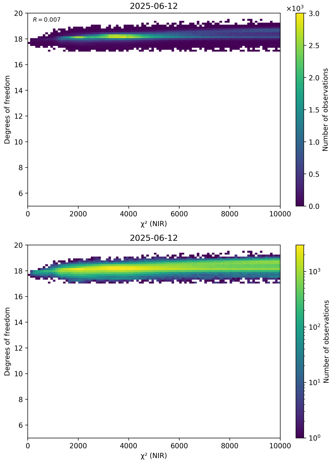
Figure 44: Scatter density plot of “ \chi^2 (NIR)” against “Degrees of freedom” for 2025-06-11 to 2025-06-13.
