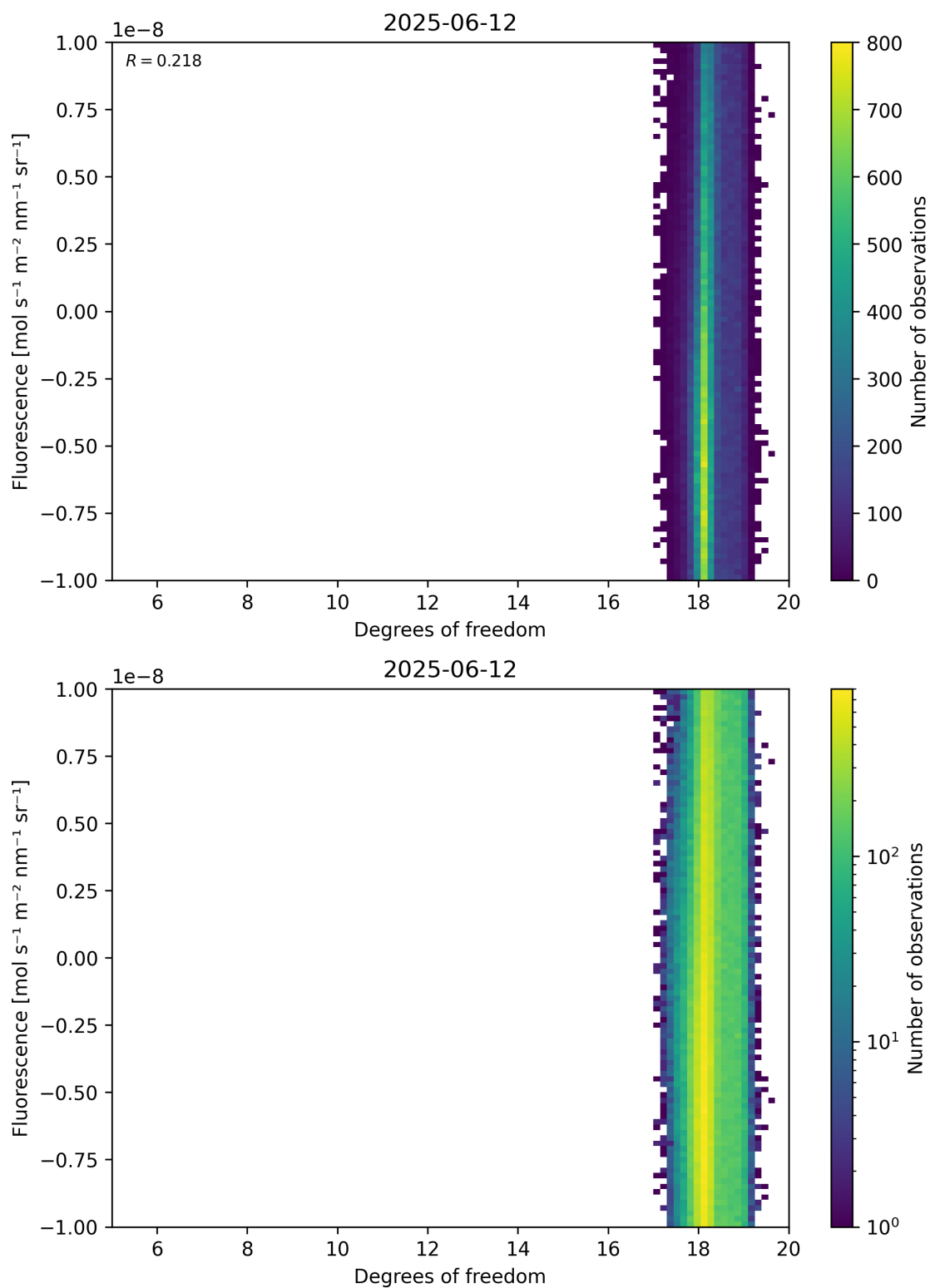
Figure 51: Scatter density plot of “Degrees of freedom” against “Fluorescence” for 2025-06-11 to 2025-06-13.
