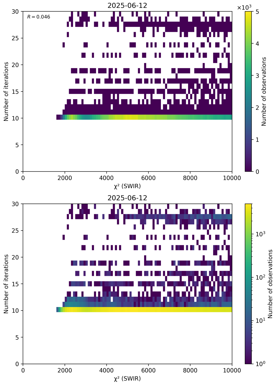
Figure 50: Scatter density plot of “ \chi^2 (SWIR)” against “Number of iterations” for 2025-06-11 to 2025-06-13.
