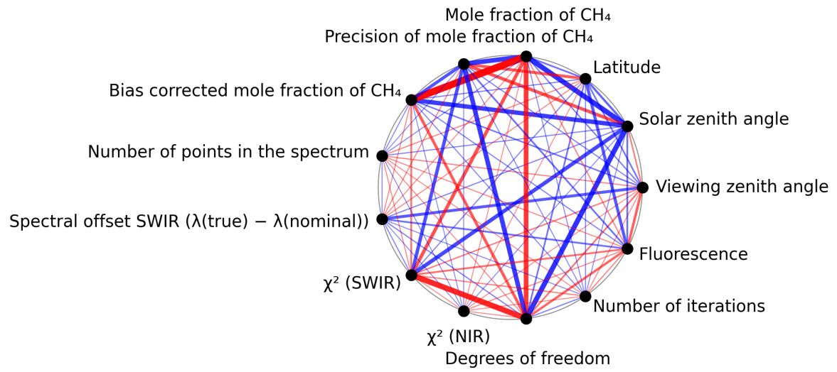
Figure 1: Map of correlation graph for 2025-06-11 to 2025-06-13.
