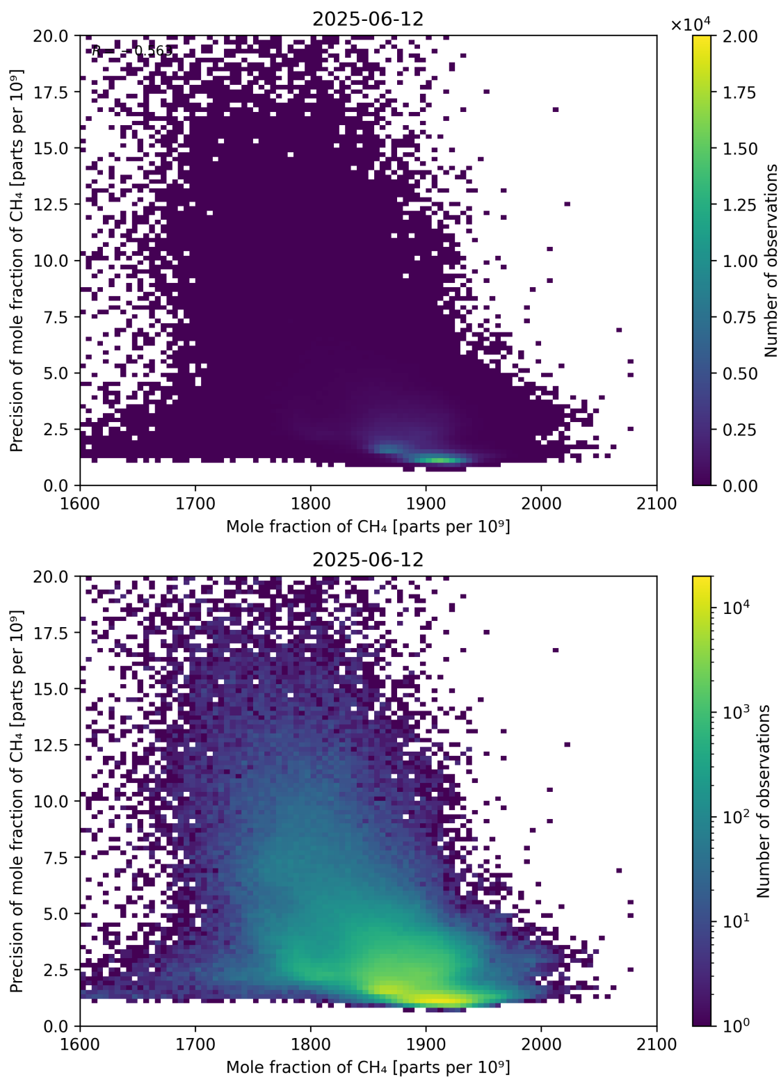
Figure 75: Scatter density plot of “Mole fraction of CH 4 ” against “Precision of mole fraction of CH 4 ” for 2025-06-11 to 2025-06-13.
