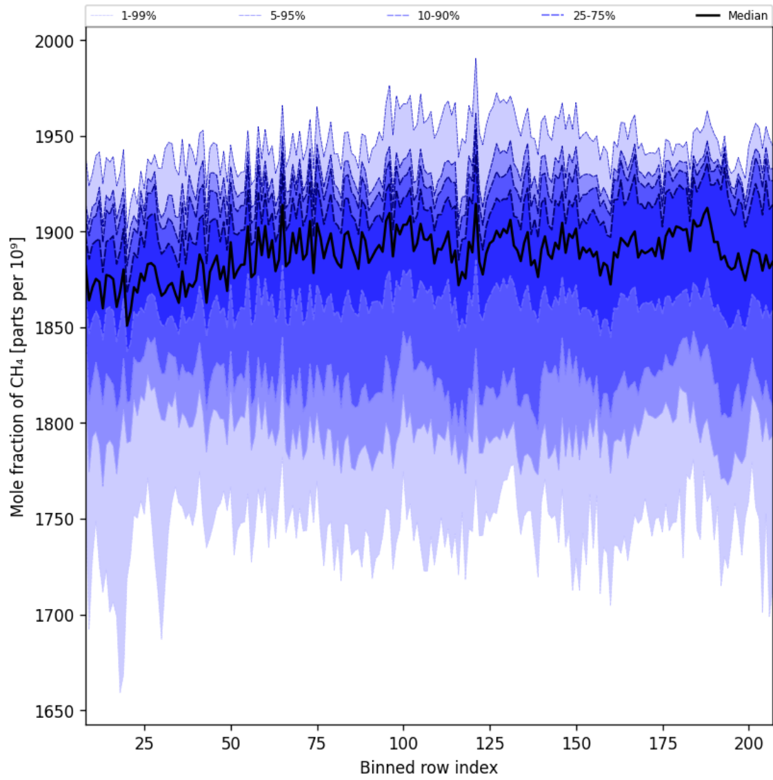
Figure 34: Along track statistics of “Mole fraction of CH 4 ” for 2025-06-11 to 2025-06-13
