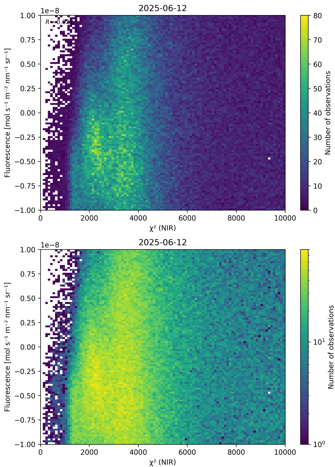
Figure 45: Scatter density plot of “ \chi^2 (NIR)” against “Fluorescence” for 2025-06-11 to 2025-06-13.
