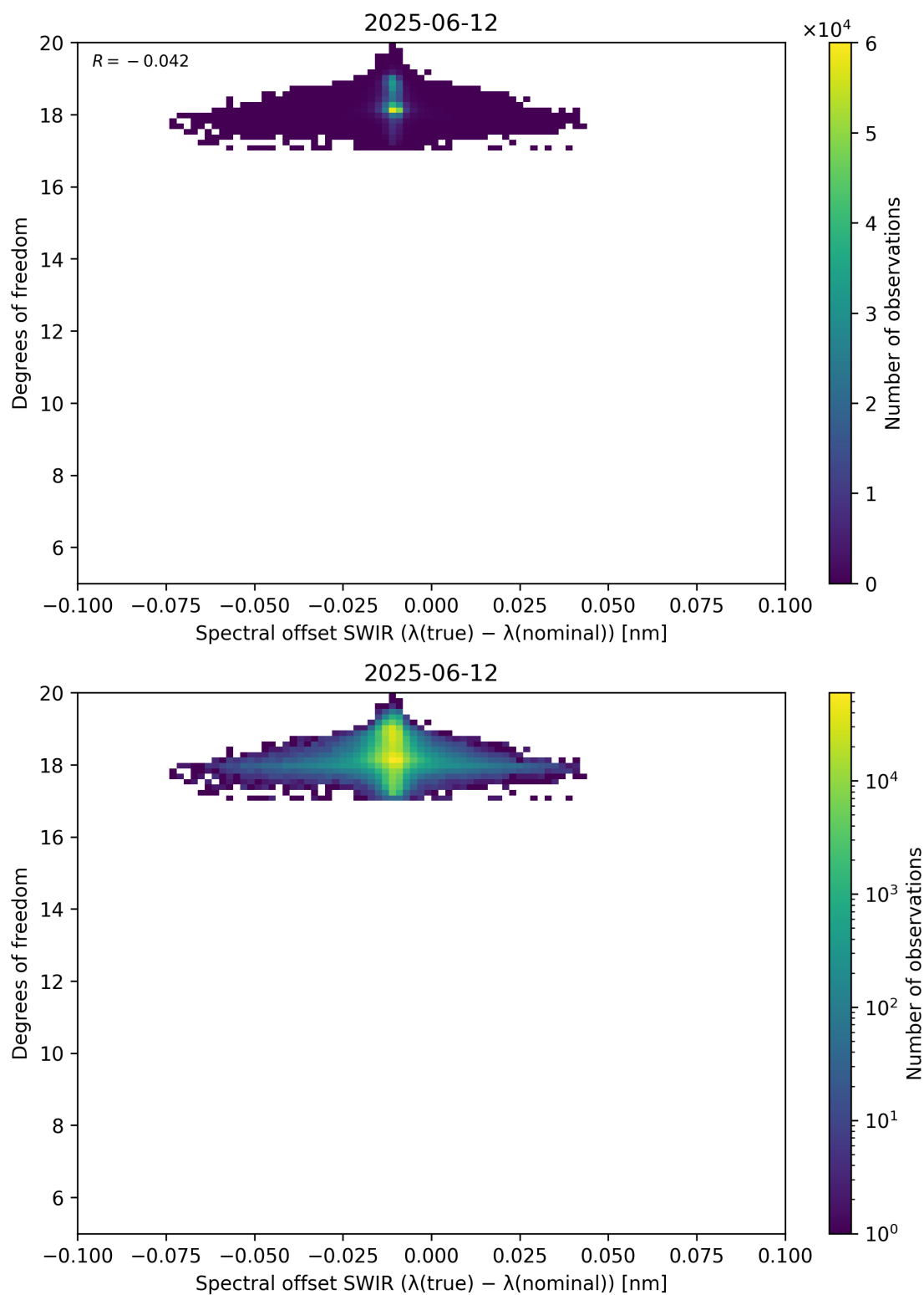
Figure 119: Scatter density plot of “Spectral offset SWIR ( \lambda_{\text{true}} - \lambda_{\text{nominal}} )” against “Degrees of freedom” for 2025-06-11 to 2025-06-13.
