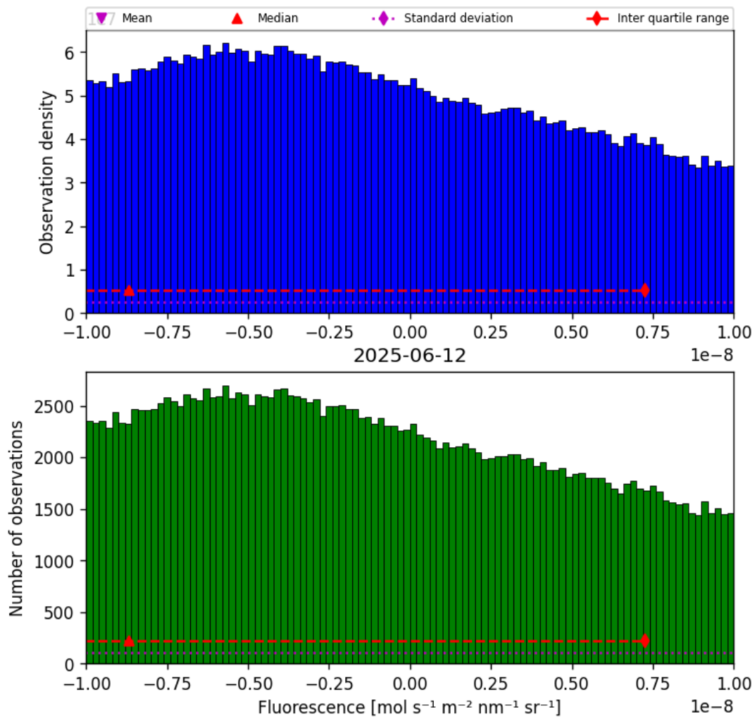
Figure 32: Histogram of “Fluorescence” for 2025-06-11 to 2025-06-13
