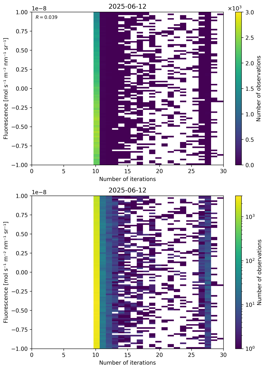
Figure 87: Scatter density plot of “Number of iterations” against “Fluorescence” for 2025-06-11 to 2025-06-13.
