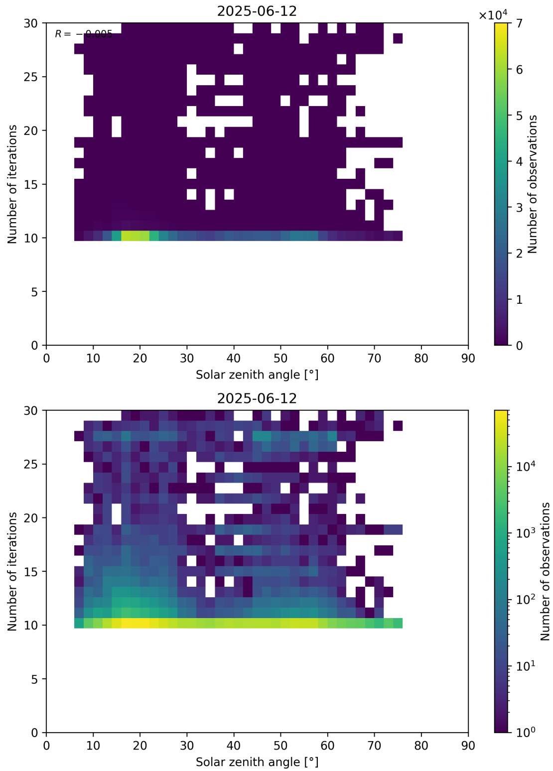
Figure 102: Scatter density plot of “Solar zenith angle” against “Number of iterations” for 2025-06-11 to 2025-06-13.
