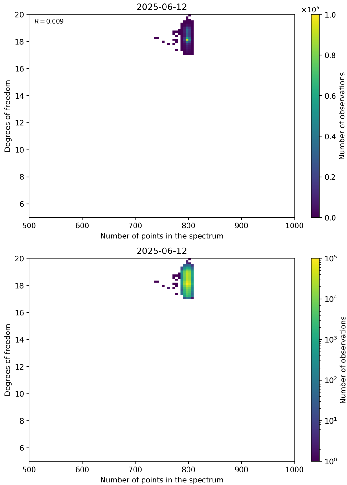
Figure 90: Scatter density plot of “Number of points in the spectrum” against “Degrees of freedom” for 2025-06-11 to 2025-06-13.
