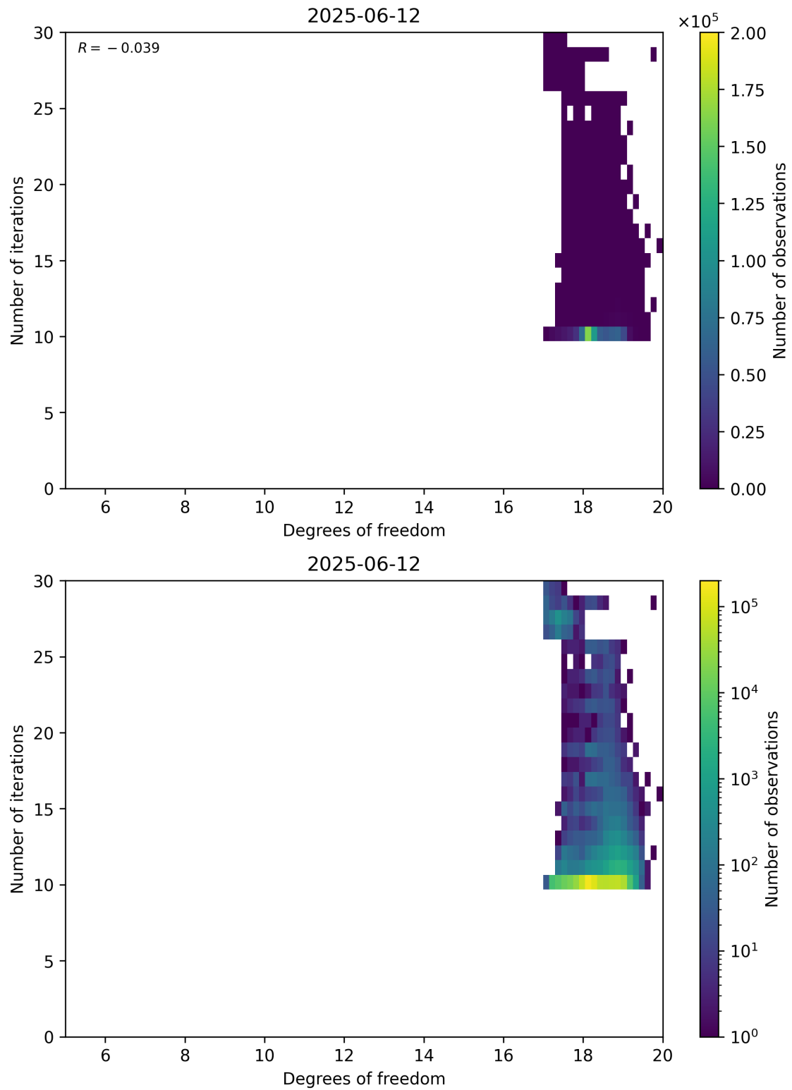
Figure 52: Scatter density plot of “Degrees of freedom” against “Number of iterations” for 2025-06-11 to 2025-06-13.
