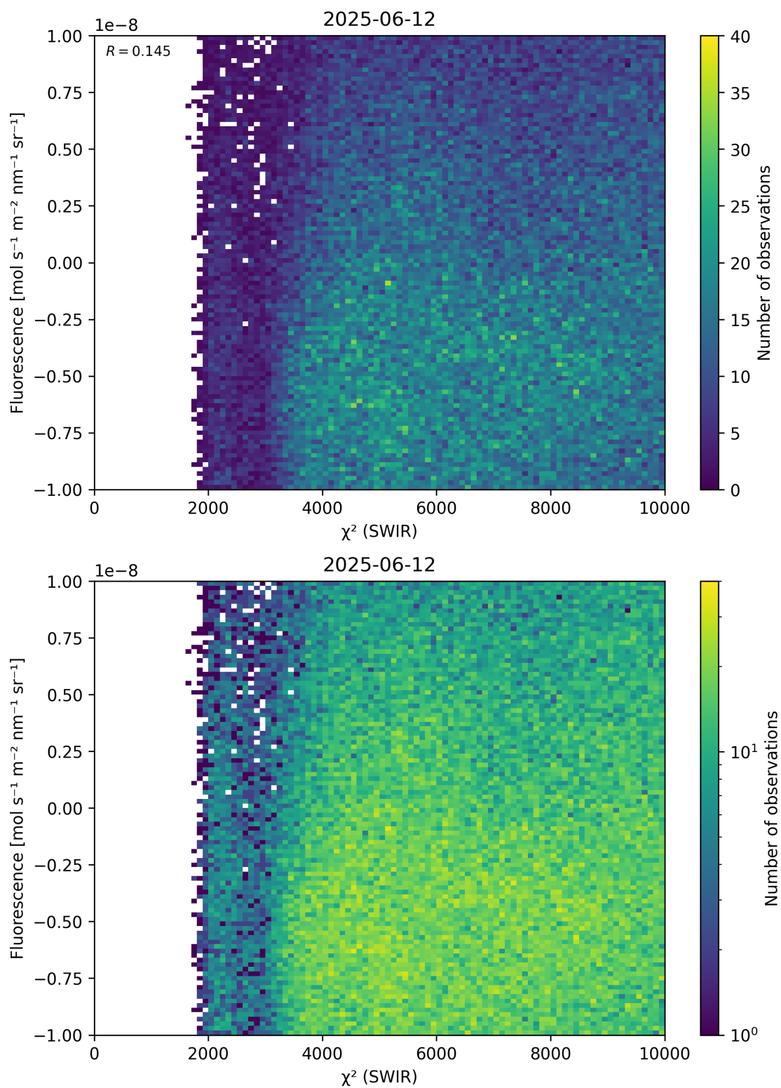
Figure 49: Scatter density plot of “ \chi^2 (SWIR)” against “Fluorescence” for 2025-06-11 to 2025-06-13.
