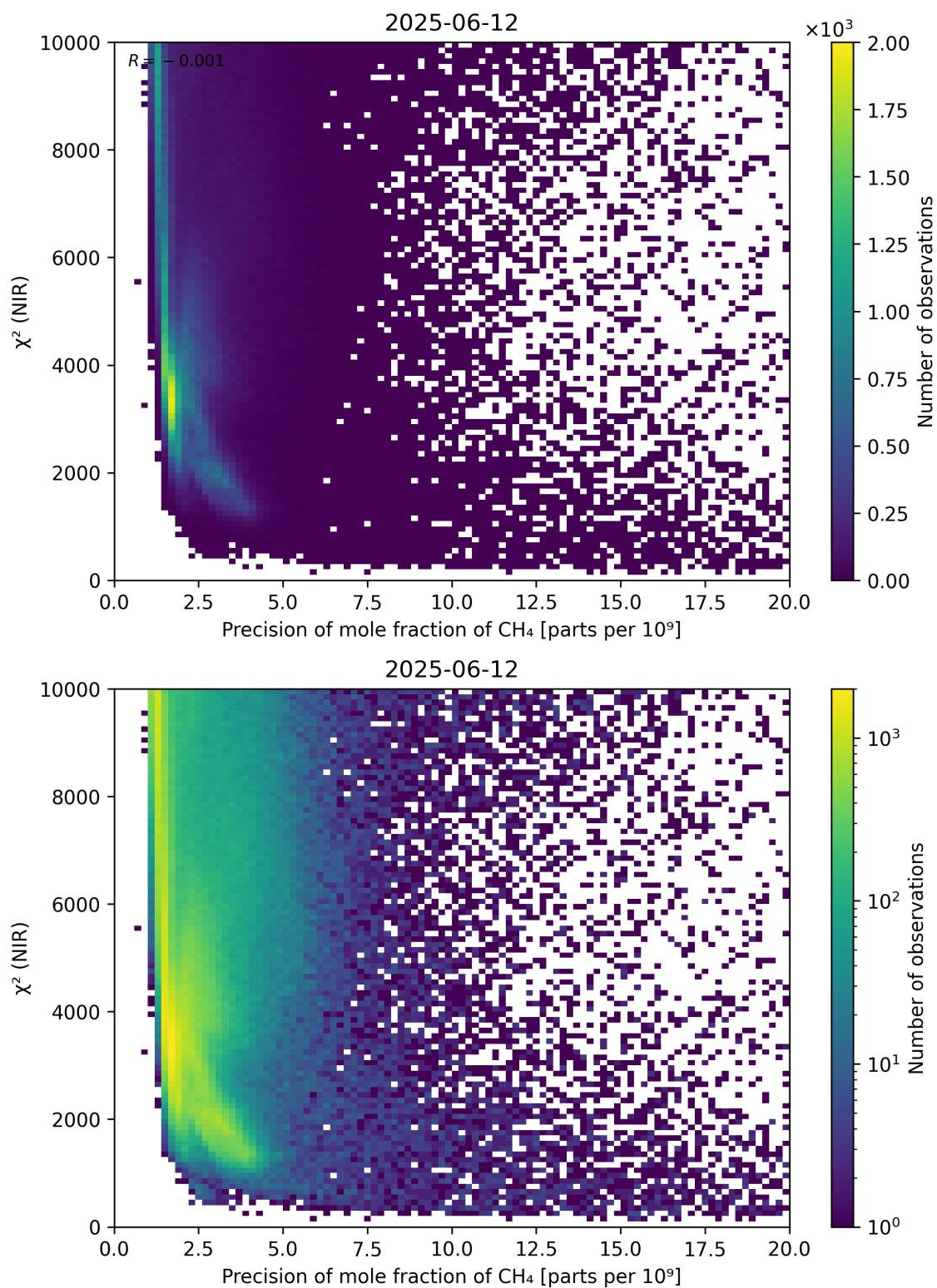
Figure 78: Scatter density plot of “Precision of mole fraction of \text{CH}_4 ” against “ \chi^2 (NIR)” for 2025-06-11 to 2025-06-13.
