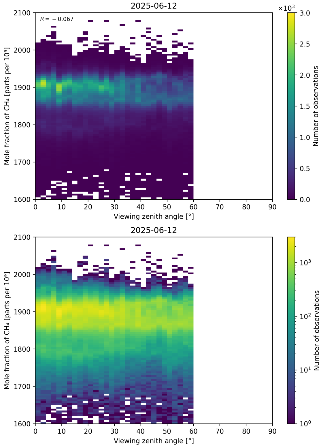
Figure 110: Scatter density plot of “Viewing zenith angle” against “Mole fraction of CH 4 ” for 2025-06-11 to 2025-06-13.
