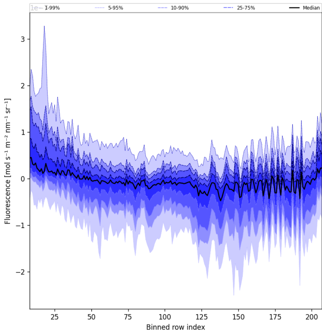
Figure 43: Along track statistics of “Fluorescence” for 2025-06-11 to 2025-06-13
