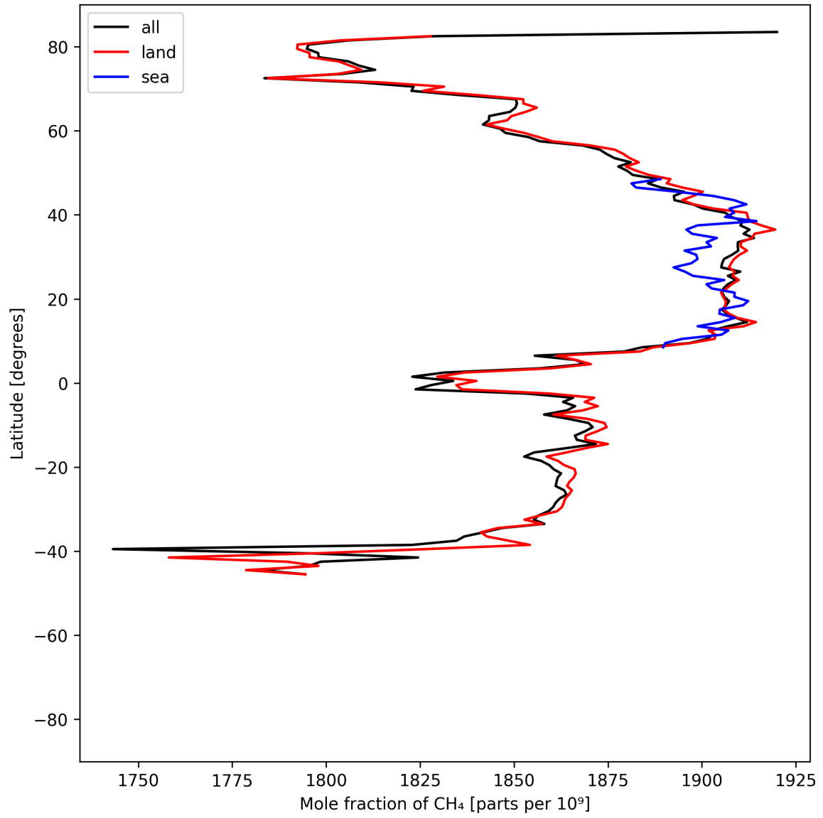
Figure 12: Zonal average of “Mole fraction of CH 4 ” for 2025-06-11 to 2025-06-13.
