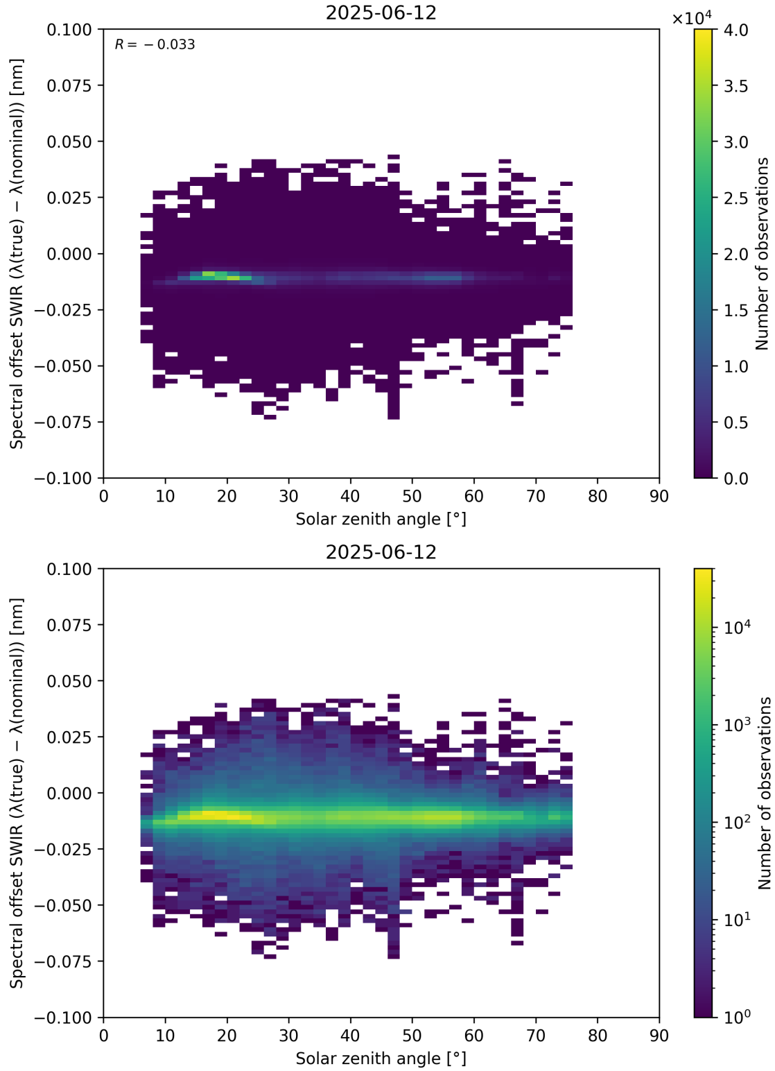
Figure 104: Scatter density plot of “Solar zenith angle” against “Spectral offset SWIR ( \lambda_{\text{true}} - \lambda_{\text{nominal}} )” for 2025-06-11 to 2025-06-13.
