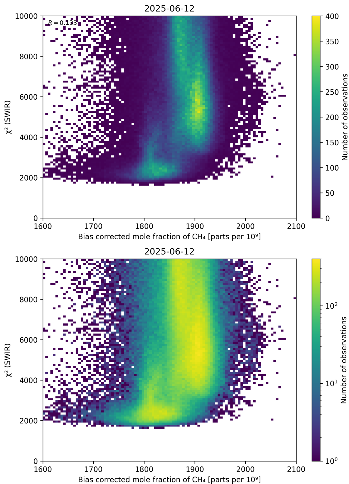
Figure 64: Scatter density plot of “Bias corrected mole fraction of \text{CH}_4 ” against “ \chi^2 (SWIR)” for 2025-06-11 to 2025-06-13.
