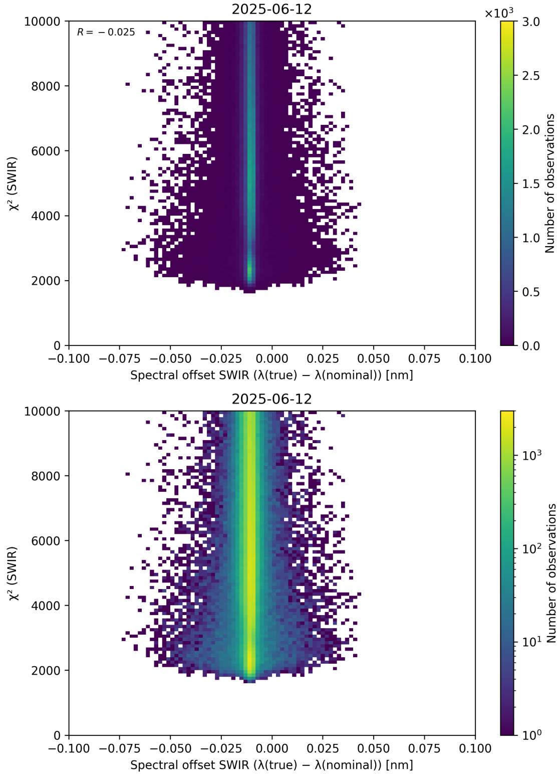
Figure 118: Scatter density plot of “Spectral offset SWIR ( \lambda_{\text{true}} - \lambda_{\text{nominal}} )” against “ \chi^2 (SWIR)” for 2025-06-11 to 2025-06-13.
