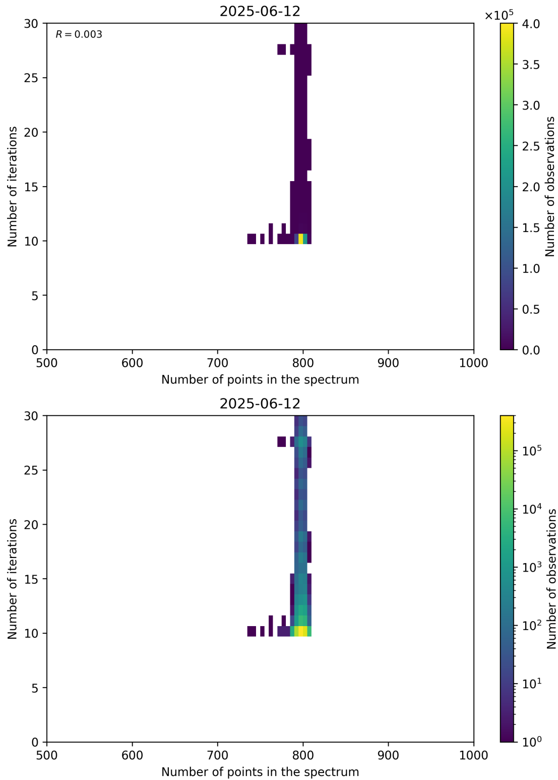
Figure 92: Scatter density plot of “Number of points in the spectrum” against “Number of iterations” for 2025-06-11 to 2025-06-13.
