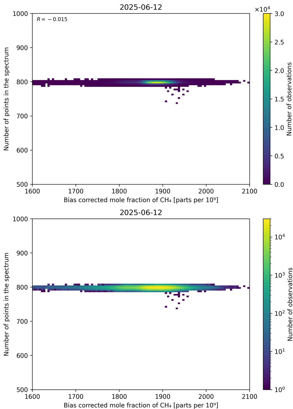
Figure 68: Scatter density plot of “Bias corrected mole fraction of CH 4 ” against “Number of points in the spectrum” for 2025-06-11 to 2025-06-13.
