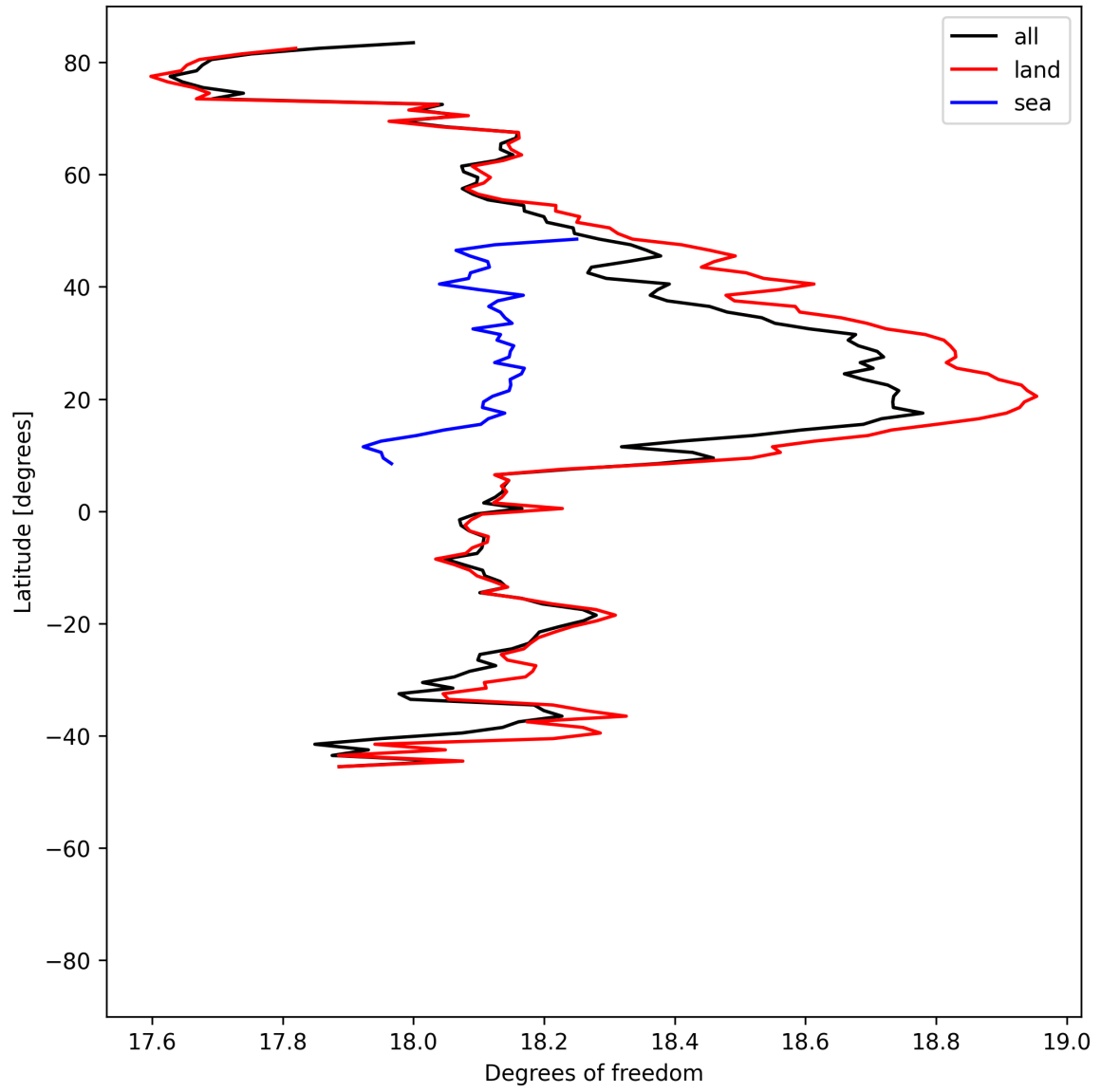
Figure 19: Zonal average of “Degrees of freedom” for 2025-06-11 to 2025-06-13.
