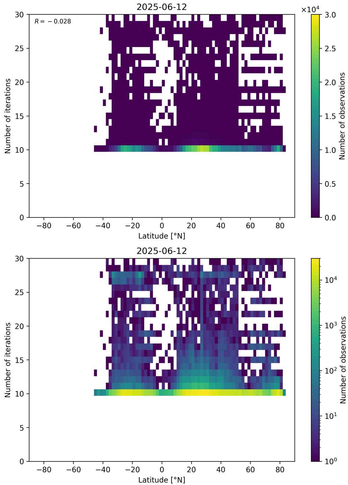
Figure 60: Scatter density plot of “Latitude” against “Number of iterations” for 2025-06-11 to 2025-06-13.
