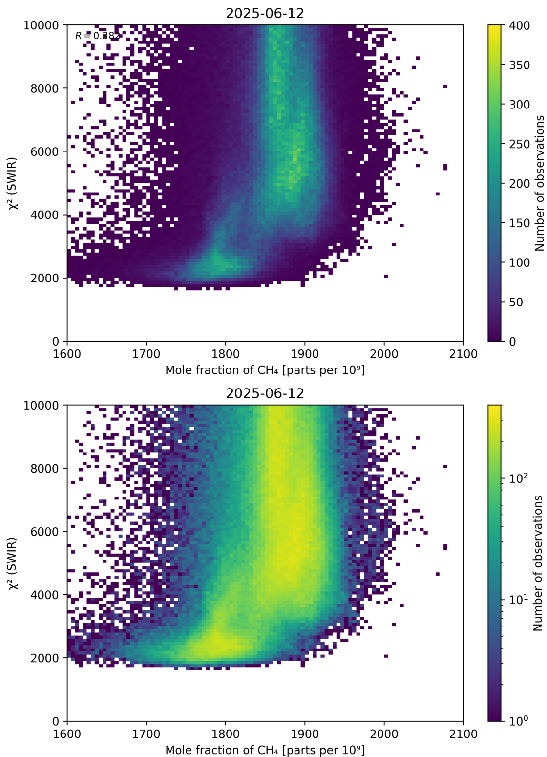
Figure 71: Scatter density plot of “Mole fraction of \text{CH}_4 ” against “ \chi^2 (SWIR)” for 2025-06-11 to 2025-06-13.
