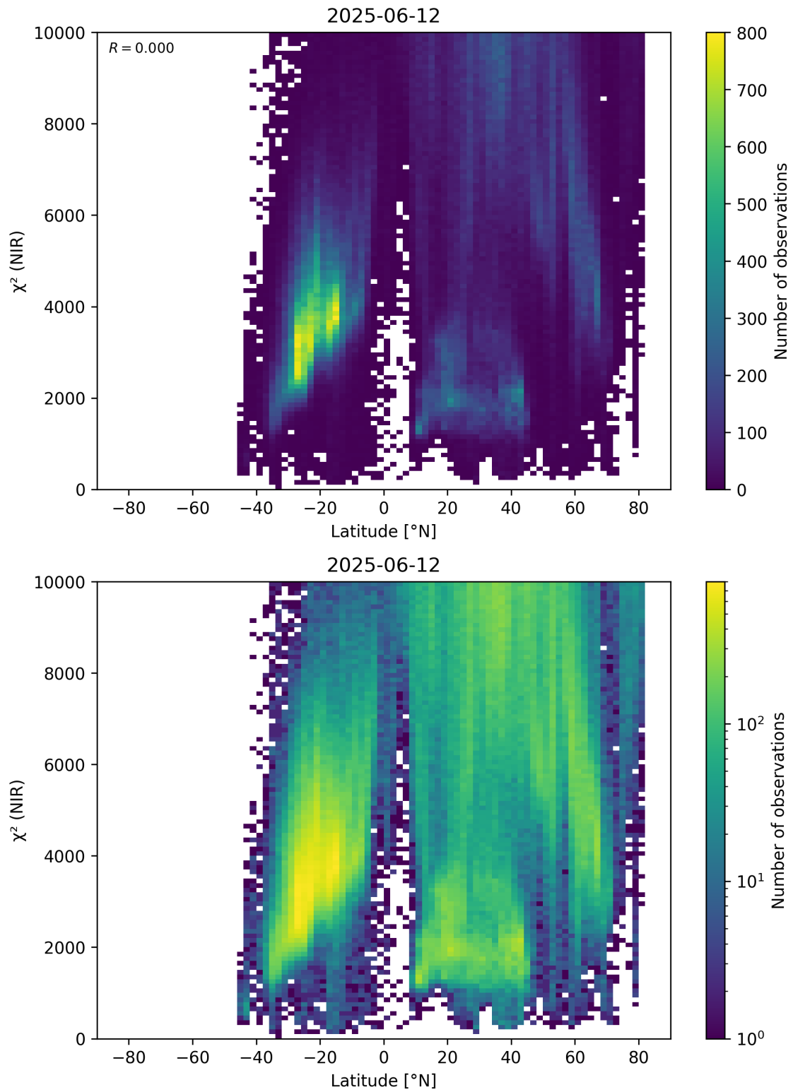
Figure 53: Scatter density plot of “Latitude” against “ \chi^2 (NIR)” for 2025-06-11 to 2025-06-13.
