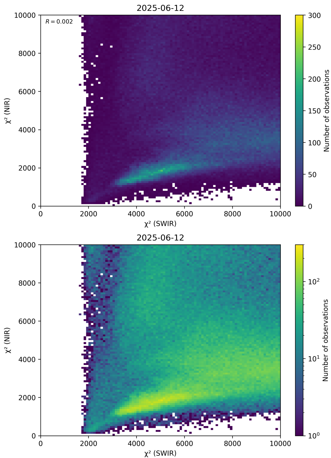
Figure 47: Scatter density plot of “ \chi^2 (SWIR)” against “ \chi^2 (NIR)” for 2025-06-11 to 2025-06-13.
