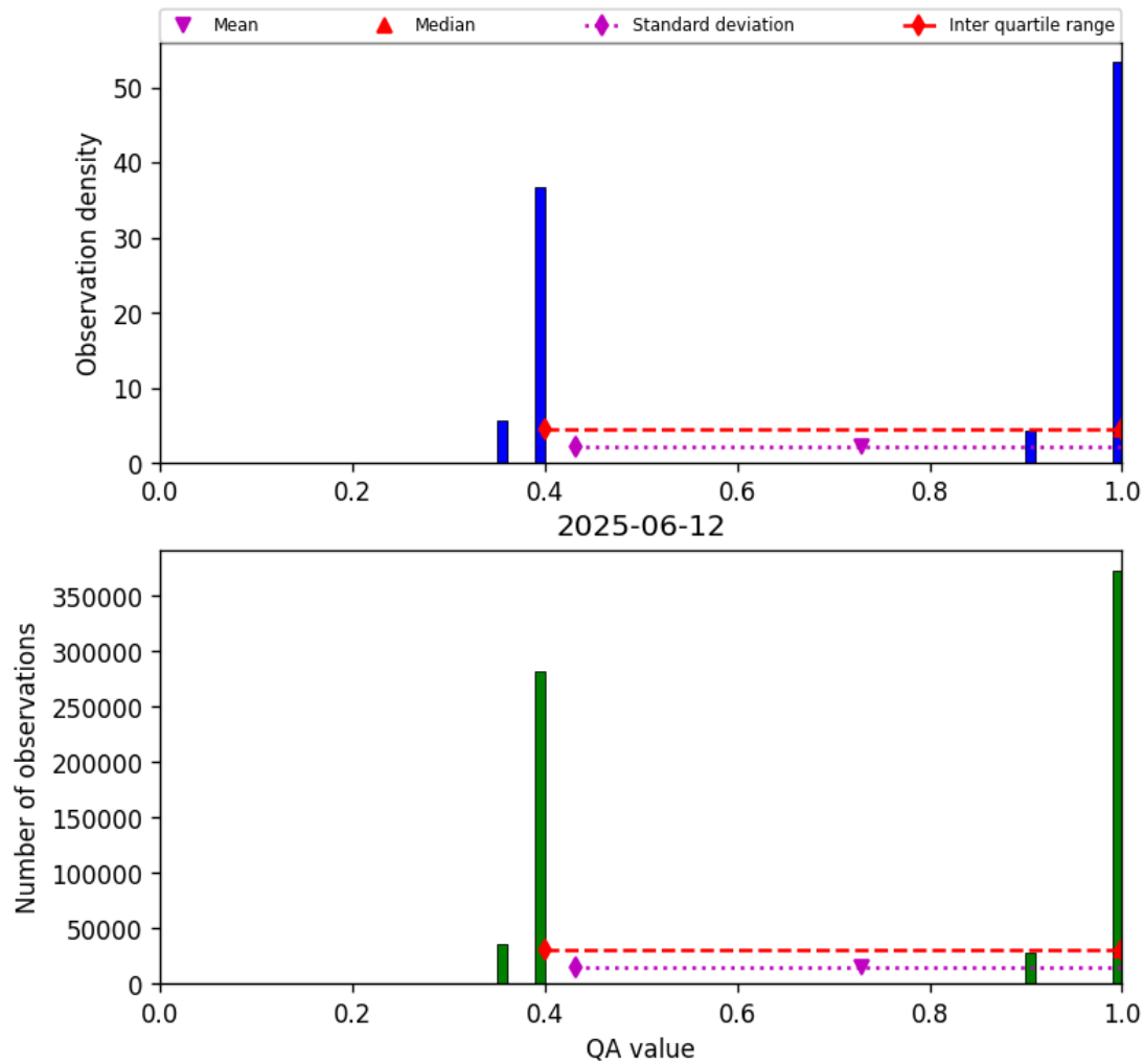
Figure 22: Histogram of “QA value” for 2025-06-11 to 2025-06-13
