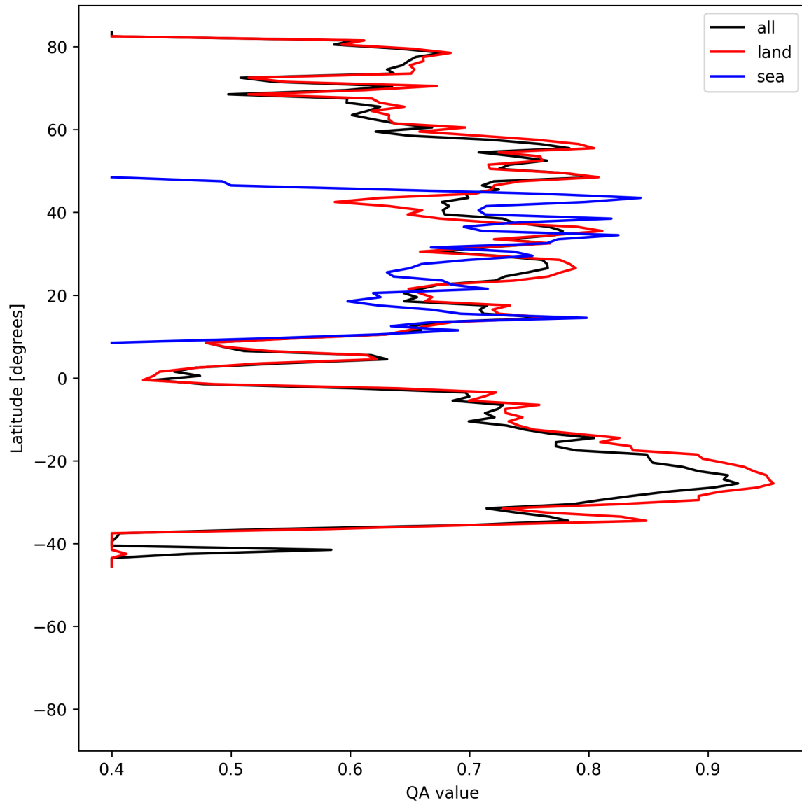
Figure 11: Zonal average of “QA value” for 2025-06-11 to 2025-06-13.
