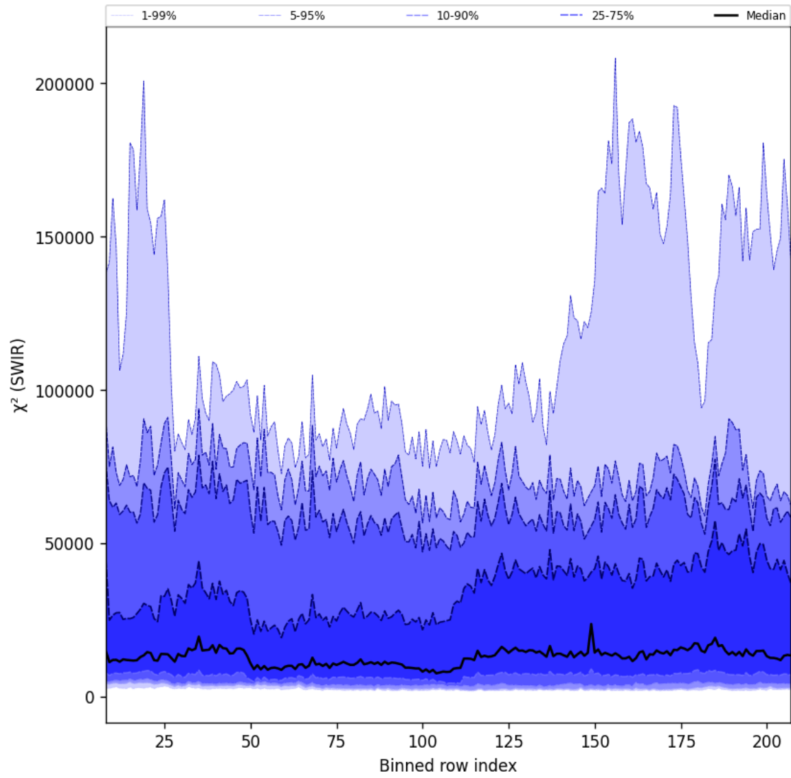
Figure 39: Along track statistics of " \chi^2 (SWIR)" for 2025-06-11 to 2025-06-13
