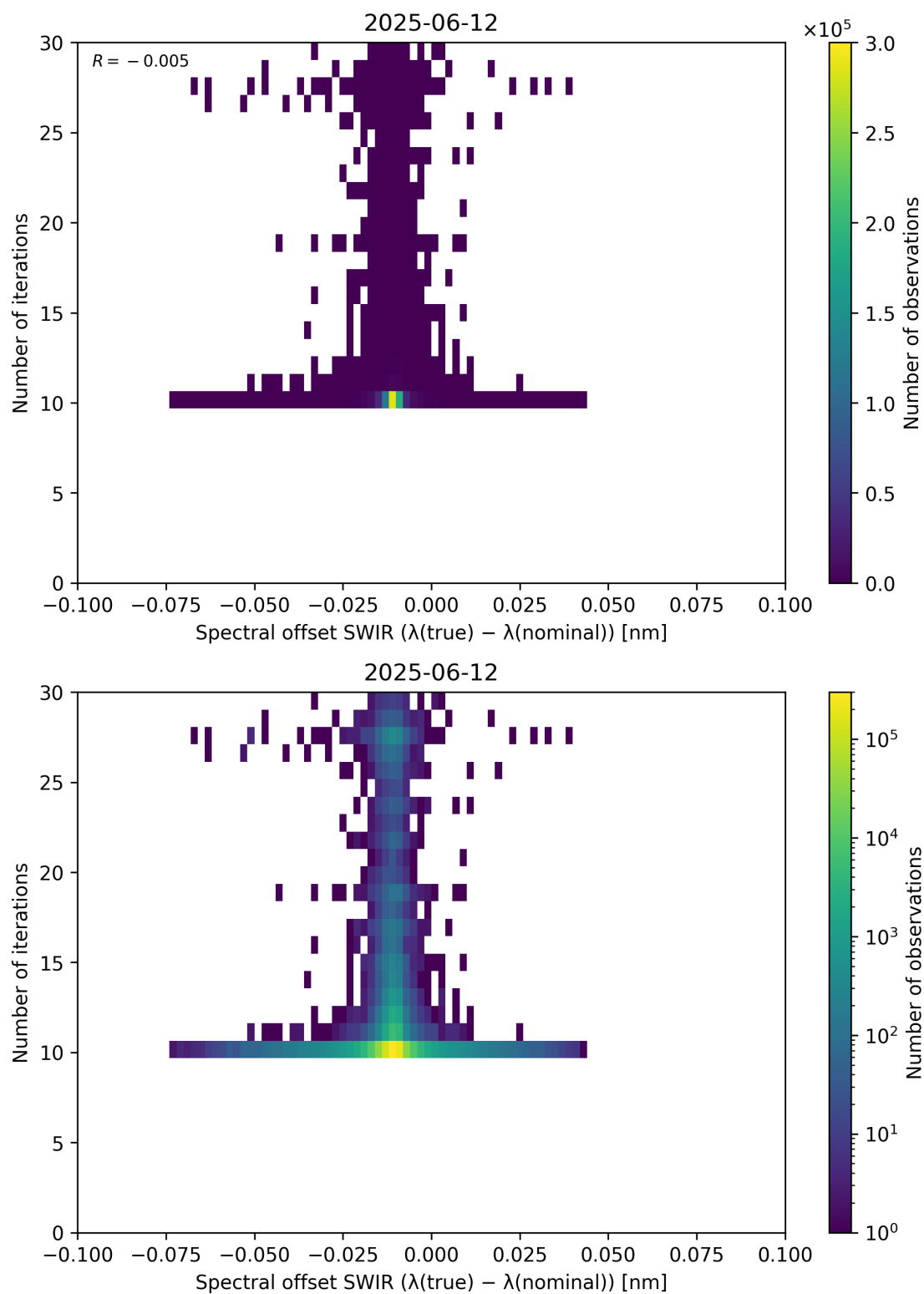
Figure 121: Scatter density plot of “Spectral offset SWIR ( \lambda_{\text{true}} - \lambda_{\text{nominal}} )” against “Number of iterations” for 2025-06-11 to 2025-06-13.
