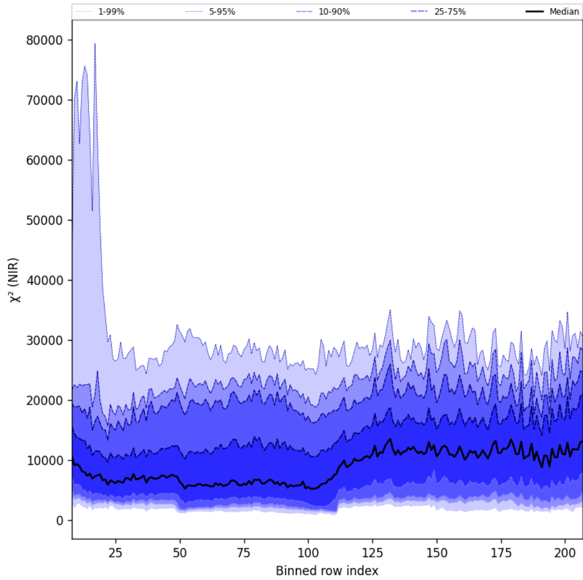
Figure 40: Along track statistics of “ \chi^2 (NIR)” for 2025-06-11 to 2025-06-13
