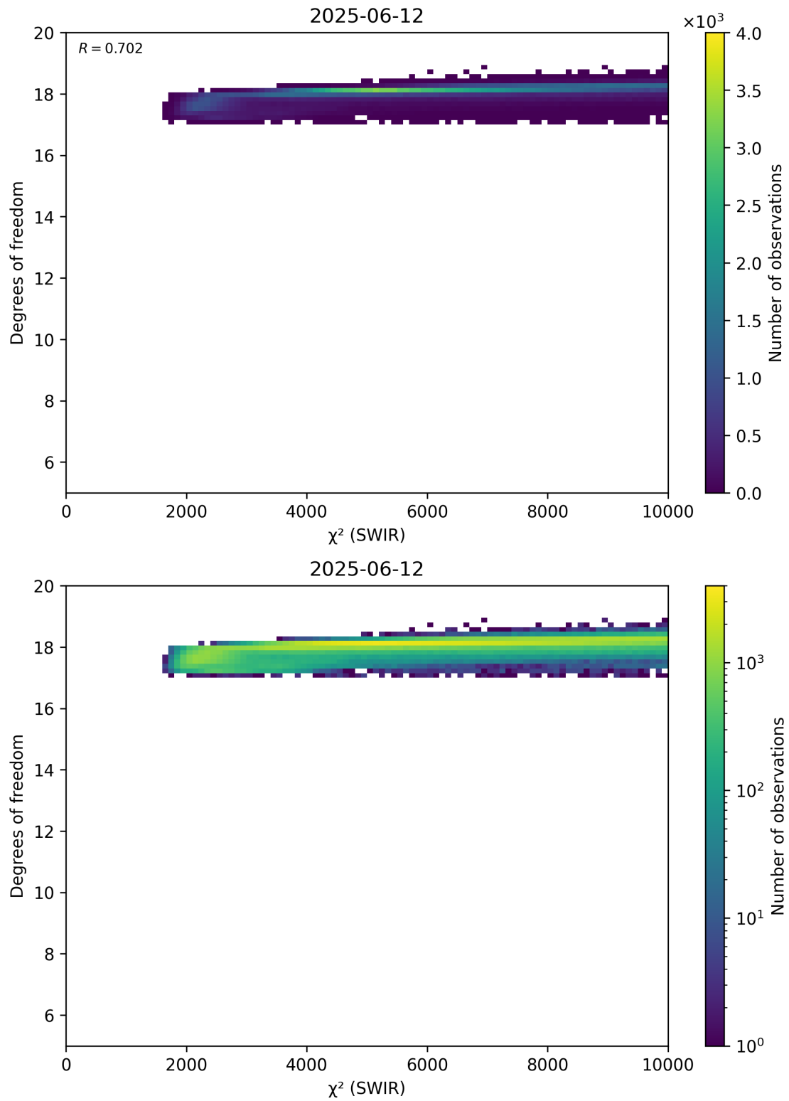
Figure 48: Scatter density plot of “ \chi^2 (SWIR)” against “Degrees of freedom” for 2025-06-11 to 2025-06-13.
