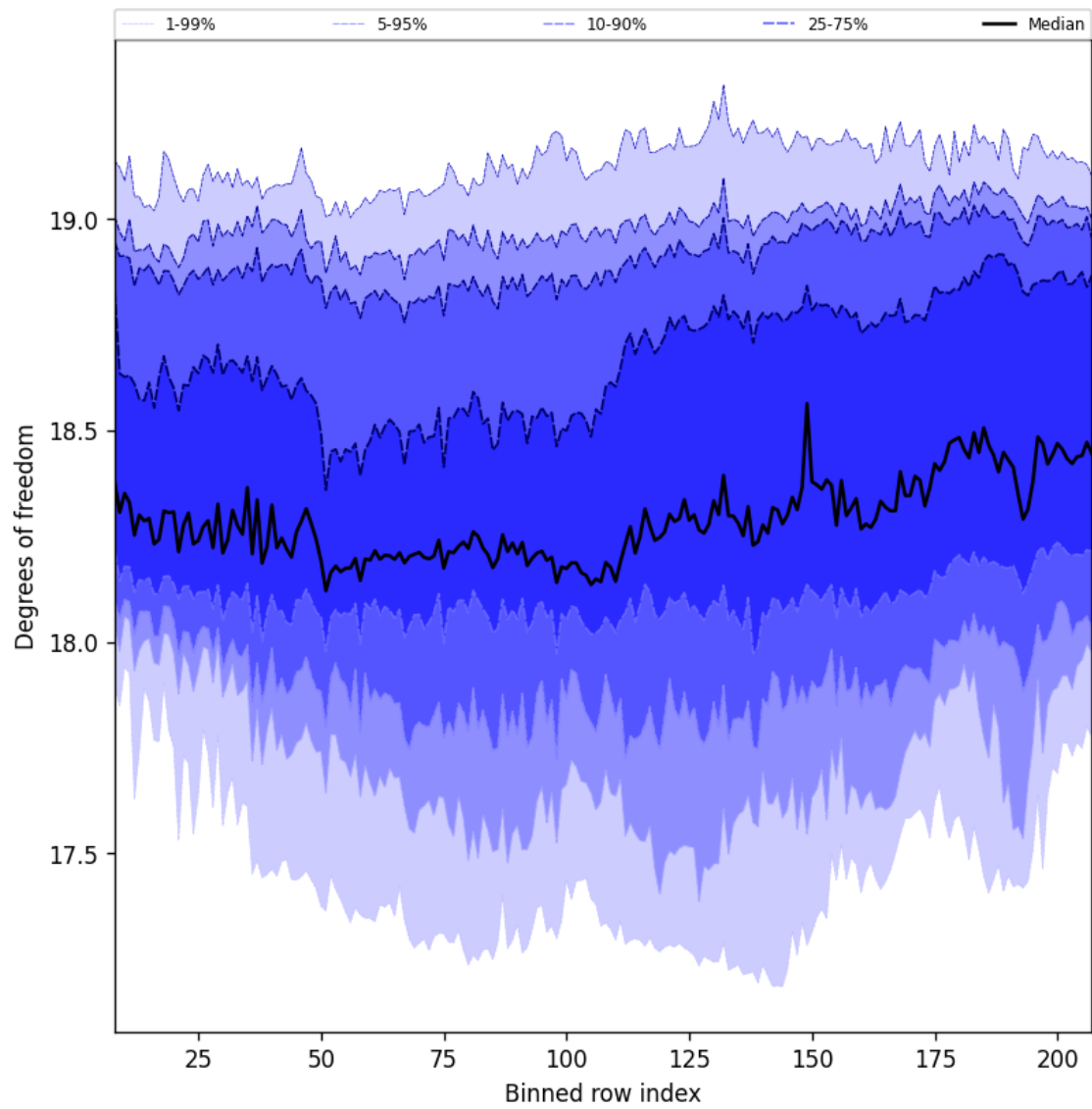
Figure 41: Along track statistics of “Degrees of freedom” for 2025-06-11 to 2025-06-13
