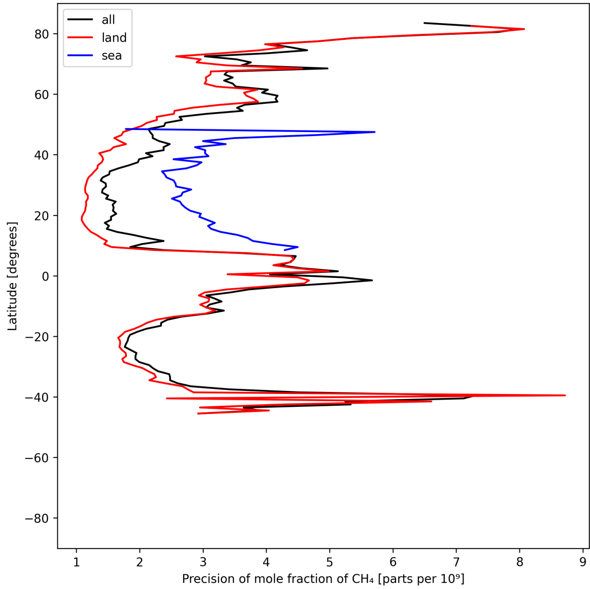
Figure 13: Zonal average of “Precision of mole fraction of CH 4 ” for 2025-06-11 to 2025-06-13.
