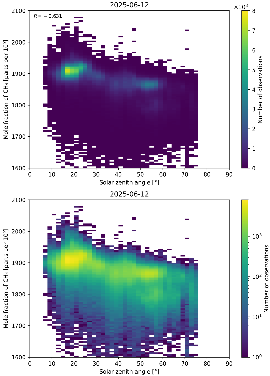
Figure 99: Scatter density plot of “Solar zenith angle” against “Mole fraction of CH 4 ” for 2025-06-11 to 2025-06-13.
