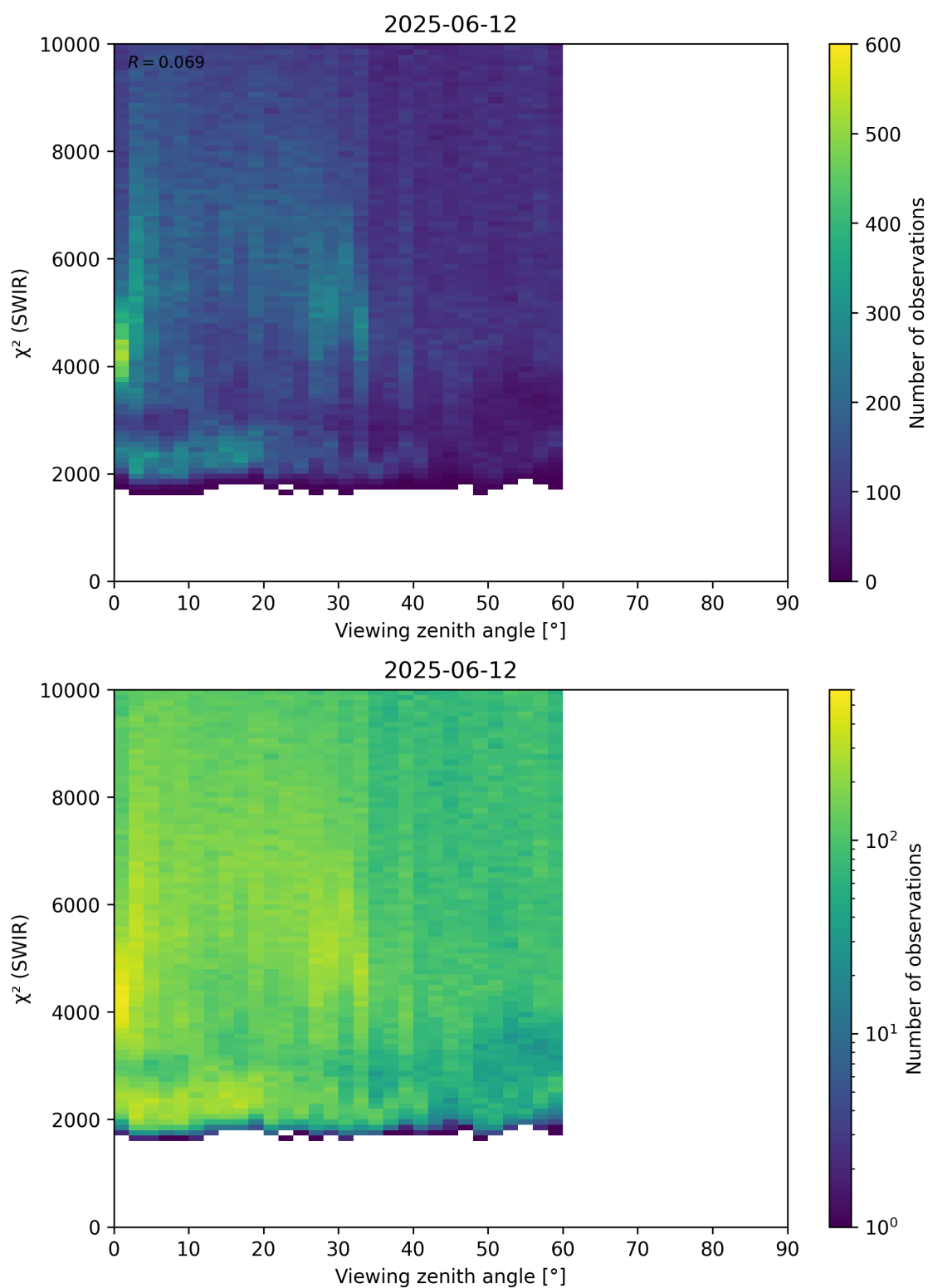
Figure 106: Scatter density plot of “Viewing zenith angle” against “ \chi^2 (SWIR)” for 2025-06-11 to 2025-06-13.
