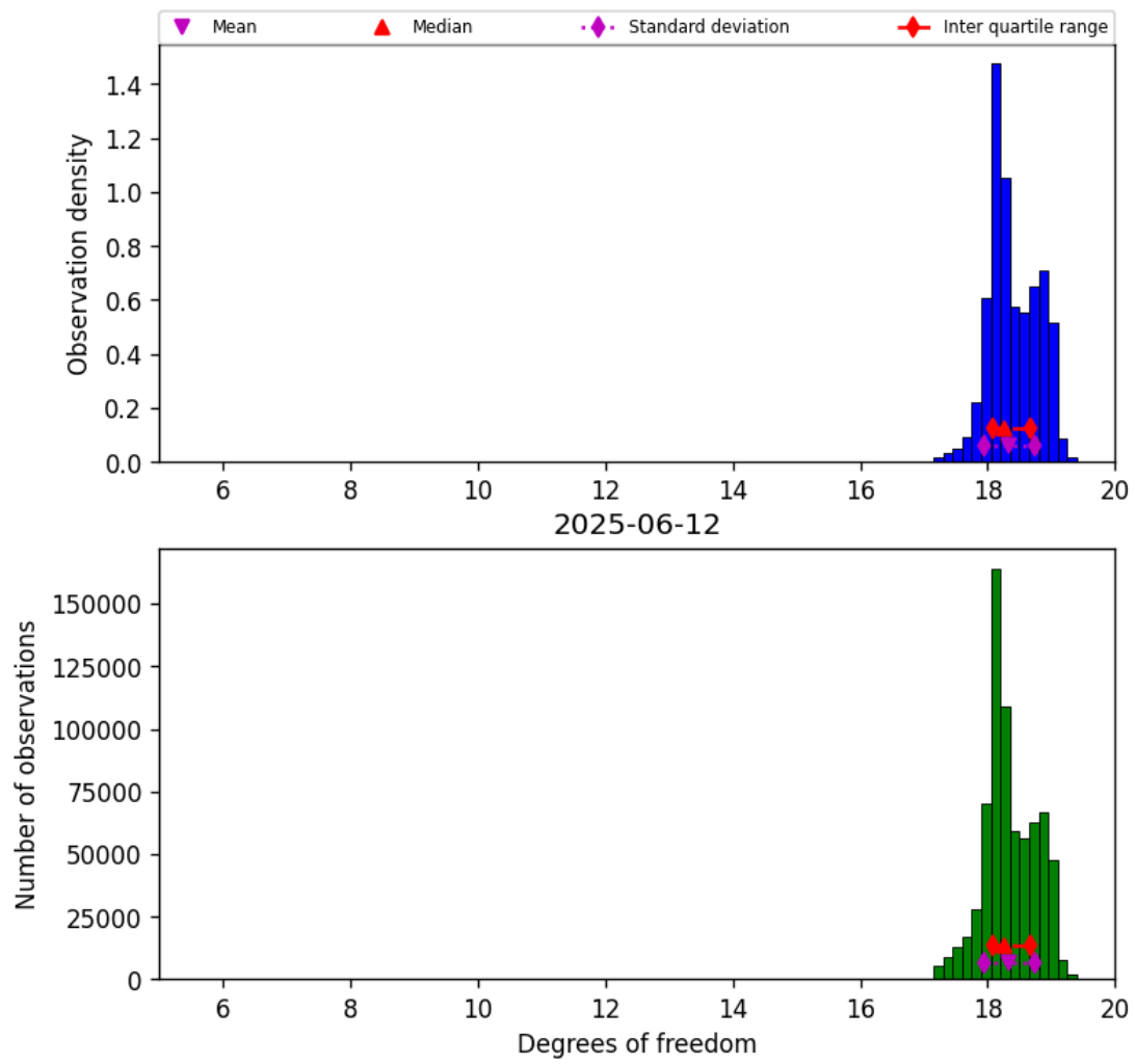
Figure 30: Histogram of “Degrees of freedom” for 2025-06-11 to 2025-06-13
