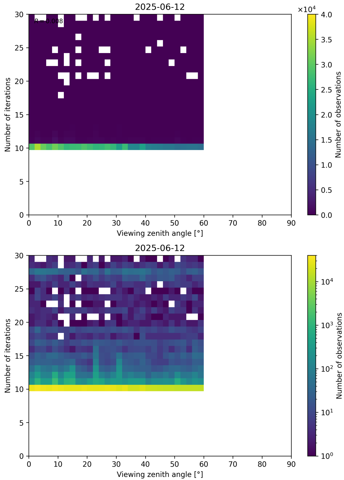
Figure 113: Scatter density plot of “Viewing zenith angle” against “Number of iterations” for 2025-06-11 to 2025-06-13.
