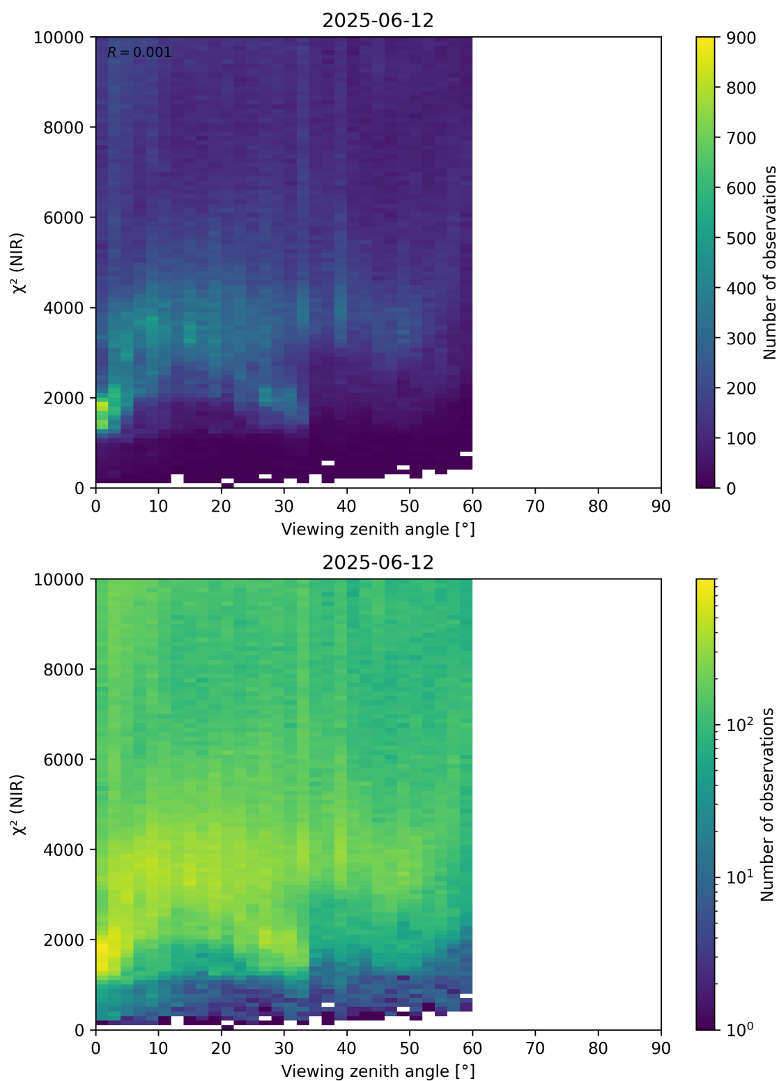
Figure 105: Scatter density plot of “Viewing zenith angle” against “ \chi^2 (NIR)” for 2025-06-11 to 2025-06-13.
