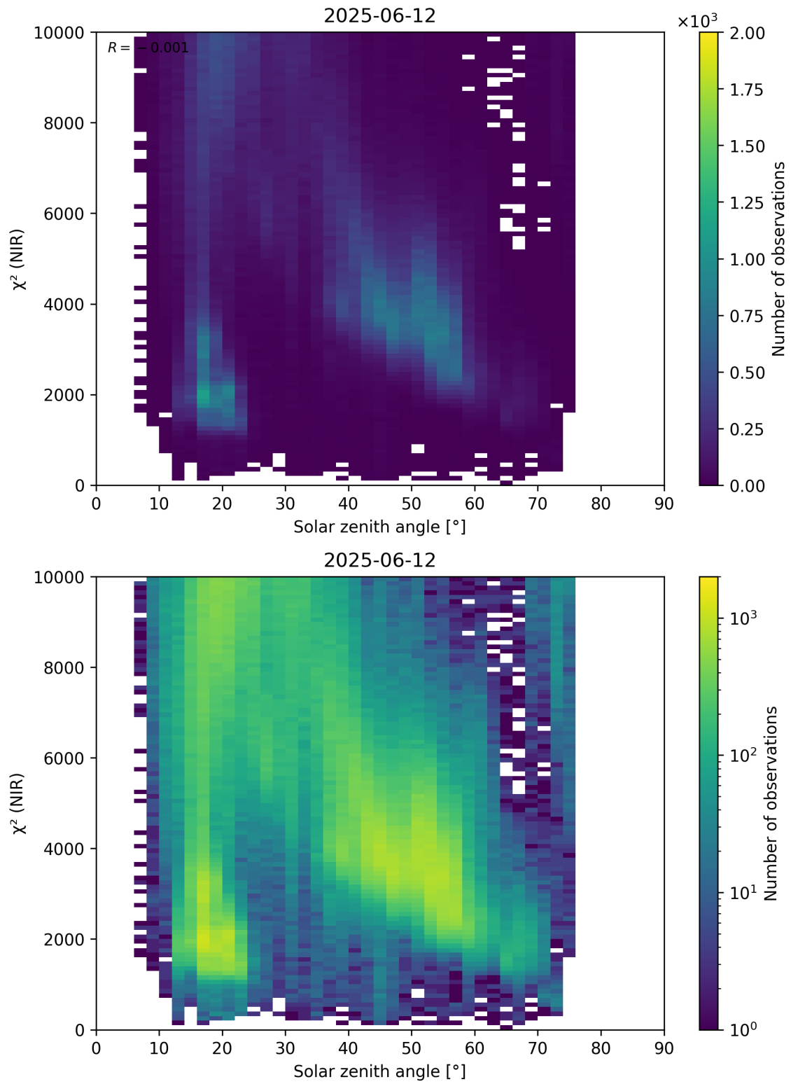
Figure 94: Scatter density plot of “Solar zenith angle” against “ \chi^2 (NIR)” for 2025-06-11 to 2025-06-13.
