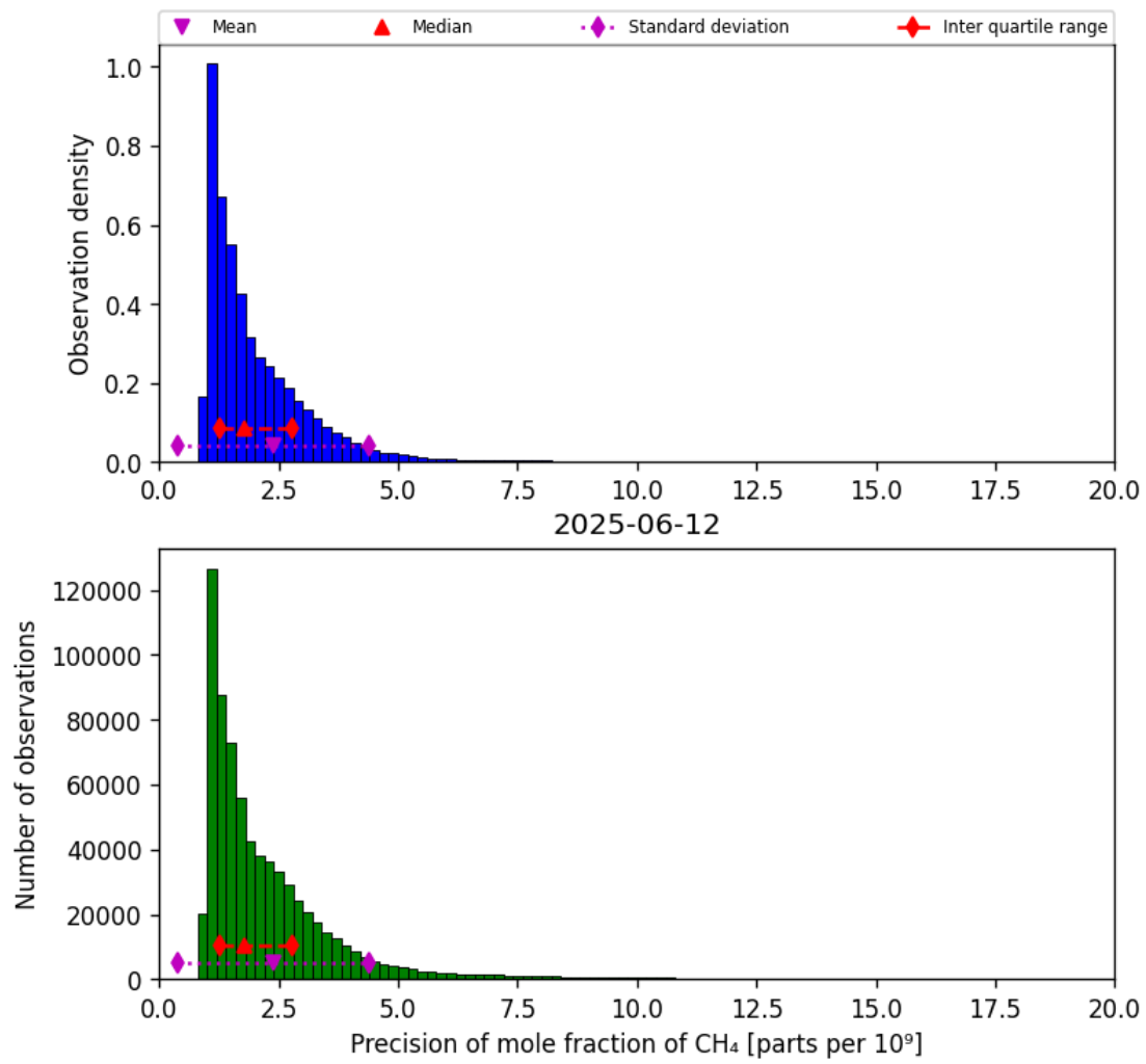
Figure 24: Histogram of “Precision of mole fraction of CH 4 ” for 2025-06-11 to 2025-06-13
