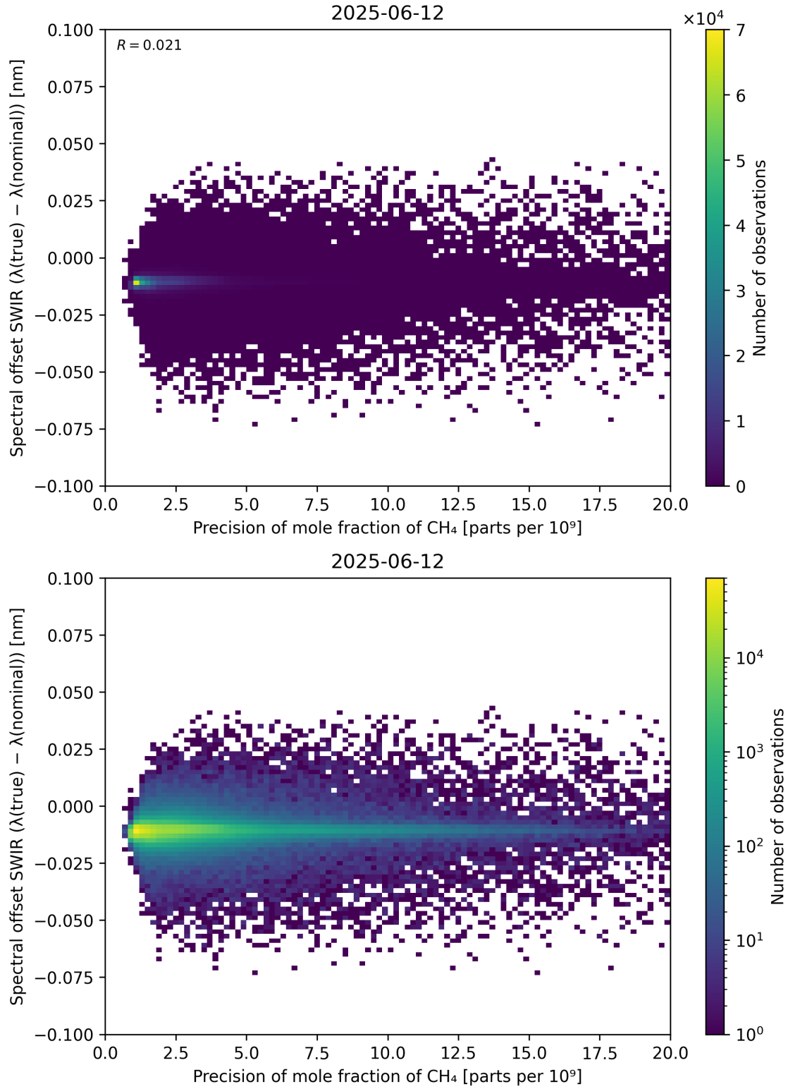
Figure 85: Scatter density plot of “Precision of mole fraction of CH 4 ” against “Spectral offset SWIR ( \lambda_{\text{true}} - \lambda_{\text{nominal}} )” for 2025-06-11 to 2025-06-13.
