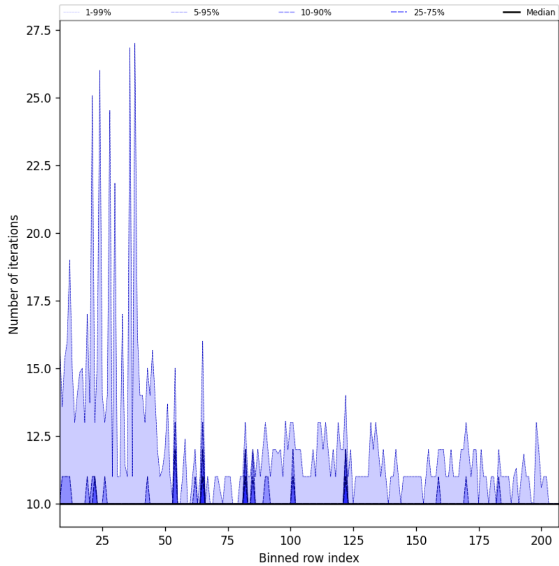
Figure 42: Along track statistics of “Number of iterations” for 2025-06-11 to 2025-06-13
