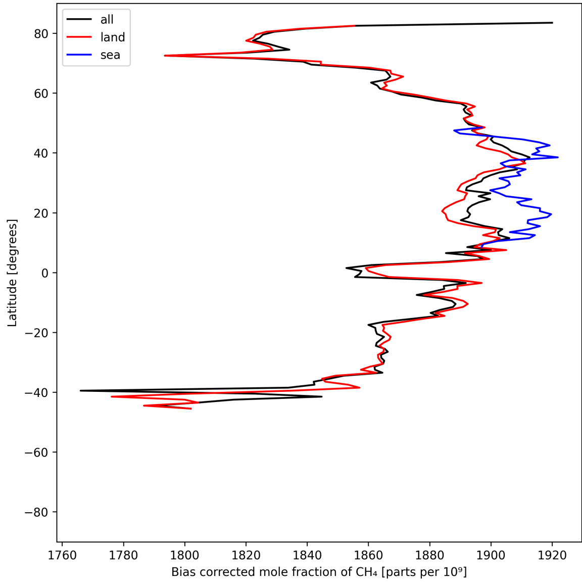
Figure 14: Zonal average of “Bias corrected mole fraction of CH 4 ” for 2025-06-11 to 2025-06-13.
