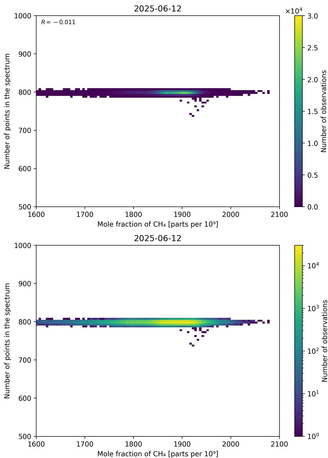
Figure 77: Scatter density plot of “Mole fraction of CH 4 ” against “Number of points in the spectrum” for 2025-06-11 to 2025-06-13.
