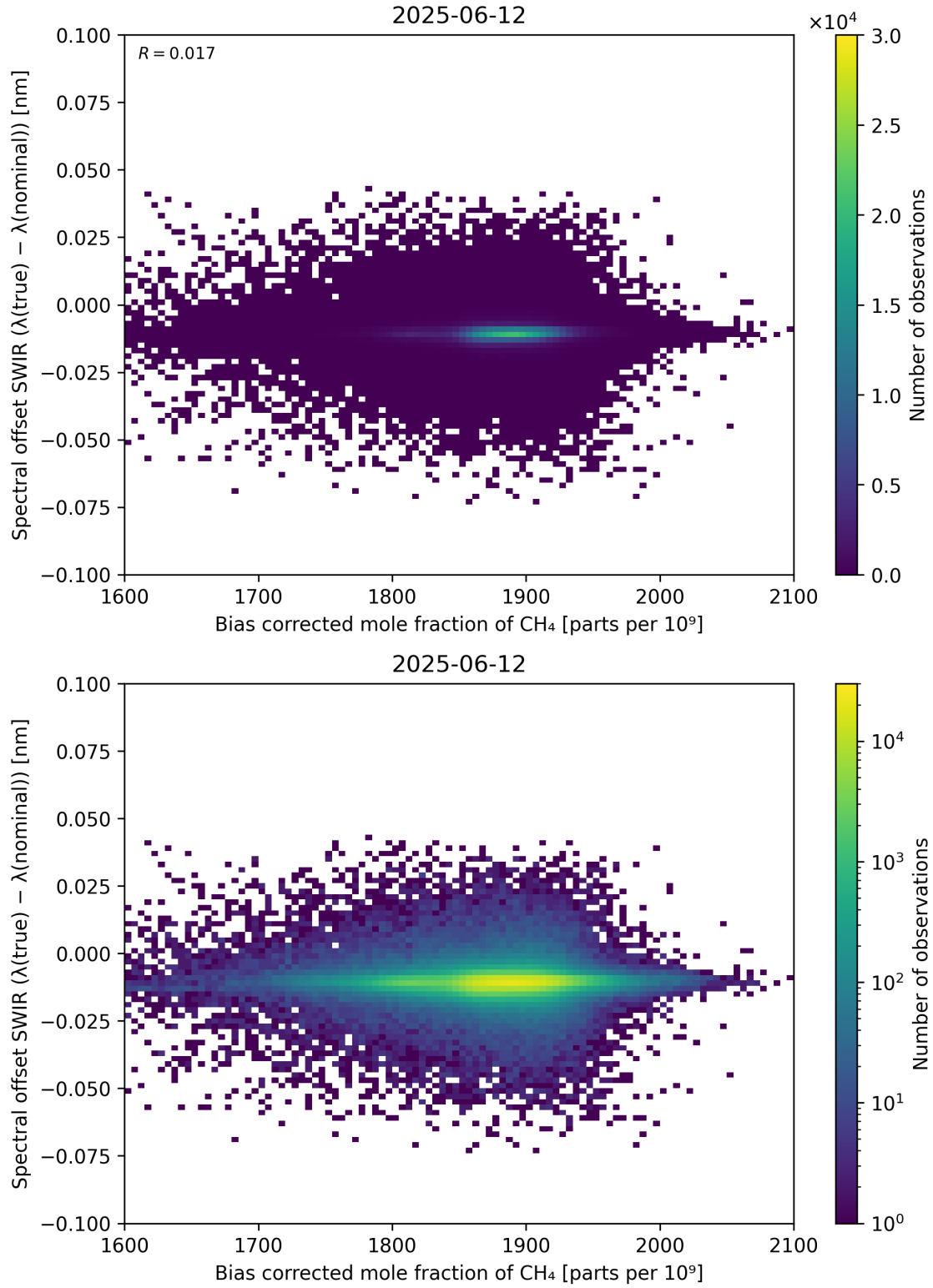
Figure 69: Scatter density plot of “Bias corrected mole fraction of \text{CH}_4 ” against “Spectral offset SWIR ( \lambda_{\text{true}} - \lambda_{\text{nominal}} )” for 2025-06-11 to 2025-06-13.
