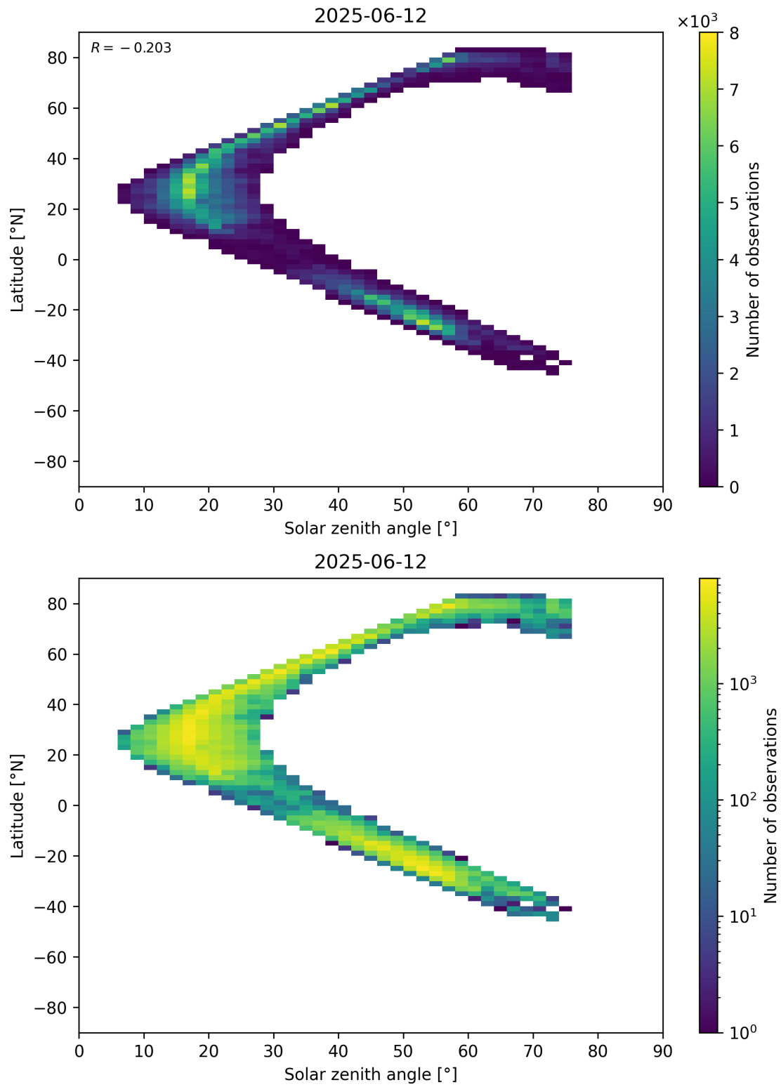
Figure 98: Scatter density plot of “Solar zenith angle” against “Latitude” for 2025-06-11 to 2025-06-13.
