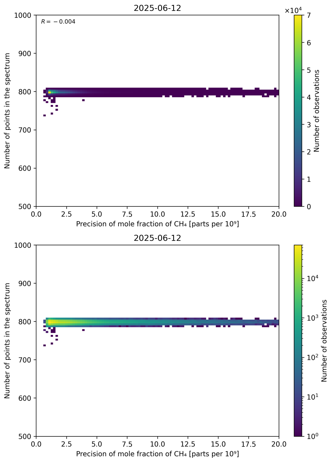
Figure 84: Scatter density plot of “Precision of mole fraction of CH 4 ” against “Number of points in the spectrum” for 2025-06-11 to 2025-06-13.
