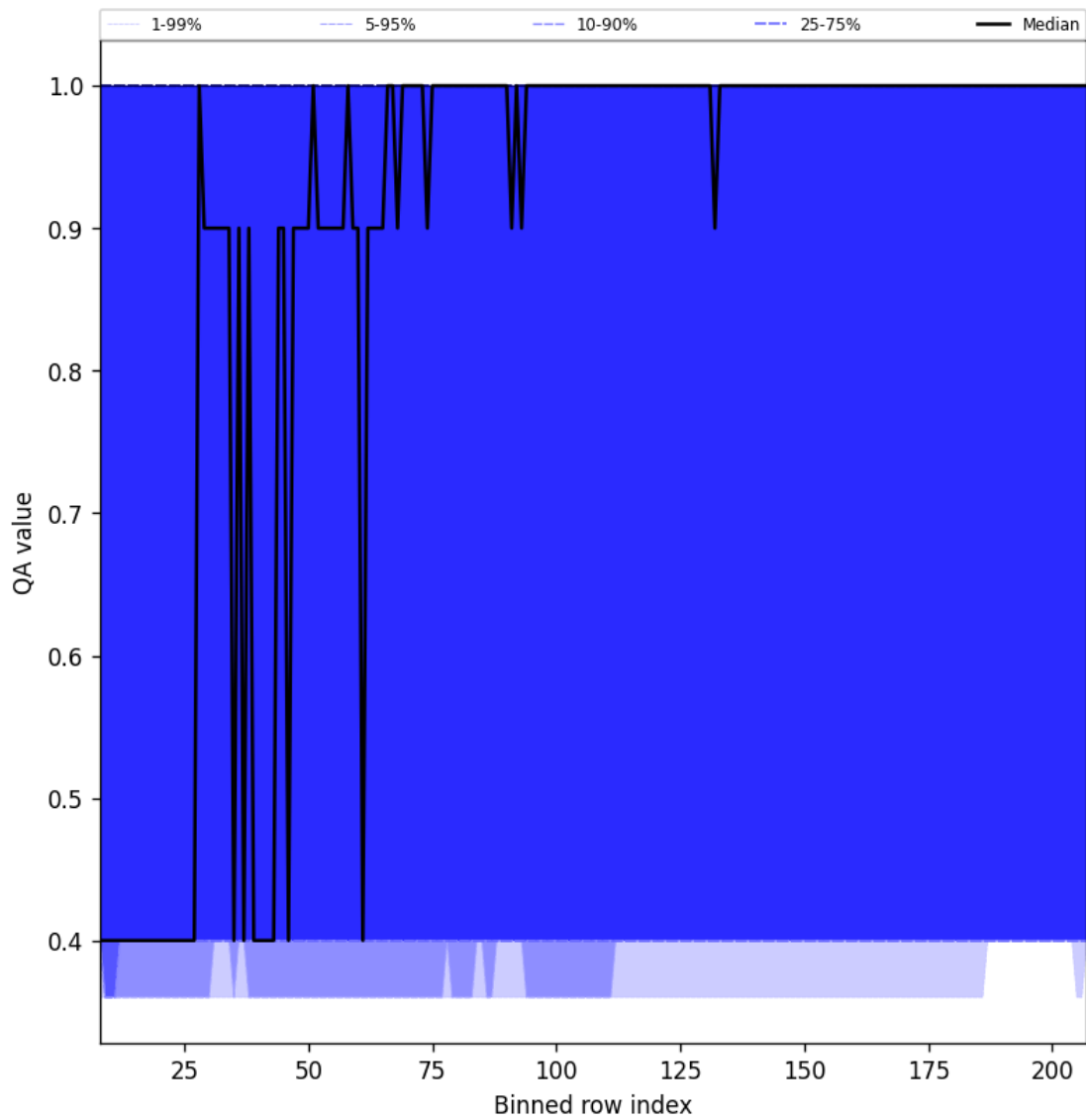
Figure 33: Along track statistics of “QA value” for 2025-06-11 to 2025-06-13
