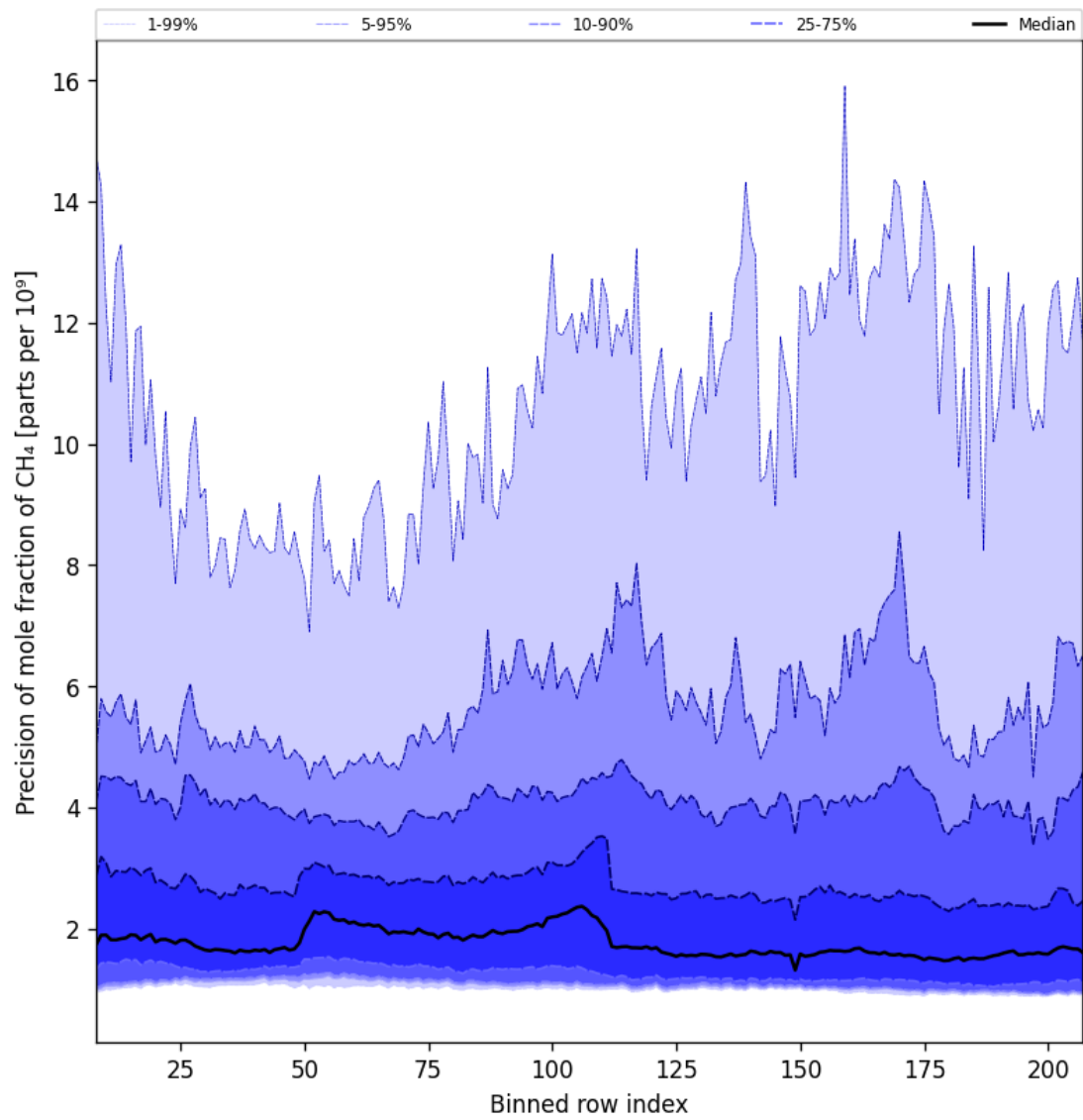
Figure 35: Along track statistics of “Precision of mole fraction of CH 4 ” for 2025-06-11 to 2025-06-13
