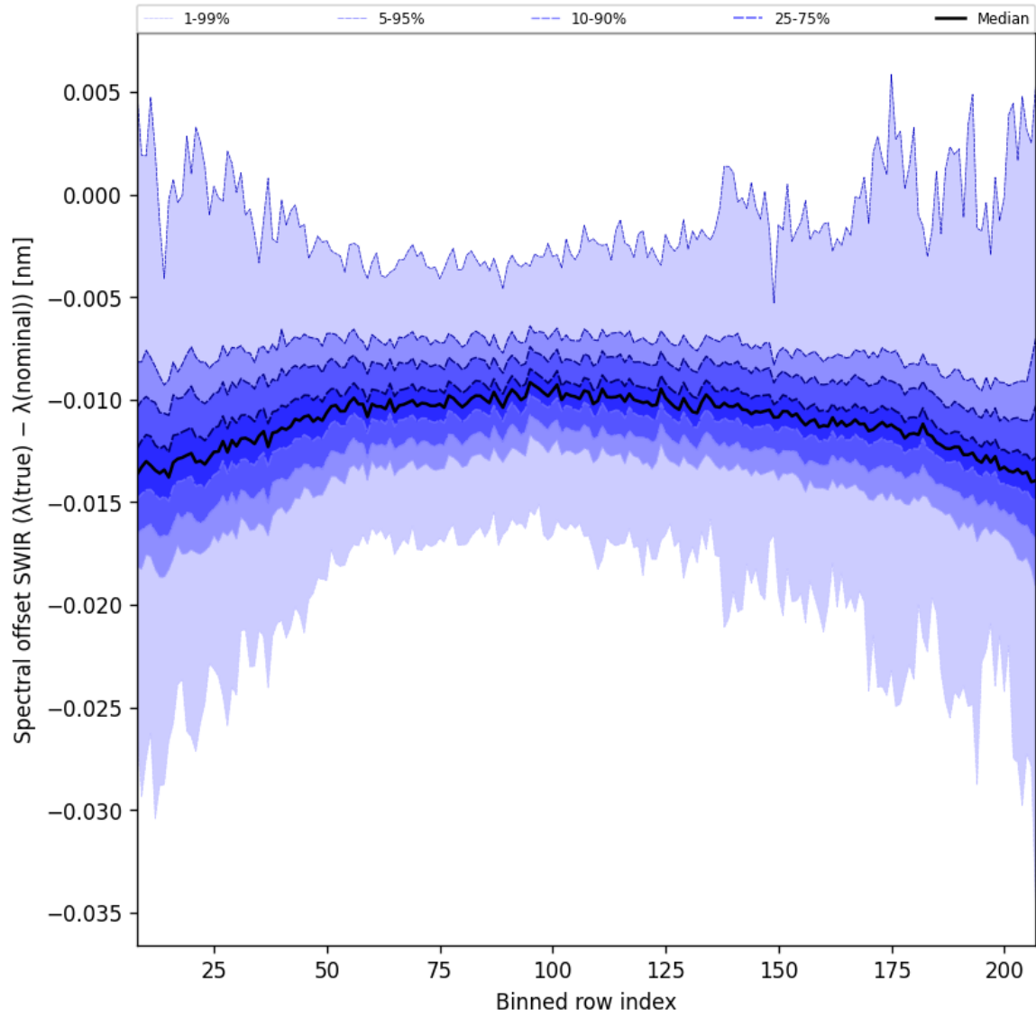
Figure 38: Along track statistics of “Spectral offset SWIR ( \lambda_{\text{true}} - \lambda_{\text{nominal}} )” for 2025-06-11 to 2025-06-13
