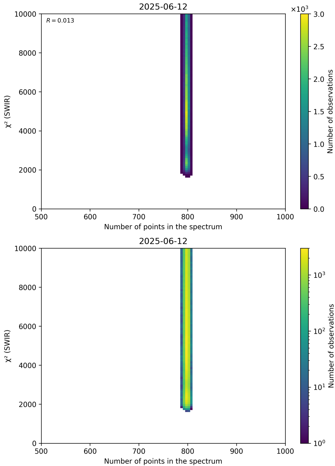
Figure 89: Scatter density plot of “Number of points in the spectrum” against “ \chi^2 (SWIR)” for 2025-06-11 to 2025-06-13.
