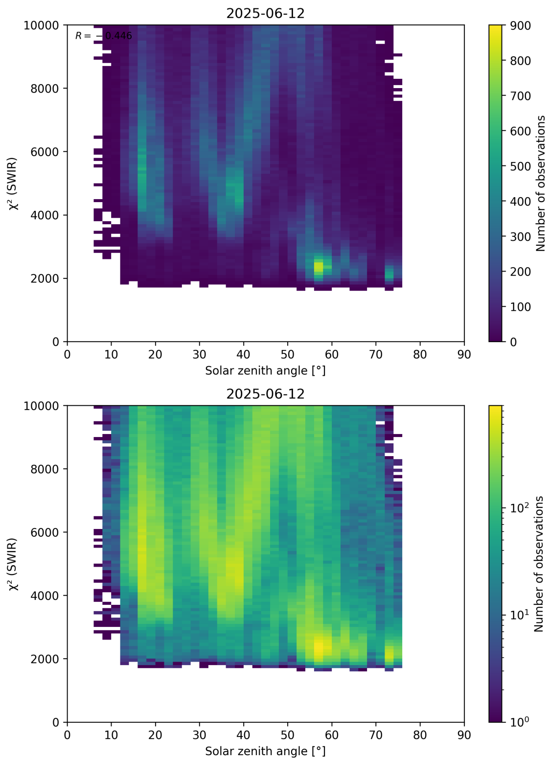
Figure 95: Scatter density plot of “Solar zenith angle” against “ \chi^2 (SWIR)” for 2025-06-11 to 2025-06-13.
