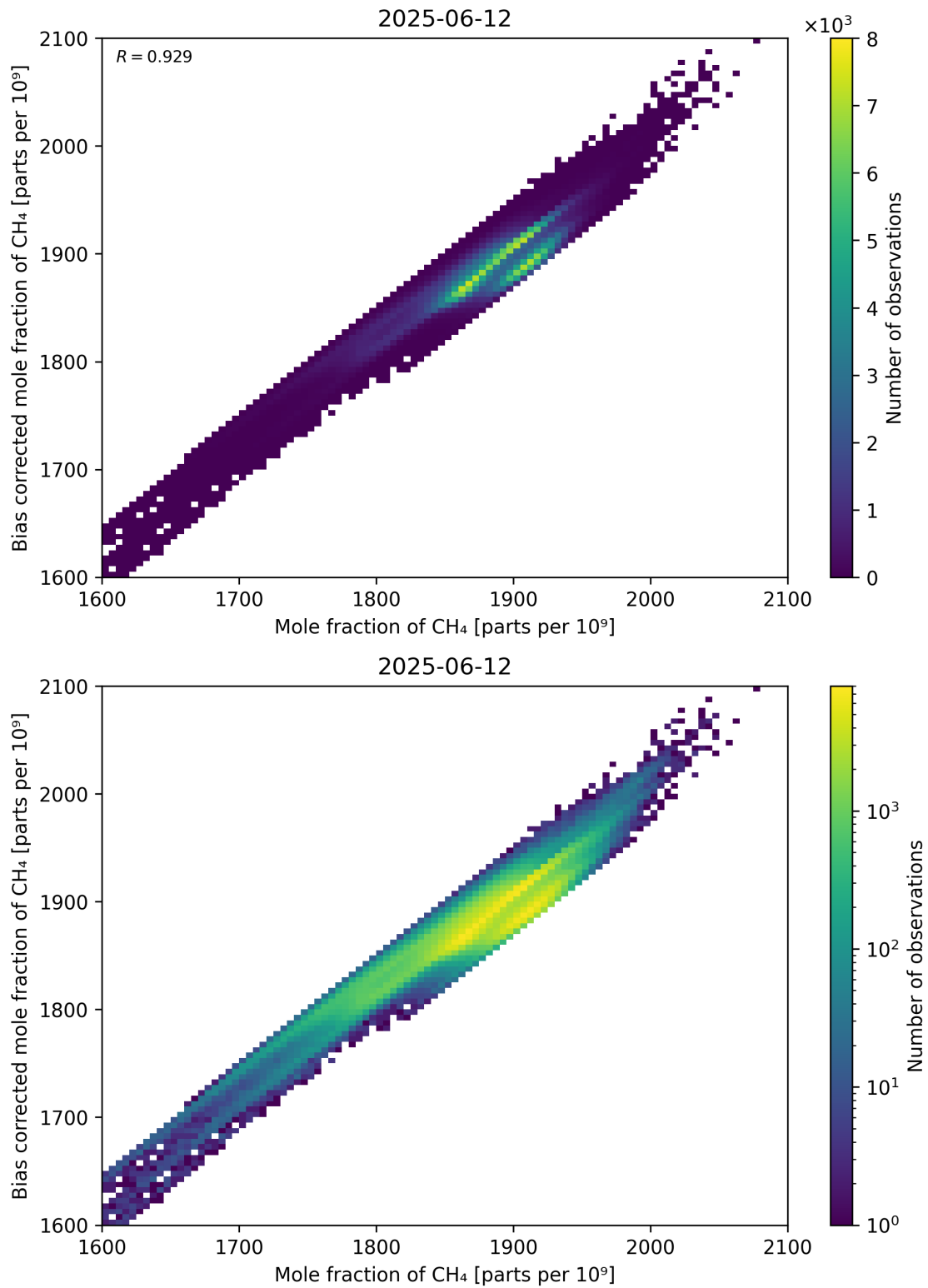
Figure 74: Scatter density plot of “Mole fraction of CH 4 ” against “Bias corrected mole fraction of CH 4 ” for 2025-06-11 to 2025-06-13.
