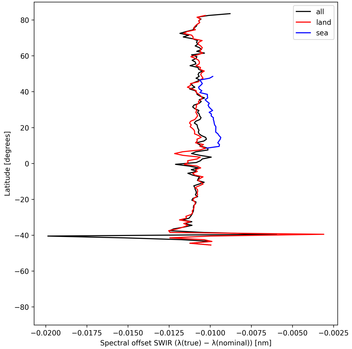
Figure 16: Zonal average of “Spectral offset SWIR ( \lambda_{\text{true}} - \lambda_{\text{nominal}} )” for 2025-06-11 to 2025-06-13.
