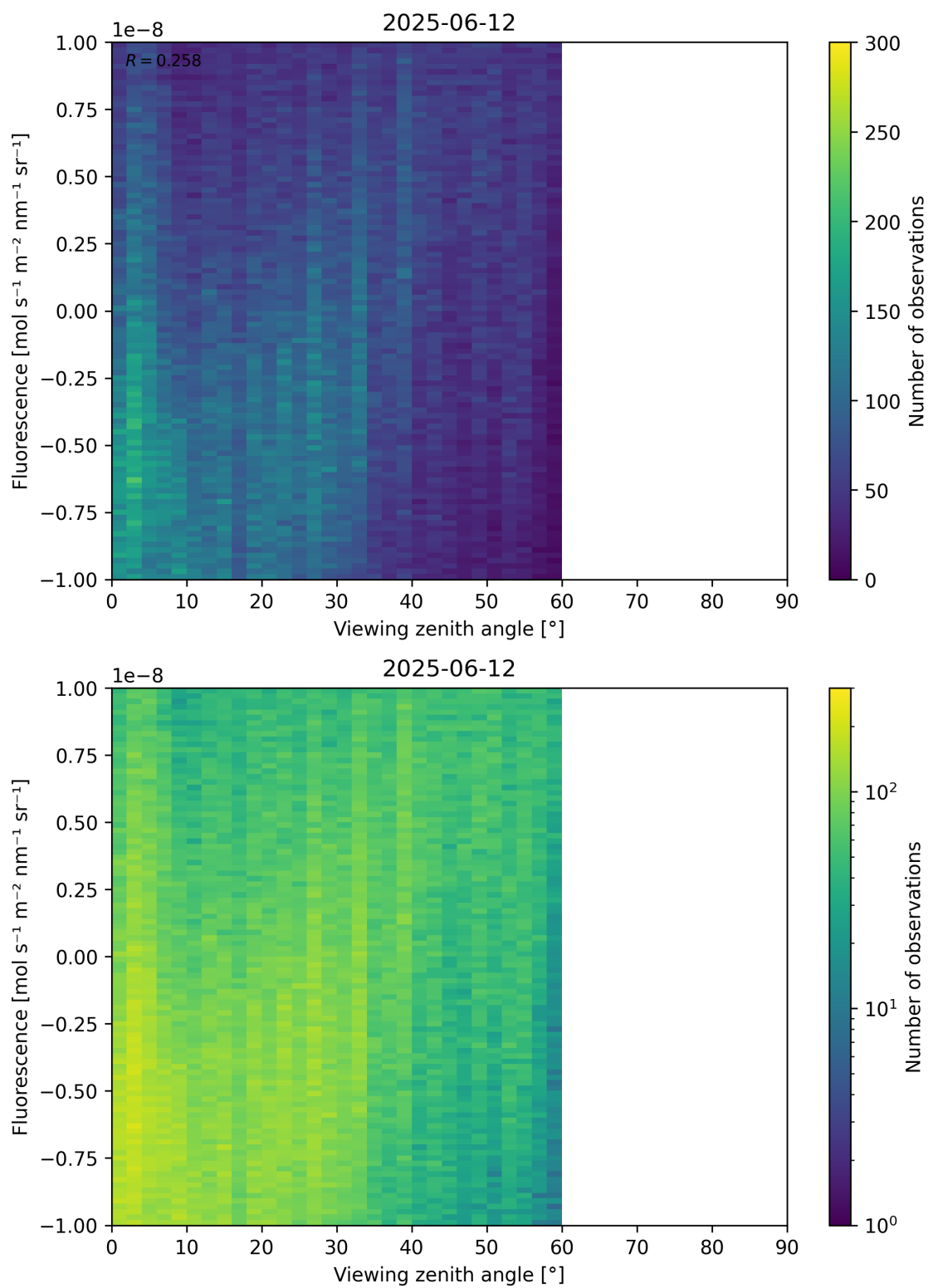
Figure 108: Scatter density plot of “Viewing zenith angle” against “Fluorescence” for 2025-06-11 to 2025-06-13.
