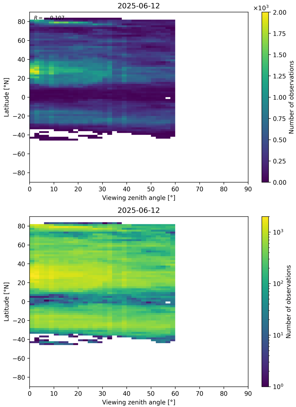
Figure 109: Scatter density plot of “Viewing zenith angle” against “Latitude” for 2025-06-11 to 2025-06-13.
