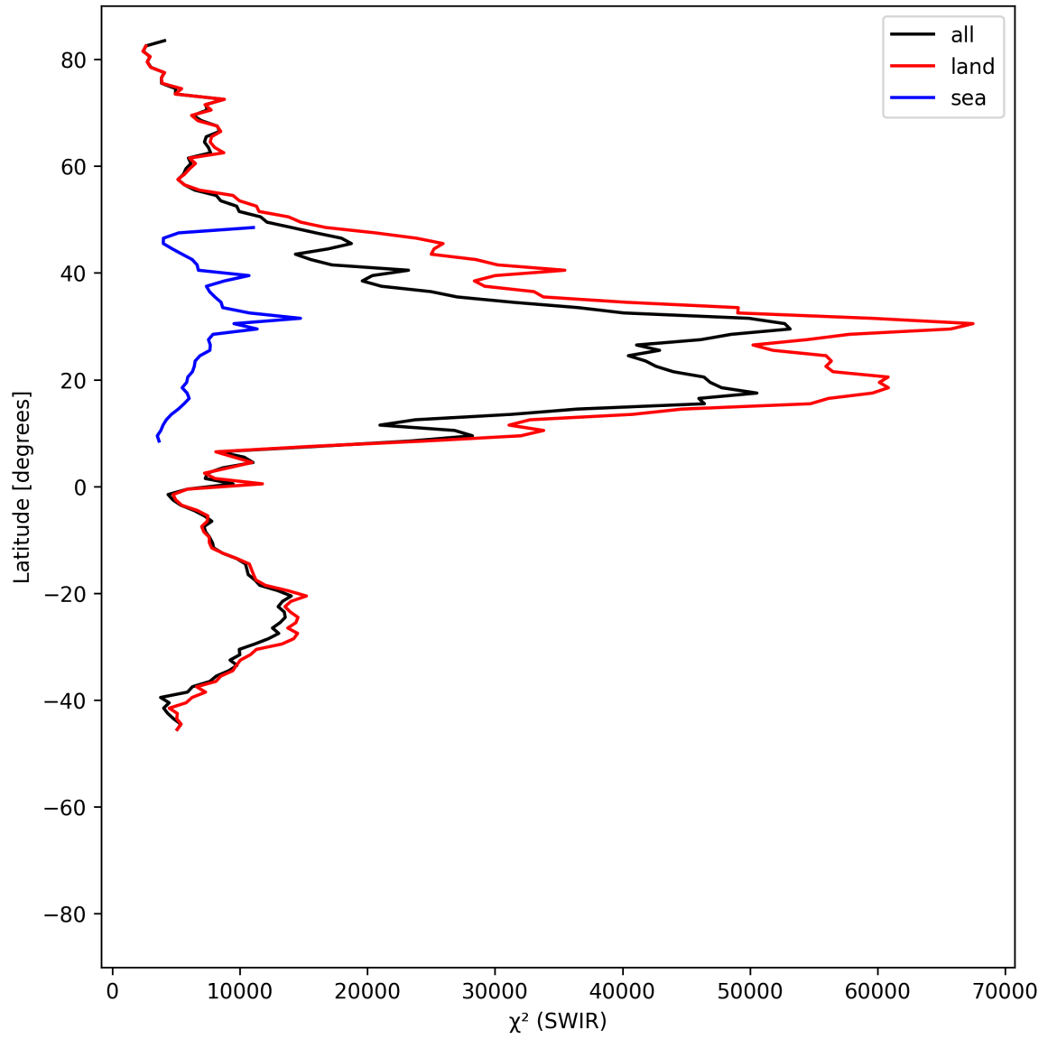
Figure 17: Zonal average of “ \chi^2 (SWIR)” for 2025-06-11 to 2025-06-13.
