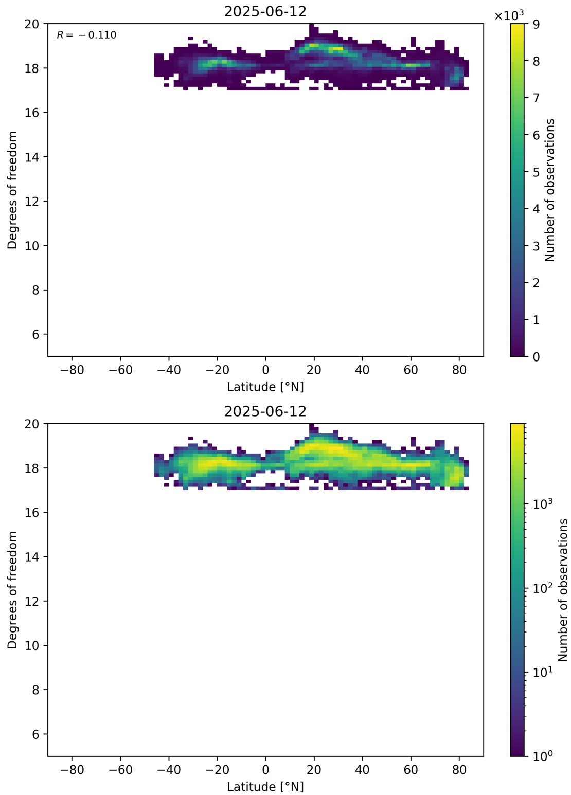
Figure 55: Scatter density plot of “Latitude” against “Degrees of freedom” for 2025-06-11 to 2025-06-13.
