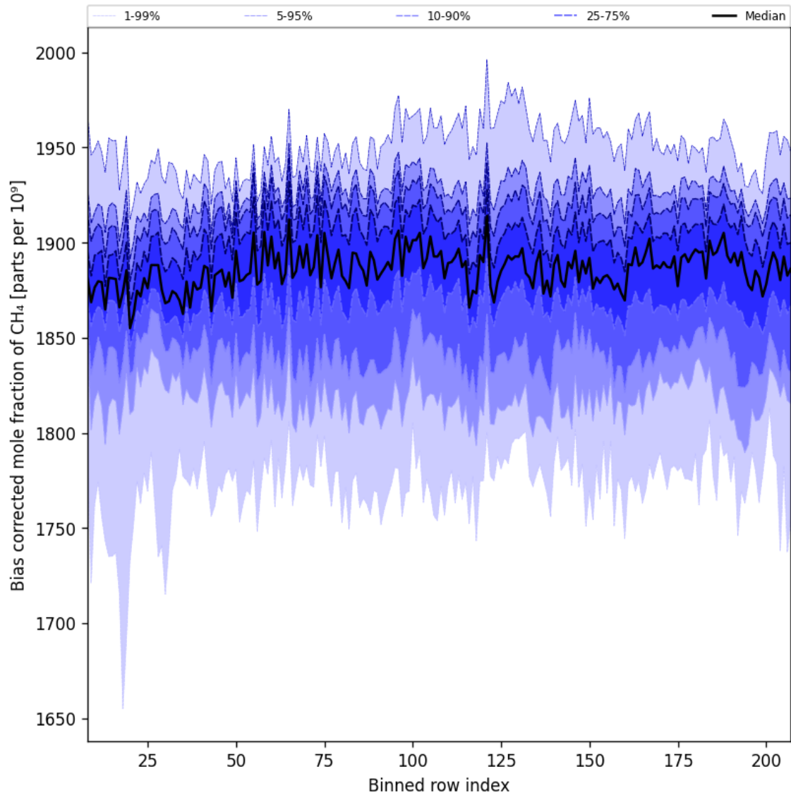
Figure 36: Along track statistics of “Bias corrected mole fraction of CH 4 ” for 2025-06-11 to 2025-06-13
