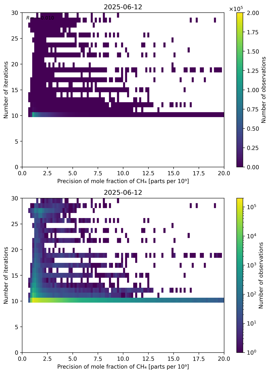
Figure 83: Scatter density plot of “Precision of mole fraction of CH 4 ” against “Number of iterations” for 2025-06-11 to 2025-06-13.
