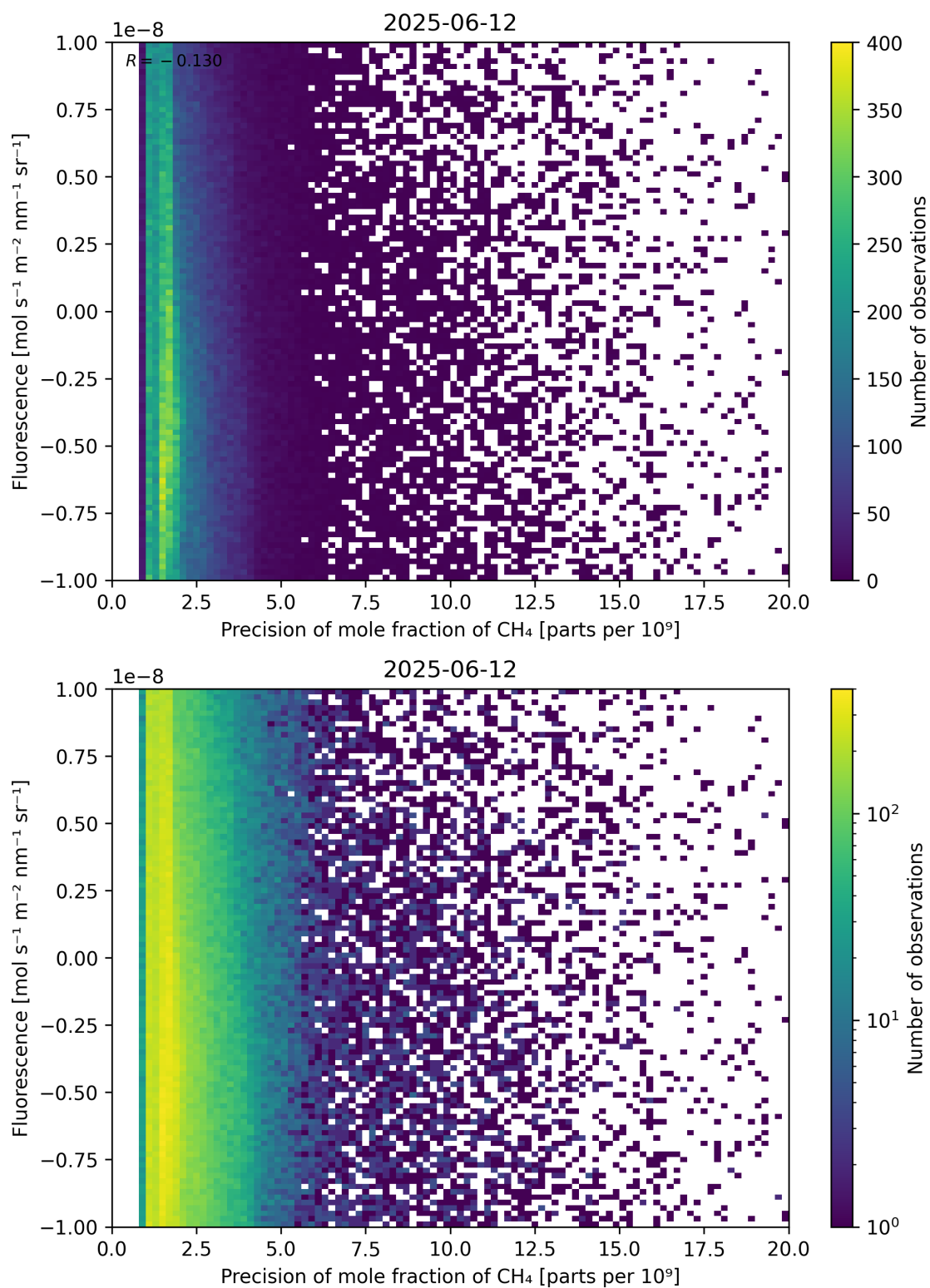
Figure 81: Scatter density plot of “Precision of mole fraction of CH 4 ” against “Fluorescence” for 2025-06-11 to 2025-06-13.
