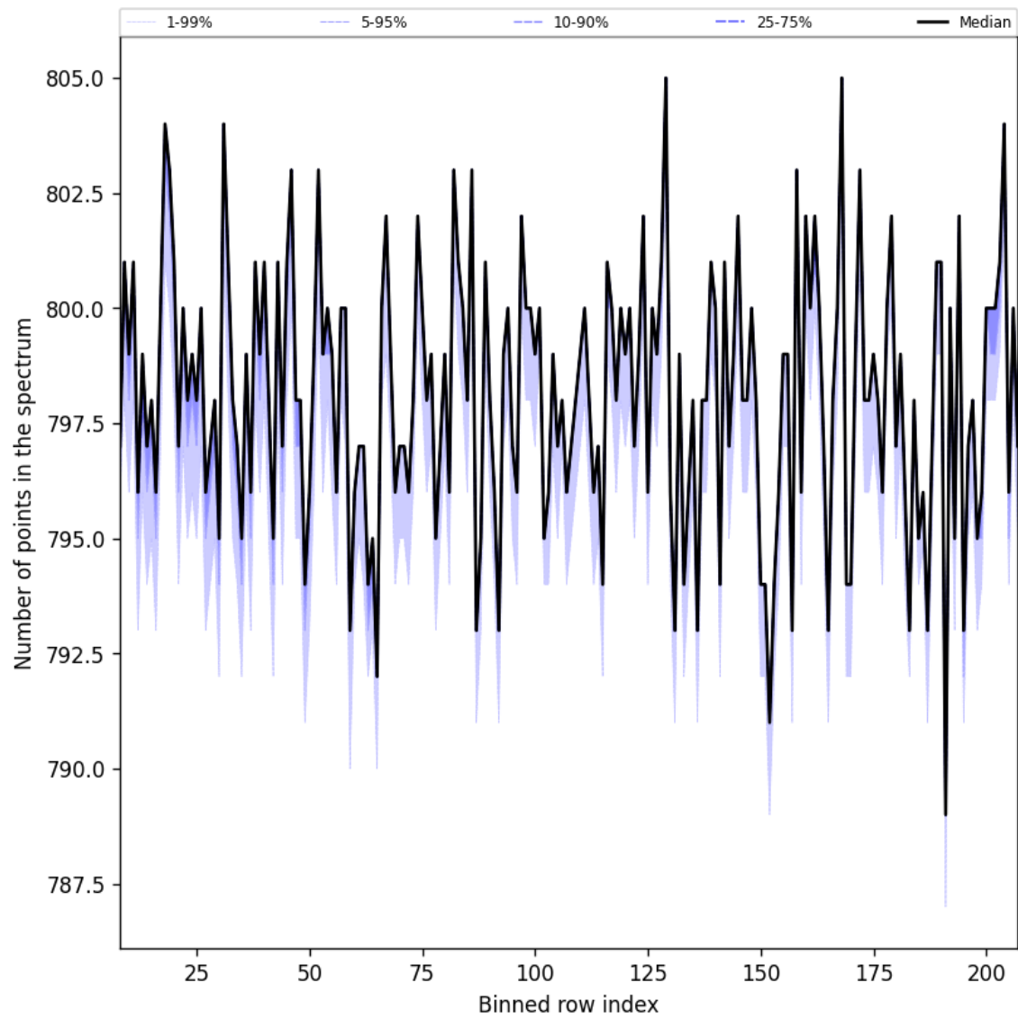
Figure 37: Along track statistics of “Number of points in the spectrum” for 2025-06-11 to 2025-06-13
