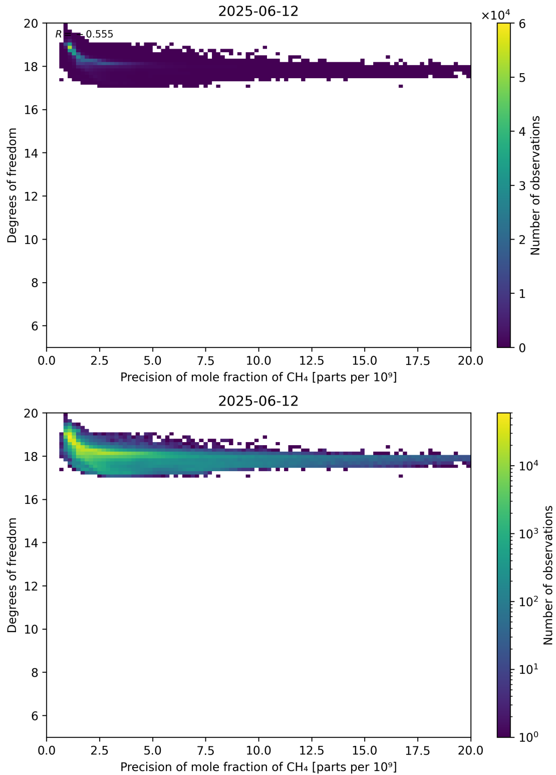
Figure 80: Scatter density plot of “Precision of mole fraction of CH 4 ” against “Degrees of freedom” for 2025-06-11 to 2025-06-13.
