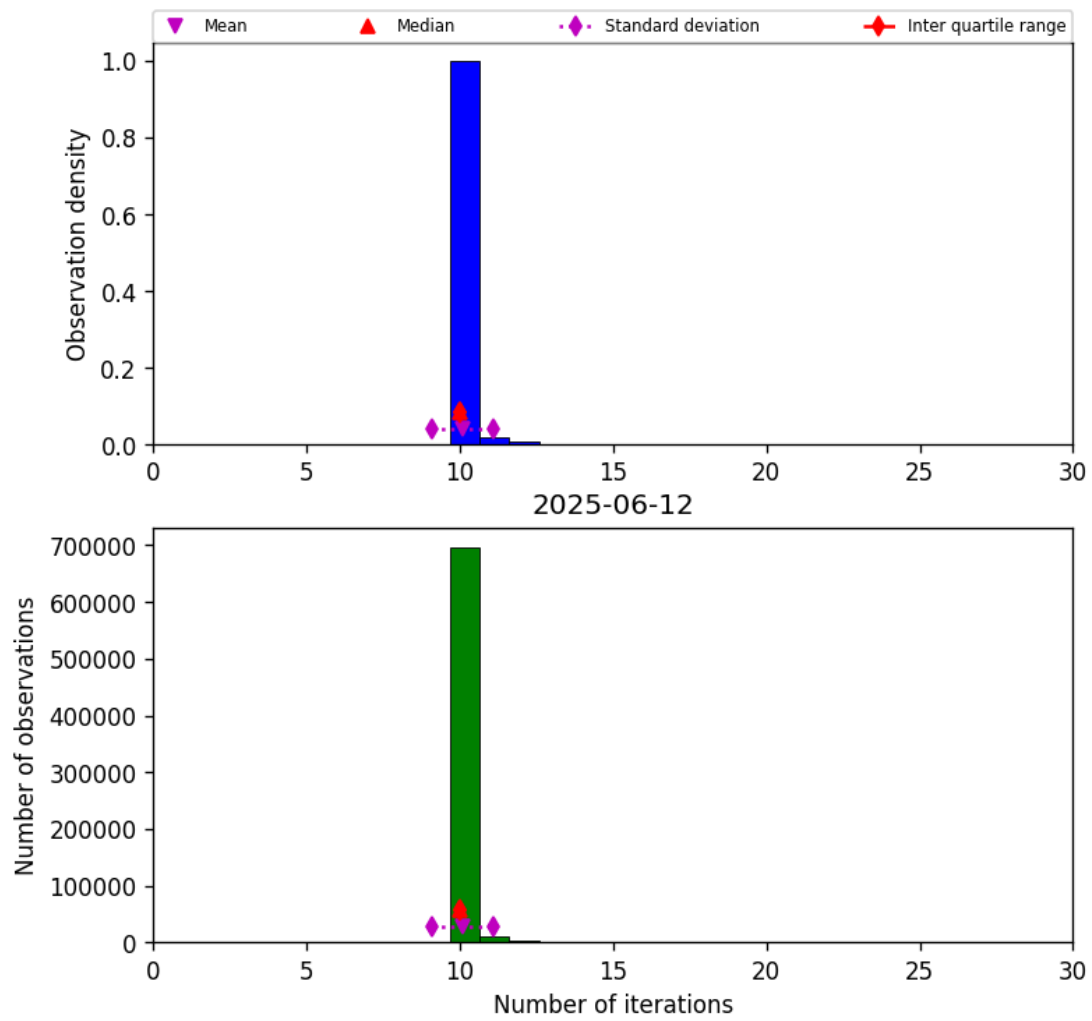
Figure 31: Histogram of “Number of iterations” for 2025-06-11 to 2025-06-13
