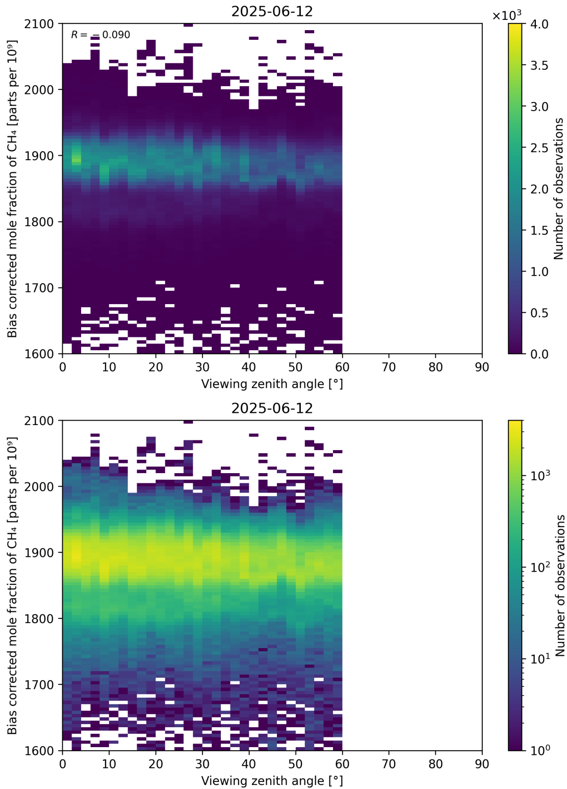
Figure 111: Scatter density plot of “Viewing zenith angle” against “Bias corrected mole fraction of CH 4 ” for 2025-06-11 to 2025-06-13.
