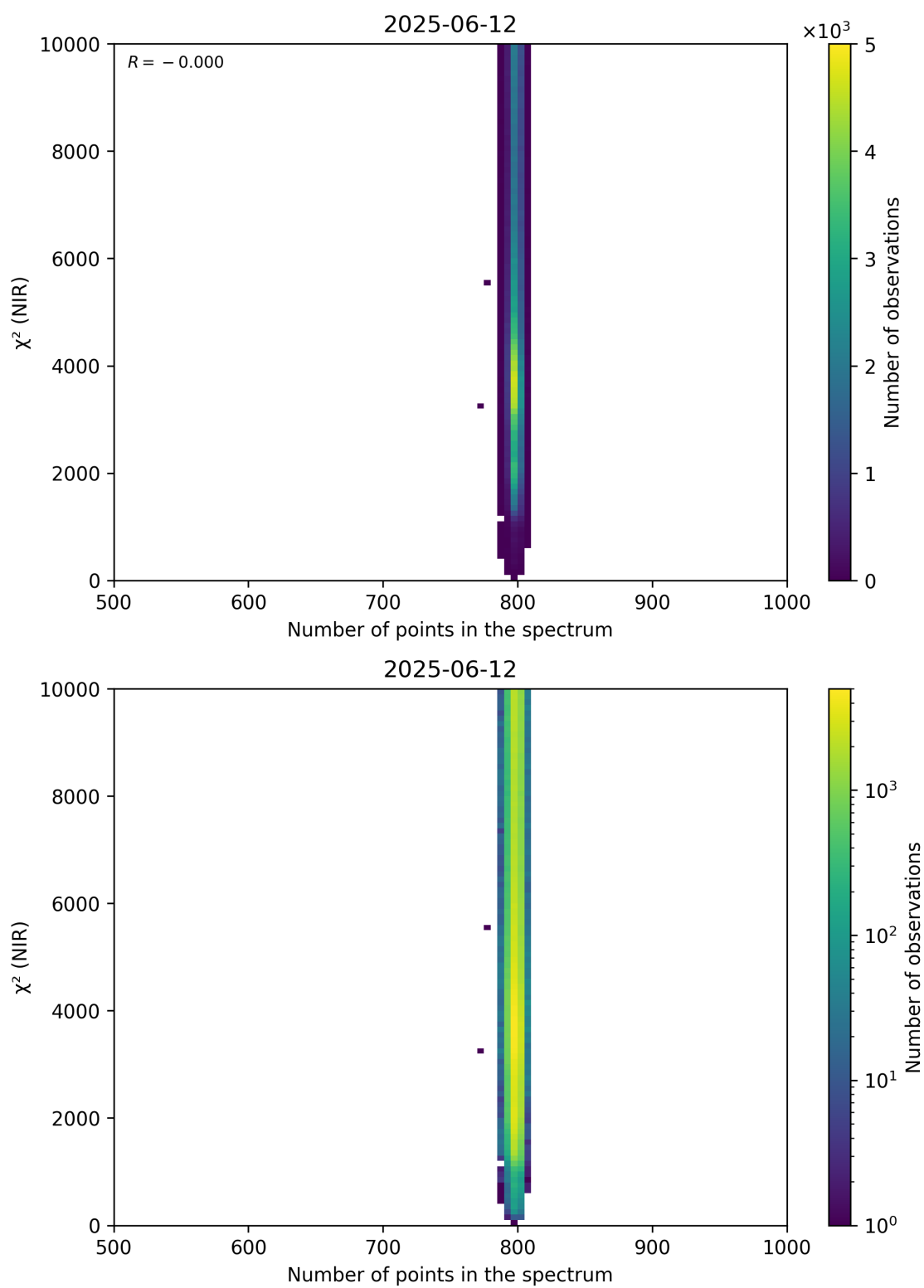
Figure 88: Scatter density plot of “Number of points in the spectrum” against “ \chi^2 (NIR)” for 2025-06-11 to 2025-06-13.
