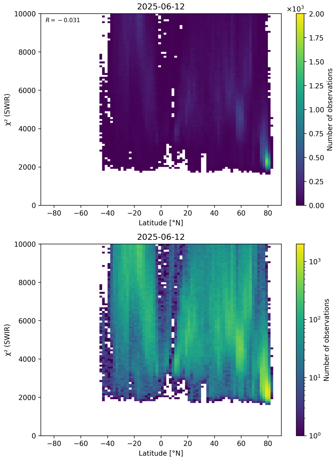
Figure 54: Scatter density plot of “Latitude” against “ \chi^2 (SWIR)” for 2025-06-11 to 2025-06-13.
