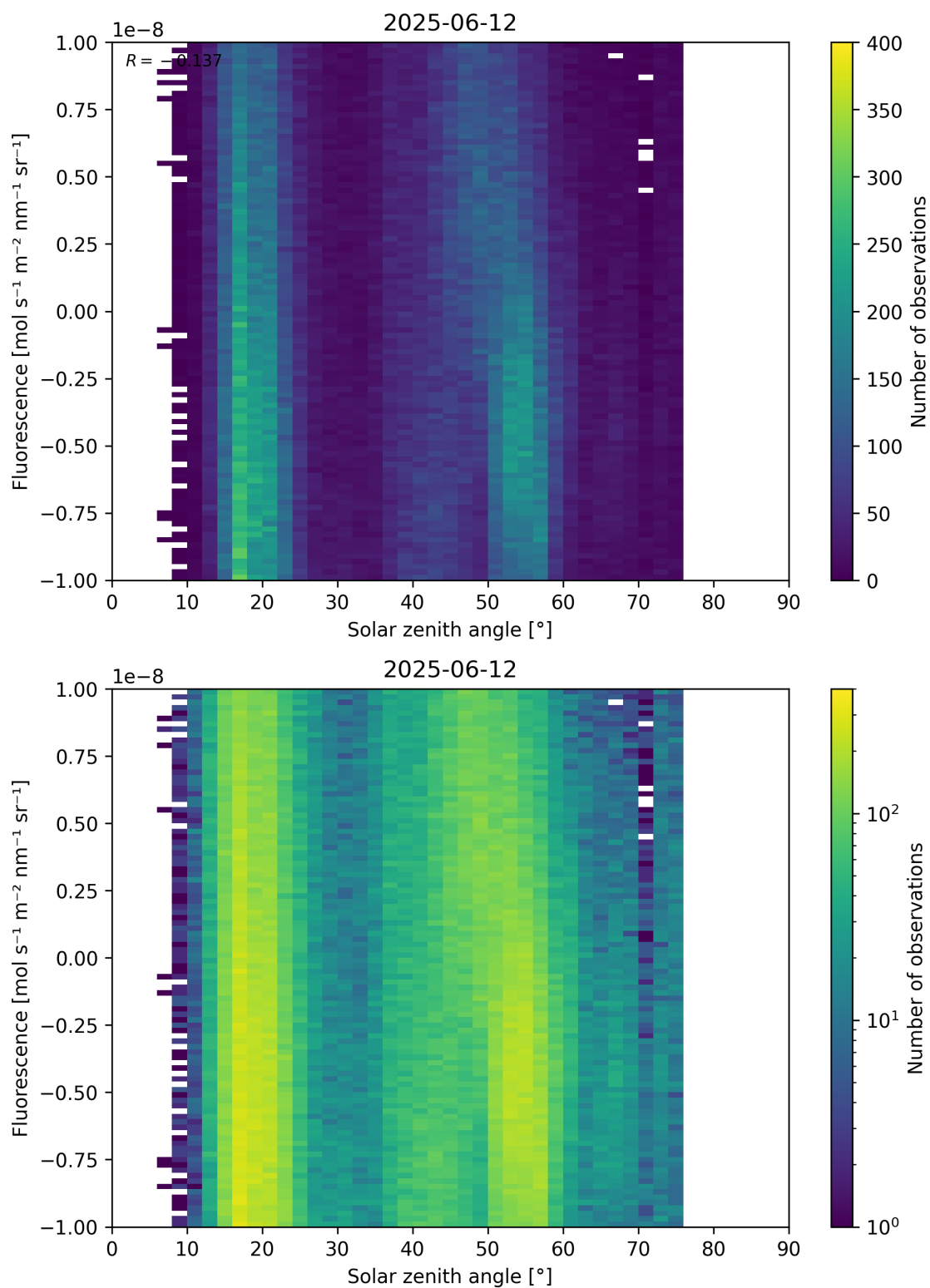
Figure 97: Scatter density plot of “Solar zenith angle” against “Fluorescence” for 2025-06-11 to 2025-06-13.
