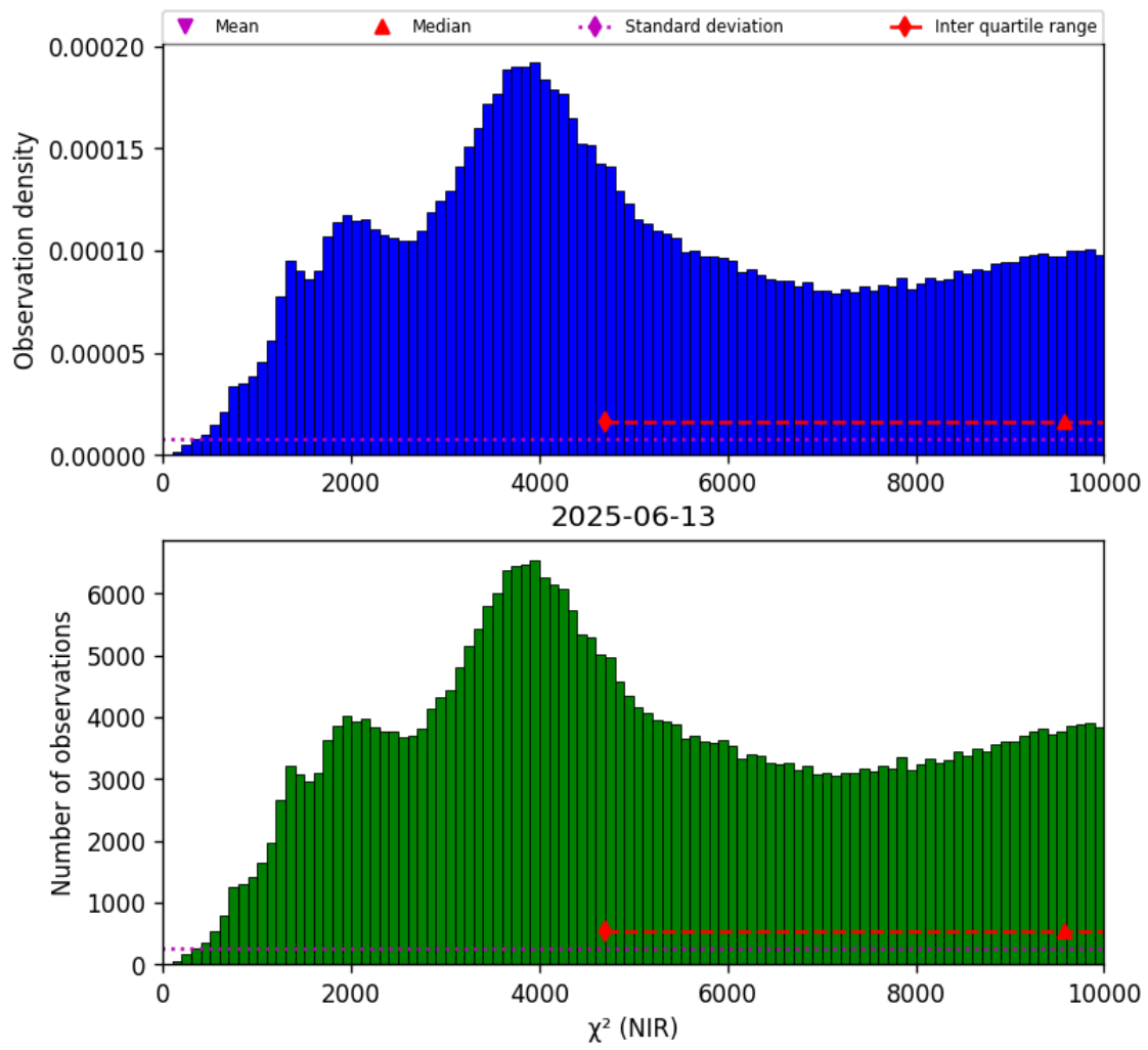
Figure 29: Histogram of “ \chi^2 (NIR)” for 2025-06-12 to 2025-06-14
