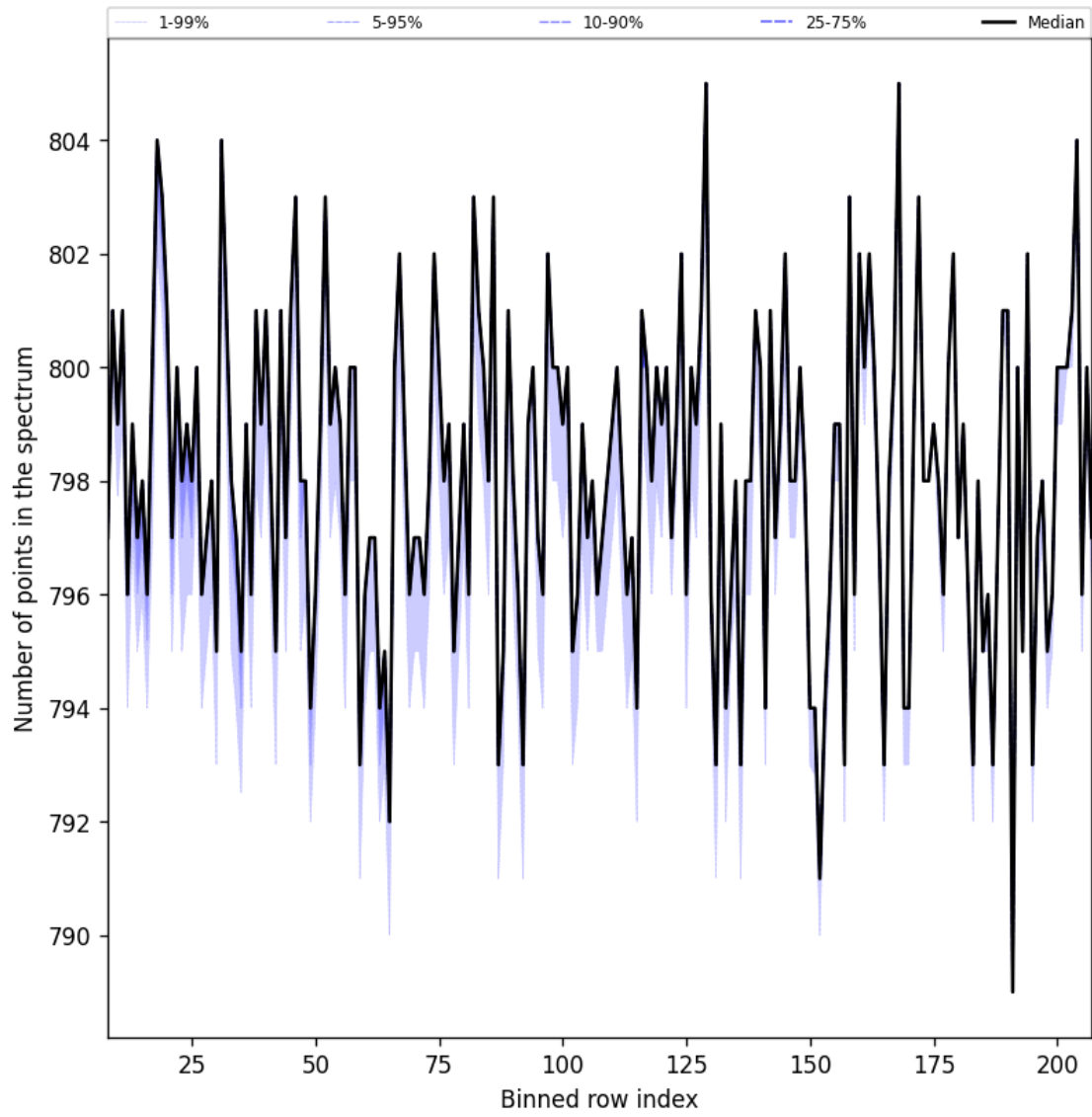
Figure 37: Along track statistics of “Number of points in the spectrum” for 2025-06-12 to 2025-06-14
