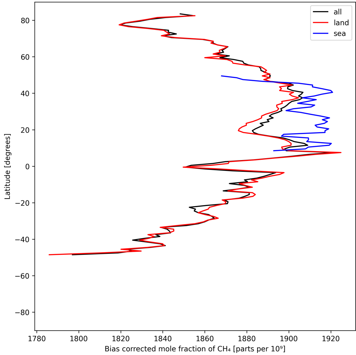
Figure 14: Zonal average of “Bias corrected mole fraction of \text{CH}_4 ” for 2025-06-12 to 2025-06-14.
