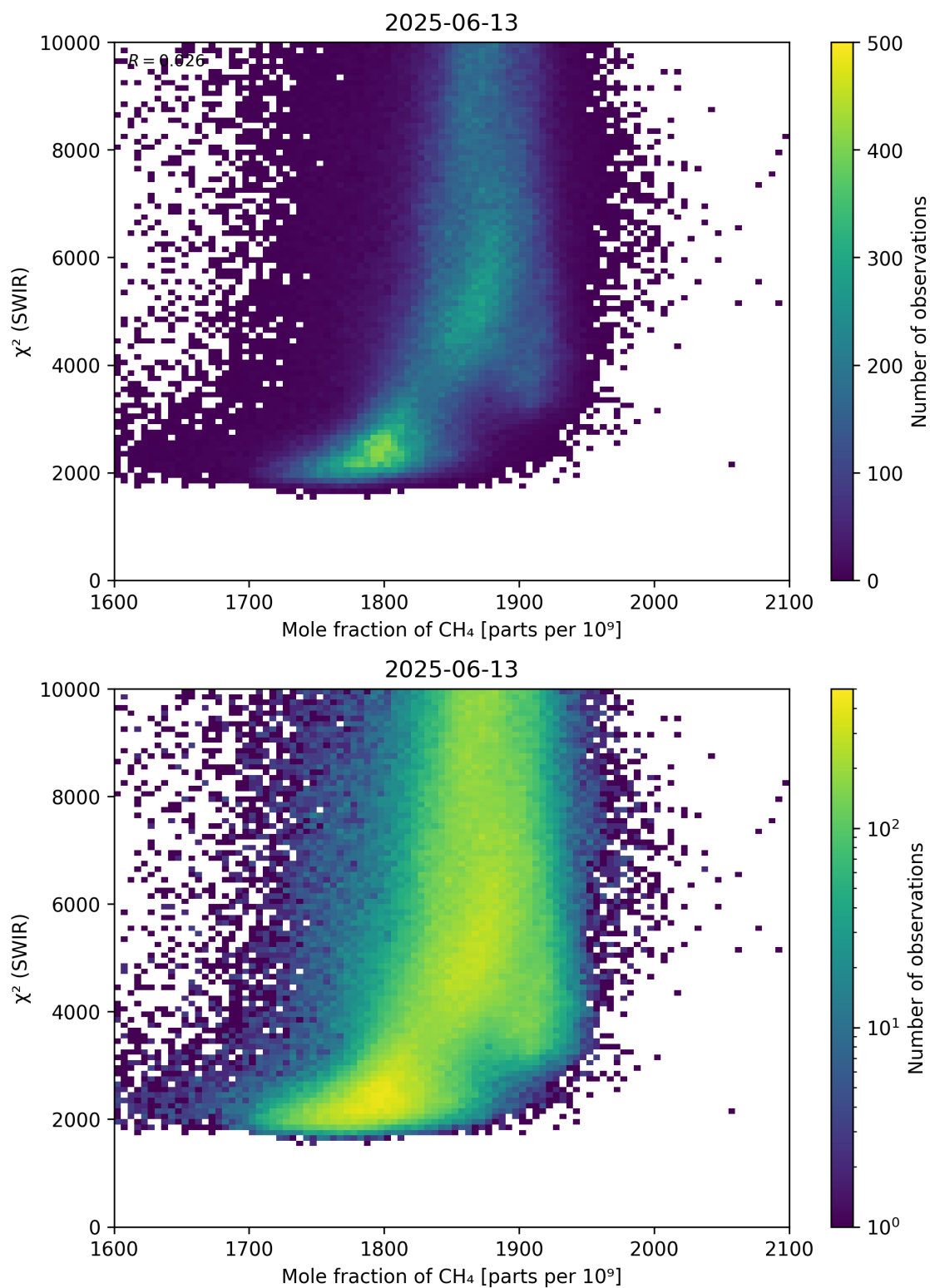
Figure 71: Scatter density plot of “Mole fraction of \text{CH}_4 ” against “ \chi^2 (SWIR)” for 2025-06-12 to 2025-06-14.
