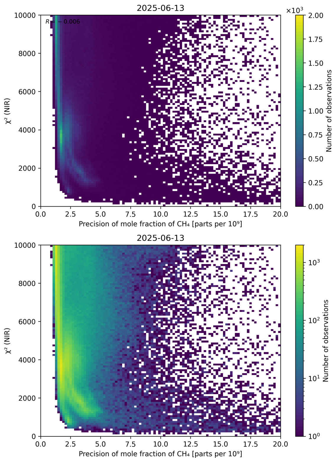
Figure 78: Scatter density plot of “Precision of mole fraction of \text{CH}_4 ” against “ \chi^2 (NIR)” for 2025-06-12 to 2025-06-14.
