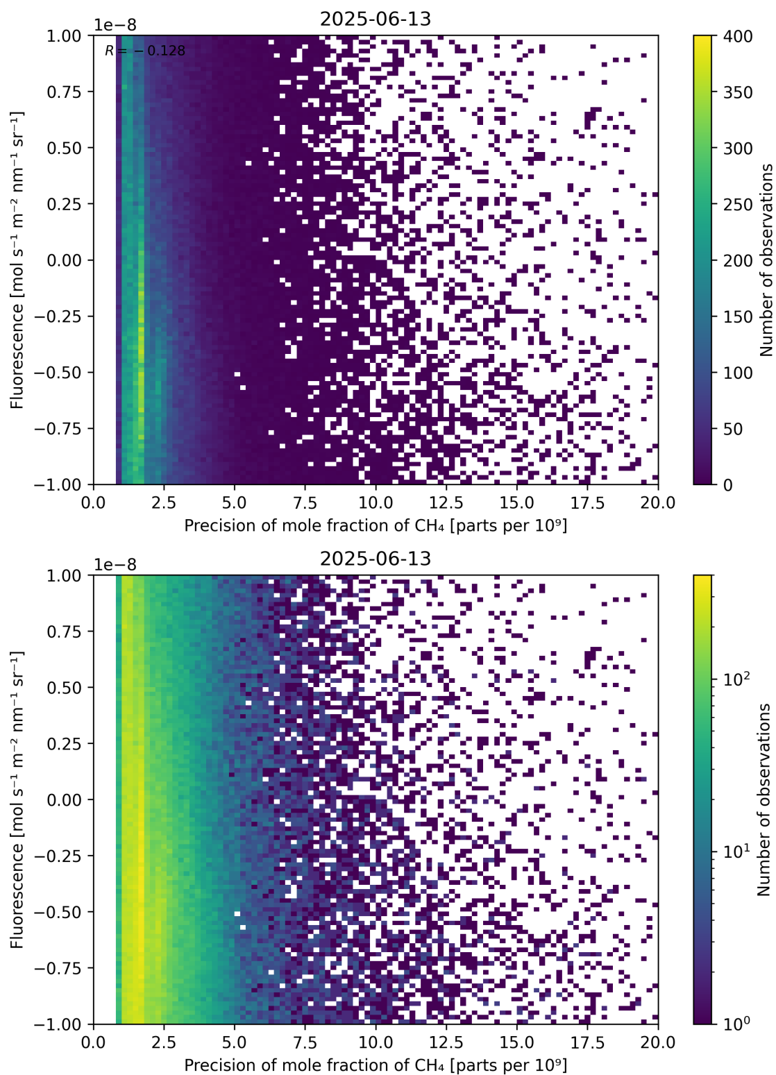
Figure 81: Scatter density plot of “Precision of mole fraction of CH 4 ” against “Fluorescence” for 2025-06-12 to 2025-06-14.
