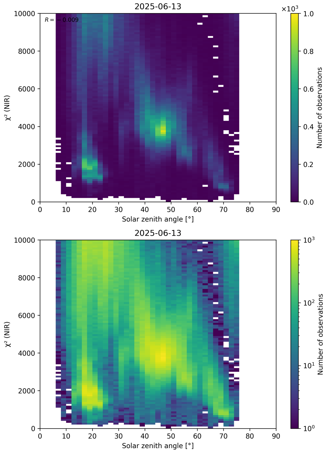
Figure 94: Scatter density plot of “Solar zenith angle” against “ \chi^2 (NIR)” for 2025-06-12 to 2025-06-14.
