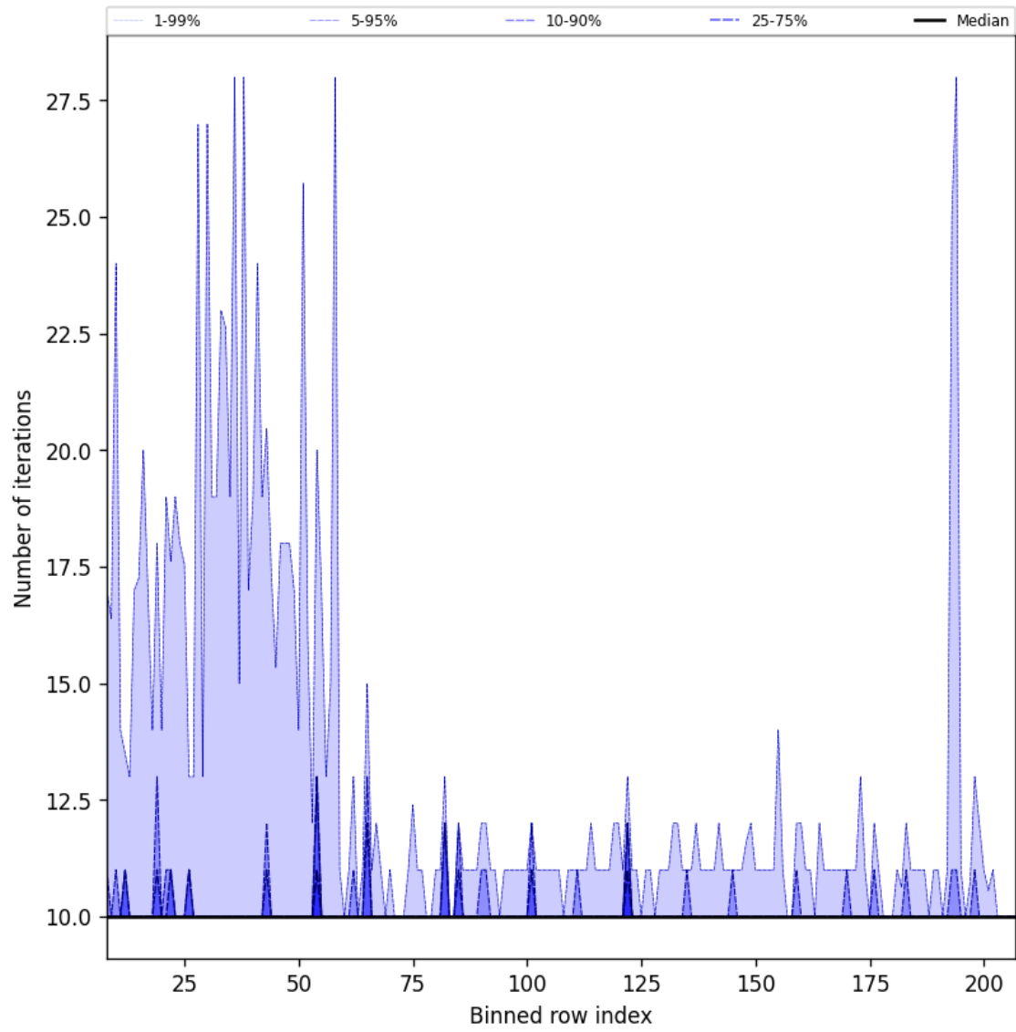
Figure 42: Along track statistics of “Number of iterations” for 2025-06-12 to 2025-06-14
