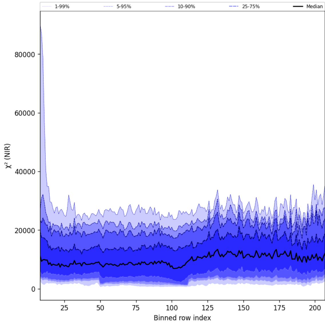
Figure 40: Along track statistics of “ \chi^2 (NIR)” for 2025-06-12 to 2025-06-14
