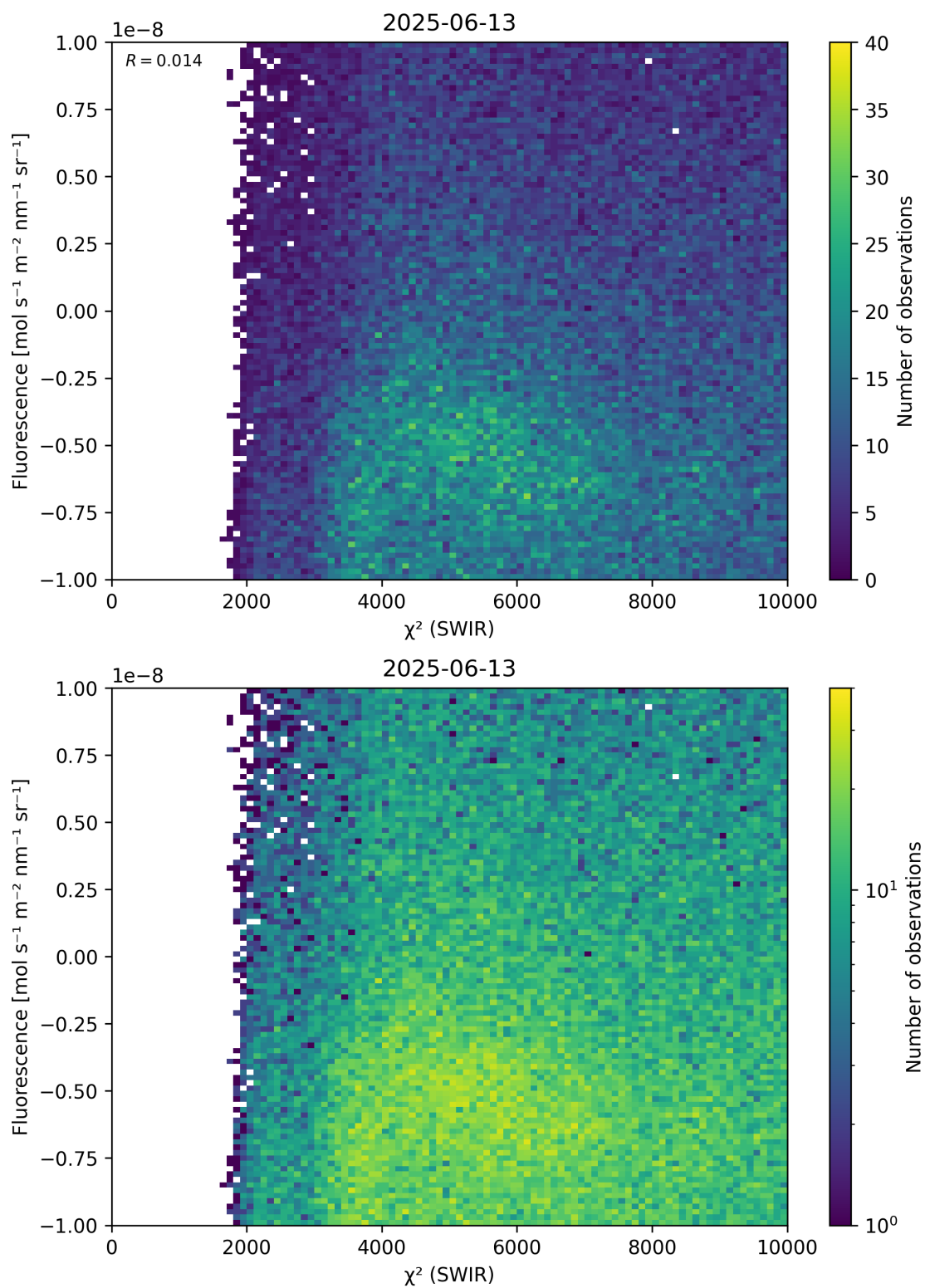
Figure 49: Scatter density plot of “ \chi^2 (SWIR)” against “Fluorescence” for 2025-06-12 to 2025-06-14.
