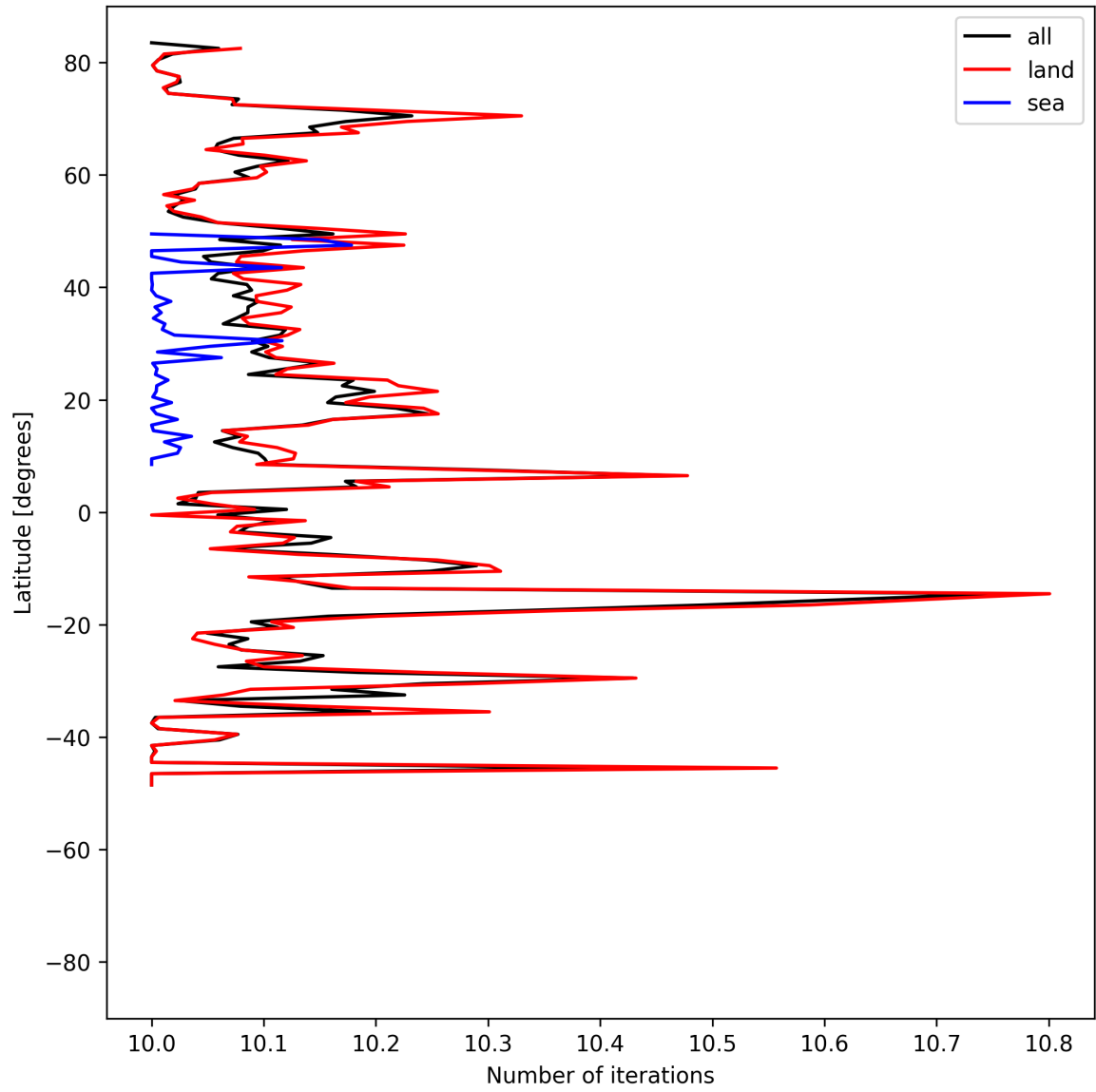
Figure 20: Zonal average of “Number of iterations” for 2025-06-12 to 2025-06-14.
