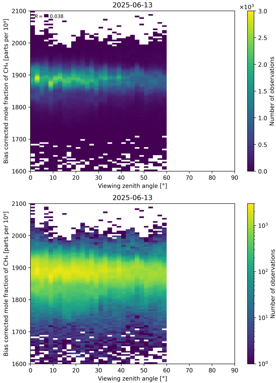
Figure 111: Scatter density plot of “Viewing zenith angle” against “Bias corrected mole fraction of CH 4 ” for 2025-06-12 to 2025-06-14.
