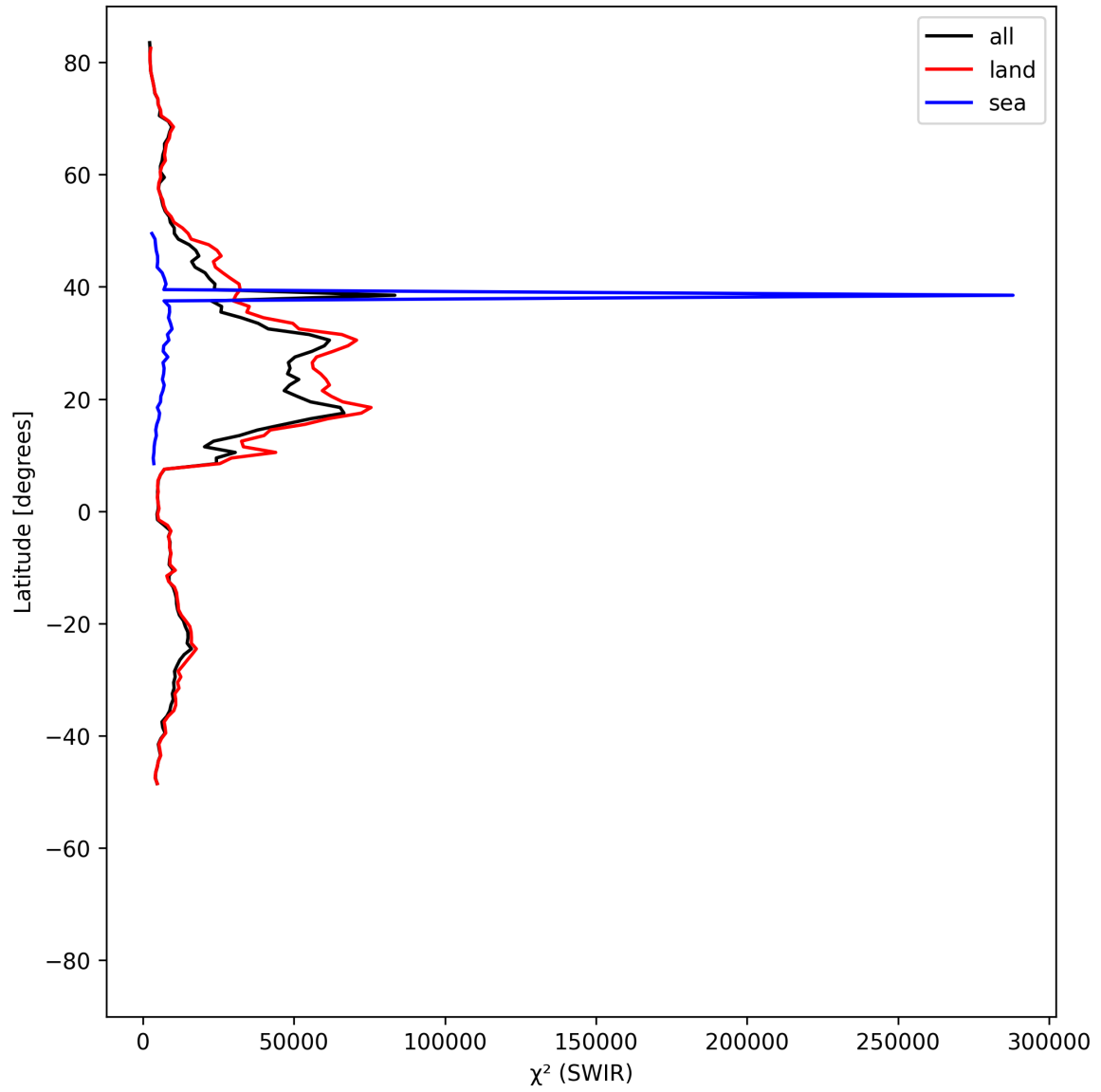
Figure 17: Zonal average of “ \chi^2 (SWIR)” for 2025-06-12 to 2025-06-14.
