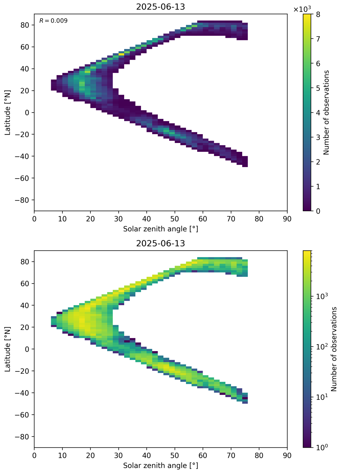
Figure 98: Scatter density plot of “Solar zenith angle” against “Latitude” for 2025-06-12 to 2025-06-14.
