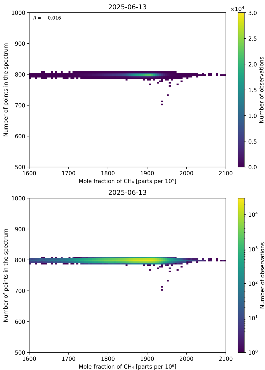
Figure 77: Scatter density plot of “Mole fraction of CH 4 ” against “Number of points in the spectrum” for 2025-06-12 to 2025-06-14.
