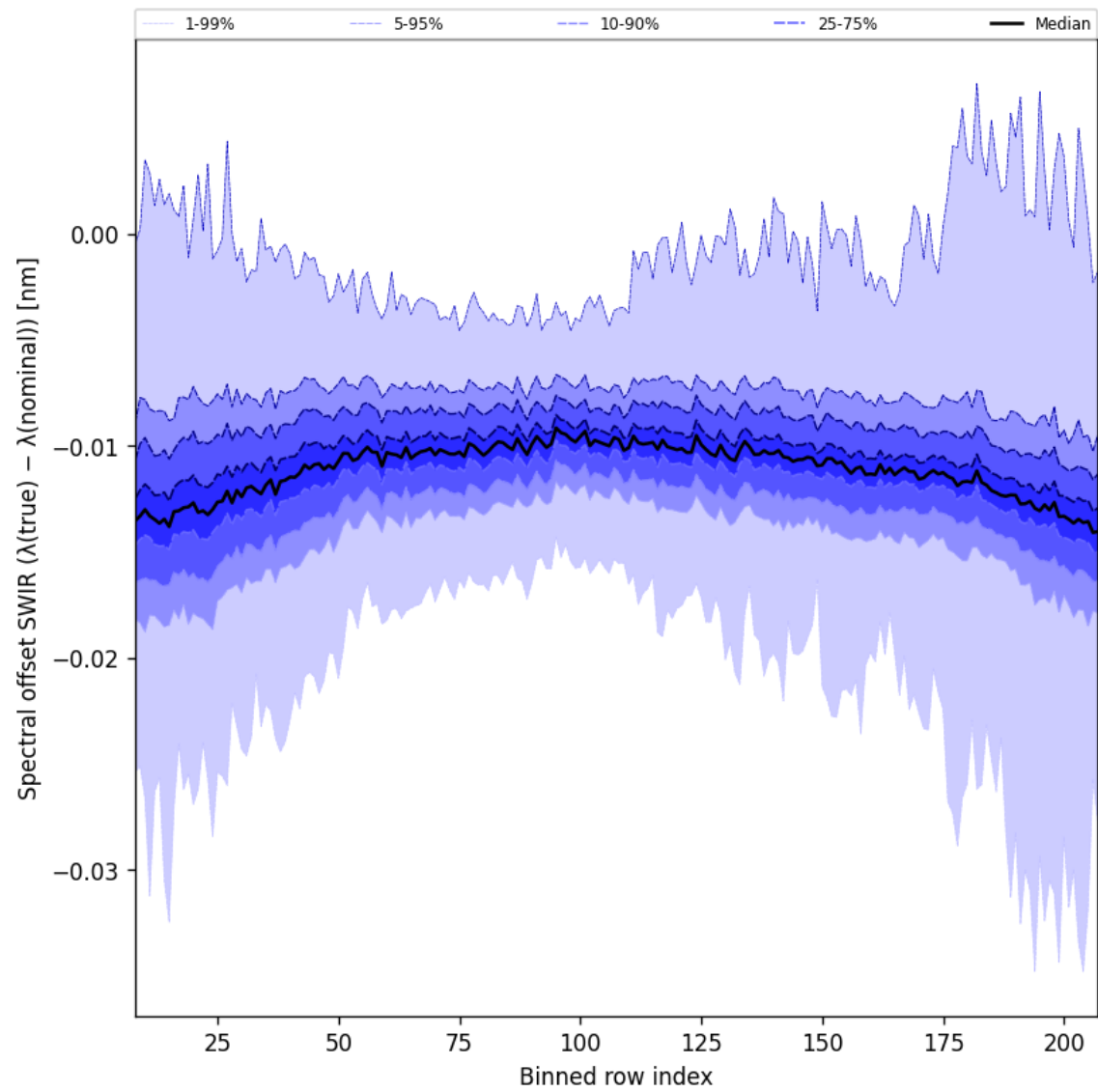
Figure 38: Along track statistics of “Spectral offset SWIR ( \lambda_{\text{true}} - \lambda_{\text{nominal}} )” for 2025-06-12 to 2025-06-14
