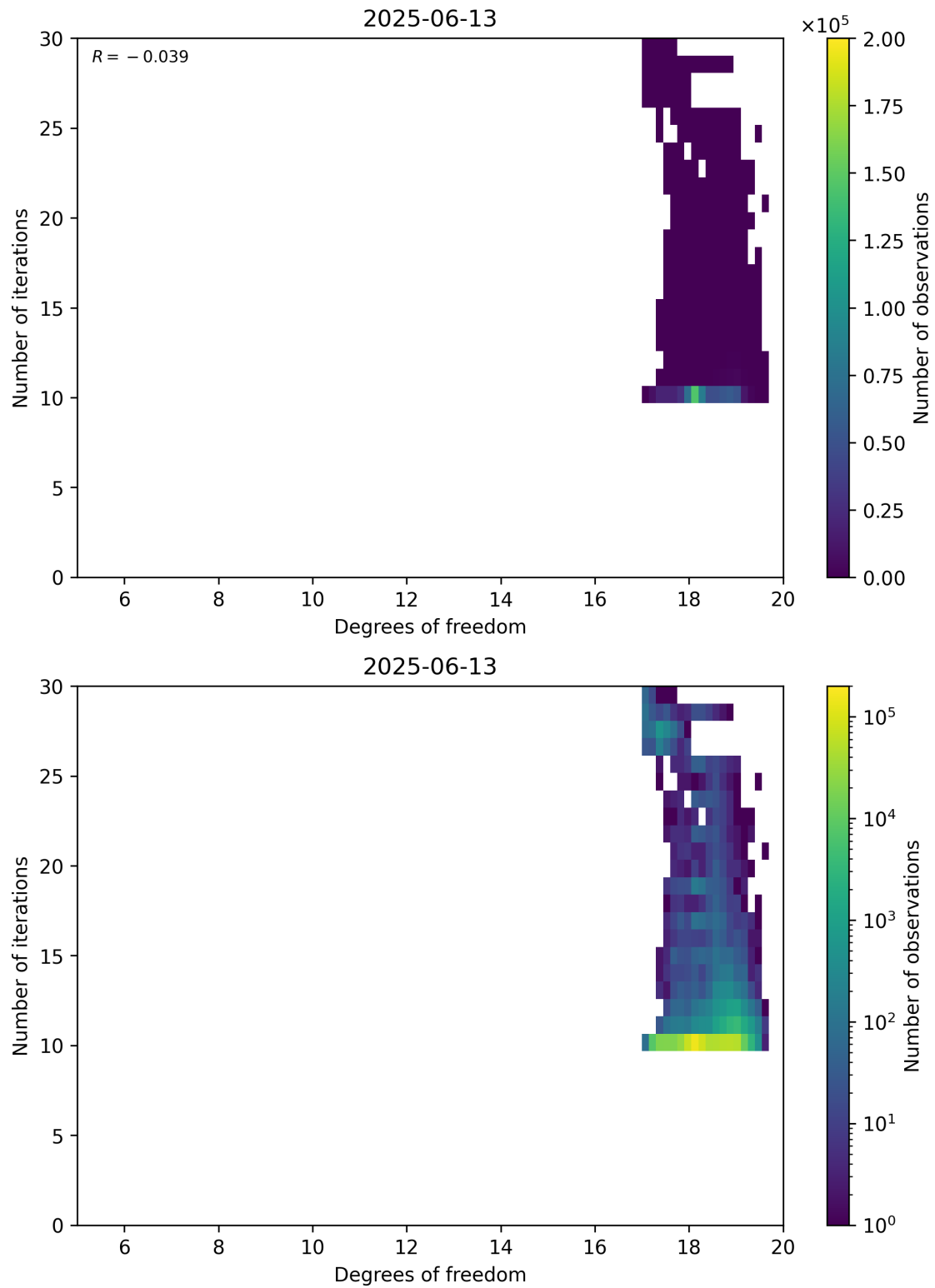
Figure 52: Scatter density plot of “Degrees of freedom” against “Number of iterations” for 2025-06-12 to 2025-06-14.
