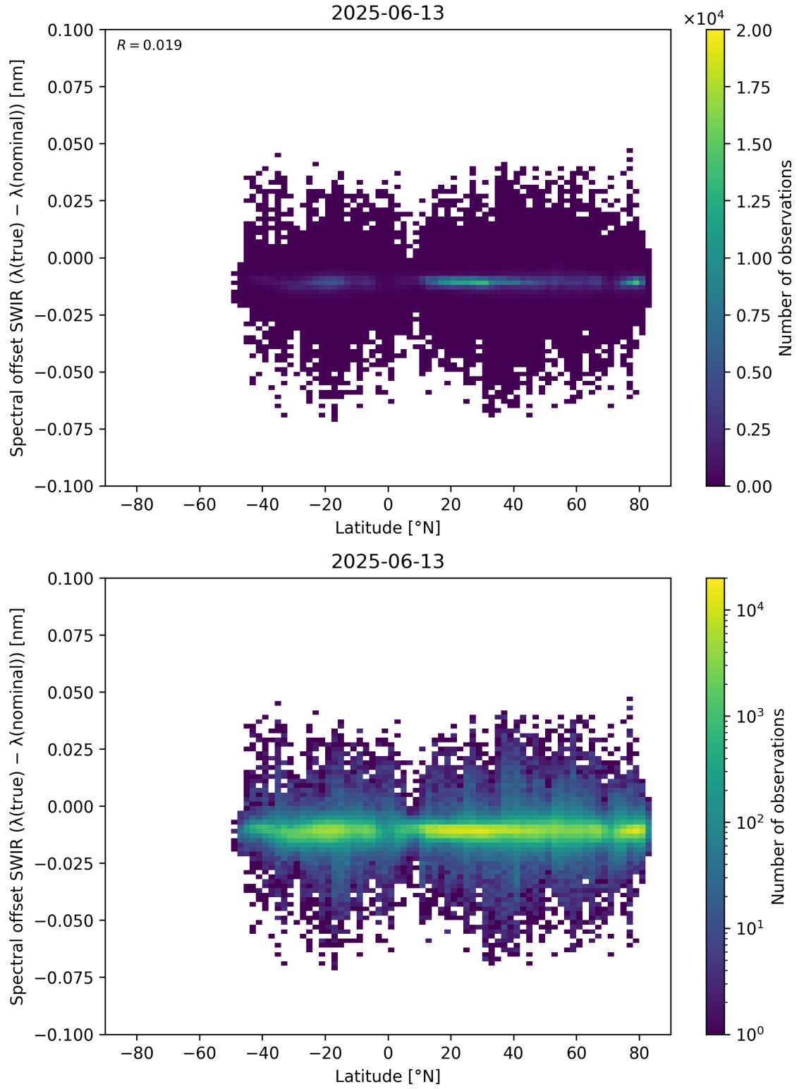
Figure 62: Scatter density plot of “Latitude” against “Spectral offset SWIR ( \lambda_{\text{true}} - \lambda_{\text{nominal}} )” for 2025-06-12 to 2025-06-14.
