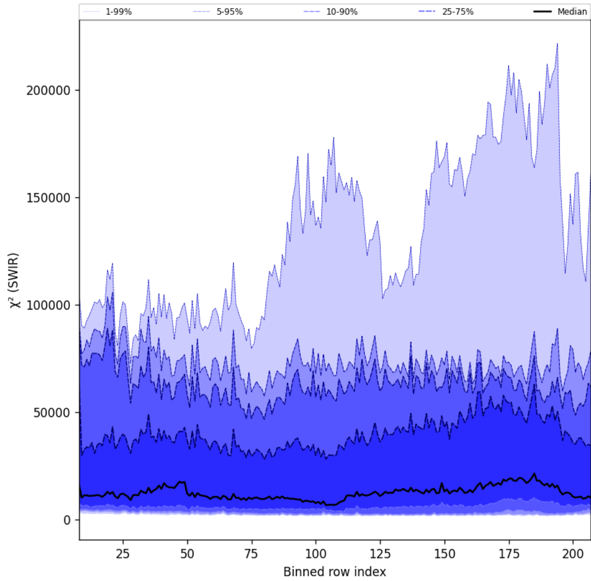
Figure 39: Along track statistics of “ \chi^2 (SWIR)” for 2025-06-12 to 2025-06-14
