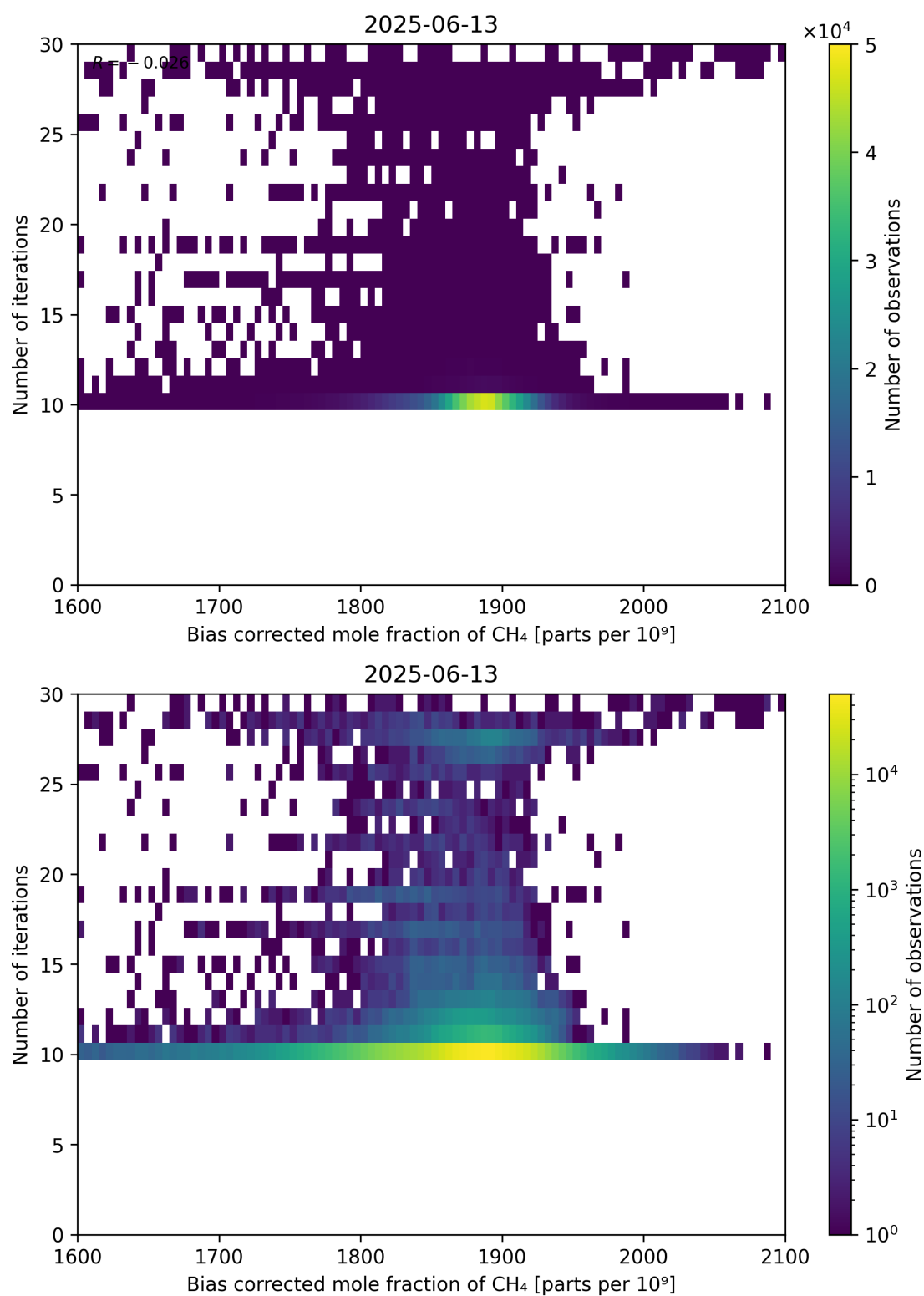
Figure 67: Scatter density plot of “Bias corrected mole fraction of CH 4 ” against “Number of iterations” for 2025-06-12 to 2025-06-14.
