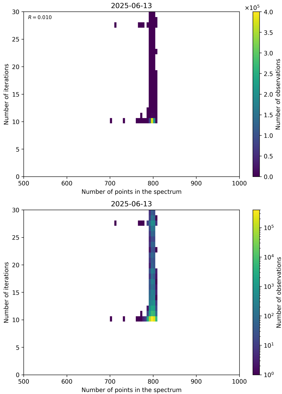
Figure 92: Scatter density plot of “Number of points in the spectrum” against “Number of iterations” for 2025-06-12 to 2025-06-14.
