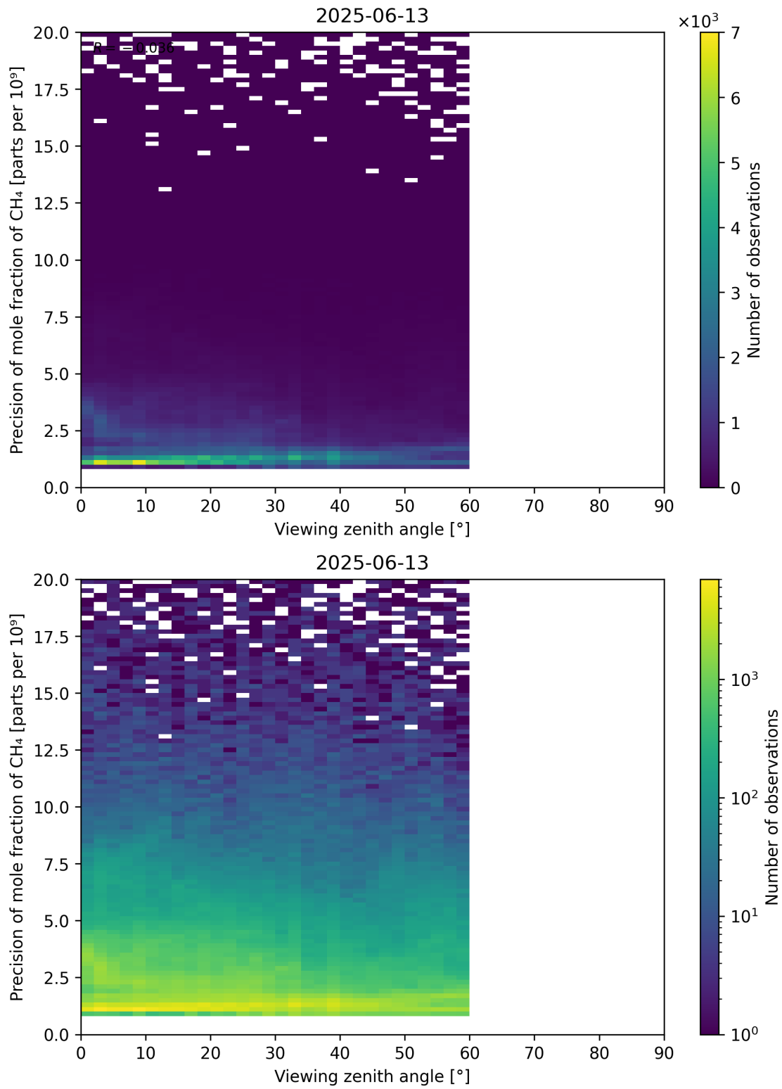
Figure 112: Scatter density plot of “Viewing zenith angle” against “Precision of mole fraction of CH 4 ” for 2025-06-12 to 2025-06-14.
