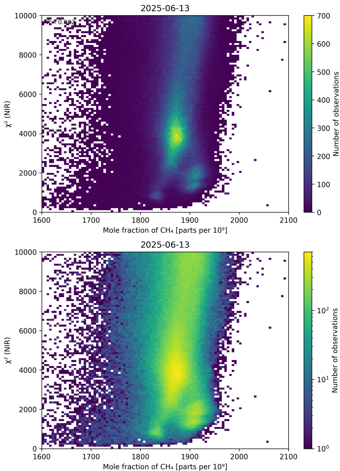
Figure 70: Scatter density plot of “Mole fraction of \text{CH}_4 ” against “ \chi^2 (NIR)” for 2025-06-12 to 2025-06-14.
