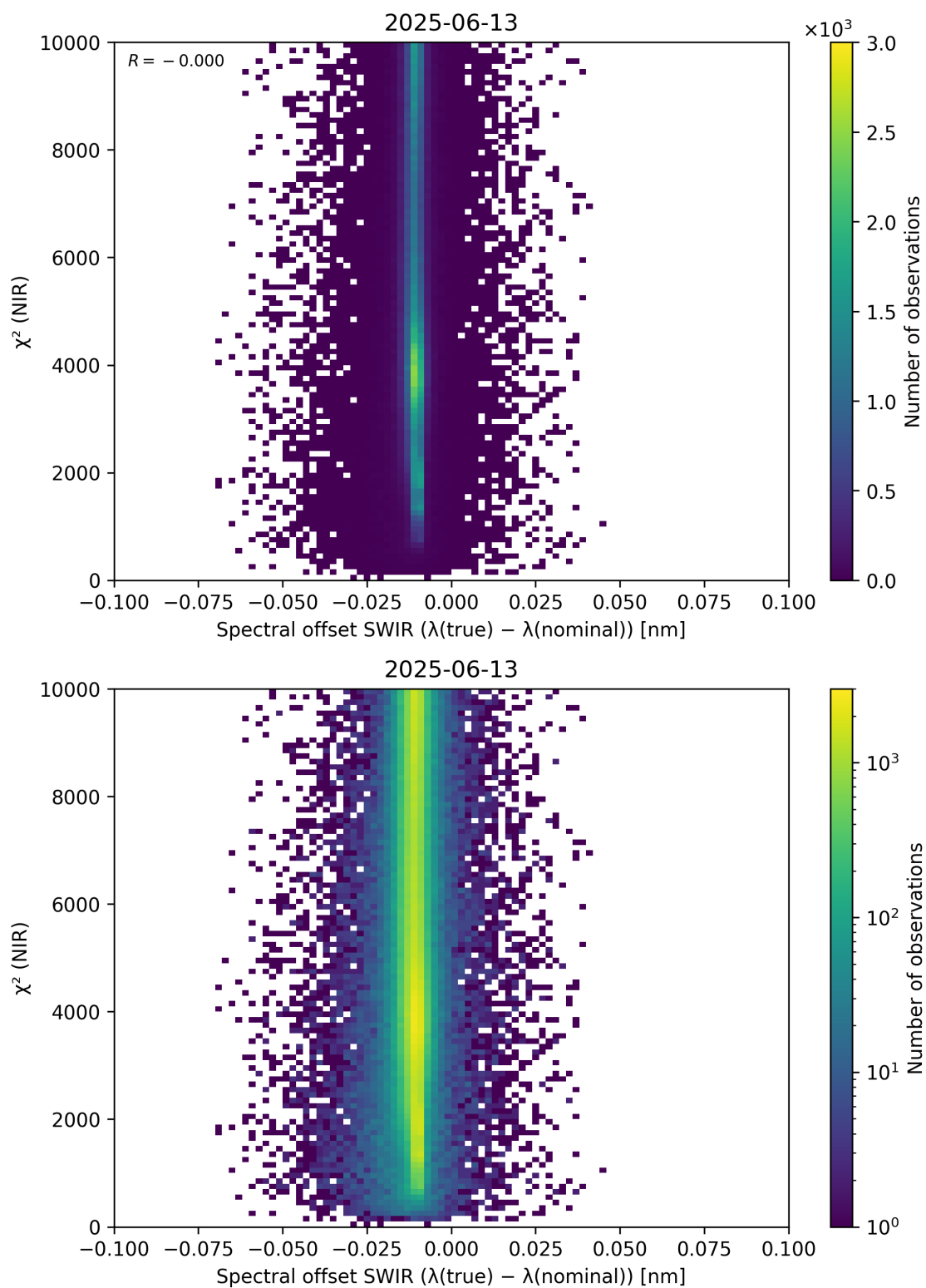
Figure 117: Scatter density plot of “Spectral offset SWIR ( \lambda_{\text{true}} - \lambda_{\text{nominal}} )” against “ \chi^2 (NIR)” for 2025-06-12 to 2025-06-14.
