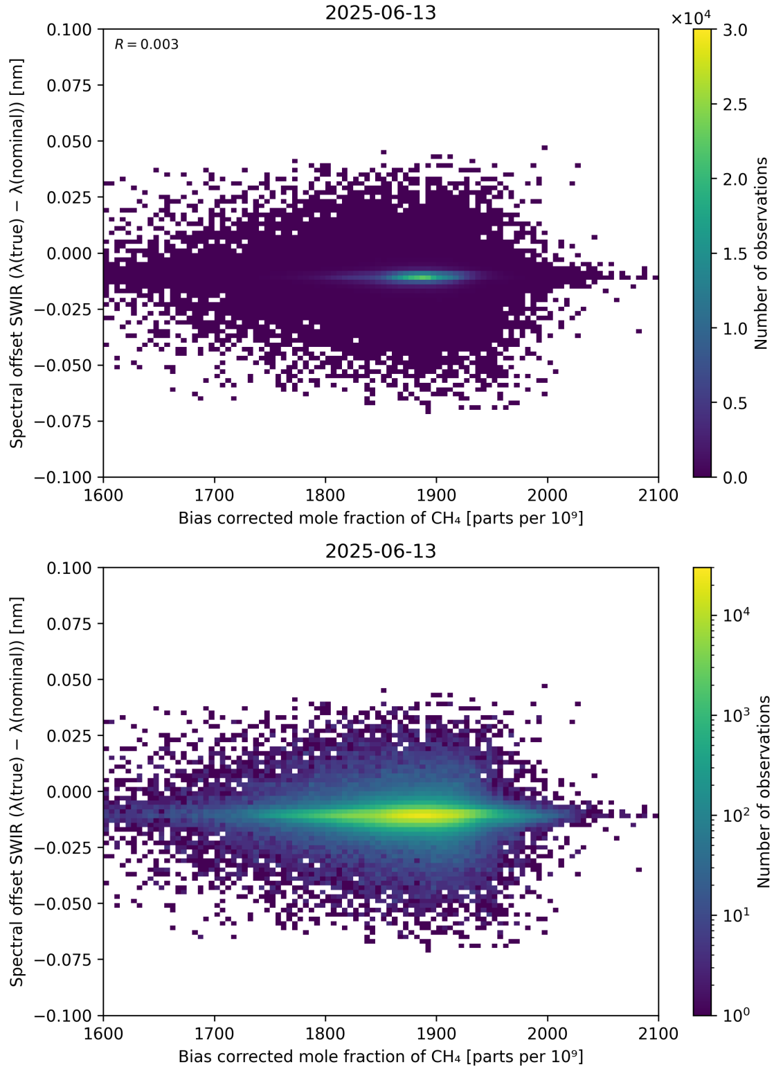
Figure 69: Scatter density plot of “Bias corrected mole fraction of \text{CH}_4 ” against “Spectral offset SWIR ( \lambda_{\text{true}} - \lambda_{\text{nominal}} )” for 2025-06-12 to 2025-06-14.
