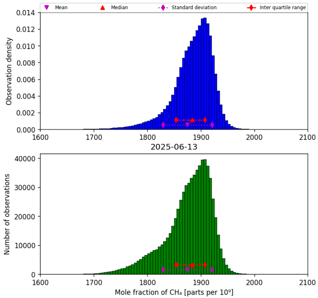
Figure 23: Histogram of “Mole fraction of CH 4 ” for 2025-06-12 to 2025-06-14
