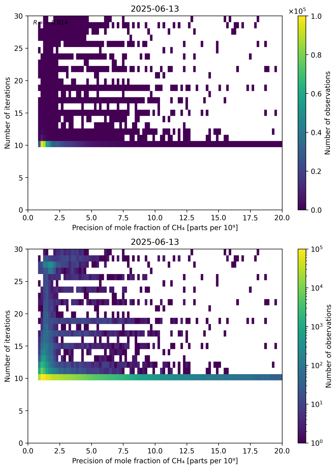
Figure 83: Scatter density plot of “Precision of mole fraction of CH 4 ” against “Number of iterations” for 2025-06-12 to 2025-06-14.
