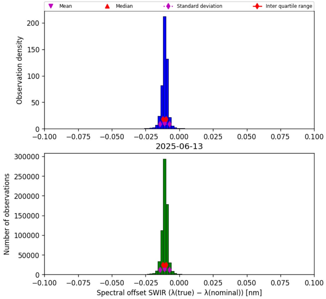
Figure 27: Histogram of “Spectral offset SWIR ( \lambda_{\text{true}} - \lambda_{\text{nominal}} )” for 2025-06-12 to 2025-06-14
