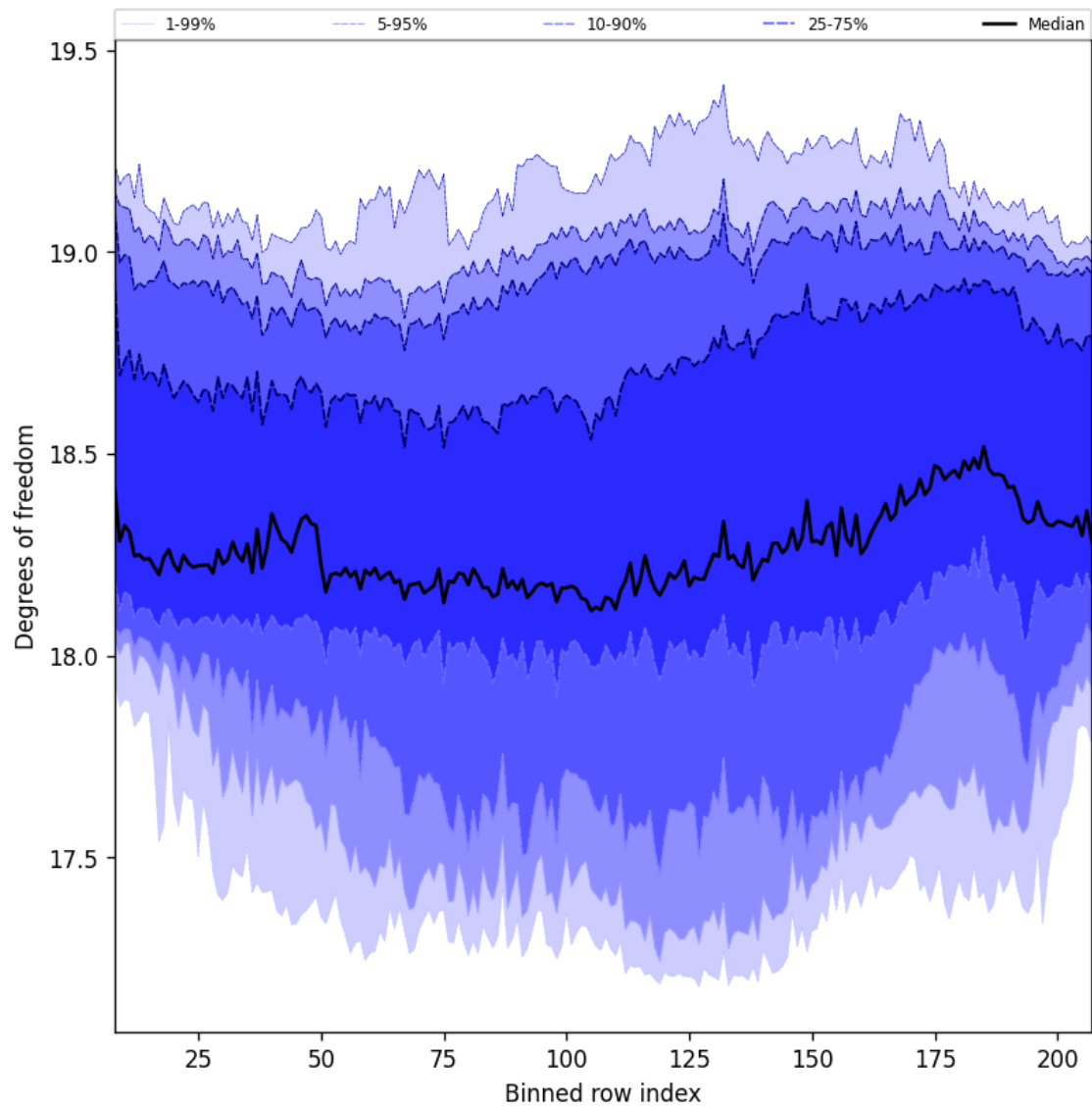
Figure 41: Along track statistics of “Degrees of freedom” for 2025-06-12 to 2025-06-14
