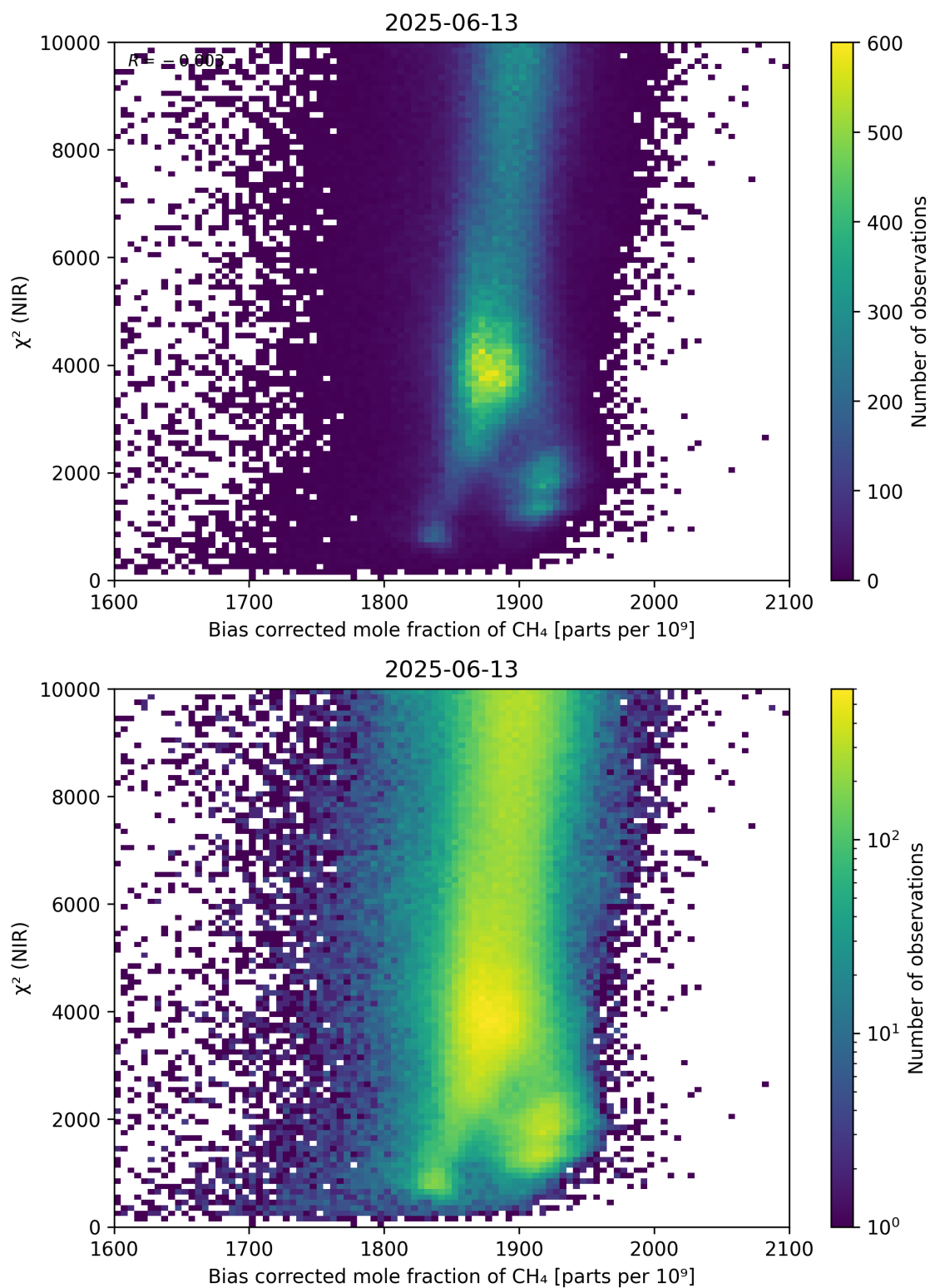
Figure 63: Scatter density plot of “Bias corrected mole fraction of \text{CH}_4 ” against “ \chi^2 (NIR)” for 2025-06-12 to 2025-06-14.
