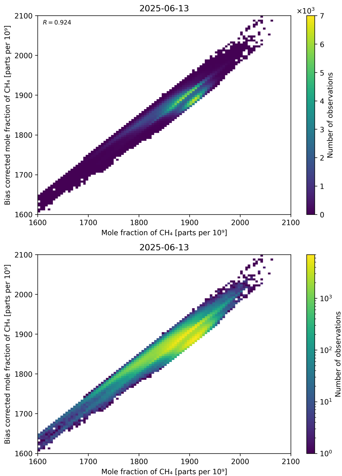
Figure 74: Scatter density plot of “Mole fraction of CH 4 ” against “Bias corrected mole fraction of CH 4 ” for 2025-06-12 to 2025-06-14.
