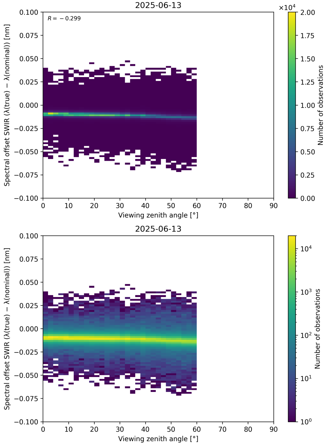
Figure 116: Scatter density plot of “Viewing zenith angle” against “Spectral offset SWIR ( \lambda_{\text{true}} - \lambda_{\text{nominal}} )” for 2025-06-12 to 2025-06-14.
