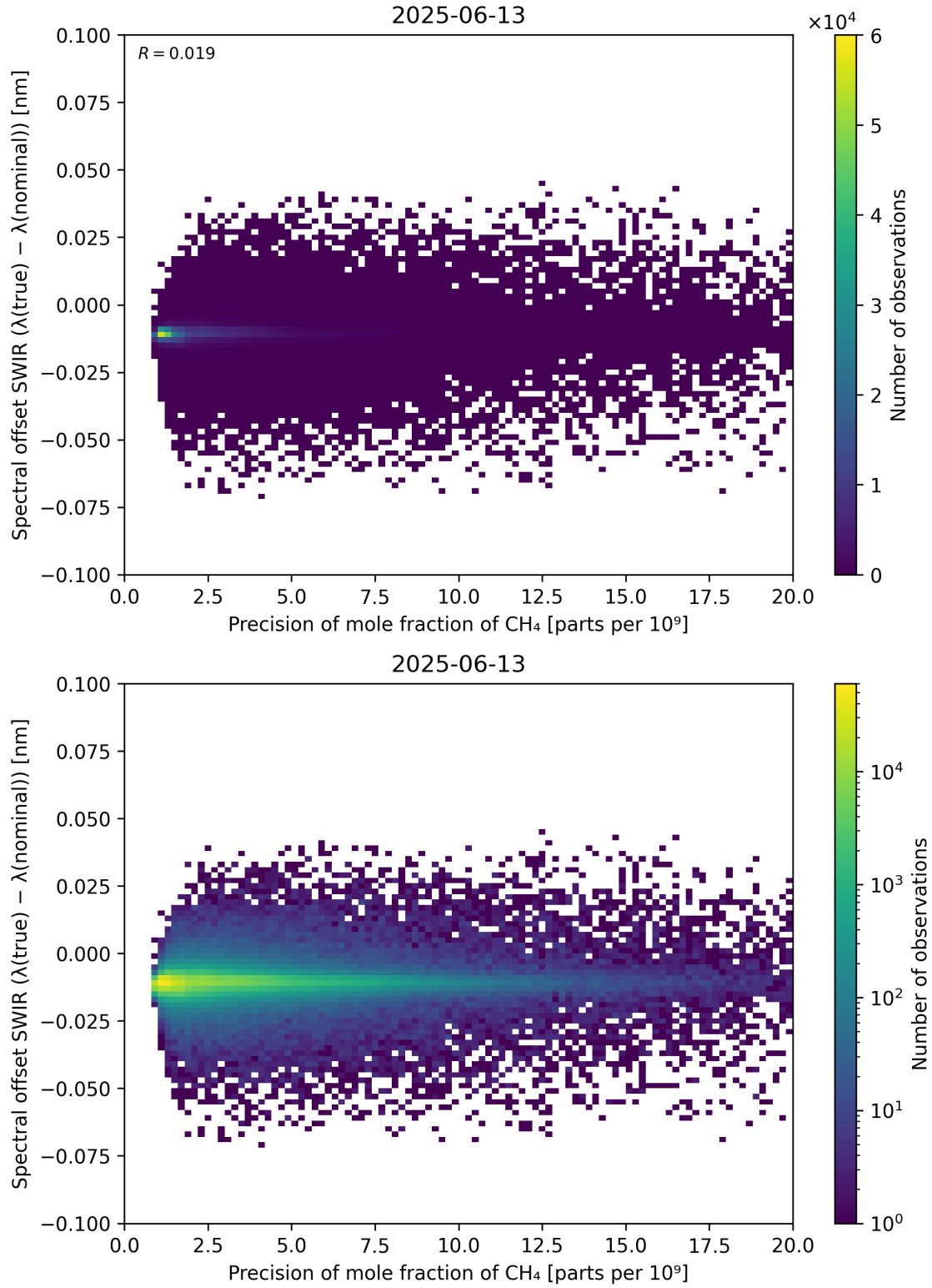
Figure 85: Scatter density plot of “Precision of mole fraction of \text{CH}_4 ” against “Spectral offset SWIR ( \lambda_{\text{true}} - \lambda_{\text{nominal}} )” for 2025-06-12 to 2025-06-14.
