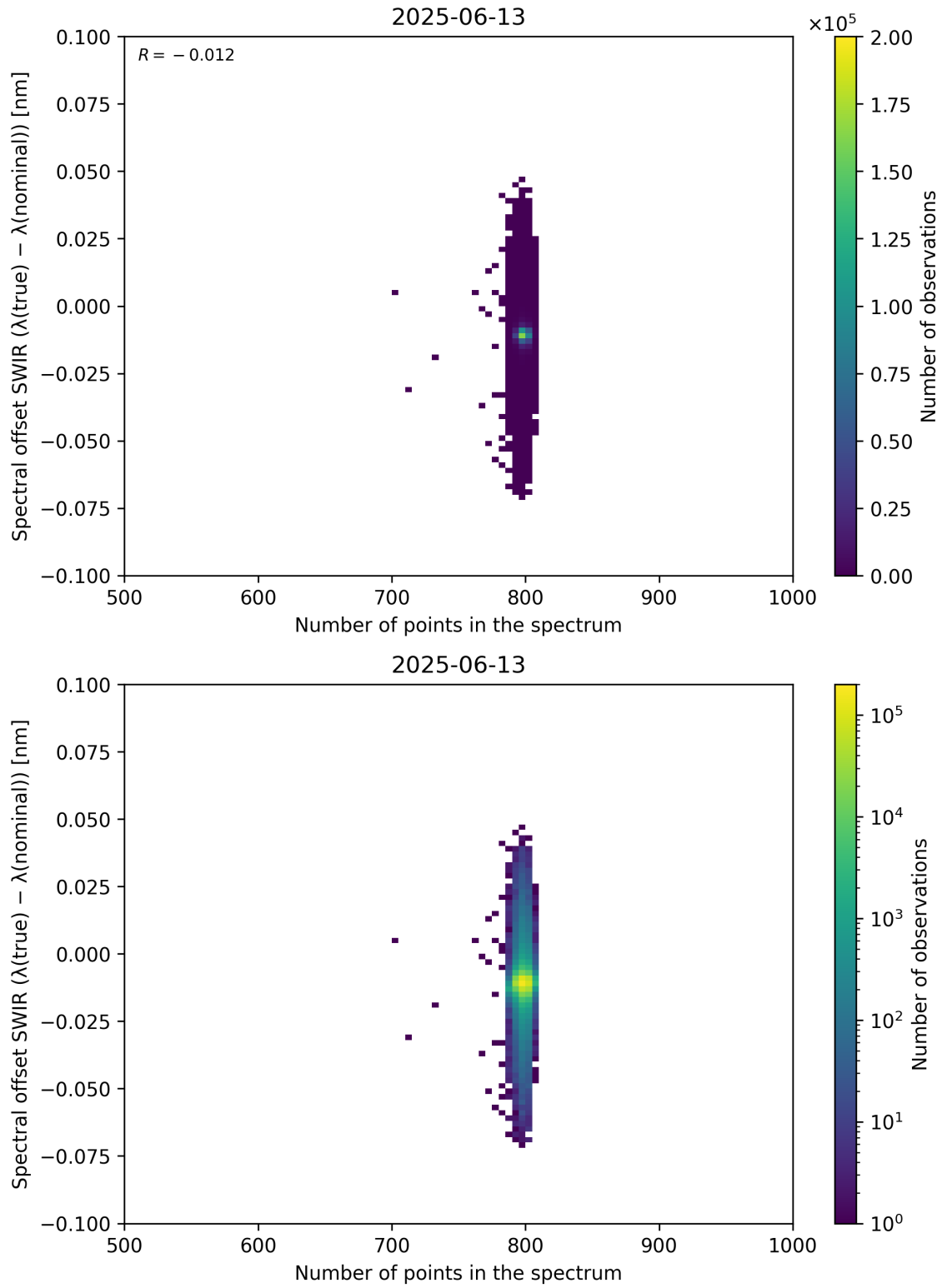
Figure 93: Scatter density plot of “Number of points in the spectrum” against “Spectral offset SWIR ( \lambda_{\text{true}} - \lambda_{\text{nominal}} )” for 2025-06-12 to 2025-06-14.
