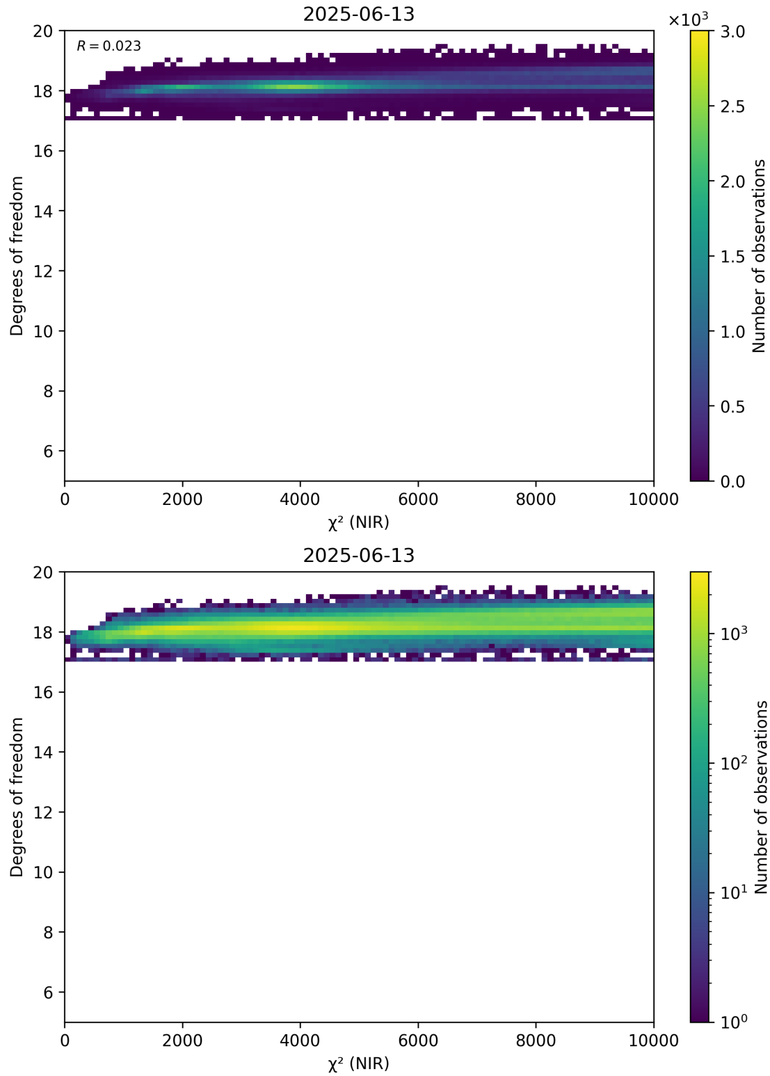
Figure 44: Scatter density plot of “ \chi^2 (NIR)” against “Degrees of freedom” for 2025-06-12 to 2025-06-14.
