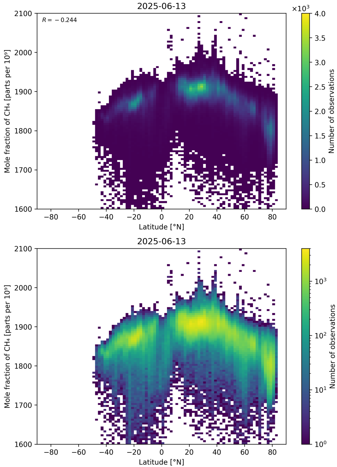
Figure 57: Scatter density plot of “Latitude” against “Mole fraction of CH 4 ” for 2025-06-12 to 2025-06-14.
