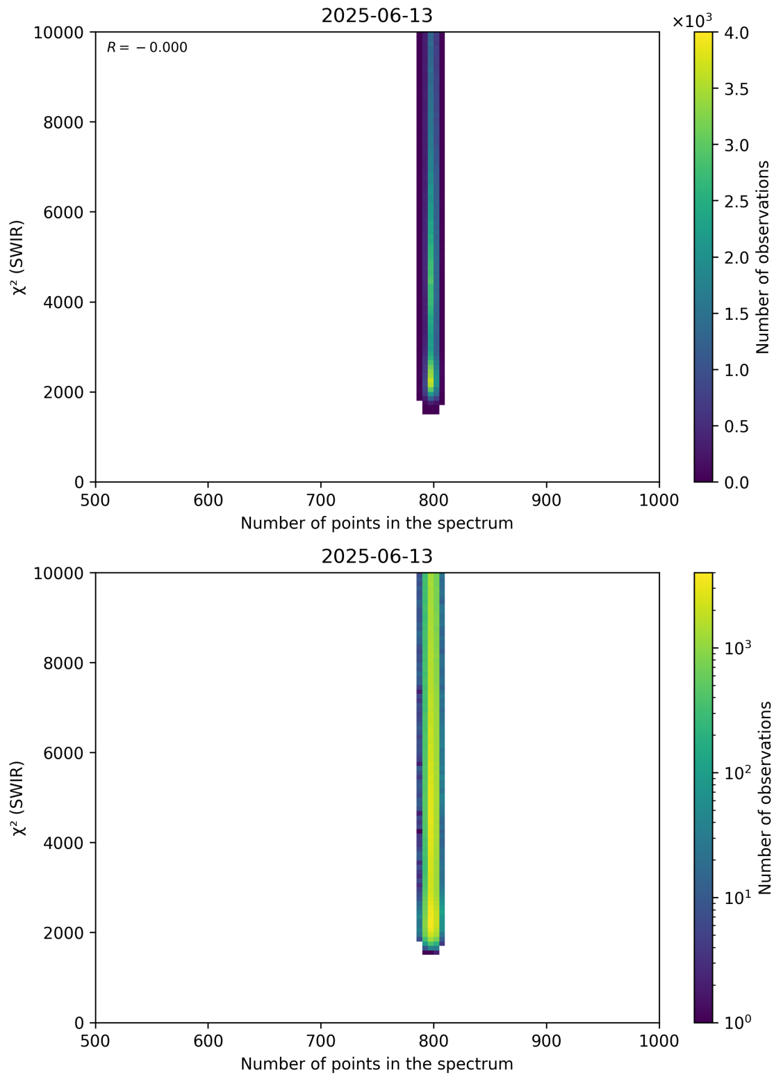
Figure 89: Scatter density plot of “Number of points in the spectrum” against “ \chi^2 (SWIR)” for 2025-06-12 to 2025-06-14.
