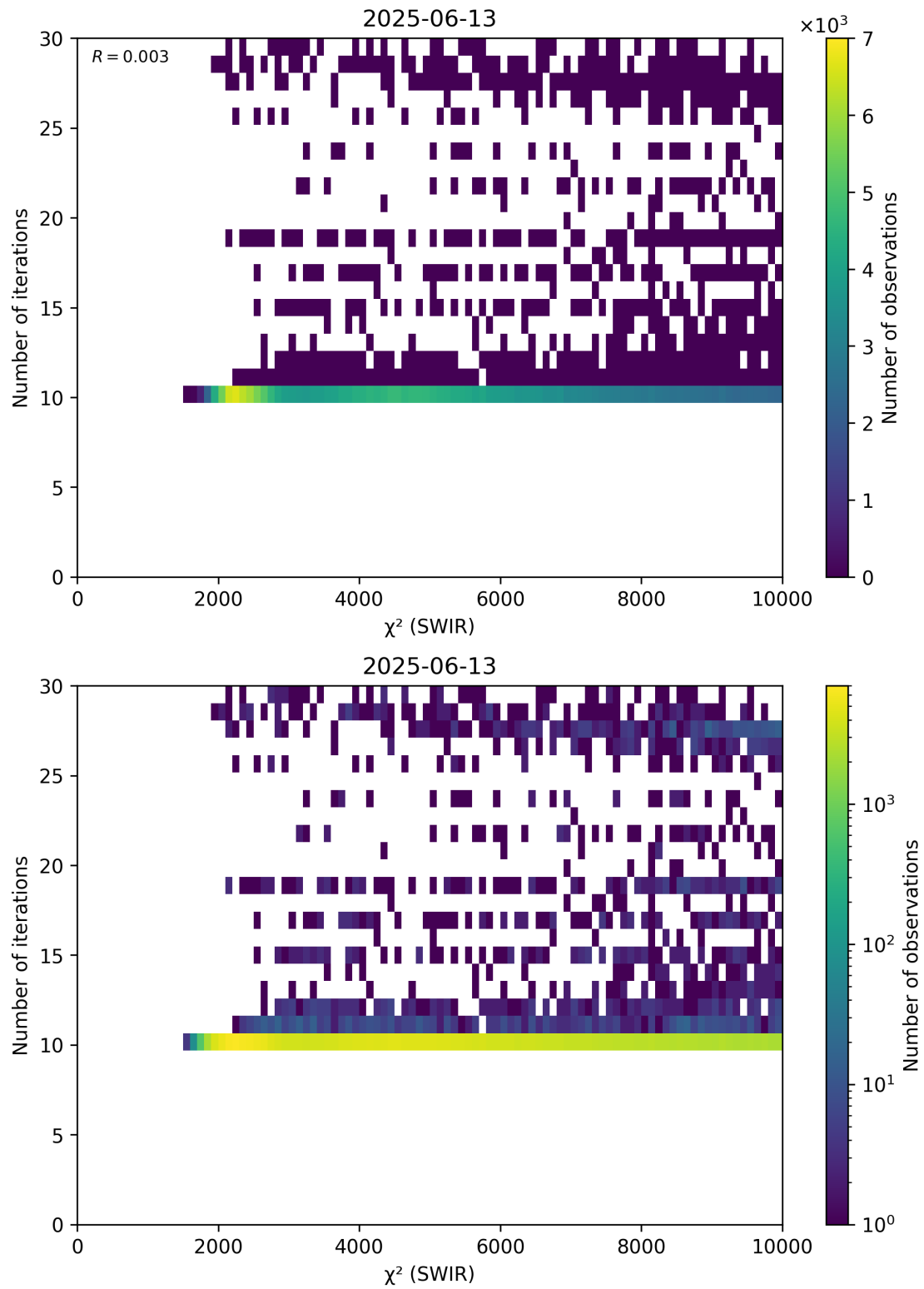
Figure 50: Scatter density plot of “ \chi^2 (SWIR)” against “Number of iterations” for 2025-06-12 to 2025-06-14.
