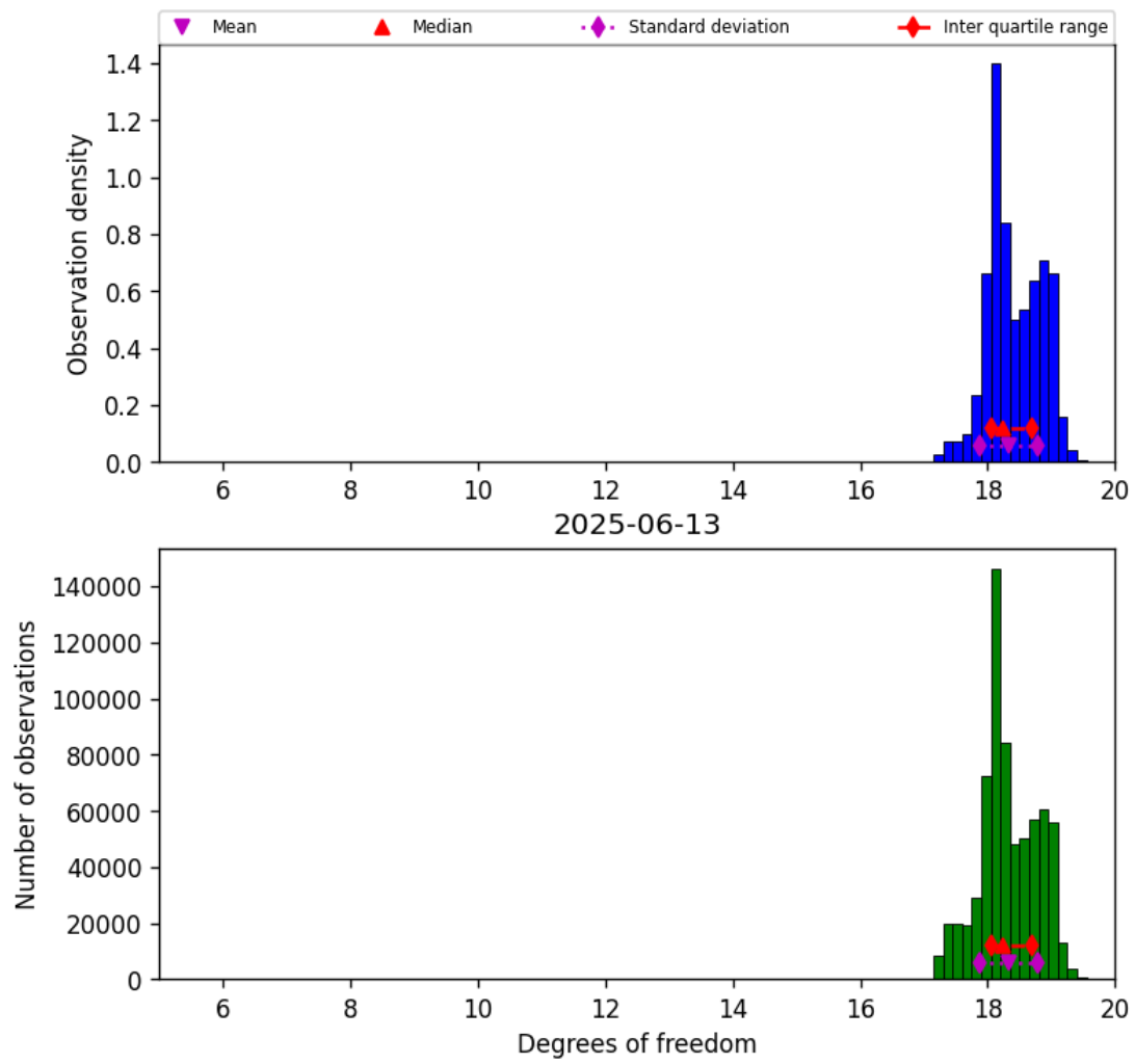
Figure 30: Histogram of “Degrees of freedom” for 2025-06-12 to 2025-06-14
