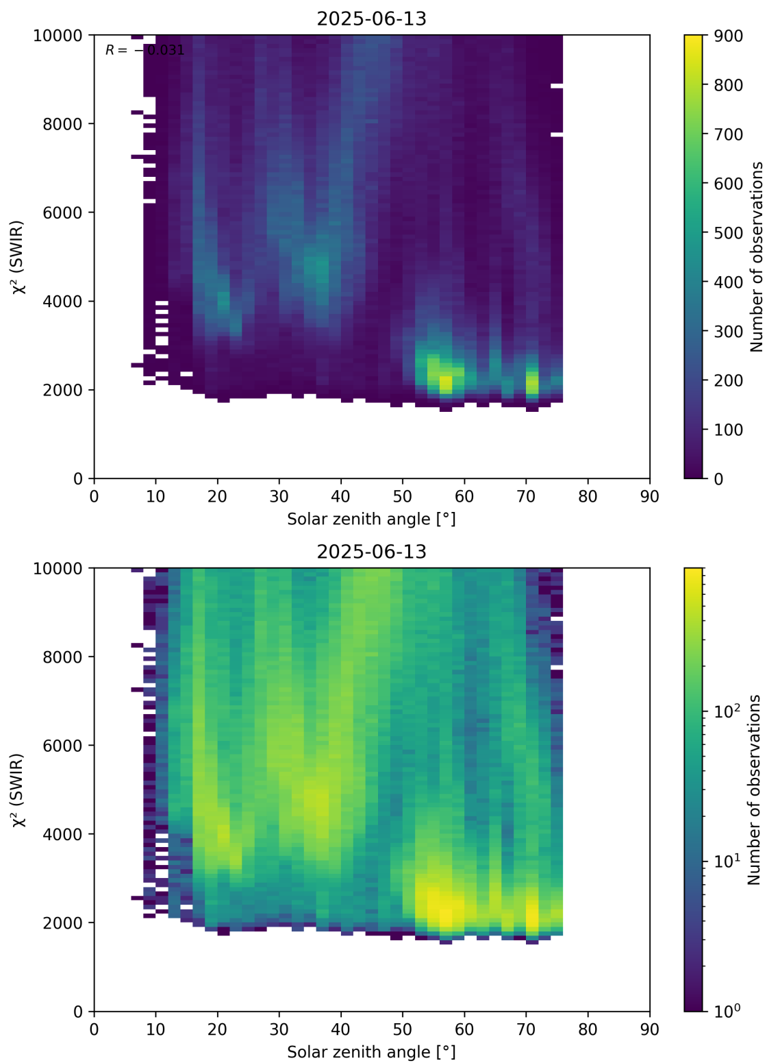
Figure 95: Scatter density plot of “Solar zenith angle” against “ \chi^2 (SWIR)” for 2025-06-12 to 2025-06-14.
