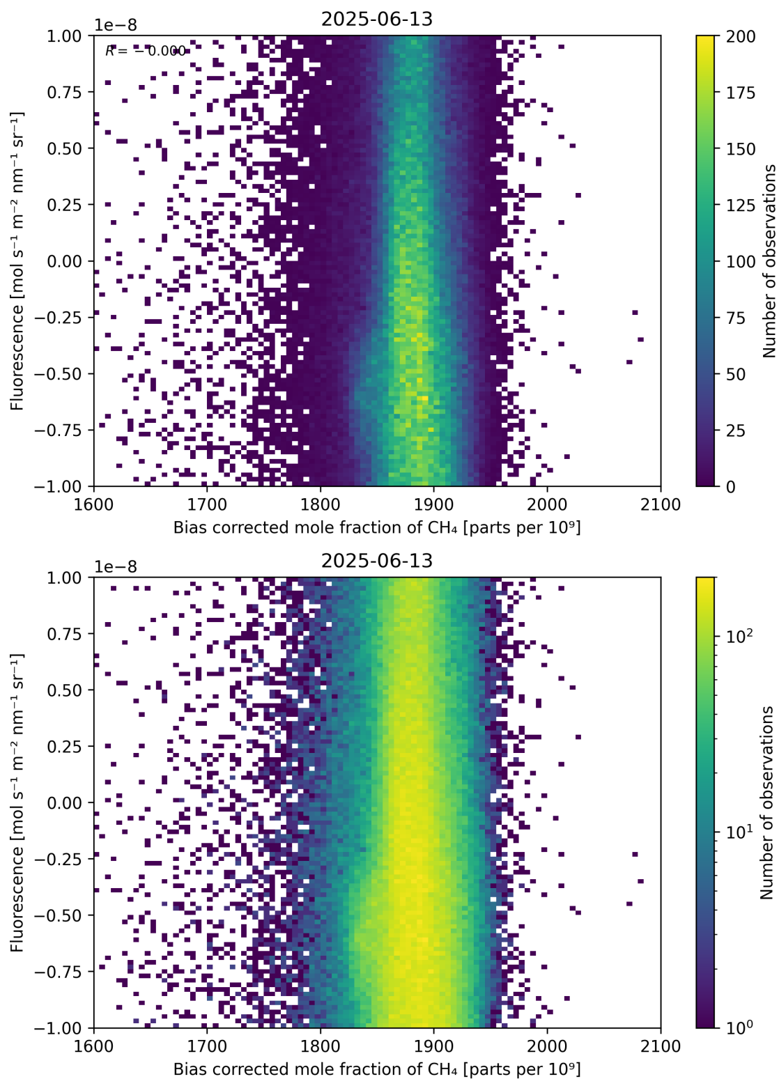
Figure 66: Scatter density plot of “Bias corrected mole fraction of \text{CH}_4 ” against “Fluorescence” for 2025-06-12 to 2025-06-14.
