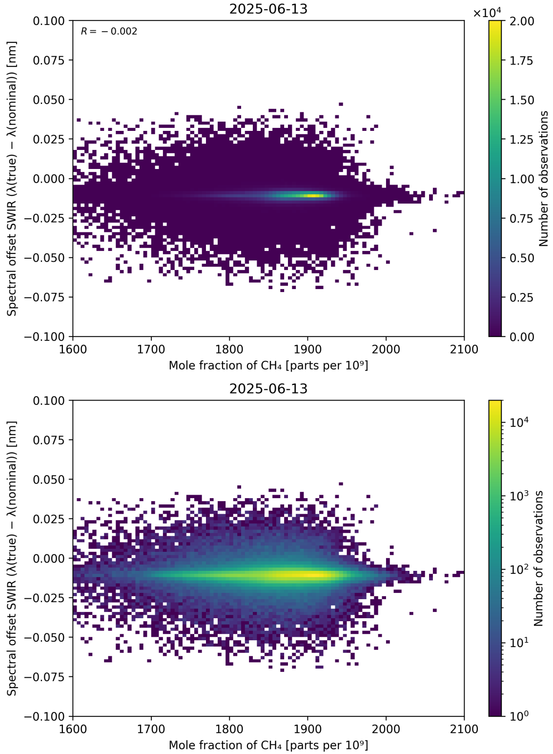
Figure 86: Scatter density plot of “Mole fraction of CH 4 ” against “Spectral offset SWIR ( \lambda_{\text{true}} - \lambda_{\text{nominal}} )” for 2025-06-12 to 2025-06-14.
