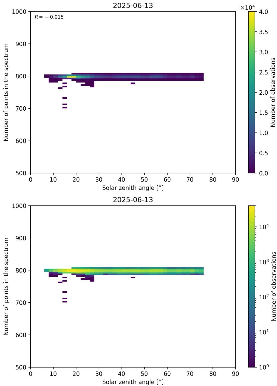
Figure 103: Scatter density plot of “Solar zenith angle” against “Number of points in the spectrum” for 2025-06-12 to 2025-06-14.
