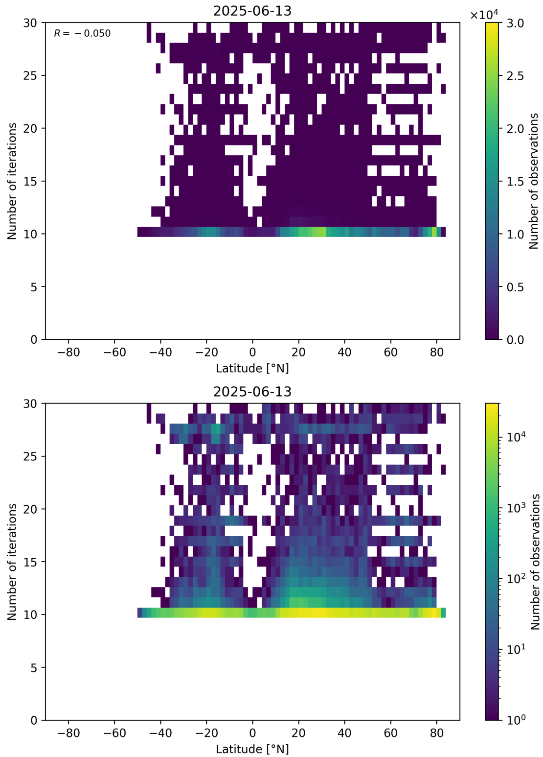
Figure 60: Scatter density plot of “Latitude” against “Number of iterations” for 2025-06-12 to 2025-06-14.
