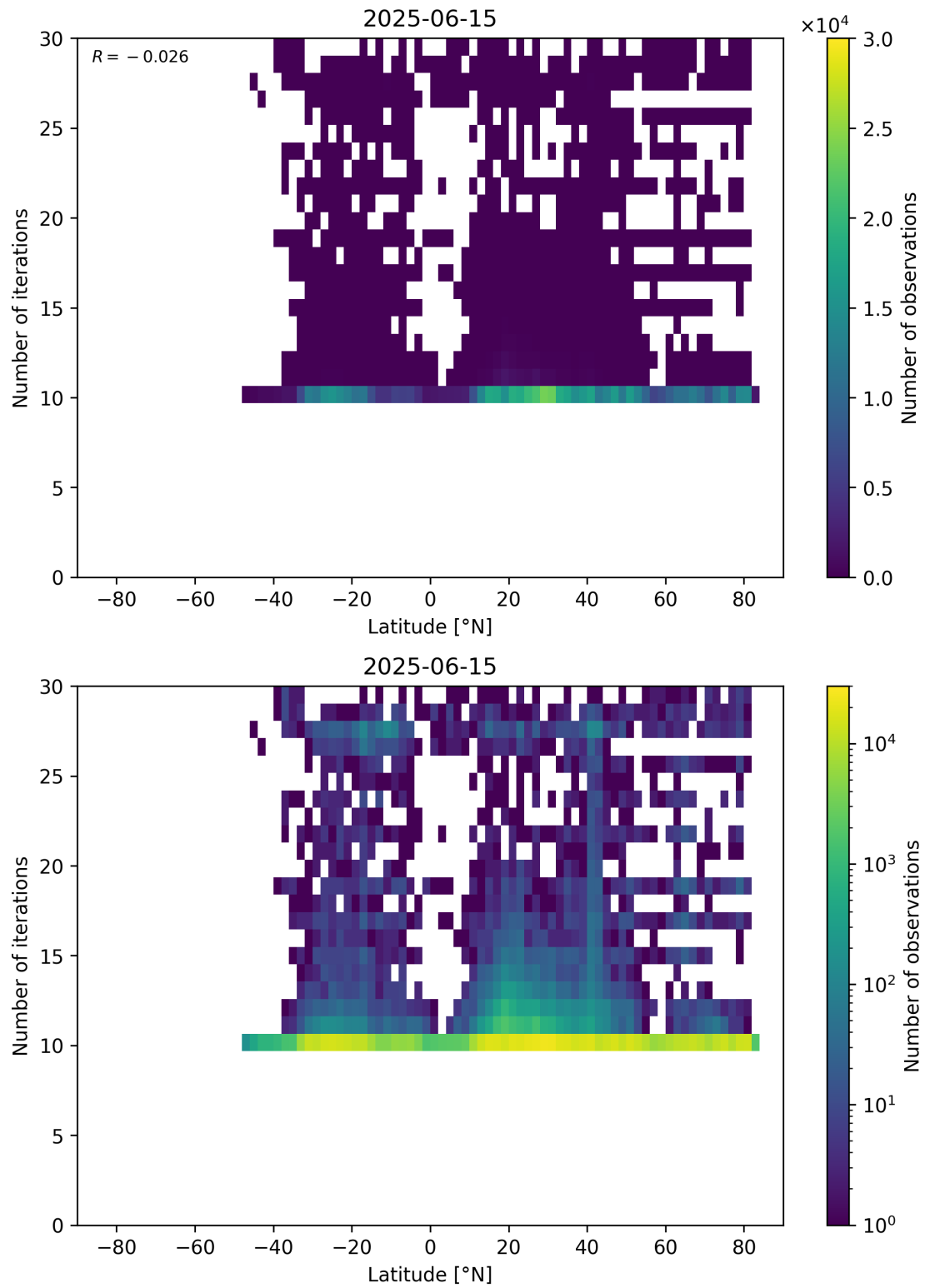
Figure 60: Scatter density plot of “Latitude” against “Number of iterations” for 2025-06-14 to 2025-06-16.
