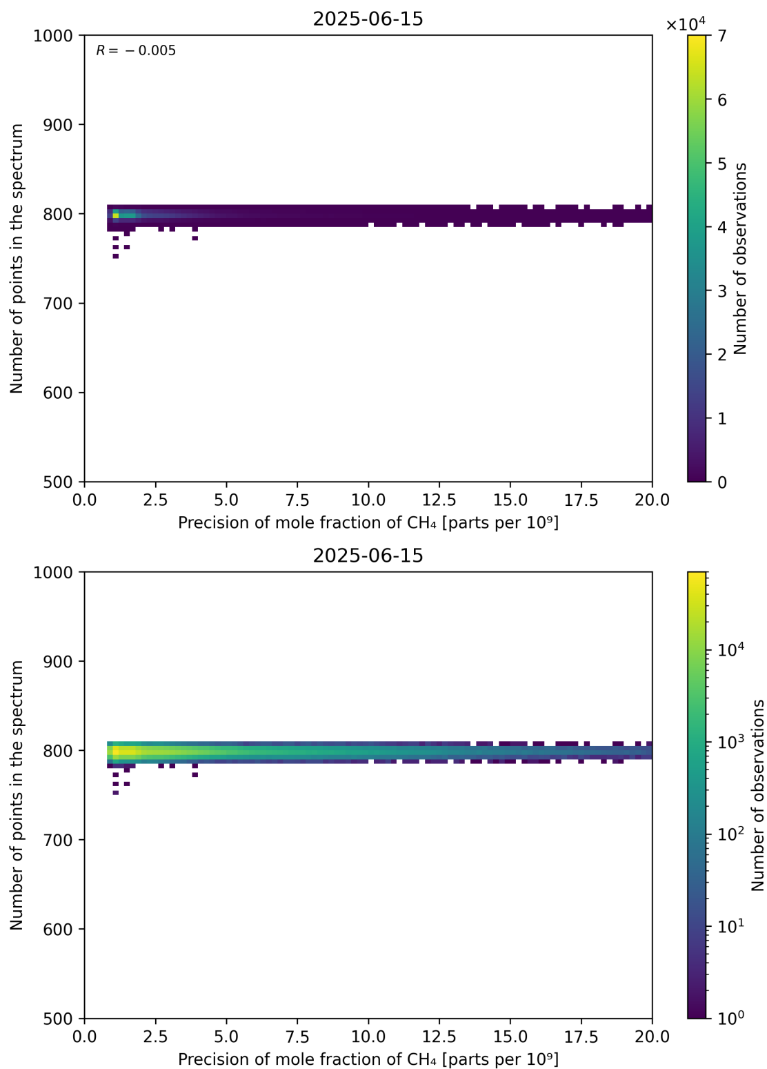
Figure 84: Scatter density plot of “Precision of mole fraction of CH 4 ” against “Number of points in the spectrum” for 2025-06-14 to 2025-06-16.
