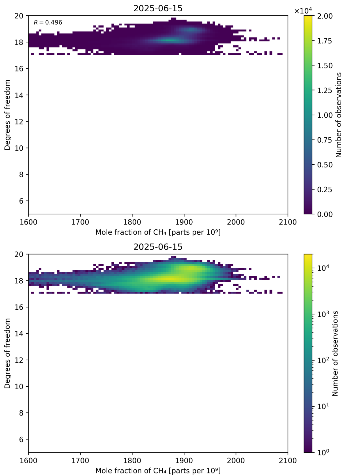
Figure 72: Scatter density plot of “Mole fraction of CH 4 ” against “Degrees of freedom” for 2025-06-14 to 2025-06-16.
