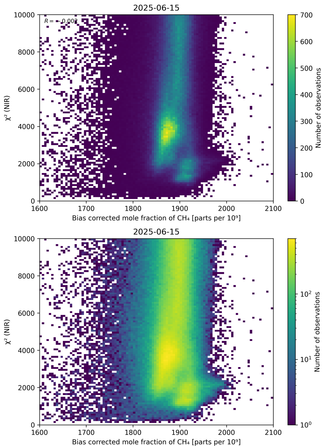
Figure 63: Scatter density plot of “Bias corrected mole fraction of CH 4 ” against “ \chi^2 (NIR)” for 2025-06-14 to 2025-06-16.
