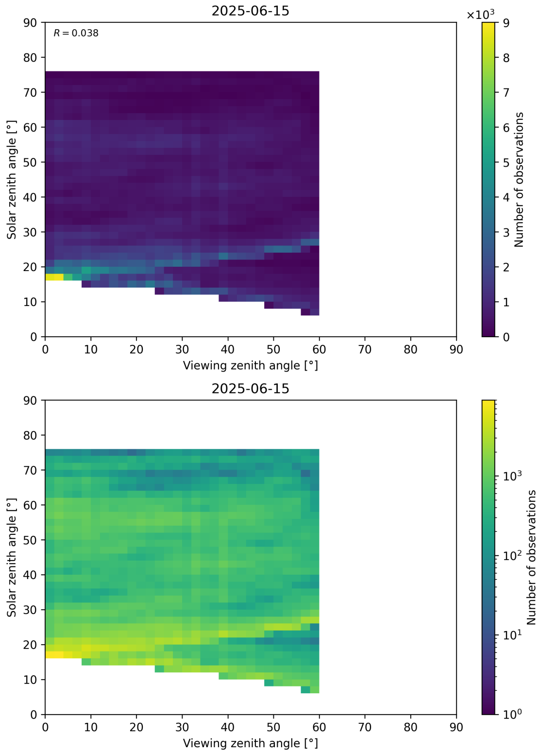
Figure 115: Scatter density plot of “Viewing zenith angle” against “Solar zenith angle” for 2025-06-14 to 2025-06-16.
