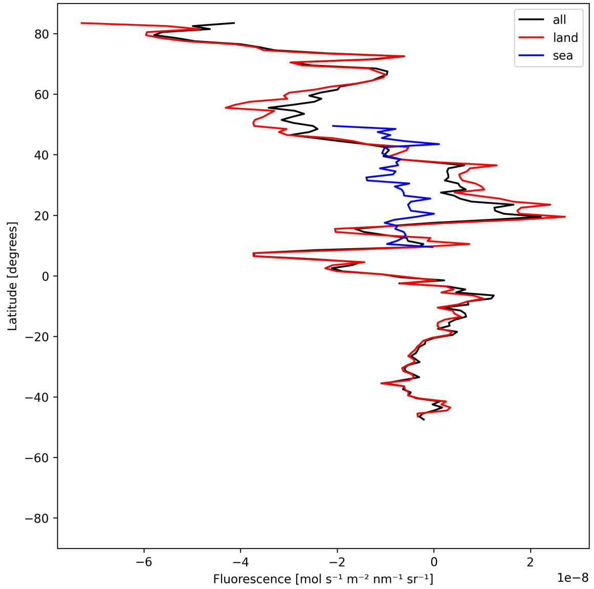
Figure 21: Zonal average of “Fluorescence” for 2025-06-14 to 2025-06-16.
