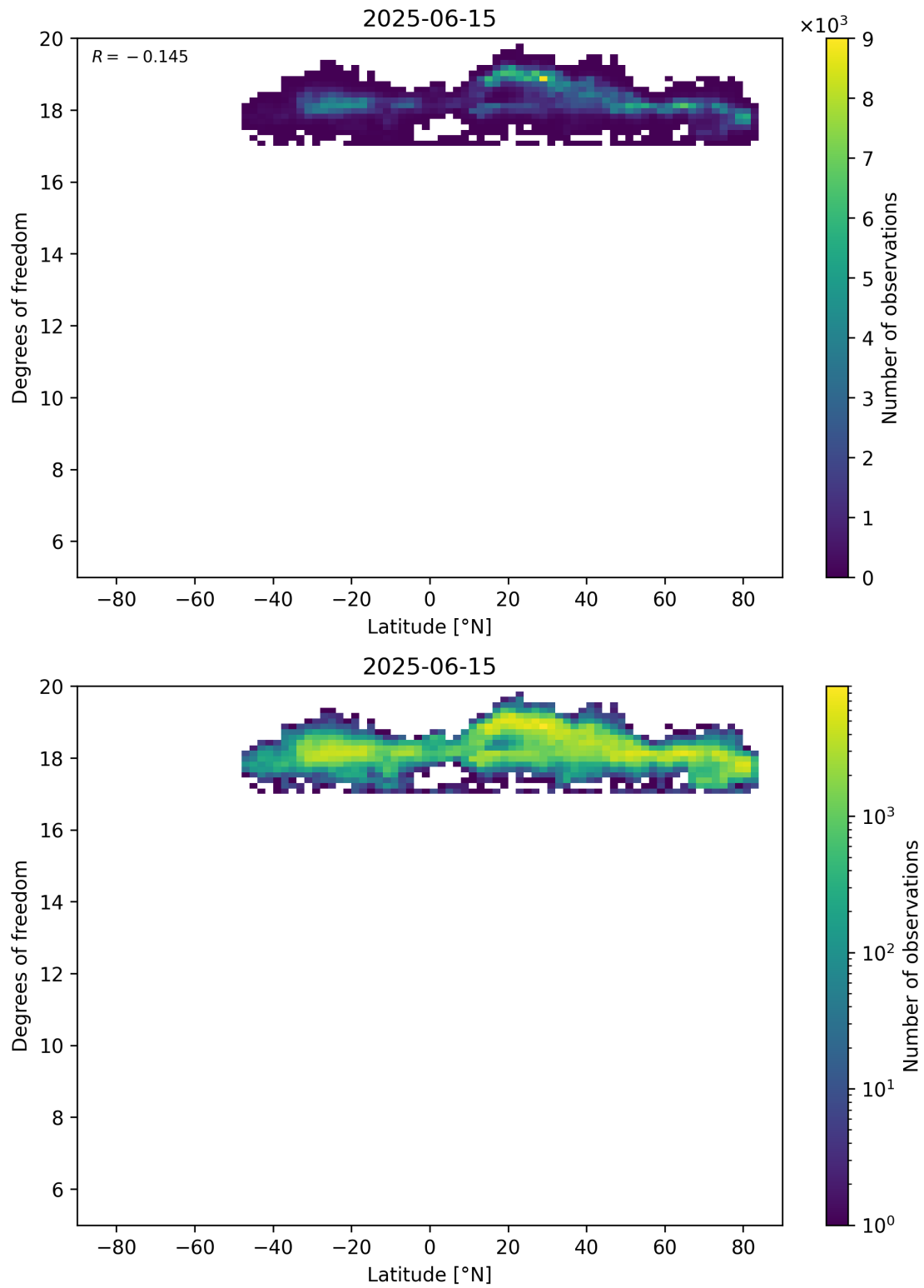
Figure 55: Scatter density plot of “Latitude” against “Degrees of freedom” for 2025-06-14 to 2025-06-16.
