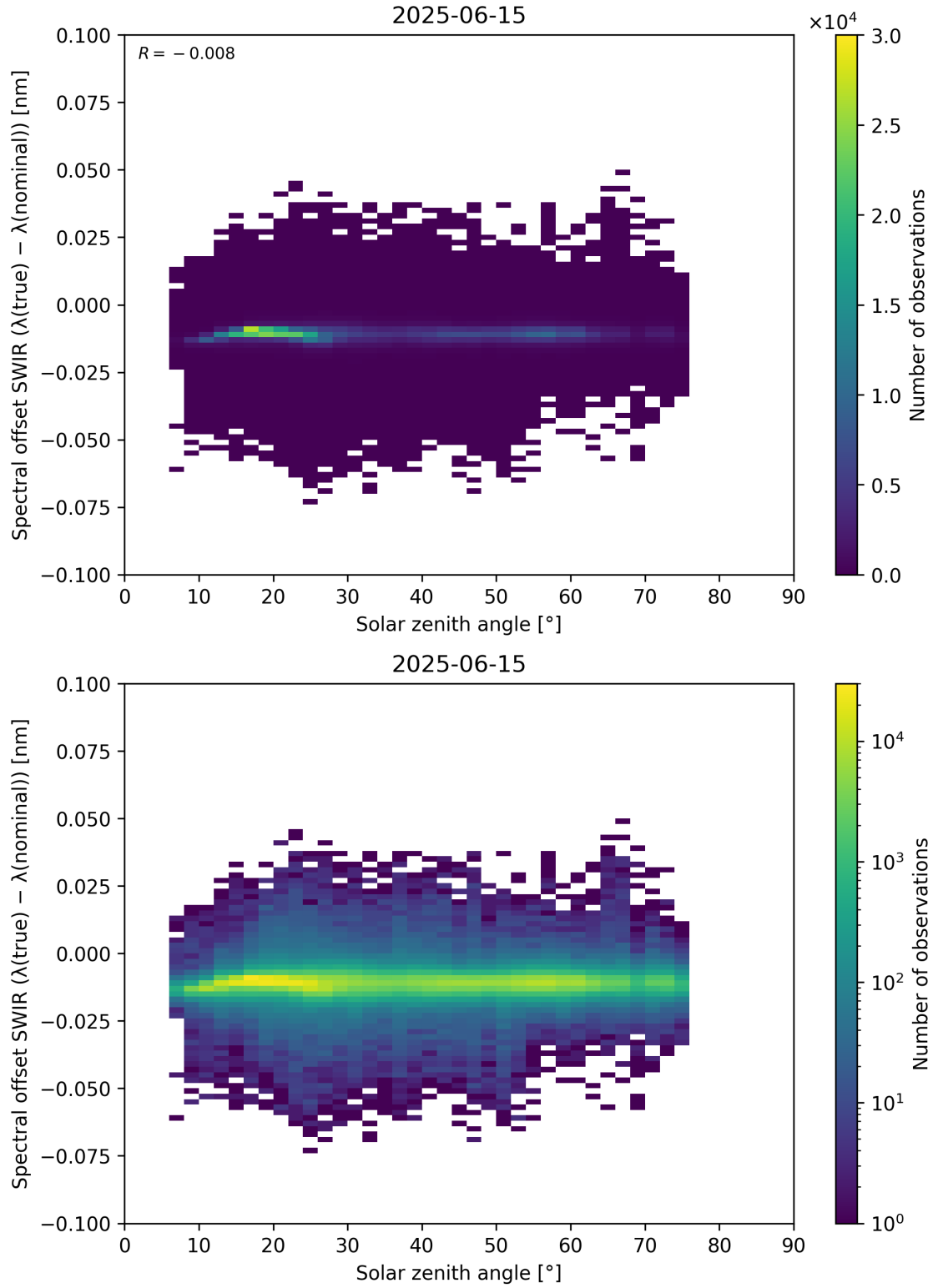
Figure 104: Scatter density plot of “Solar zenith angle” against “Spectral offset SWIR ( \lambda_{\text{true}} - \lambda_{\text{nominal}} )” for 2025-06-14 to 2025-06-16.
