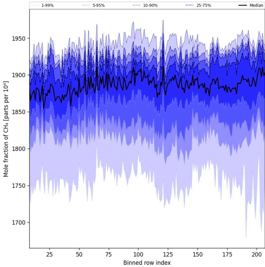
Figure 34: Along track statistics of “Mole fraction of CH 4 ” for 2025-06-14 to 2025-06-16
