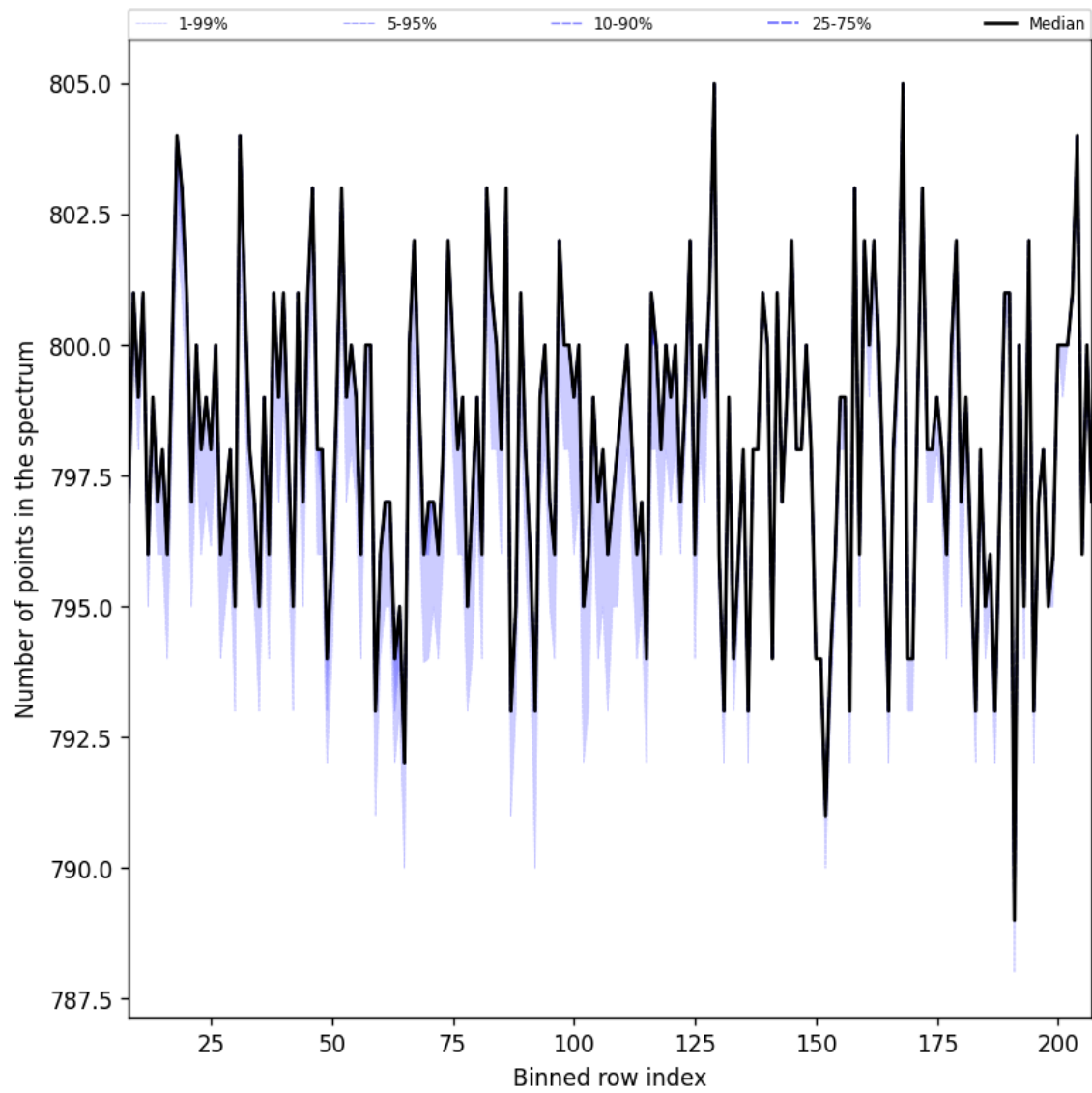
Figure 37: Along track statistics of “Number of points in the spectrum” for 2025-06-14 to 2025-06-16
