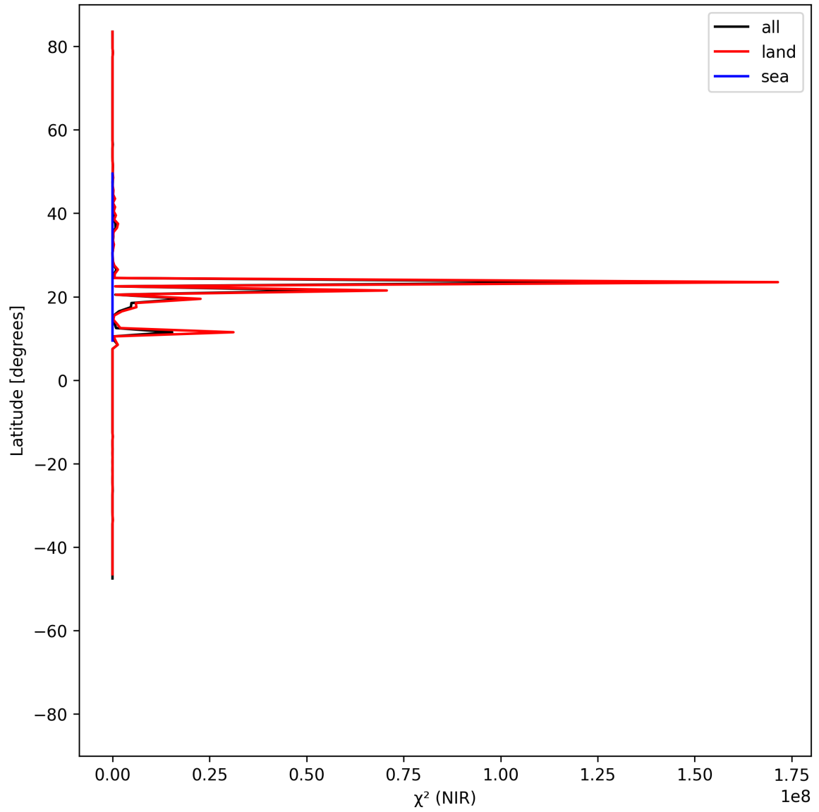
Figure 18: Zonal average of “ \chi^2 (NIR)” for 2025-06-14 to 2025-06-16.
