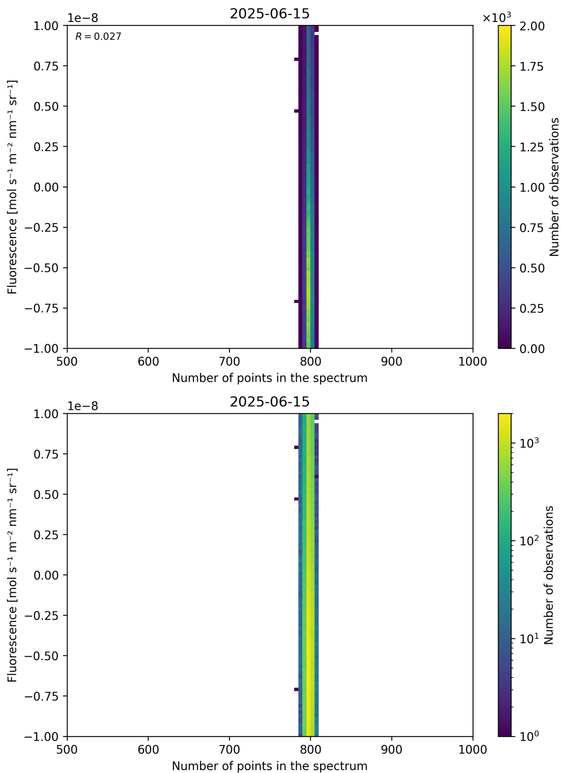
Figure 91: Scatter density plot of “Number of points in the spectrum” against “Fluorescence” for 2025-06-14 to 2025-06-16.
