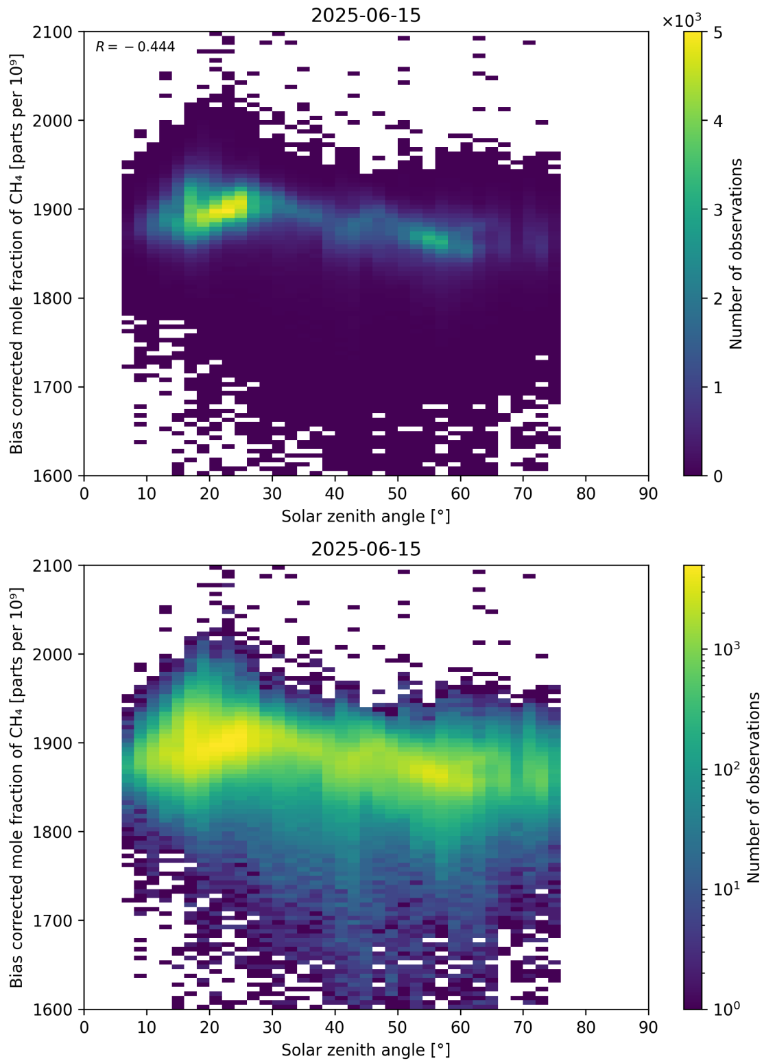
Figure 100: Scatter density plot of “Solar zenith angle” against “Bias corrected mole fraction of CH 4 ” for 2025-06-14 to 2025-06-16.
