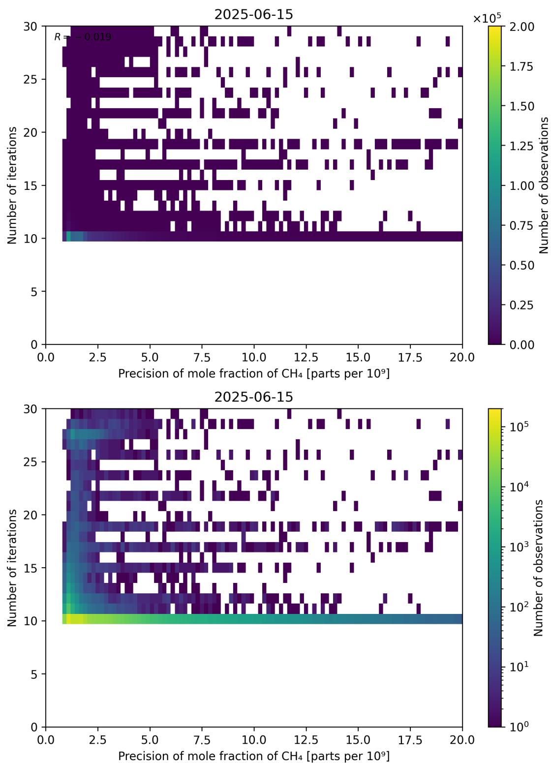
Figure 83: Scatter density plot of “Precision of mole fraction of CH 4 ” against “Number of iterations” for 2025-06-14 to 2025-06-16.
