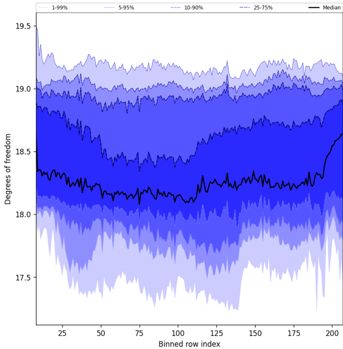
Figure 41: Along track statistics of “Degrees of freedom” for 2025-06-14 to 2025-06-16
