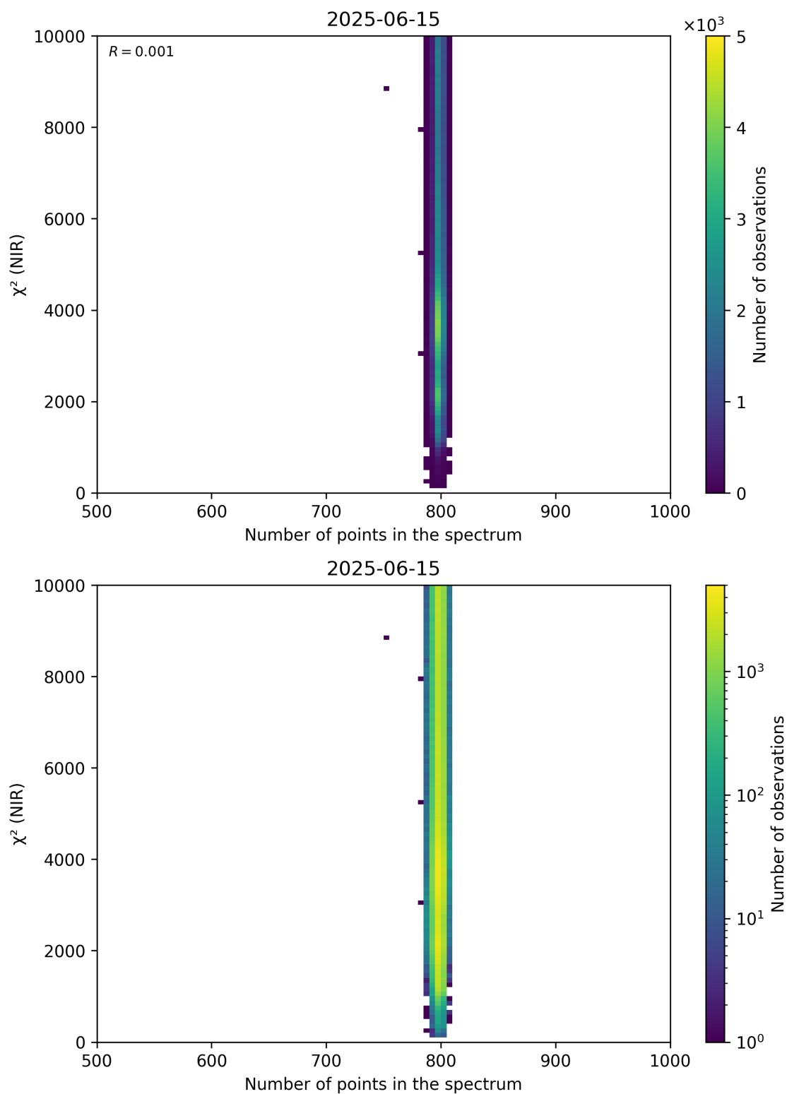
Figure 88: Scatter density plot of “Number of points in the spectrum” against “ \chi^2 (NIR)” for 2025-06-14 to 2025-06-16.
