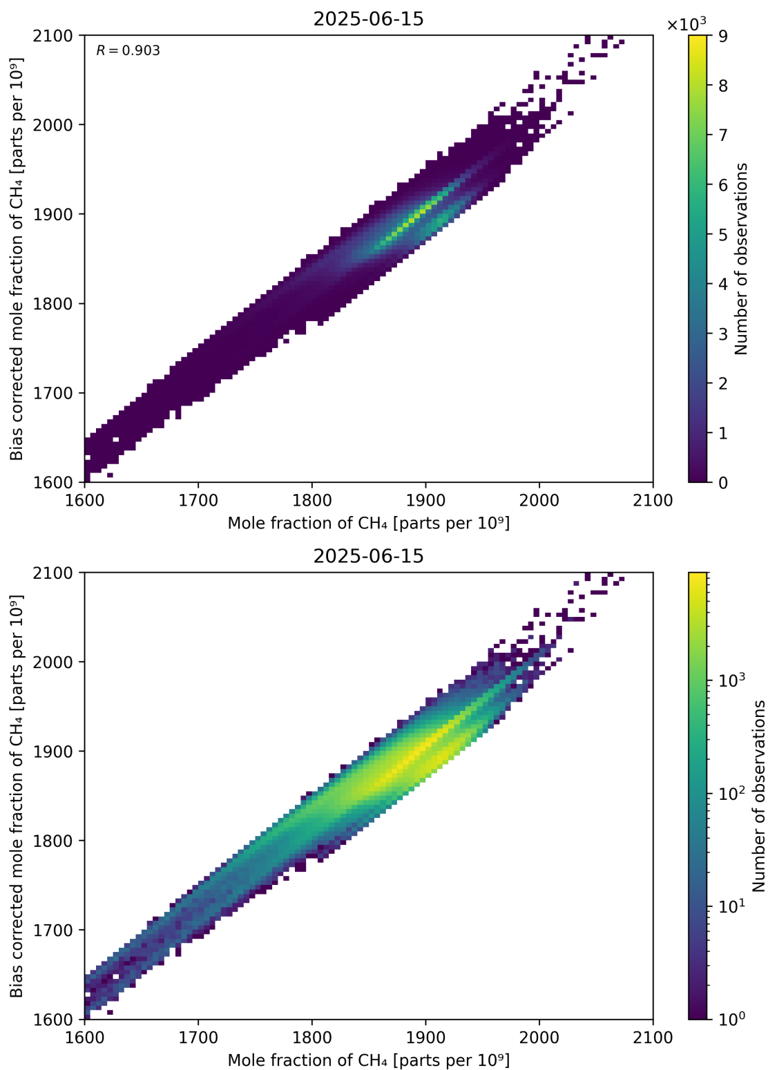
Figure 74: Scatter density plot of “Mole fraction of CH 4 ” against “Bias corrected mole fraction of CH 4 ” for 2025-06-14 to 2025-06-16.
