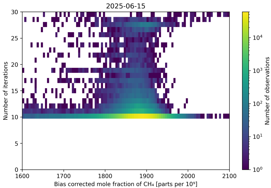
Figure 67: Scatter density plot of “Bias corrected mole fraction of CH 4 ” against “Number of iterations” for 2025-06-14 to 2025-06-16.
