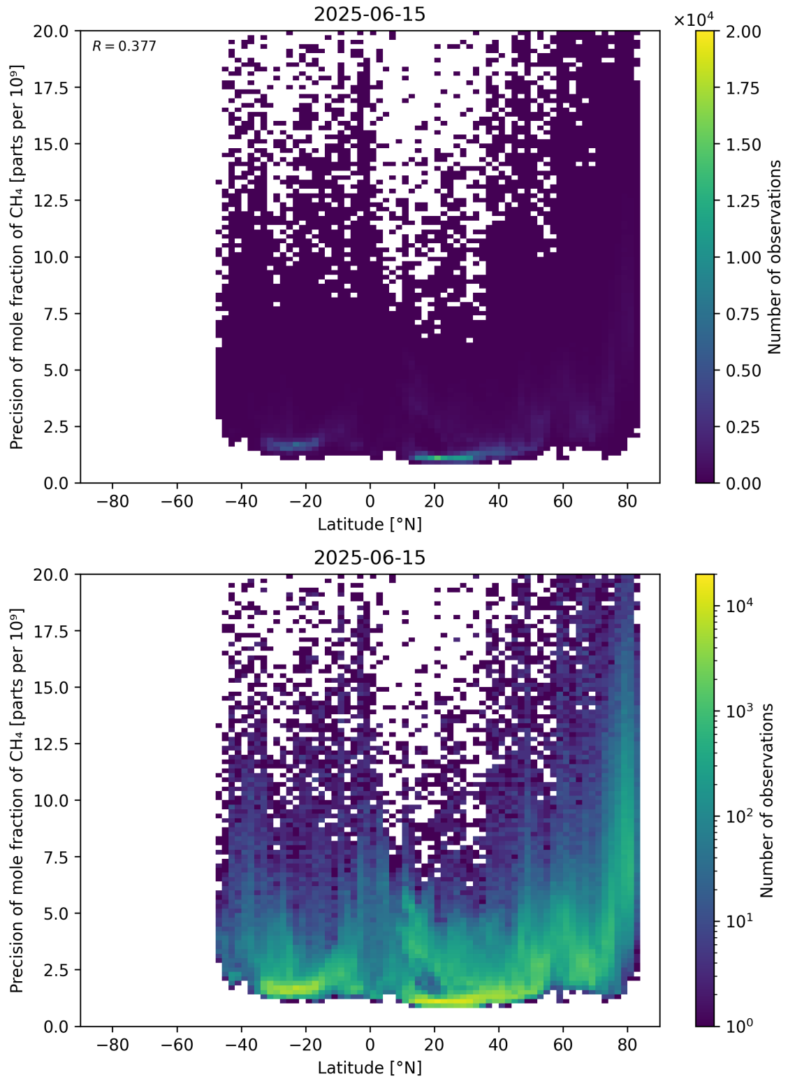
Figure 59: Scatter density plot of “Latitude” against “Precision of mole fraction of \text{CH}_4 ” for 2025-06-14 to 2025-06-16.
