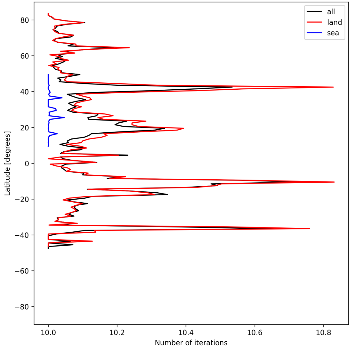
Figure 20: Zonal average of “Number of iterations” for 2025-06-14 to 2025-06-16.
