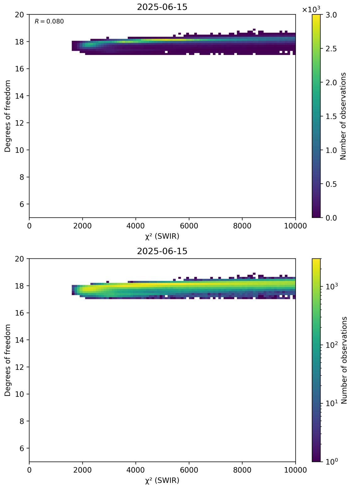
Figure 48: Scatter density plot of “ \chi^2 (SWIR)” against “Degrees of freedom” for 2025-06-14 to 2025-06-16.
