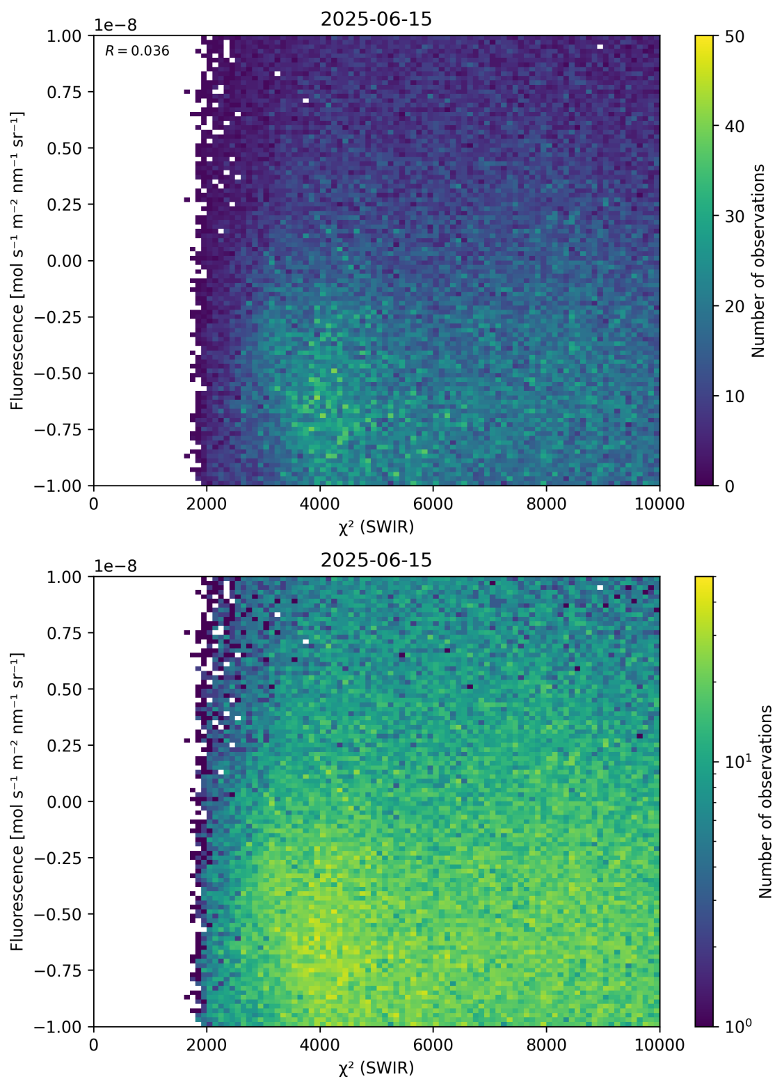
Figure 49: Scatter density plot of “ \chi^2 (SWIR)” against “Fluorescence” for 2025-06-14 to 2025-06-16.
