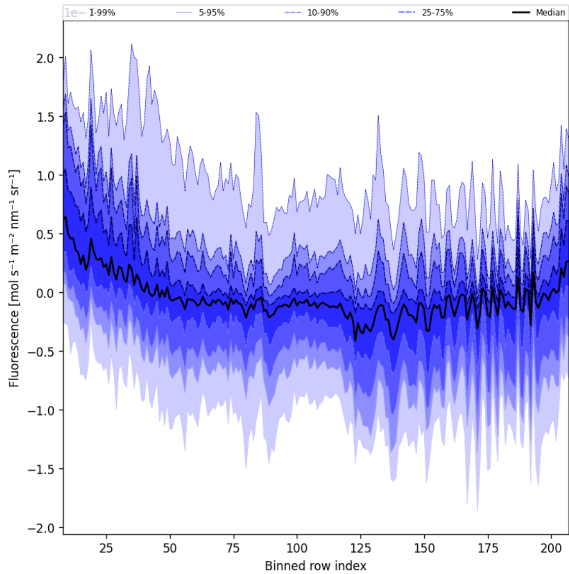
Figure 43: Along track statistics of “Fluorescence” for 2025-06-14 to 2025-06-16
