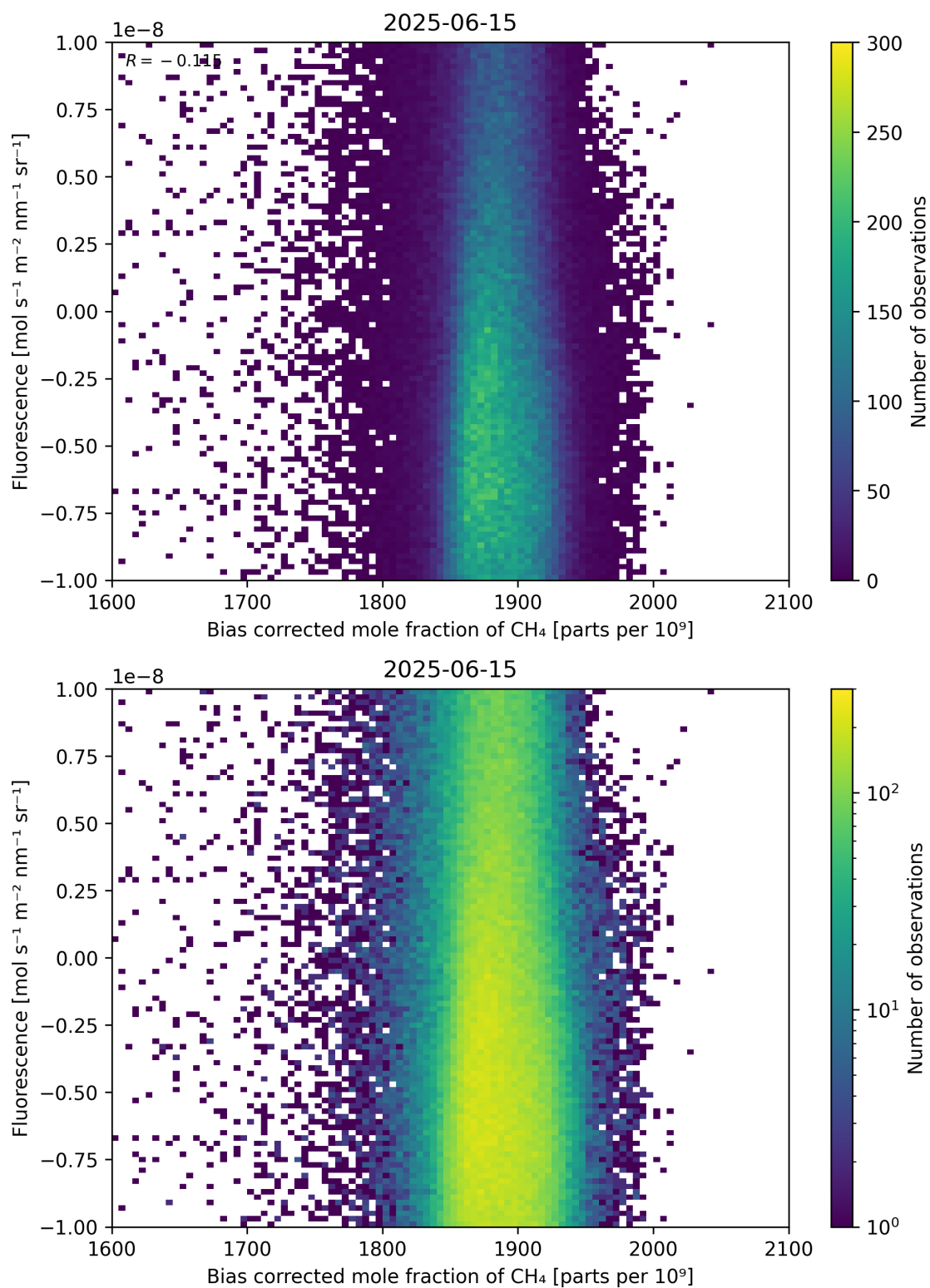
Figure 66: Scatter density plot of “Bias corrected mole fraction of \text{CH}_4 ” against “Fluorescence” for 2025-06-14 to 2025-06-16.
