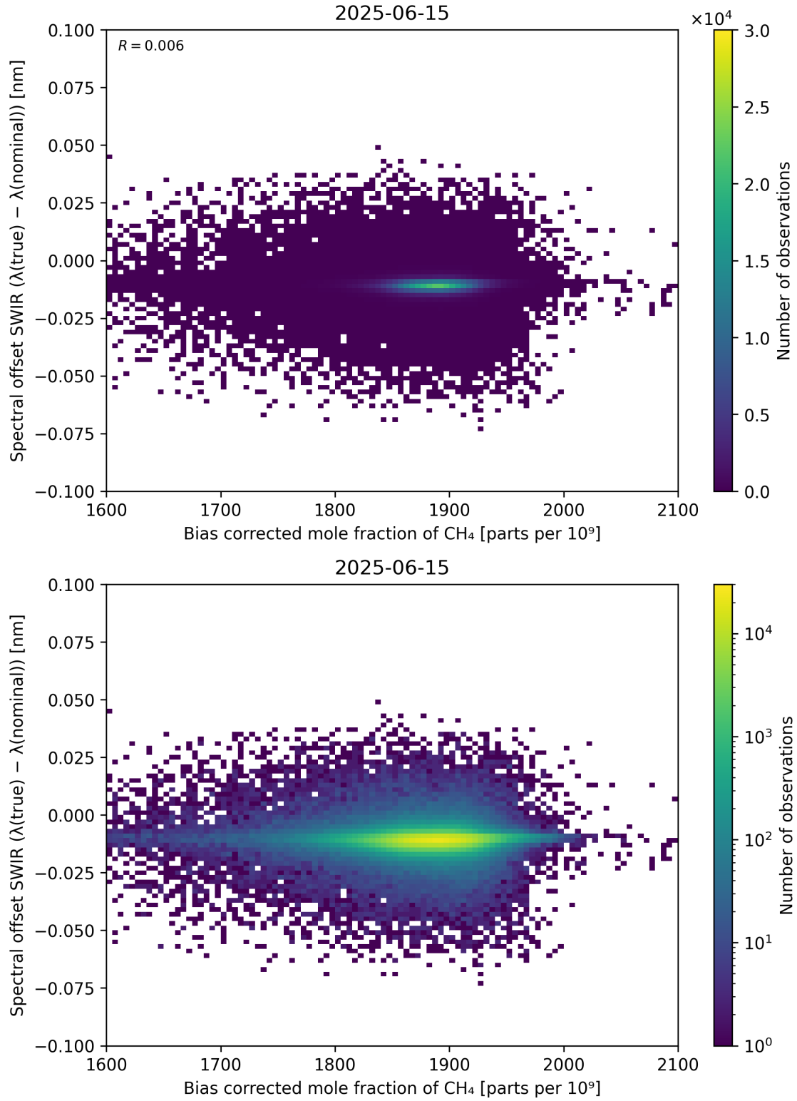
Figure 69: Scatter density plot of “Bias corrected mole fraction of \text{CH}_4 ” against “Spectral offset SWIR ( \lambda_{\text{true}} - \lambda_{\text{nominal}} )” for 2025-06-14 to 2025-06-16.
