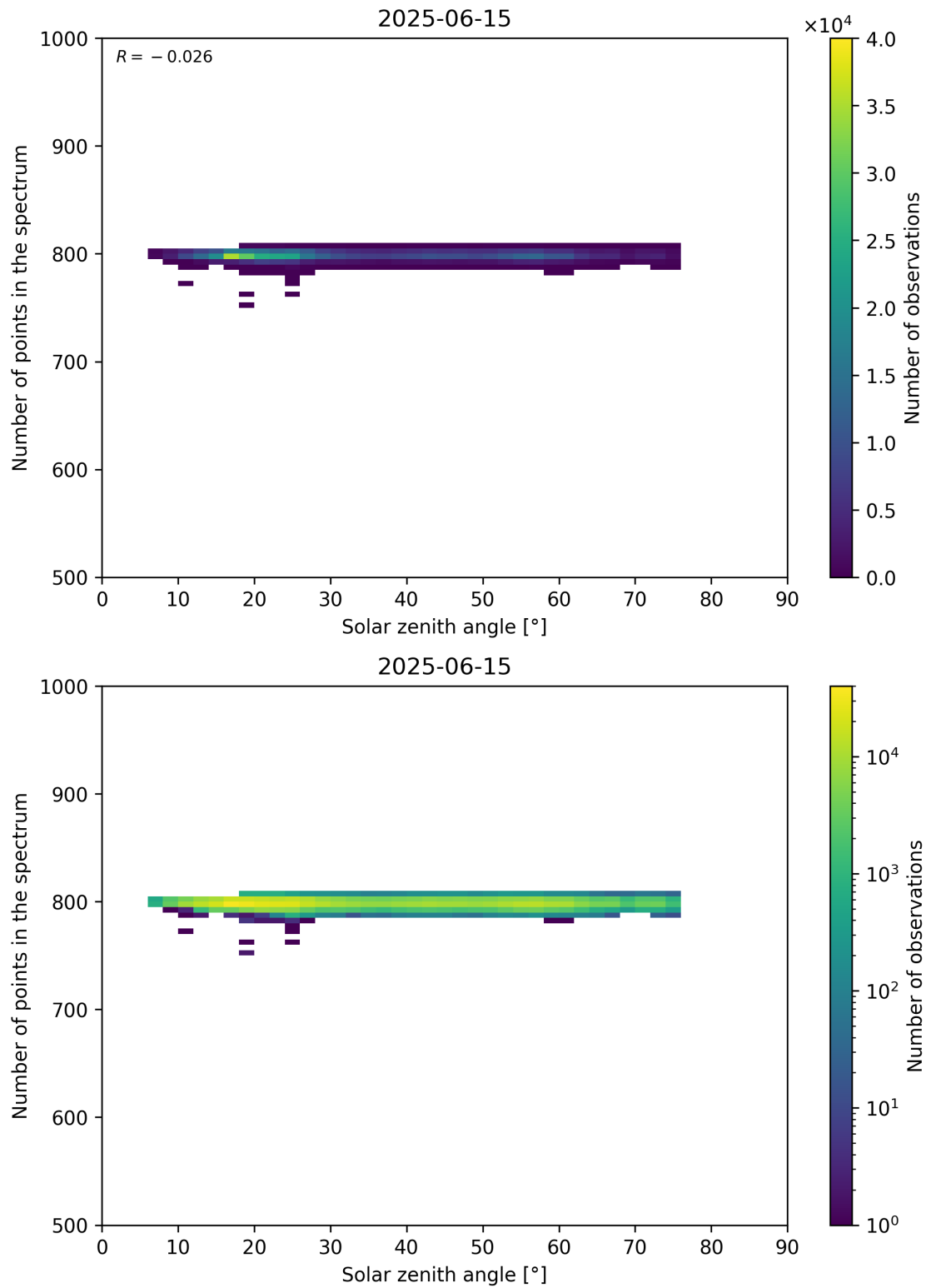
Figure 103: Scatter density plot of “Solar zenith angle” against “Number of points in the spectrum” for 2025-06-14 to 2025-06-16.
