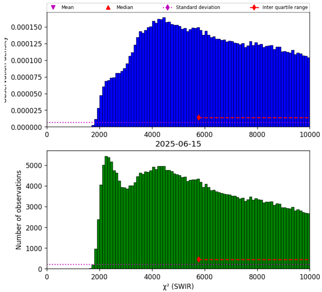
Figure 28: Histogram of “ \chi^2 (SWIR)” for 2025-06-14 to 2025-06-16
