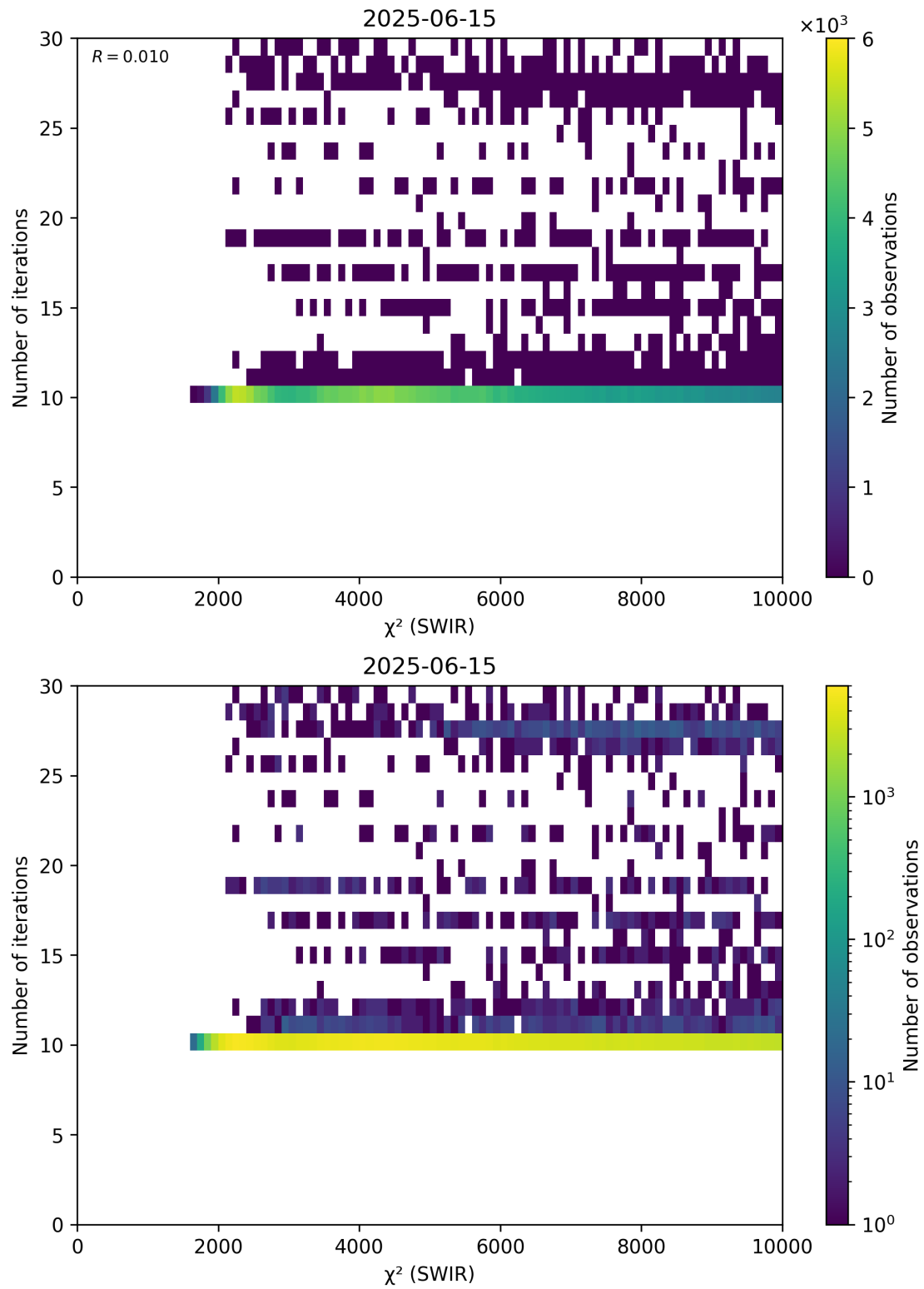
Figure 50: Scatter density plot of “ \chi^2 (SWIR)” against “Number of iterations” for 2025-06-14 to 2025-06-16.
