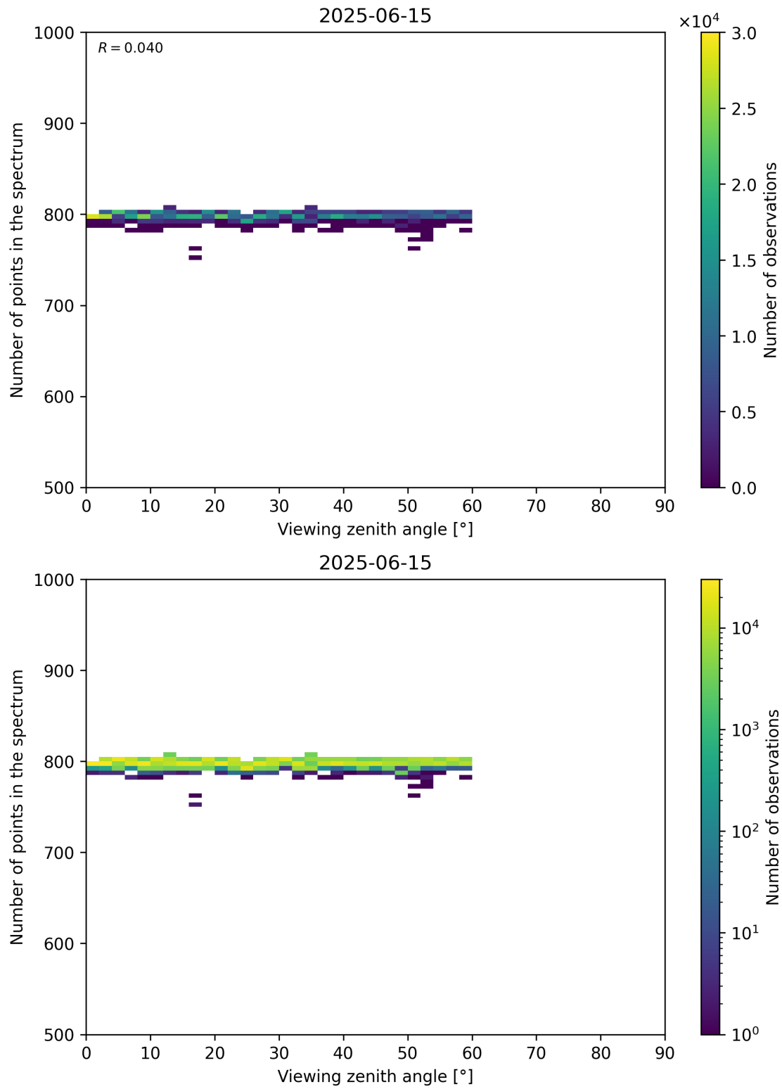
Figure 114: Scatter density plot of “Viewing zenith angle” against “Number of points in the spectrum” for 2025-06-14 to 2025-06-16.
