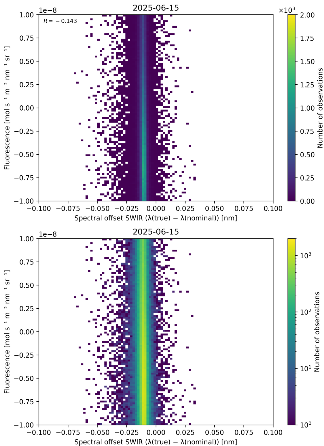
Figure 120: Scatter density plot of “Spectral offset SWIR ( \lambda_{\text{true}} - \lambda_{\text{nominal}} )” against “Fluorescence” for 2025-06-14 to 2025-06-16.
