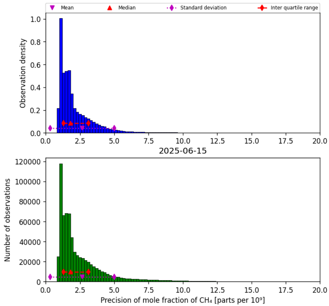
Figure 24: Histogram of “Precision of mole fraction of CH 4 ” for 2025-06-14 to 2025-06-16
