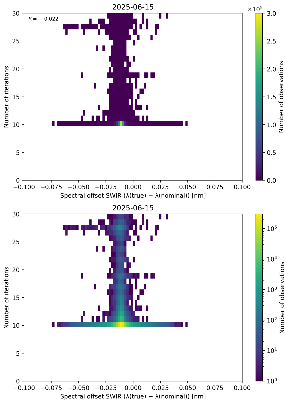
Figure 121: Scatter density plot of “Spectral offset SWIR ( \lambda_{\text{true}} - \lambda_{\text{nominal}} )” against “Number of iterations” for 2025-06-14 to 2025-06-16.
