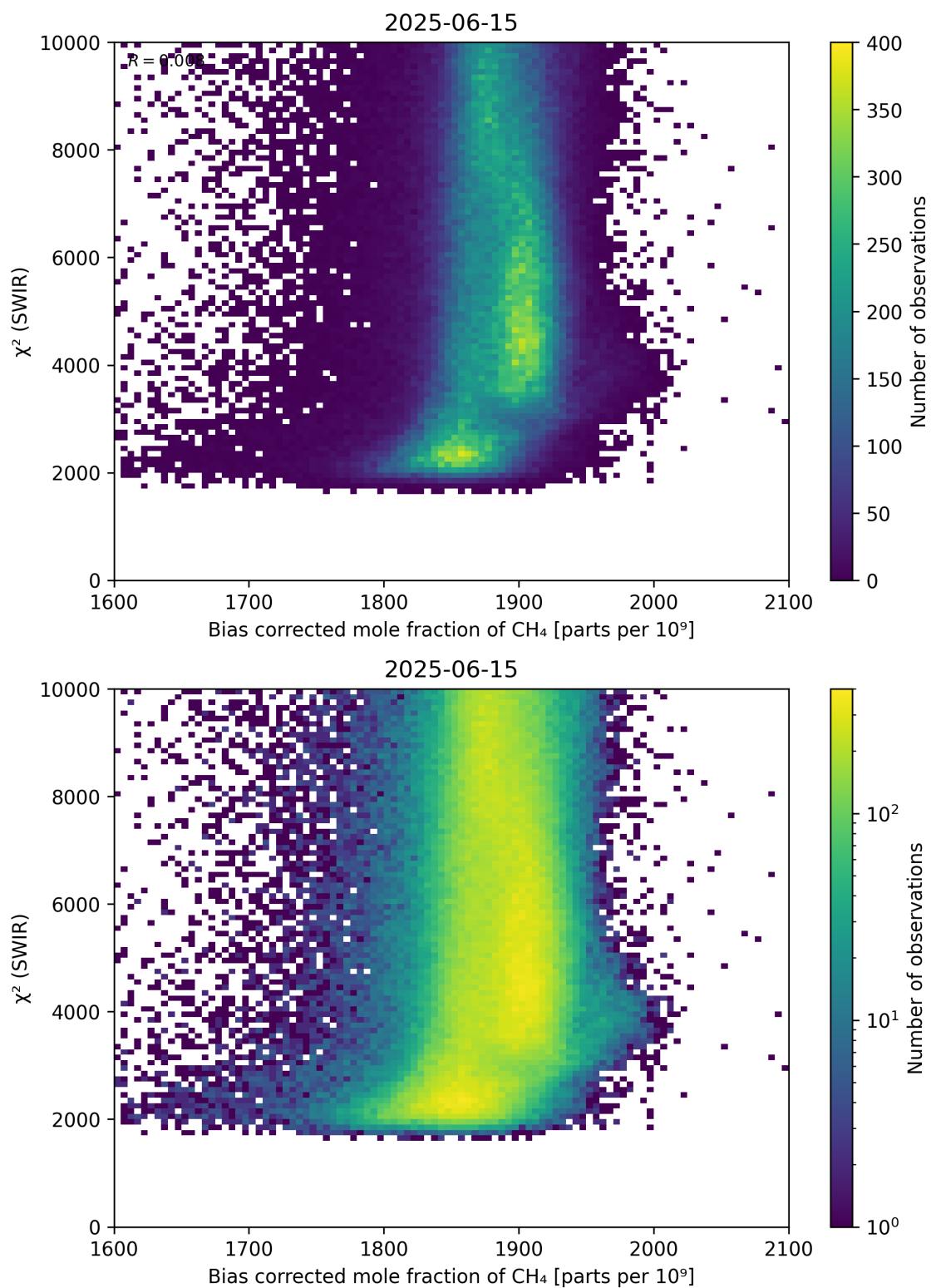
Figure 64: Scatter density plot of “Bias corrected mole fraction of CH 4 ” against “ \chi^2 (SWIR)” for 2025-06-14 to 2025-06-16.
