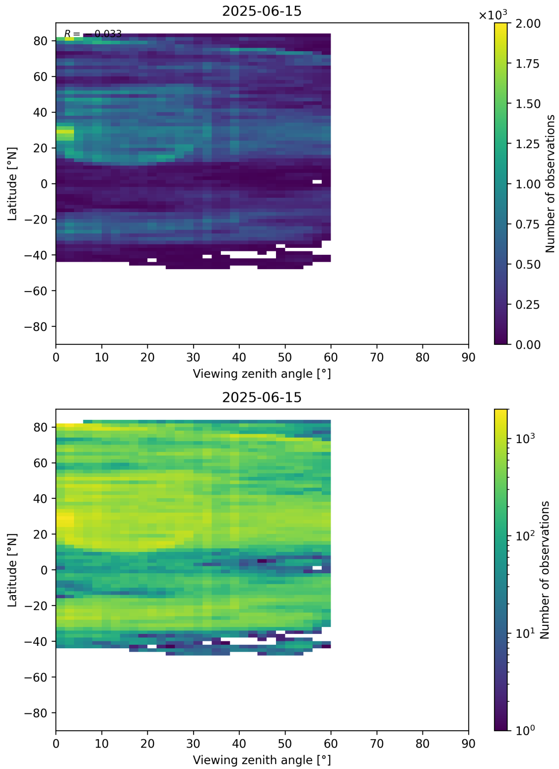
Figure 109: Scatter density plot of “Viewing zenith angle” against “Latitude” for 2025-06-14 to 2025-06-16.
