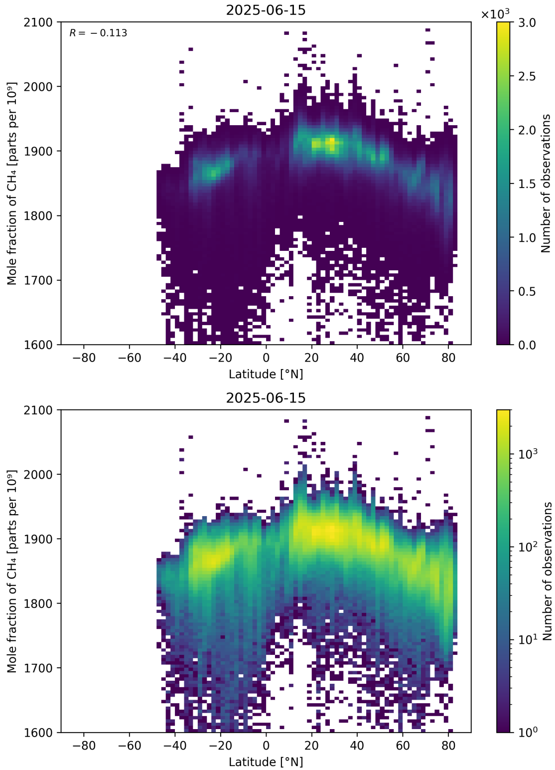
Figure 57: Scatter density plot of “Latitude” against “Mole fraction of CH 4 ” for 2025-06-14 to 2025-06-16.
