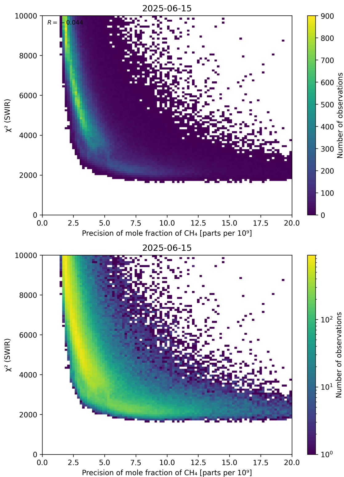
Figure 79: Scatter density plot of “Precision of mole fraction of CH 4 ” against “ \chi^2 (SWIR)” for 2025-06-14 to 2025-06-16.
