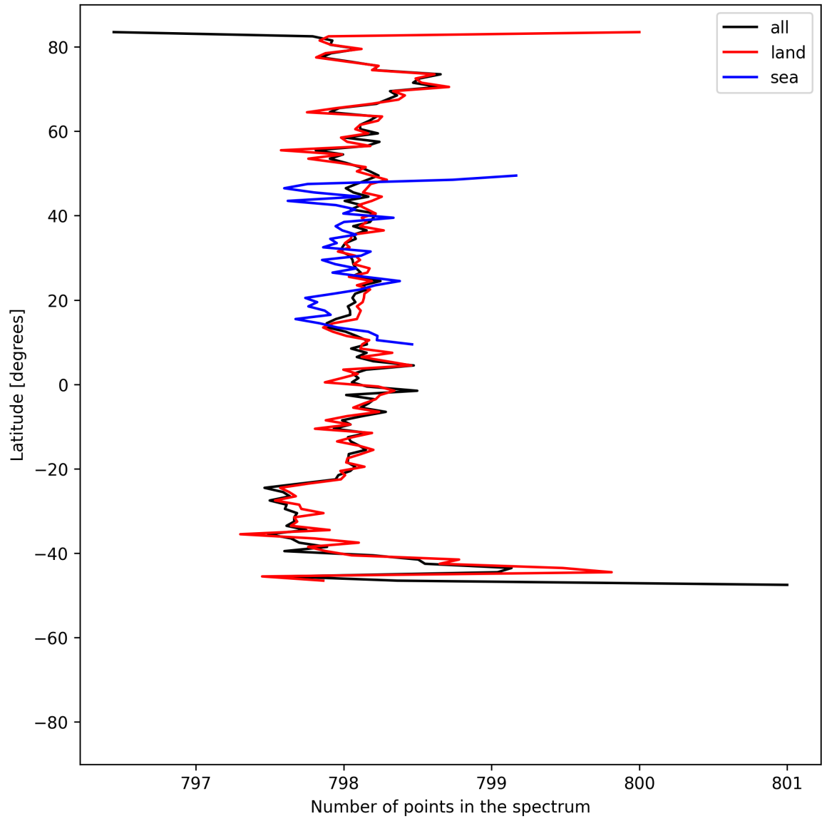
Figure 15: Zonal average of “Number of points in the spectrum” for 2025-06-14 to 2025-06-16.
