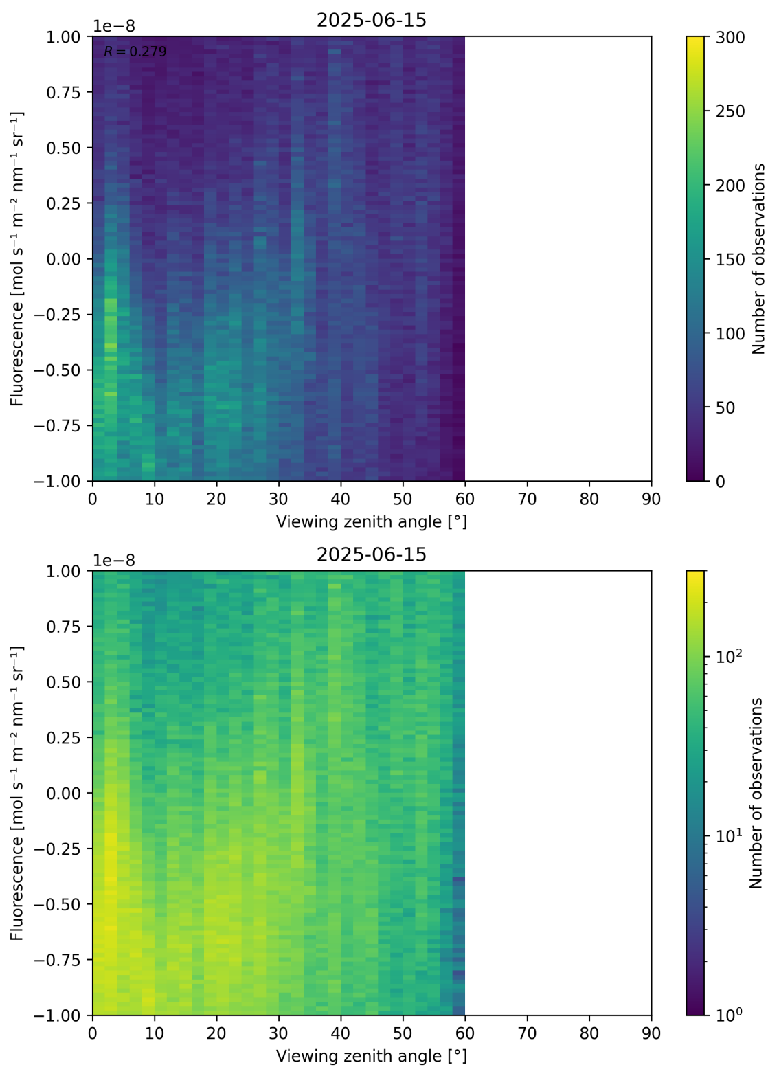
Figure 108: Scatter density plot of “Viewing zenith angle” against “Fluorescence” for 2025-06-14 to 2025-06-16.
