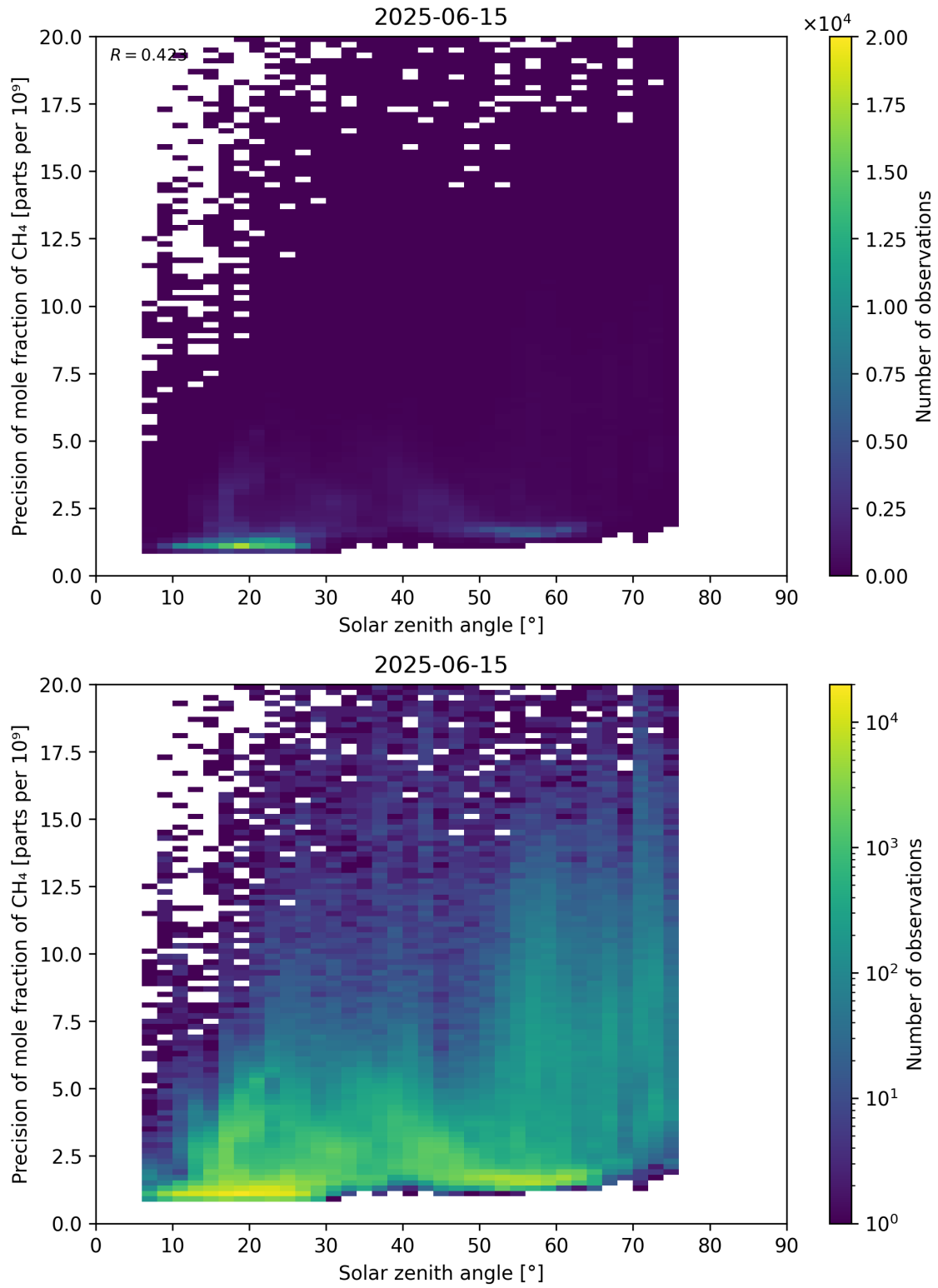
Figure 101: Scatter density plot of “Solar zenith angle” against “Precision of mole fraction of CH 4 ” for 2025-06-14 to 2025-06-16.
