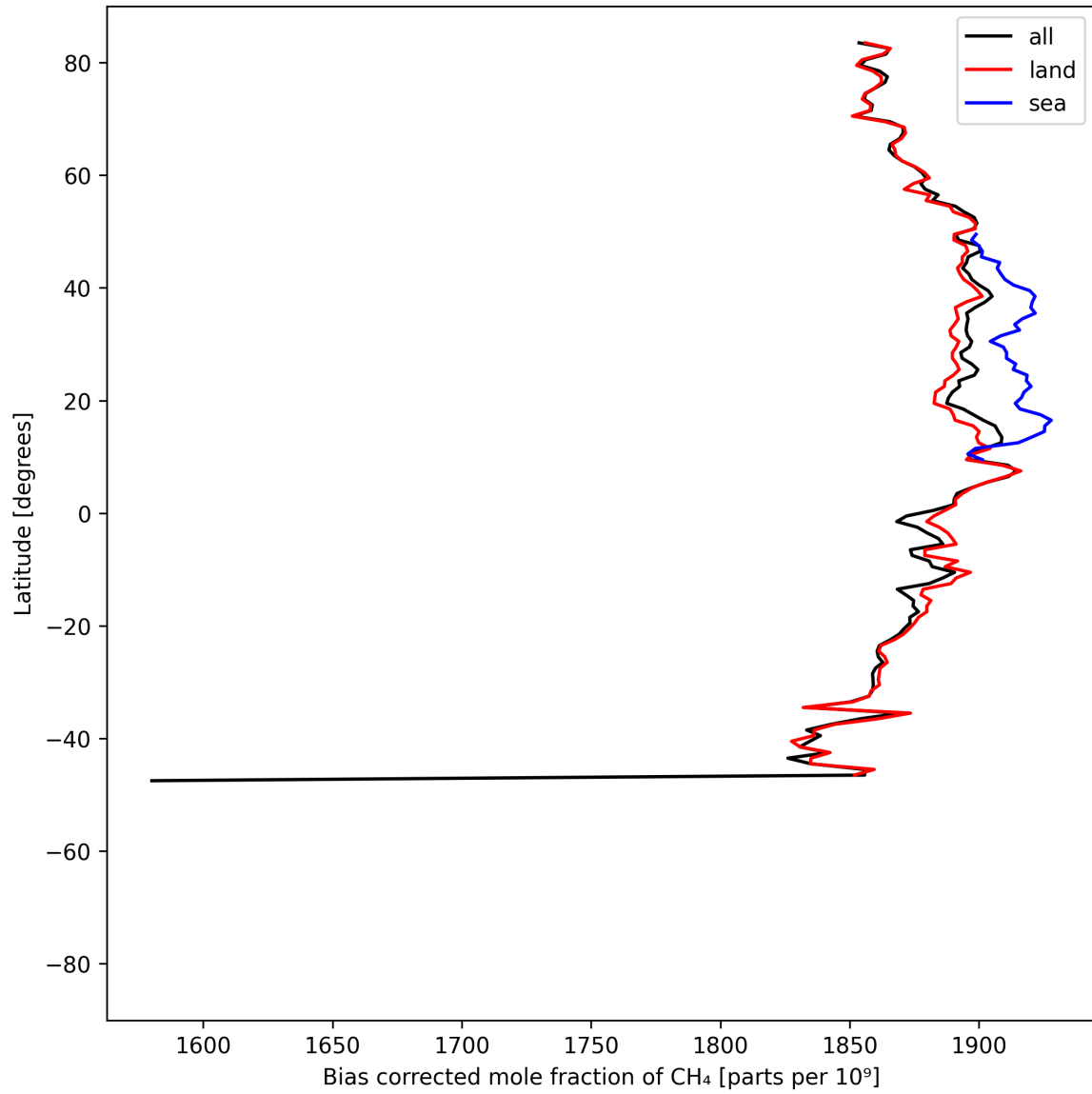
Figure 14: Zonal average of “Bias corrected mole fraction of CH 4 ” for 2025-06-14 to 2025-06-16.
