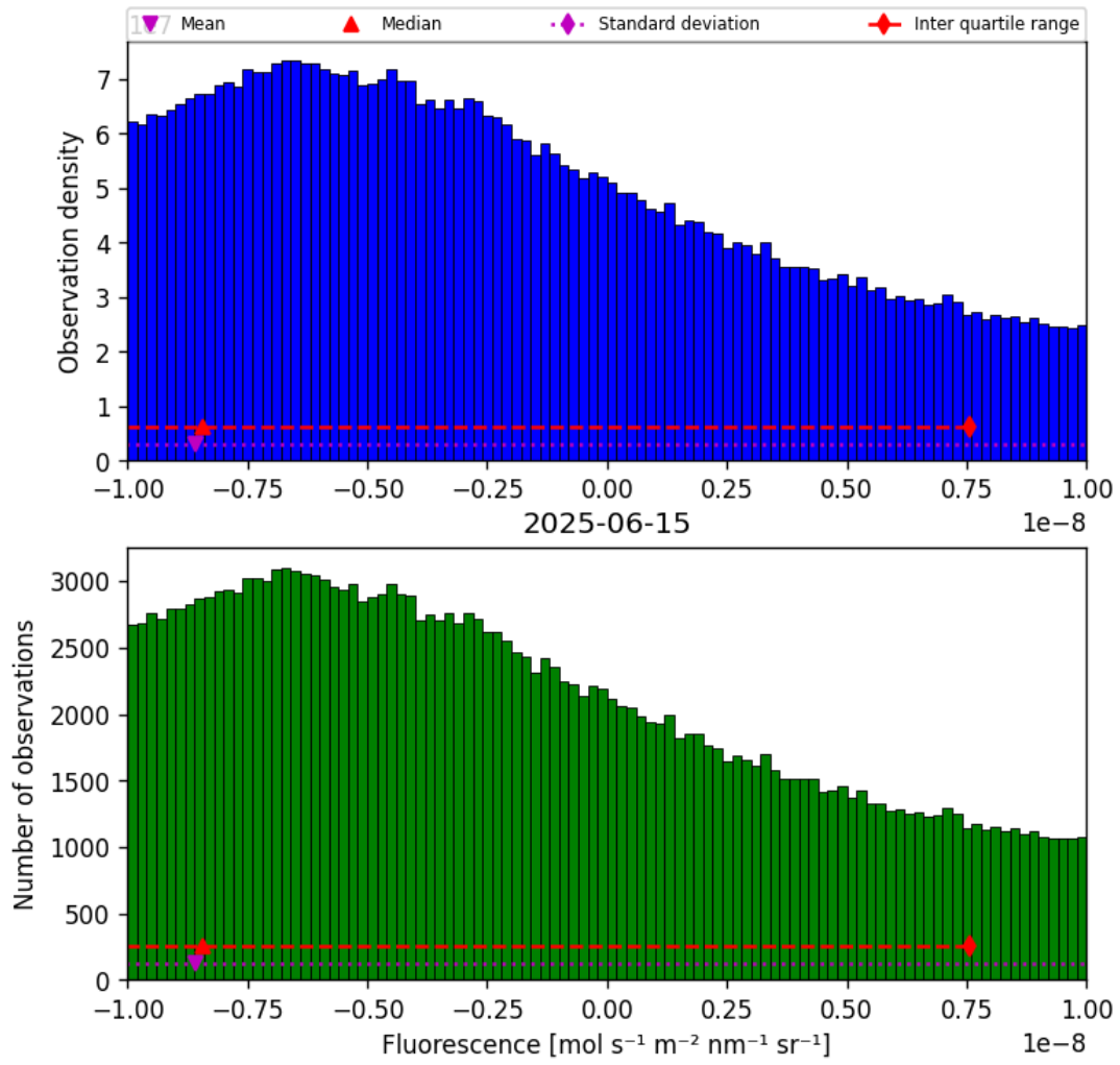
Figure 32: Histogram of “Fluorescence” for 2025-06-14 to 2025-06-16
