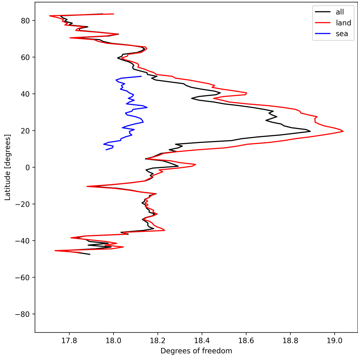
Figure 19: Zonal average of “Degrees of freedom” for 2025-06-14 to 2025-06-16.
