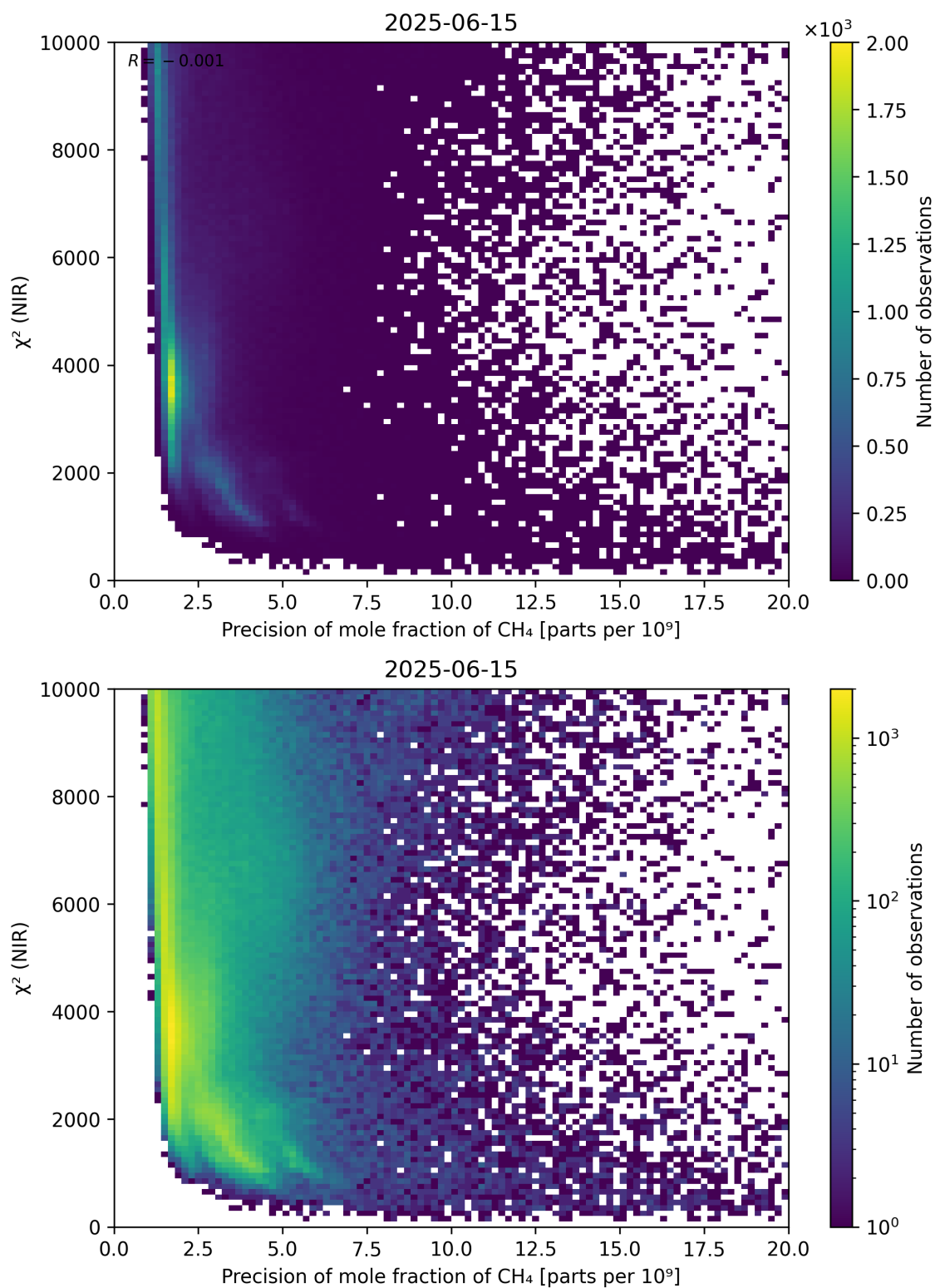
Figure 78: Scatter density plot of “Precision of mole fraction of CH 4 ” against “ \chi^2 (NIR)” for 2025-06-14 to 2025-06-16.
