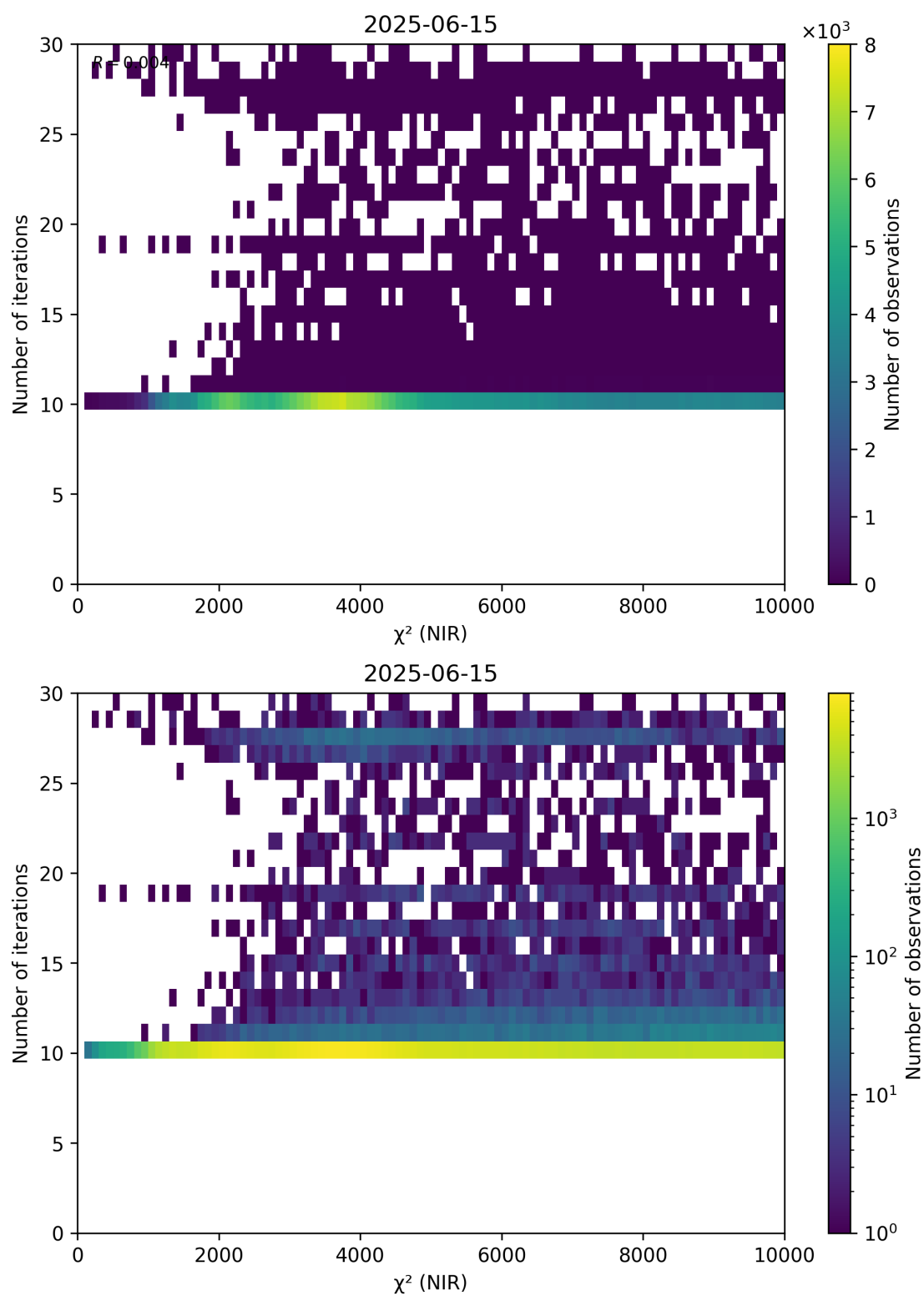
Figure 46: Scatter density plot of “ \chi^2 (NIR)” against “Number of iterations” for 2025-06-14 to 2025-06-16.
