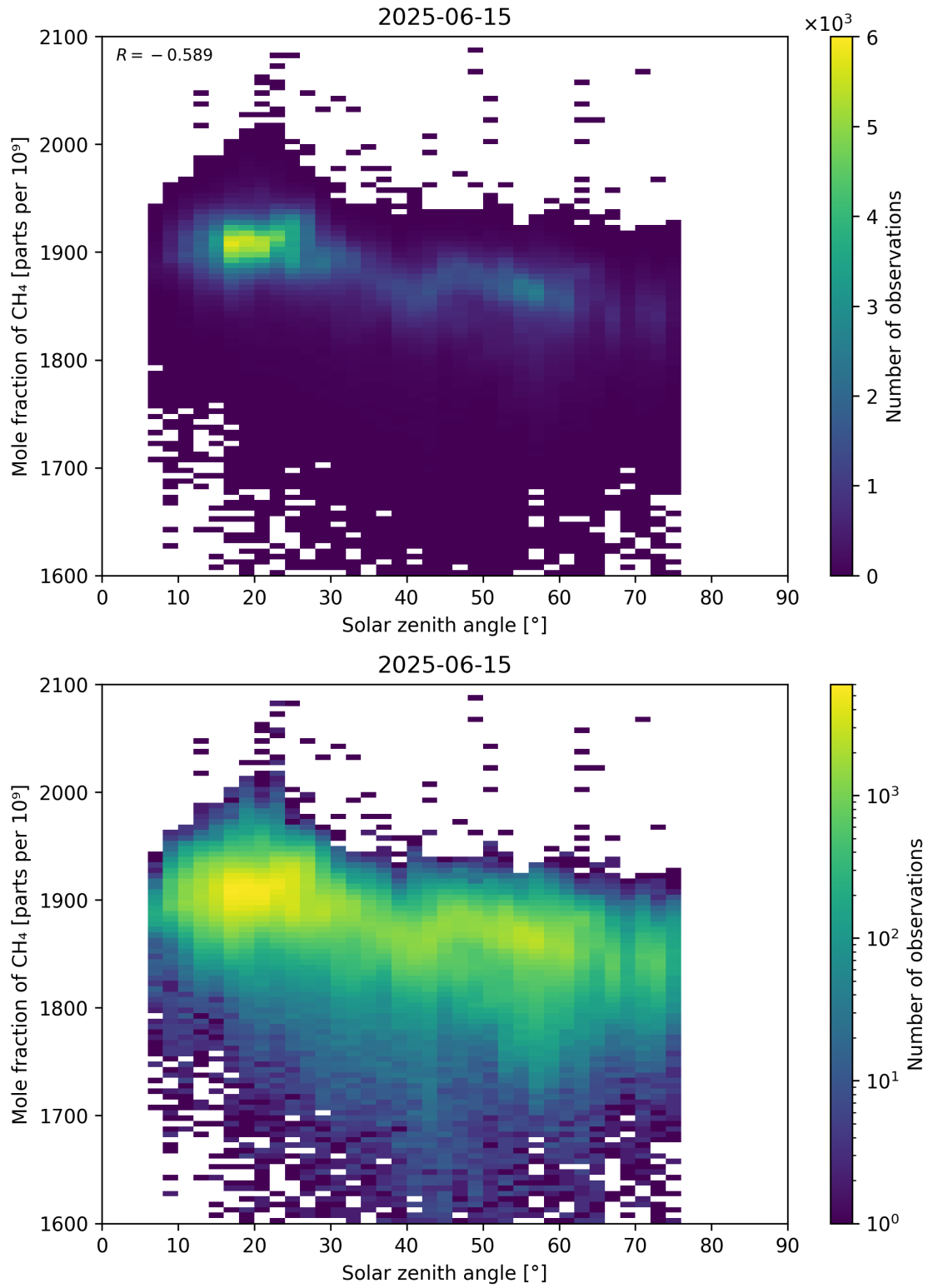
Figure 99: Scatter density plot of “Solar zenith angle” against “Mole fraction of \text{CH}_4 ” for 2025-06-14 to 2025-06-16.
