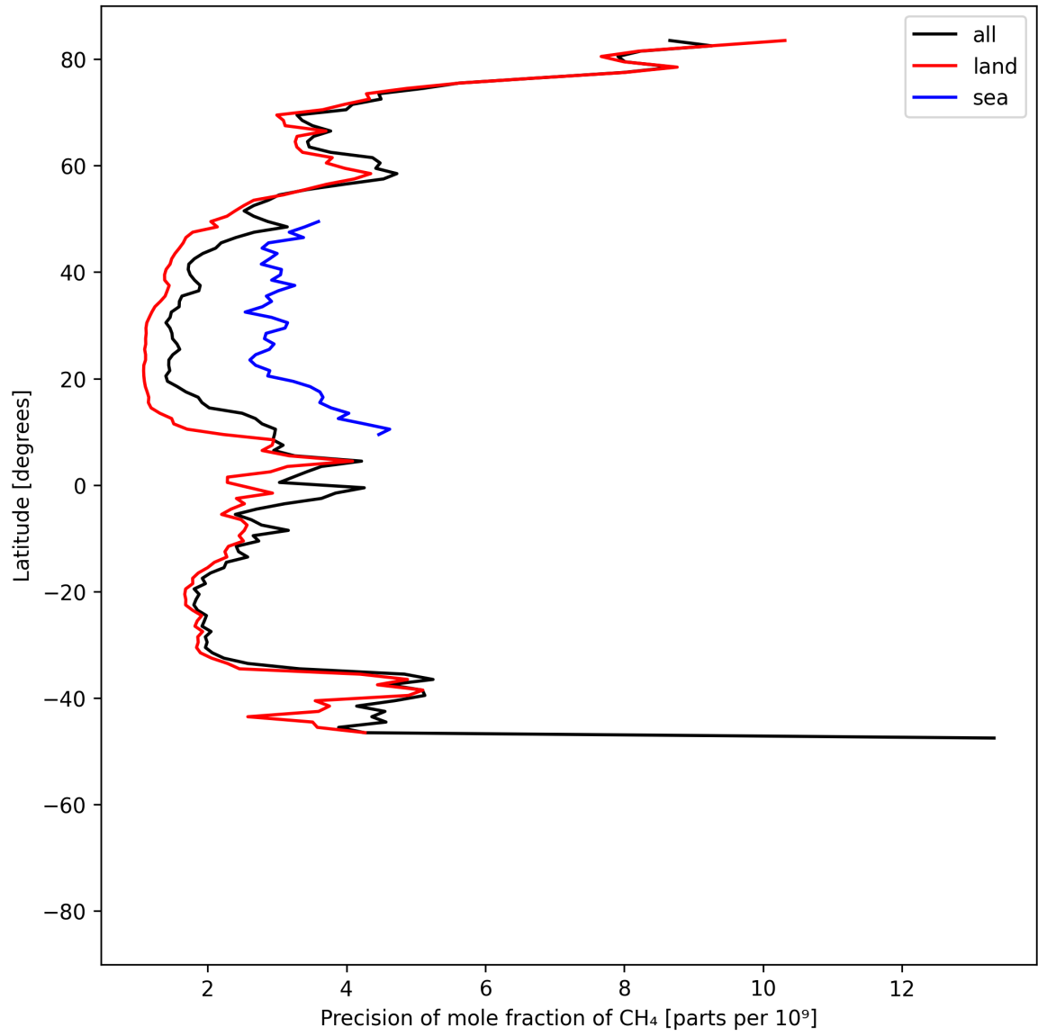
Figure 13: Zonal average of “Precision of mole fraction of CH 4 ” for 2025-06-14 to 2025-06-16.
