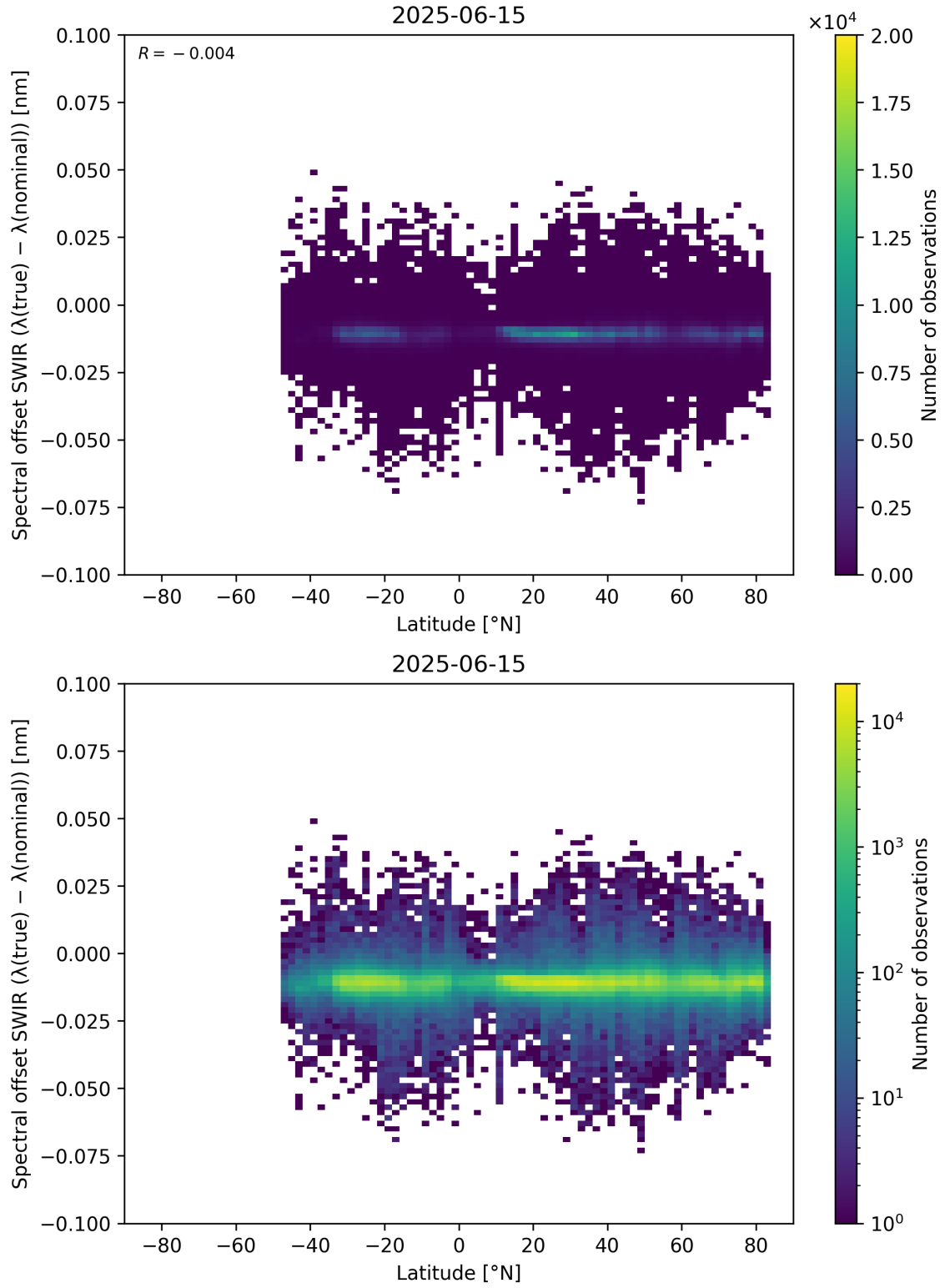
Figure 62: Scatter density plot of “Latitude” against “Spectral offset SWIR ( \lambda_{\text{true}} - \lambda_{\text{nominal}} )” for 2025-06-14 to 2025-06-16.
