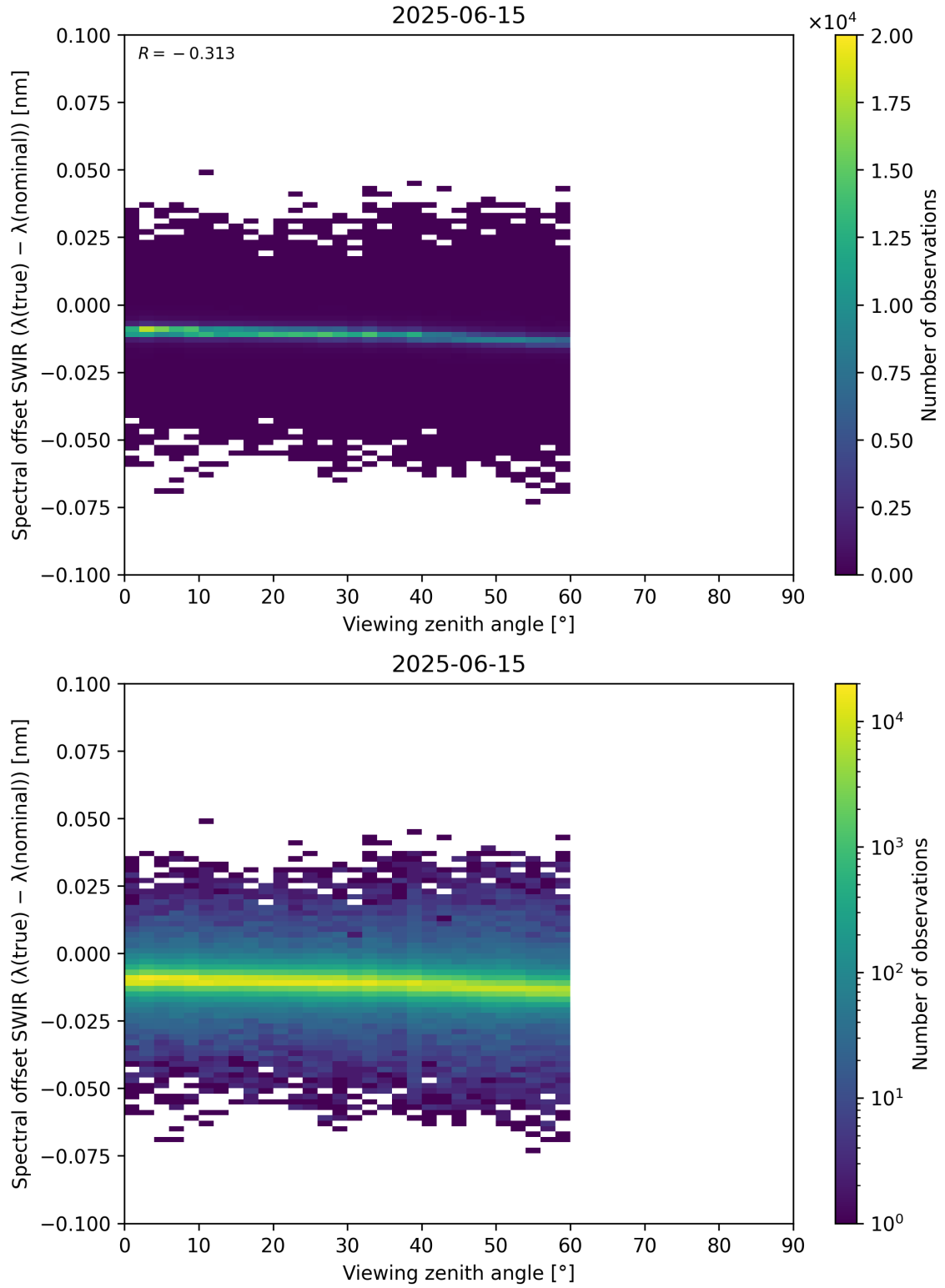
Figure 116: Scatter density plot of “Viewing zenith angle” against “Spectral offset SWIR ( \lambda_{\text{true}} - \lambda_{\text{nominal}} )” for 2025-06-14 to 2025-06-16.
