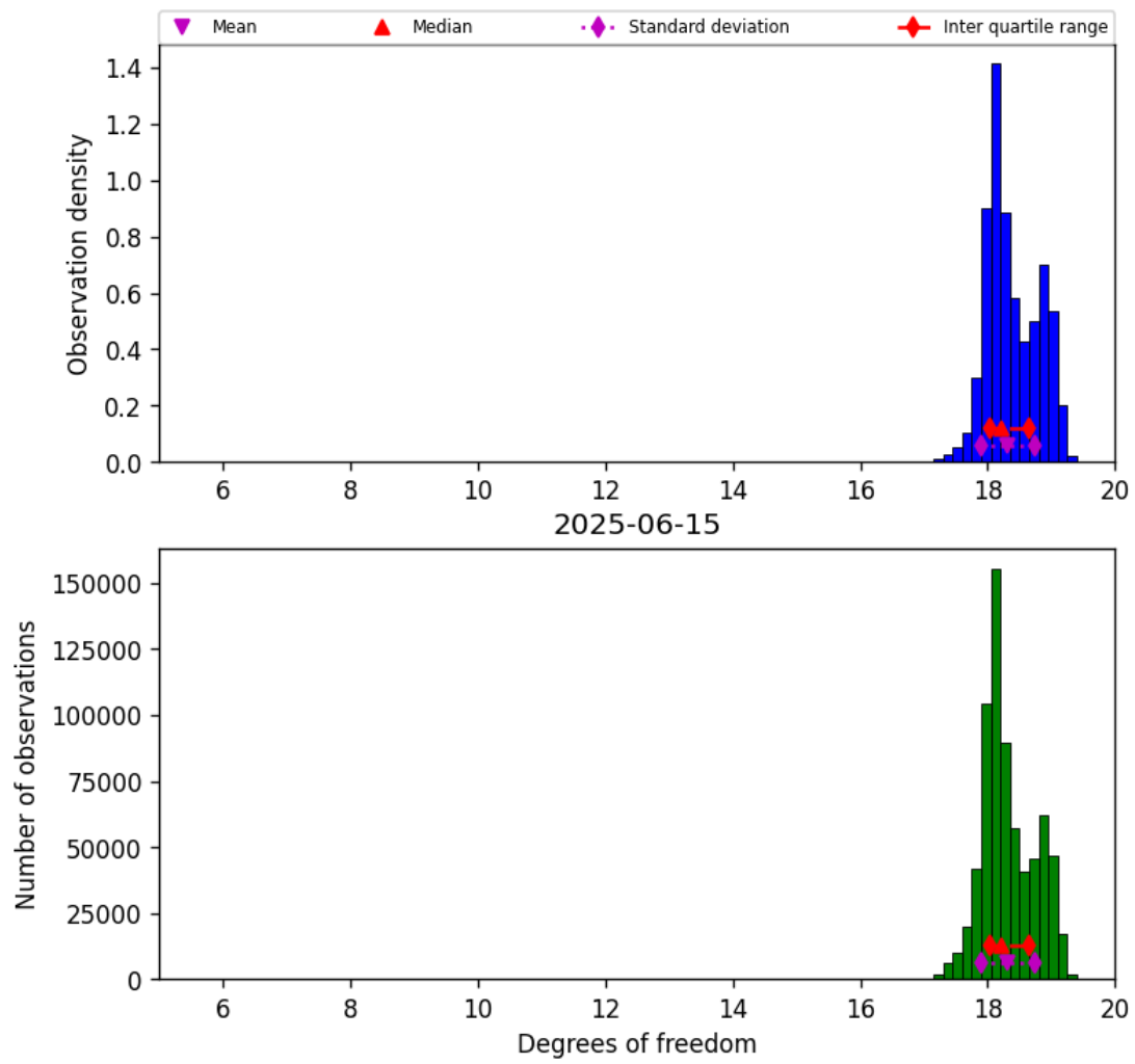
Figure 30: Histogram of “Degrees of freedom” for 2025-06-14 to 2025-06-16
