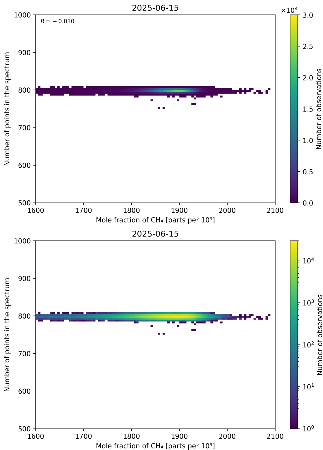
Figure 77: Scatter density plot of “Mole fraction of CH 4 ” against “Number of points in the spectrum” for 2025-06-14 to 2025-06-16.
