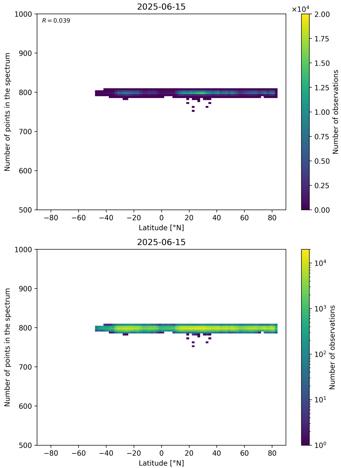
Figure 61: Scatter density plot of “Latitude” against “Number of points in the spectrum” for 2025-06-14 to 2025-06-16.
