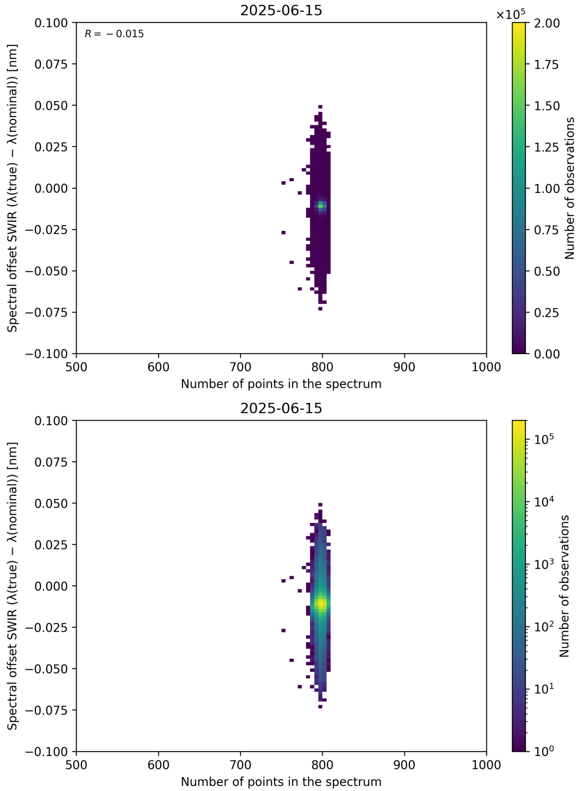
Figure 93: Scatter density plot of “Number of points in the spectrum” against “Spectral offset SWIR ( \lambda_{\text{true}} - \lambda_{\text{nominal}} )” for 2025-06-14 to 2025-06-16.
