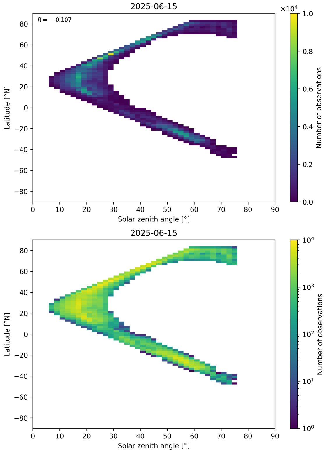
Figure 98: Scatter density plot of “Solar zenith angle” against “Latitude” for 2025-06-14 to 2025-06-16.
