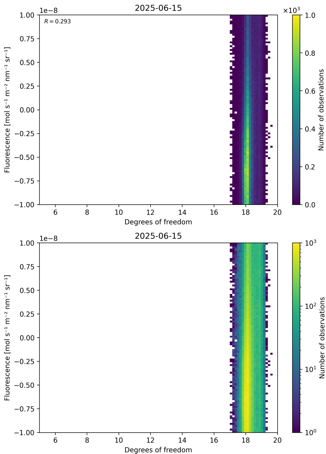
Figure 51: Scatter density plot of “Degrees of freedom” against “Fluorescence” for 2025-06-14 to 2025-06-16.
