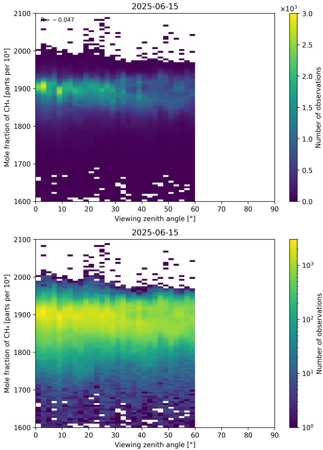
Figure 110: Scatter density plot of “Viewing zenith angle” against “Mole fraction of CH 4 ” for 2025-06-14 to 2025-06-16.
