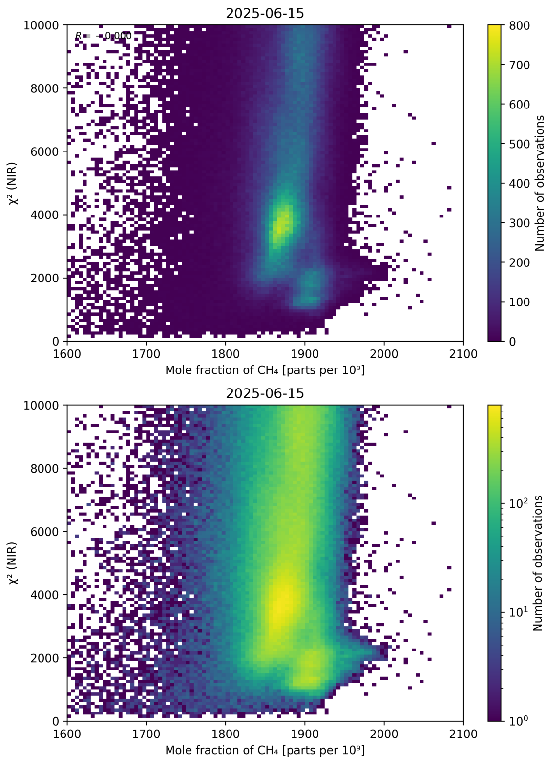
Figure 70: Scatter density plot of “Mole fraction of \text{CH}_4 ” against “ \chi^2 (NIR)” for 2025-06-14 to 2025-06-16.
