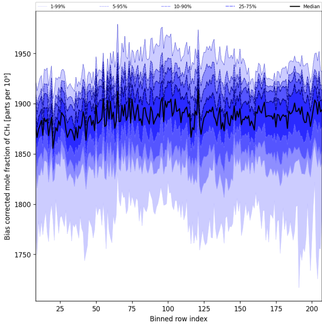
Figure 36: Along track statistics of “Bias corrected mole fraction of CH 4 ” for 2025-06-14 to 2025-06-16
