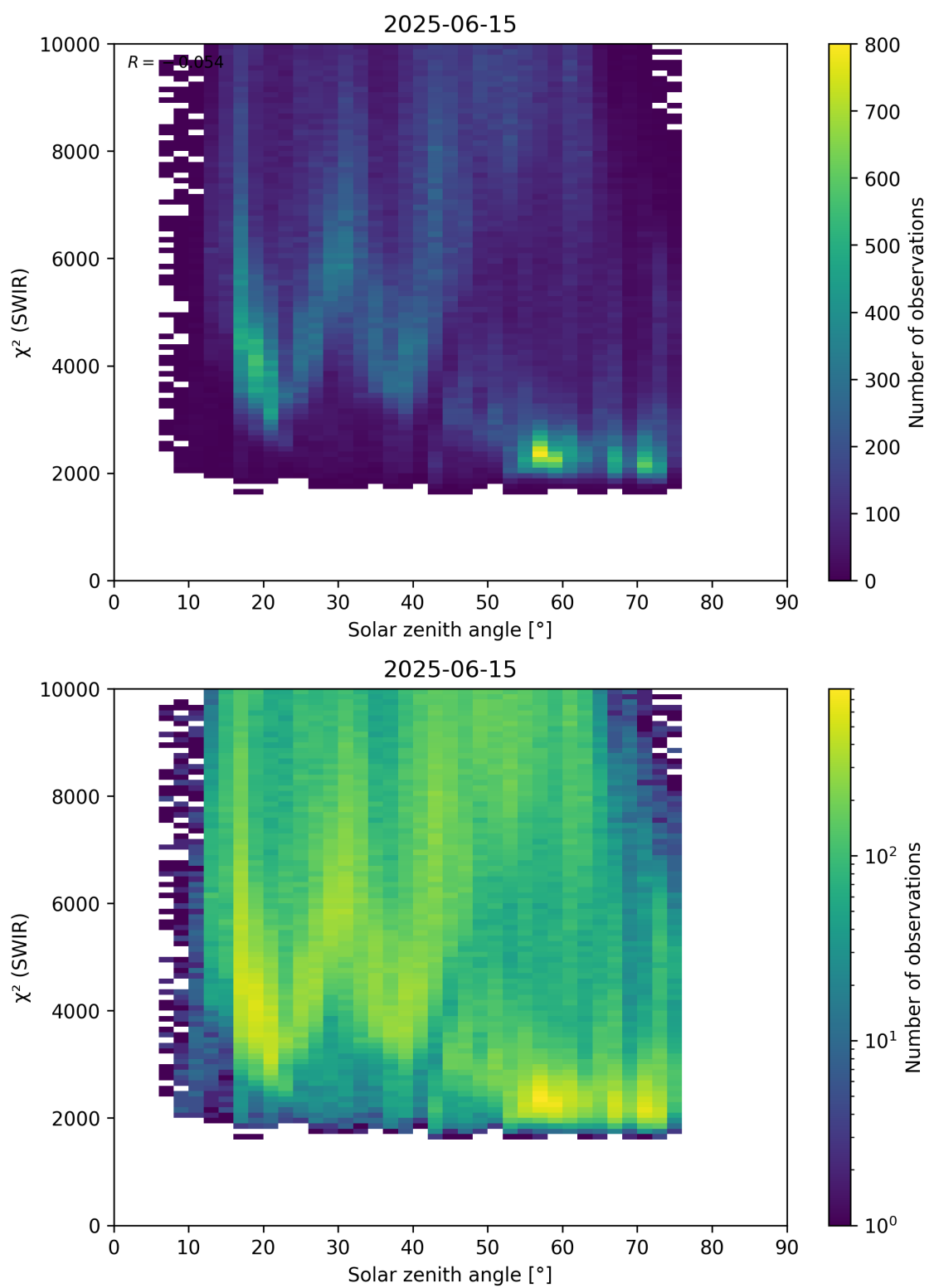
Figure 95: Scatter density plot of “Solar zenith angle” against “ \chi^2 (SWIR)” for 2025-06-14 to 2025-06-16.
