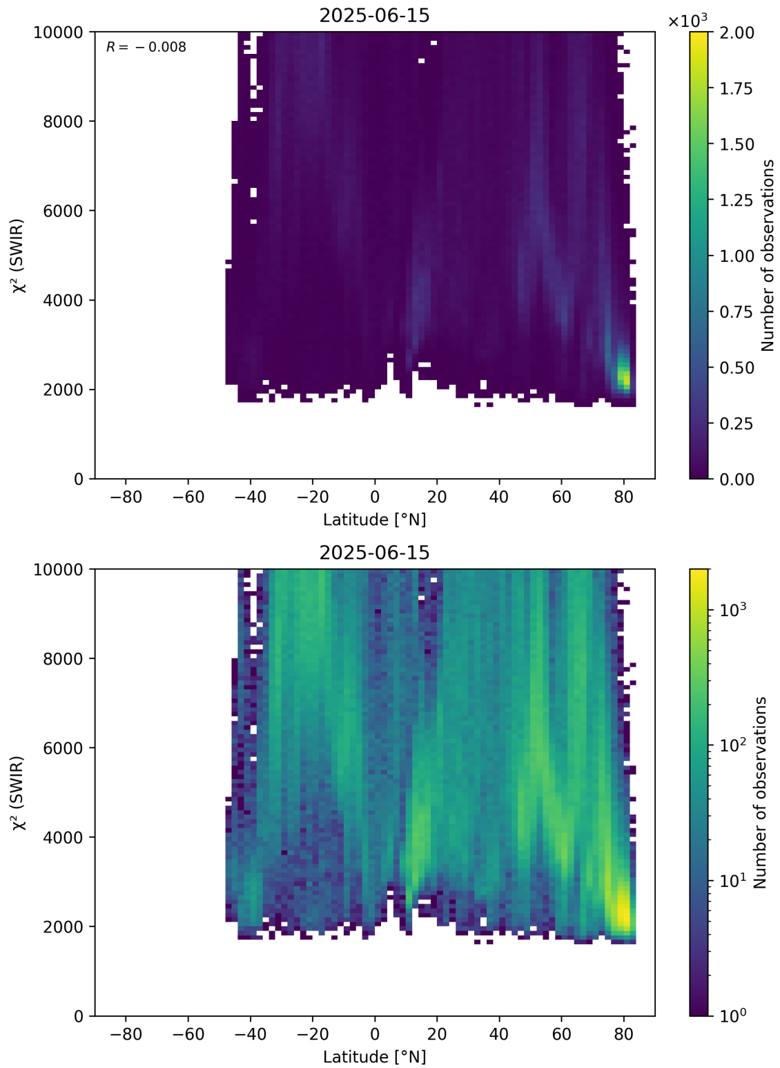
Figure 54: Scatter density plot of “Latitude” against “ \chi^2 (SWIR)” for 2025-06-14 to 2025-06-16.
