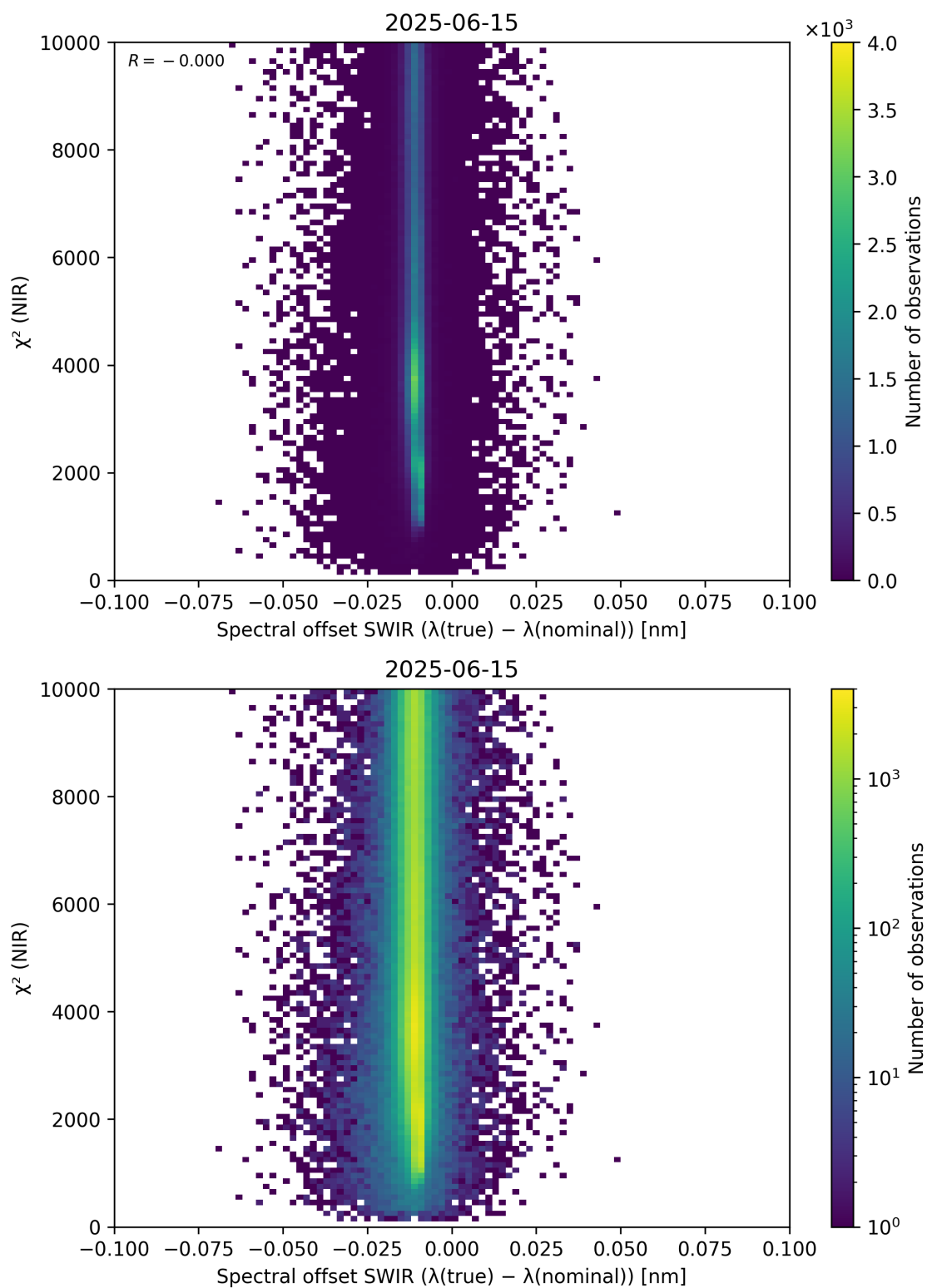
Figure 117: Scatter density plot of “Spectral offset SWIR ( \lambda_{\text{true}} - \lambda_{\text{nominal}} )” against “ \chi^2 (NIR)” for 2025-06-14 to 2025-06-16.
