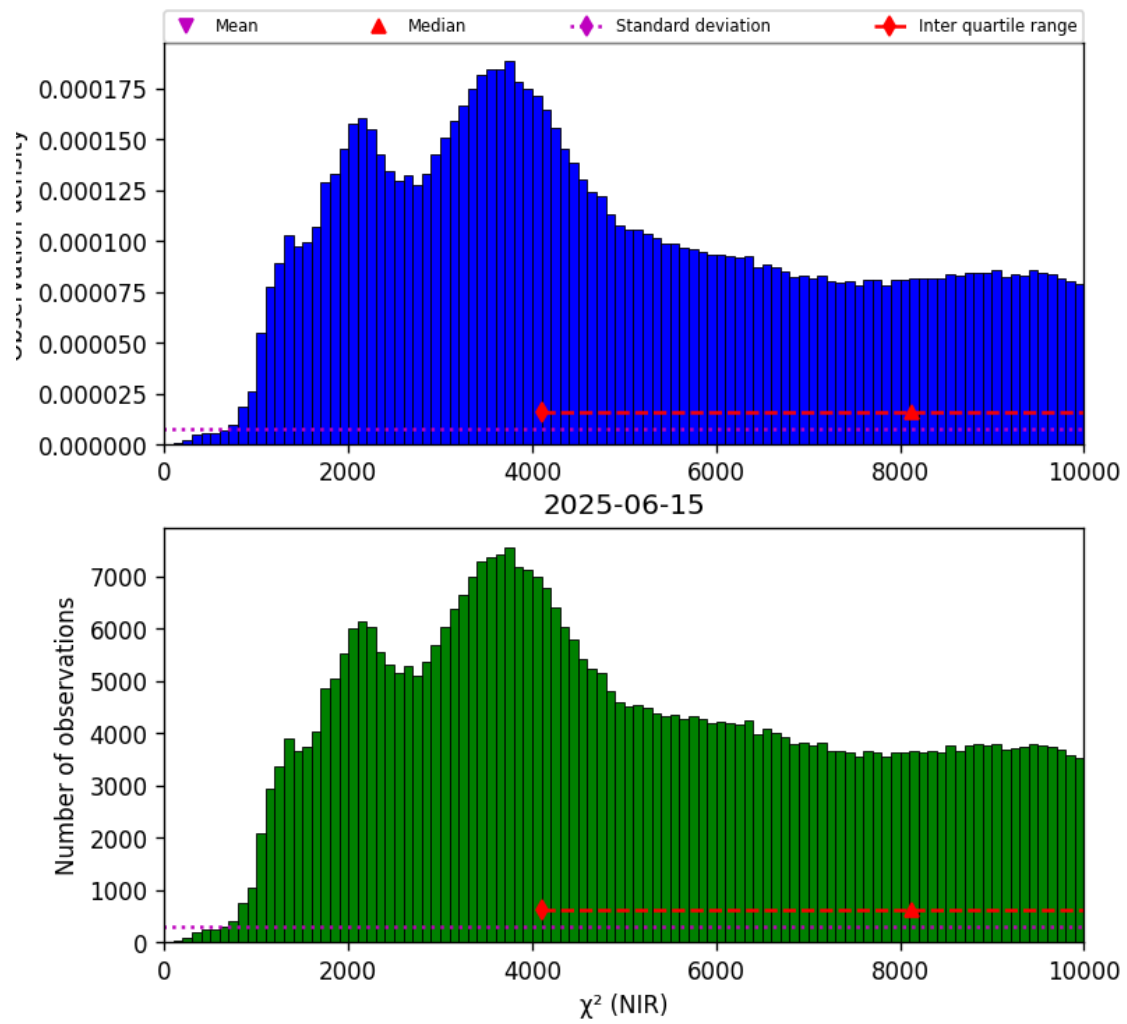
Figure 29: Histogram of “ \chi^2 (NIR)” for 2025-06-14 to 2025-06-16
