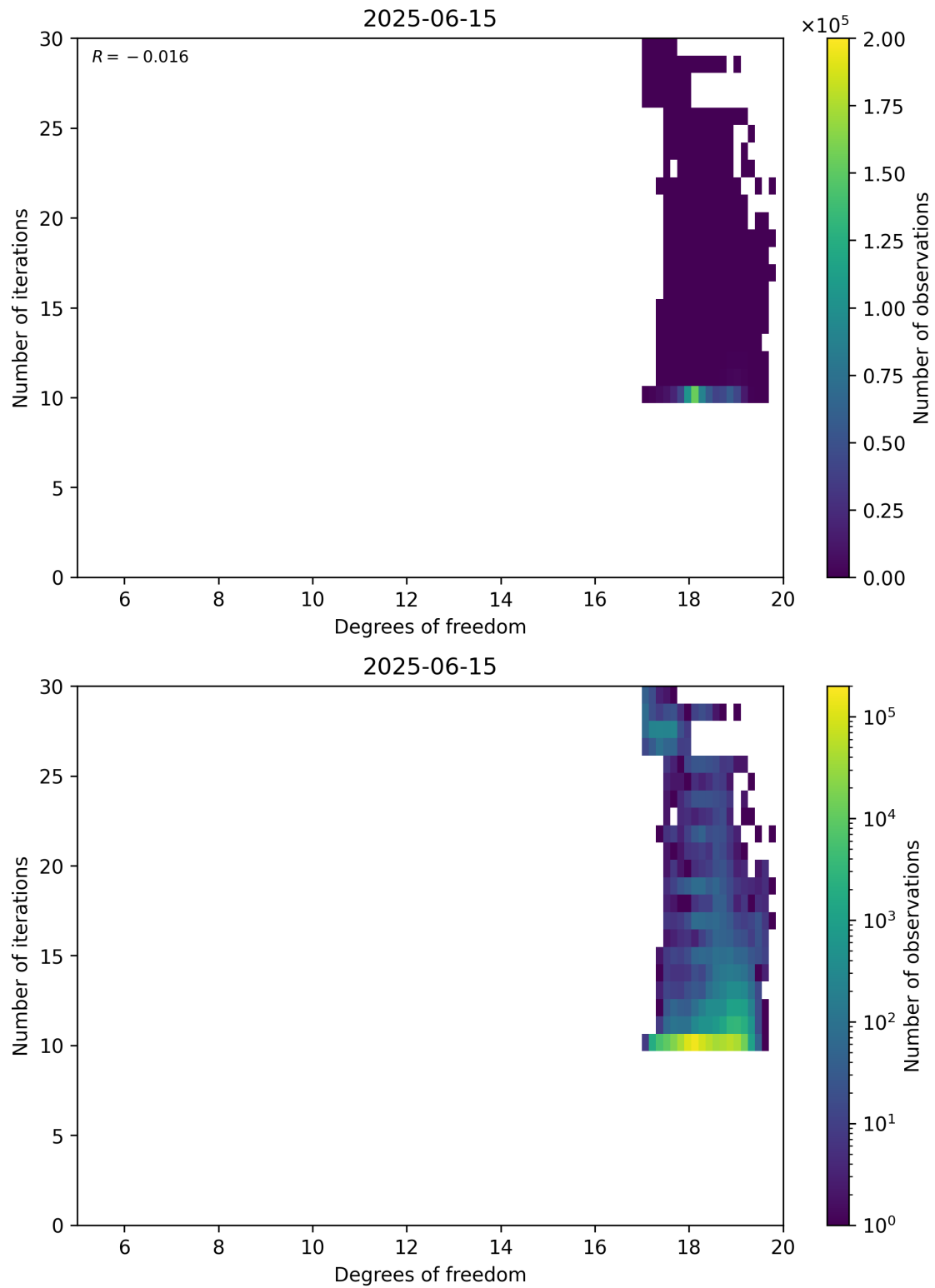
Figure 52: Scatter density plot of “Degrees of freedom” against “Number of iterations” for 2025-06-14 to 2025-06-16.
