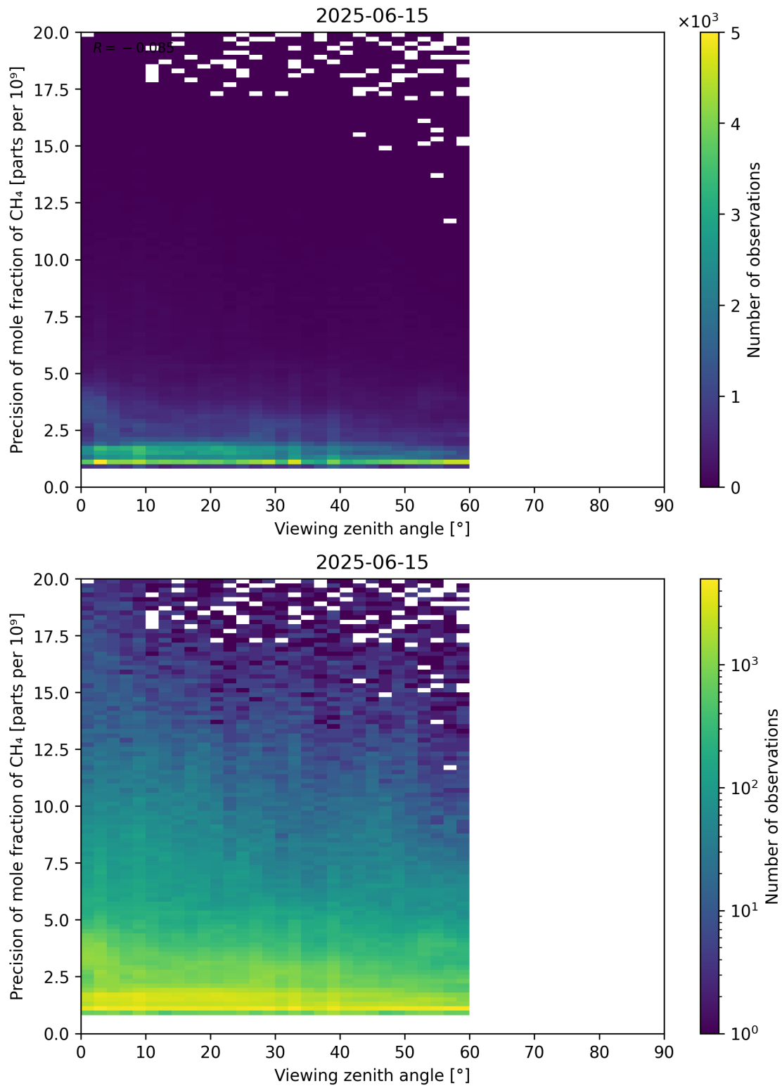
Figure 112: Scatter density plot of “Viewing zenith angle” against “Precision of mole fraction of CH 4 ” for 2025-06-14 to 2025-06-16.
