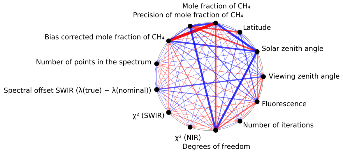
Figure 1: Map of correlation graph for 2025-06-14 to 2025-06-16.
