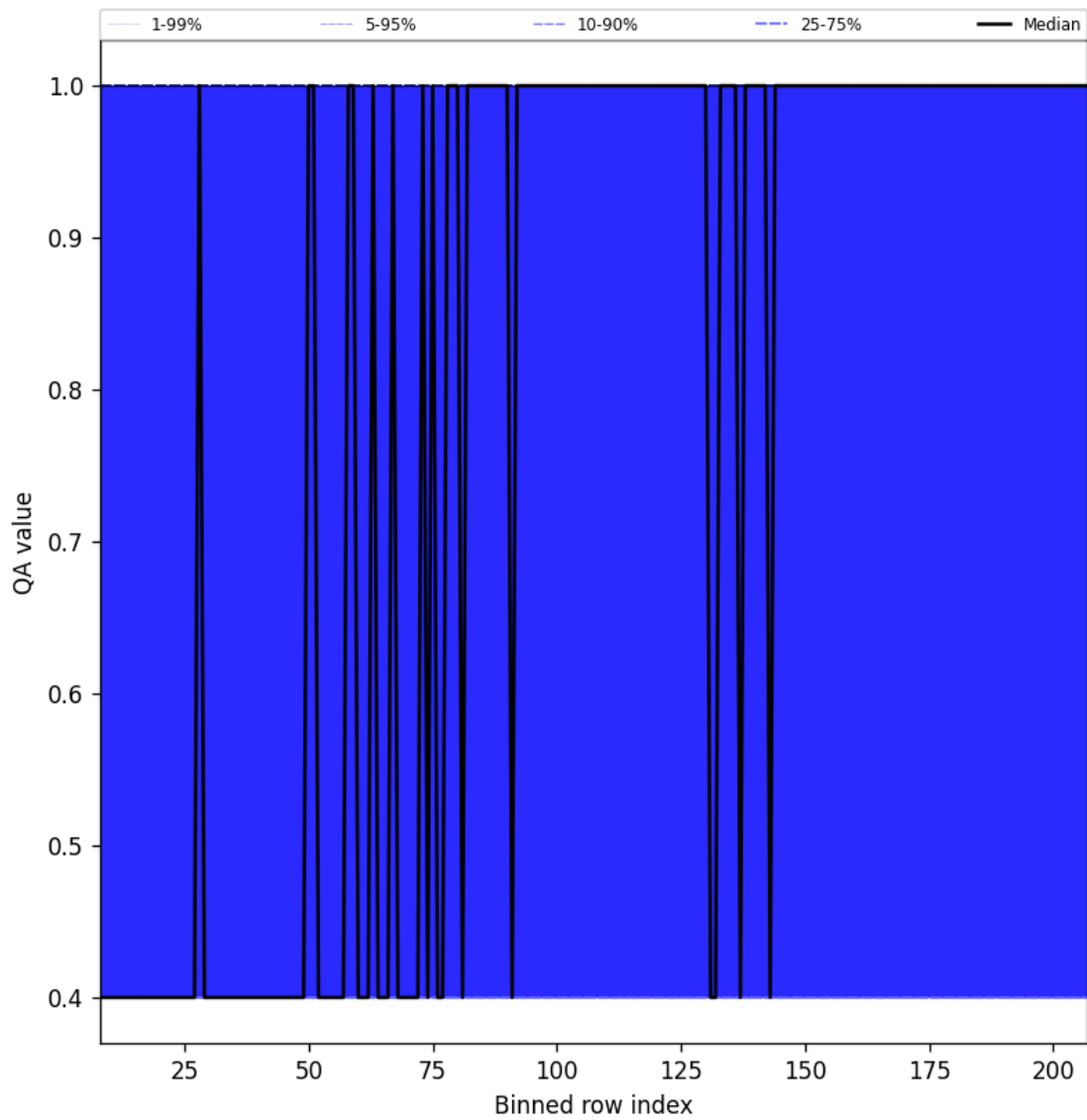
Figure 33: Along track statistics of “QA value” for 2025-06-14 to 2025-06-16
