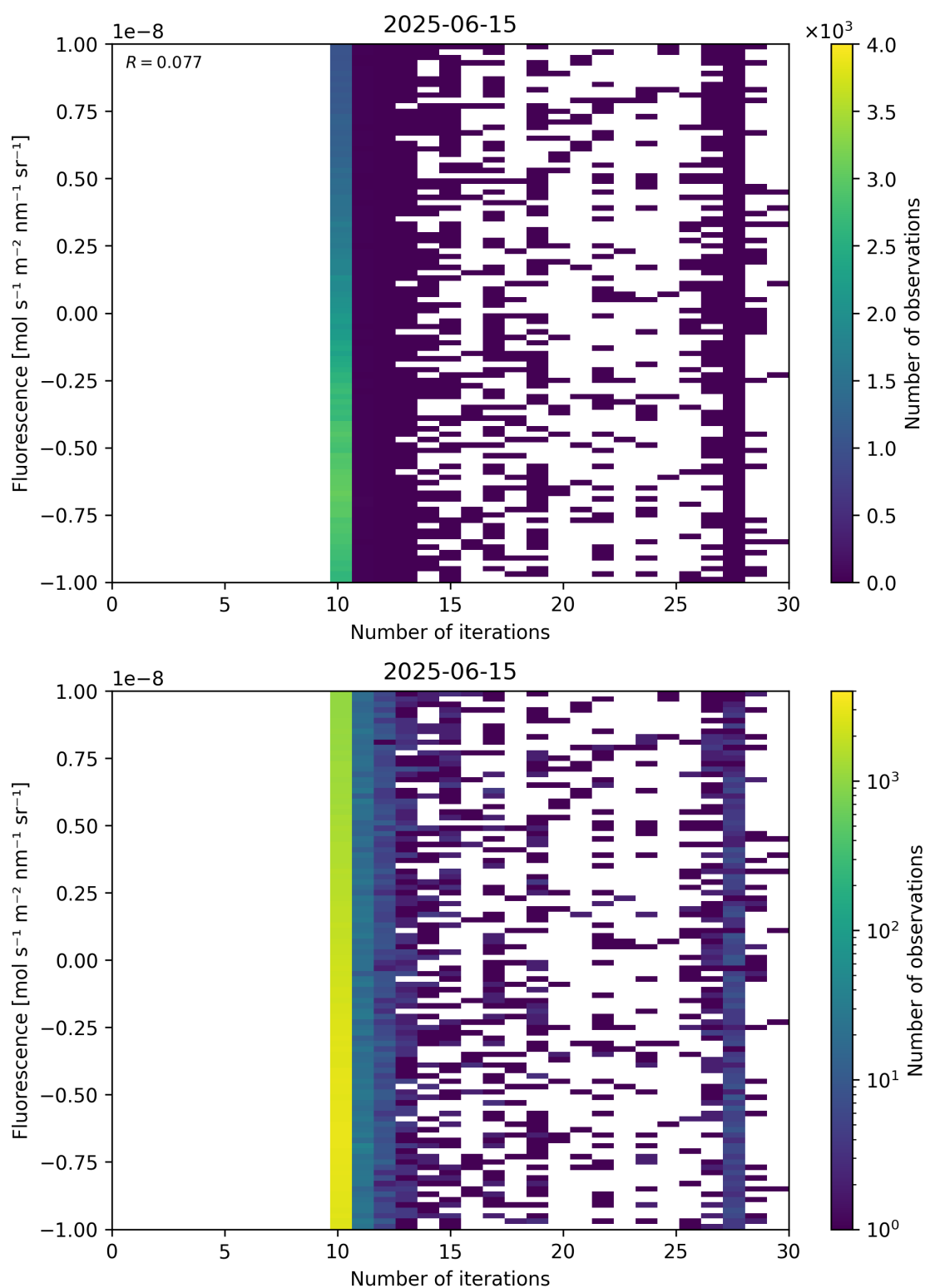
Figure 87: Scatter density plot of “Number of iterations” against “Fluorescence” for 2025-06-14 to 2025-06-16.
