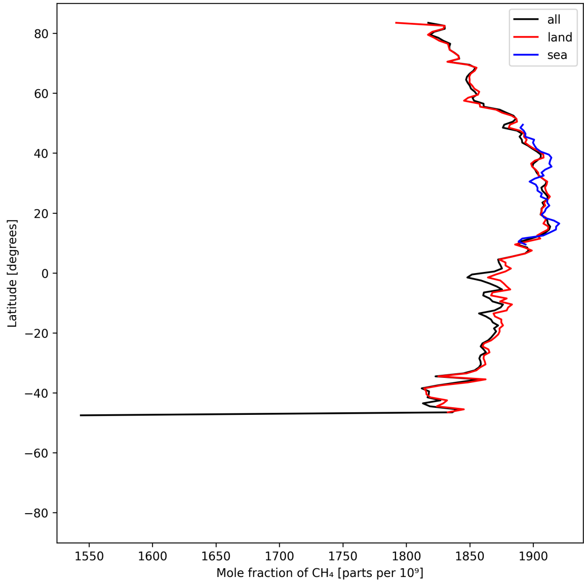
Figure 12: Zonal average of “Mole fraction of CH 4 ” for 2025-06-14 to 2025-06-16.
