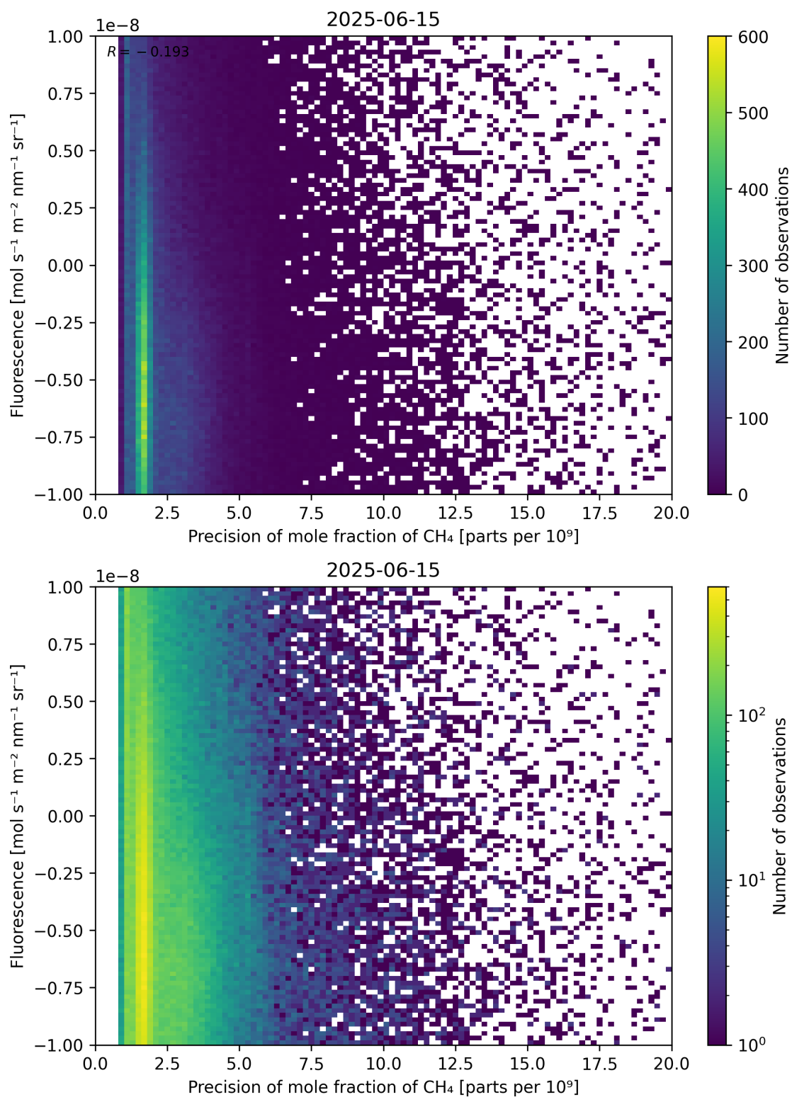
Figure 81: Scatter density plot of “Precision of mole fraction of \text{CH}_4 ” against “Fluorescence” for 2025-06-14 to 2025-06-16.
