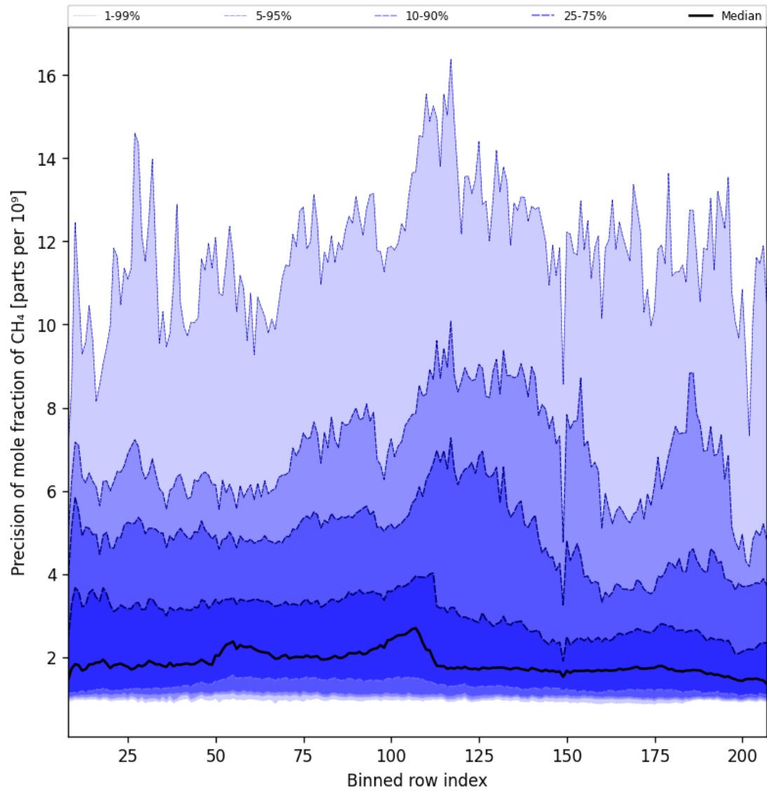
Figure 35: Along track statistics of “Precision of mole fraction of CH 4 ” for 2025-06-14 to 2025-06-16
