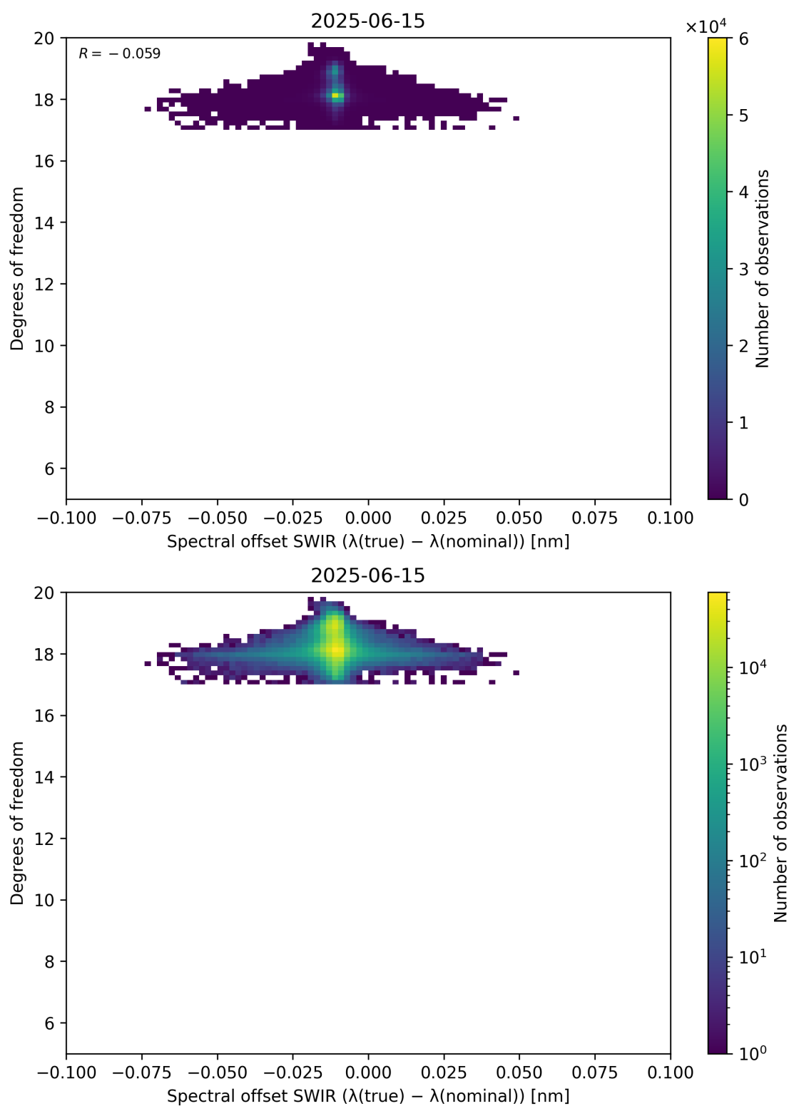
Figure 119: Scatter density plot of “Spectral offset SWIR ( \lambda_{\text{true}} - \lambda_{\text{nominal}} )” against “Degrees of freedom” for 2025-06-14 to 2025-06-16.
