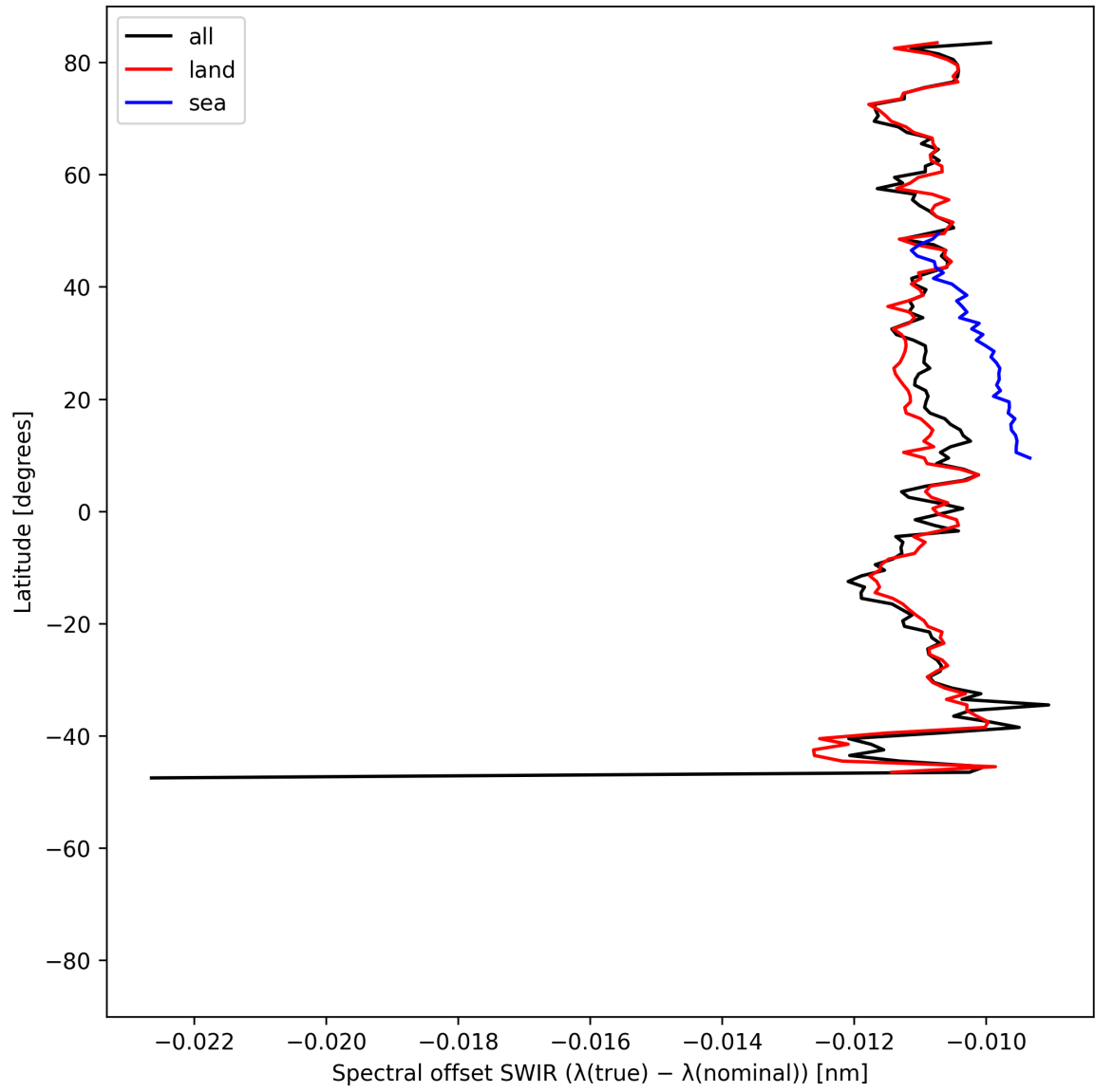
Figure 16: Zonal average of “Spectral offset SWIR ( \lambda_{\text{true}} - \lambda_{\text{nominal}} )” for 2025-06-14 to 2025-06-16.
