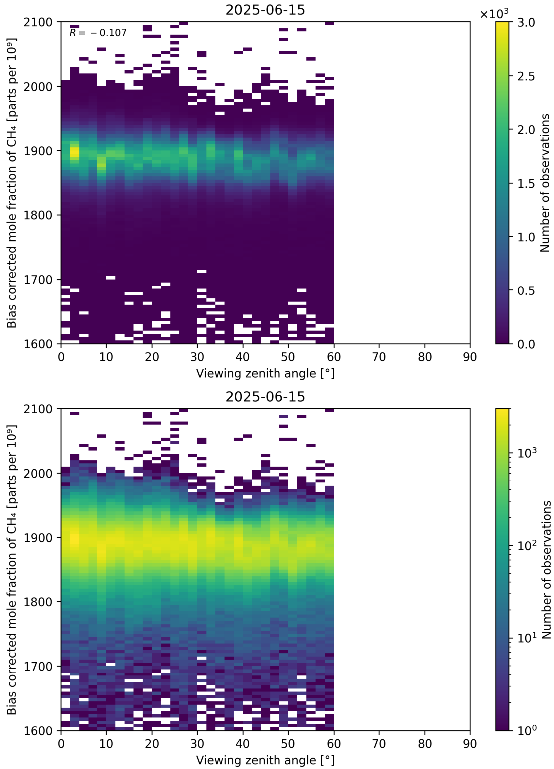
Figure 111: Scatter density plot of “Viewing zenith angle” against “Bias corrected mole fraction of CH 4 ” for 2025-06-14 to 2025-06-16.
