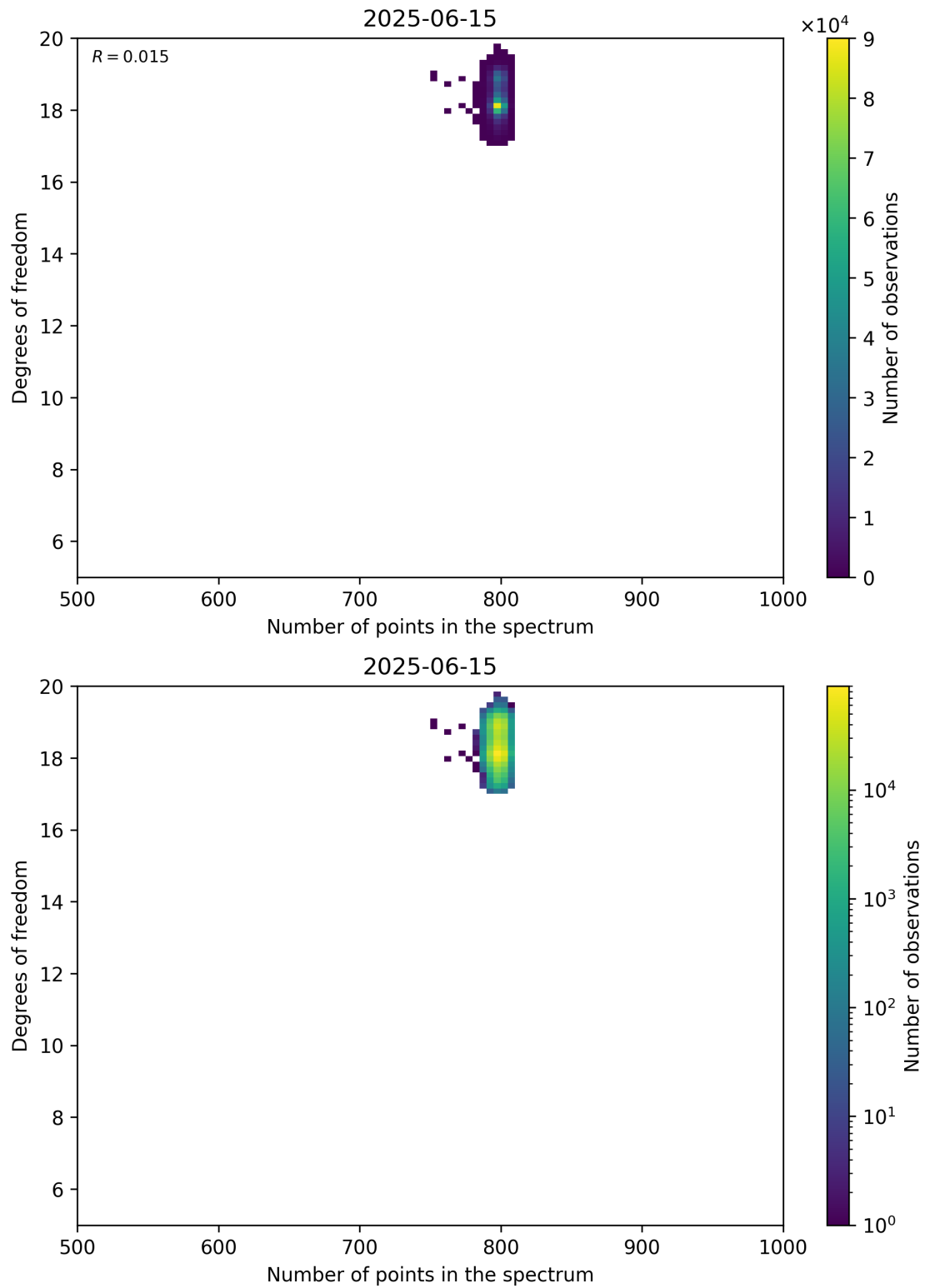
Figure 90: Scatter density plot of “Number of points in the spectrum” against “Degrees of freedom” for 2025-06-14 to 2025-06-16.
