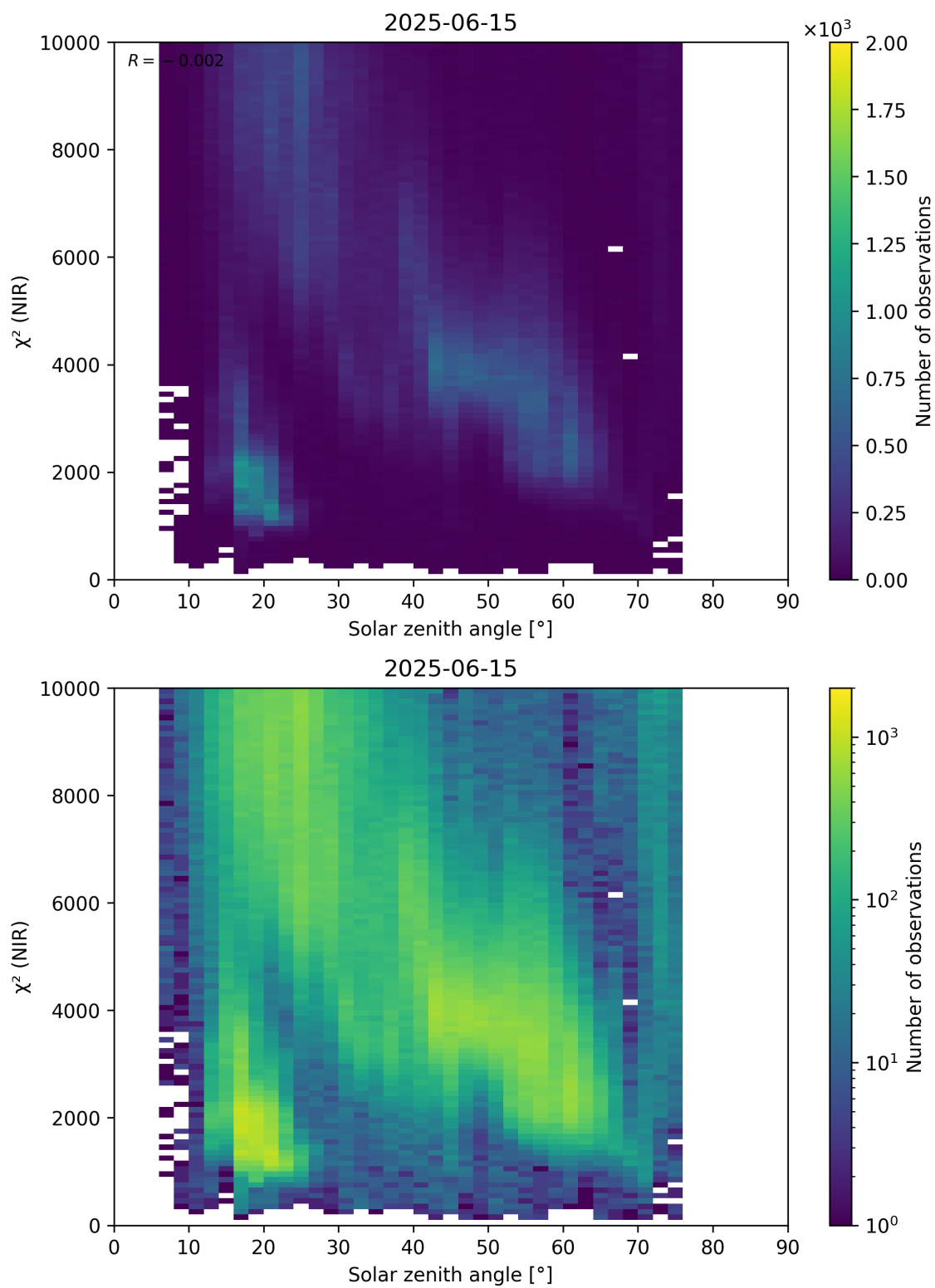
Figure 94: Scatter density plot of “Solar zenith angle” against “ \chi^2 (NIR)” for 2025-06-14 to 2025-06-16.
