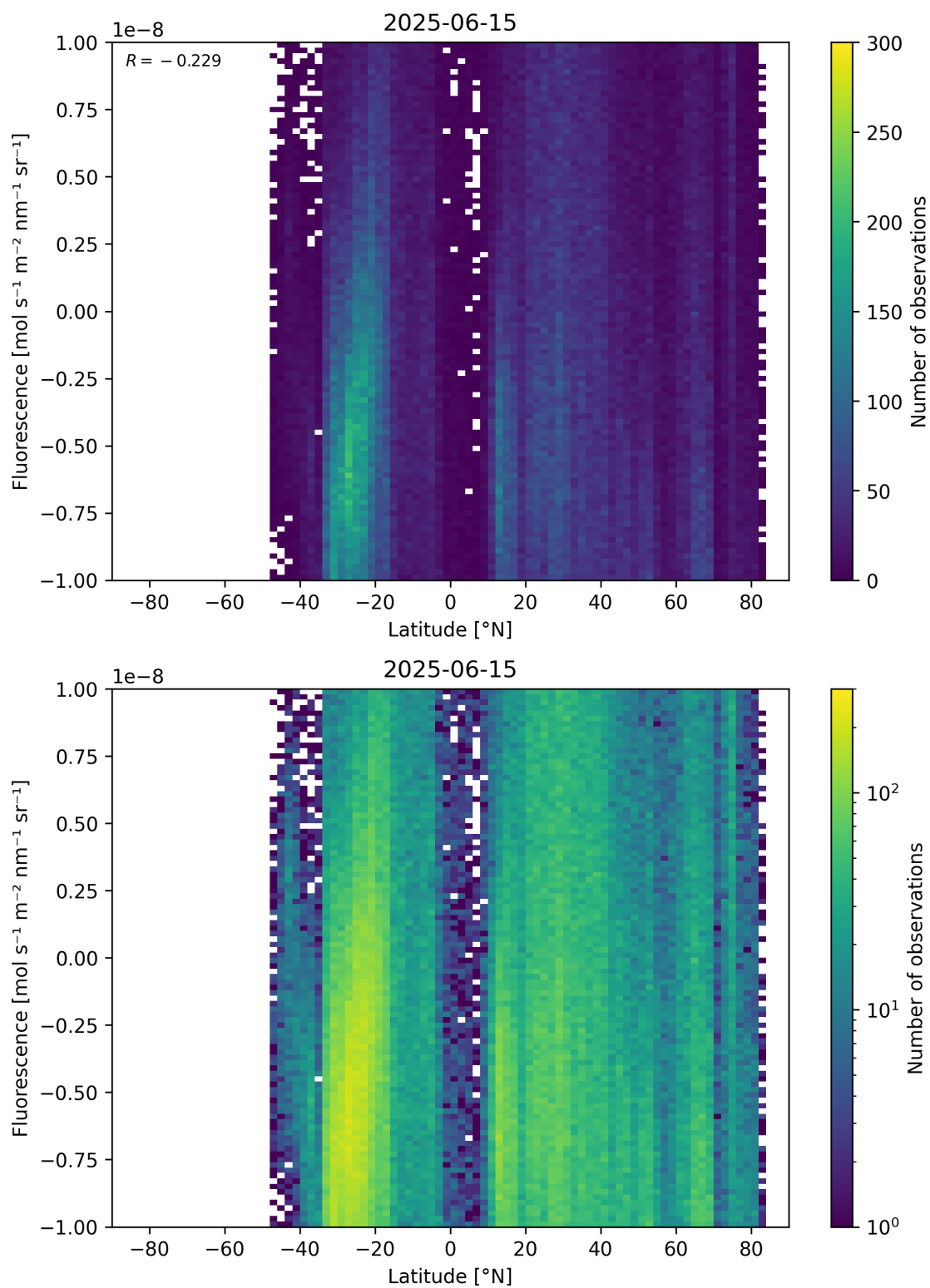
Figure 56: Scatter density plot of “Latitude” against “Fluorescence” for 2025-06-14 to 2025-06-16.
