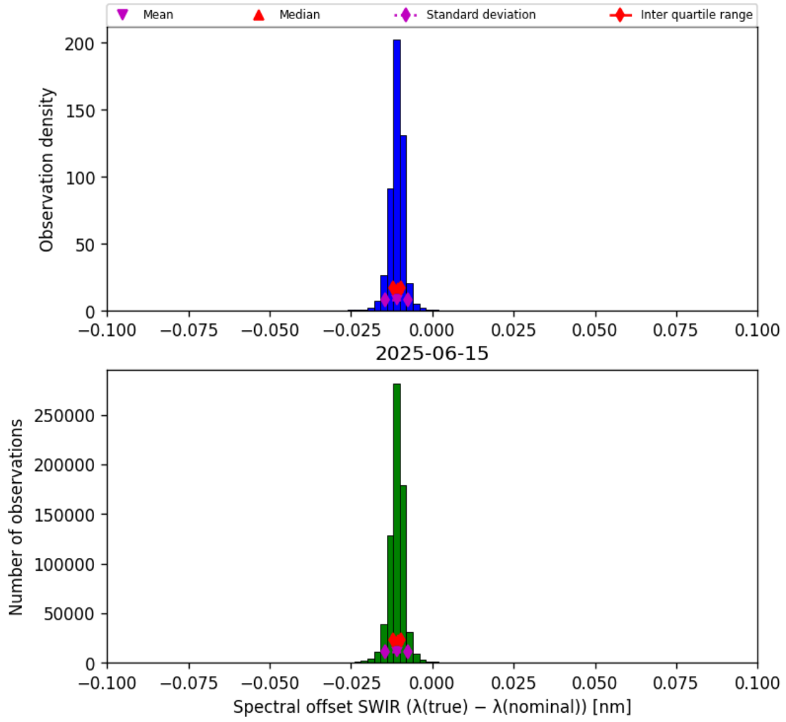
Figure 27: Histogram of “Spectral offset SWIR ( \lambda_{\text{true}} - \lambda_{\text{nominal}} )” for 2025-06-14 to 2025-06-16
