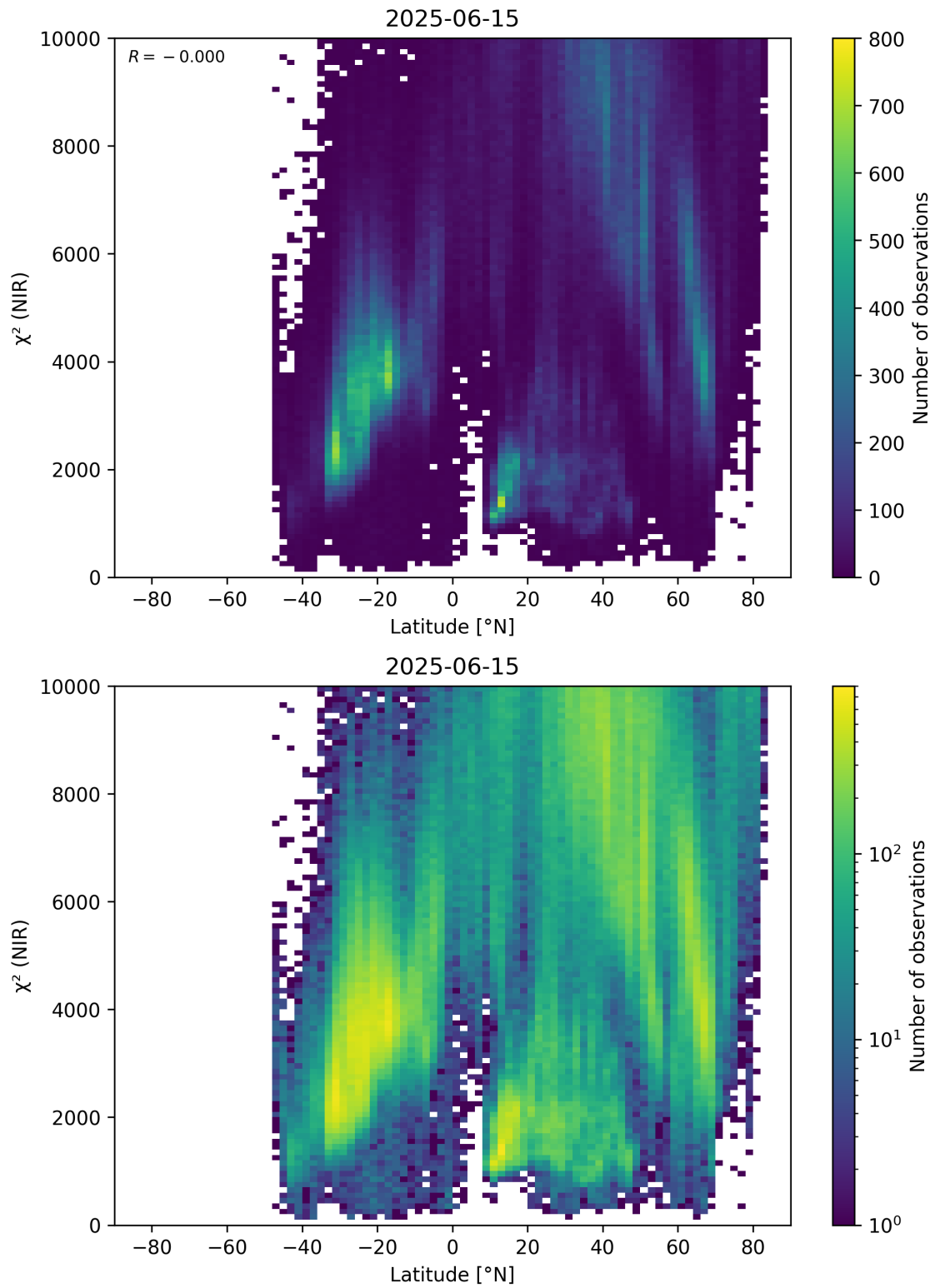
Figure 53: Scatter density plot of “Latitude” against “ \chi^2 (NIR)” for 2025-06-14 to 2025-06-16.
