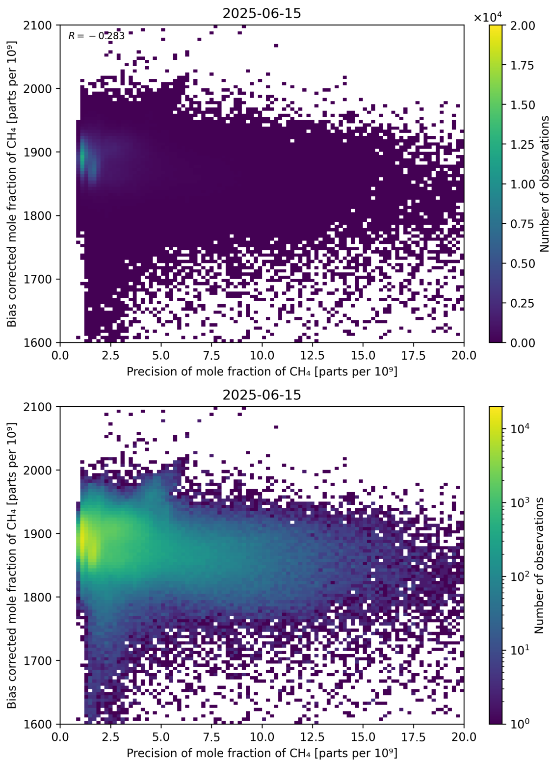
Figure 82: Scatter density plot of “Precision of mole fraction of CH 4 ” against “Bias corrected mole fraction of CH 4 ” for 2025-06-14 to 2025-06-16.
