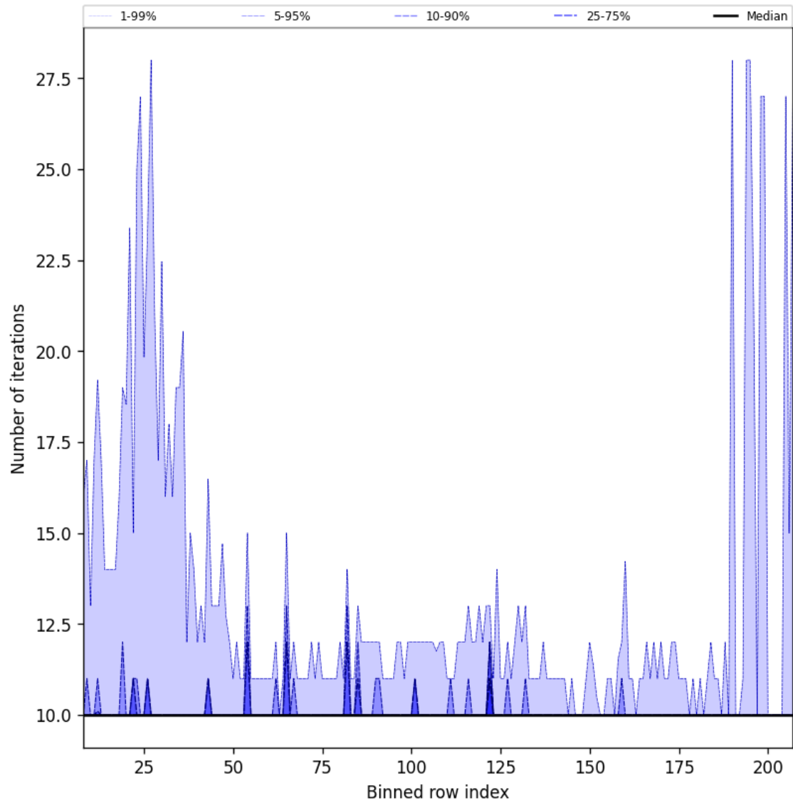
Figure 42: Along track statistics of “Number of iterations” for 2025-06-14 to 2025-06-16
