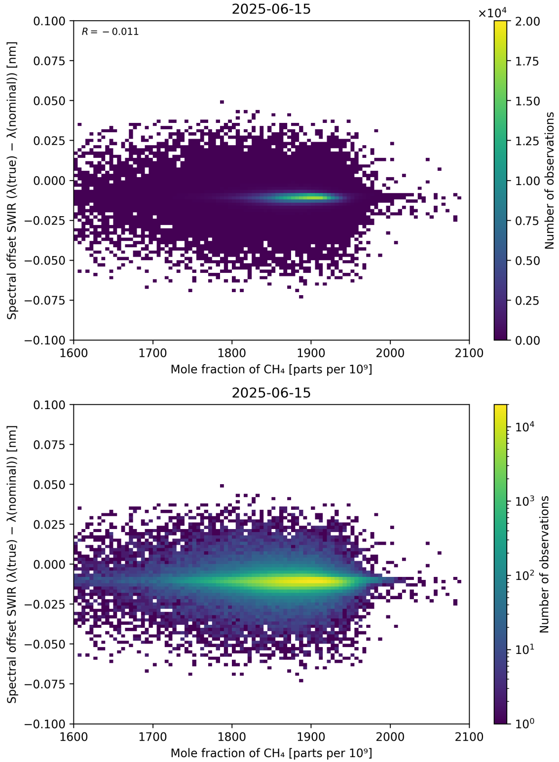
Figure 86: Scatter density plot of “Mole fraction of CH 4 ” against “Spectral offset SWIR ( \lambda_{\text{true}} - \lambda_{\text{nominal}} )” for 2025-06-14 to 2025-06-16.
