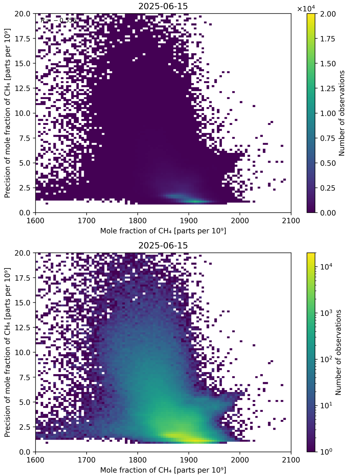
Figure 75: Scatter density plot of “Mole fraction of CH 4 ” against “Precision of mole fraction of CH 4 ” for 2025-06-14 to 2025-06-16.
