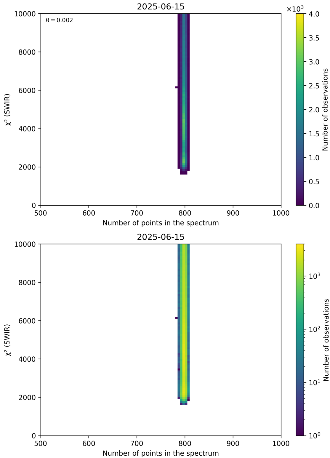
Figure 89: Scatter density plot of “Number of points in the spectrum” against “ \chi^2 (SWIR)” for 2025-06-14 to 2025-06-16.
