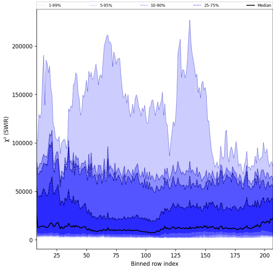
Figure 39: Along track statistics of “ \chi^2 (SWIR)” for 2025-06-14 to 2025-06-16
