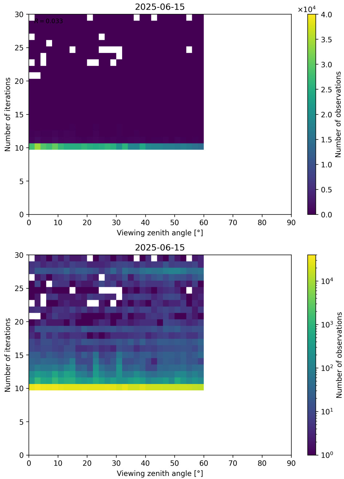
Figure 113: Scatter density plot of “Viewing zenith angle” against “Number of iterations” for 2025-06-14 to 2025-06-16.
