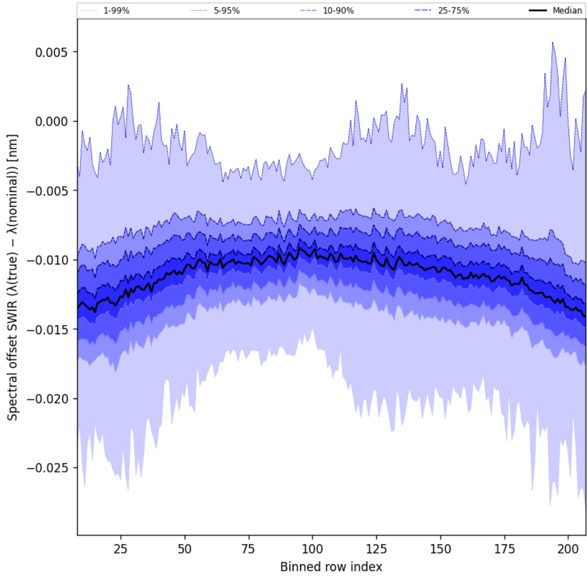
Figure 38: Along track statistics of “Spectral offset SWIR ( \lambda_{\text{true}} - \lambda_{\text{nominal}} )” for 2025-06-14 to 2025-06-16
