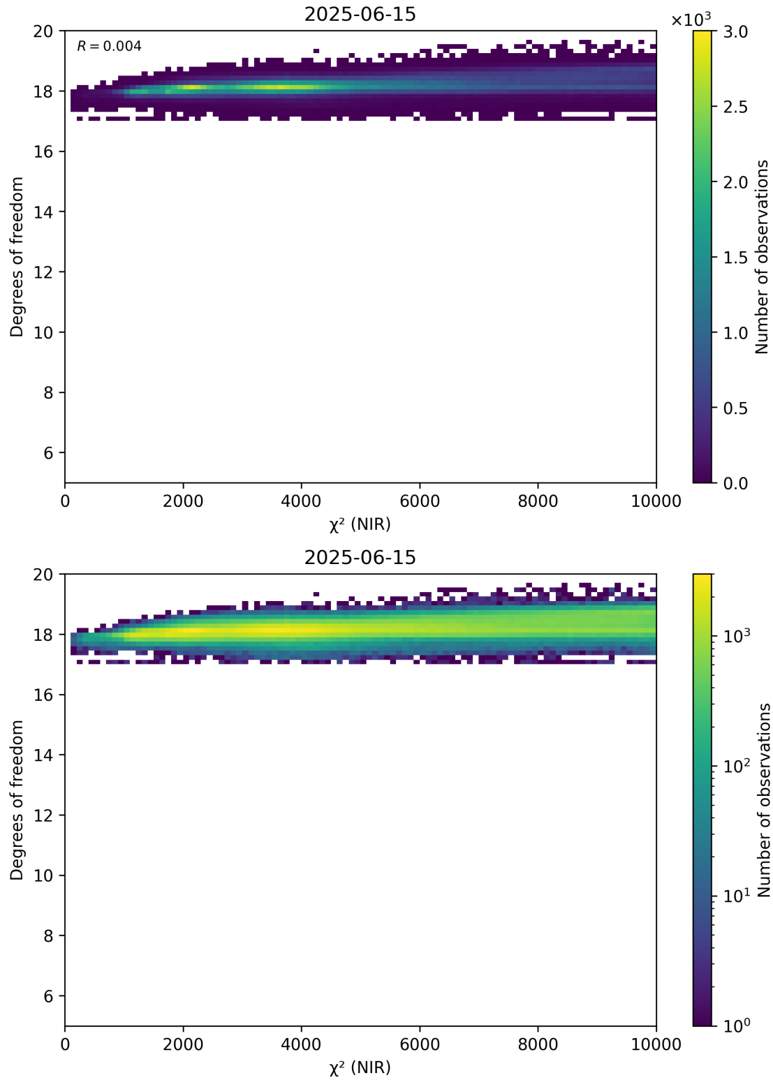
Figure 44: Scatter density plot of “ \chi^2 (NIR)” against “Degrees of freedom” for 2025-06-14 to 2025-06-16.
