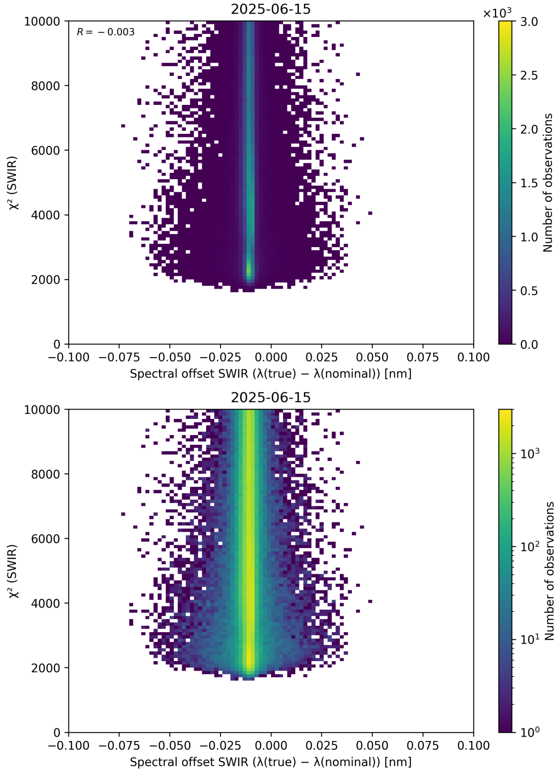
Figure 118: Scatter density plot of “Spectral offset SWIR ( \lambda_{\text{true}} - \lambda_{\text{nominal}} )” against “ \chi^2 (SWIR)” for 2025-06-14 to 2025-06-16.
