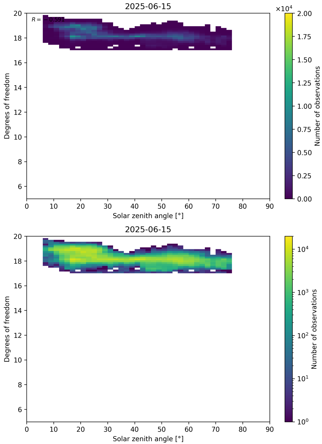
Figure 96: Scatter density plot of “Solar zenith angle” against “Degrees of freedom” for 2025-06-14 to 2025-06-16.
