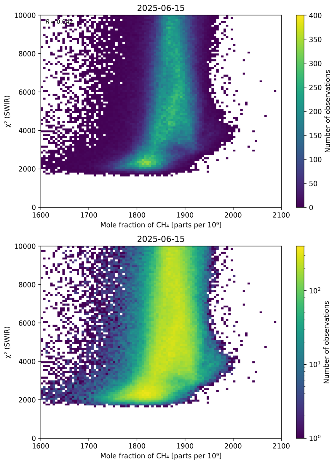
Figure 71: Scatter density plot of “Mole fraction of \text{CH}_4 ” against “ \chi^2 (SWIR)” for 2025-06-14 to 2025-06-16.
