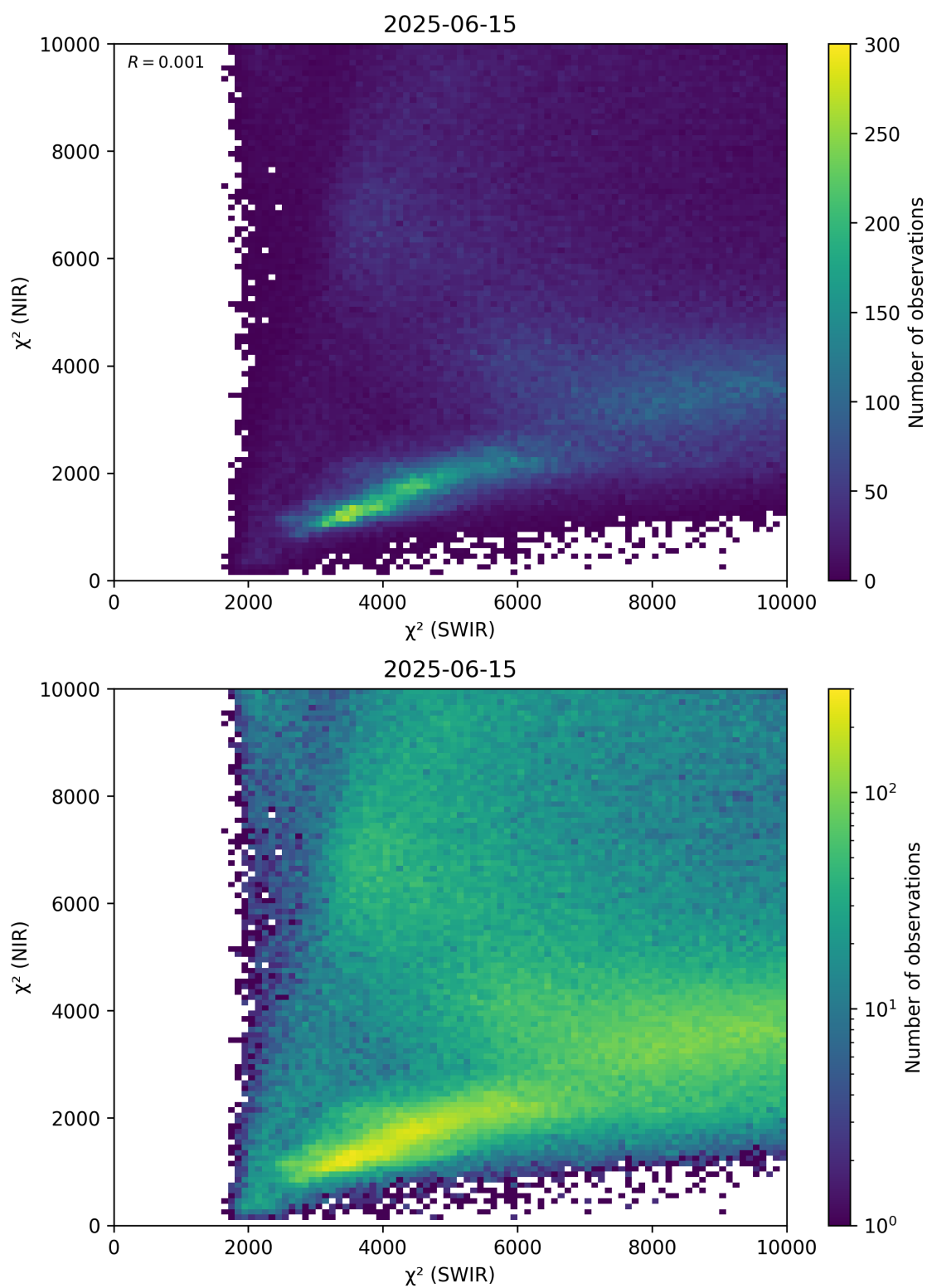
Figure 47: Scatter density plot of “ \chi^2 (SWIR)” against “ \chi^2 (NIR)” for 2025-06-14 to 2025-06-16.
