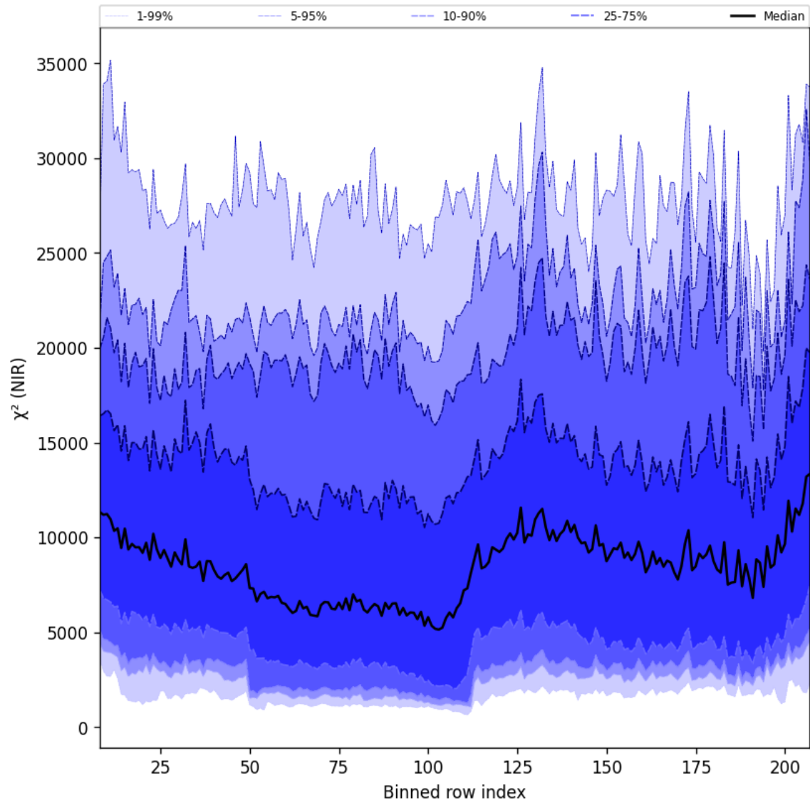
Figure 40: Along track statistics of “ \chi^2 (NIR)” for 2025-06-14 to 2025-06-16
