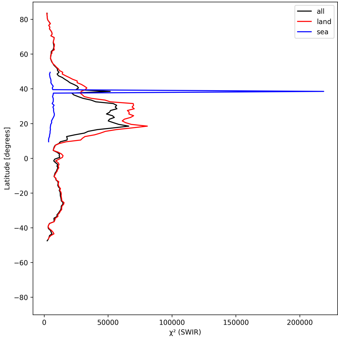
Figure 17: Zonal average of “ \chi^2 (SWIR)” for 2025-06-14 to 2025-06-16.
