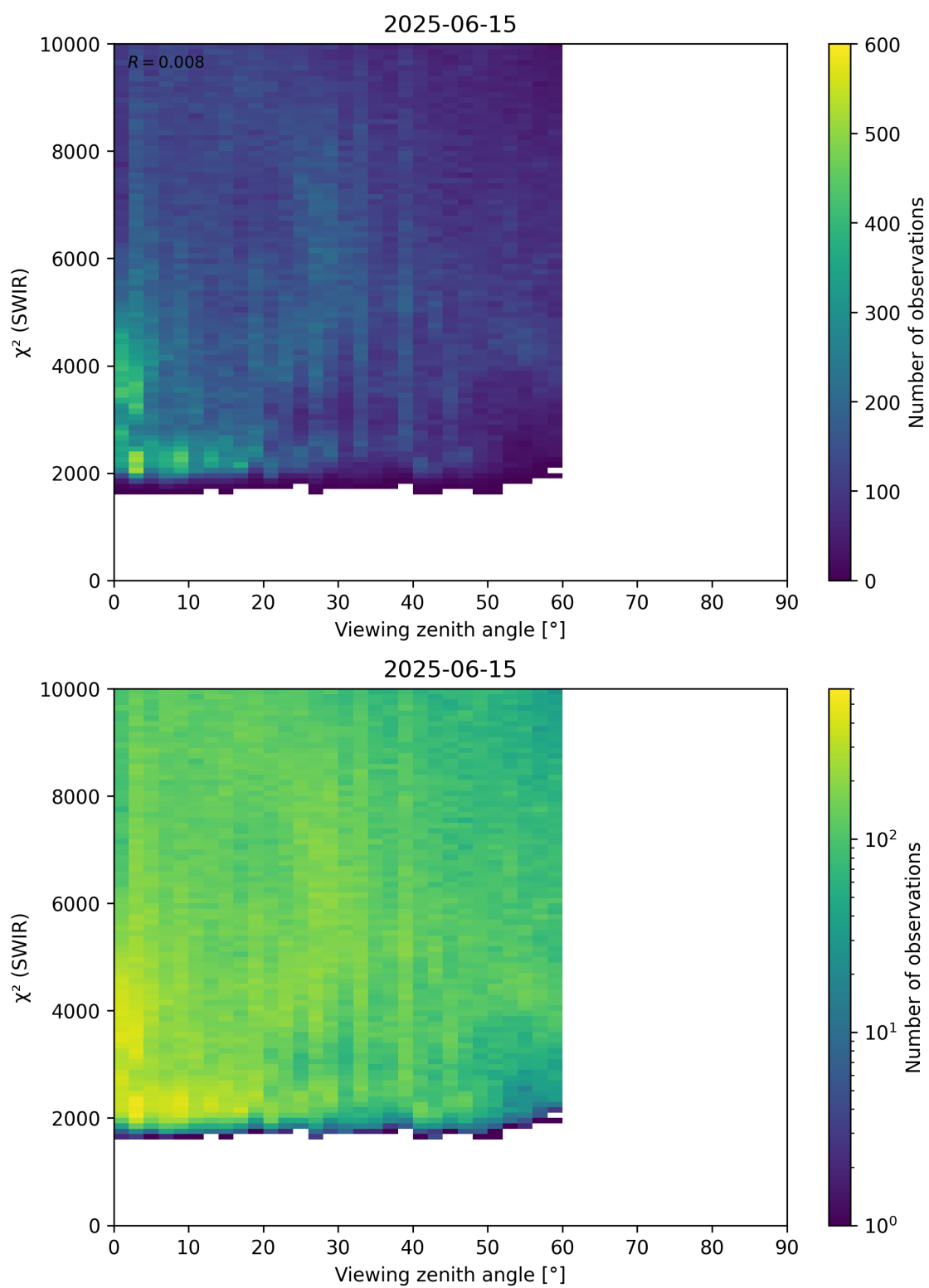
Figure 106: Scatter density plot of “Viewing zenith angle” against “ \chi^2 (SWIR)” for 2025-06-14 to 2025-06-16.
