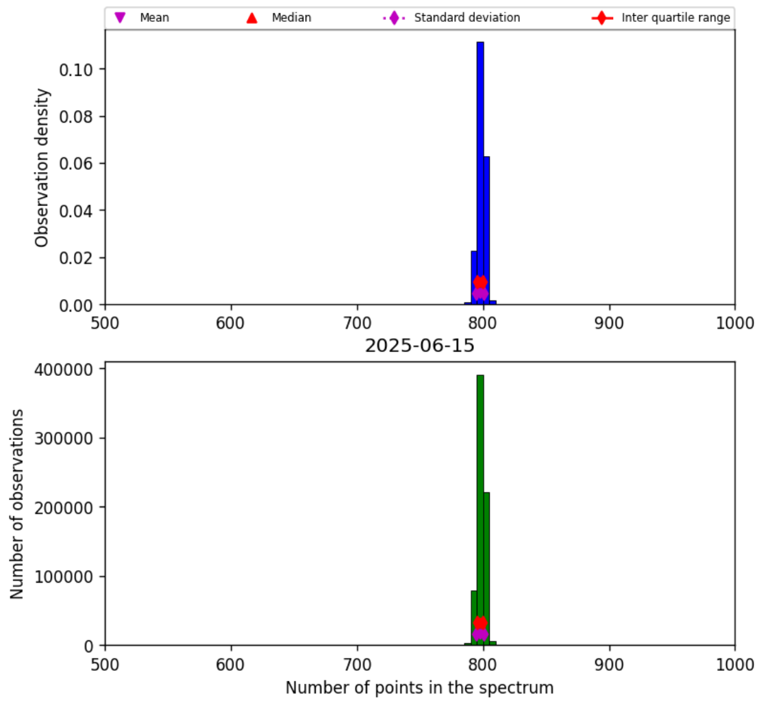
Figure 26: Histogram of “Number of points in the spectrum” for 2025-06-14 to 2025-06-16
