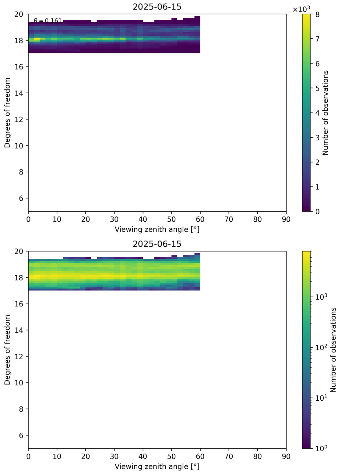
Figure 107: Scatter density plot of “Viewing zenith angle” against “Degrees of freedom” for 2025-06-14 to 2025-06-16.
