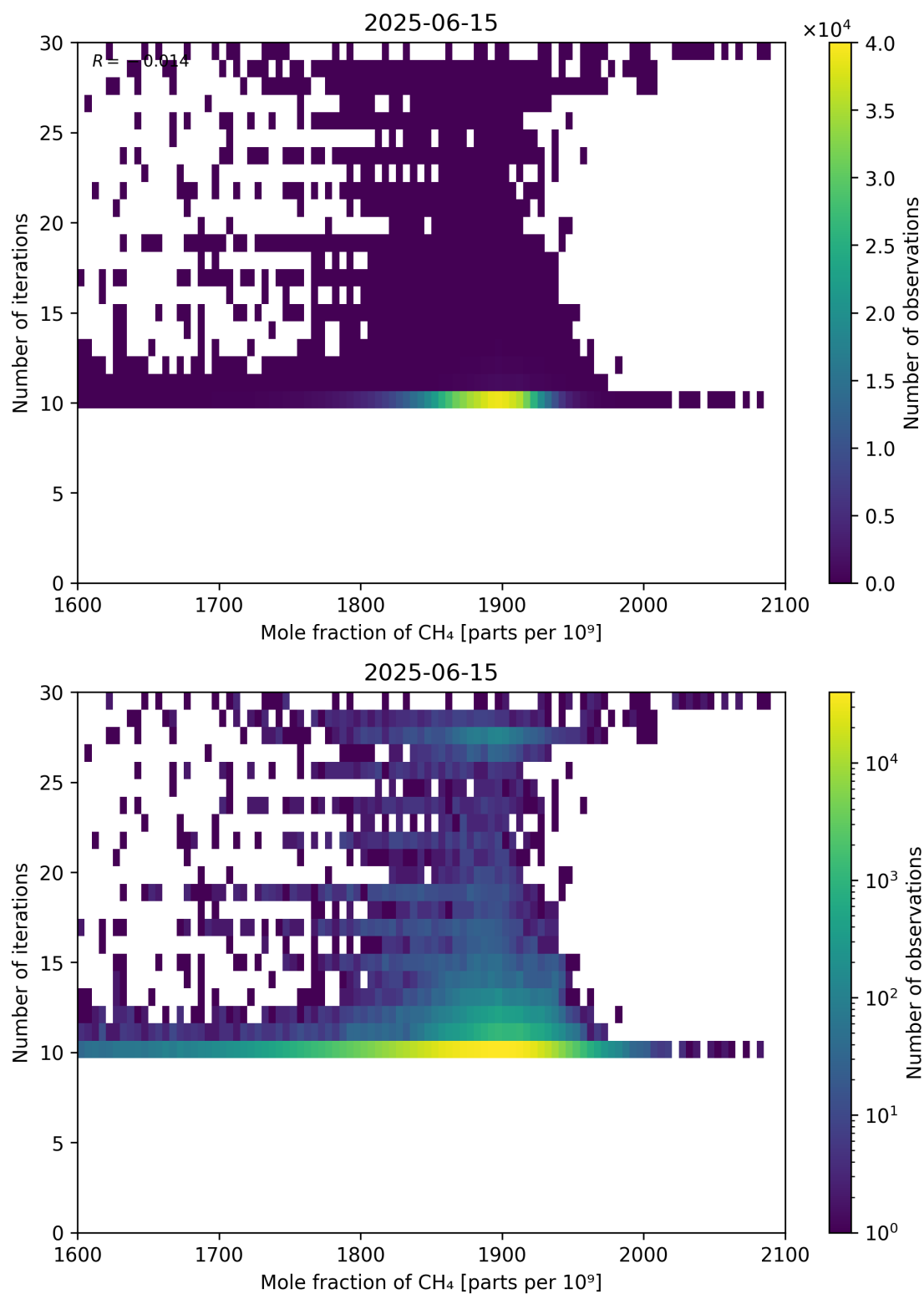
Figure 76: Scatter density plot of “Mole fraction of CH 4 ” against “Number of iterations” for 2025-06-14 to 2025-06-16.
