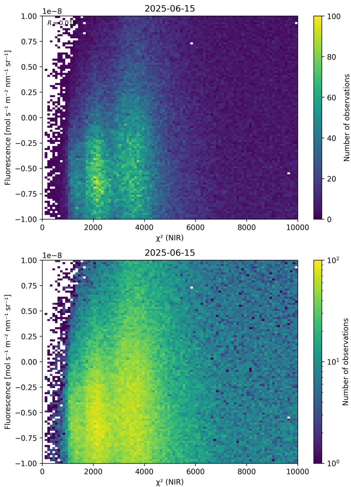
Figure 45: Scatter density plot of “ \chi^2 (NIR)” against “Fluorescence” for 2025-06-14 to 2025-06-16.
