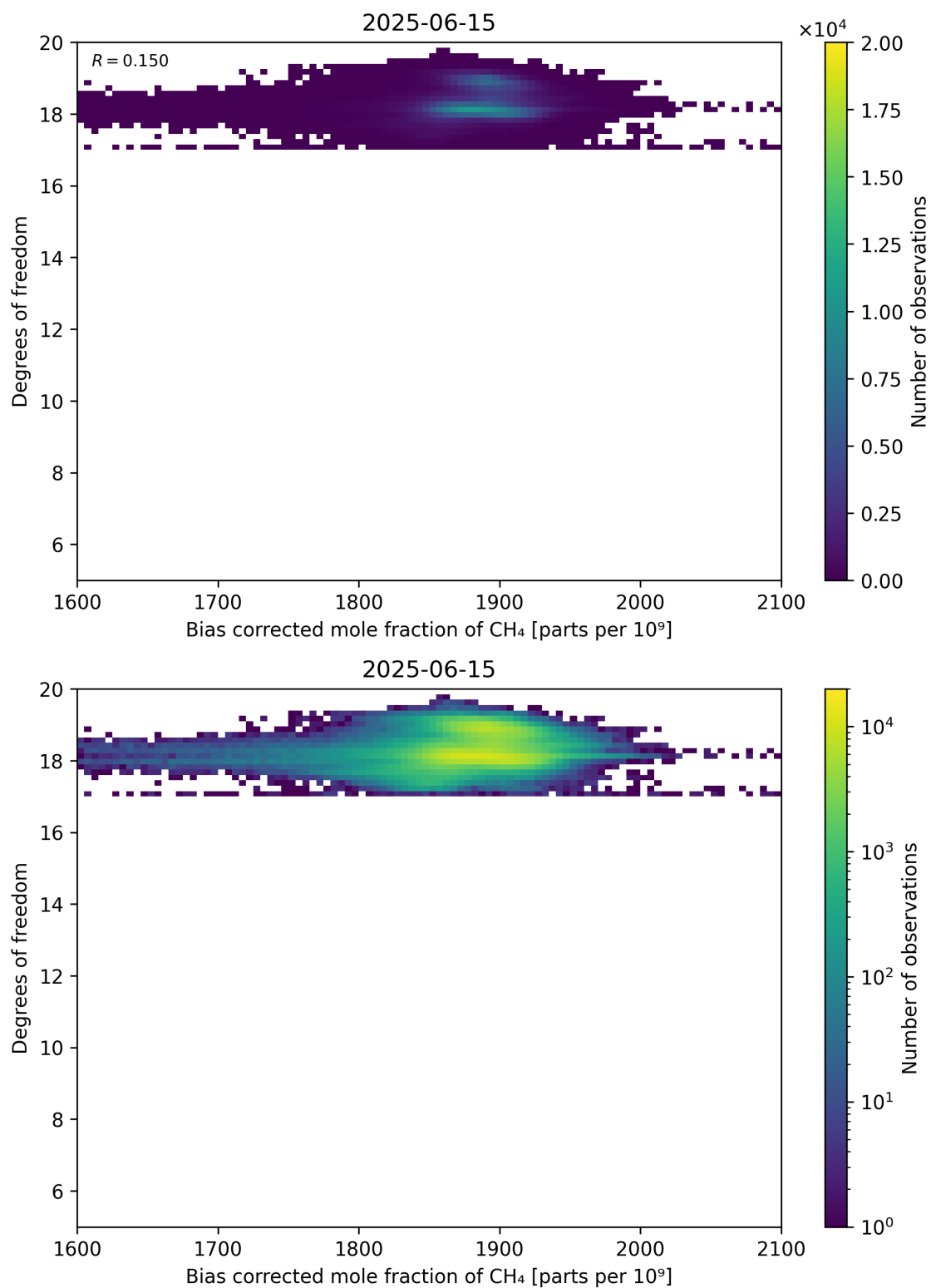
Figure 65: Scatter density plot of “Bias corrected mole fraction of \text{CH}_4 ” against “Degrees of freedom” for 2025-06-14 to 2025-06-16.
