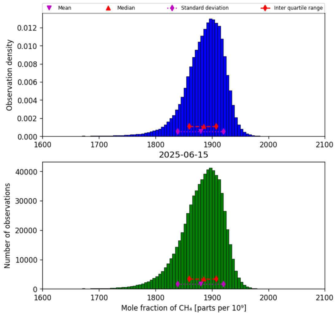
Figure 23: Histogram of “Mole fraction of CH 4 ” for 2025-06-14 to 2025-06-16
