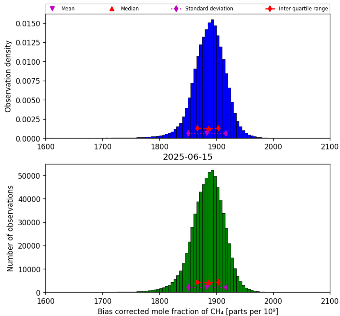
Figure 25: Histogram of “Bias corrected mole fraction of CH 4 ” for 2025-06-14 to 2025-06-16
