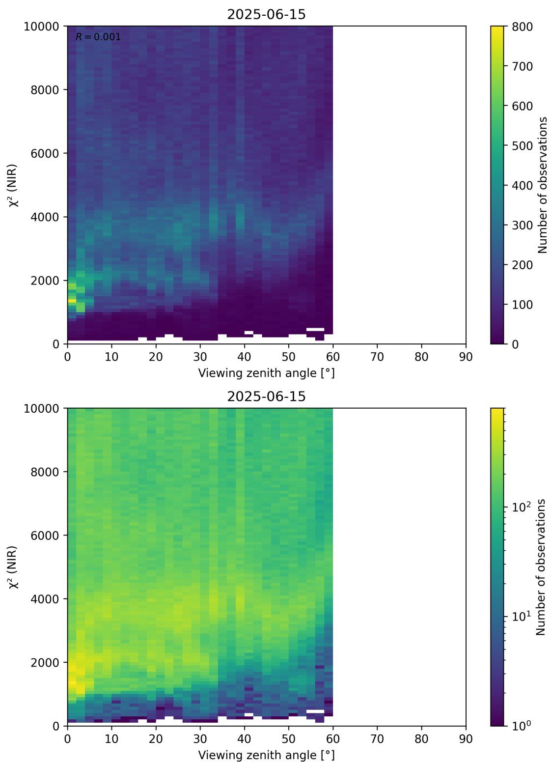
Figure 105: Scatter density plot of “Viewing zenith angle” against “ \chi^2 (NIR)” for 2025-06-14 to 2025-06-16.
