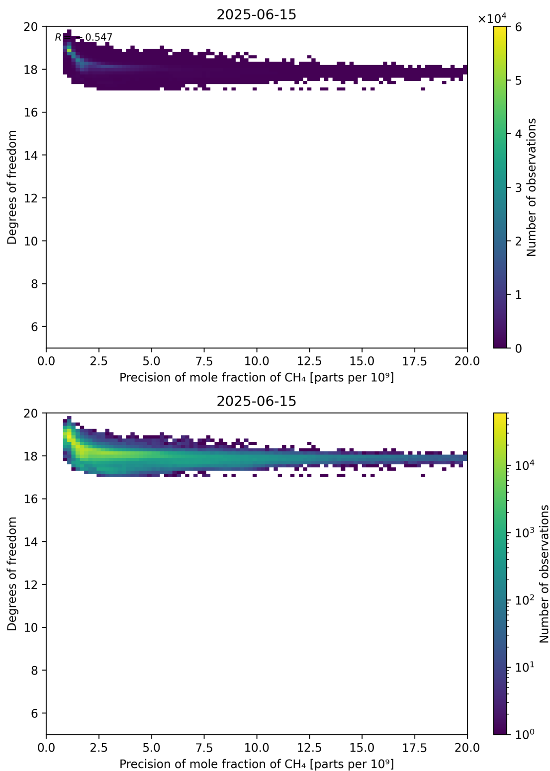
Figure 80: Scatter density plot of “Precision of mole fraction of CH 4 ” against “Degrees of freedom” for 2025-06-14 to 2025-06-16.
