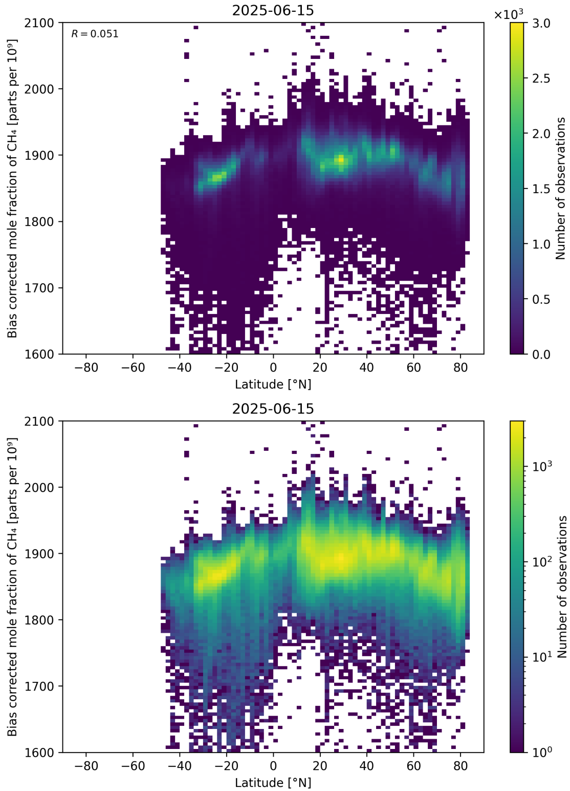
Figure 58: Scatter density plot of “Latitude” against “Bias corrected mole fraction of CH 4 ” for 2025-06-14 to 2025-06-16.
