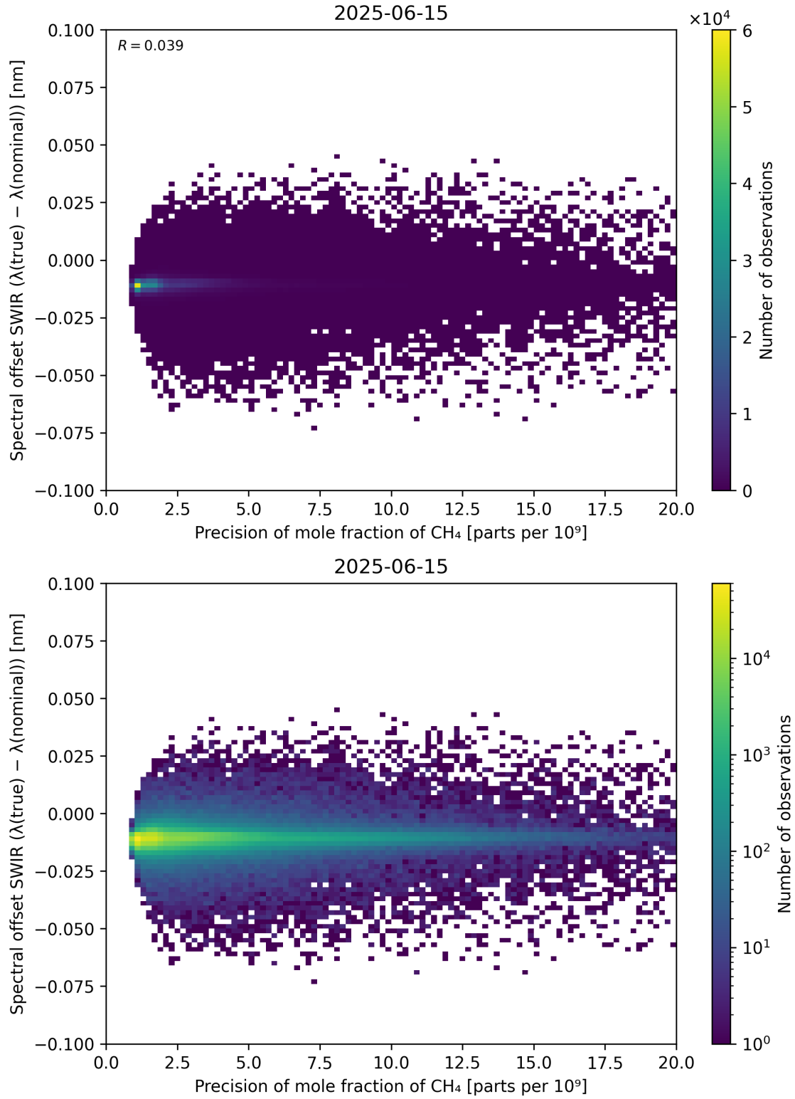
Figure 85: Scatter density plot of “Precision of mole fraction of \text{CH}_4 ” against “Spectral offset SWIR ( \lambda_{\text{true}} - \lambda_{\text{nominal}} )” for 2025-06-14 to 2025-06-16.
