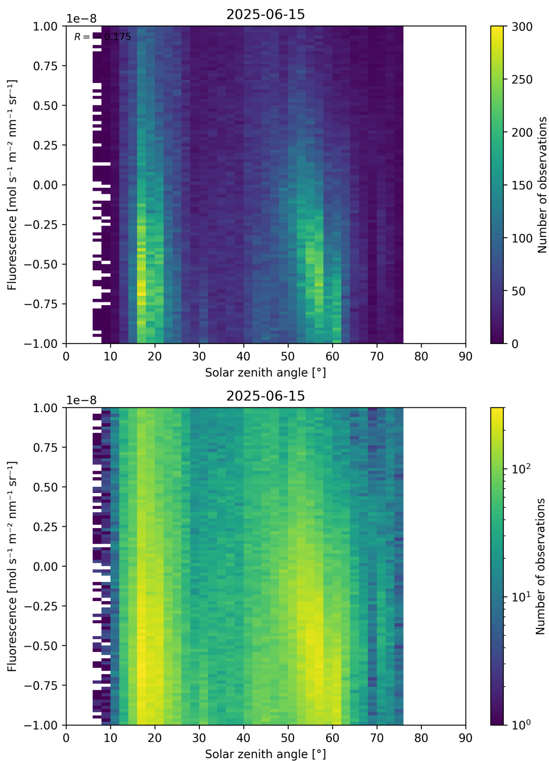
Figure 97: Scatter density plot of “Solar zenith angle” against “Fluorescence” for 2025-06-14 to 2025-06-16.
