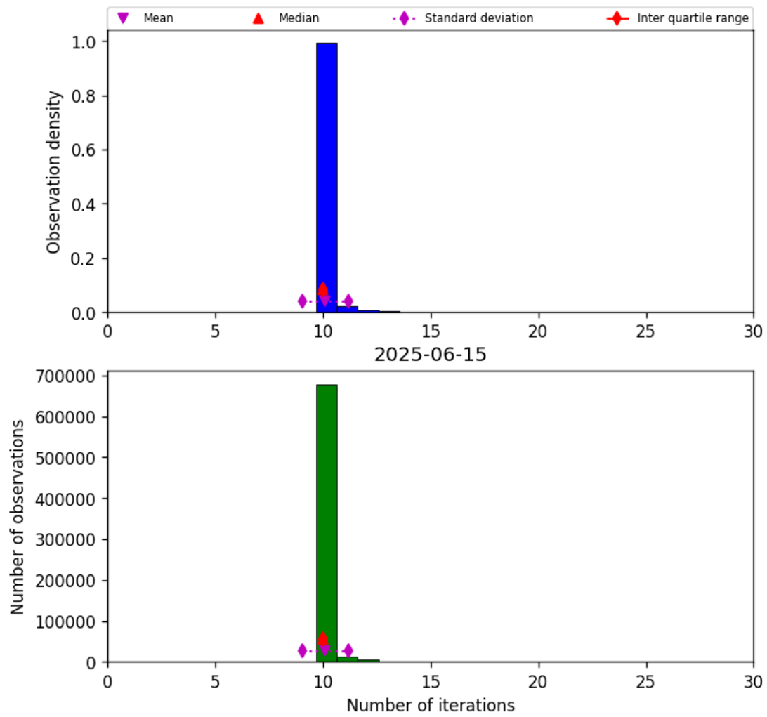
Figure 31: Histogram of “Number of iterations” for 2025-06-14 to 2025-06-16
