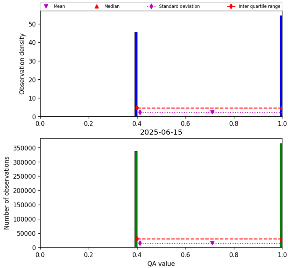
Figure 22: Histogram of “QA value” for 2025-06-14 to 2025-06-16
