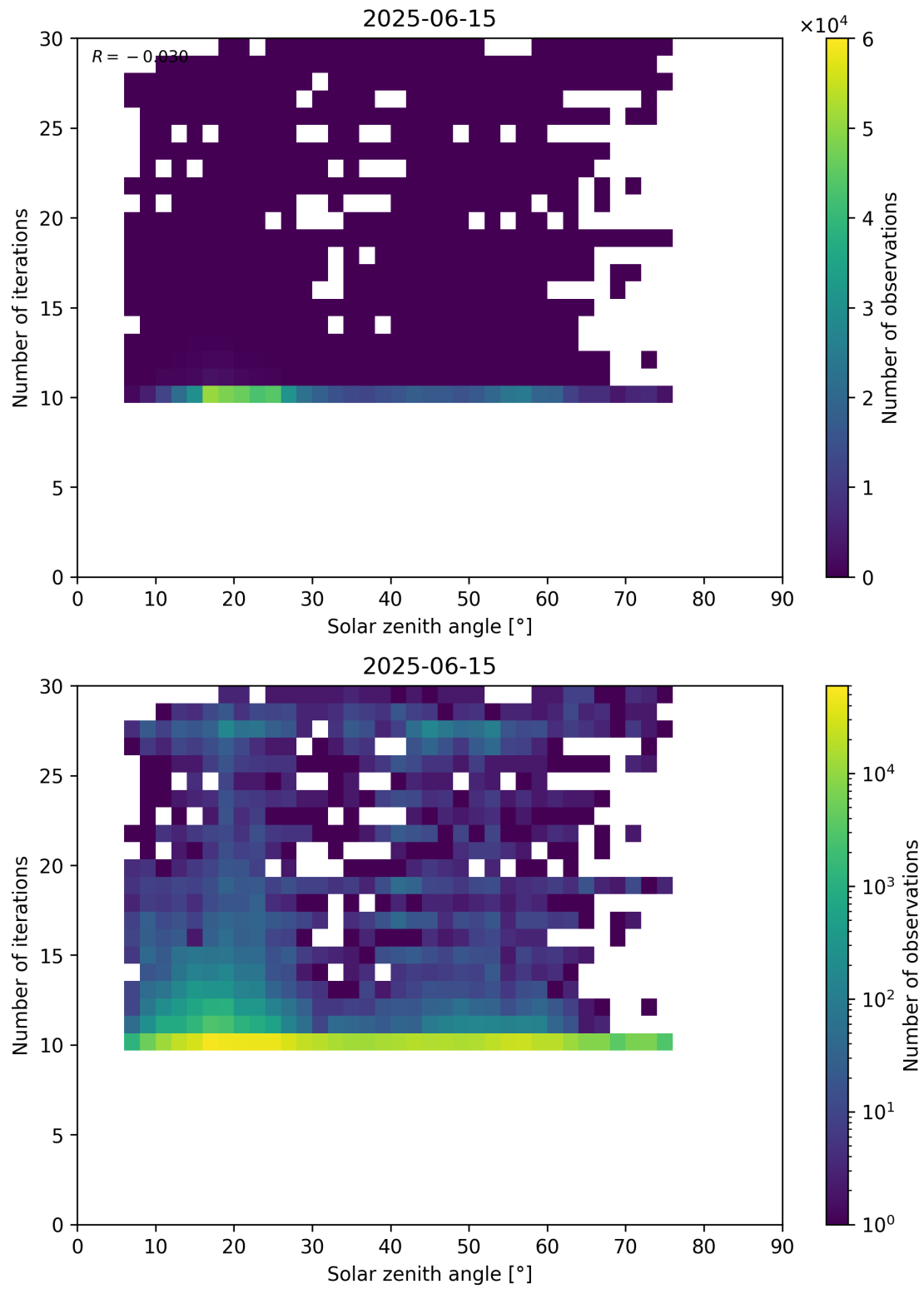
Figure 102: Scatter density plot of “Solar zenith angle” against “Number of iterations” for 2025-06-14 to 2025-06-16.
