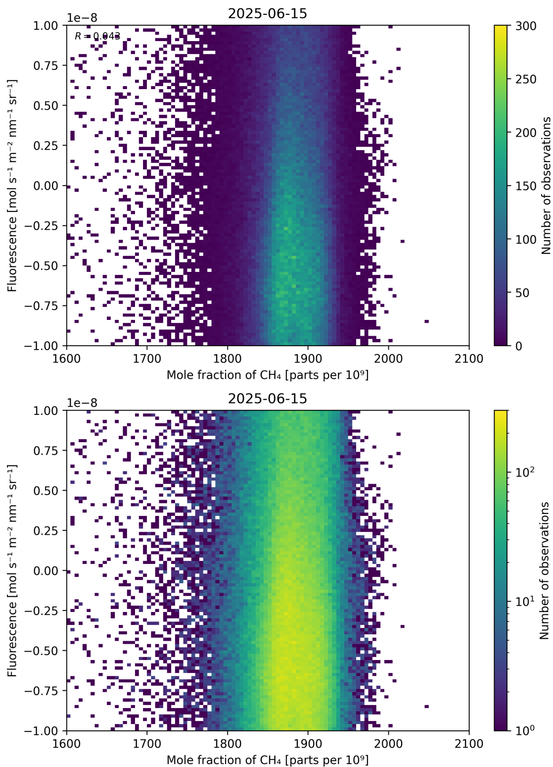
Figure 73: Scatter density plot of “Mole fraction of \text{CH}_4 ” against “Fluorescence” for 2025-06-14 to 2025-06-16.
