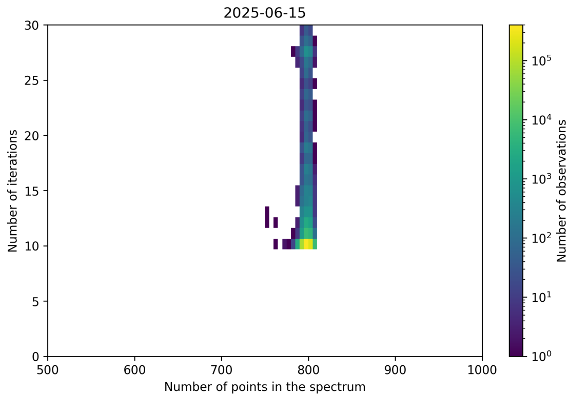
Figure 92: Scatter density plot of “Number of points in the spectrum” against “Number of iterations” for 2025-06-14 to 2025-06-16.
