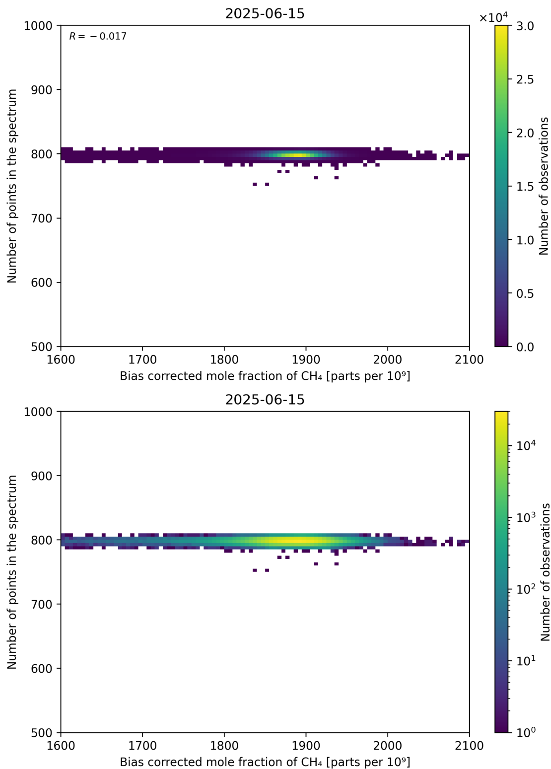
Figure 68: Scatter density plot of “Bias corrected mole fraction of CH 4 ” against “Number of points in the spectrum” for 2025-06-14 to 2025-06-16.
