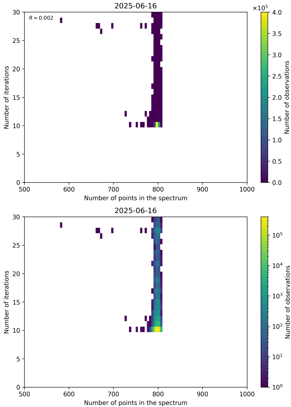
Figure 92: Scatter density plot of “Number of points in the spectrum” against “Number of iterations” for 2025-06-16 to 2025-06-17.
