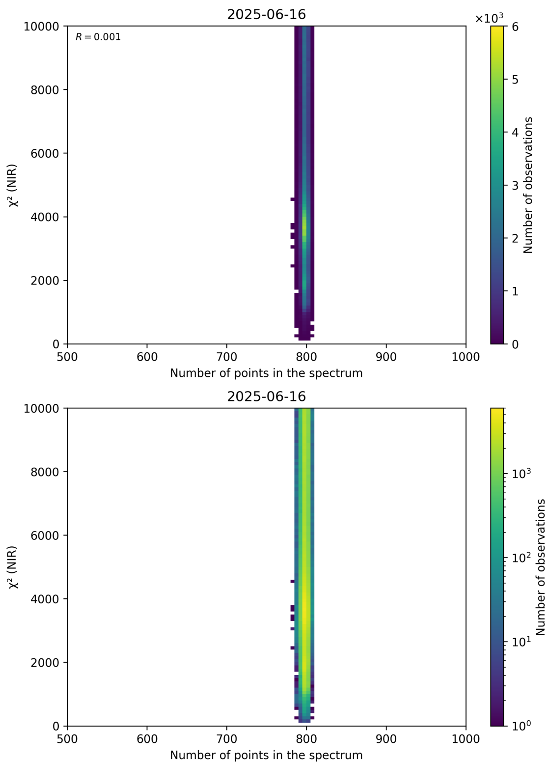
Figure 88: Scatter density plot of “Number of points in the spectrum” against “ \chi^2 (NIR)” for 2025-06-16 to 2025-06-17.
