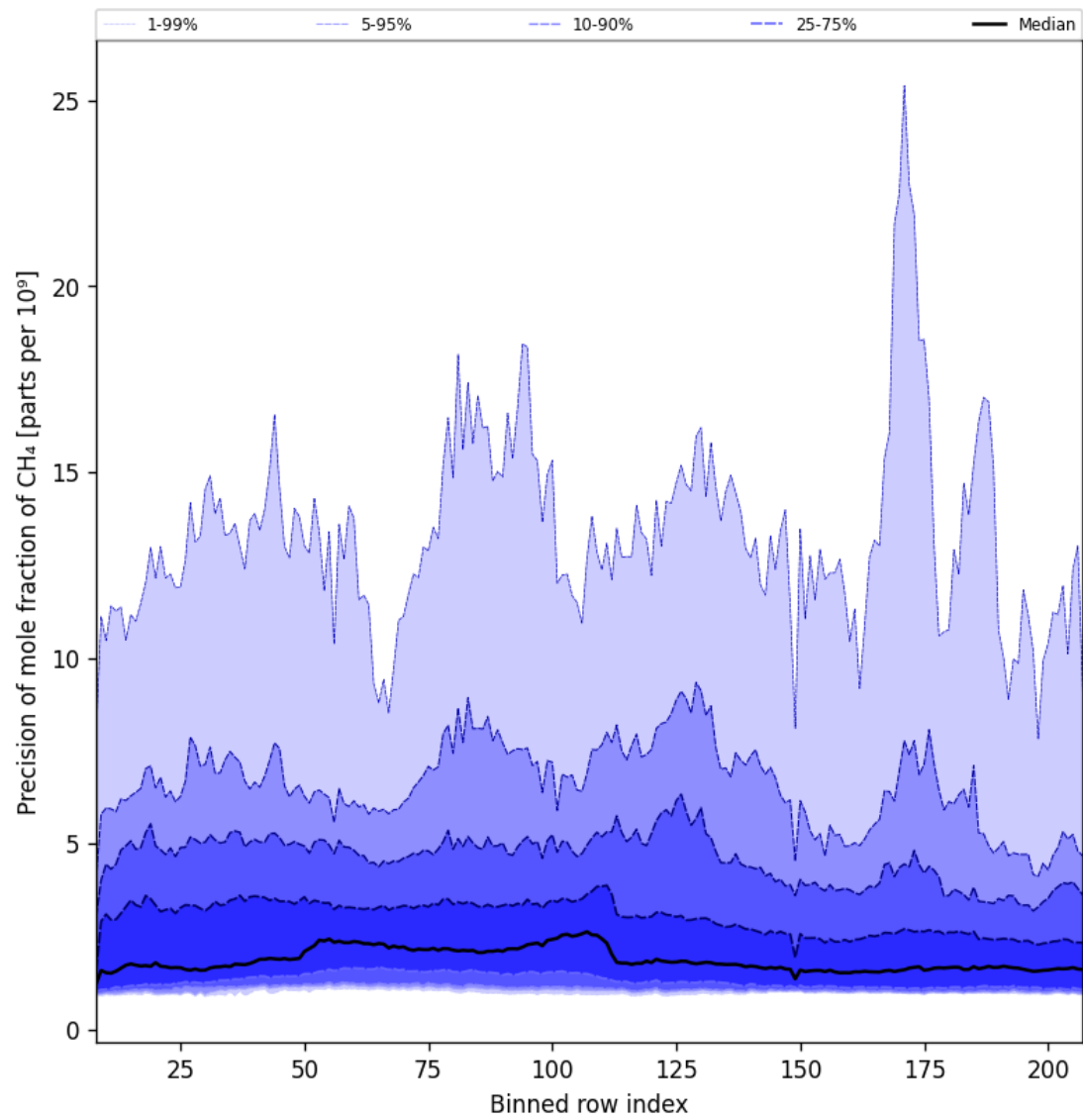
Figure 35: Along track statistics of “Precision of mole fraction of CH 4 ” for 2025-06-16 to 2025-06-17
