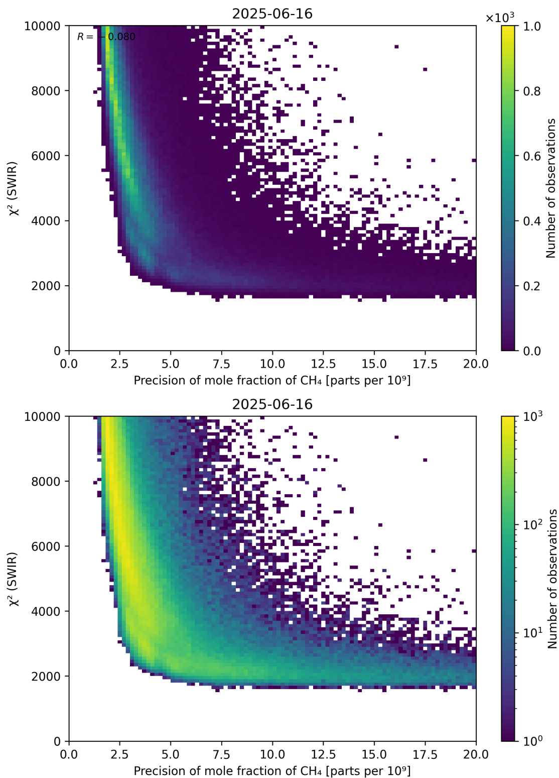
Figure 79: Scatter density plot of “Precision of mole fraction of \text{CH}_4 ” against “ \chi^2 (SWIR)” for 2025-06-16 to 2025-06-17.
