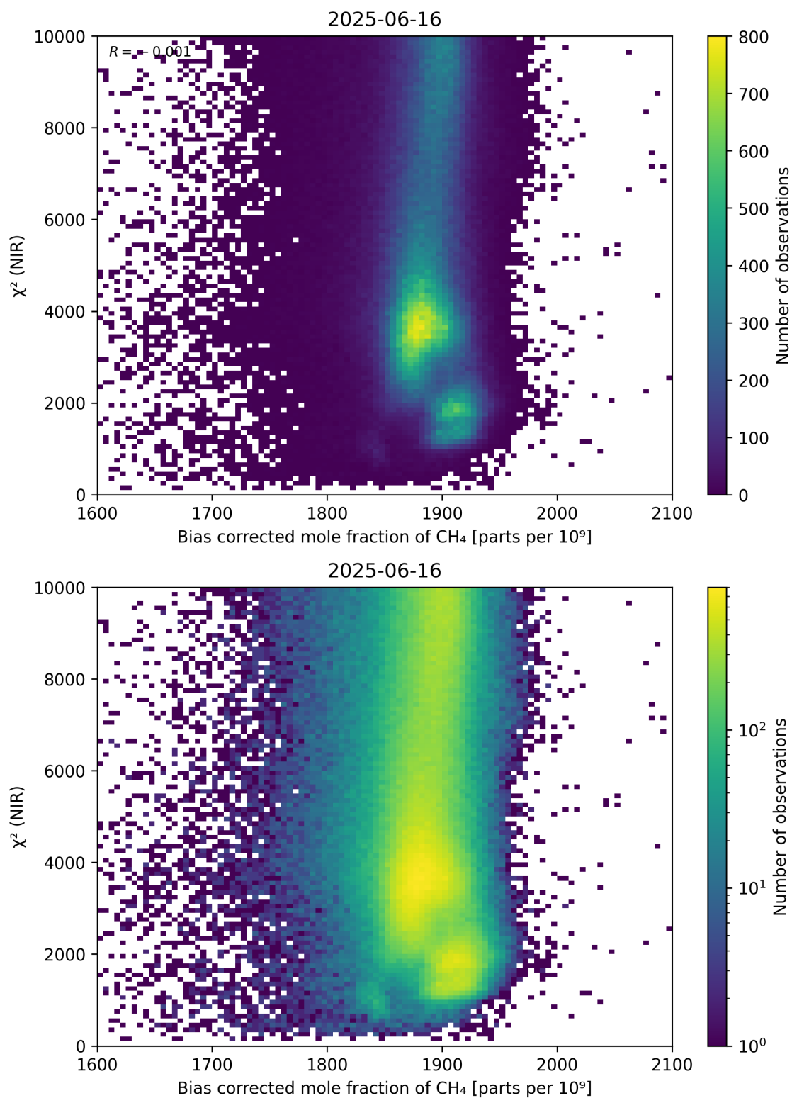
Figure 63: Scatter density plot of “Bias corrected mole fraction of \text{CH}_4 ” against “ \chi^2 (NIR)” for 2025-06-16 to 2025-06-17.
