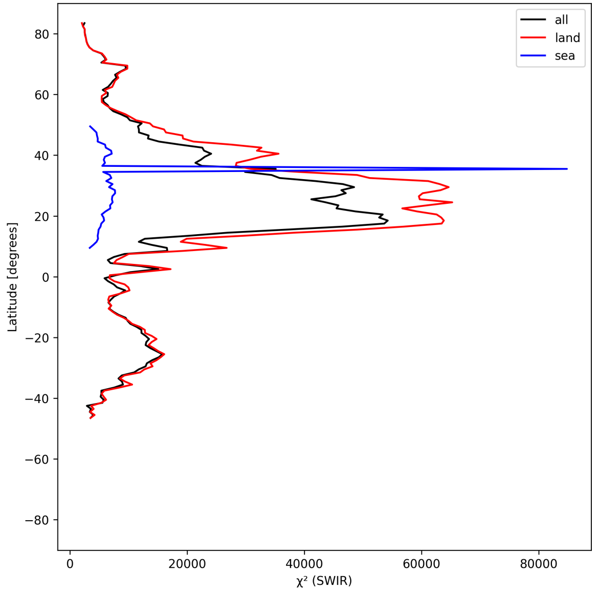
Figure 17: Zonal average of “ \chi^2 (SWIR)” for 2025-06-16 to 2025-06-17.
