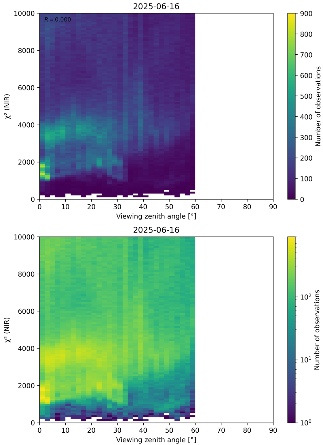
Figure 105: Scatter density plot of “Viewing zenith angle” against “ \chi^2 (NIR)” for 2025-06-16 to 2025-06-17.
