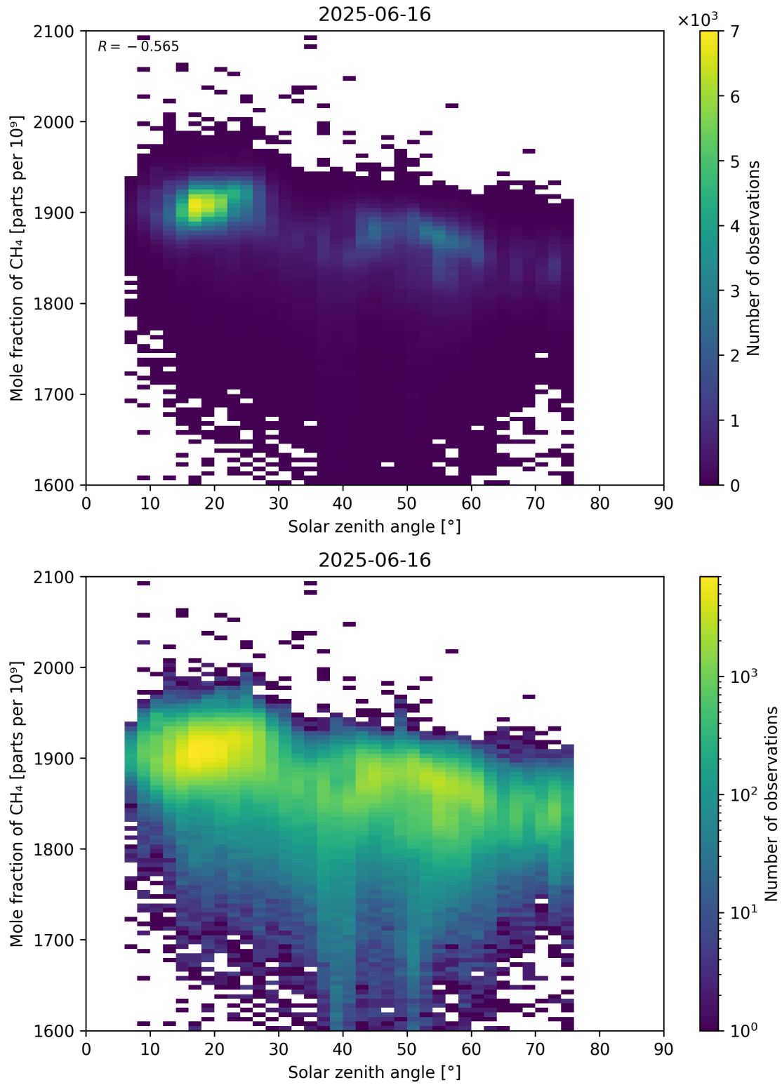
Figure 99: Scatter density plot of “Solar zenith angle” against “Mole fraction of \text{CH}_4 ” for 2025-06-16 to 2025-06-17.
