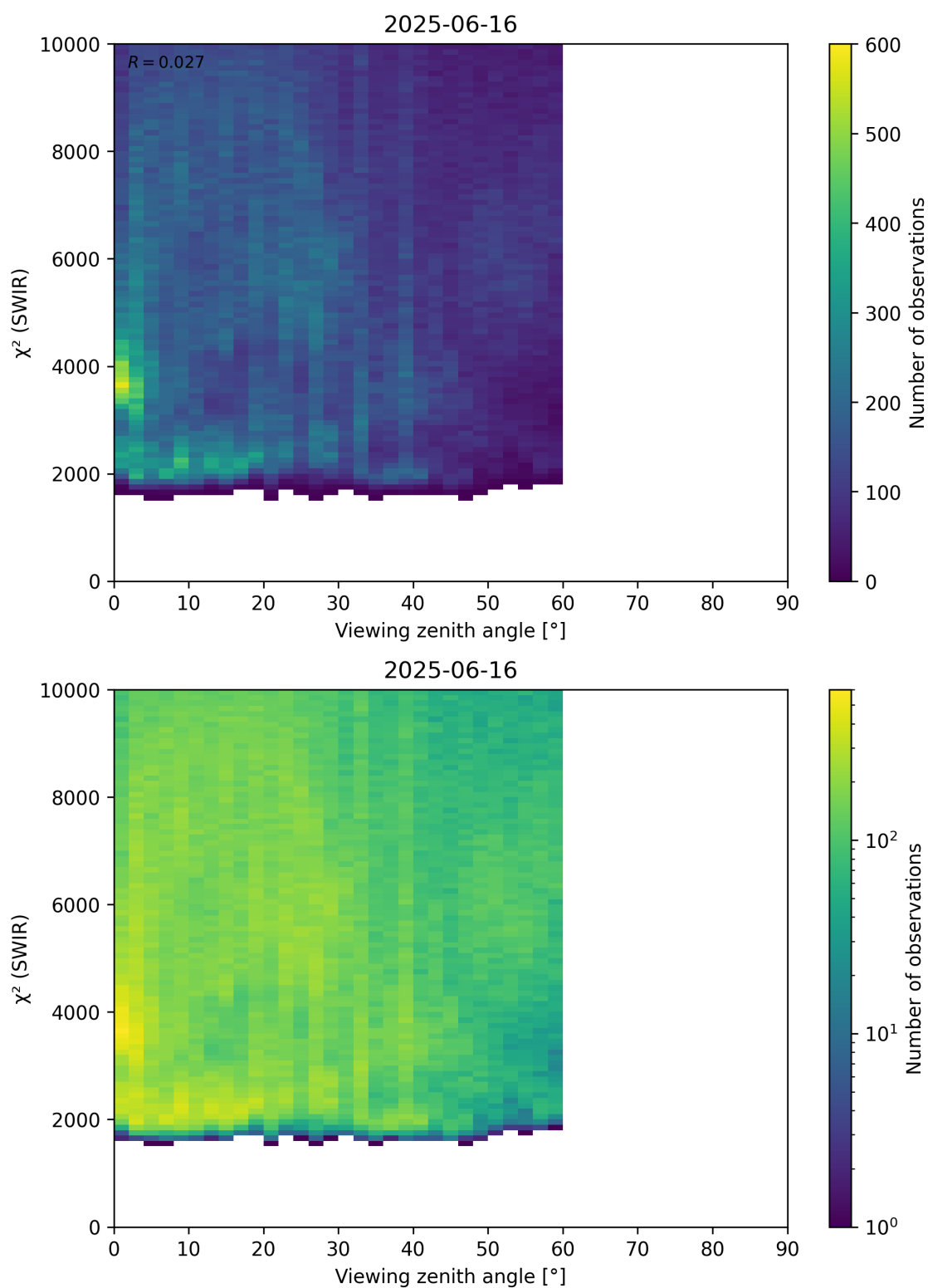
Figure 106: Scatter density plot of “Viewing zenith angle” against “ \chi^2 (SWIR)” for 2025-06-16 to 2025-06-17.
