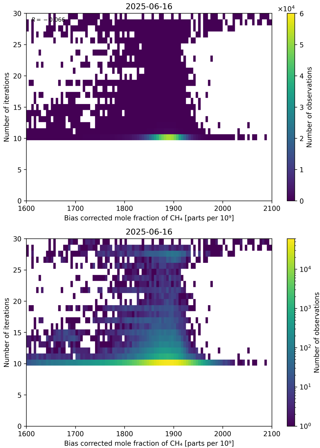
Figure 67: Scatter density plot of “Bias corrected mole fraction of \text{CH}_4 ” against “Number of iterations” for 2025-06-16 to 2025-06-17.
