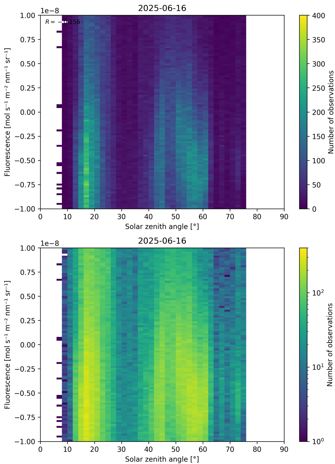
Figure 97: Scatter density plot of “Solar zenith angle” against “Fluorescence” for 2025-06-16 to 2025-06-17.
