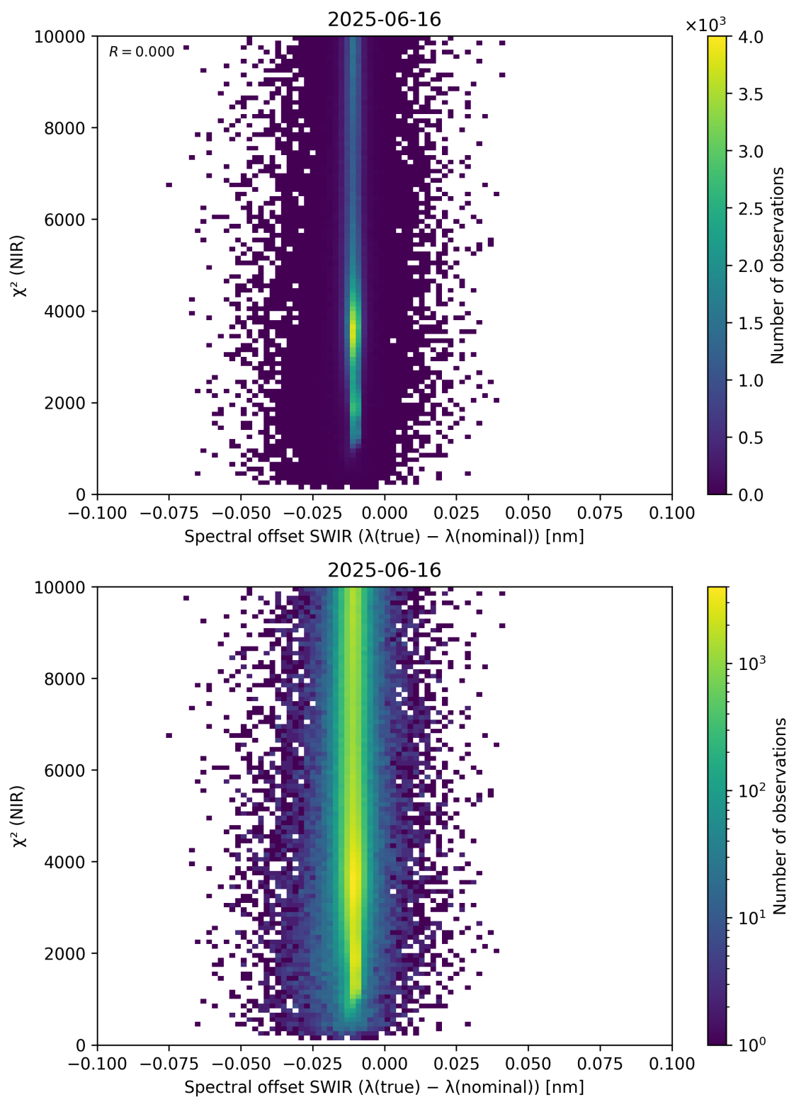
Figure 117: Scatter density plot of “Spectral offset SWIR ( \lambda_{\text{true}} - \lambda_{\text{nominal}} )” against “ \chi^2 (NIR)” for 2025-06-16 to 2025-06-17.
