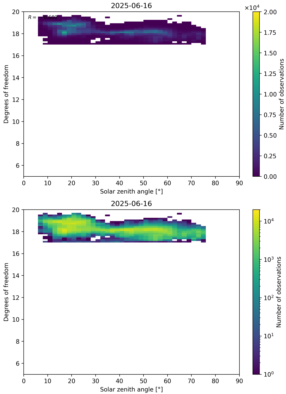
Figure 96: Scatter density plot of “Solar zenith angle” against “Degrees of freedom” for 2025-06-16 to 2025-06-17.
