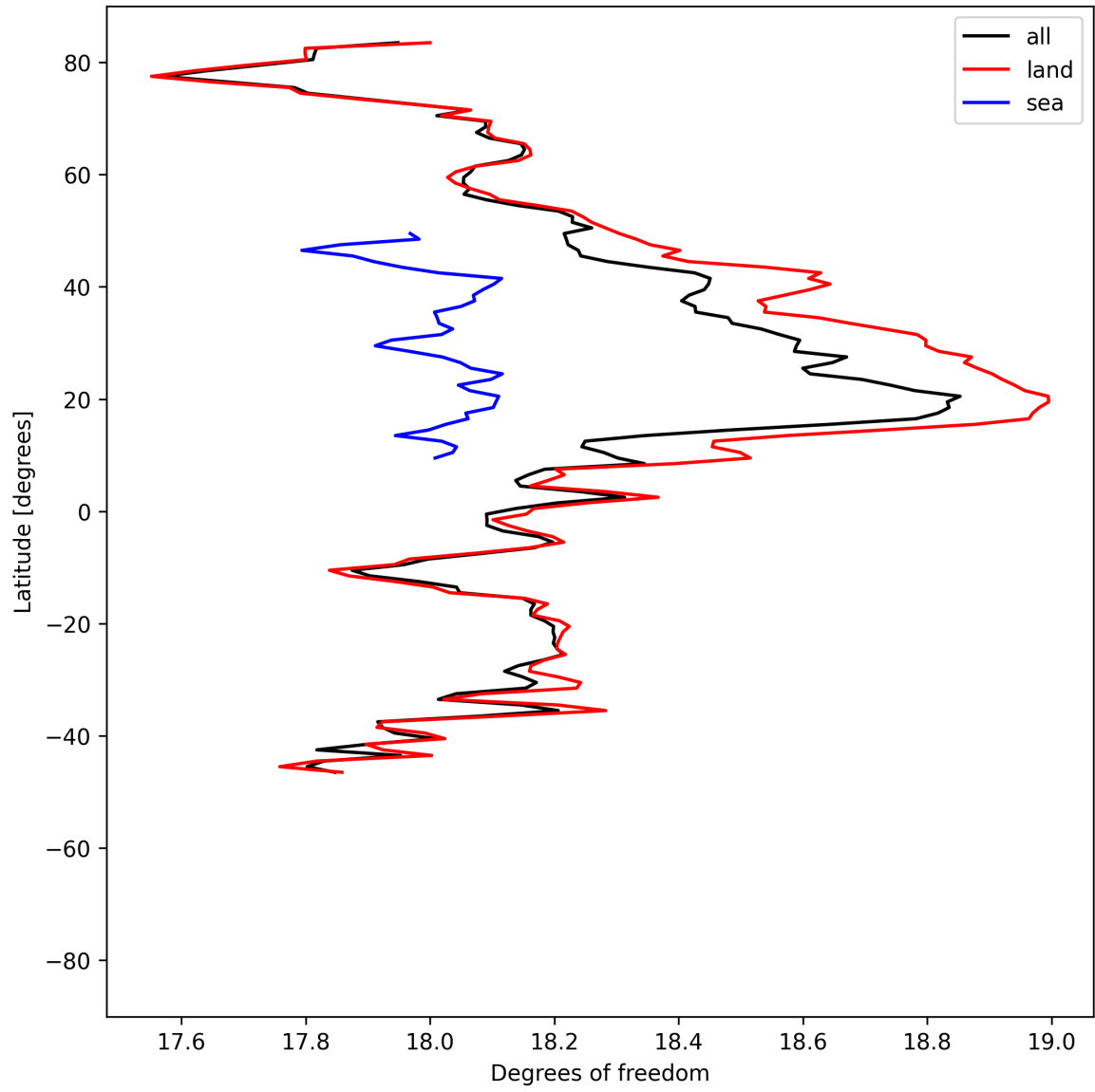
Figure 19: Zonal average of “Degrees of freedom” for 2025-06-16 to 2025-06-17.
