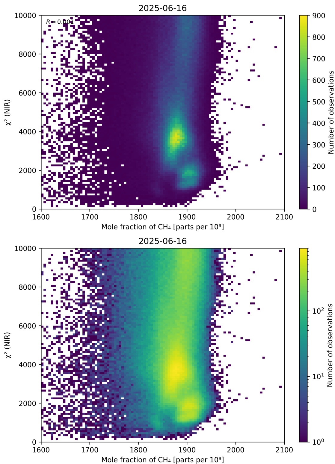
Figure 70: Scatter density plot of “Mole fraction of \text{CH}_4 ” against “ \chi^2 (NIR)” for 2025-06-16 to 2025-06-17.
