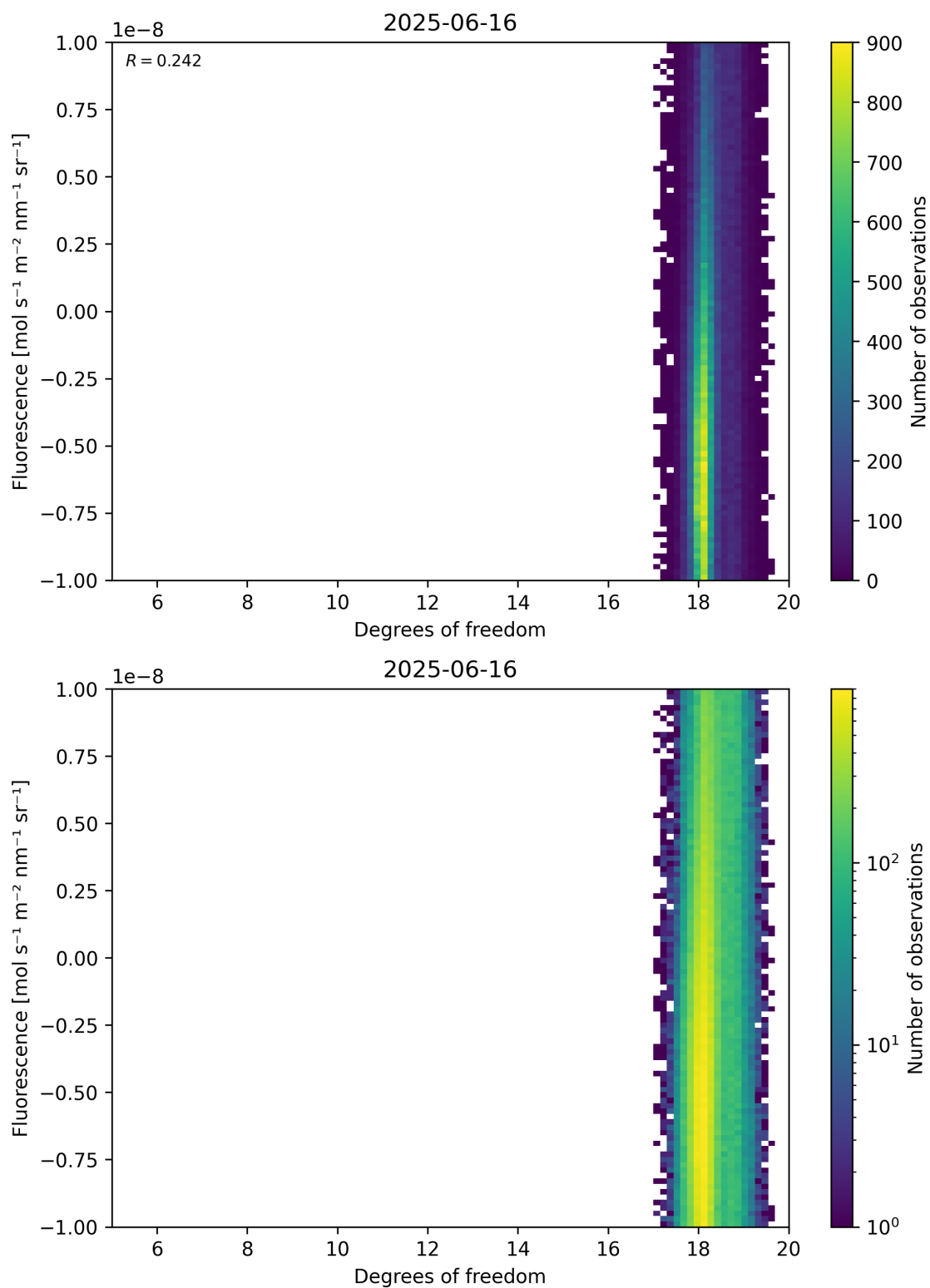
Figure 51: Scatter density plot of “Degrees of freedom” against “Fluorescence” for 2025-06-16 to 2025-06-17.
