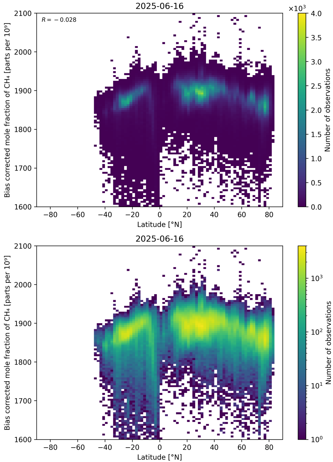
Figure 58: Scatter density plot of “Latitude” against “Bias corrected mole fraction of \text{CH}_4 ” for 2025-06-16 to 2025-06-17.
