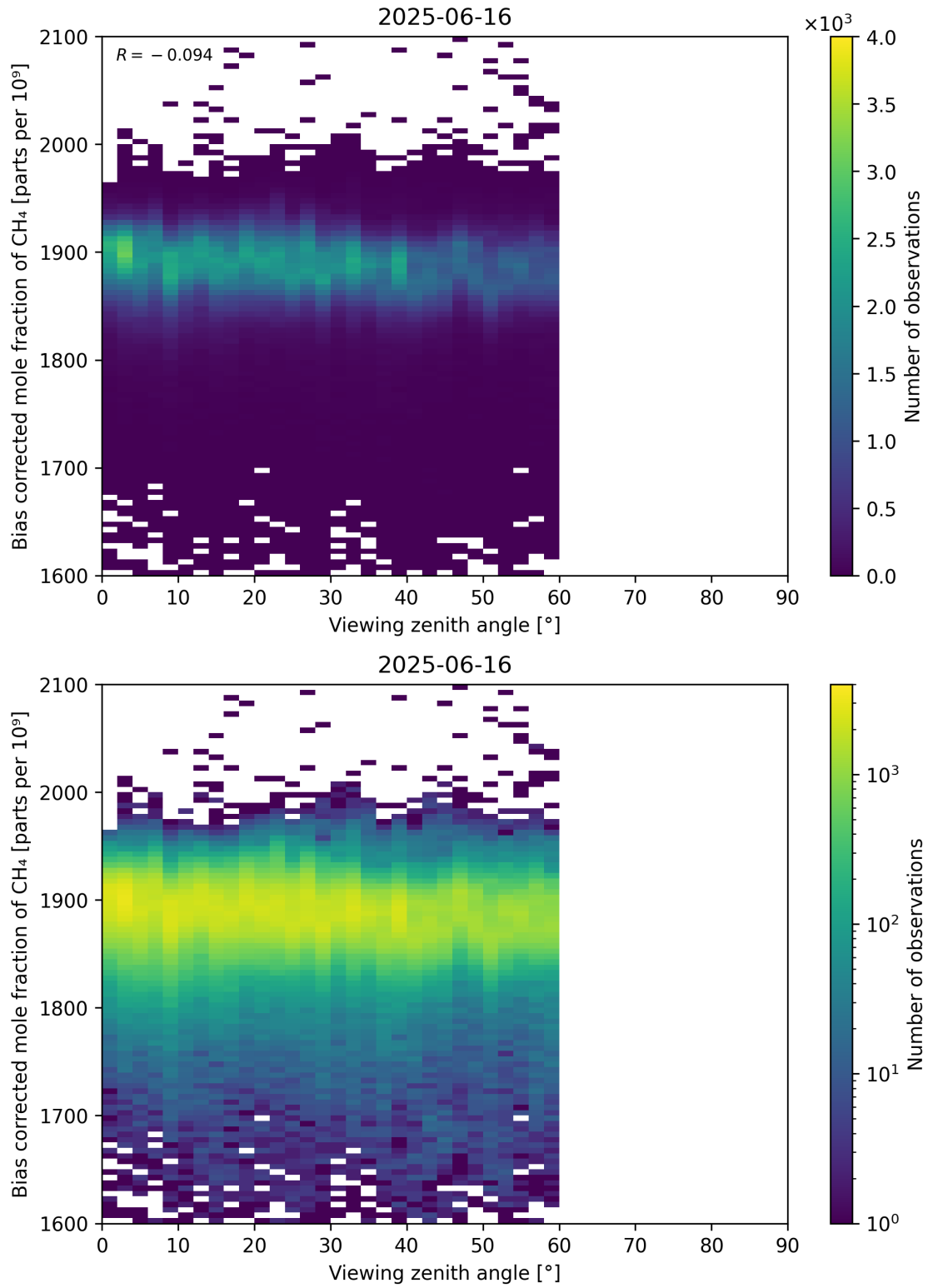
Figure 111: Scatter density plot of “Viewing zenith angle” against “Bias corrected mole fraction of CH 4 ” for 2025-06-16 to 2025-06-17.
