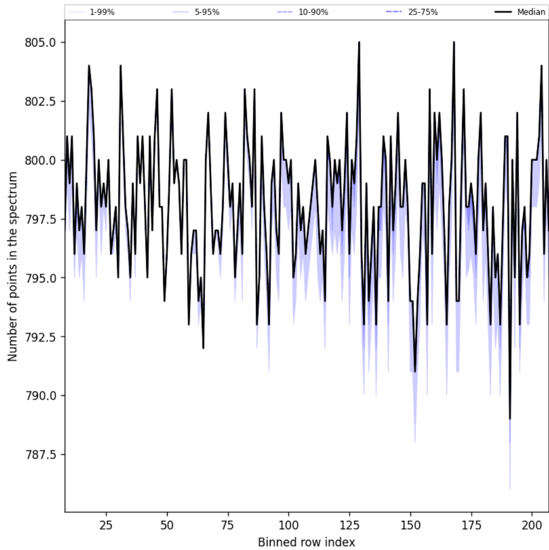
Figure 37: Along track statistics of “Number of points in the spectrum” for 2025-06-16 to 2025-06-17
