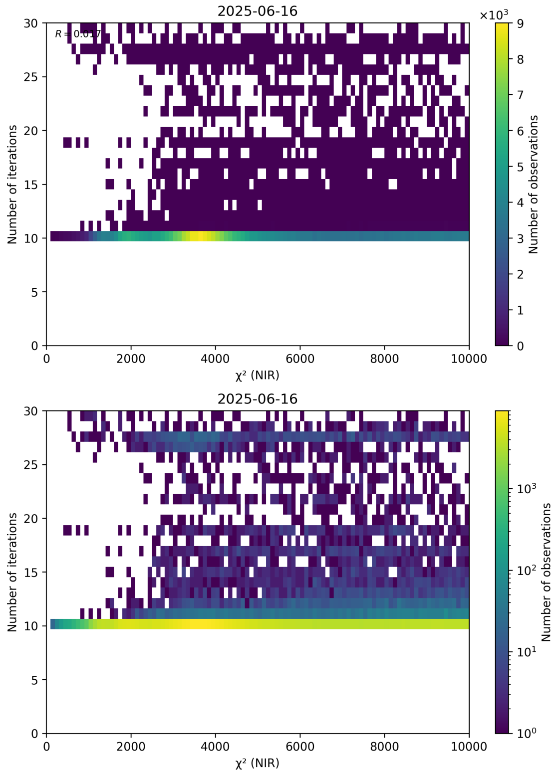
Figure 46: Scatter density plot of “ \chi^2 (NIR)” against “Number of iterations” for 2025-06-16 to 2025-06-17.
