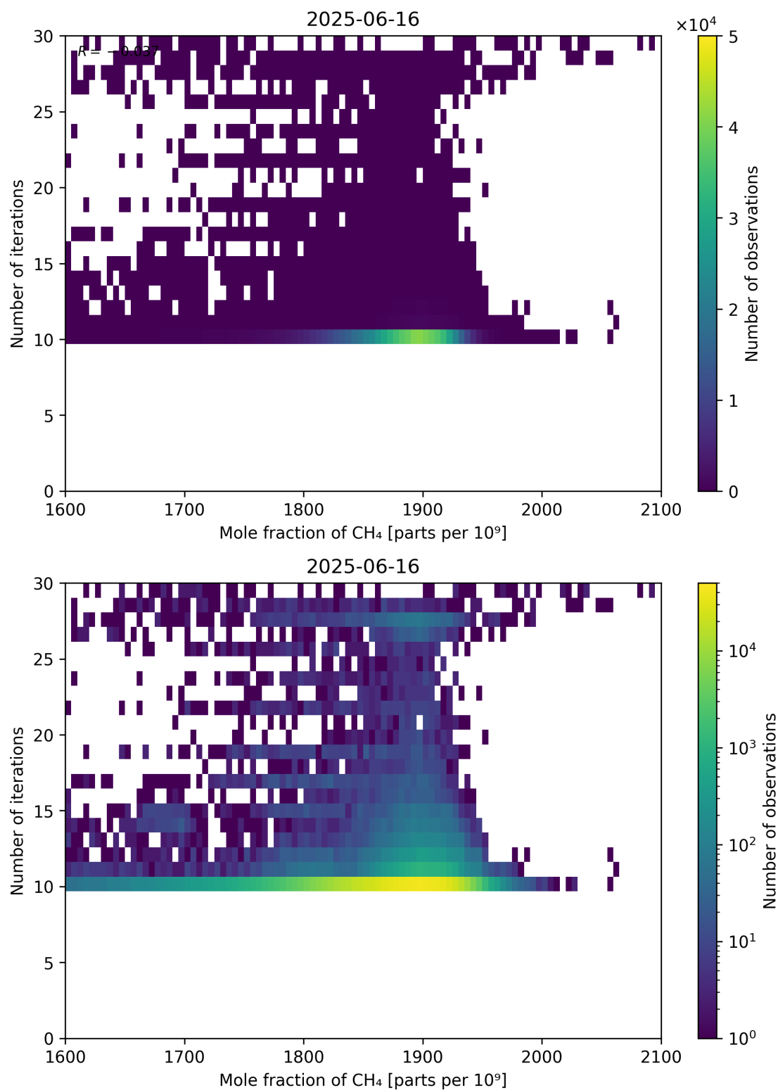
Figure 76: Scatter density plot of “Mole fraction of CH 4 ” against “Number of iterations” for 2025-06-16 to 2025-06-17.
