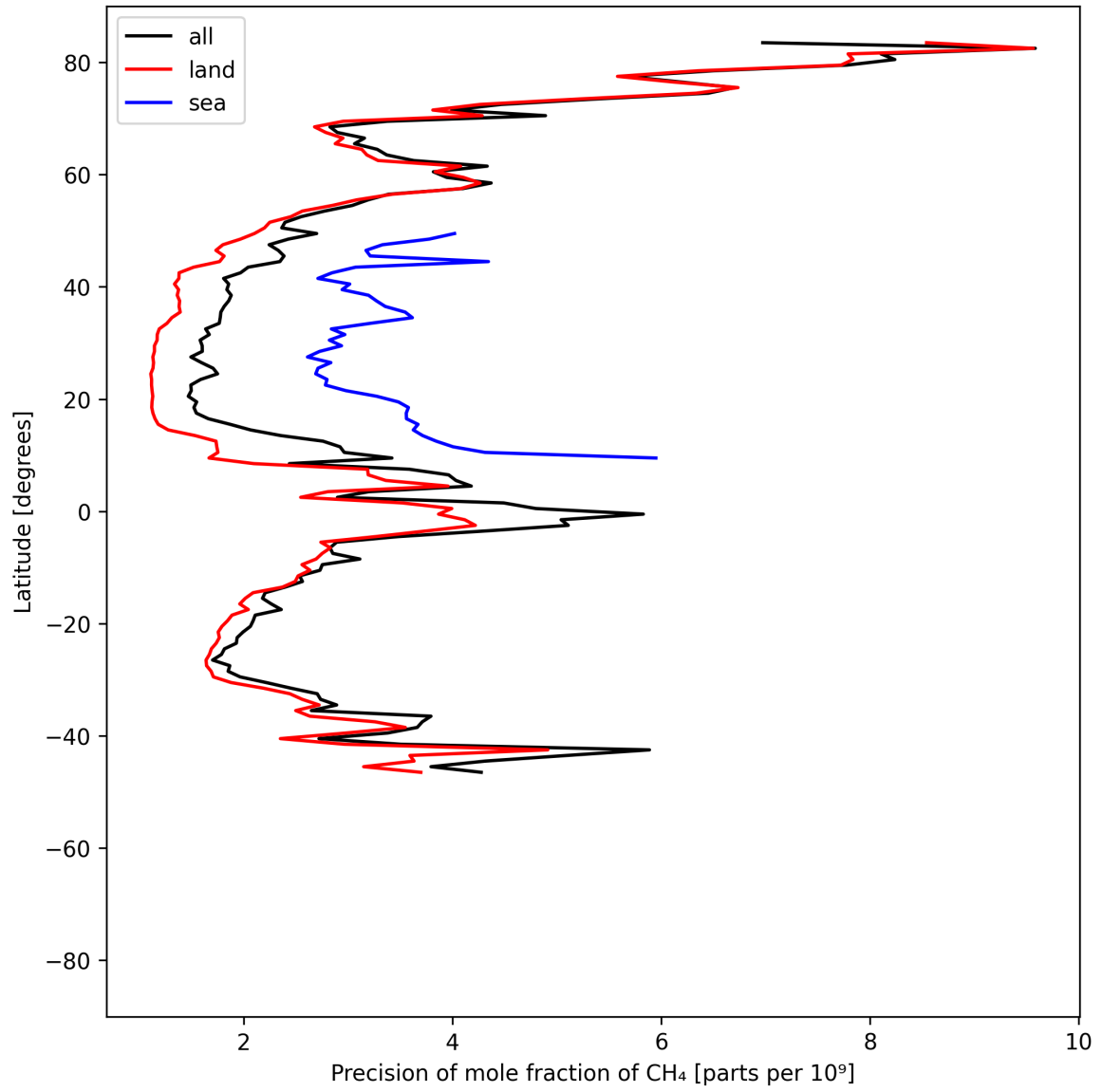
Figure 13: Zonal average of “Precision of mole fraction of \text{CH}_4 ” for 2025-06-16 to 2025-06-17.
