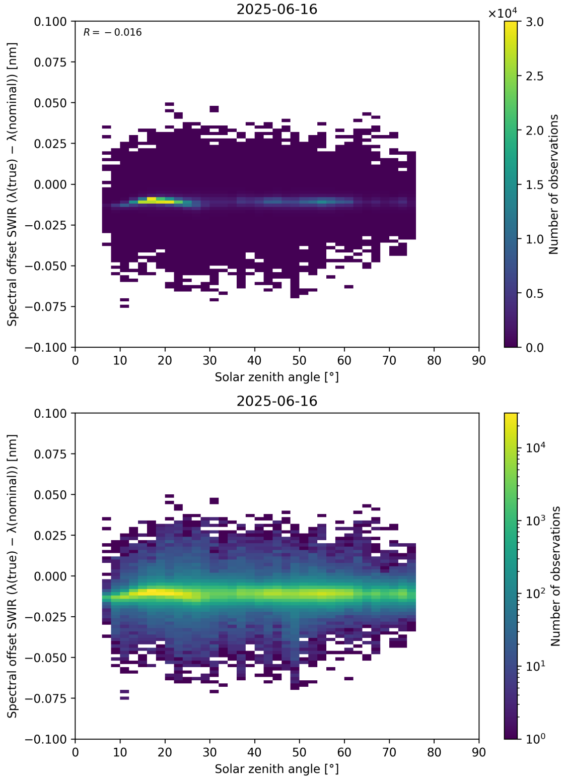
Figure 104: Scatter density plot of “Solar zenith angle” against “Spectral offset SWIR ( \lambda_{\text{true}} - \lambda_{\text{nominal}} )” for 2025-06-16 to 2025-06-17.
