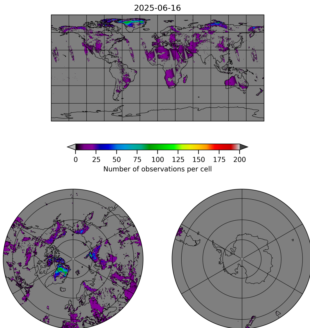
Figure 10: Map of the number of observations for 2025-06-16 to 2025-06-17
