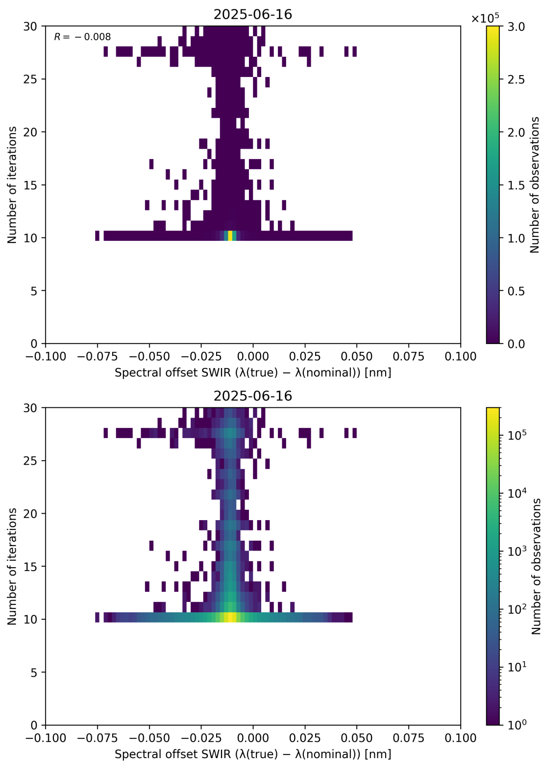
Figure 121: Scatter density plot of “Spectral offset SWIR ( \lambda_{\text{true}} - \lambda_{\text{nominal}} )” against “Number of iterations” for 2025-06-16 to 2025-06-17.
