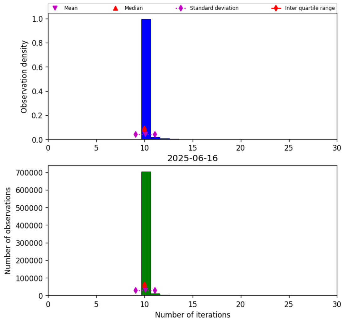
Figure 31: Histogram of “Number of iterations” for 2025-06-16 to 2025-06-17
