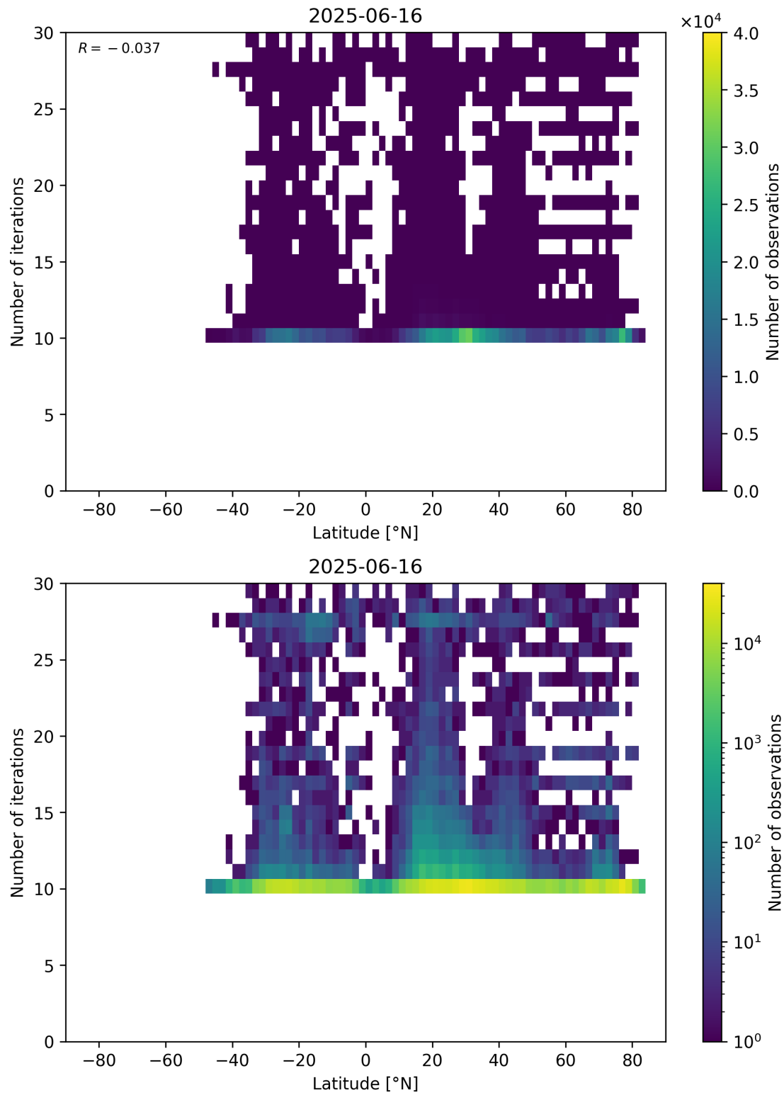
Figure 60: Scatter density plot of “Latitude” against “Number of iterations” for 2025-06-16 to 2025-06-17.
