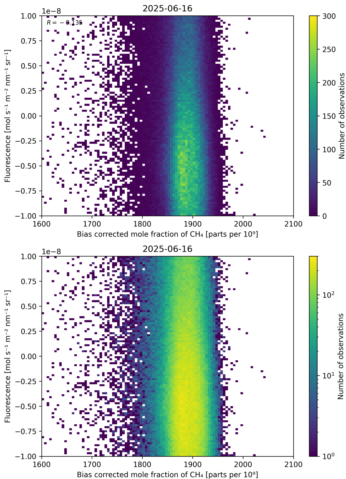
Figure 66: Scatter density plot of “Bias corrected mole fraction of \text{CH}_4 ” against “Fluorescence” for 2025-06-16 to 2025-06-17.
