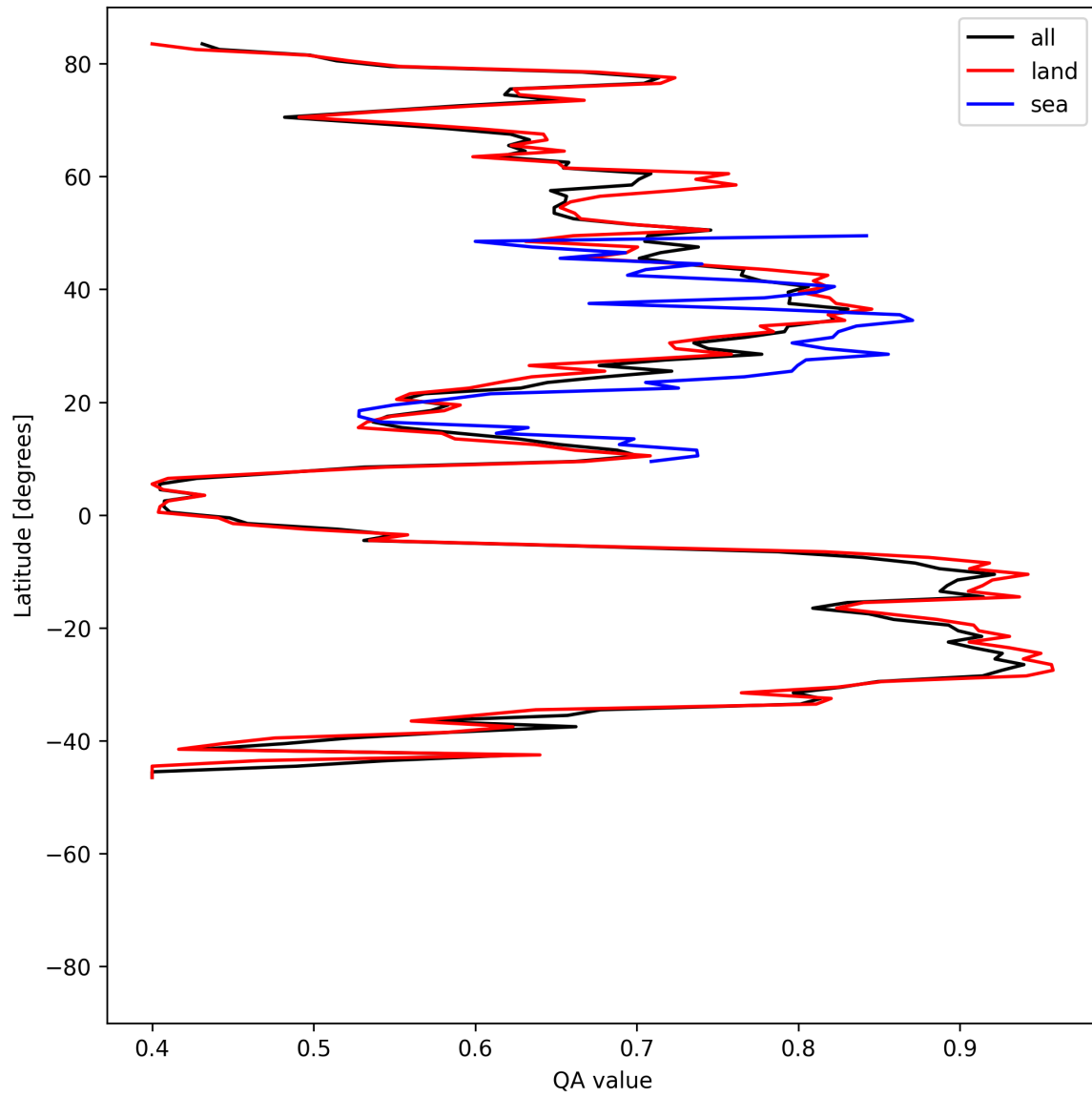
Figure 11: Zonal average of “QA value” for 2025-06-16 to 2025-06-17.
