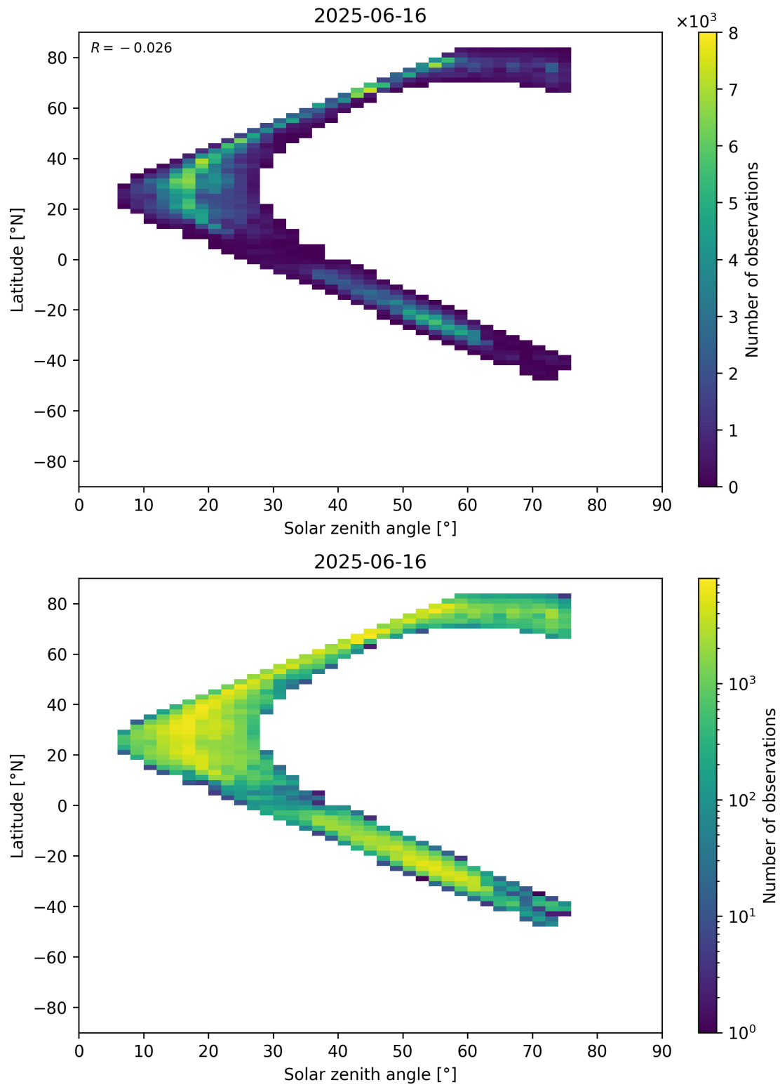
Figure 98: Scatter density plot of “Solar zenith angle” against “Latitude” for 2025-06-16 to 2025-06-17.
