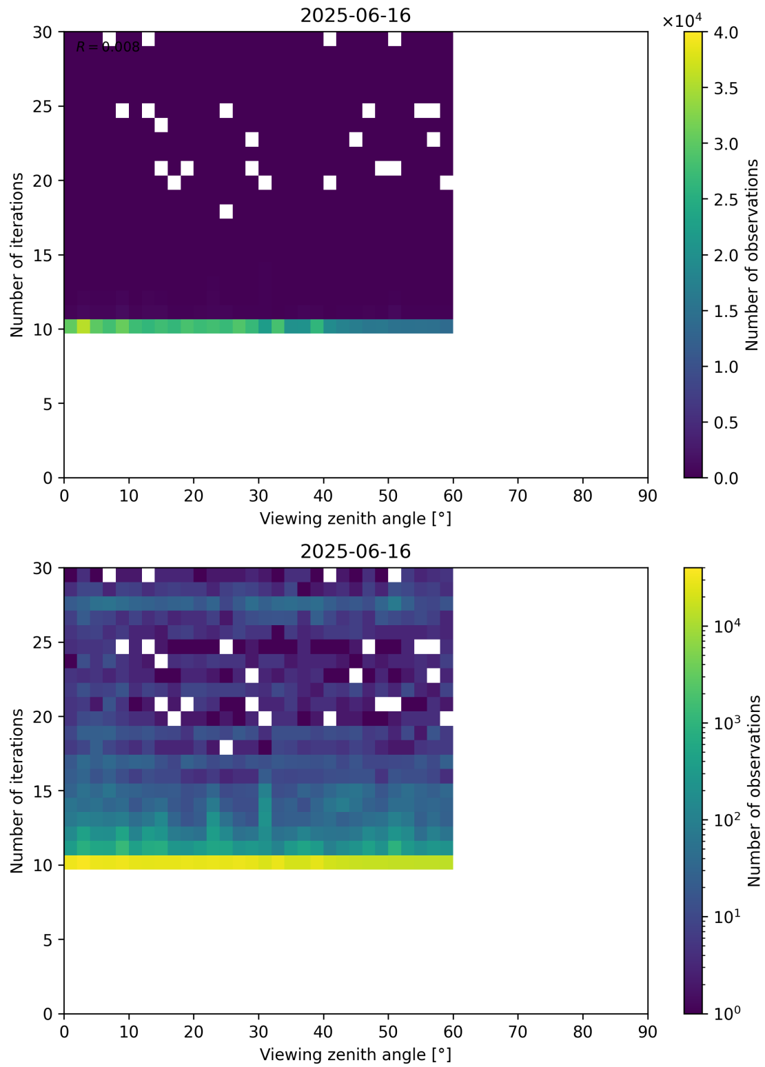
Figure 113: Scatter density plot of “Viewing zenith angle” against “Number of iterations” for 2025-06-16 to 2025-06-17.
