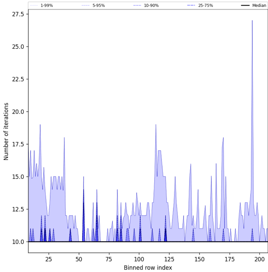
Figure 42: Along track statistics of “Number of iterations” for 2025-06-16 to 2025-06-17
