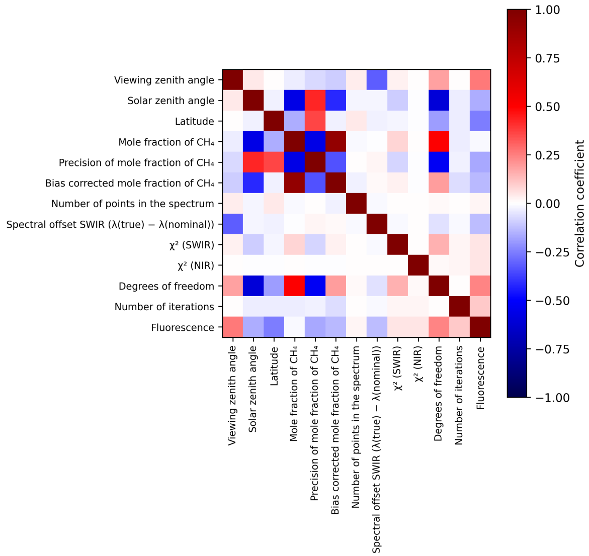
Figure 2: Map of correlation matrix for 2025-06-16 to 2025-06-17.
