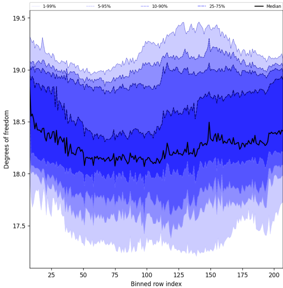
Figure 41: Along track statistics of “Degrees of freedom” for 2025-06-16 to 2025-06-17
