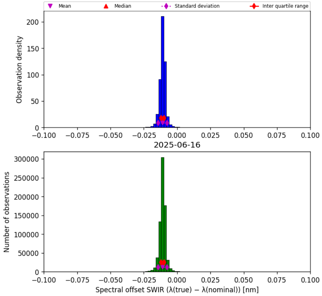
Figure 27: Histogram of “Spectral offset SWIR ( \lambda_{\text{true}} - \lambda_{\text{nominal}} )” for 2025-06-16 to 2025-06-17
