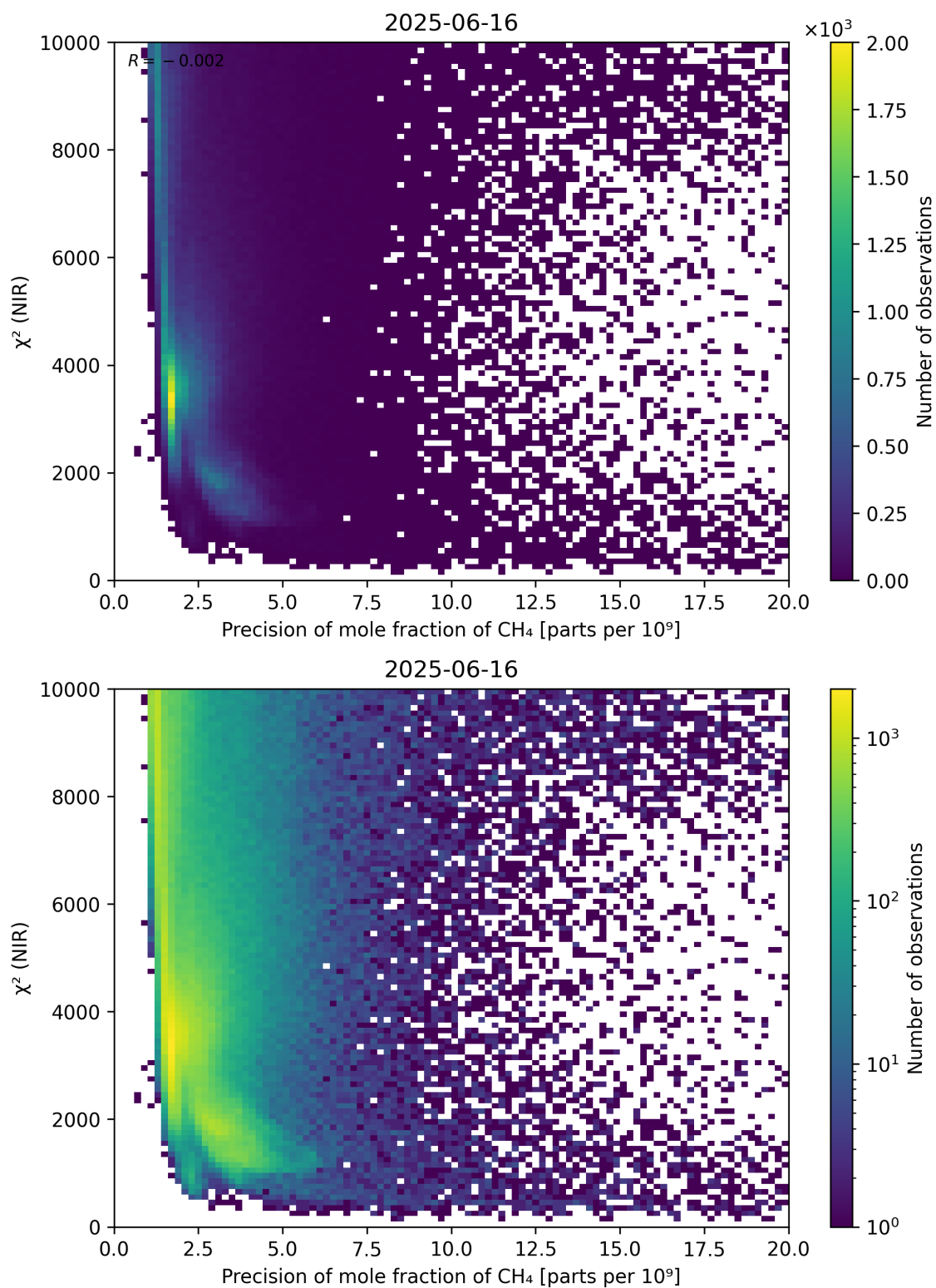
Figure 78: Scatter density plot of “Precision of mole fraction of CH 4 ” against “ \chi^2 (NIR)” for 2025-06-16 to 2025-06-17.
