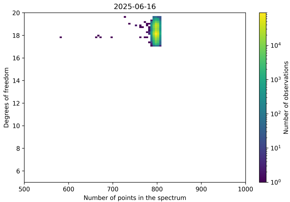
Figure 90: Scatter density plot of “Number of points in the spectrum” against “Degrees of freedom” for 2025-06-16 to 2025-06-17.
