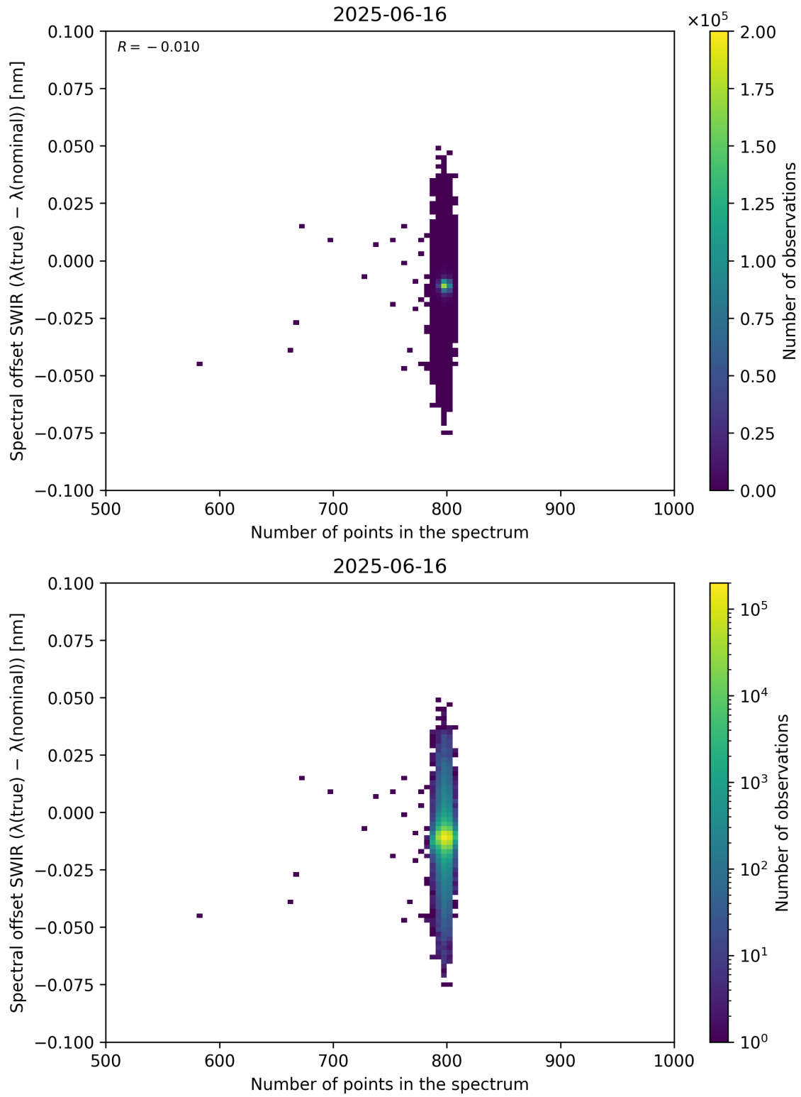
Figure 93: Scatter density plot of “Number of points in the spectrum” against “Spectral offset SWIR ( \lambda_{\text{true}} - \lambda_{\text{nominal}} )” for 2025-06-16 to 2025-06-17.
