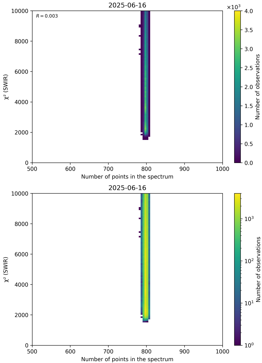
Figure 89: Scatter density plot of “Number of points in the spectrum” against “ \chi^2 (SWIR)” for 2025-06-16 to 2025-06-17.
