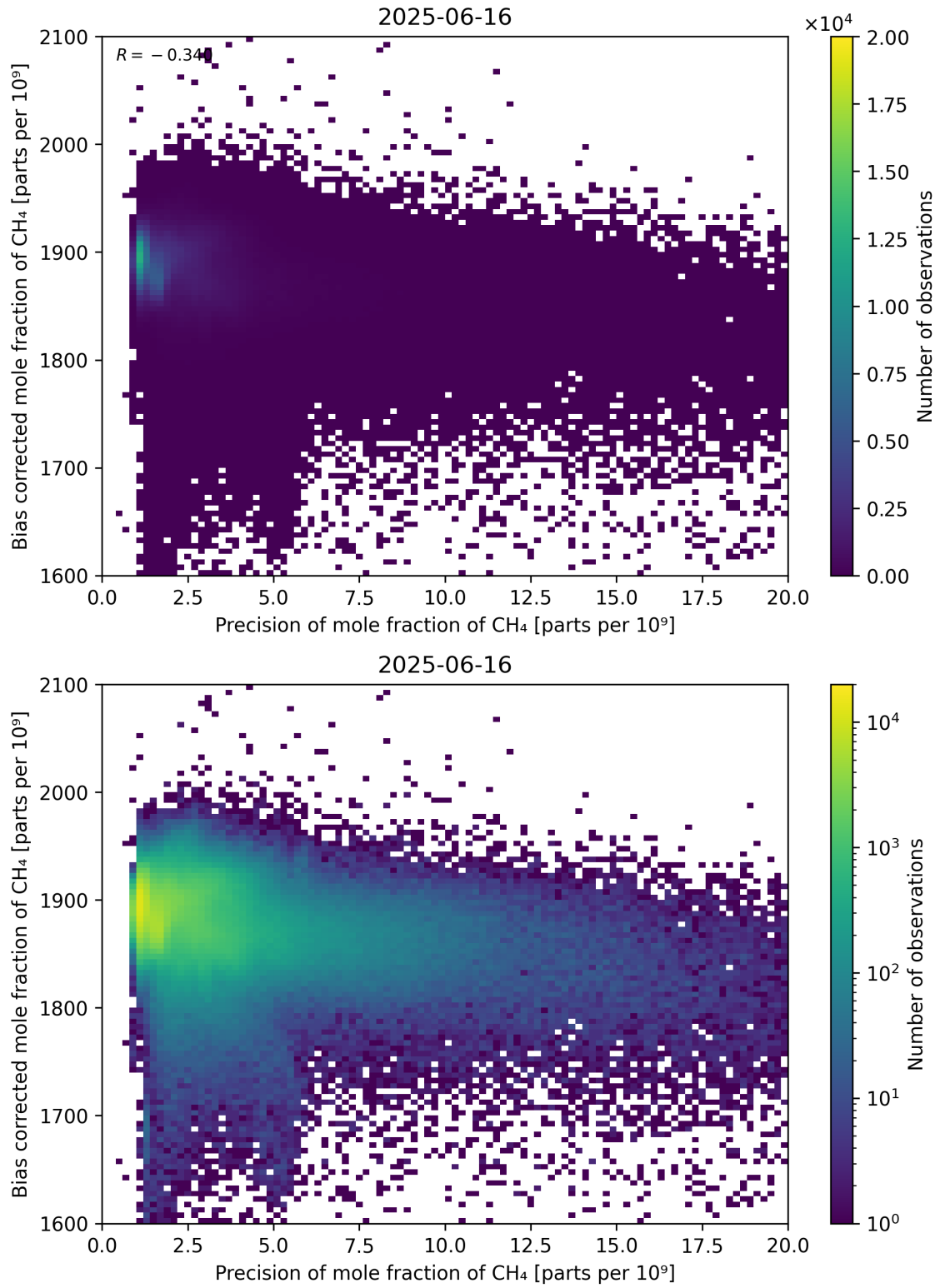
Figure 82: Scatter density plot of “Precision of mole fraction of CH 4 ” against “Bias corrected mole fraction of CH 4 ” for 2025-06-16 to 2025-06-17.
