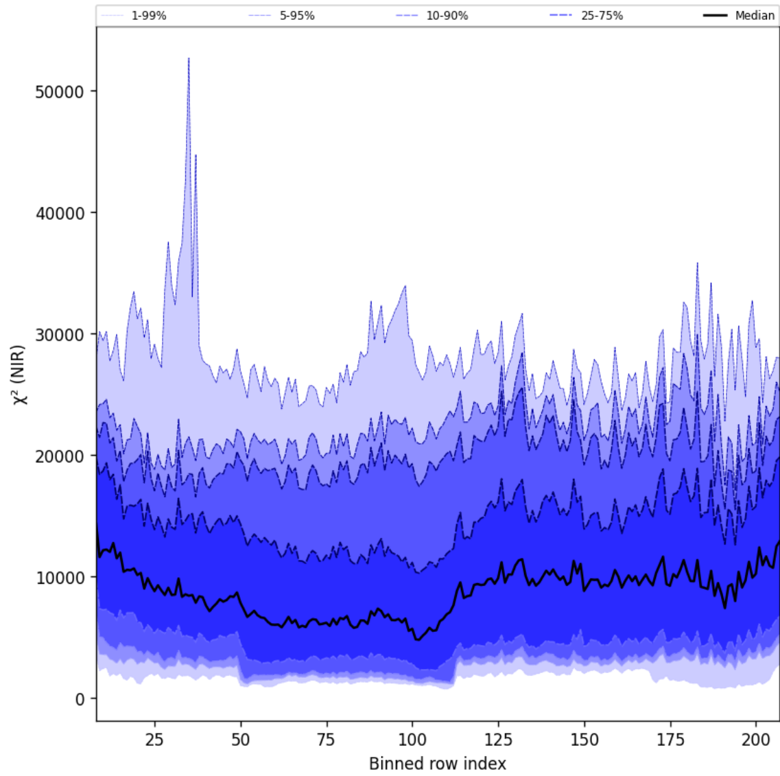
Figure 40: Along track statistics of “ \chi^2 (NIR)” for 2025-06-16 to 2025-06-17
