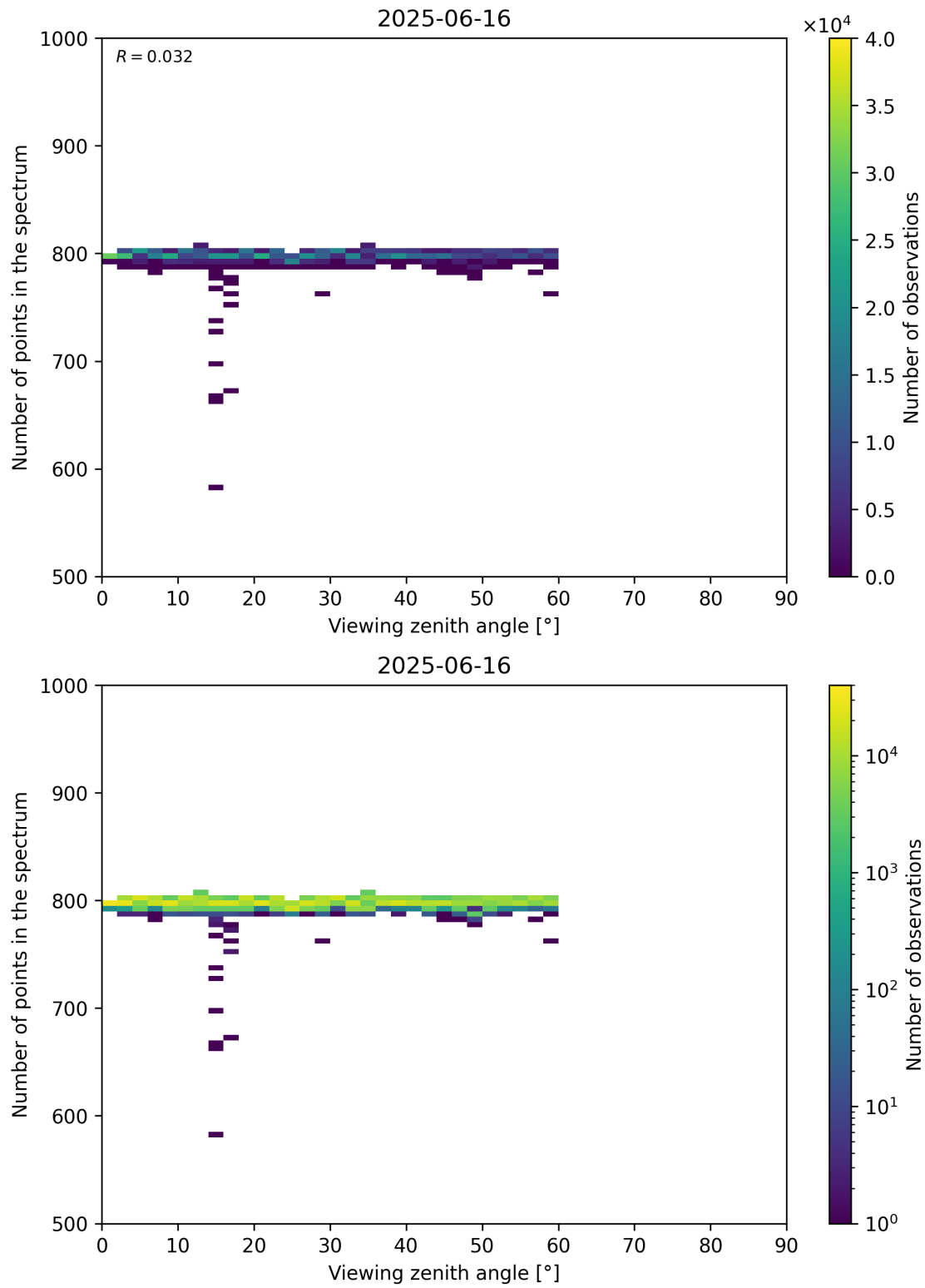
Figure 114: Scatter density plot of “Viewing zenith angle” against “Number of points in the spectrum” for 2025-06-16 to 2025-06-17.
