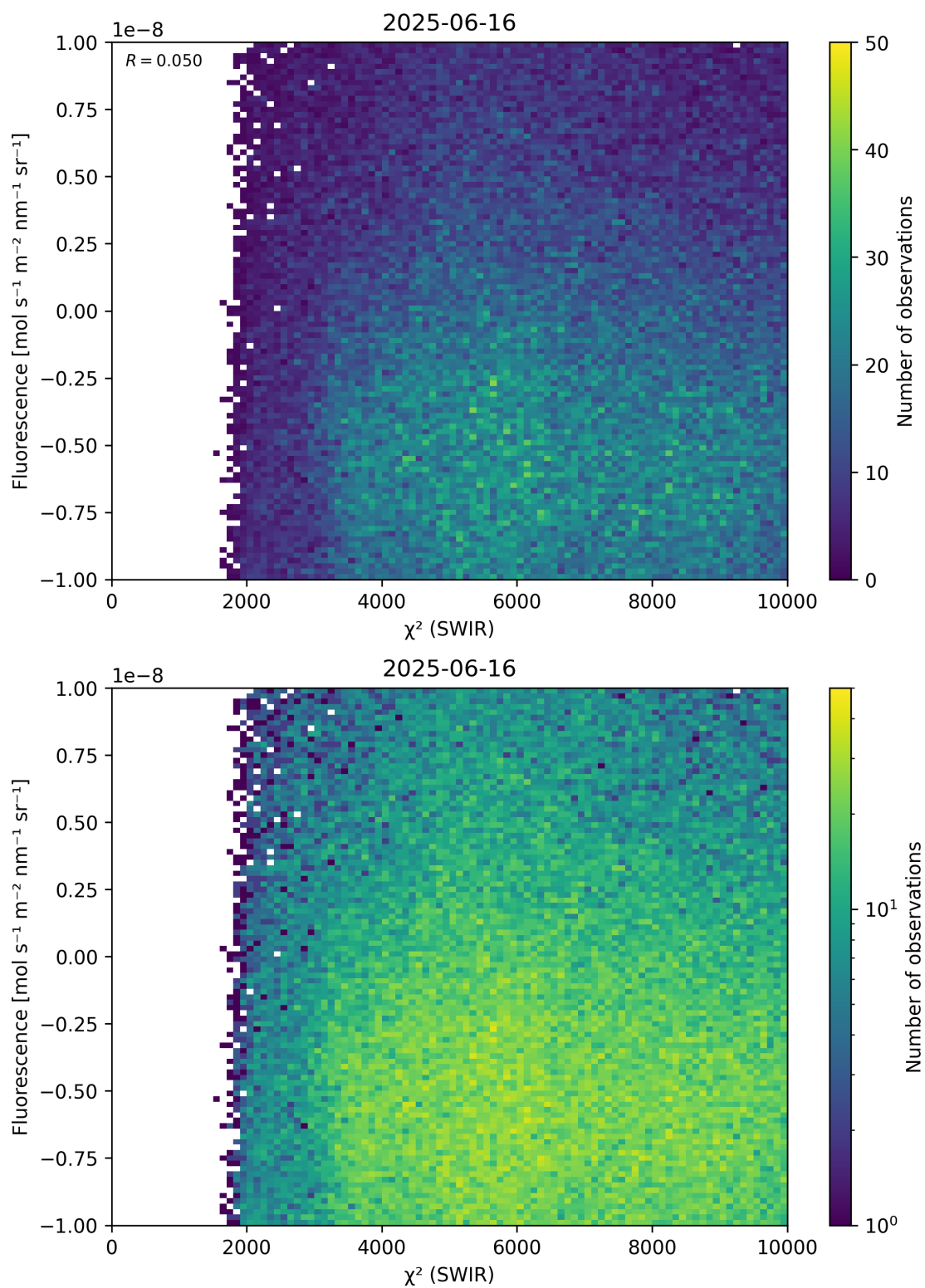
Figure 49: Scatter density plot of “ \chi^2 (SWIR)” against “Fluorescence” for 2025-06-16 to 2025-06-17.
