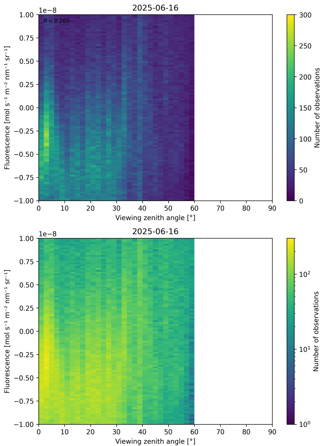
Figure 108: Scatter density plot of “Viewing zenith angle” against “Fluorescence” for 2025-06-16 to 2025-06-17.
