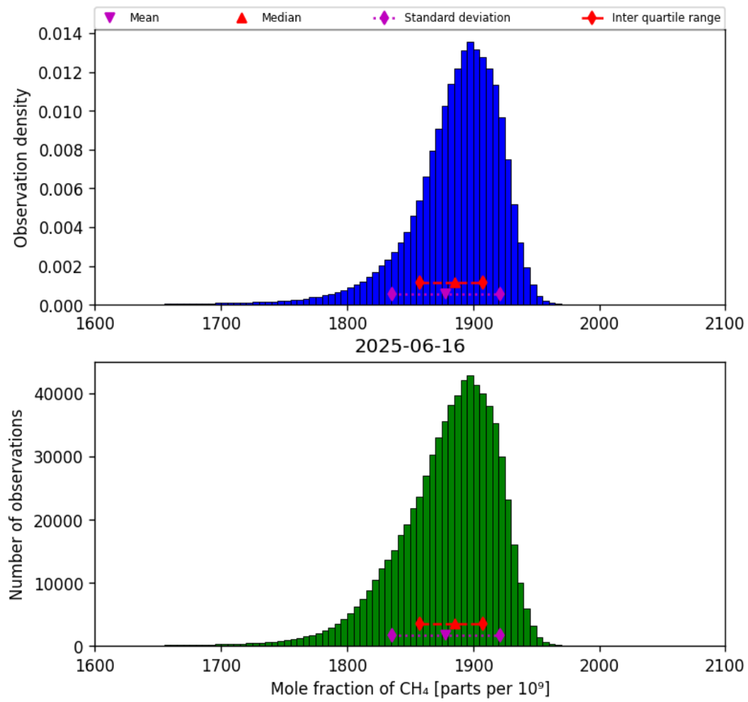
Figure 23: Histogram of “Mole fraction of CH 4 ” for 2025-06-16 to 2025-06-17
