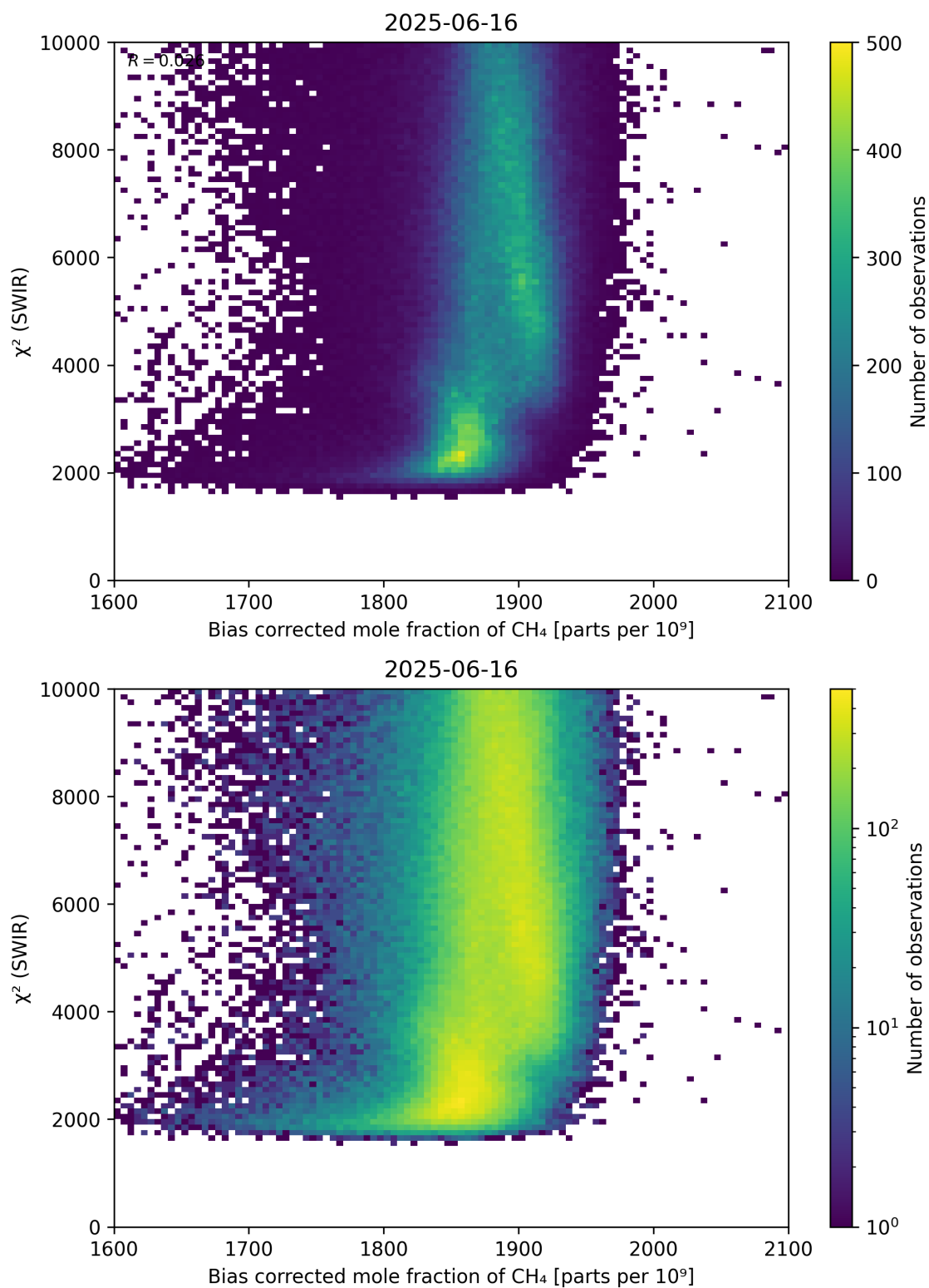
Figure 64: Scatter density plot of “Bias corrected mole fraction of \text{CH}_4 ” against “ \chi^2 (SWIR)” for 2025-06-16 to 2025-06-17.
