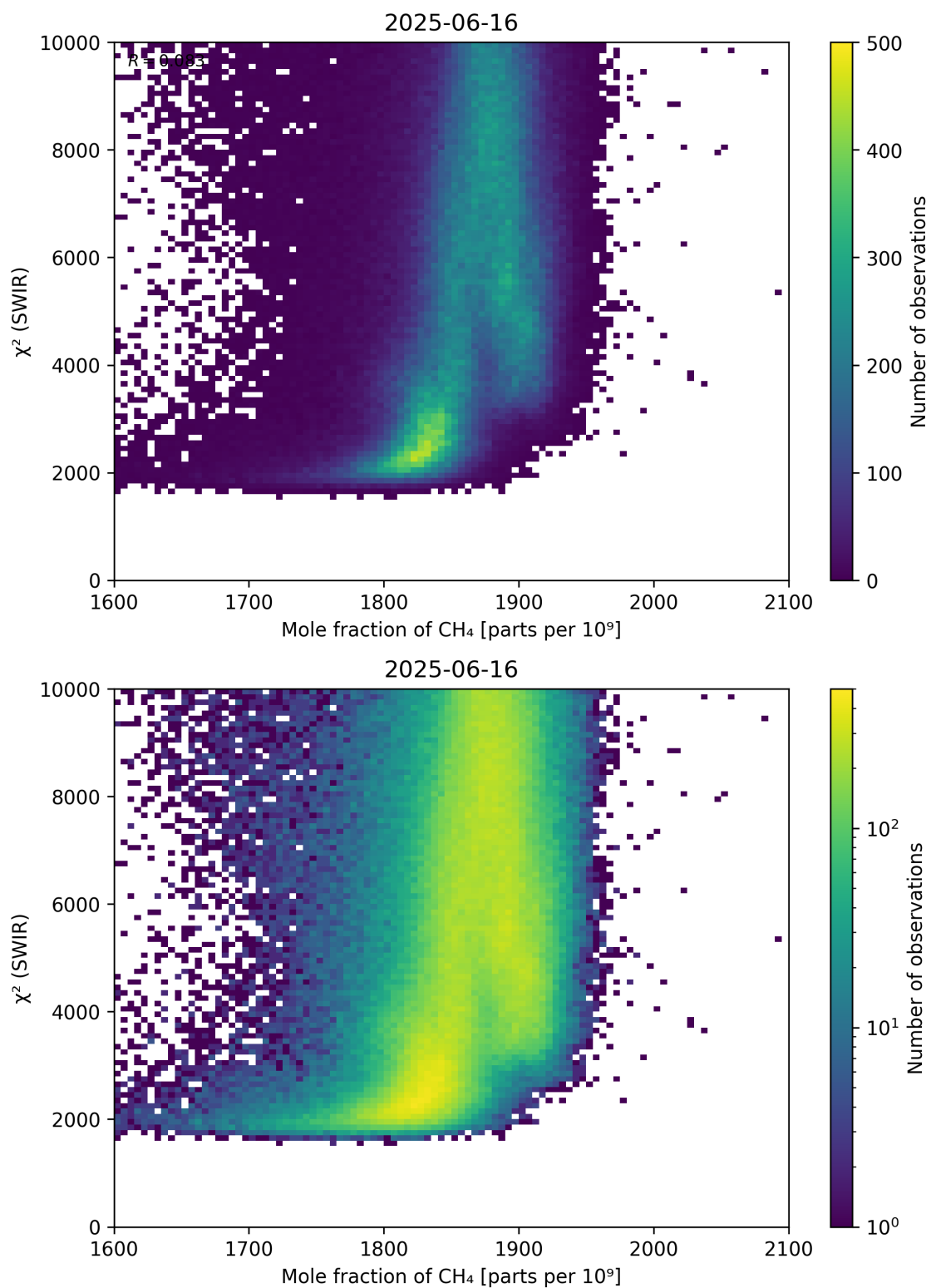
Figure 71: Scatter density plot of “Mole fraction of \text{CH}_4 ” against “ \chi^2 (SWIR)” for 2025-06-16 to 2025-06-17.
