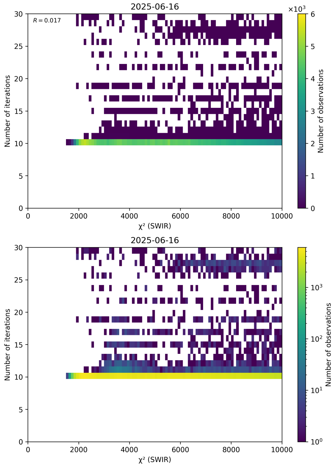
Figure 50: Scatter density plot of “ \chi^2 (SWIR)” against “Number of iterations” for 2025-06-16 to 2025-06-17.
