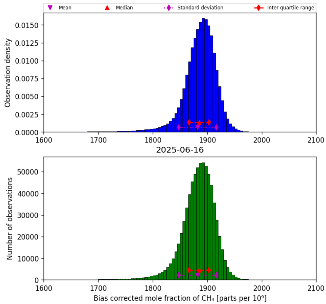
Figure 25: Histogram of “Bias corrected mole fraction of CH 4 ” for 2025-06-16 to 2025-06-17
