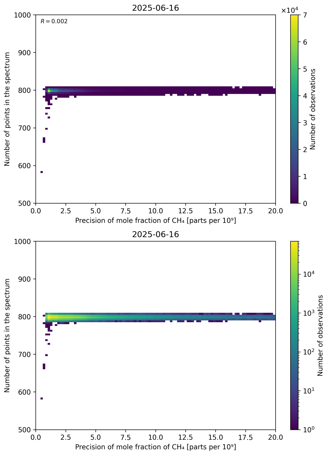
Figure 84: Scatter density plot of “Precision of mole fraction of CH 4 ” against “Number of points in the spectrum” for 2025-06-16 to 2025-06-17.
