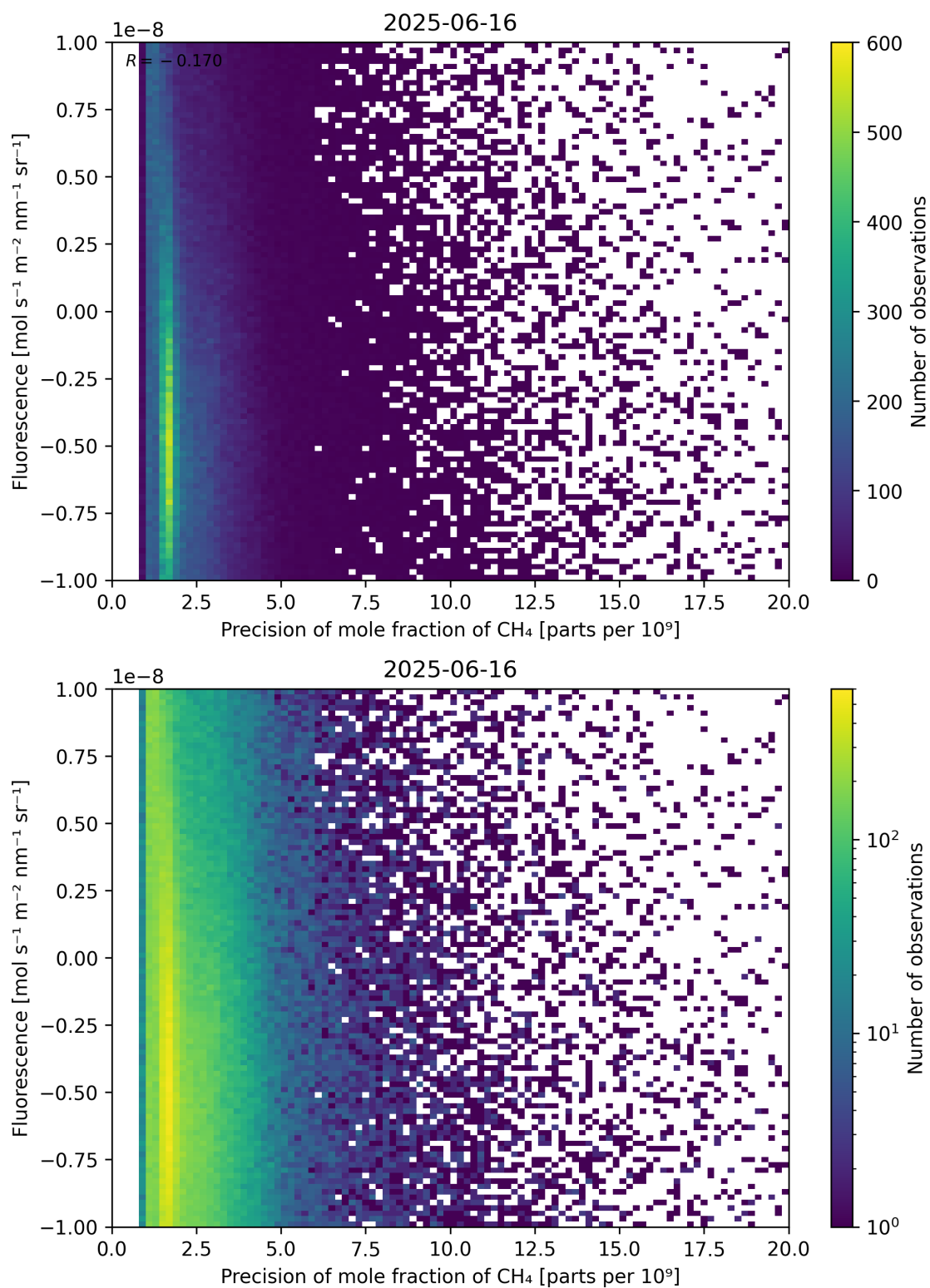
Figure 81: Scatter density plot of “Precision of mole fraction of \text{CH}_4 ” against “Fluorescence” for 2025-06-16 to 2025-06-17.
