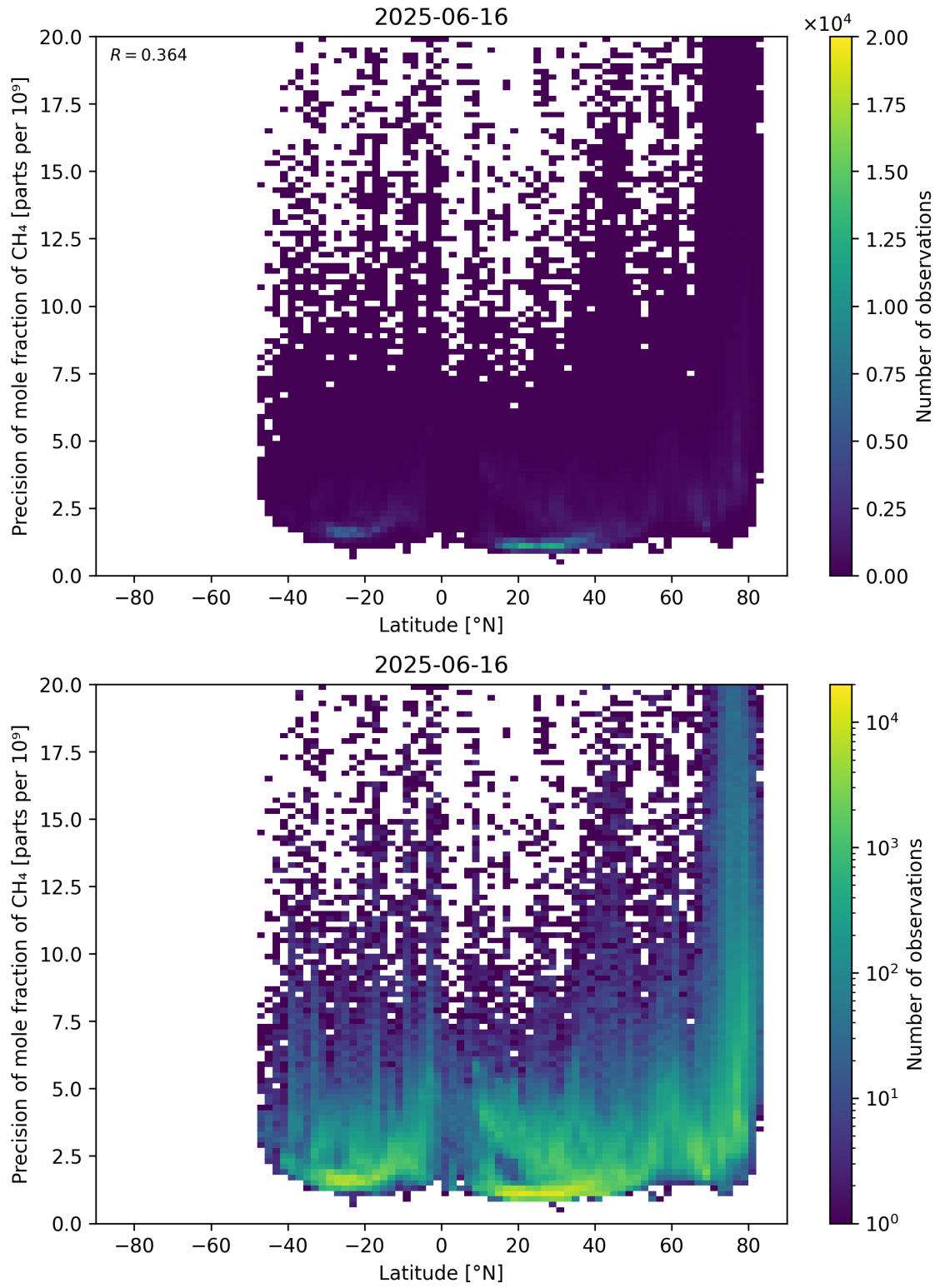
Figure 59: Scatter density plot of “Latitude” against “Precision of mole fraction of CH 4 ” for 2025-06-16 to 2025-06-17.
