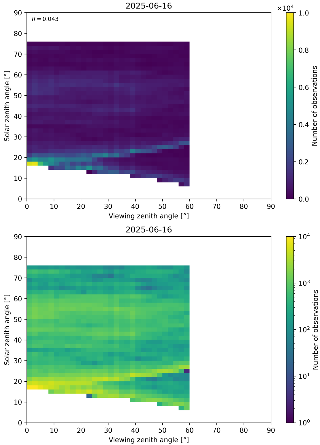
Figure 115: Scatter density plot of “Viewing zenith angle” against “Solar zenith angle” for 2025-06-16 to 2025-06-17.
