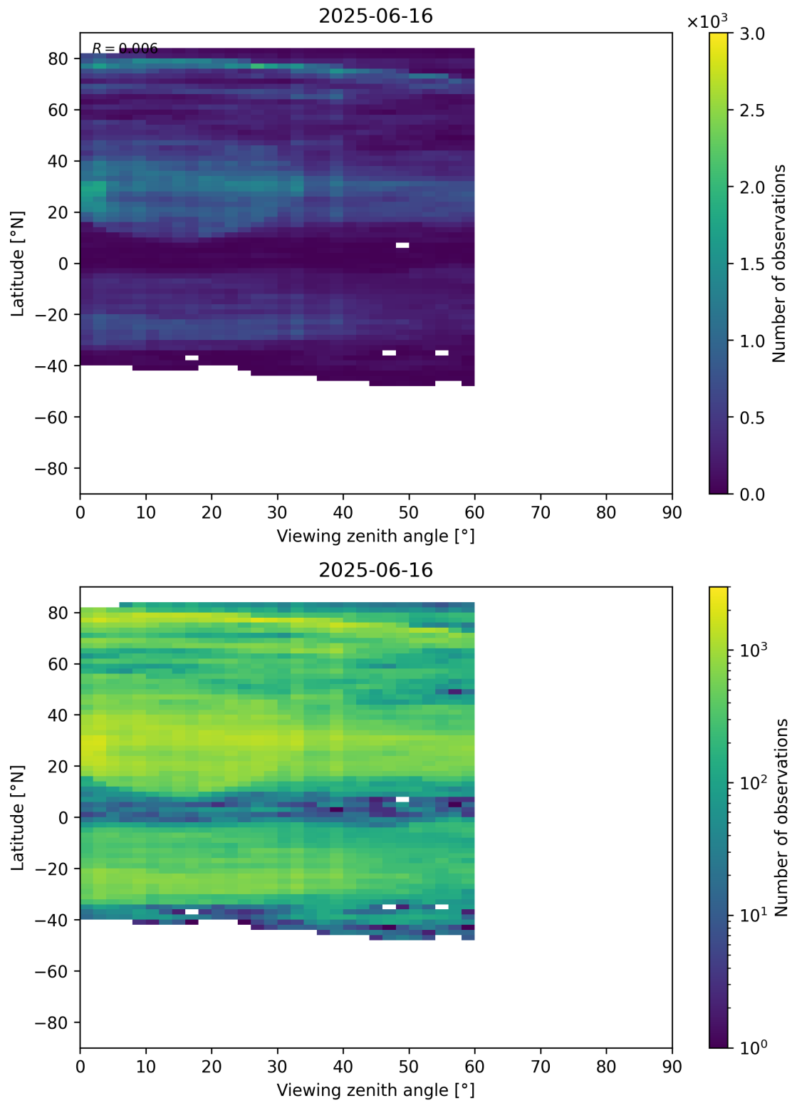
Figure 109: Scatter density plot of “Viewing zenith angle” against “Latitude” for 2025-06-16 to 2025-06-17.
