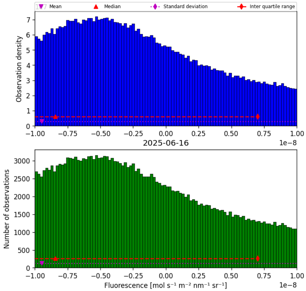
Figure 32: Histogram of “Fluorescence” for 2025-06-16 to 2025-06-17
