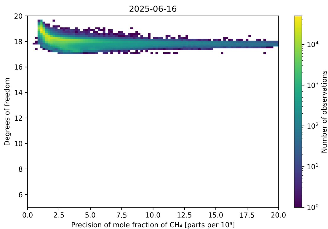
Figure 80: Scatter density plot of “Precision of mole fraction of CH 4 ” against “Degrees of freedom” for 2025-06-16 to 2025-06-17.
