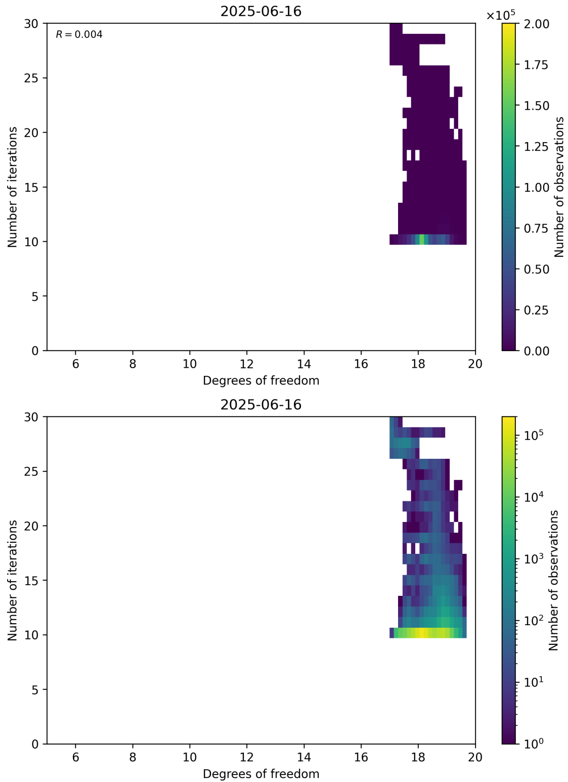
Figure 52: Scatter density plot of “Degrees of freedom” against “Number of iterations” for 2025-06-16 to 2025-06-17.
