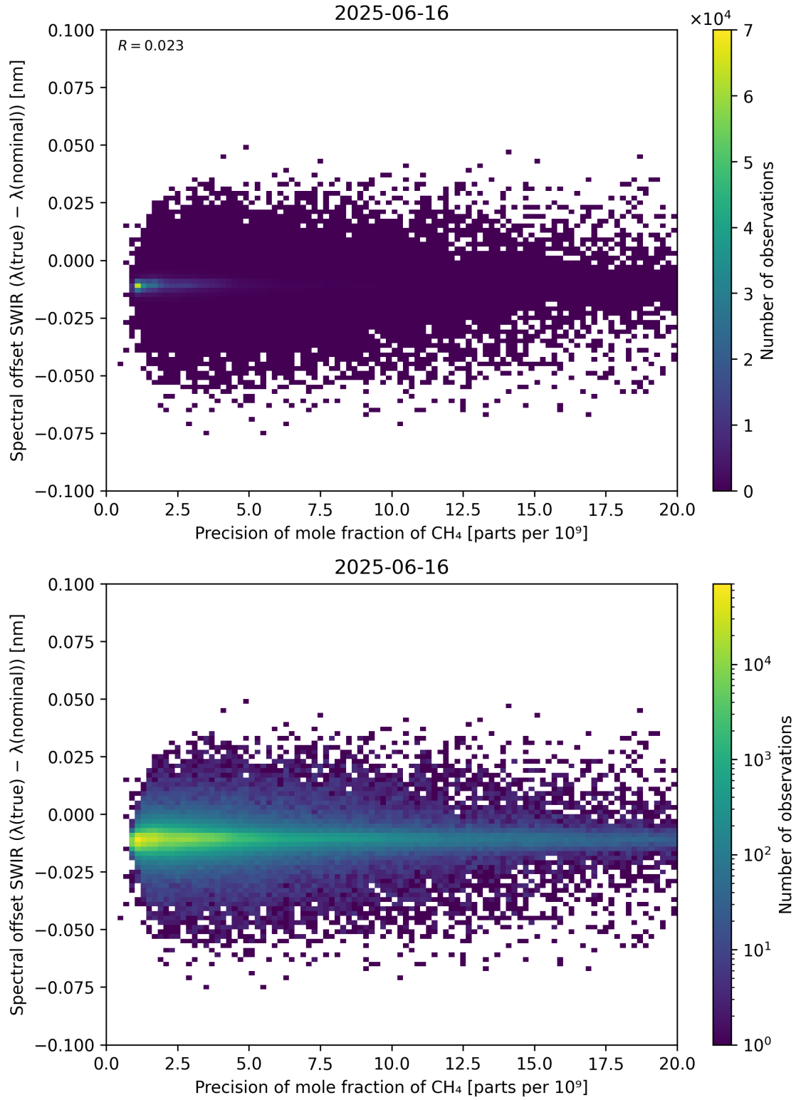
Figure 85: Scatter density plot of “Precision of mole fraction of \text{CH}_4 ” against “Spectral offset SWIR ( \lambda_{\text{true}} - \lambda_{\text{nominal}} )” for 2025-06-16 to 2025-06-17.
