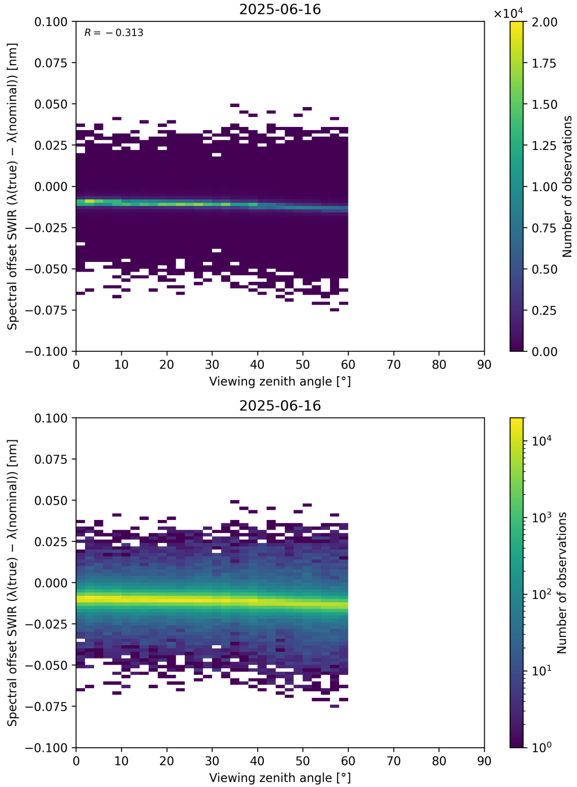
Figure 116: Scatter density plot of “Viewing zenith angle” against “Spectral offset SWIR ( \lambda_{\text{true}} - \lambda_{\text{nominal}} )” for 2025-06-16 to 2025-06-17.
