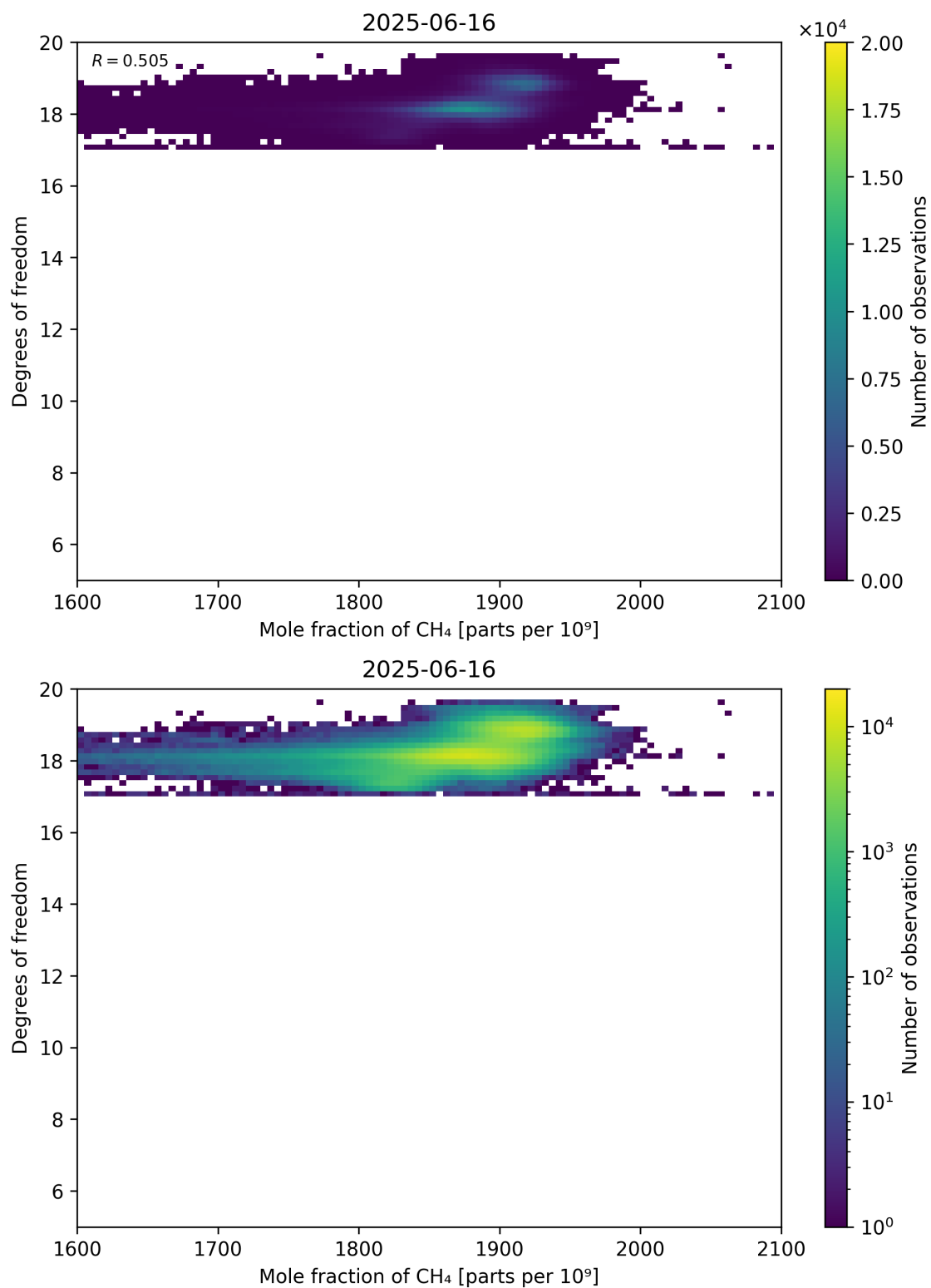
Figure 72: Scatter density plot of “Mole fraction of CH 4 ” against “Degrees of freedom” for 2025-06-16 to 2025-06-17.
