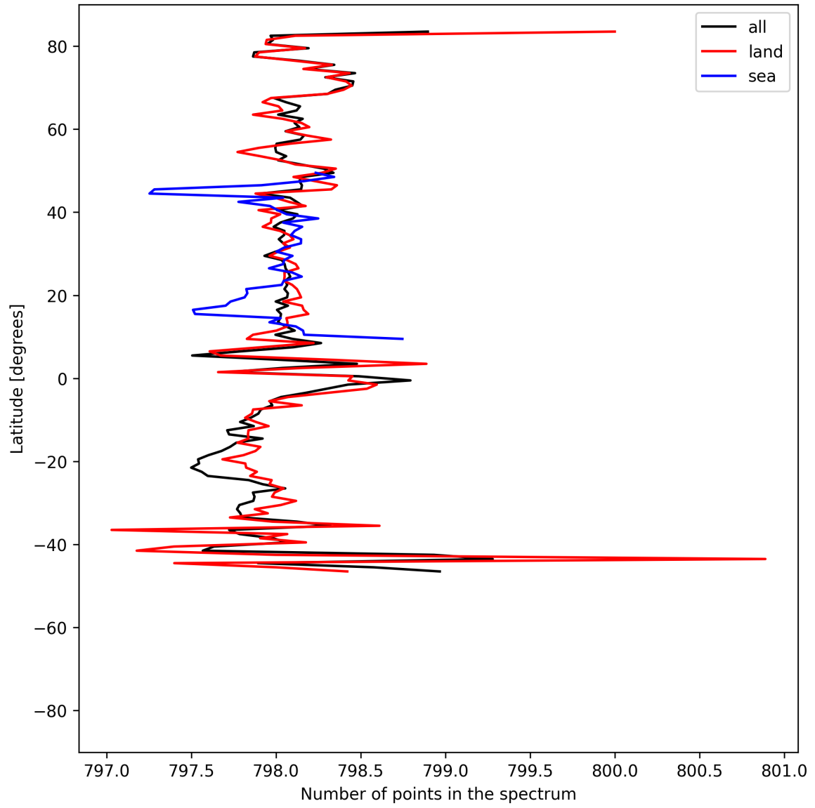
Figure 15: Zonal average of “Number of points in the spectrum” for 2025-06-16 to 2025-06-17.
