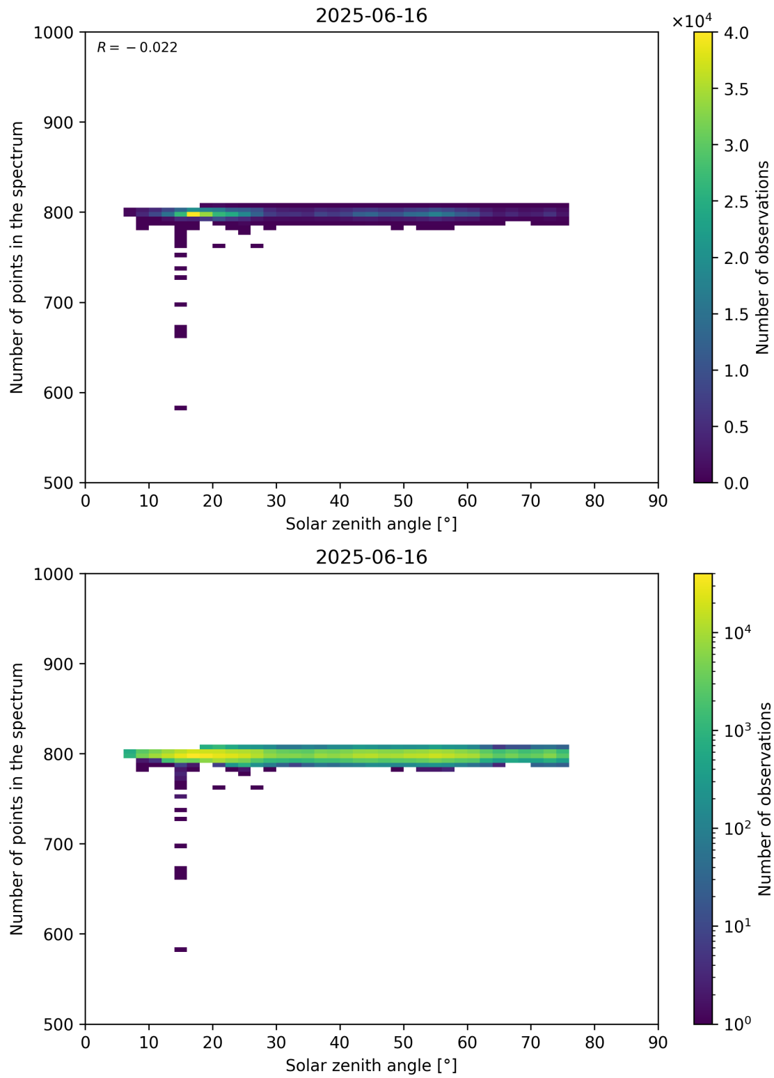
Figure 103: Scatter density plot of “Solar zenith angle” against “Number of points in the spectrum” for 2025-06-16 to 2025-06-17.
