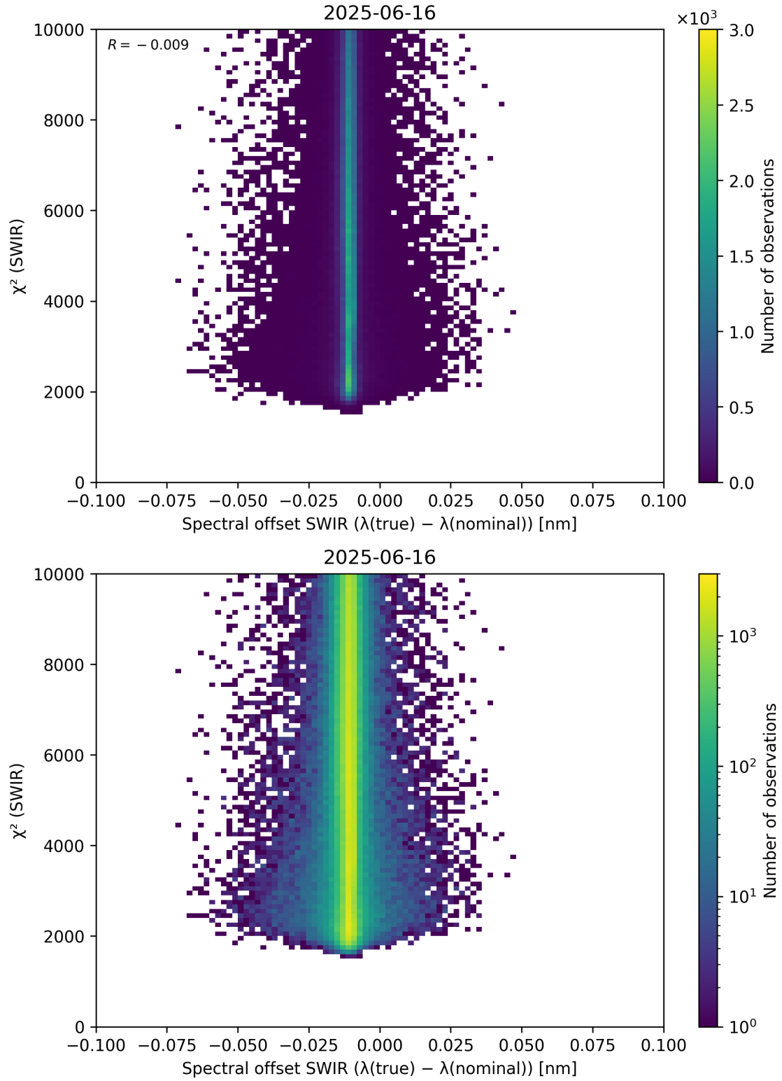
Figure 118: Scatter density plot of “Spectral offset SWIR ( \lambda_{\text{true}} - \lambda_{\text{nominal}} )” against “ \chi^2 (SWIR)” for 2025-06-16 to 2025-06-17.
