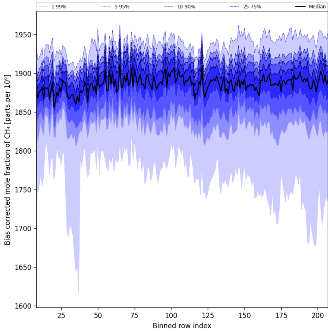
Figure 36: Along track statistics of “Bias corrected mole fraction of CH 4 ” for 2025-06-16 to 2025-06-17
