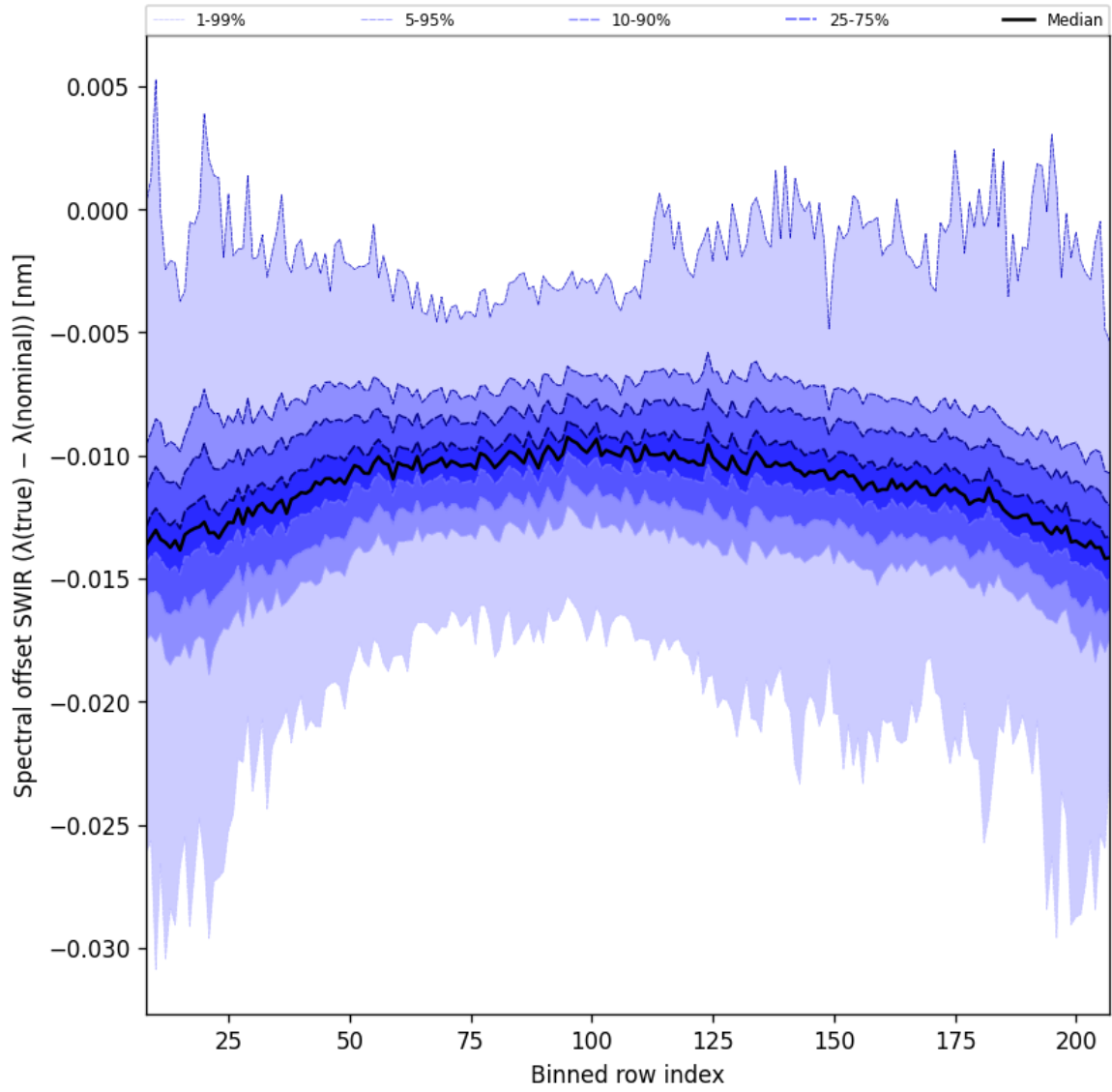
Figure 38: Along track statistics of “Spectral offset SWIR ( \lambda_{\text{true}} - \lambda_{\text{nominal}} )” for 2025-06-16 to 2025-06-17
