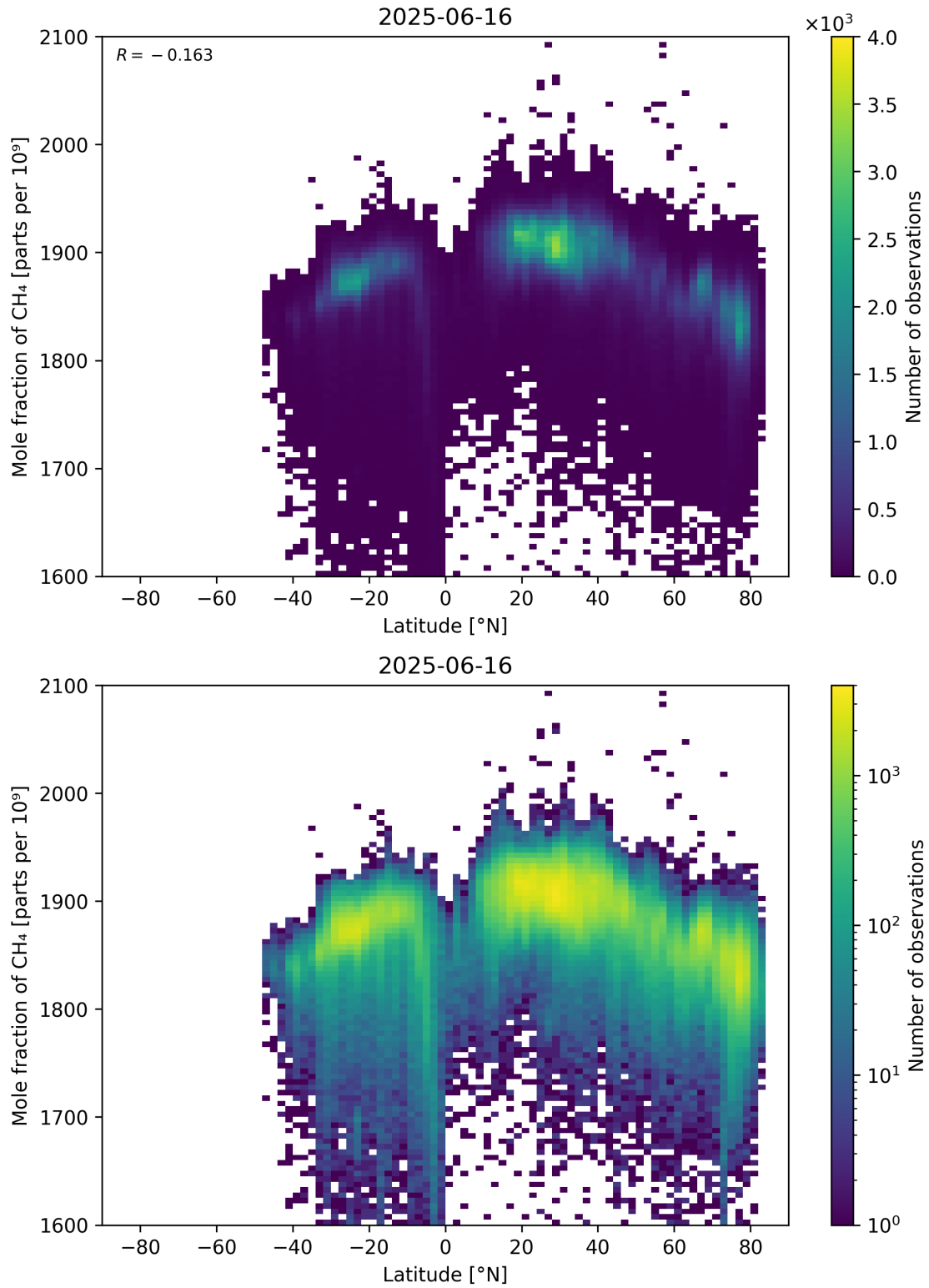
Figure 57: Scatter density plot of “Latitude” against “Mole fraction of \text{CH}_4 ” for 2025-06-16 to 2025-06-17.
