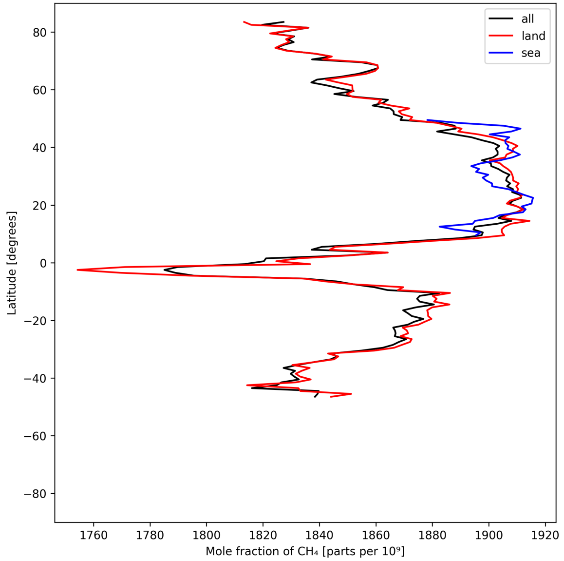
Figure 12: Zonal average of “Mole fraction of \text{CH}_4 ” for 2025-06-16 to 2025-06-17.
