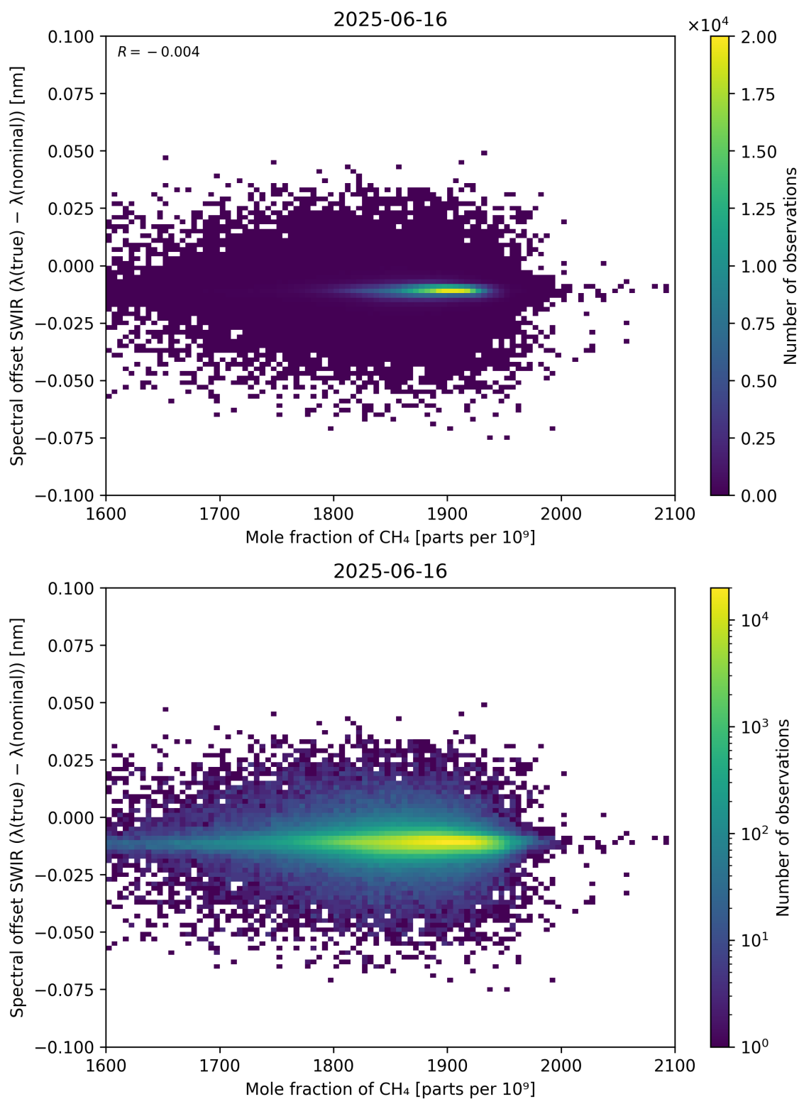
Figure 86: Scatter density plot of “Mole fraction of \text{CH}_4 ” against “Spectral offset SWIR ( \lambda_{\text{true}} - \lambda_{\text{nominal}} )” for 2025-06-16 to 2025-06-17.
