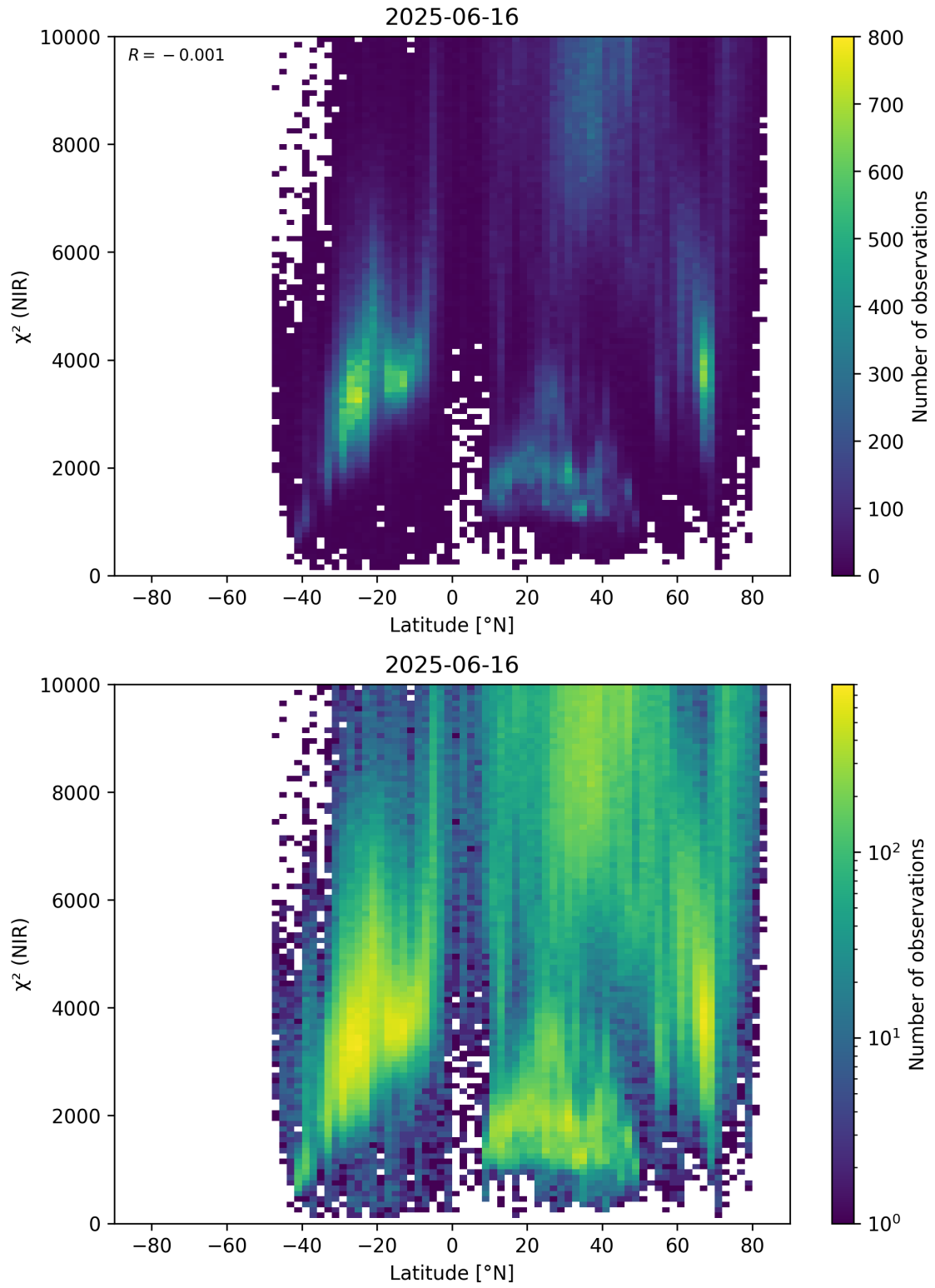
Figure 53: Scatter density plot of “Latitude” against “ \chi^2 (NIR)” for 2025-06-16 to 2025-06-17.
