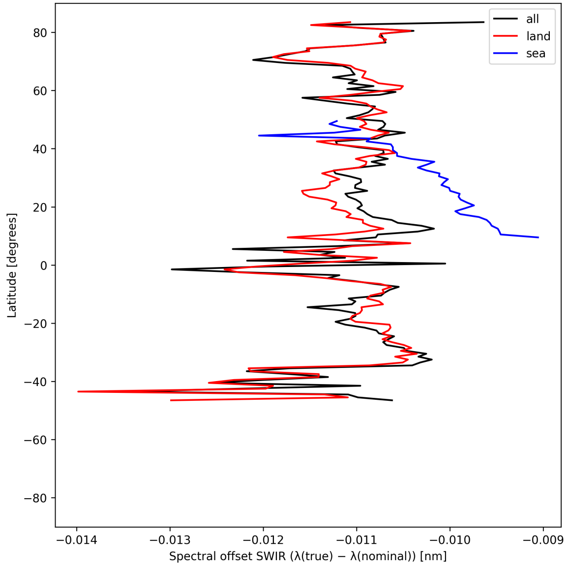
Figure 16: Zonal average of “Spectral offset SWIR ( \lambda_{\text{true}} - \lambda_{\text{nominal}} )” for 2025-06-16 to 2025-06-17.
