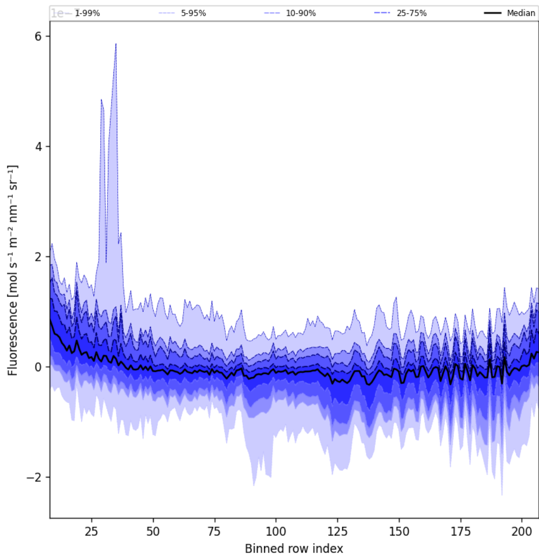
Figure 43: Along track statistics of “Fluorescence” for 2025-06-16 to 2025-06-17
