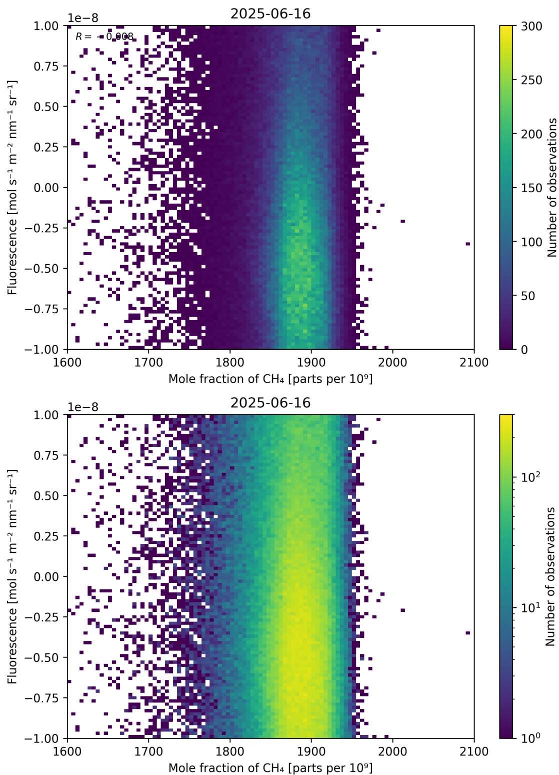
Figure 73: Scatter density plot of “Mole fraction of CH 4 ” against “Fluorescence” for 2025-06-16 to 2025-06-17.
