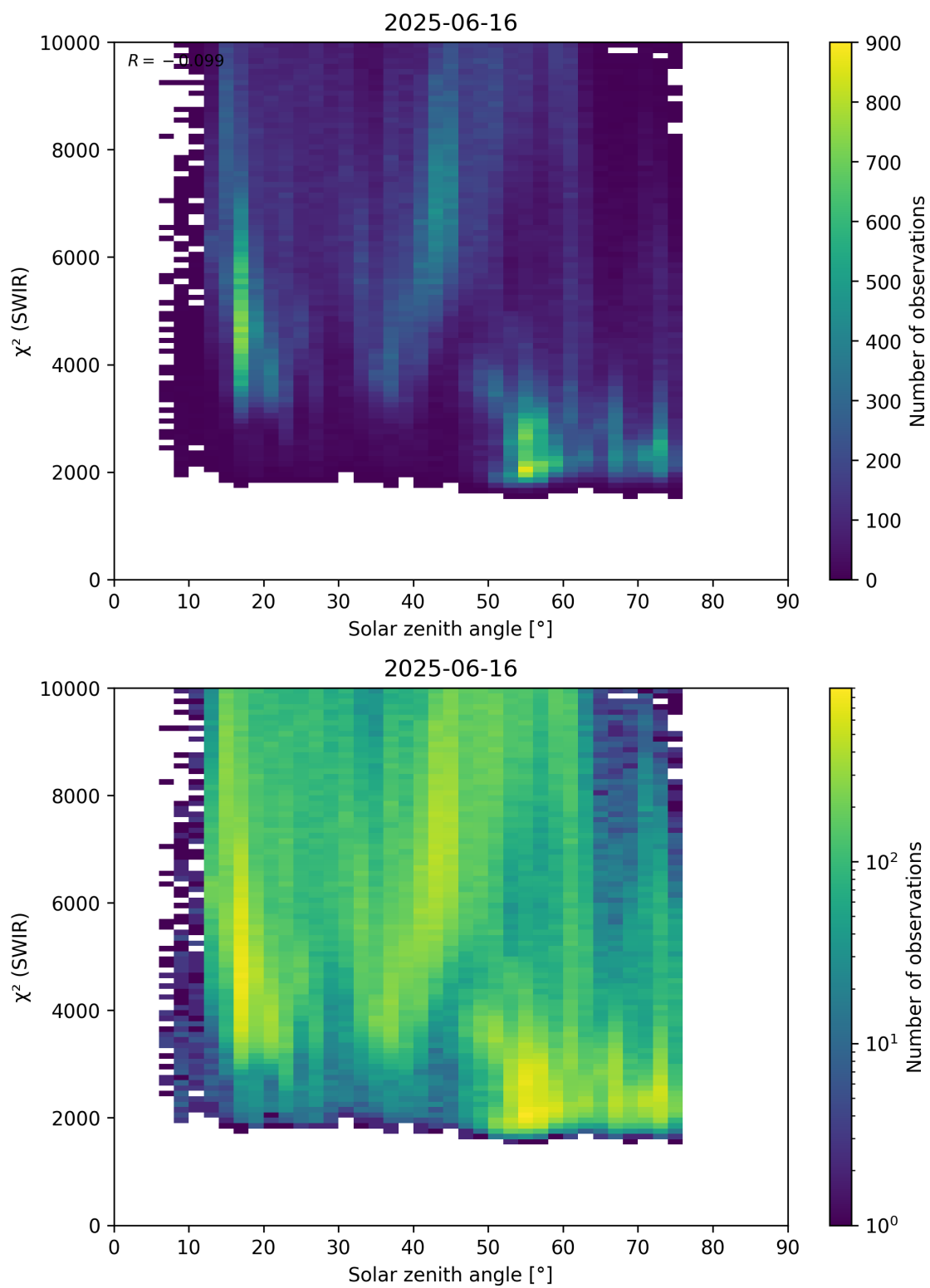
Figure 95: Scatter density plot of “Solar zenith angle” against “ \chi^2 (SWIR)” for 2025-06-16 to 2025-06-17.
