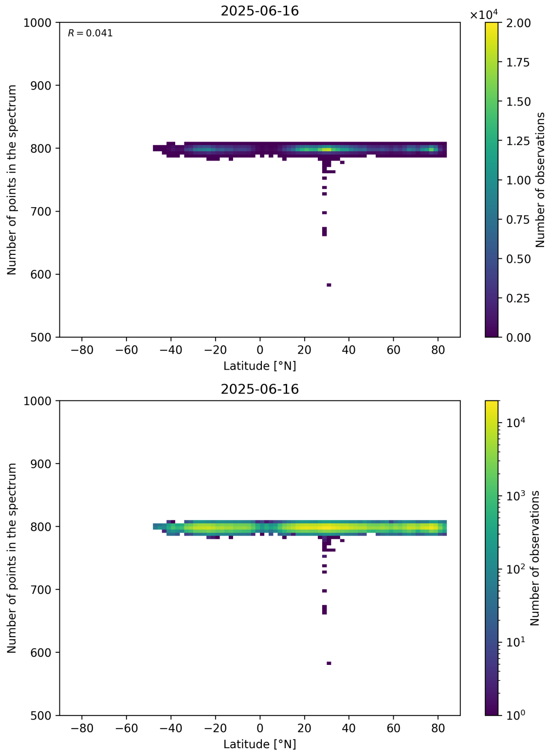
Figure 61: Scatter density plot of “Latitude” against “Number of points in the spectrum” for 2025-06-16 to 2025-06-17.
