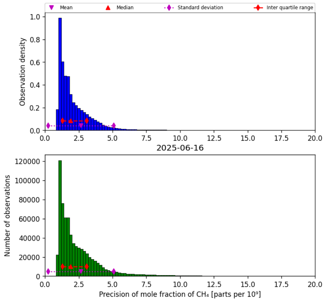
Figure 24: Histogram of “Precision of mole fraction of CH 4 ” for 2025-06-16 to 2025-06-17
