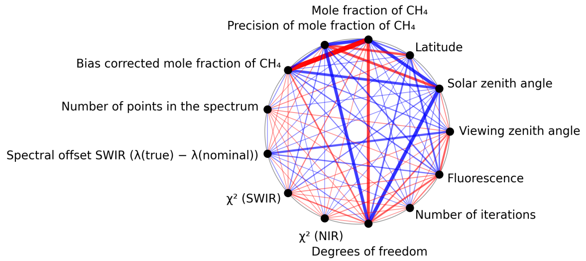
Figure 1: Map of correlation graph for 2025-06-16 to 2025-06-17.
