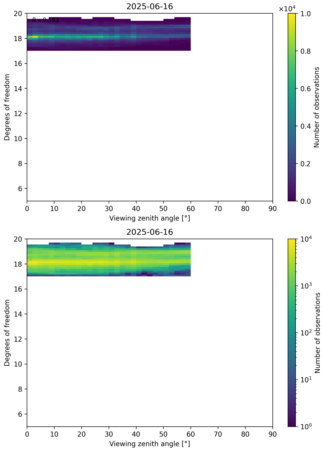
Figure 107: Scatter density plot of “Viewing zenith angle” against “Degrees of freedom” for 2025-06-16 to 2025-06-17.
