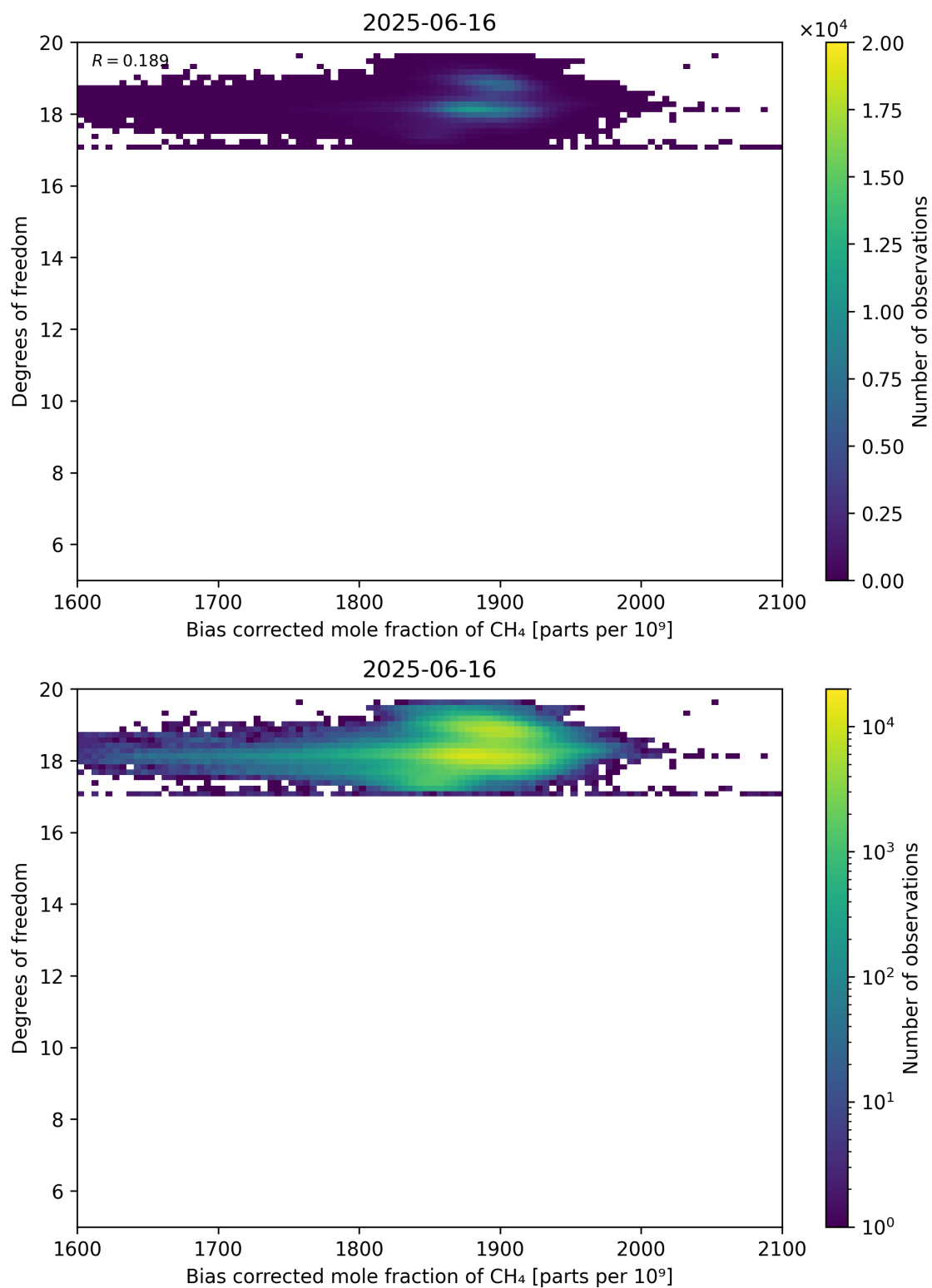
Figure 65: Scatter density plot of “Bias corrected mole fraction of CH 4 ” against “Degrees of freedom” for 2025-06-16 to 2025-06-17.
