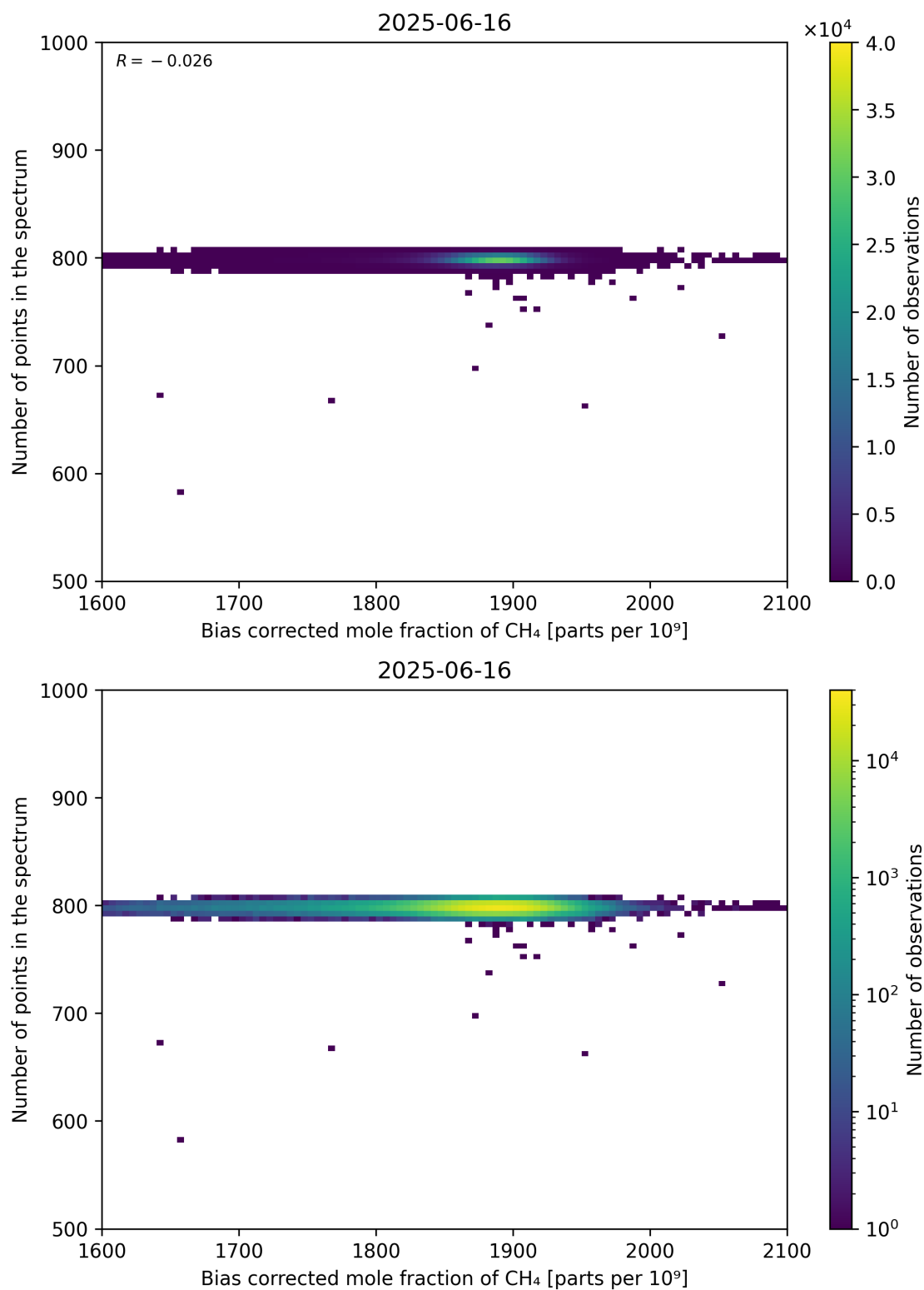
Figure 68: Scatter density plot of “Bias corrected mole fraction of CH 4 ” against “Number of points in the spectrum” for 2025-06-16 to 2025-06-17.
