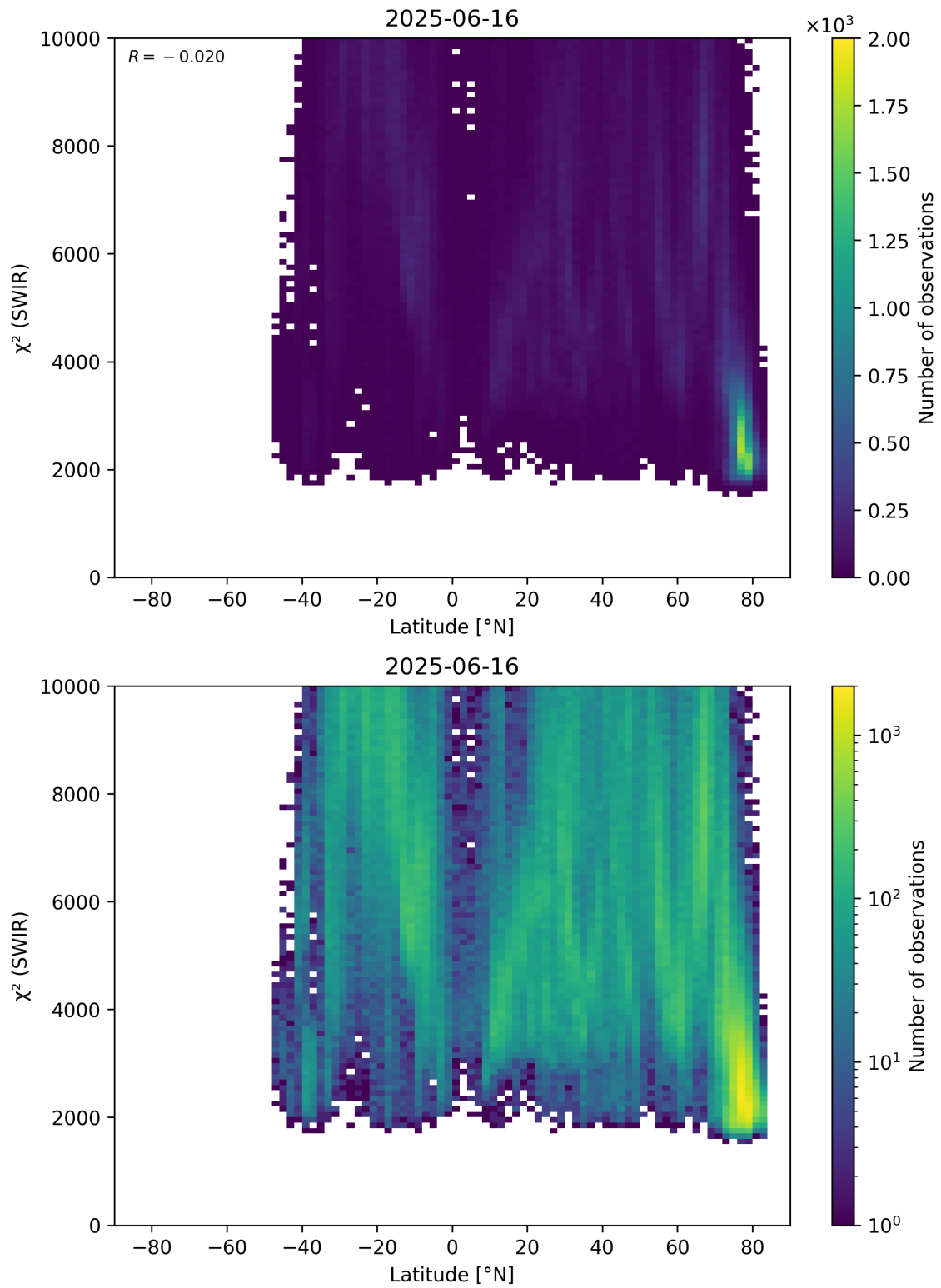
Figure 54: Scatter density plot of “Latitude” against “ \chi^2 (SWIR)” for 2025-06-16 to 2025-06-17.
