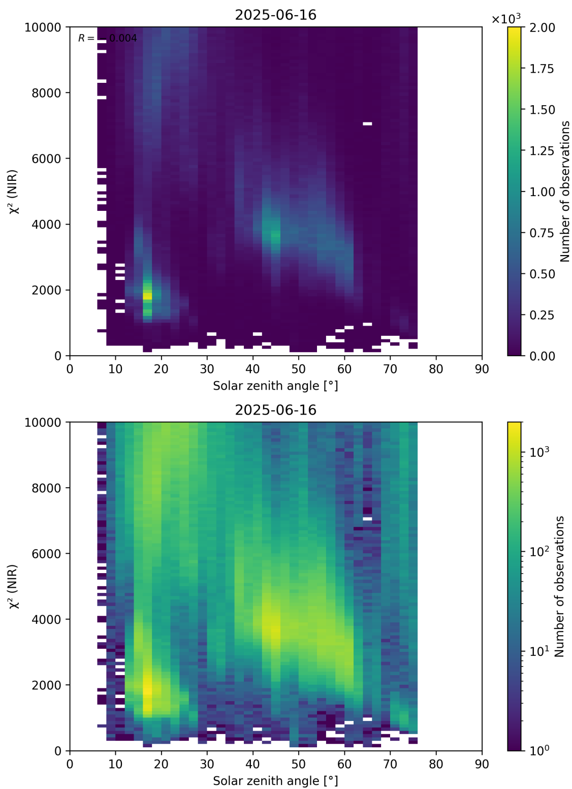
Figure 94: Scatter density plot of “Solar zenith angle” against “ \chi^2 (NIR)” for 2025-06-16 to 2025-06-17.
