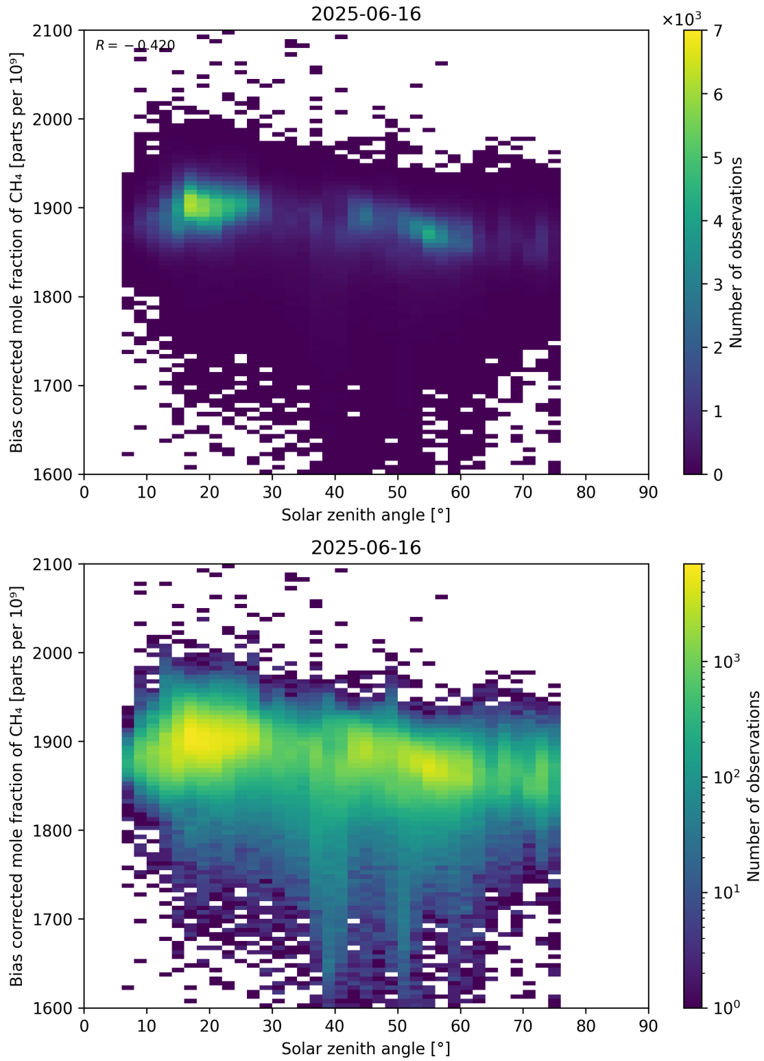
Figure 100: Scatter density plot of “Solar zenith angle” against “Bias corrected mole fraction of CH 4 ” for 2025-06-16 to 2025-06-17.
