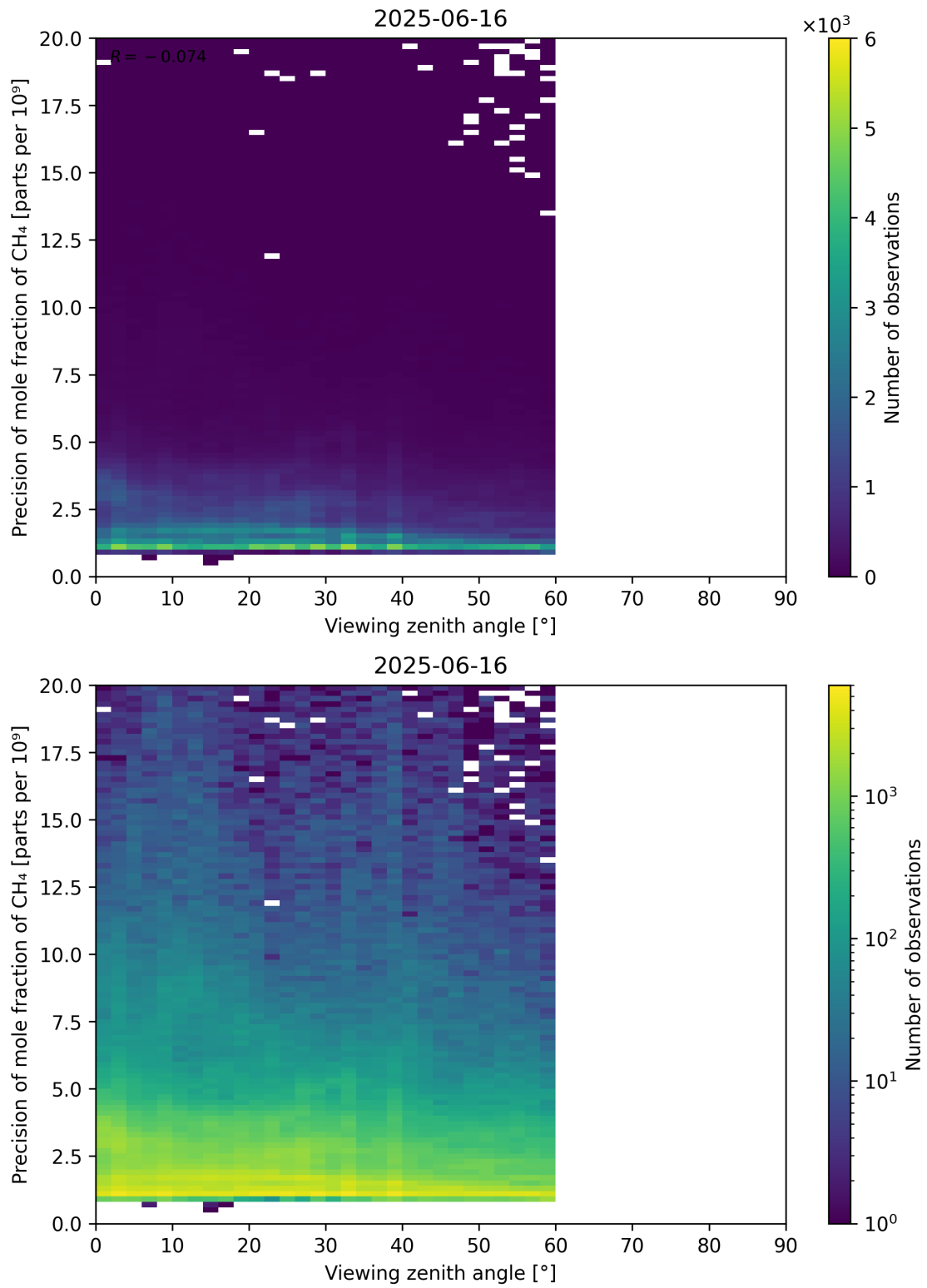
Figure 112: Scatter density plot of “Viewing zenith angle” against “Precision of mole fraction of CH 4 ” for 2025-06-16 to 2025-06-17.
