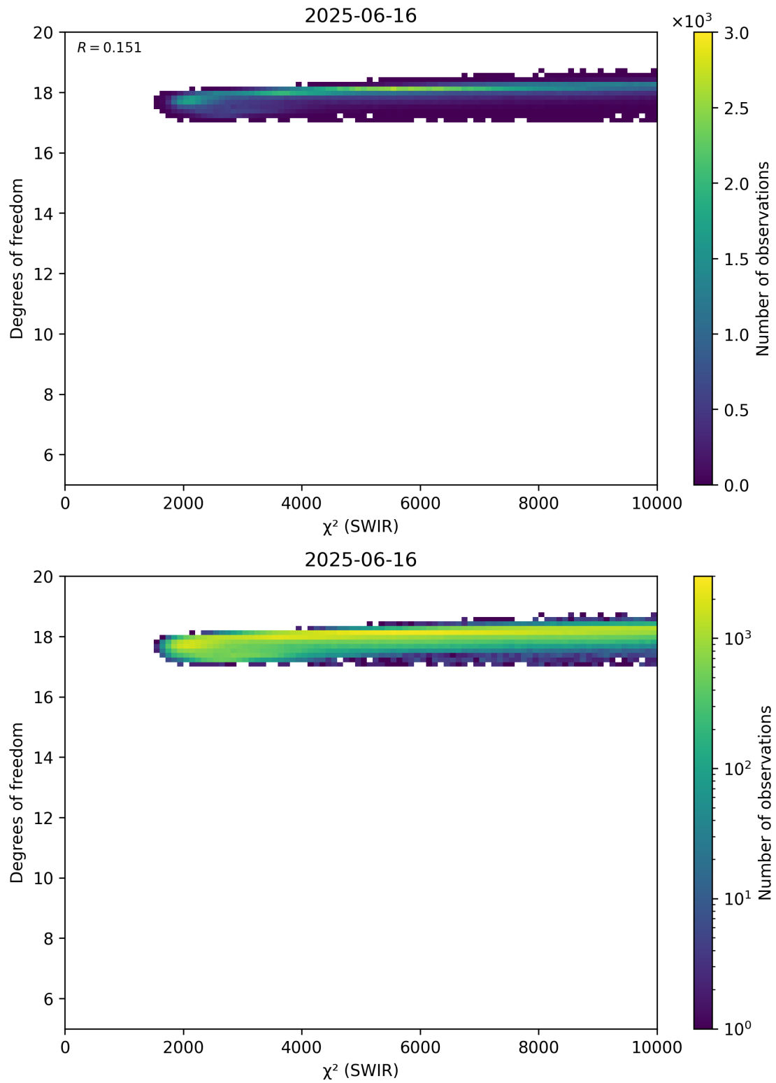
Figure 48: Scatter density plot of “ \chi^2 (SWIR)” against “Degrees of freedom” for 2025-06-16 to 2025-06-17.
