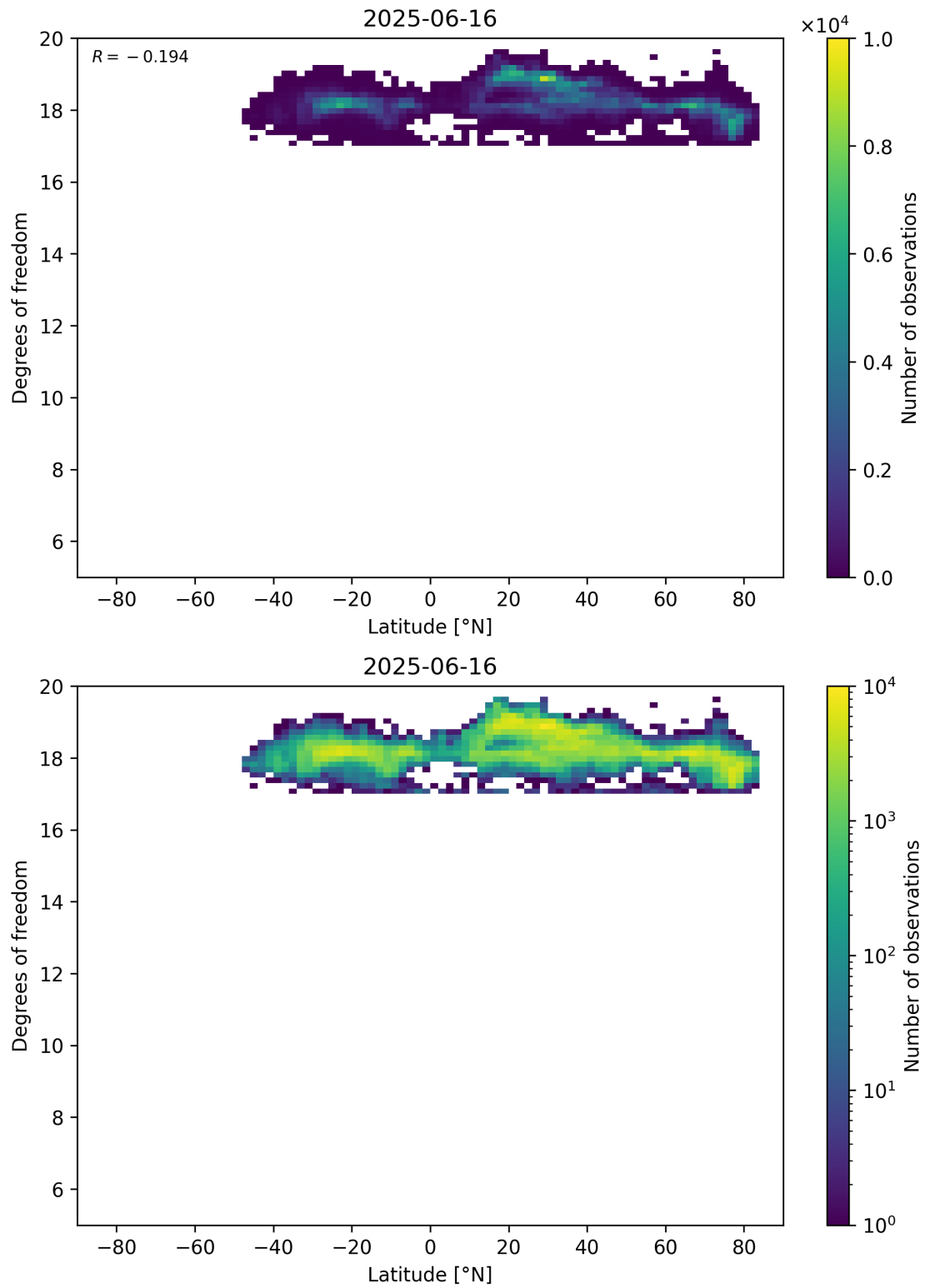
Figure 55: Scatter density plot of “Latitude” against “Degrees of freedom” for 2025-06-16 to 2025-06-17.
