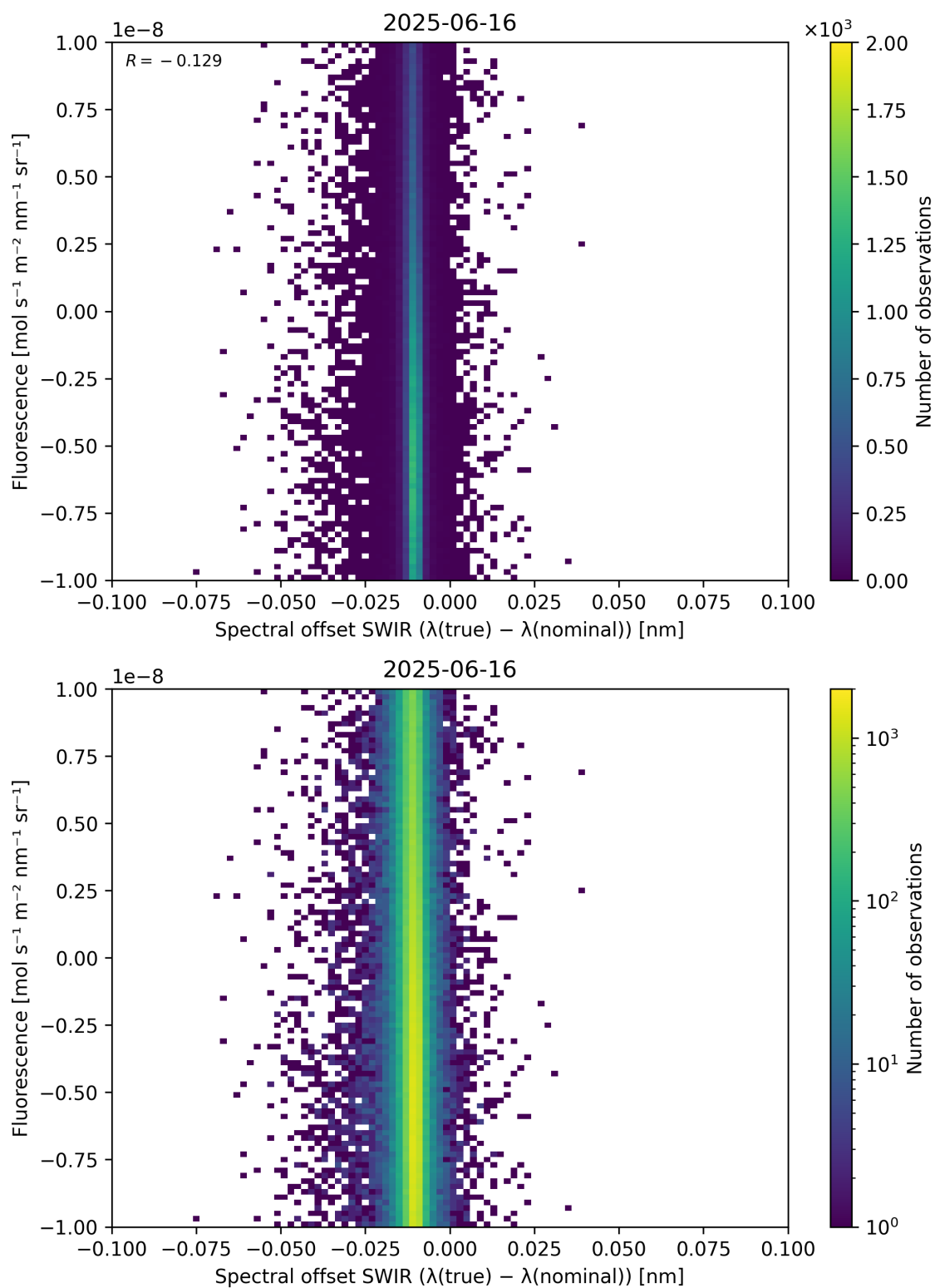
Figure 120: Scatter density plot of “Spectral offset SWIR ( \lambda_{\text{true}} - \lambda_{\text{nominal}} )” against “Fluorescence” for 2025-06-16 to 2025-06-17.
