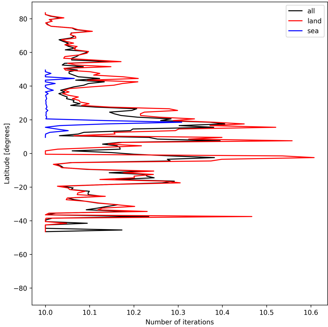
Figure 20: Zonal average of “Number of iterations” for 2025-06-16 to 2025-06-17.
