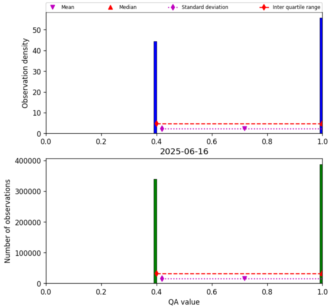
Figure 22: Histogram of “QA value” for 2025-06-16 to 2025-06-17
