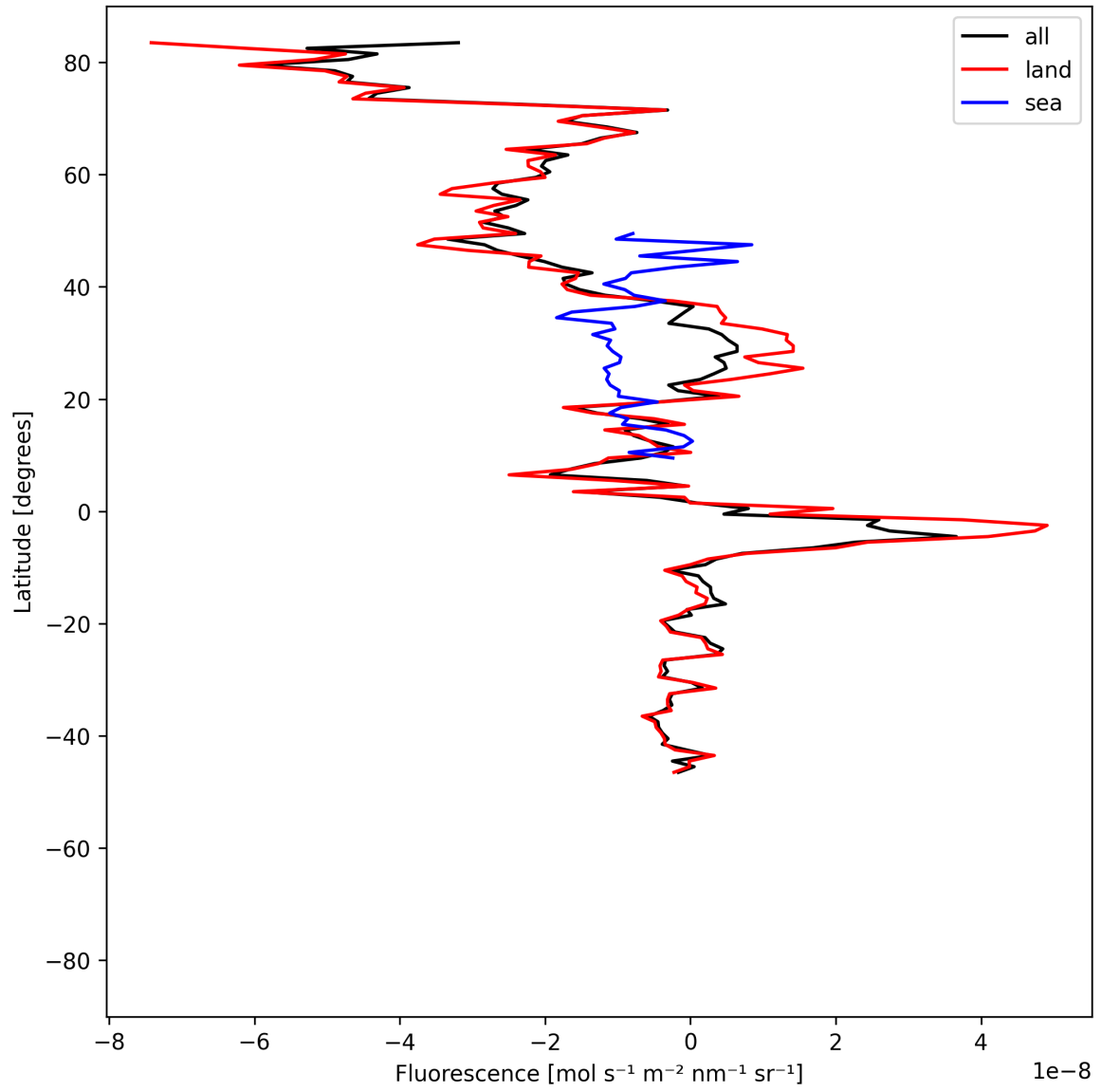
Figure 21: Zonal average of “Fluorescence” for 2025-06-16 to 2025-06-17.
