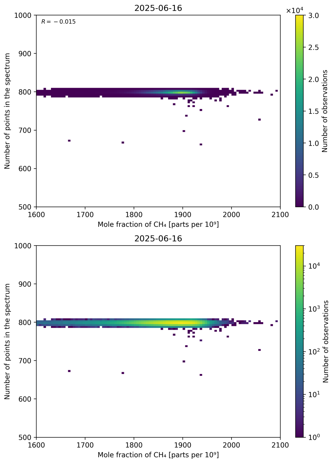
Figure 77: Scatter density plot of “Mole fraction of CH 4 ” against “Number of points in the spectrum” for 2025-06-16 to 2025-06-17.
