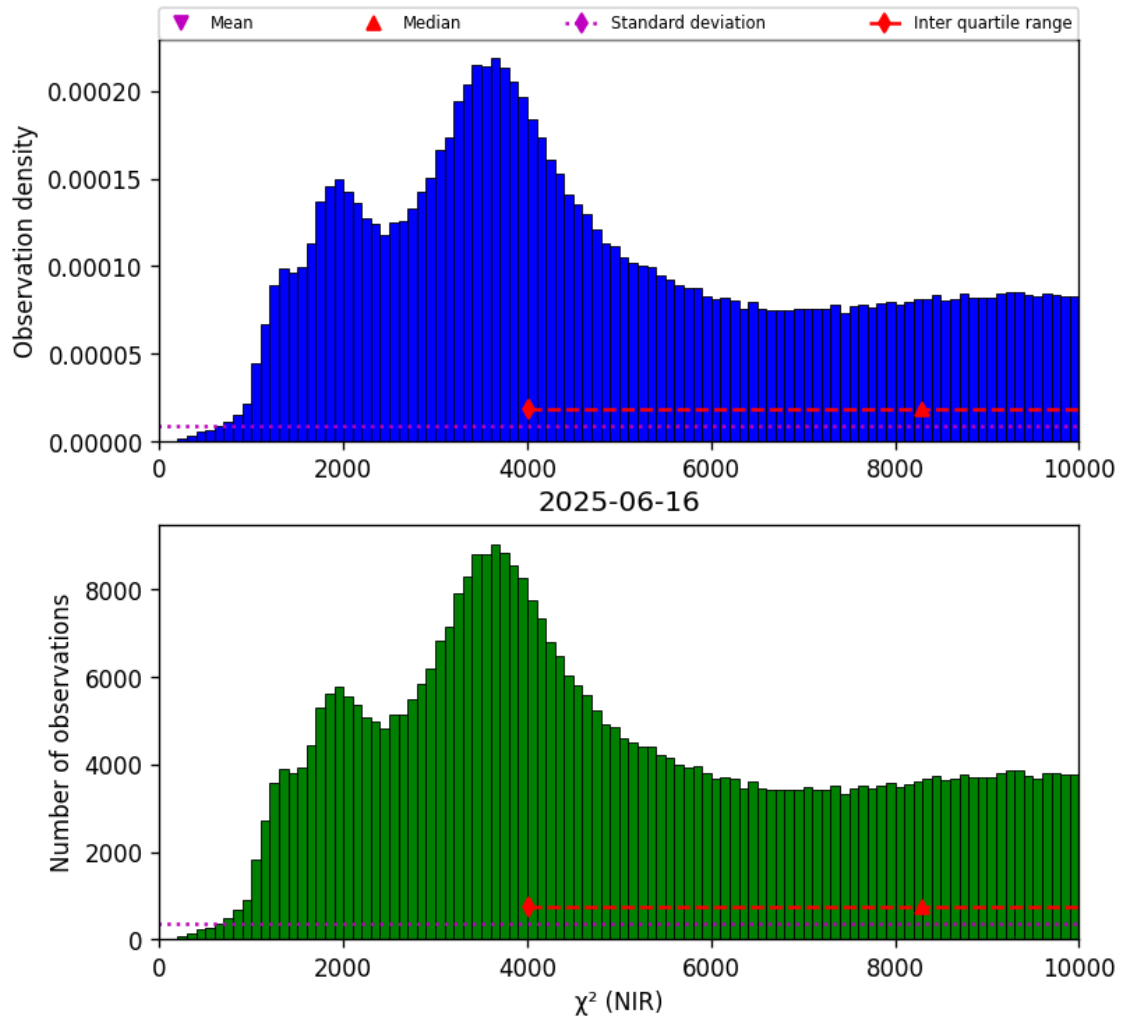
Figure 29: Histogram of “ \chi^2 (NIR)” for 2025-06-16 to 2025-06-17
