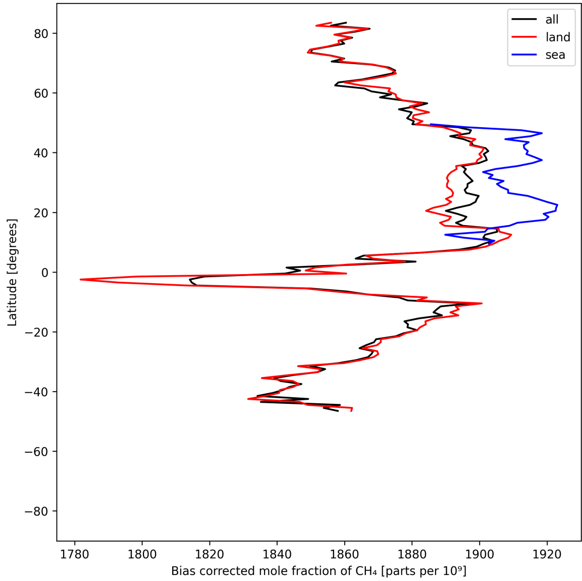
Figure 14: Zonal average of “Bias corrected mole fraction of \text{CH}_4 ” for 2025-06-16 to 2025-06-17.
