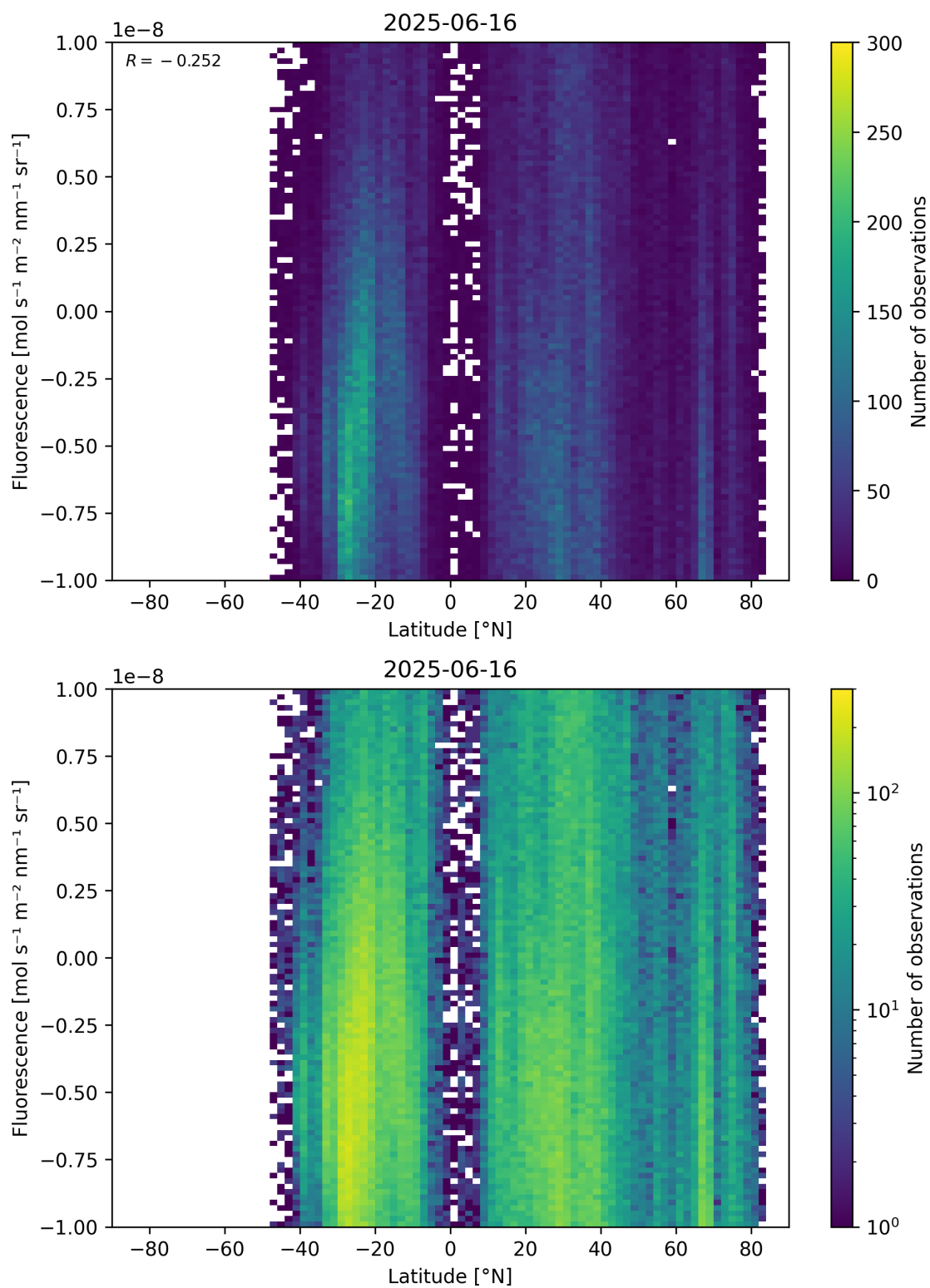
Figure 56: Scatter density plot of “Latitude” against “Fluorescence” for 2025-06-16 to 2025-06-17.
