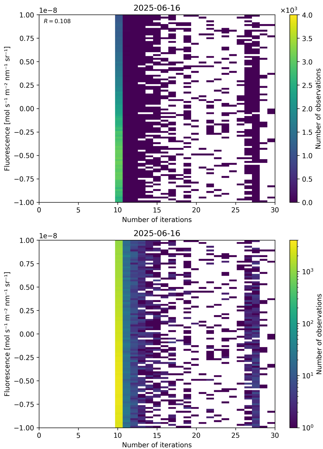
Figure 87: Scatter density plot of “Number of iterations” against “Fluorescence” for 2025-06-16 to 2025-06-17.
