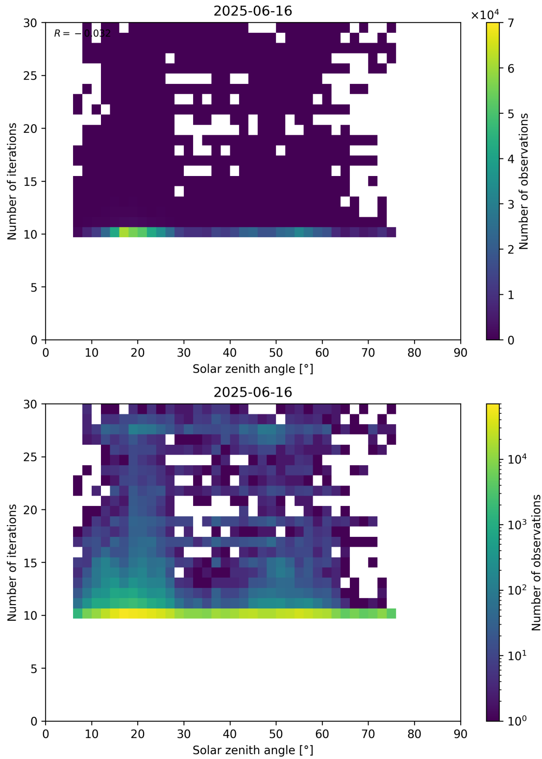
Figure 102: Scatter density plot of “Solar zenith angle” against “Number of iterations” for 2025-06-16 to 2025-06-17.
