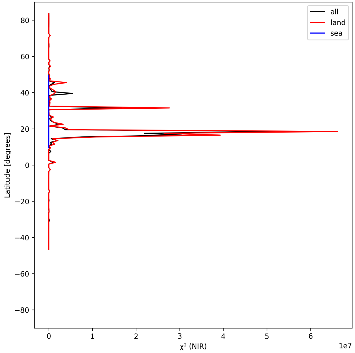
Figure 18: Zonal average of “ \chi^2 (NIR)” for 2025-06-16 to 2025-06-17.
