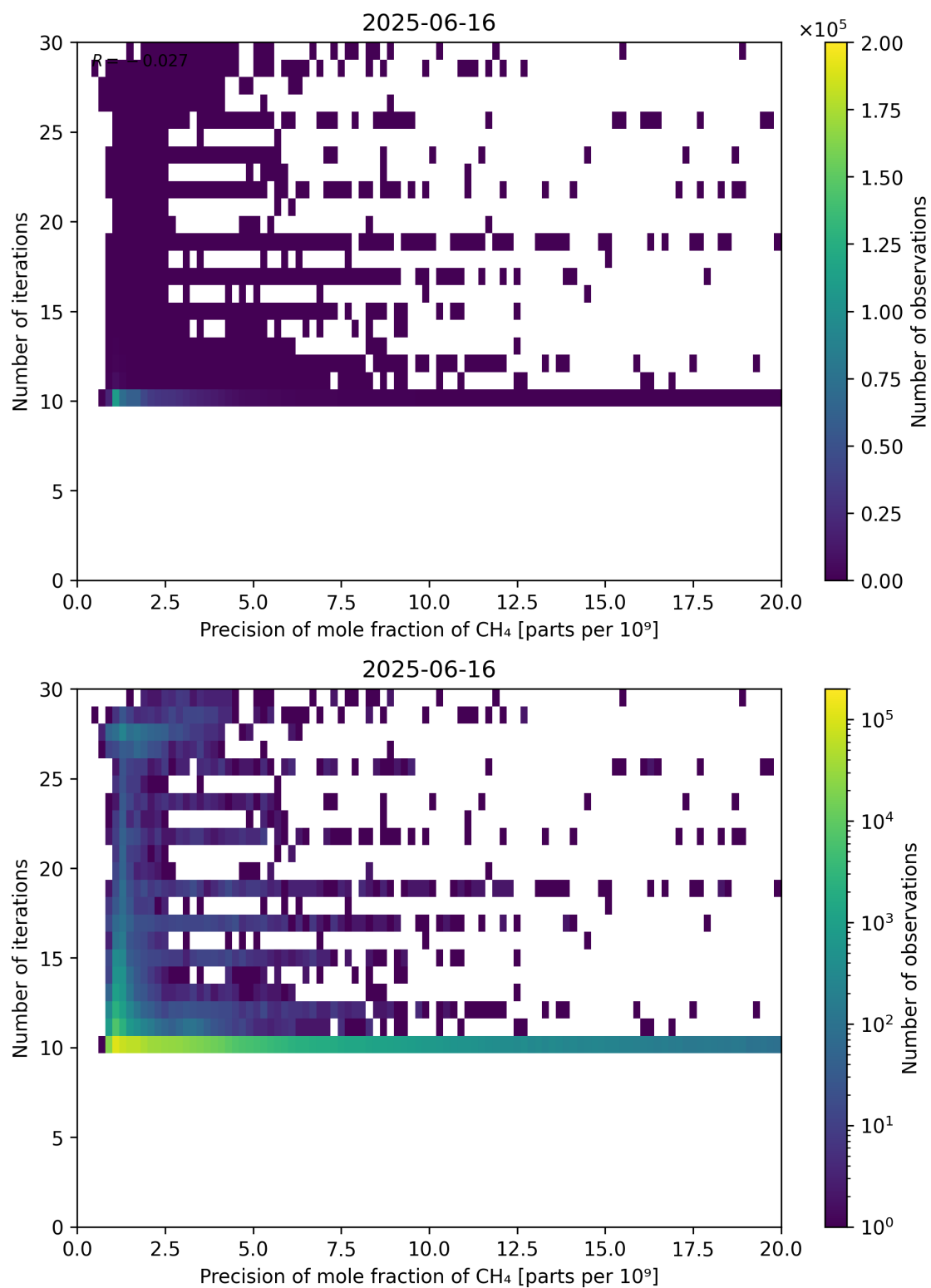
Figure 83: Scatter density plot of “Precision of mole fraction of CH 4 ” against “Number of iterations” for 2025-06-16 to 2025-06-17.
