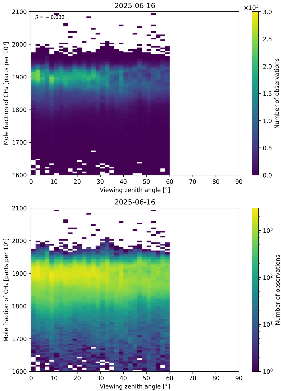
Figure 110: Scatter density plot of “Viewing zenith angle” against “Mole fraction of CH 4 ” for 2025-06-16 to 2025-06-17.
