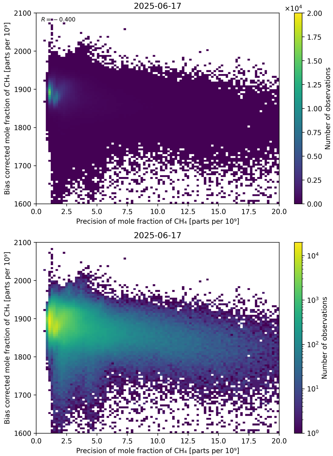
Figure 82: Scatter density plot of “Precision of mole fraction of CH 4 ” against “Bias corrected mole fraction of CH 4 ” for 2025-06-17 to 2025-06-18.
