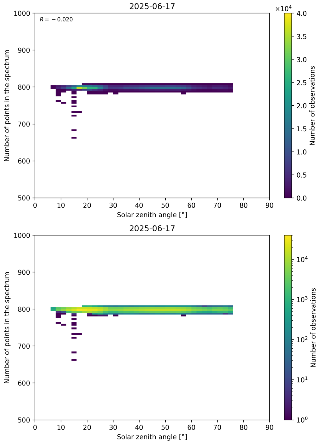
Figure 103: Scatter density plot of “Solar zenith angle” against “Number of points in the spectrum” for 2025-06-17 to 2025-06-18.
