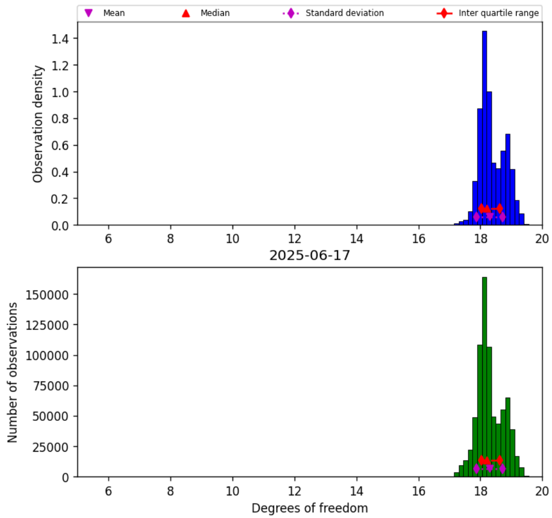
Figure 30: Histogram of “Degrees of freedom” for 2025-06-17 to 2025-06-18
