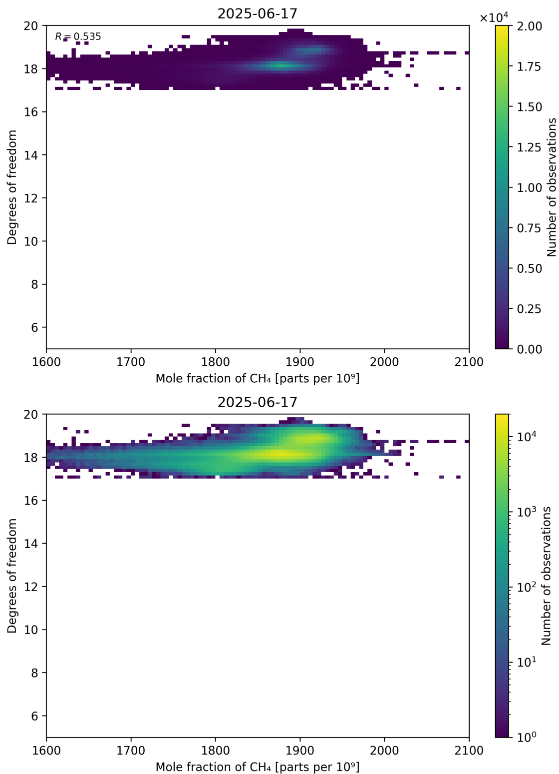
Figure 72: Scatter density plot of “Mole fraction of CH 4 ” against “Degrees of freedom” for 2025-06-17 to 2025-06-18.
