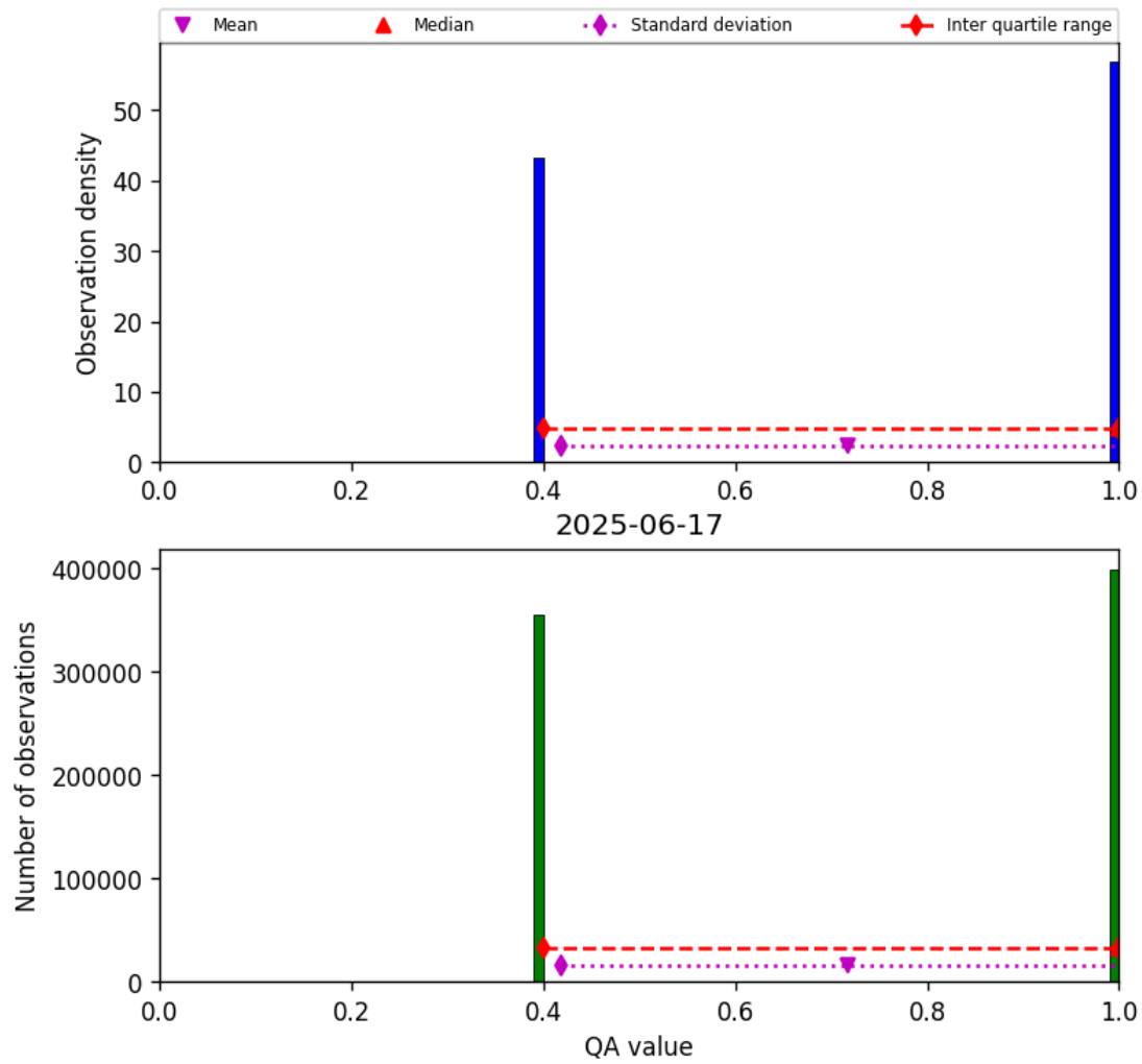
Figure 22: Histogram of "QA value" for 2025-06-17 to 2025-06-18
