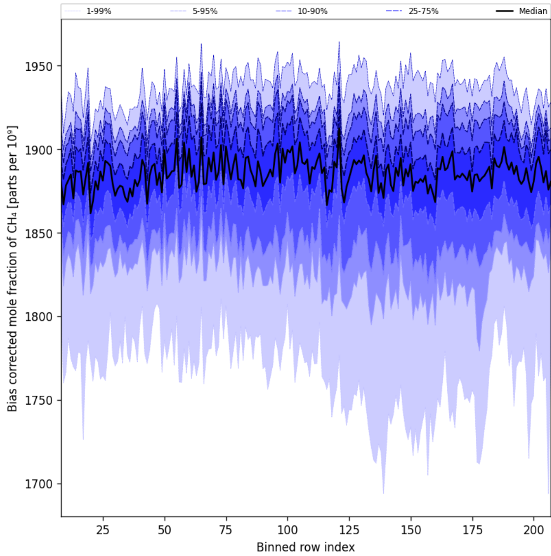
Figure 36: Along track statistics of “Bias corrected mole fraction of CH 4 ” for 2025-06-17 to 2025-06-18
