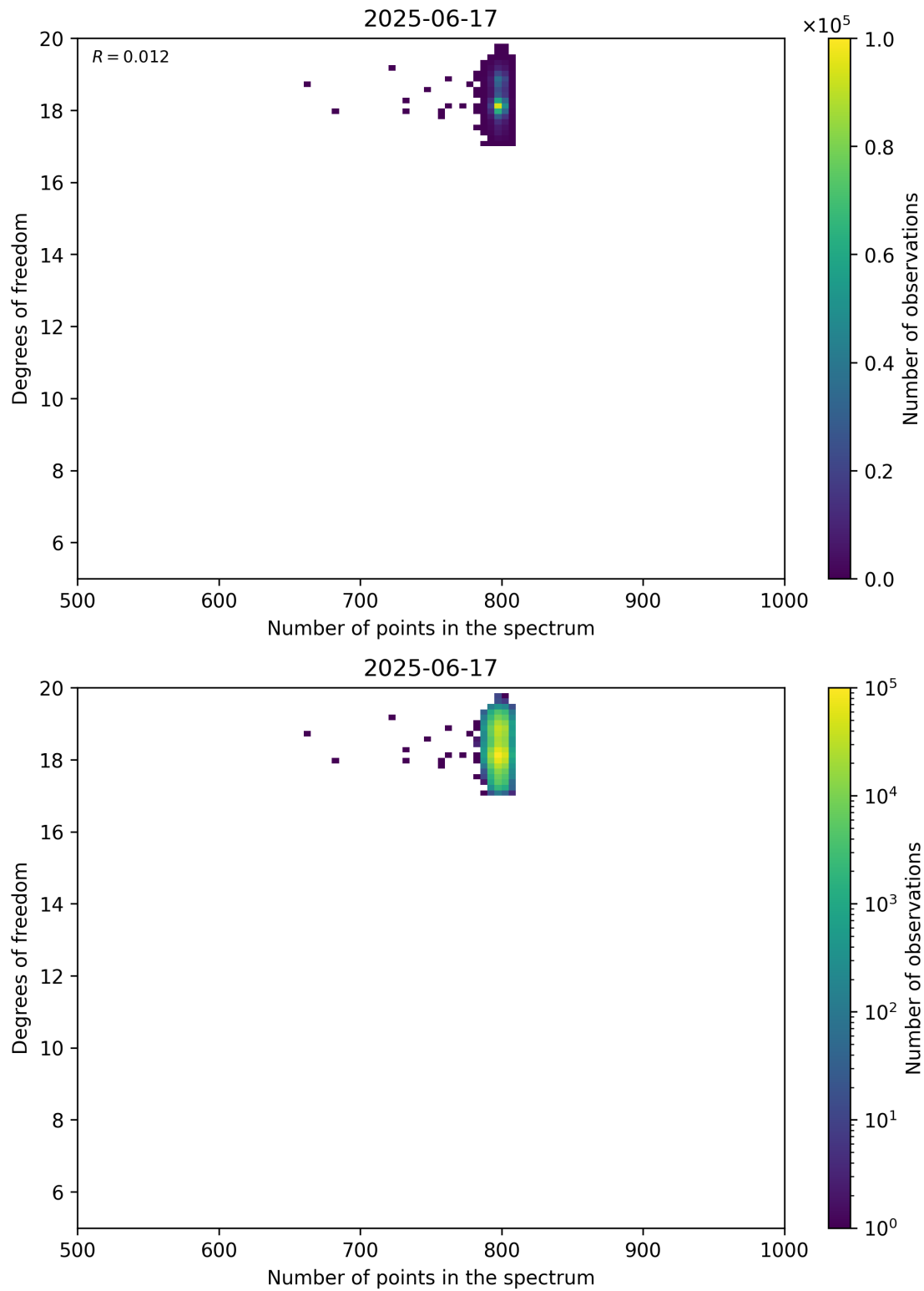
Figure 90: Scatter density plot of “Number of points in the spectrum” against “Degrees of freedom” for 2025-06-17 to 2025-06-18.
