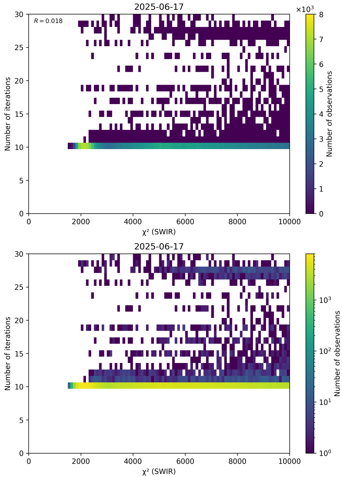
Figure 50: Scatter density plot of “ \chi^2 (SWIR)” against “Number of iterations” for 2025-06-17 to 2025-06-18.
