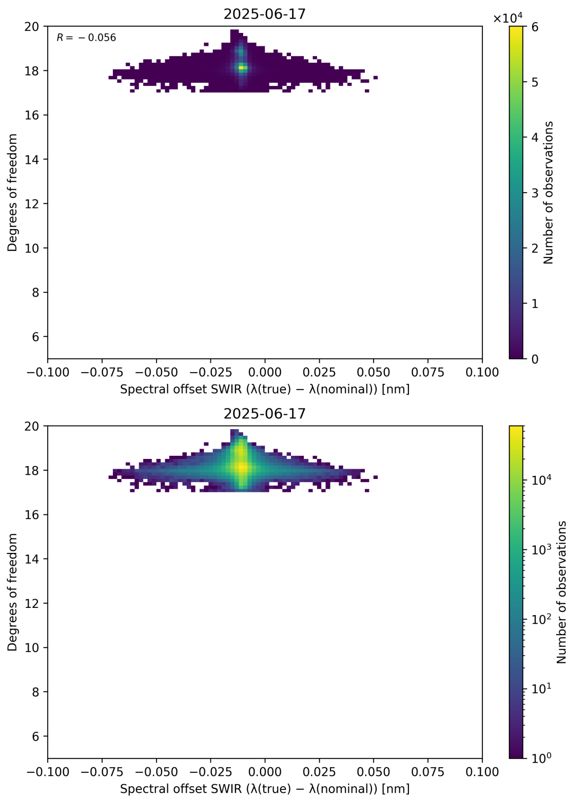
Figure 119: Scatter density plot of “Spectral offset SWIR ( \lambda_{\text{true}} - \lambda_{\text{nominal}} )” against “Degrees of freedom” for 2025-06-17 to 2025-06-18.
