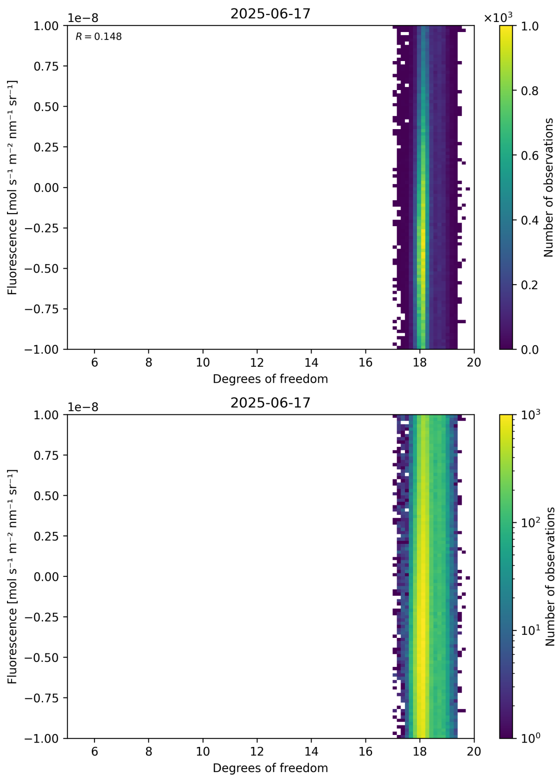
Figure 51: Scatter density plot of “Degrees of freedom” against “Fluorescence” for 2025-06-17 to 2025-06-18.
