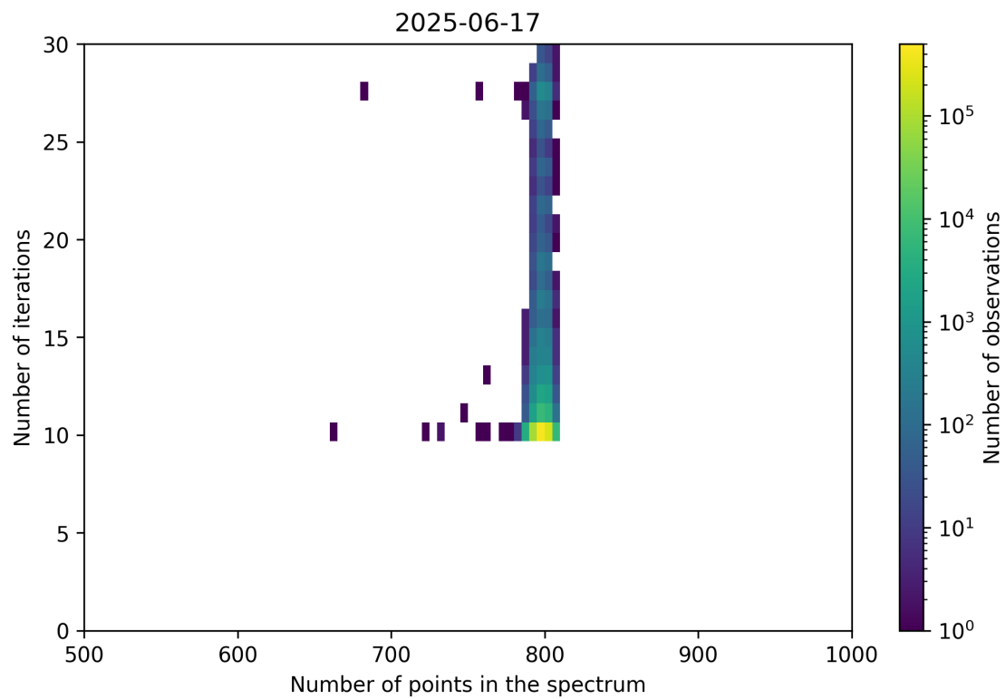
Figure 92: Scatter density plot of “Number of points in the spectrum” against “Number of iterations” for 2025-06-17 to 2025-06-18.
