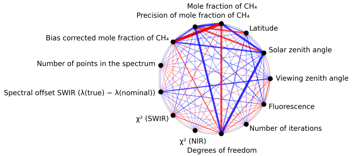
Figure 1: Map of correlation graph for 2025-06-17 to 2025-06-18.
