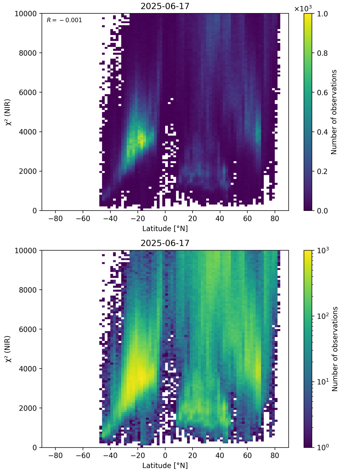
Figure 53: Scatter density plot of “Latitude” against “ \chi^2 (NIR)” for 2025-06-17 to 2025-06-18.
