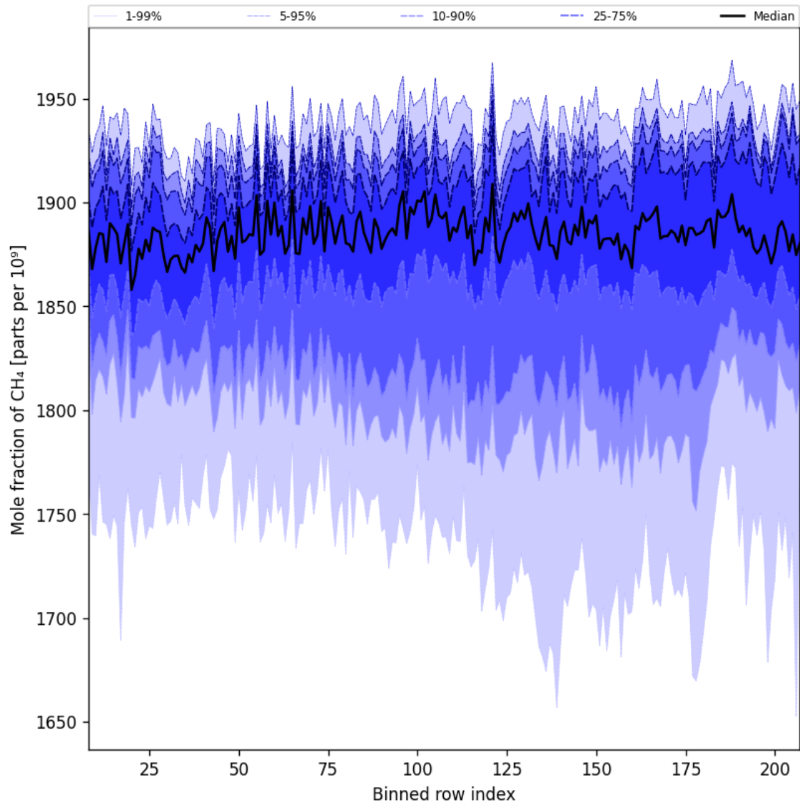
Figure 34: Along track statistics of “Mole fraction of CH 4 ” for 2025-06-17 to 2025-06-18
