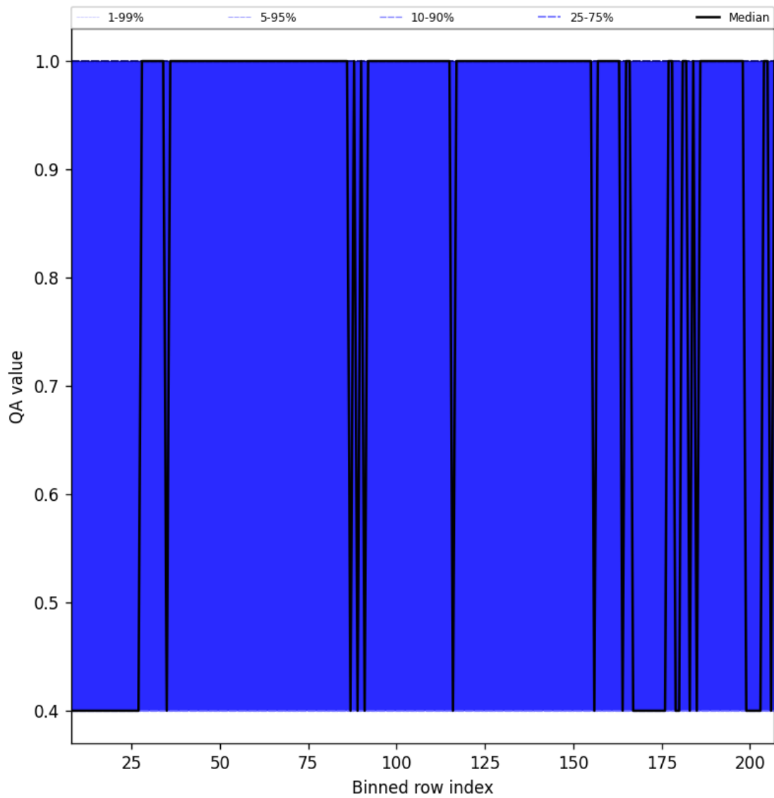
Figure 33: Along track statistics of “QA value” for 2025-06-17 to 2025-06-18
