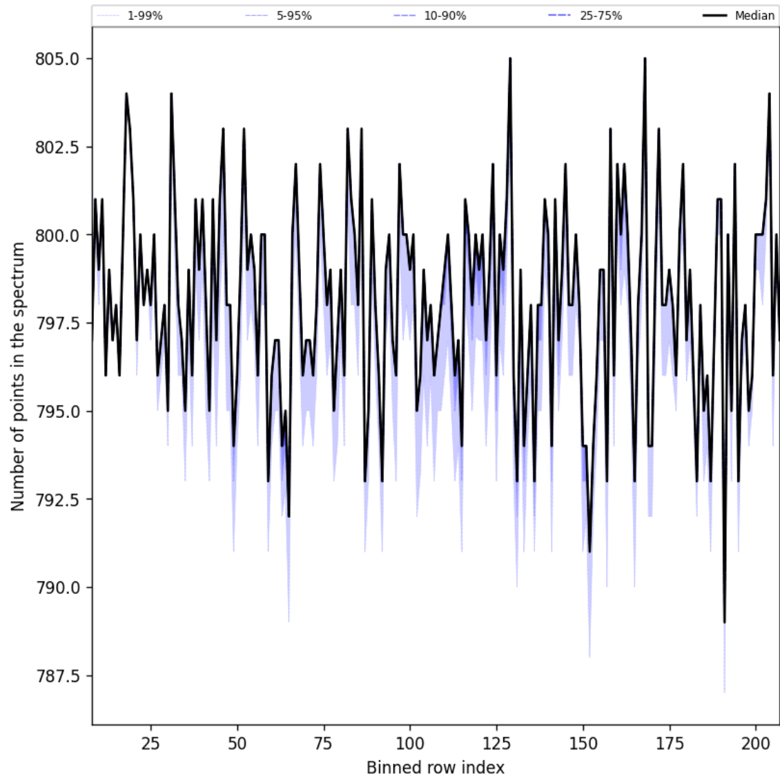
Figure 37: Along track statistics of “Number of points in the spectrum” for 2025-06-17 to 2025-06-18
