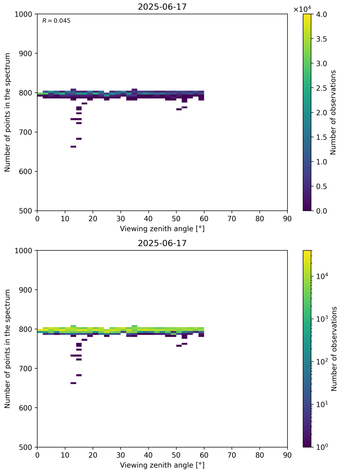
Figure 114: Scatter density plot of “Viewing zenith angle” against “Number of points in the spectrum” for 2025-06-17 to 2025-06-18.
