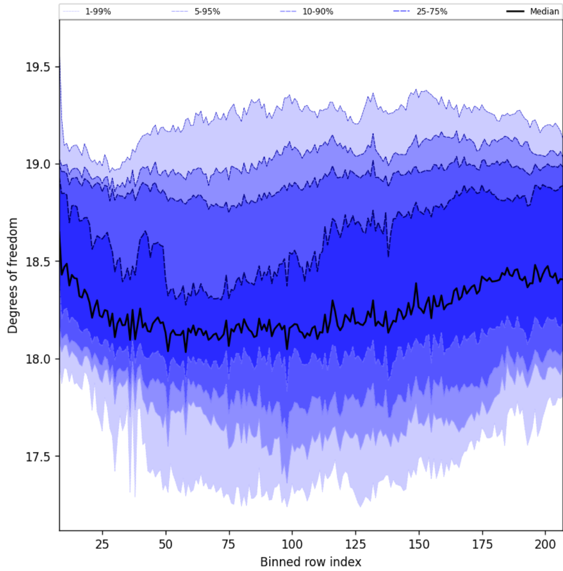
Figure 41: Along track statistics of “Degrees of freedom” for 2025-06-17 to 2025-06-18
