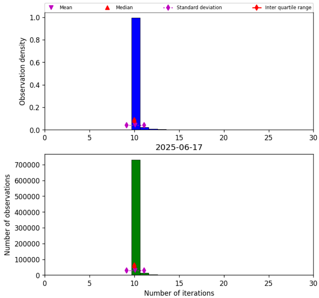
Figure 31: Histogram of "Number of iterations" for 2025-06-17 to 2025-06-18
