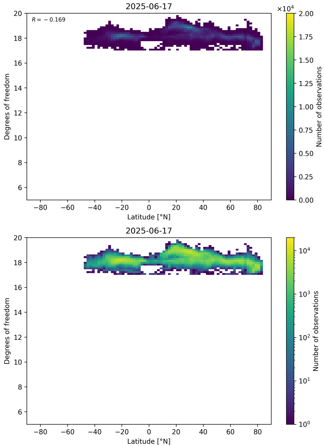
Figure 55: Scatter density plot of “Latitude” against “Degrees of freedom” for 2025-06-17 to 2025-06-18.
