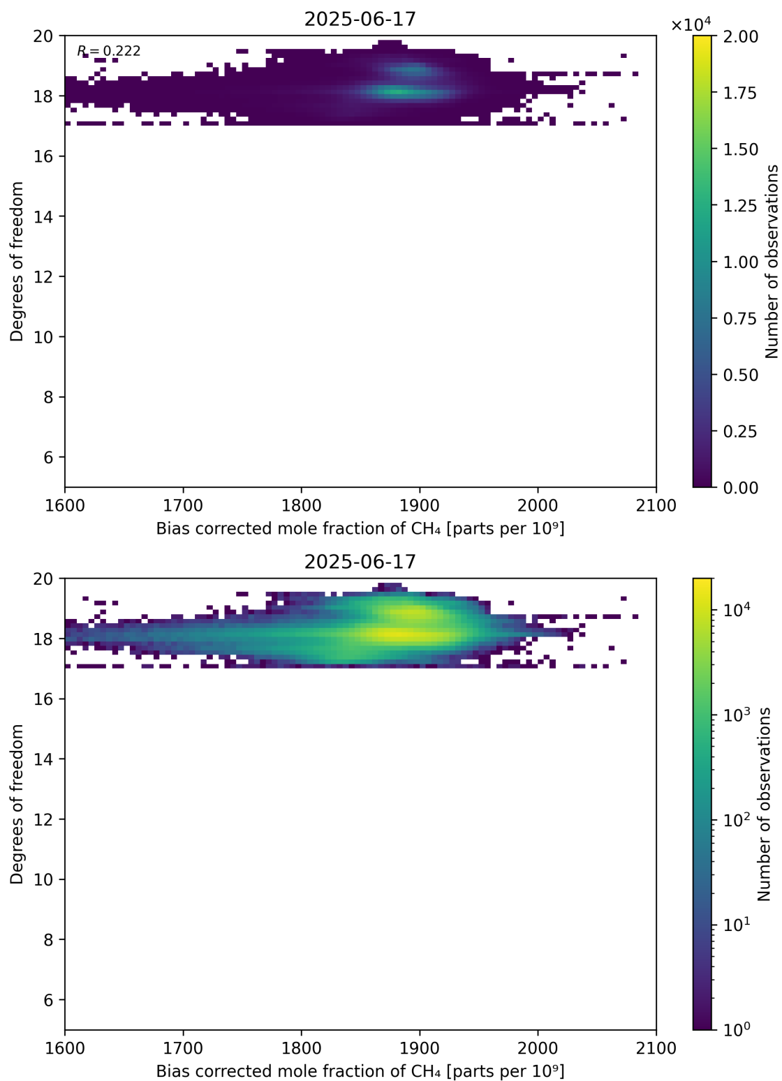
Figure 65: Scatter density plot of “Bias corrected mole fraction of CH 4 ” against “Degrees of freedom” for 2025-06-17 to 2025-06-18.
