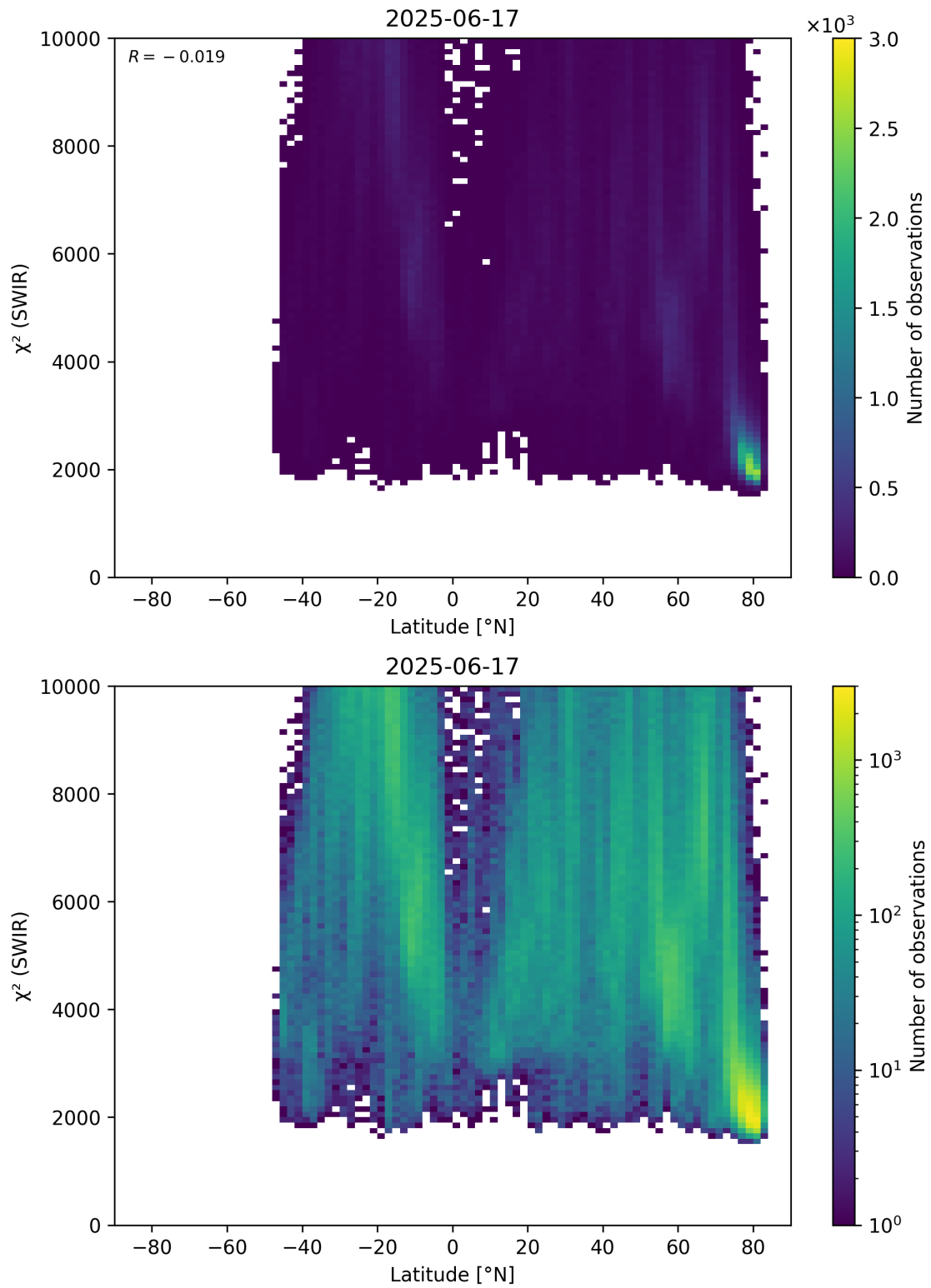
Figure 54: Scatter density plot of “Latitude” against “ \chi^2 (SWIR)” for 2025-06-17 to 2025-06-18.
