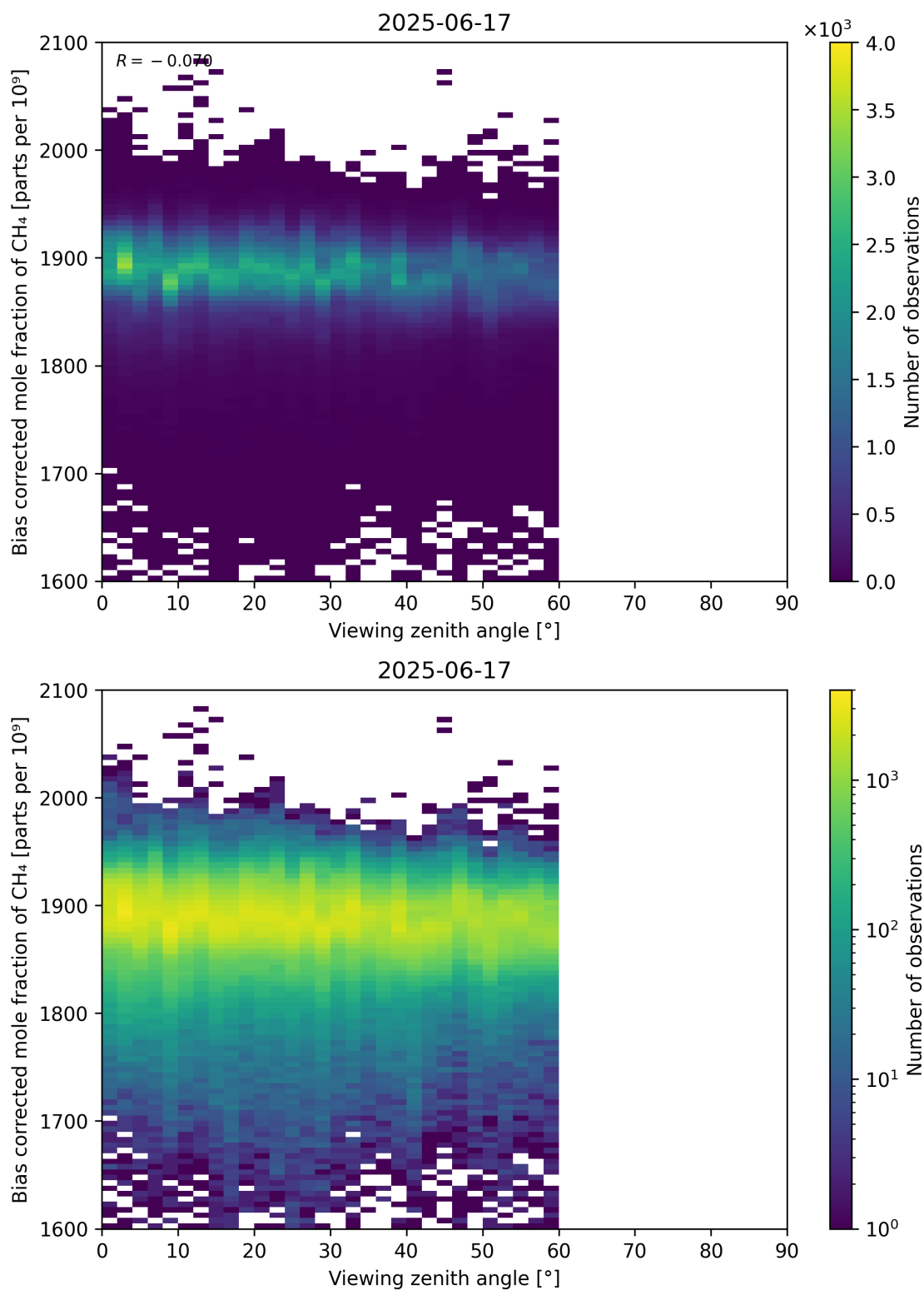
Figure 111: Scatter density plot of “Viewing zenith angle” against “Bias corrected mole fraction of CH 4 ” for 2025-06-17 to 2025-06-18.
