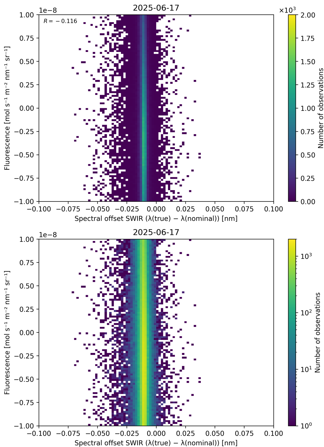
Figure 120: Scatter density plot of “Spectral offset SWIR ( \lambda_{\text{true}} - \lambda_{\text{nominal}} )” against “Fluorescence” for 2025-06-17 to 2025-06-18.
