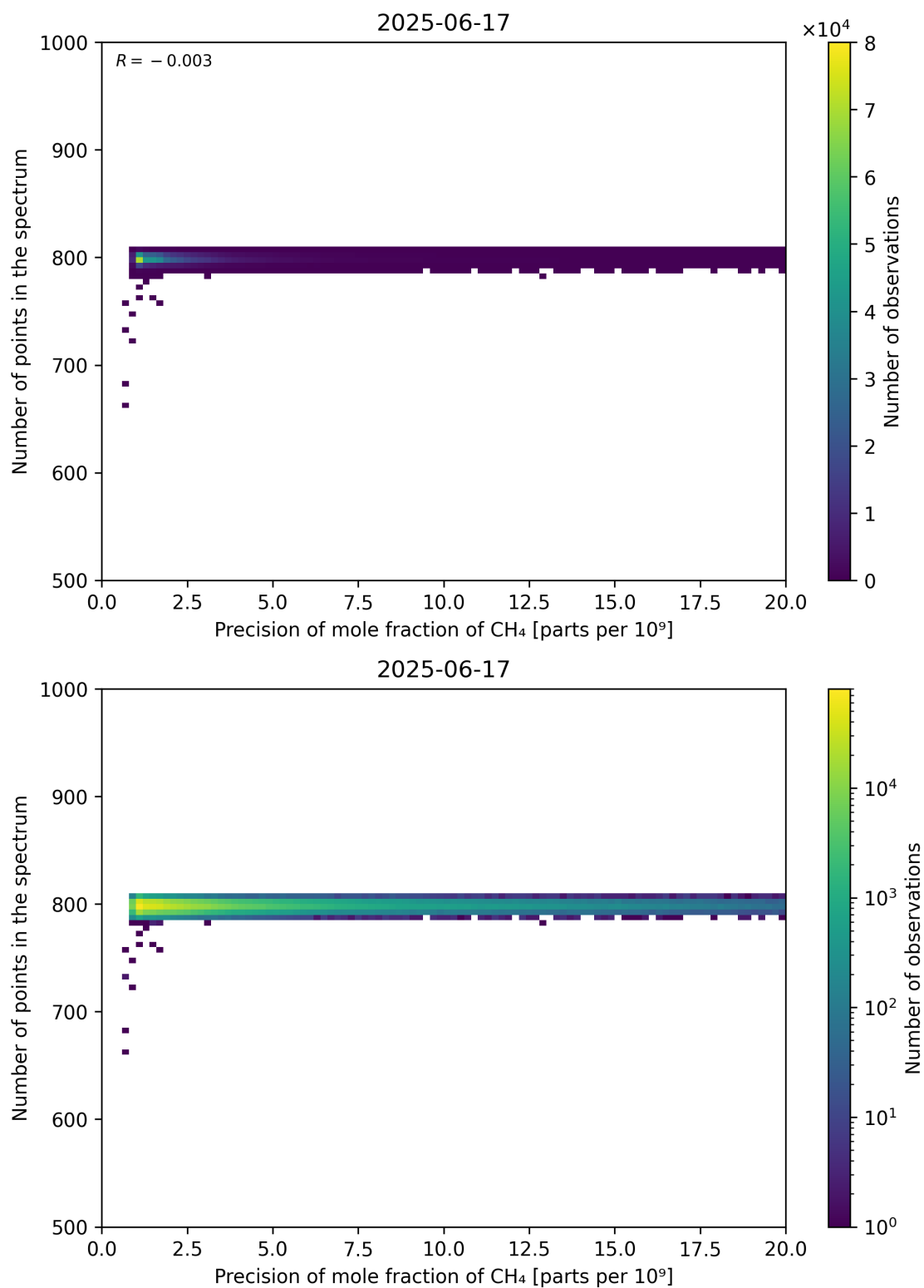
Figure 84: Scatter density plot of “Precision of mole fraction of CH 4 ” against “Number of points in the spectrum” for 2025-06-17 to 2025-06-18.
