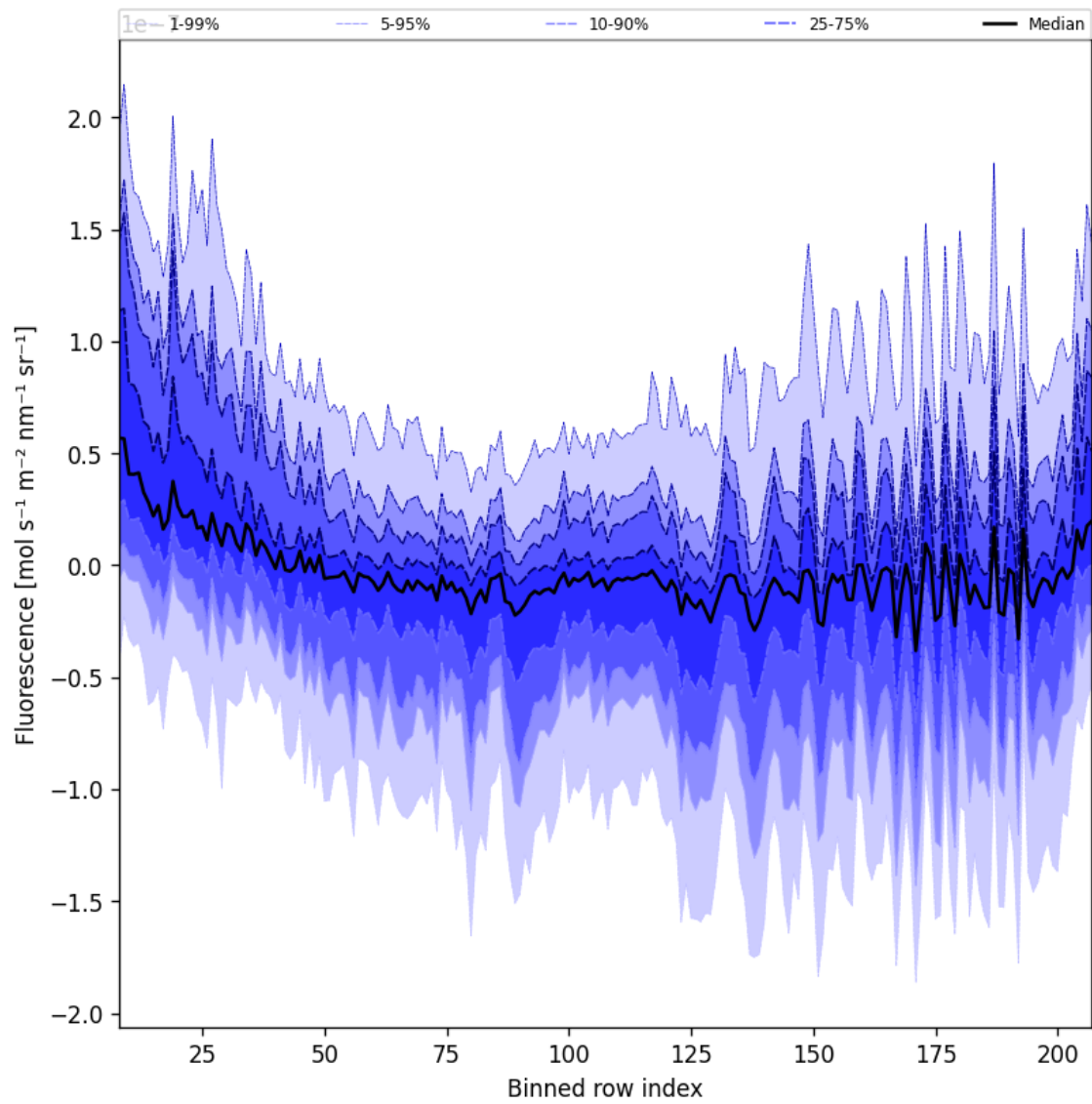
Figure 43: Along track statistics of “Fluorescence” for 2025-06-17 to 2025-06-18
