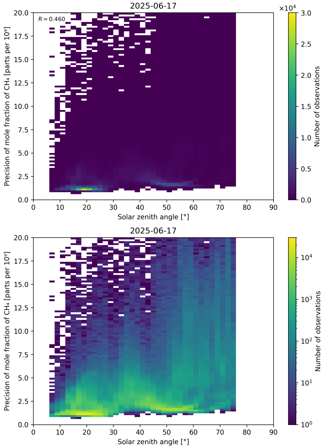
Figure 101: Scatter density plot of “Solar zenith angle” against “Precision of mole fraction of \text{CH}_4 ” for 2025-06-17 to 2025-06-18.
