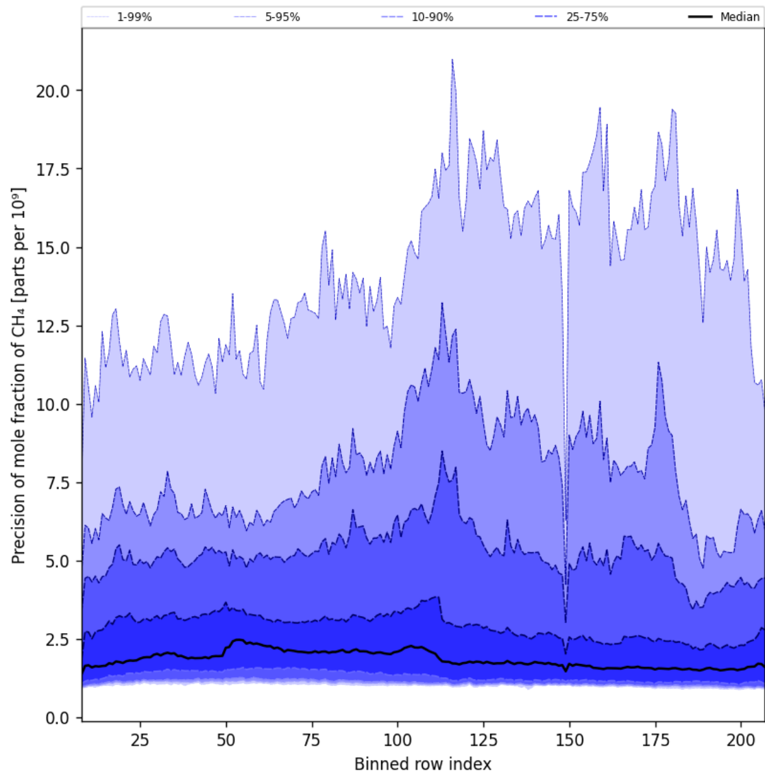
Figure 35: Along track statistics of “Precision of mole fraction of CH 4 ” for 2025-06-17 to 2025-06-18
