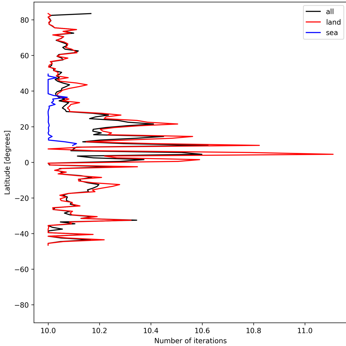
Figure 20: Zonal average of “Number of iterations” for 2025-06-17 to 2025-06-18.
