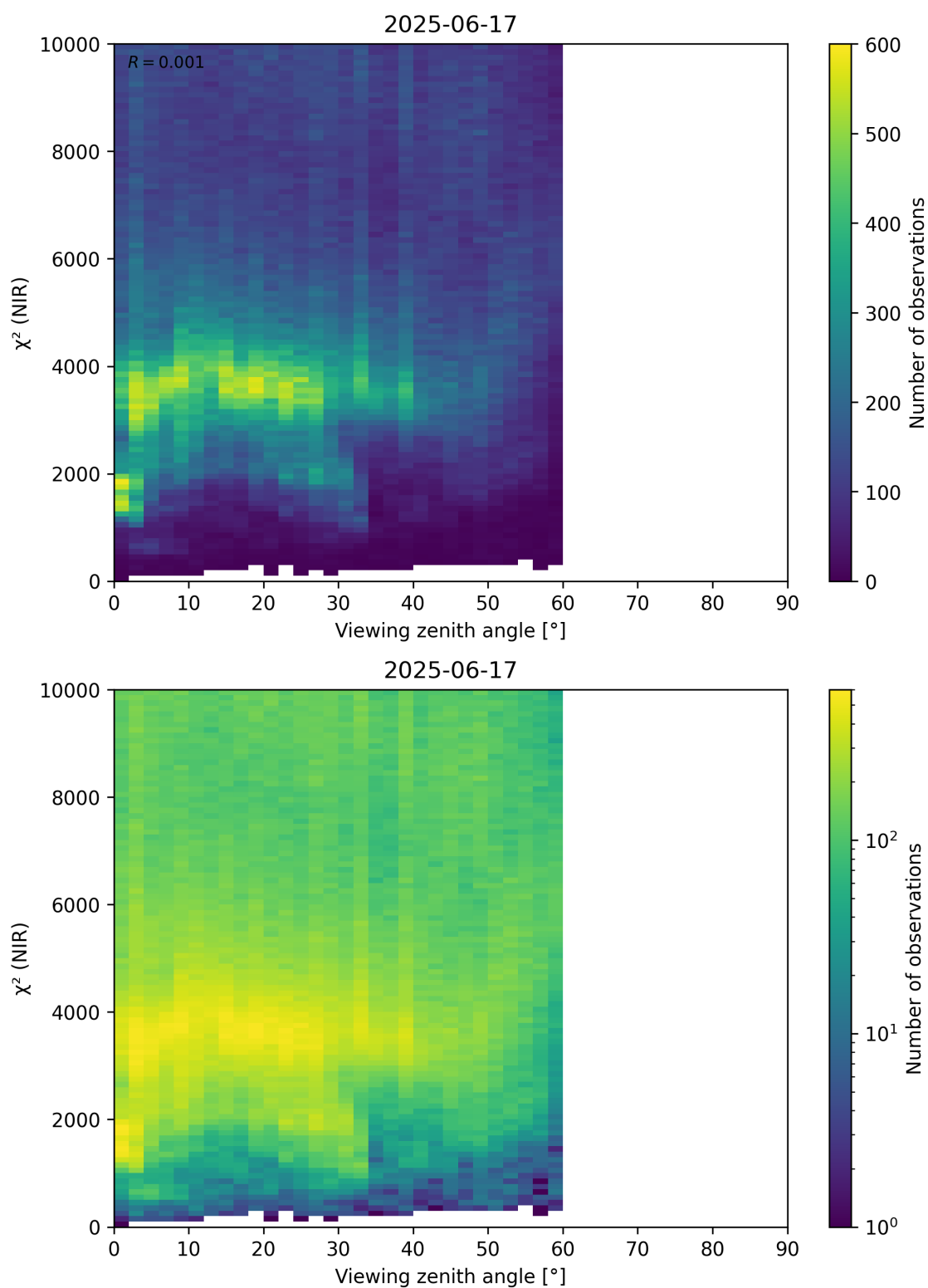
Figure 105: Scatter density plot of “Viewing zenith angle” against “ \chi^2 (NIR)” for 2025-06-17 to 2025-06-18.
