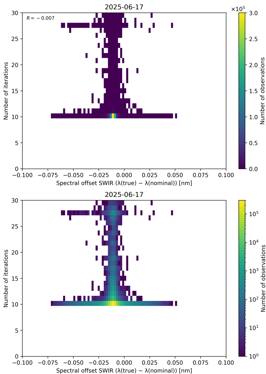
Figure 121: Scatter density plot of “Spectral offset SWIR ( \lambda_{\text{true}} - \lambda_{\text{nominal}} )” against “Number of iterations” for 2025-06-17 to 2025-06-18.
