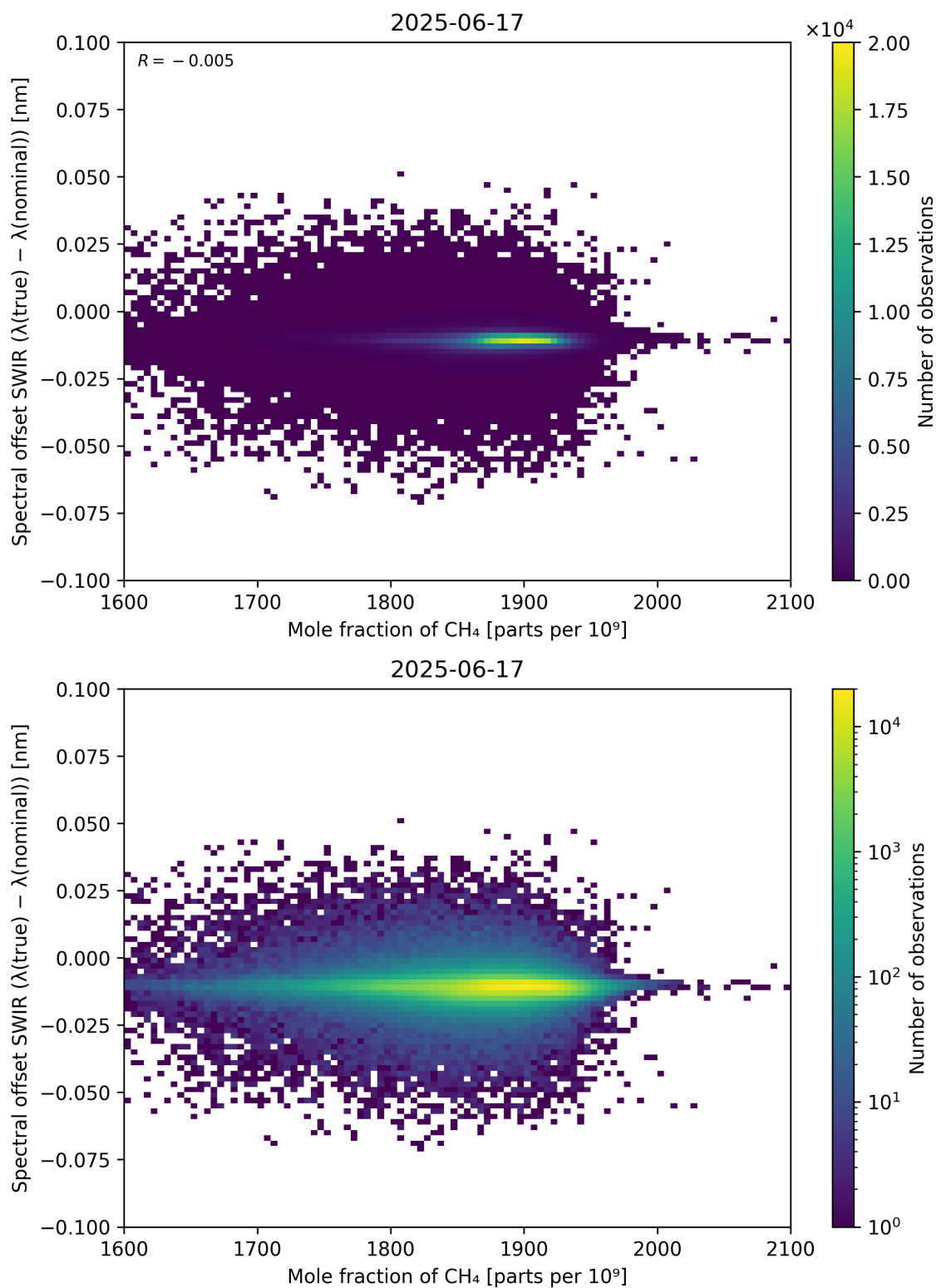
Figure 86: Scatter density plot of “Mole fraction of \text{CH}_4 ” against “Spectral offset SWIR ( \lambda_{\text{true}} - \lambda_{\text{nominal}} )” for 2025-06-17 to 2025-06-18.
