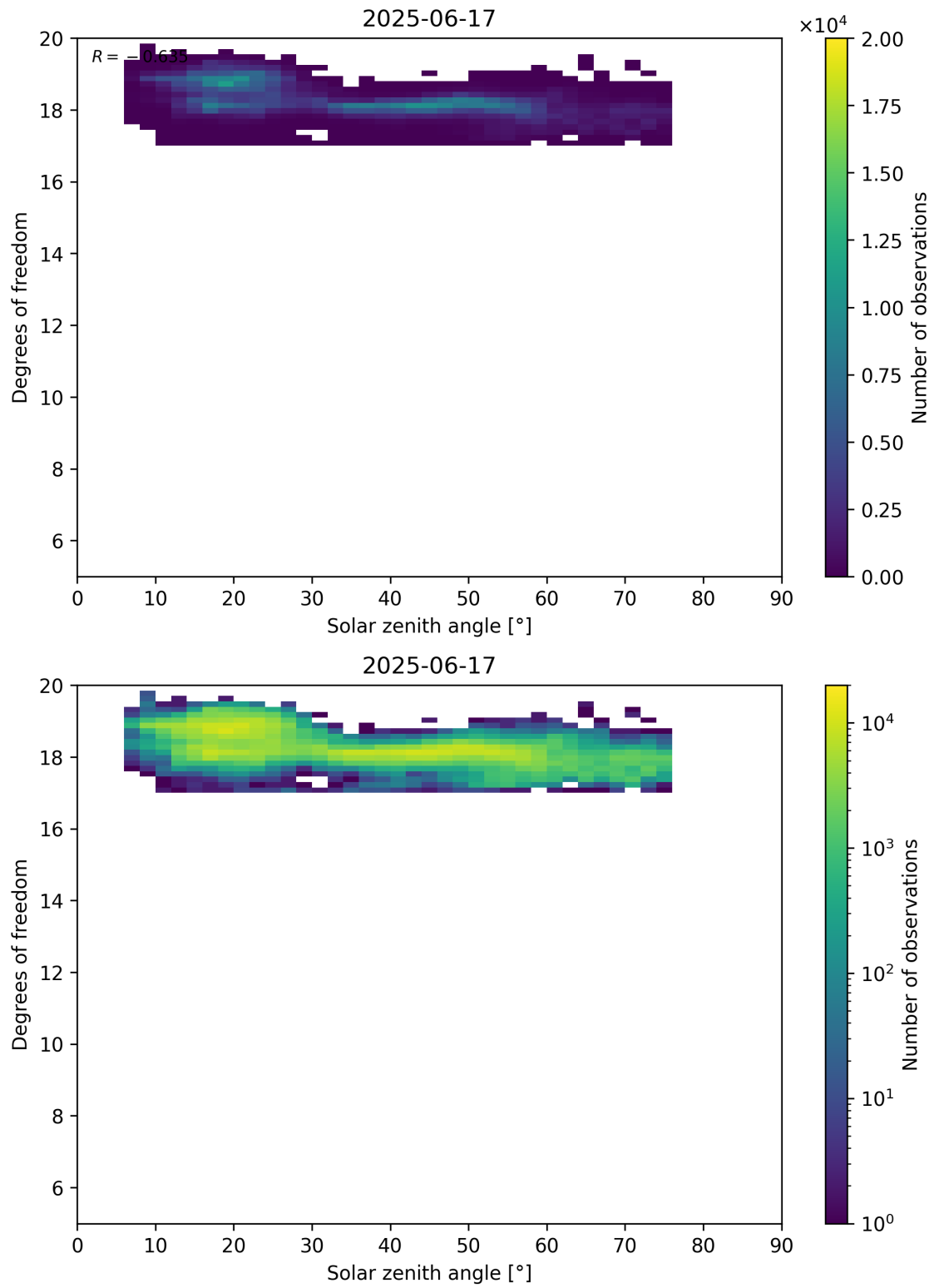
Figure 96: Scatter density plot of “Solar zenith angle” against “Degrees of freedom” for 2025-06-17 to 2025-06-18.
