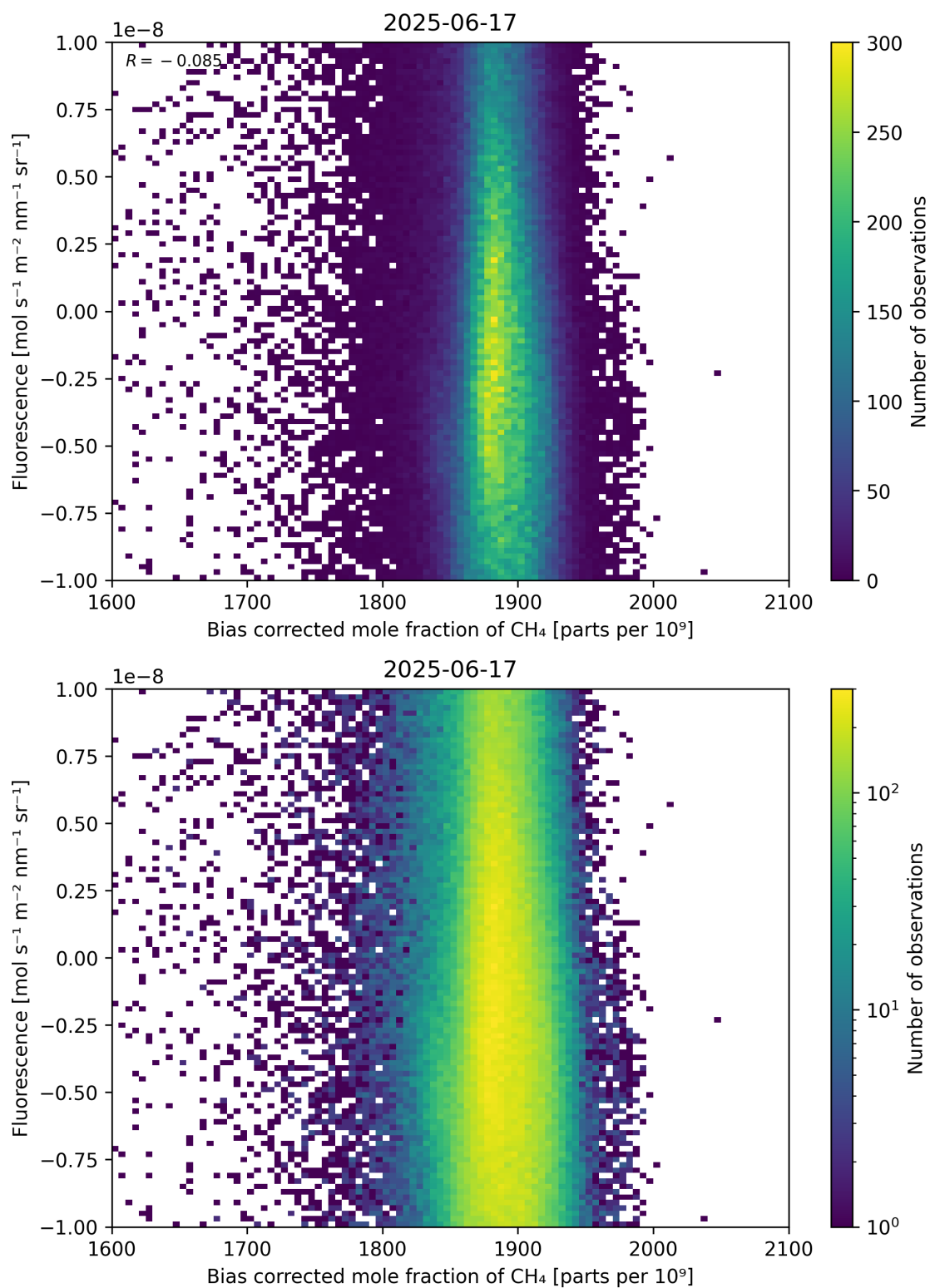
Figure 66: Scatter density plot of “Bias corrected mole fraction of \text{CH}_4 ” against “Fluorescence” for 2025-06-17 to 2025-06-18.
