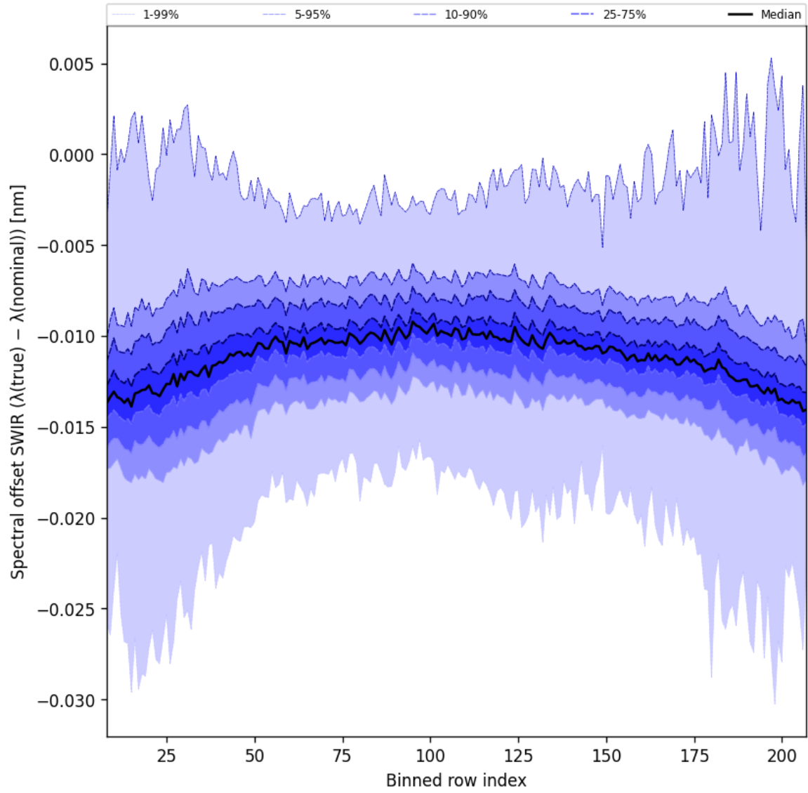
Figure 38: Along track statistics of “Spectral offset SWIR ( \lambda_{\text{true}} - \lambda_{\text{nominal}} )” for 2025-06-17 to 2025-06-18
