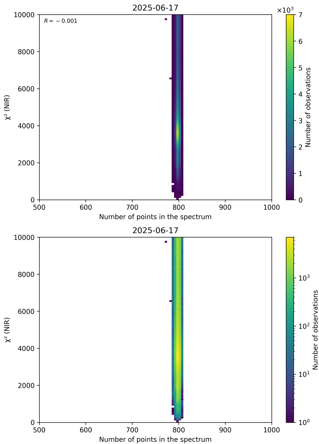
Figure 88: Scatter density plot of “Number of points in the spectrum” against “ \chi^2 (NIR)” for 2025-06-17 to 2025-06-18.
