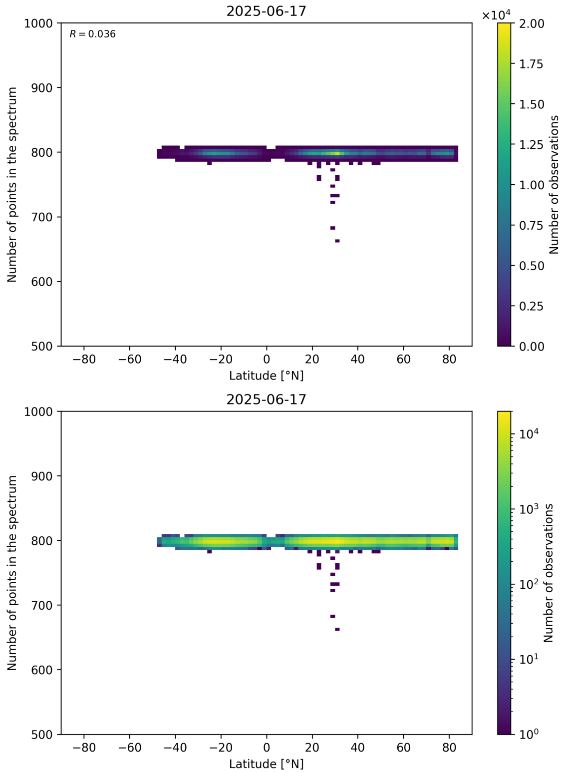
Figure 61: Scatter density plot of “Latitude” against “Number of points in the spectrum” for 2025-06-17 to 2025-06-18.
