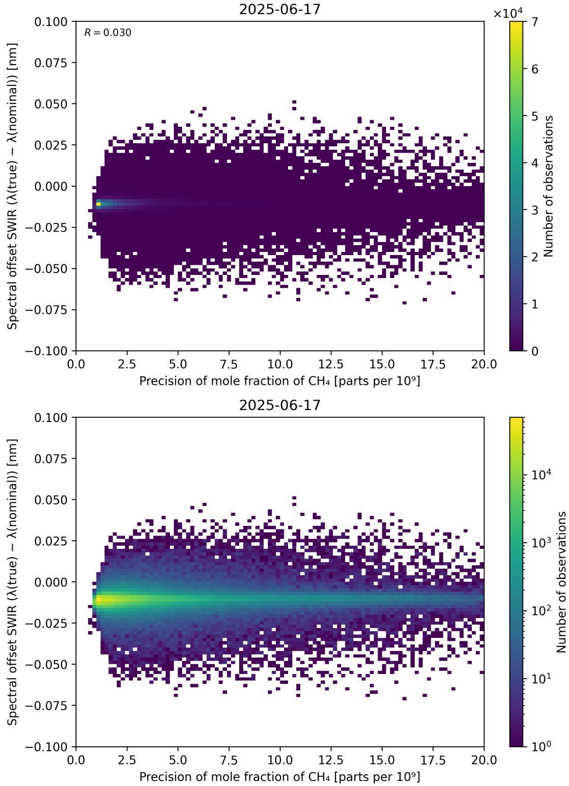
Figure 85: Scatter density plot of “Precision of mole fraction of CH 4 ” against “Spectral offset SWIR ( \lambda_{\text{true}} - \lambda_{\text{nominal}} )” for 2025-06-17 to 2025-06-18.
