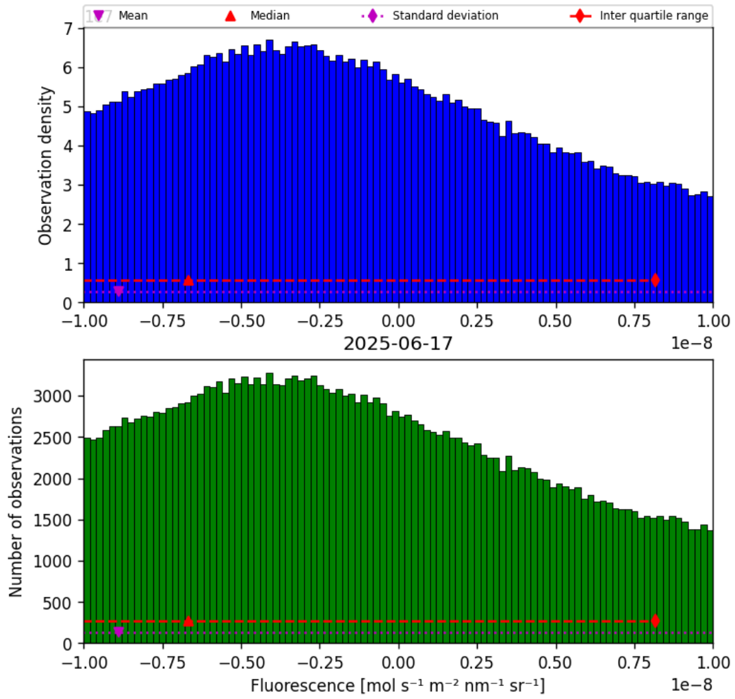
Figure 32: Histogram of “Fluorescence” for 2025-06-17 to 2025-06-18
