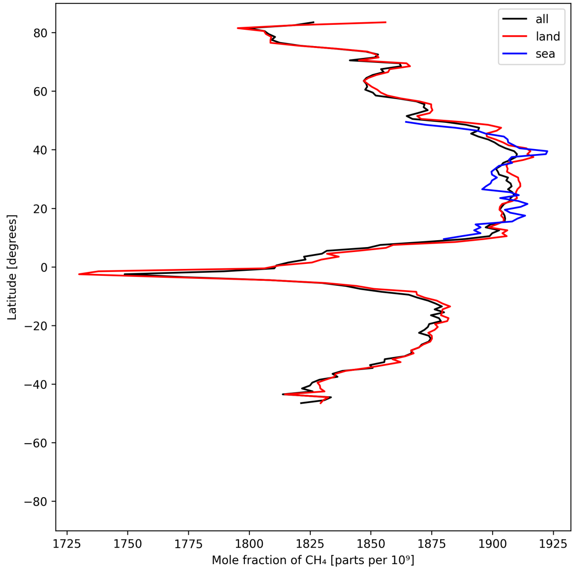
Figure 12: Zonal average of “Mole fraction of CH 4 ” for 2025-06-17 to 2025-06-18.
