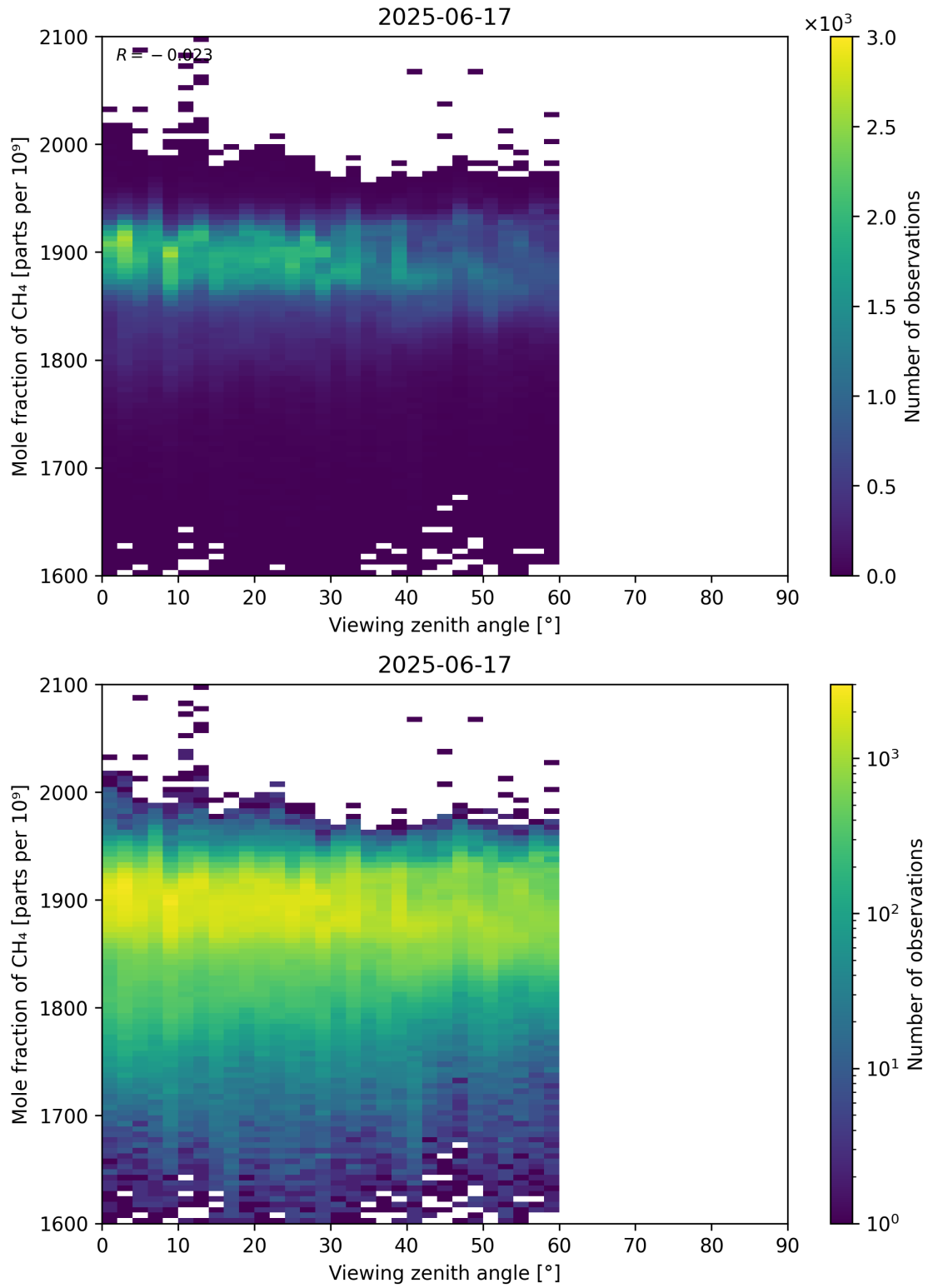
Figure 110: Scatter density plot of “Viewing zenith angle” against “Mole fraction of CH 4 ” for 2025-06-17 to 2025-06-18.
