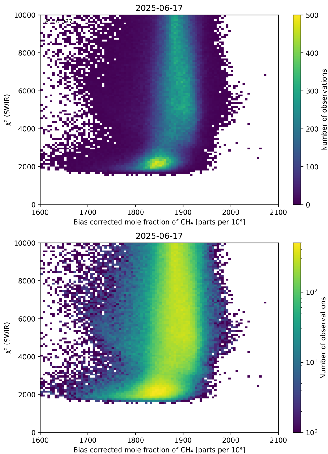
Figure 64: Scatter density plot of “Bias corrected mole fraction of \text{CH}_4 ” against “ \chi^2 (SWIR)” for 2025-06-17 to 2025-06-18.
