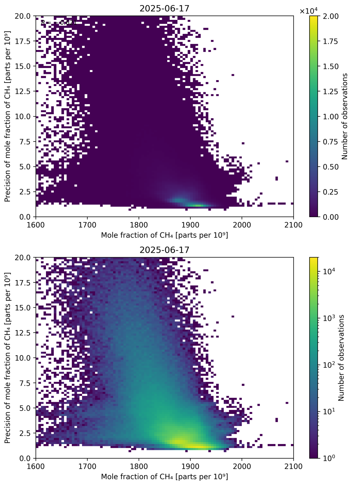
Figure 75: Scatter density plot of “Mole fraction of CH 4 ” against “Precision of mole fraction of CH 4 ” for 2025-06-17 to 2025-06-18.
