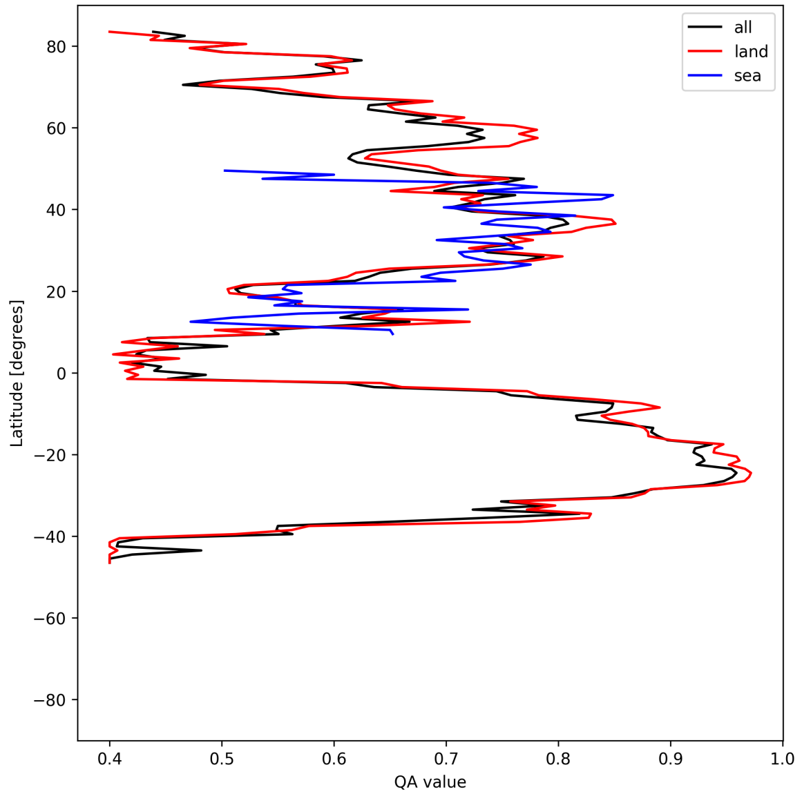
Figure 11: Zonal average of “QA value” for 2025-06-17 to 2025-06-18.
