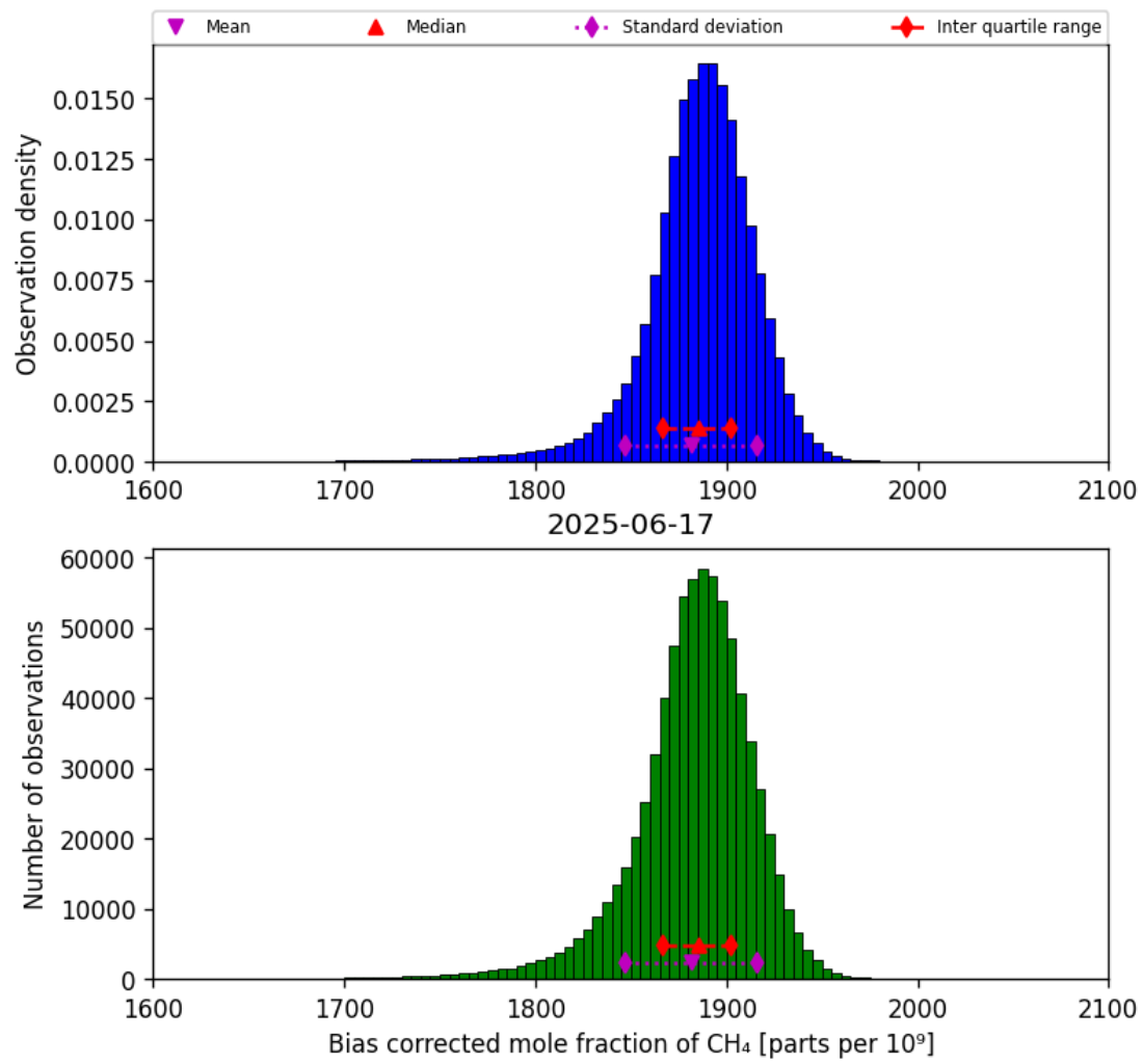
Figure 25: Histogram of “Bias corrected mole fraction of CH 4 ” for 2025-06-17 to 2025-06-18
