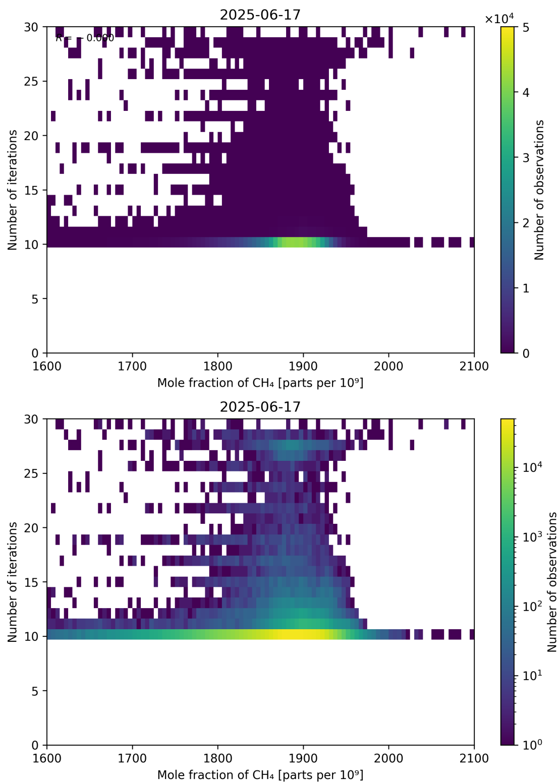
Figure 76: Scatter density plot of “Mole fraction of CH 4 ” against “Number of iterations” for 2025-06-17 to 2025-06-18.
