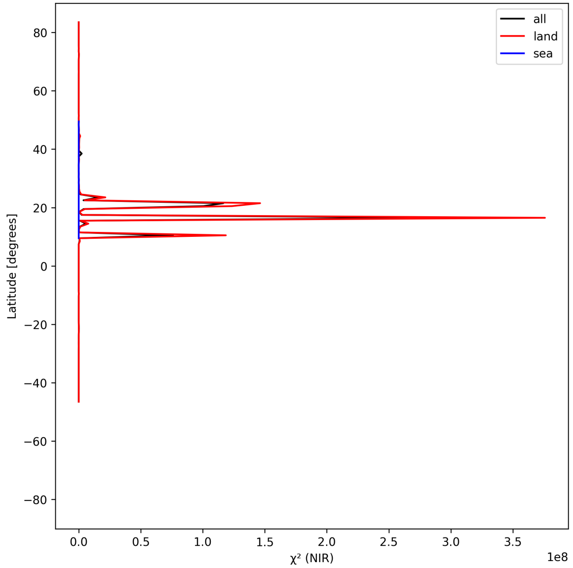
Figure 18: Zonal average of “ \chi^2 (NIR)” for 2025-06-17 to 2025-06-18.
