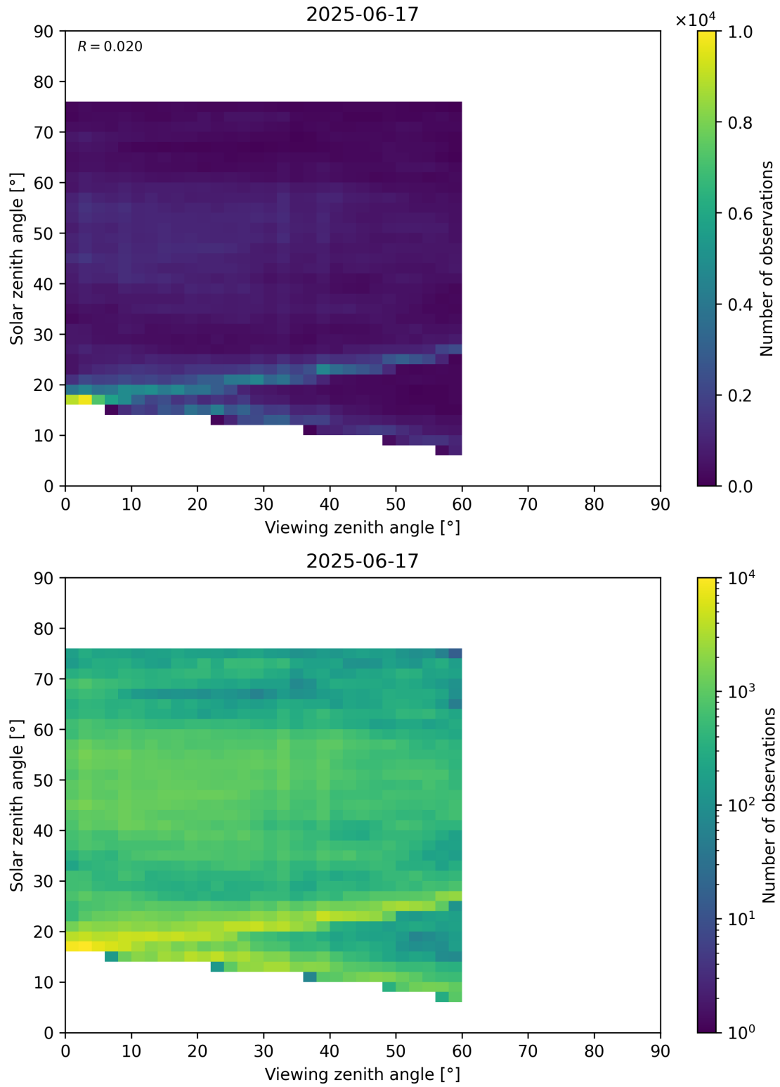
Figure 115: Scatter density plot of “Viewing zenith angle” against “Solar zenith angle” for 2025-06-17 to 2025-06-18.
