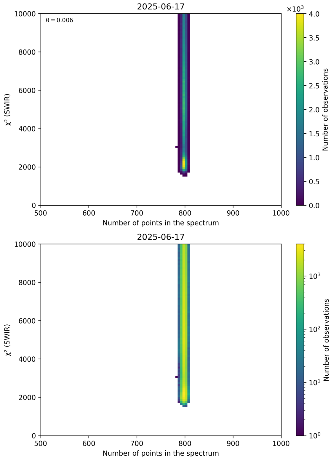
Figure 89: Scatter density plot of “Number of points in the spectrum” against “ \chi^2 (SWIR)” for 2025-06-17 to 2025-06-18.
