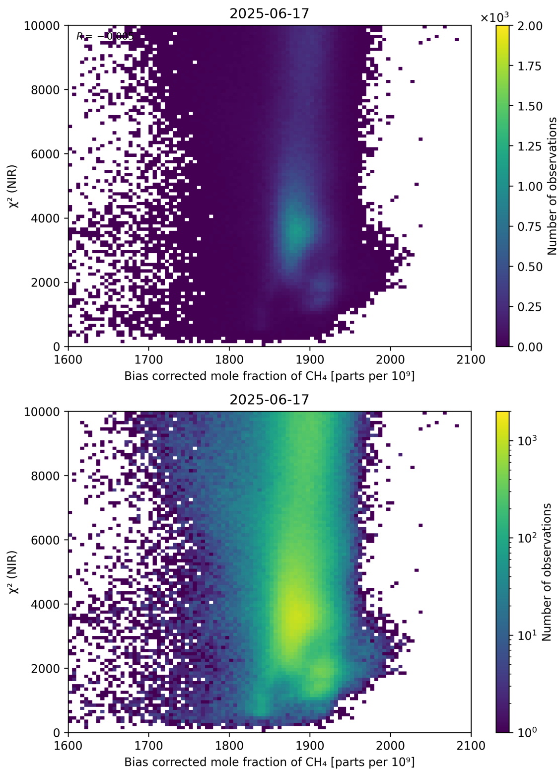
Figure 63: Scatter density plot of “Bias corrected mole fraction of CH 4 ” against “ \chi^2 (NIR)” for 2025-06-17 to 2025-06-18.
