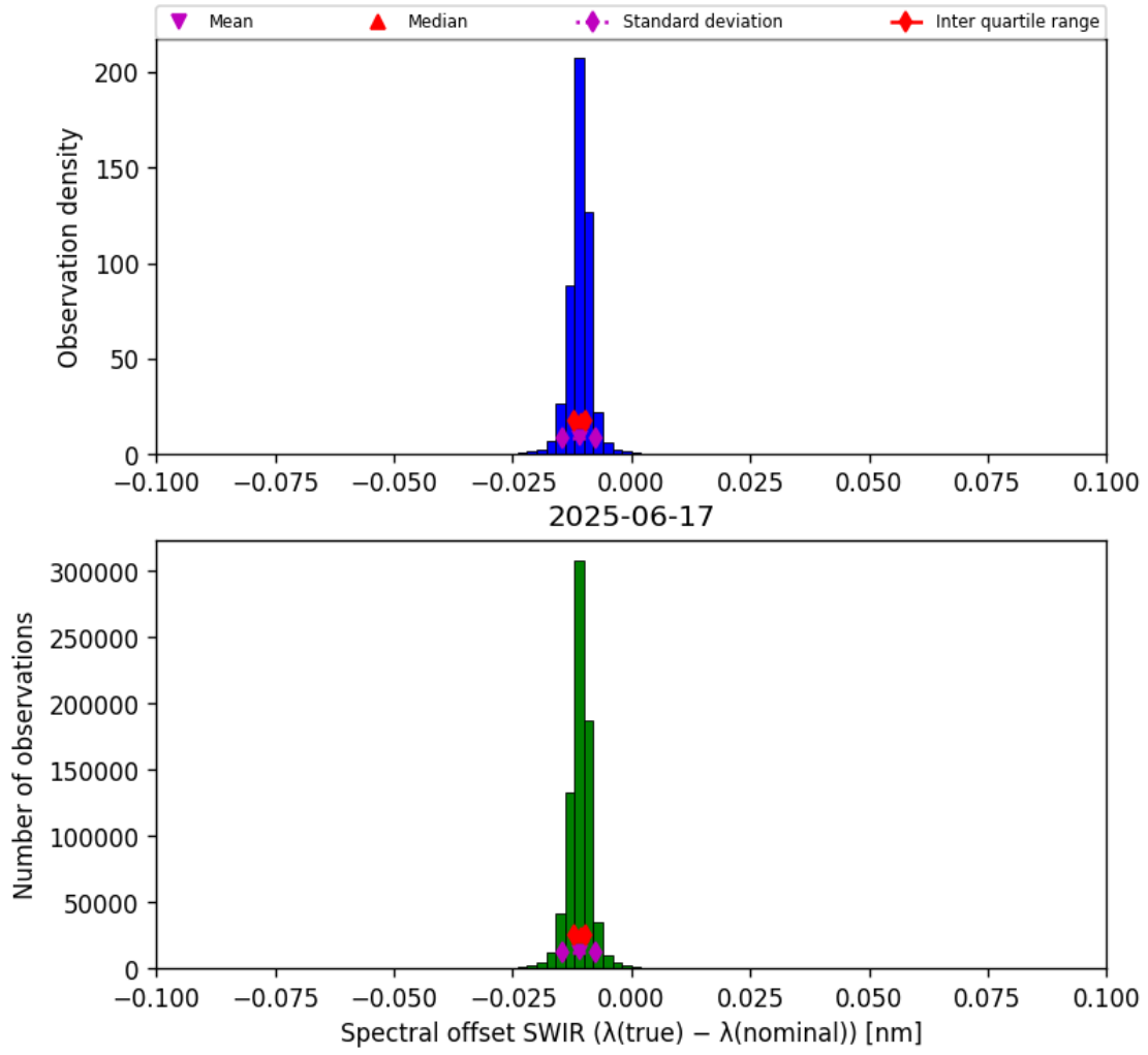
Figure 27: Histogram of “Spectral offset SWIR ( \lambda_{\text{true}} - \lambda_{\text{nominal}} )” for 2025-06-17 to 2025-06-18
