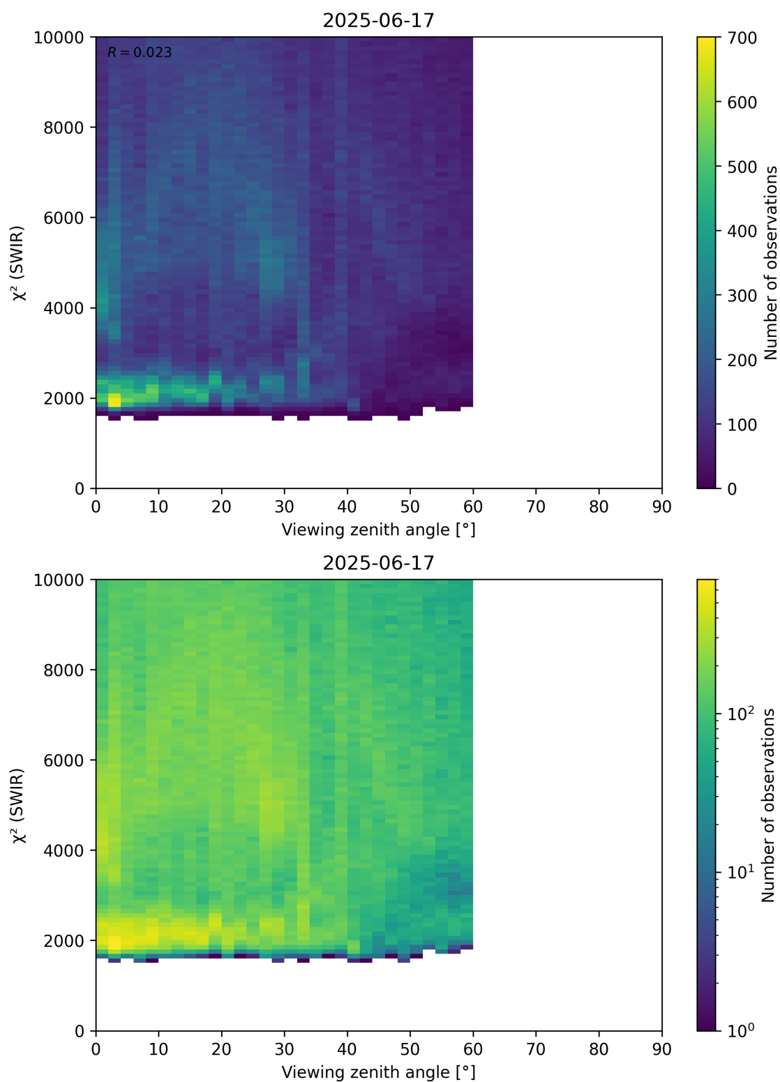
Figure 106: Scatter density plot of “Viewing zenith angle” against “ \chi^2 (SWIR)” for 2025-06-17 to 2025-06-18.
