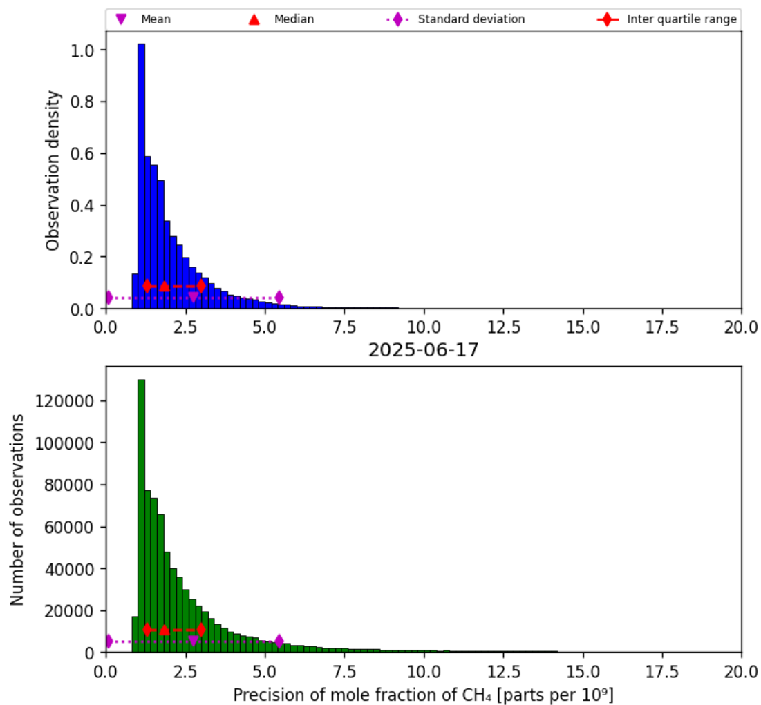
Figure 24: Histogram of “Precision of mole fraction of CH 4 ” for 2025-06-17 to 2025-06-18
