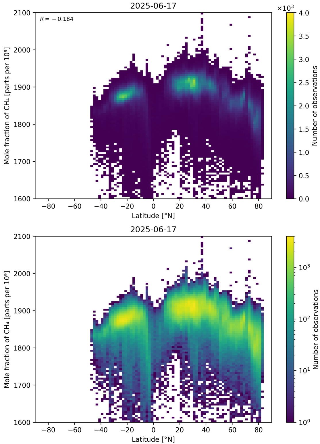
Figure 57: Scatter density plot of “Latitude” against “Mole fraction of CH 4 ” for 2025-06-17 to 2025-06-18.
