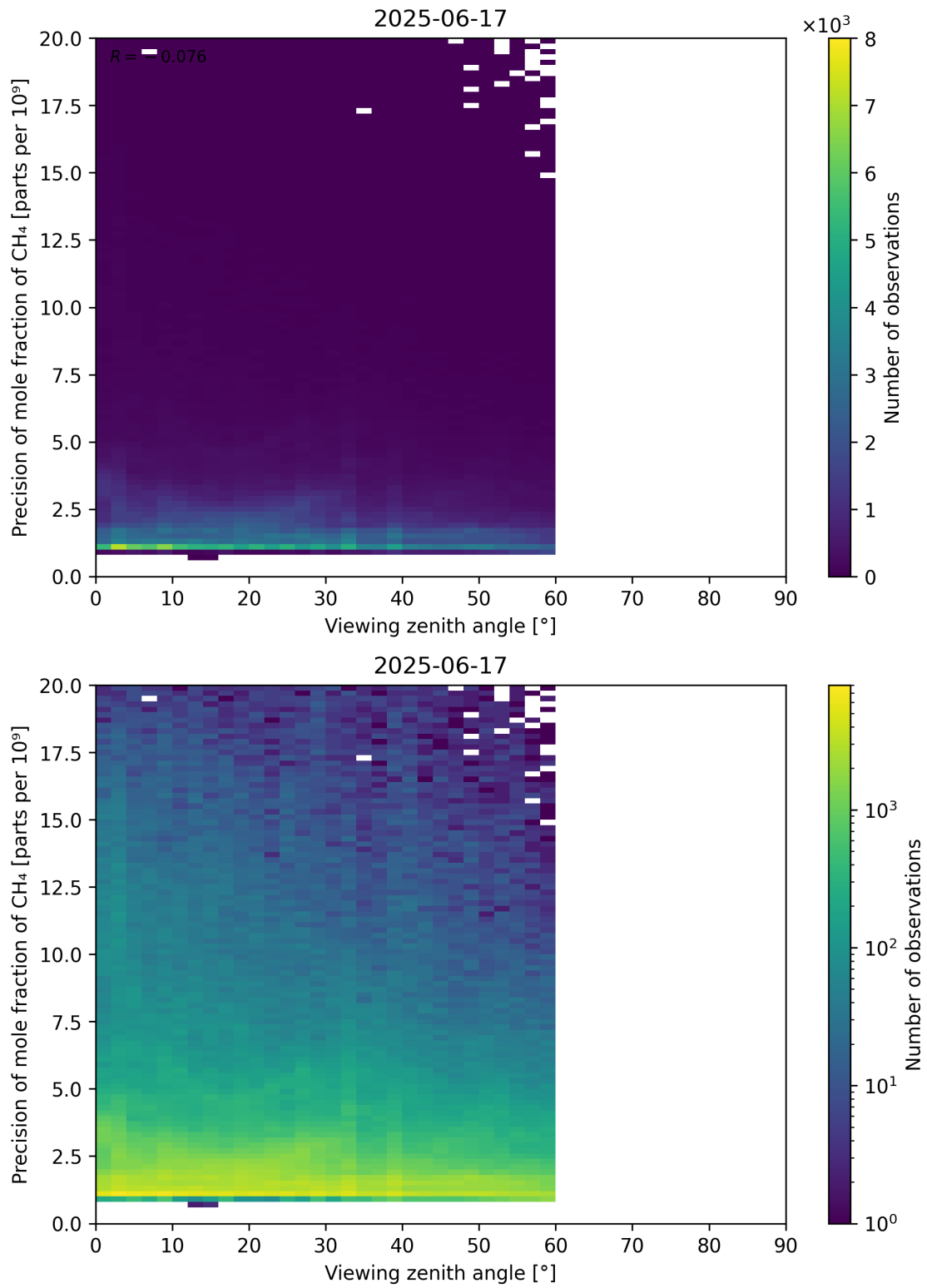
Figure 112: Scatter density plot of “Viewing zenith angle” against “Precision of mole fraction of CH 4 ” for 2025-06-17 to 2025-06-18.
