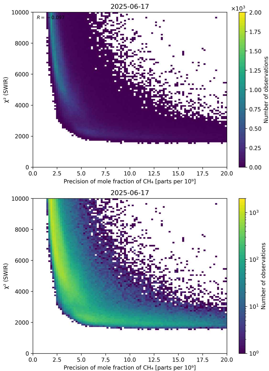
Figure 79: Scatter density plot of “Precision of mole fraction of \text{CH}_4 ” against “ \chi^2 (SWIR)” for 2025-06-17 to 2025-06-18.
