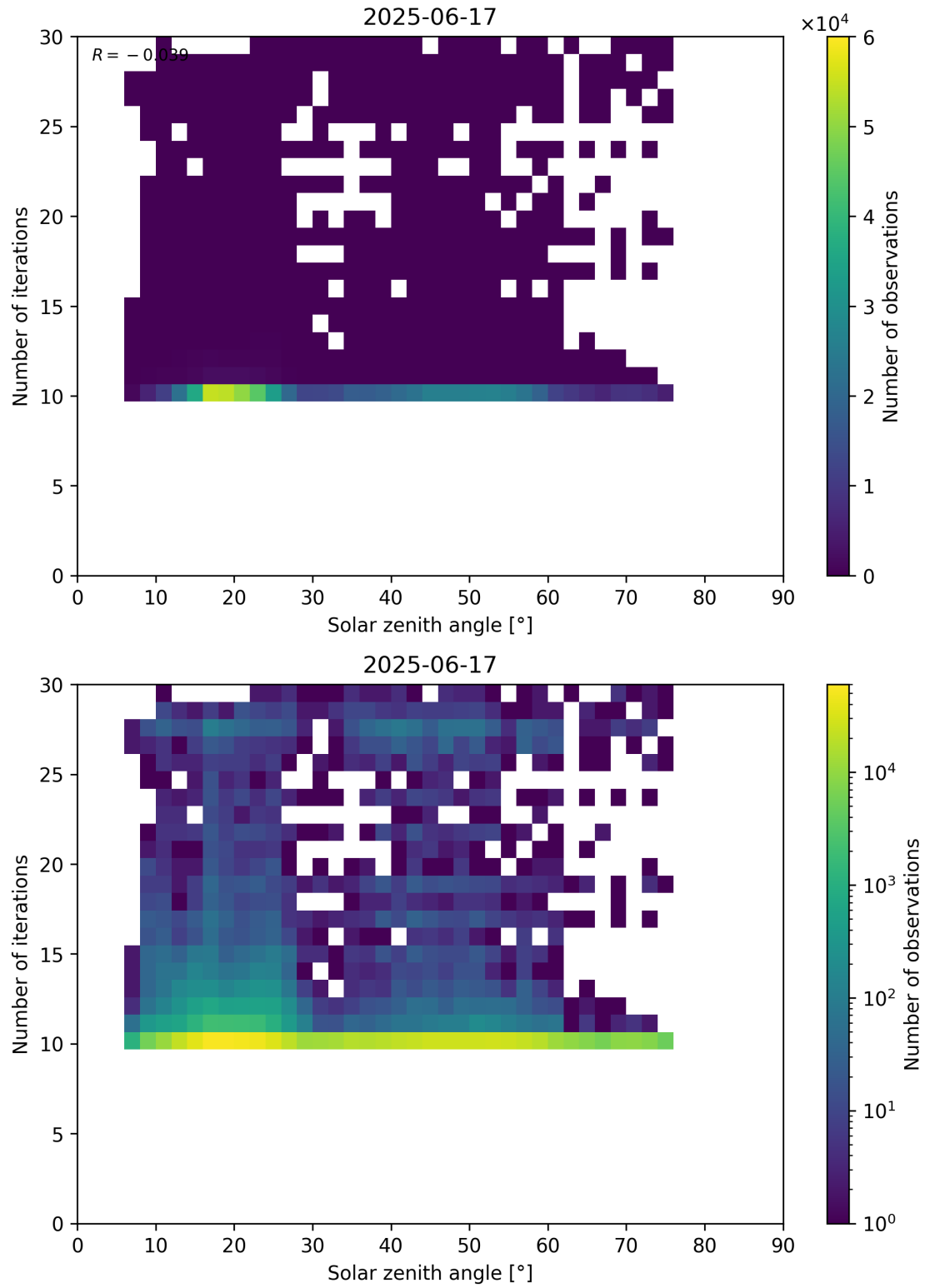
Figure 102: Scatter density plot of “Solar zenith angle” against “Number of iterations” for 2025-06-17 to 2025-06-18.
