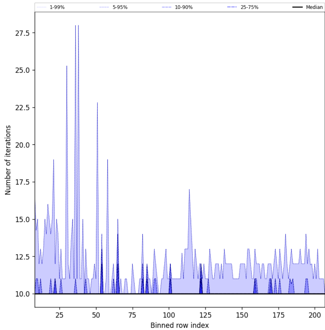
Figure 42: Along track statistics of “Number of iterations” for 2025-06-17 to 2025-06-18
