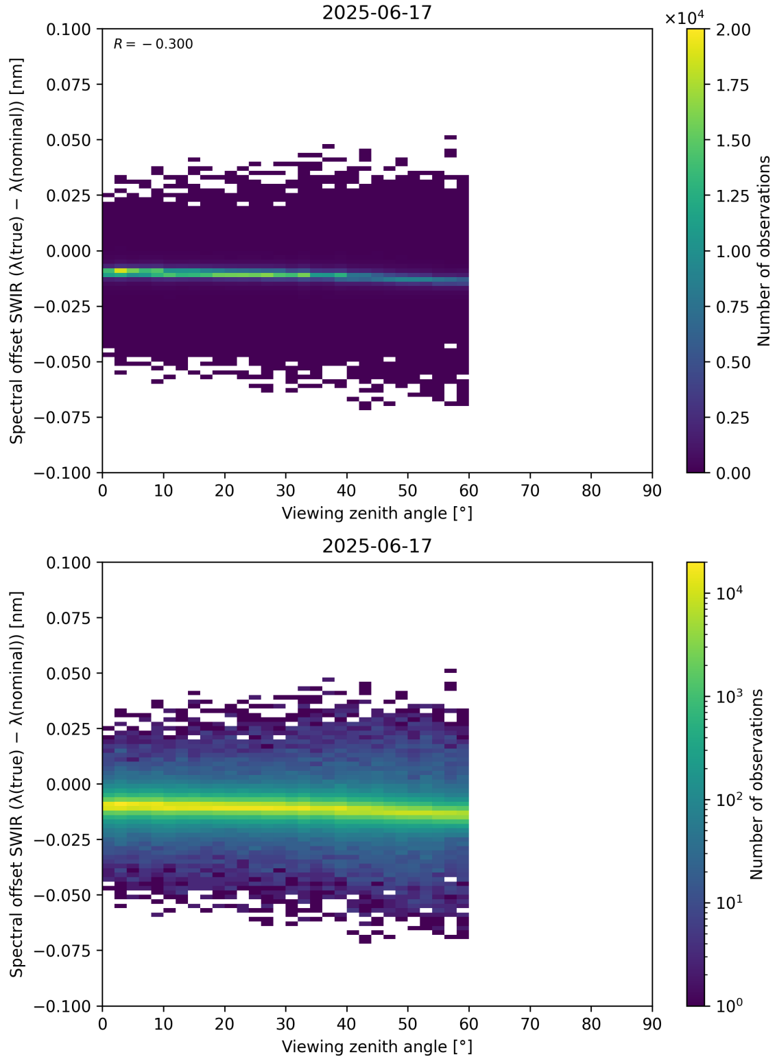
Figure 116: Scatter density plot of “Viewing zenith angle” against “Spectral offset SWIR ( \lambda_{\text{true}} - \lambda_{\text{nominal}} )” for 2025-06-17 to 2025-06-18.
