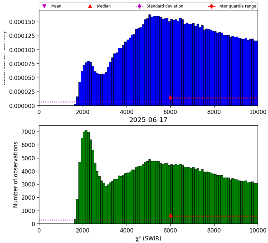
Figure 28: Histogram of “ \chi^2 (SWIR)” for 2025-06-17 to 2025-06-18
