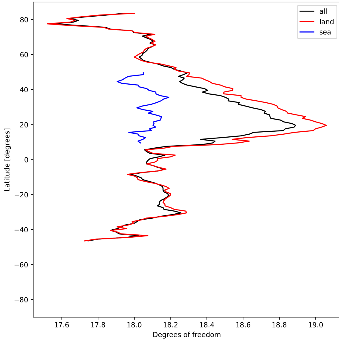
Figure 19: Zonal average of “Degrees of freedom” for 2025-06-17 to 2025-06-18.
