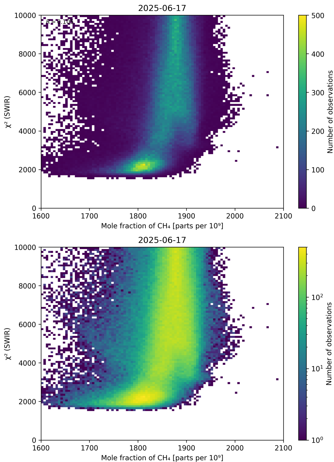
Figure 71: Scatter density plot of “Mole fraction of \text{CH}_4 ” against “ \chi^2 (SWIR)” for 2025-06-17 to 2025-06-18.
