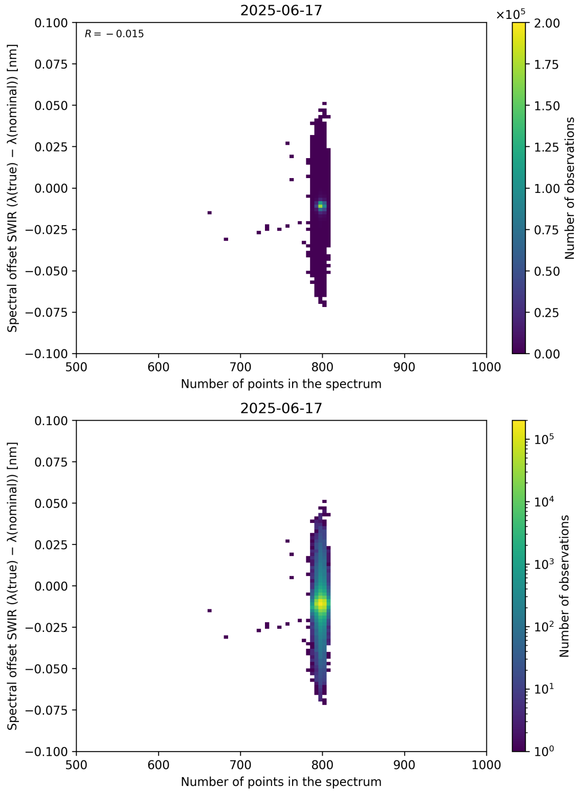
Figure 93: Scatter density plot of “Number of points in the spectrum” against “Spectral offset SWIR ( \lambda_{\text{true}} - \lambda_{\text{nominal}} )” for 2025-06-17 to 2025-06-18.
