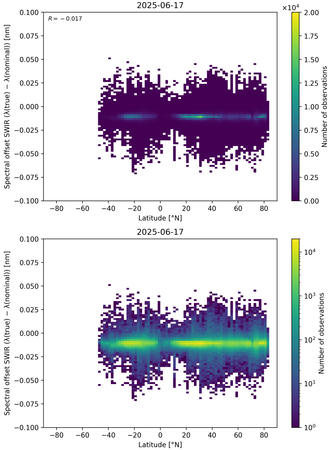
Figure 62: Scatter density plot of “Latitude” against “Spectral offset SWIR ( \lambda_{\text{true}} - \lambda_{\text{nominal}} )” for 2025-06-17 to 2025-06-18.
