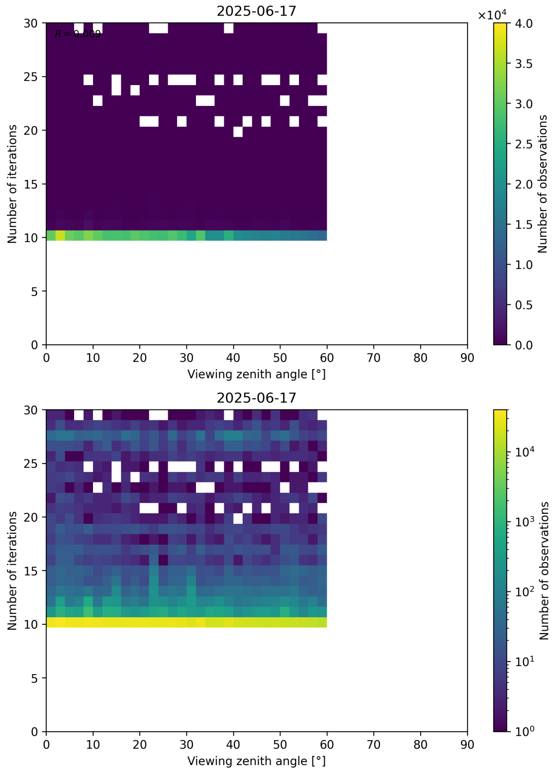
Figure 113: Scatter density plot of “Viewing zenith angle” against “Number of iterations” for 2025-06-17 to 2025-06-18.
