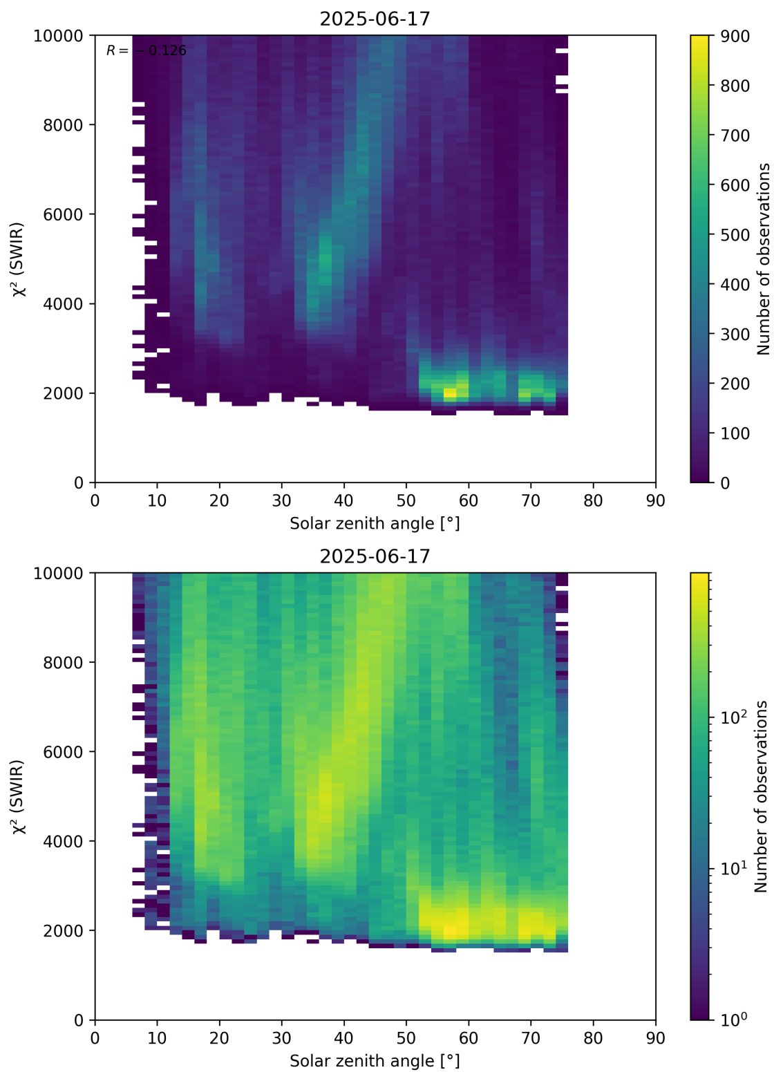
Figure 95: Scatter density plot of “Solar zenith angle” against “ \chi^2 (SWIR)” for 2025-06-17 to 2025-06-18.
