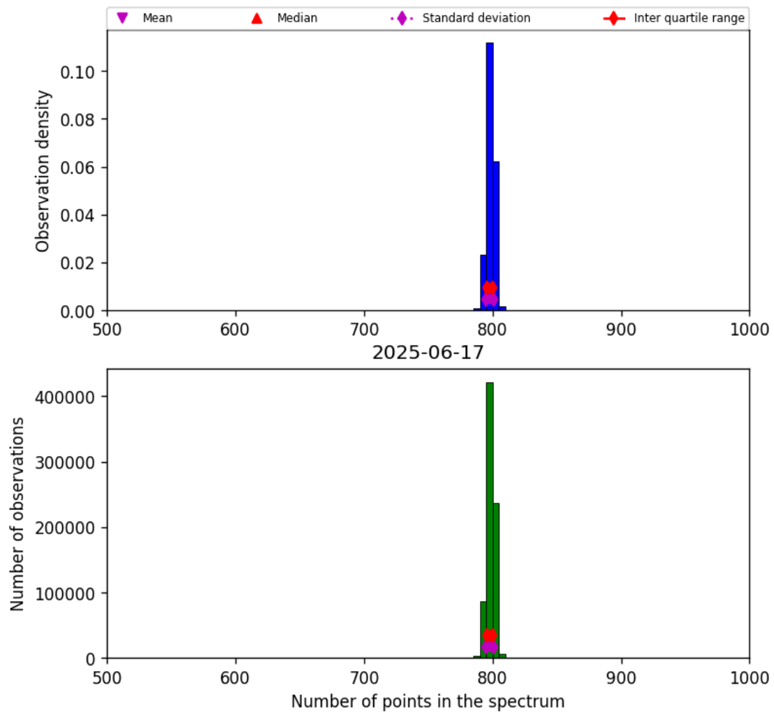
Figure 26: Histogram of “Number of points in the spectrum” for 2025-06-17 to 2025-06-18
