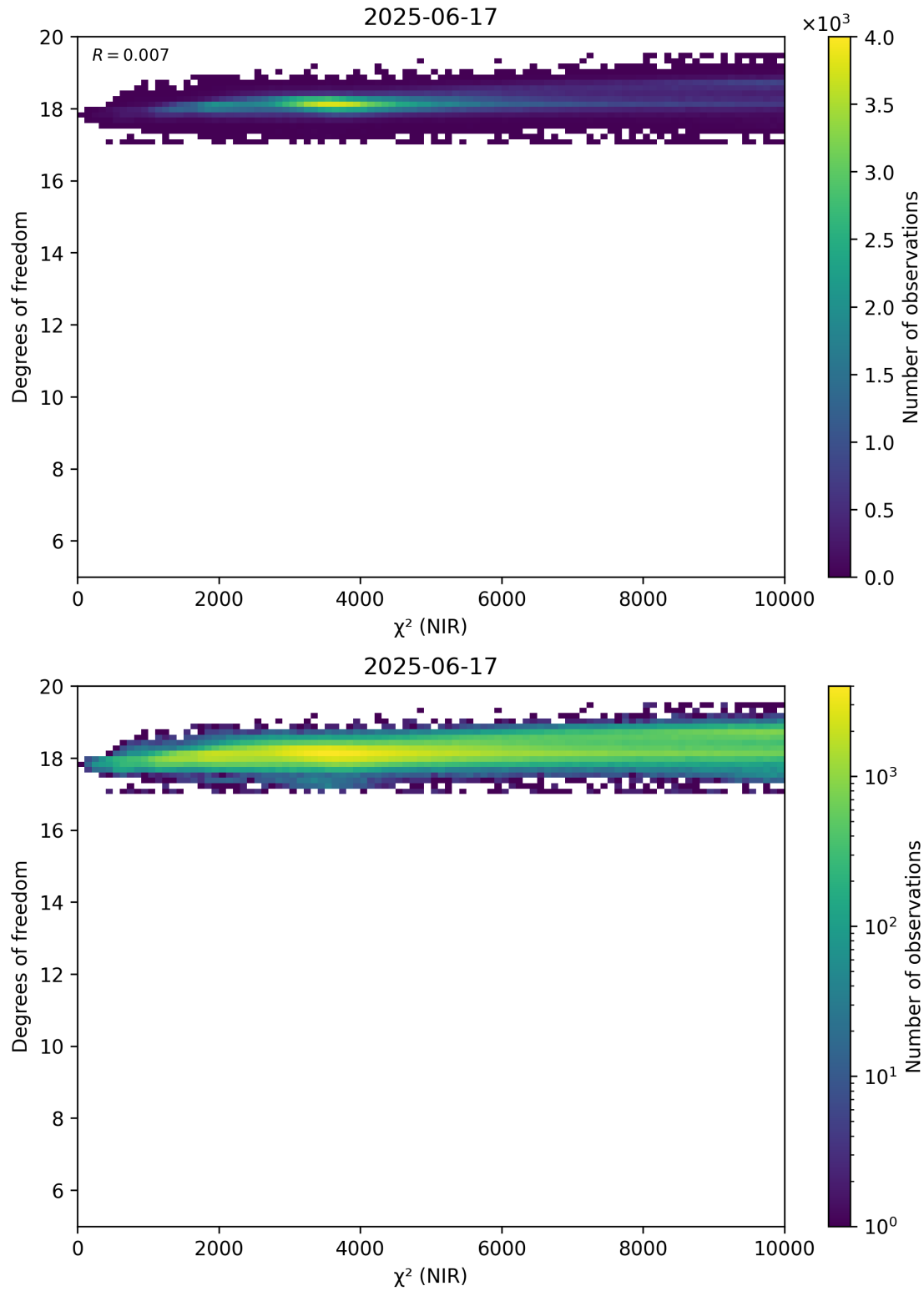
Figure 44: Scatter density plot of “ \chi^2 (NIR)” against “Degrees of freedom” for 2025-06-17 to 2025-06-18.
