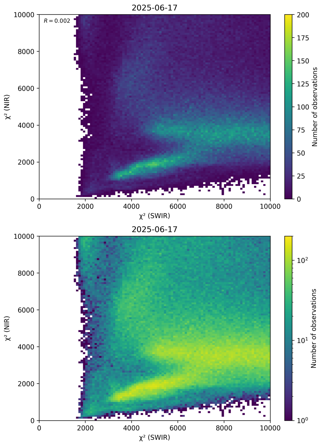
Figure 47: Scatter density plot of “ \chi^2 (SWIR)” against “ \chi^2 (NIR)” for 2025-06-17 to 2025-06-18.
