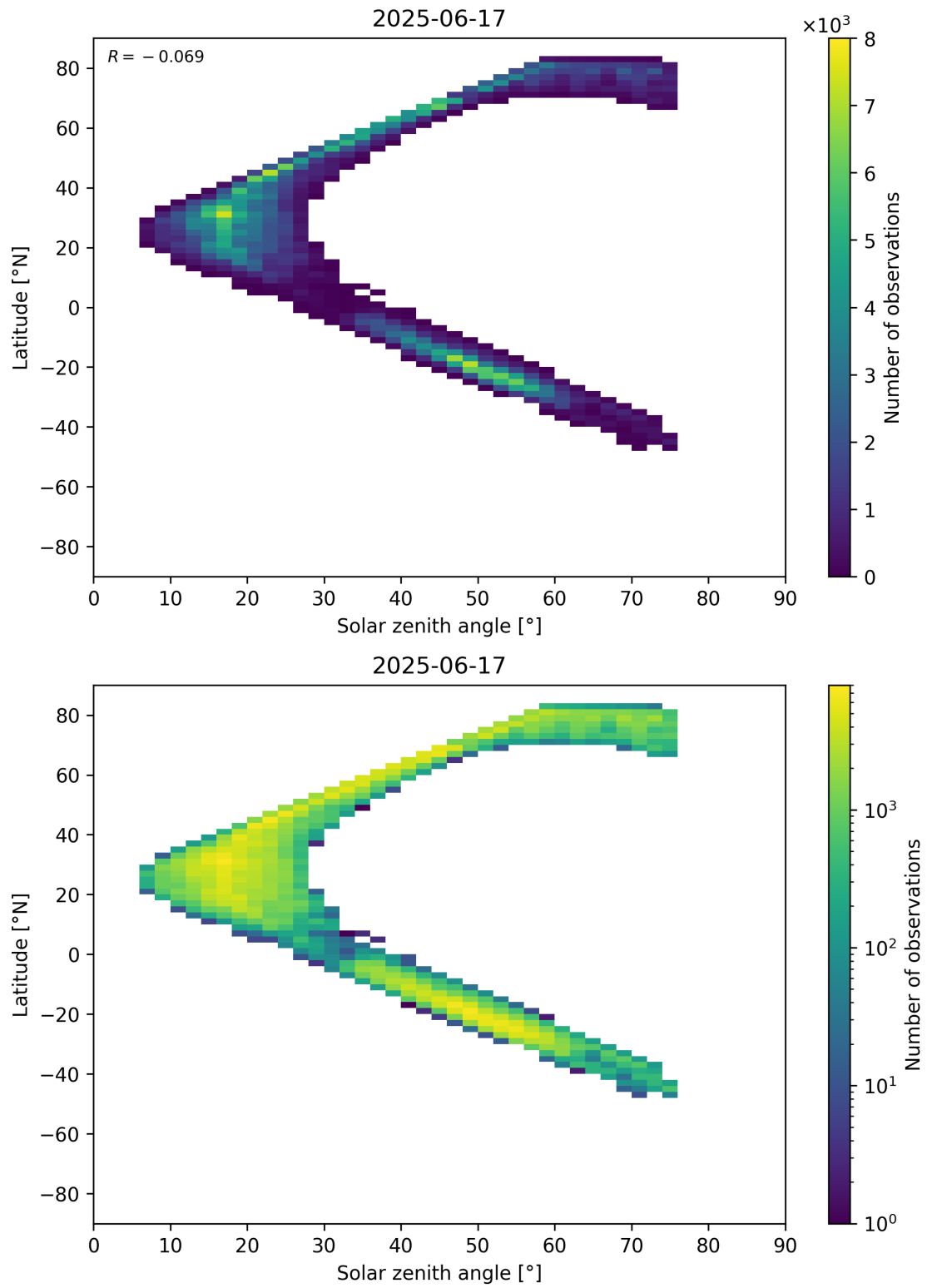
Figure 98: Scatter density plot of “Solar zenith angle” against “Latitude” for 2025-06-17 to 2025-06-18.
