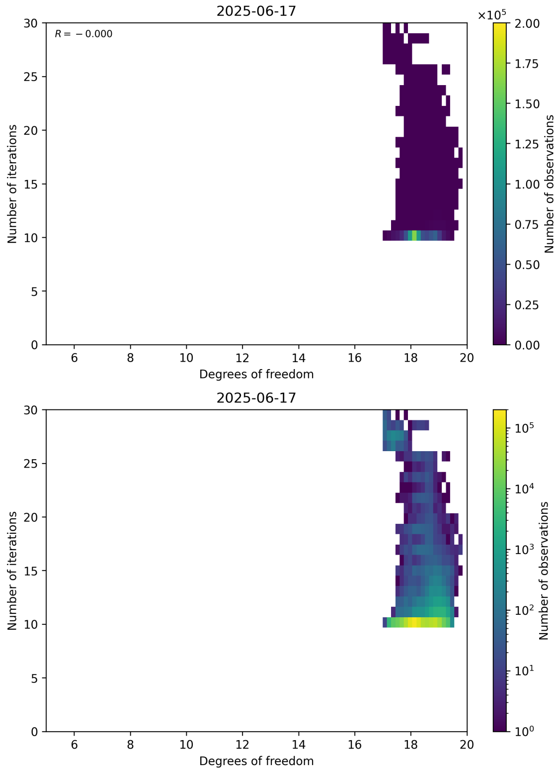
Figure 52: Scatter density plot of “Degrees of freedom” against “Number of iterations” for 2025-06-17 to 2025-06-18.
