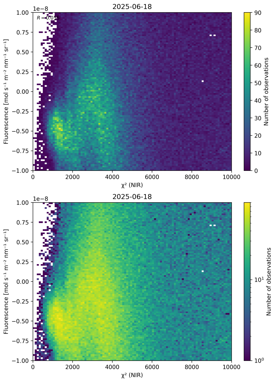
Figure 45: Scatter density plot of “ \chi^2 (NIR)” against “Fluorescence” for 2025-06-17 to 2025-06-19.
