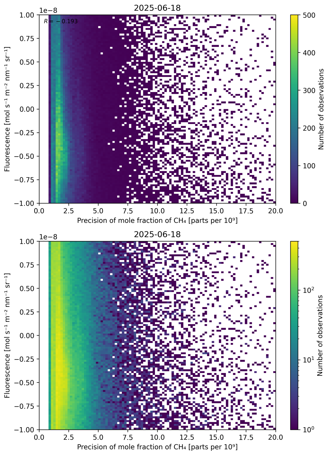
Figure 81: Scatter density plot of “Precision of mole fraction of CH 4 ” against “Fluorescence” for 2025-06-17 to 2025-06-19.
