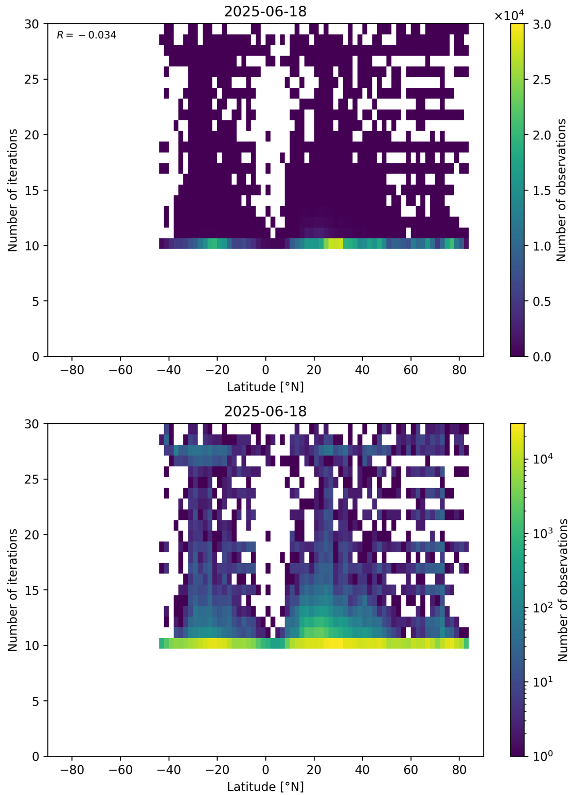
Figure 60: Scatter density plot of “Latitude” against “Number of iterations” for 2025-06-17 to 2025-06-19.
