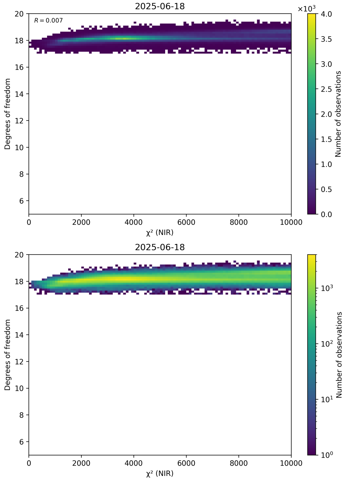
Figure 44: Scatter density plot of “ \chi^2 (NIR)” against “Degrees of freedom” for 2025-06-17 to 2025-06-19.
