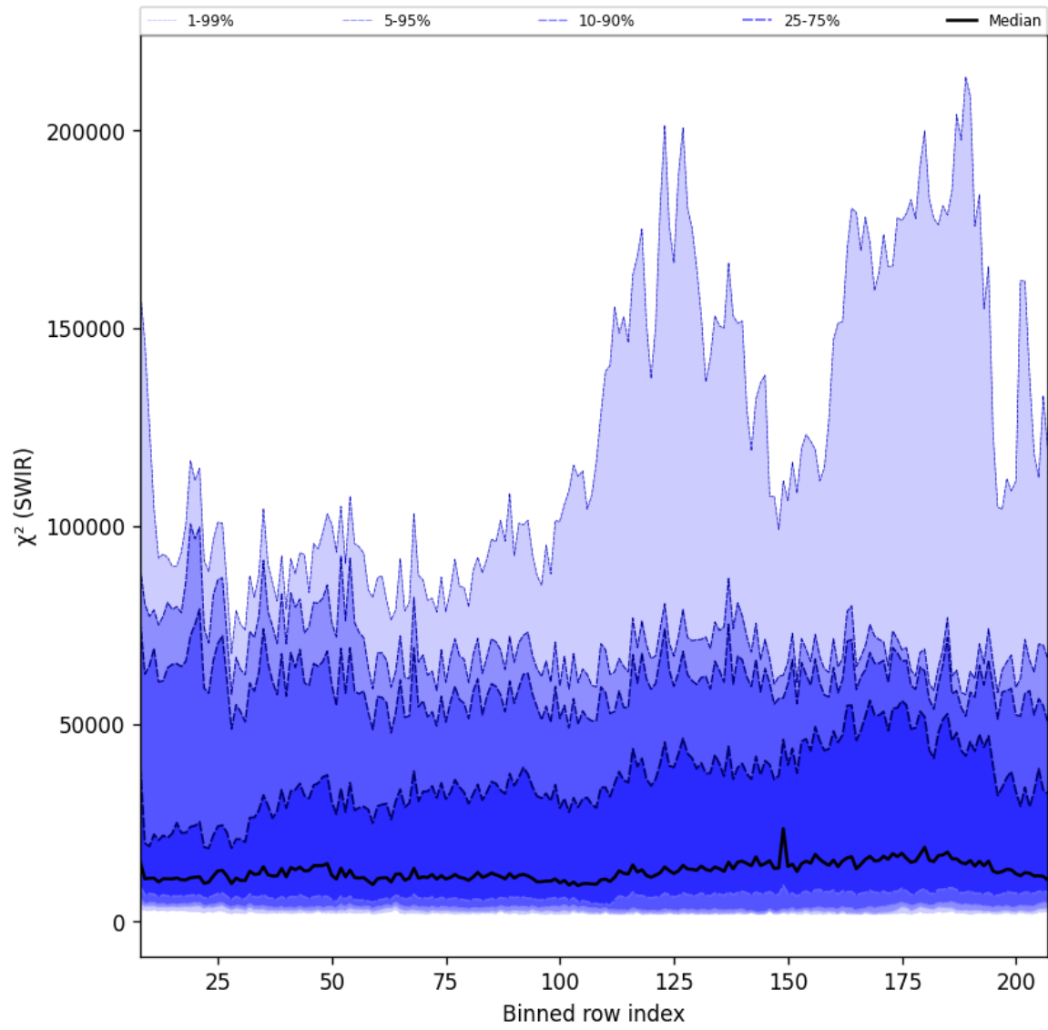
Figure 39: Along track statistics of " \chi^2 (SWIR)" for 2025-06-17 to 2025-06-19
