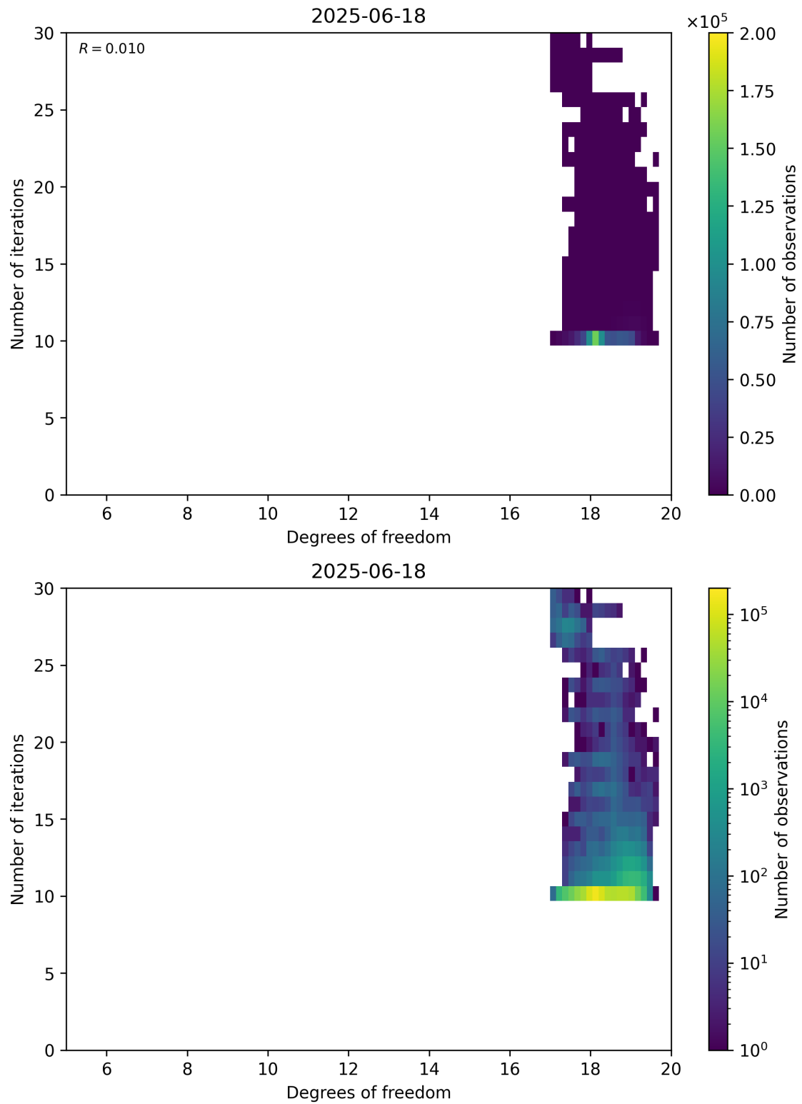
Figure 52: Scatter density plot of “Degrees of freedom” against “Number of iterations” for 2025-06-17 to 2025-06-19.
