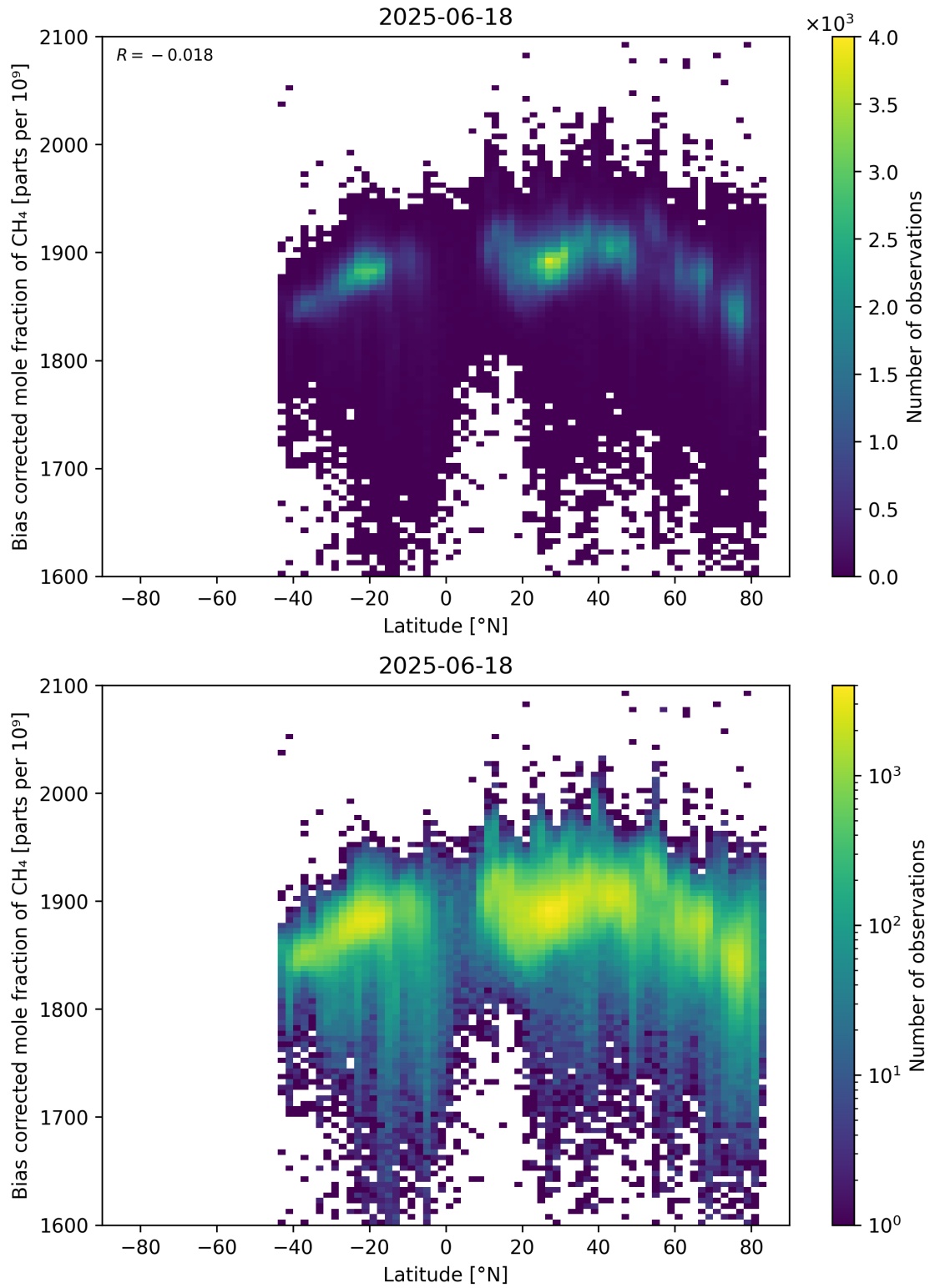
Figure 58: Scatter density plot of “Latitude” against “Bias corrected mole fraction of CH 4 ” for 2025-06-17 to 2025-06-19.
