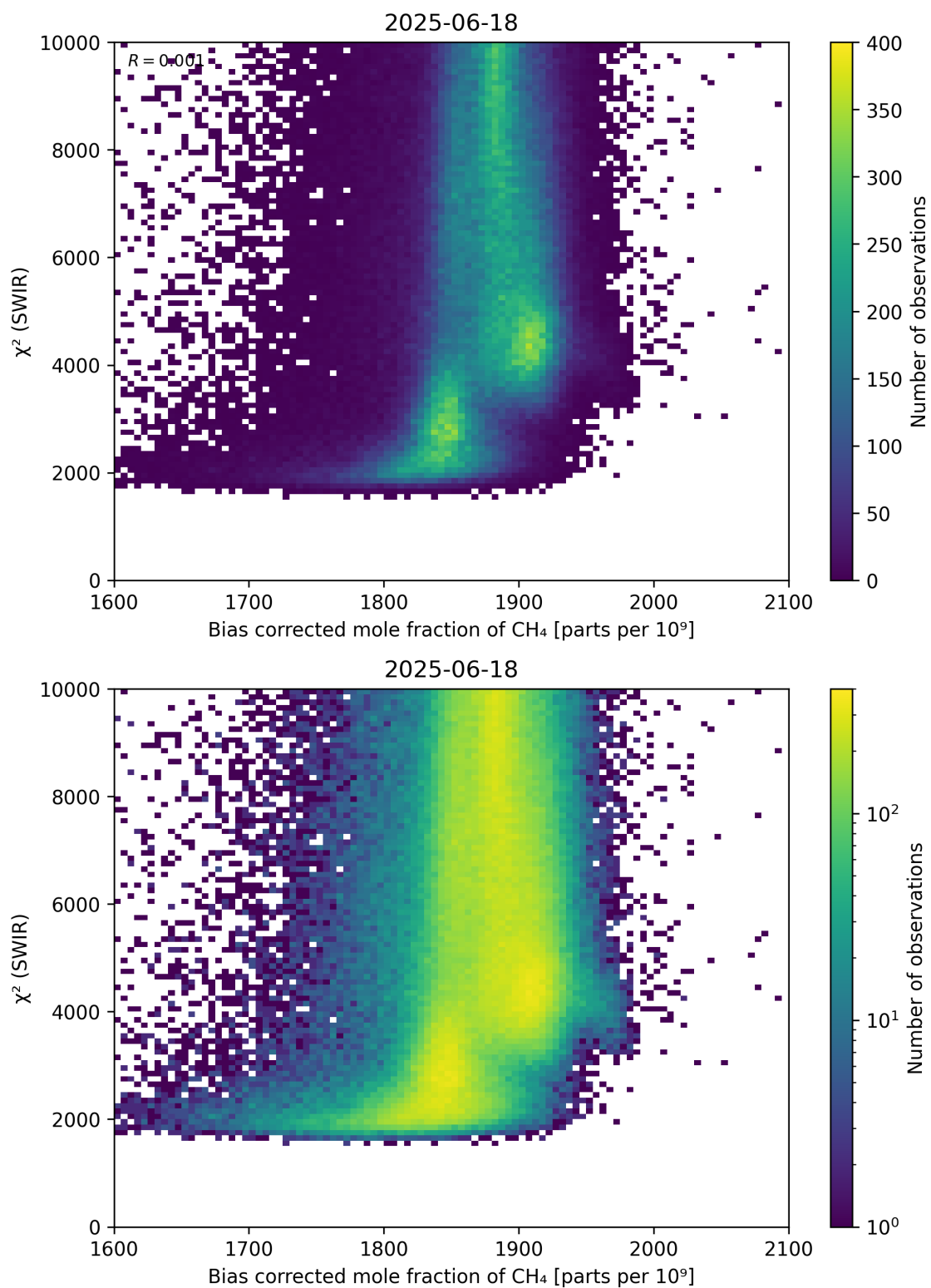
Figure 64: Scatter density plot of “Bias corrected mole fraction of CH 4 ” against “ \chi^2 (SWIR)” for 2025-06-17 to 2025-06-19.
