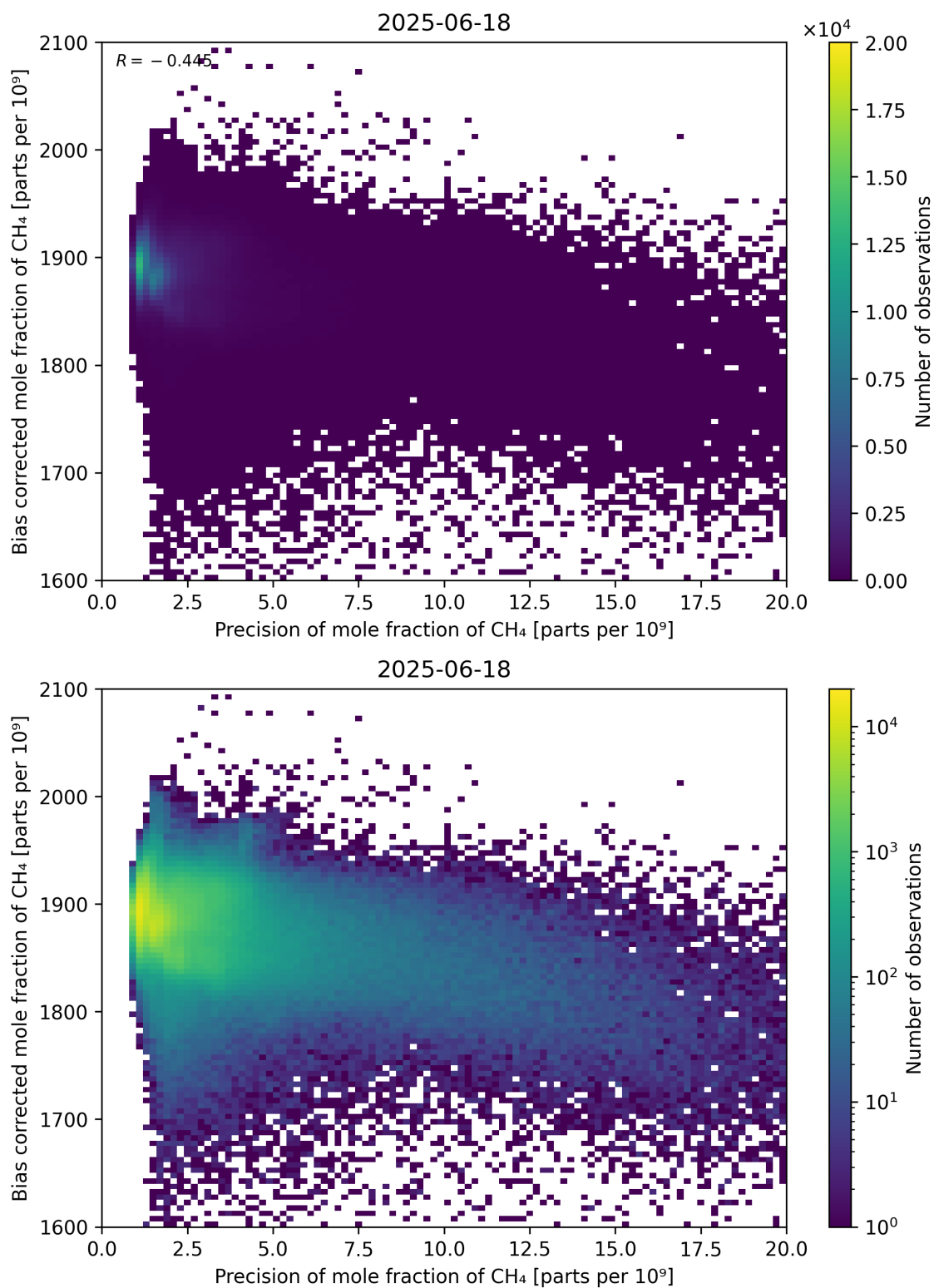
Figure 82: Scatter density plot of “Precision of mole fraction of CH 4 ” against “Bias corrected mole fraction of CH 4 ” for 2025-06-17 to 2025-06-19.
