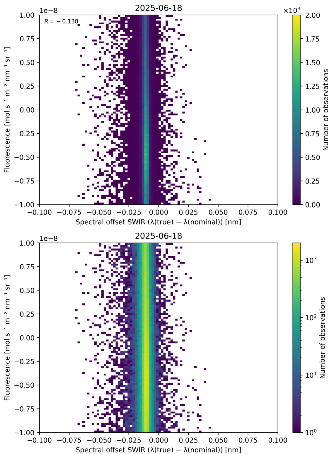
Figure 120: Scatter density plot of “Spectral offset SWIR ( \lambda_{\text{true}} - \lambda_{\text{nominal}} )” against “Fluorescence” for 2025-06-17 to 2025-06-19.
