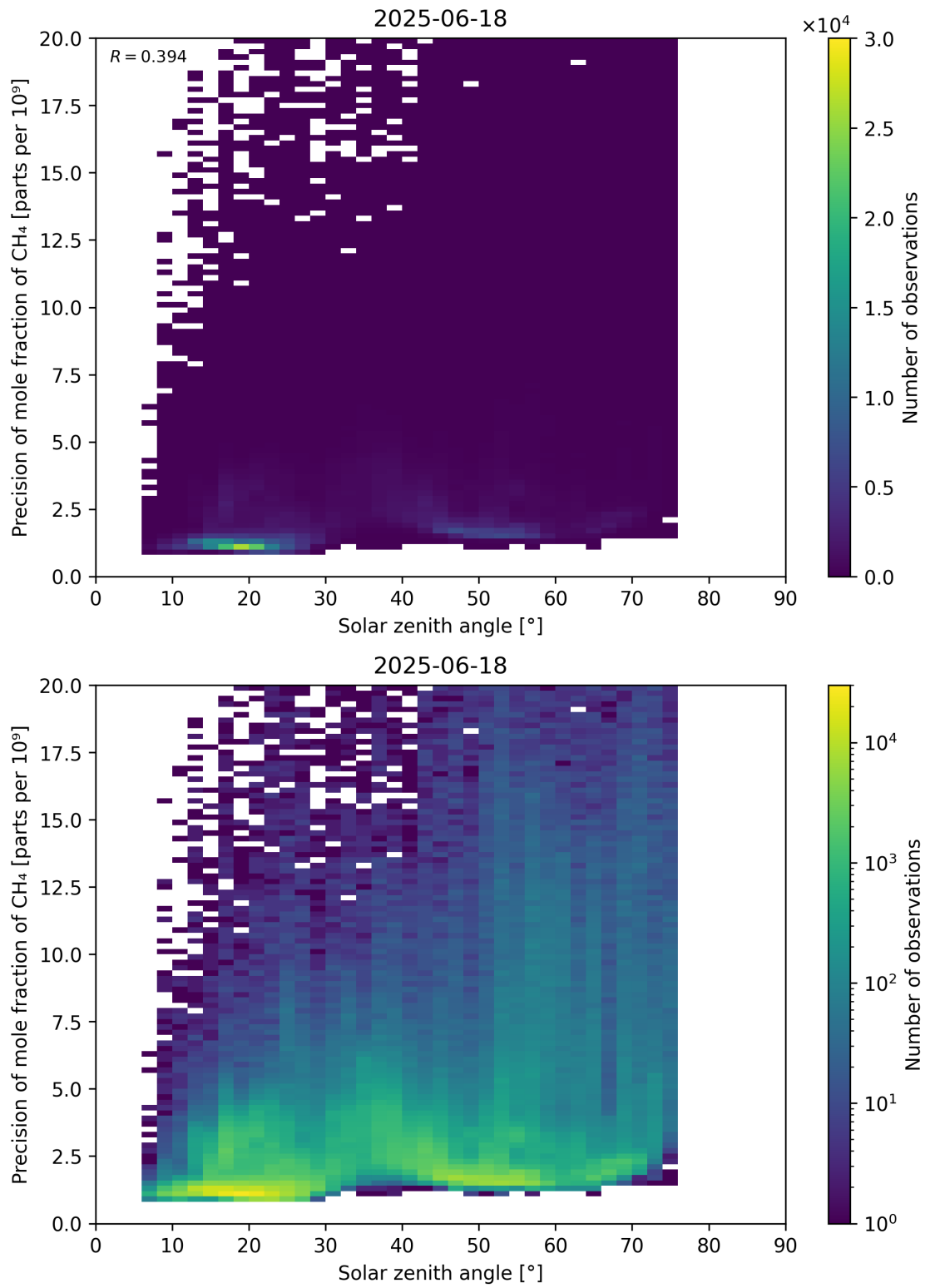
Figure 101: Scatter density plot of “Solar zenith angle” against “Precision of mole fraction of CH 4 ” for 2025-06-17 to 2025-06-19.
