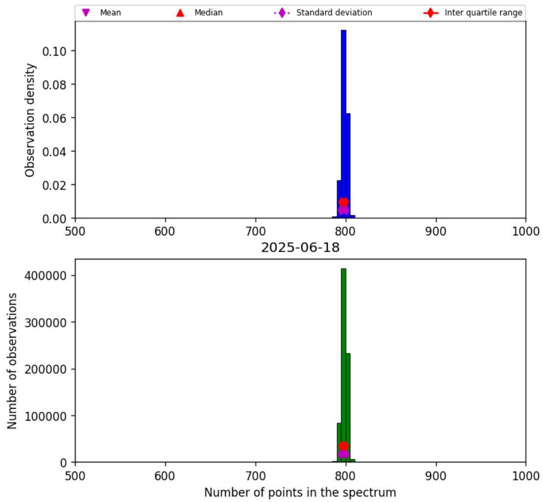
Figure 26: Histogram of “Number of points in the spectrum” for 2025-06-17 to 2025-06-19
