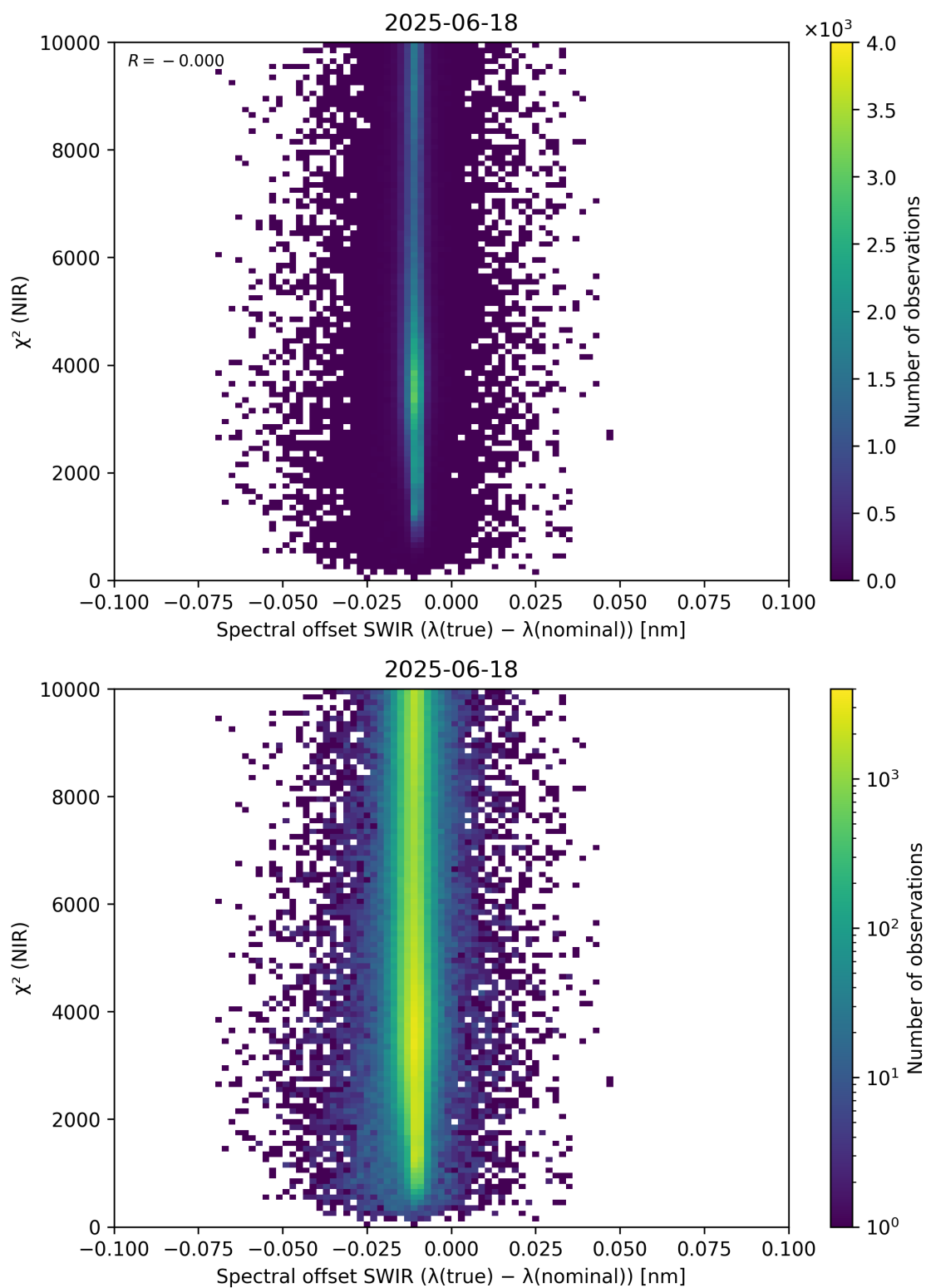
Figure 117: Scatter density plot of “Spectral offset SWIR ( \lambda_{\text{true}} - \lambda_{\text{nominal}} )” against “ \chi^2 (NIR)” for 2025-06-17 to 2025-06-19.
