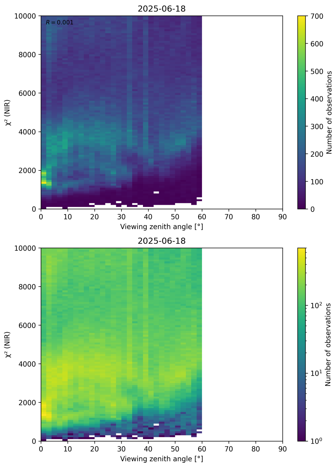
Figure 105: Scatter density plot of “Viewing zenith angle” against “ \chi^2 (NIR)” for 2025-06-17 to 2025-06-19.
