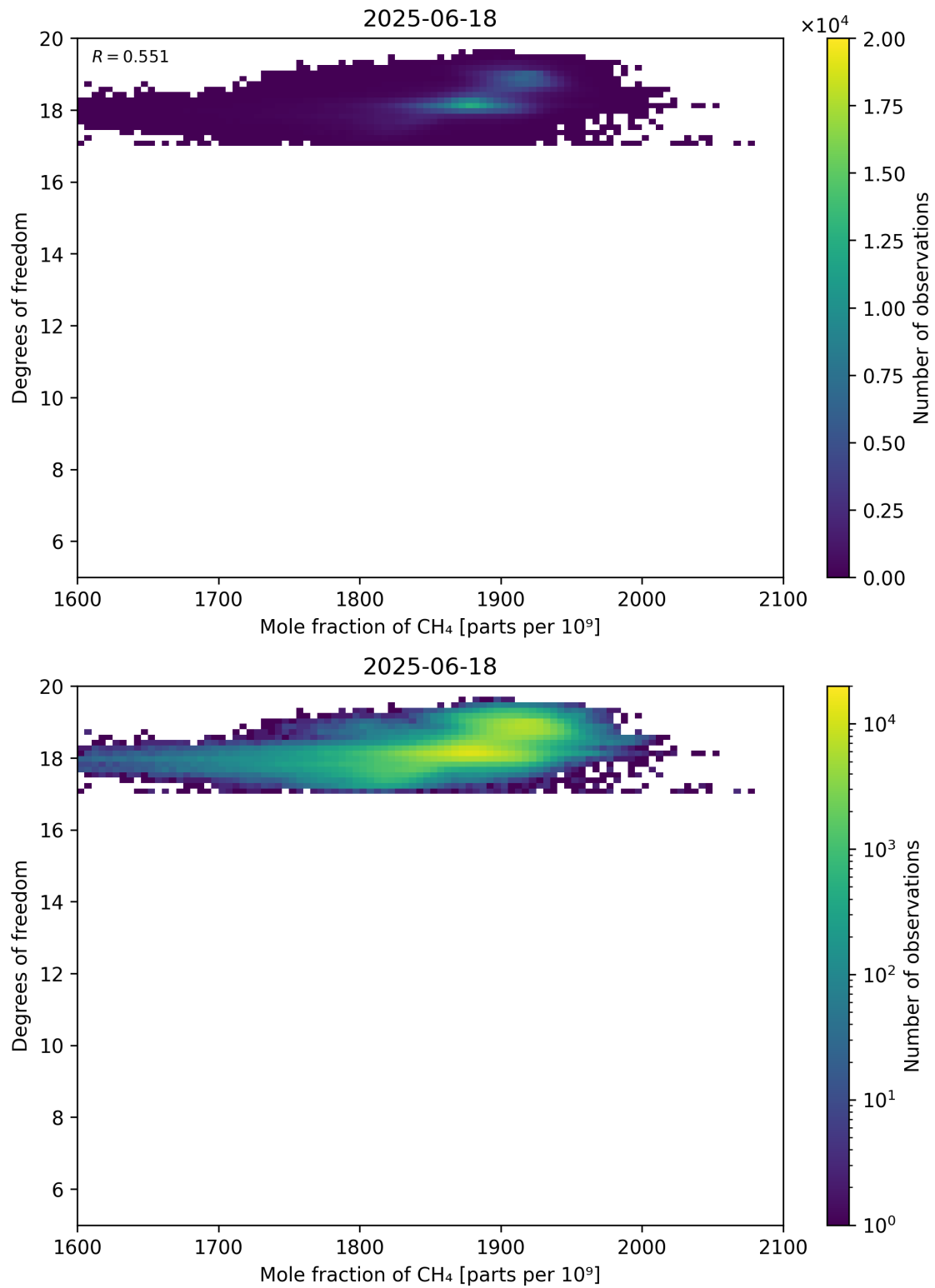
Figure 72: Scatter density plot of “Mole fraction of CH 4 ” against “Degrees of freedom” for 2025-06-17 to 2025-06-19.
