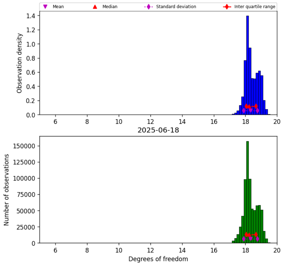
Figure 30: Histogram of “Degrees of freedom” for 2025-06-17 to 2025-06-19
