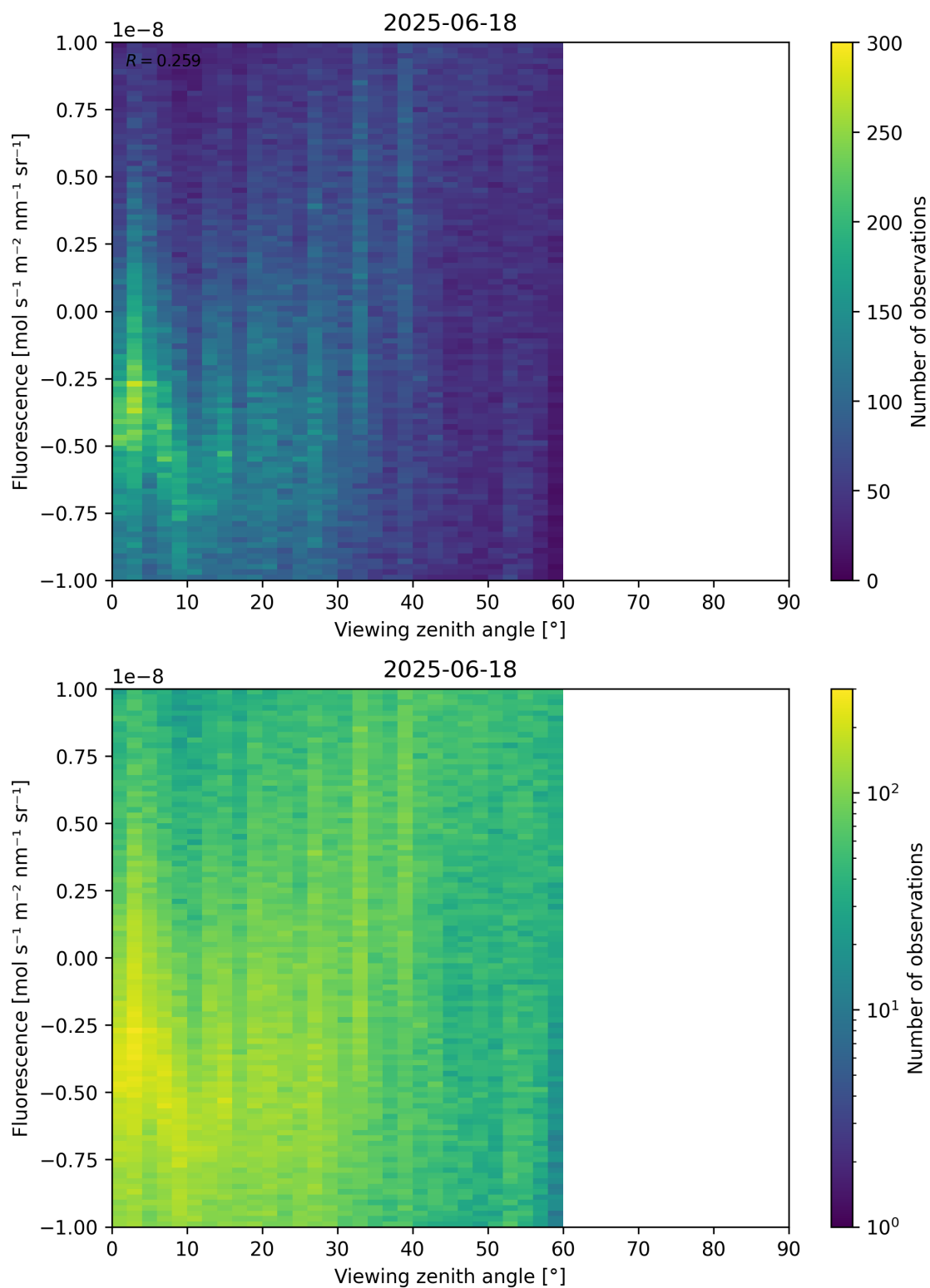
Figure 108: Scatter density plot of “Viewing zenith angle” against “Fluorescence” for 2025-06-17 to 2025-06-19.
