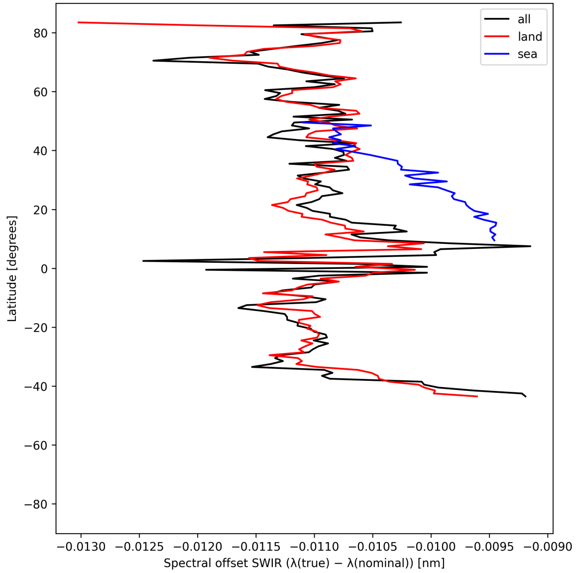
Figure 16: Zonal average of “Spectral offset SWIR ( \lambda_{\text{true}} - \lambda_{\text{nominal}} )” for 2025-06-17 to 2025-06-19.
