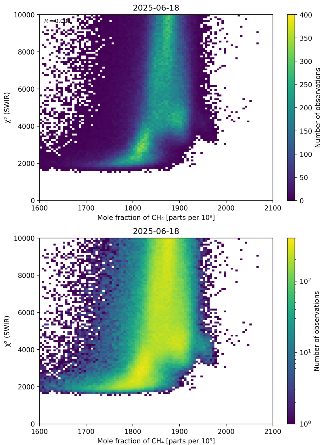
Figure 71: Scatter density plot of “Mole fraction of CH 4 ” against “ \chi^2 (SWIR)” for 2025-06-17 to 2025-06-19.
