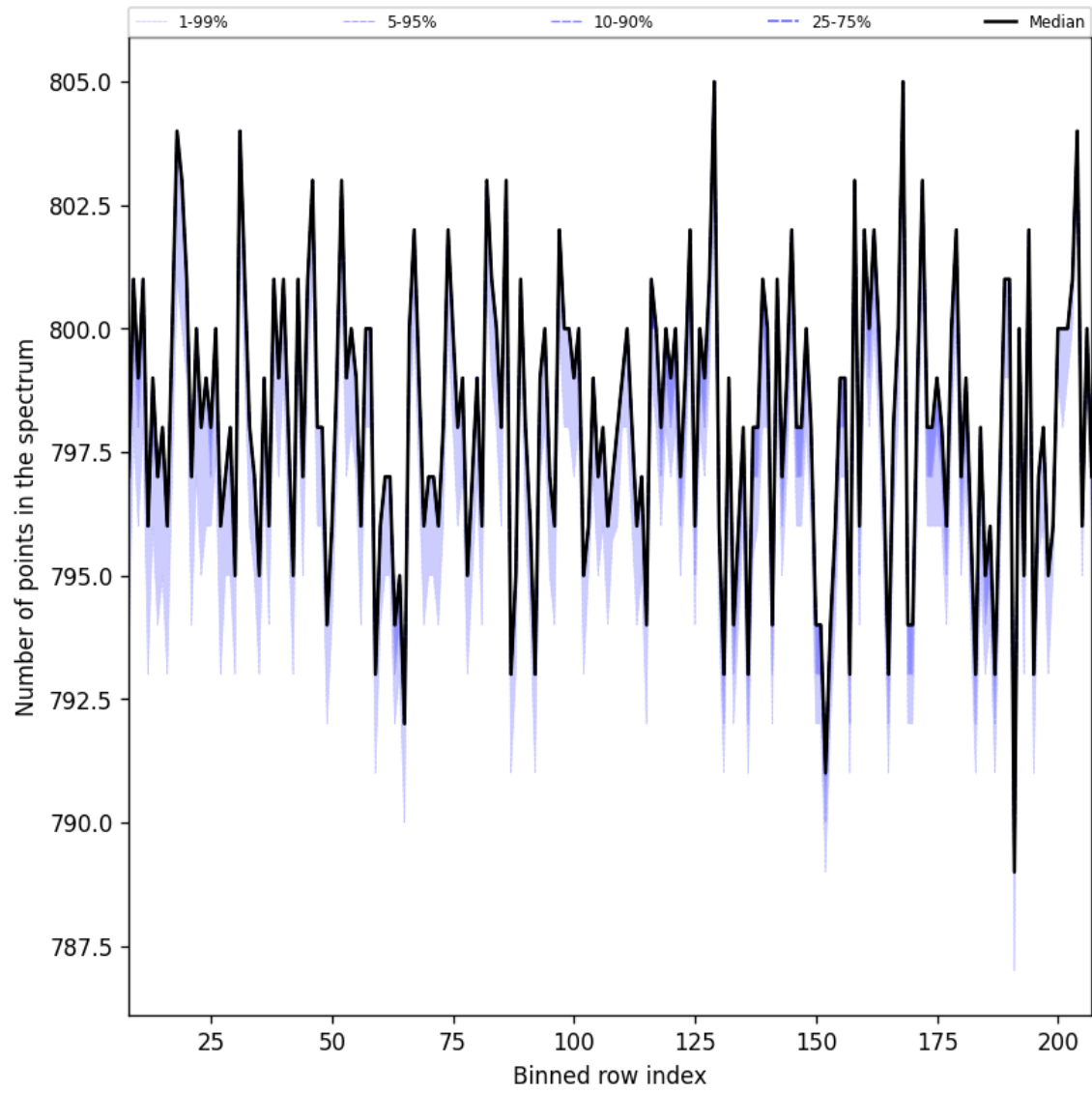
Figure 37: Along track statistics of “Number of points in the spectrum” for 2025-06-17 to 2025-06-19
