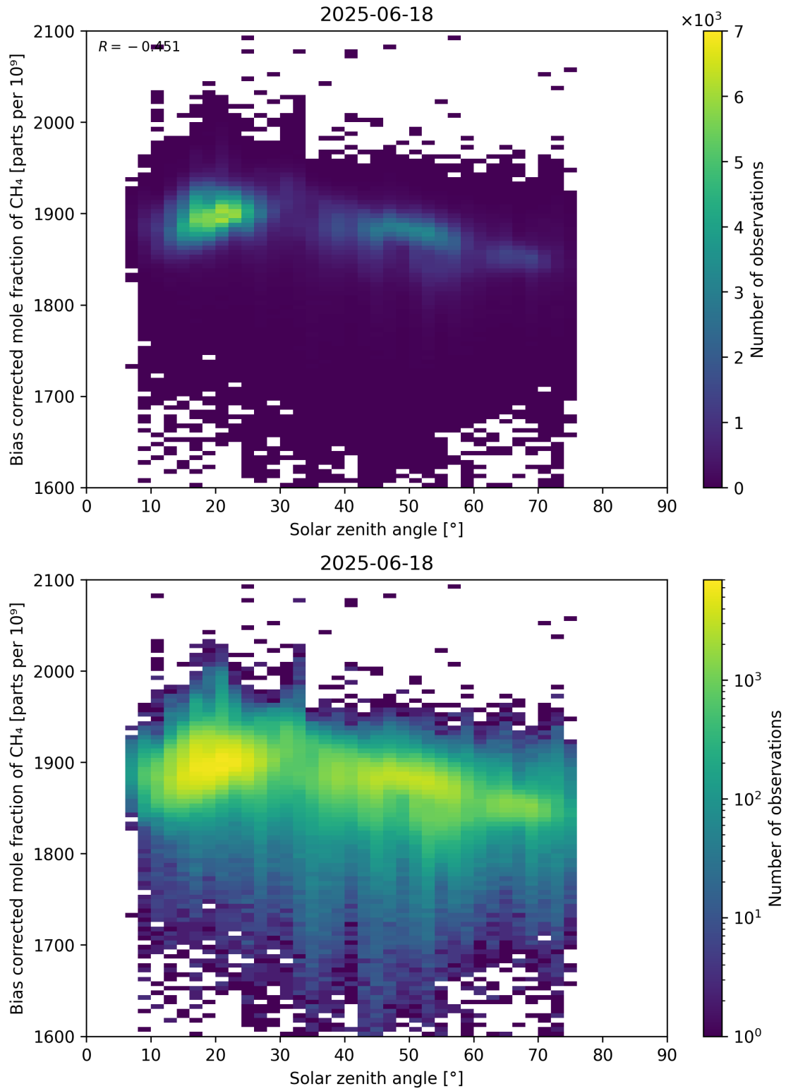
Figure 100: Scatter density plot of “Solar zenith angle” against “Bias corrected mole fraction of \text{CH}_4 ” for 2025-06-17 to 2025-06-19.
