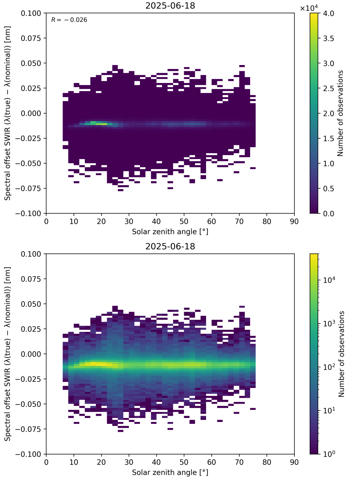
Figure 104: Scatter density plot of “Solar zenith angle” against “Spectral offset SWIR ( \lambda_{\text{true}} - \lambda_{\text{nominal}} )” for 2025-06-17 to 2025-06-19.
