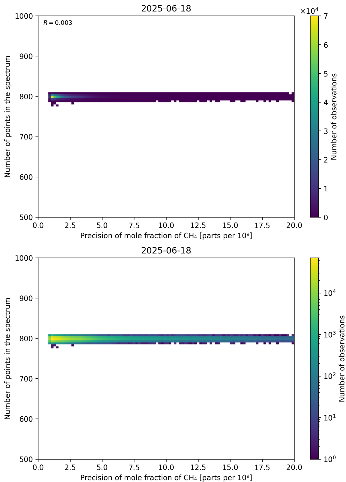
Figure 84: Scatter density plot of “Precision of mole fraction of CH 4 ” against “Number of points in the spectrum” for 2025-06-17 to 2025-06-19.
