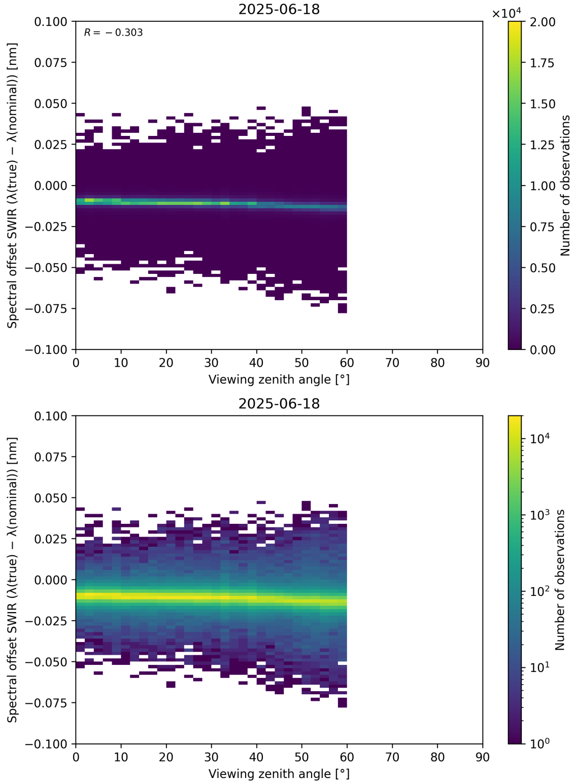
Figure 116: Scatter density plot of “Viewing zenith angle” against “Spectral offset SWIR ( \lambda_{\text{true}} - \lambda_{\text{nominal}} )” for 2025-06-17 to 2025-06-19.
