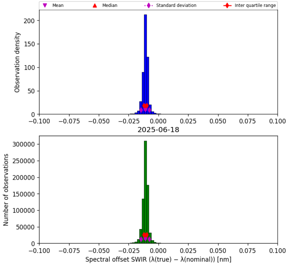
Figure 27: Histogram of “Spectral offset SWIR ( \lambda_{\text{true}} - \lambda_{\text{nominal}} )” for 2025-06-17 to 2025-06-19
