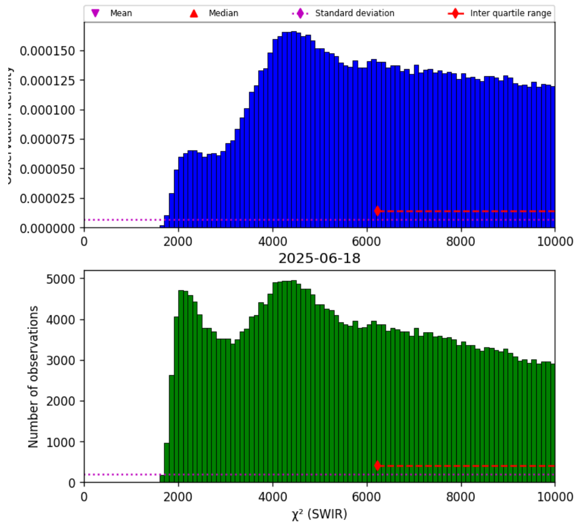
Figure 28: Histogram of “ \chi^2 (SWIR)” for 2025-06-17 to 2025-06-19
