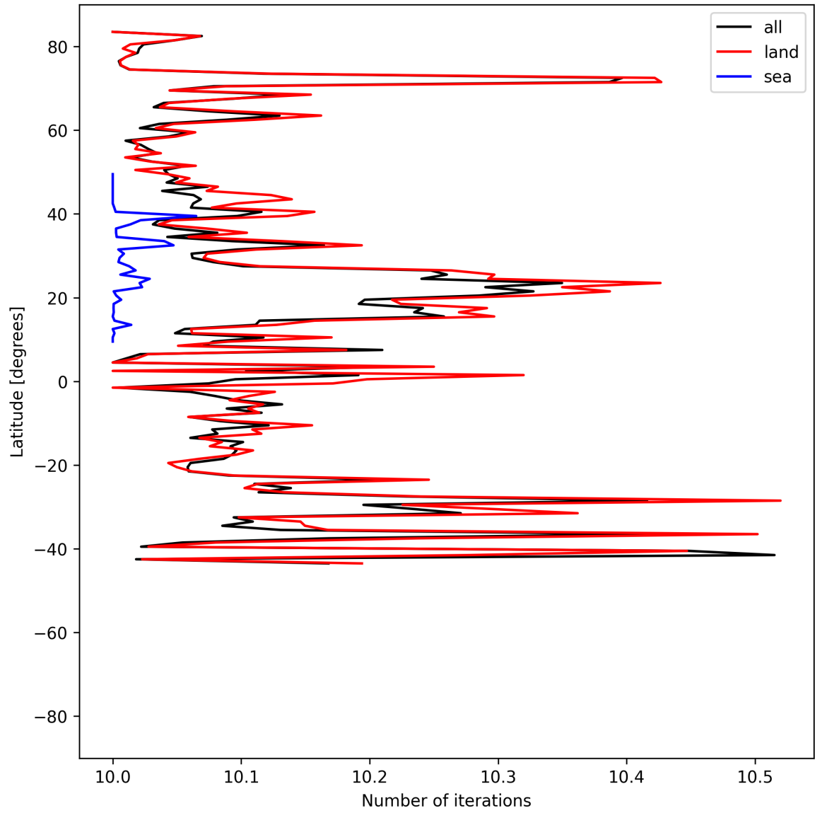
Figure 20: Zonal average of “Number of iterations” for 2025-06-17 to 2025-06-19.
