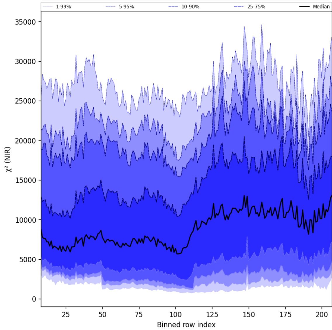
Figure 40: Along track statistics of " \chi^2 (NIR)" for 2025-06-17 to 2025-06-19
