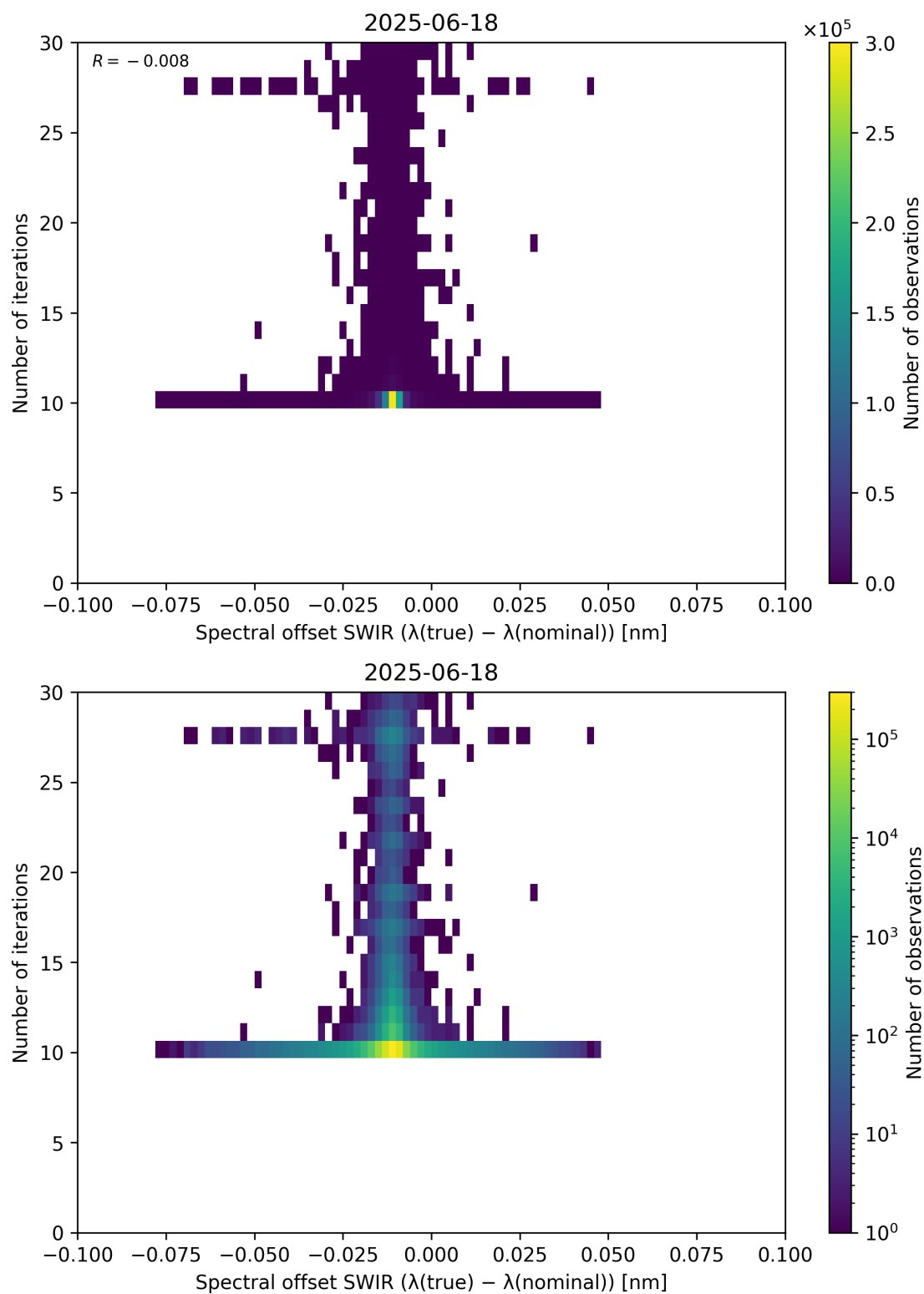
Figure 121: Scatter density plot of “Spectral offset SWIR ( \lambda_{\text{true}} - \lambda_{\text{nominal}} )” against “Number of iterations” for 2025-06-17 to 2025-06-19.
