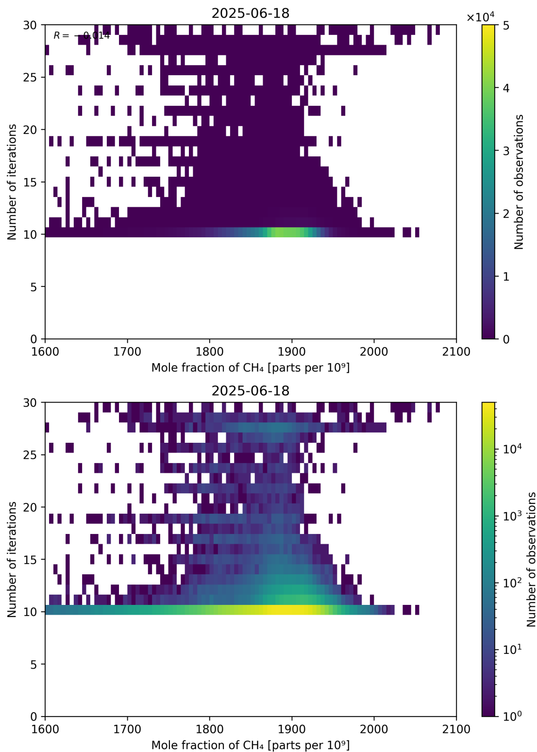
Figure 76: Scatter density plot of “Mole fraction of CH 4 ” against “Number of iterations” for 2025-06-17 to 2025-06-19.
