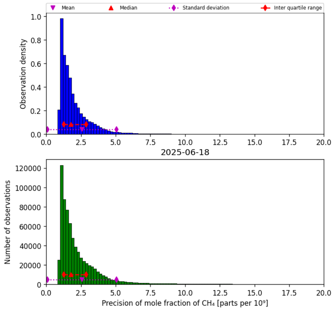
Figure 24: Histogram of “Precision of mole fraction of CH 4 ” for 2025-06-17 to 2025-06-19
