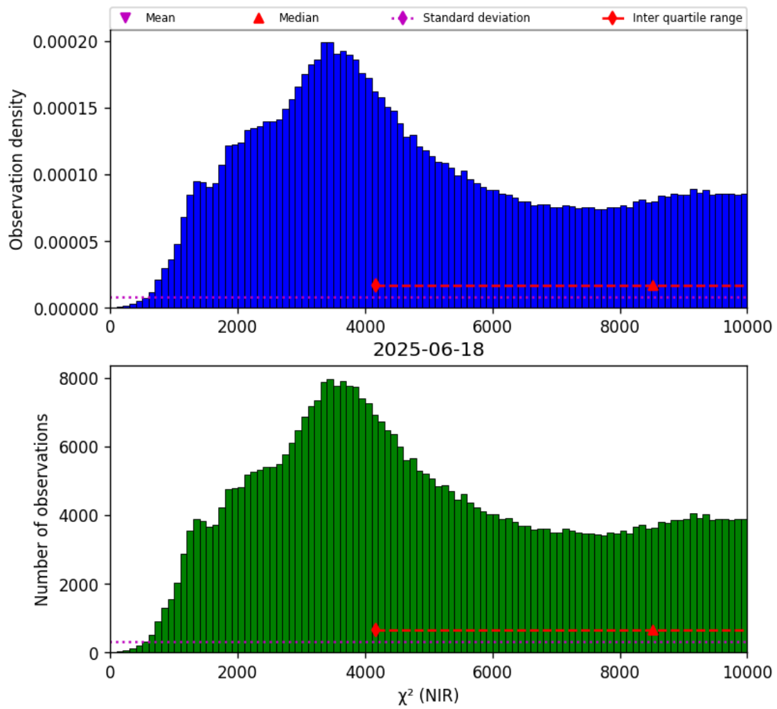
Figure 29: Histogram of “ \chi^2 (NIR)” for 2025-06-17 to 2025-06-19
