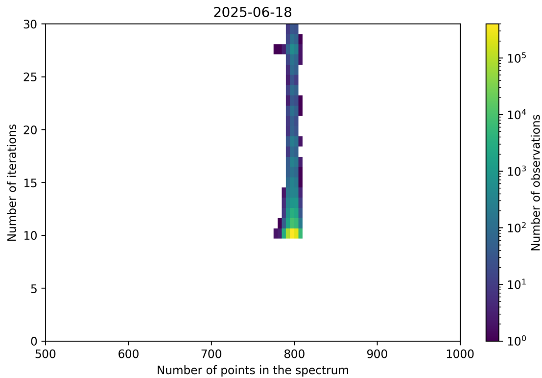
Figure 92: Scatter density plot of “Number of points in the spectrum” against “Number of iterations” for 2025-06-17 to 2025-06-19.
