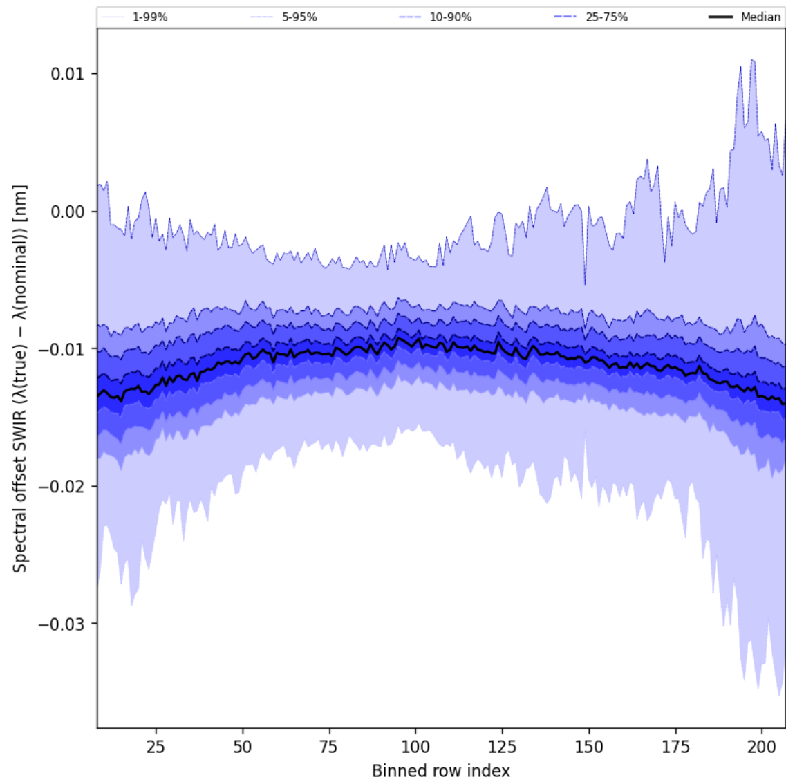
Figure 38: Along track statistics of “Spectral offset SWIR ( \lambda_{\text{true}} - \lambda_{\text{nominal}} )” for 2025-06-17 to 2025-06-19
