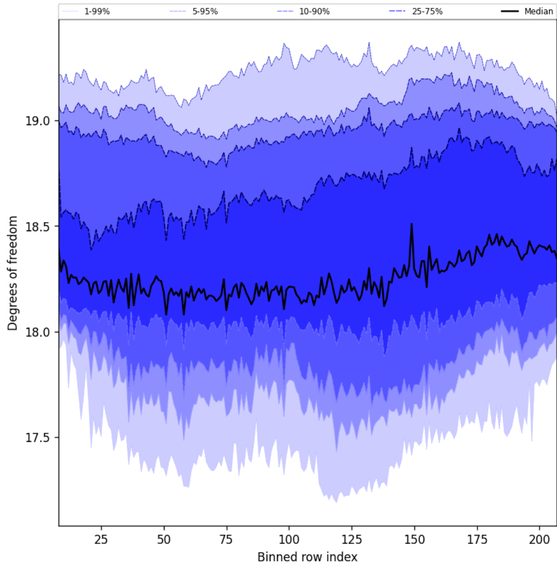
Figure 41: Along track statistics of “Degrees of freedom” for 2025-06-17 to 2025-06-19
