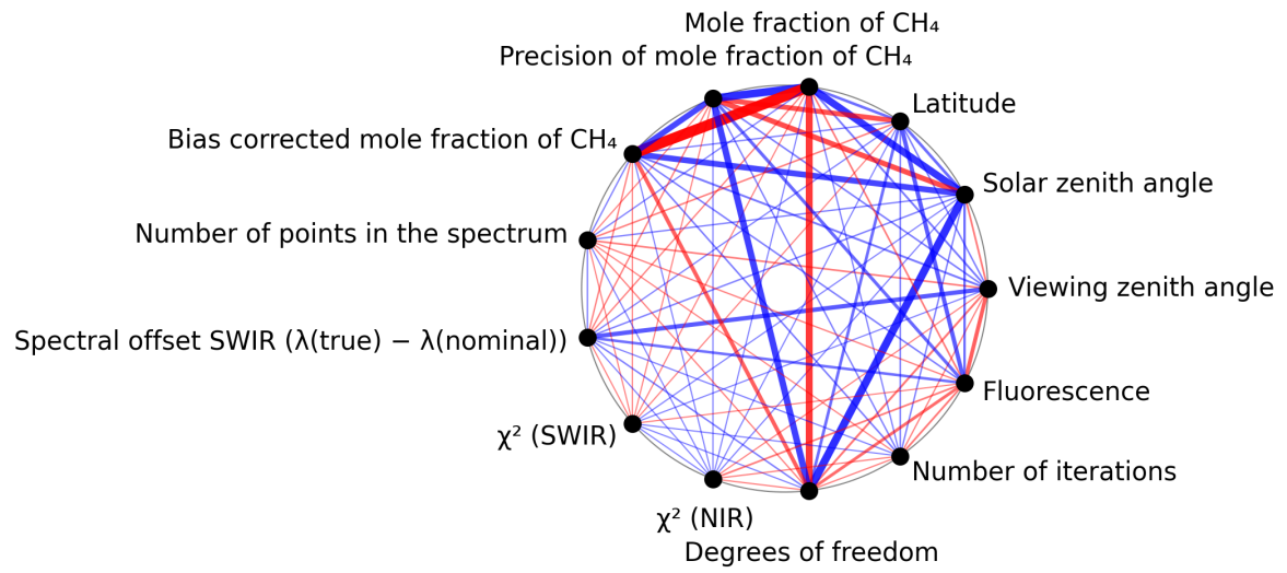
Figure 1: Map of correlation graph for 2025-06-17 to 2025-06-19.
