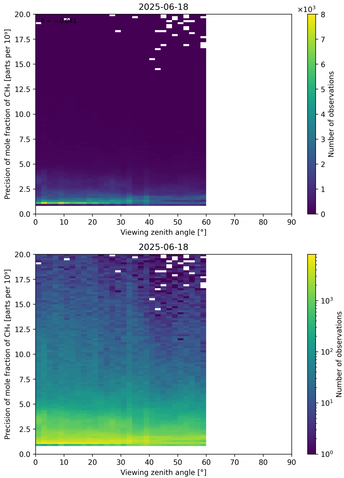
Figure 112: Scatter density plot of “Viewing zenith angle” against “Precision of mole fraction of CH 4 ” for 2025-06-17 to 2025-06-19.
