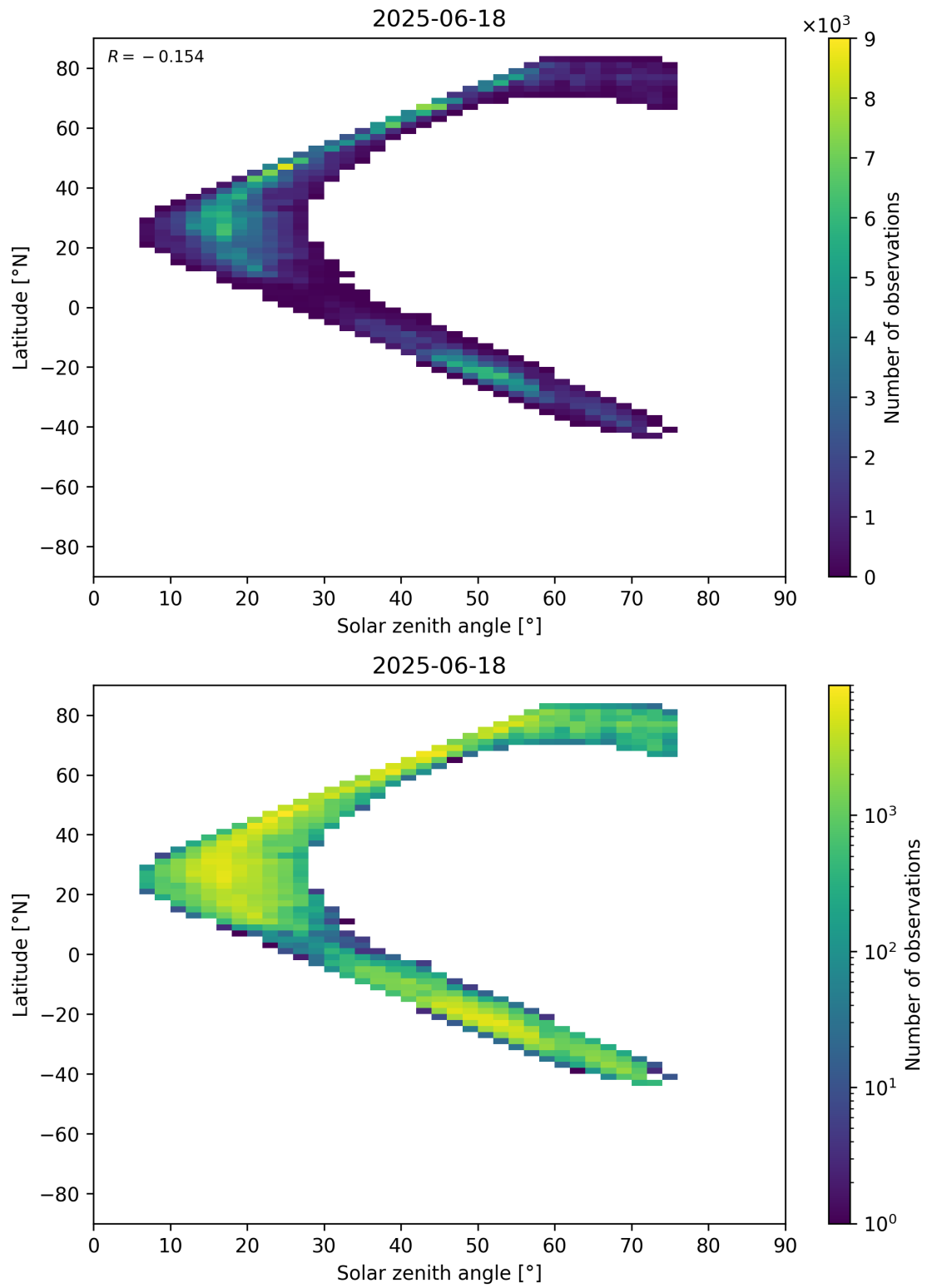
Figure 98: Scatter density plot of “Solar zenith angle” against “Latitude” for 2025-06-17 to 2025-06-19.
