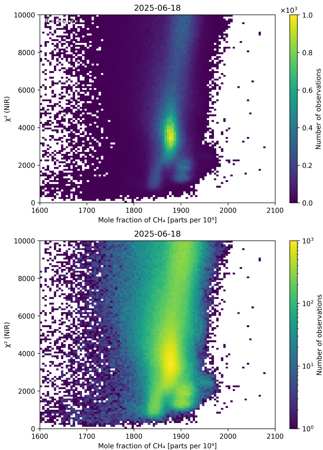
Figure 70: Scatter density plot of “Mole fraction of \text{CH}_4 ” against “ \chi^2 (NIR)” for 2025-06-17 to 2025-06-19.
