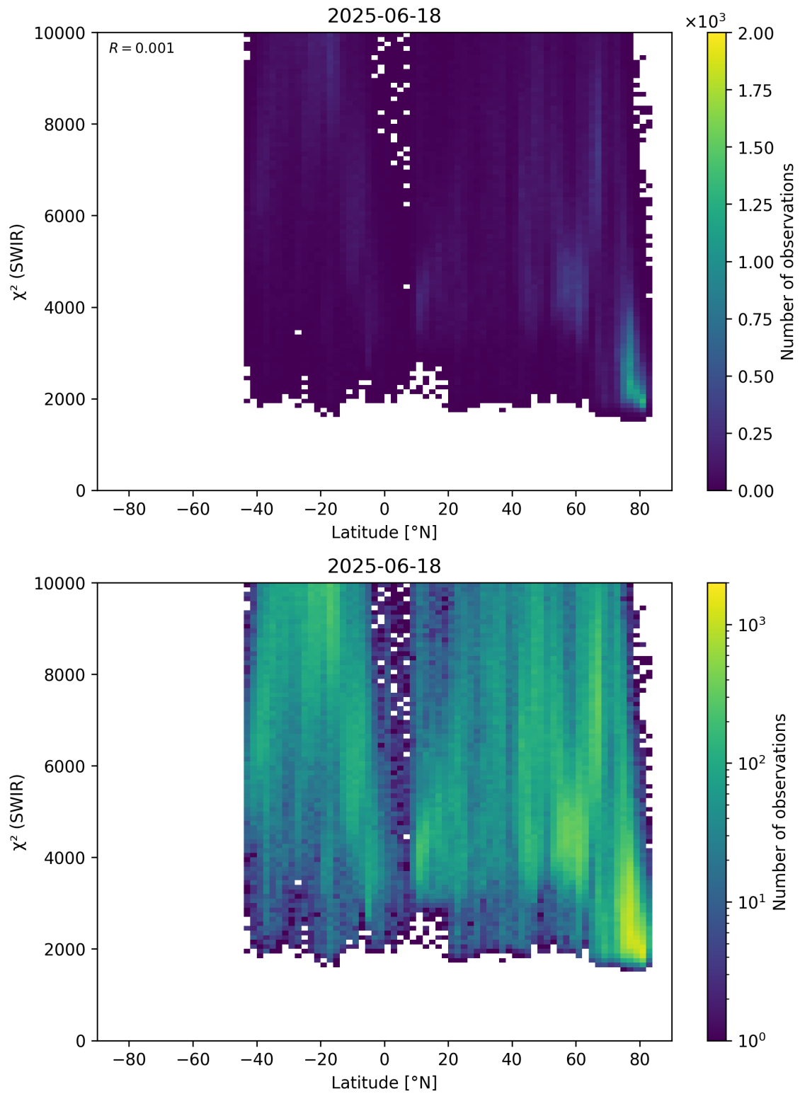
Figure 54: Scatter density plot of “Latitude” against “ \chi^2 (SWIR)” for 2025-06-17 to 2025-06-19.
