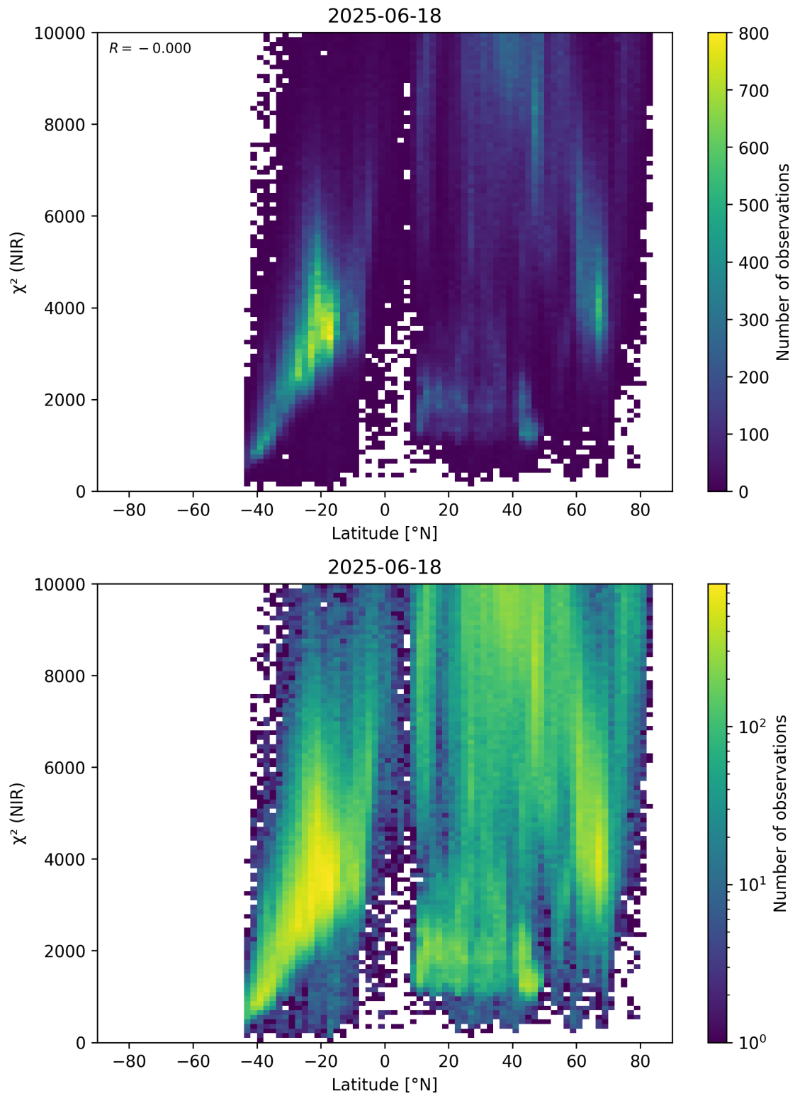
Figure 53: Scatter density plot of “Latitude” against “ \chi^2 (NIR)” for 2025-06-17 to 2025-06-19.
