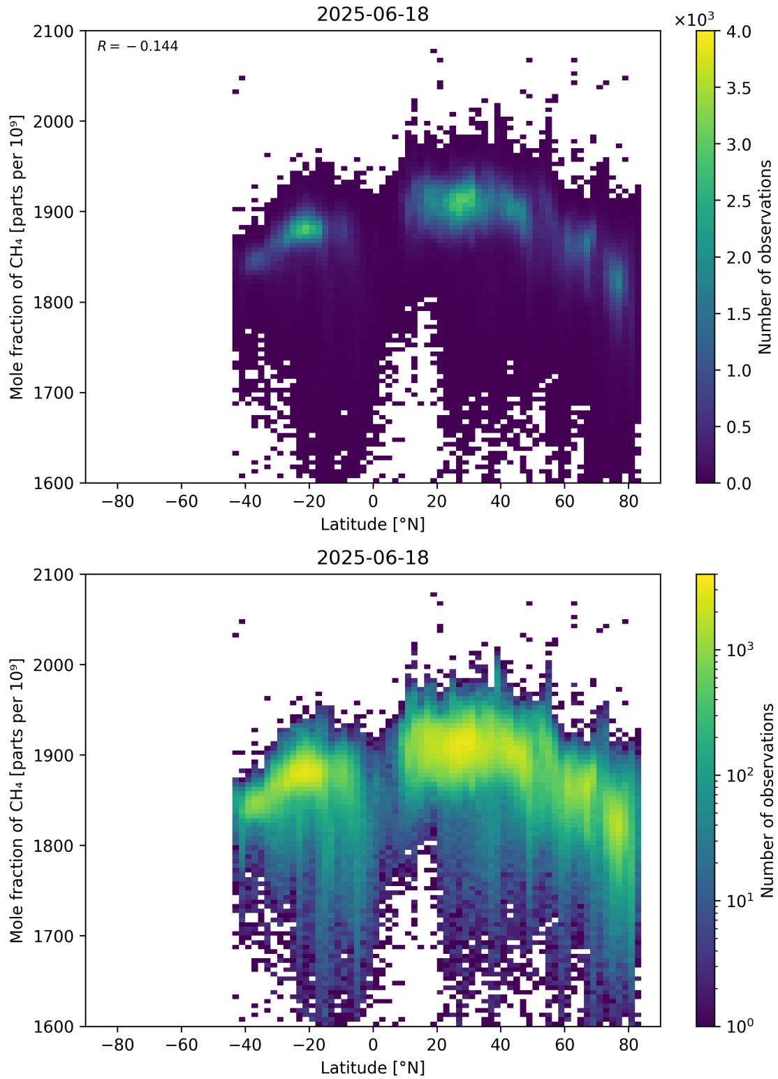
Figure 57: Scatter density plot of “Latitude” against “Mole fraction of CH 4 ” for 2025-06-17 to 2025-06-19.
