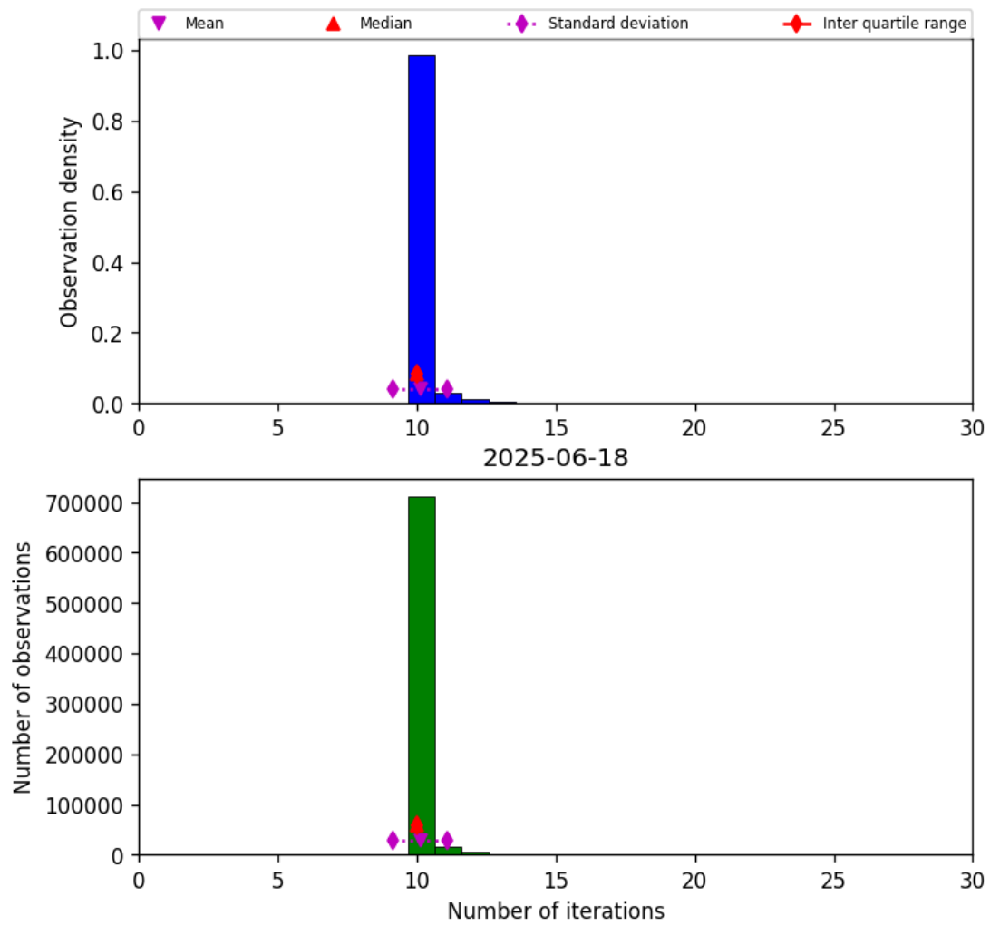
Figure 31: Histogram of “Number of iterations” for 2025-06-17 to 2025-06-19
