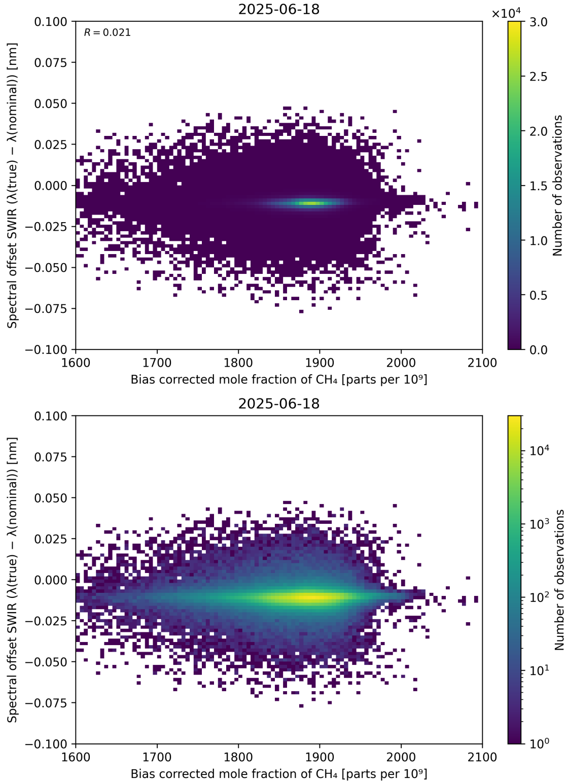
Figure 69: Scatter density plot of “Bias corrected mole fraction of \text{CH}_4 ” against “Spectral offset SWIR ( \lambda_{\text{true}} - \lambda_{\text{nominal}} )” for 2025-06-17 to 2025-06-19.
