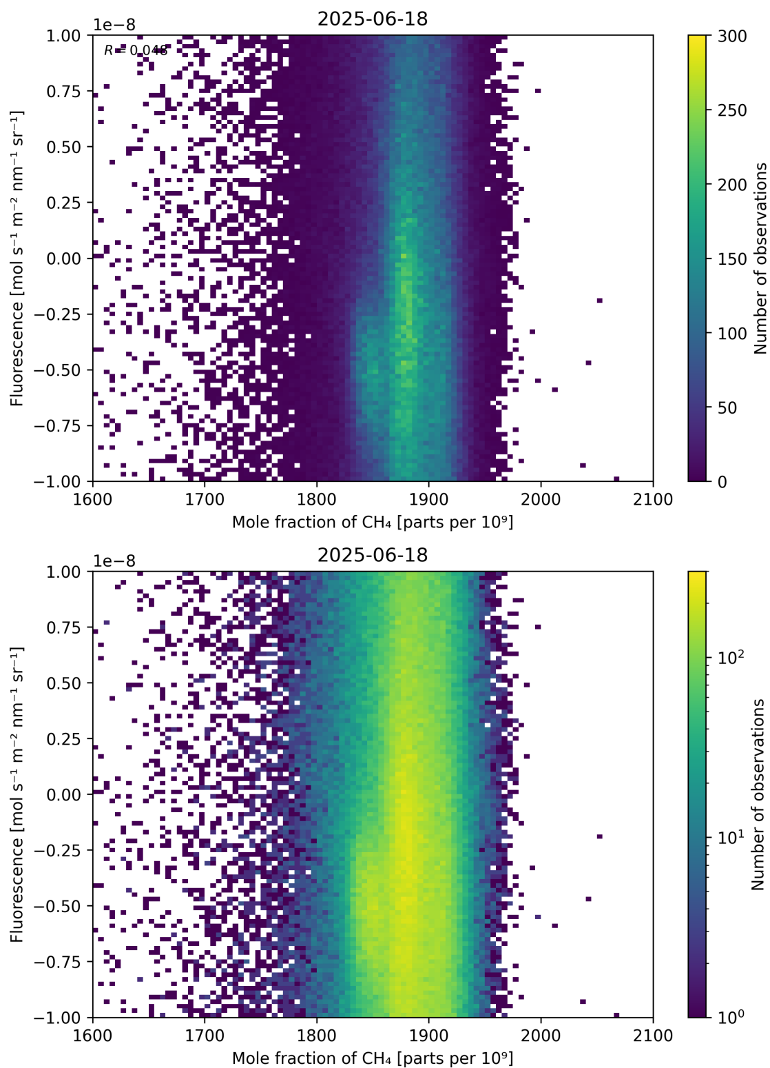
Figure 73: Scatter density plot of “Mole fraction of \text{CH}_4 ” against “Fluorescence” for 2025-06-17 to 2025-06-19.
