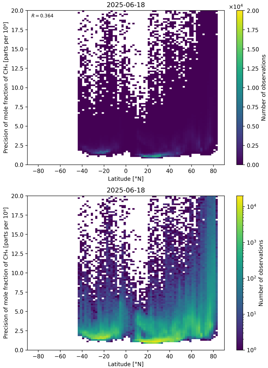
Figure 59: Scatter density plot of “Latitude” against “Precision of mole fraction of \text{CH}_4 ” for 2025-06-17 to 2025-06-19.
