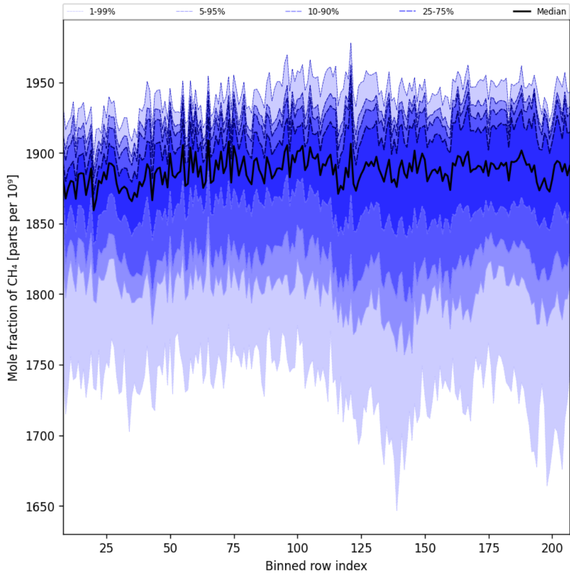
Figure 34: Along track statistics of “Mole fraction of CH 4 ” for 2025-06-17 to 2025-06-19
