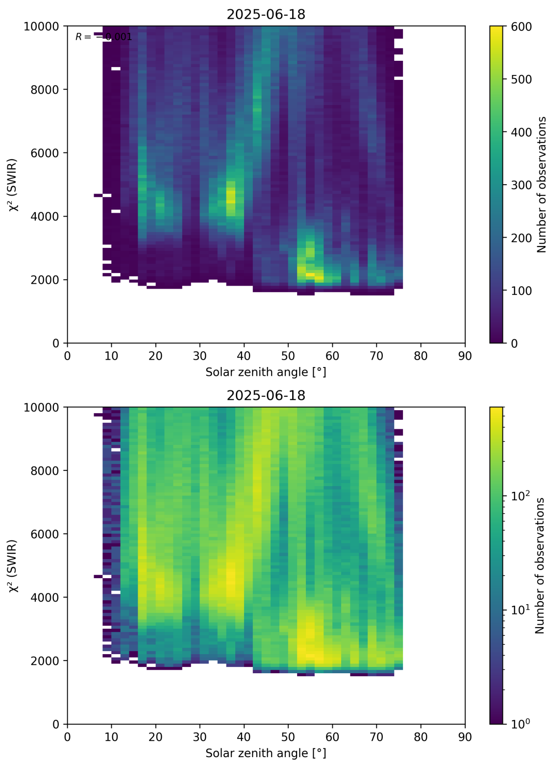
Figure 95: Scatter density plot of “Solar zenith angle” against “ \chi^2 (SWIR)” for 2025-06-17 to 2025-06-19.
