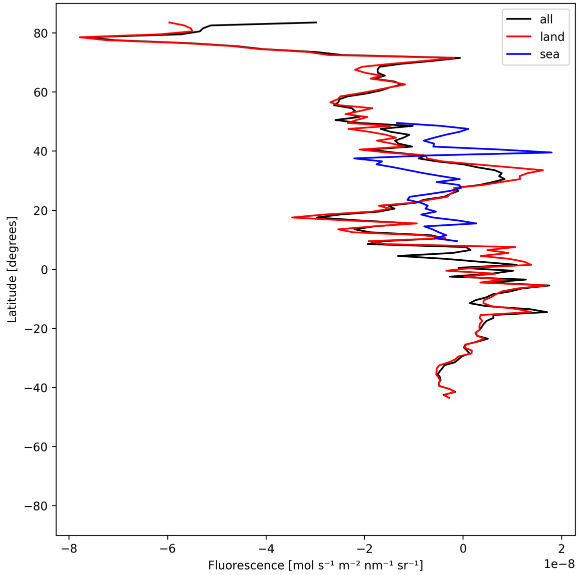
Figure 21: Zonal average of “Fluorescence” for 2025-06-17 to 2025-06-19.
