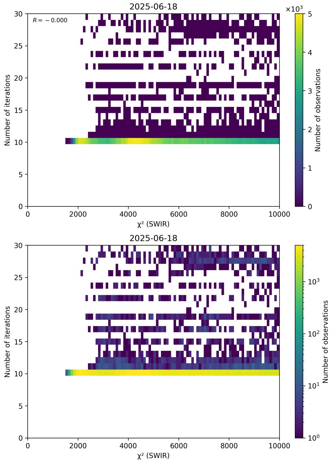
Figure 50: Scatter density plot of “ \chi^2 (SWIR)” against “Number of iterations” for 2025-06-17 to 2025-06-19.
