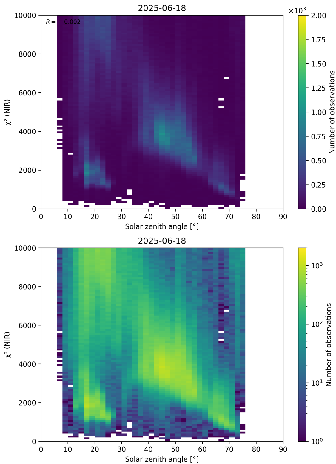
Figure 94: Scatter density plot of “Solar zenith angle” against “ \chi^2 (NIR)” for 2025-06-17 to 2025-06-19.
