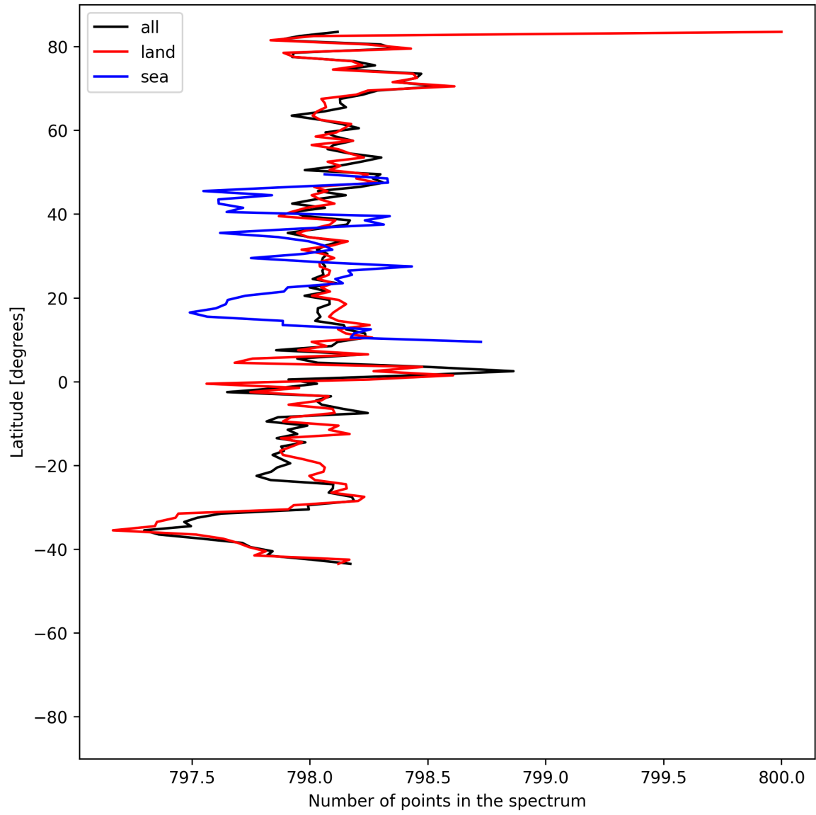
Figure 15: Zonal average of “Number of points in the spectrum” for 2025-06-17 to 2025-06-19.
