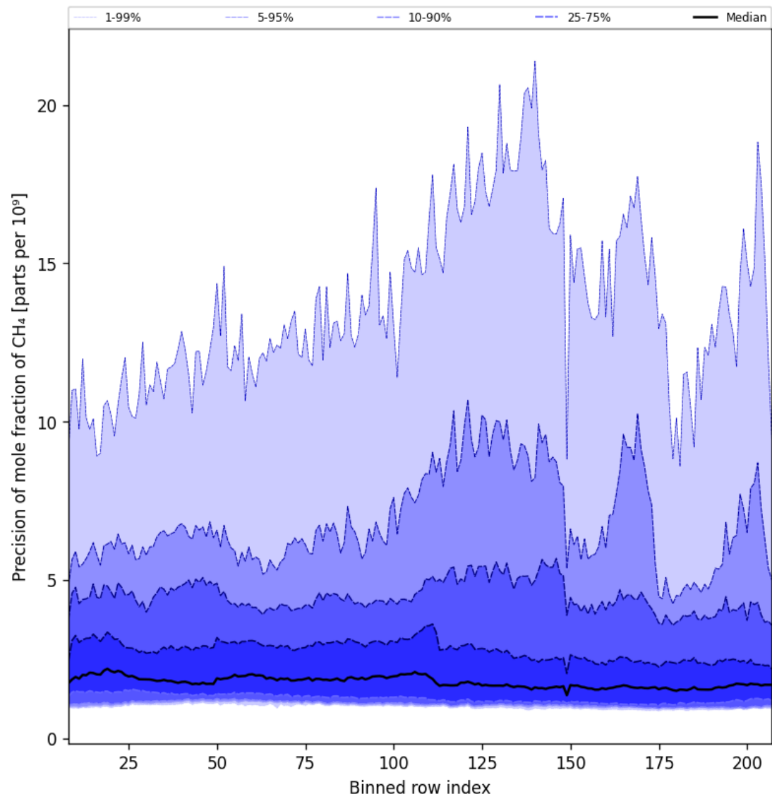
Figure 35: Along track statistics of “Precision of mole fraction of CH 4 ” for 2025-06-17 to 2025-06-19
