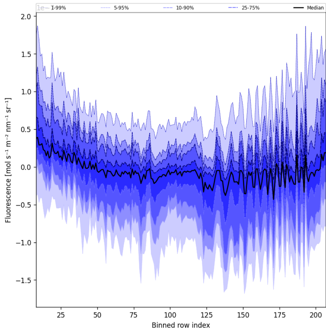
Figure 43: Along track statistics of “Fluorescence” for 2025-06-17 to 2025-06-19
