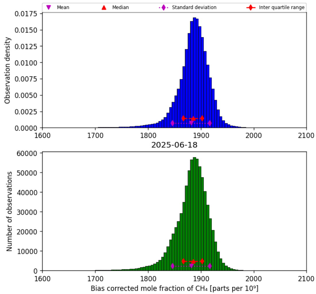
Figure 25: Histogram of “Bias corrected mole fraction of CH 4 ” for 2025-06-17 to 2025-06-19
