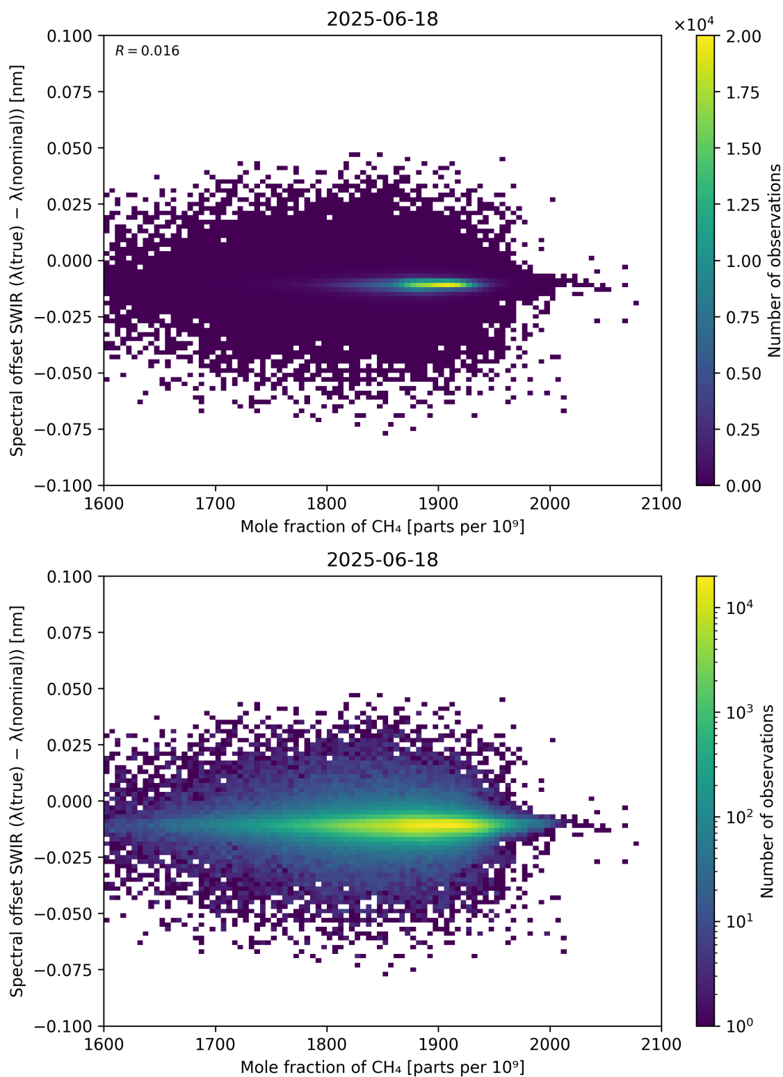
Figure 86: Scatter density plot of “Mole fraction of CH 4 ” against “Spectral offset SWIR ( \lambda_{\text{true}} - \lambda_{\text{nominal}} )” for 2025-06-17 to 2025-06-19.
