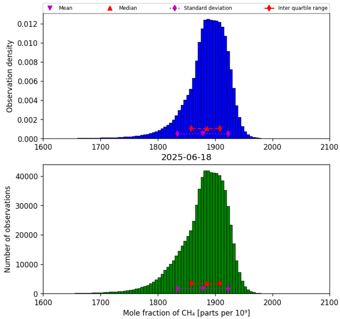
Figure 23: Histogram of “Mole fraction of CH 4 ” for 2025-06-17 to 2025-06-19
