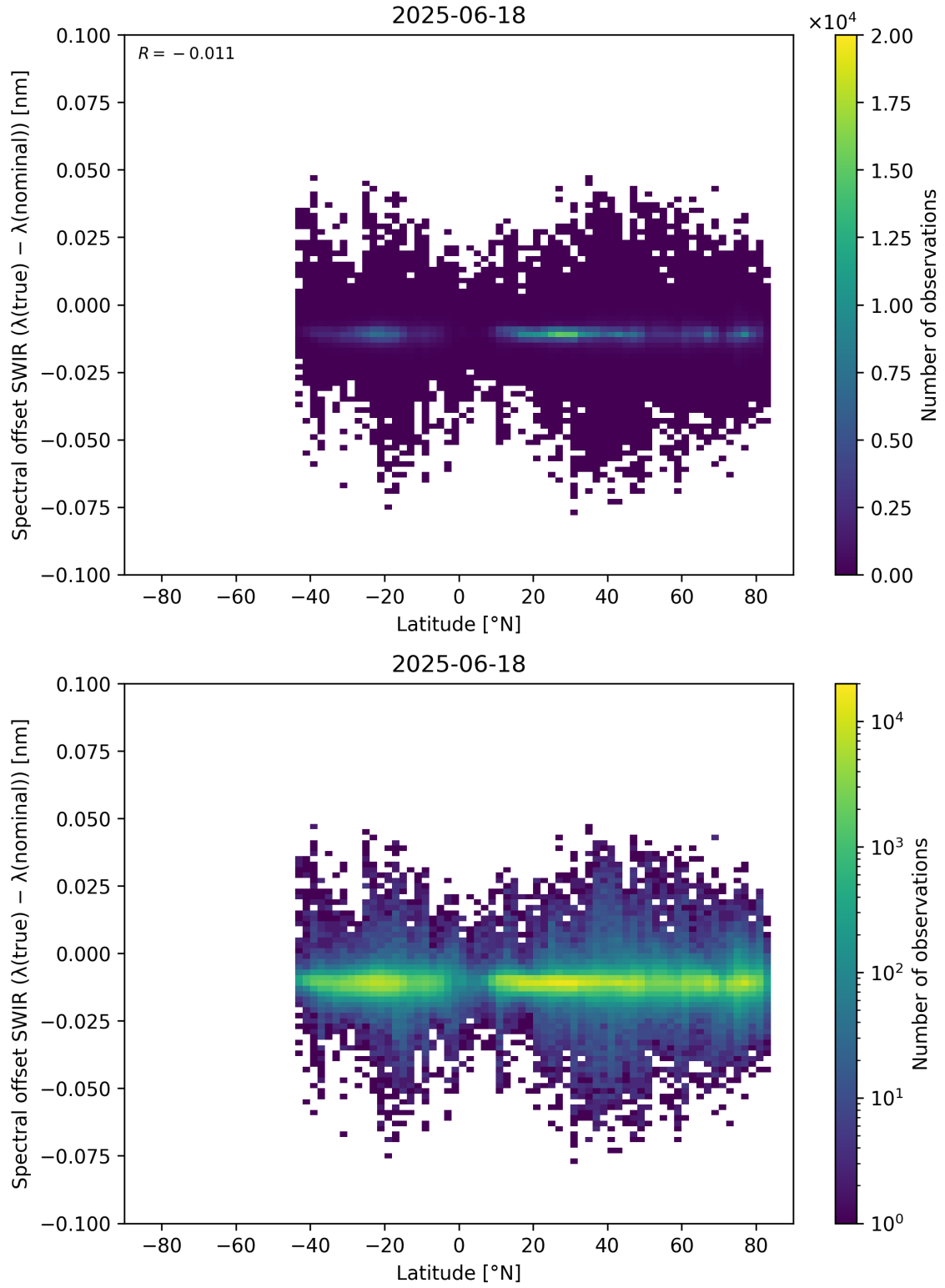
Figure 62: Scatter density plot of “Latitude” against “Spectral offset SWIR ( \lambda_{\text{true}} - \lambda_{\text{nominal}} )” for 2025-06-17 to 2025-06-19.
