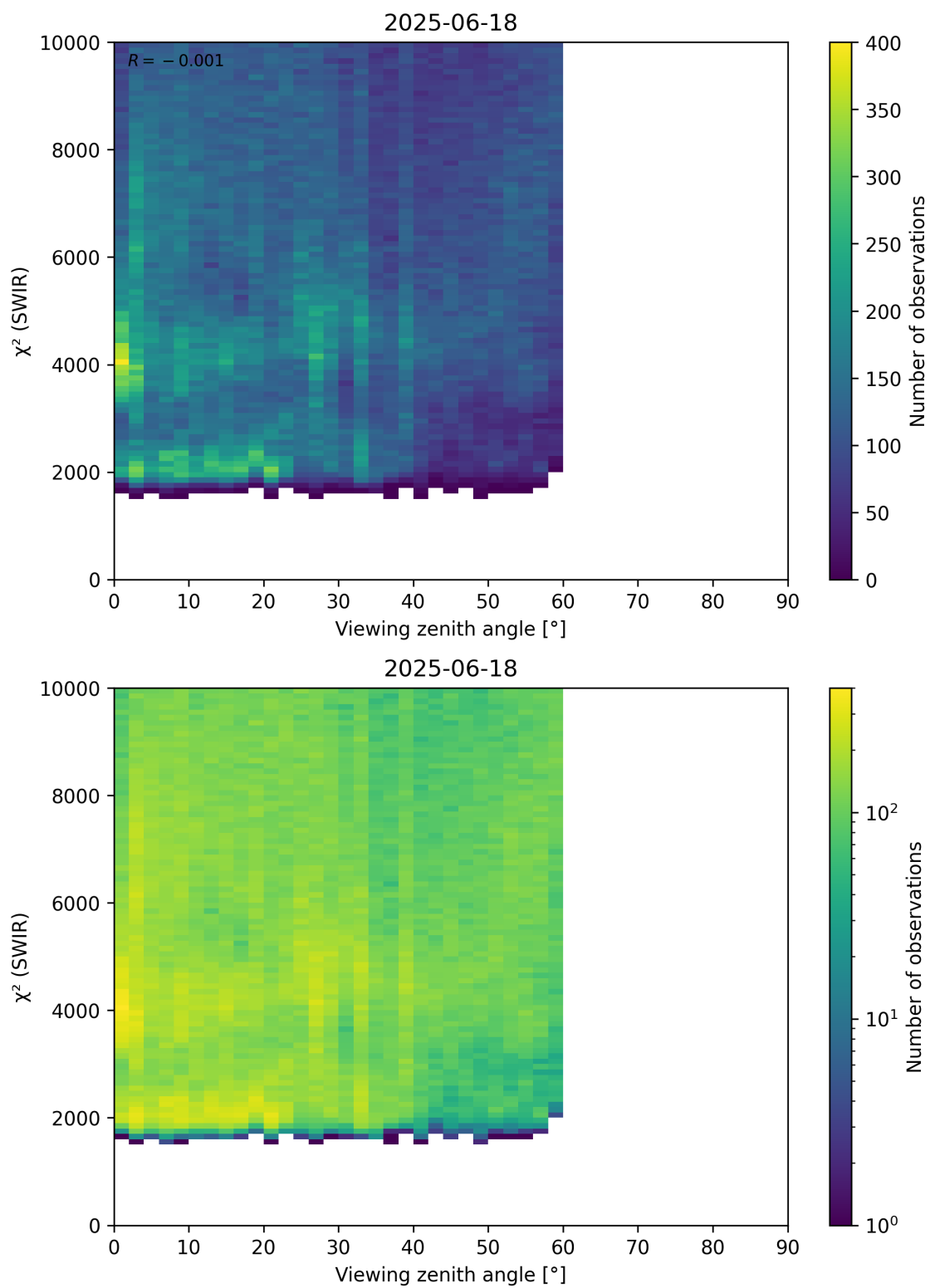
Figure 106: Scatter density plot of “Viewing zenith angle” against “ \chi^2 (SWIR)” for 2025-06-17 to 2025-06-19.
