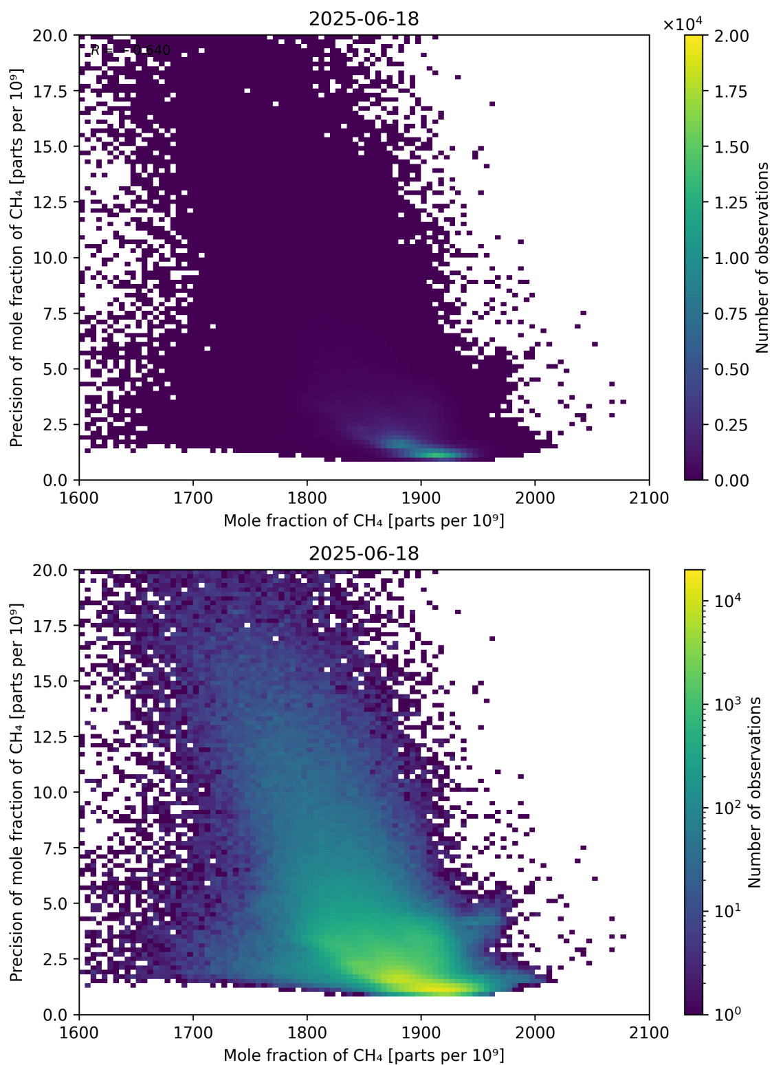
Figure 75: Scatter density plot of “Mole fraction of CH 4 ” against “Precision of mole fraction of CH 4 ” for 2025-06-17 to 2025-06-19.
