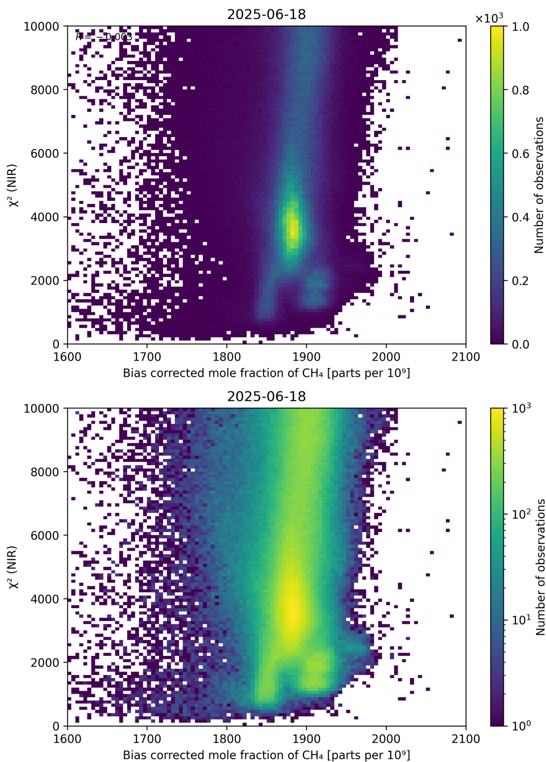
Figure 63: Scatter density plot of “Bias corrected mole fraction of \text{CH}_4 ” against “ \chi^2 (NIR)” for 2025-06-17 to 2025-06-19.
