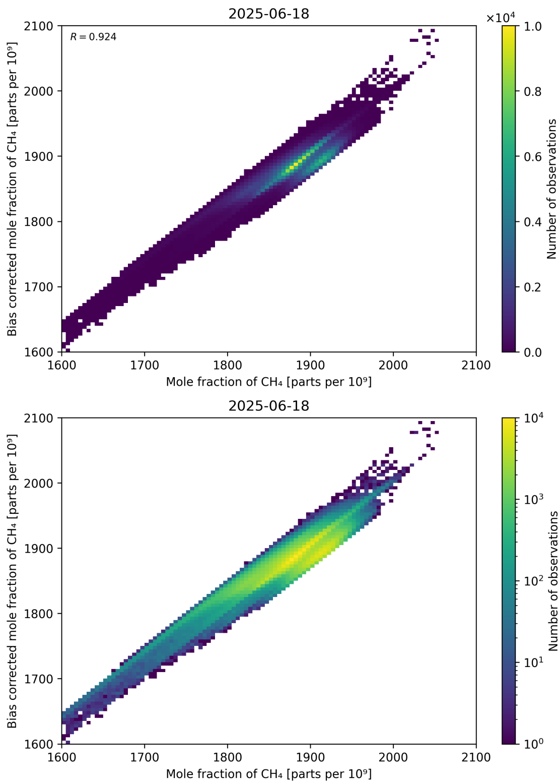
Figure 74: Scatter density plot of “Mole fraction of CH 4 ” against “Bias corrected mole fraction of CH 4 ” for 2025-06-17 to 2025-06-19.
