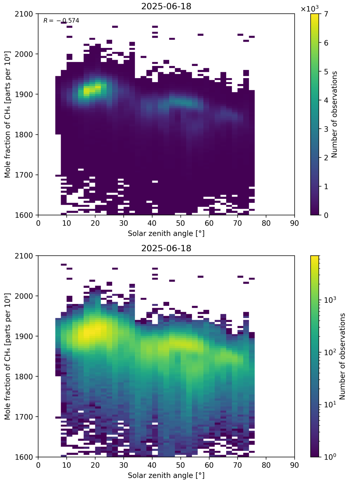
Figure 99: Scatter density plot of “Solar zenith angle” against “Mole fraction of CH 4 ” for 2025-06-17 to 2025-06-19.
