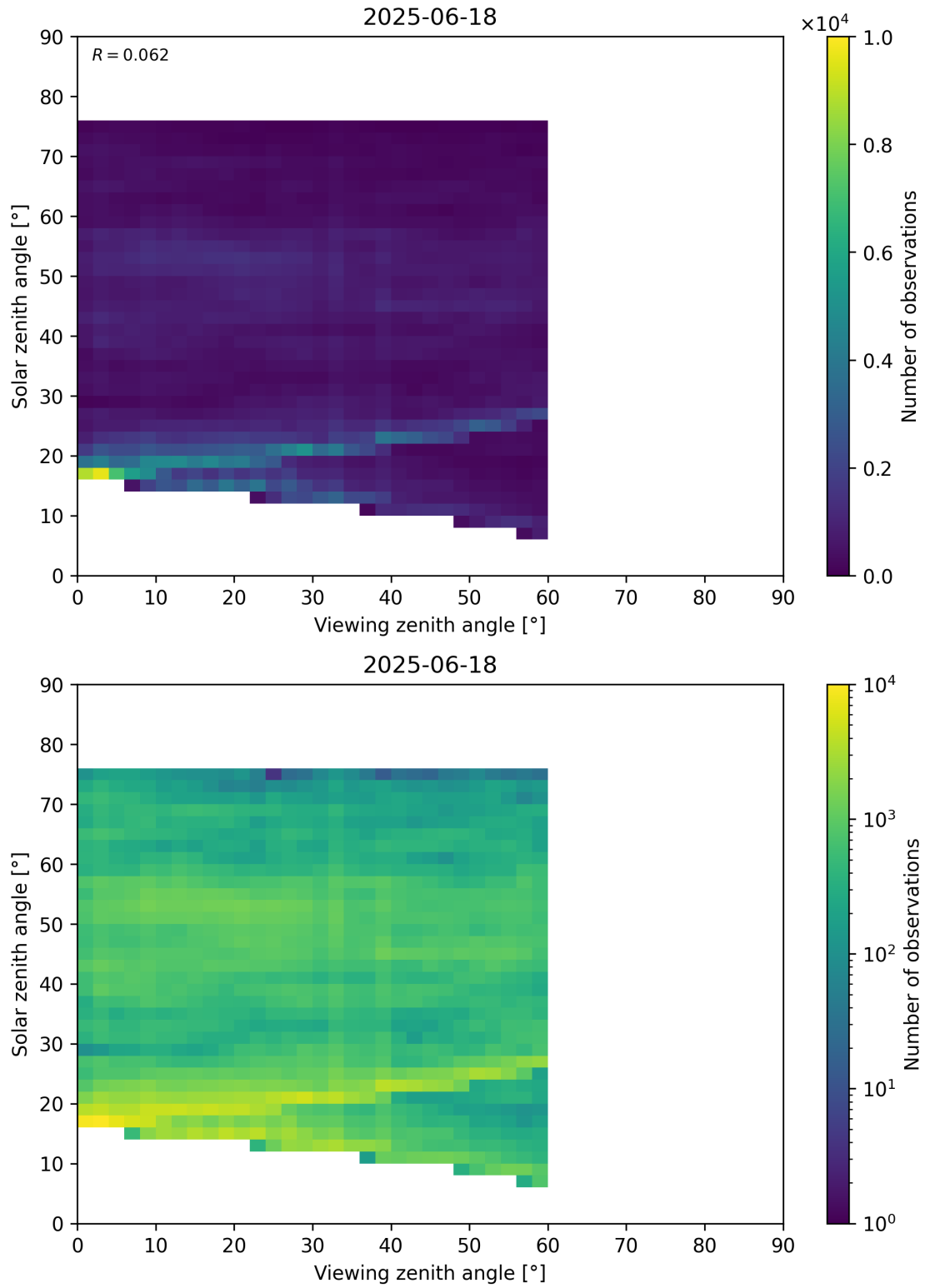
Figure 115: Scatter density plot of “Viewing zenith angle” against “Solar zenith angle” for 2025-06-17 to 2025-06-19.
