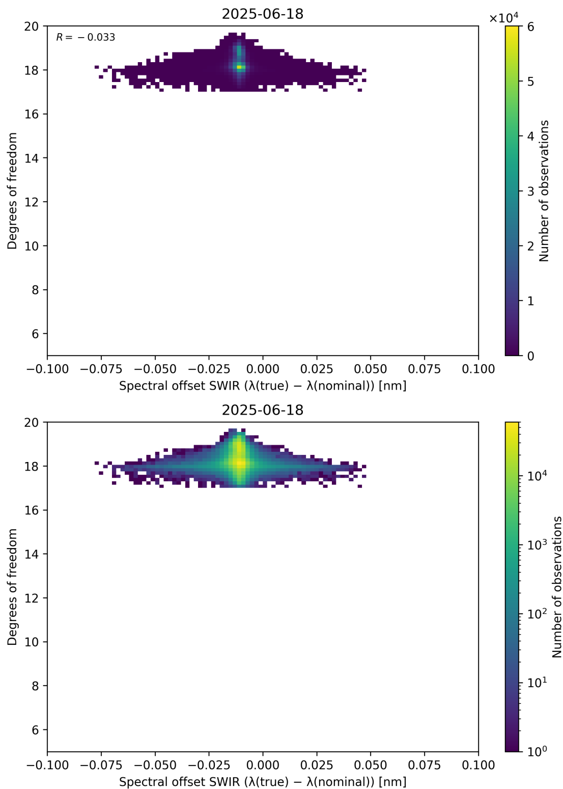
Figure 119: Scatter density plot of “Spectral offset SWIR ( \lambda_{\text{true}} - \lambda_{\text{nominal}} )” against “Degrees of freedom” for 2025-06-17 to 2025-06-19.
