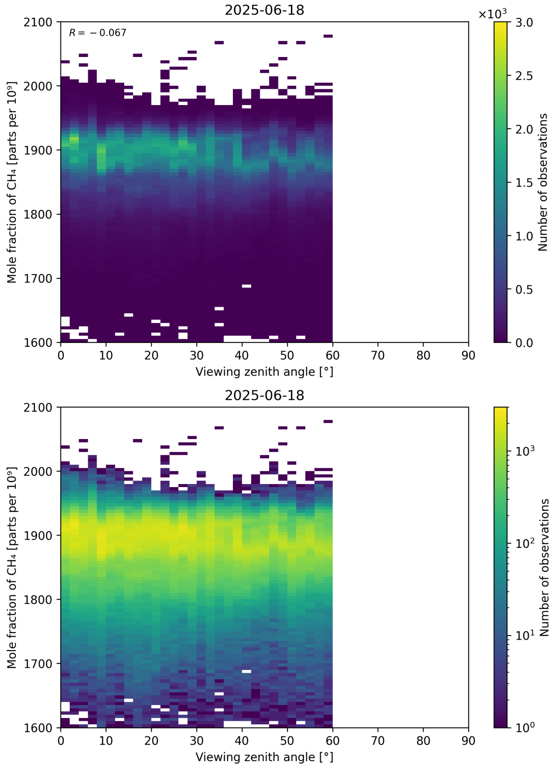
Figure 110: Scatter density plot of “Viewing zenith angle” against “Mole fraction of CH 4 ” for 2025-06-17 to 2025-06-19.
