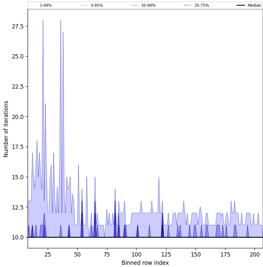
Figure 42: Along track statistics of “Number of iterations” for 2025-06-17 to 2025-06-19
