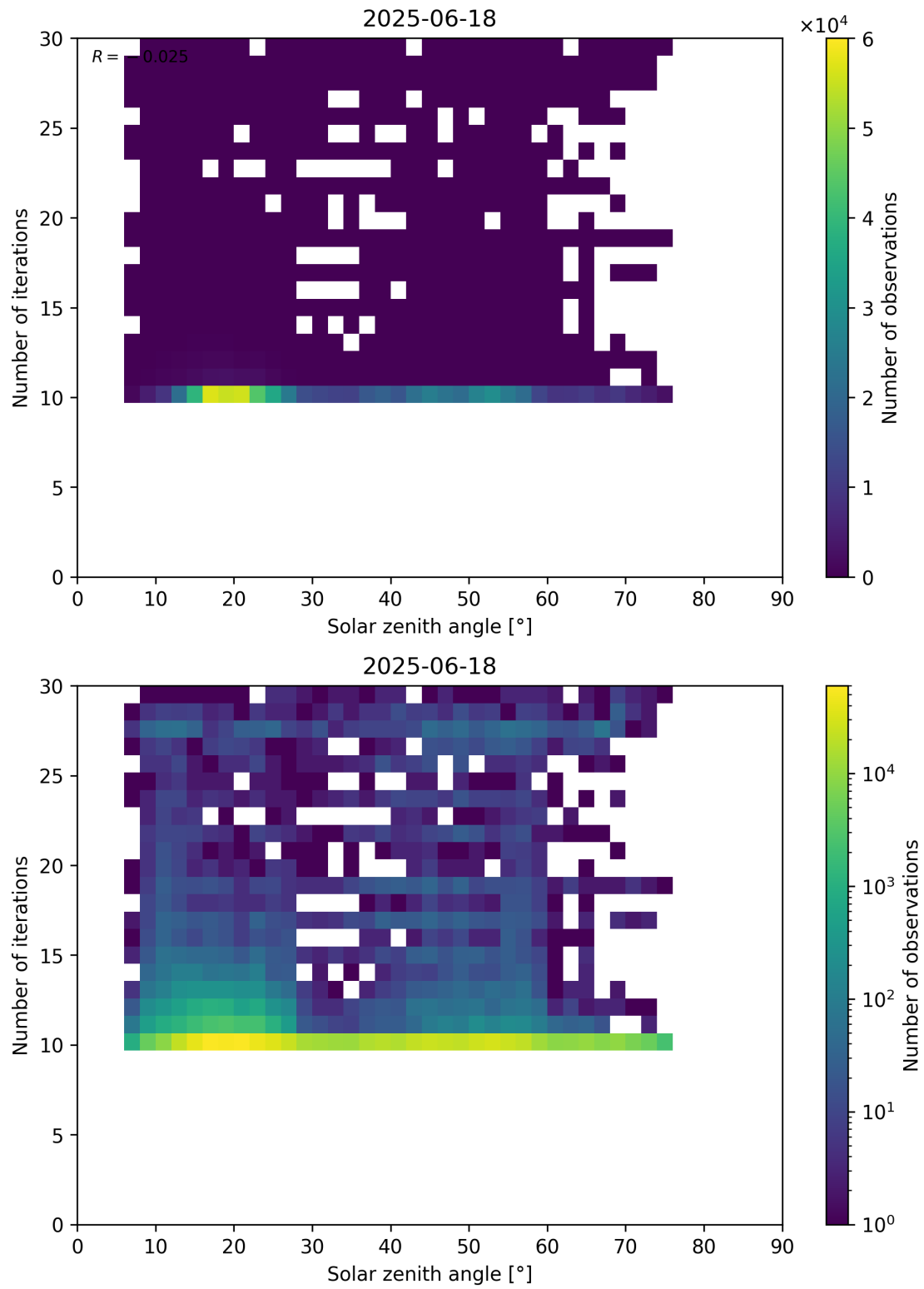
Figure 102: Scatter density plot of “Solar zenith angle” against “Number of iterations” for 2025-06-17 to 2025-06-19.
