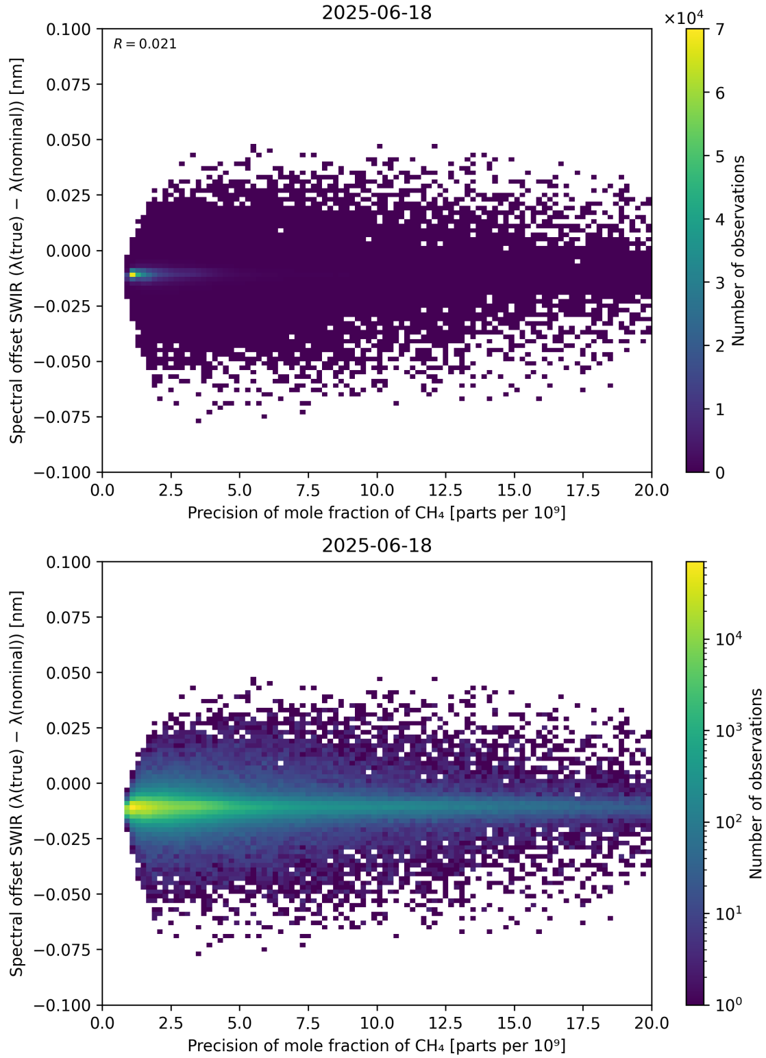
Figure 85: Scatter density plot of “Precision of mole fraction of CH 4 ” against “Spectral offset SWIR ( \lambda_{\text{true}} - \lambda_{\text{nominal}} )” for 2025-06-17 to 2025-06-19.
