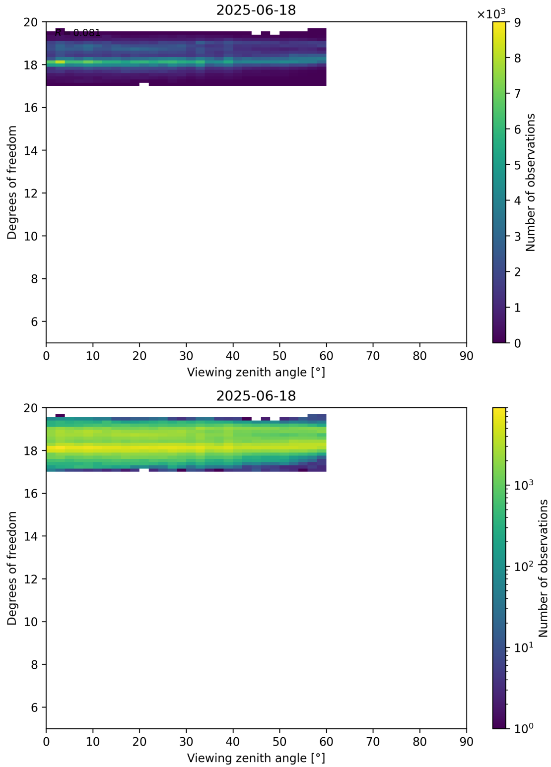
Figure 107: Scatter density plot of “Viewing zenith angle” against “Degrees of freedom” for 2025-06-17 to 2025-06-19.
