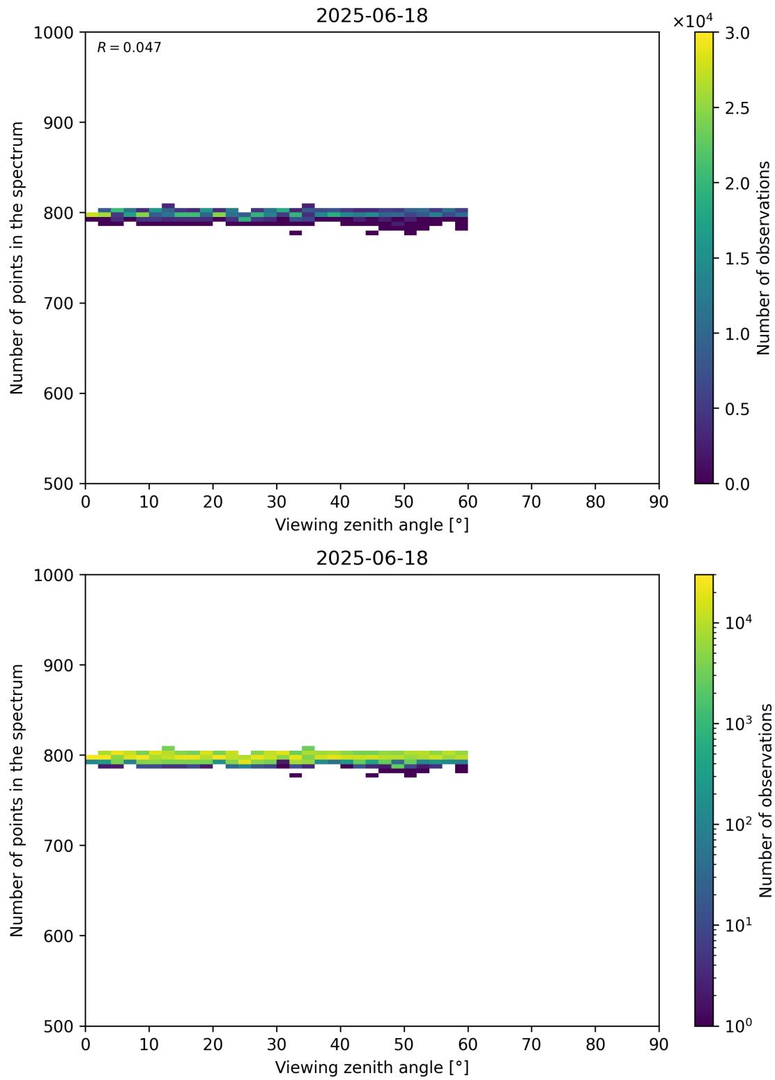
Figure 114: Scatter density plot of “Viewing zenith angle” against “Number of points in the spectrum” for 2025-06-17 to 2025-06-19.
