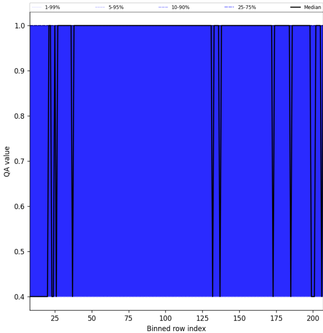
Figure 33: Along track statistics of “QA value” for 2025-06-17 to 2025-06-19
