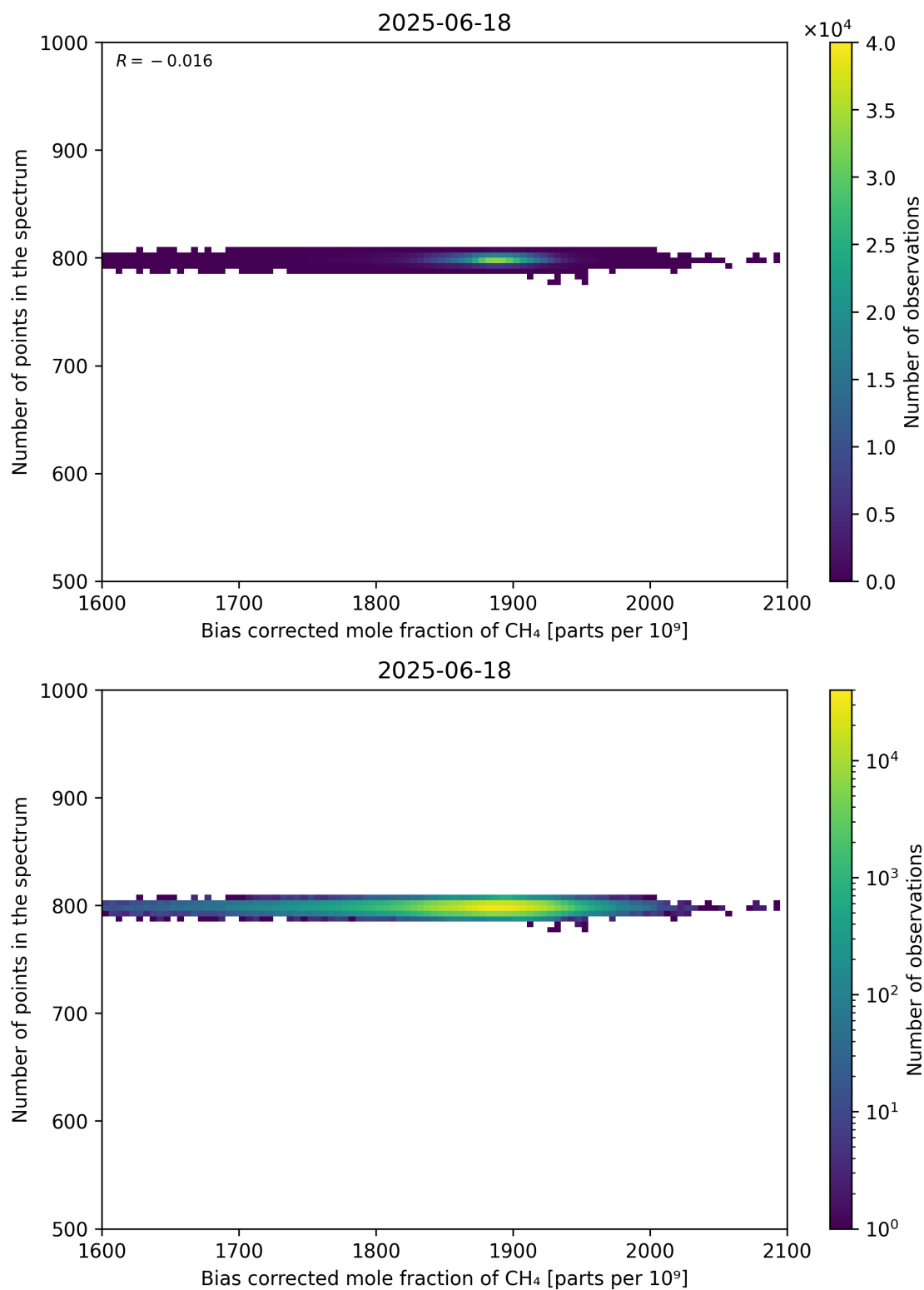
Figure 68: Scatter density plot of “Bias corrected mole fraction of CH 4 ” against “Number of points in the spectrum” for 2025-06-17 to 2025-06-19.
