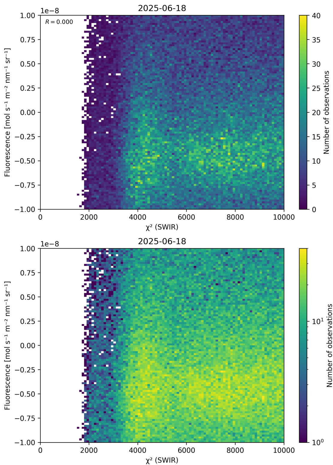
Figure 49: Scatter density plot of “ \chi^2 (SWIR)” against “Fluorescence” for 2025-06-17 to 2025-06-19.
