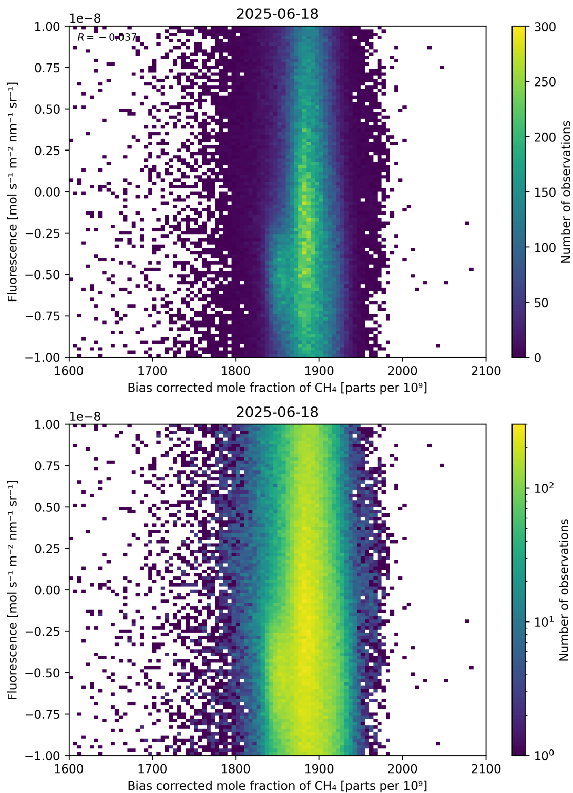
Figure 66: Scatter density plot of “Bias corrected mole fraction of \text{CH}_4 ” against “Fluorescence” for 2025-06-17 to 2025-06-19.
