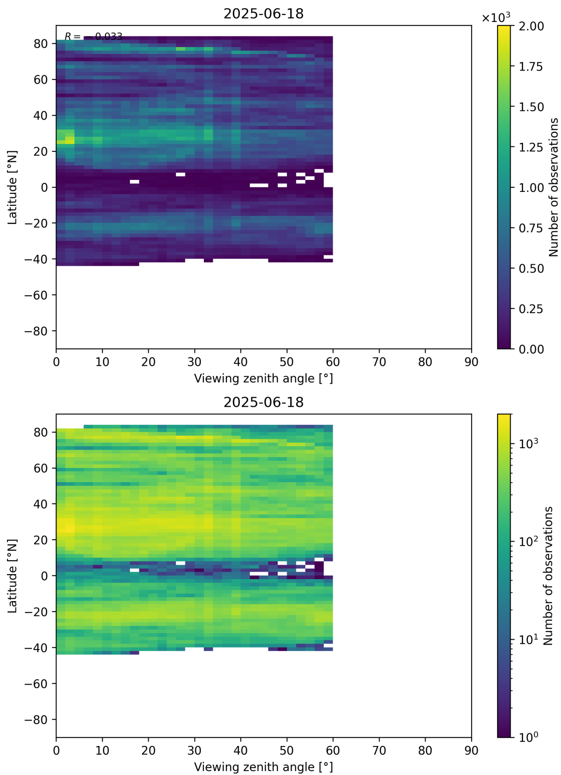
Figure 109: Scatter density plot of “Viewing zenith angle” against “Latitude” for 2025-06-17 to 2025-06-19.
