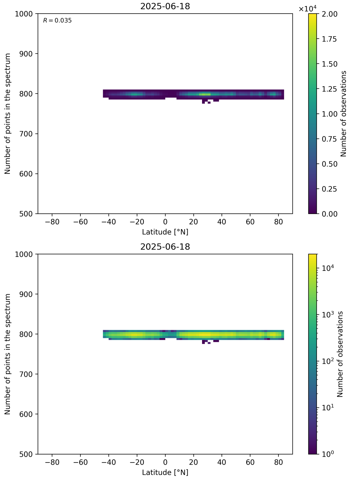
Figure 61: Scatter density plot of “Latitude” against “Number of points in the spectrum” for 2025-06-17 to 2025-06-19.
