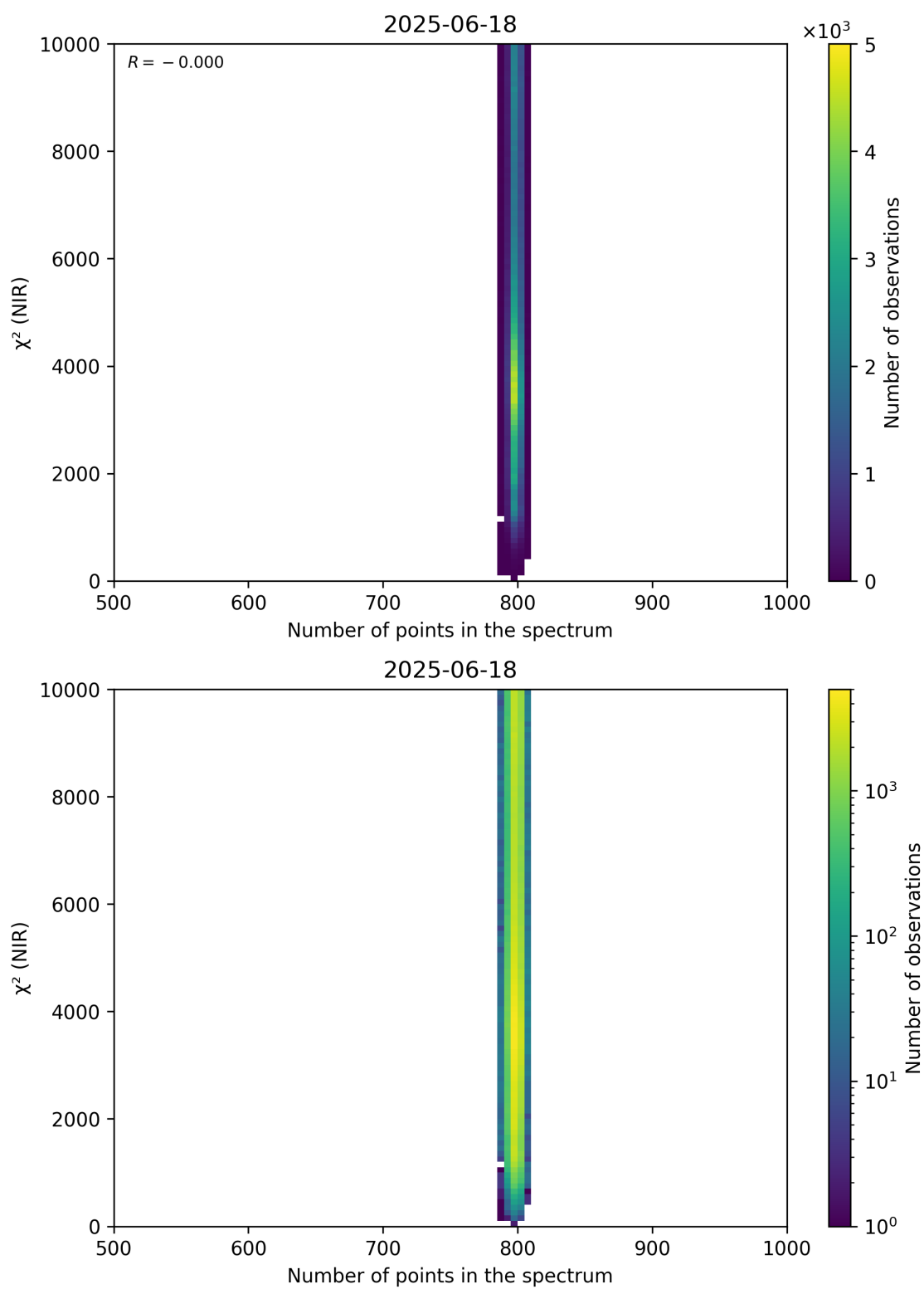
Figure 88: Scatter density plot of “Number of points in the spectrum” against “ \chi^2 (NIR)” for 2025-06-17 to 2025-06-19.
