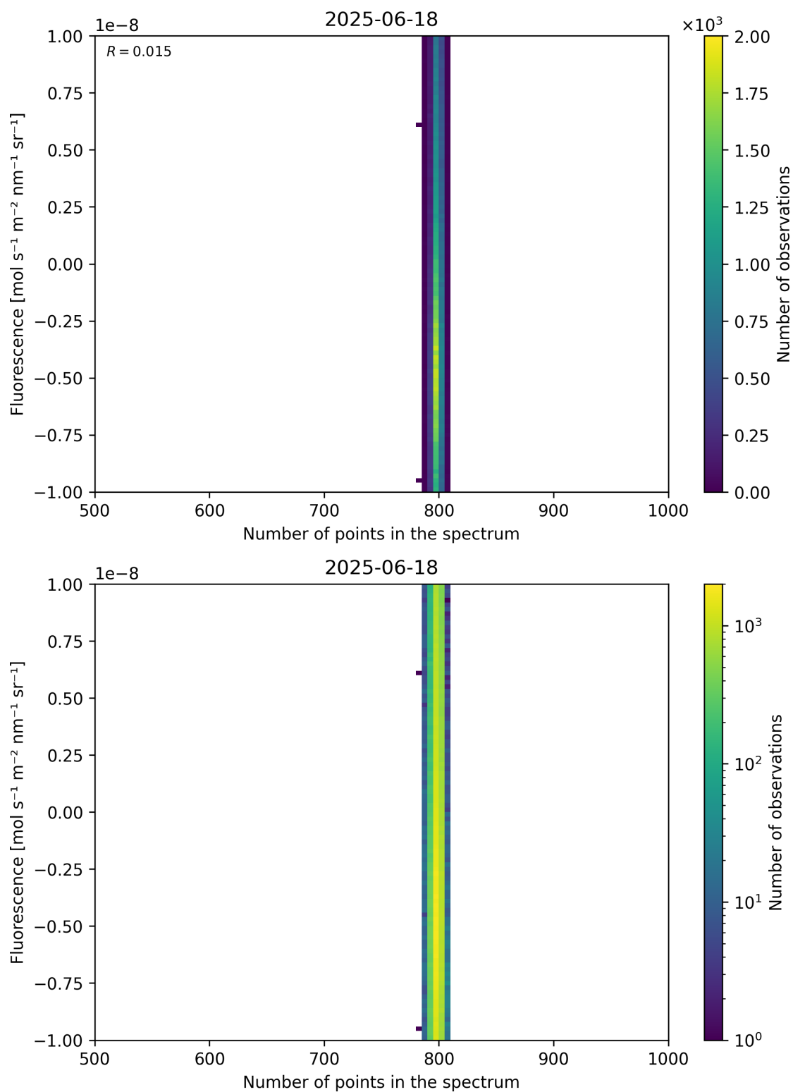
Figure 91: Scatter density plot of “Number of points in the spectrum” against “Fluorescence” for 2025-06-17 to 2025-06-19.
