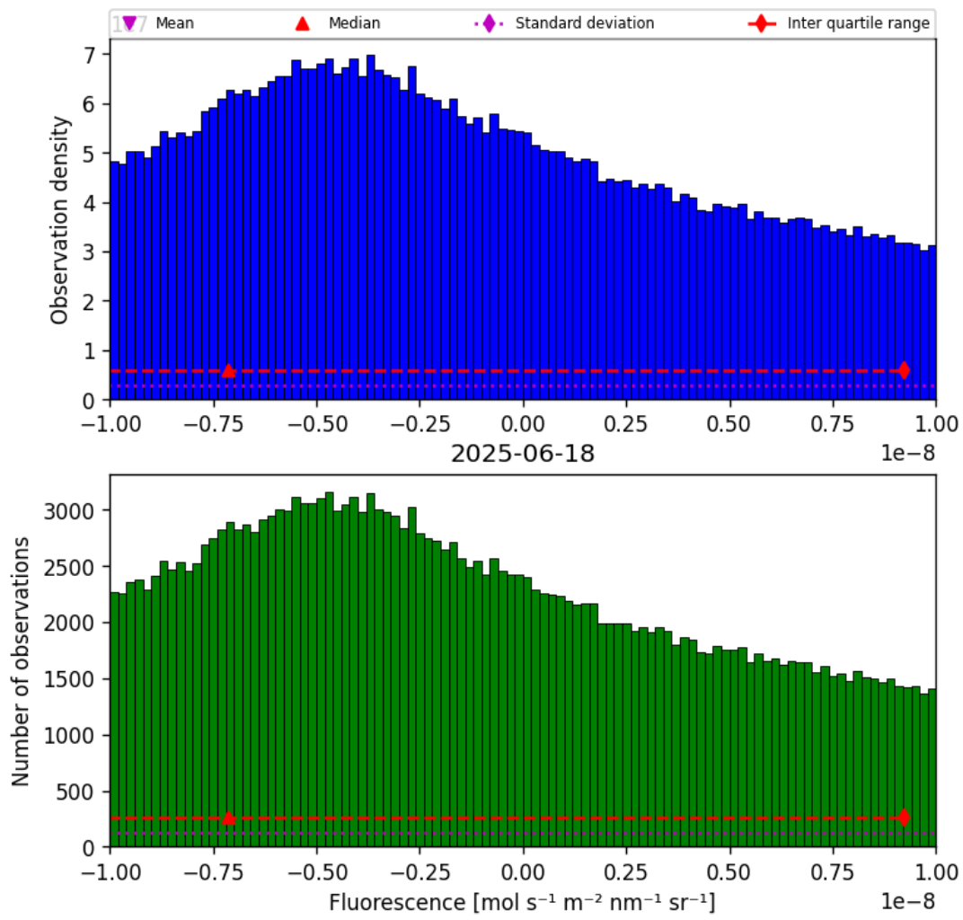
Figure 32: Histogram of “Fluorescence” for 2025-06-17 to 2025-06-19
