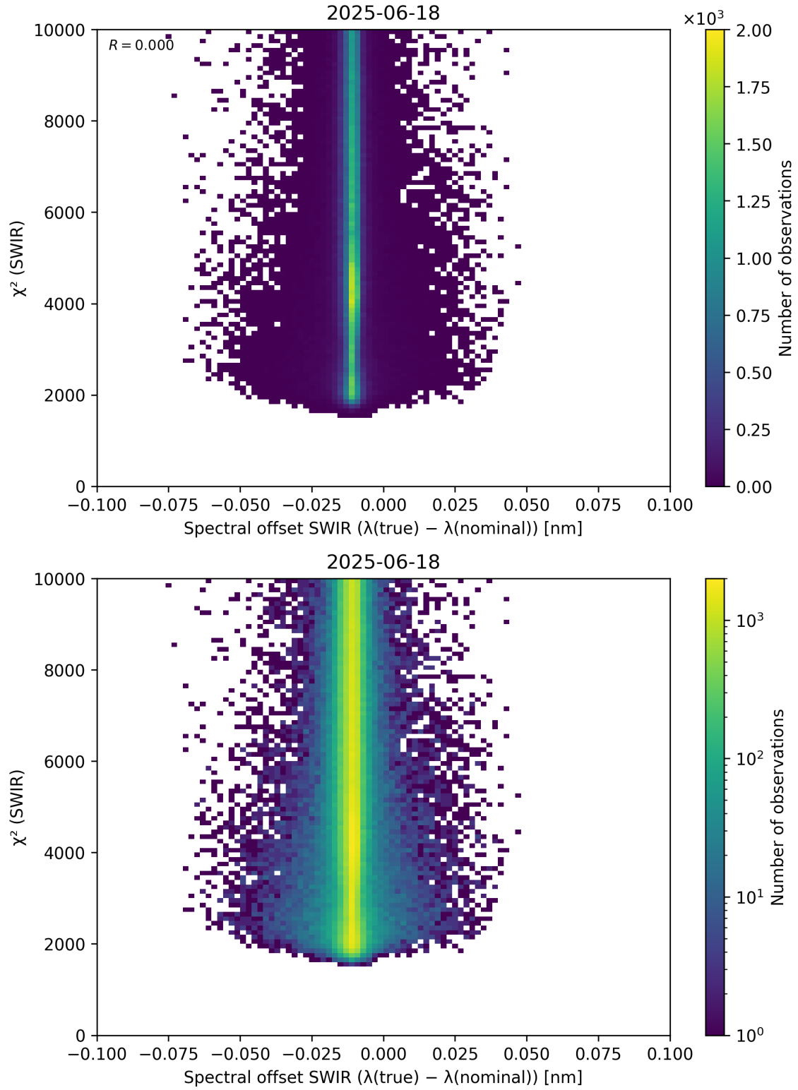
Figure 118: Scatter density plot of “Spectral offset SWIR ( \lambda_{\text{true}} - \lambda_{\text{nominal}} )” against “ \chi^2 (SWIR)” for 2025-06-17 to 2025-06-19.
