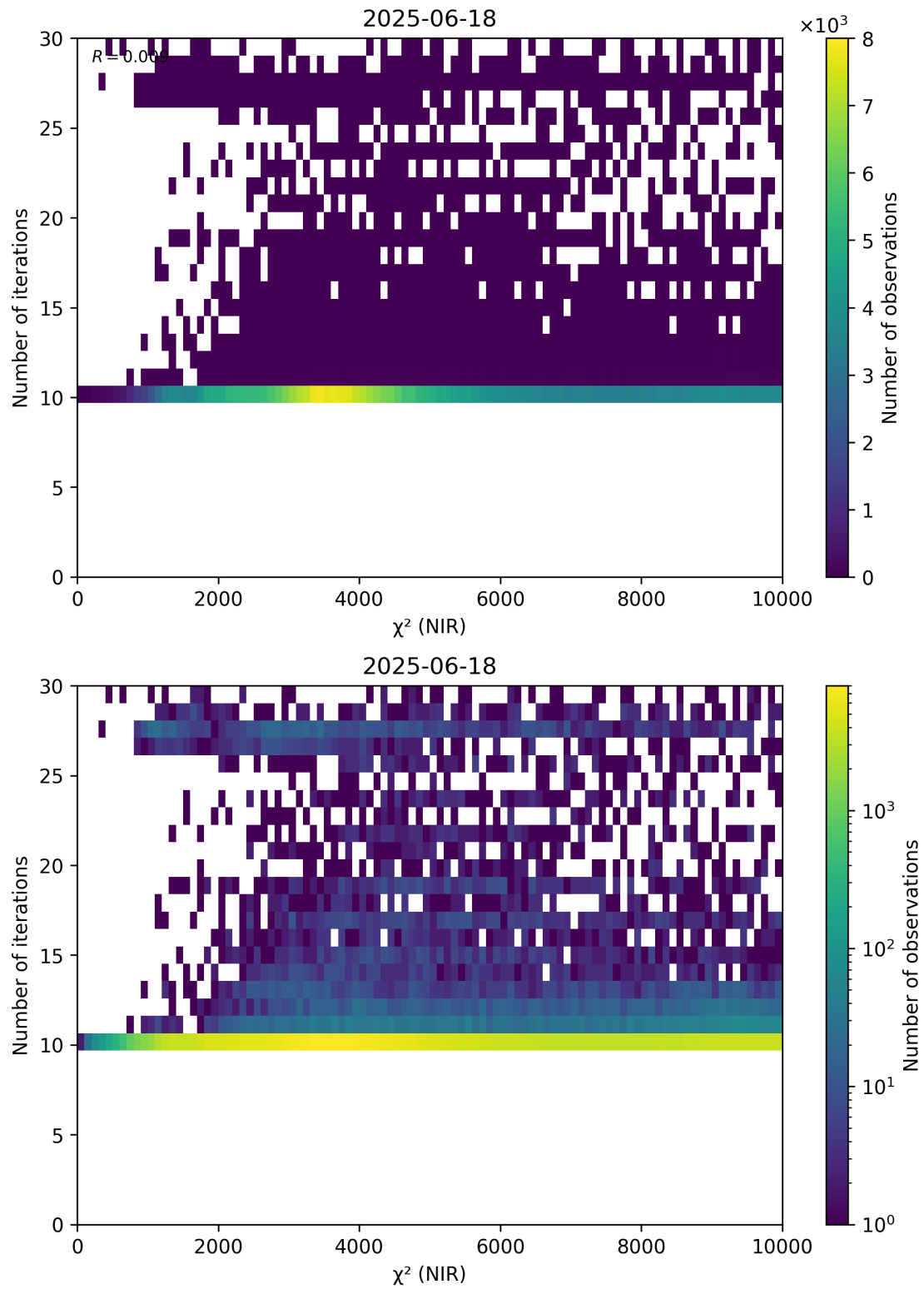
Figure 46: Scatter density plot of “ \chi^2 (NIR)” against “Number of iterations” for 2025-06-17 to 2025-06-19.
