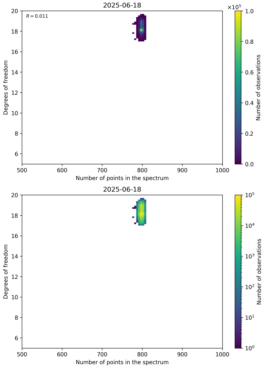
Figure 90: Scatter density plot of “Number of points in the spectrum” against “Degrees of freedom” for 2025-06-17 to 2025-06-19.
