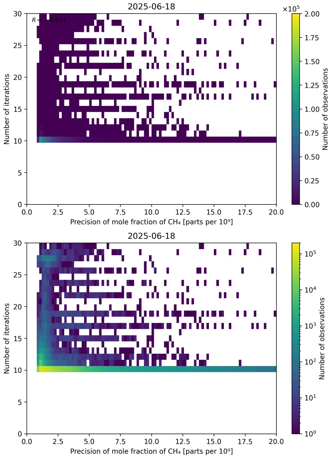
Figure 83: Scatter density plot of “Precision of mole fraction of CH 4 ” against “Number of iterations” for 2025-06-17 to 2025-06-19.
