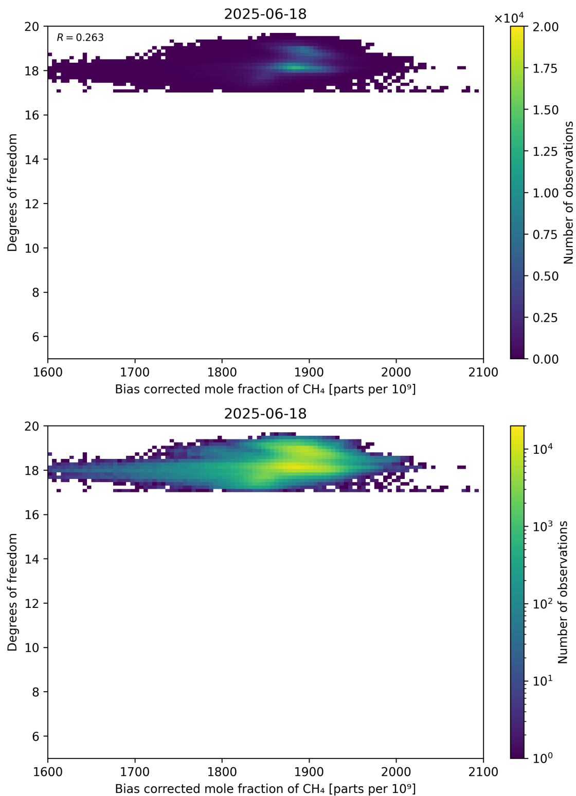
Figure 65: Scatter density plot of “Bias corrected mole fraction of CH 4 ” against “Degrees of freedom” for 2025-06-17 to 2025-06-19.
