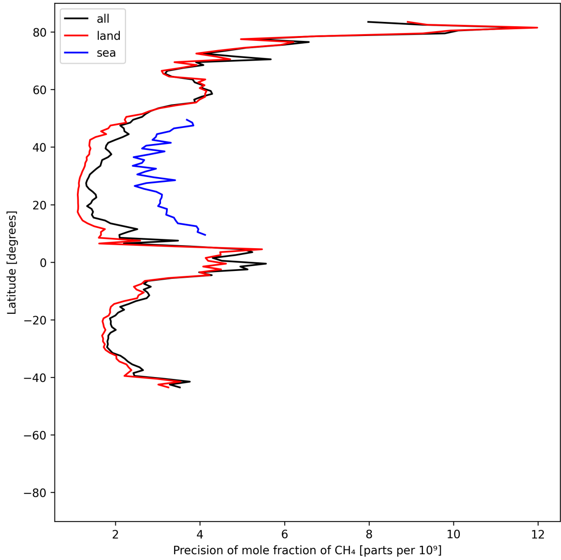
Figure 13: Zonal average of “Precision of mole fraction of CH 4 ” for 2025-06-17 to 2025-06-19.
