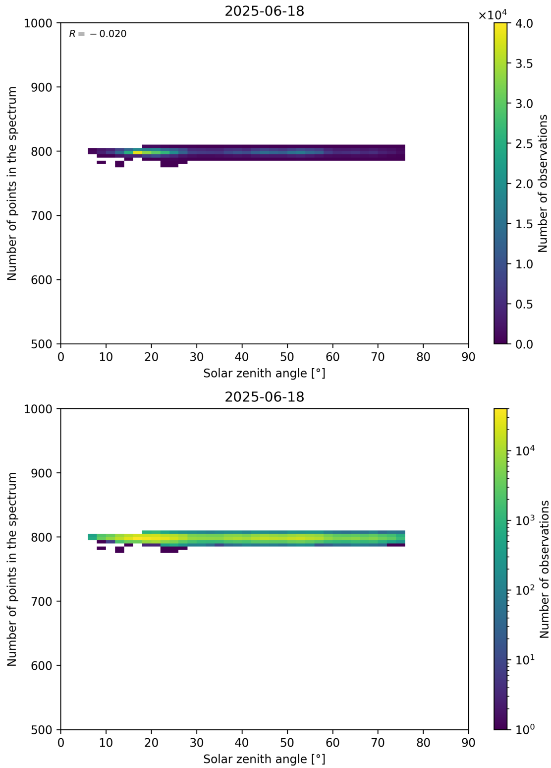
Figure 103: Scatter density plot of “Solar zenith angle” against “Number of points in the spectrum” for 2025-06-17 to 2025-06-19.
