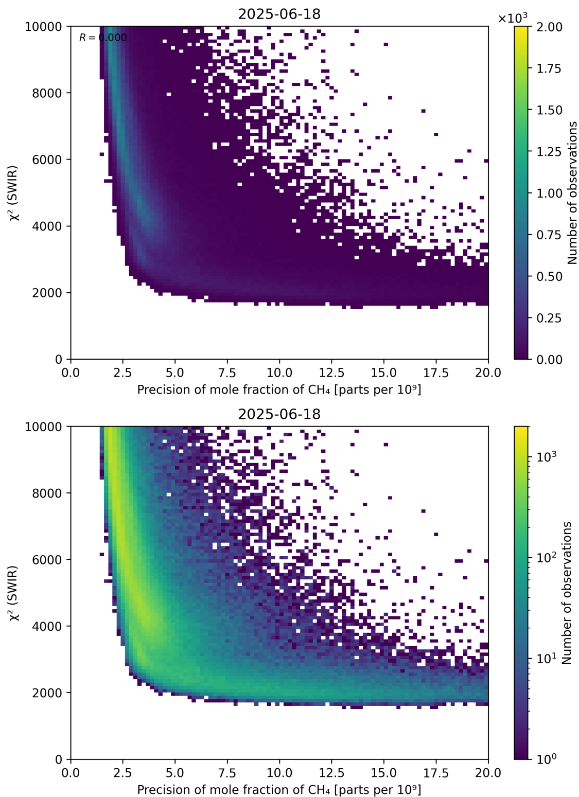
Figure 79: Scatter density plot of “Precision of mole fraction of \text{CH}_4 ” against “ \chi^2 (SWIR)” for 2025-06-17 to 2025-06-19.
