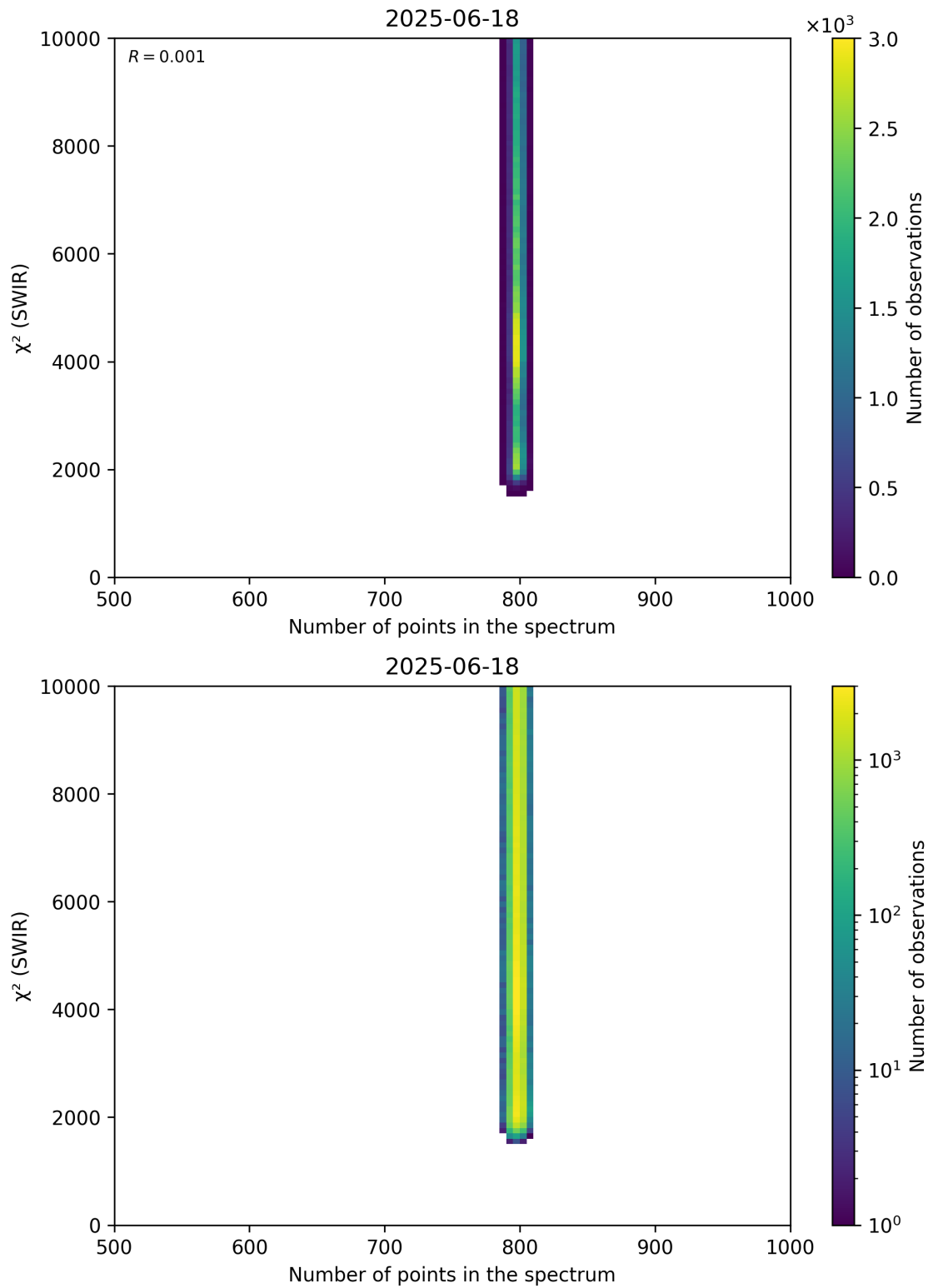
Figure 89: Scatter density plot of “Number of points in the spectrum” against “ \chi^2 (SWIR)” for 2025-06-17 to 2025-06-19.
