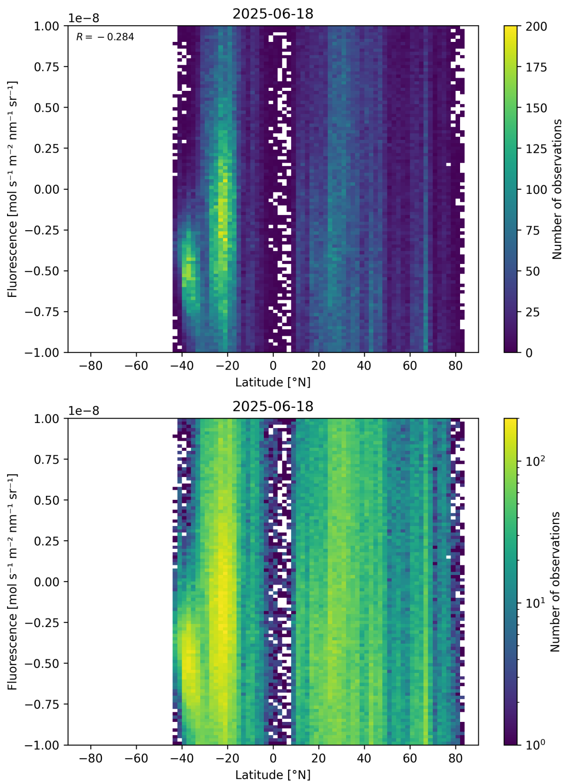
Figure 56: Scatter density plot of “Latitude” against “Fluorescence” for 2025-06-17 to 2025-06-19.
