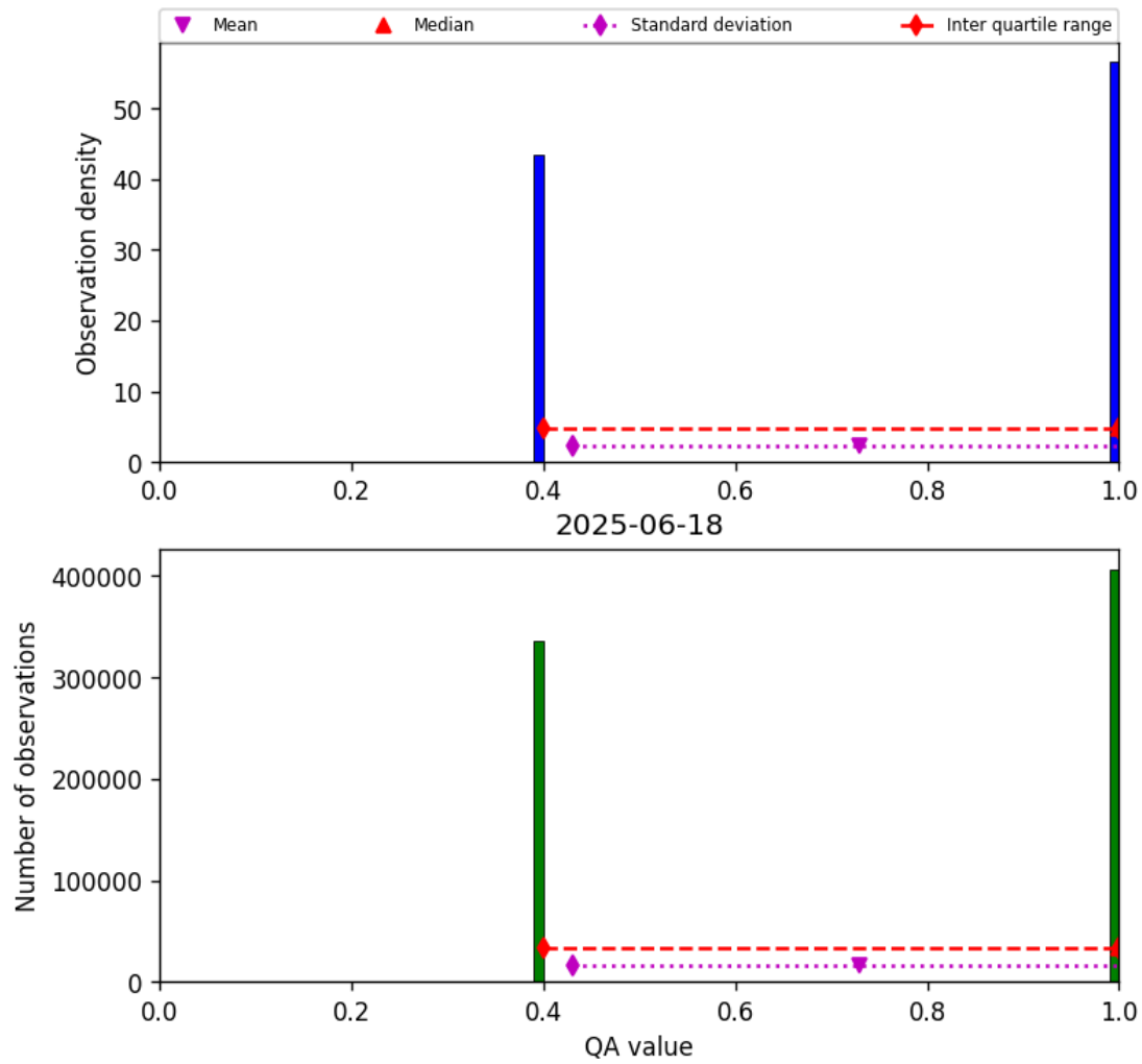
Figure 22: Histogram of “QA value” for 2025-06-17 to 2025-06-19
