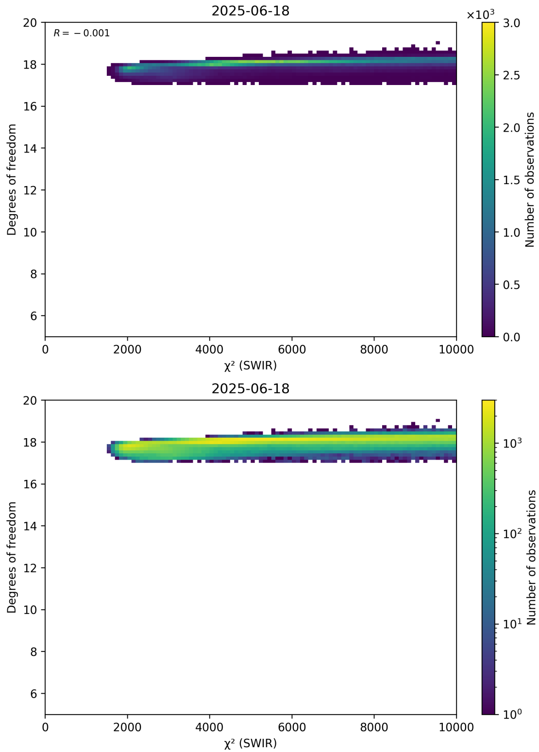
Figure 48: Scatter density plot of “ \chi^2 (SWIR)” against “Degrees of freedom” for 2025-06-17 to 2025-06-19.
