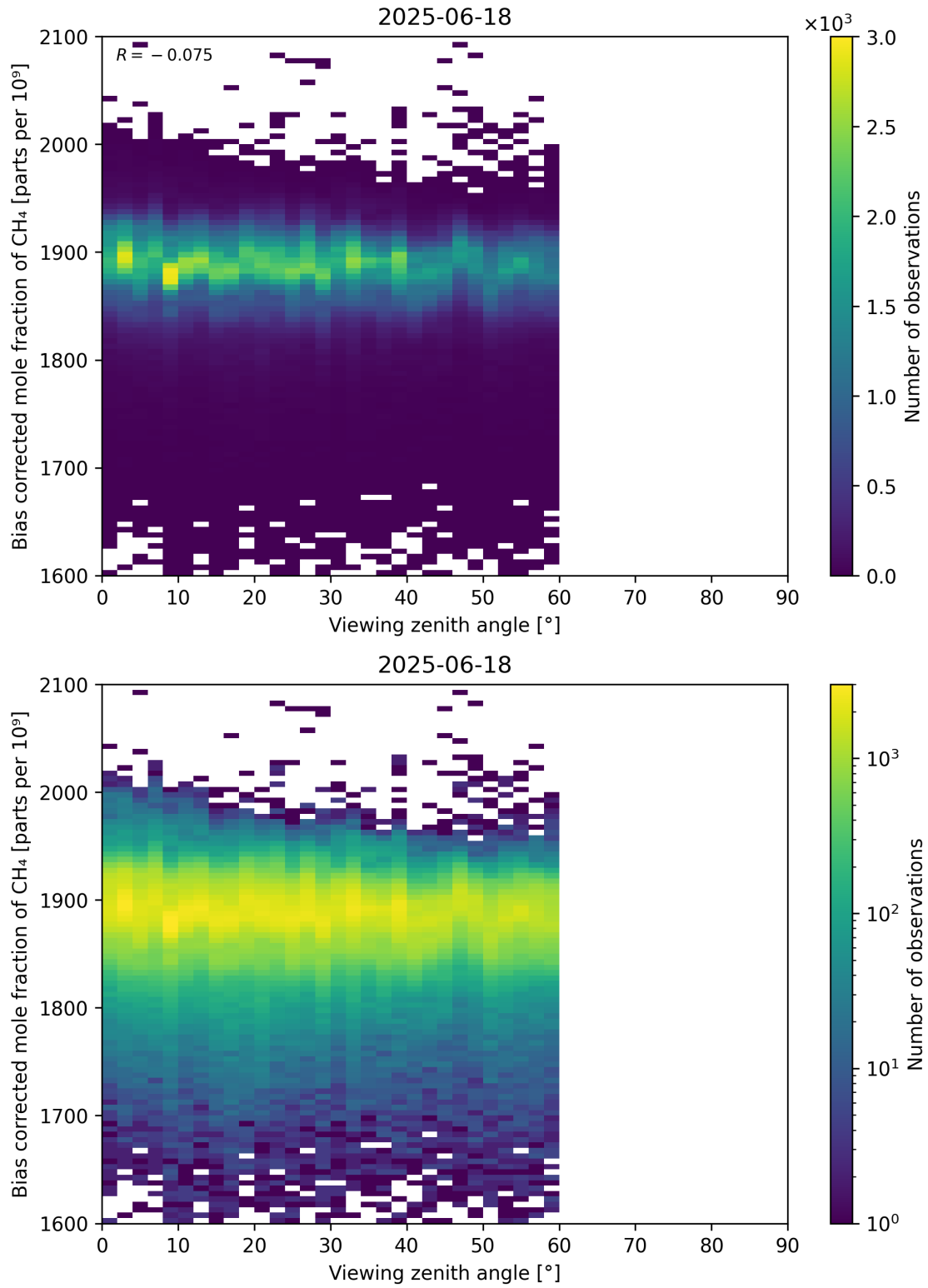
Figure 111: Scatter density plot of “Viewing zenith angle” against “Bias corrected mole fraction of CH 4 ” for 2025-06-17 to 2025-06-19.
