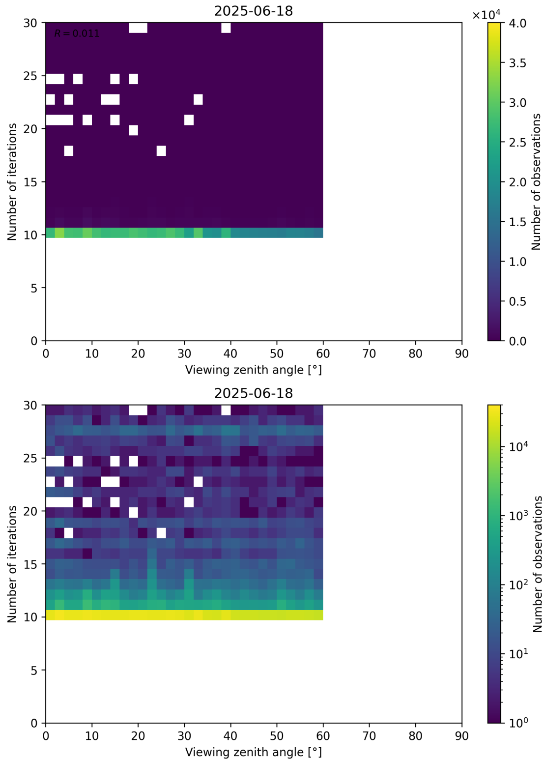
Figure 113: Scatter density plot of “Viewing zenith angle” against “Number of iterations” for 2025-06-17 to 2025-06-19.
