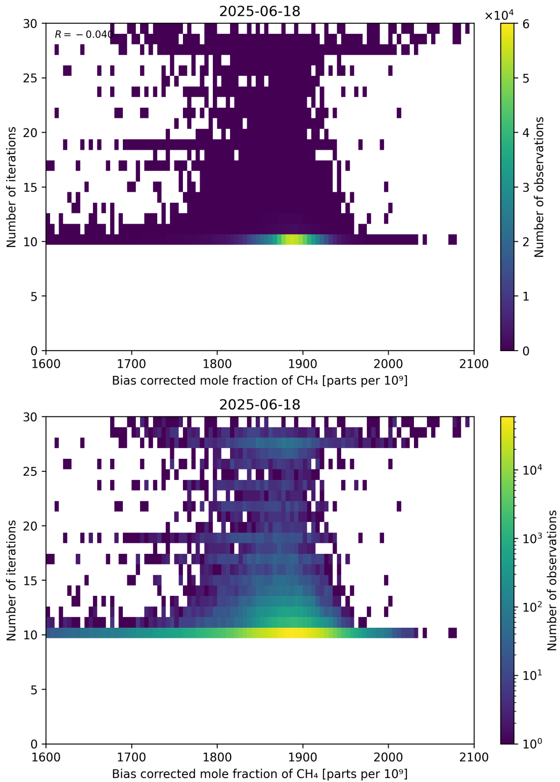
Figure 67: Scatter density plot of “Bias corrected mole fraction of CH 4 ” against “Number of iterations” for 2025-06-17 to 2025-06-19.
