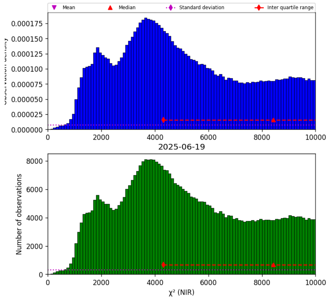
Figure 29: Histogram of “ \chi^2 (NIR)” for 2025-06-18 to 2025-06-20
