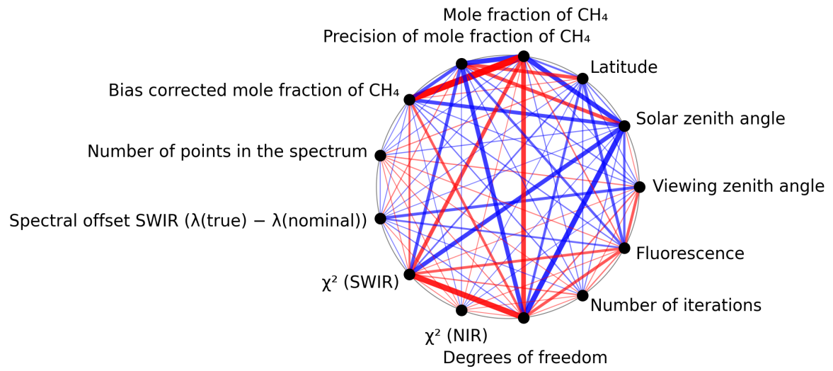
Figure 1: Map of correlation graph for 2025-06-18 to 2025-06-20.
