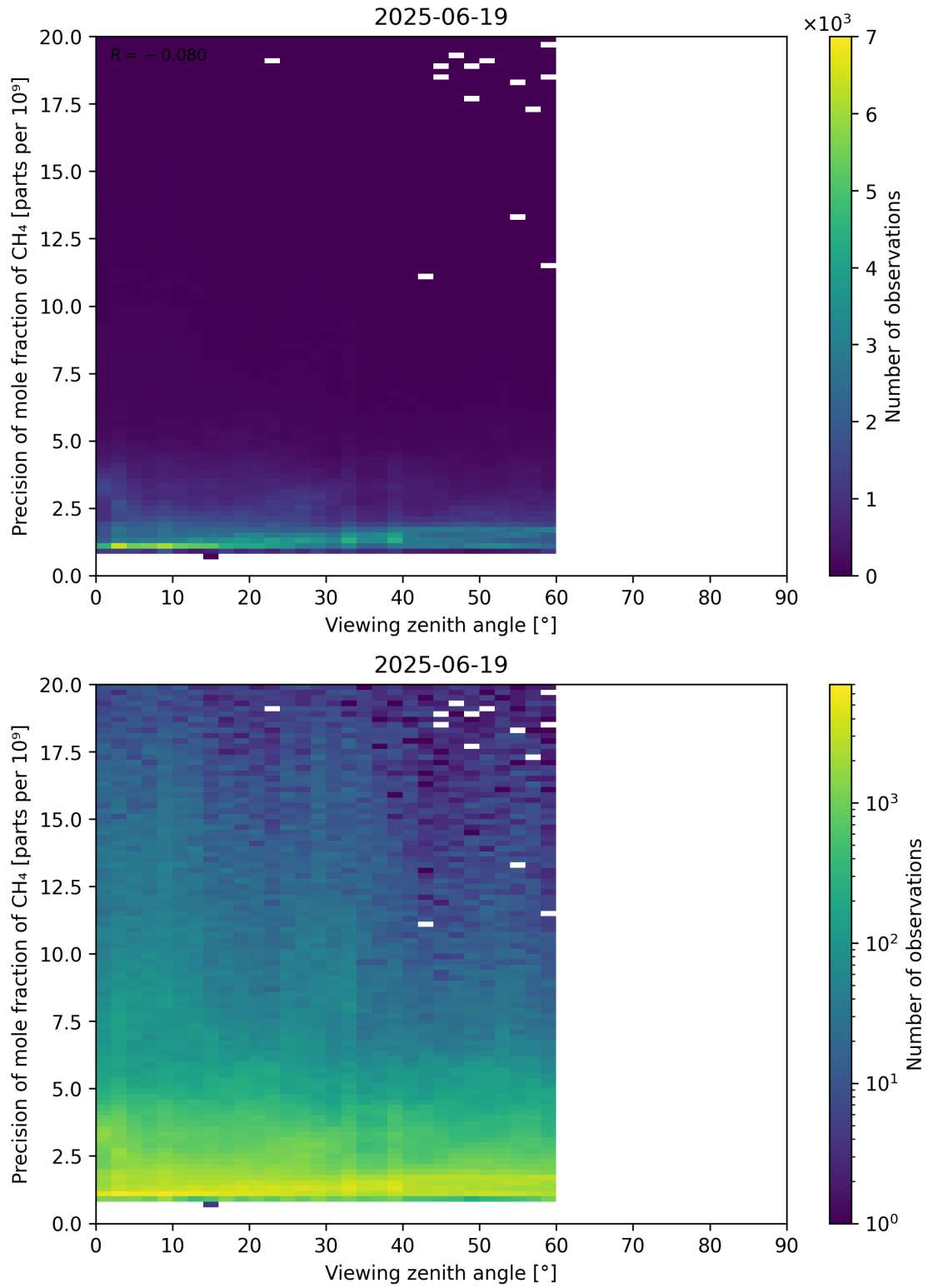
Figure 112: Scatter density plot of “Viewing zenith angle” against “Precision of mole fraction of CH 4 ” for 2025-06-18 to 2025-06-20.
