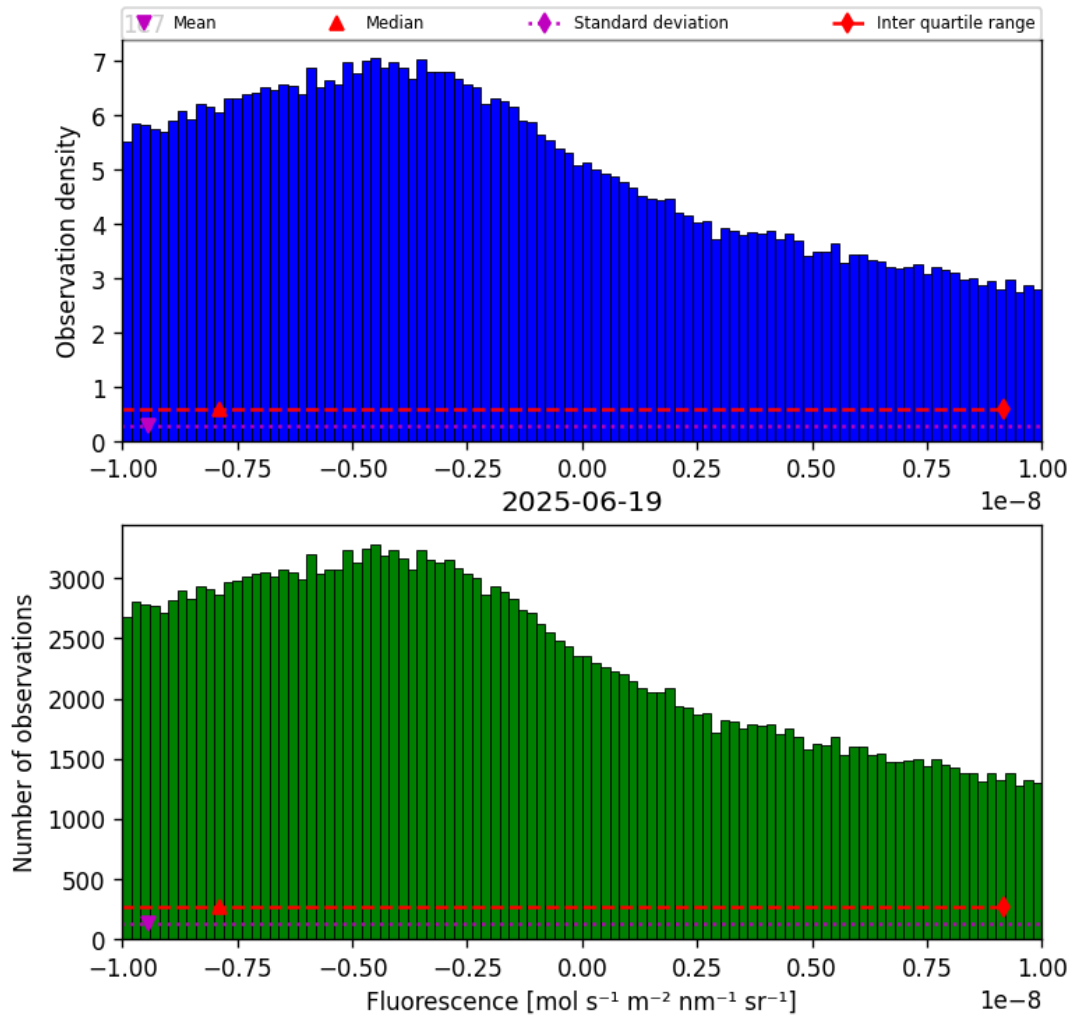
Figure 32: Histogram of “Fluorescence” for 2025-06-18 to 2025-06-20
