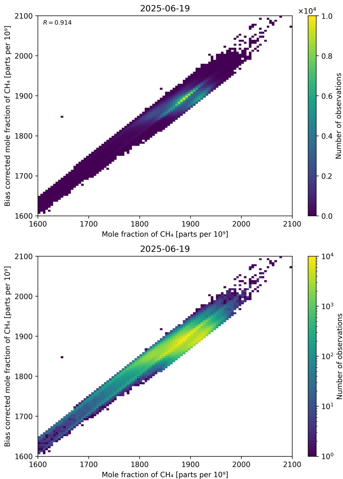
Figure 74: Scatter density plot of “Mole fraction of CH 4 ” against “Bias corrected mole fraction of CH 4 ” for 2025-06-18 to 2025-06-20.
