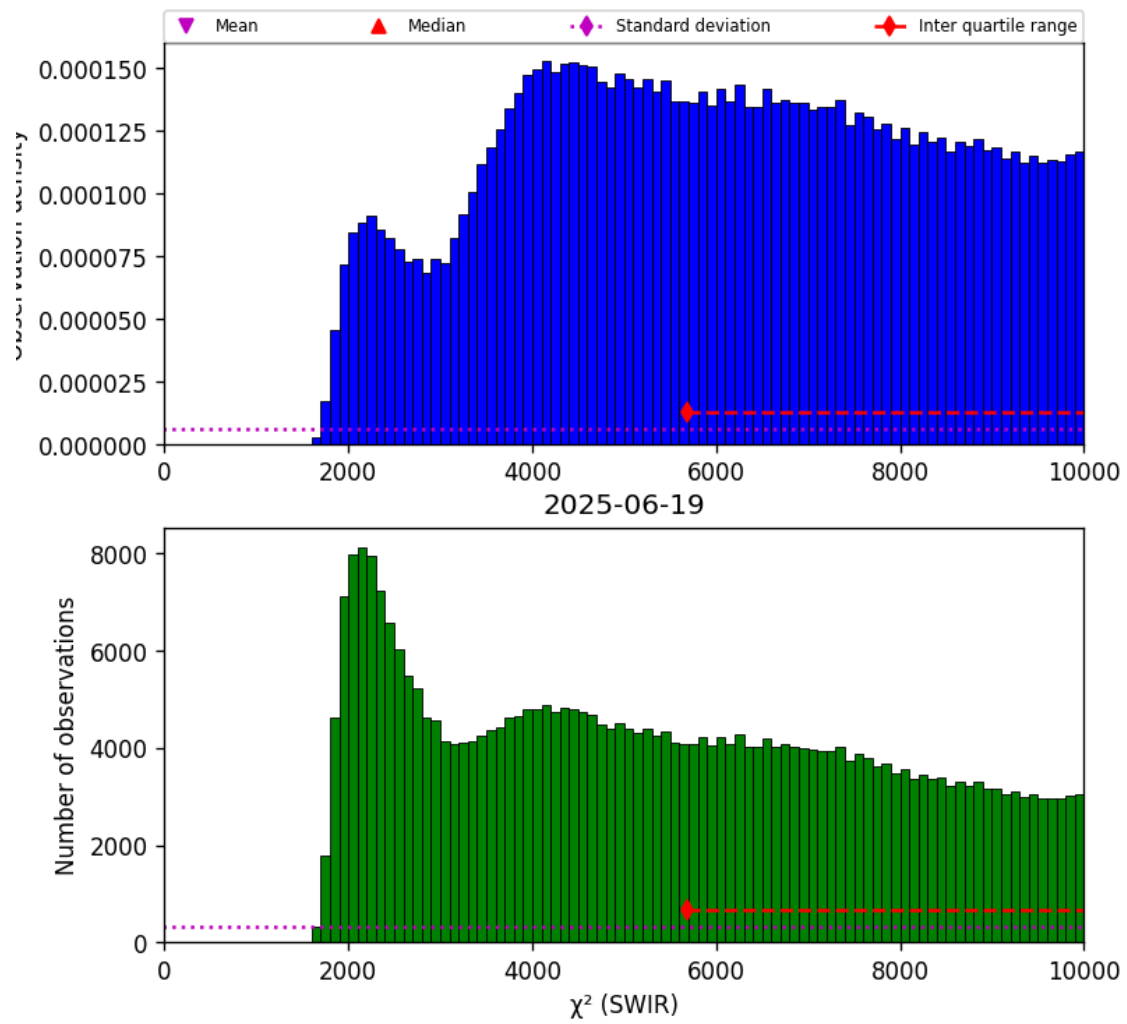
Figure 28: Histogram of “ \chi^2 (SWIR)” for 2025-06-18 to 2025-06-20
