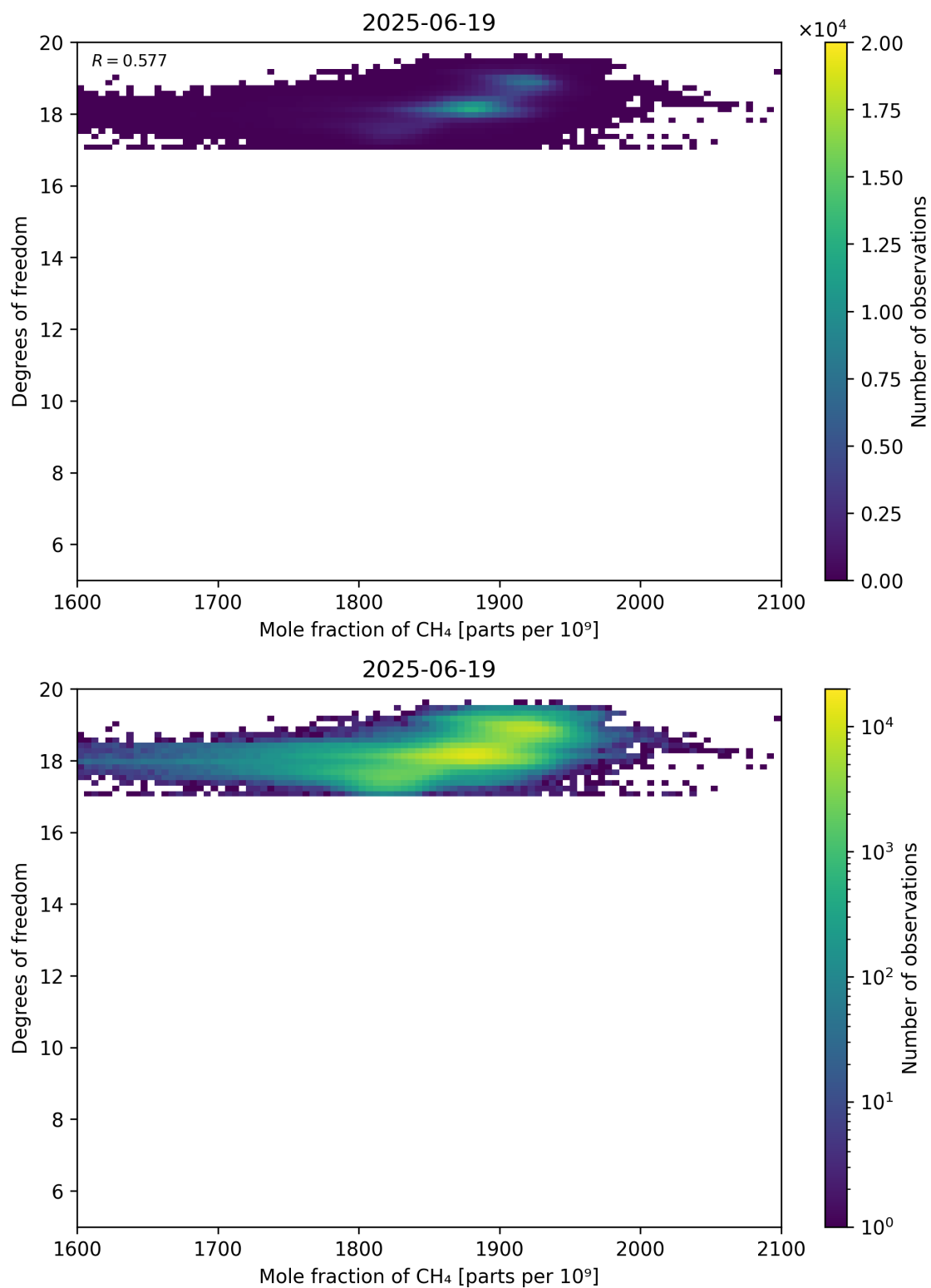
Figure 72: Scatter density plot of “Mole fraction of CH 4 ” against “Degrees of freedom” for 2025-06-18 to 2025-06-20.
