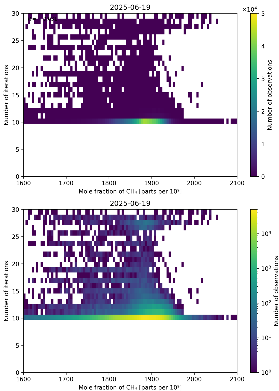
Figure 76: Scatter density plot of “Mole fraction of CH 4 ” against “Number of iterations” for 2025-06-18 to 2025-06-20.
