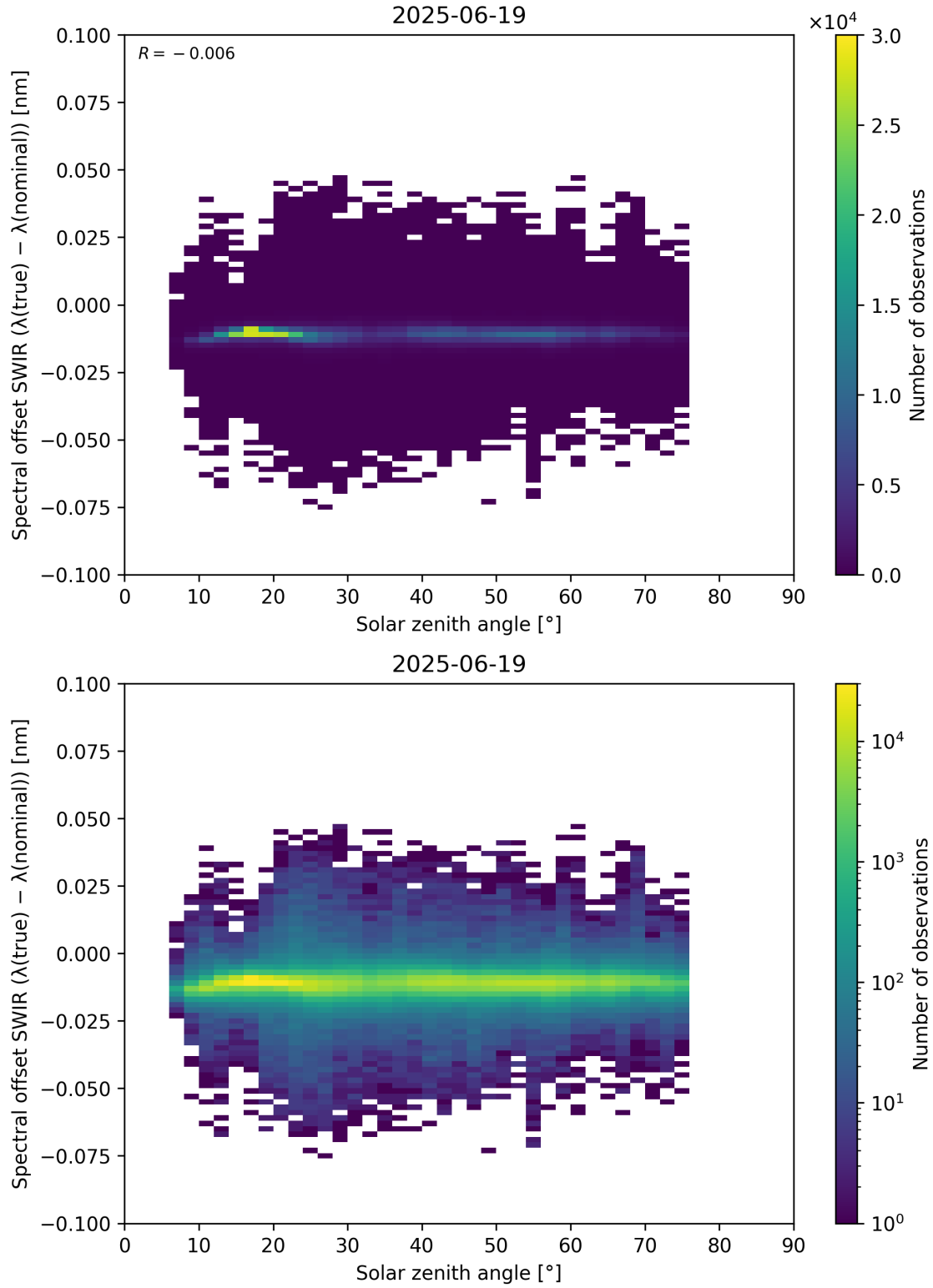
Figure 104: Scatter density plot of “Solar zenith angle” against “Spectral offset SWIR ( \lambda_{\text{true}} - \lambda_{\text{nominal}} )” for 2025-06-18 to 2025-06-20.
