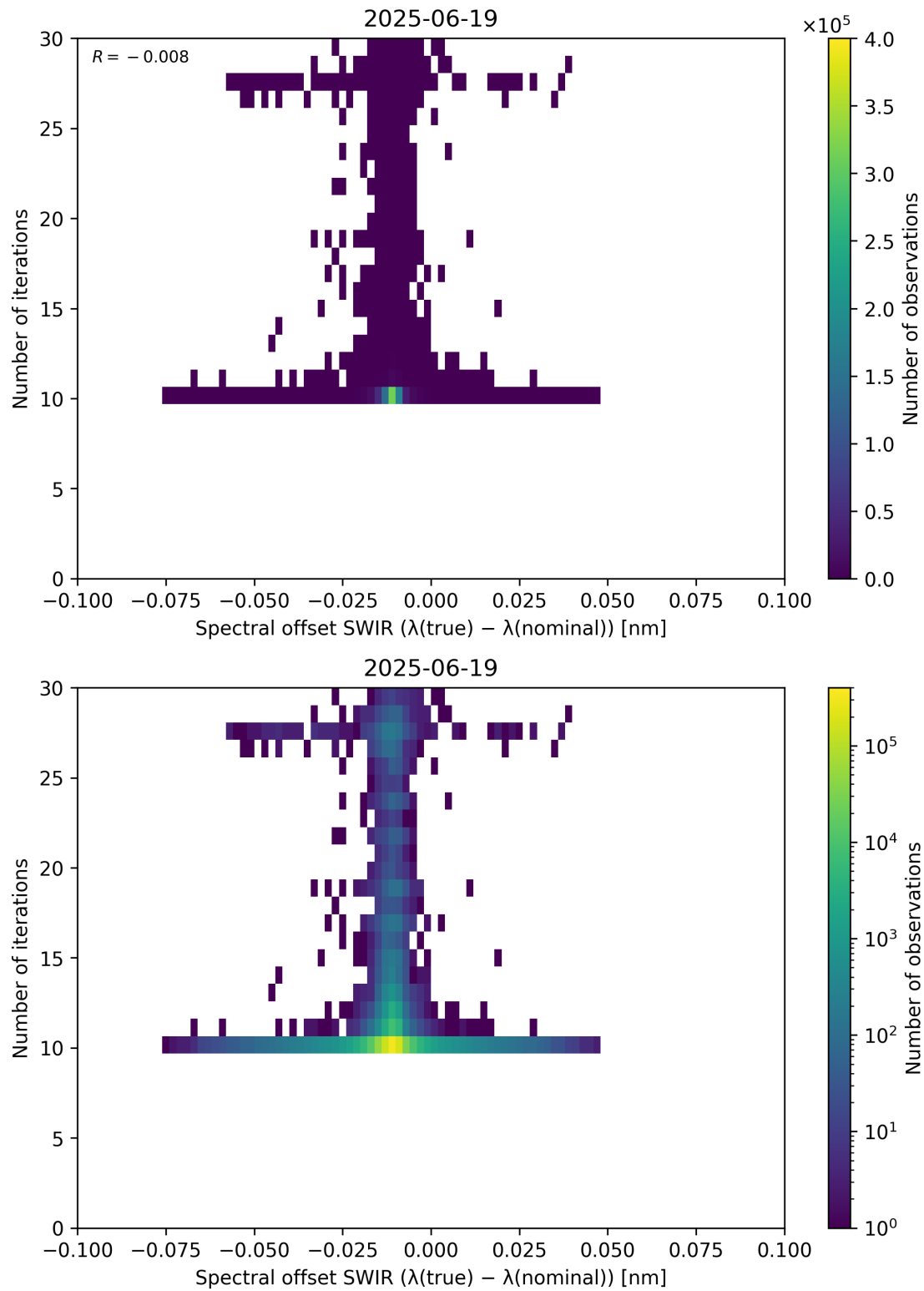
Figure 121: Scatter density plot of “Spectral offset SWIR ( \lambda_{\text{true}} - \lambda_{\text{nominal}} )” against “Number of iterations” for 2025-06-18 to 2025-06-20.
