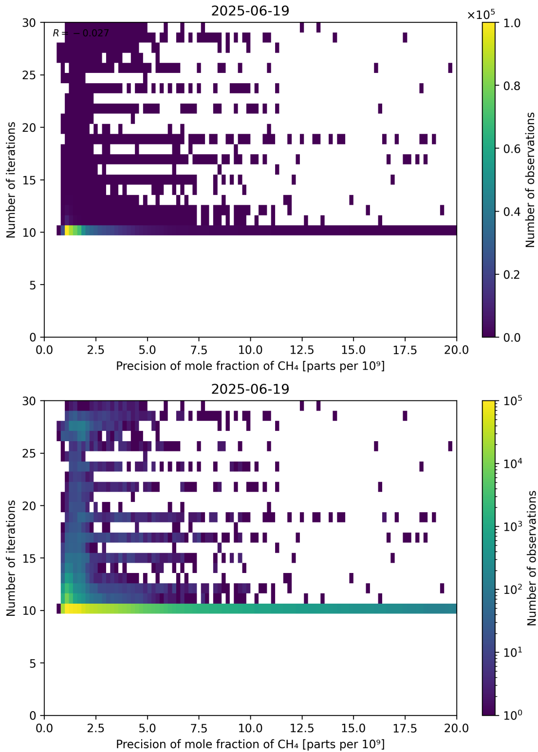
Figure 83: Scatter density plot of “Precision of mole fraction of CH 4 ” against “Number of iterations” for 2025-06-18 to 2025-06-20.
