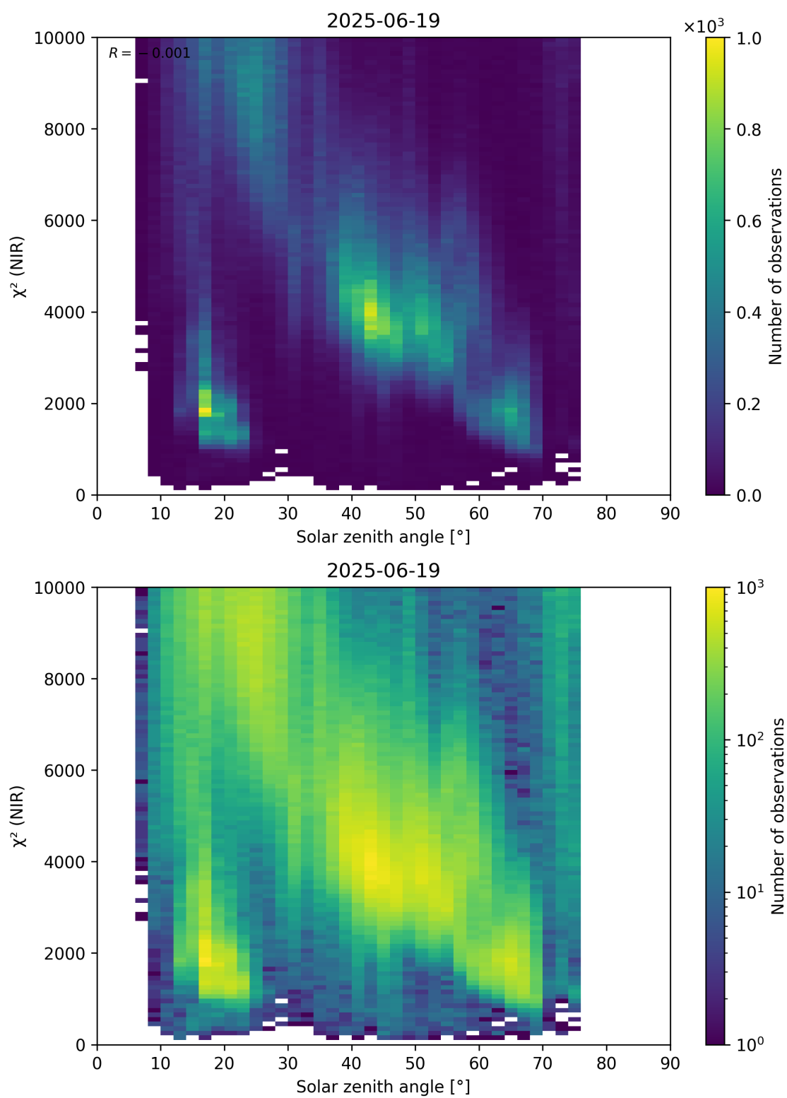
Figure 94: Scatter density plot of “Solar zenith angle” against “ \chi^2 (NIR)” for 2025-06-18 to 2025-06-20.
