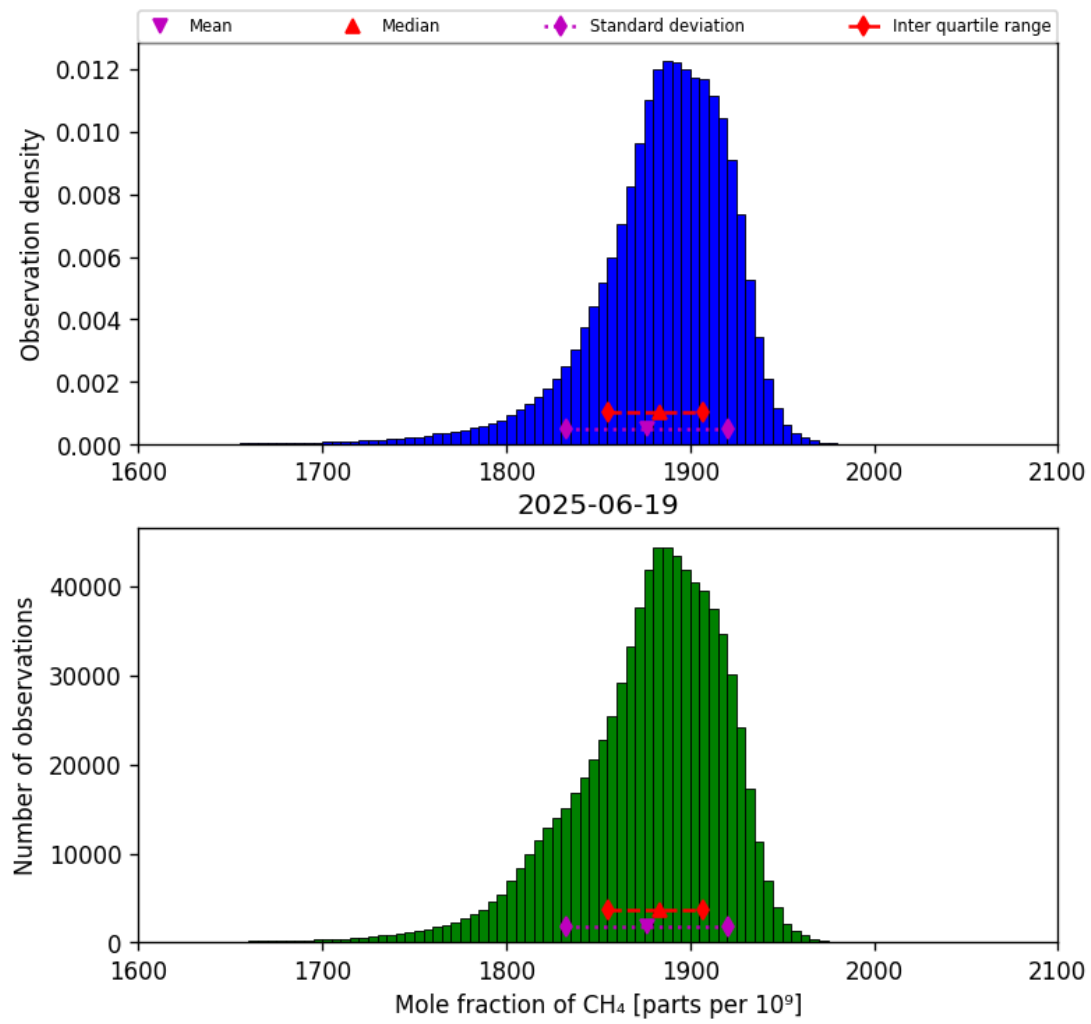
Figure 23: Histogram of “Mole fraction of CH 4 ” for 2025-06-18 to 2025-06-20
