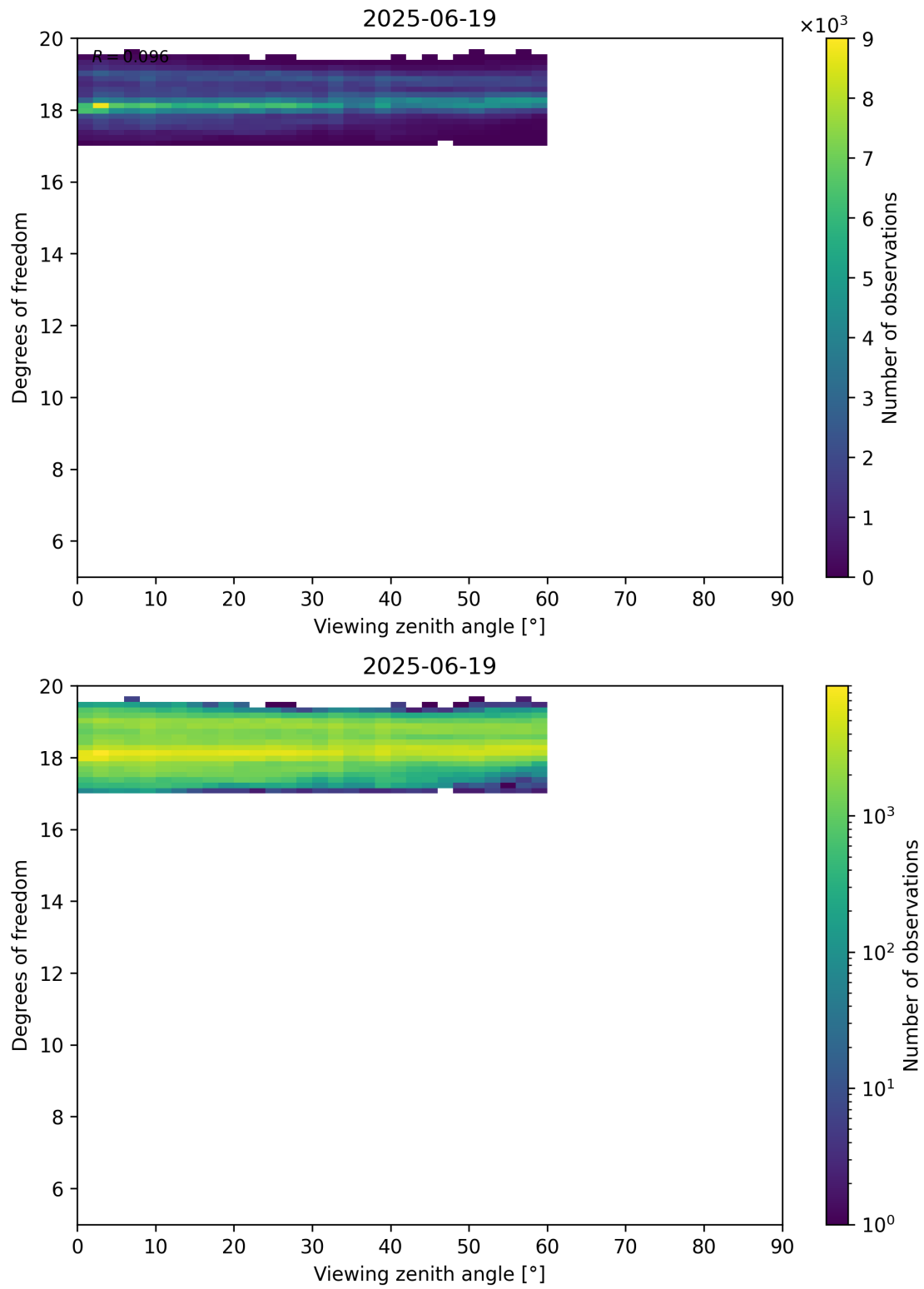
Figure 107: Scatter density plot of “Viewing zenith angle” against “Degrees of freedom” for 2025-06-18 to 2025-06-20.
