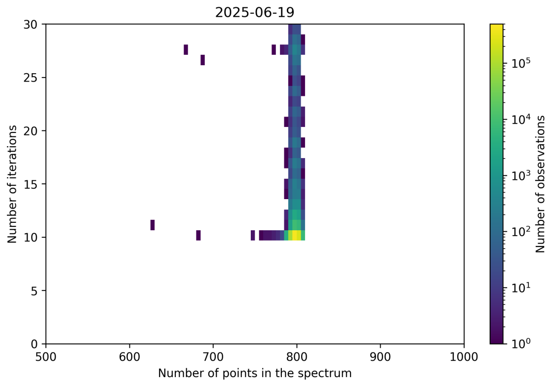
Figure 92: Scatter density plot of “Number of points in the spectrum” against “Number of iterations” for 2025-06-18 to 2025-06-20.
