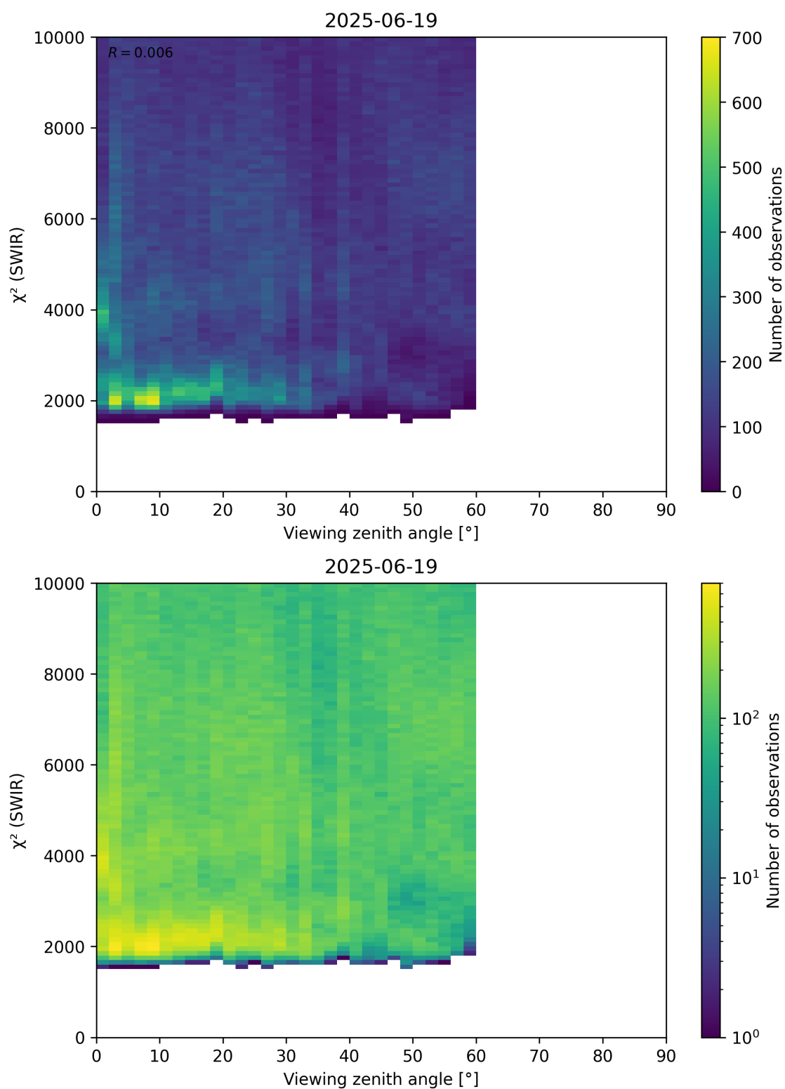
Figure 106: Scatter density plot of “Viewing zenith angle” against “ \chi^2 (SWIR)” for 2025-06-18 to 2025-06-20.
