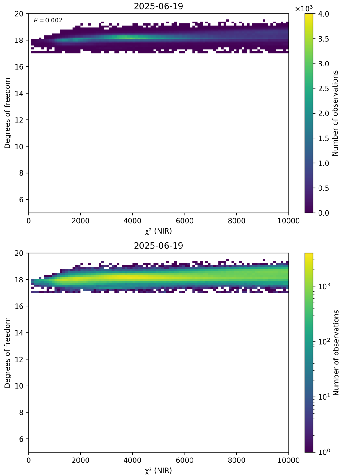
Figure 44: Scatter density plot of “ \chi^2 (NIR)” against “Degrees of freedom” for 2025-06-18 to 2025-06-20.
