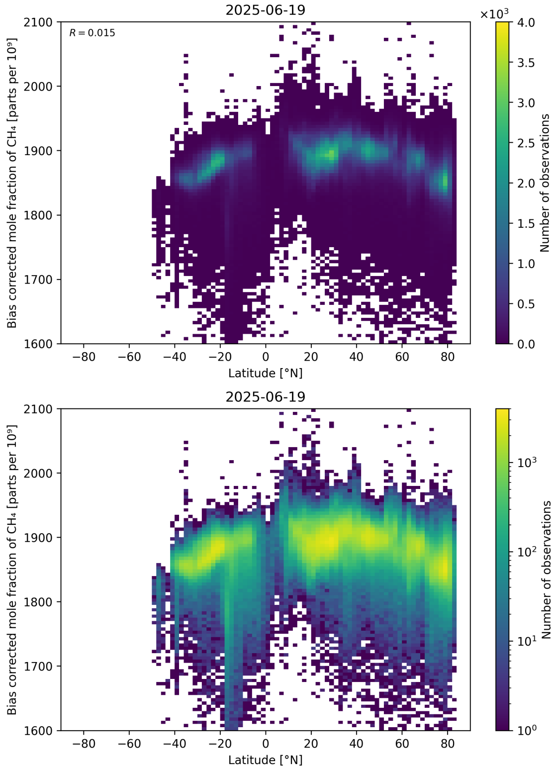
Figure 58: Scatter density plot of “Latitude” against “Bias corrected mole fraction of CH 4 ” for 2025-06-18 to 2025-06-20.
