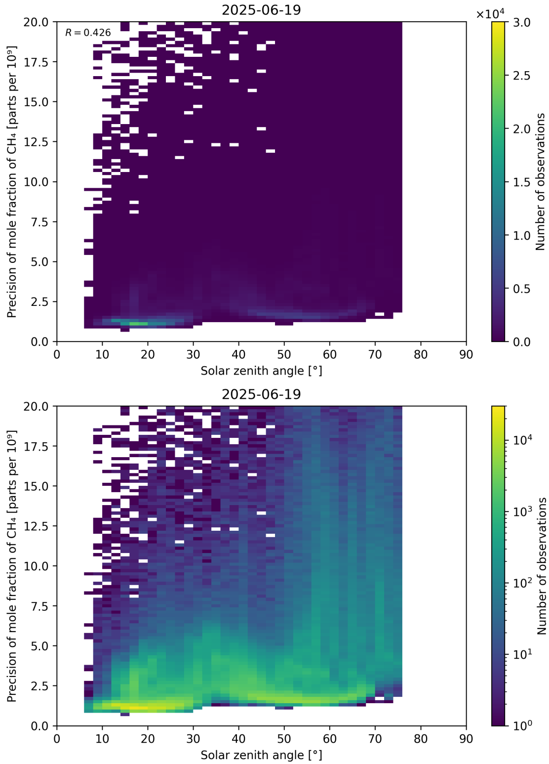
Figure 101: Scatter density plot of “Solar zenith angle” against “Precision of mole fraction of \text{CH}_4 ” for 2025-06-18 to 2025-06-20.
