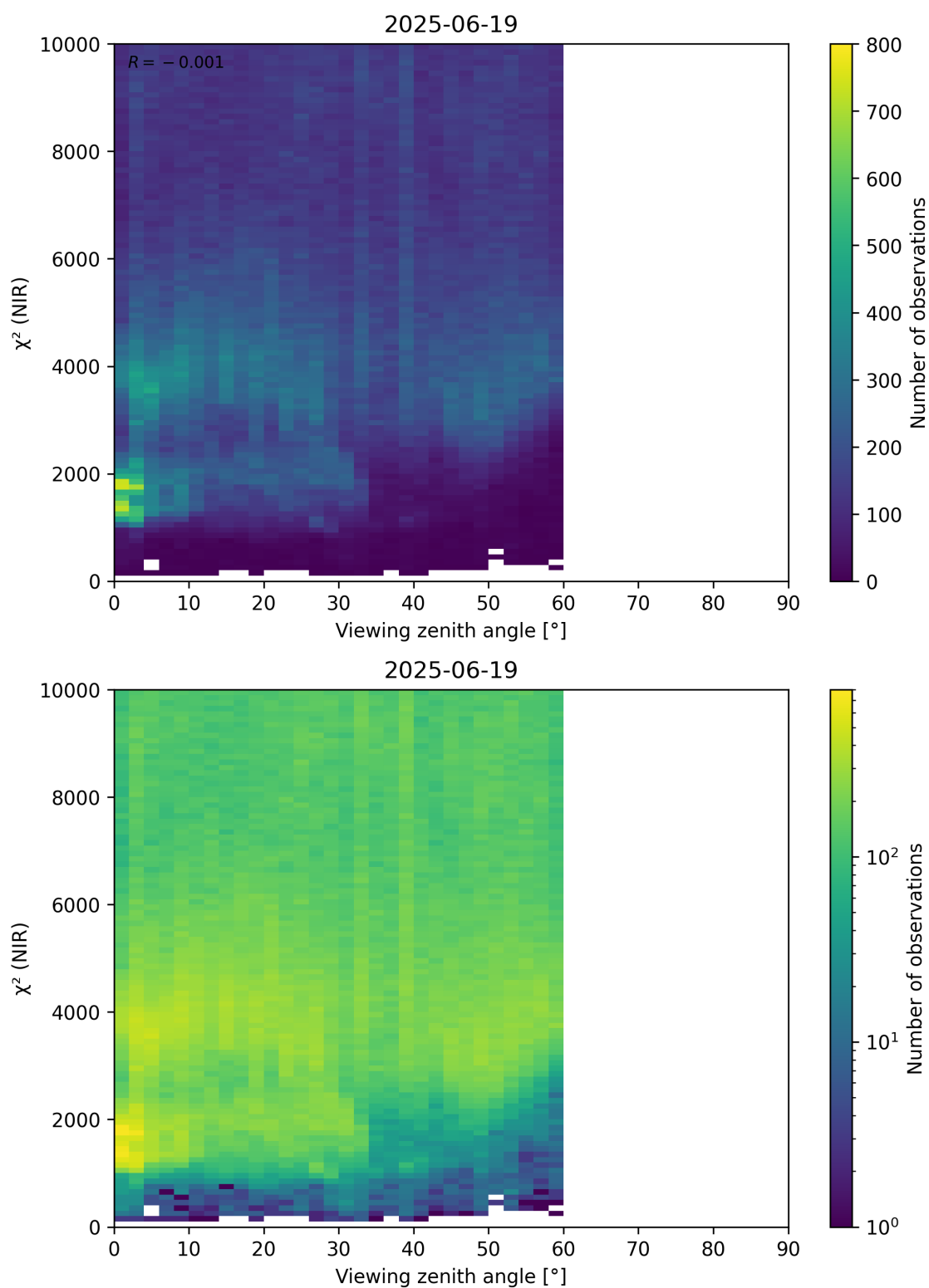
Figure 105: Scatter density plot of “Viewing zenith angle” against “ \chi^2 (NIR)” for 2025-06-18 to 2025-06-20.
