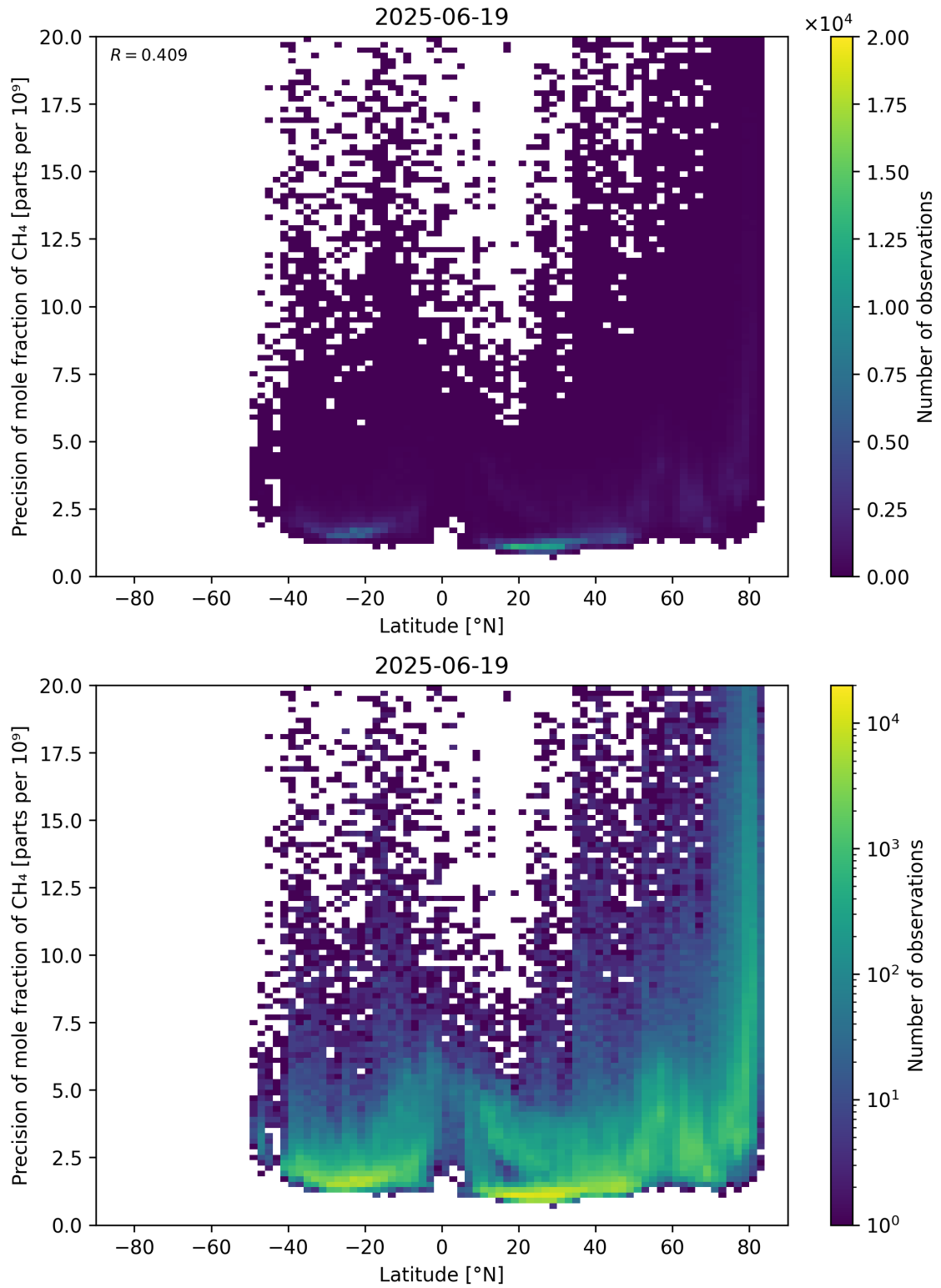
Figure 59: Scatter density plot of “Latitude” against “Precision of mole fraction of \text{CH}_4 ” for 2025-06-18 to 2025-06-20.
