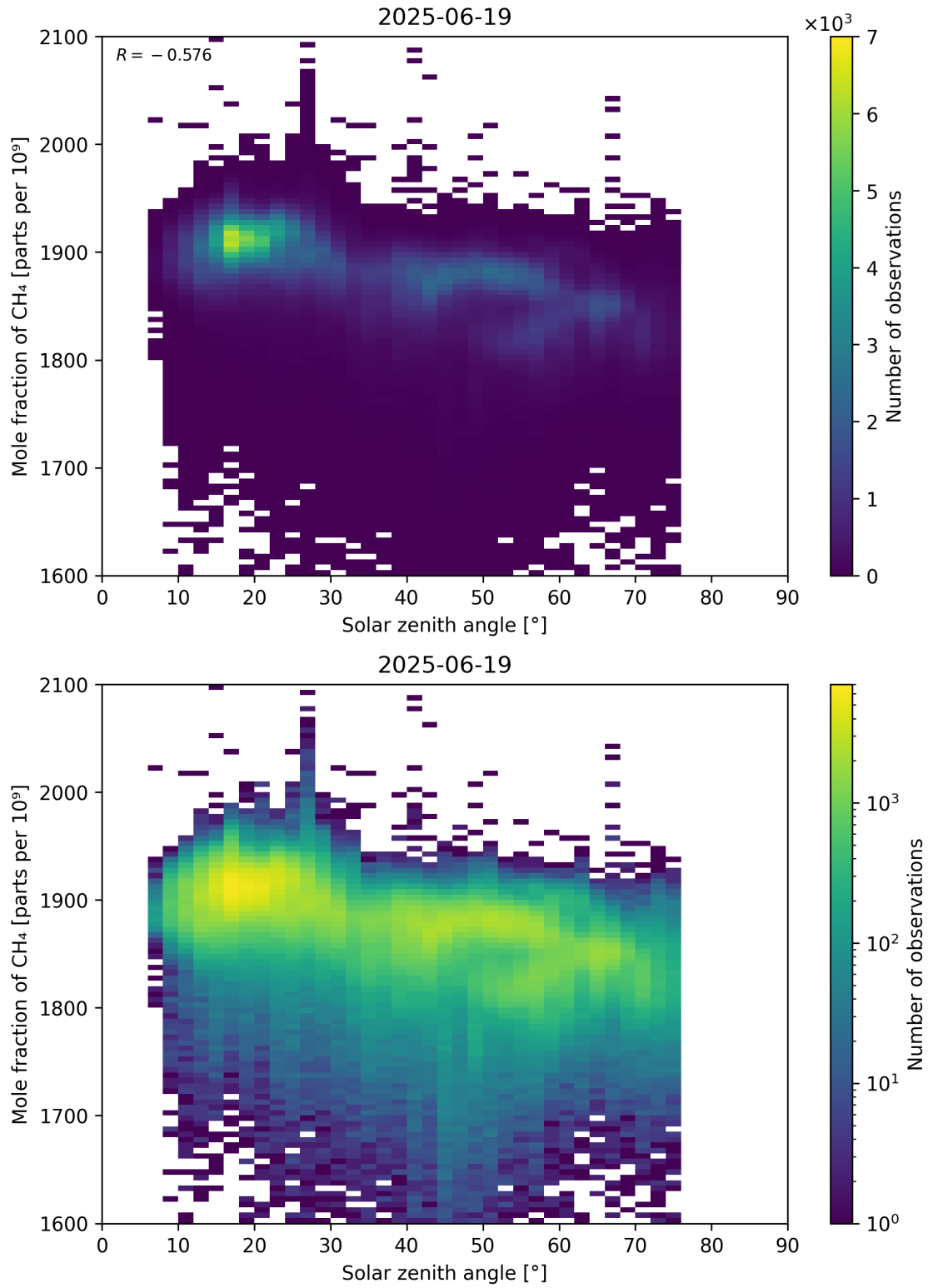
Figure 99: Scatter density plot of “Solar zenith angle” against “Mole fraction of CH 4 ” for 2025-06-18 to 2025-06-20.
