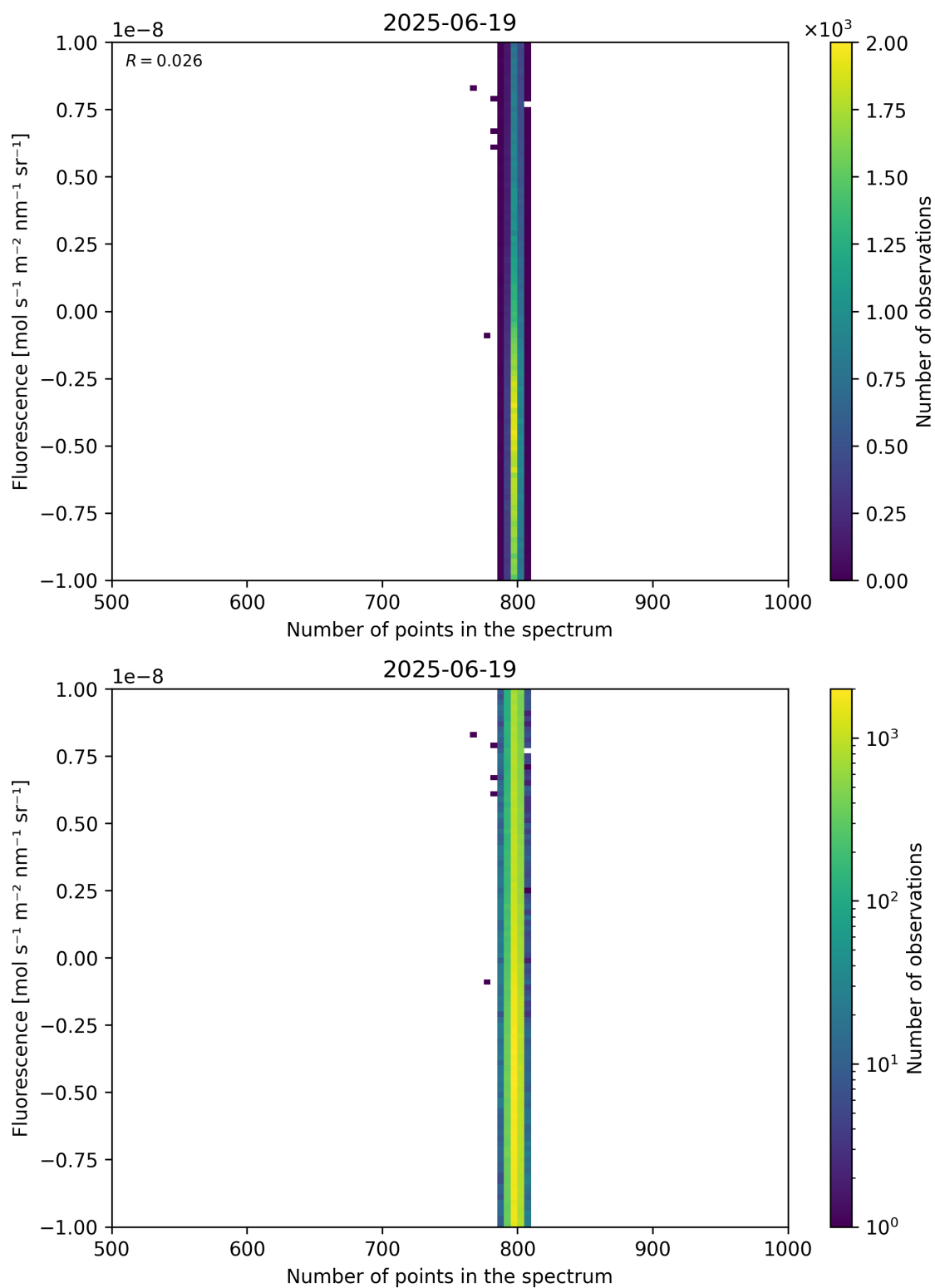
Figure 91: Scatter density plot of “Number of points in the spectrum” against “Fluorescence” for 2025-06-18 to 2025-06-20.
