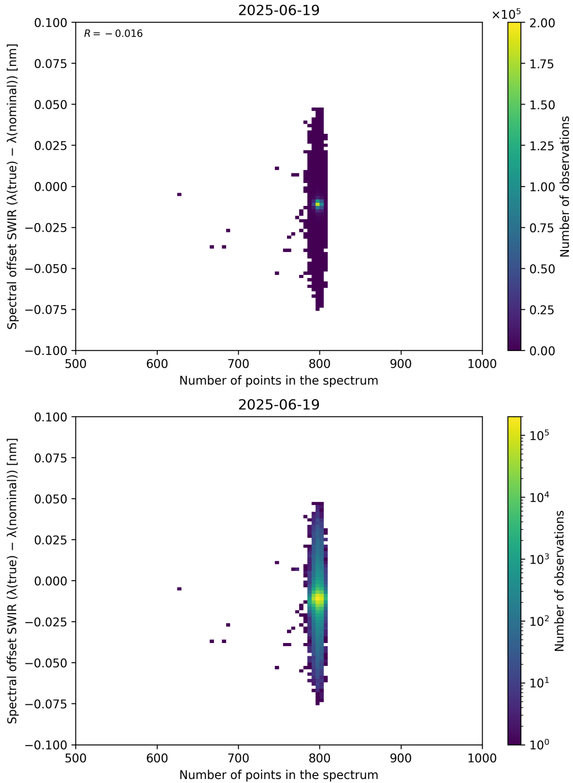
Figure 93: Scatter density plot of “Number of points in the spectrum” against “Spectral offset SWIR ( \lambda_{\text{true}} - \lambda_{\text{nominal}} )” for 2025-06-18 to 2025-06-20.
