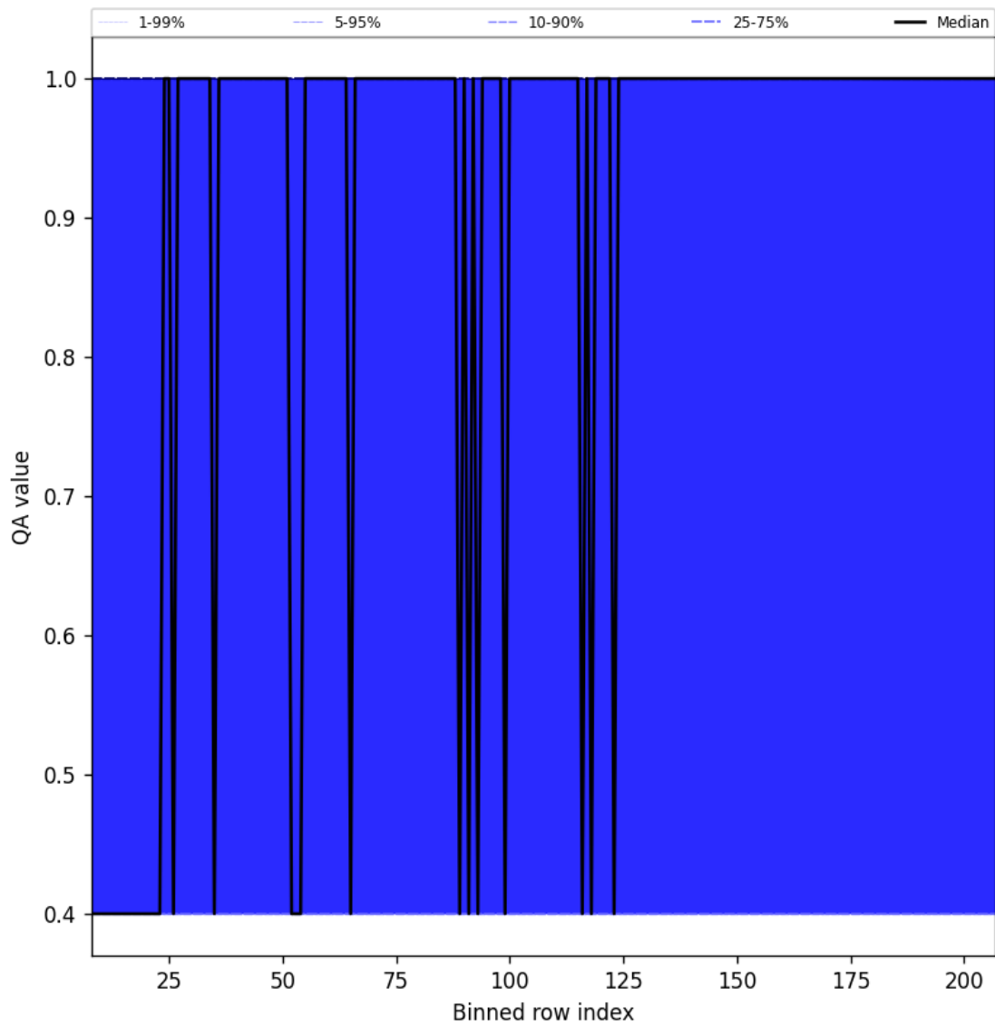
Figure 33: Along track statistics of “QA value” for 2025-06-18 to 2025-06-20
