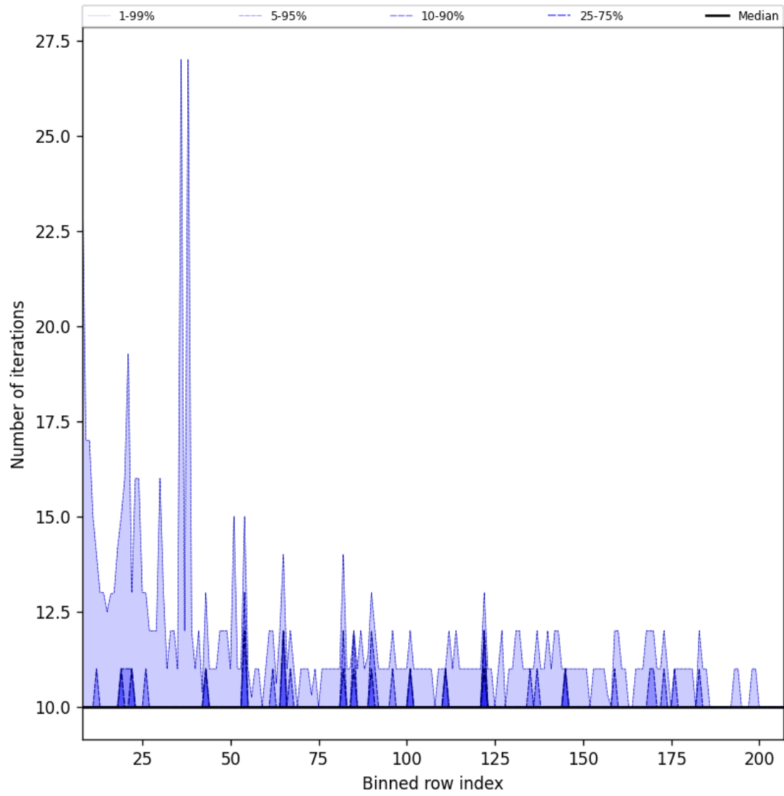
Figure 42: Along track statistics of “Number of iterations” for 2025-06-18 to 2025-06-20
