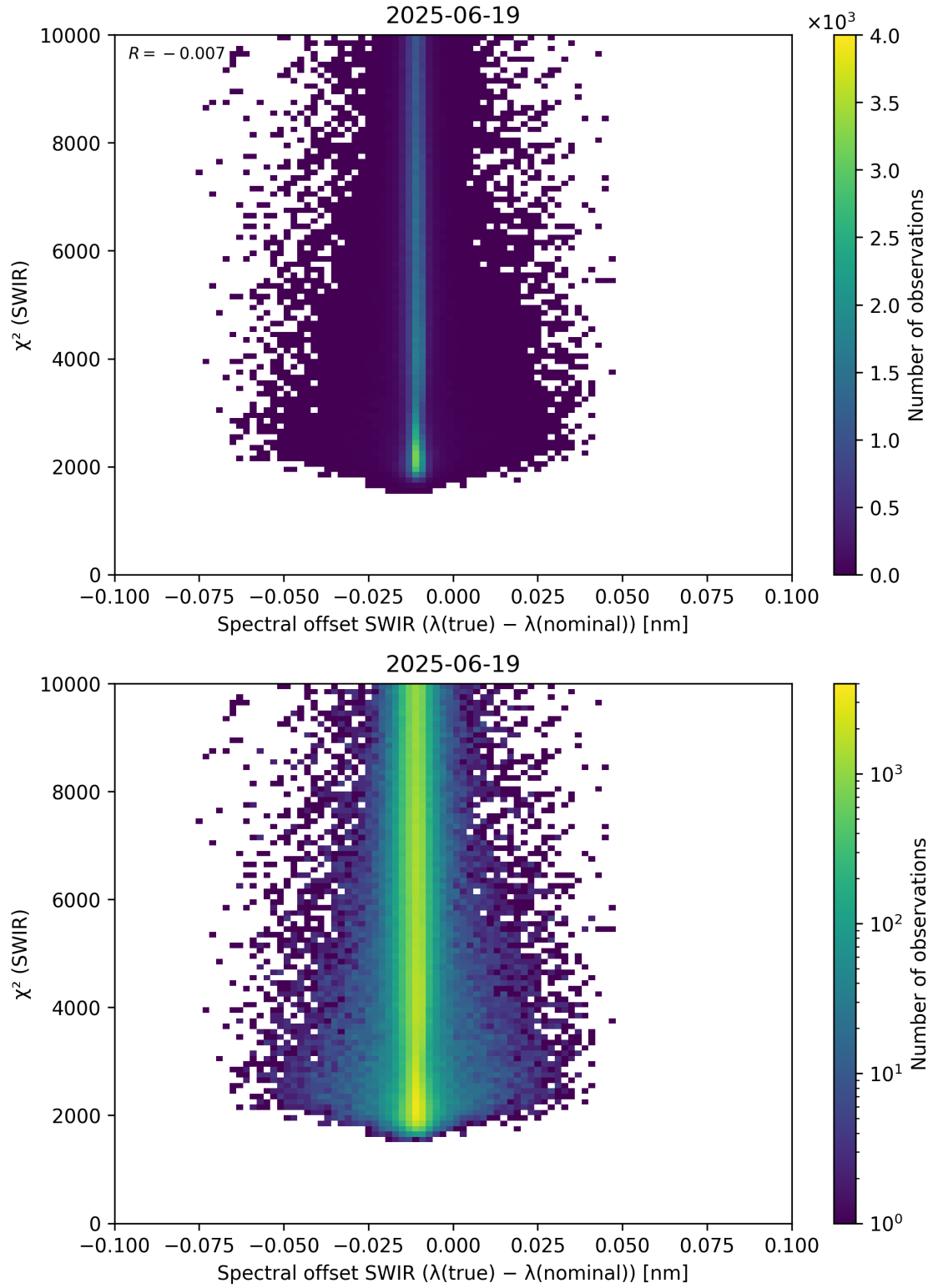
Figure 118: Scatter density plot of “Spectral offset SWIR ( \lambda_{\text{true}} - \lambda_{\text{nominal}} )” against “ \chi^2 (SWIR)” for 2025-06-18 to 2025-06-20.
