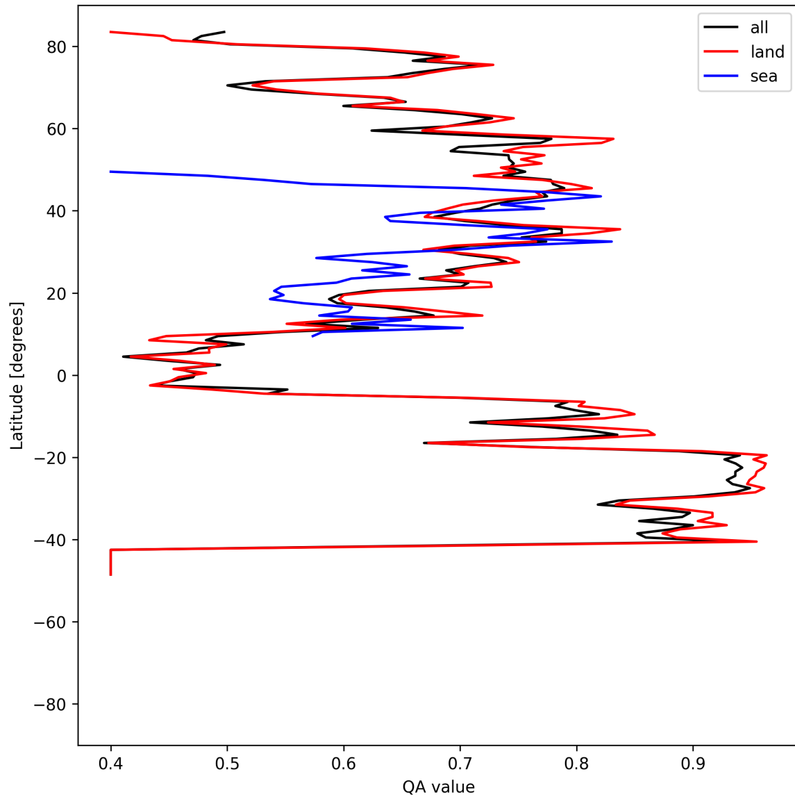
Figure 11: Zonal average of “QA value” for 2025-06-18 to 2025-06-20.
