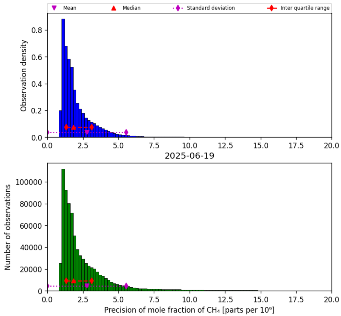
Figure 24: Histogram of “Precision of mole fraction of CH 4 ” for 2025-06-18 to 2025-06-20
