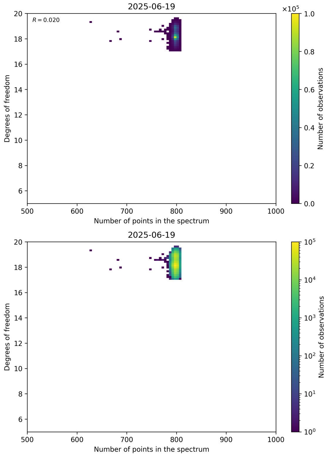
Figure 90: Scatter density plot of “Number of points in the spectrum” against “Degrees of freedom” for 2025-06-18 to 2025-06-20.
