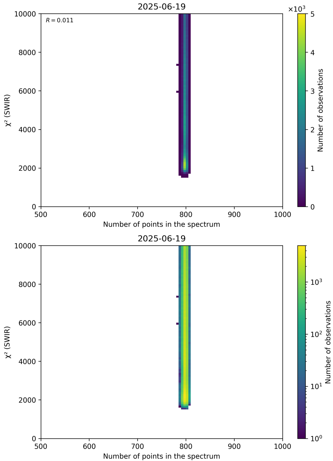
Figure 89: Scatter density plot of “Number of points in the spectrum” against “ \chi^2 (SWIR)” for 2025-06-18 to 2025-06-20.
