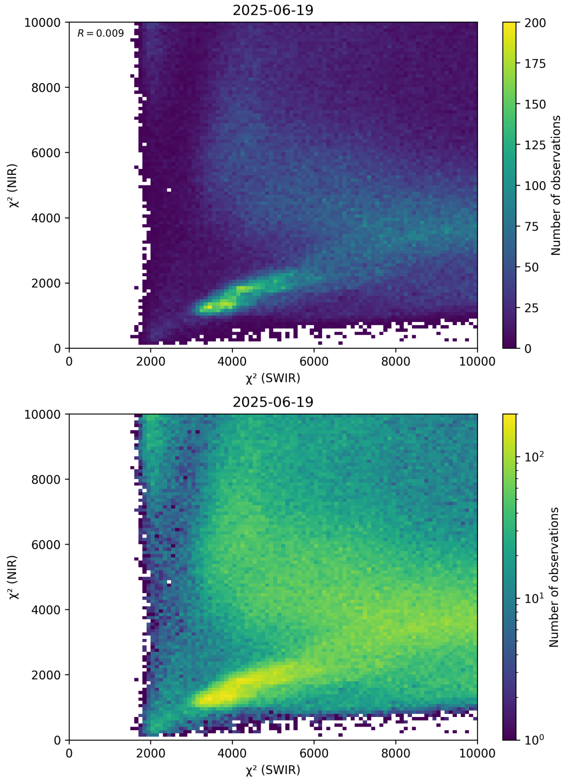
Figure 47: Scatter density plot of “ \chi^2 (SWIR)” against “ \chi^2 (NIR)” for 2025-06-18 to 2025-06-20.
