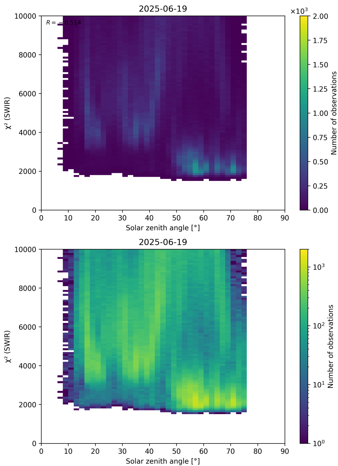
Figure 95: Scatter density plot of “Solar zenith angle” against “ \chi^2 (SWIR)” for 2025-06-18 to 2025-06-20.
