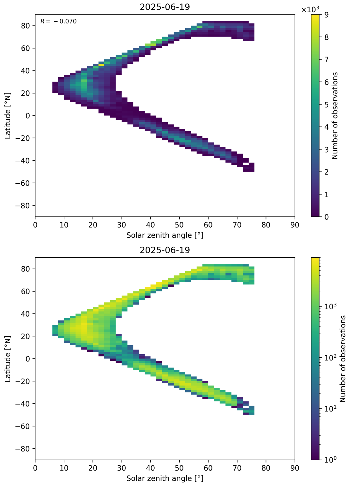
Figure 98: Scatter density plot of “Solar zenith angle” against “Latitude” for 2025-06-18 to 2025-06-20.
