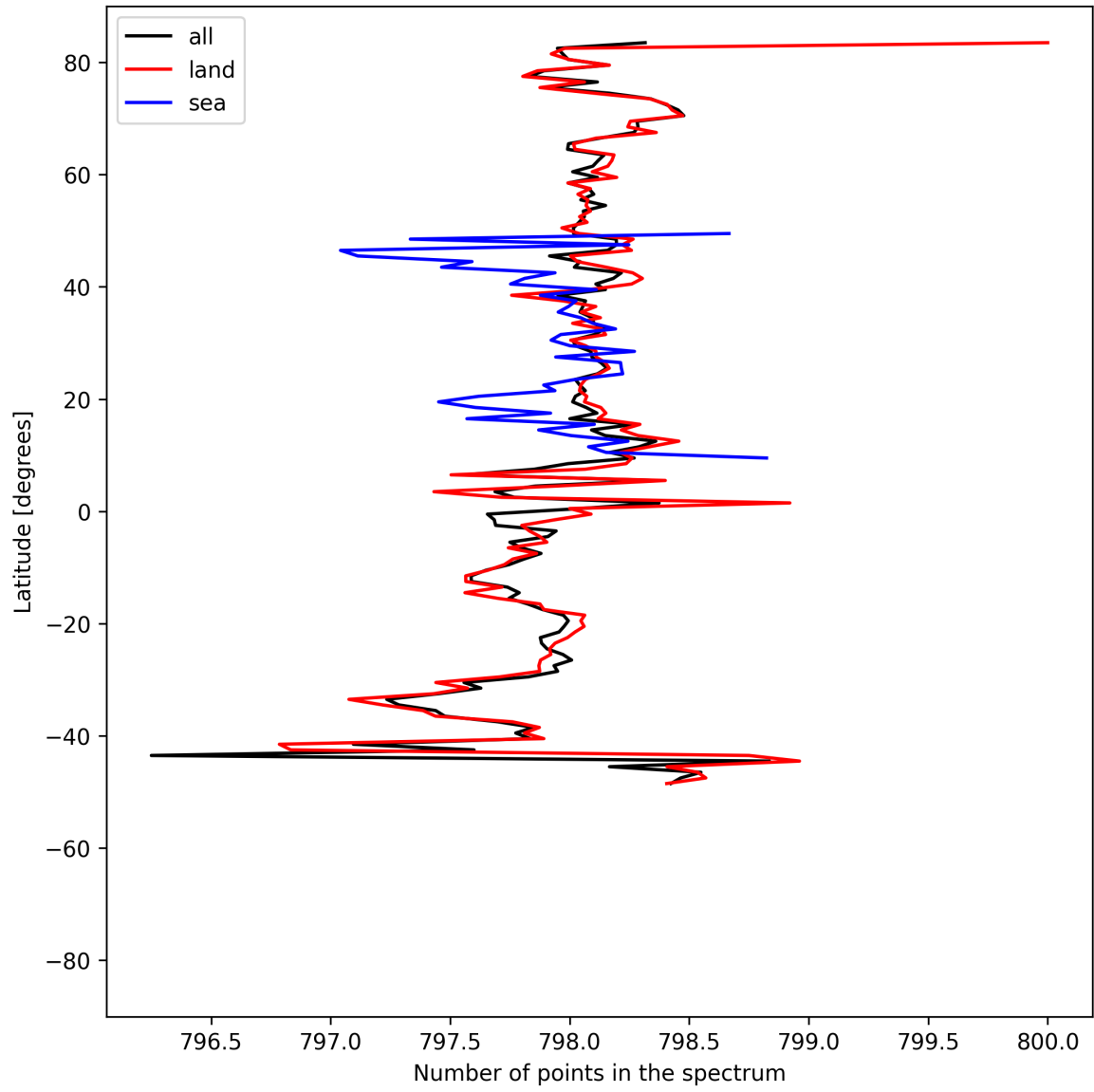
Figure 15: Zonal average of “Number of points in the spectrum” for 2025-06-18 to 2025-06-20.
