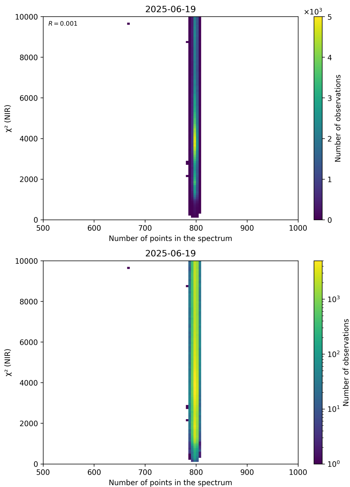
Figure 88: Scatter density plot of “Number of points in the spectrum” against “ \chi^2 (NIR)” for 2025-06-18 to 2025-06-20.
