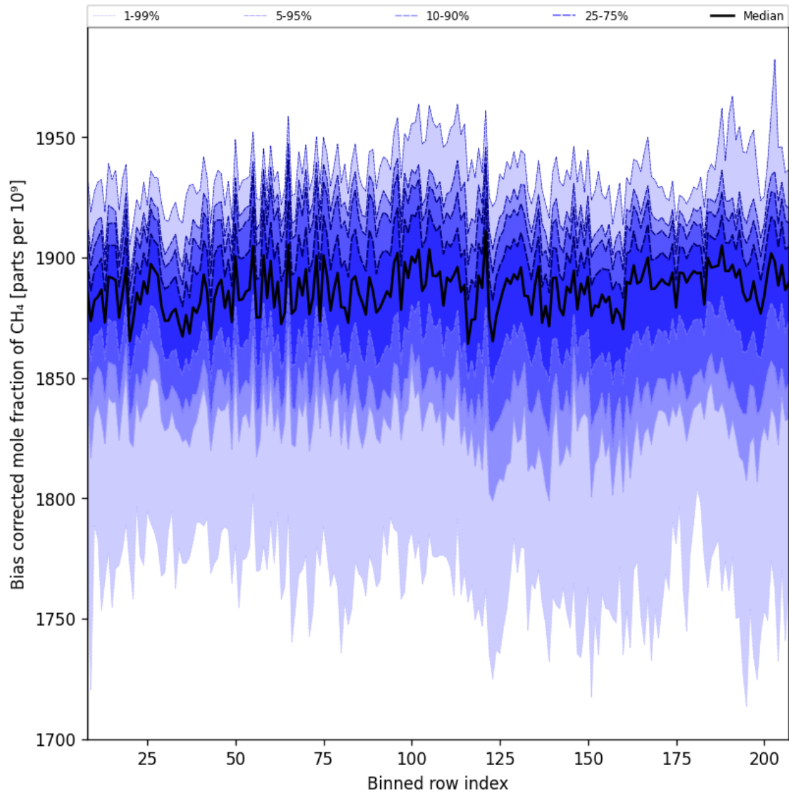
Figure 36: Along track statistics of “Bias corrected mole fraction of CH 4 ” for 2025-06-18 to 2025-06-20
