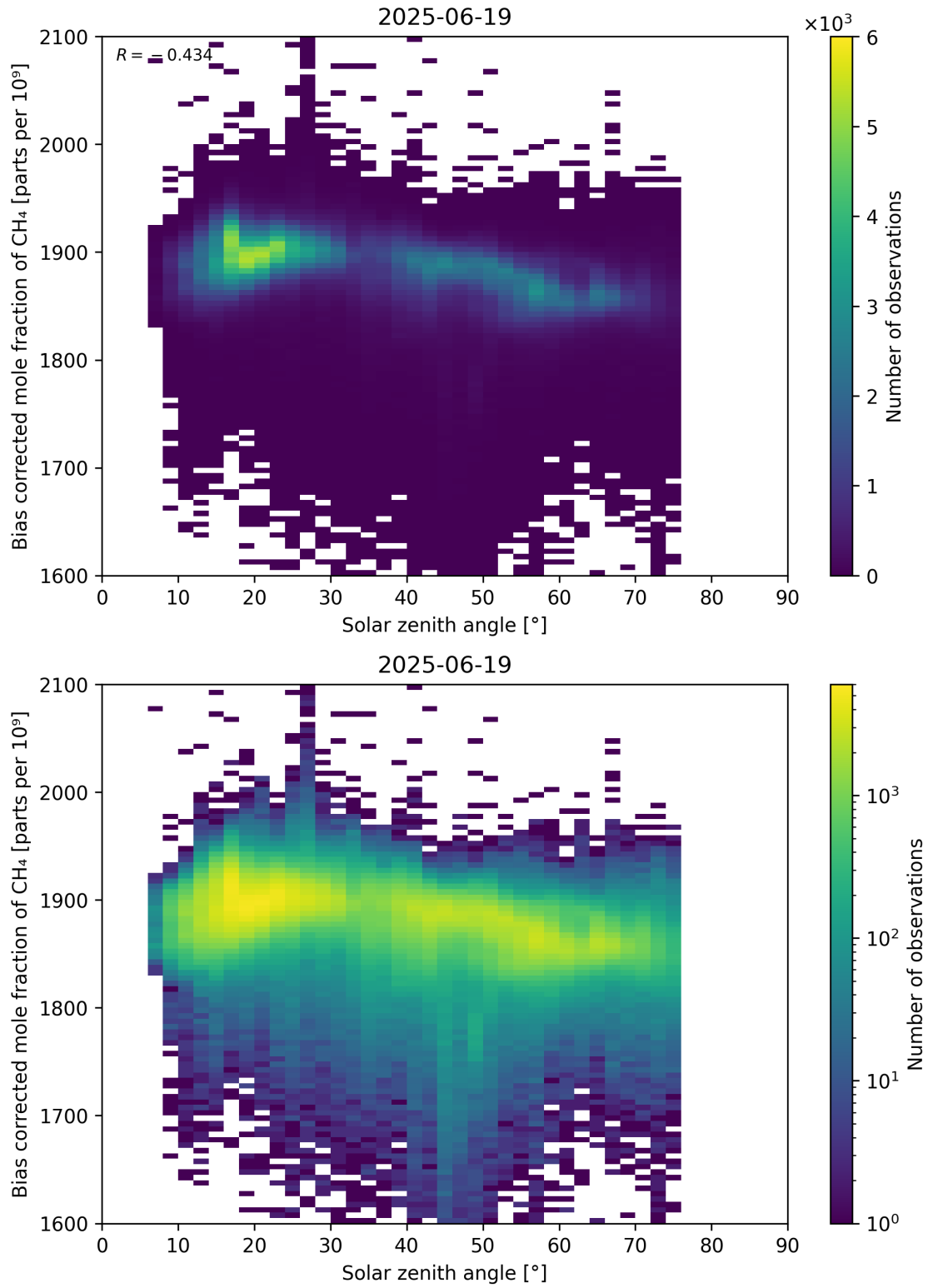
Figure 100: Scatter density plot of “Solar zenith angle” against “Bias corrected mole fraction of CH 4 ” for 2025-06-18 to 2025-06-20.
