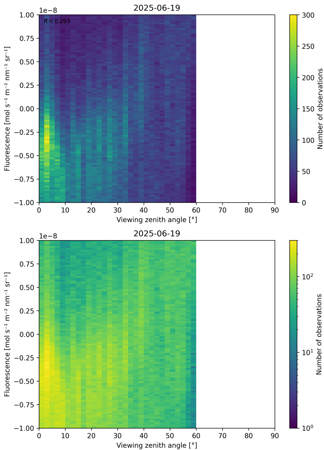
Figure 108: Scatter density plot of “Viewing zenith angle” against “Fluorescence” for 2025-06-18 to 2025-06-20.
