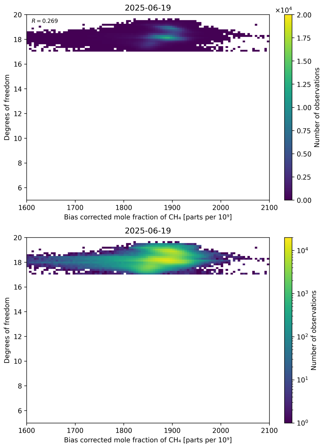
Figure 65: Scatter density plot of “Bias corrected mole fraction of CH 4 ” against “Degrees of freedom” for 2025-06-18 to 2025-06-20.
