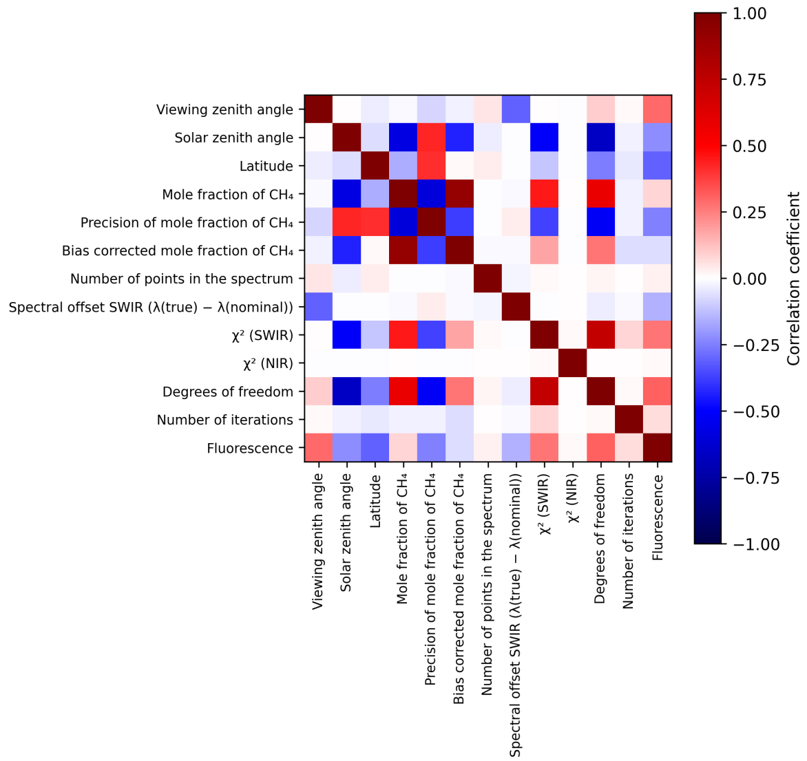
Figure 2: Map of correlation matrix for 2025-06-18 to 2025-06-20.
