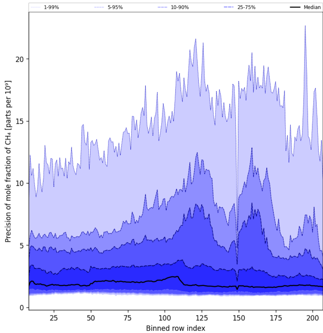
Figure 35: Along track statistics of “Precision of mole fraction of CH 4 ” for 2025-06-18 to 2025-06-20
