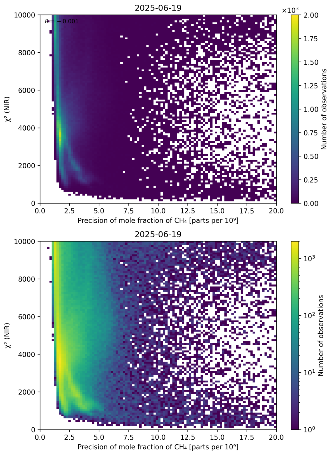
Figure 78: Scatter density plot of “Precision of mole fraction of CH 4 ” against “ \chi^2 (NIR)” for 2025-06-18 to 2025-06-20.
