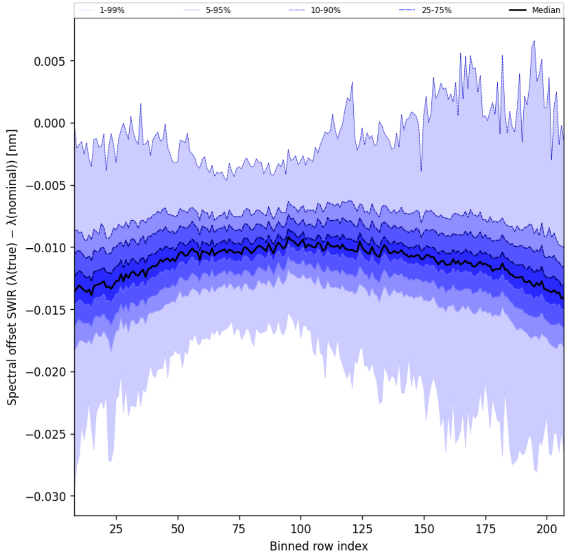
Figure 38: Along track statistics of “Spectral offset SWIR ( \lambda_{\text{true}} - \lambda_{\text{nominal}} )” for 2025-06-18 to 2025-06-20
