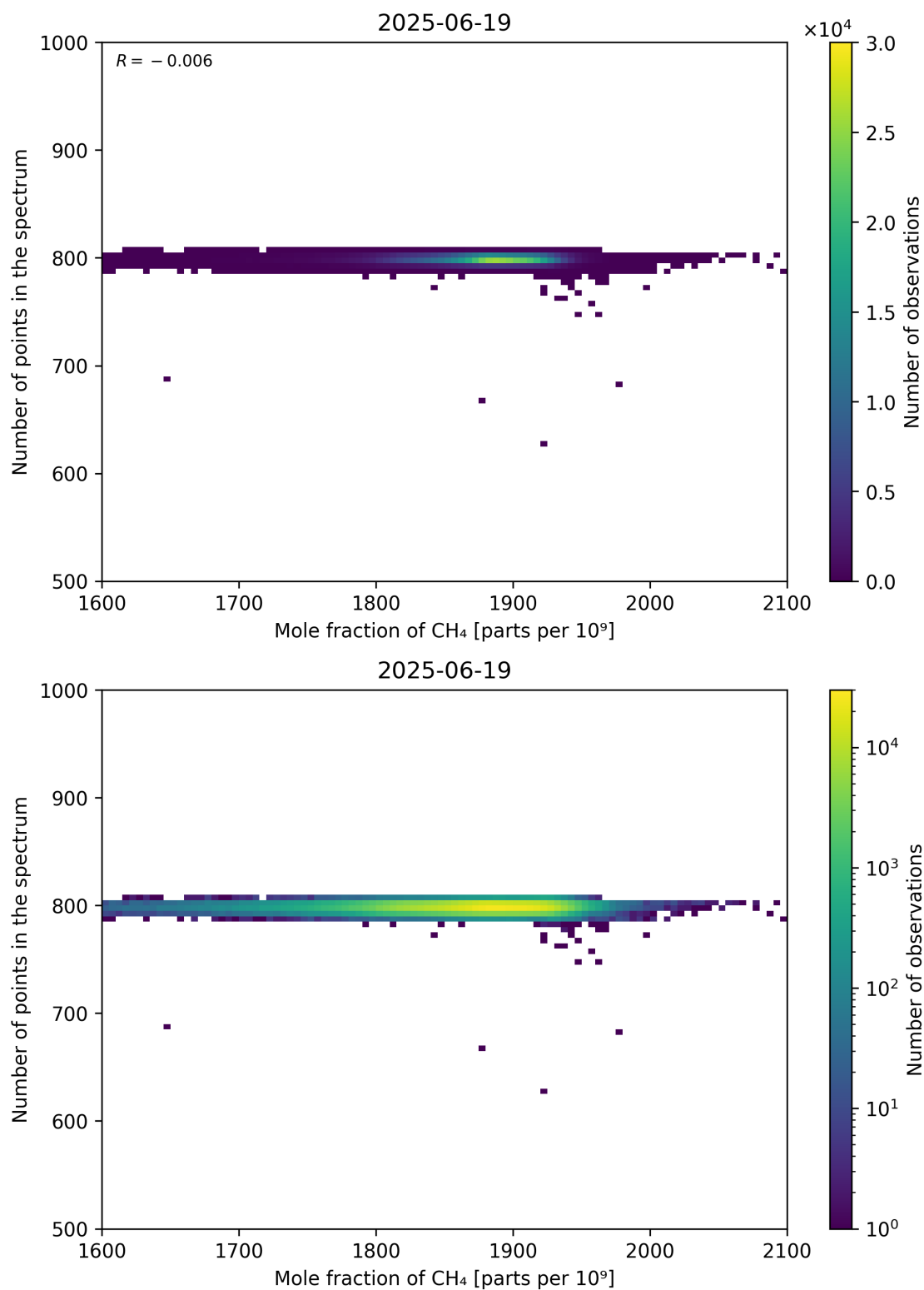
Figure 77: Scatter density plot of “Mole fraction of CH 4 ” against “Number of points in the spectrum” for 2025-06-18 to 2025-06-20.
