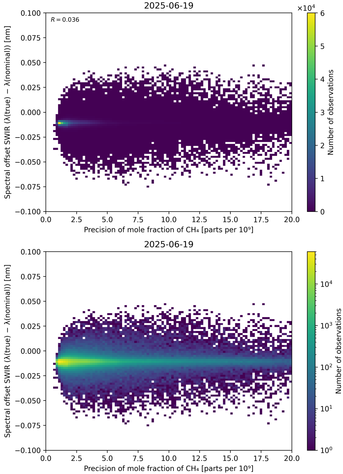
Figure 85: Scatter density plot of “Precision of mole fraction of CH 4 ” against “Spectral offset SWIR ( \lambda_{\text{true}} - \lambda_{\text{nominal}} )” for 2025-06-18 to 2025-06-20.
