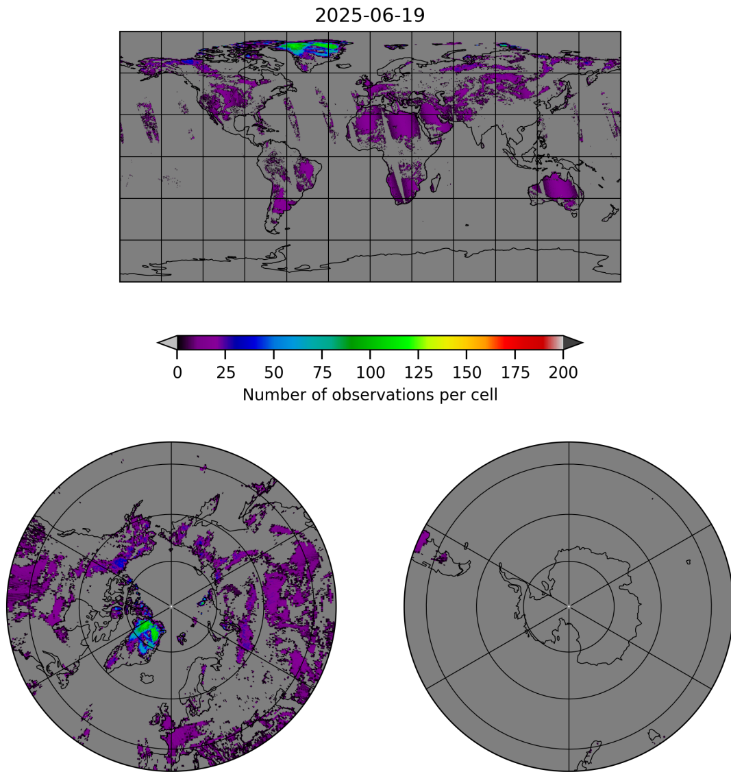
Figure 10: Map of the number of observations for 2025-06-18 to 2025-06-20
