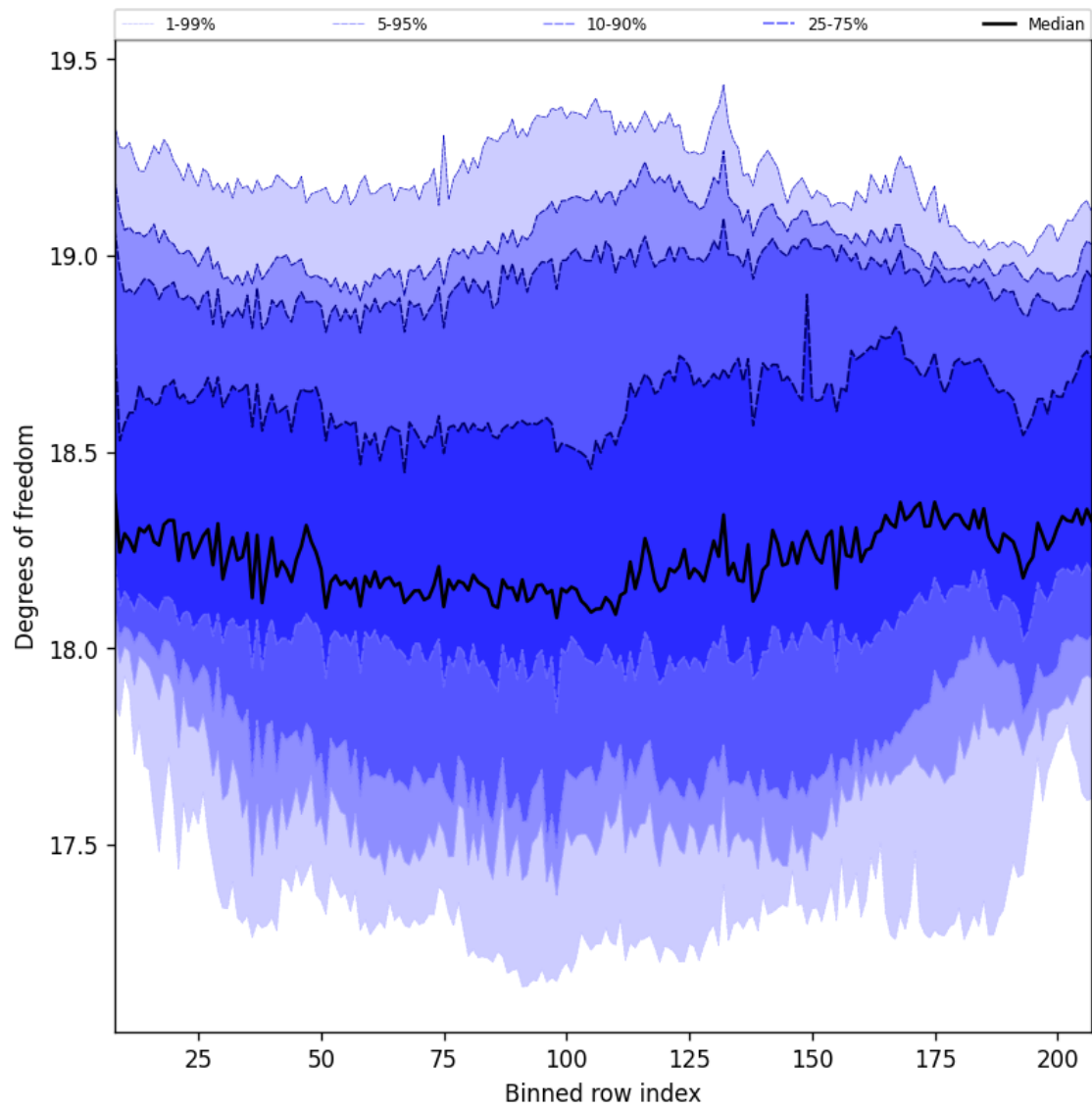
Figure 41: Along track statistics of “Degrees of freedom” for 2025-06-18 to 2025-06-20
