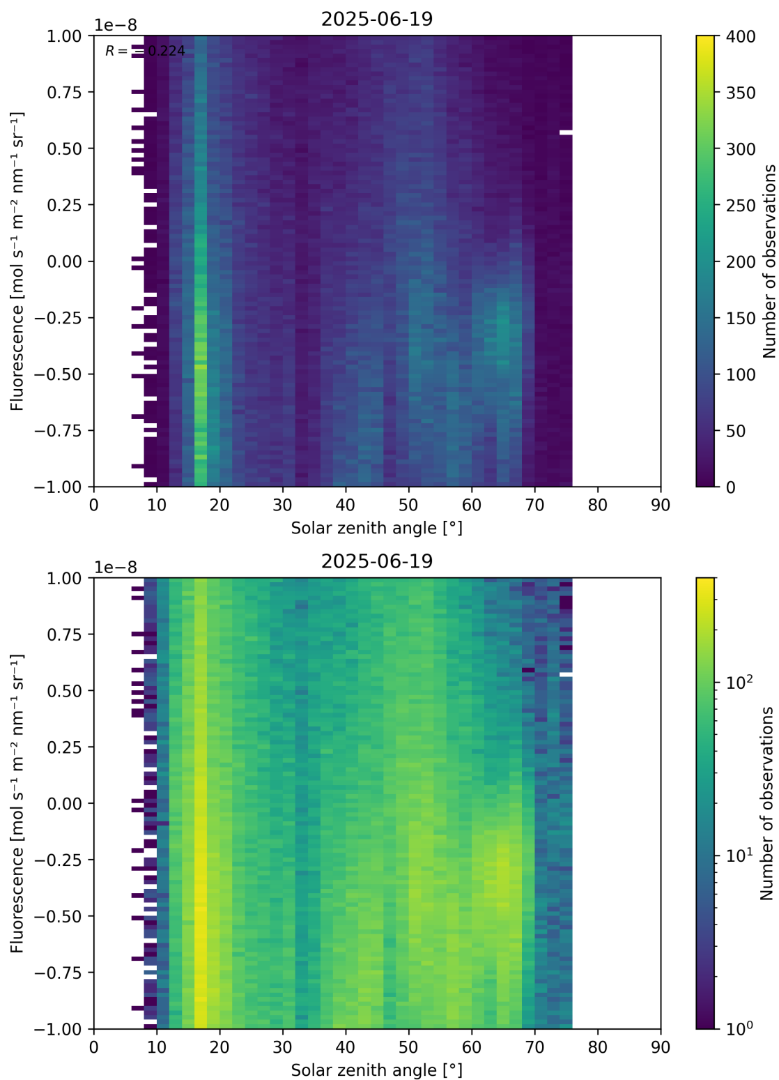
Figure 97: Scatter density plot of “Solar zenith angle” against “Fluorescence” for 2025-06-18 to 2025-06-20.
