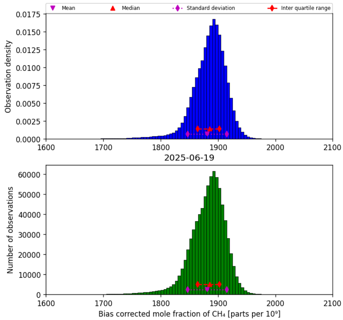
Figure 25: Histogram of “Bias corrected mole fraction of CH 4 ” for 2025-06-18 to 2025-06-20
