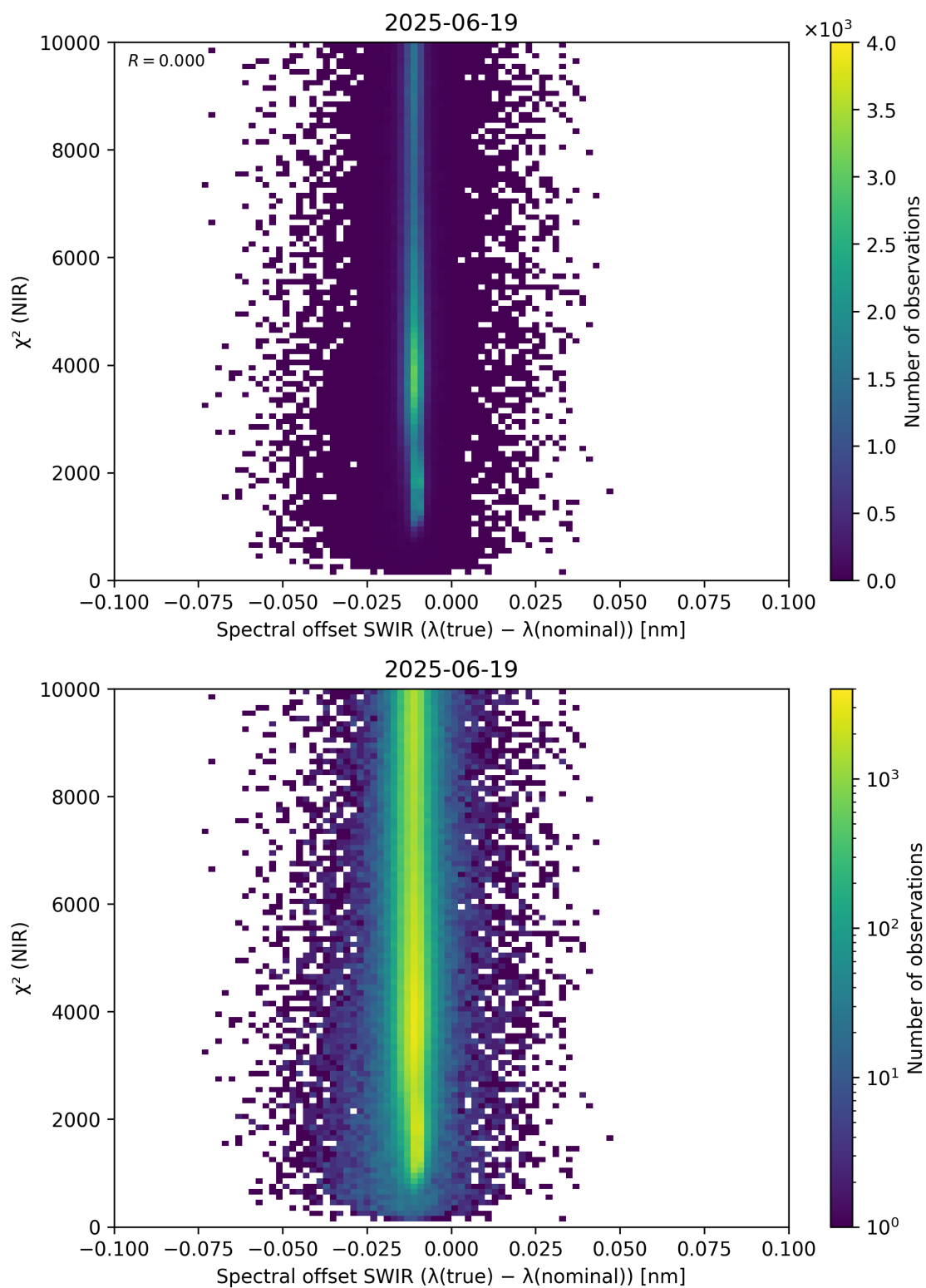
Figure 117: Scatter density plot of “Spectral offset SWIR ( \lambda_{\text{true}} - \lambda_{\text{nominal}} )” against “ \chi^2 (NIR)” for 2025-06-18 to 2025-06-20.
