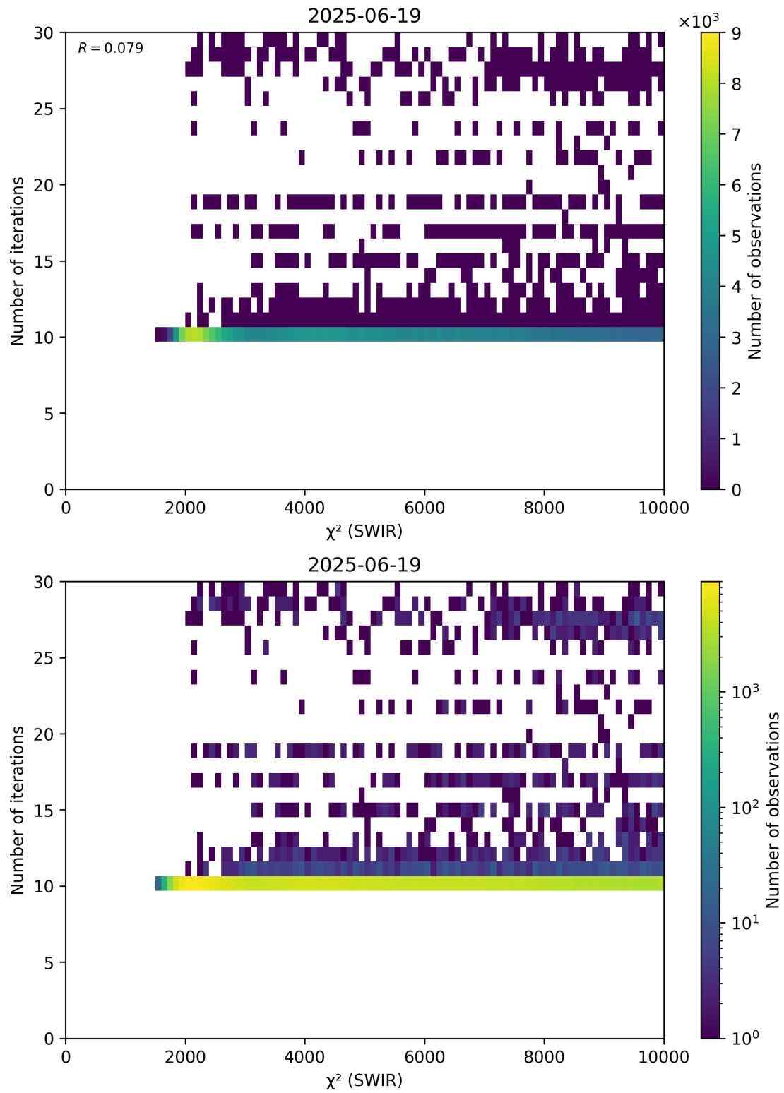
Figure 50: Scatter density plot of “ \chi^2 (SWIR)” against “Number of iterations” for 2025-06-18 to 2025-06-20.
