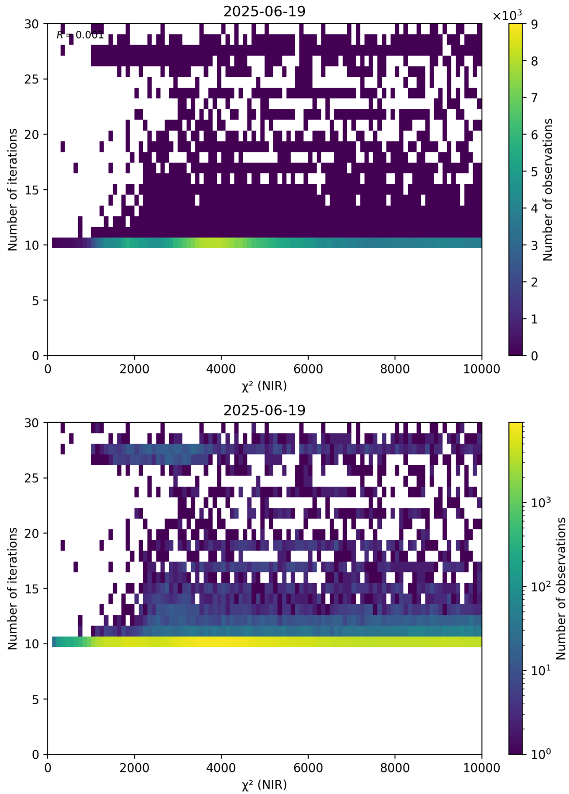
Figure 46: Scatter density plot of “ \chi^2 (NIR)” against “Number of iterations” for 2025-06-18 to 2025-06-20.
