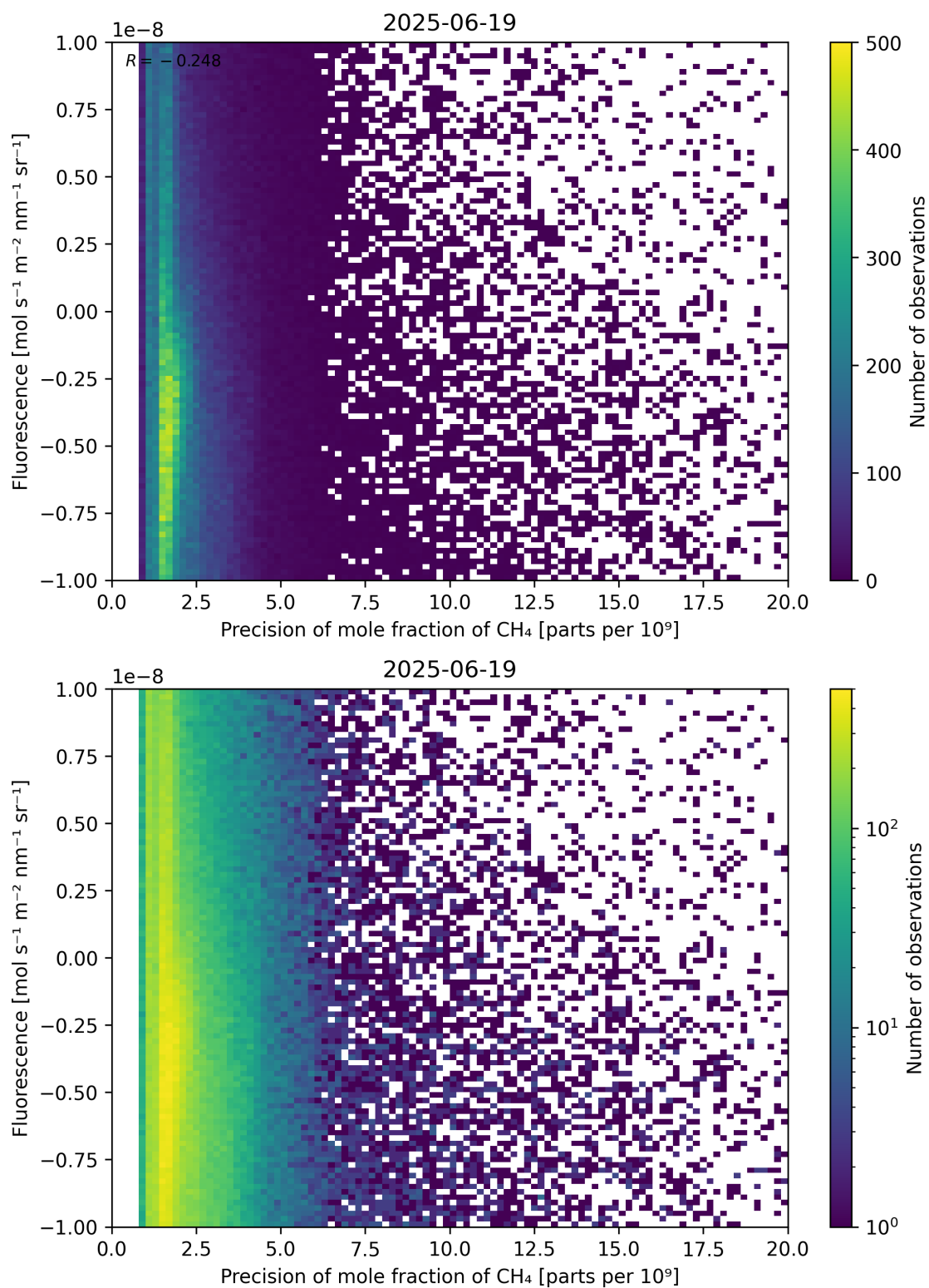
Figure 81: Scatter density plot of “Precision of mole fraction of CH 4 ” against “Fluorescence” for 2025-06-18 to 2025-06-20.
