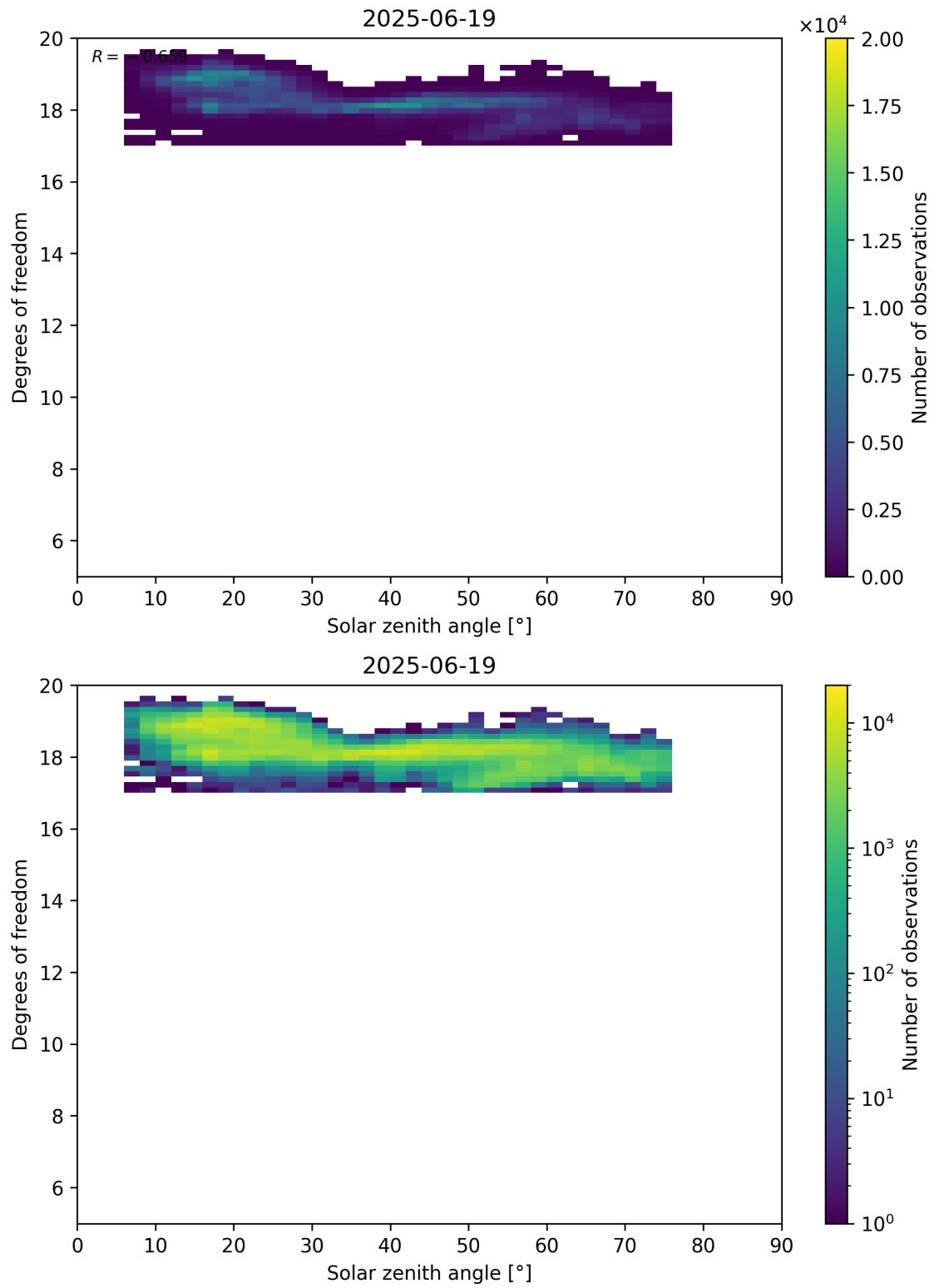
Figure 96: Scatter density plot of “Solar zenith angle” against “Degrees of freedom” for 2025-06-18 to 2025-06-20.
