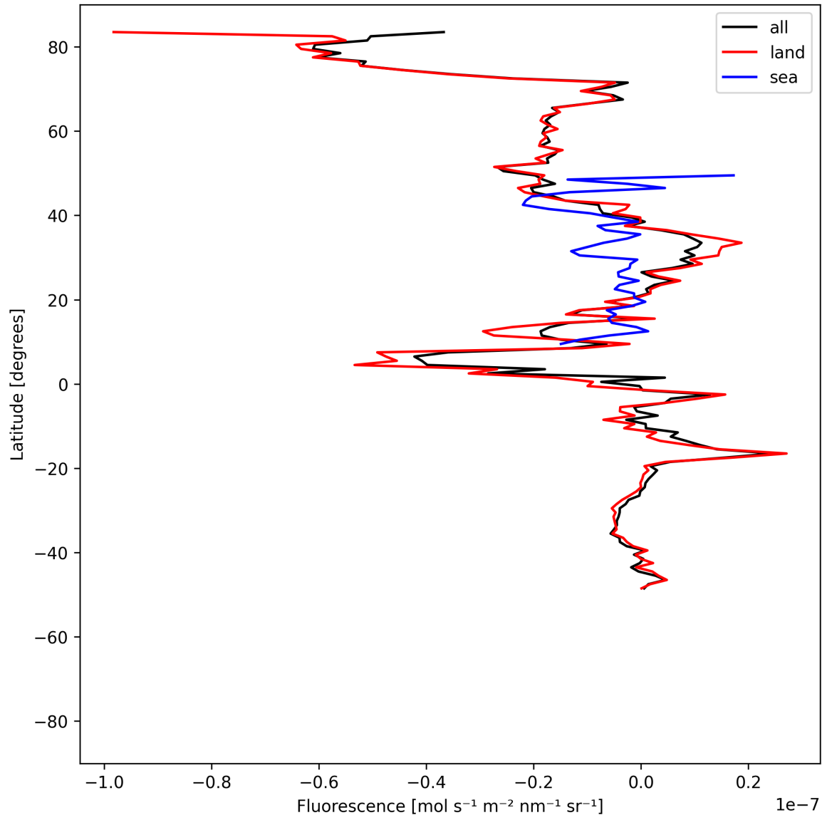
Figure 21: Zonal average of “Fluorescence” for 2025-06-18 to 2025-06-20.
