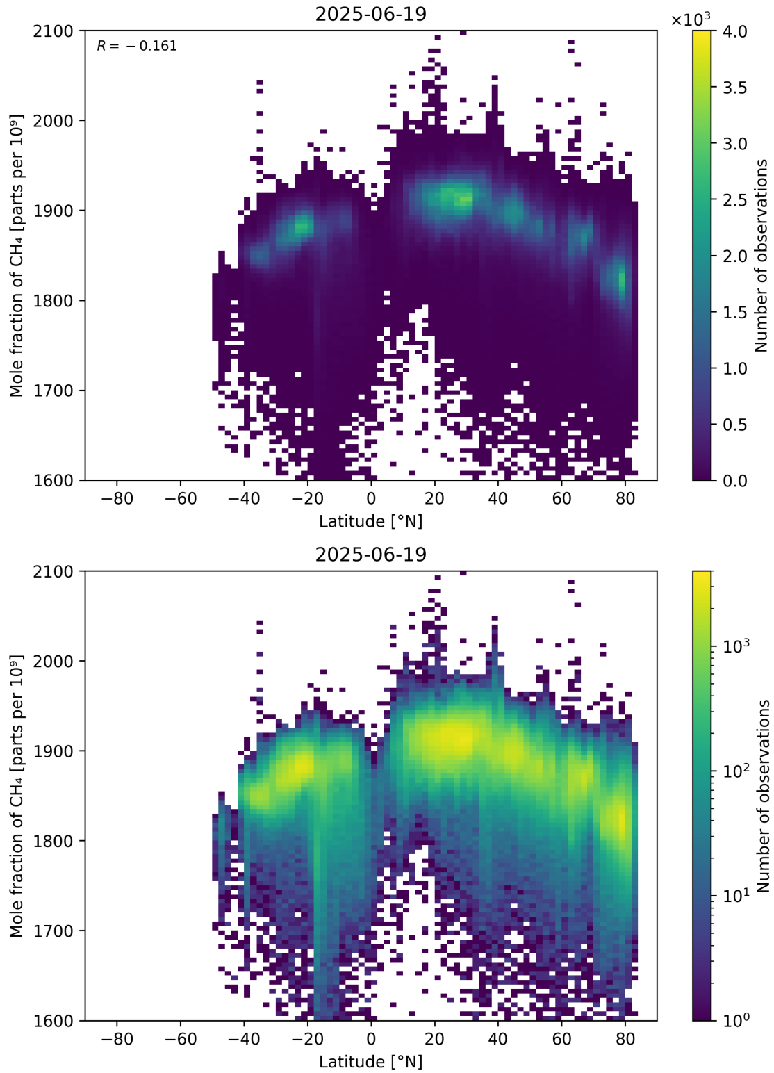
Figure 57: Scatter density plot of “Latitude” against “Mole fraction of CH 4 ” for 2025-06-18 to 2025-06-20.
