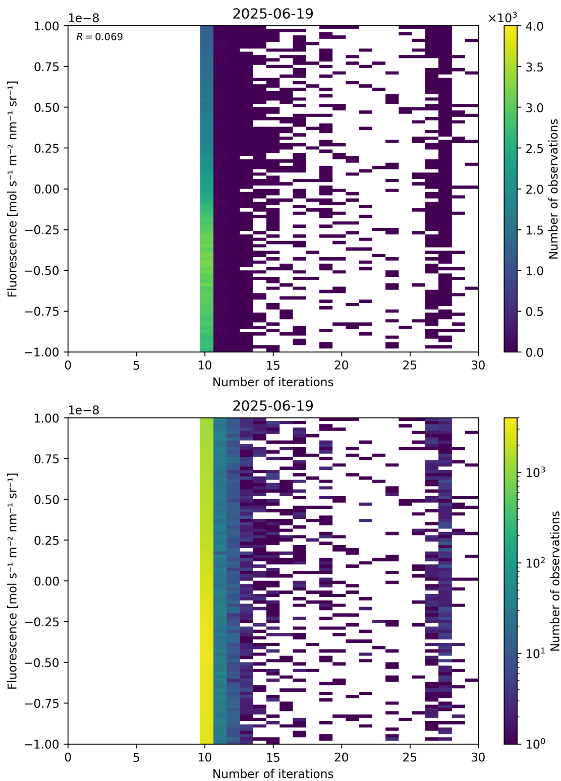
Figure 87: Scatter density plot of "Number of iterations" against "Fluorescence" for 2025-06-18 to 2025-06-20.
