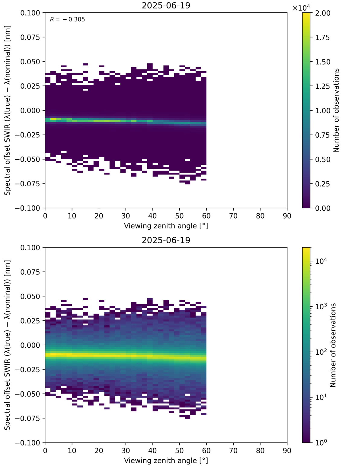
Figure 116: Scatter density plot of “Viewing zenith angle” against “Spectral offset SWIR ( \lambda_{\text{true}} - \lambda_{\text{nominal}} )” for 2025-06-18 to 2025-06-20.
