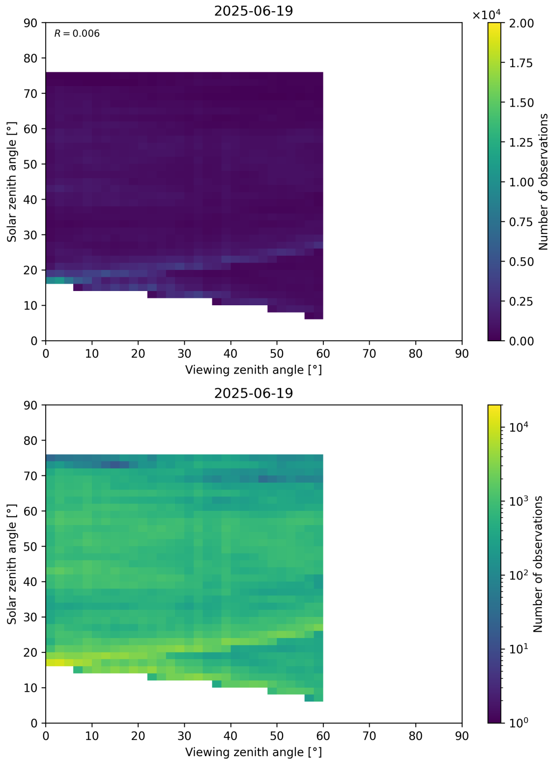
Figure 115: Scatter density plot of “Viewing zenith angle” against “Solar zenith angle” for 2025-06-18 to 2025-06-20.
