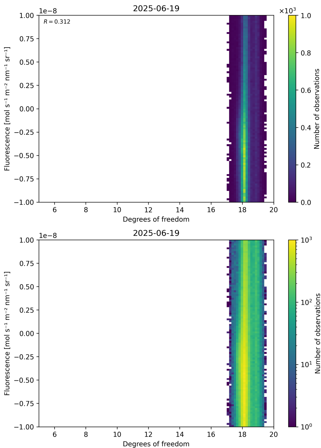
Figure 51: Scatter density plot of “Degrees of freedom” against “Fluorescence” for 2025-06-18 to 2025-06-20.
