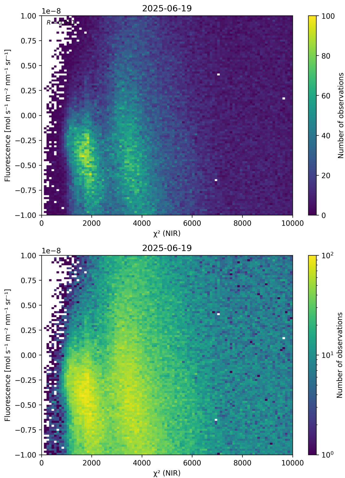
Figure 45: Scatter density plot of “ \chi^2 (NIR)” against “Fluorescence” for 2025-06-18 to 2025-06-20.
