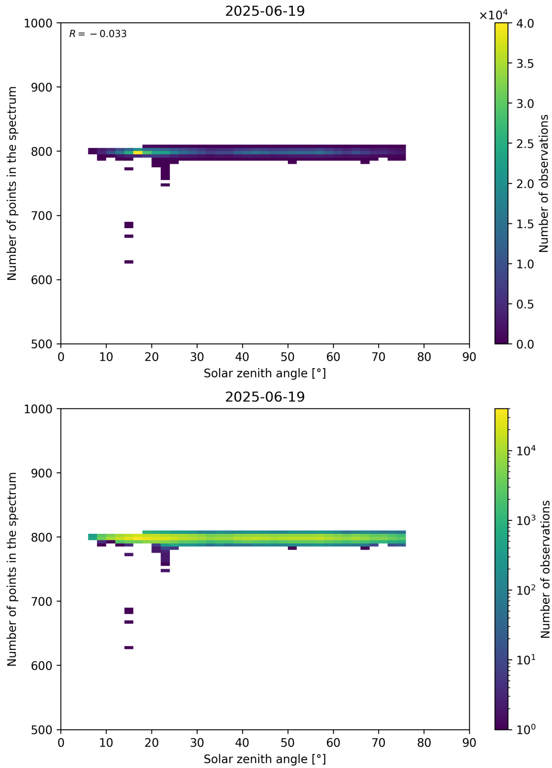
Figure 103: Scatter density plot of “Solar zenith angle” against “Number of points in the spectrum” for 2025-06-18 to 2025-06-20.
