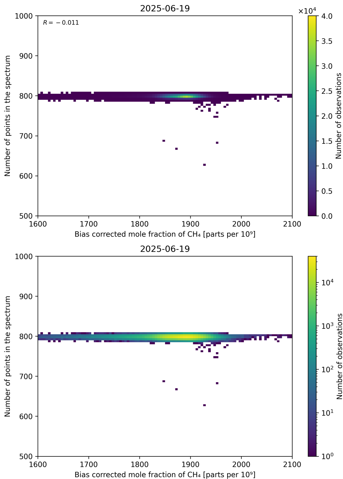
Figure 68: Scatter density plot of “Bias corrected mole fraction of CH 4 ” against “Number of points in the spectrum” for 2025-06-18 to 2025-06-20.
