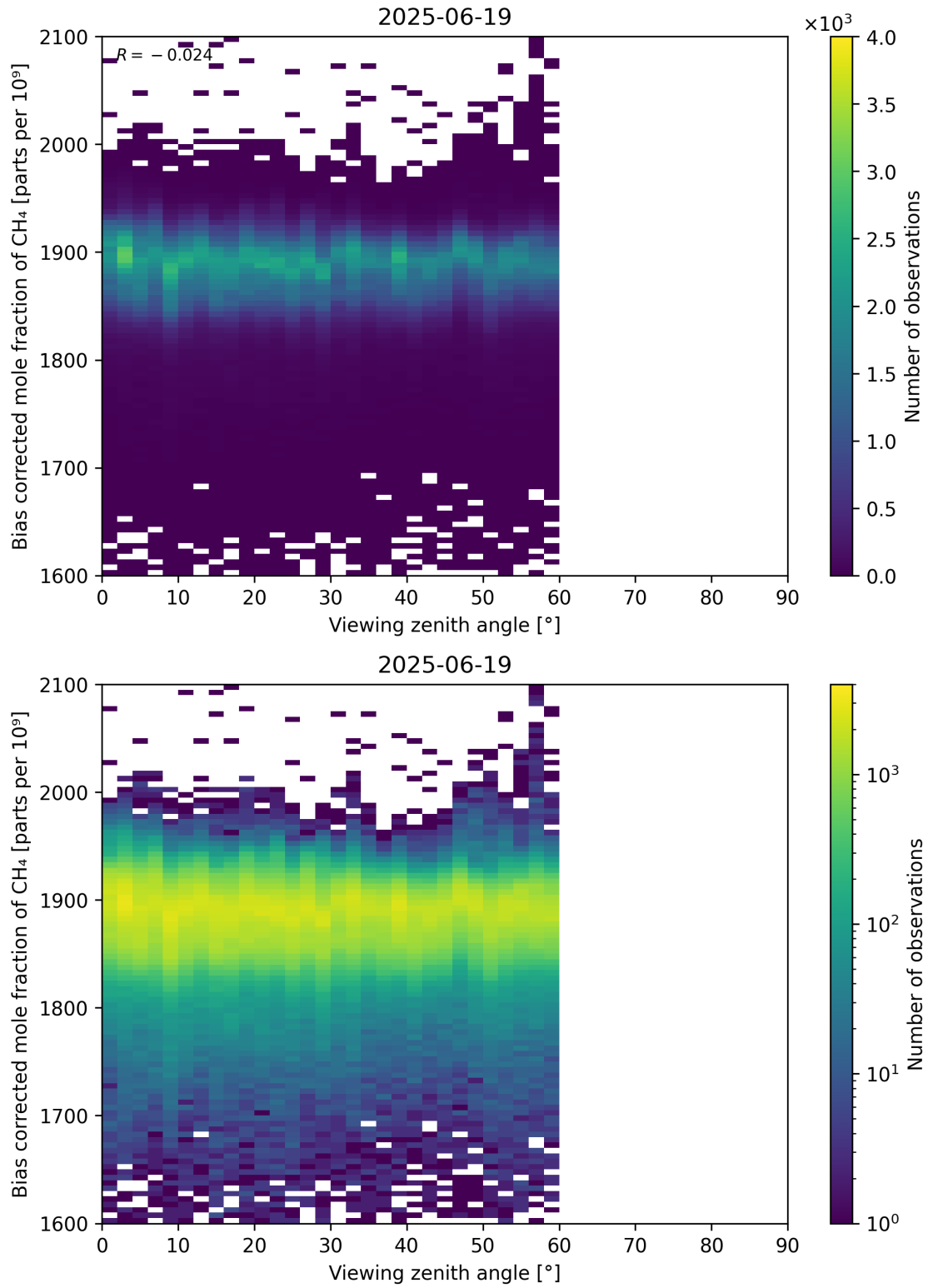
Figure 111: Scatter density plot of “Viewing zenith angle” against “Bias corrected mole fraction of CH 4 ” for 2025-06-18 to 2025-06-20.
