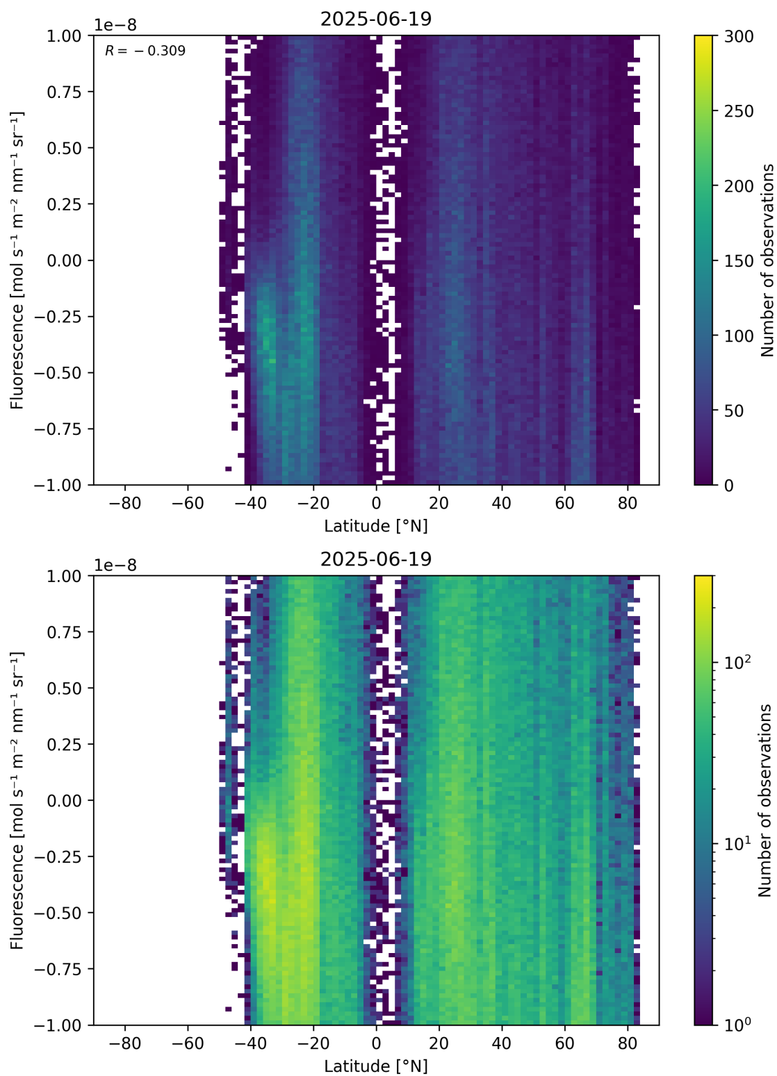
Figure 56: Scatter density plot of “Latitude” against “Fluorescence” for 2025-06-18 to 2025-06-20.
