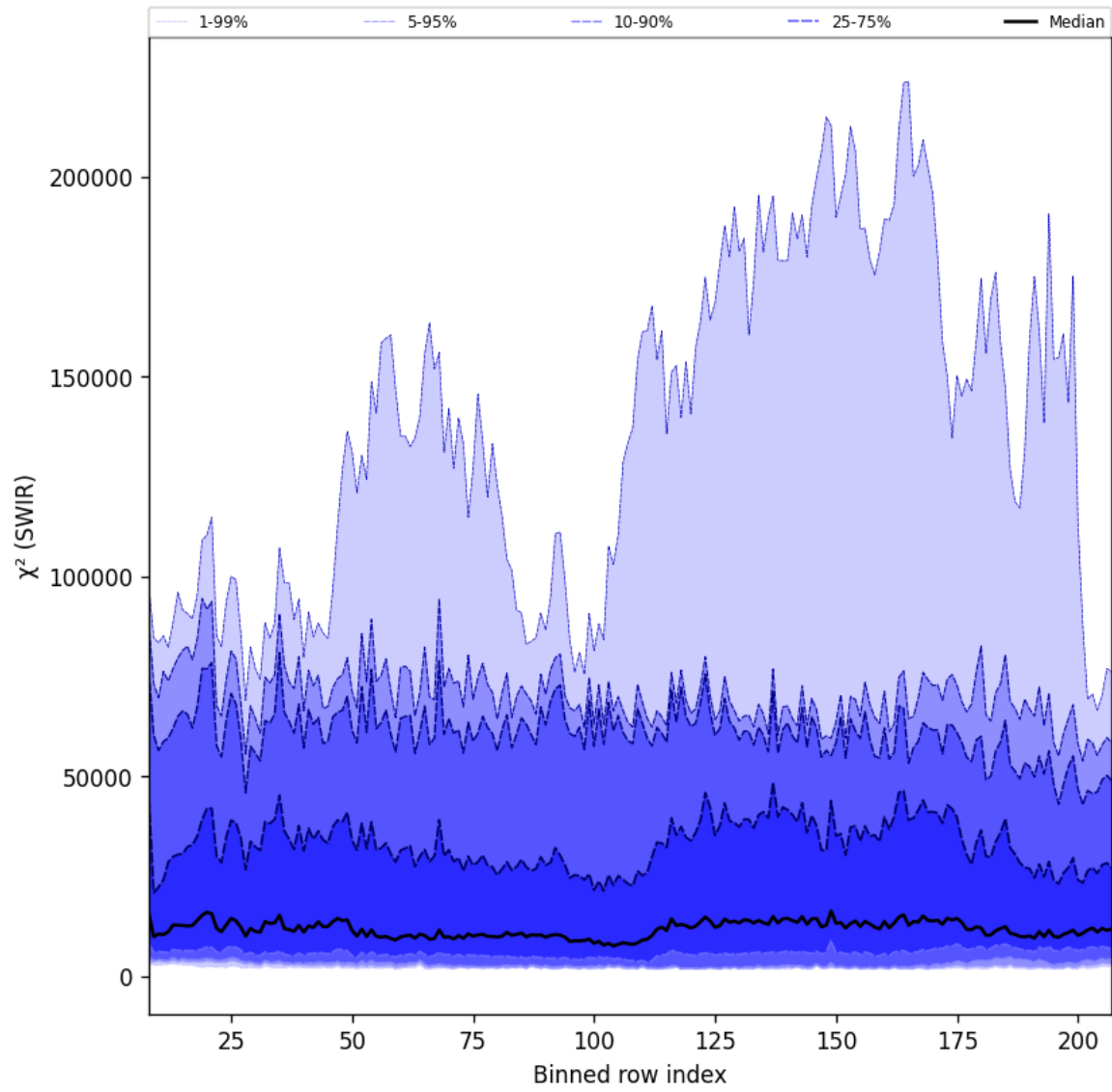
Figure 39: Along track statistics of " \chi^2 (SWIR)" for 2025-06-18 to 2025-06-20
