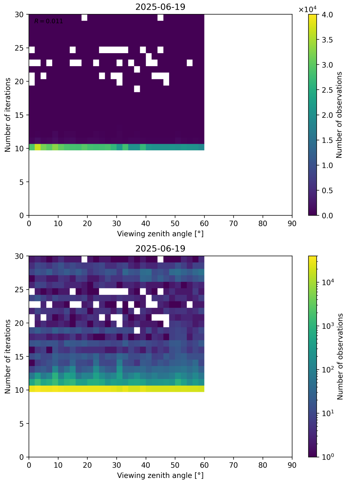
Figure 113: Scatter density plot of “Viewing zenith angle” against “Number of iterations” for 2025-06-18 to 2025-06-20.
