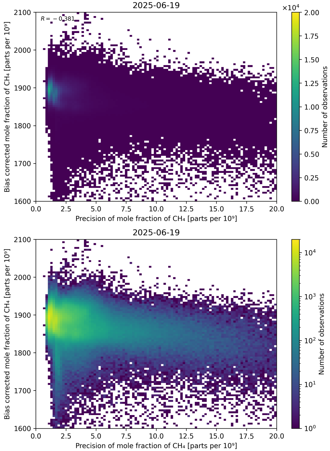
Figure 82: Scatter density plot of “Precision of mole fraction of CH 4 ” against “Bias corrected mole fraction of CH 4 ” for 2025-06-18 to 2025-06-20.
