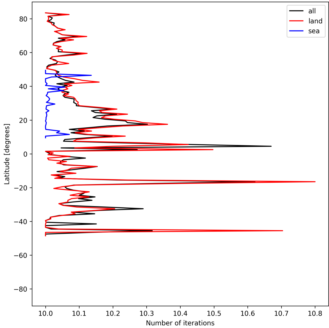
Figure 20: Zonal average of “Number of iterations” for 2025-06-18 to 2025-06-20.
