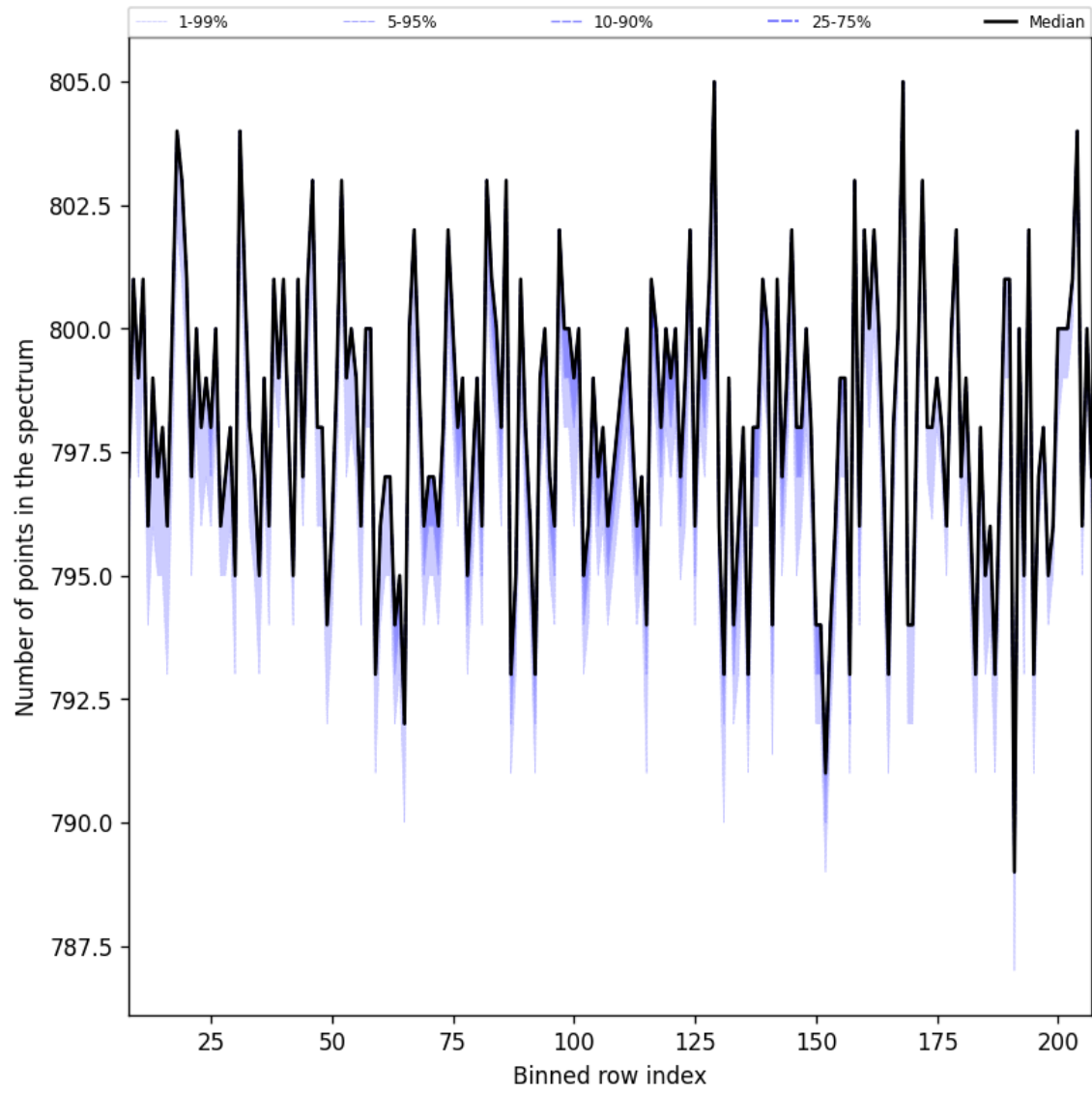
Figure 37: Along track statistics of “Number of points in the spectrum” for 2025-06-18 to 2025-06-20
