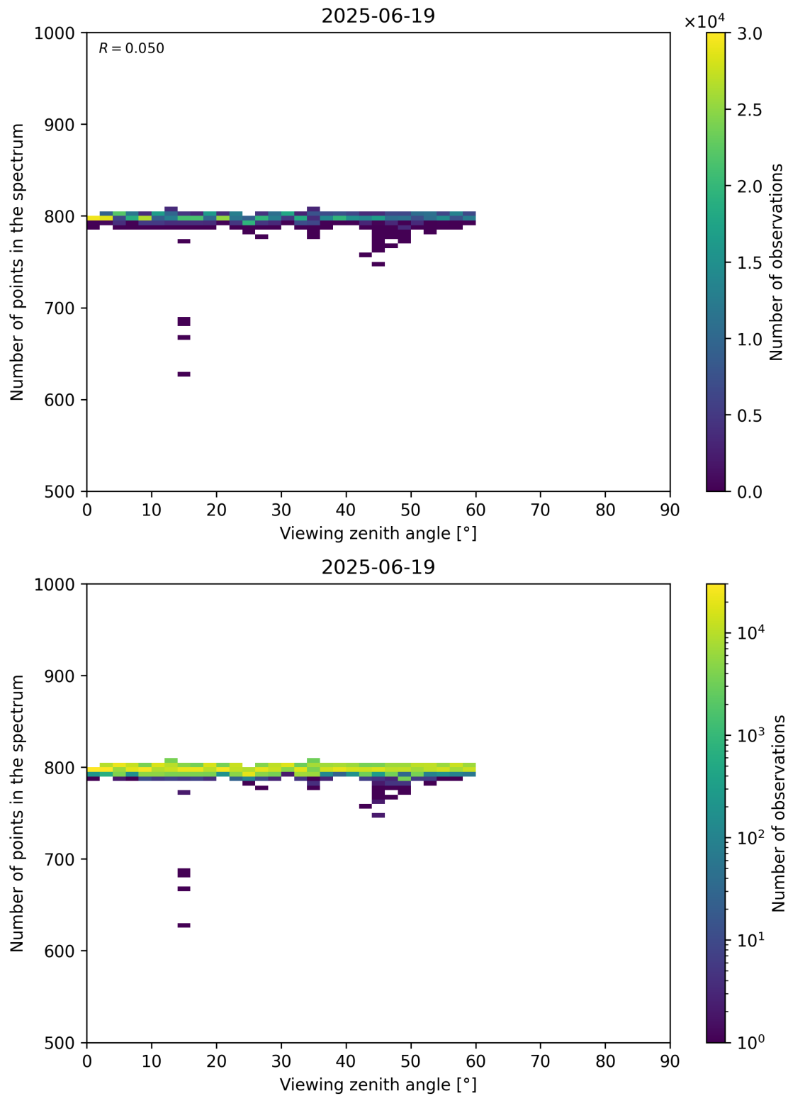
Figure 114: Scatter density plot of “Viewing zenith angle” against “Number of points in the spectrum” for 2025-06-18 to 2025-06-20.
