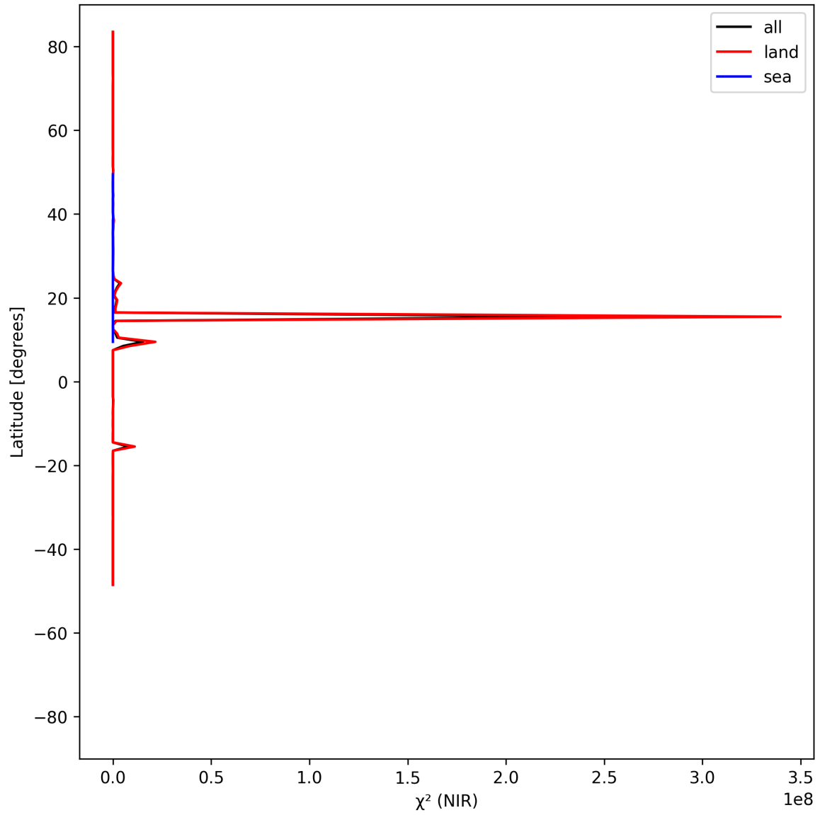
Figure 18: Zonal average of “ \chi^2 (NIR)” for 2025-06-18 to 2025-06-20.
