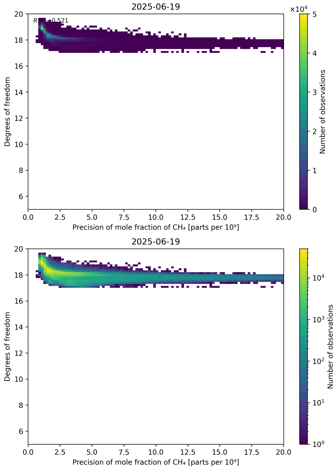
Figure 80: Scatter density plot of “Precision of mole fraction of CH 4 ” against “Degrees of freedom” for 2025-06-18 to 2025-06-20.
