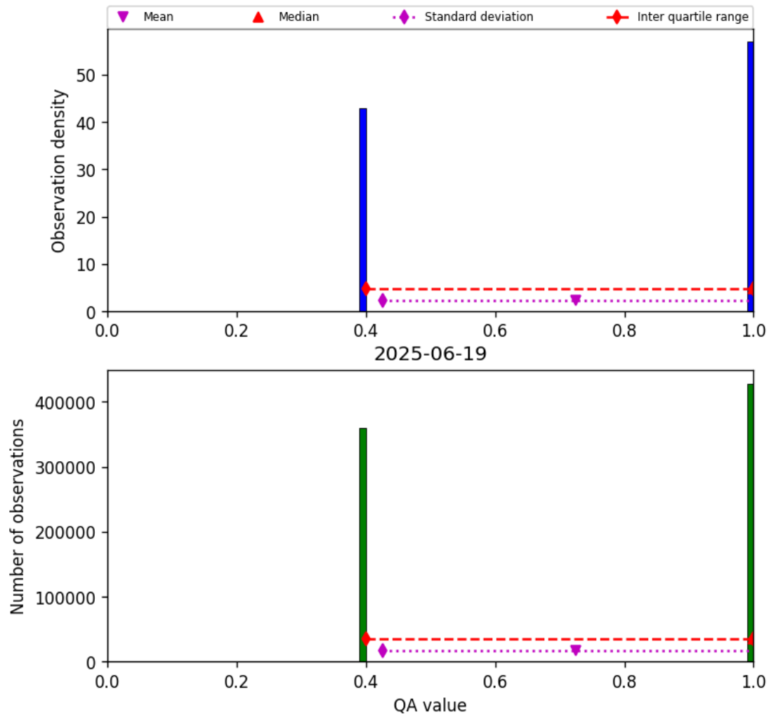
Figure 22: Histogram of “QA value” for 2025-06-18 to 2025-06-20
