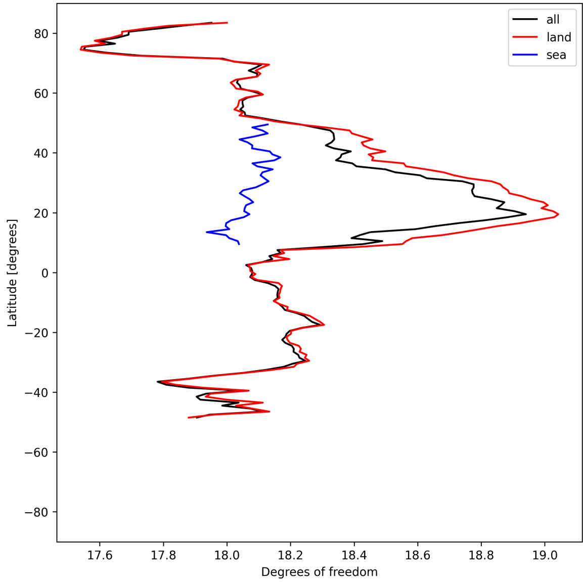
Figure 19: Zonal average of “Degrees of freedom” for 2025-06-18 to 2025-06-20.
