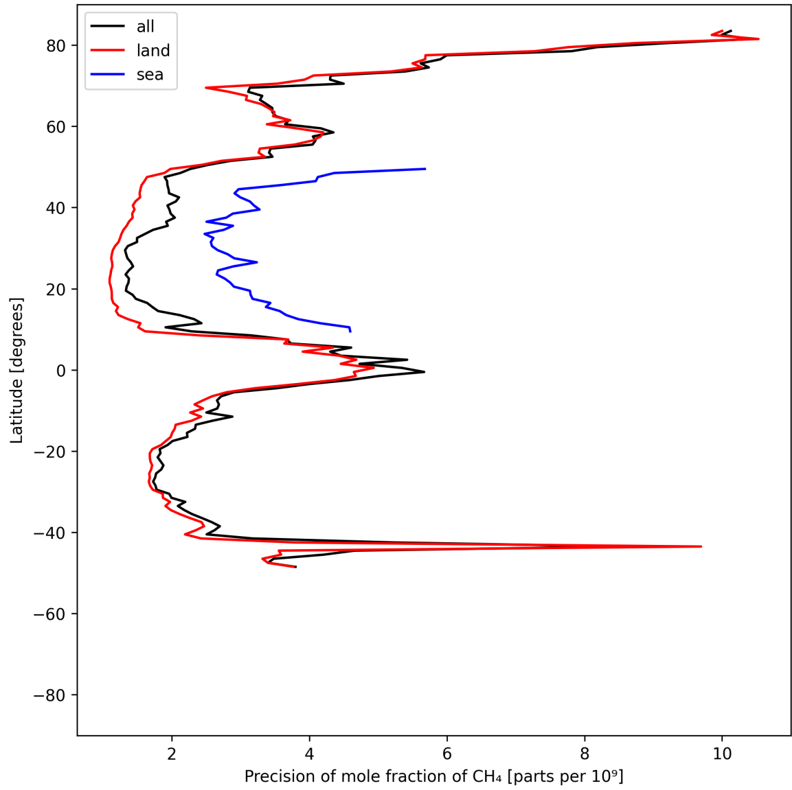
Figure 13: Zonal average of “Precision of mole fraction of CH 4 ” for 2025-06-18 to 2025-06-20.
