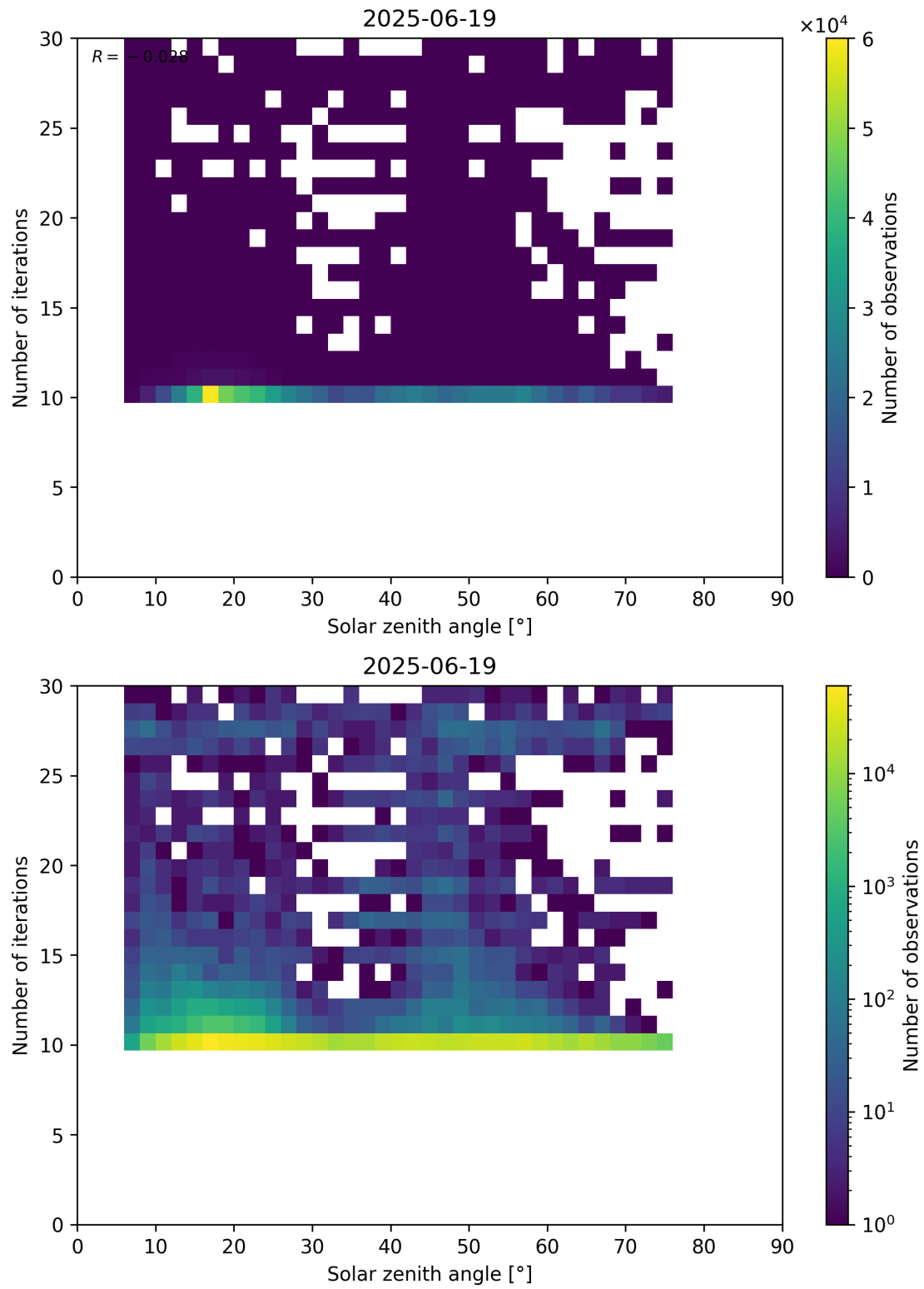
Figure 102: Scatter density plot of “Solar zenith angle” against “Number of iterations” for 2025-06-18 to 2025-06-20.
