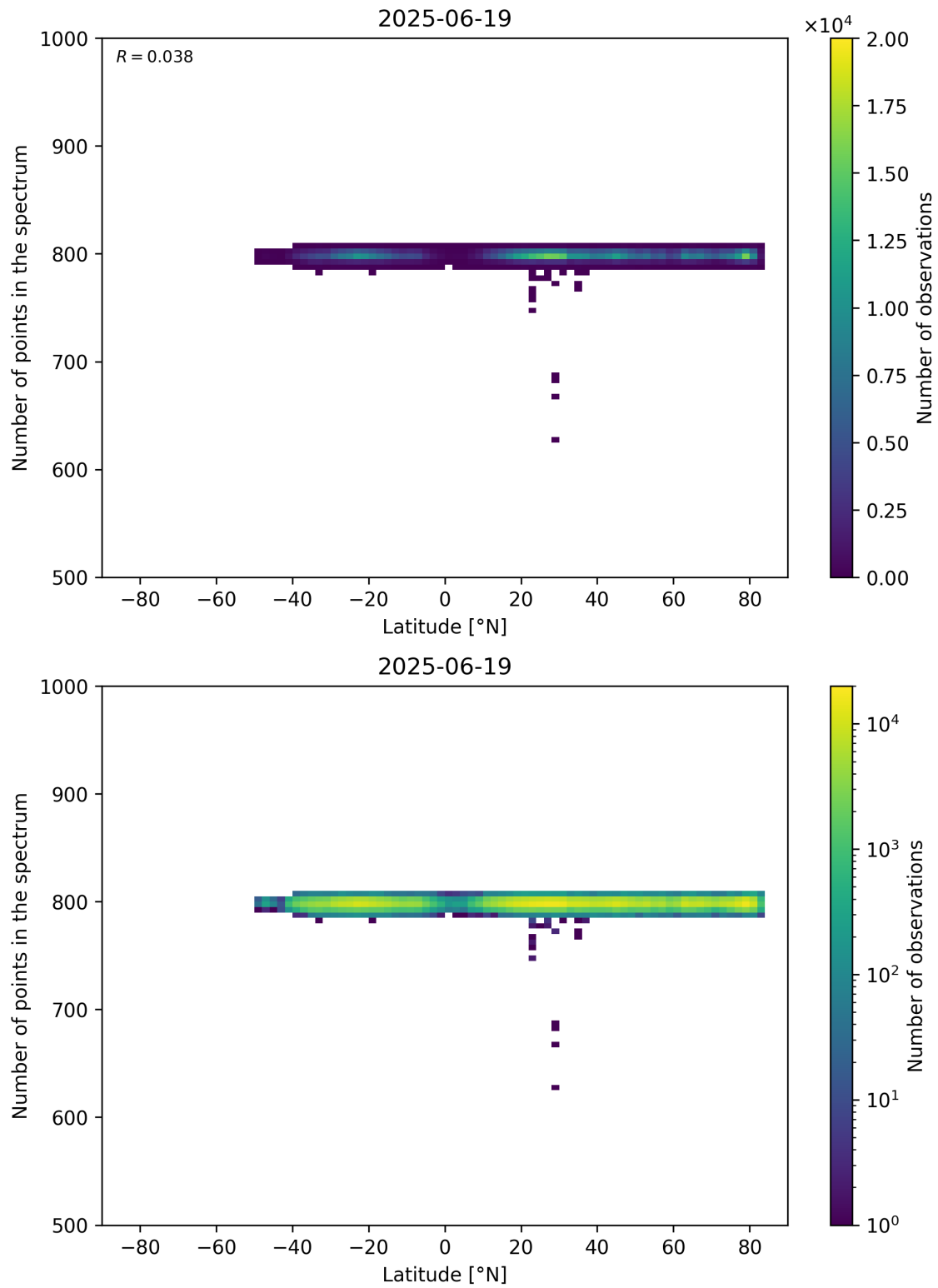
Figure 61: Scatter density plot of “Latitude” against “Number of points in the spectrum” for 2025-06-18 to 2025-06-20.
