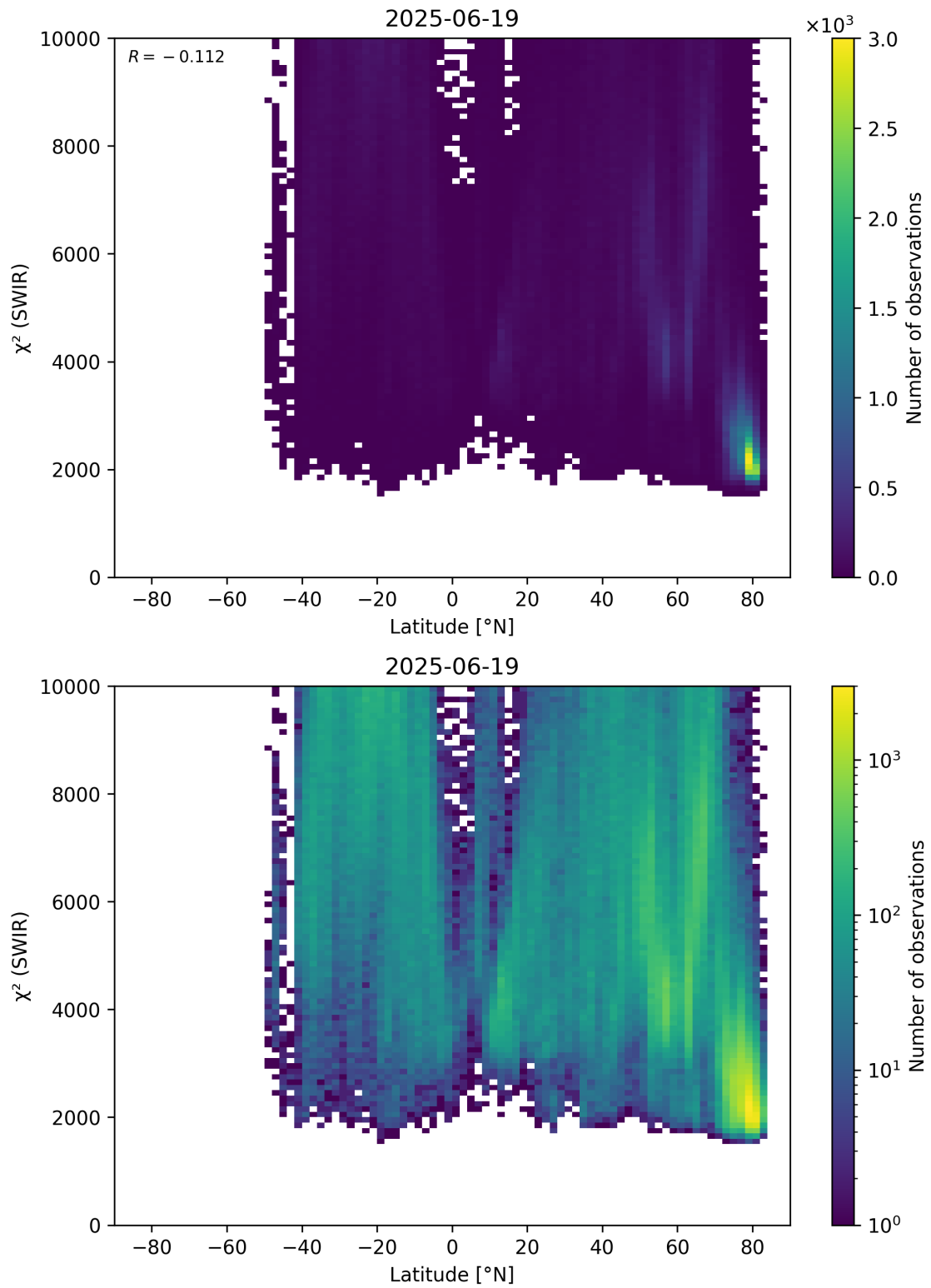
Figure 54: Scatter density plot of “Latitude” against “ \chi^2 (SWIR)” for 2025-06-18 to 2025-06-20.
