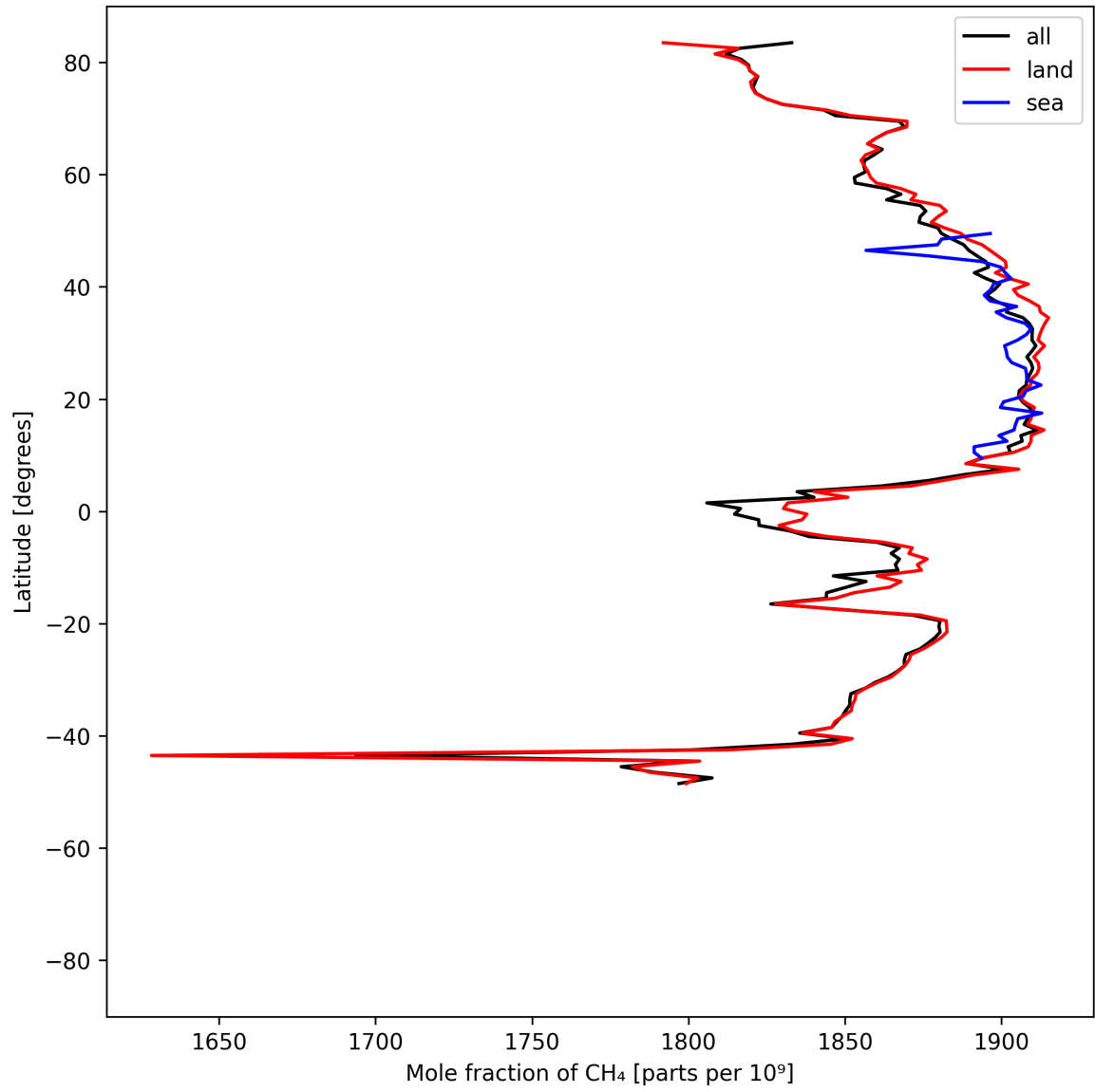
Figure 12: Zonal average of “Mole fraction of \text{CH}_4 ” for 2025-06-18 to 2025-06-20.
