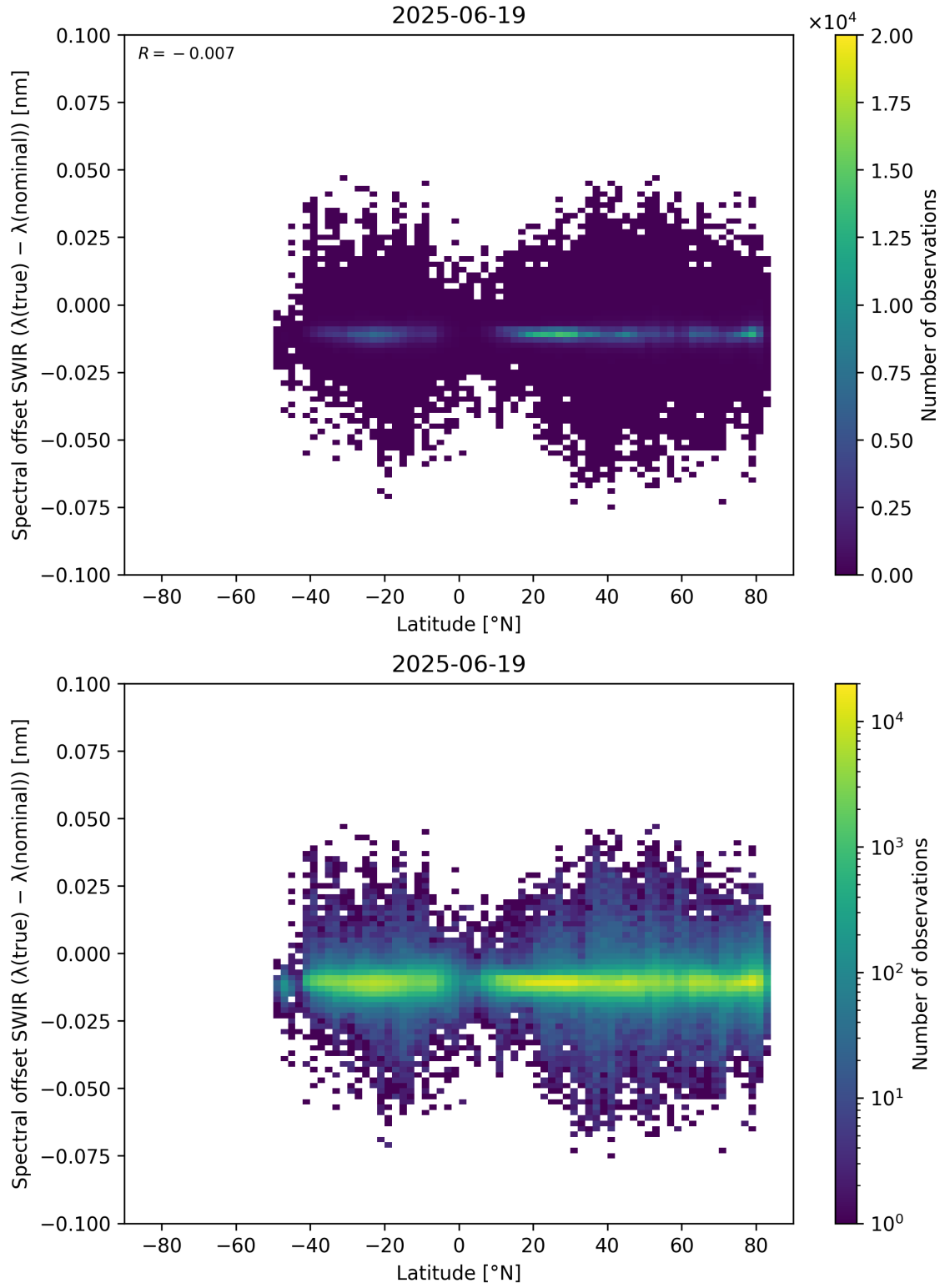
Figure 62: Scatter density plot of “Latitude” against “Spectral offset SWIR ( \lambda_{\text{true}} - \lambda_{\text{nominal}} )” for 2025-06-18 to 2025-06-20.
