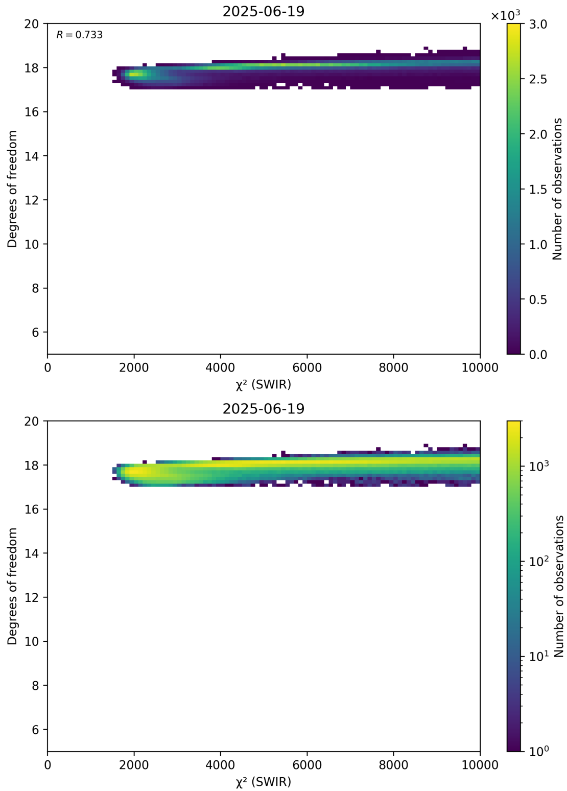
Figure 48: Scatter density plot of “ \chi^2 (SWIR)” against “Degrees of freedom” for 2025-06-18 to 2025-06-20.
