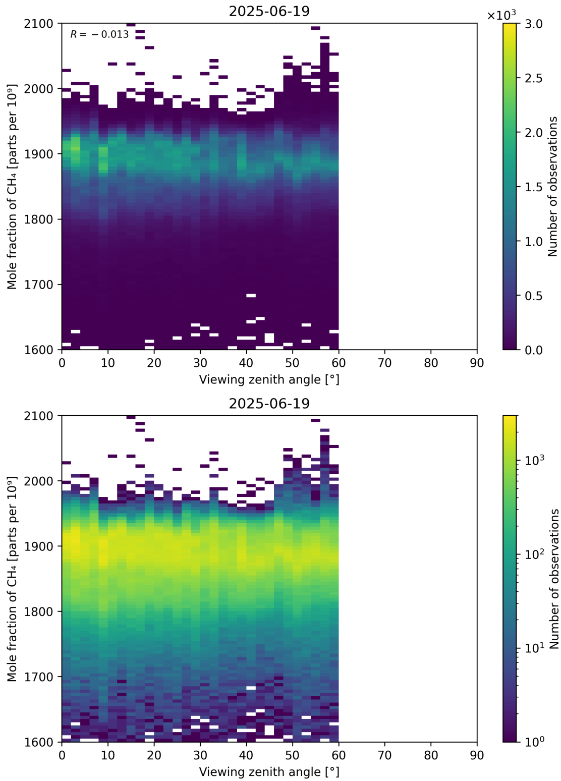
Figure 110: Scatter density plot of “Viewing zenith angle” against “Mole fraction of CH 4 ” for 2025-06-18 to 2025-06-20.
