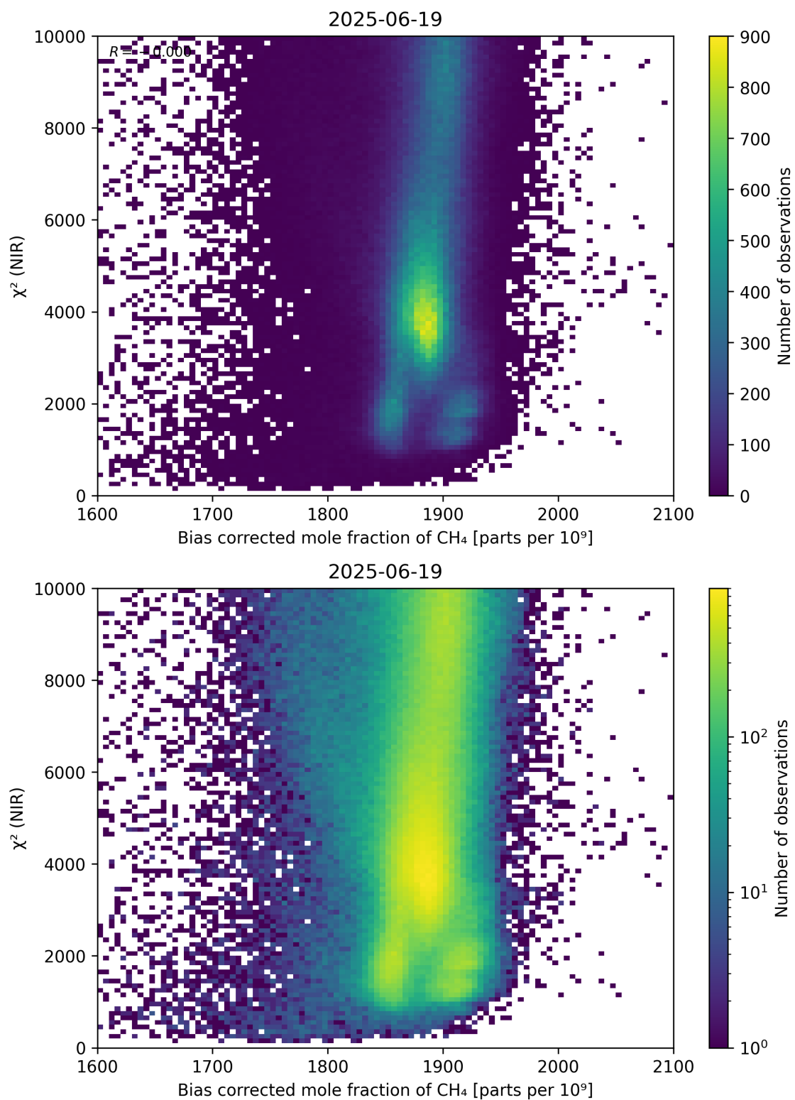
Figure 63: Scatter density plot of “Bias corrected mole fraction of \text{CH}_4 ” against “ \chi^2 (NIR)” for 2025-06-18 to 2025-06-20.
