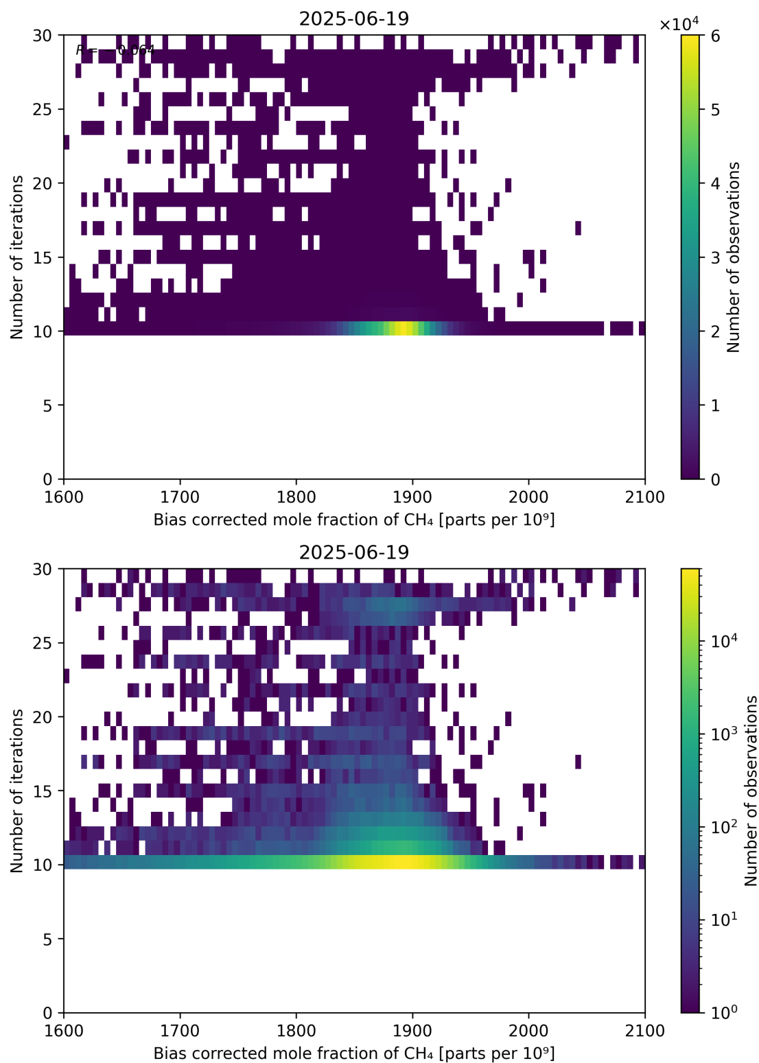
Figure 67: Scatter density plot of “Bias corrected mole fraction of CH 4 ” against “Number of iterations” for 2025-06-18 to 2025-06-20.
