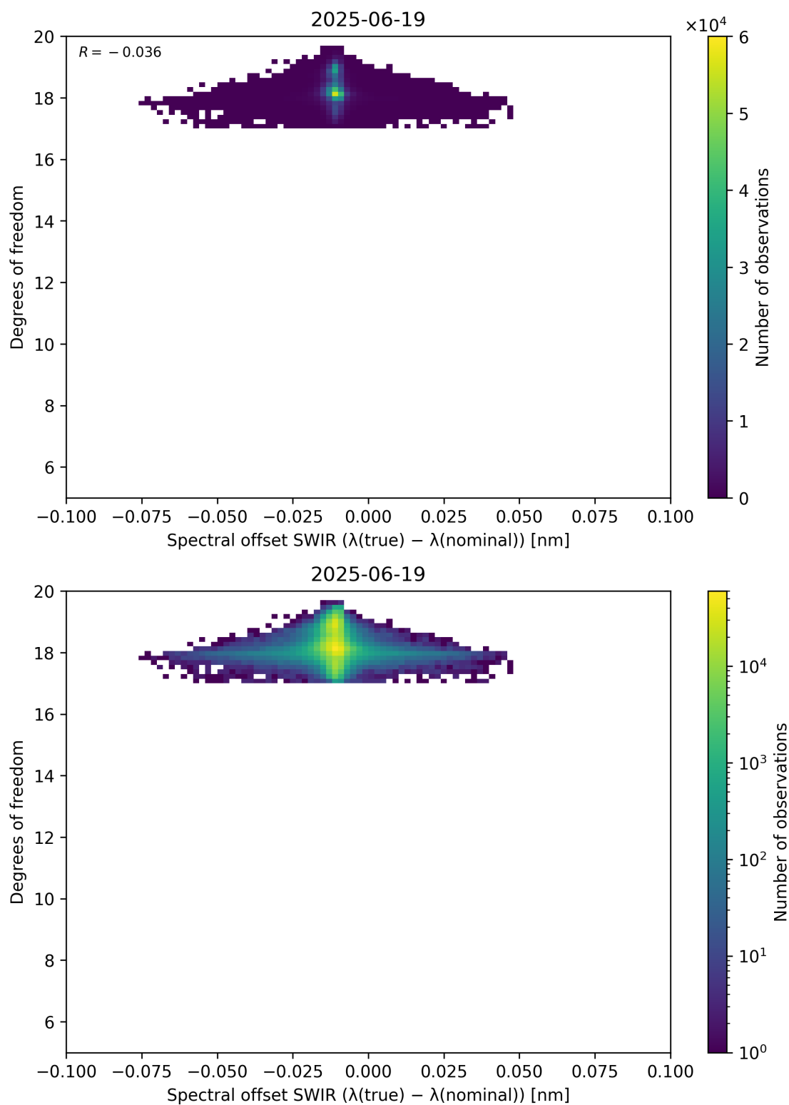
Figure 119: Scatter density plot of “Spectral offset SWIR ( \lambda_{\text{true}} - \lambda_{\text{nominal}} )” against “Degrees of freedom” for 2025-06-18 to 2025-06-20.
