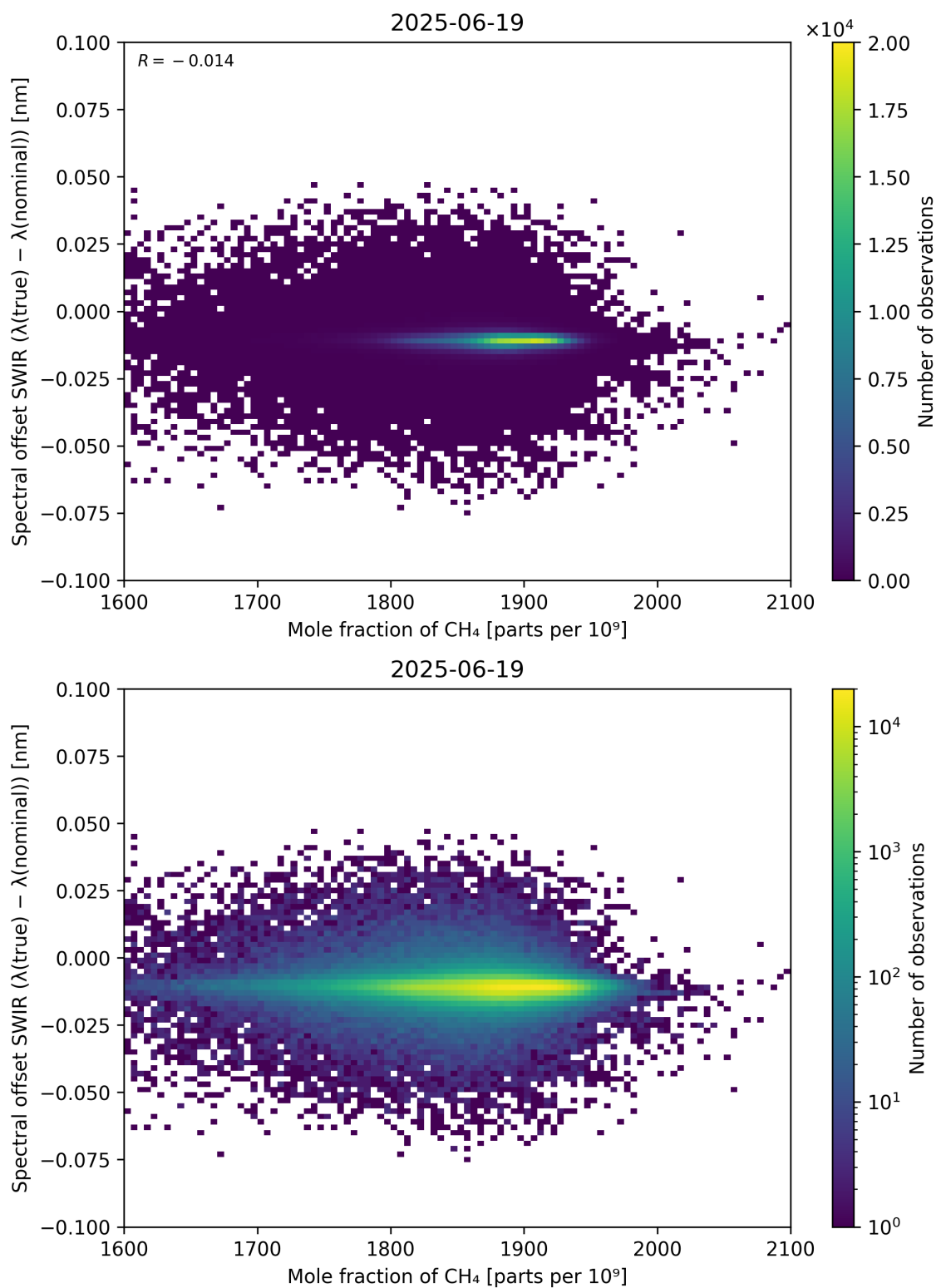
Figure 86: Scatter density plot of “Mole fraction of CH 4 ” against “Spectral offset SWIR ( \lambda_{\text{true}} - \lambda_{\text{nominal}} )” for 2025-06-18 to 2025-06-20.
