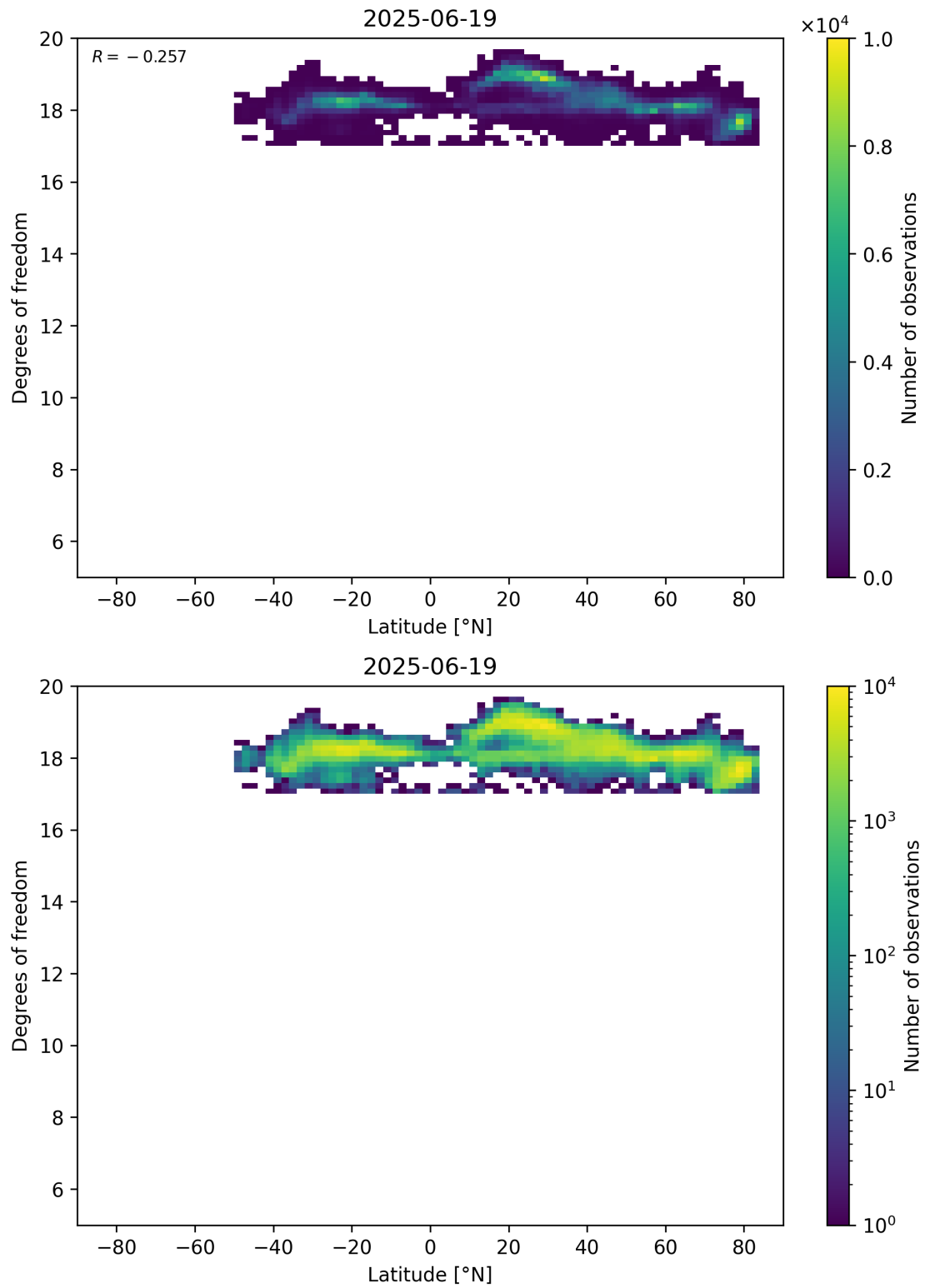
Figure 55: Scatter density plot of “Latitude” against “Degrees of freedom” for 2025-06-18 to 2025-06-20.
