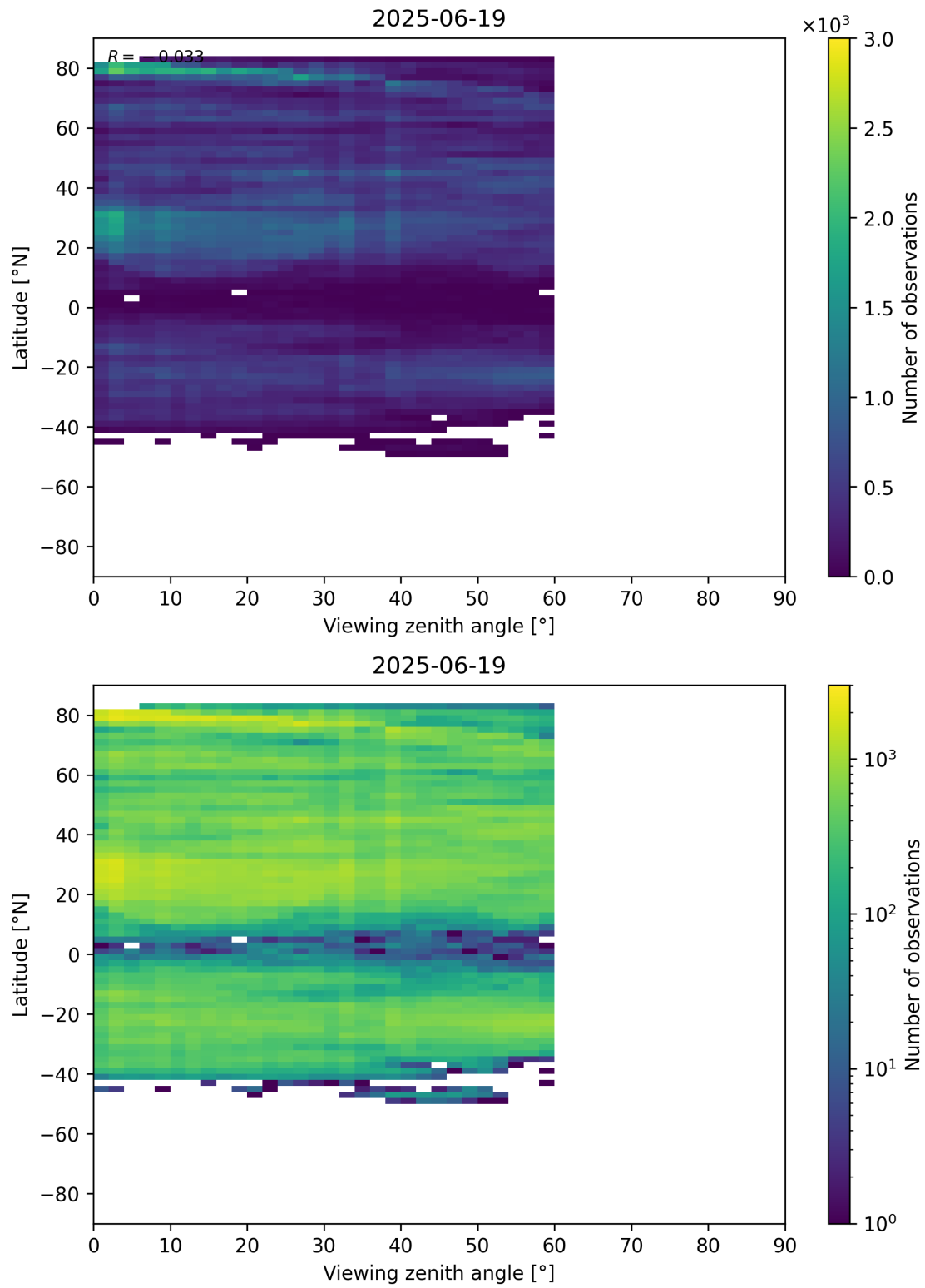
Figure 109: Scatter density plot of “Viewing zenith angle” against “Latitude” for 2025-06-18 to 2025-06-20.
