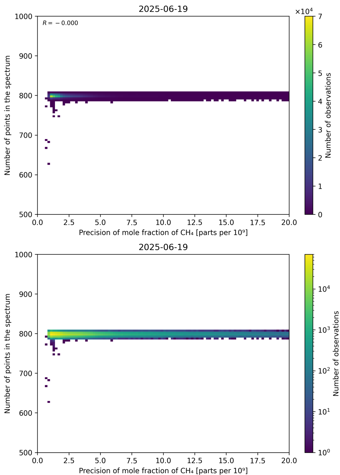
Figure 84: Scatter density plot of “Precision of mole fraction of CH 4 ” against “Number of points in the spectrum” for 2025-06-18 to 2025-06-20.
