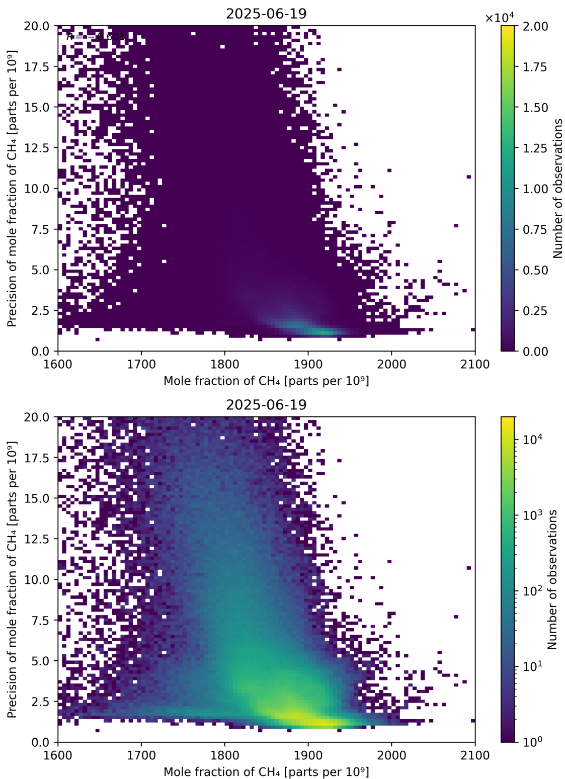
Figure 75: Scatter density plot of “Mole fraction of CH 4 ” against “Precision of mole fraction of CH 4 ” for 2025-06-18 to 2025-06-20.
