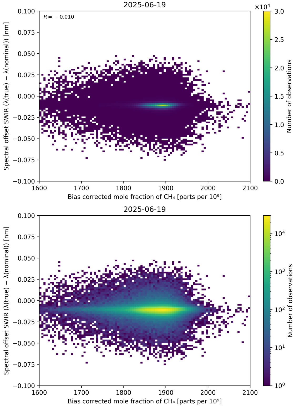
Figure 69: Scatter density plot of “Bias corrected mole fraction of CH 4 ” against “Spectral offset SWIR ( \lambda_{\text{true}} - \lambda_{\text{nominal}} )” for 2025-06-18 to 2025-06-20.
