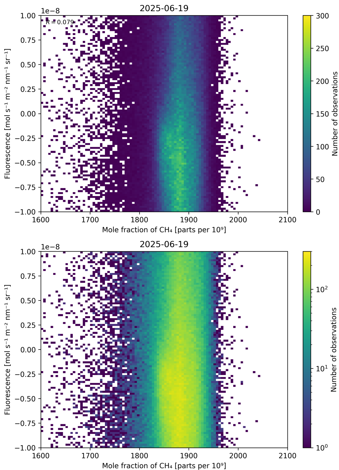
Figure 73: Scatter density plot of “Mole fraction of \text{CH}_4 ” against “Fluorescence” for 2025-06-18 to 2025-06-20.
