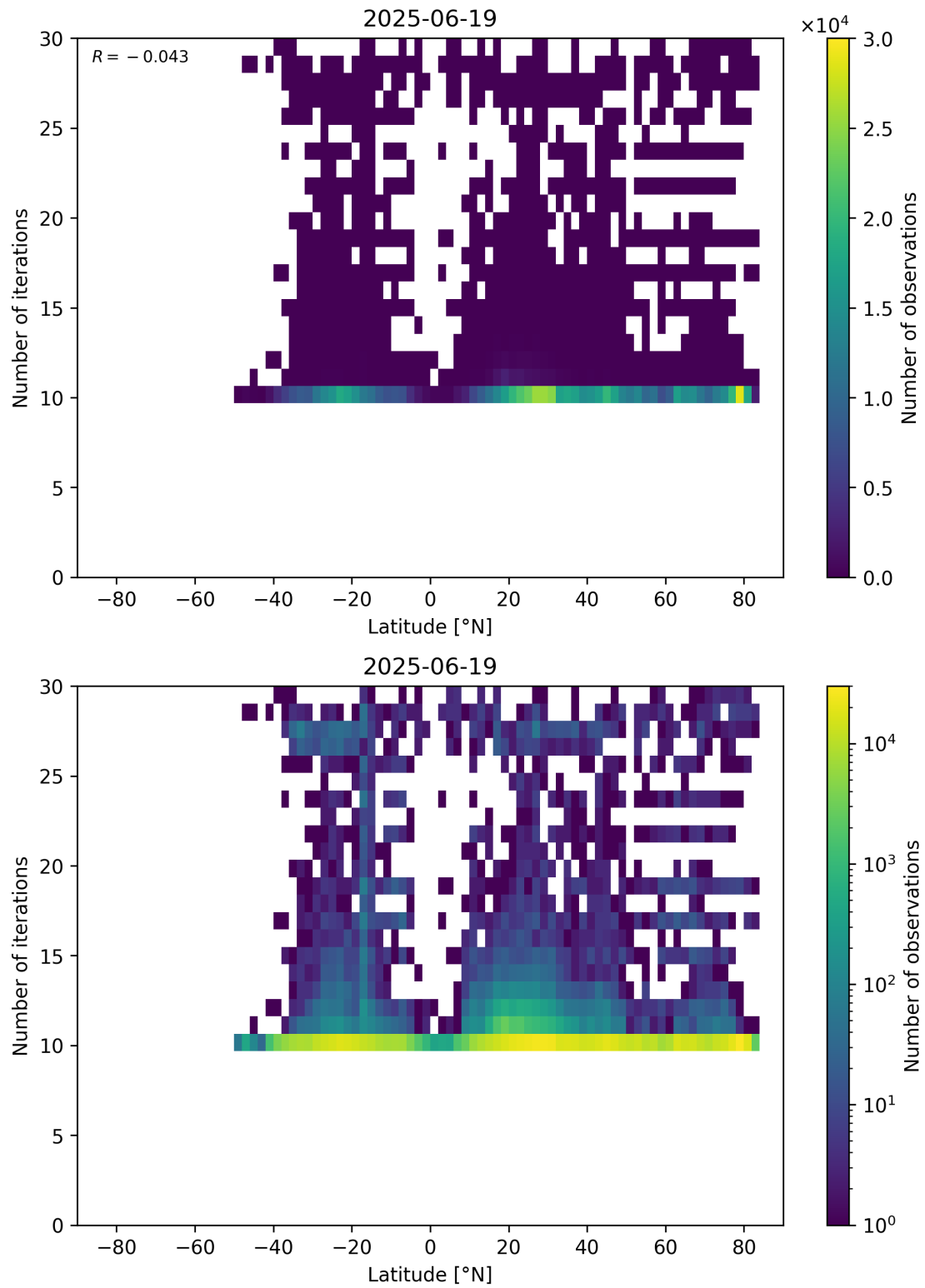
Figure 60: Scatter density plot of “Latitude” against “Number of iterations” for 2025-06-18 to 2025-06-20.
