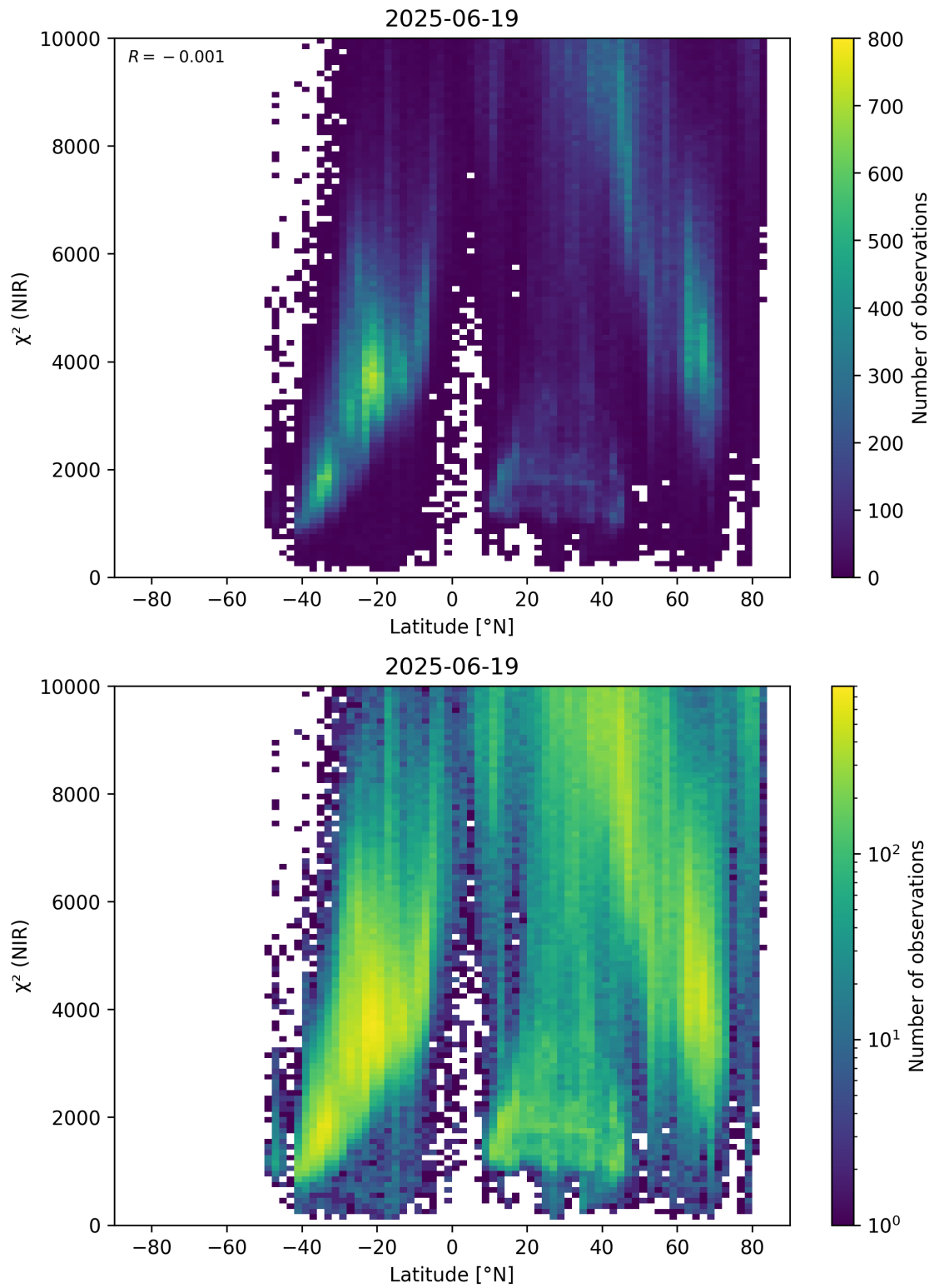
Figure 53: Scatter density plot of “Latitude” against “ \chi^2 (NIR)” for 2025-06-18 to 2025-06-20.
