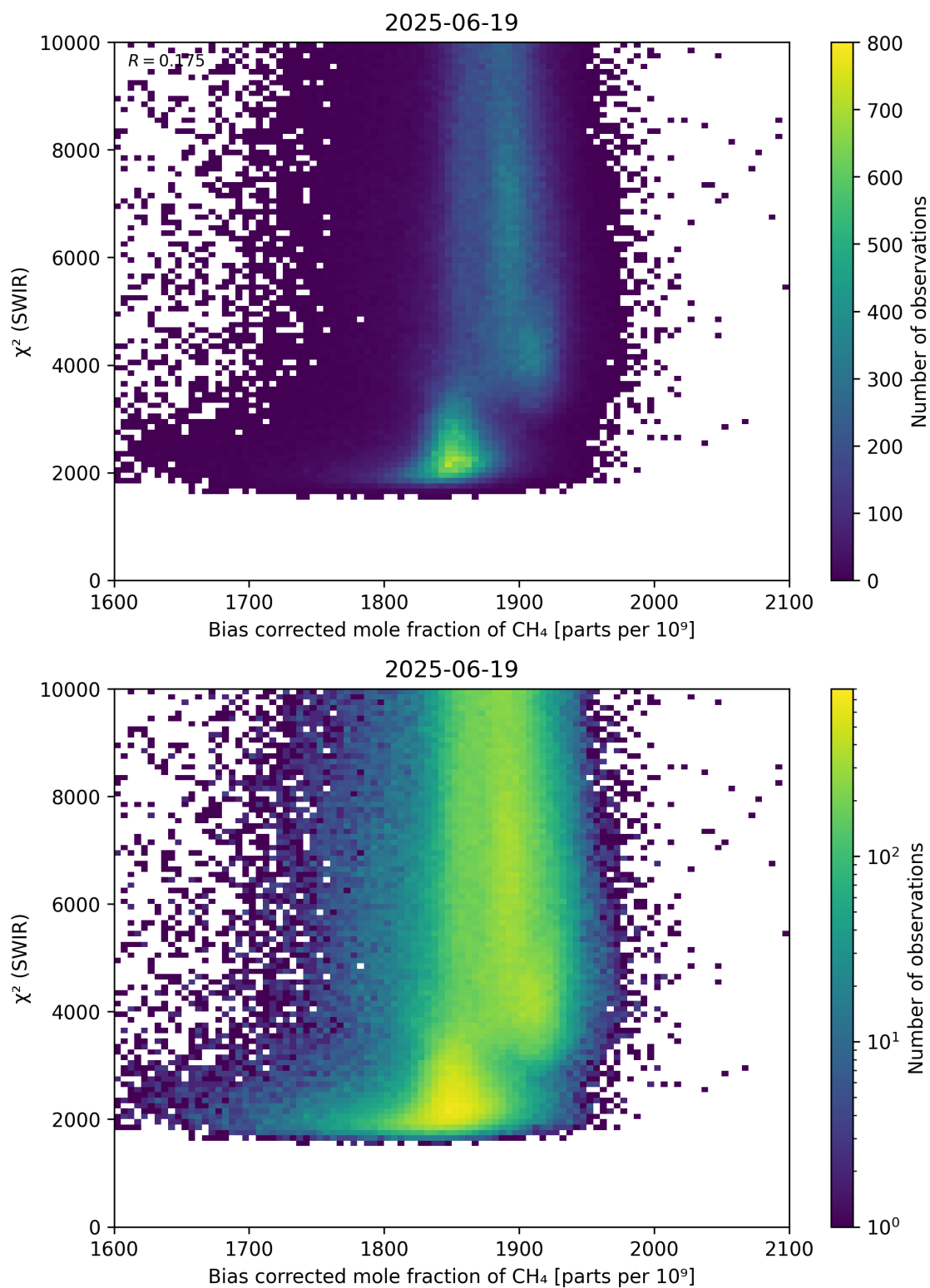
Figure 64: Scatter density plot of “Bias corrected mole fraction of CH 4 ” against “ \chi^2 (SWIR)” for 2025-06-18 to 2025-06-20.
