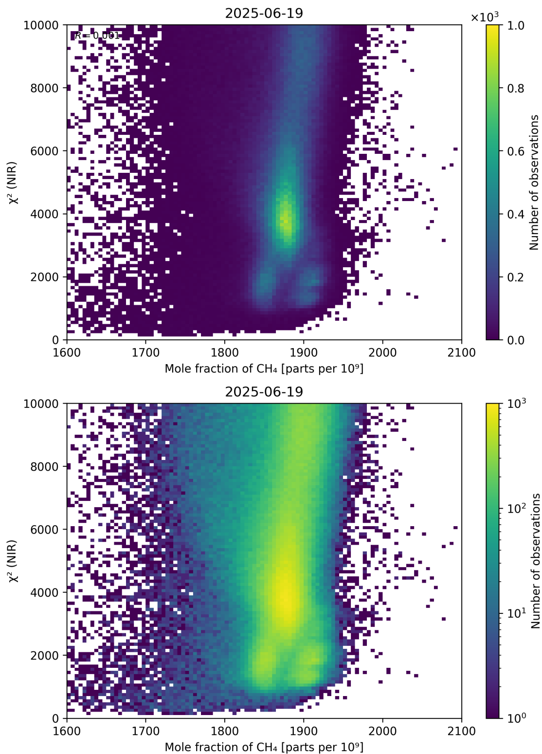
Figure 70: Scatter density plot of “Mole fraction of CH 4 ” against “ \chi^2 (NIR)” for 2025-06-18 to 2025-06-20.
