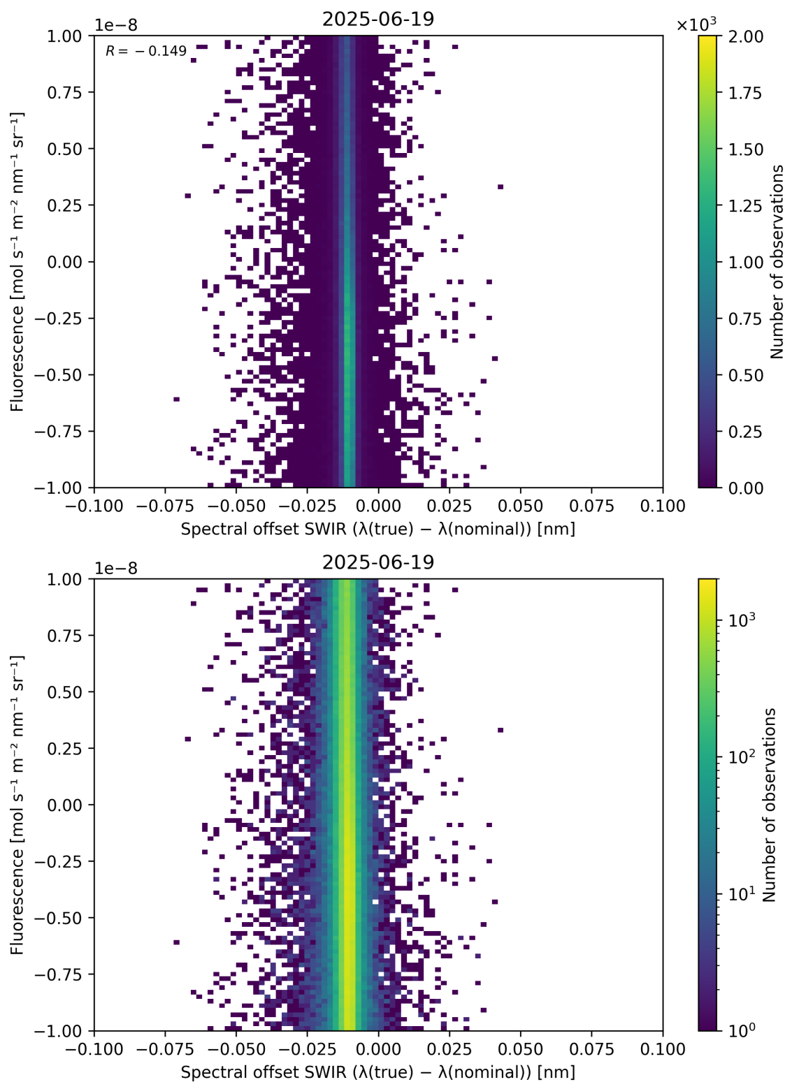
Figure 120: Scatter density plot of “Spectral offset SWIR ( \lambda_{\text{true}} - \lambda_{\text{nominal}} )” against “Fluorescence” for 2025-06-18 to 2025-06-20.
