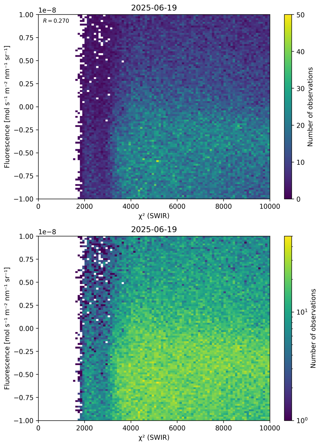
Figure 49: Scatter density plot of “ \chi^2 (SWIR)” against “Fluorescence” for 2025-06-18 to 2025-06-20.
