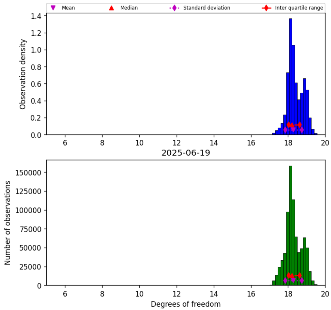
Figure 30: Histogram of “Degrees of freedom” for 2025-06-18 to 2025-06-20
