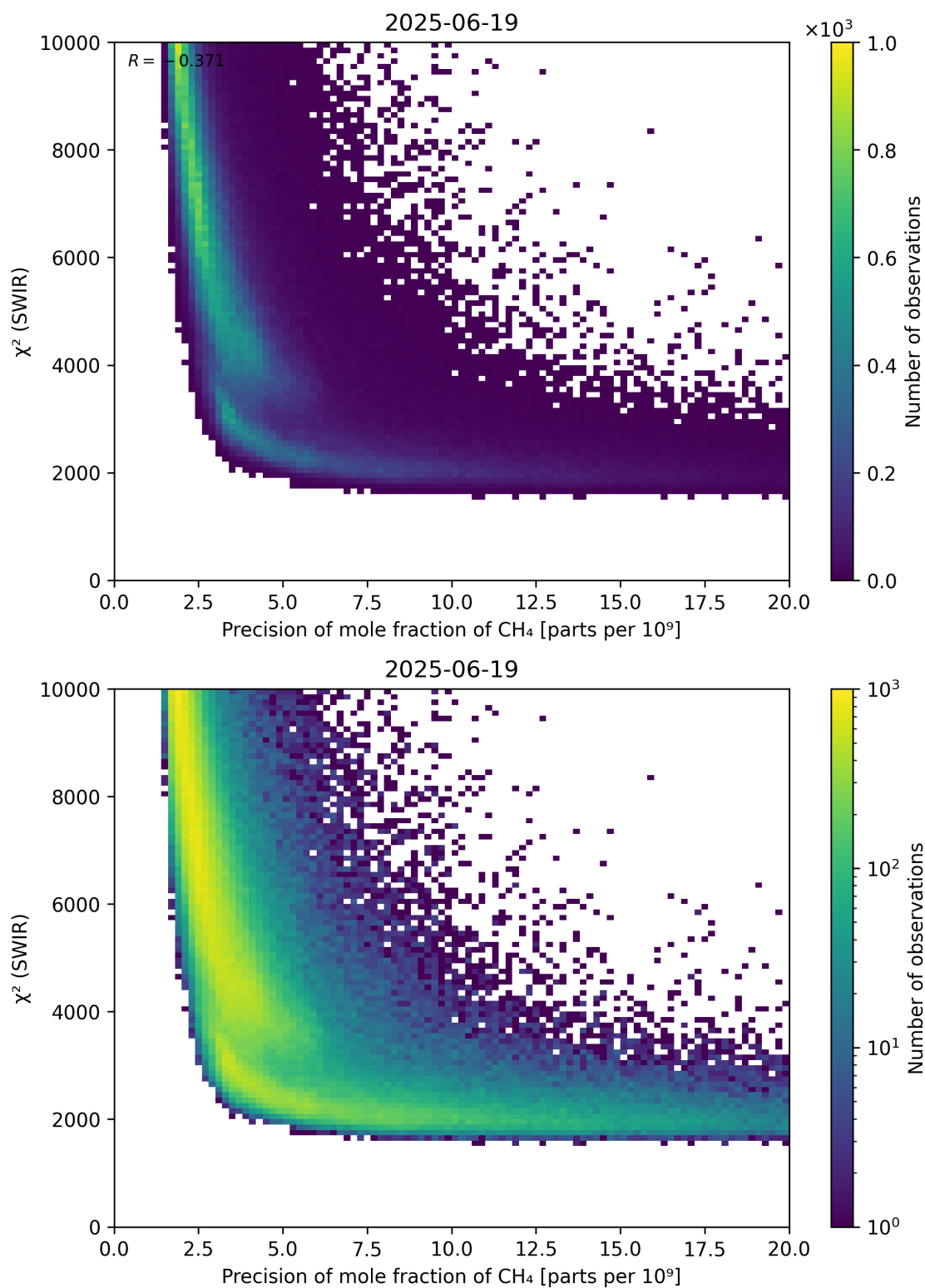
Figure 79: Scatter density plot of “Precision of mole fraction of \text{CH}_4 ” against “ \chi^2 (SWIR)” for 2025-06-18 to 2025-06-20.
