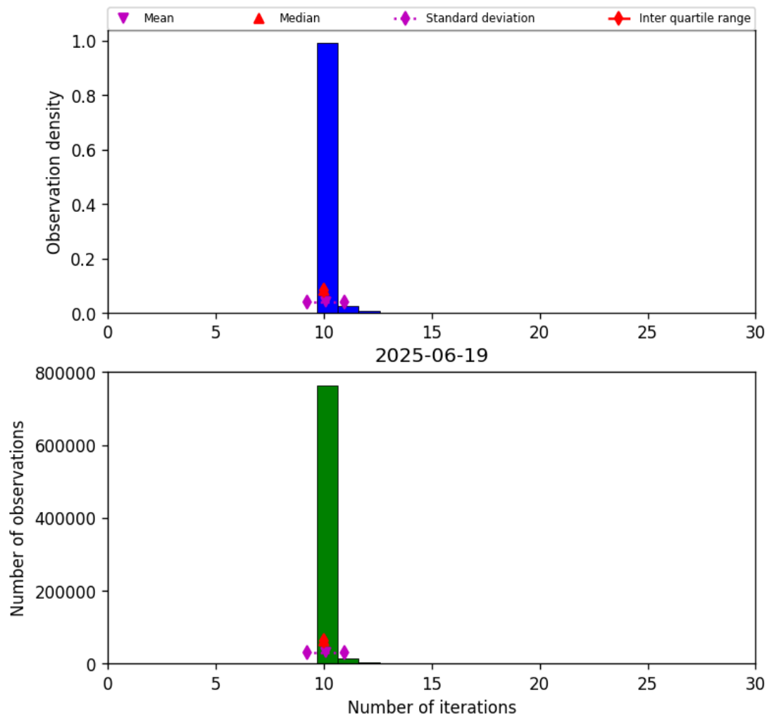
Figure 31: Histogram of “Number of iterations” for 2025-06-18 to 2025-06-20
