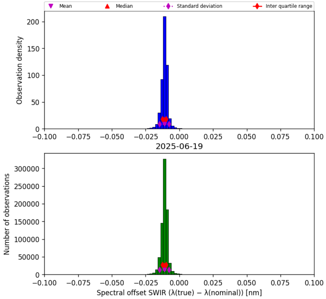
Figure 27: Histogram of “Spectral offset SWIR ( \lambda_{\text{true}} - \lambda_{\text{nominal}} )” for 2025-06-18 to 2025-06-20
