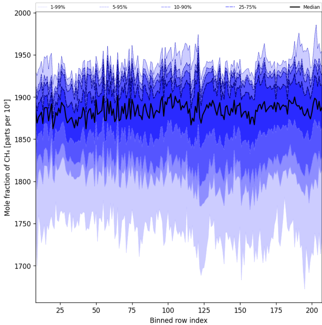
Figure 34: Along track statistics of “Mole fraction of CH 4 ” for 2025-06-18 to 2025-06-20
