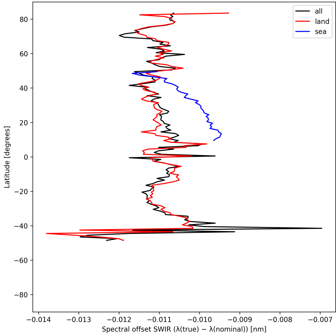
Figure 16: Zonal average of “Spectral offset SWIR ( \lambda_{\text{true}} - \lambda_{\text{nominal}} )” for 2025-06-18 to 2025-06-20.
