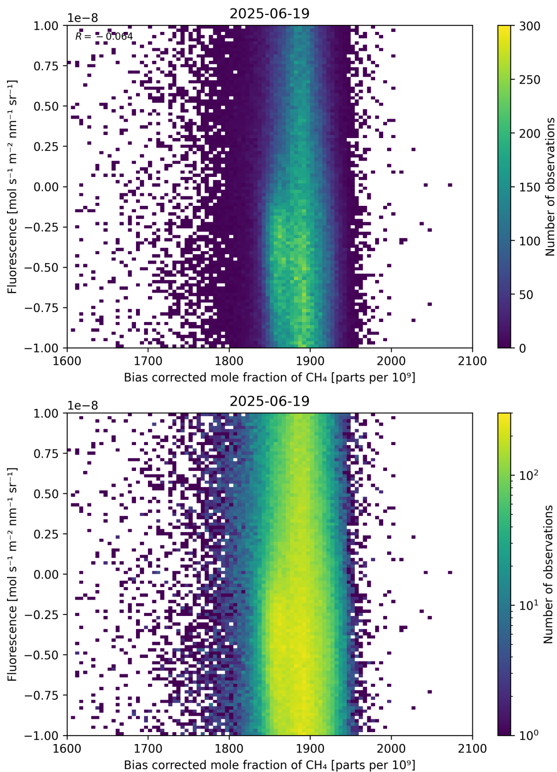
Figure 66: Scatter density plot of “Bias corrected mole fraction of \text{CH}_4 ” against “Fluorescence” for 2025-06-18 to 2025-06-20.
