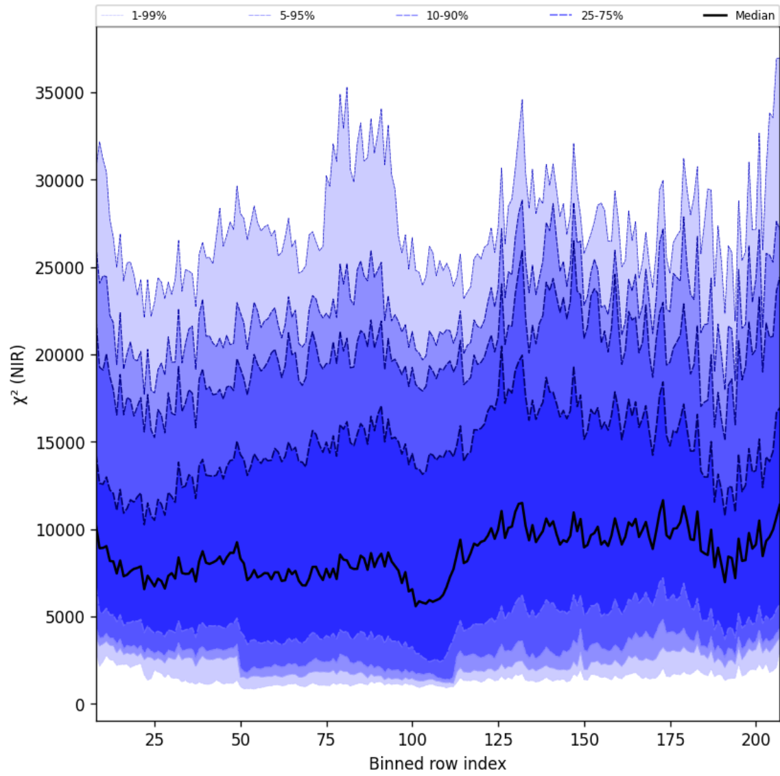
Figure 40: Along track statistics of “ \chi^2 (NIR)” for 2025-06-18 to 2025-06-20
