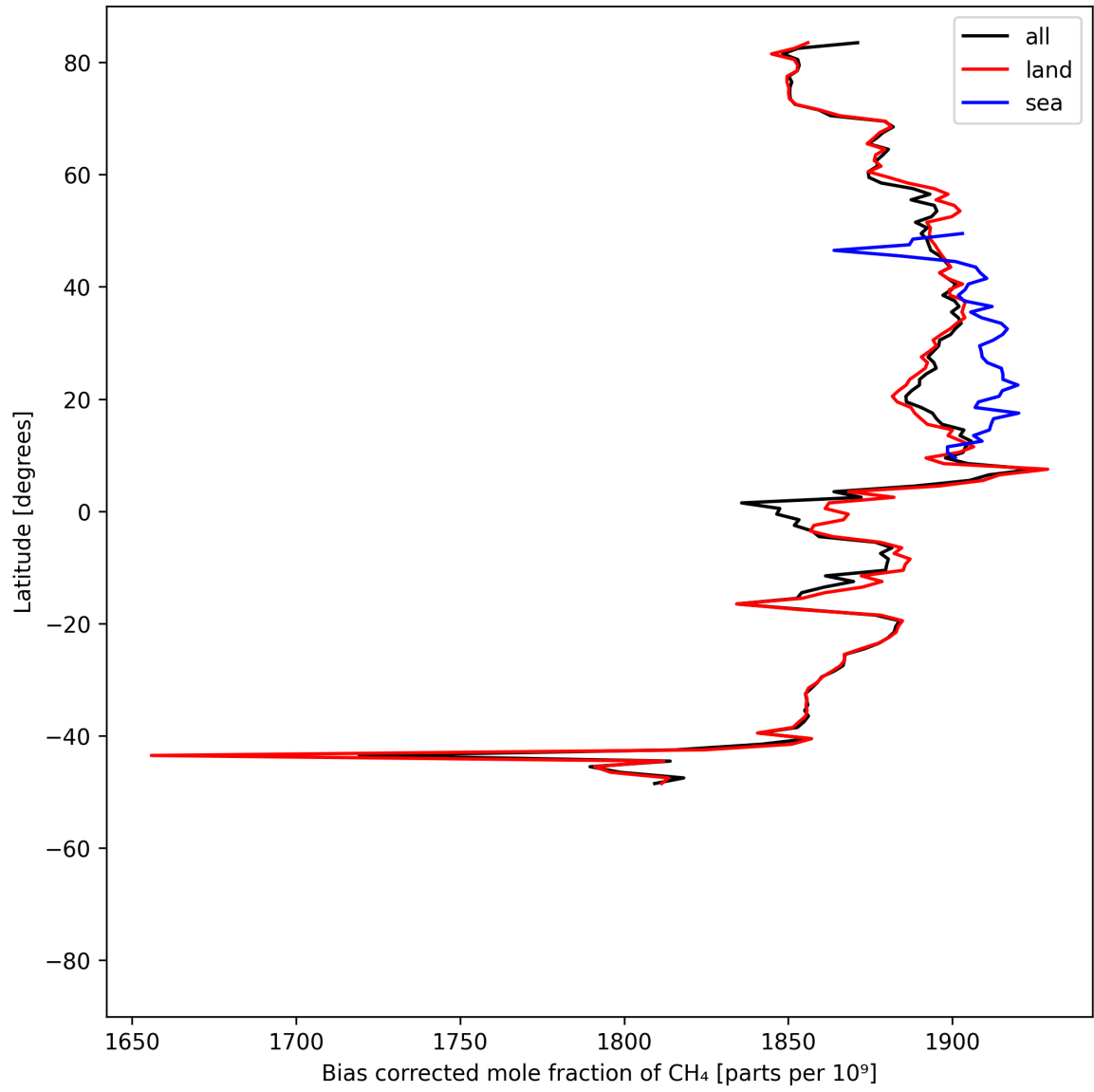
Figure 14: Zonal average of “Bias corrected mole fraction of \text{CH}_4 ” for 2025-06-18 to 2025-06-20.
