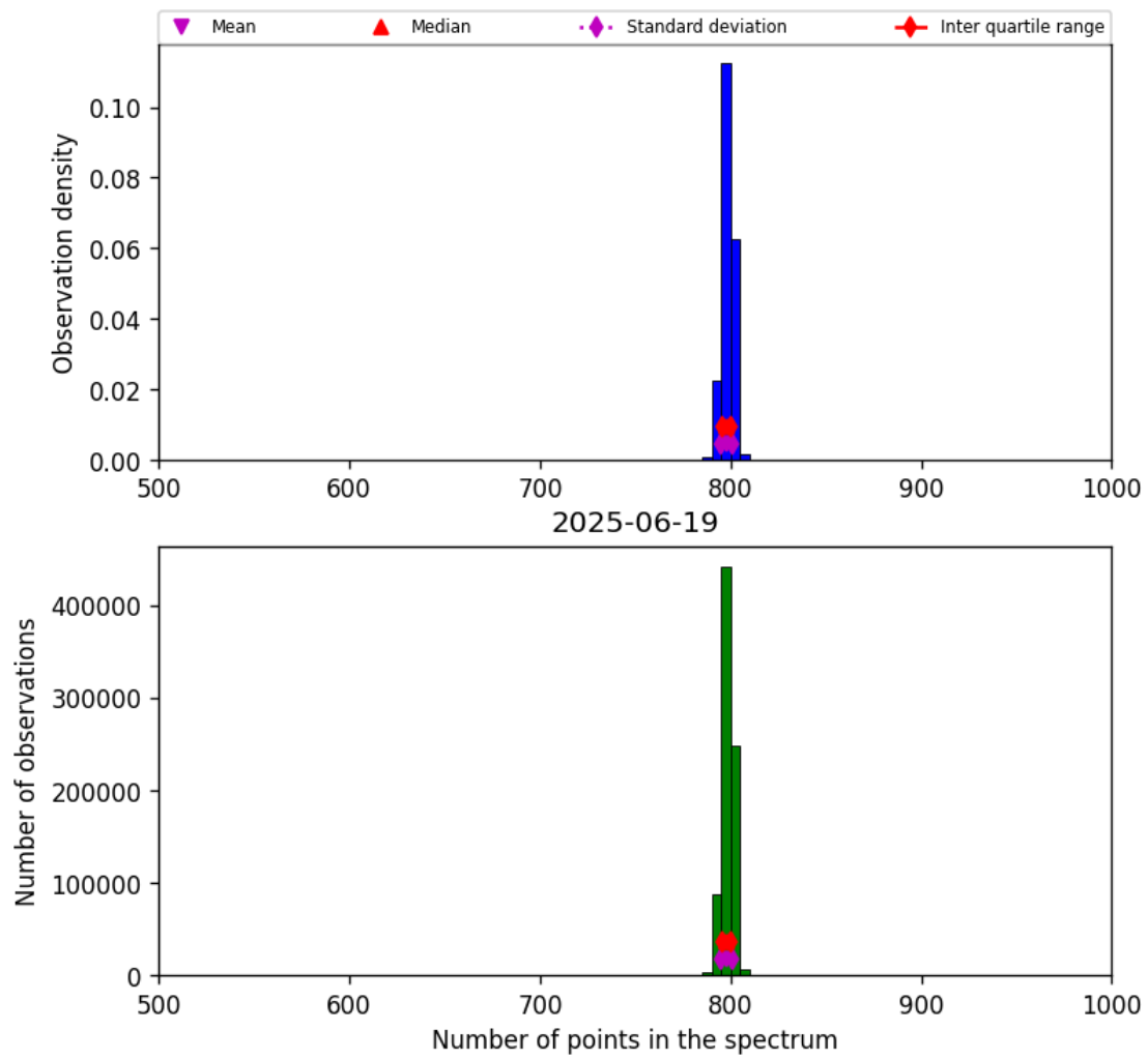
Figure 26: Histogram of “Number of points in the spectrum” for 2025-06-18 to 2025-06-20
