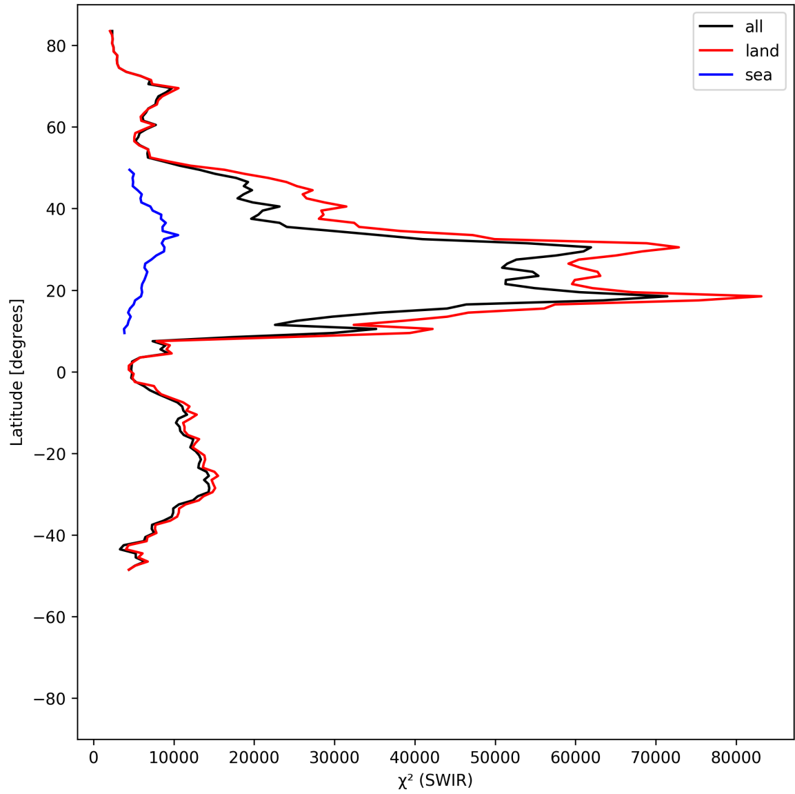
Figure 17: Zonal average of “ \chi^2 (SWIR)” for 2025-06-18 to 2025-06-20.
