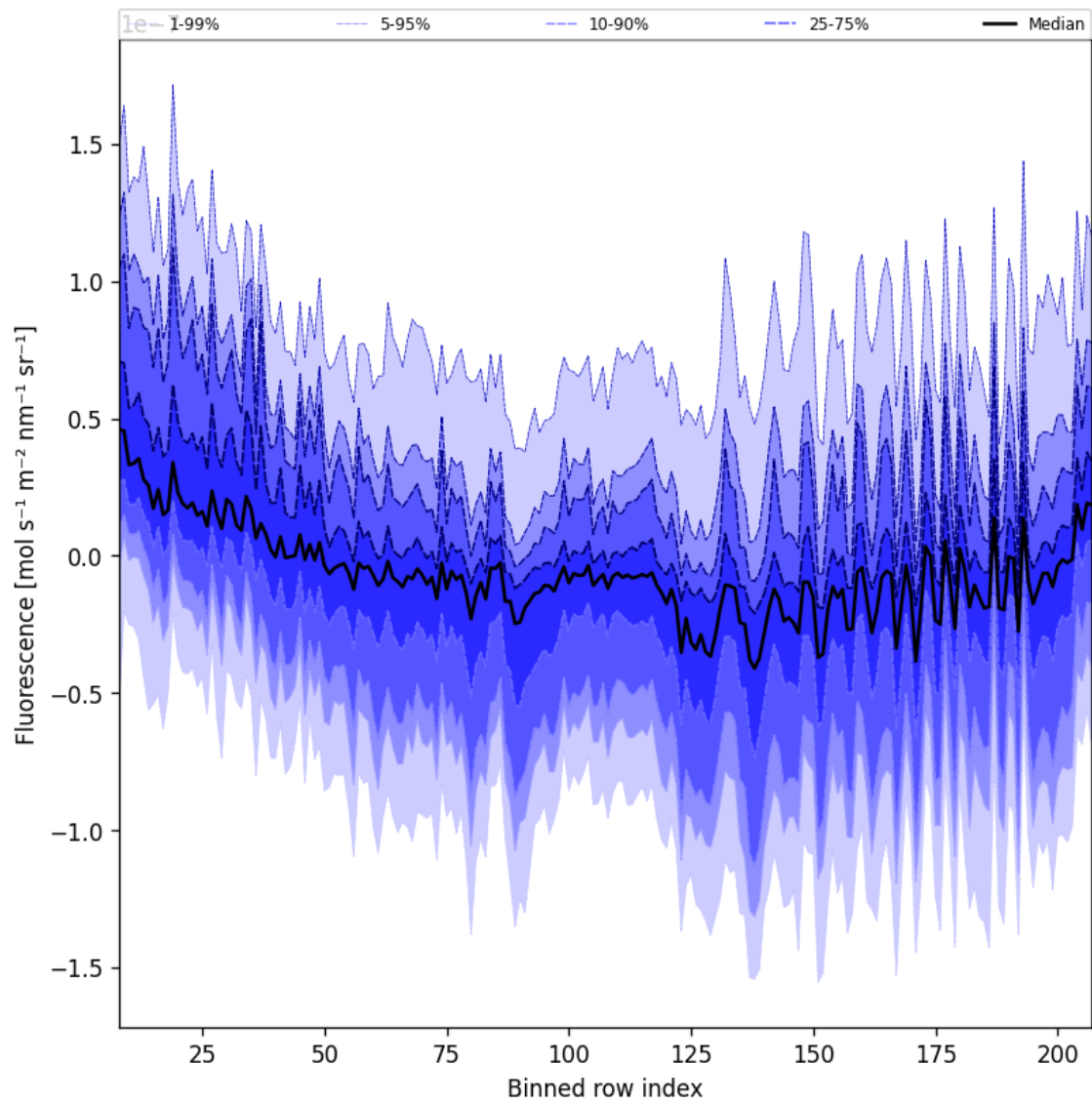
Figure 43: Along track statistics of “Fluorescence” for 2025-06-18 to 2025-06-20
