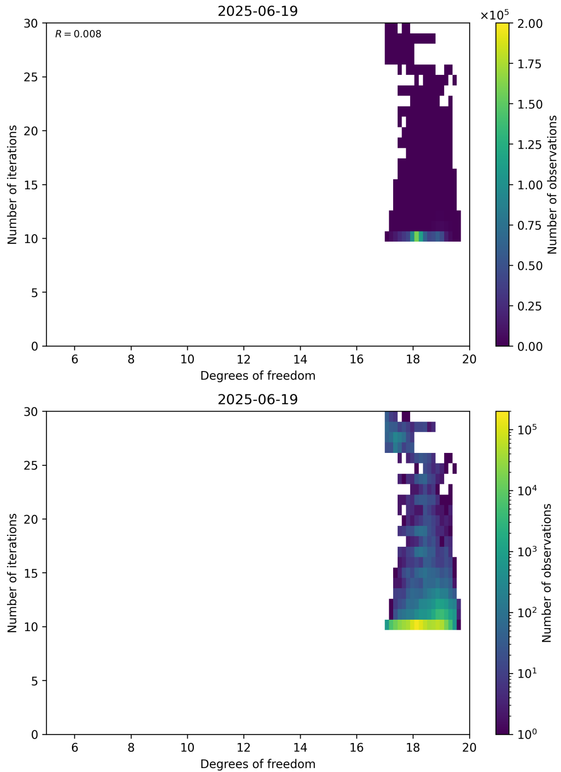
Figure 52: Scatter density plot of “Degrees of freedom” against “Number of iterations” for 2025-06-18 to 2025-06-20.
