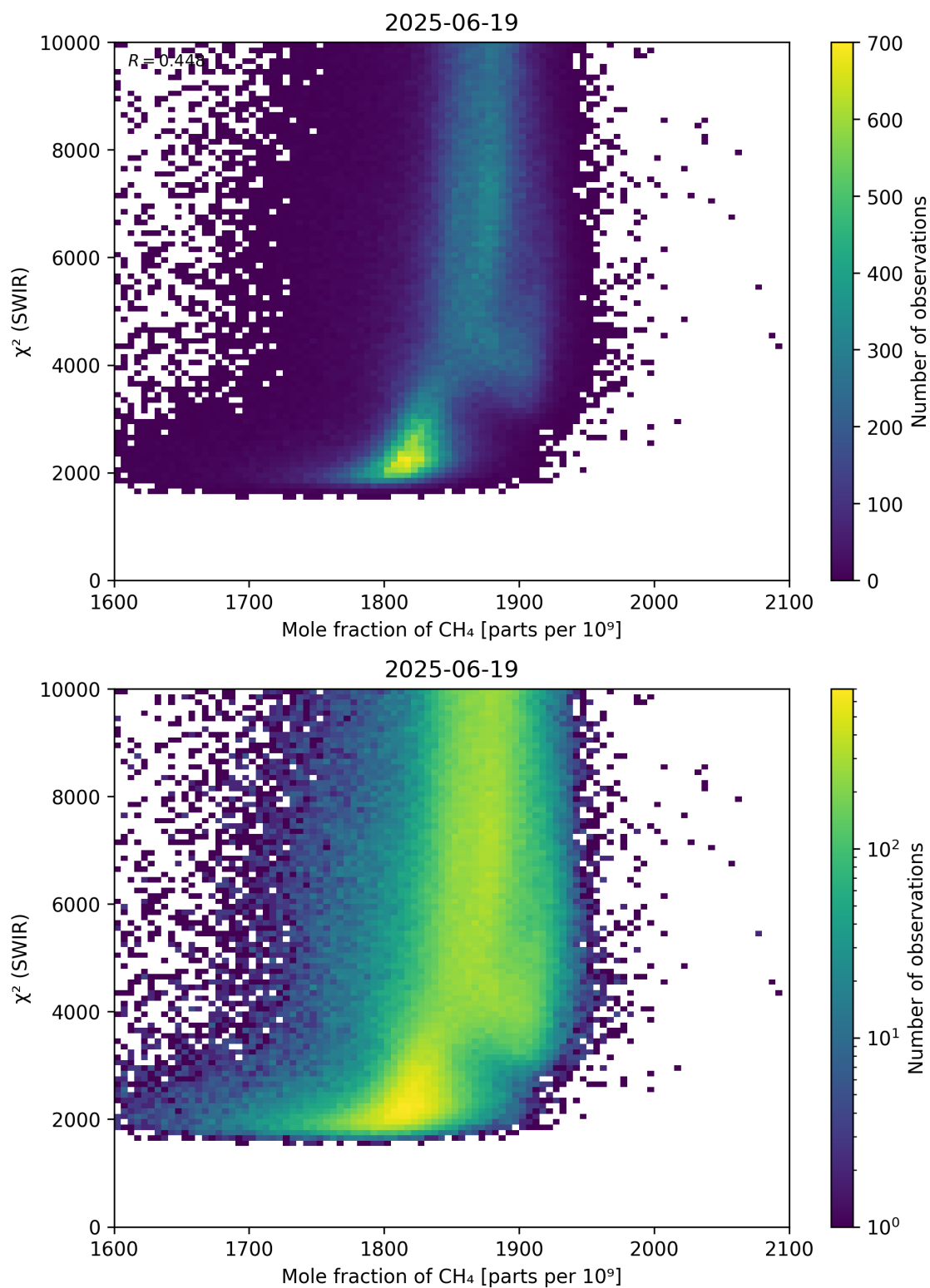
Figure 71: Scatter density plot of “Mole fraction of \text{CH}_4 ” against “ \chi^2 (SWIR)” for 2025-06-18 to 2025-06-20.
