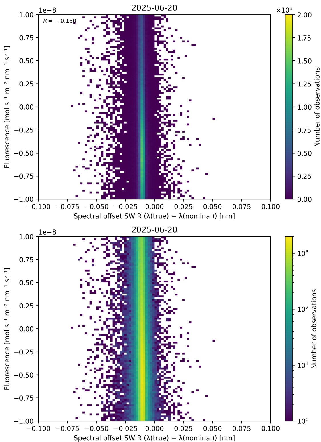
Figure 120: Scatter density plot of “Spectral offset SWIR ( \lambda_{\text{true}} - \lambda_{\text{nominal}} )” against “Fluorescence” for 2025-06-19 to 2025-06-21.
