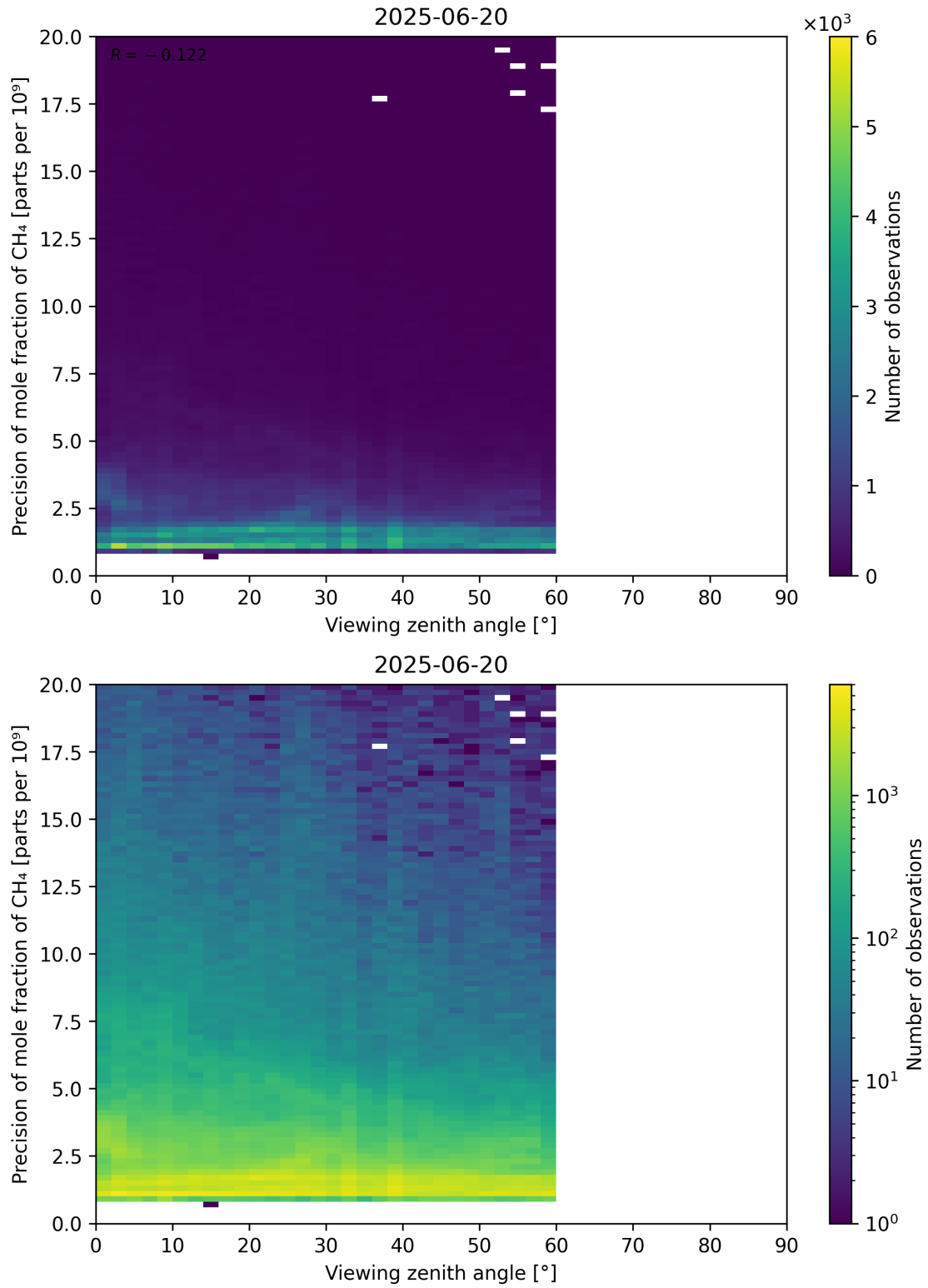
Figure 112: Scatter density plot of “Viewing zenith angle” against “Precision of mole fraction of CH 4 ” for 2025-06-19 to 2025-06-21.
