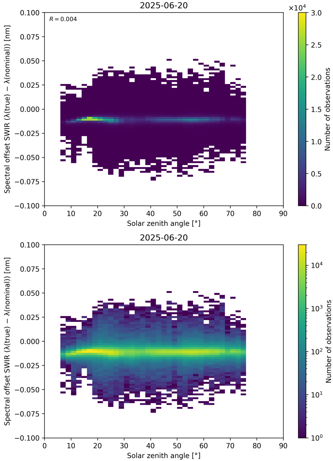
Figure 104: Scatter density plot of “Solar zenith angle” against “Spectral offset SWIR ( \lambda_{\text{true}} - \lambda_{\text{nominal}} )” for 2025-06-19 to 2025-06-21.
