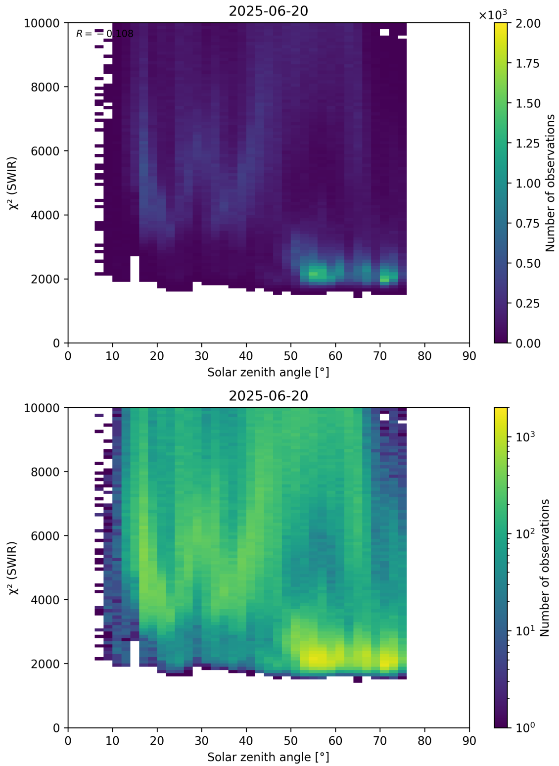
Figure 95: Scatter density plot of “Solar zenith angle” against “ \chi^2 (SWIR)” for 2025-06-19 to 2025-06-21.
