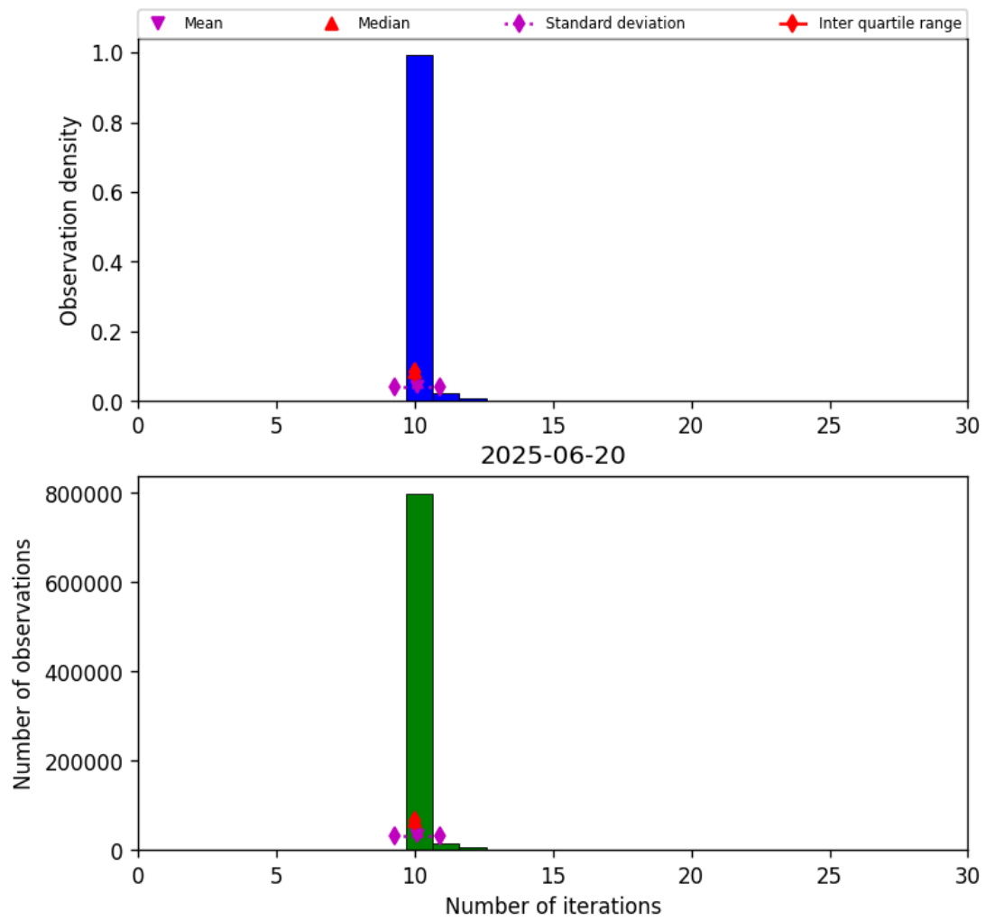
Figure 31: Histogram of “Number of iterations” for 2025-06-19 to 2025-06-21
