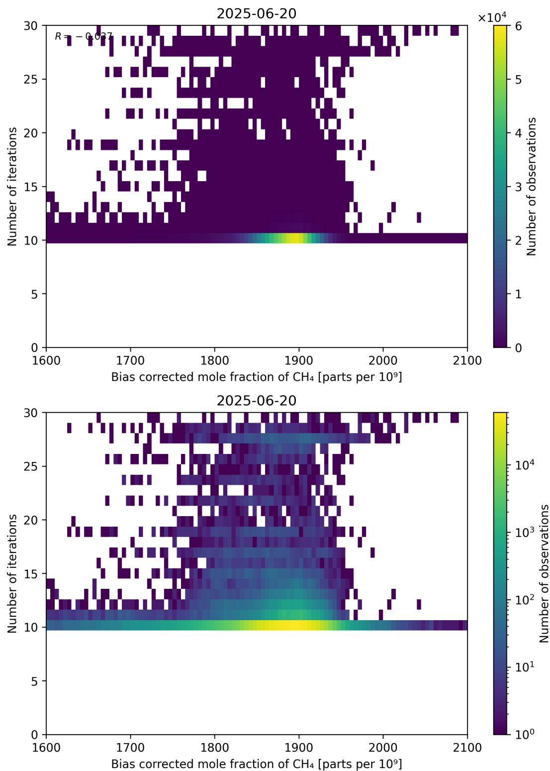
Figure 67: Scatter density plot of “Bias corrected mole fraction of CH 4 ” against “Number of iterations” for 2025-06-19 to 2025-06-21.
