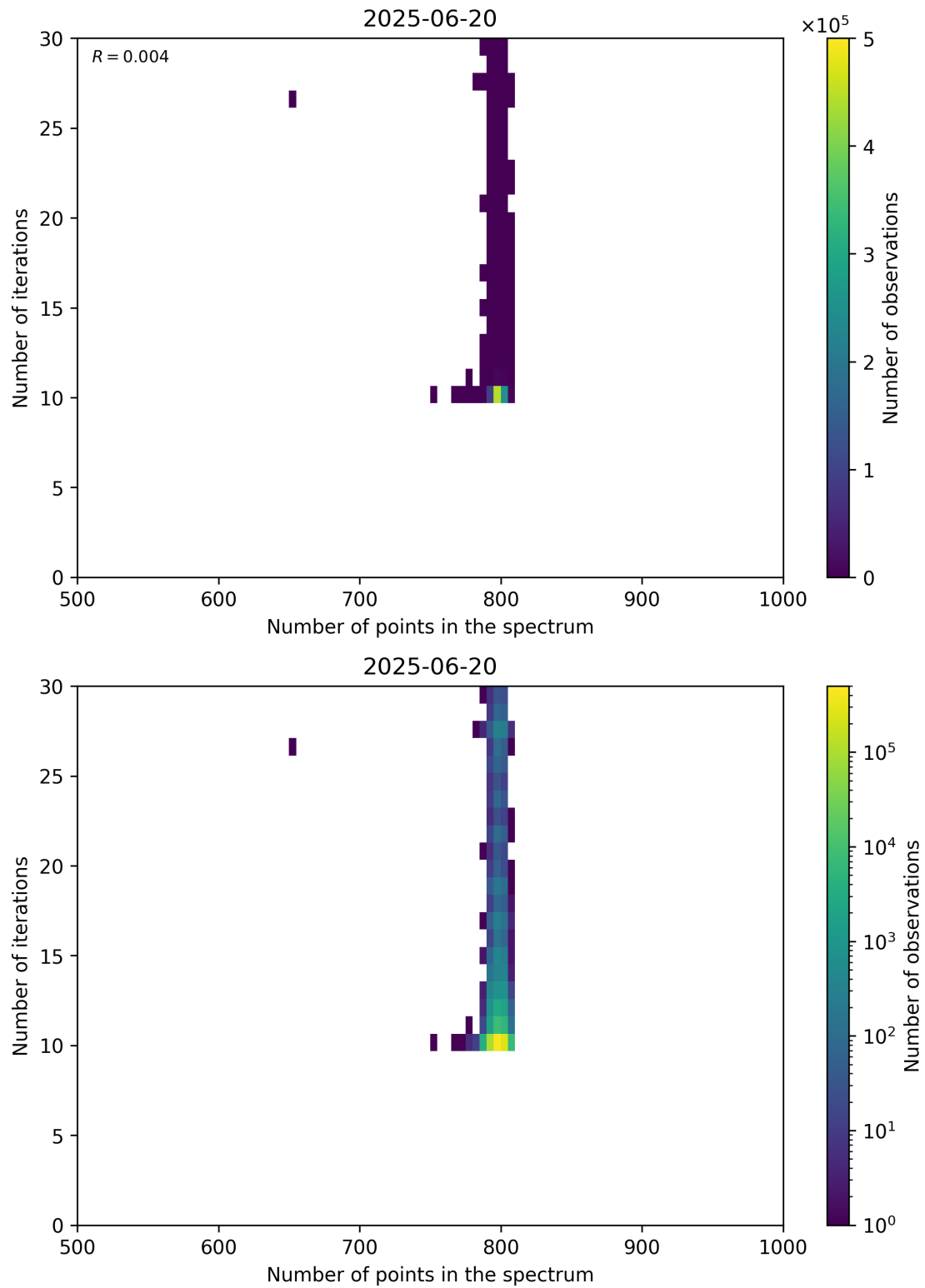
Figure 92: Scatter density plot of “Number of points in the spectrum” against “Number of iterations” for 2025-06-19 to 2025-06-21.
