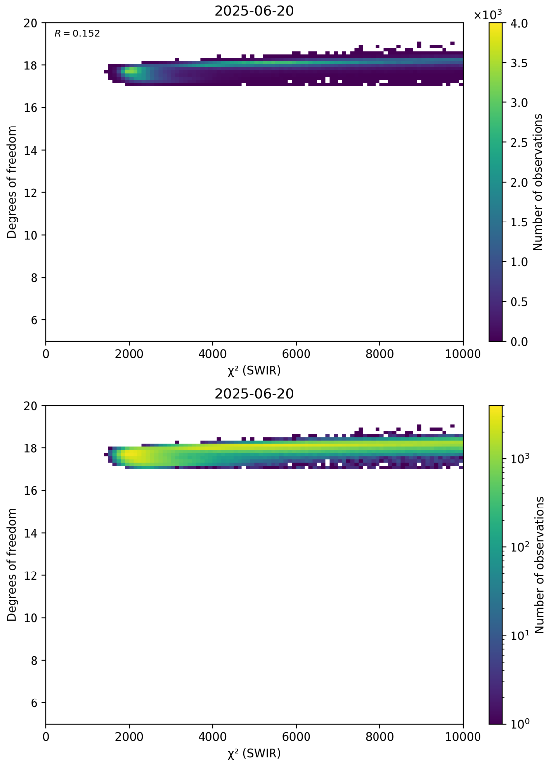
Figure 48: Scatter density plot of “ \chi^2 (SWIR)” against “Degrees of freedom” for 2025-06-19 to 2025-06-21.
