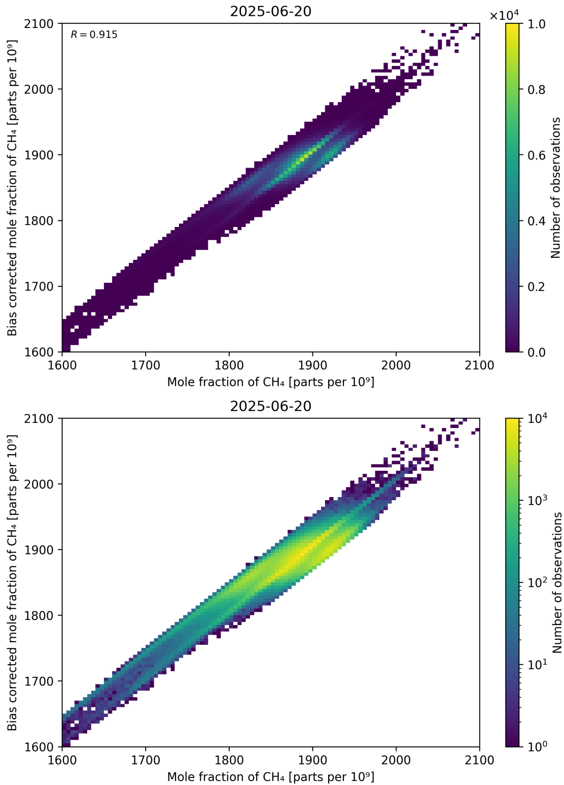
Figure 74: Scatter density plot of “Mole fraction of CH 4 ” against “Bias corrected mole fraction of CH 4 ” for 2025-06-19 to 2025-06-21.
