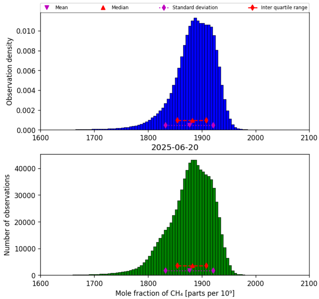
Figure 23: Histogram of “Mole fraction of CH 4 ” for 2025-06-19 to 2025-06-21
