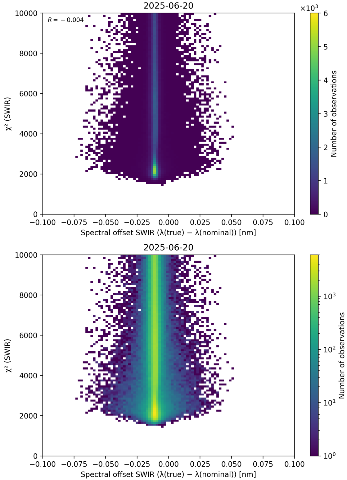
Figure 118: Scatter density plot of “Spectral offset SWIR ( \lambda_{\text{true}} - \lambda_{\text{nominal}} )” against “ \chi^2 (SWIR)” for 2025-06-19 to 2025-06-21.
