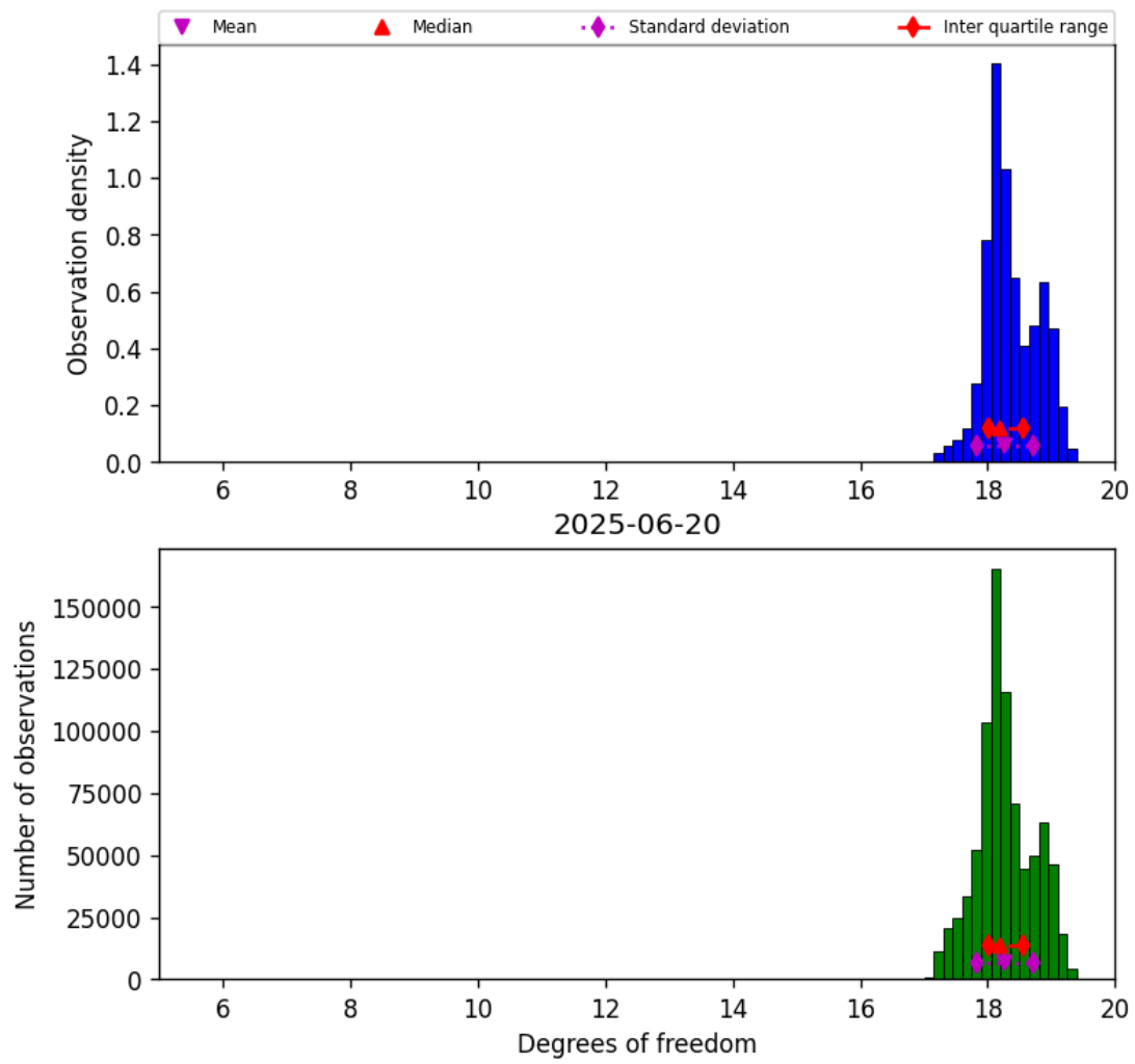
Figure 30: Histogram of “Degrees of freedom” for 2025-06-19 to 2025-06-21
