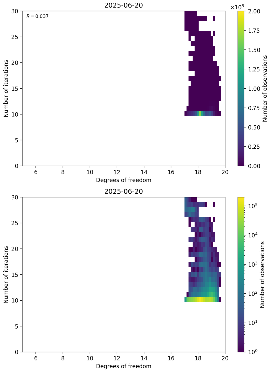
Figure 52: Scatter density plot of “Degrees of freedom” against “Number of iterations” for 2025-06-19 to 2025-06-21.
