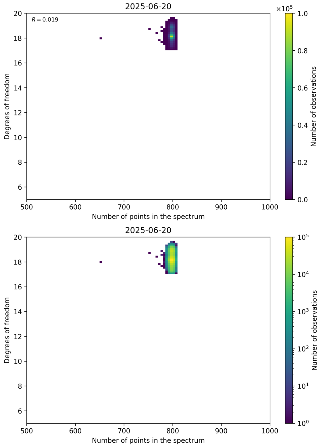
Figure 90: Scatter density plot of “Number of points in the spectrum” against “Degrees of freedom” for 2025-06-19 to 2025-06-21.
