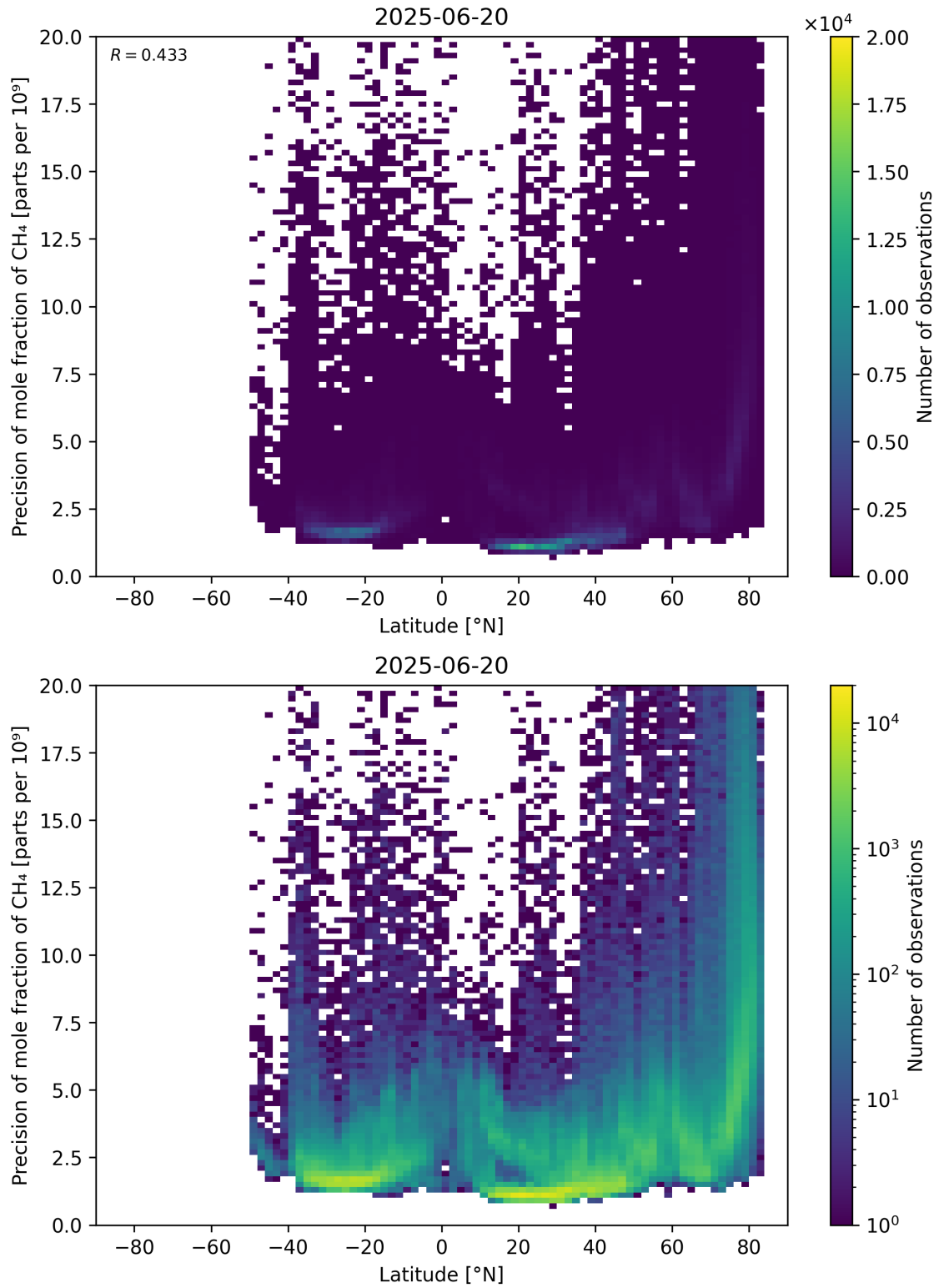
Figure 59: Scatter density plot of “Latitude” against “Precision of mole fraction of \text{CH}_4 ” for 2025-06-19 to 2025-06-21.
