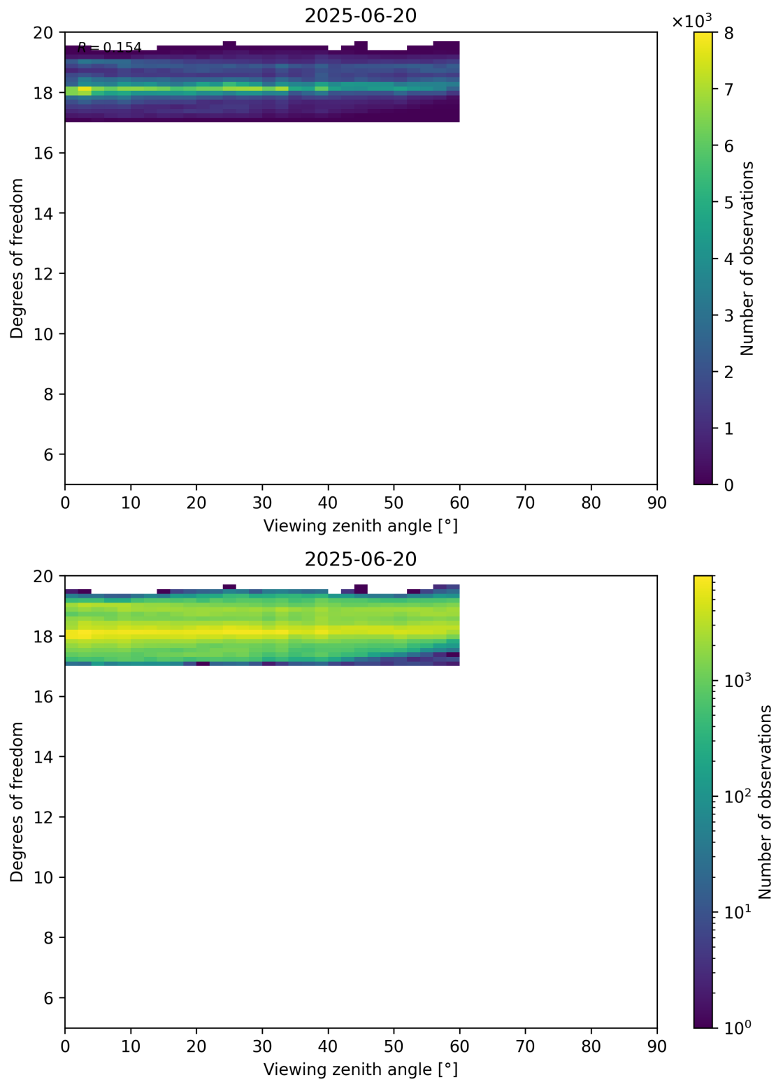
Figure 107: Scatter density plot of “Viewing zenith angle” against “Degrees of freedom” for 2025-06-19 to 2025-06-21.
