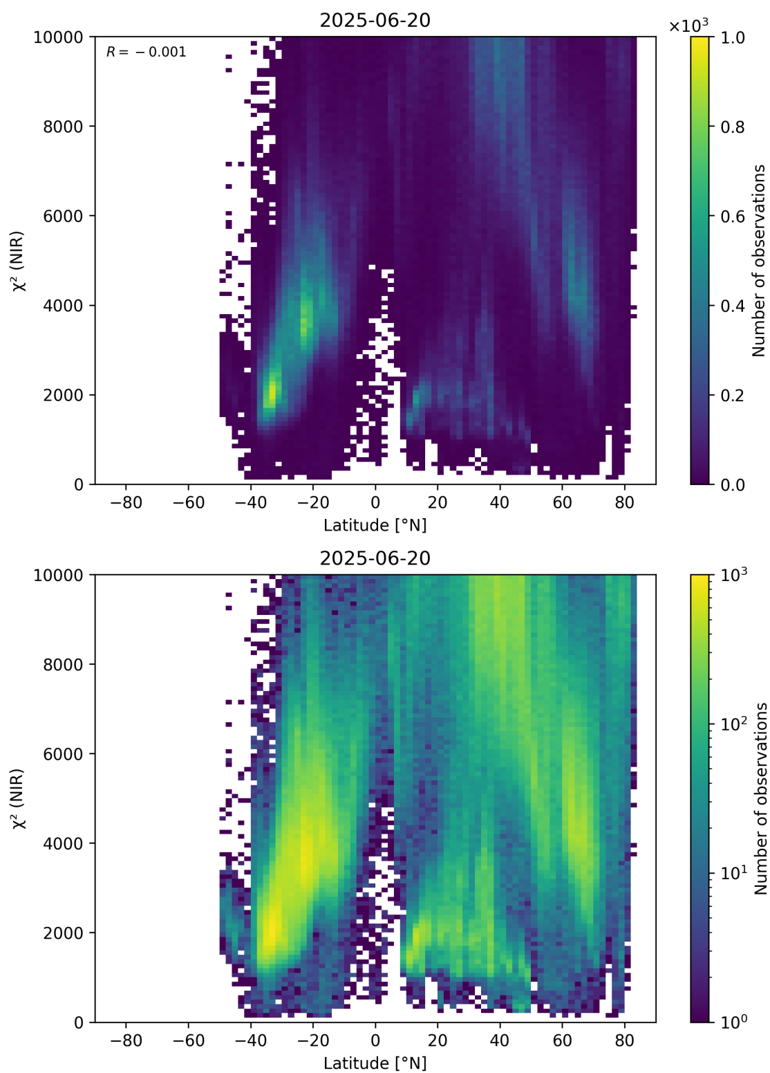
Figure 53: Scatter density plot of “Latitude” against “ \chi^2 (NIR)” for 2025-06-19 to 2025-06-21.
