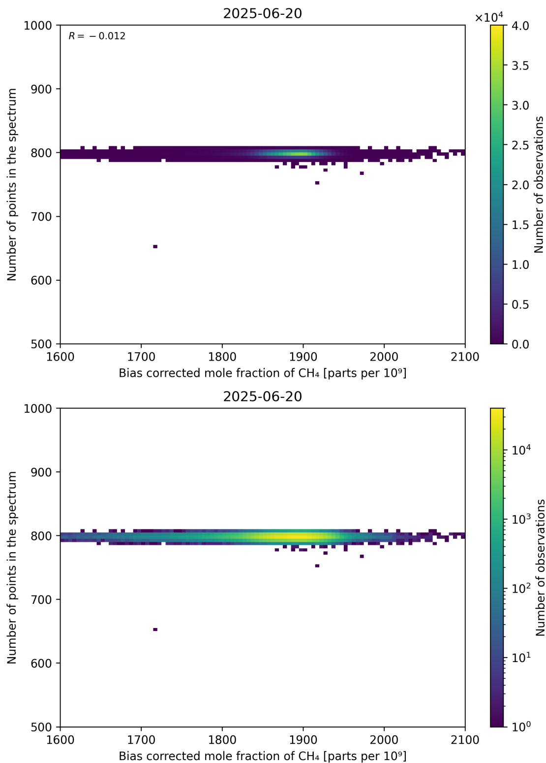
Figure 68: Scatter density plot of “Bias corrected mole fraction of CH 4 ” against “Number of points in the spectrum” for 2025-06-19 to 2025-06-21.
