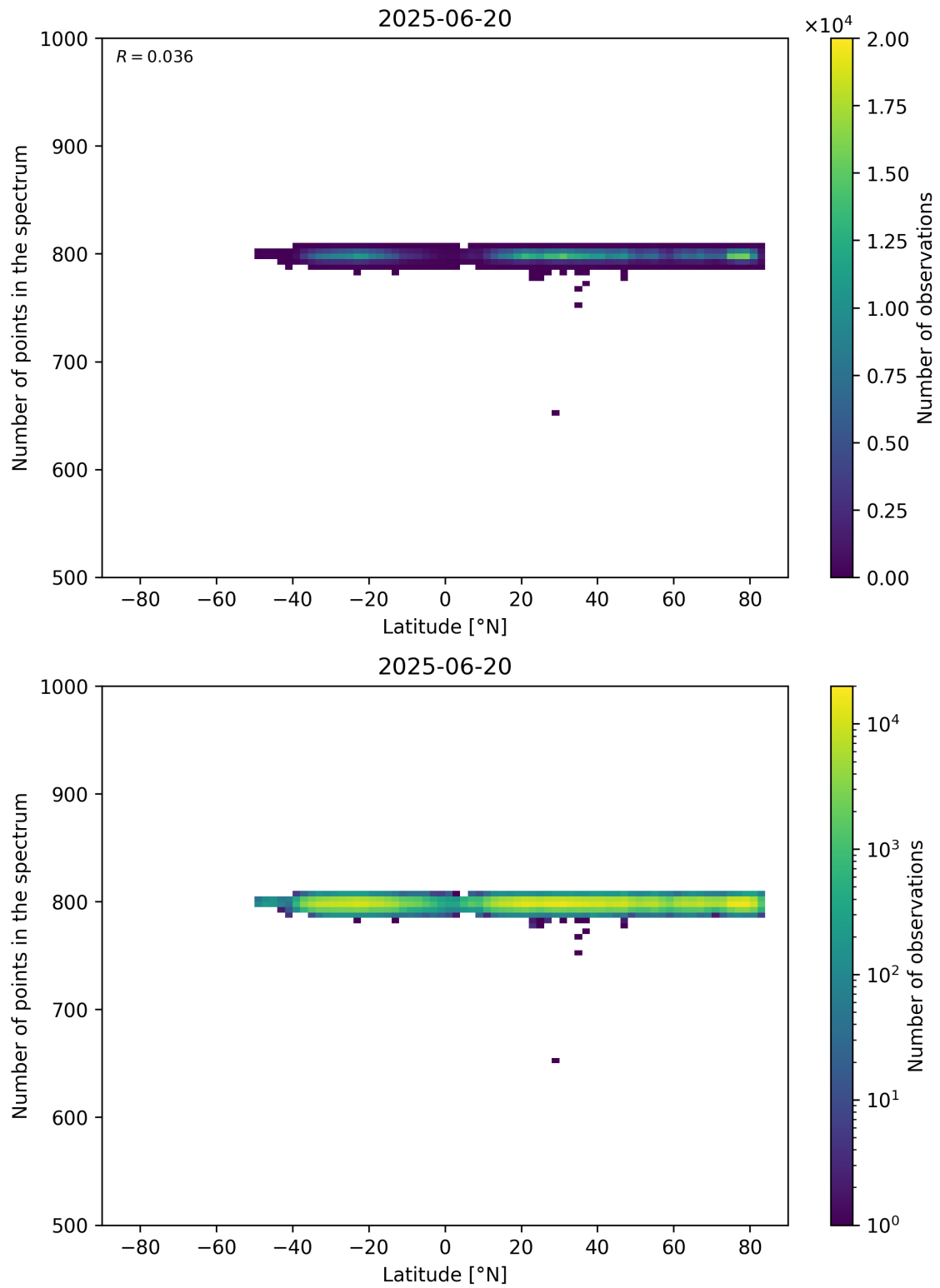
Figure 61: Scatter density plot of “Latitude” against “Number of points in the spectrum” for 2025-06-19 to 2025-06-21.
