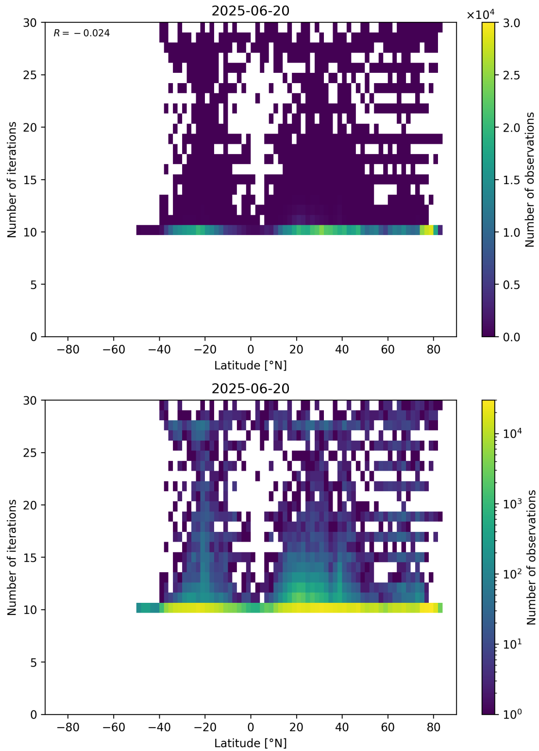
Figure 60: Scatter density plot of “Latitude” against “Number of iterations” for 2025-06-19 to 2025-06-21.
