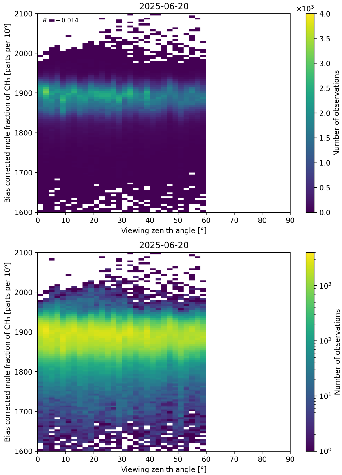
Figure 111: Scatter density plot of “Viewing zenith angle” against “Bias corrected mole fraction of CH 4 ” for 2025-06-19 to 2025-06-21.
