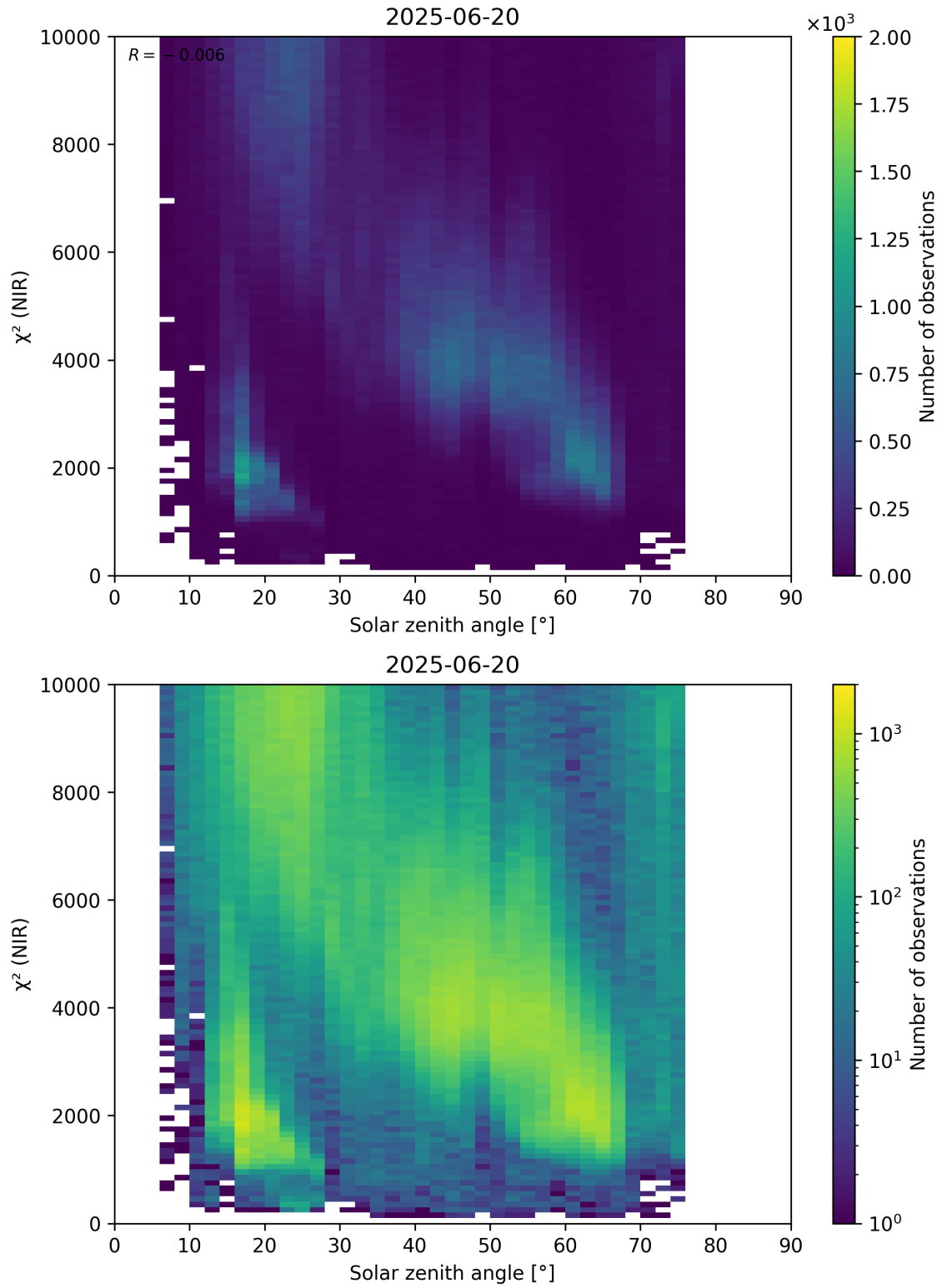
Figure 94: Scatter density plot of “Solar zenith angle” against “ \chi^2 (NIR)” for 2025-06-19 to 2025-06-21.
