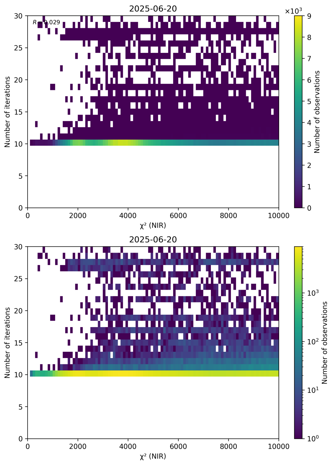
Figure 46: Scatter density plot of “ \chi^2 (NIR)” against “Number of iterations” for 2025-06-19 to 2025-06-21.
