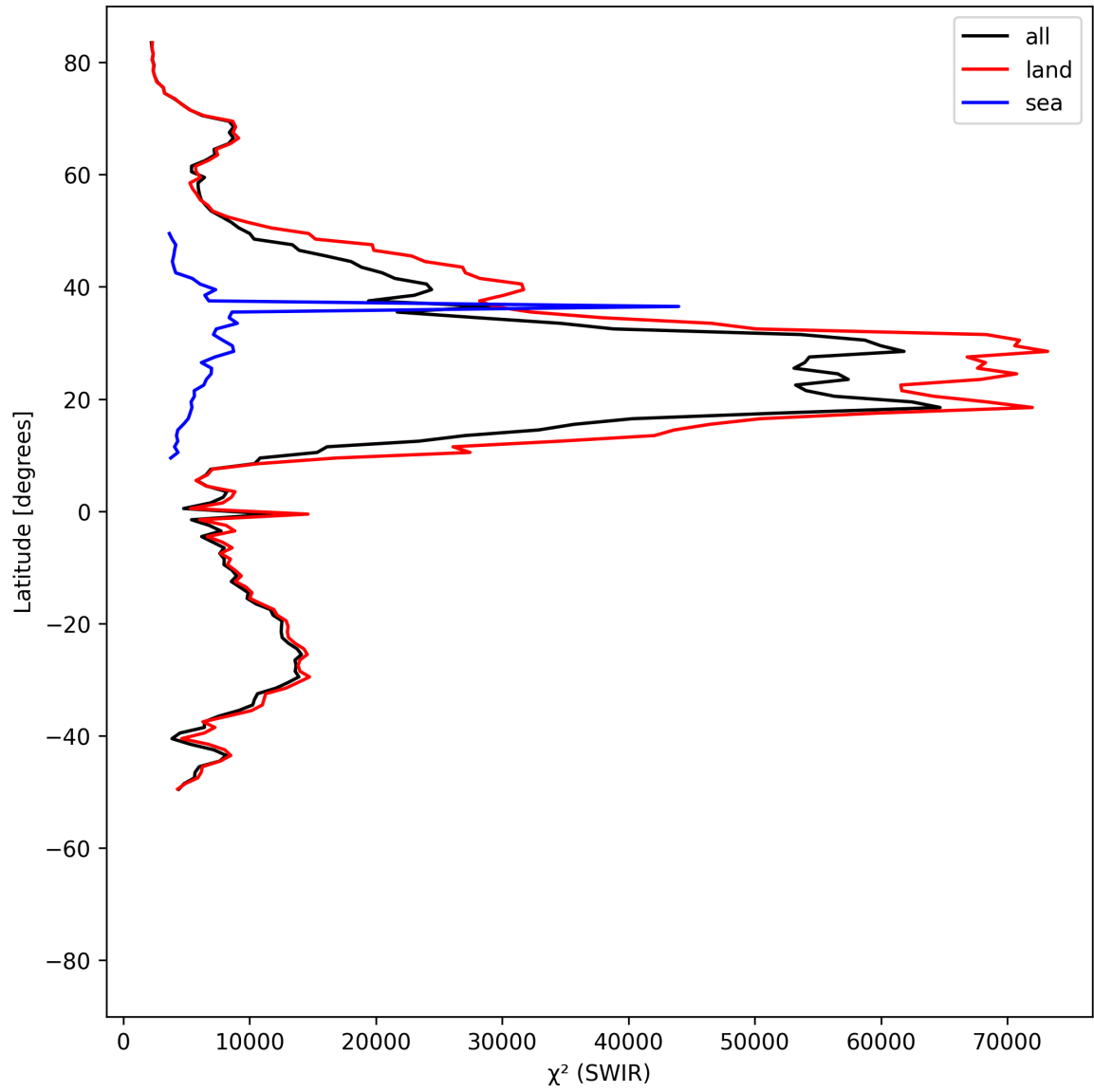
Figure 17: Zonal average of “ \chi^2 (SWIR)” for 2025-06-19 to 2025-06-21.
