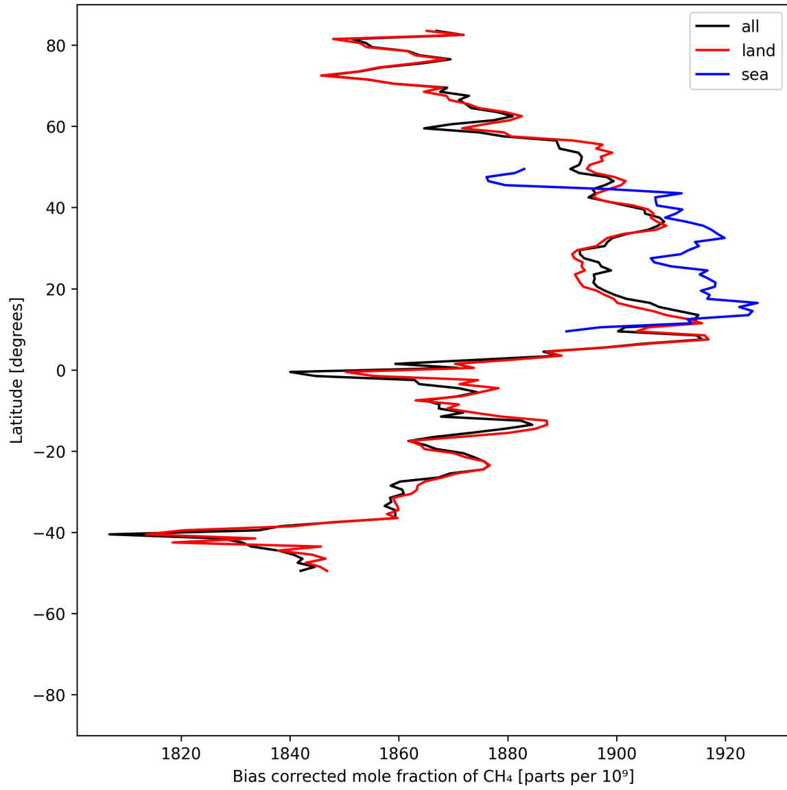
Figure 14: Zonal average of “Bias corrected mole fraction of \text{CH}_4 ” for 2025-06-19 to 2025-06-21.
