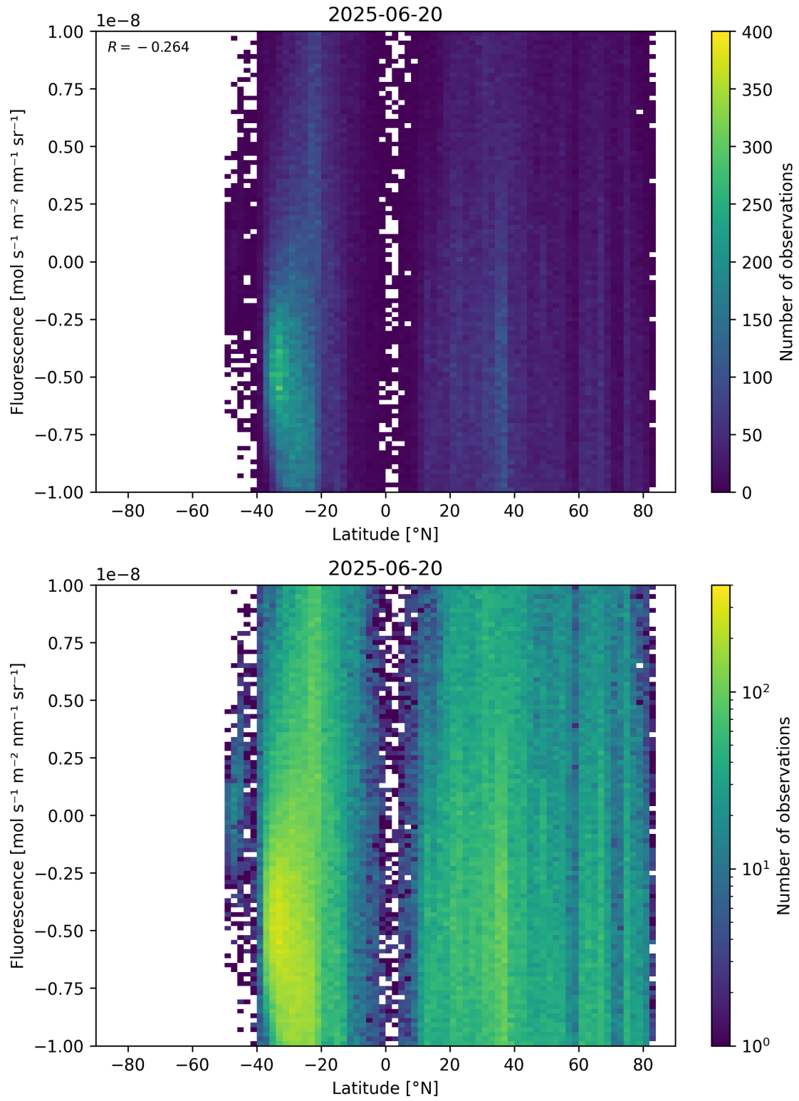
Figure 56: Scatter density plot of “Latitude” against “Fluorescence” for 2025-06-19 to 2025-06-21.
