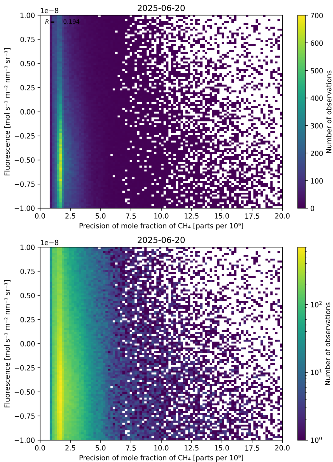
Figure 81: Scatter density plot of “Precision of mole fraction of \text{CH}_4 ” against “Fluorescence” for 2025-06-19 to 2025-06-21.
