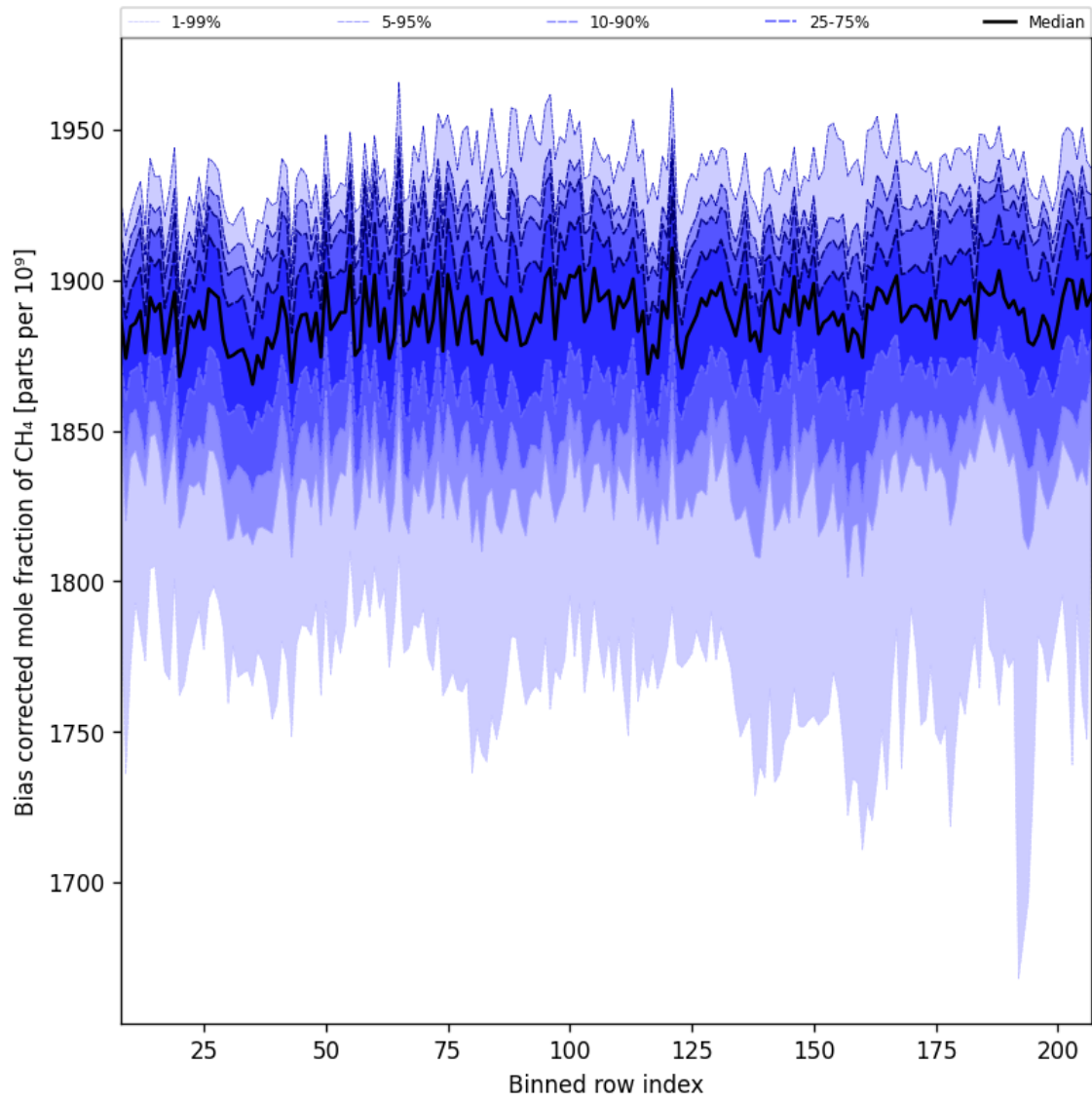
Figure 36: Along track statistics of “Bias corrected mole fraction of CH 4 ” for 2025-06-19 to 2025-06-21
