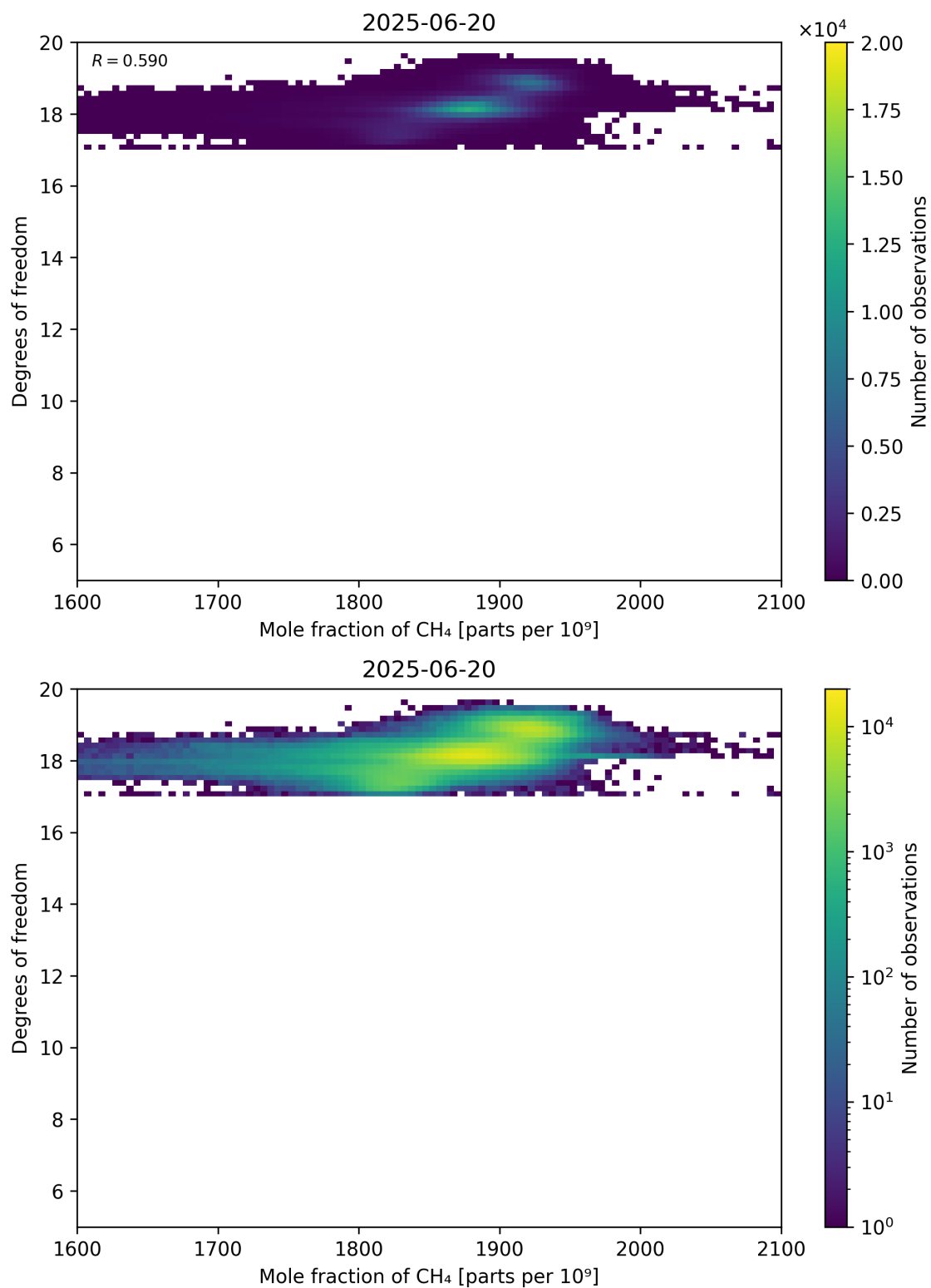
Figure 72: Scatter density plot of “Mole fraction of CH 4 ” against “Degrees of freedom” for 2025-06-19 to 2025-06-21.
