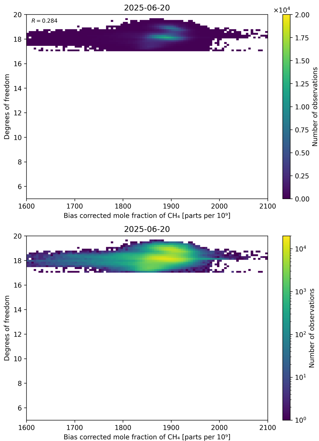
Figure 65: Scatter density plot of “Bias corrected mole fraction of CH 4 ” against “Degrees of freedom” for 2025-06-19 to 2025-06-21.
