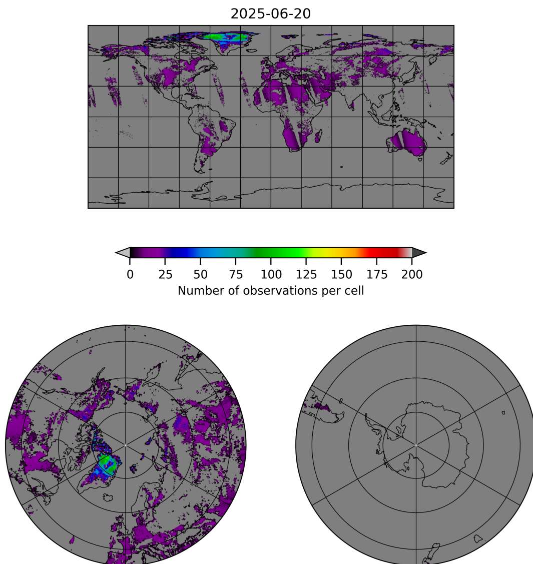
Figure 10: Map of the number of observations for 2025-06-19 to 2025-06-21
