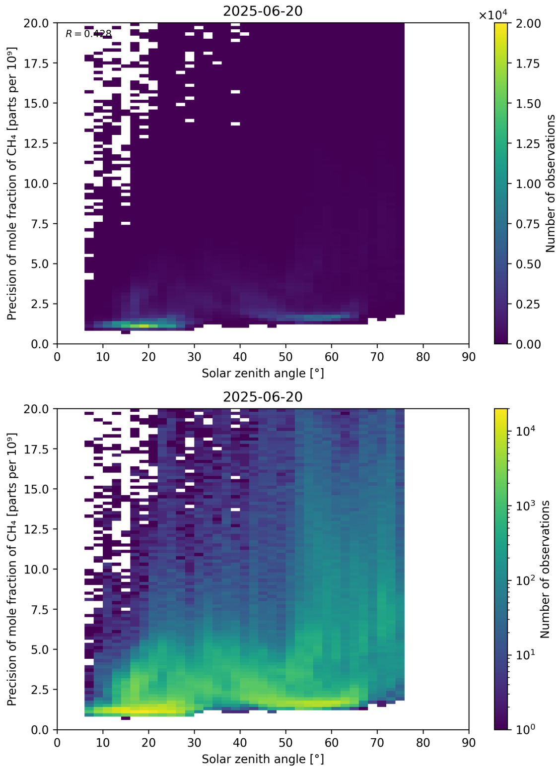
Figure 101: Scatter density plot of “Solar zenith angle” against “Precision of mole fraction of CH 4 ” for 2025-06-19 to 2025-06-21.
