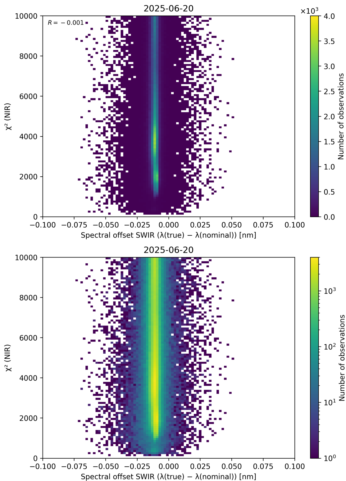
Figure 117: Scatter density plot of “Spectral offset SWIR ( \lambda_{\text{true}} - \lambda_{\text{nominal}} )” against “ \chi^2 (NIR)” for 2025-06-19 to 2025-06-21.
