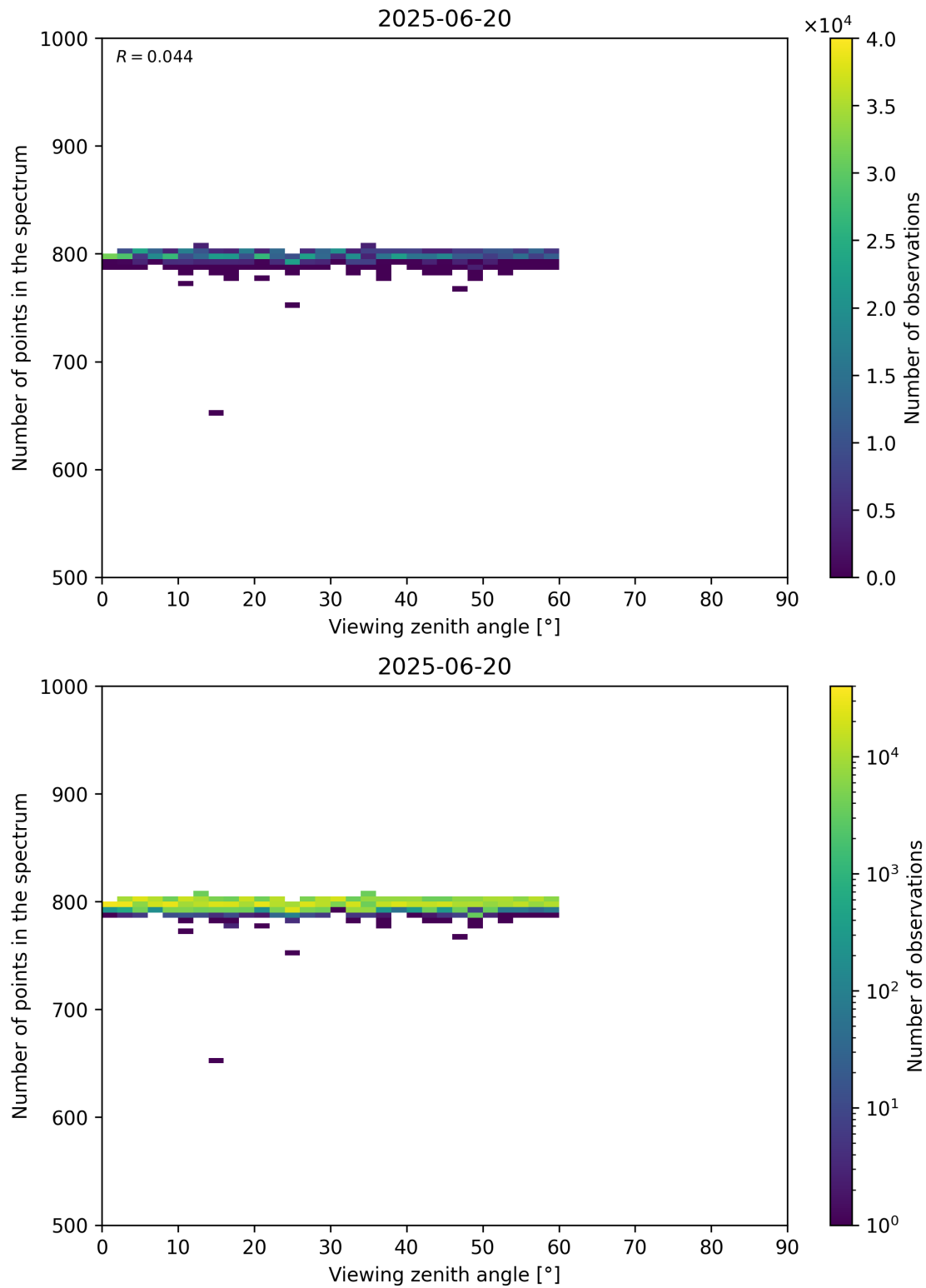
Figure 114: Scatter density plot of “Viewing zenith angle” against “Number of points in the spectrum” for 2025-06-19 to 2025-06-21.
