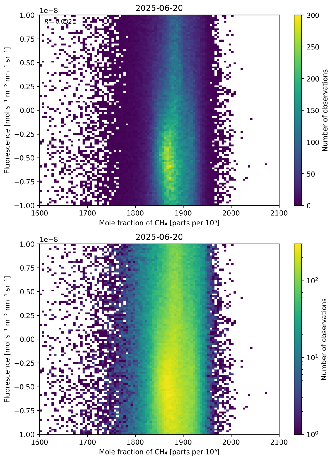
Figure 73: Scatter density plot of “Mole fraction of \text{CH}_4 ” against “Fluorescence” for 2025-06-19 to 2025-06-21.
