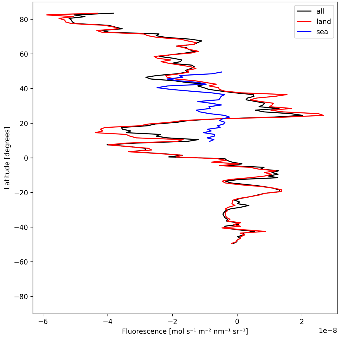
Figure 21: Zonal average of “Fluorescence” for 2025-06-19 to 2025-06-21.
