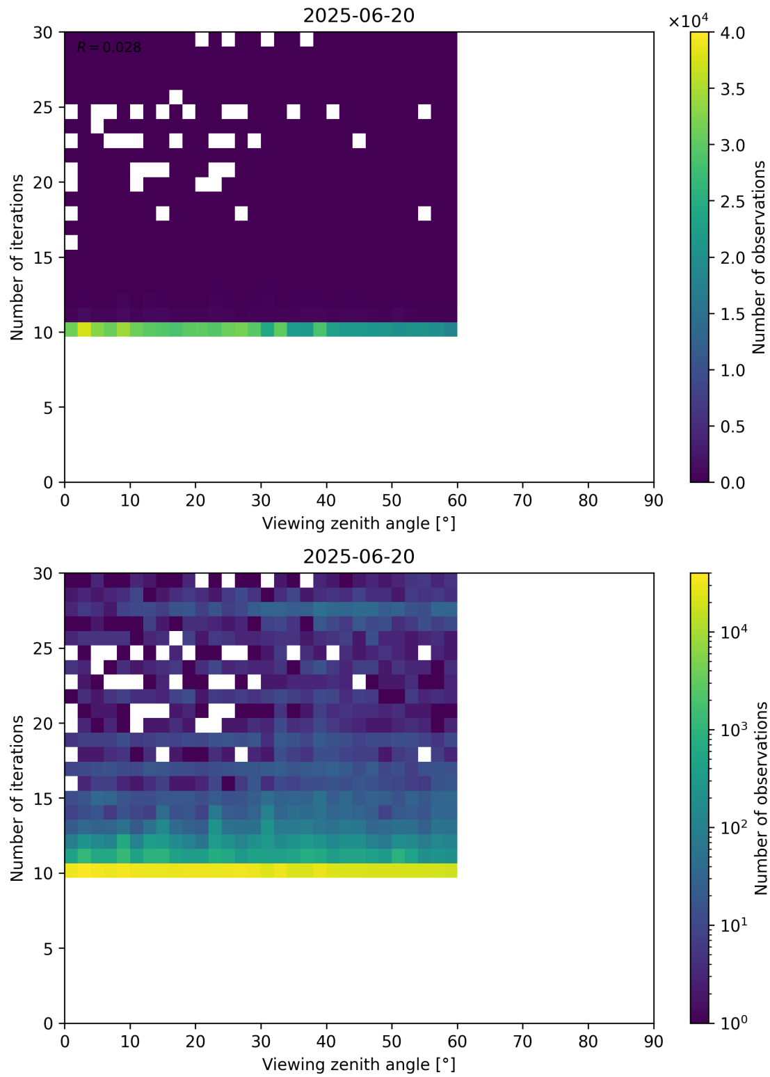
Figure 113: Scatter density plot of “Viewing zenith angle” against “Number of iterations” for 2025-06-19 to 2025-06-21.
