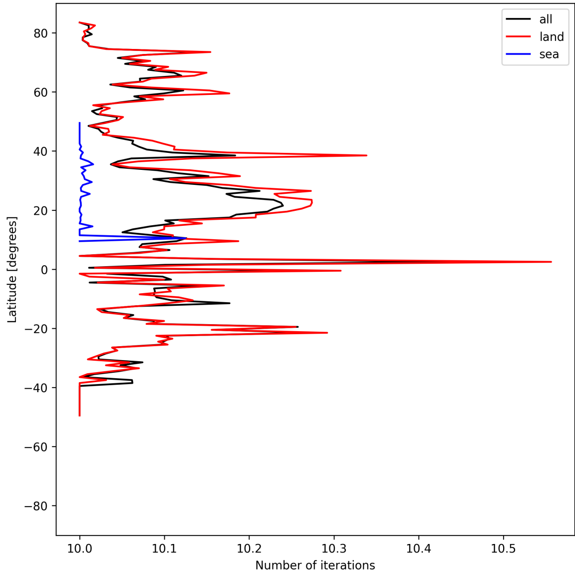
Figure 20: Zonal average of “Number of iterations” for 2025-06-19 to 2025-06-21.
