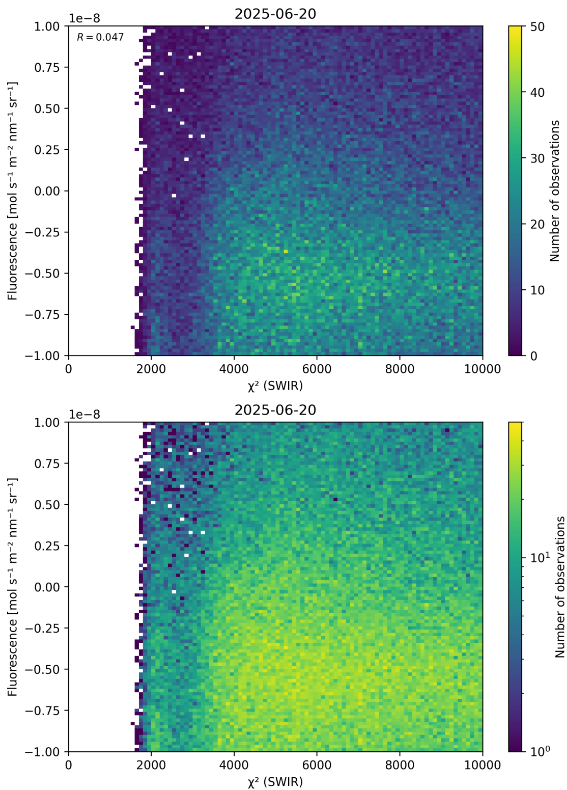
Figure 49: Scatter density plot of “ \chi^2 (SWIR)” against “Fluorescence” for 2025-06-19 to 2025-06-21.
