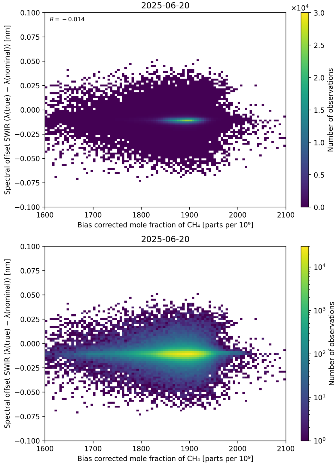
Figure 69: Scatter density plot of “Bias corrected mole fraction of \text{CH}_4 ” against “Spectral offset SWIR ( \lambda_{\text{true}} - \lambda_{\text{nominal}} )” for 2025-06-19 to 2025-06-21.
