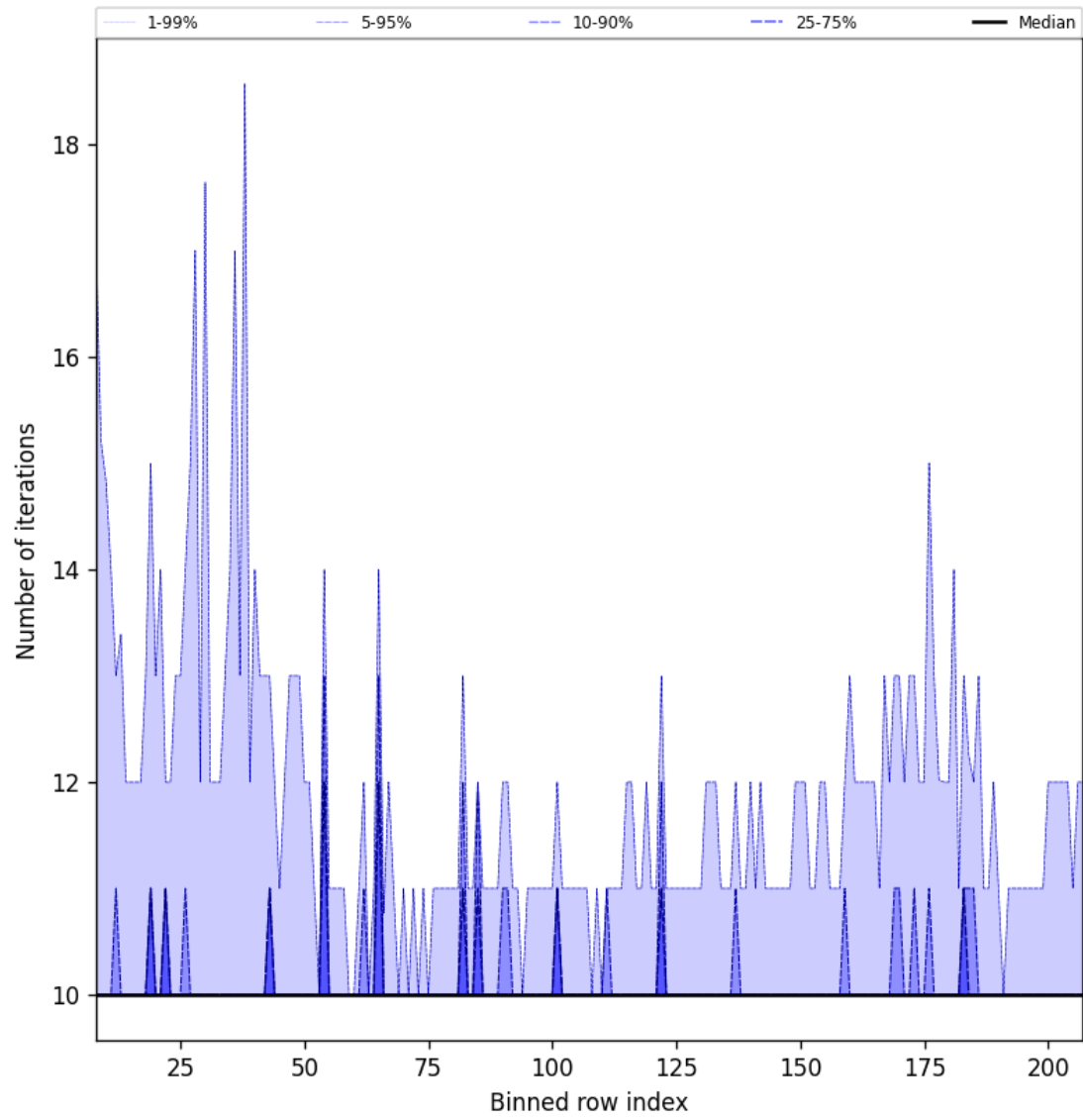
Figure 42: Along track statistics of “Number of iterations” for 2025-06-19 to 2025-06-21
