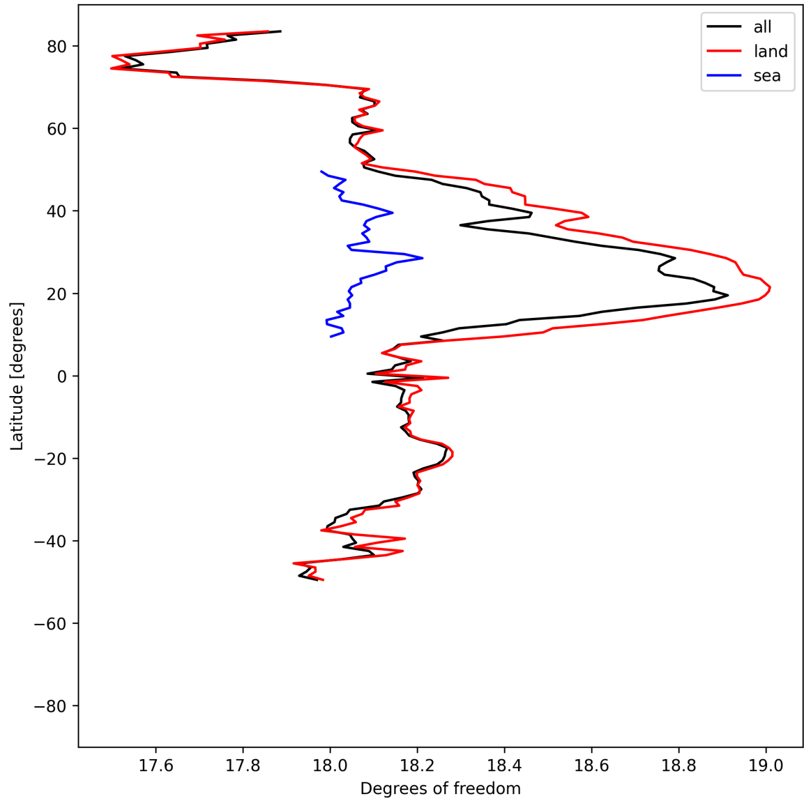
Figure 19: Zonal average of “Degrees of freedom” for 2025-06-19 to 2025-06-21.
