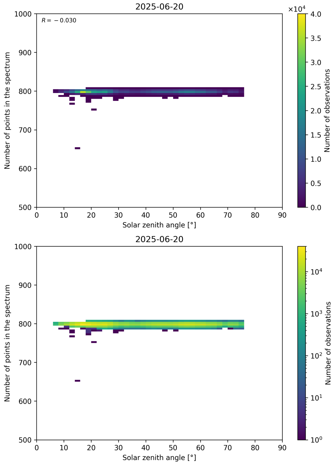
Figure 103: Scatter density plot of “Solar zenith angle” against “Number of points in the spectrum” for 2025-06-19 to 2025-06-21.
