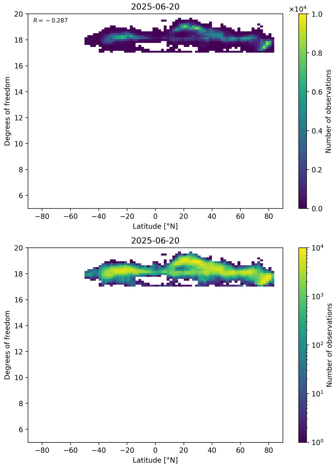
Figure 55: Scatter density plot of “Latitude” against “Degrees of freedom” for 2025-06-19 to 2025-06-21.
