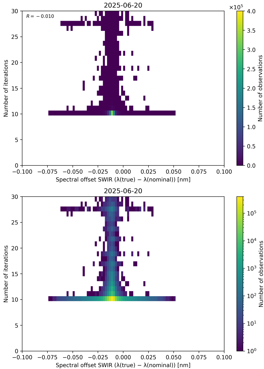
Figure 121: Scatter density plot of “Spectral offset SWIR ( \lambda_{\text{true}} - \lambda_{\text{nominal}} )” against “Number of iterations” for 2025-06-19 to 2025-06-21.
