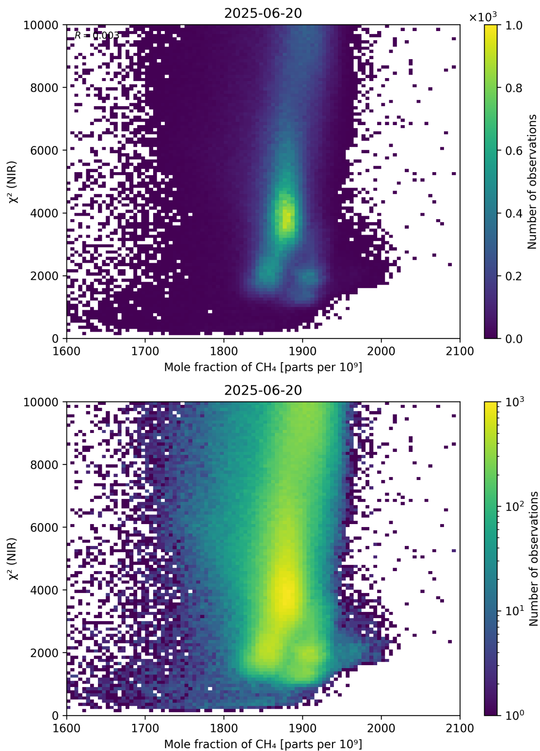
Figure 70: Scatter density plot of “Mole fraction of \text{CH}_4 ” against “ \chi^2 (NIR)” for 2025-06-19 to 2025-06-21.
