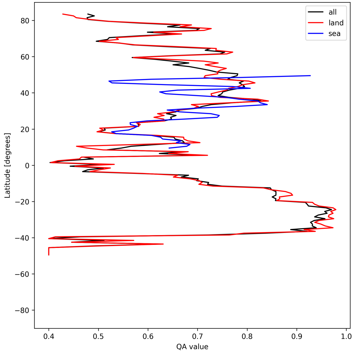
Figure 11: Zonal average of “QA value” for 2025-06-19 to 2025-06-21.
