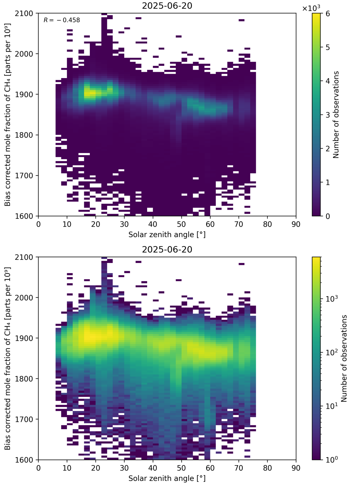
Figure 100: Scatter density plot of “Solar zenith angle” against “Bias corrected mole fraction of \text{CH}_4 ” for 2025-06-19 to 2025-06-21.
