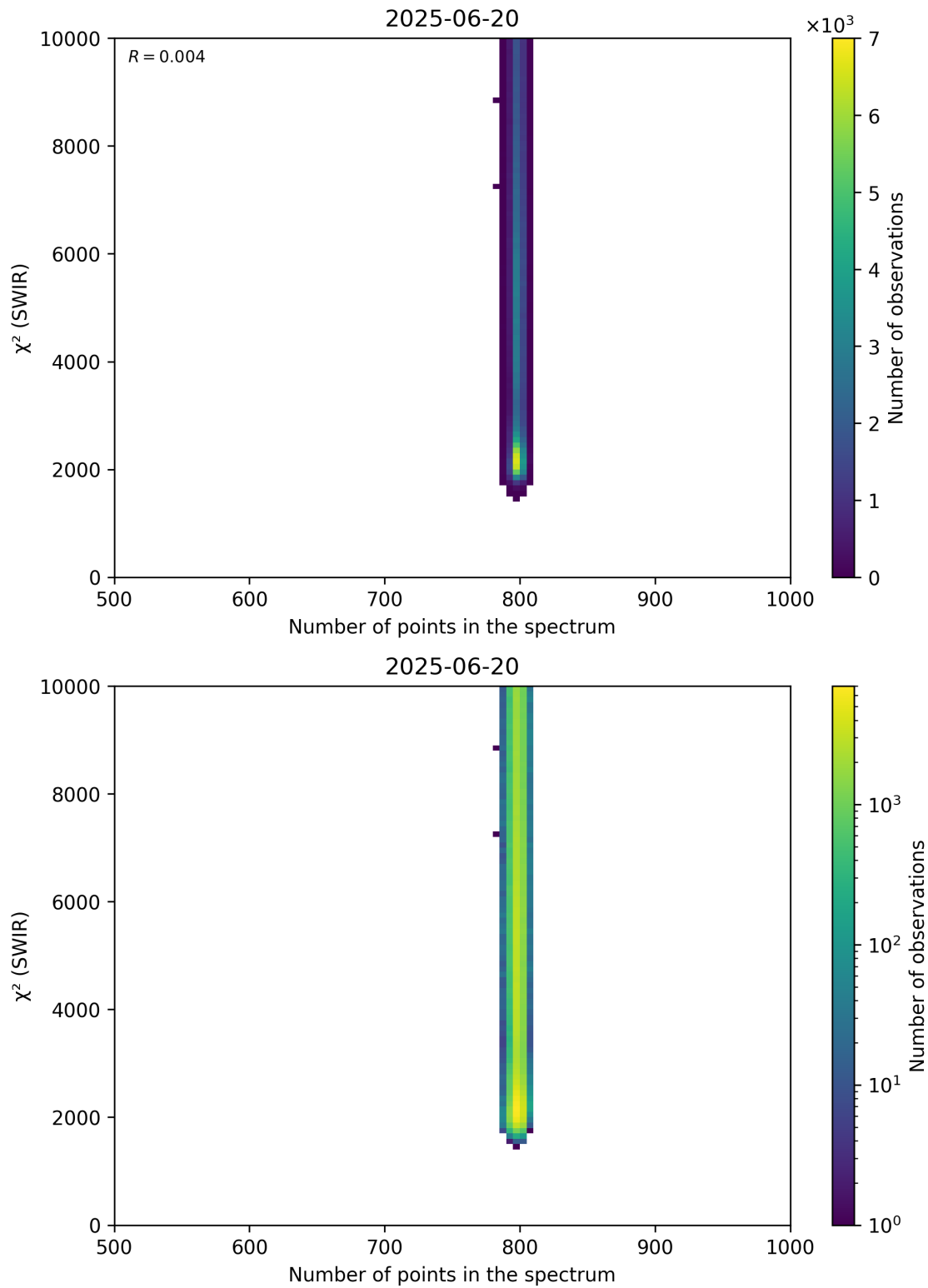
Figure 89: Scatter density plot of “Number of points in the spectrum” against “ \chi^2 (SWIR)” for 2025-06-19 to 2025-06-21.
