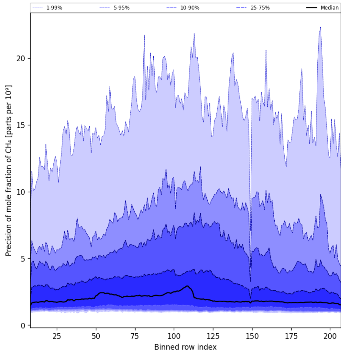
Figure 35: Along track statistics of “Precision of mole fraction of CH 4 ” for 2025-06-19 to 2025-06-21
