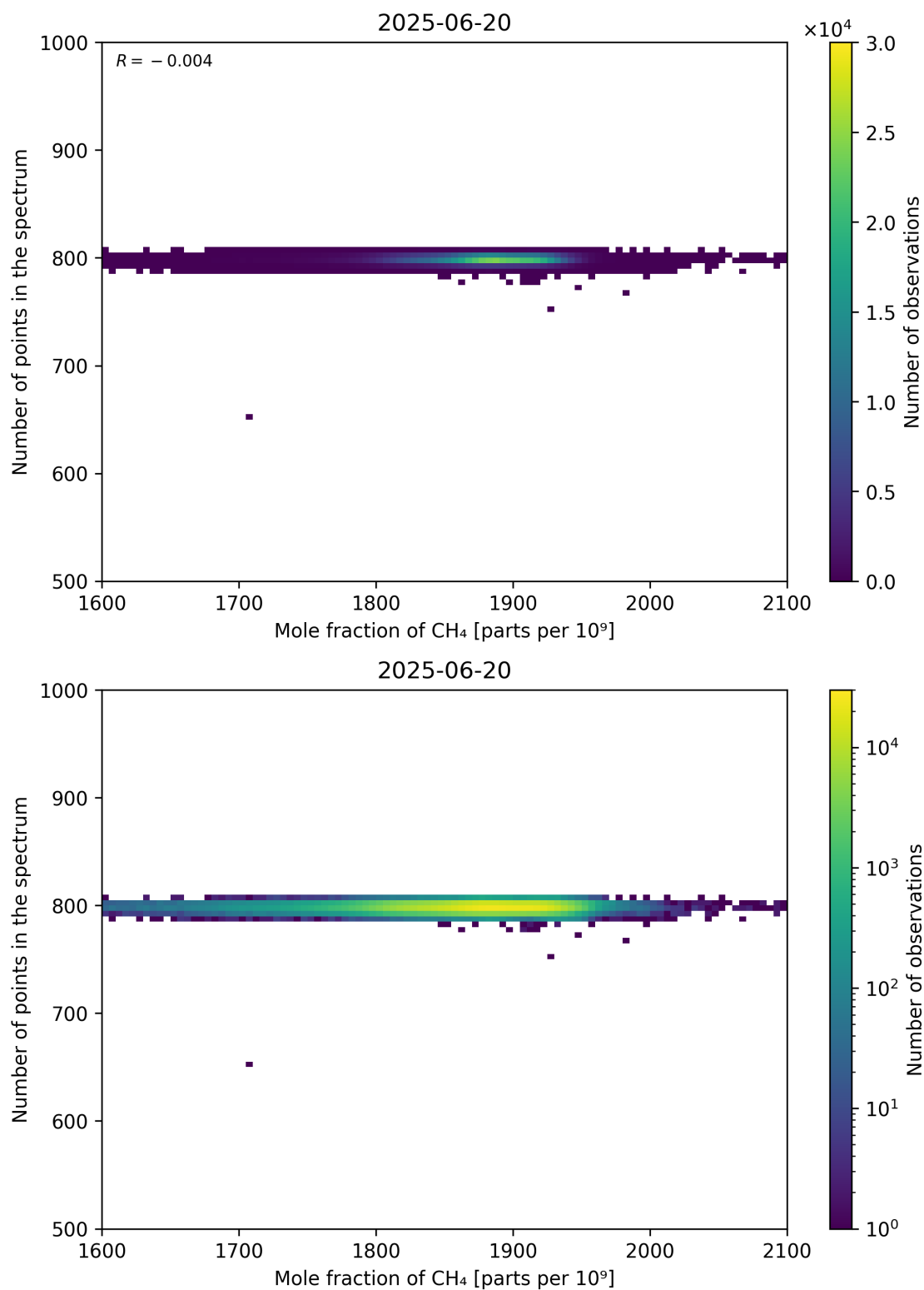
Figure 77: Scatter density plot of “Mole fraction of CH 4 ” against “Number of points in the spectrum” for 2025-06-19 to 2025-06-21.
