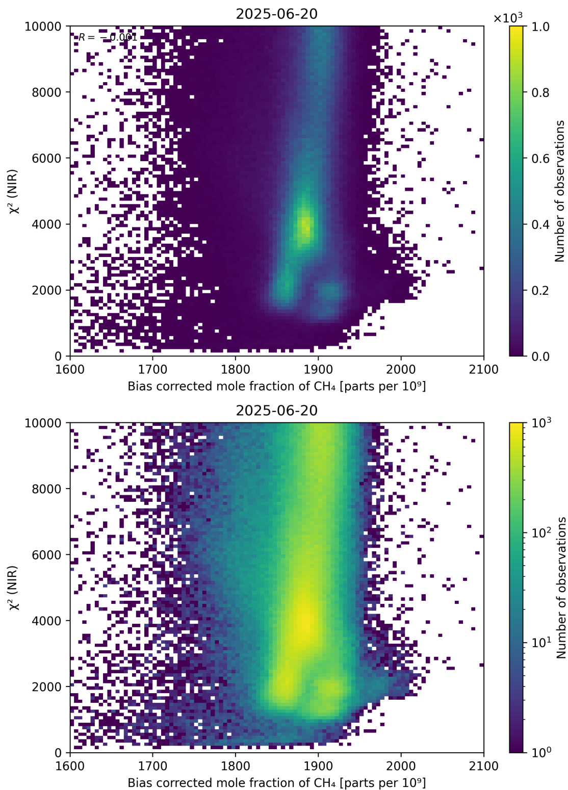
Figure 63: Scatter density plot of “Bias corrected mole fraction of \text{CH}_4 ” against “ \chi^2 (NIR)” for 2025-06-19 to 2025-06-21.
