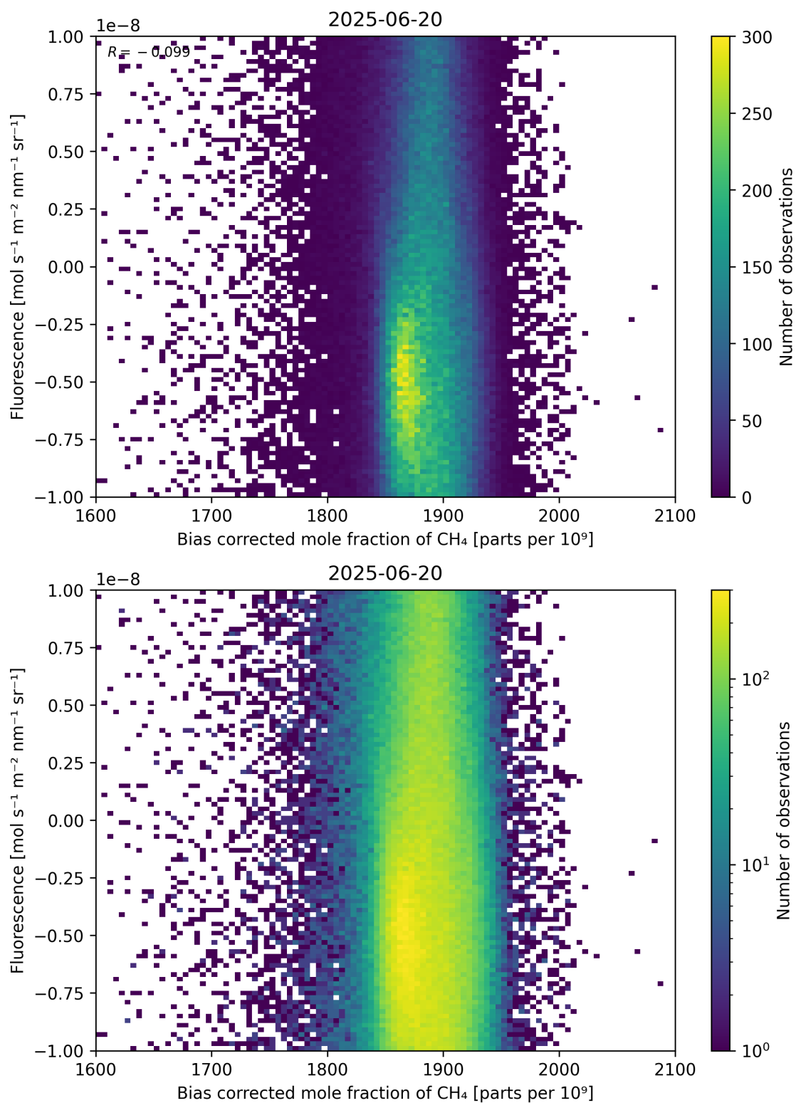
Figure 66: Scatter density plot of “Bias corrected mole fraction of \text{CH}_4 ” against “Fluorescence” for 2025-06-19 to 2025-06-21.
