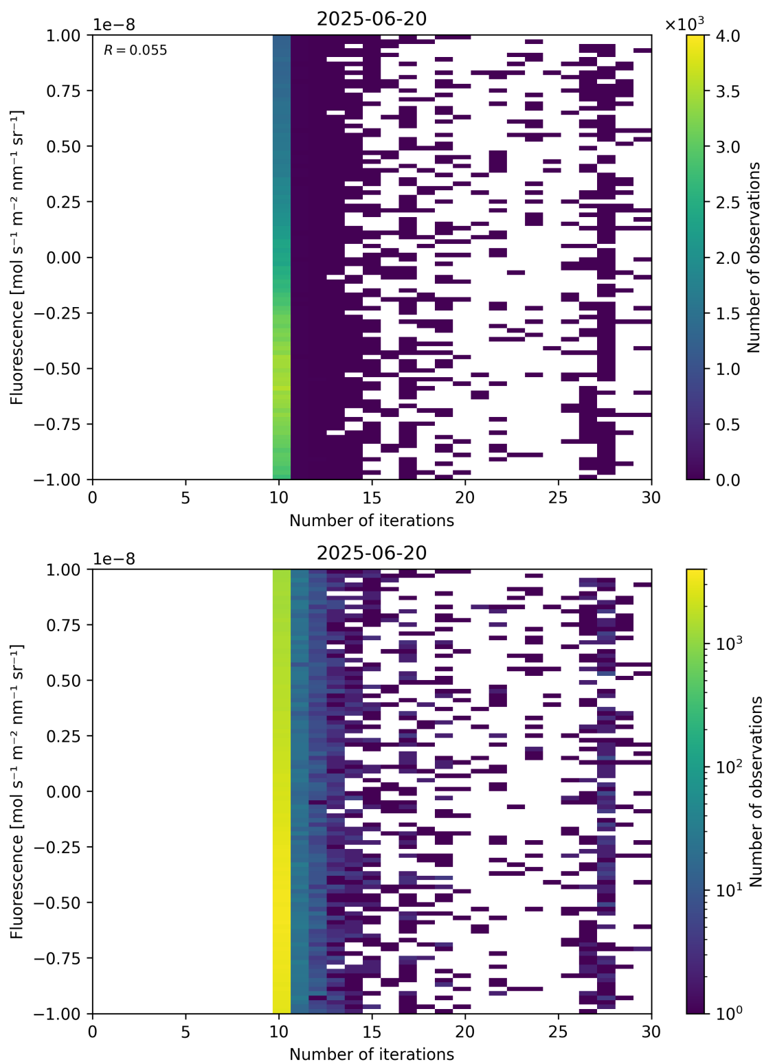
Figure 87: Scatter density plot of “Number of iterations” against “Fluorescence” for 2025-06-19 to 2025-06-21.
