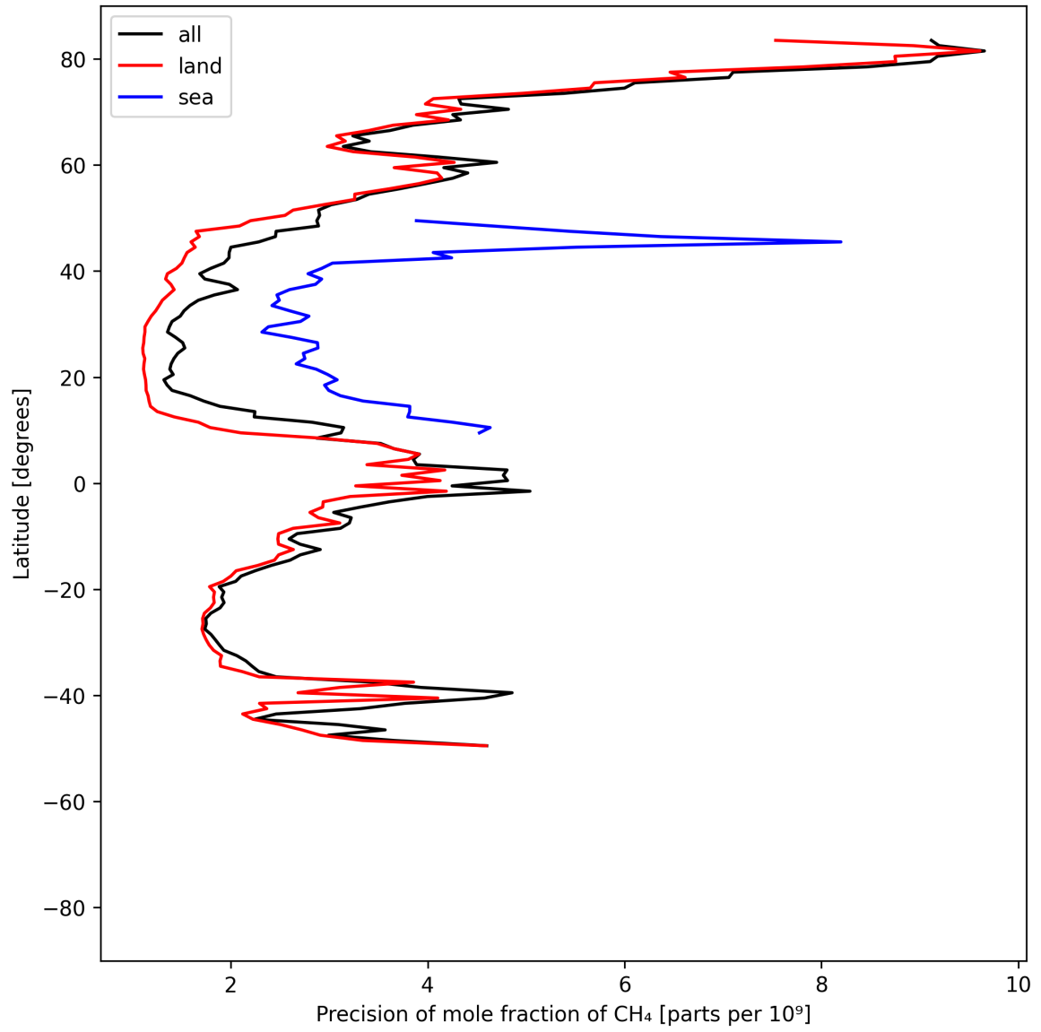
Figure 13: Zonal average of “Precision of mole fraction of CH 4 ” for 2025-06-19 to 2025-06-21.
