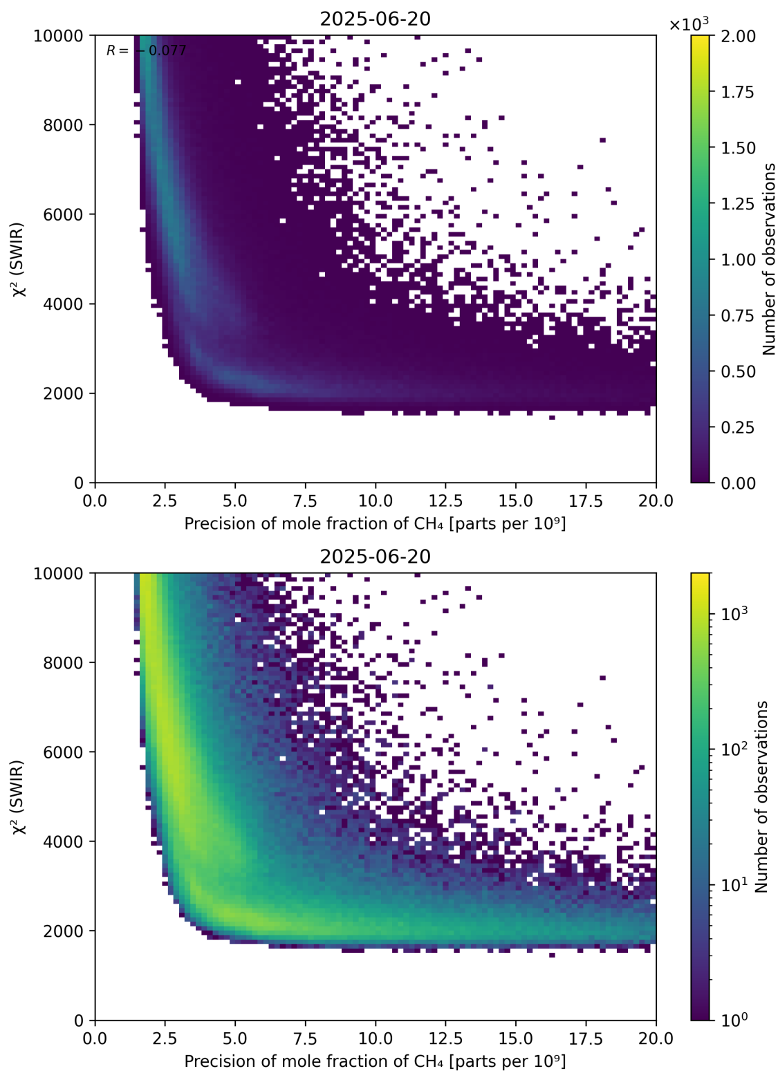
Figure 79: Scatter density plot of “Precision of mole fraction of \text{CH}_4 ” against “ \chi^2 (SWIR)” for 2025-06-19 to 2025-06-21.
