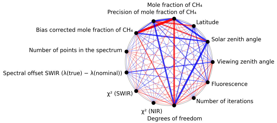
Figure 1: Map of correlation graph for 2025-06-19 to 2025-06-21.
