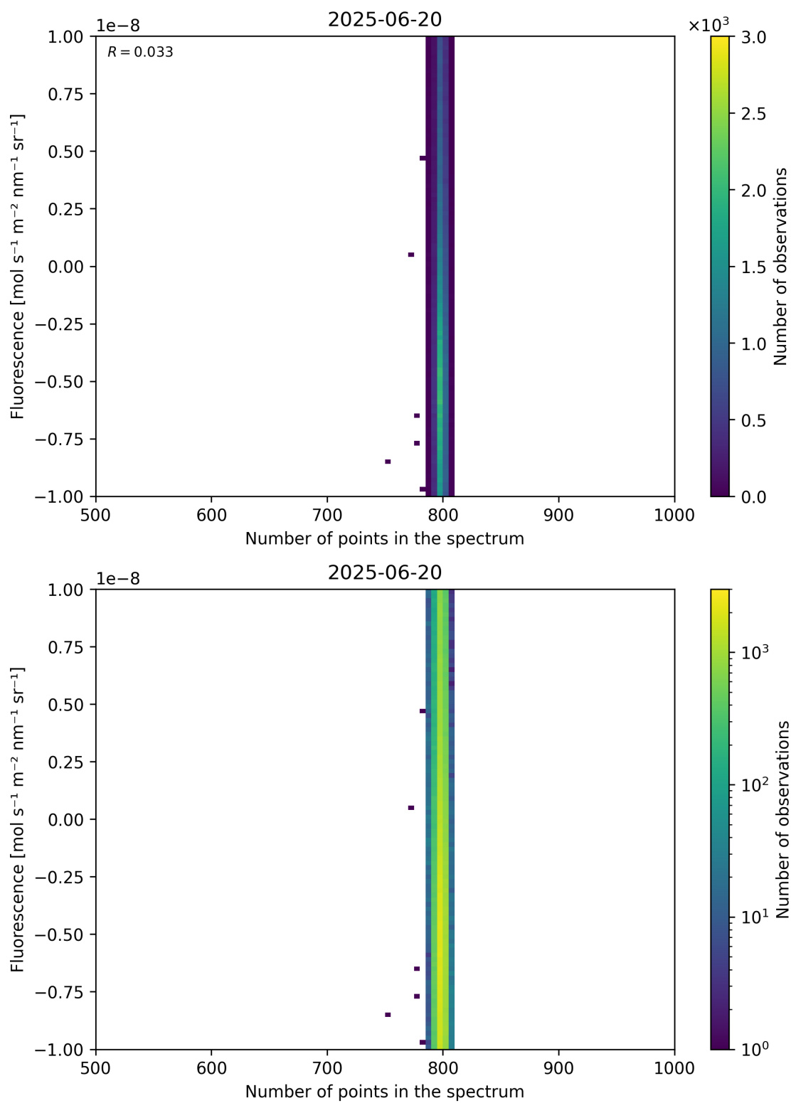
Figure 91: Scatter density plot of “Number of points in the spectrum” against “Fluorescence” for 2025-06-19 to 2025-06-21.
