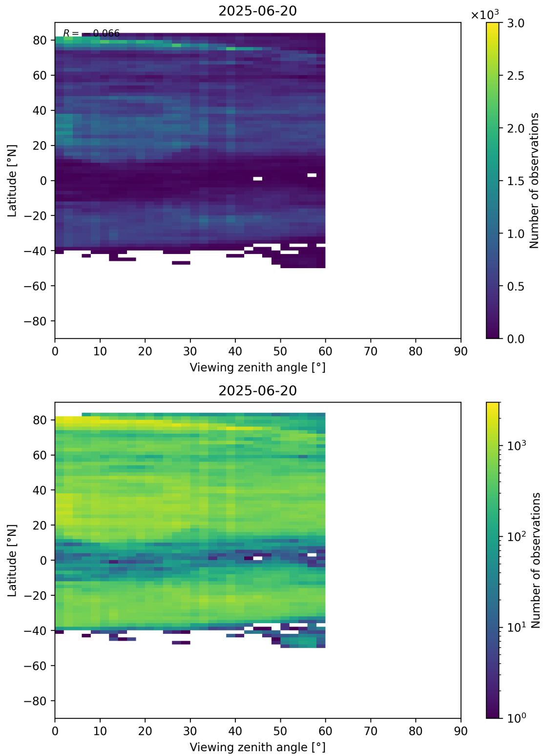
Figure 109: Scatter density plot of “Viewing zenith angle” against “Latitude” for 2025-06-19 to 2025-06-21.
