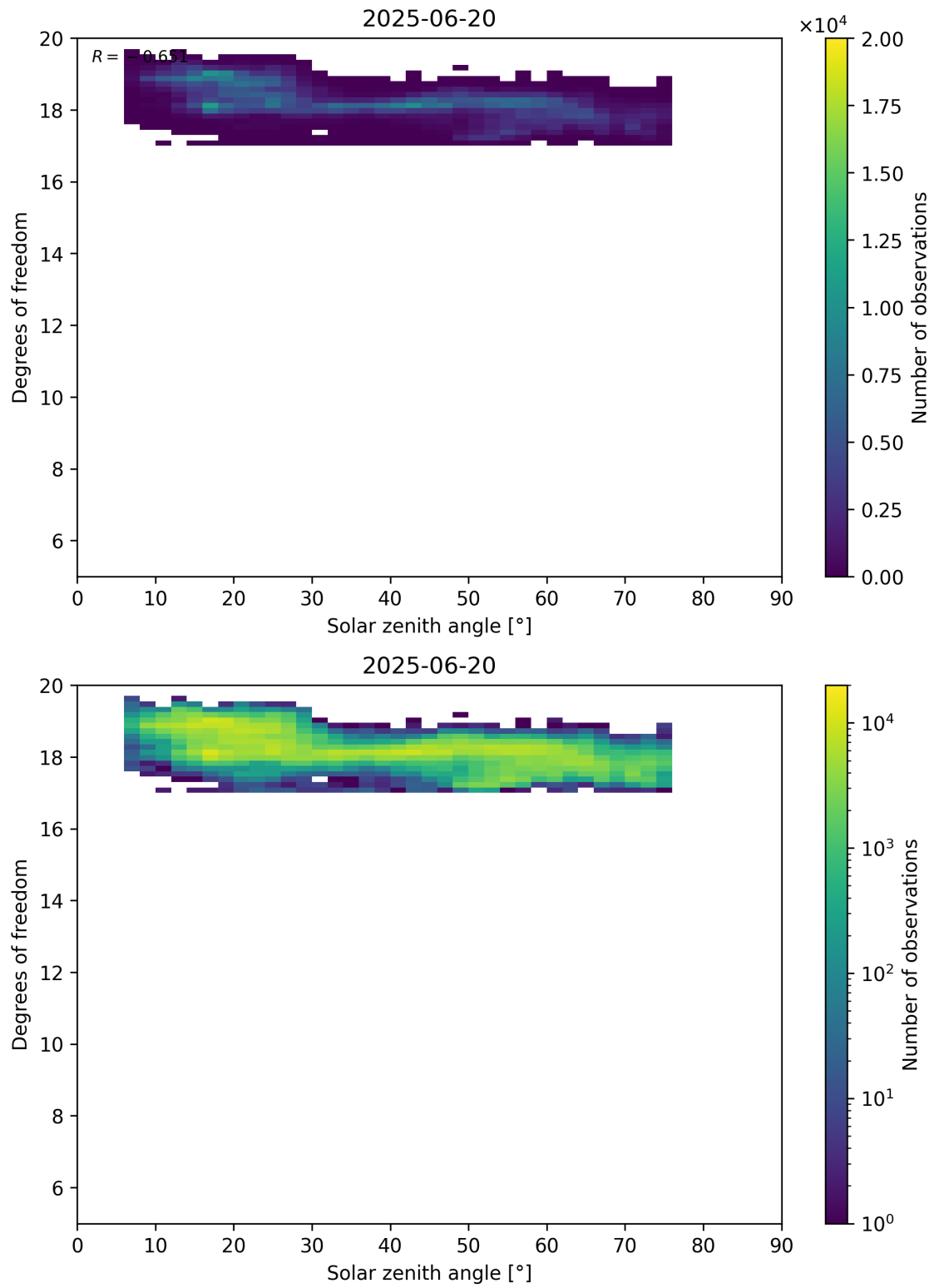
Figure 96: Scatter density plot of “Solar zenith angle” against “Degrees of freedom” for 2025-06-19 to 2025-06-21.
