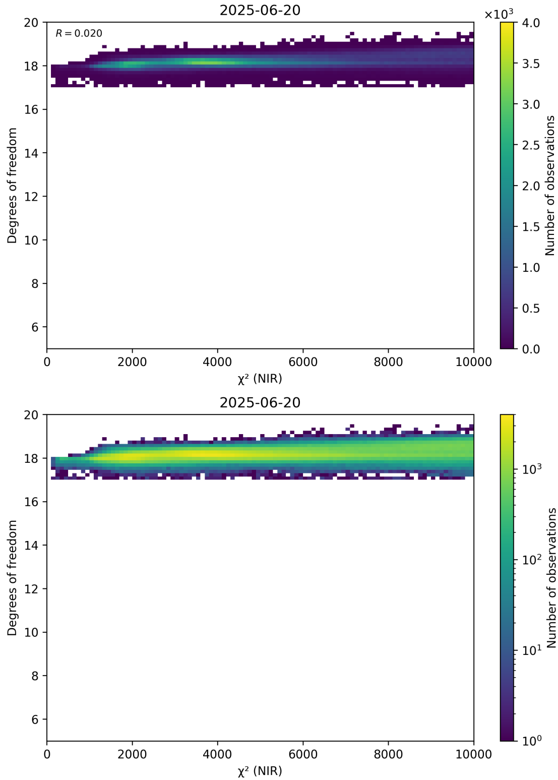
Figure 44: Scatter density plot of “ \chi^2 (NIR)” against “Degrees of freedom” for 2025-06-19 to 2025-06-21.
