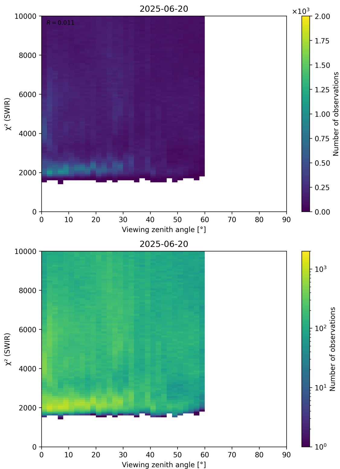
Figure 106: Scatter density plot of “Viewing zenith angle” against “ \chi^2 (SWIR)” for 2025-06-19 to 2025-06-21.
