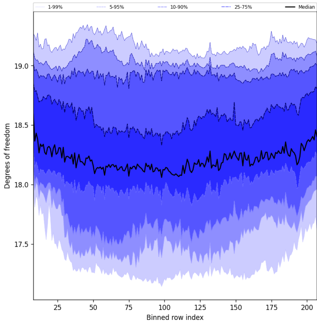
Figure 41: Along track statistics of “Degrees of freedom” for 2025-06-19 to 2025-06-21
