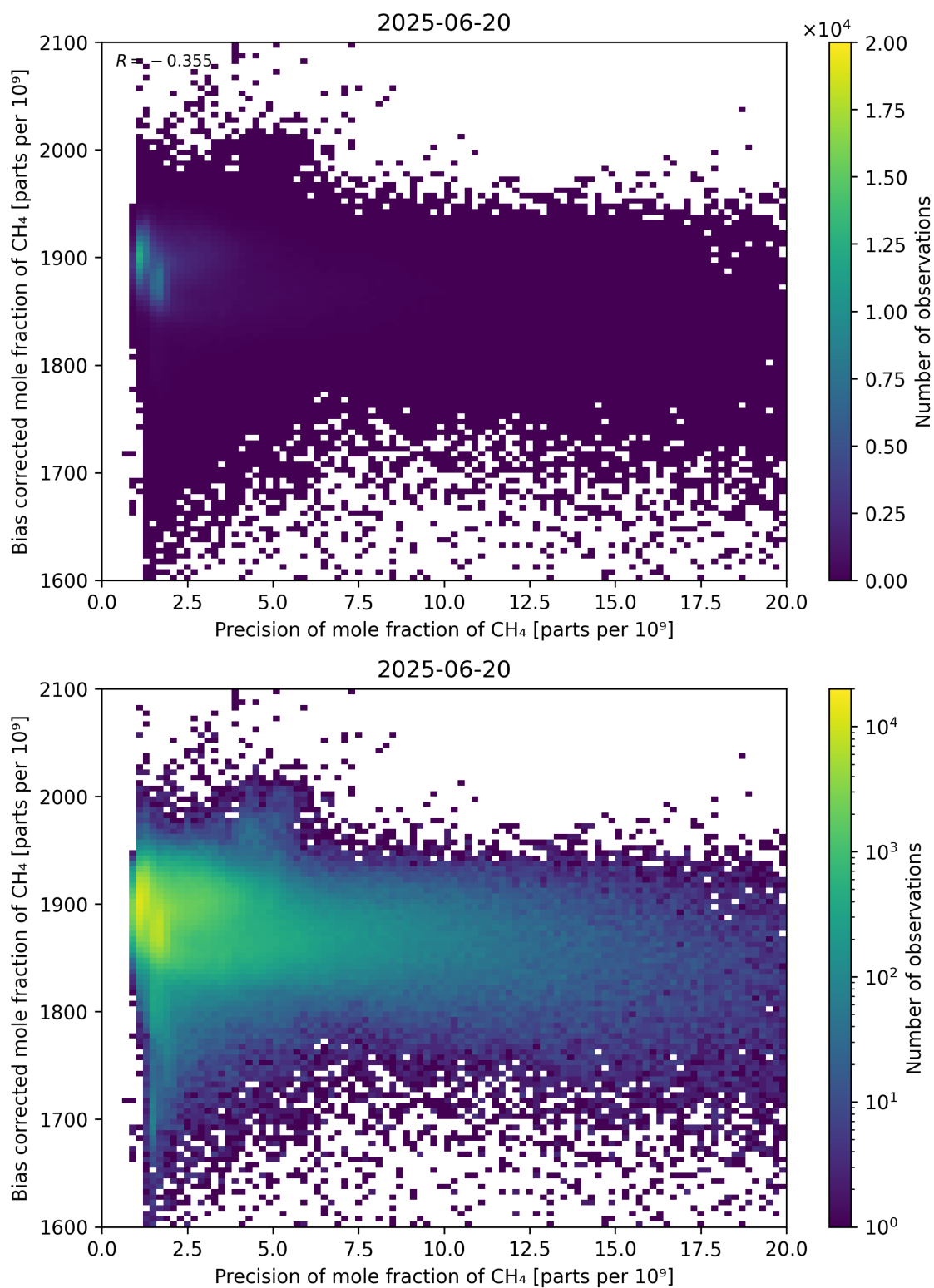
Figure 82: Scatter density plot of “Precision of mole fraction of CH 4 ” against “Bias corrected mole fraction of CH 4 ” for 2025-06-19 to 2025-06-21.
