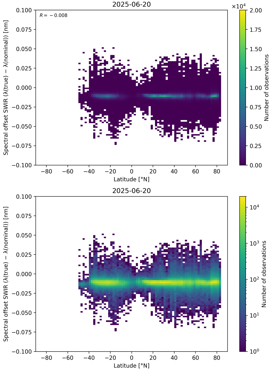
Figure 62: Scatter density plot of “Latitude” against “Spectral offset SWIR ( \lambda_{\text{true}} - \lambda_{\text{nominal}} )” for 2025-06-19 to 2025-06-21.
