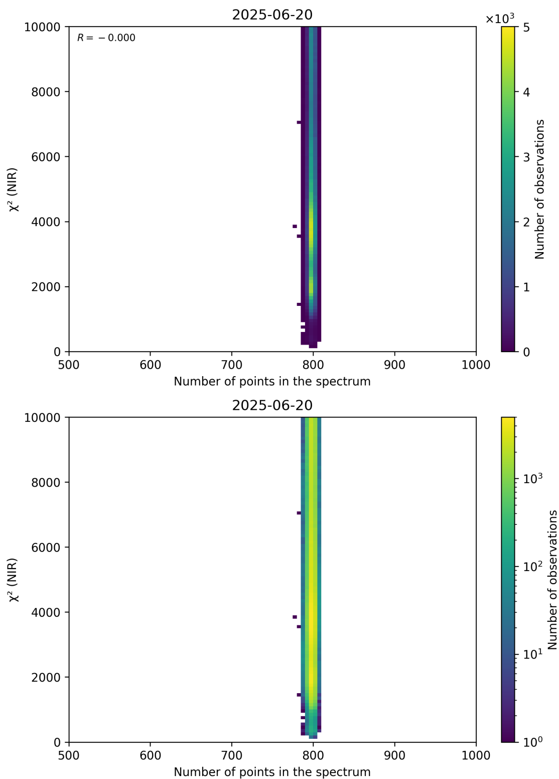
Figure 88: Scatter density plot of “Number of points in the spectrum” against “ \chi^2 (NIR)” for 2025-06-19 to 2025-06-21.
