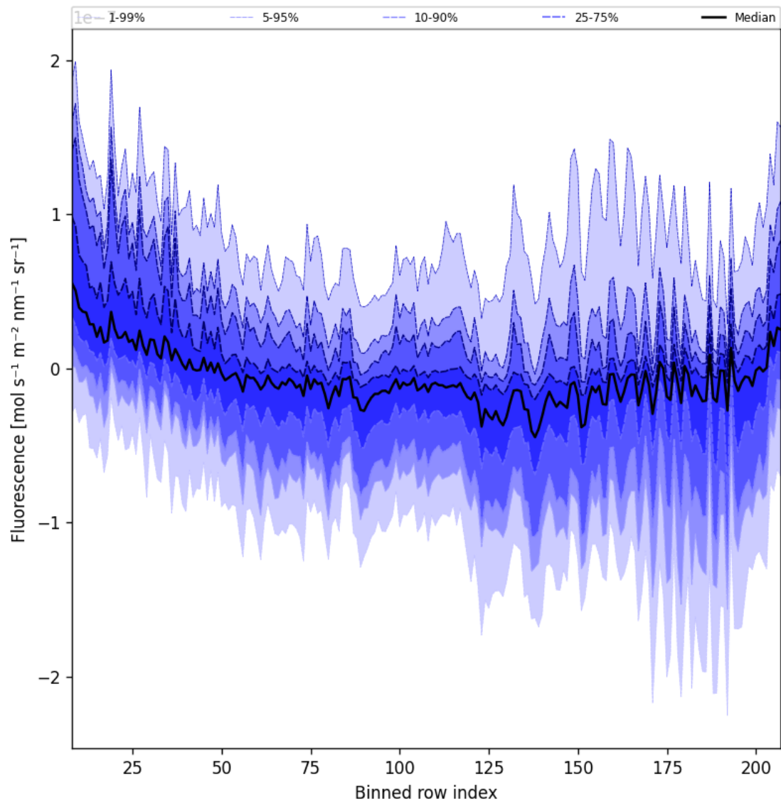
Figure 43: Along track statistics of “Fluorescence” for 2025-06-19 to 2025-06-21
