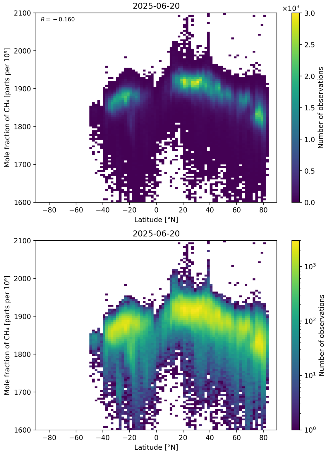
Figure 57: Scatter density plot of “Latitude” against “Mole fraction of \text{CH}_4 ” for 2025-06-19 to 2025-06-21.
