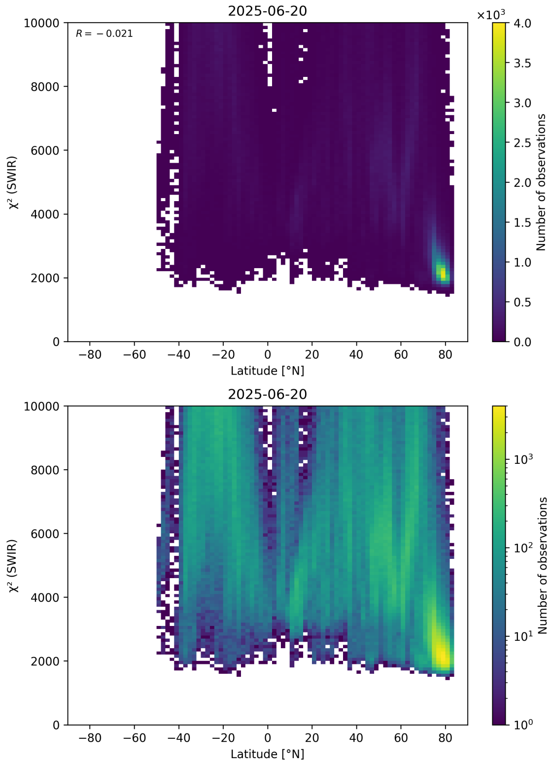
Figure 54: Scatter density plot of “Latitude” against “ \chi^2 (SWIR)” for 2025-06-19 to 2025-06-21.
