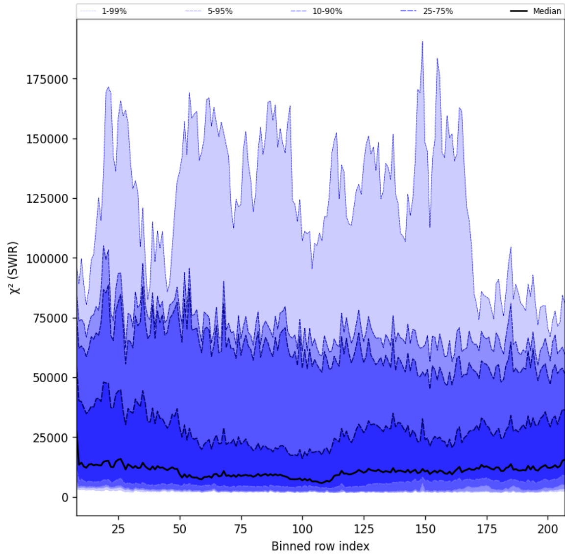
Figure 39: Along track statistics of “ \chi^2 (SWIR)” for 2025-06-19 to 2025-06-21
