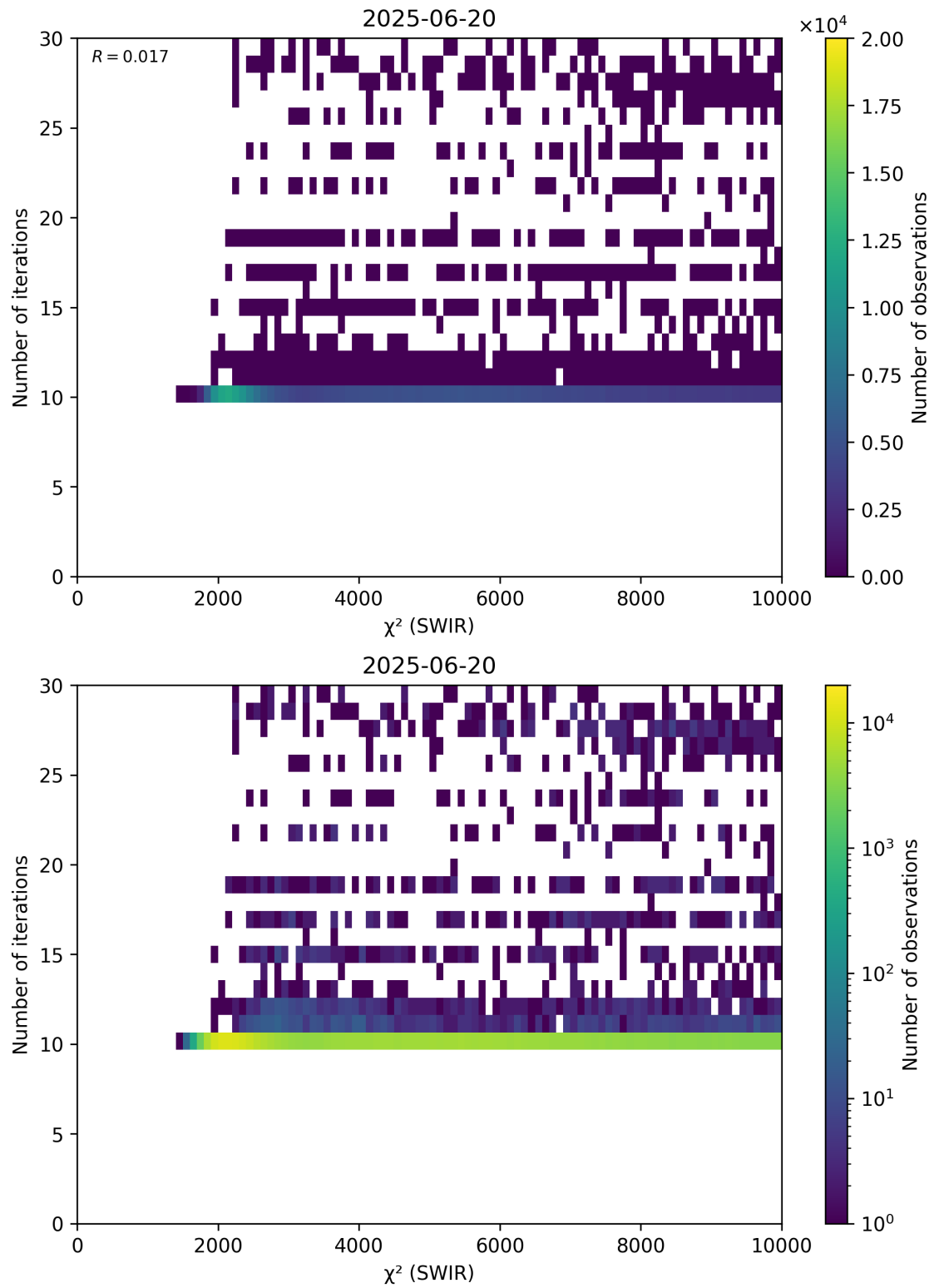
Figure 50: Scatter density plot of “ \chi^2 (SWIR)” against “Number of iterations” for 2025-06-19 to 2025-06-21.
