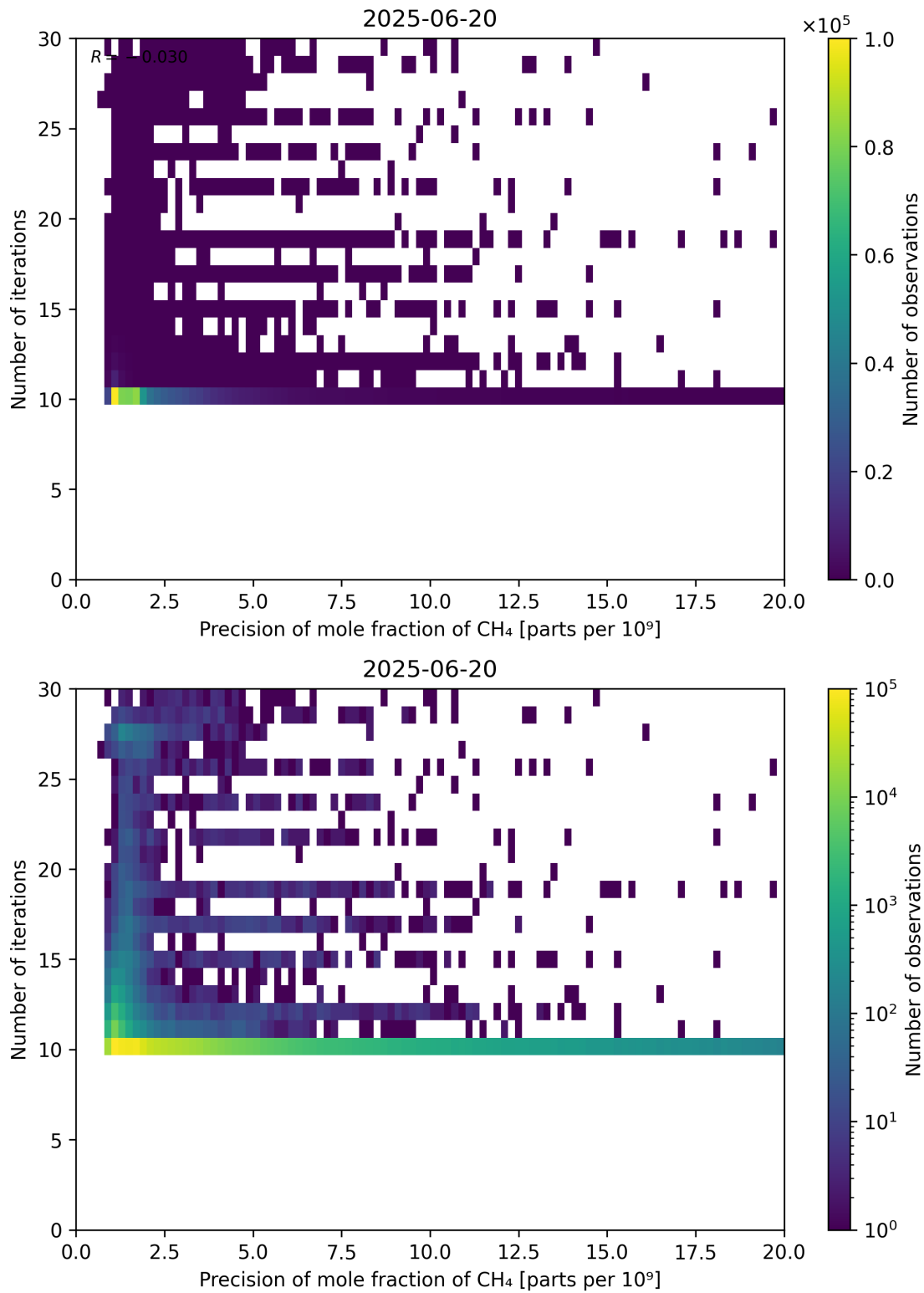
Figure 83: Scatter density plot of “Precision of mole fraction of CH 4 ” against “Number of iterations” for 2025-06-19 to 2025-06-21.
