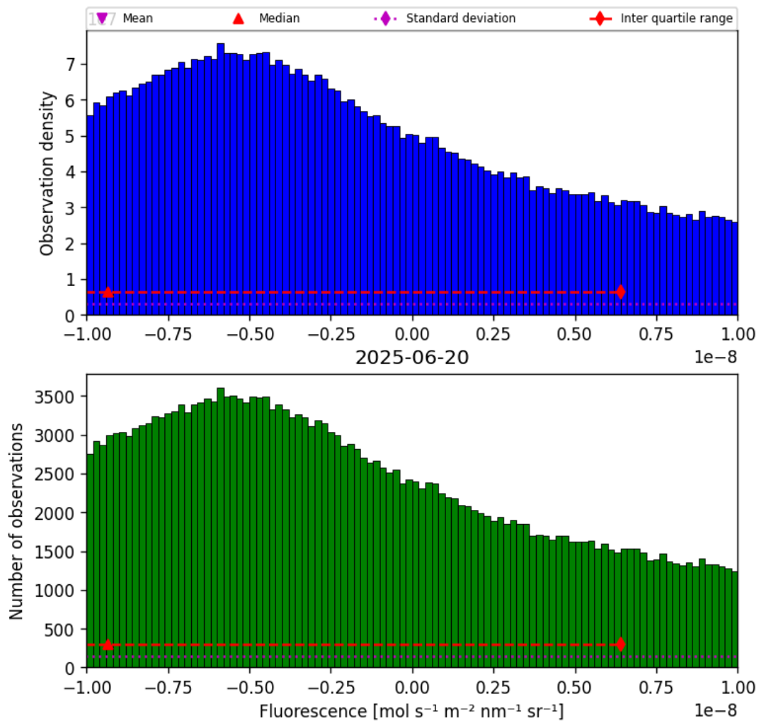
Figure 32: Histogram of “Fluorescence” for 2025-06-19 to 2025-06-21
