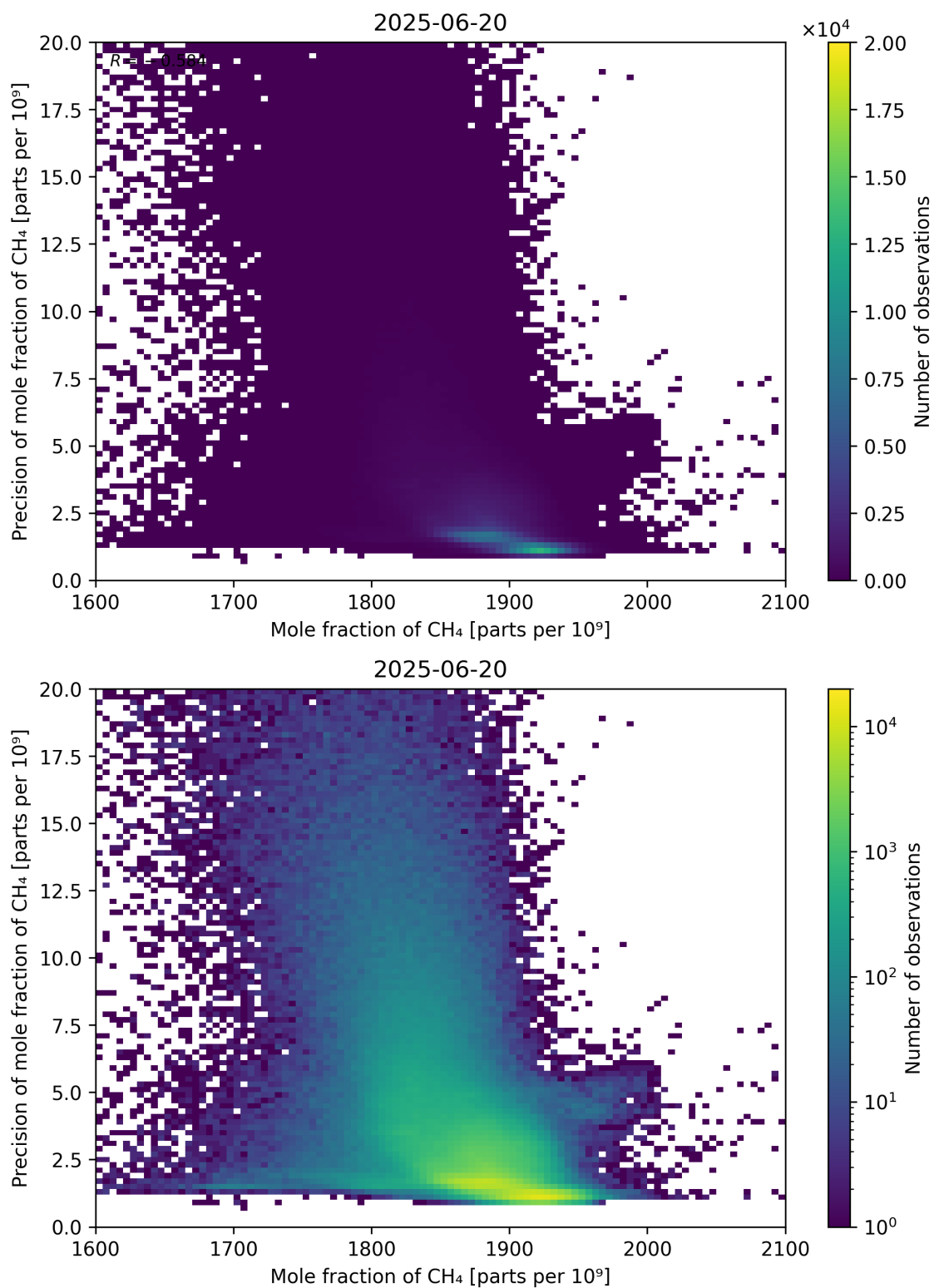
Figure 75: Scatter density plot of “Mole fraction of CH 4 ” against “Precision of mole fraction of CH 4 ” for 2025-06-19 to 2025-06-21.
