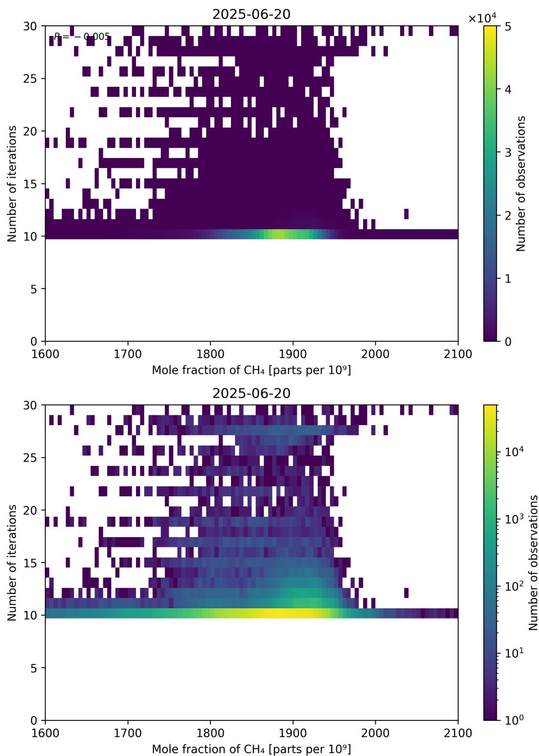
Figure 76: Scatter density plot of “Mole fraction of CH 4 ” against “Number of iterations” for 2025-06-19 to 2025-06-21.
