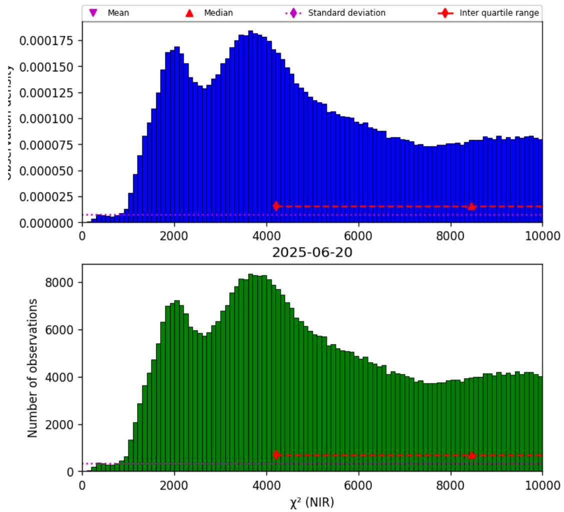
Figure 29: Histogram of “ \chi^2 (NIR)” for 2025-06-19 to 2025-06-21
