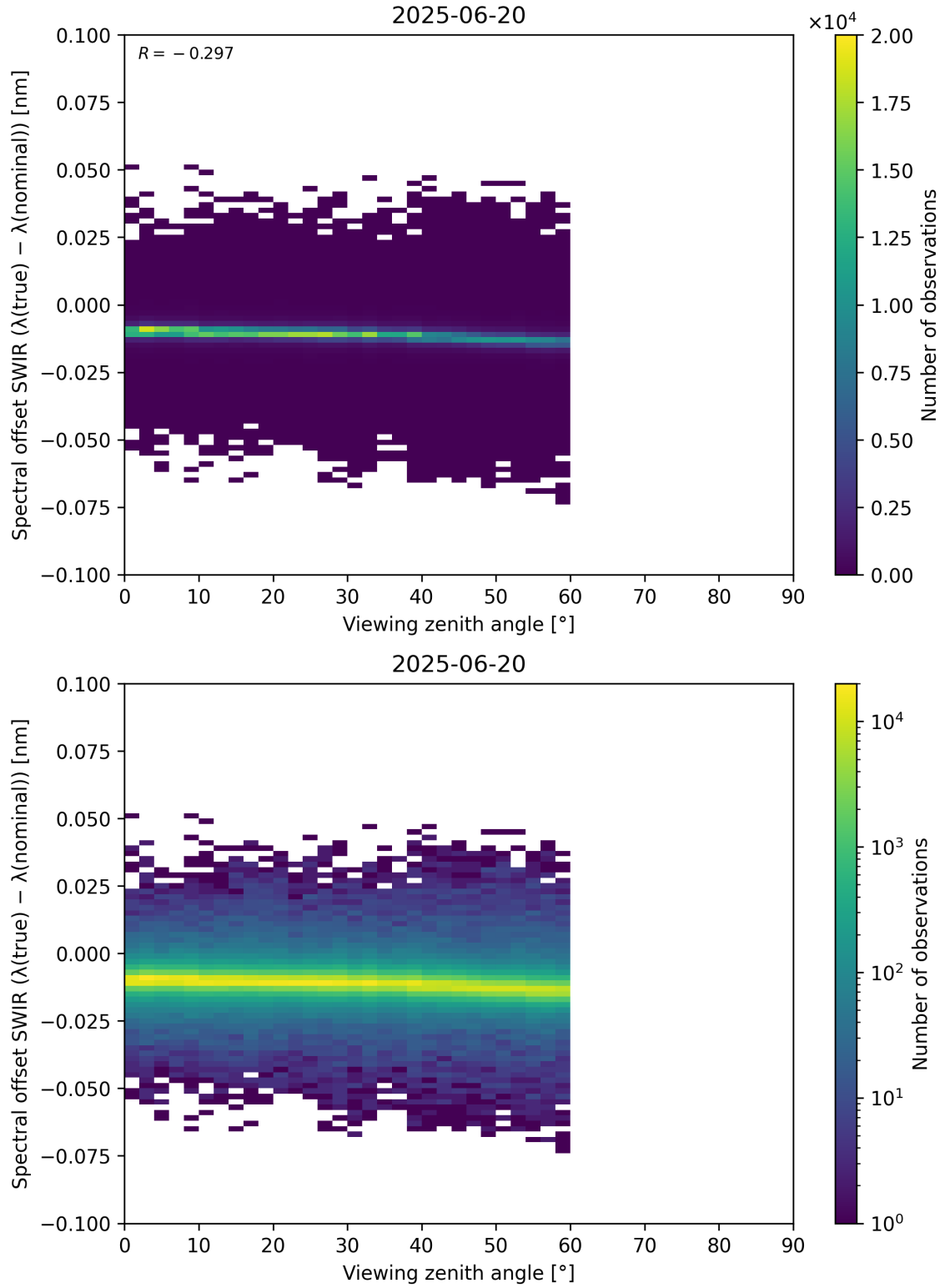
Figure 116: Scatter density plot of “Viewing zenith angle” against “Spectral offset SWIR ( \lambda_{\text{true}} - \lambda_{\text{nominal}} )” for 2025-06-19 to 2025-06-21.
