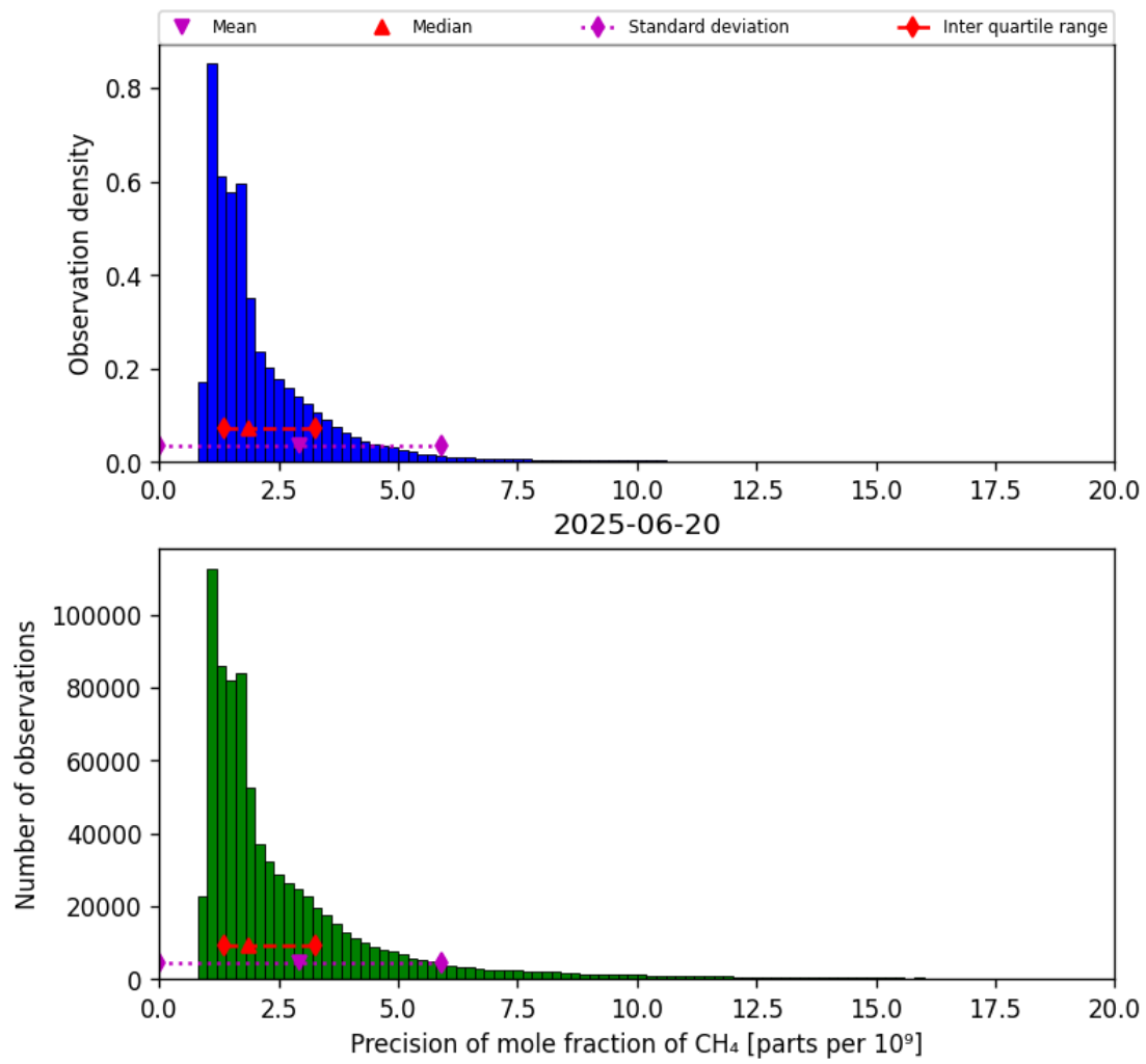
Figure 24: Histogram of “Precision of mole fraction of CH 4 ” for 2025-06-19 to 2025-06-21
