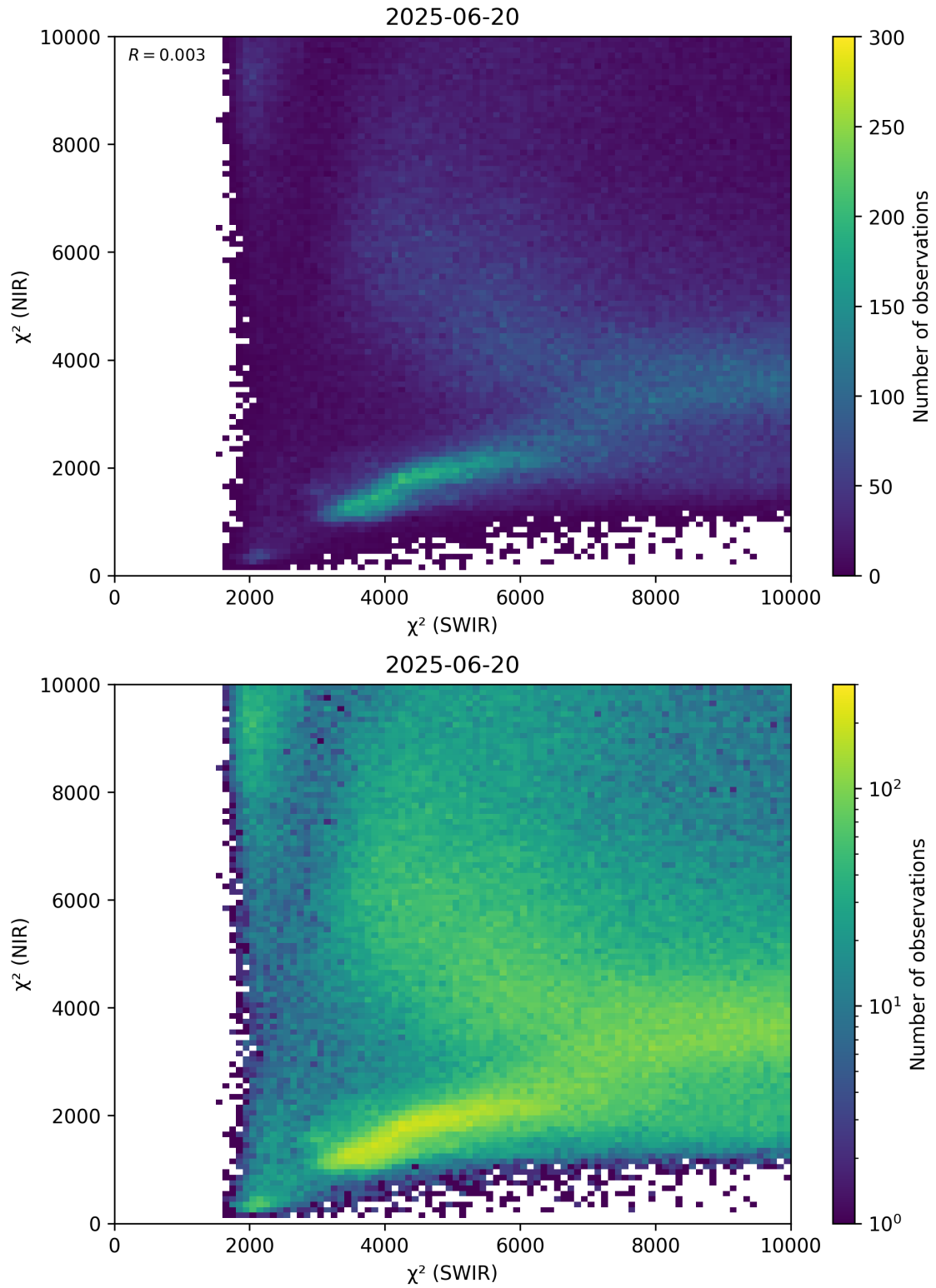
Figure 47: Scatter density plot of “ \chi^2 (SWIR)” against “ \chi^2 (NIR)” for 2025-06-19 to 2025-06-21.
