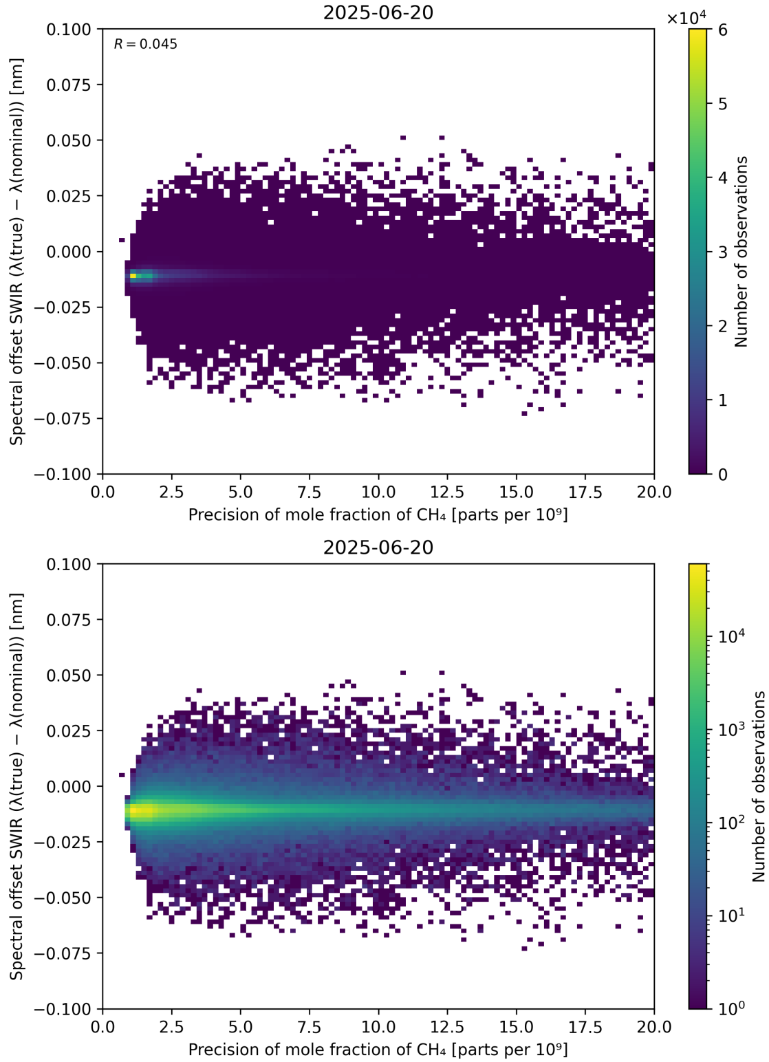
Figure 85: Scatter density plot of “Precision of mole fraction of CH 4 ” against “Spectral offset SWIR ( \lambda_{\text{true}} - \lambda_{\text{nominal}} )” for 2025-06-19 to 2025-06-21.
