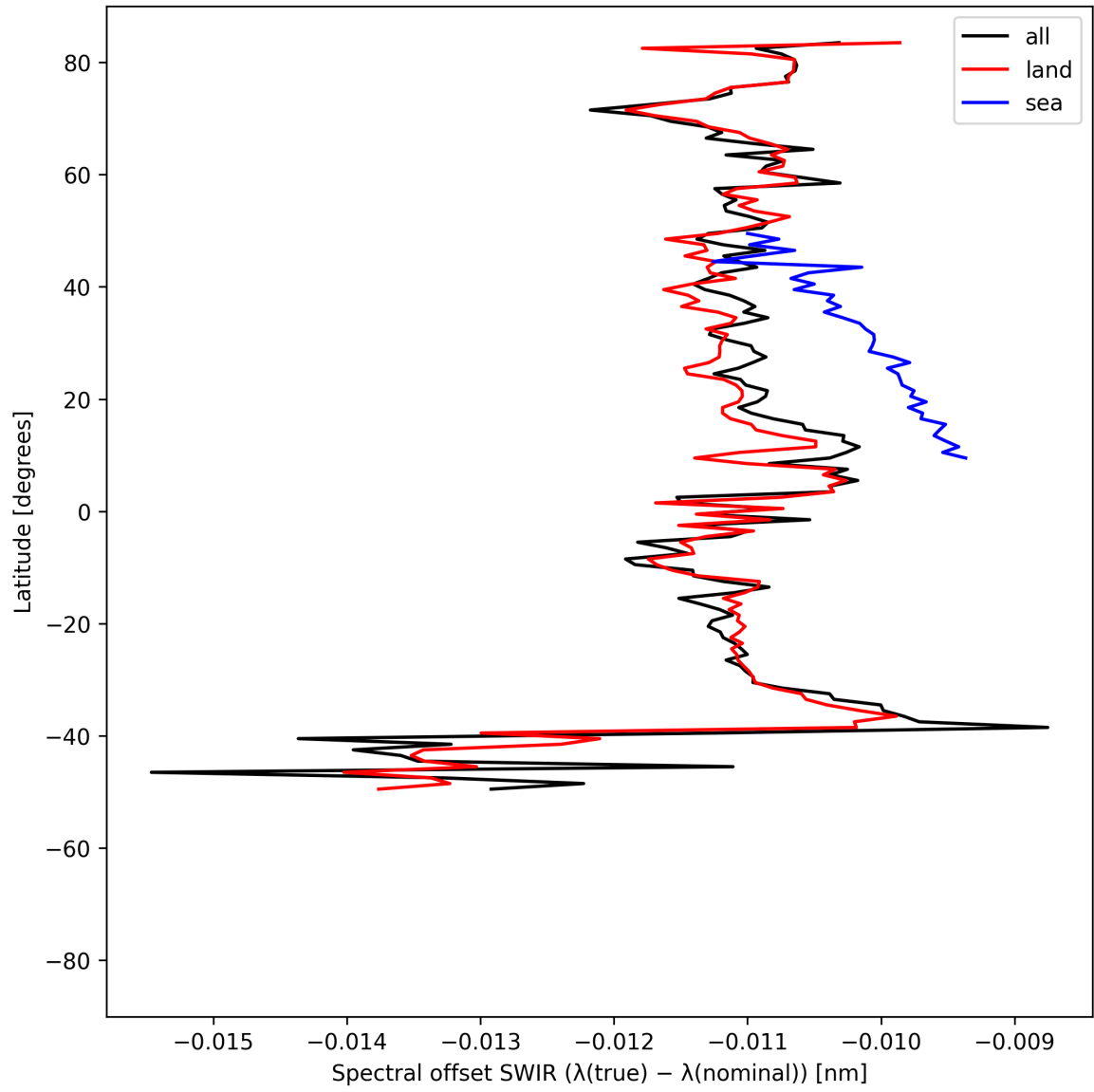
Figure 16: Zonal average of “Spectral offset SWIR ( \lambda_{\text{true}} - \lambda_{\text{nominal}} )” for 2025-06-19 to 2025-06-21.
