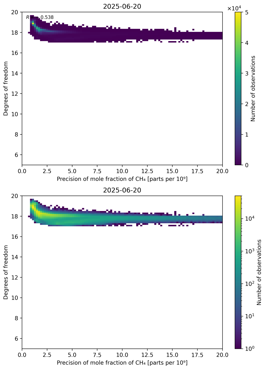
Figure 80: Scatter density plot of “Precision of mole fraction of CH 4 ” against “Degrees of freedom” for 2025-06-19 to 2025-06-21.
