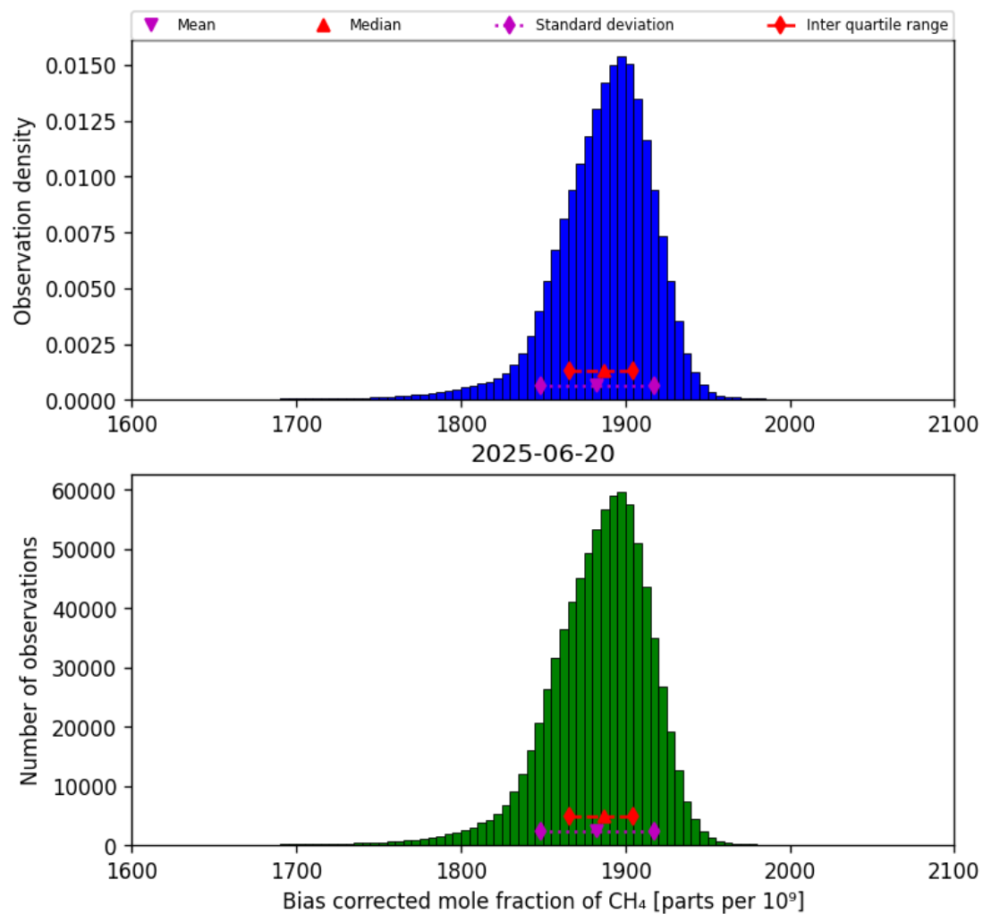
Figure 25: Histogram of “Bias corrected mole fraction of CH 4 ” for 2025-06-19 to 2025-06-21
