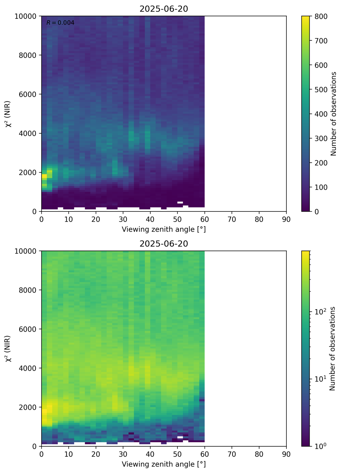
Figure 105: Scatter density plot of “Viewing zenith angle” against “ \chi^2 (NIR)” for 2025-06-19 to 2025-06-21.
