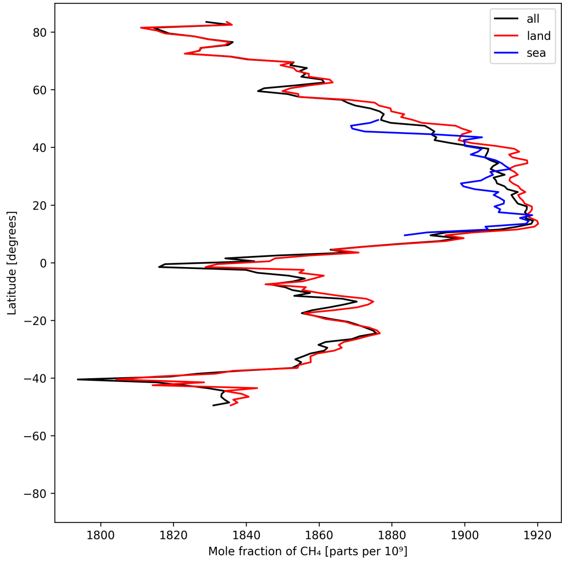
Figure 12: Zonal average of “Mole fraction of \text{CH}_4 ” for 2025-06-19 to 2025-06-21.
