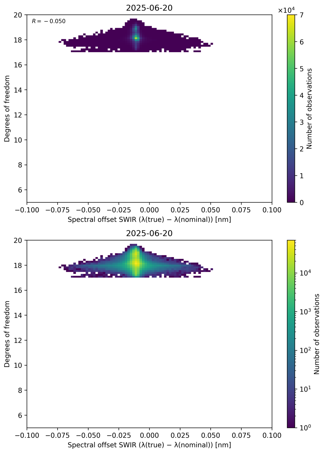
Figure 119: Scatter density plot of “Spectral offset SWIR ( \lambda_{\text{true}} - \lambda_{\text{nominal}} )” against “Degrees of freedom” for 2025-06-19 to 2025-06-21.
