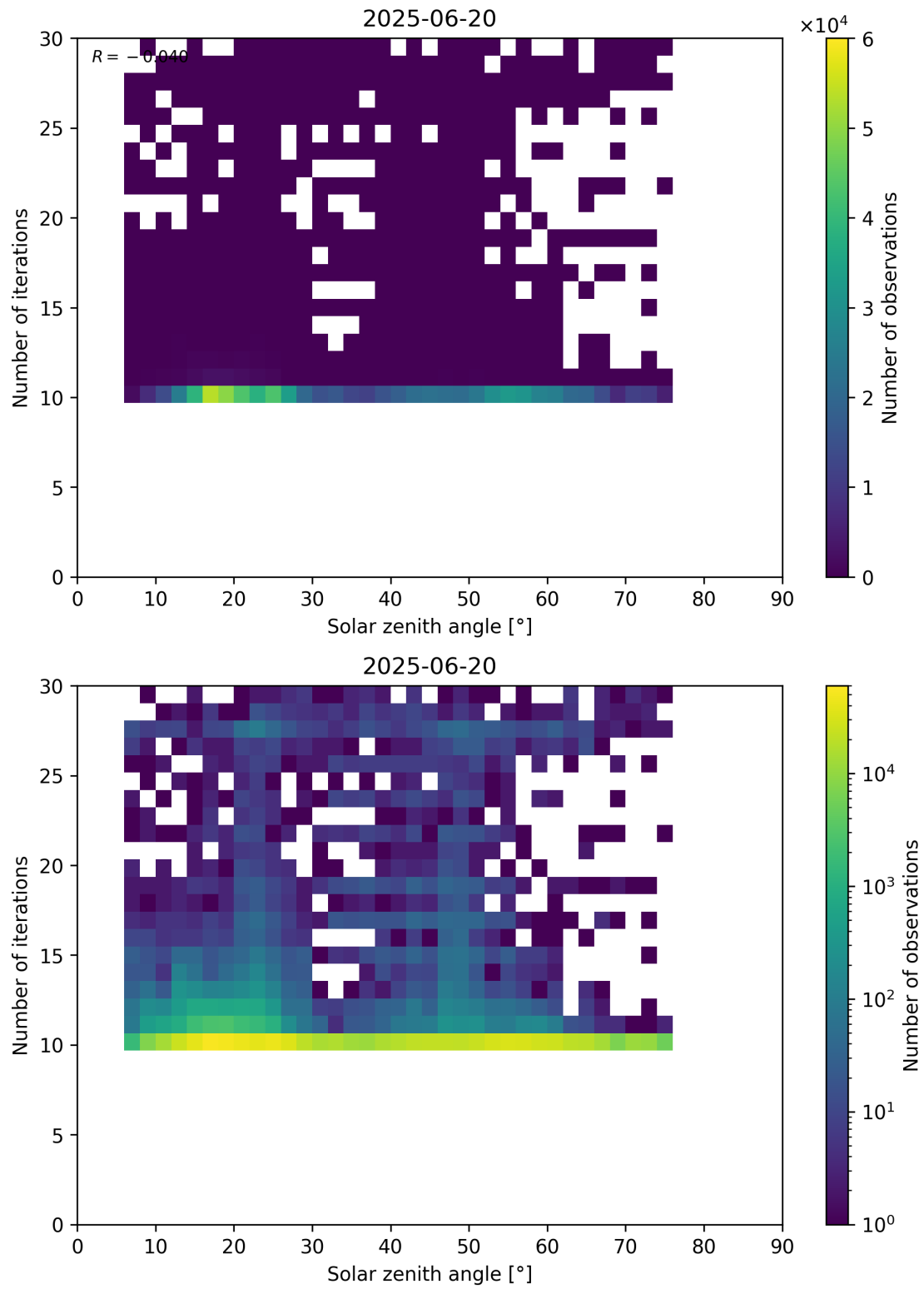
Figure 102: Scatter density plot of “Solar zenith angle” against “Number of iterations” for 2025-06-19 to 2025-06-21.
