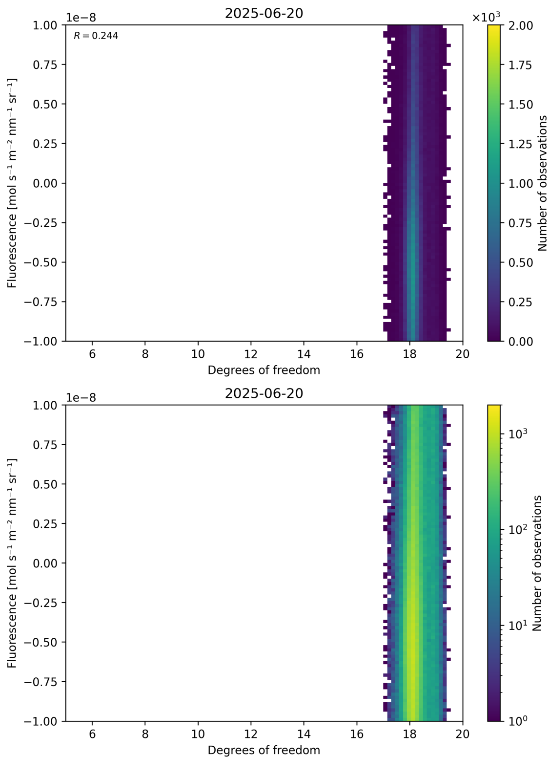
Figure 51: Scatter density plot of “Degrees of freedom” against “Fluorescence” for 2025-06-19 to 2025-06-21.
