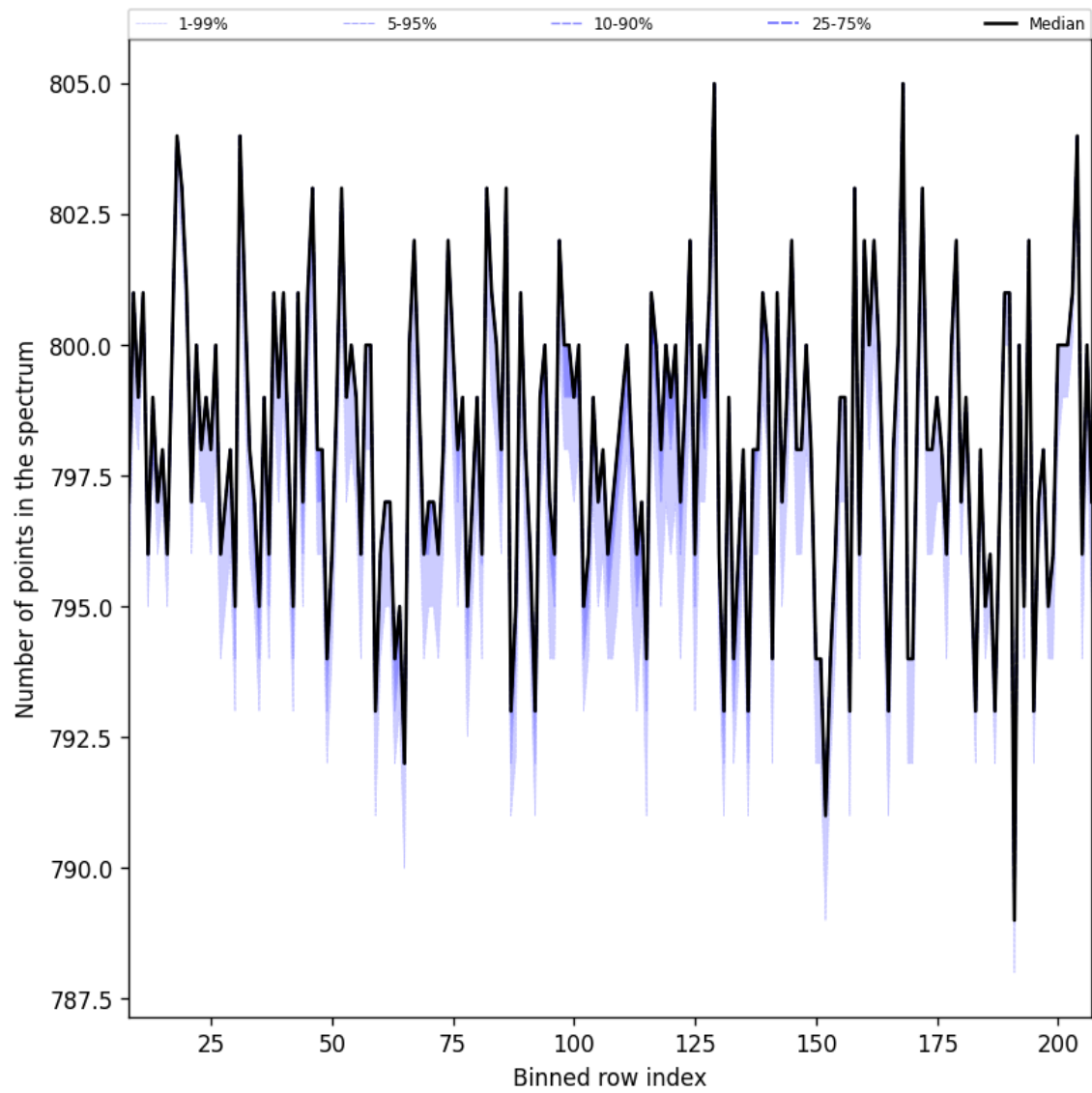
Figure 37: Along track statistics of “Number of points in the spectrum” for 2025-06-19 to 2025-06-21
