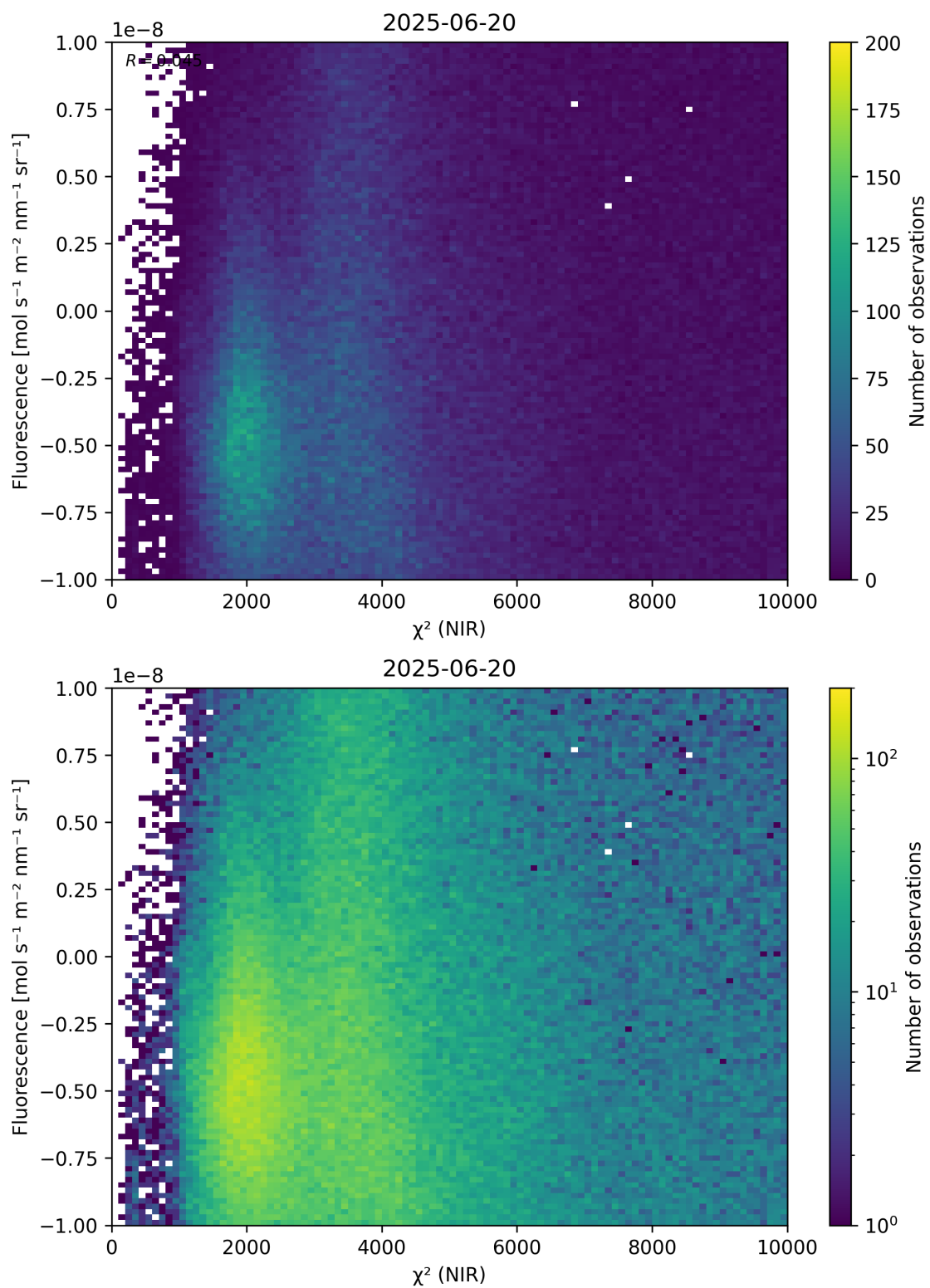
Figure 45: Scatter density plot of “ \chi^2 (NIR)” against “Fluorescence” for 2025-06-19 to 2025-06-21.
