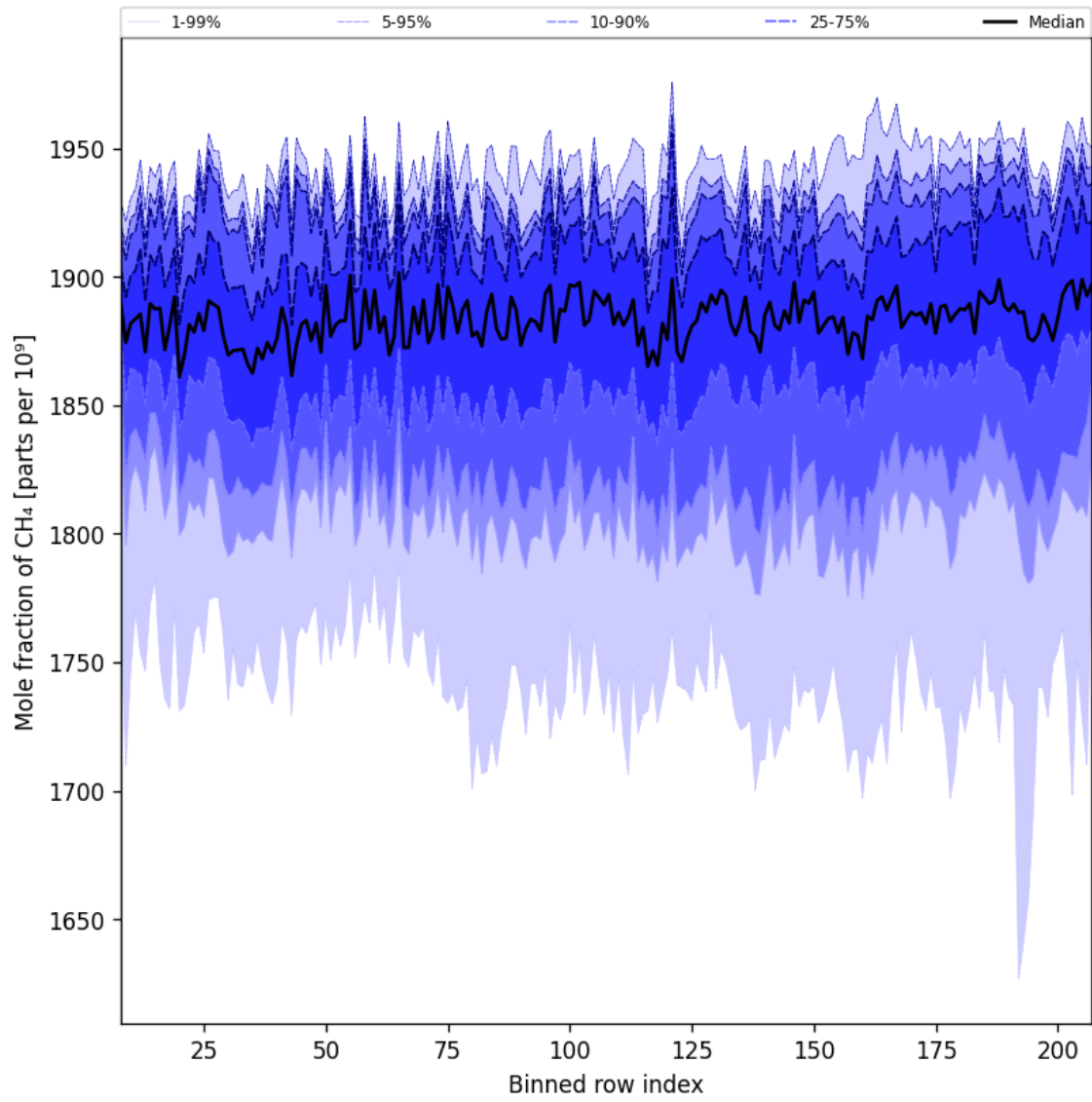
Figure 34: Along track statistics of “Mole fraction of CH 4 ” for 2025-06-19 to 2025-06-21
