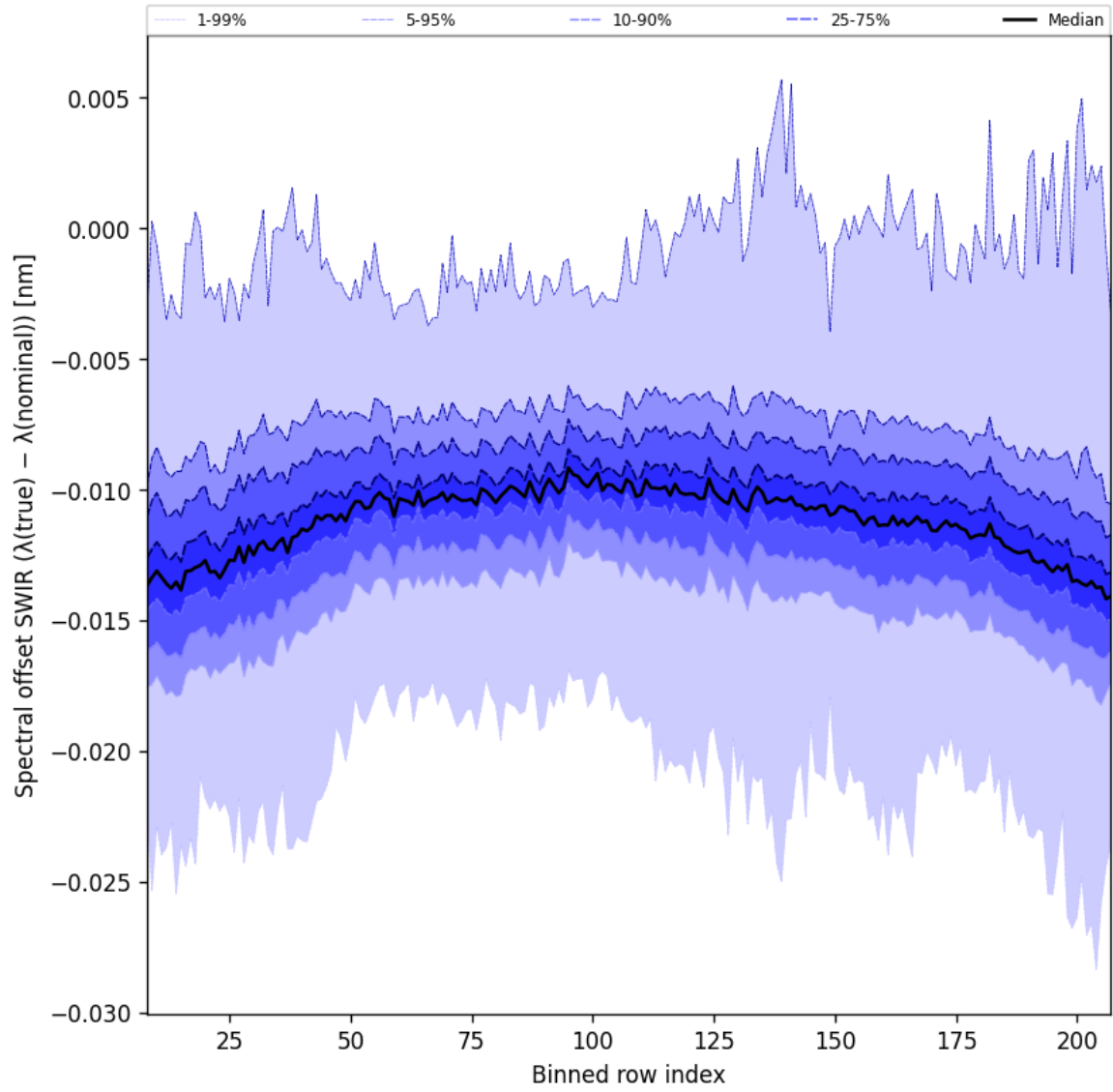
Figure 38: Along track statistics of “Spectral offset SWIR ( \lambda_{\text{true}} - \lambda_{\text{nominal}} )” for 2025-06-19 to 2025-06-21
