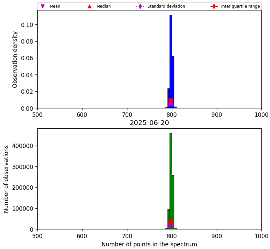
Figure 26: Histogram of “Number of points in the spectrum” for 2025-06-19 to 2025-06-21
