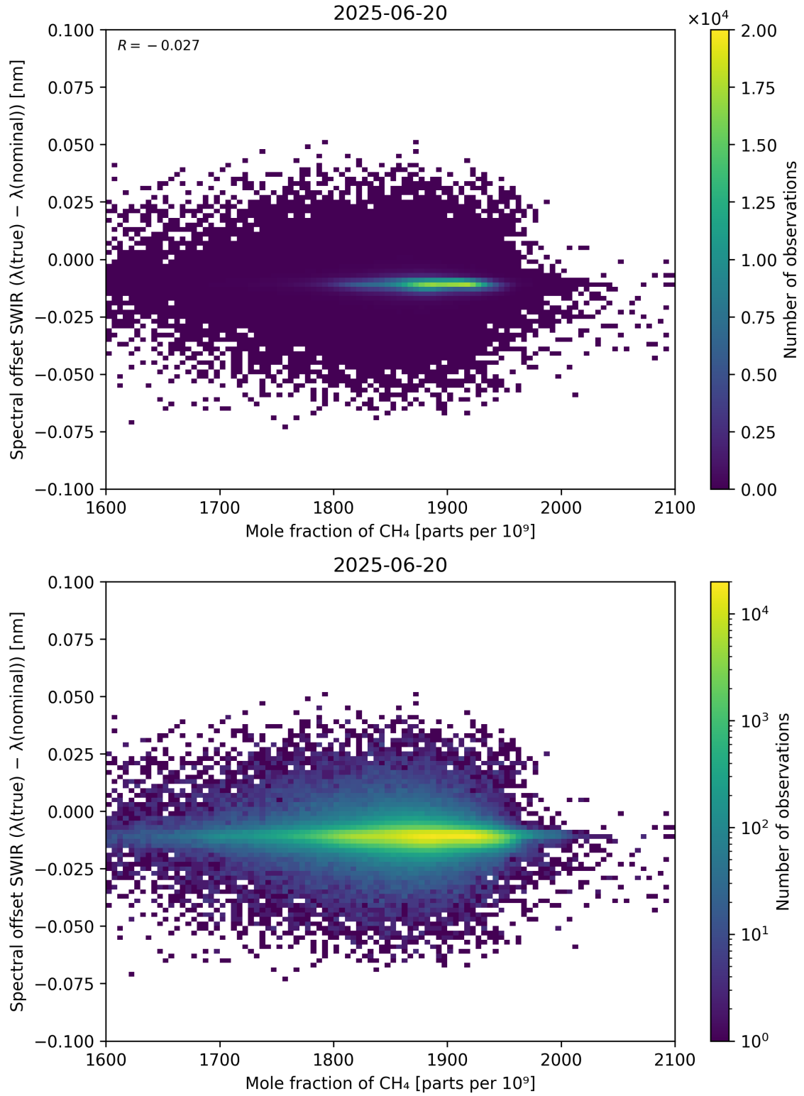
Figure 86: Scatter density plot of “Mole fraction of CH 4 ” against “Spectral offset SWIR ( \lambda_{\text{true}} - \lambda_{\text{nominal}} )” for 2025-06-19 to 2025-06-21.
