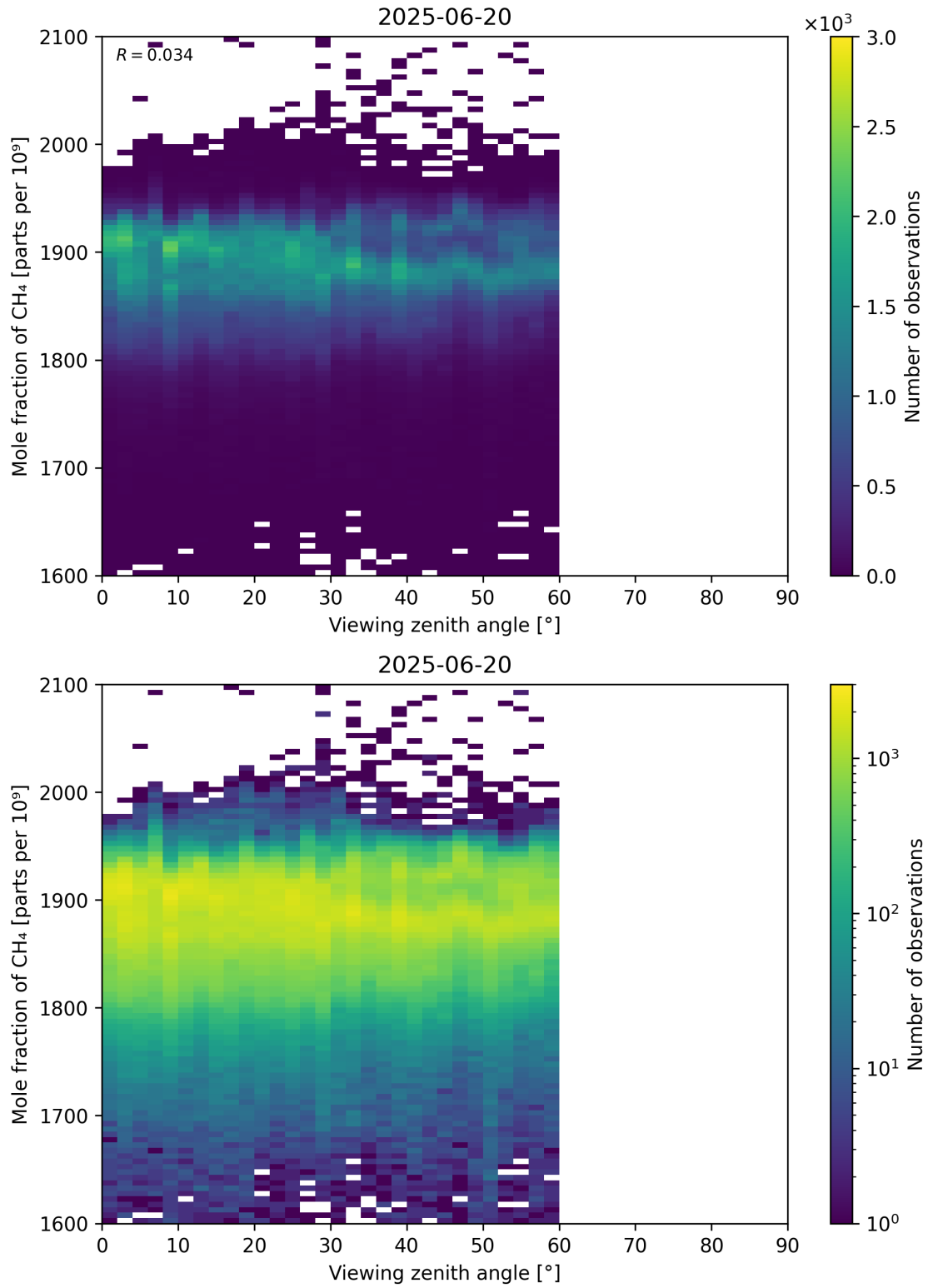
Figure 110: Scatter density plot of “Viewing zenith angle” against “Mole fraction of CH 4 ” for 2025-06-19 to 2025-06-21.
