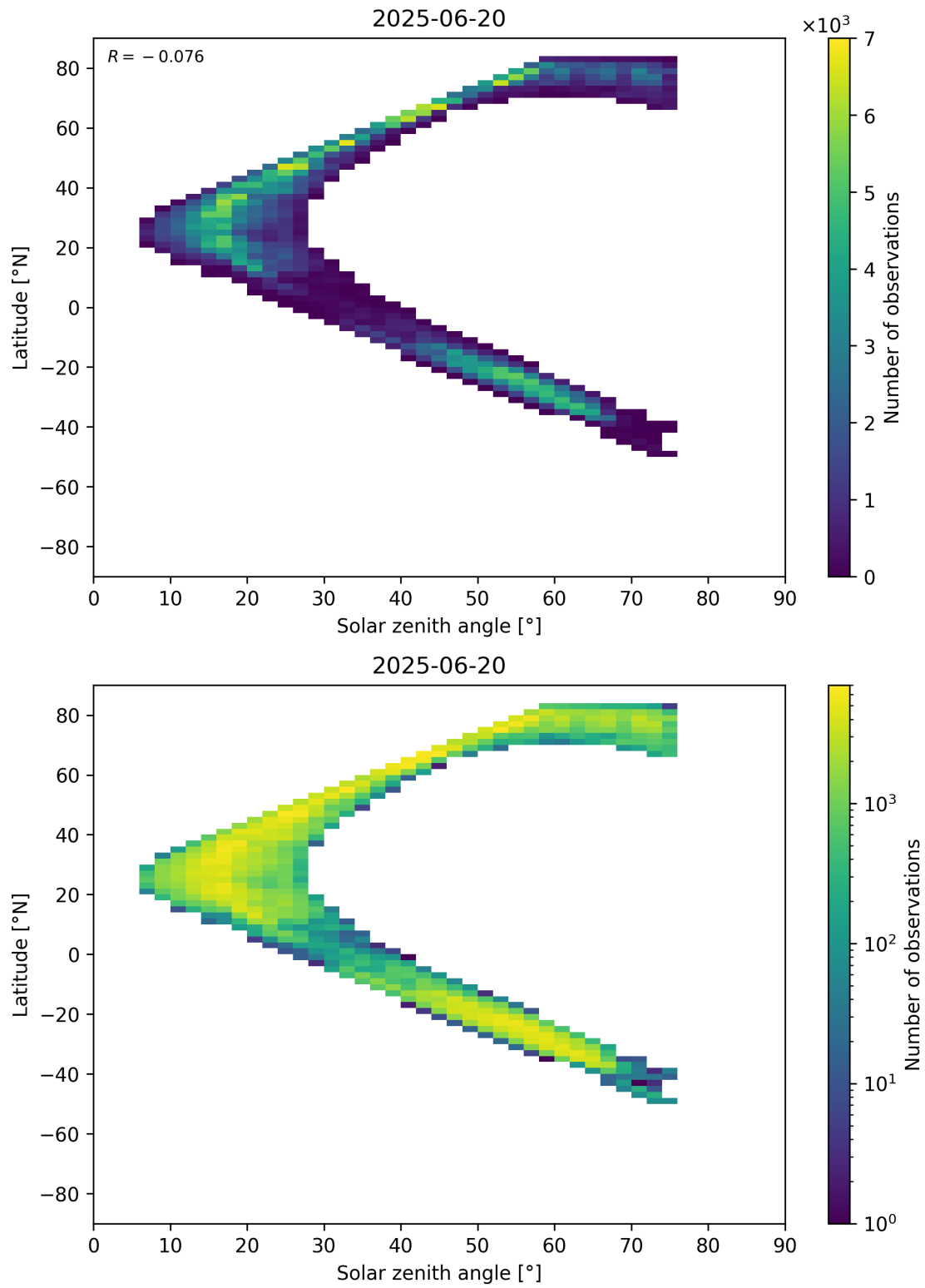
Figure 98: Scatter density plot of “Solar zenith angle” against “Latitude” for 2025-06-19 to 2025-06-21.
