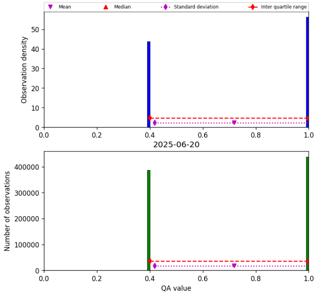
Figure 22: Histogram of “QA value” for 2025-06-19 to 2025-06-21
