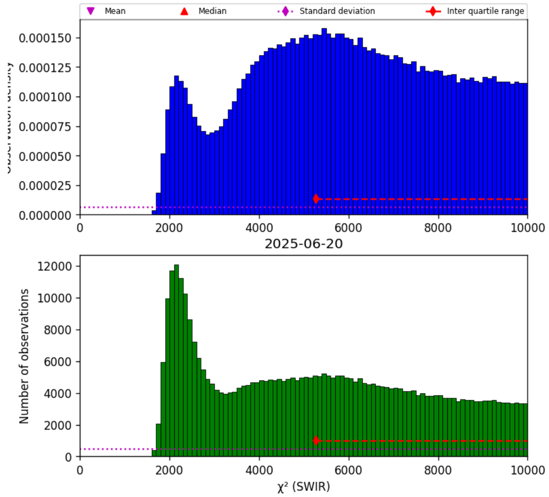
Figure 28: Histogram of “ \chi^2 (SWIR)” for 2025-06-19 to 2025-06-21
