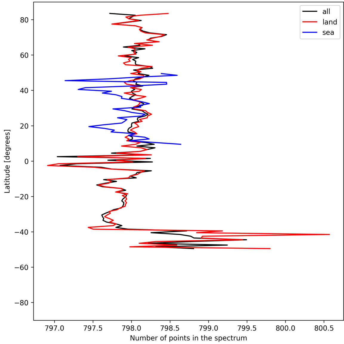
Figure 15: Zonal average of “Number of points in the spectrum” for 2025-06-19 to 2025-06-21.
