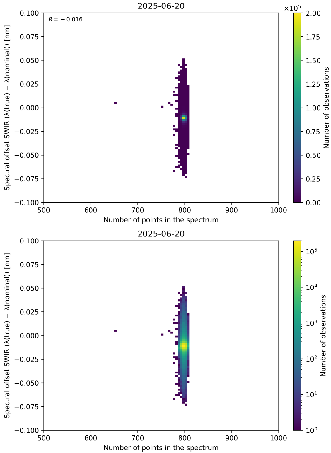
Figure 93: Scatter density plot of “Number of points in the spectrum” against “Spectral offset SWIR ( \lambda_{\text{true}} - \lambda_{\text{nominal}} )” for 2025-06-19 to 2025-06-21.
