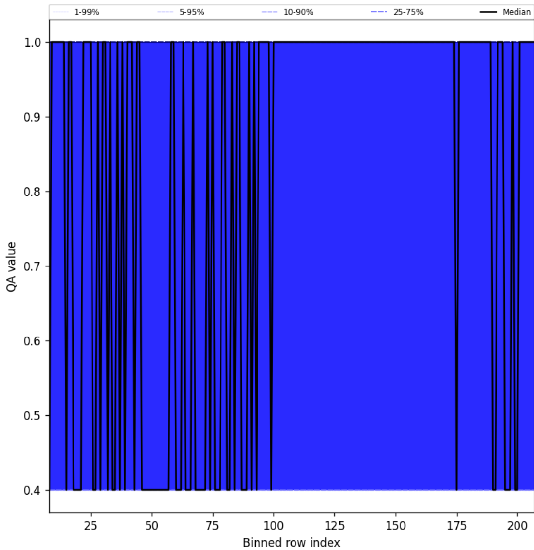
Figure 33: Along track statistics of “QA value” for 2025-06-19 to 2025-06-21
