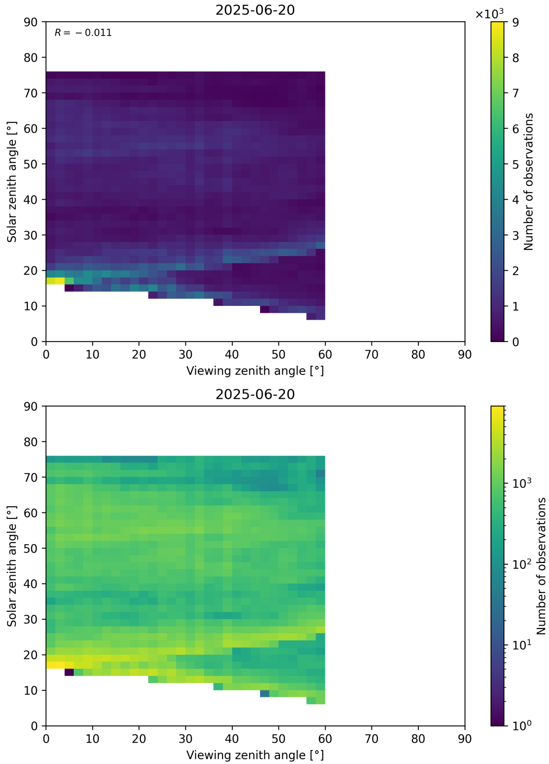
Figure 115: Scatter density plot of “Viewing zenith angle” against “Solar zenith angle” for 2025-06-19 to 2025-06-21.
