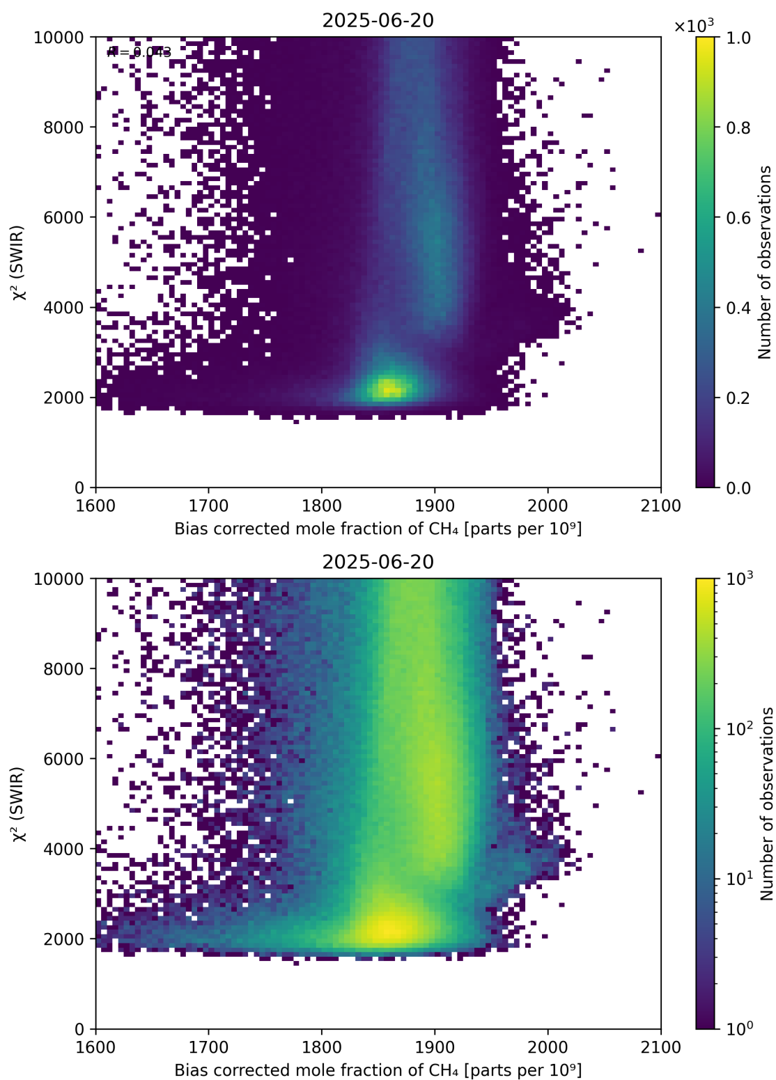
Figure 64: Scatter density plot of “Bias corrected mole fraction of CH 4 ” against “ \chi^2 (SWIR)” for 2025-06-19 to 2025-06-21.
