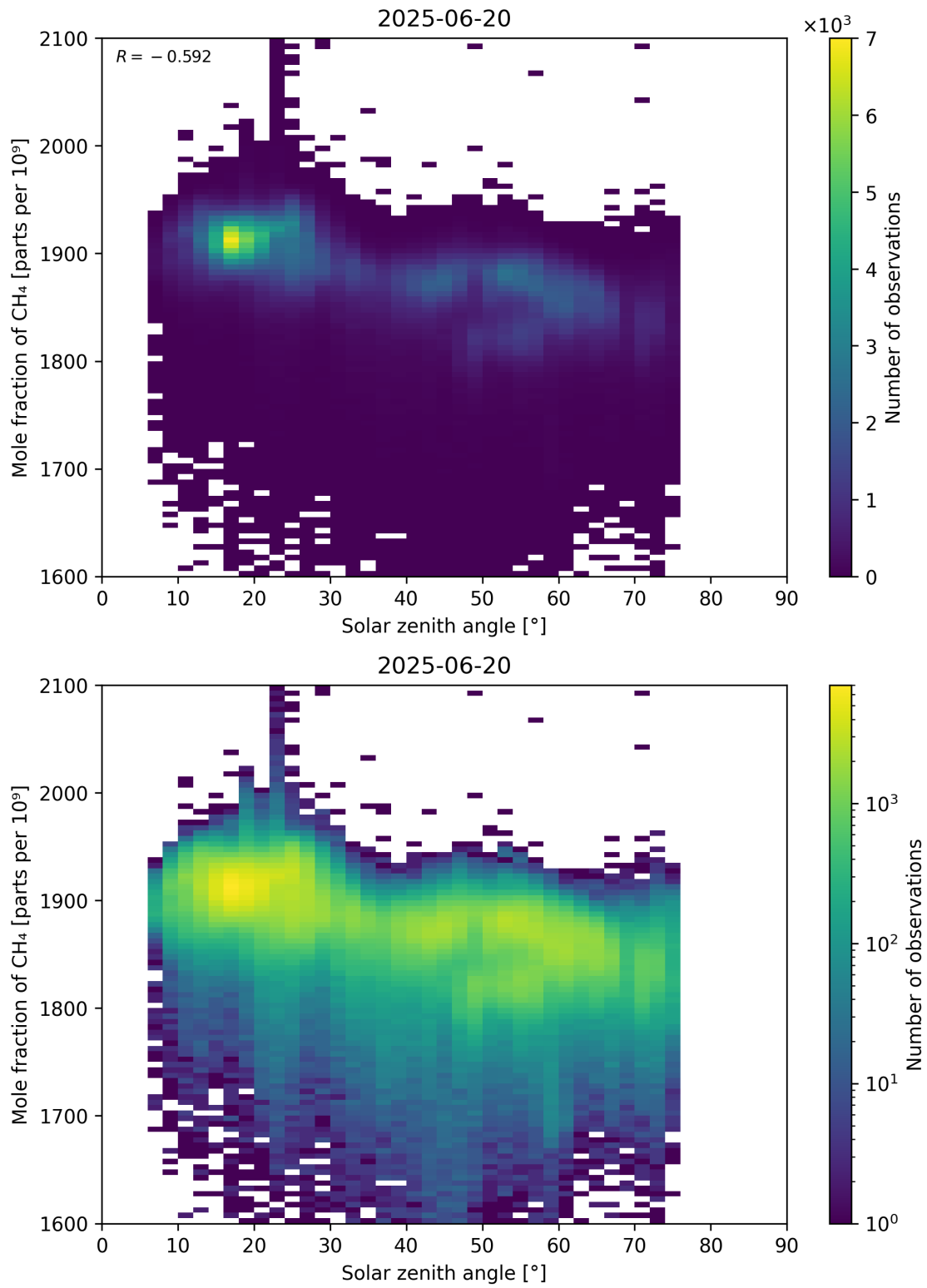
Figure 99: Scatter density plot of “Solar zenith angle” against “Mole fraction of CH 4 ” for 2025-06-19 to 2025-06-21.
