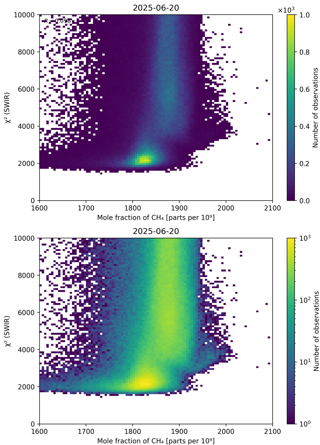
Figure 71: Scatter density plot of “Mole fraction of \text{CH}_4 ” against “ \chi^2 (SWIR)” for 2025-06-19 to 2025-06-21.
