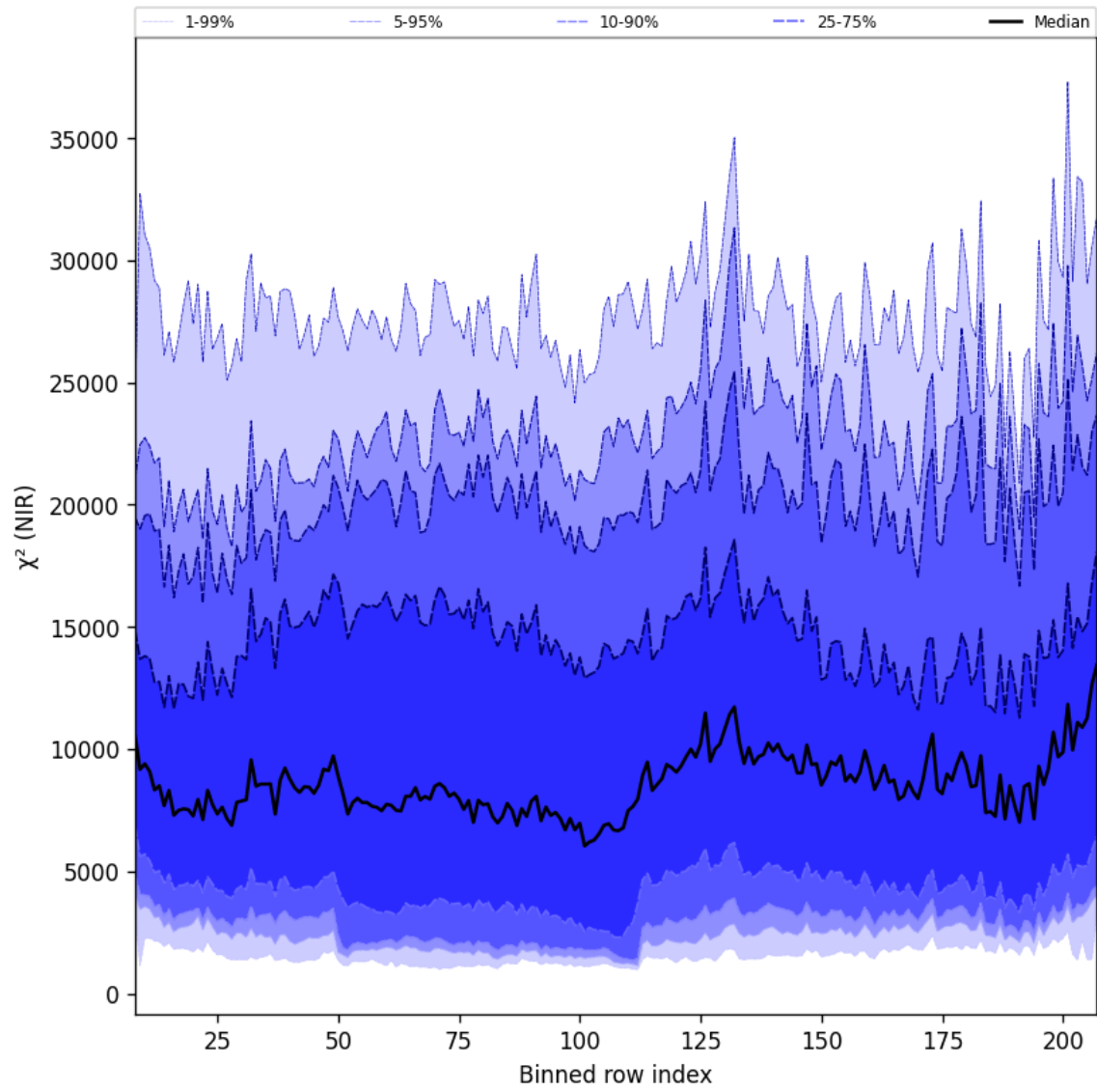
Figure 40: Along track statistics of “ \chi^2 (NIR)” for 2025-06-19 to 2025-06-21
