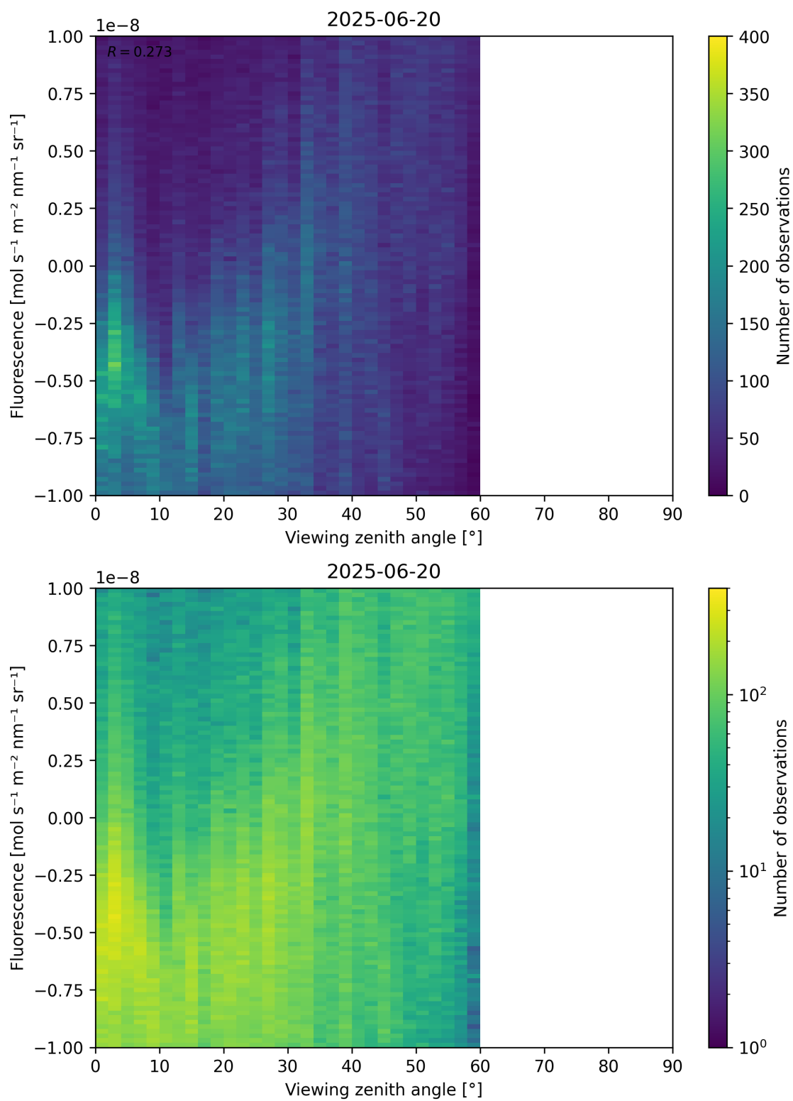
Figure 108: Scatter density plot of “Viewing zenith angle” against “Fluorescence” for 2025-06-19 to 2025-06-21.
