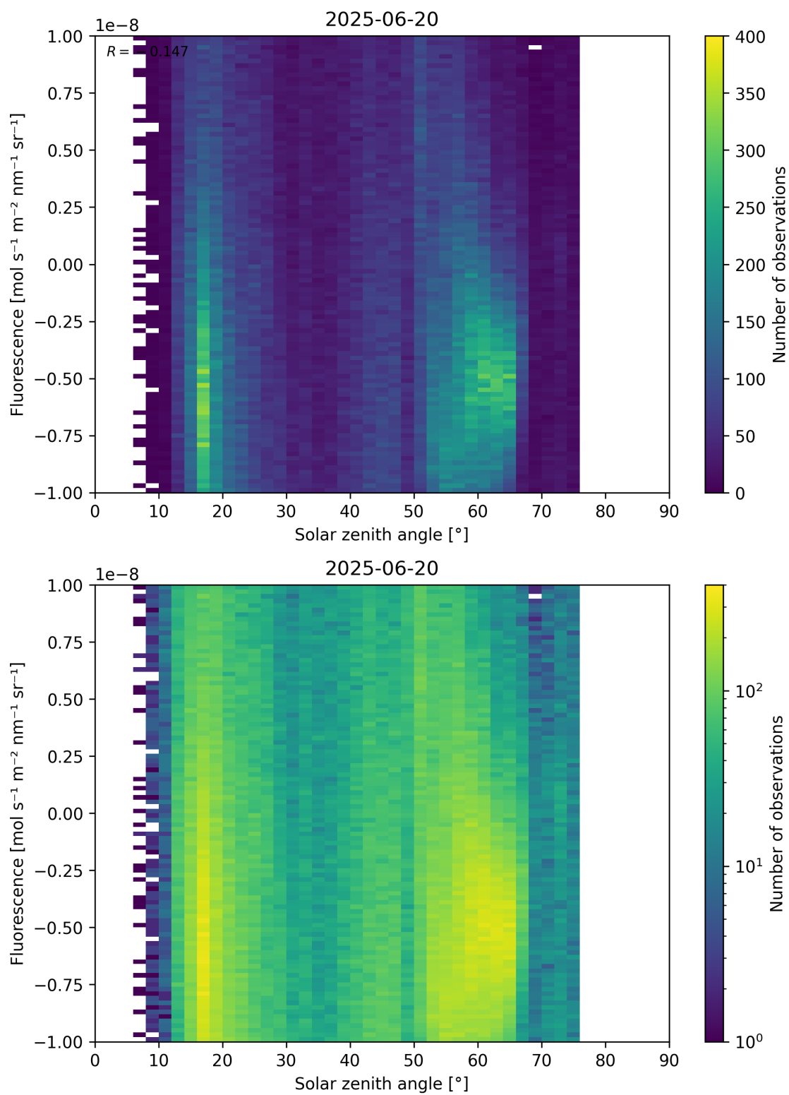
Figure 97: Scatter density plot of “Solar zenith angle” against “Fluorescence” for 2025-06-19 to 2025-06-21.
