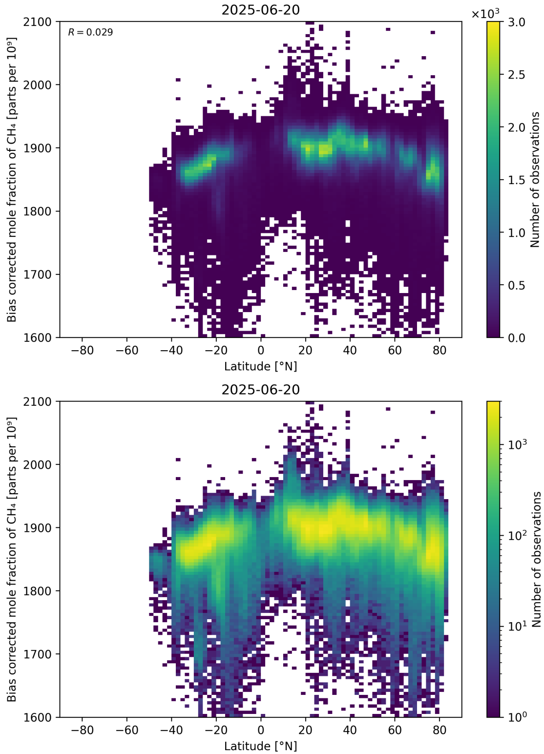
Figure 58: Scatter density plot of “Latitude” against “Bias corrected mole fraction of \text{CH}_4 ” for 2025-06-19 to 2025-06-21.
