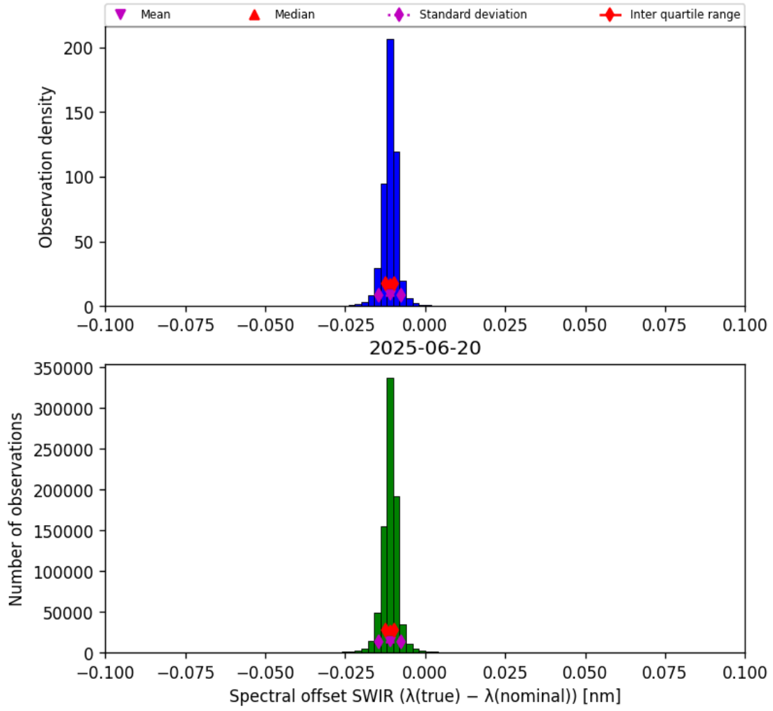
Figure 27: Histogram of “Spectral offset SWIR ( \lambda_{\text{true}} - \lambda_{\text{nominal}} )” for 2025-06-19 to 2025-06-21
