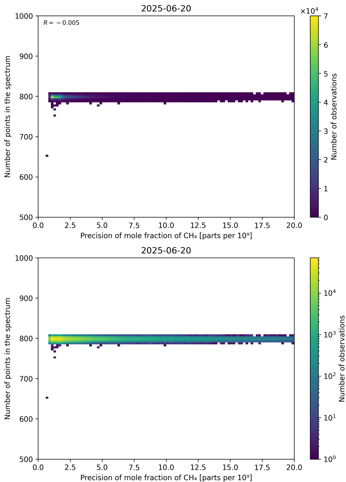
Figure 84: Scatter density plot of “Precision of mole fraction of CH 4 ” against “Number of points in the spectrum” for 2025-06-19 to 2025-06-21.
