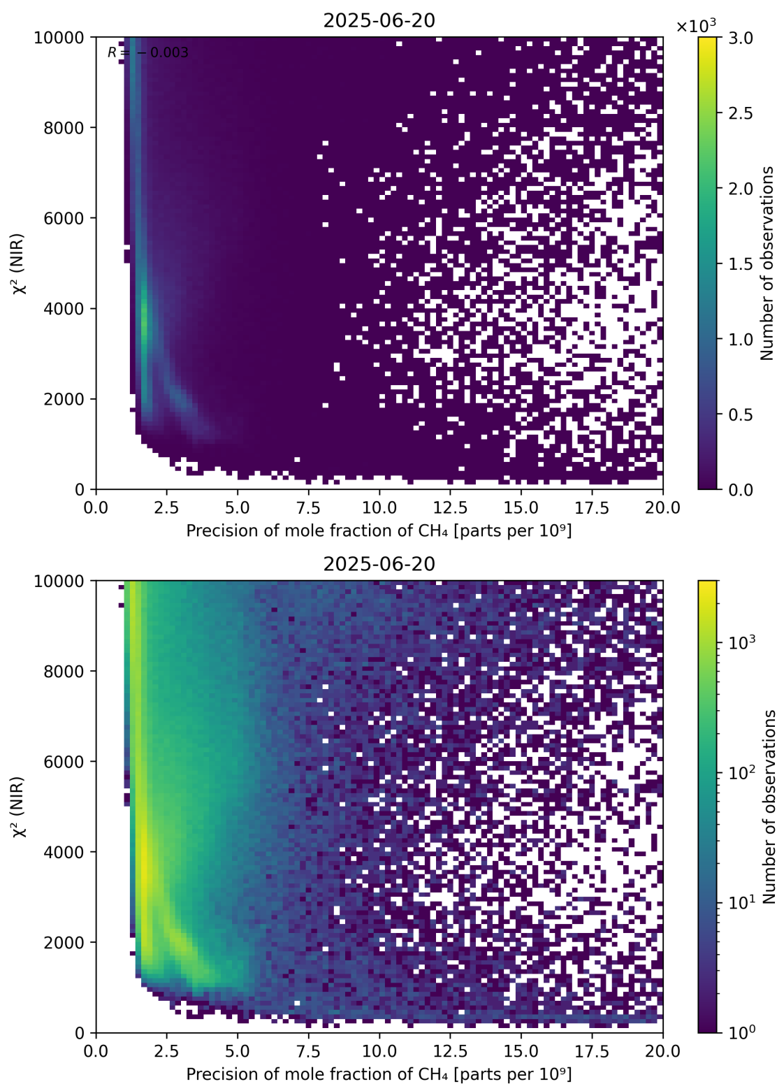
Figure 78: Scatter density plot of “Precision of mole fraction of CH 4 ” against “ \chi^2 (NIR)” for 2025-06-19 to 2025-06-21.
