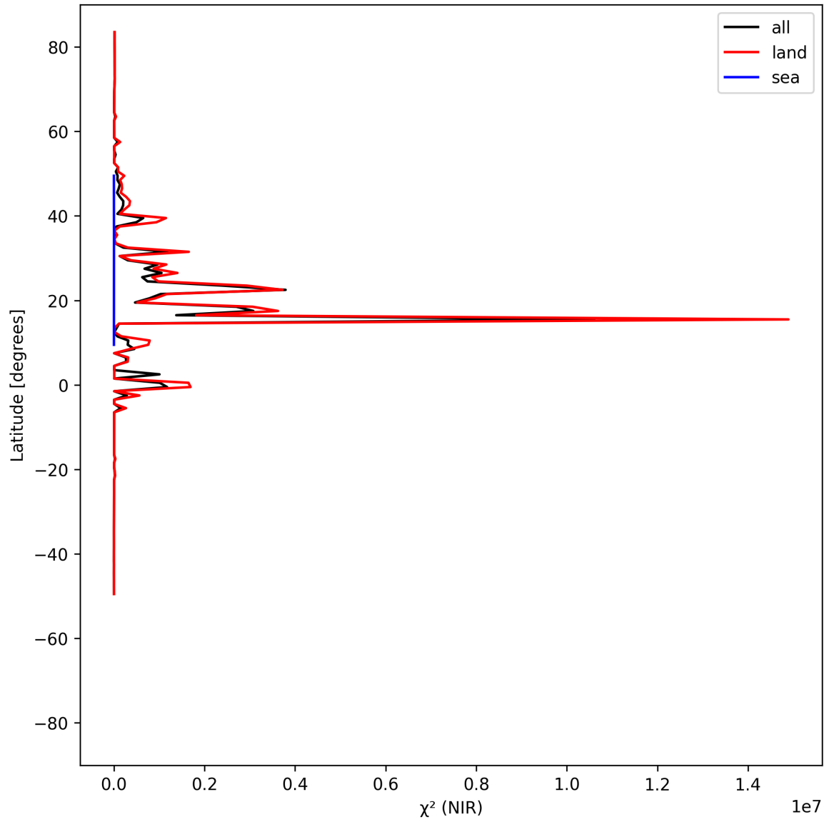
Figure 18: Zonal average of “ \chi^2 (NIR)” for 2025-06-19 to 2025-06-21.
