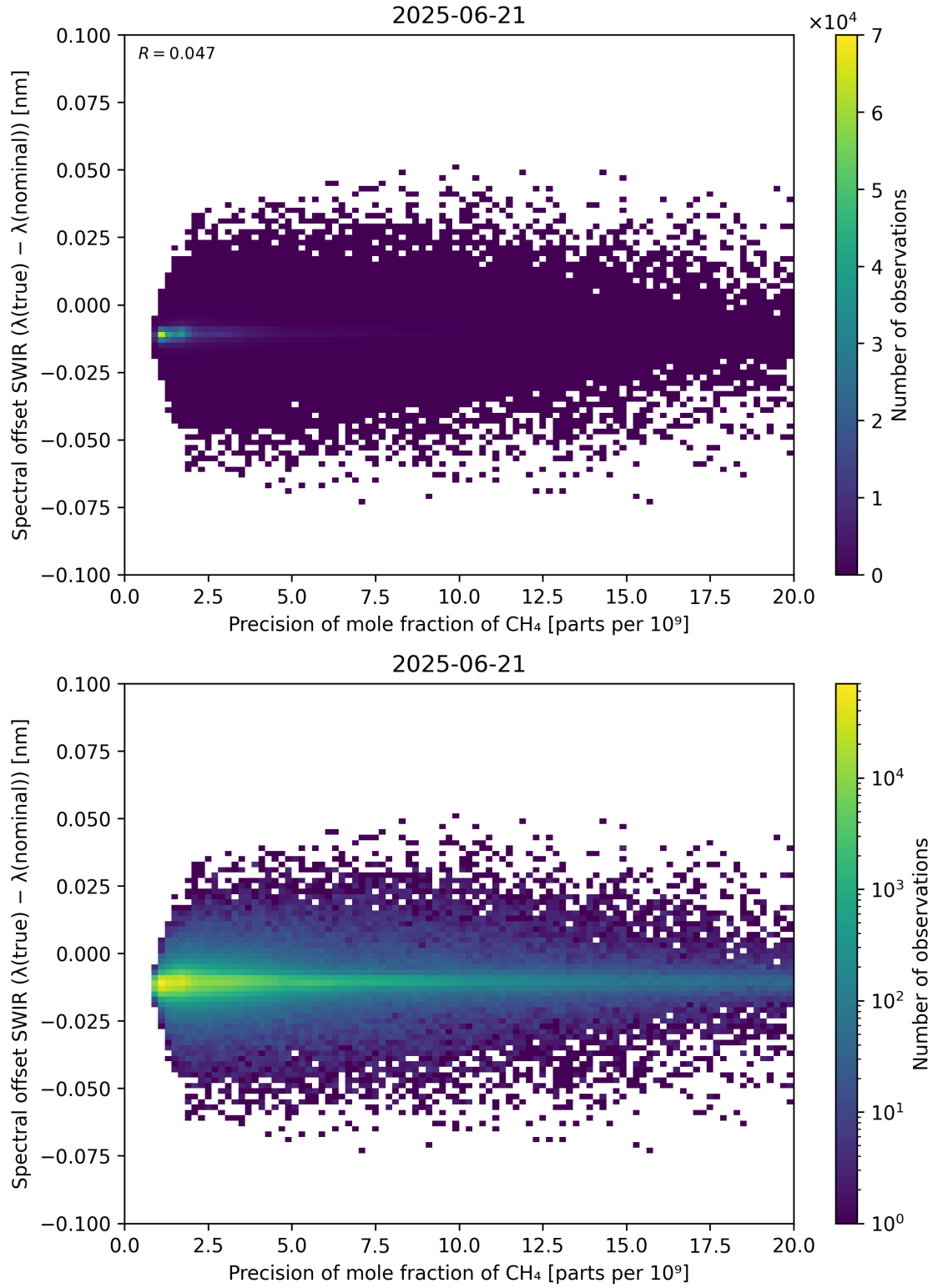
Figure 85: Scatter density plot of “Precision of mole fraction of CH 4 ” against “Spectral offset SWIR ( \lambda_{\text{true}} - \lambda_{\text{nominal}} )” for 2025-06-20 to 2025-06-22.
