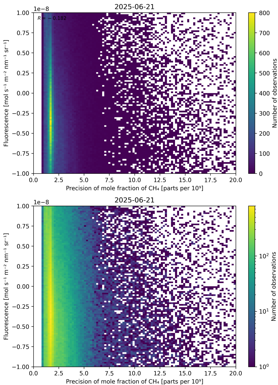
Figure 81: Scatter density plot of “Precision of mole fraction of \text{CH}_4 ” against “Fluorescence” for 2025-06-20 to 2025-06-22.
