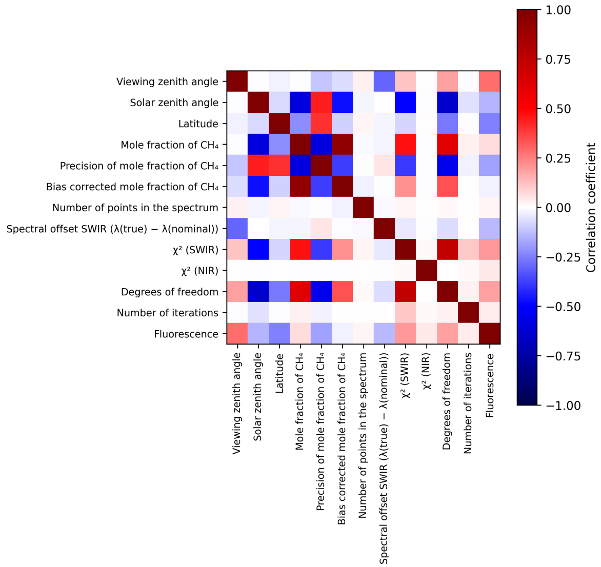
Figure 2: Map of correlation matrix for 2025-06-20 to 2025-06-22.
