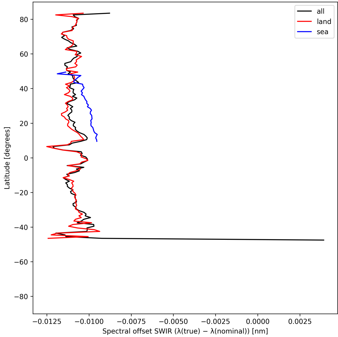
Figure 16: Zonal average of “Spectral offset SWIR ( \lambda_{\text{true}} - \lambda_{\text{nominal}} )” for 2025-06-20 to 2025-06-22.
