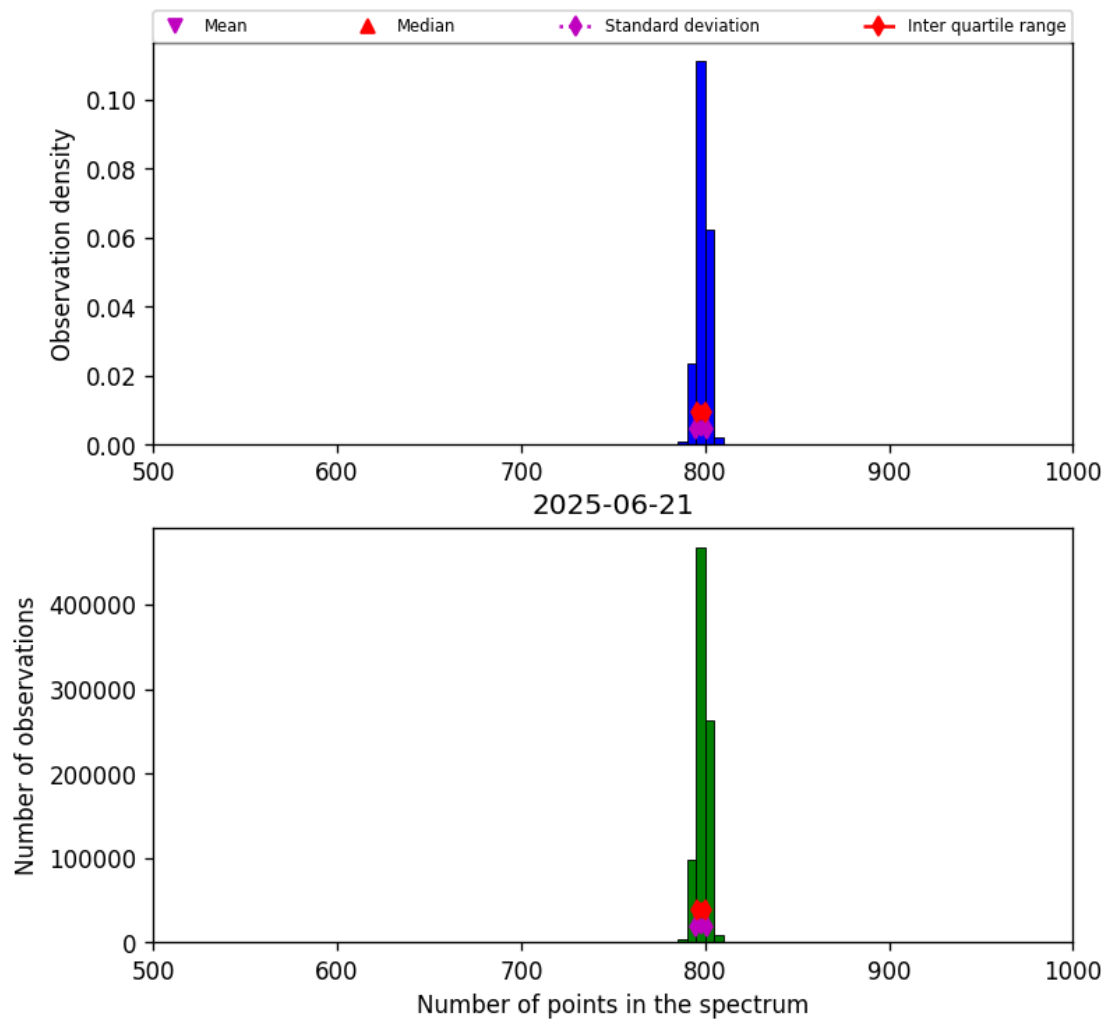
Figure 26: Histogram of “Number of points in the spectrum” for 2025-06-20 to 2025-06-22
