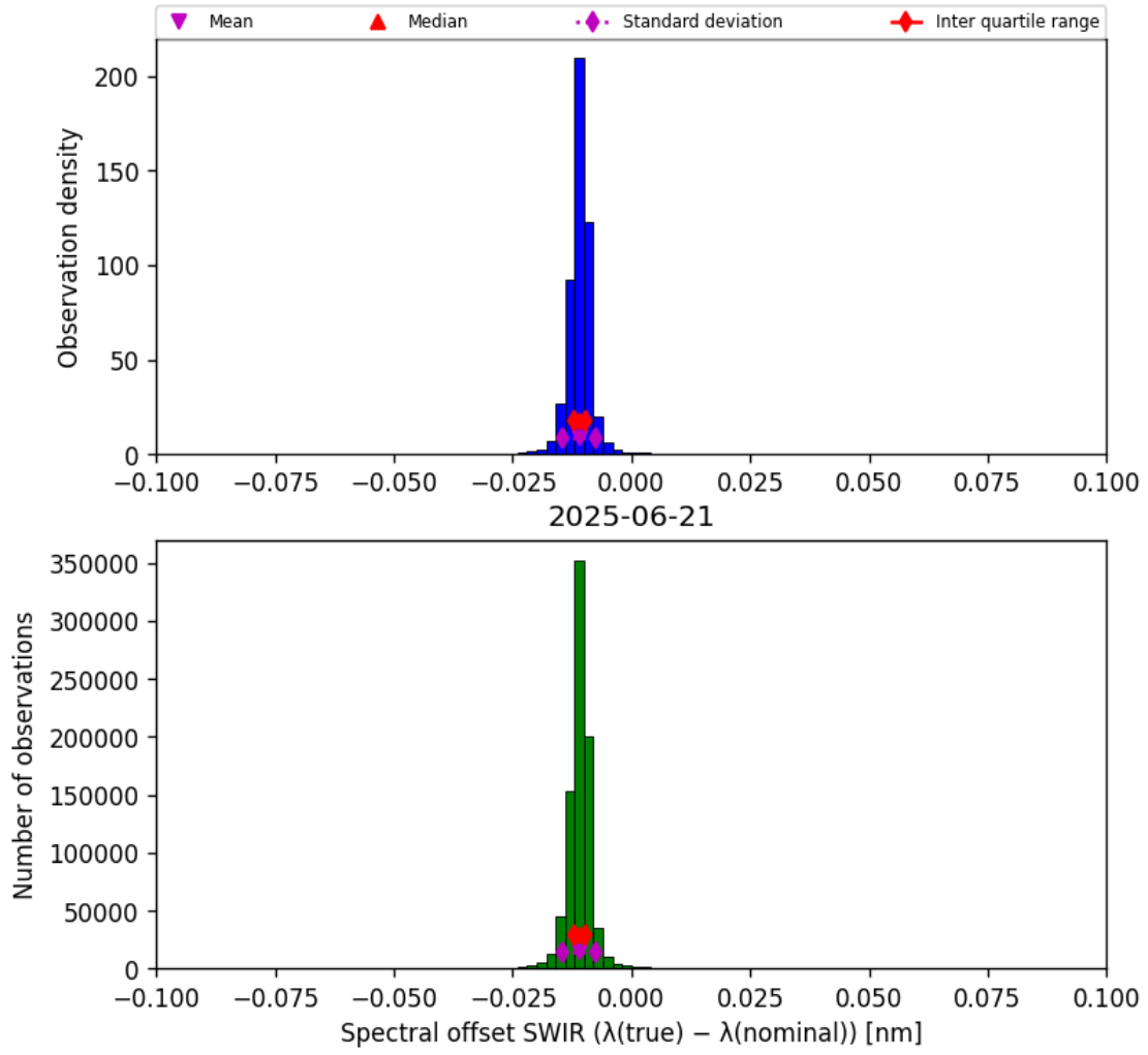
Figure 27: Histogram of “Spectral offset SWIR ( \lambda_{\text{true}} - \lambda_{\text{nominal}} )” for 2025-06-20 to 2025-06-22
