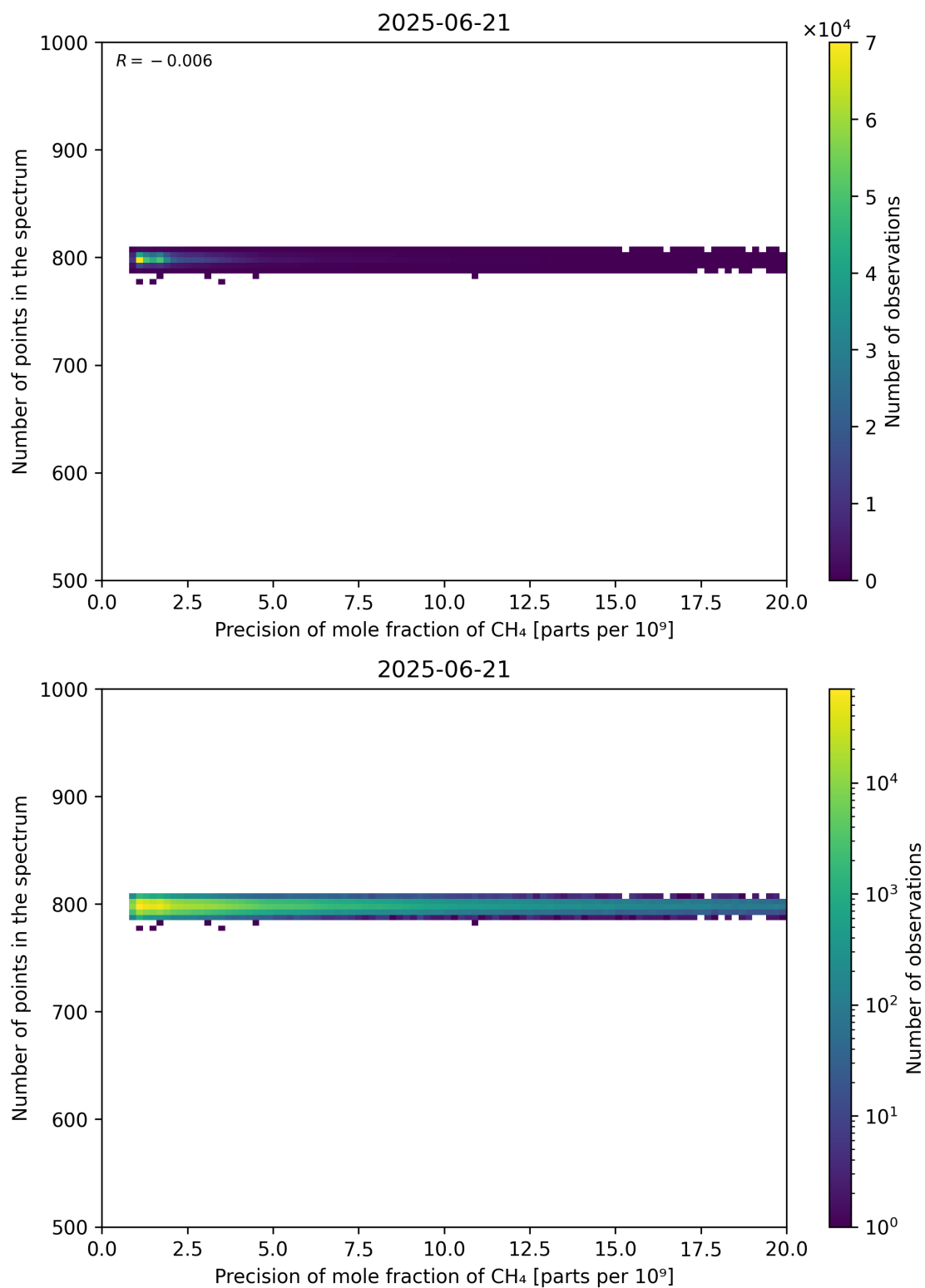
Figure 84: Scatter density plot of “Precision of mole fraction of CH 4 ” against “Number of points in the spectrum” for 2025-06-20 to 2025-06-22.
