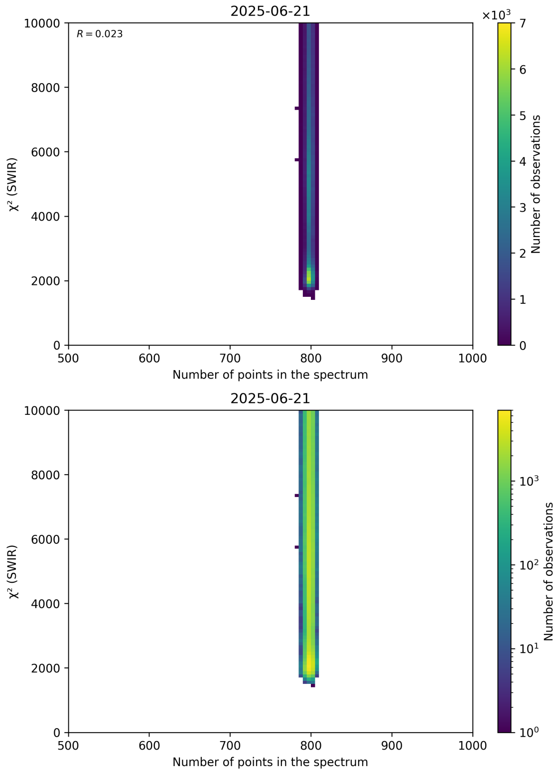
Figure 89: Scatter density plot of “Number of points in the spectrum” against “ \chi^2 (SWIR)” for 2025-06-20 to 2025-06-22.
