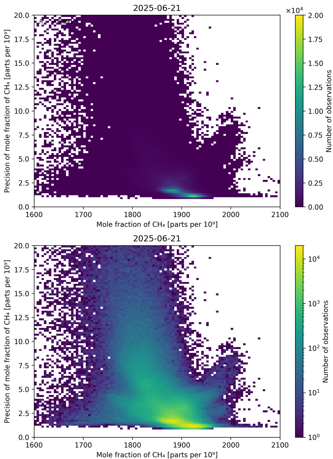
Figure 75: Scatter density plot of “Mole fraction of CH 4 ” against “Precision of mole fraction of CH 4 ” for 2025-06-20 to 2025-06-22.
