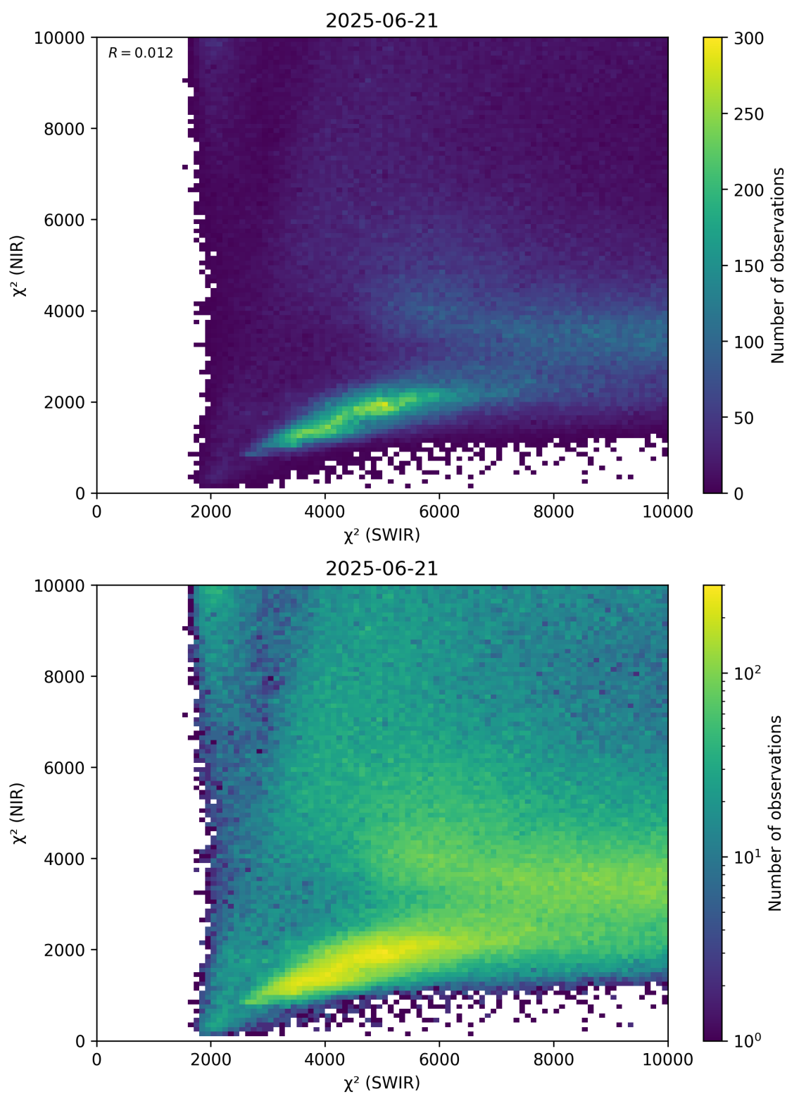
Figure 47: Scatter density plot of “ \chi^2 (SWIR)” against “ \chi^2 (NIR)” for 2025-06-20 to 2025-06-22.
