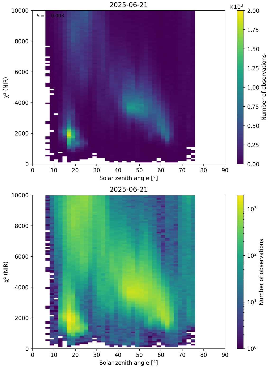
Figure 94: Scatter density plot of “Solar zenith angle” against “ \chi^2 (NIR)” for 2025-06-20 to 2025-06-22.
