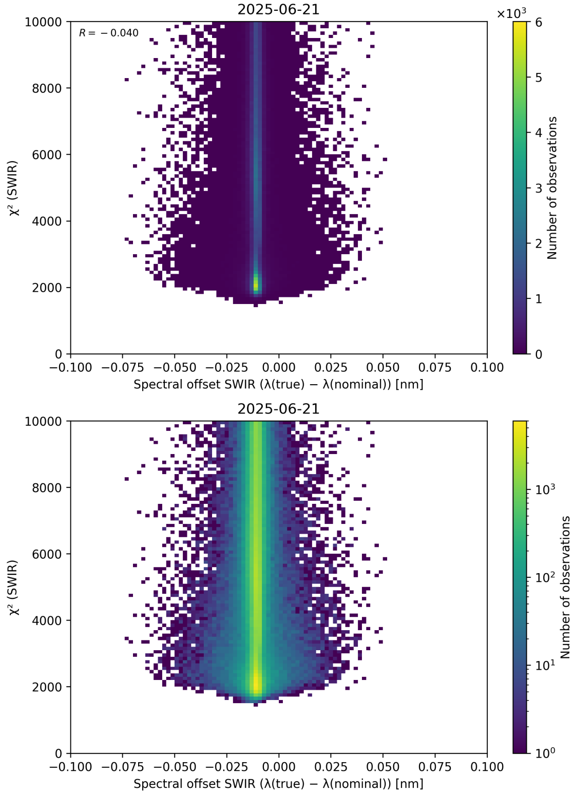
Figure 118: Scatter density plot of “Spectral offset SWIR ( \lambda_{\text{true}} - \lambda_{\text{nominal}} )” against “ \chi^2 (SWIR)” for 2025-06-20 to 2025-06-22.
