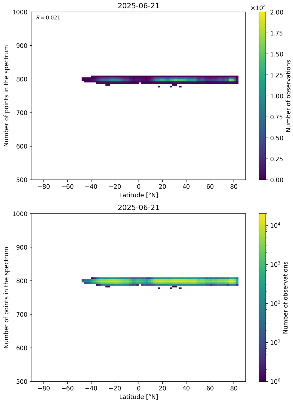
Figure 61: Scatter density plot of “Latitude” against “Number of points in the spectrum” for 2025-06-20 to 2025-06-22.
