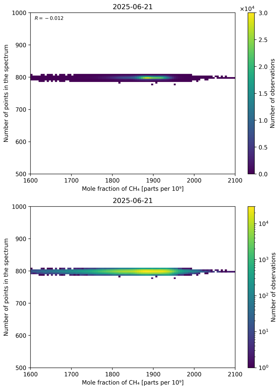
Figure 77: Scatter density plot of “Mole fraction of CH 4 ” against “Number of points in the spectrum” for 2025-06-20 to 2025-06-22.
