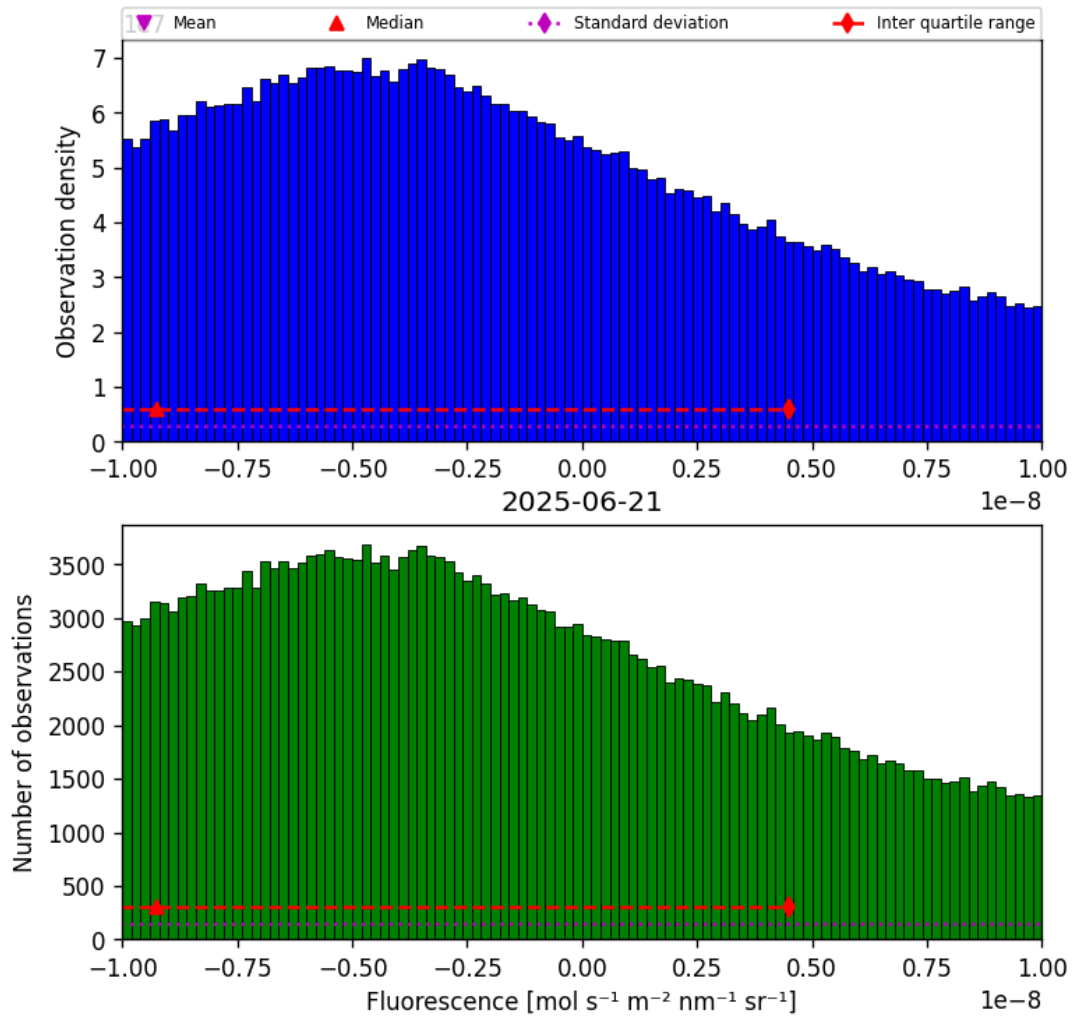
Figure 32: Histogram of “Fluorescence” for 2025-06-20 to 2025-06-22
