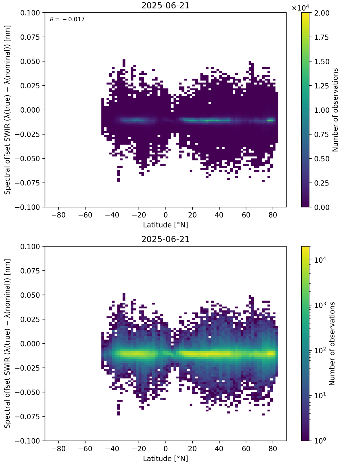
Figure 62: Scatter density plot of “Latitude” against “Spectral offset SWIR ( \lambda_{\text{true}} - \lambda_{\text{nominal}} )” for 2025-06-20 to 2025-06-22.
