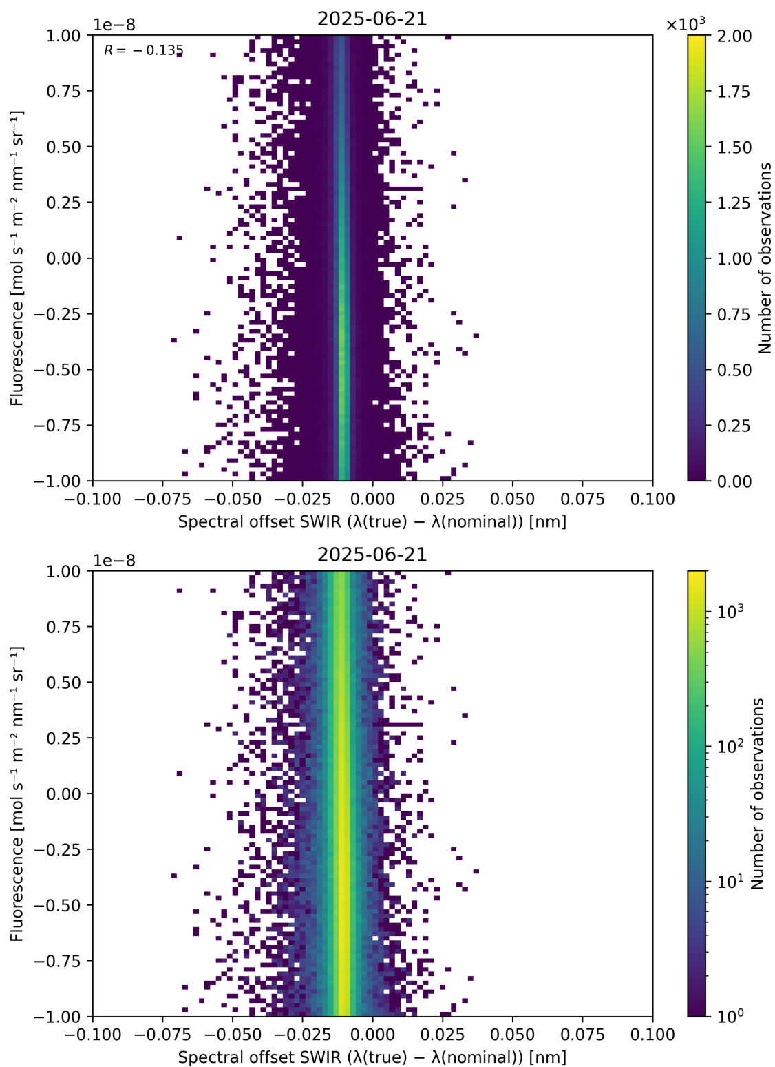
Figure 120: Scatter density plot of “Spectral offset SWIR ( \lambda_{\text{true}} - \lambda_{\text{nominal}} )” against “Fluorescence” for 2025-06-20 to 2025-06-22.
