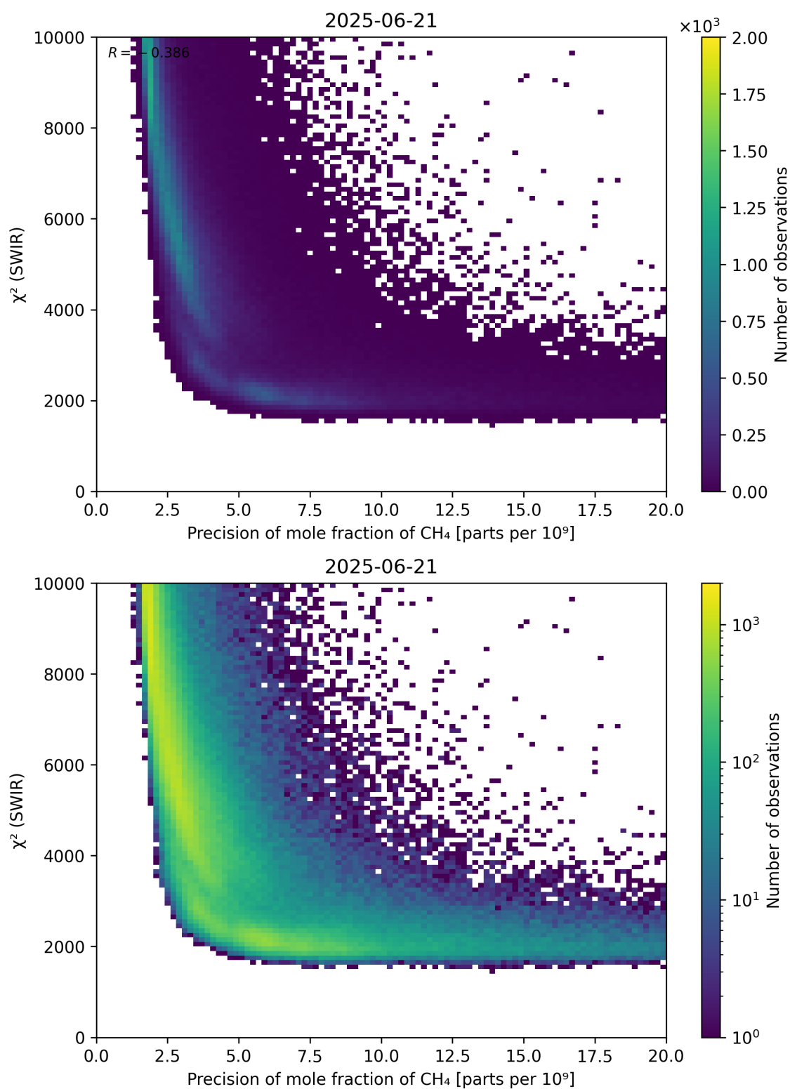
Figure 79: Scatter density plot of “Precision of mole fraction of \text{CH}_4 ” against “ \chi^2 (SWIR)” for 2025-06-20 to 2025-06-22.
