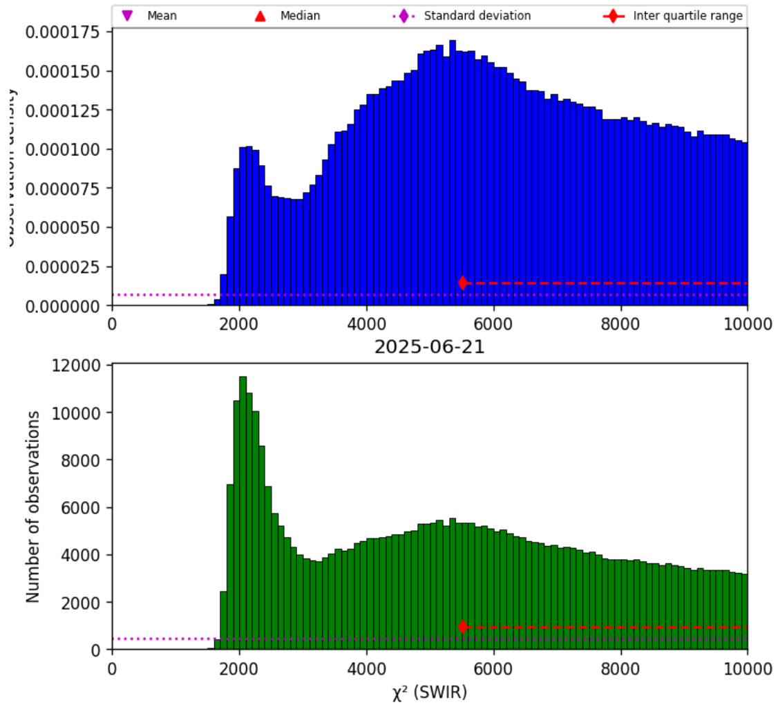
Figure 28: Histogram of “ \chi^2 (SWIR)” for 2025-06-20 to 2025-06-22
