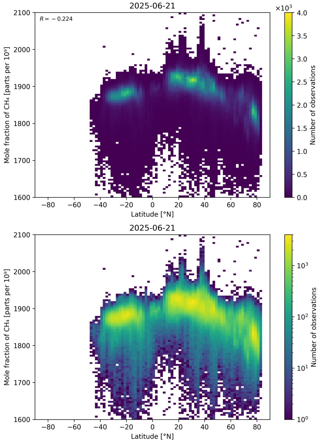
Figure 57: Scatter density plot of “Latitude” against “Mole fraction of CH 4 ” for 2025-06-20 to 2025-06-22.
