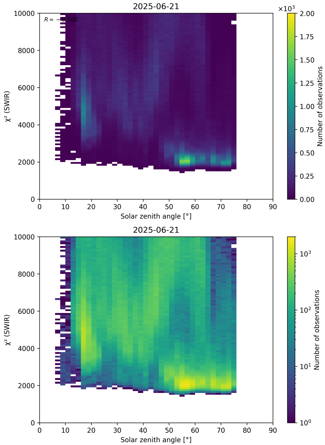
Figure 95: Scatter density plot of “Solar zenith angle” against “ \chi^2 (SWIR)” for 2025-06-20 to 2025-06-22.
