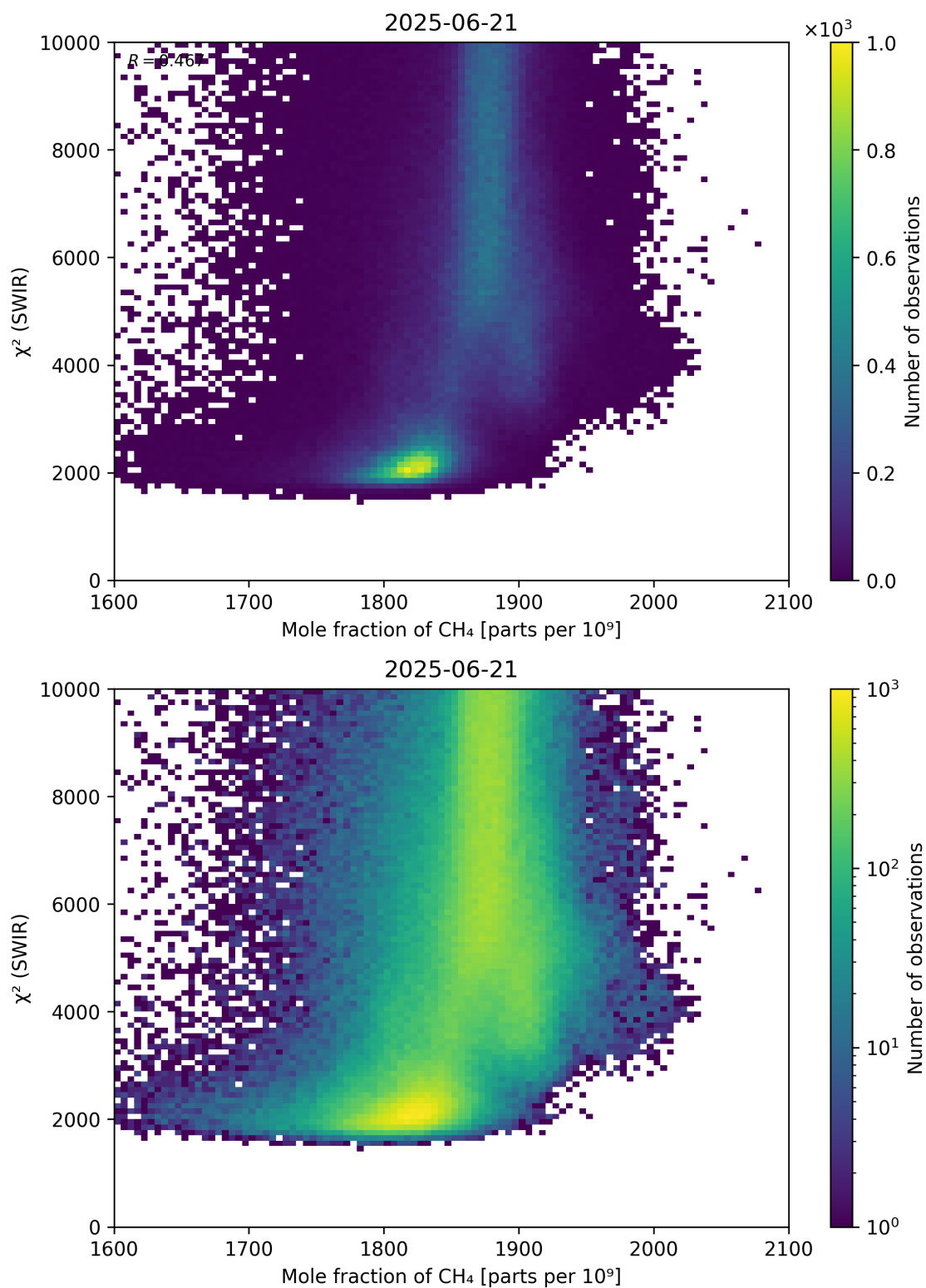
Figure 71: Scatter density plot of “Mole fraction of \text{CH}_4 ” against “ \chi^2 (SWIR)” for 2025-06-20 to 2025-06-22.
