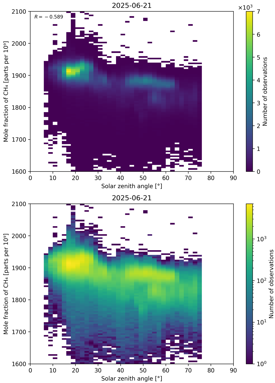
Figure 99: Scatter density plot of “Solar zenith angle” against “Mole fraction of \text{CH}_4 ” for 2025-06-20 to 2025-06-22.
