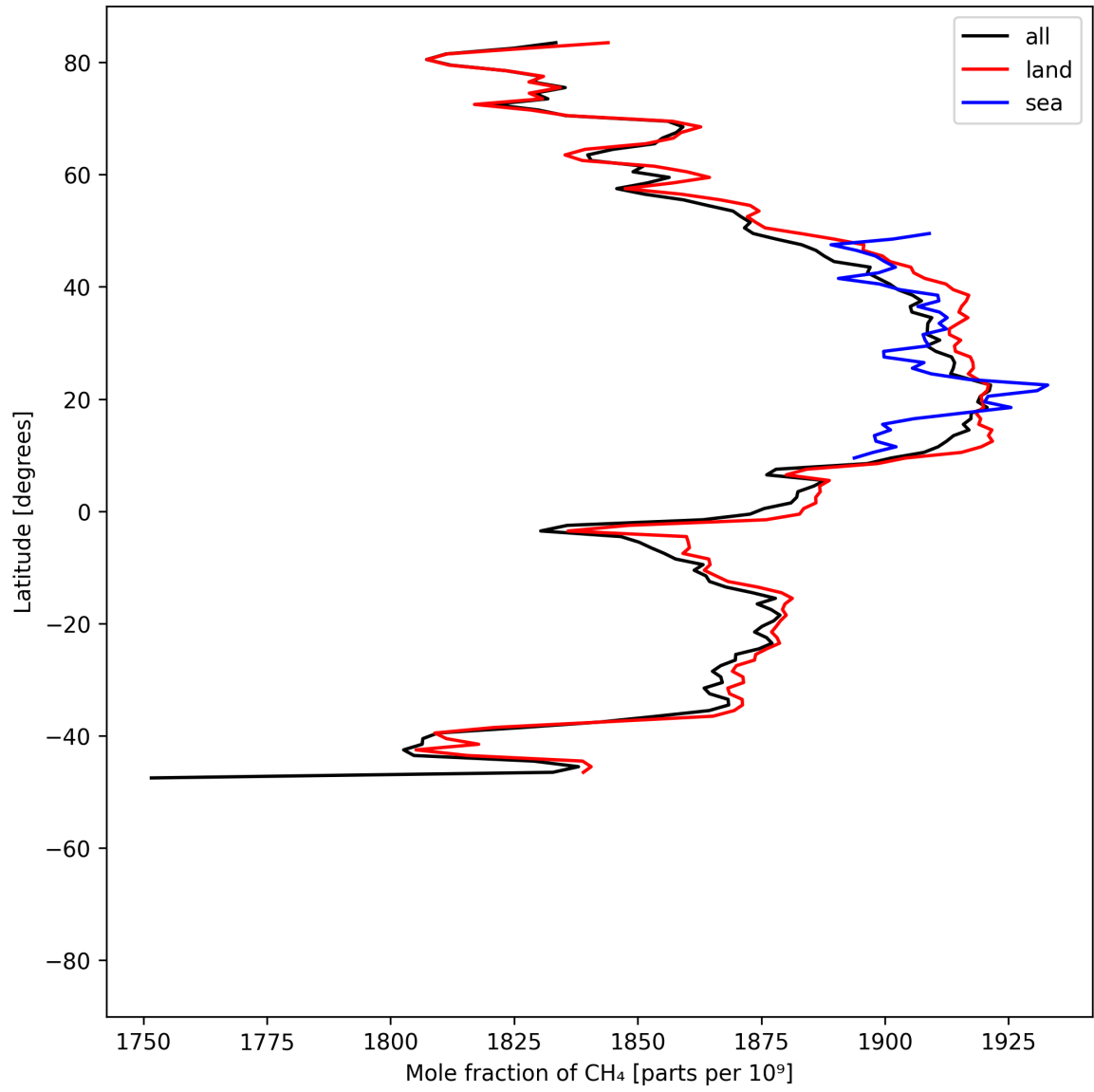
Figure 12: Zonal average of “Mole fraction of CH 4 ” for 2025-06-20 to 2025-06-22.
