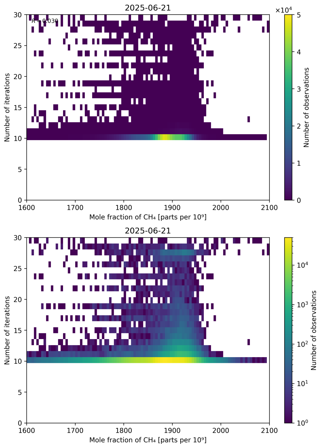
Figure 76: Scatter density plot of “Mole fraction of CH 4 ” against “Number of iterations” for 2025-06-20 to 2025-06-22.
