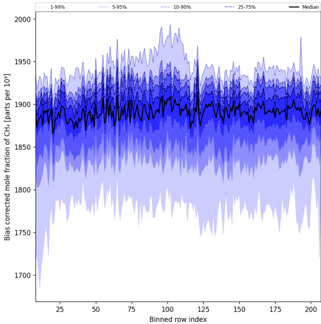
Figure 36: Along track statistics of “Bias corrected mole fraction of CH 4 ” for 2025-06-20 to 2025-06-22
