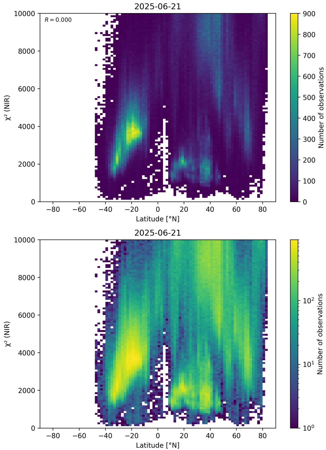
Figure 53: Scatter density plot of “Latitude” against “ \chi^2 (NIR)” for 2025-06-20 to 2025-06-22.
