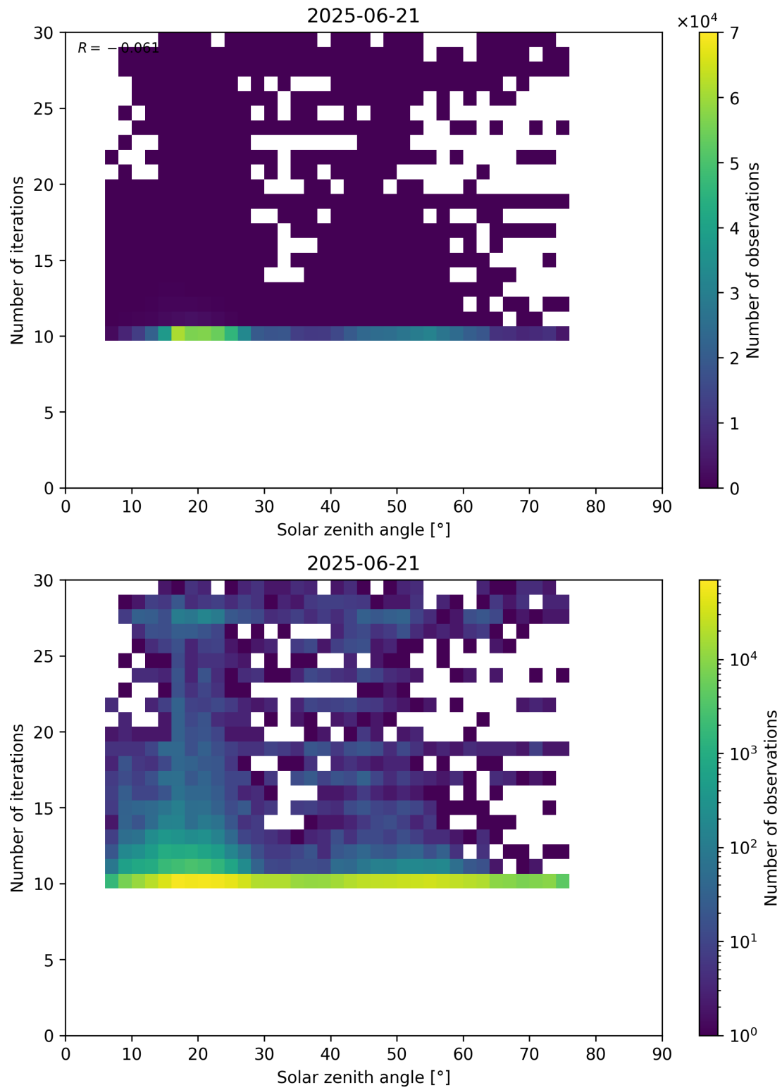
Figure 102: Scatter density plot of “Solar zenith angle” against “Number of iterations” for 2025-06-20 to 2025-06-22.
