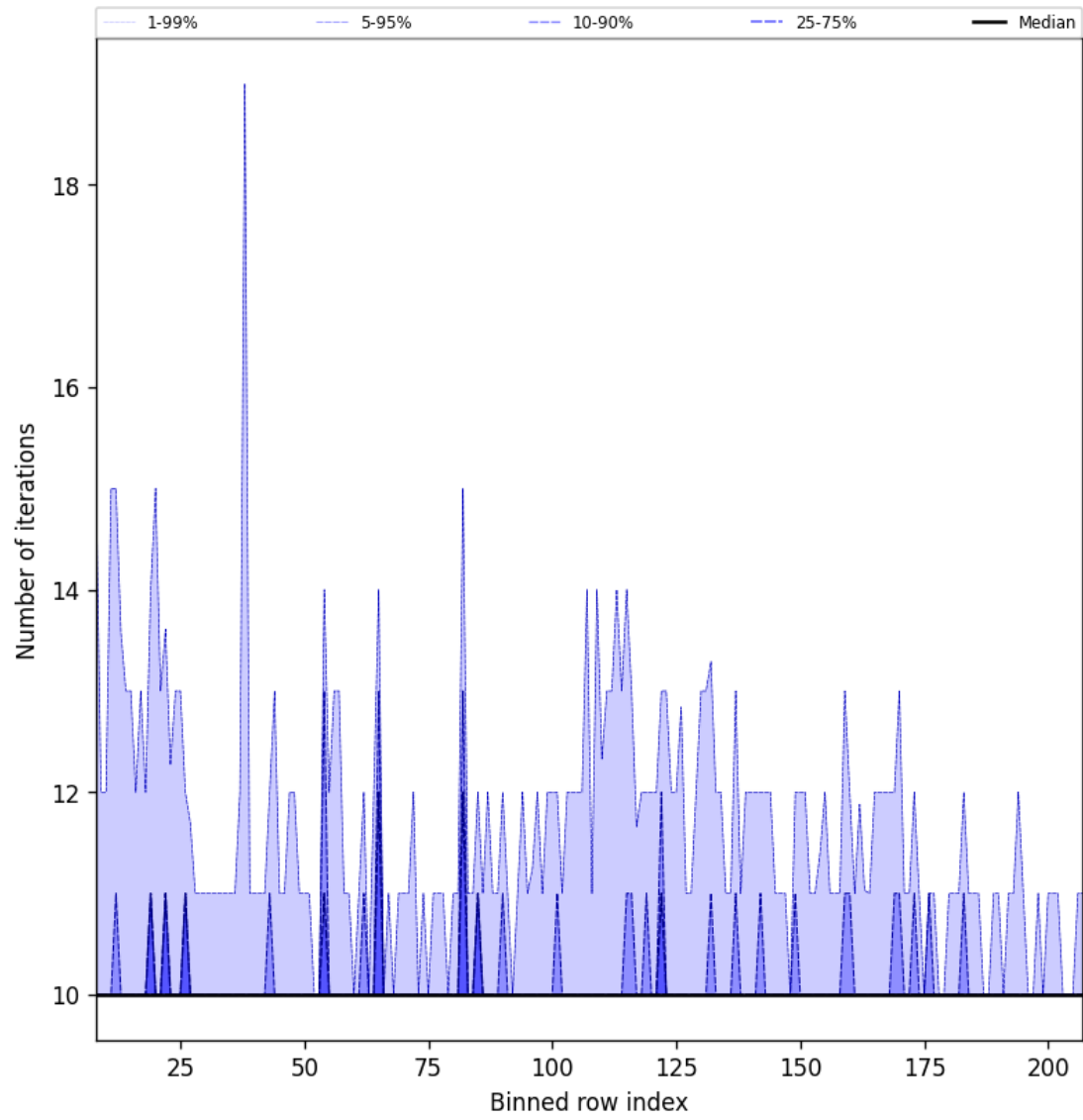
Figure 42: Along track statistics of “Number of iterations” for 2025-06-20 to 2025-06-22
