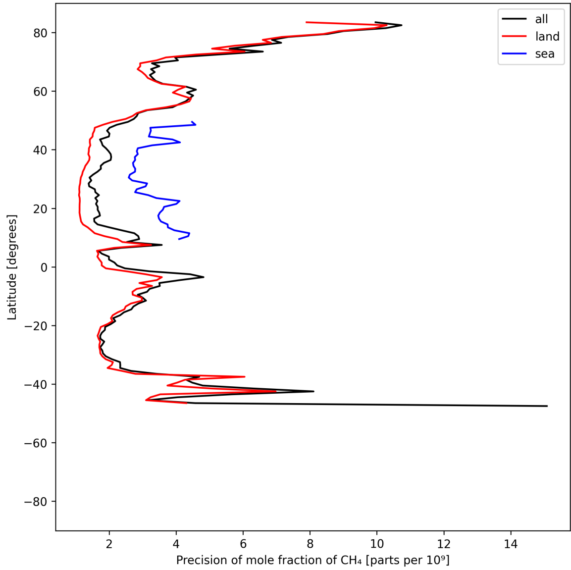
Figure 13: Zonal average of “Precision of mole fraction of CH 4 ” for 2025-06-20 to 2025-06-22.
