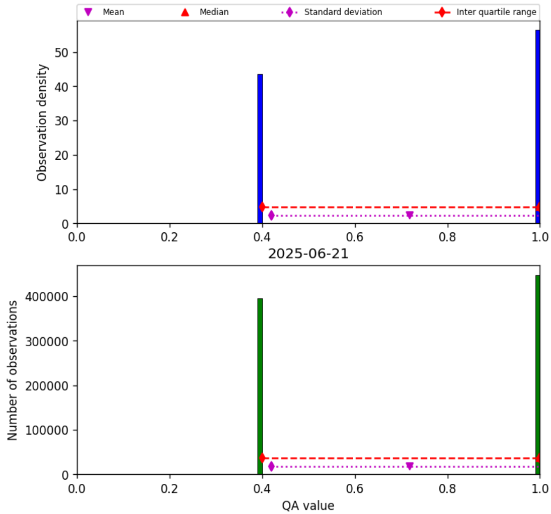
Figure 22: Histogram of “QA value” for 2025-06-20 to 2025-06-22
