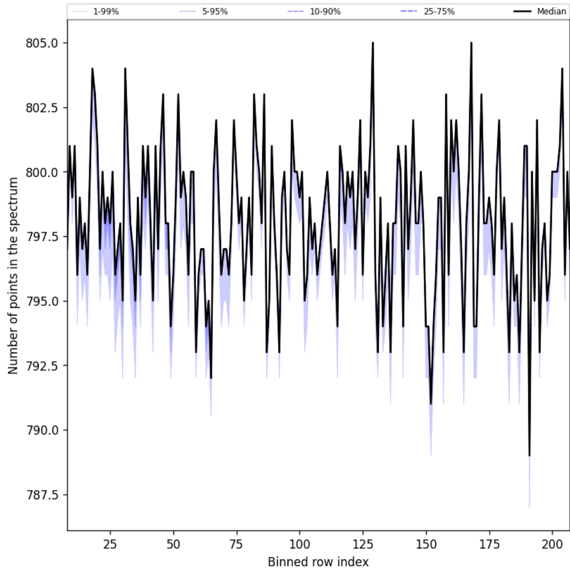
Figure 37: Along track statistics of “Number of points in the spectrum” for 2025-06-20 to 2025-06-22
