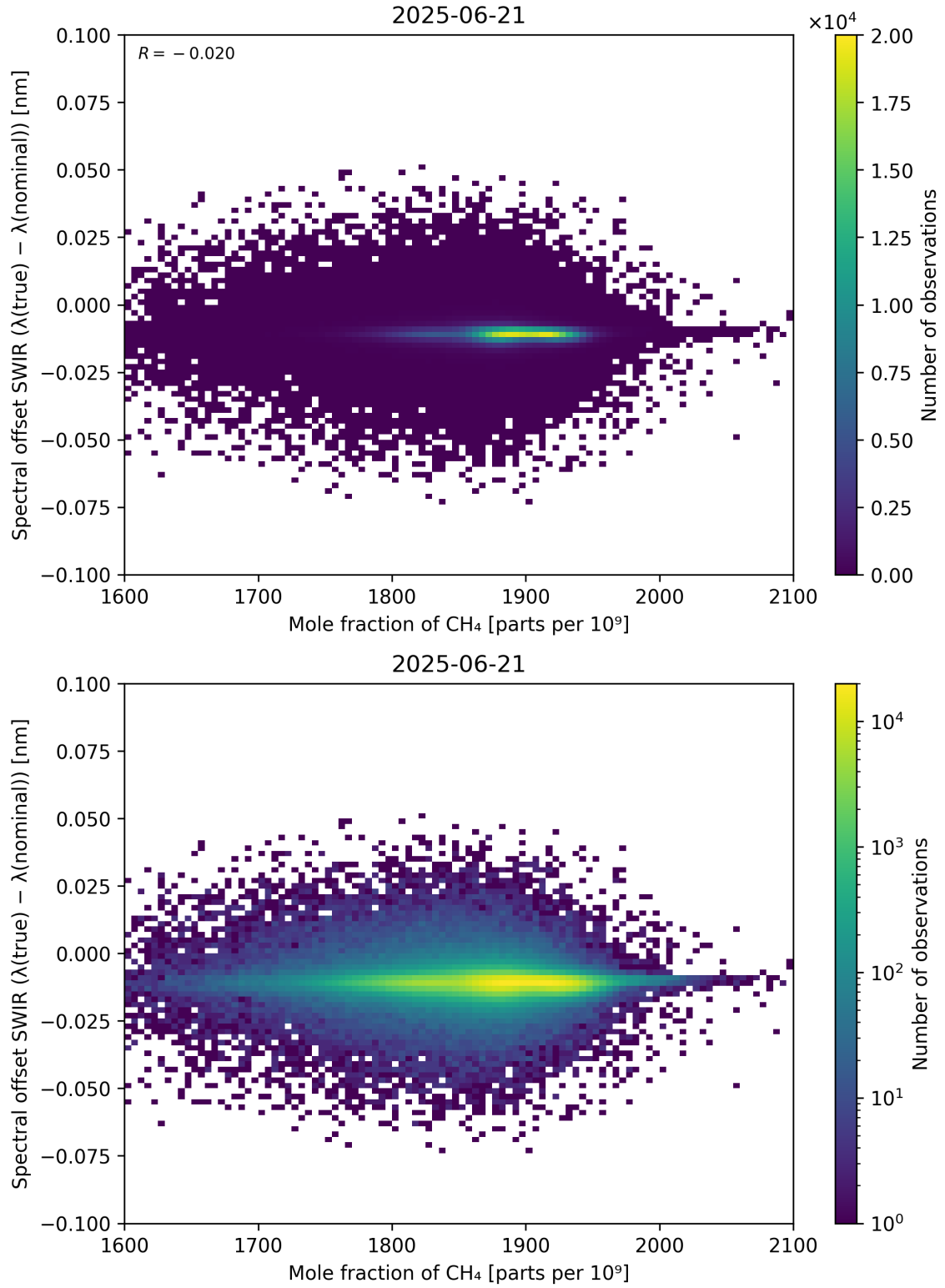
Figure 86: Scatter density plot of “Mole fraction of \text{CH}_4 ” against “Spectral offset SWIR ( \lambda_{\text{true}} - \lambda_{\text{nominal}} )” for 2025-06-20 to 2025-06-22.
