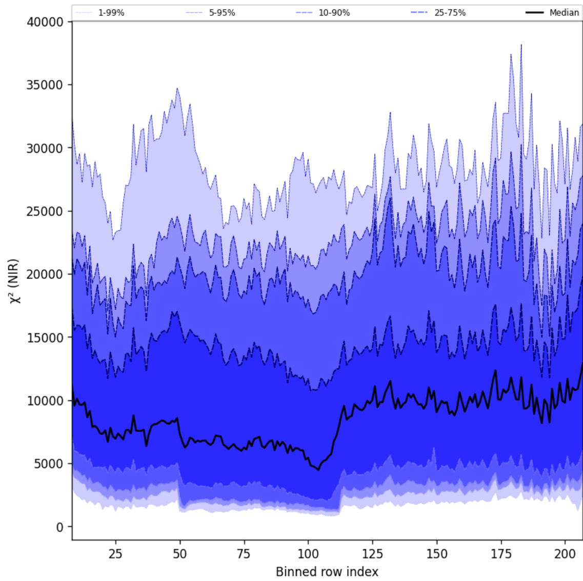
Figure 40: Along track statistics of “ \chi^2 (NIR)” for 2025-06-20 to 2025-06-22
