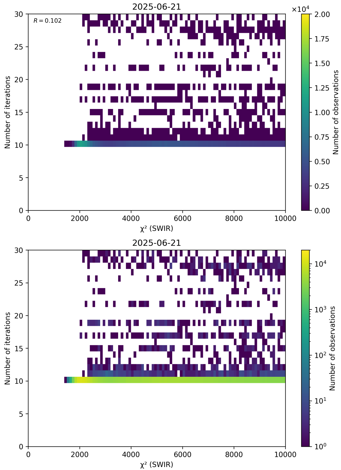
Figure 50: Scatter density plot of “ \chi^2 (SWIR)” against “Number of iterations” for 2025-06-20 to 2025-06-22.
