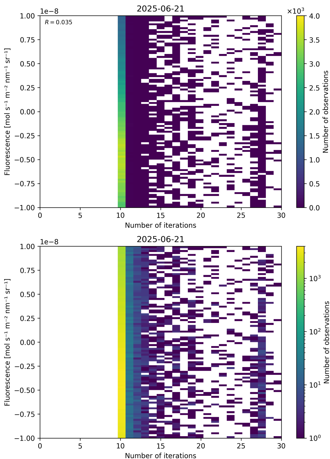
Figure 87: Scatter density plot of “Number of iterations” against “Fluorescence” for 2025-06-20 to 2025-06-22.
