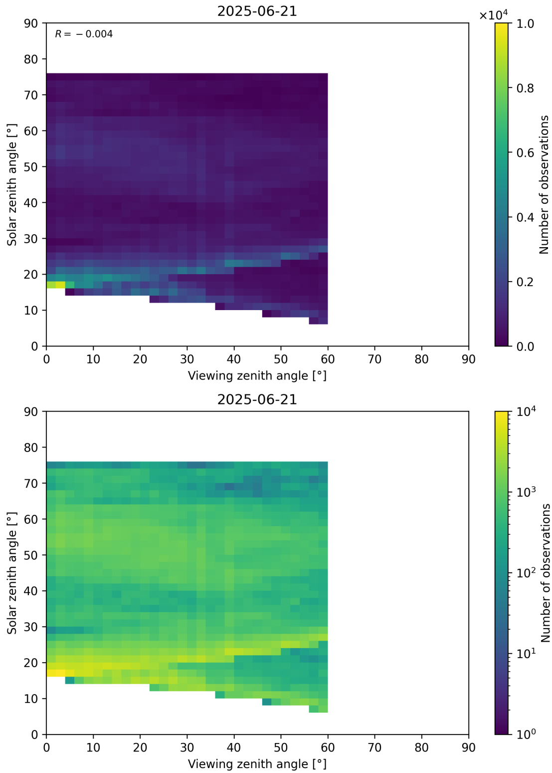
Figure 115: Scatter density plot of “Viewing zenith angle” against “Solar zenith angle” for 2025-06-20 to 2025-06-22.
