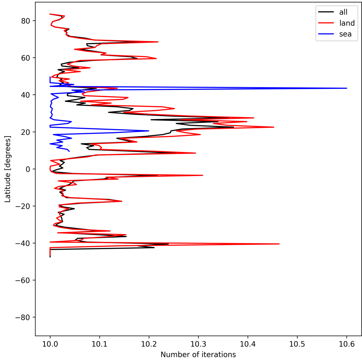
Figure 20: Zonal average of “Number of iterations” for 2025-06-20 to 2025-06-22.
