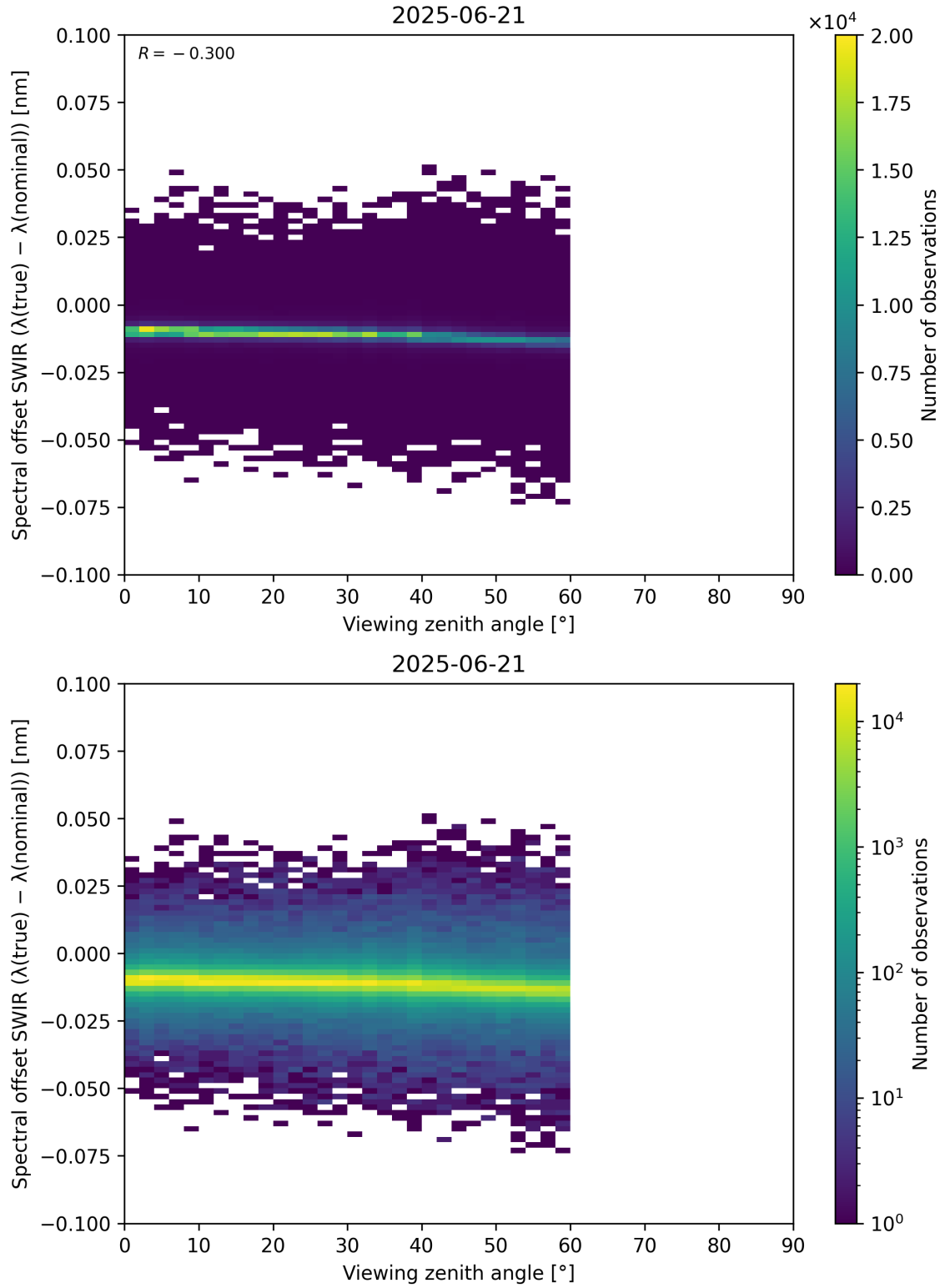
Figure 116: Scatter density plot of “Viewing zenith angle” against “Spectral offset SWIR ( \lambda_{\text{true}} - \lambda_{\text{nominal}} )” for 2025-06-20 to 2025-06-22.
