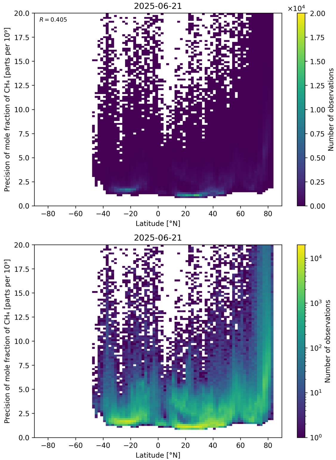
Figure 59: Scatter density plot of “Latitude” against “Precision of mole fraction of \text{CH}_4 ” for 2025-06-20 to 2025-06-22.
