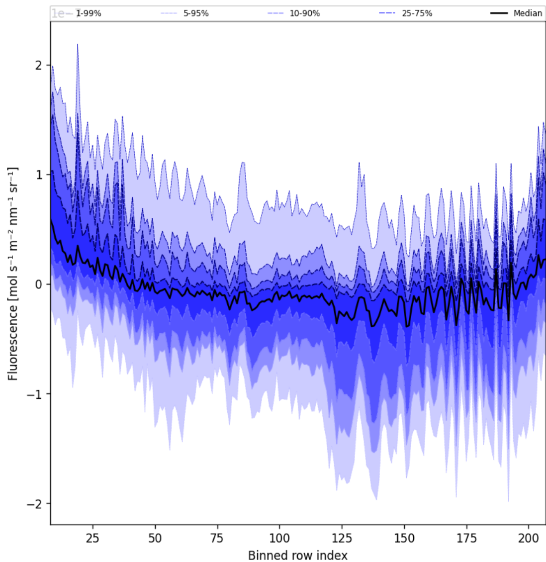
Figure 43: Along track statistics of “Fluorescence” for 2025-06-20 to 2025-06-22
