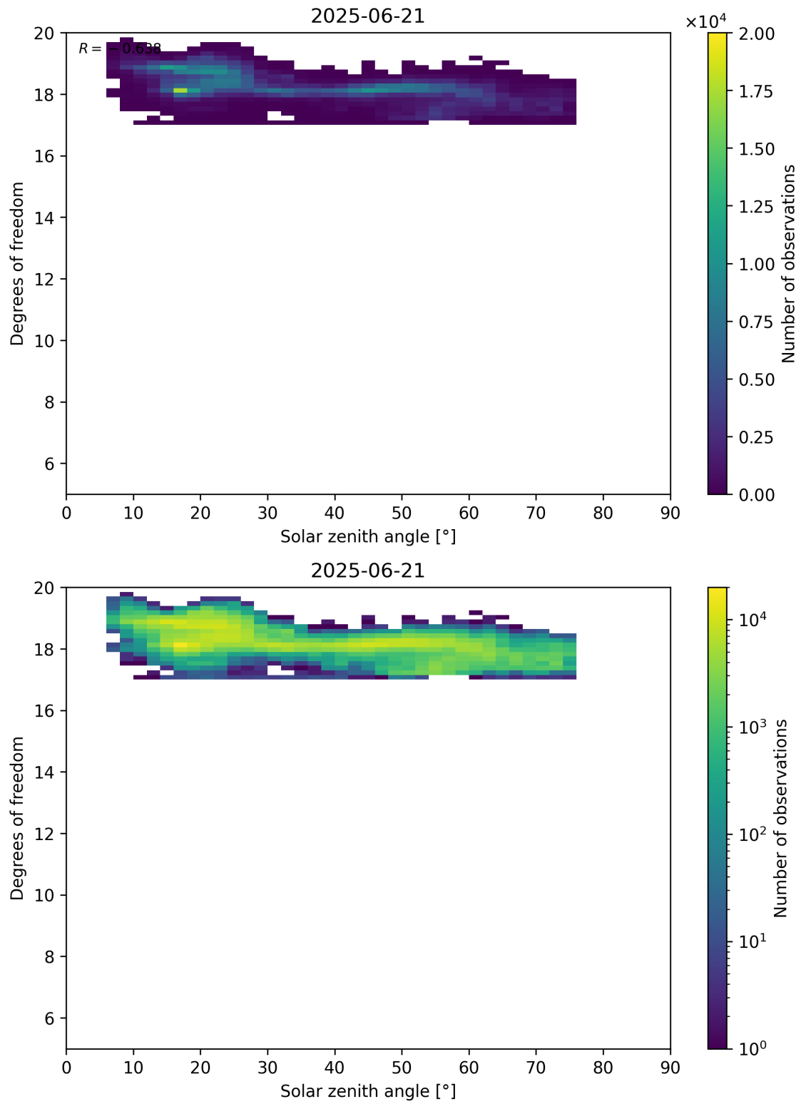
Figure 96: Scatter density plot of “Solar zenith angle” against “Degrees of freedom” for 2025-06-20 to 2025-06-22.
