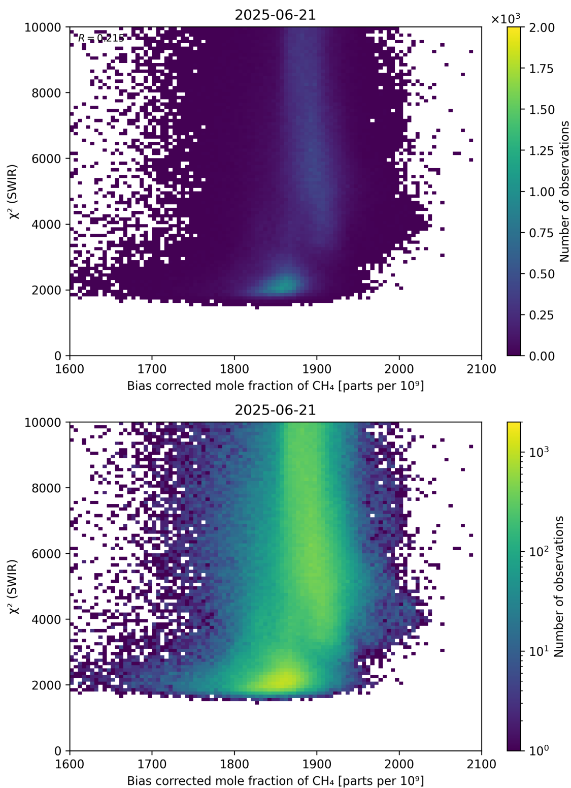
Figure 64: Scatter density plot of “Bias corrected mole fraction of \text{CH}_4 ” against “ \chi^2 (SWIR)” for 2025-06-20 to 2025-06-22.
