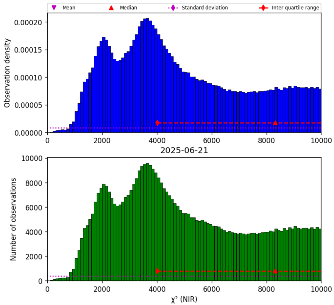
Figure 29: Histogram of “ \chi^2 (NIR)” for 2025-06-20 to 2025-06-22
