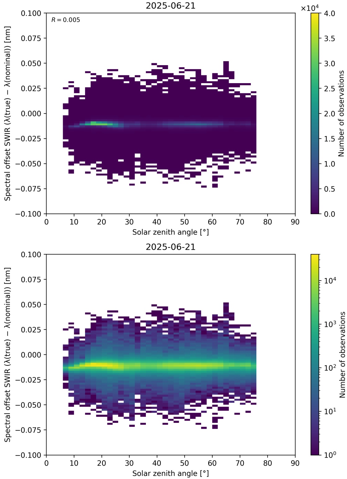
Figure 104: Scatter density plot of “Solar zenith angle” against “Spectral offset SWIR ( \lambda_{\text{true}} - \lambda_{\text{nominal}} )” for 2025-06-20 to 2025-06-22.
