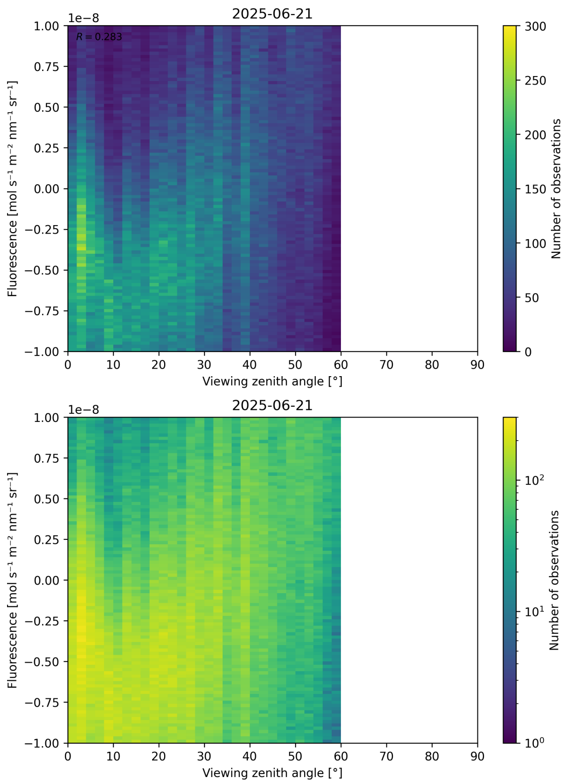
Figure 108: Scatter density plot of “Viewing zenith angle” against “Fluorescence” for 2025-06-20 to 2025-06-22.
