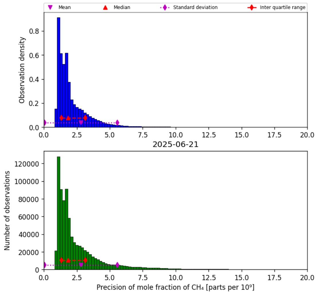
Figure 24: Histogram of “Precision of mole fraction of CH 4 ” for 2025-06-20 to 2025-06-22
