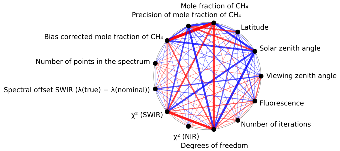
Figure 1: Map of correlation graph for 2025-06-20 to 2025-06-22.
