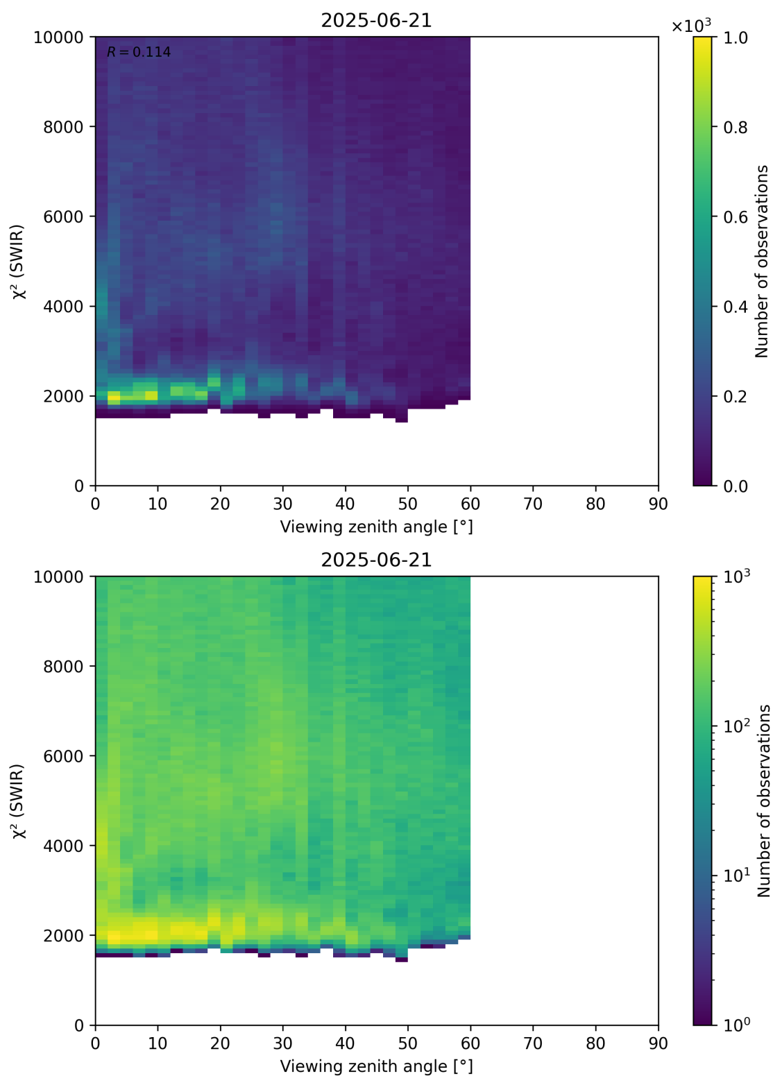
Figure 106: Scatter density plot of “Viewing zenith angle” against “ \chi^2 (SWIR)” for 2025-06-20 to 2025-06-22.
