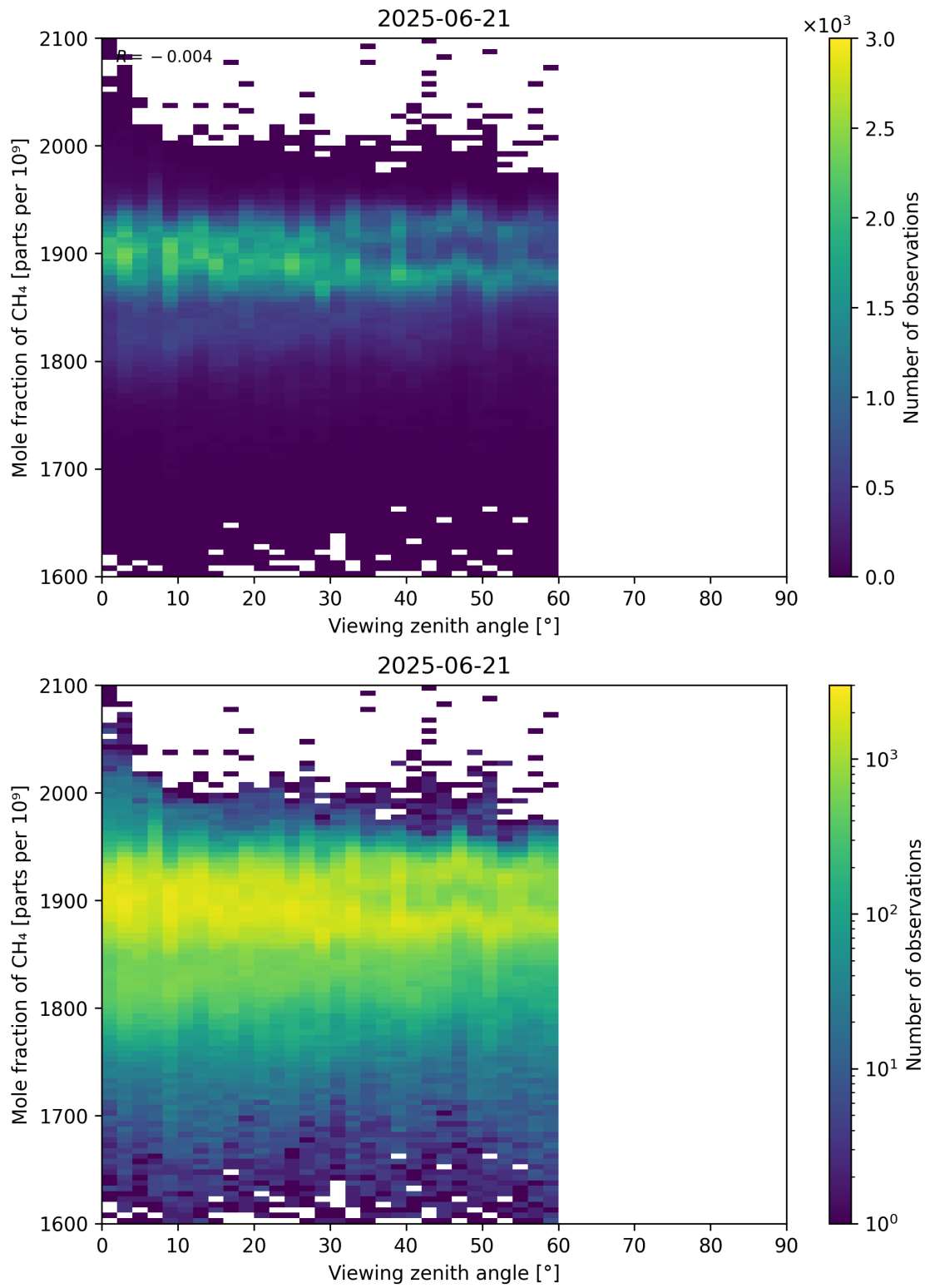
Figure 110: Scatter density plot of “Viewing zenith angle” against “Mole fraction of CH 4 ” for 2025-06-20 to 2025-06-22.
