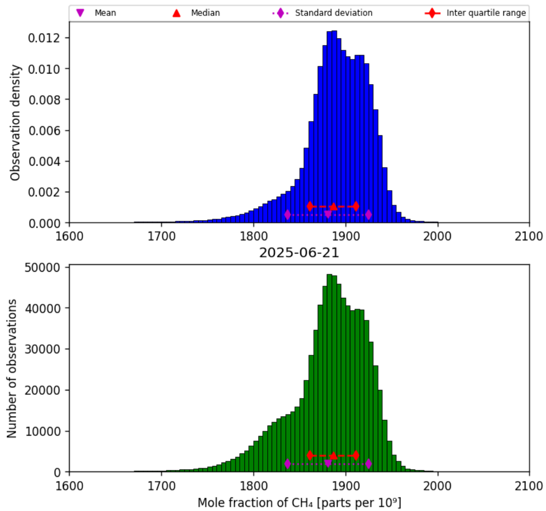
Figure 23: Histogram of “Mole fraction of CH 4 ” for 2025-06-20 to 2025-06-22
