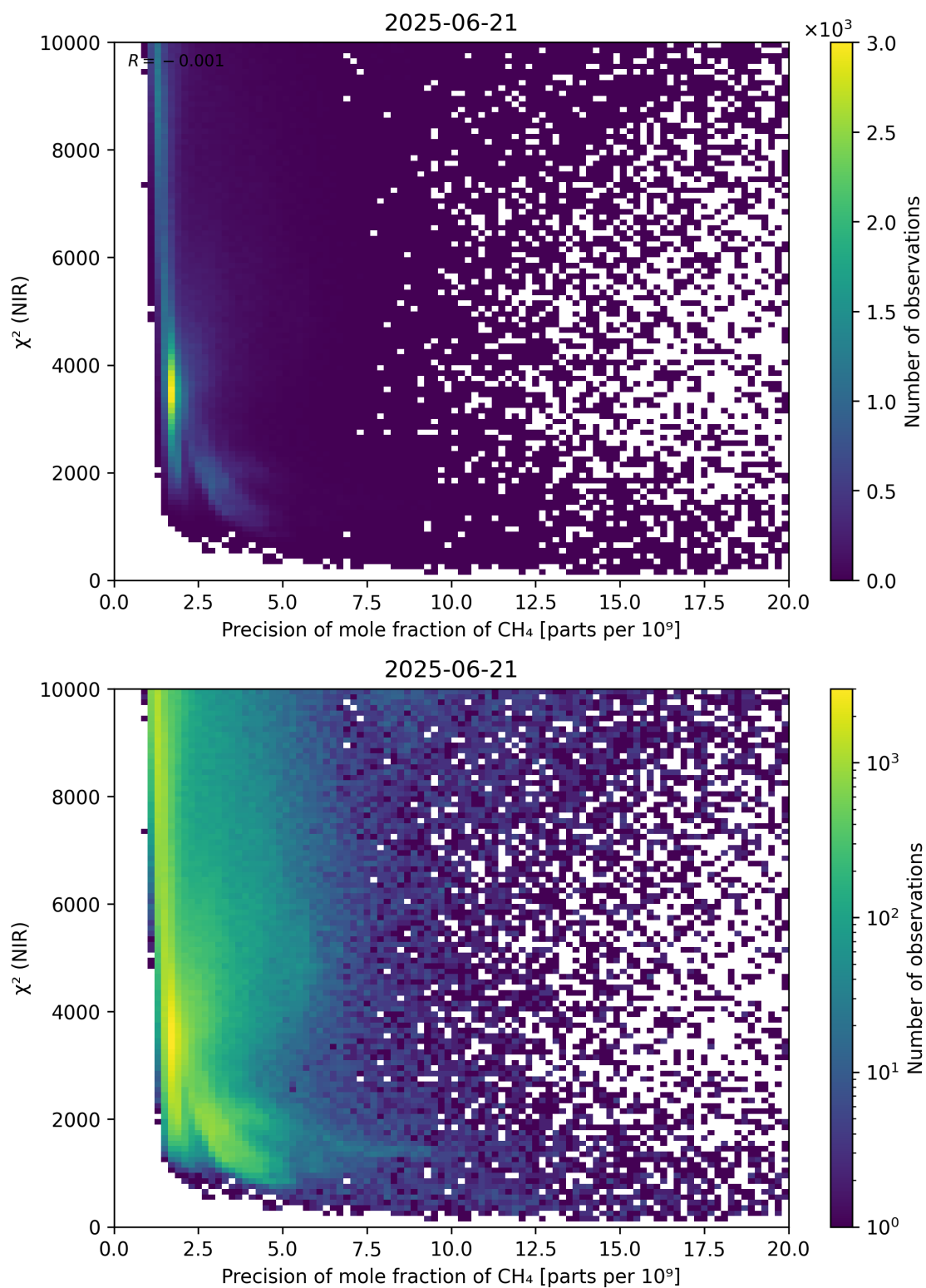
Figure 78: Scatter density plot of “Precision of mole fraction of CH 4 ” against “ \chi^2 (NIR)” for 2025-06-20 to 2025-06-22.
