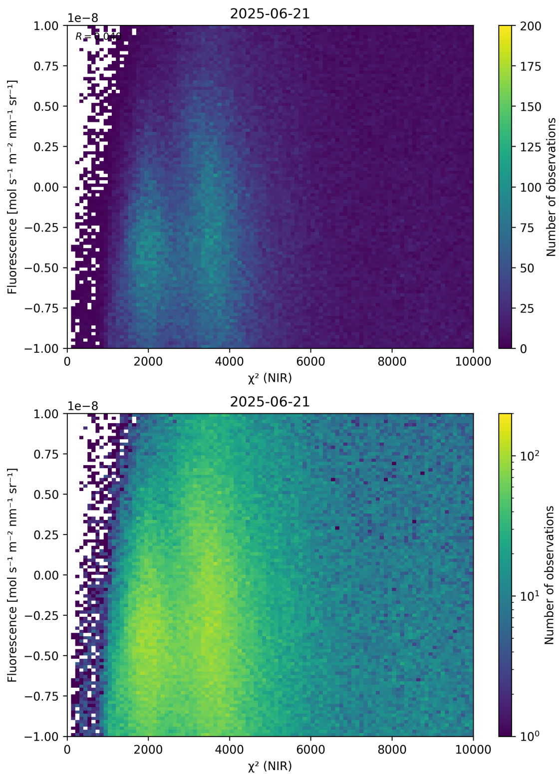
Figure 45: Scatter density plot of “ \chi^2 (NIR)” against “Fluorescence” for 2025-06-20 to 2025-06-22.
