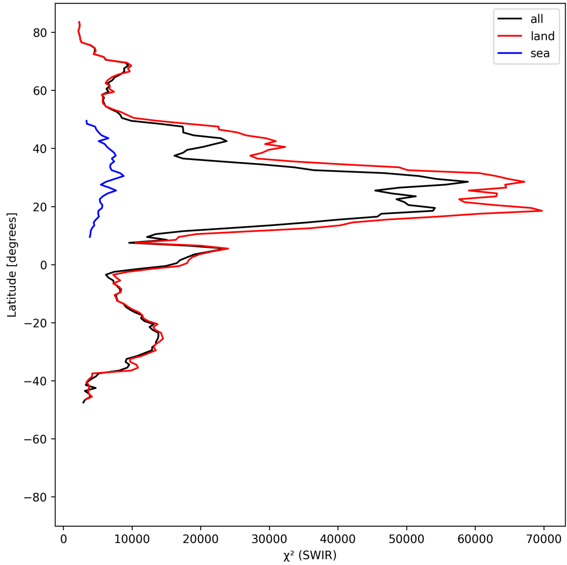
Figure 17: Zonal average of “ \chi^2 (SWIR)” for 2025-06-20 to 2025-06-22.
