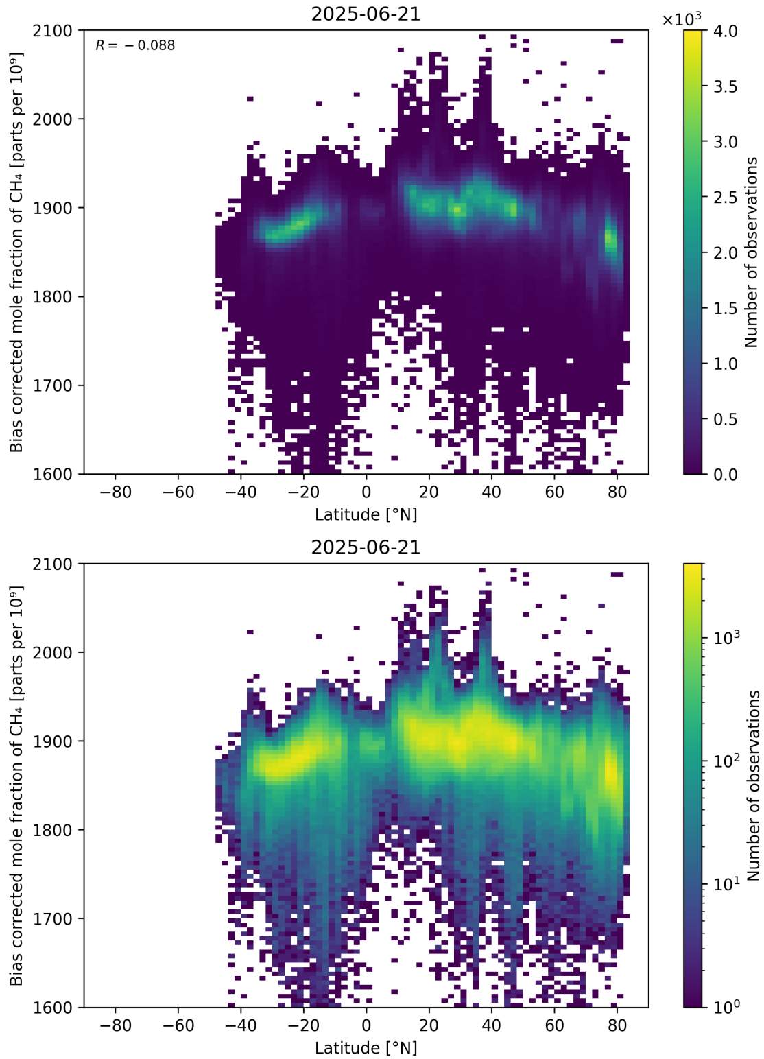
Figure 58: Scatter density plot of “Latitude” against “Bias corrected mole fraction of \text{CH}_4 ” for 2025-06-20 to 2025-06-22.
