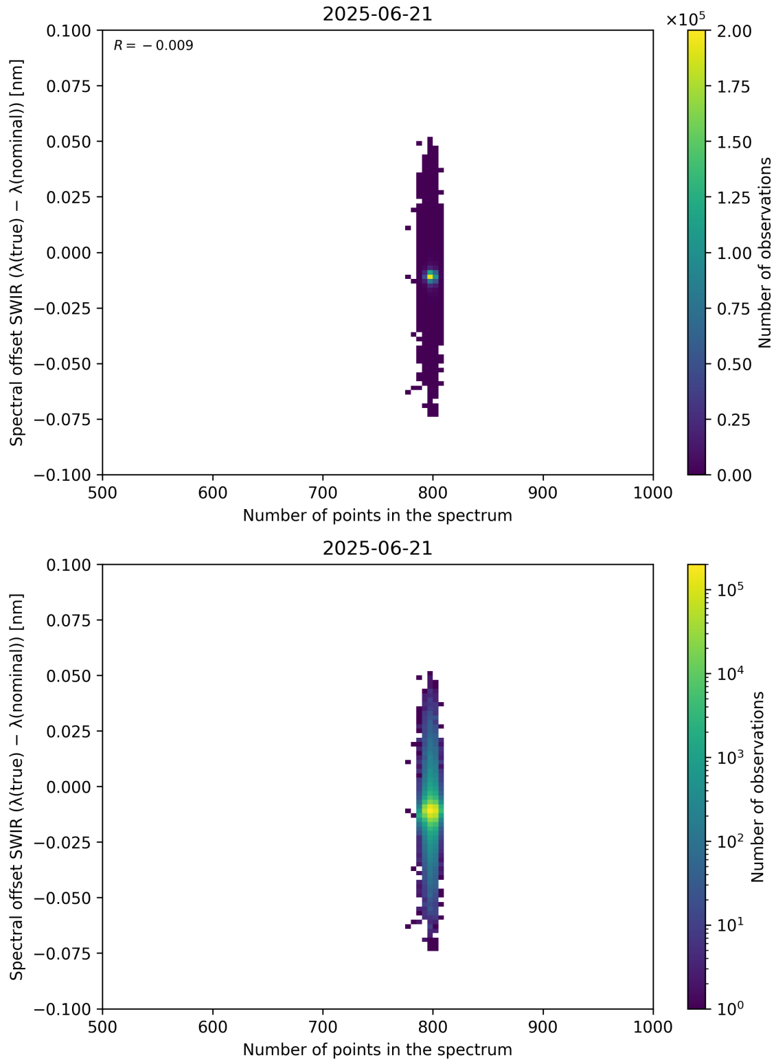
Figure 93: Scatter density plot of “Number of points in the spectrum” against “Spectral offset SWIR ( \lambda_{\text{true}} - \lambda_{\text{nominal}} )” for 2025-06-20 to 2025-06-22.
