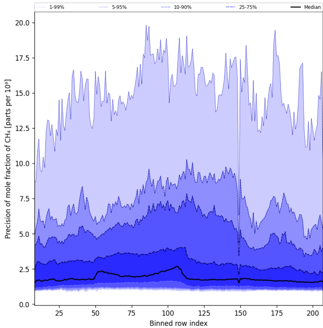
Figure 35: Along track statistics of “Precision of mole fraction of CH 4 ” for 2025-06-20 to 2025-06-22
