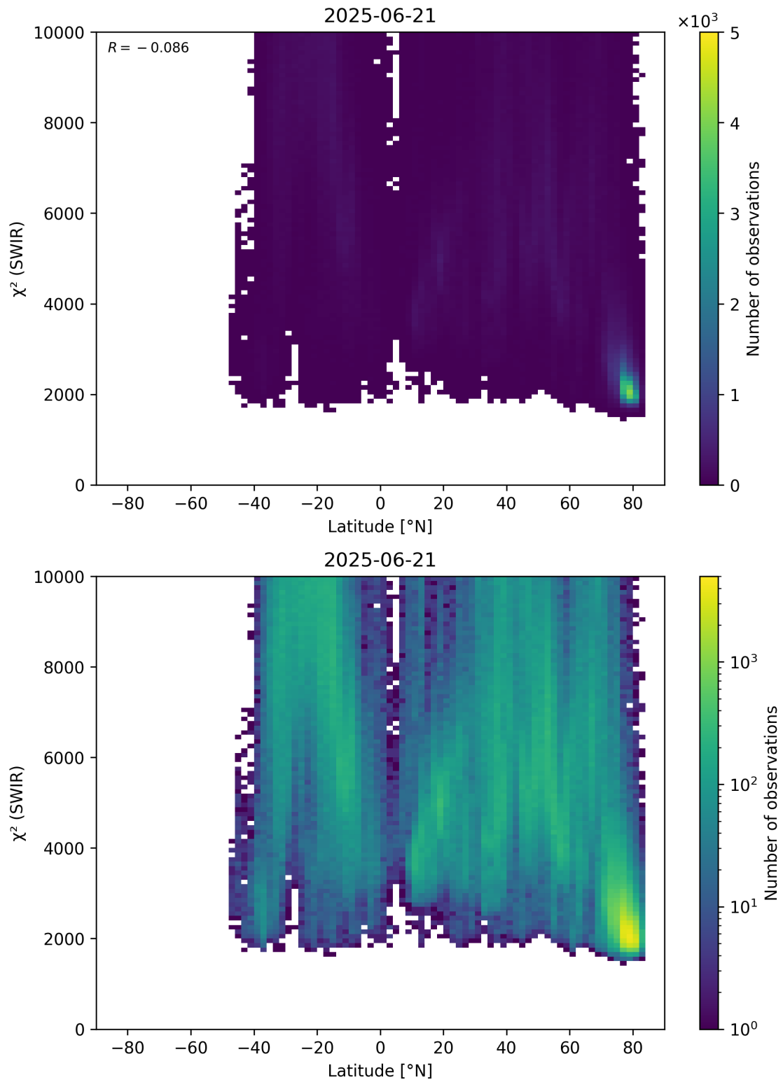
Figure 54: Scatter density plot of “Latitude” against “ \chi^2 (SWIR)” for 2025-06-20 to 2025-06-22.
