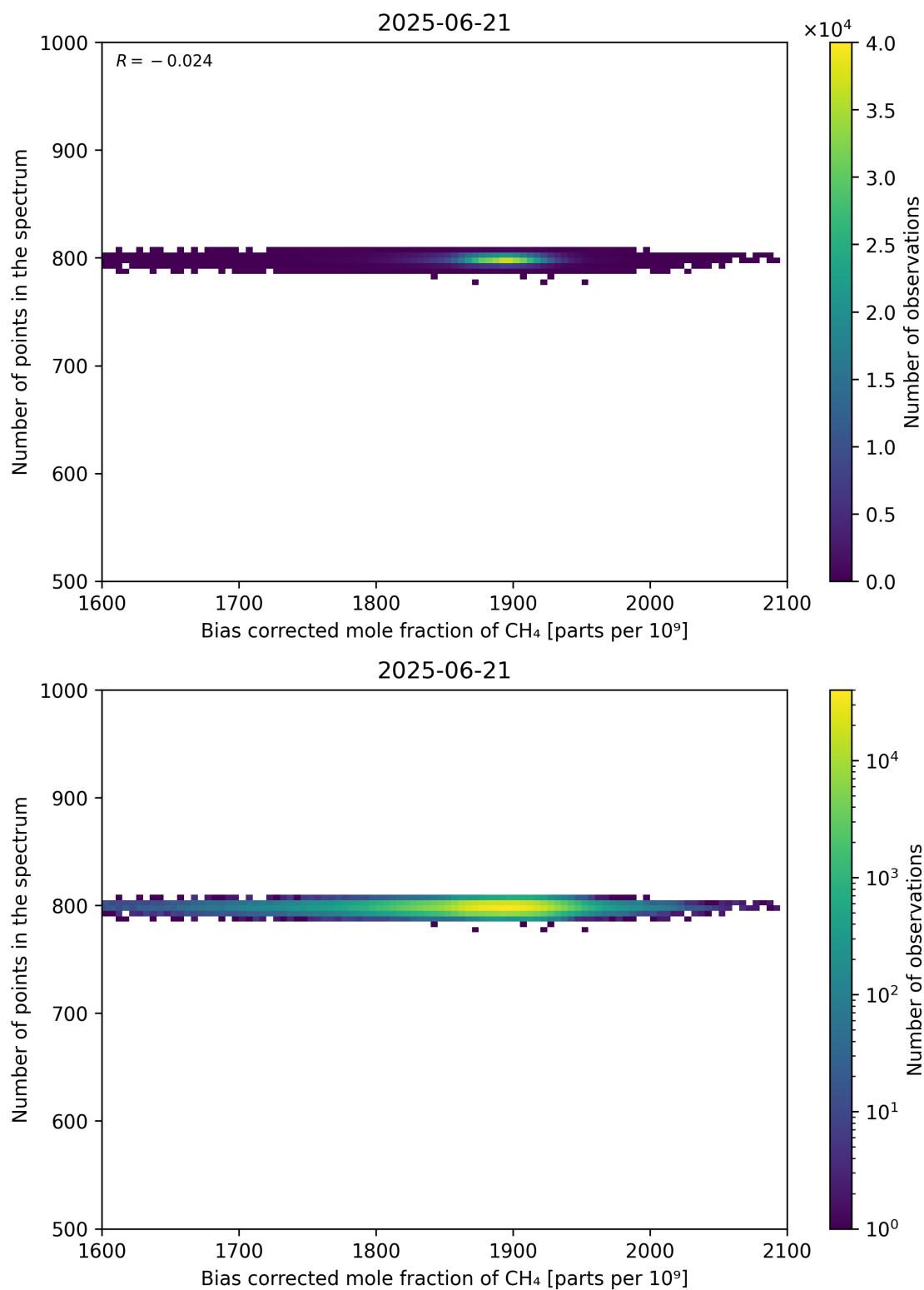
Figure 68: Scatter density plot of “Bias corrected mole fraction of CH 4 ” against “Number of points in the spectrum” for 2025-06-20 to 2025-06-22.
