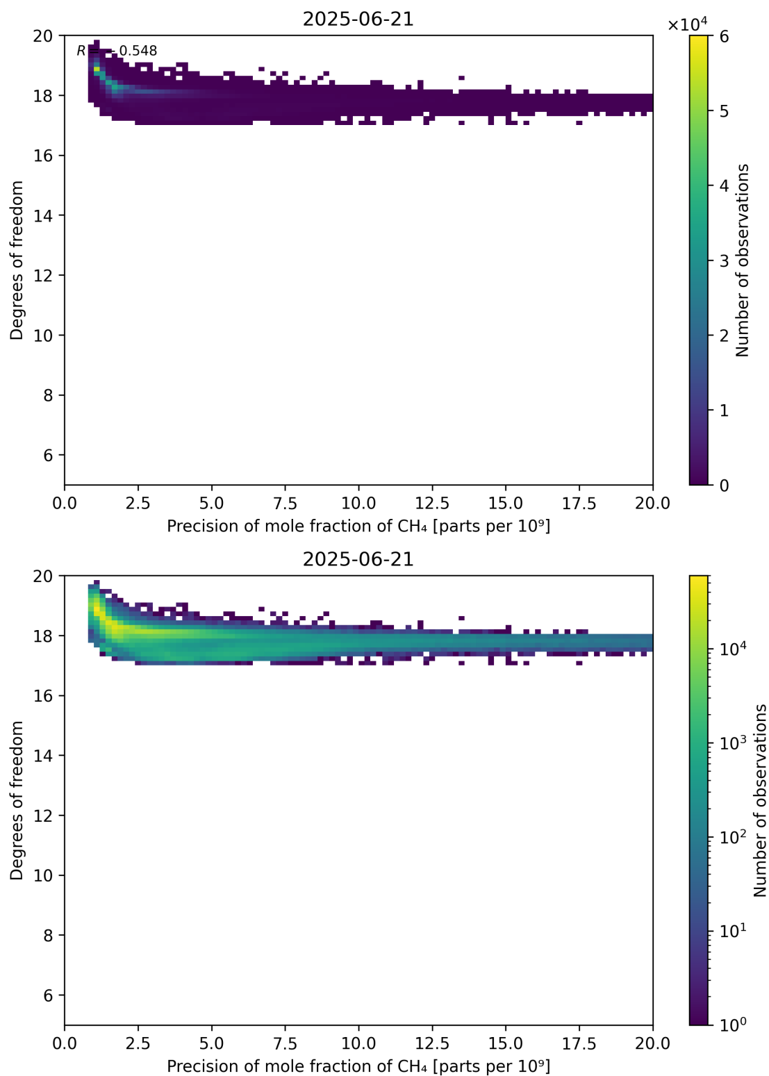
Figure 80: Scatter density plot of “Precision of mole fraction of CH 4 ” against “Degrees of freedom” for 2025-06-20 to 2025-06-22.
