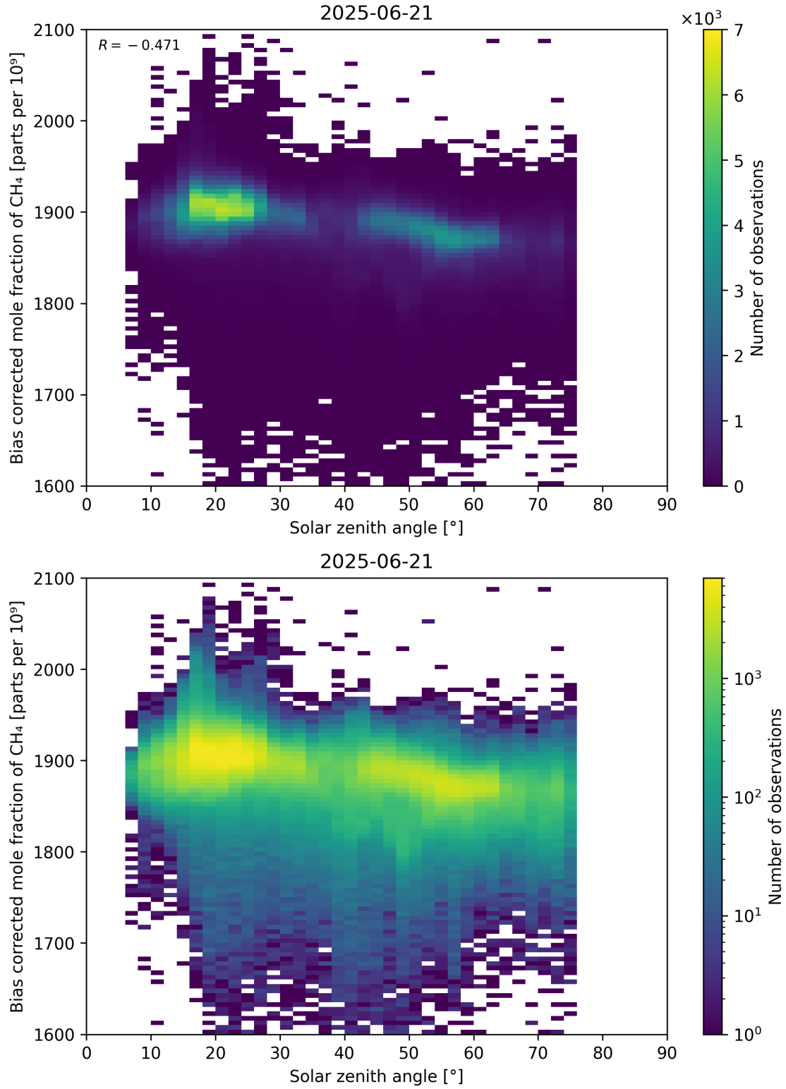
Figure 100: Scatter density plot of “Solar zenith angle” against “Bias corrected mole fraction of \text{CH}_4 ” for 2025-06-20 to 2025-06-22.
