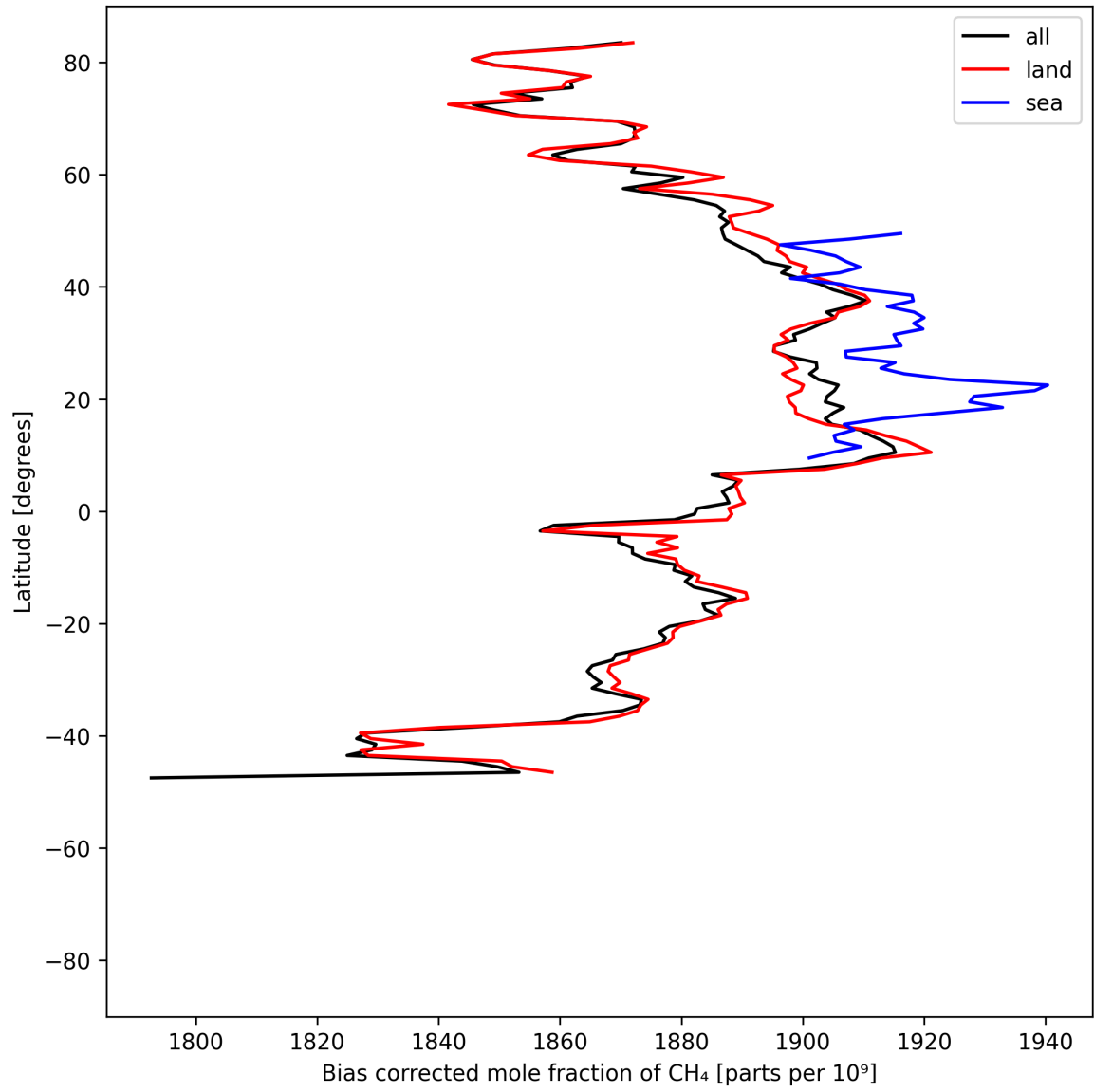
Figure 14: Zonal average of “Bias corrected mole fraction of CH 4 ” for 2025-06-20 to 2025-06-22.
