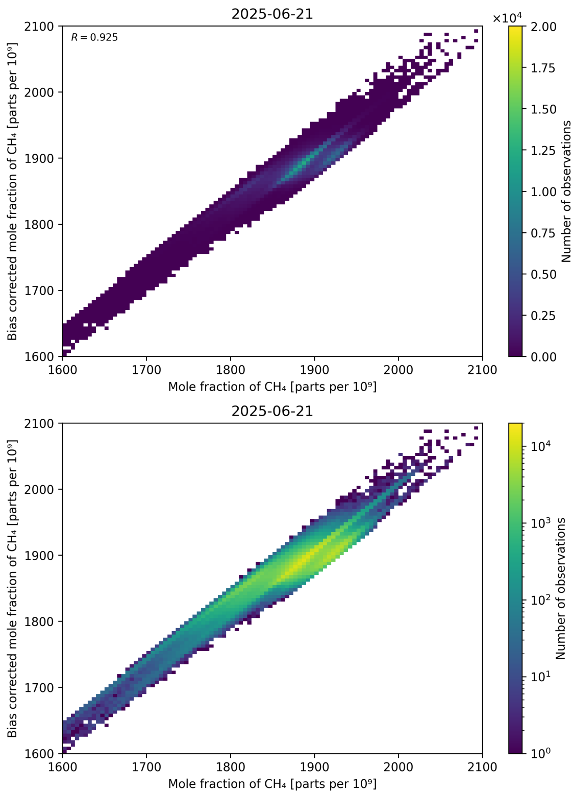
Figure 74: Scatter density plot of “Mole fraction of CH 4 ” against “Bias corrected mole fraction of CH 4 ” for 2025-06-20 to 2025-06-22.
