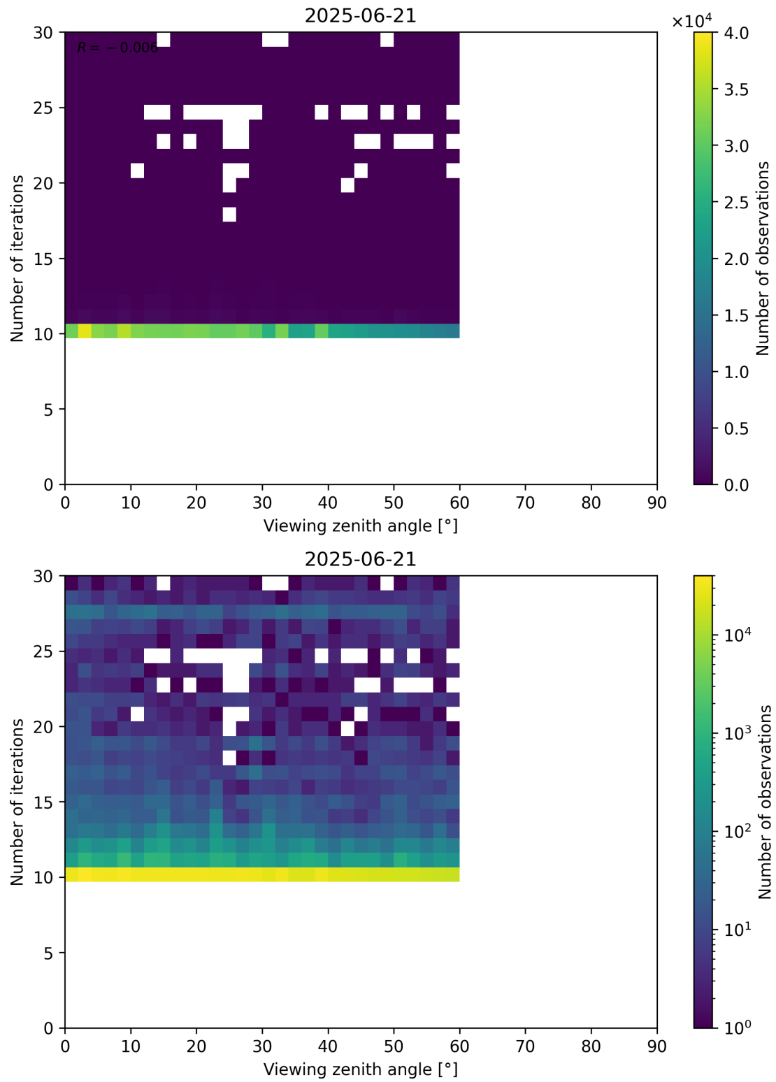
Figure 113: Scatter density plot of “Viewing zenith angle” against “Number of iterations” for 2025-06-20 to 2025-06-22.
