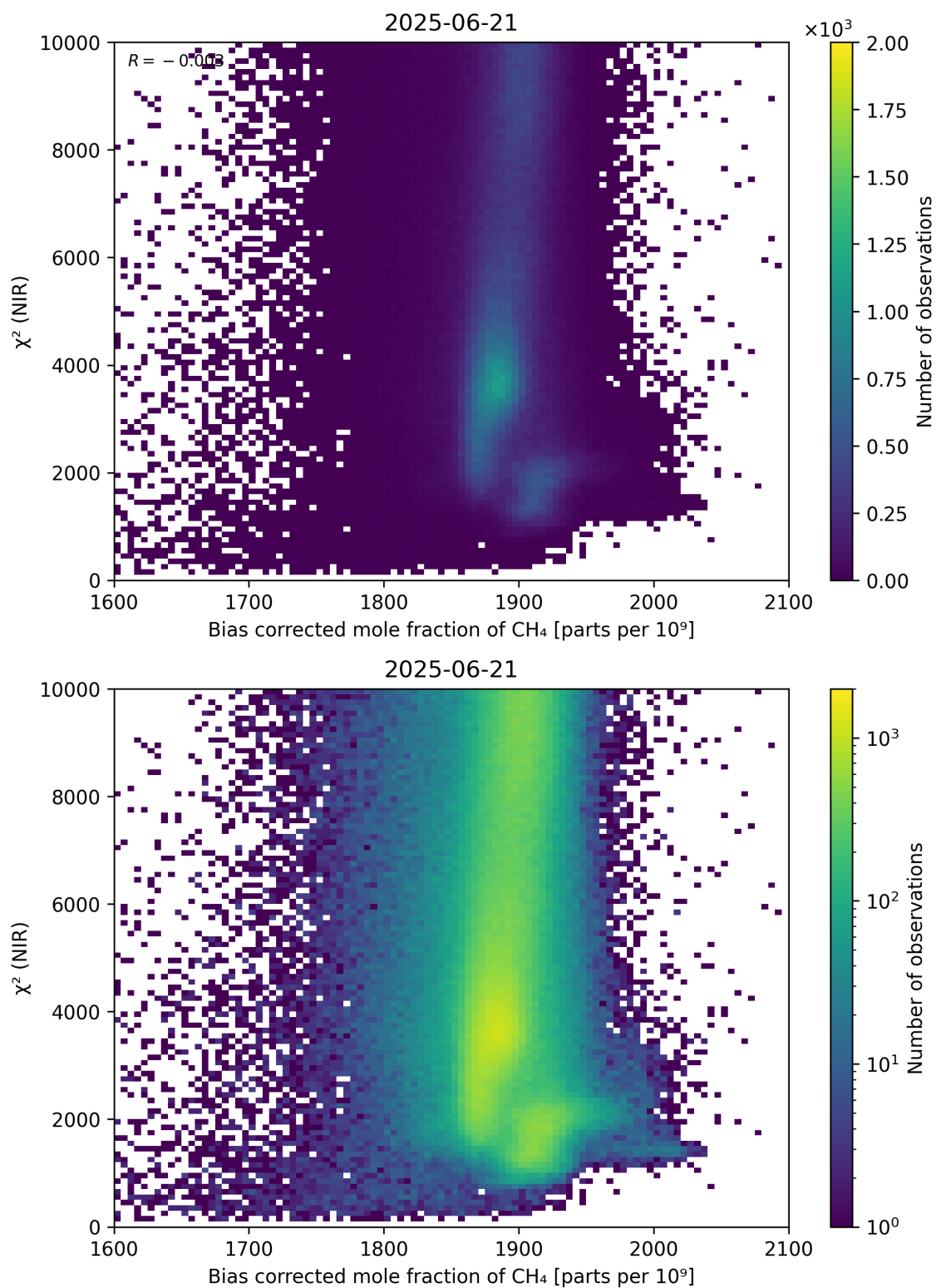
Figure 63: Scatter density plot of “Bias corrected mole fraction of CH 4 ” against “ \chi^2 (NIR)” for 2025-06-20 to 2025-06-22.
