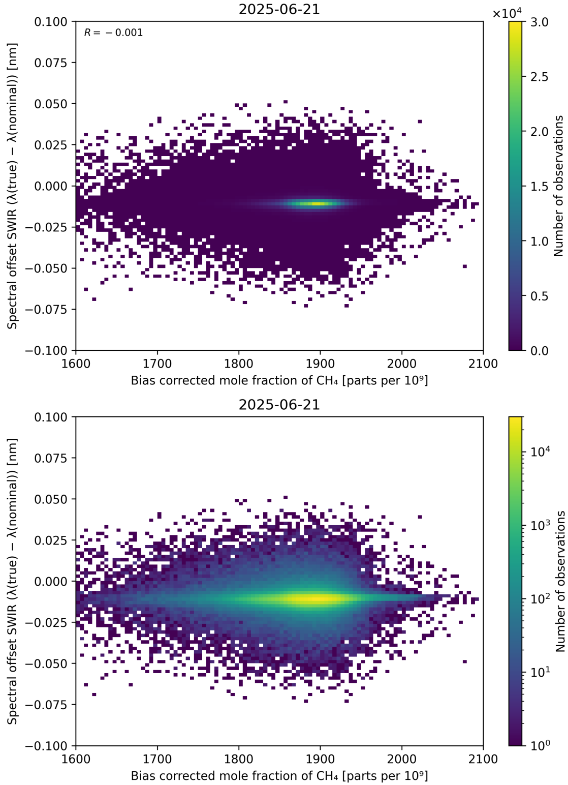
Figure 69: Scatter density plot of “Bias corrected mole fraction of \text{CH}_4 ” against “Spectral offset SWIR ( \lambda_{\text{true}} - \lambda_{\text{nominal}} )” for 2025-06-20 to 2025-06-22.
