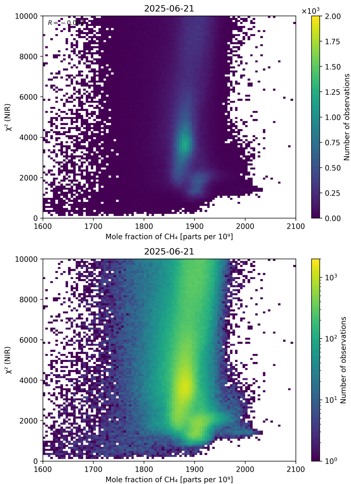
Figure 70: Scatter density plot of “Mole fraction of \text{CH}_4 ” against “ \chi^2 (NIR)” for 2025-06-20 to 2025-06-22.
