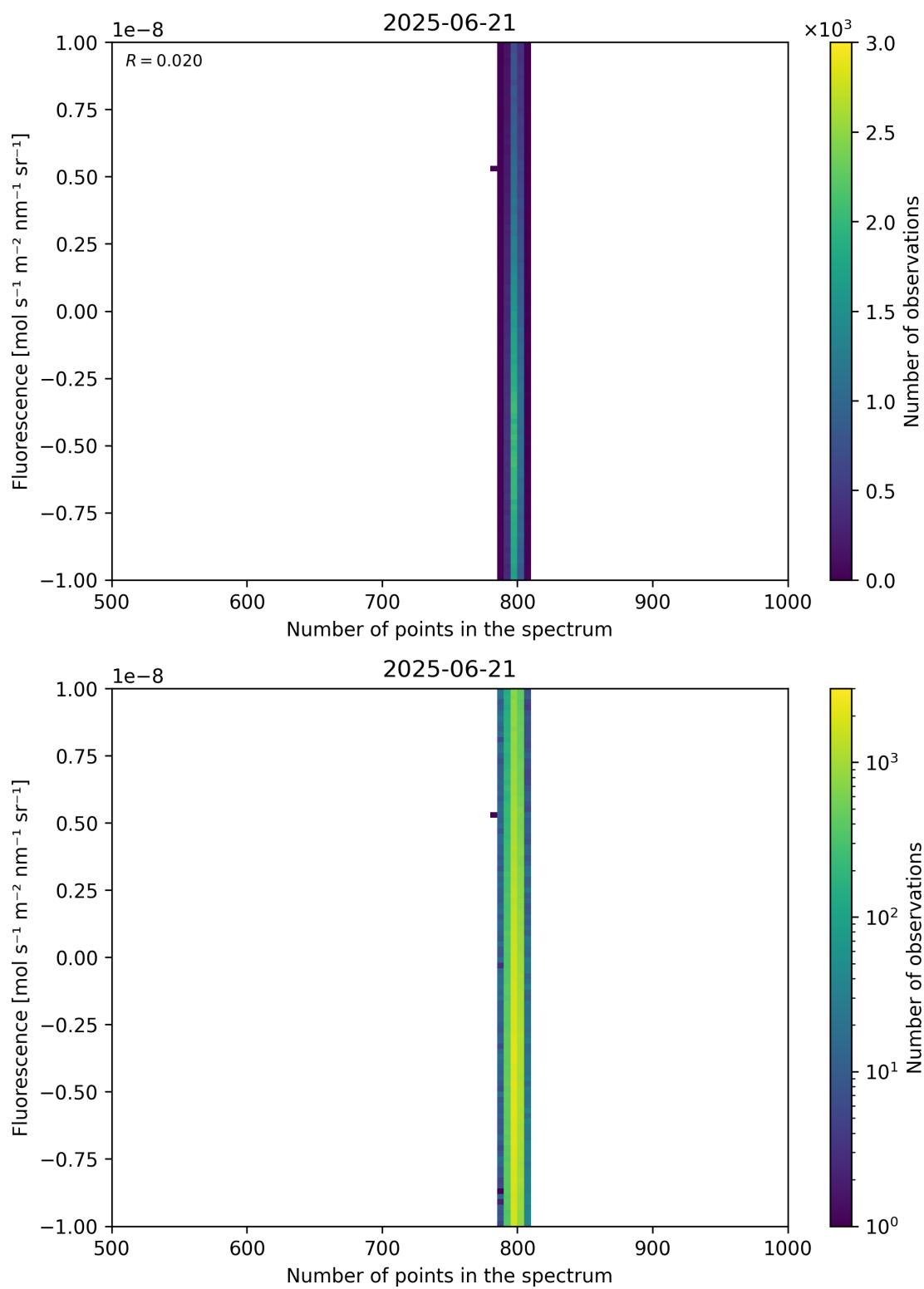
Figure 91: Scatter density plot of “Number of points in the spectrum” against “Fluorescence” for 2025-06-20 to 2025-06-22.
