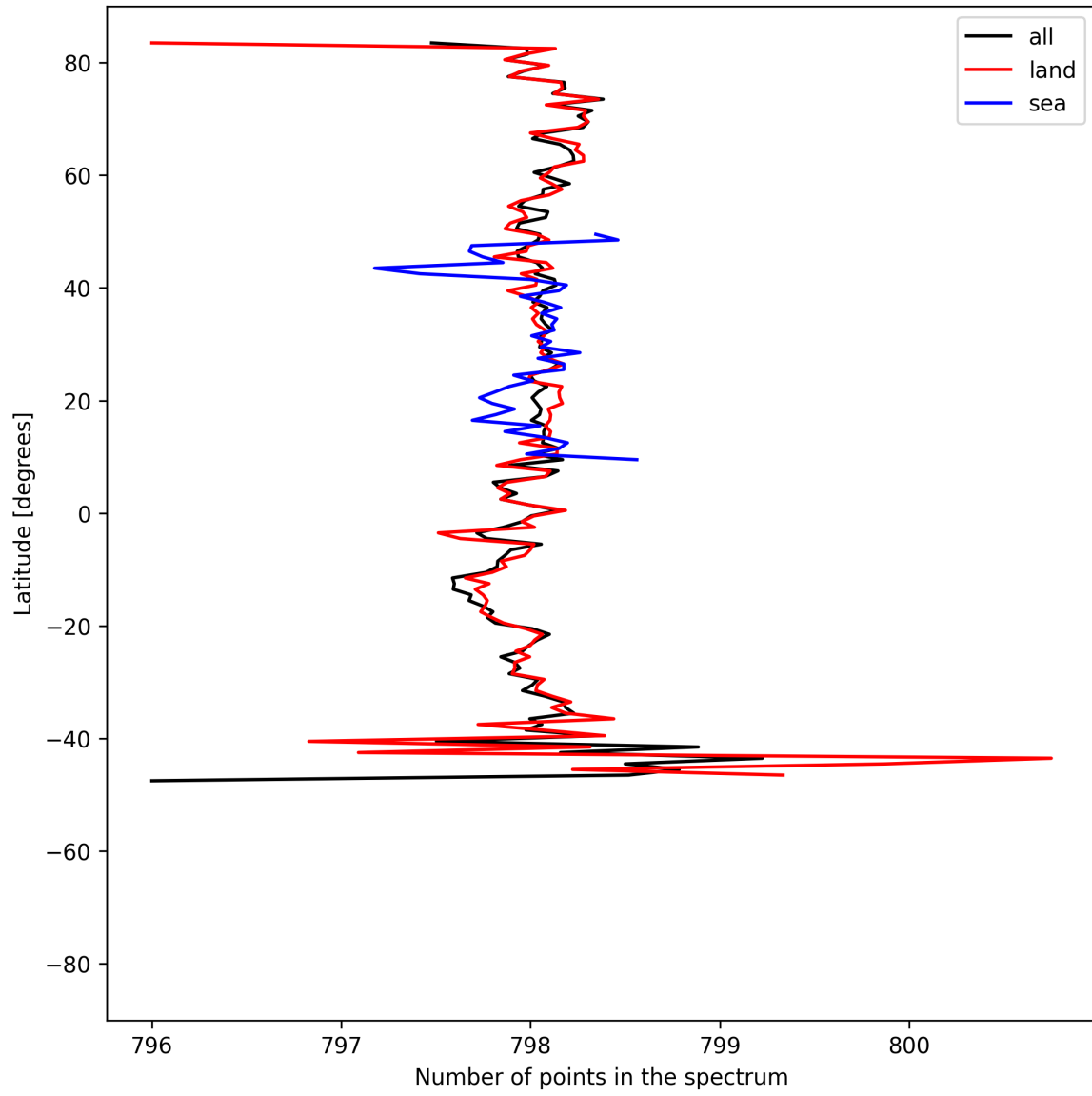
Figure 15: Zonal average of “Number of points in the spectrum” for 2025-06-20 to 2025-06-22.
