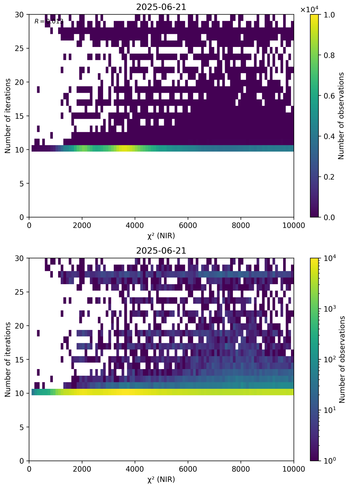
Figure 46: Scatter density plot of “ \chi^2 (NIR)” against “Number of iterations” for 2025-06-20 to 2025-06-22.
