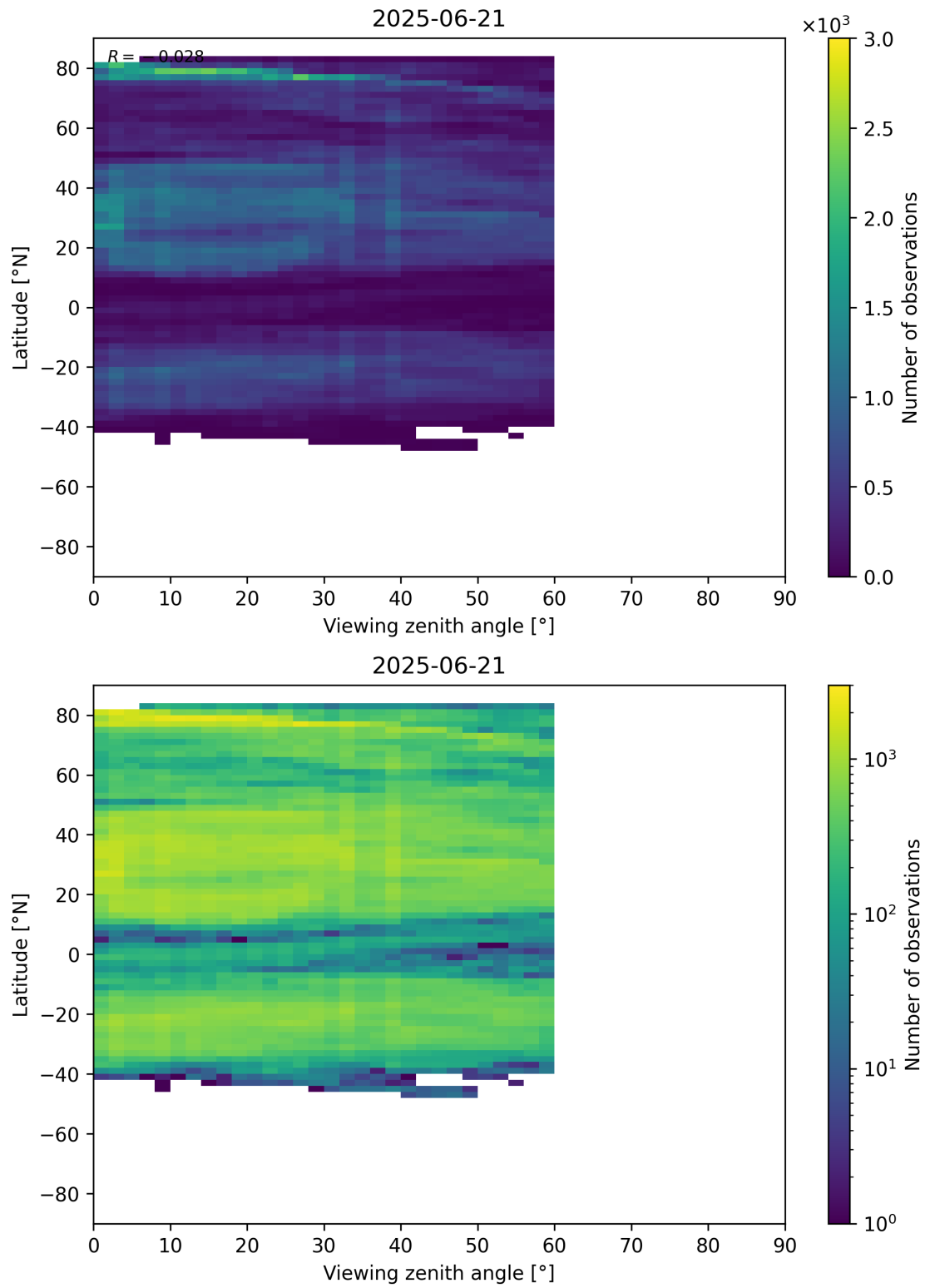
Figure 109: Scatter density plot of “Viewing zenith angle” against “Latitude” for 2025-06-20 to 2025-06-22.
