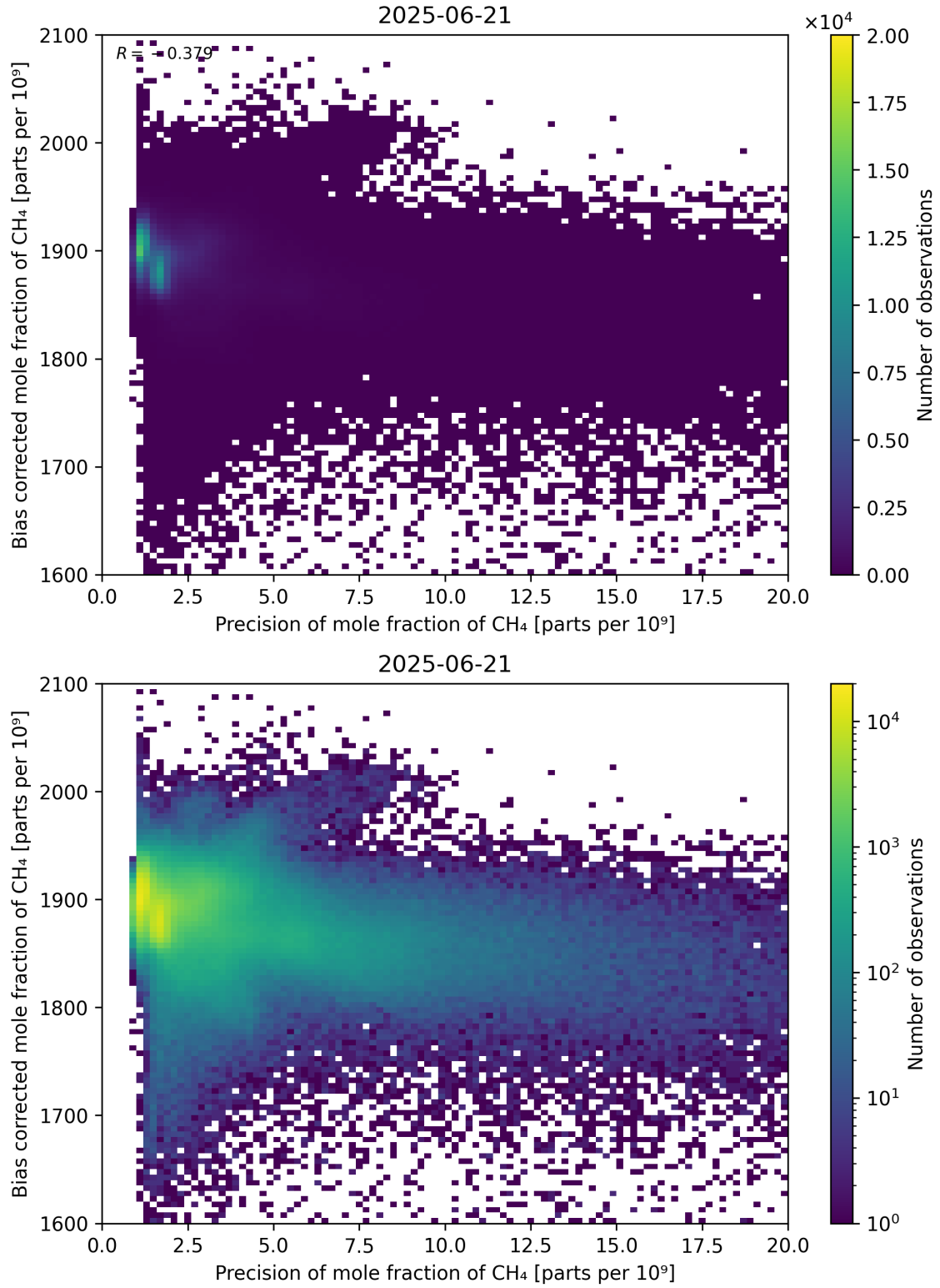
Figure 82: Scatter density plot of “Precision of mole fraction of CH 4 ” against “Bias corrected mole fraction of CH 4 ” for 2025-06-20 to 2025-06-22.
