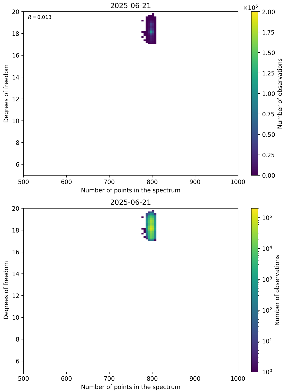
Figure 90: Scatter density plot of “Number of points in the spectrum” against “Degrees of freedom” for 2025-06-20 to 2025-06-22.
