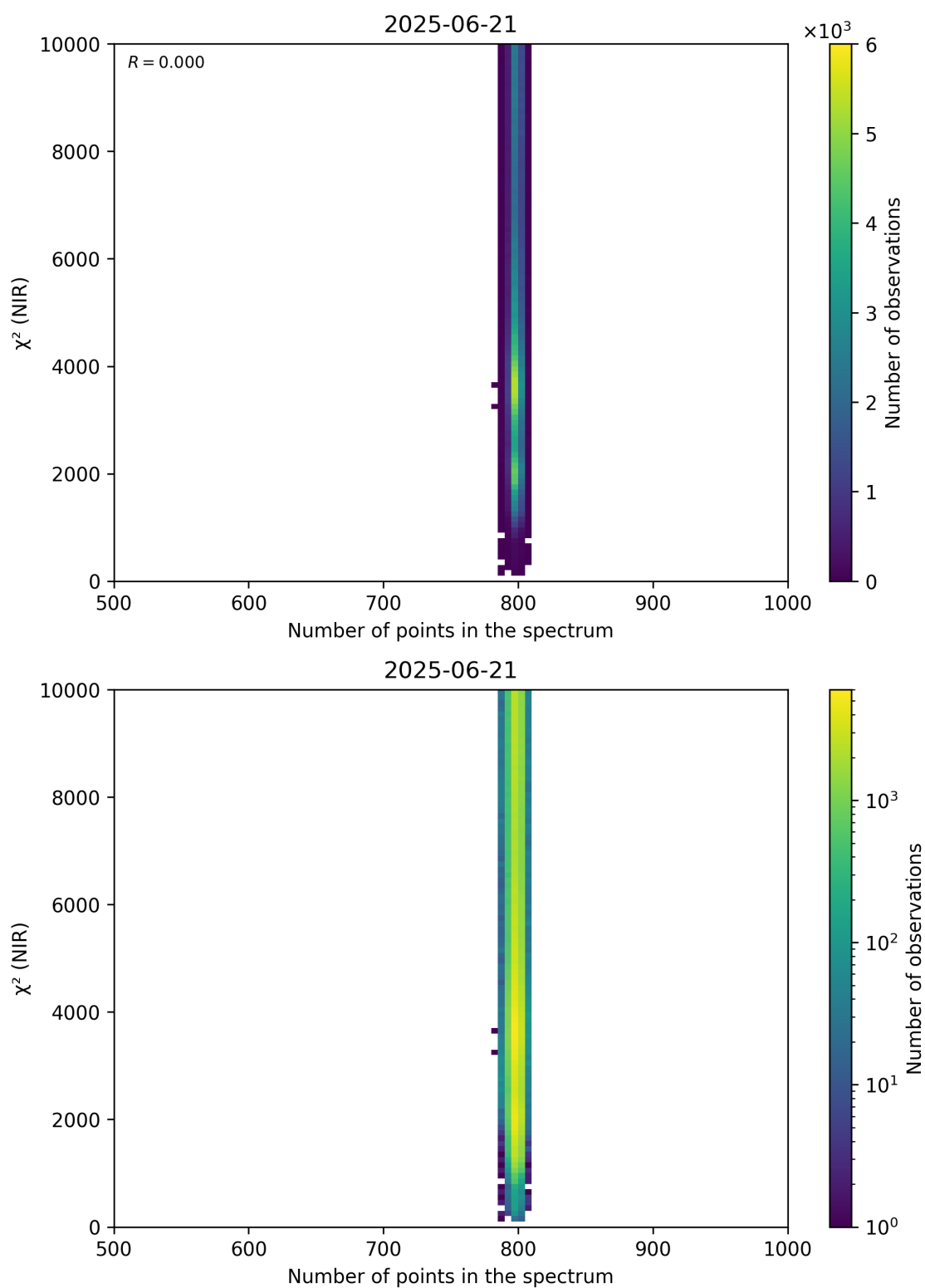
Figure 88: Scatter density plot of “Number of points in the spectrum” against “ \chi^2 (NIR)” for 2025-06-20 to 2025-06-22.
