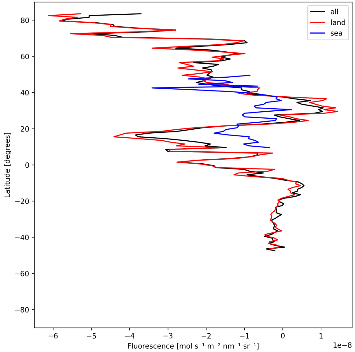
Figure 21: Zonal average of “Fluorescence” for 2025-06-20 to 2025-06-22.
