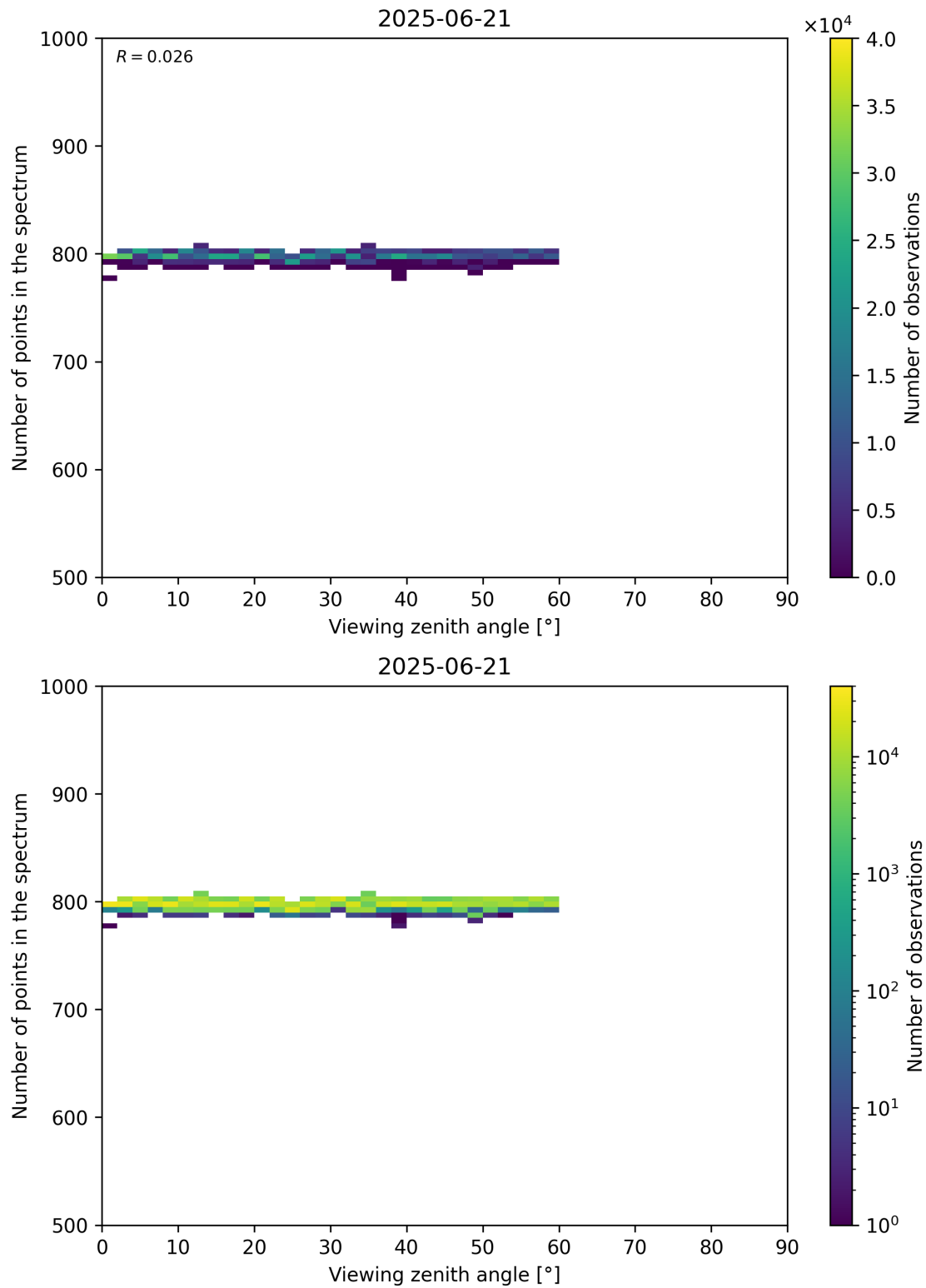
Figure 114: Scatter density plot of “Viewing zenith angle” against “Number of points in the spectrum” for 2025-06-20 to 2025-06-22.
