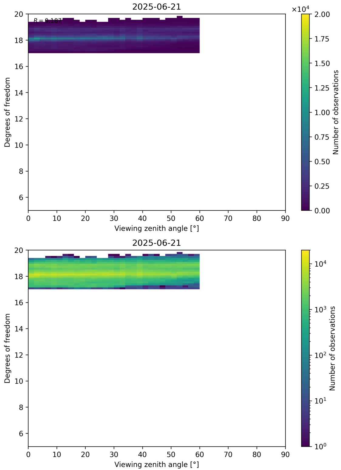
Figure 107: Scatter density plot of “Viewing zenith angle” against “Degrees of freedom” for 2025-06-20 to 2025-06-22.
