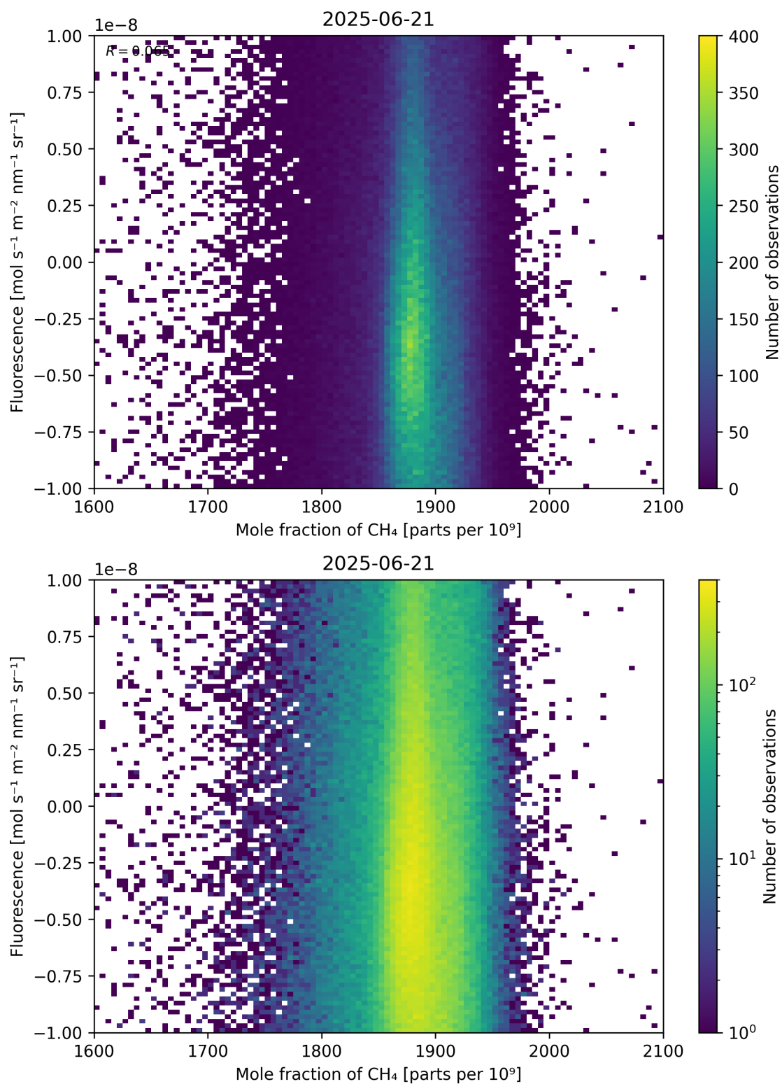
Figure 73: Scatter density plot of “Mole fraction of \text{CH}_4 ” against “Fluorescence” for 2025-06-20 to 2025-06-22.
