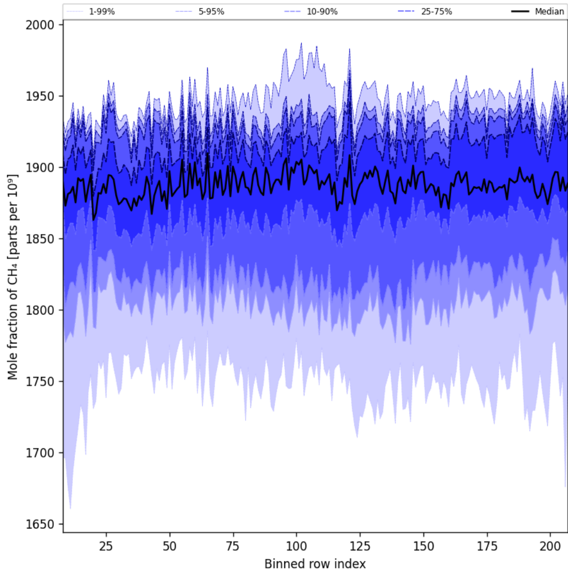
Figure 34: Along track statistics of “Mole fraction of CH 4 ” for 2025-06-20 to 2025-06-22
