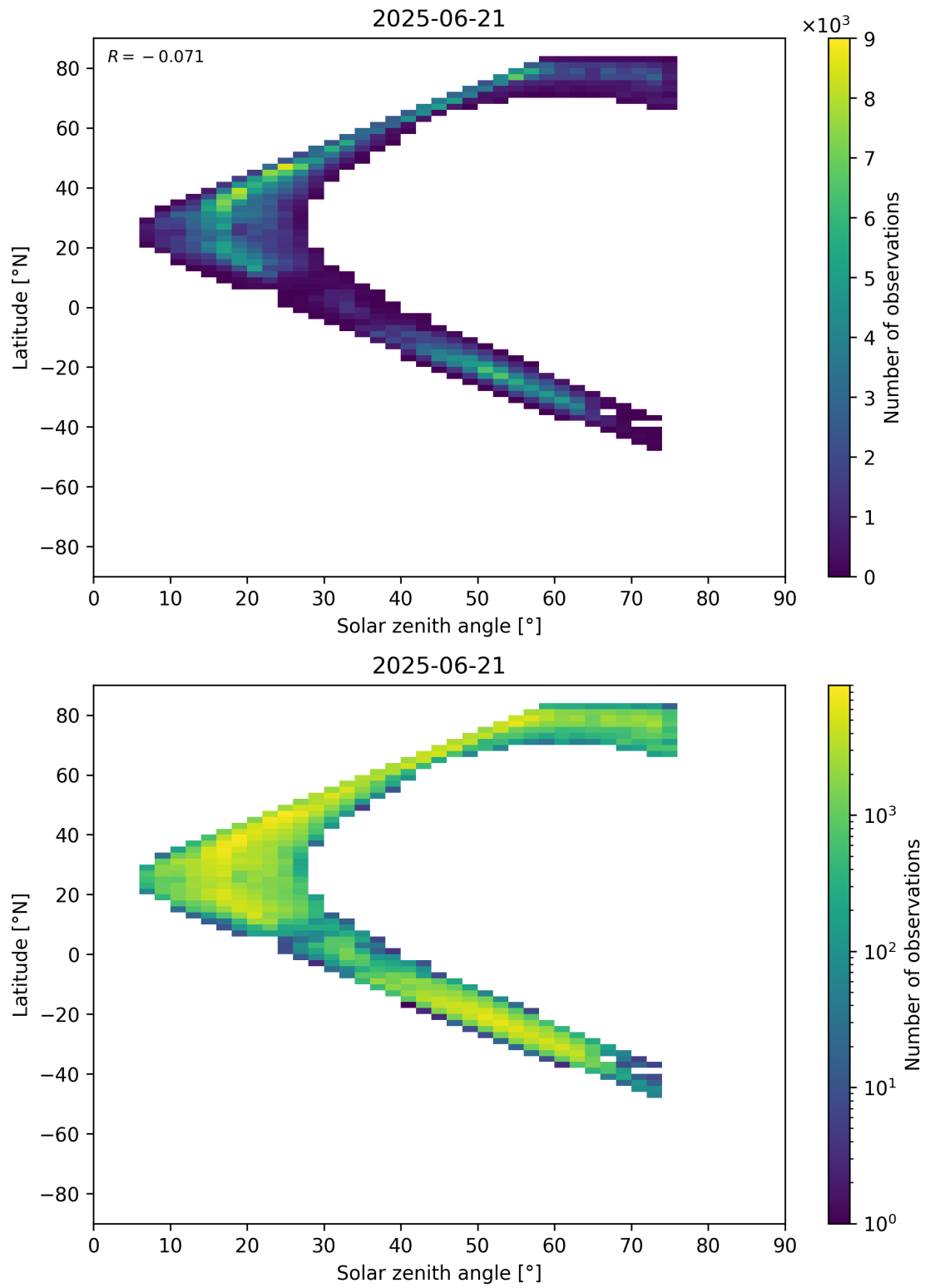
Figure 98: Scatter density plot of “Solar zenith angle” against “Latitude” for 2025-06-20 to 2025-06-22.
