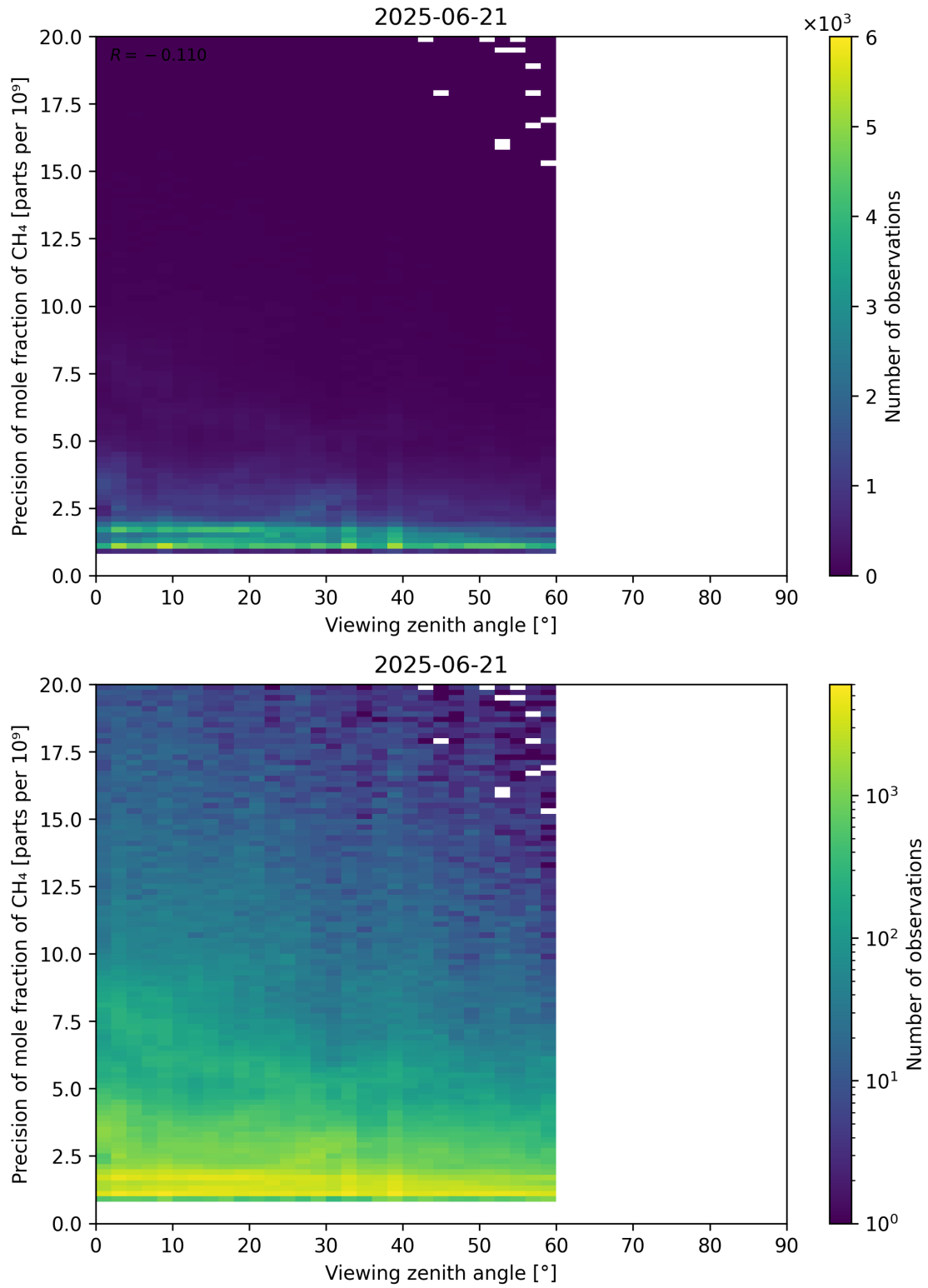
Figure 112: Scatter density plot of “Viewing zenith angle” against “Precision of mole fraction of CH 4 ” for 2025-06-20 to 2025-06-22.
