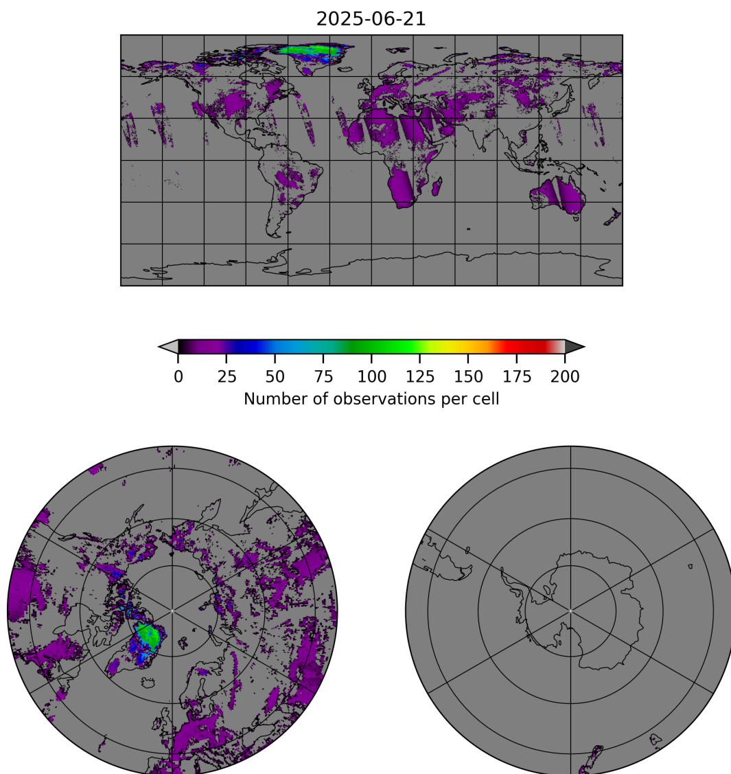
Figure 10: Map of the number of observations for 2025-06-20 to 2025-06-22
