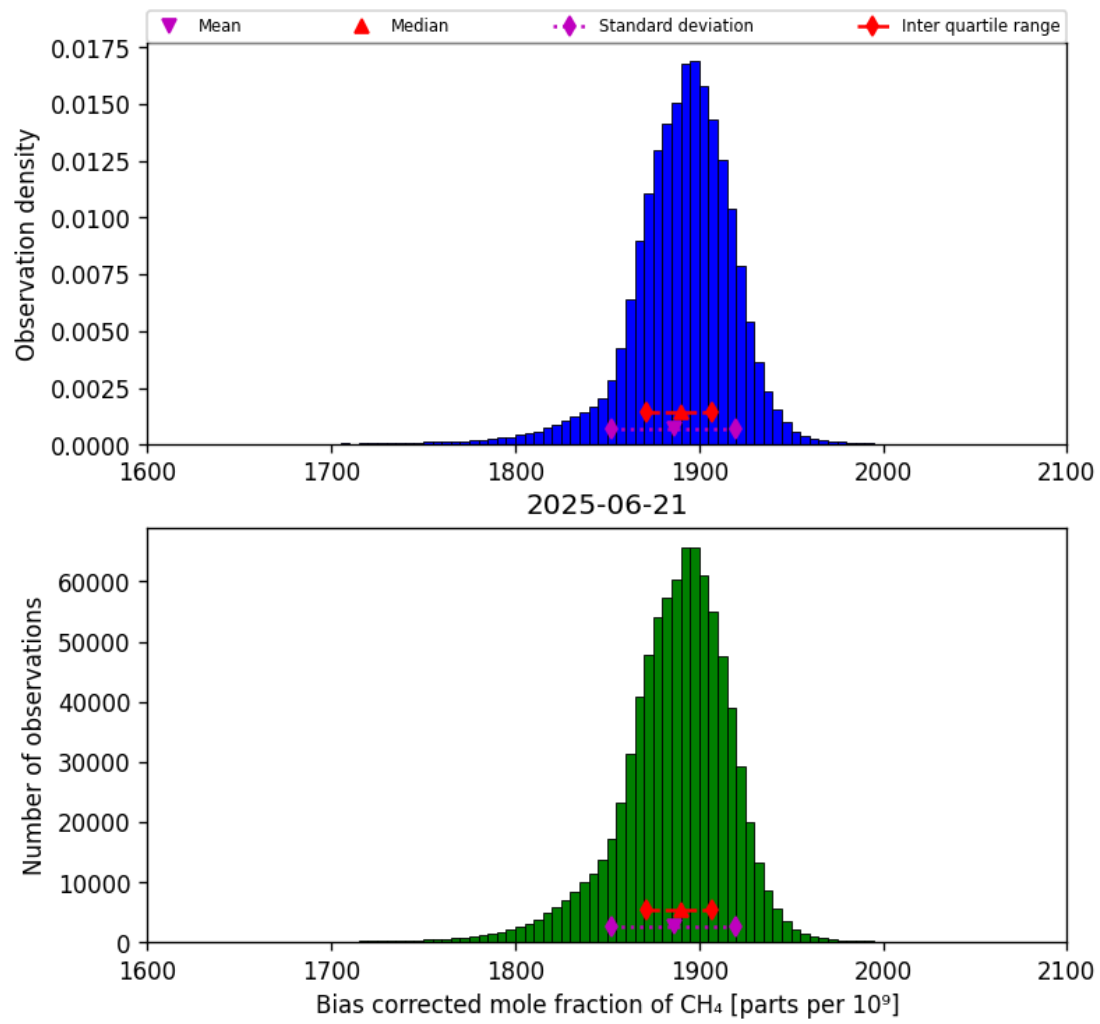
Figure 25: Histogram of “Bias corrected mole fraction of CH 4 ” for 2025-06-20 to 2025-06-22
