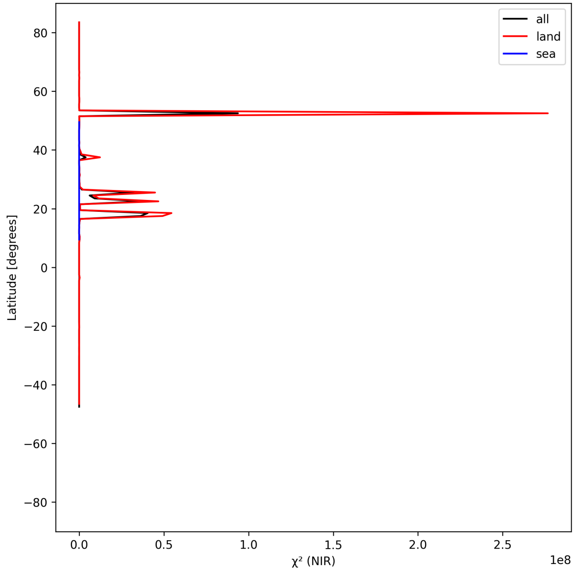
Figure 18: Zonal average of “ \chi^2 (NIR)” for 2025-06-20 to 2025-06-22.
