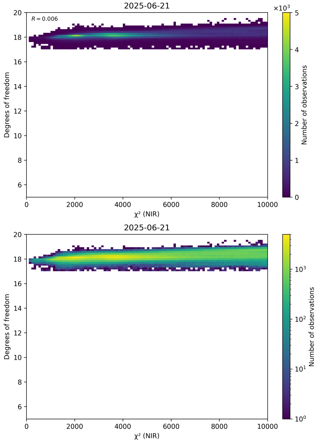
Figure 44: Scatter density plot of “ \chi^2 (NIR)” against “Degrees of freedom” for 2025-06-20 to 2025-06-22.
