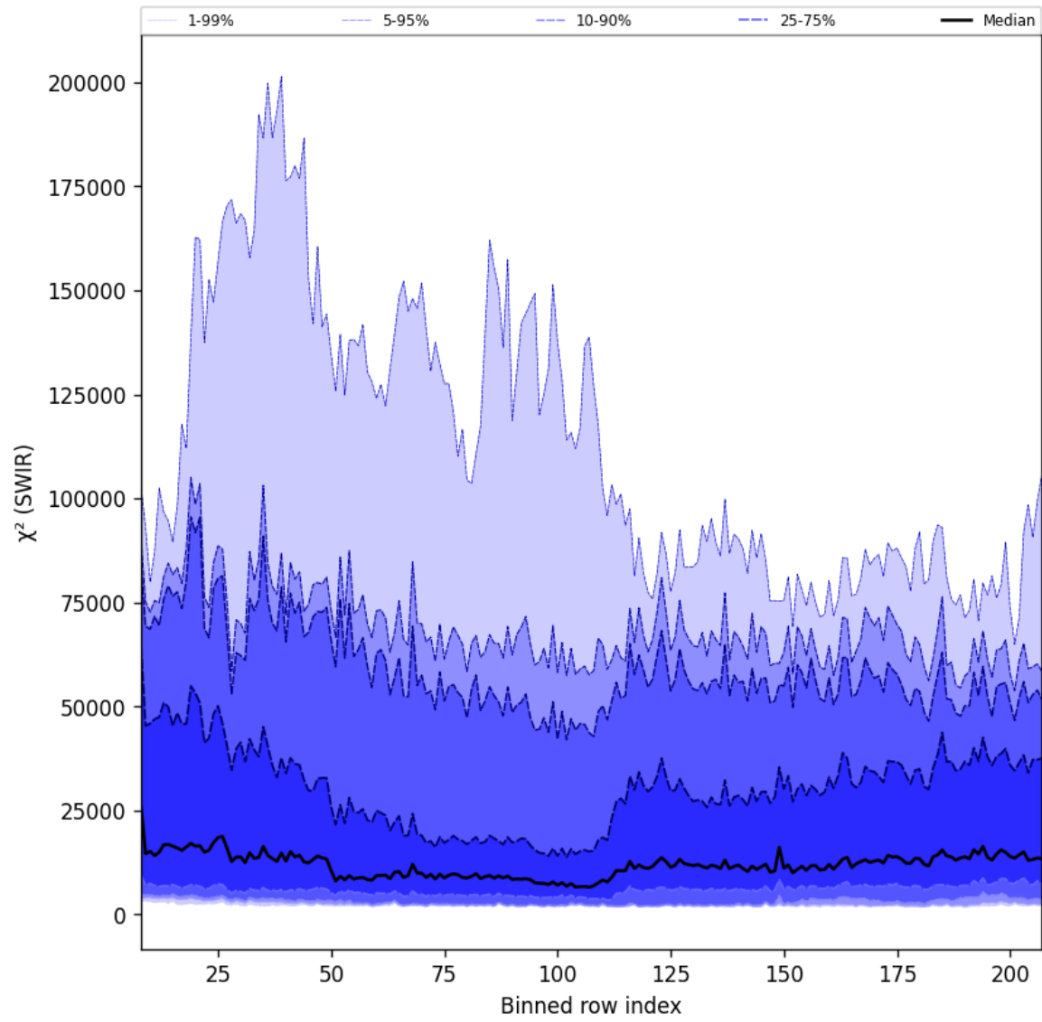
Figure 39: Along track statistics of “ \chi^2 (SWIR)” for 2025-06-20 to 2025-06-22
