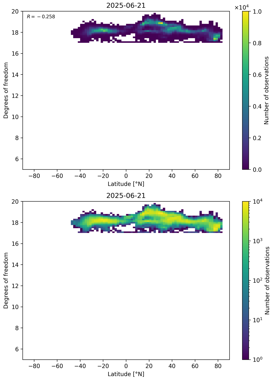
Figure 55: Scatter density plot of “Latitude” against “Degrees of freedom” for 2025-06-20 to 2025-06-22.
