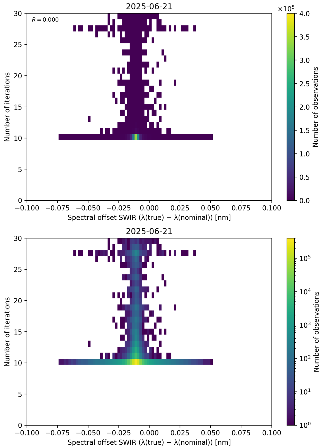
Figure 121: Scatter density plot of “Spectral offset SWIR ( \lambda_{\text{true}} - \lambda_{\text{nominal}} )” against “Number of iterations” for 2025-06-20 to 2025-06-22.
