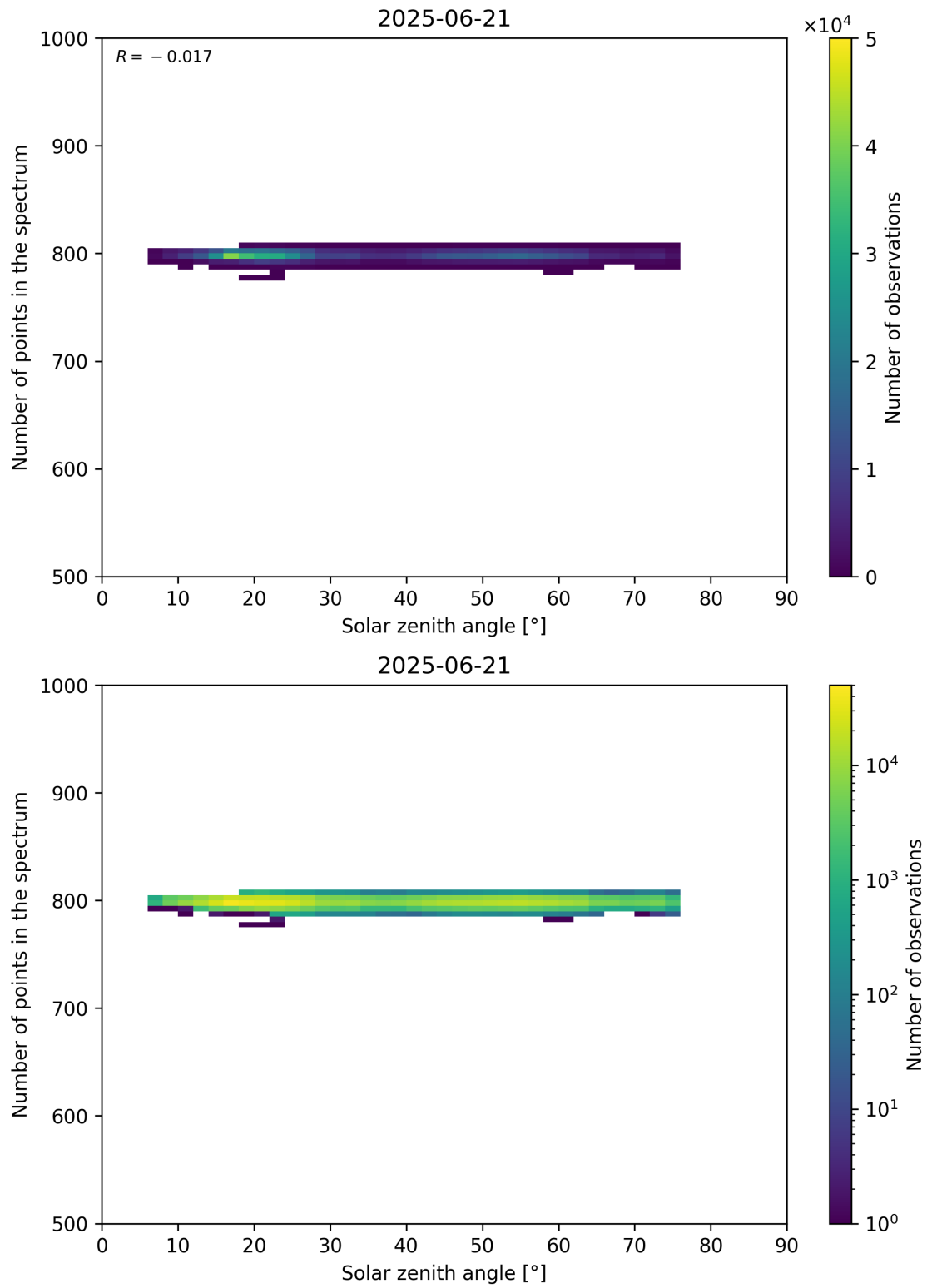
Figure 103: Scatter density plot of “Solar zenith angle” against “Number of points in the spectrum” for 2025-06-20 to 2025-06-22.
