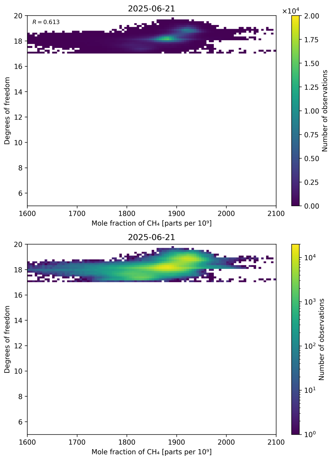
Figure 72: Scatter density plot of “Mole fraction of CH 4 ” against “Degrees of freedom” for 2025-06-20 to 2025-06-22.
