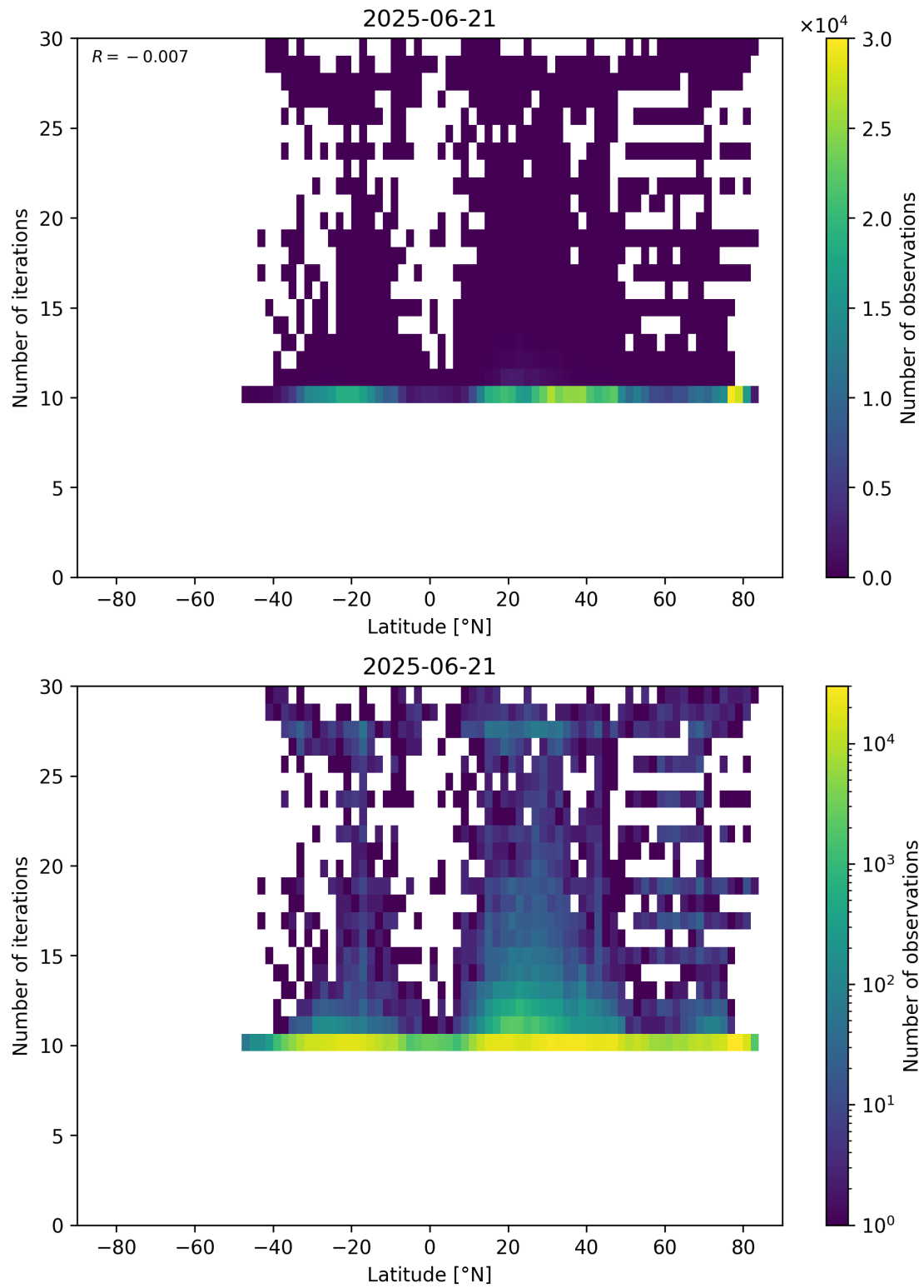
Figure 60: Scatter density plot of “Latitude” against “Number of iterations” for 2025-06-20 to 2025-06-22.
