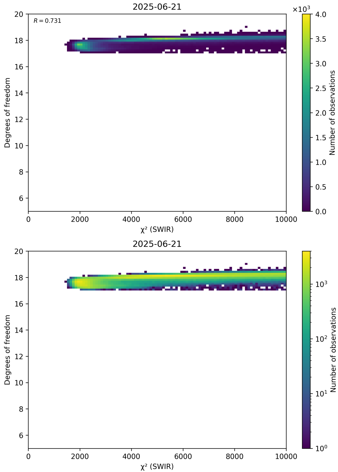
Figure 48: Scatter density plot of “ \chi^2 (SWIR)” against “Degrees of freedom” for 2025-06-20 to 2025-06-22.
