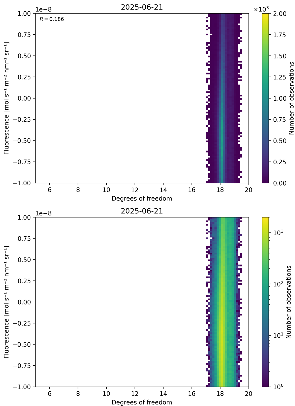
Figure 51: Scatter density plot of “Degrees of freedom” against “Fluorescence” for 2025-06-20 to 2025-06-22.
