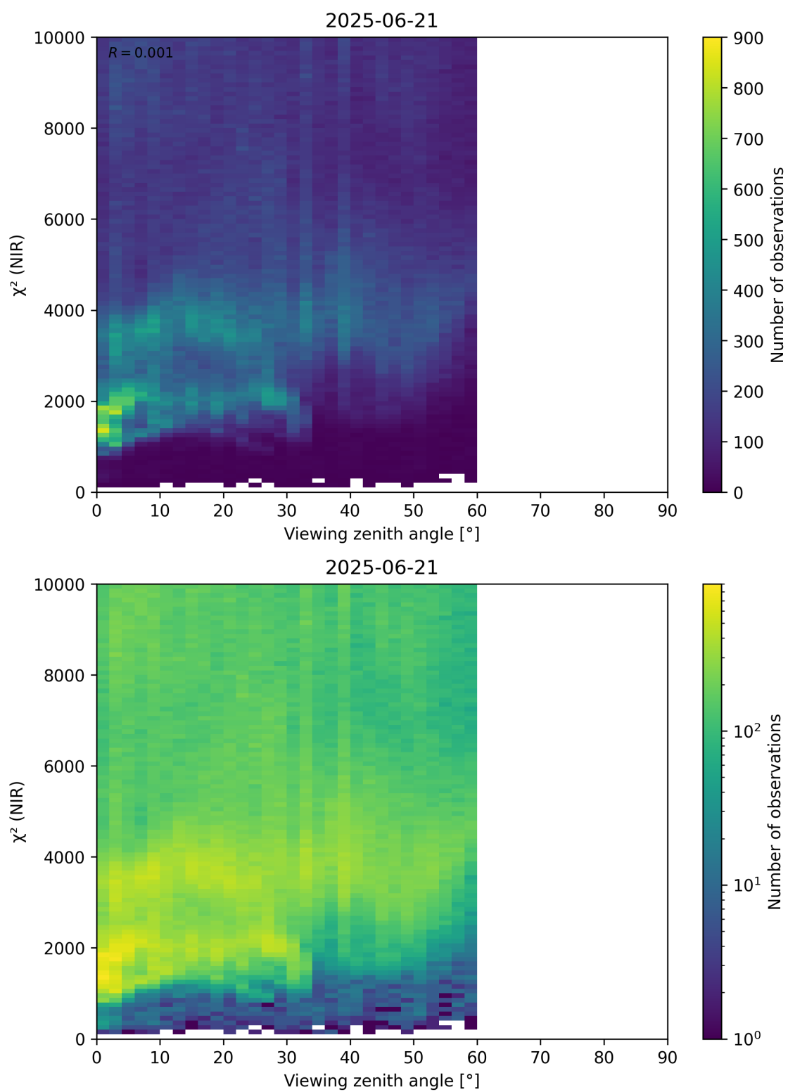
Figure 105: Scatter density plot of “Viewing zenith angle” against “ \chi^2 (NIR)” for 2025-06-20 to 2025-06-22.
