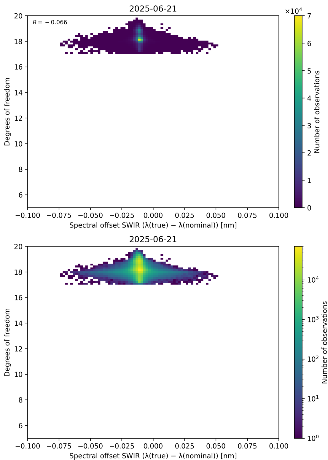
Figure 119: Scatter density plot of “Spectral offset SWIR ( \lambda_{\text{true}} - \lambda_{\text{nominal}} )” against “Degrees of freedom” for 2025-06-20 to 2025-06-22.
