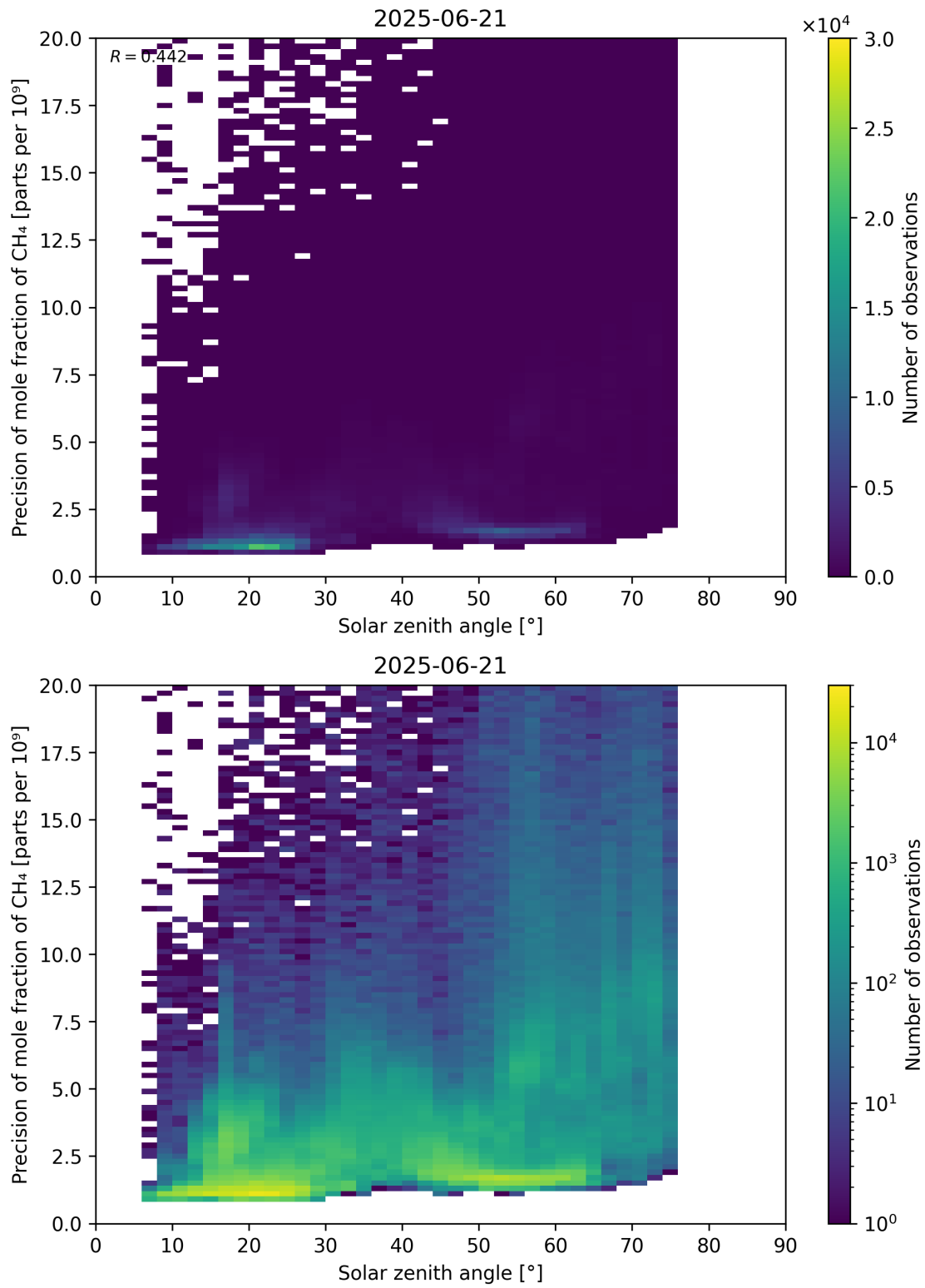
Figure 101: Scatter density plot of “Solar zenith angle” against “Precision of mole fraction of \text{CH}_4 ” for 2025-06-20 to 2025-06-22.
