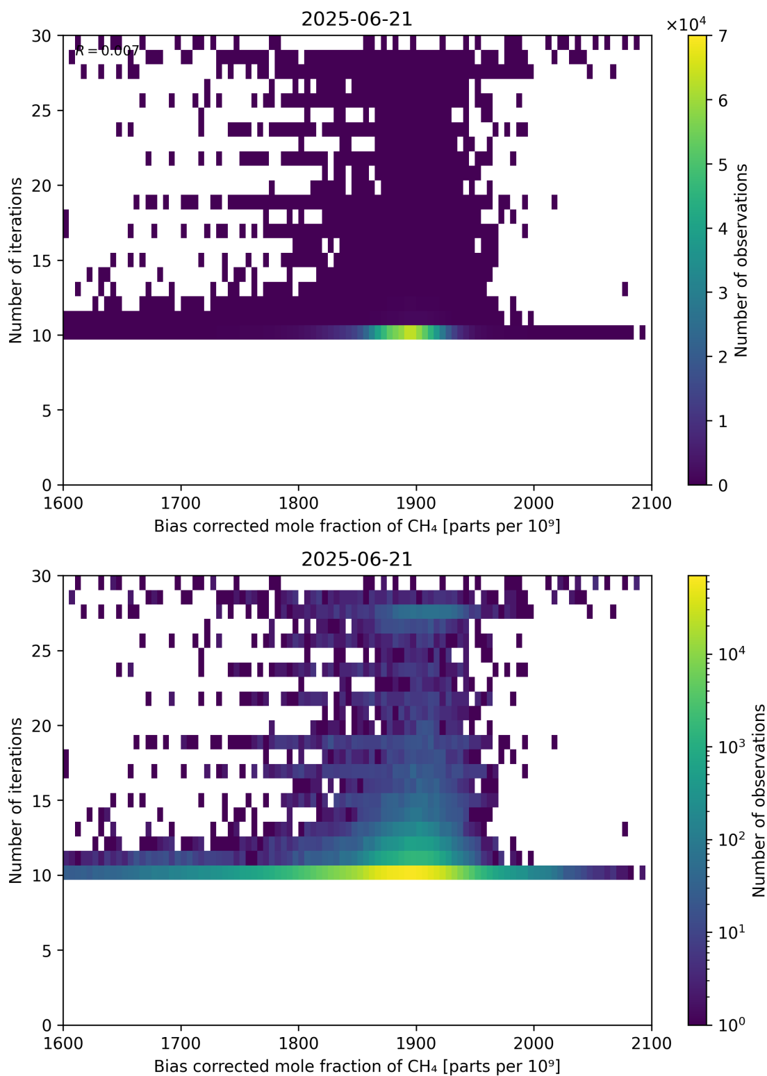
Figure 67: Scatter density plot of “Bias corrected mole fraction of \text{CH}_4 ” against “Number of iterations” for 2025-06-20 to 2025-06-22.
