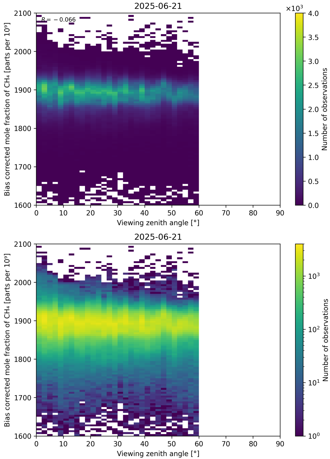
Figure 111: Scatter density plot of “Viewing zenith angle” against “Bias corrected mole fraction of CH 4 ” for 2025-06-20 to 2025-06-22.
