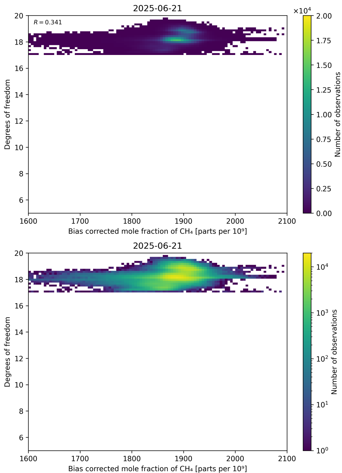
Figure 65: Scatter density plot of “Bias corrected mole fraction of CH 4 ” against “Degrees of freedom” for 2025-06-20 to 2025-06-22.
