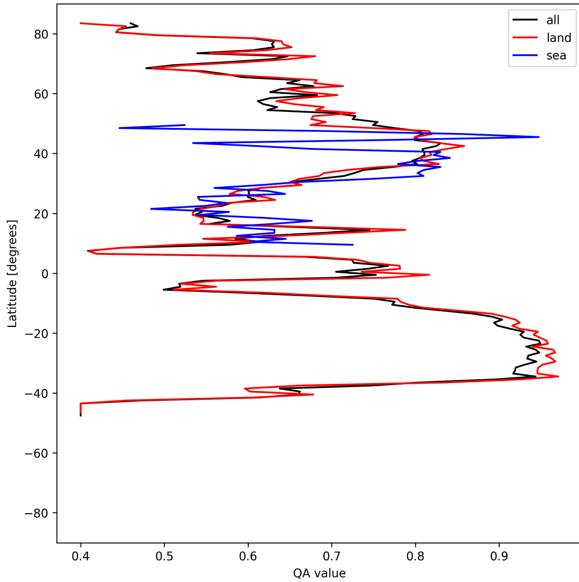
Figure 11: Zonal average of “QA value” for 2025-06-20 to 2025-06-22.
