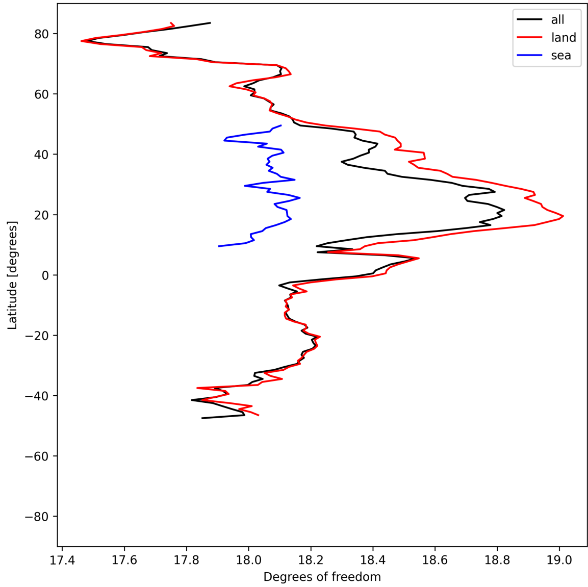
Figure 19: Zonal average of “Degrees of freedom” for 2025-06-20 to 2025-06-22.
