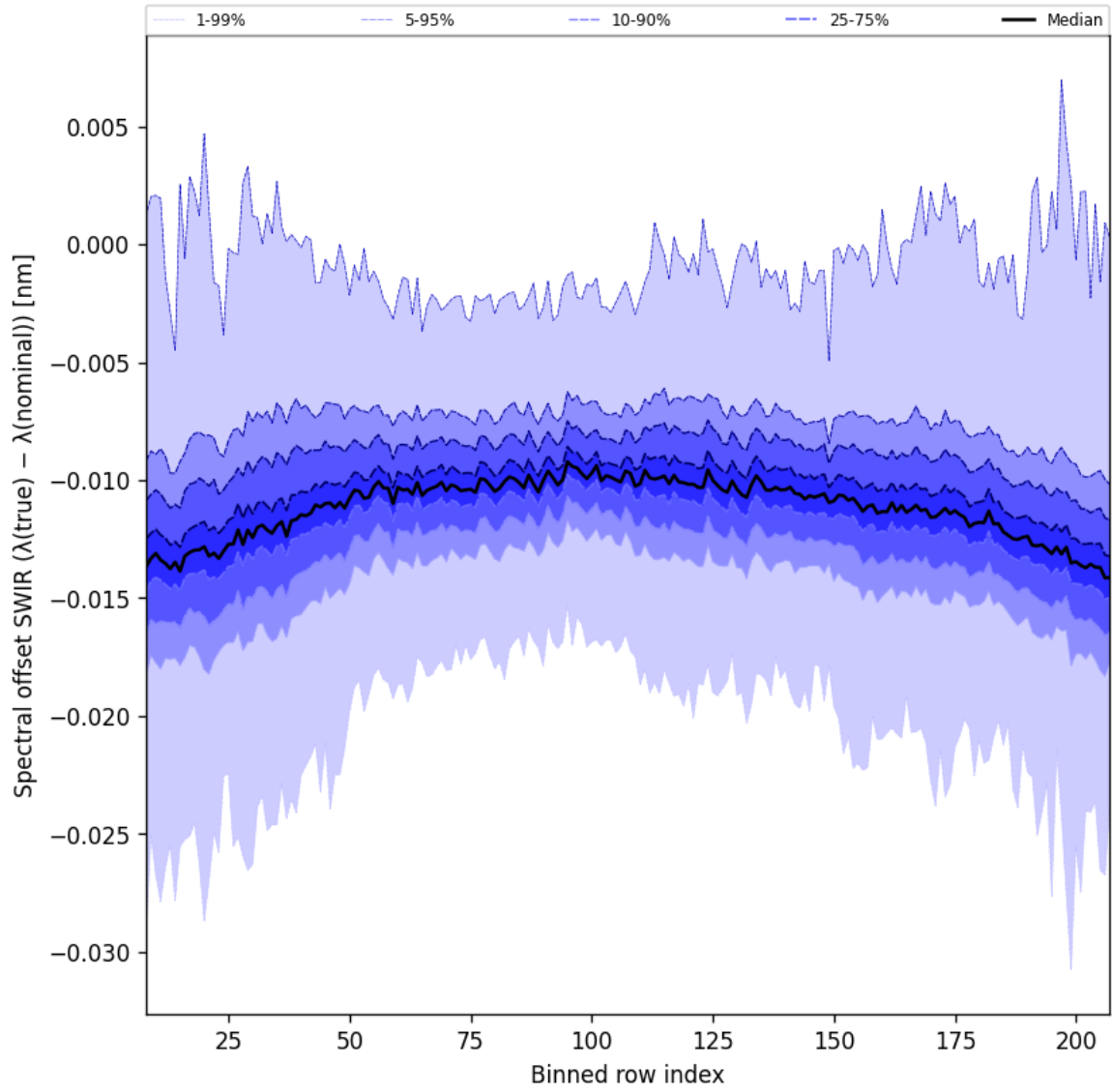
Figure 38: Along track statistics of “Spectral offset SWIR ( \lambda_{\text{true}} - \lambda_{\text{nominal}} )” for 2025-06-20 to 2025-06-22
