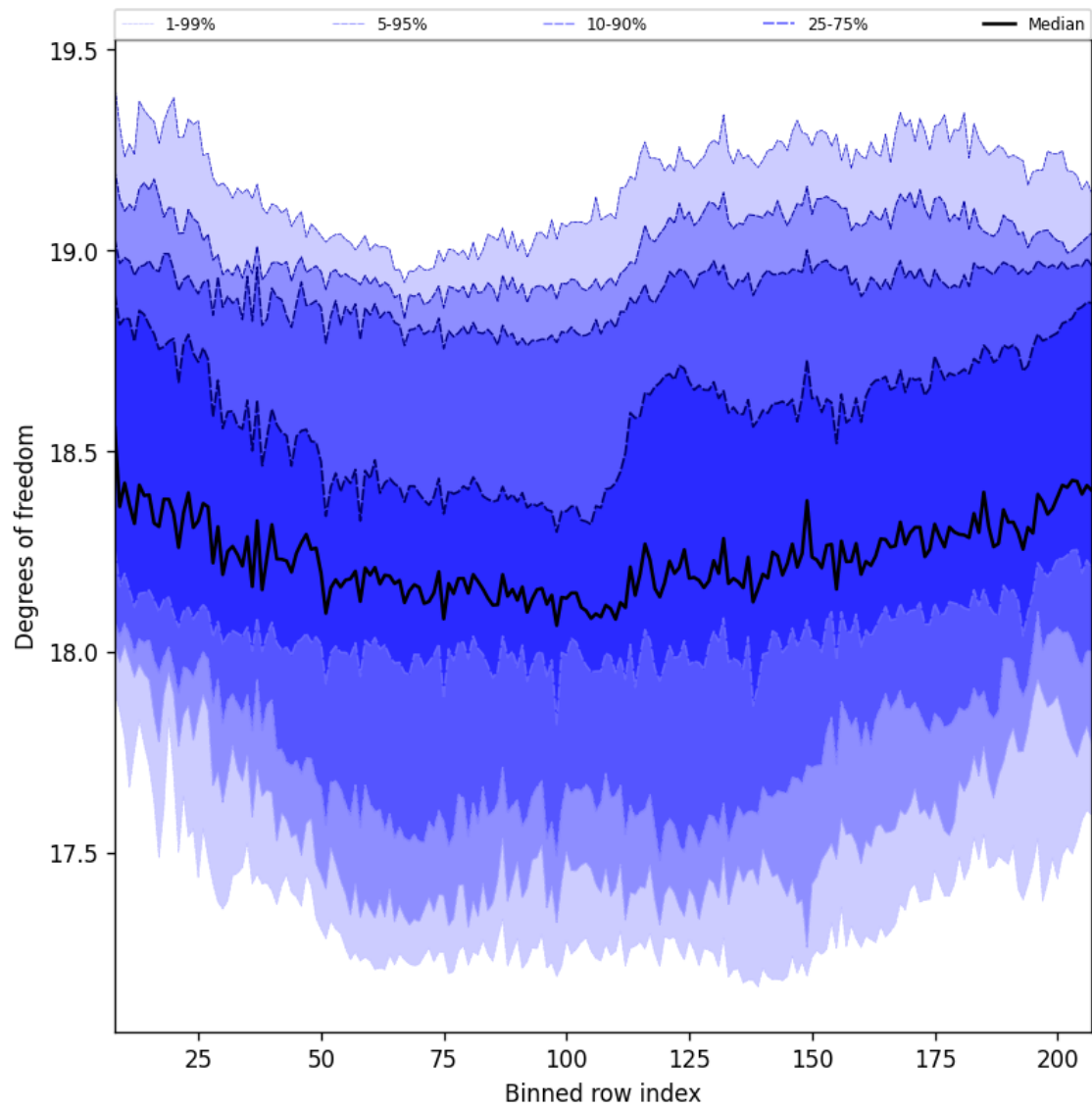
Figure 41: Along track statistics of “Degrees of freedom” for 2025-06-20 to 2025-06-22
