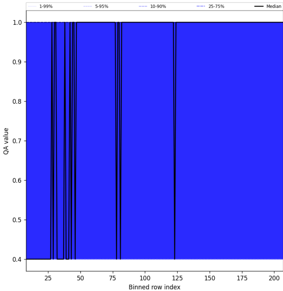
Figure 33: Along track statistics of “QA value” for 2025-06-20 to 2025-06-22
