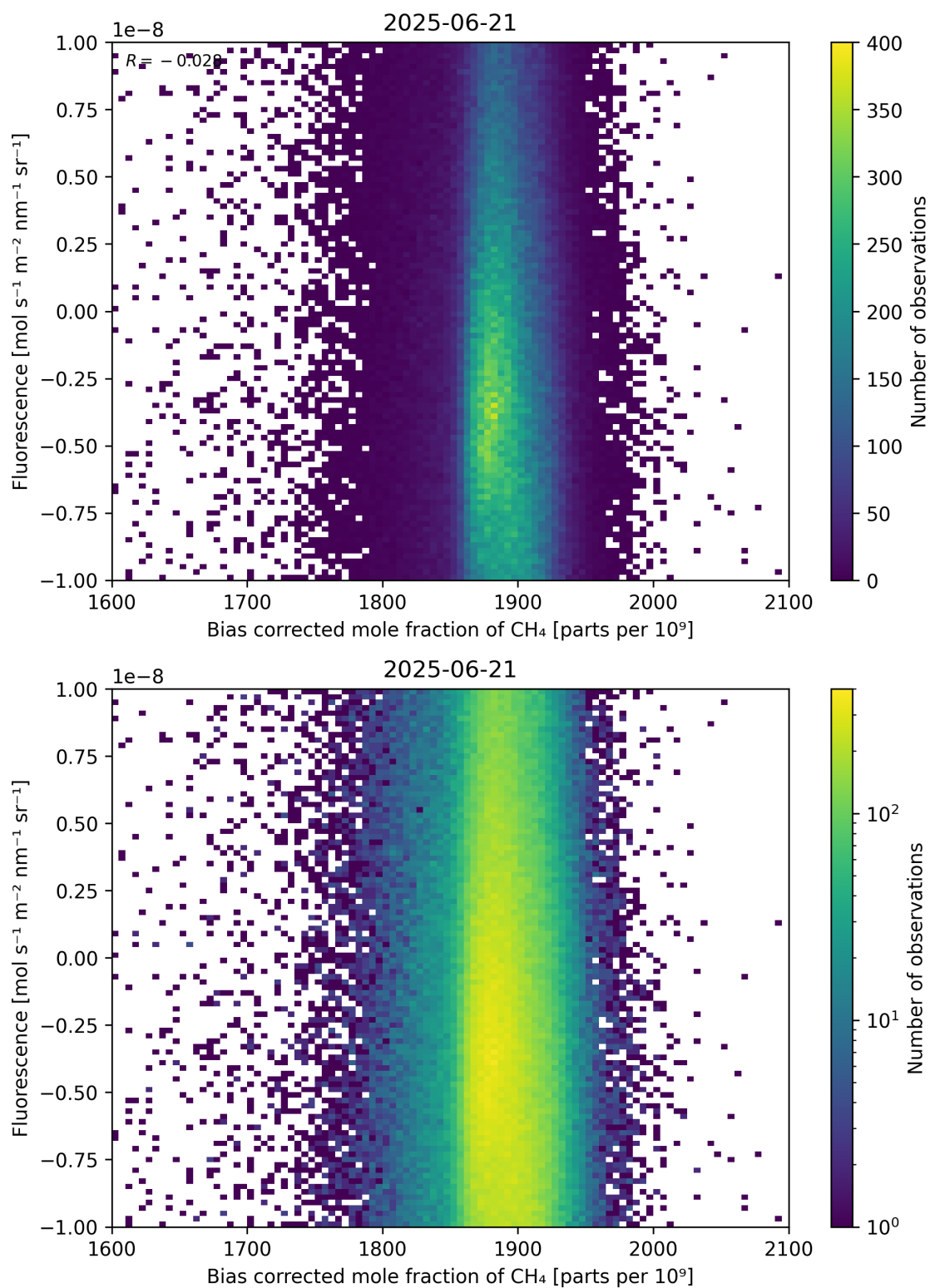
Figure 66: Scatter density plot of “Bias corrected mole fraction of CH 4 ” against “Fluorescence” for 2025-06-20 to 2025-06-22.
