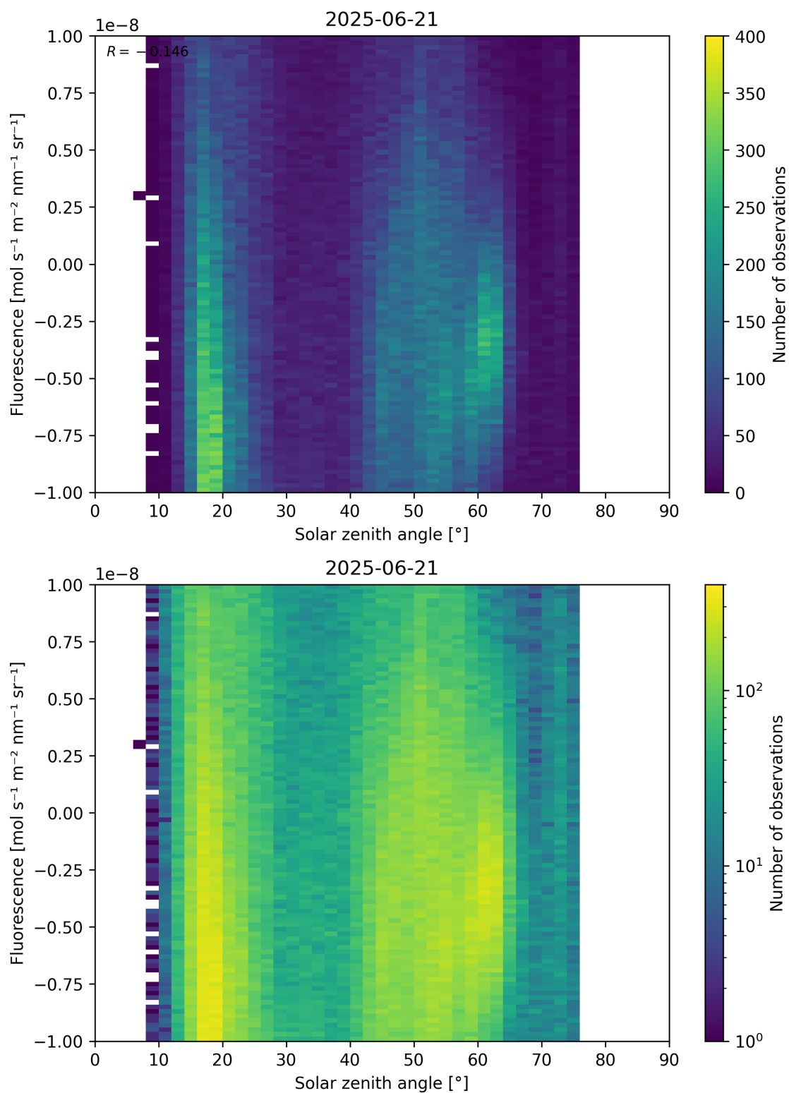
Figure 97: Scatter density plot of “Solar zenith angle” against “Fluorescence” for 2025-06-20 to 2025-06-22.
