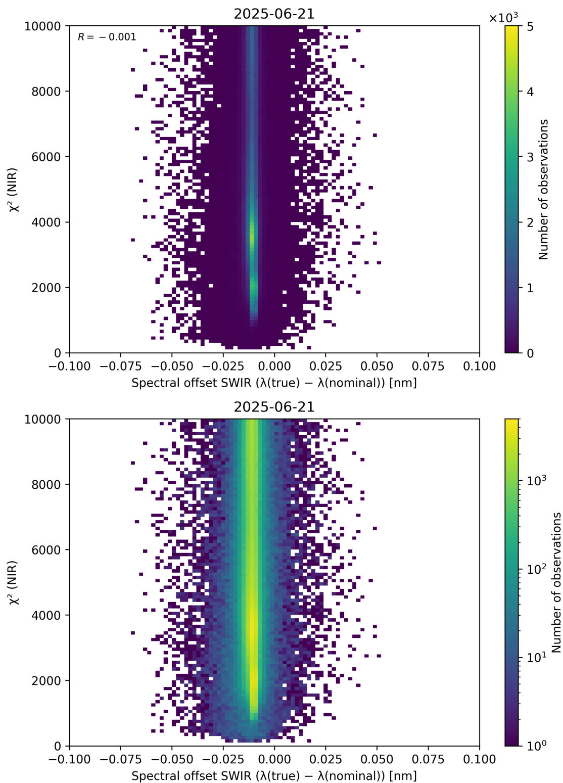
Figure 117: Scatter density plot of “Spectral offset SWIR ( \lambda_{\text{true}} - \lambda_{\text{nominal}} )” against “ \chi^2 (NIR)” for 2025-06-20 to 2025-06-22.
