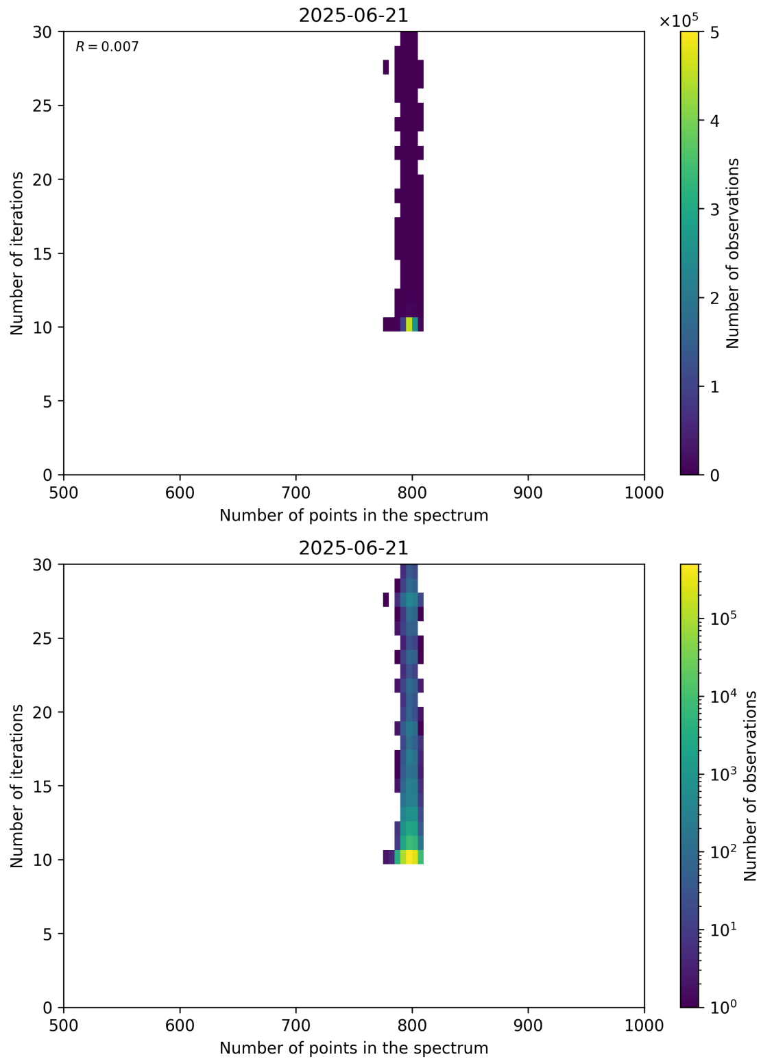
Figure 92: Scatter density plot of “Number of points in the spectrum” against “Number of iterations” for 2025-06-20 to 2025-06-22.
