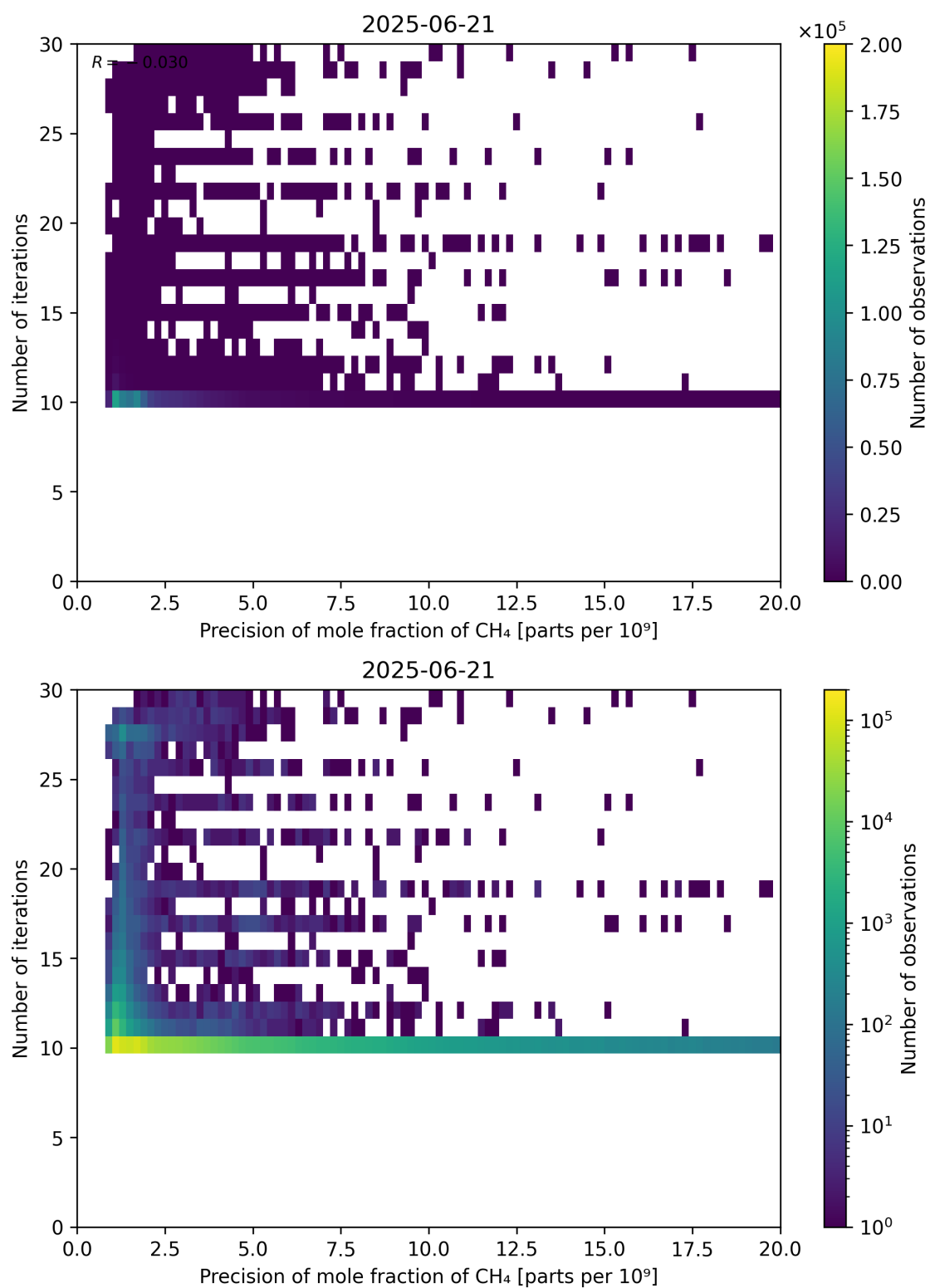
Figure 83: Scatter density plot of “Precision of mole fraction of CH 4 ” against “Number of iterations” for 2025-06-20 to 2025-06-22.
