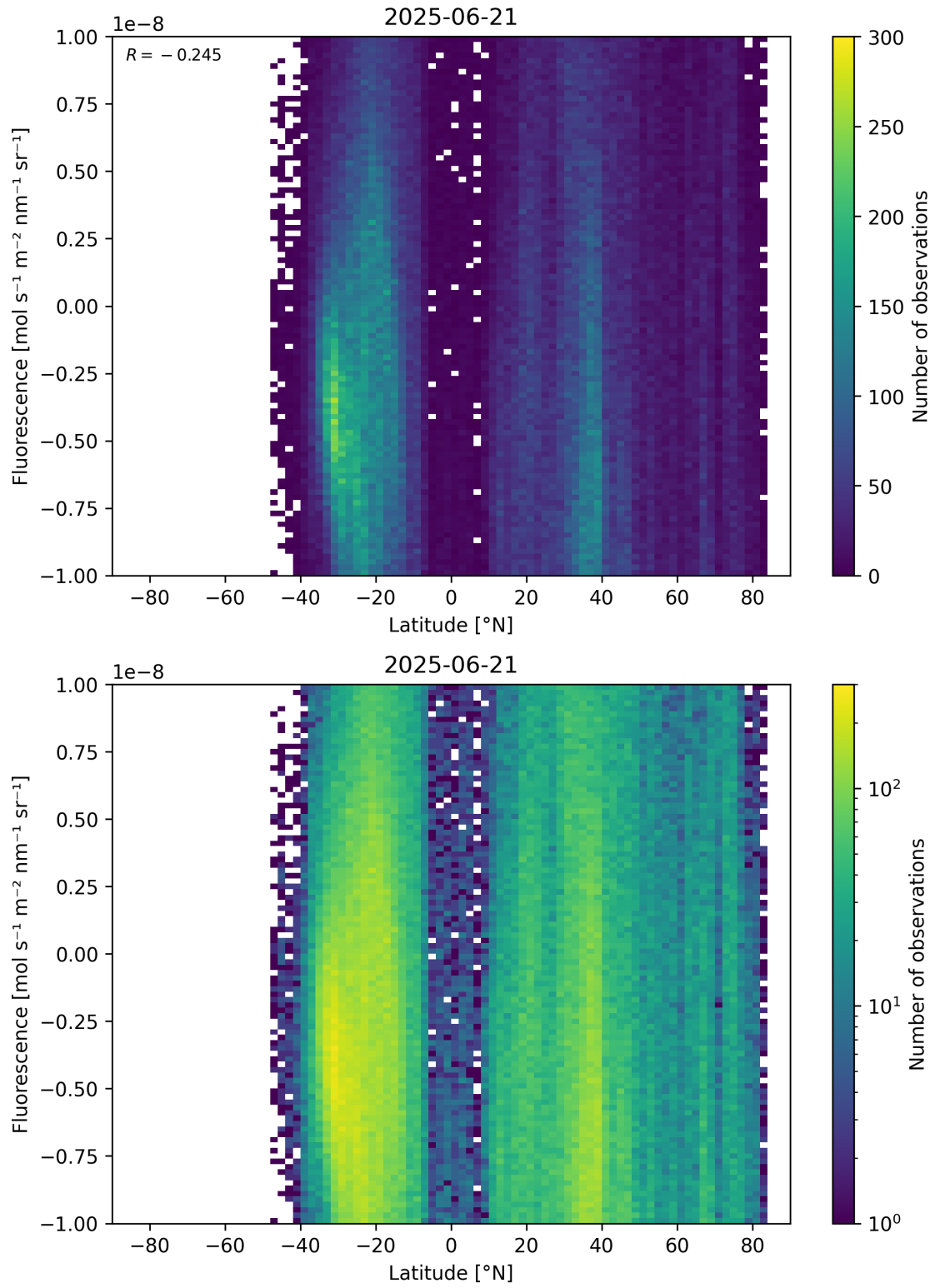
Figure 56: Scatter density plot of “Latitude” against “Fluorescence” for 2025-06-20 to 2025-06-22.
