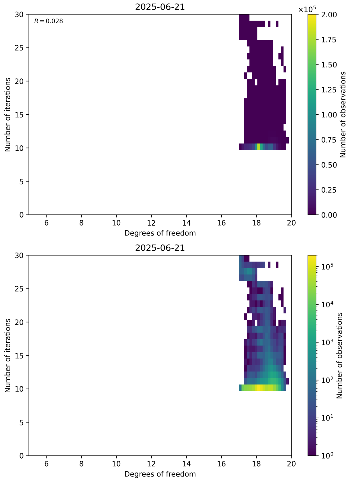
Figure 52: Scatter density plot of “Degrees of freedom” against “Number of iterations” for 2025-06-20 to 2025-06-22.
