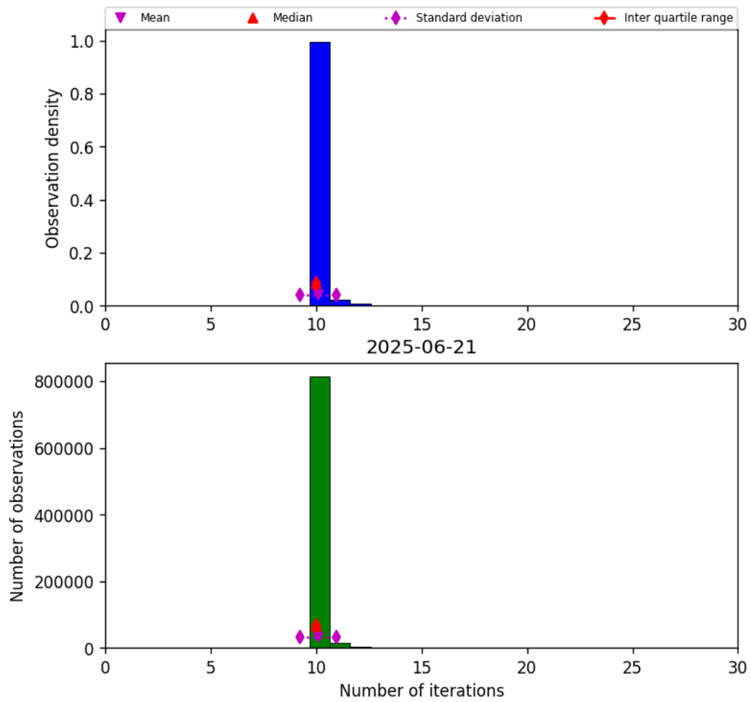
Figure 31: Histogram of "Number of iterations" for 2025-06-20 to 2025-06-22
