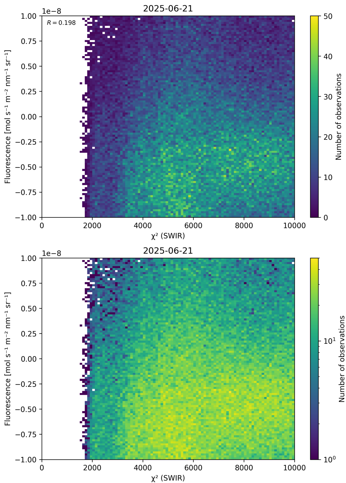
Figure 49: Scatter density plot of “ \chi^2 (SWIR)” against “Fluorescence” for 2025-06-20 to 2025-06-22.
