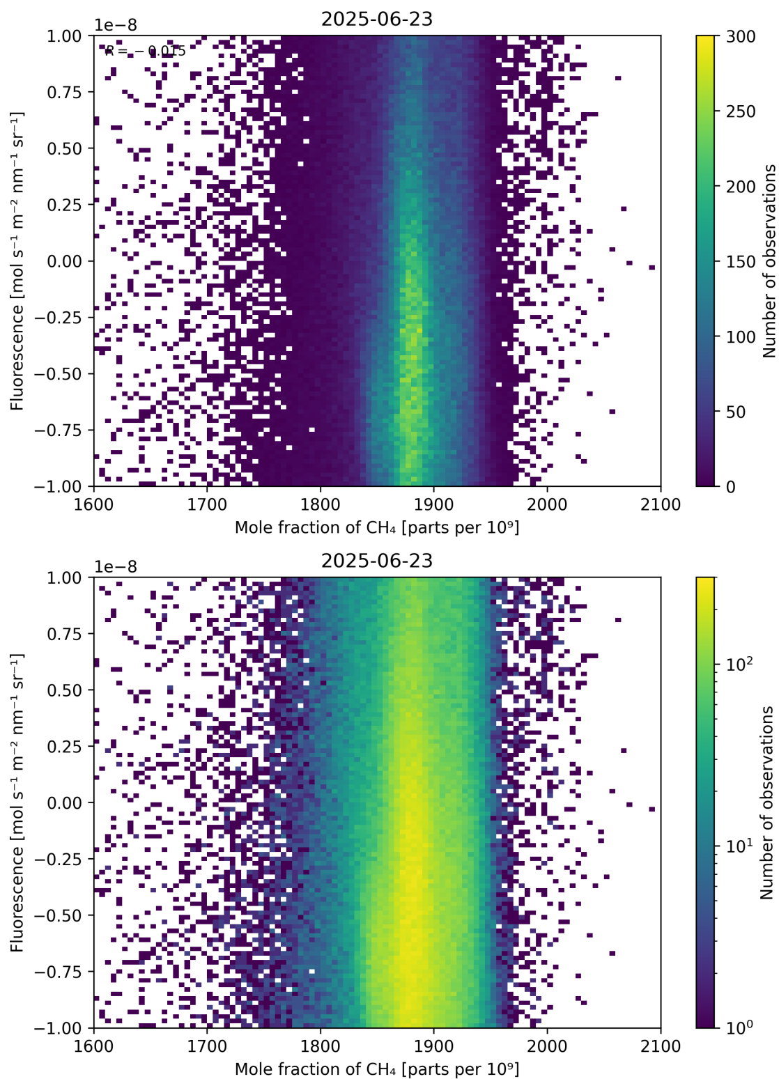
Figure 73: Scatter density plot of “Mole fraction of \text{CH}_4 ” against “Fluorescence” for 2025-06-22 to 2025-06-24.
