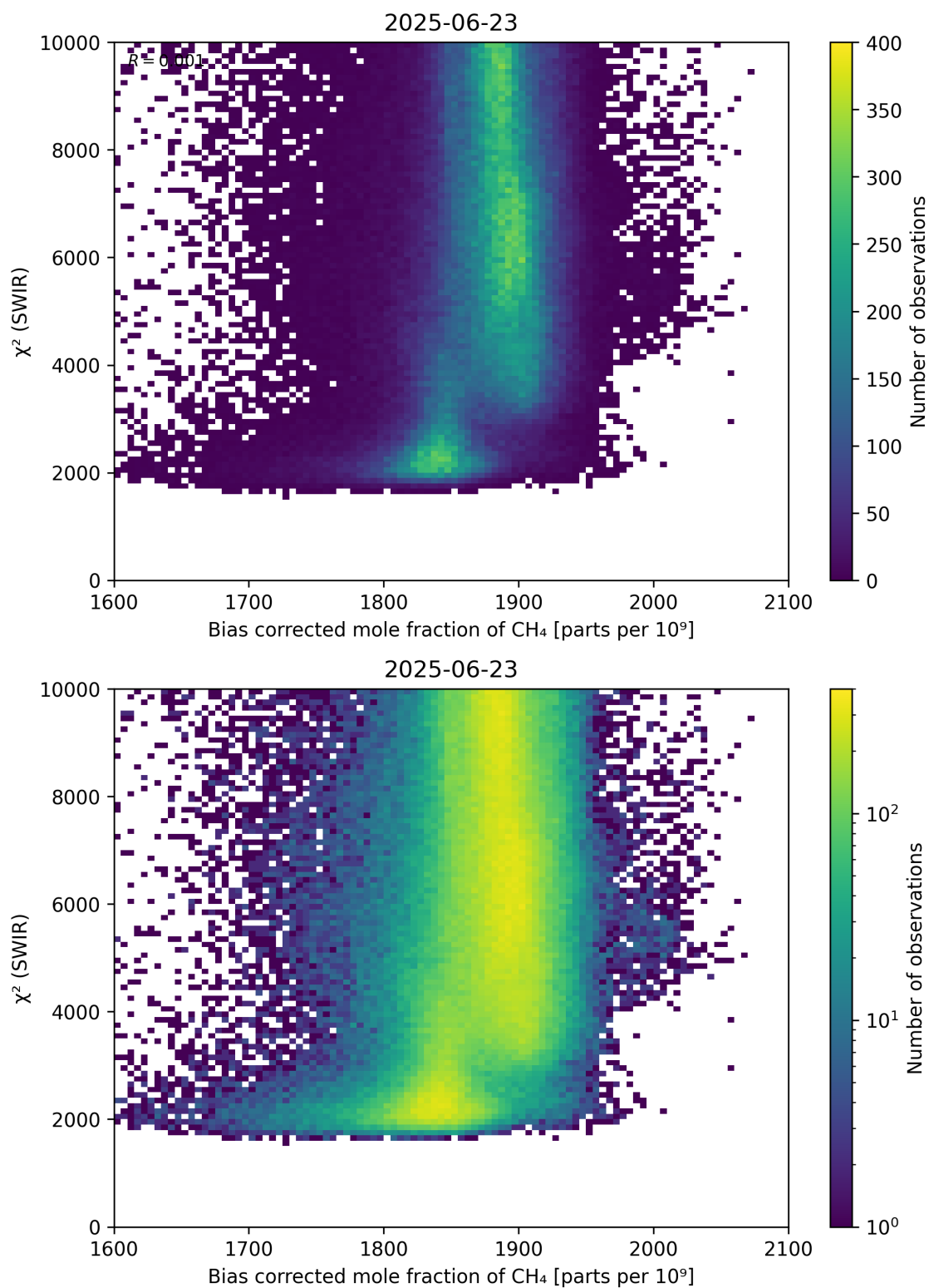
Figure 64: Scatter density plot of “Bias corrected mole fraction of \text{CH}_4 ” against “ \chi^2 (SWIR)” for 2025-06-22 to 2025-06-24.
