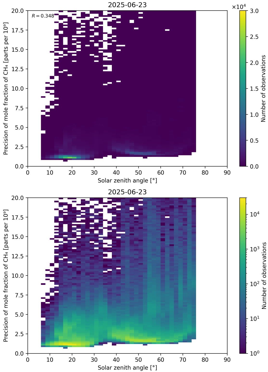
Figure 101: Scatter density plot of “Solar zenith angle” against “Precision of mole fraction of CH 4 ” for 2025-06-22 to 2025-06-24.
