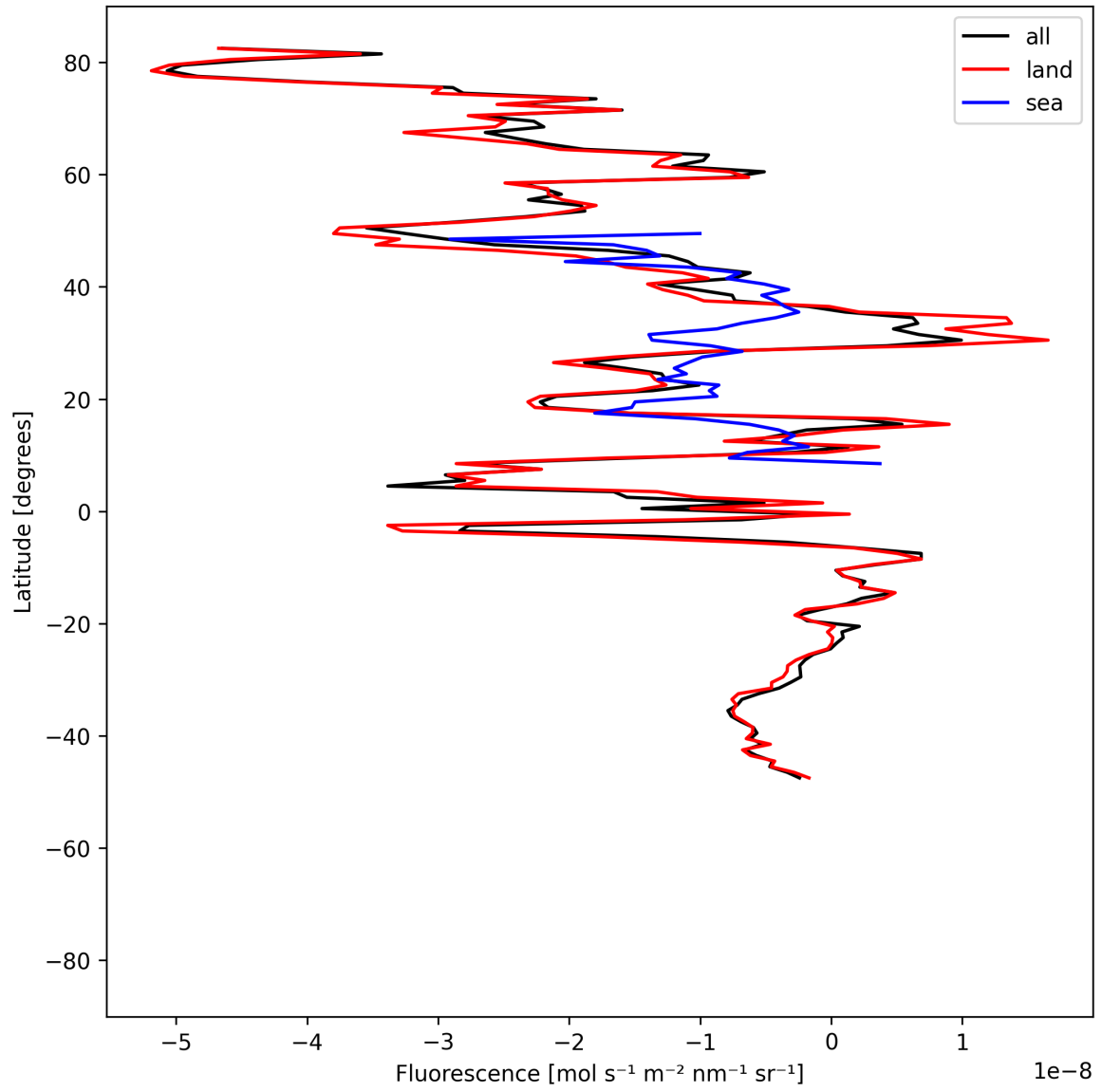
Figure 21: Zonal average of “Fluorescence” for 2025-06-22 to 2025-06-24.
