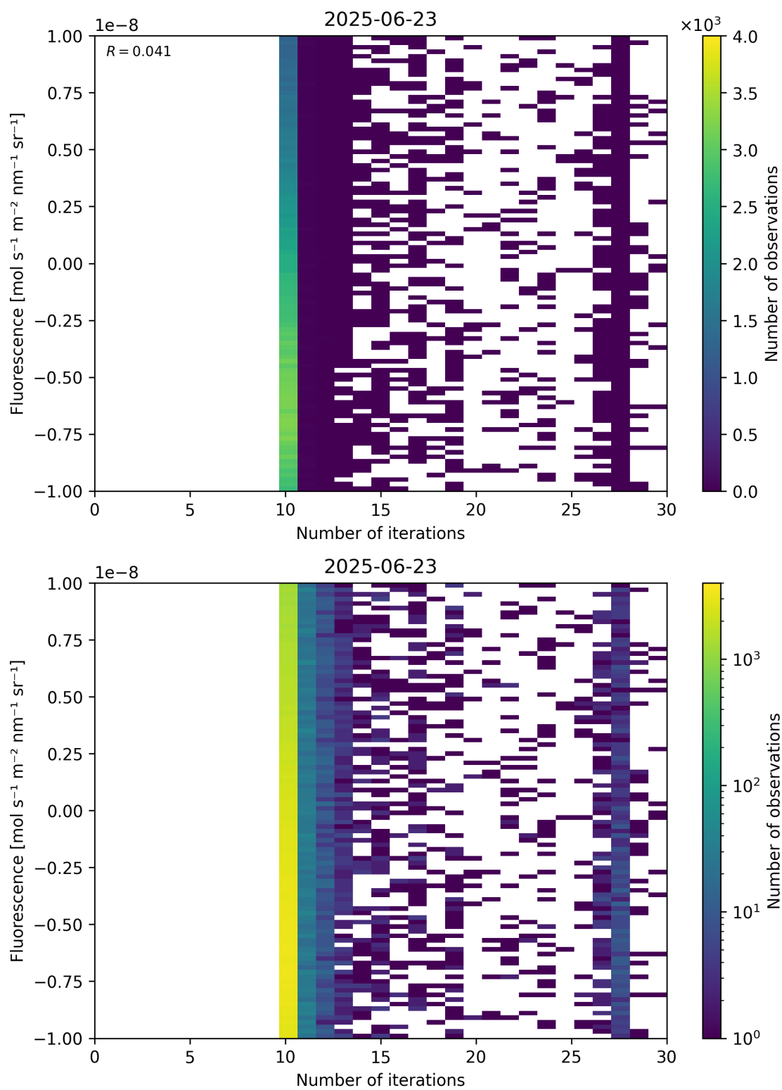
Figure 87: Scatter density plot of “Number of iterations” against “Fluorescence” for 2025-06-22 to 2025-06-24.
