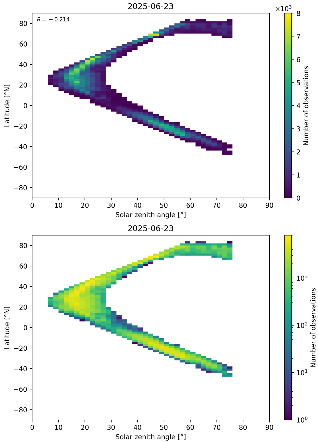
Figure 98: Scatter density plot of “Solar zenith angle” against “Latitude” for 2025-06-22 to 2025-06-24.
