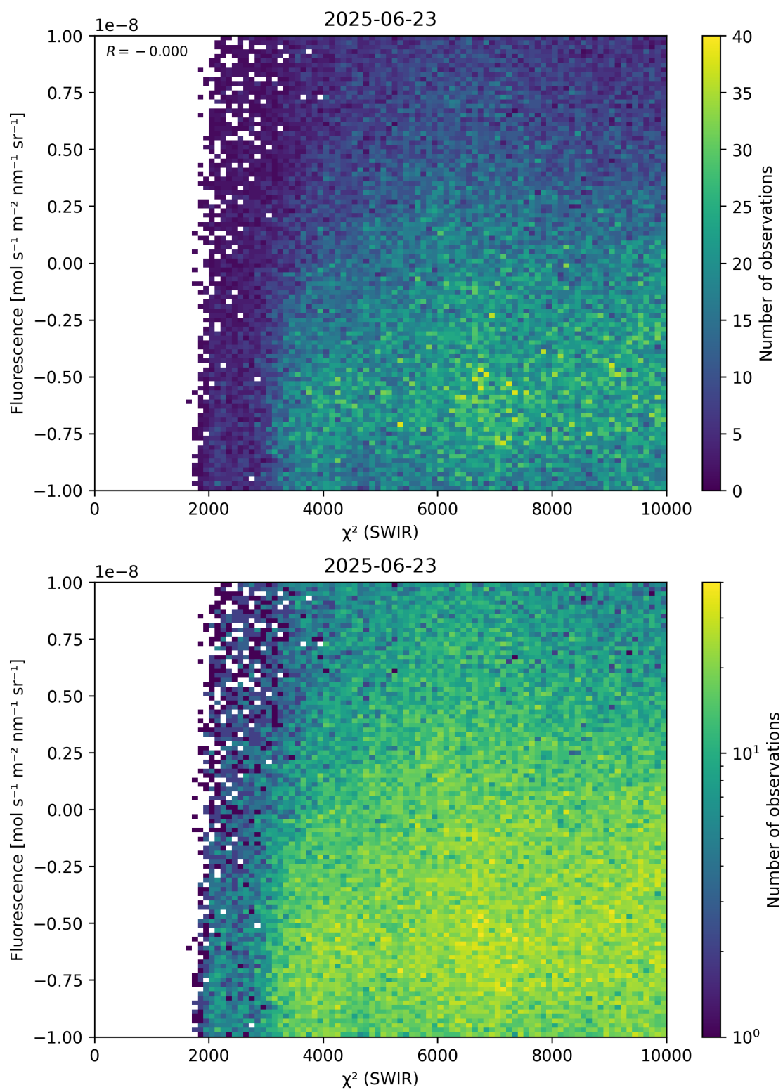
Figure 49: Scatter density plot of “ \chi^2 (SWIR)” against “Fluorescence” for 2025-06-22 to 2025-06-24.
