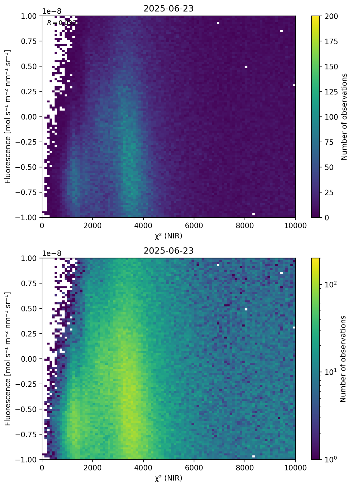
Figure 45: Scatter density plot of “ \chi^2 (NIR)” against “Fluorescence” for 2025-06-22 to 2025-06-24.
