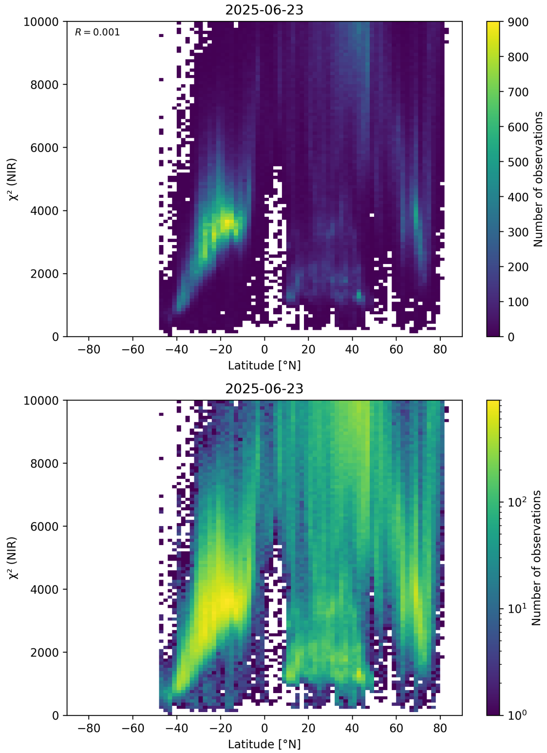
Figure 53: Scatter density plot of “Latitude” against “ \chi^2 (NIR)” for 2025-06-22 to 2025-06-24.
