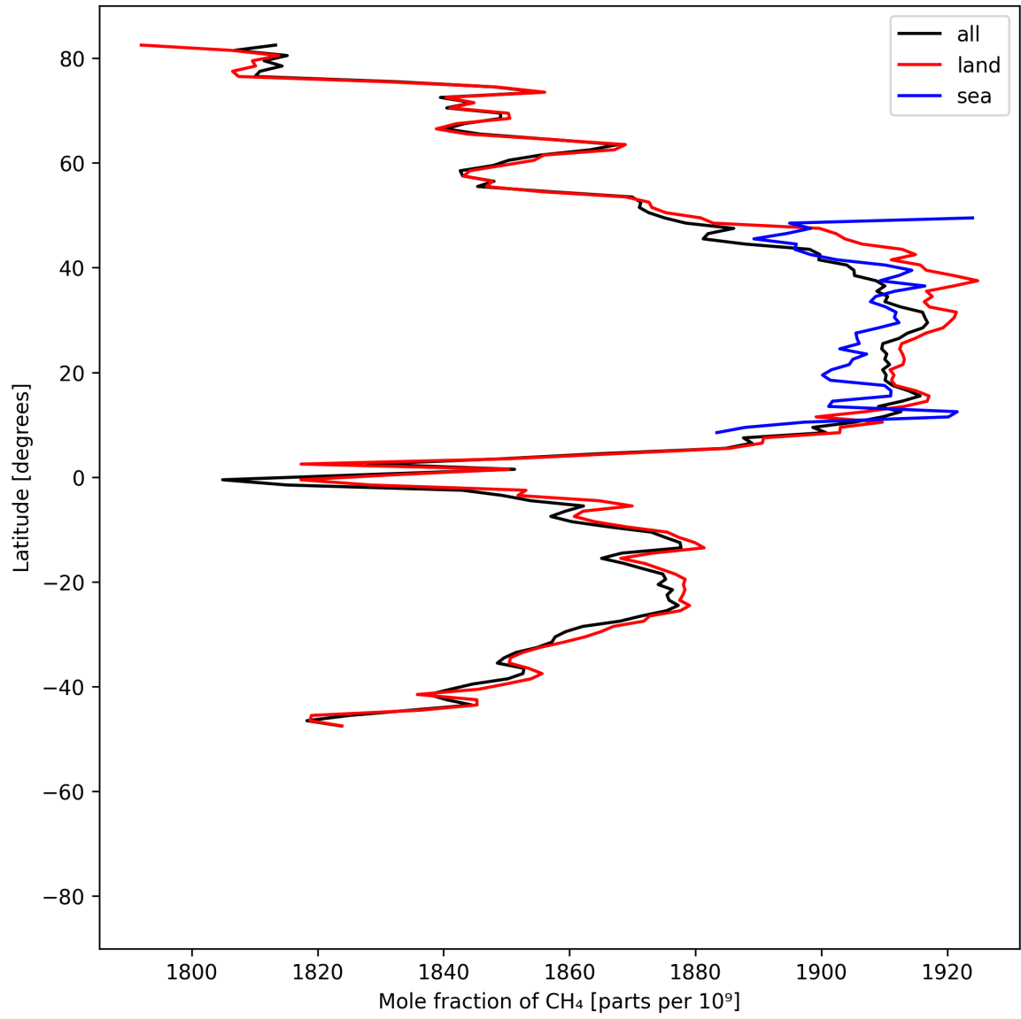
Figure 12: Zonal average of “Mole fraction of CH 4 ” for 2025-06-22 to 2025-06-24.
