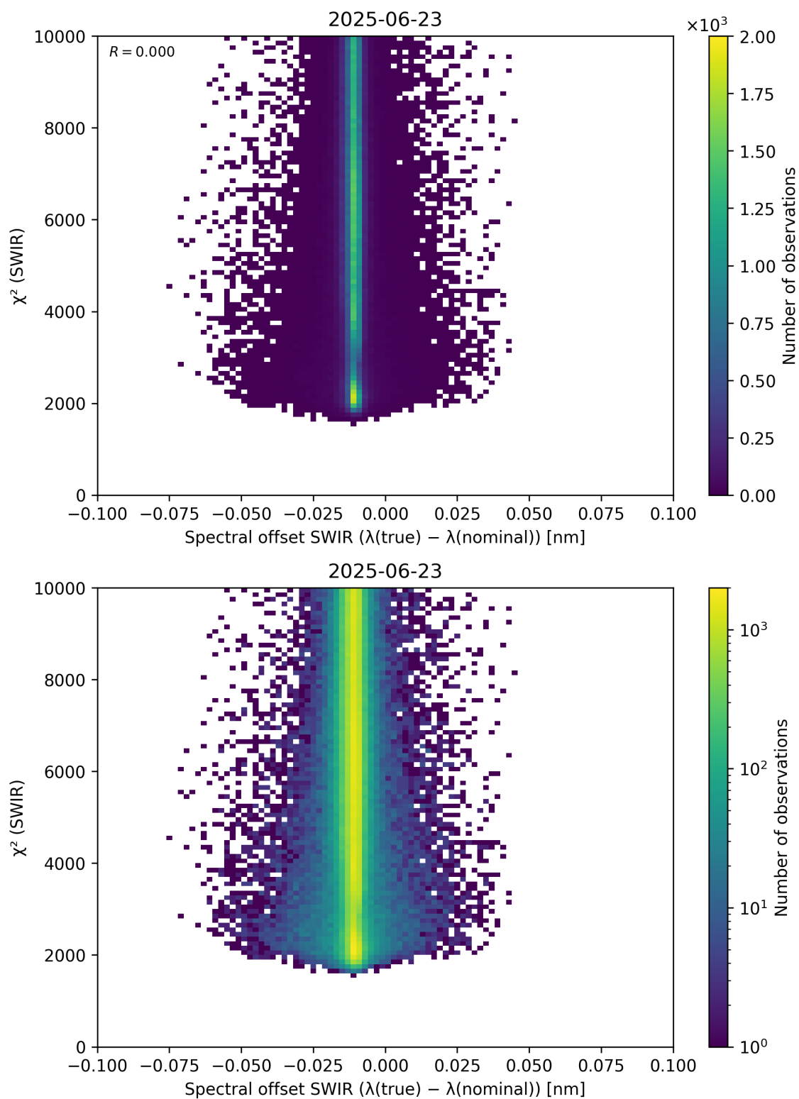
Figure 118: Scatter density plot of “Spectral offset SWIR ( \lambda_{\text{true}} - \lambda_{\text{nominal}} )” against “ \chi^2 (SWIR)” for 2025-06-22 to 2025-06-24.
