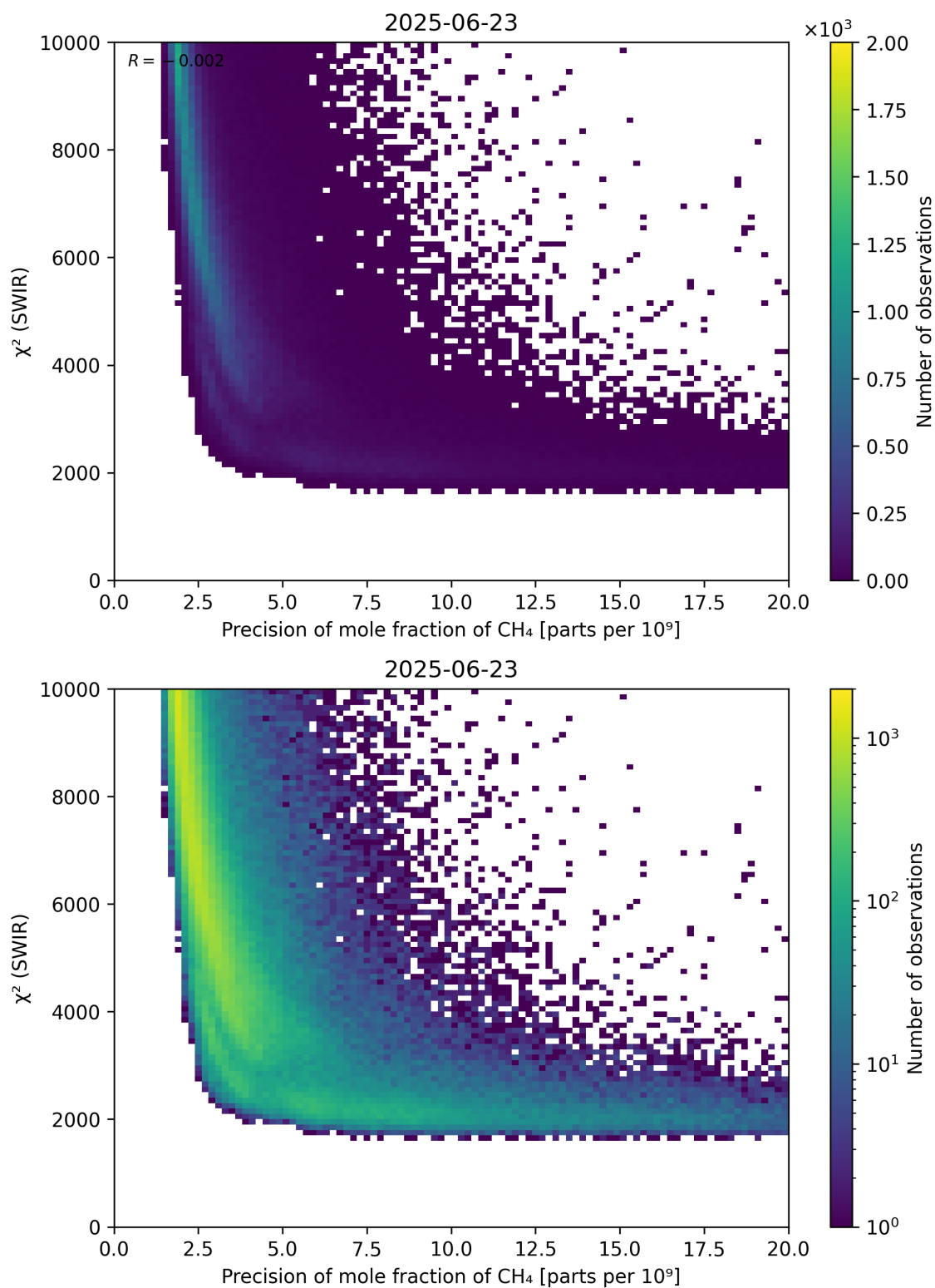
Figure 79: Scatter density plot of “Precision of mole fraction of \text{CH}_4 ” against “ \chi^2 (SWIR)” for 2025-06-22 to 2025-06-24.
