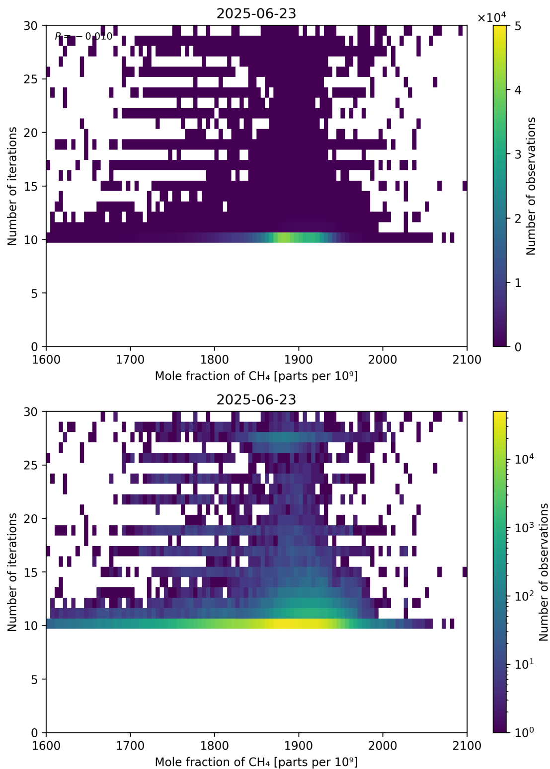
Figure 76: Scatter density plot of “Mole fraction of CH 4 ” against “Number of iterations” for 2025-06-22 to 2025-06-24.
