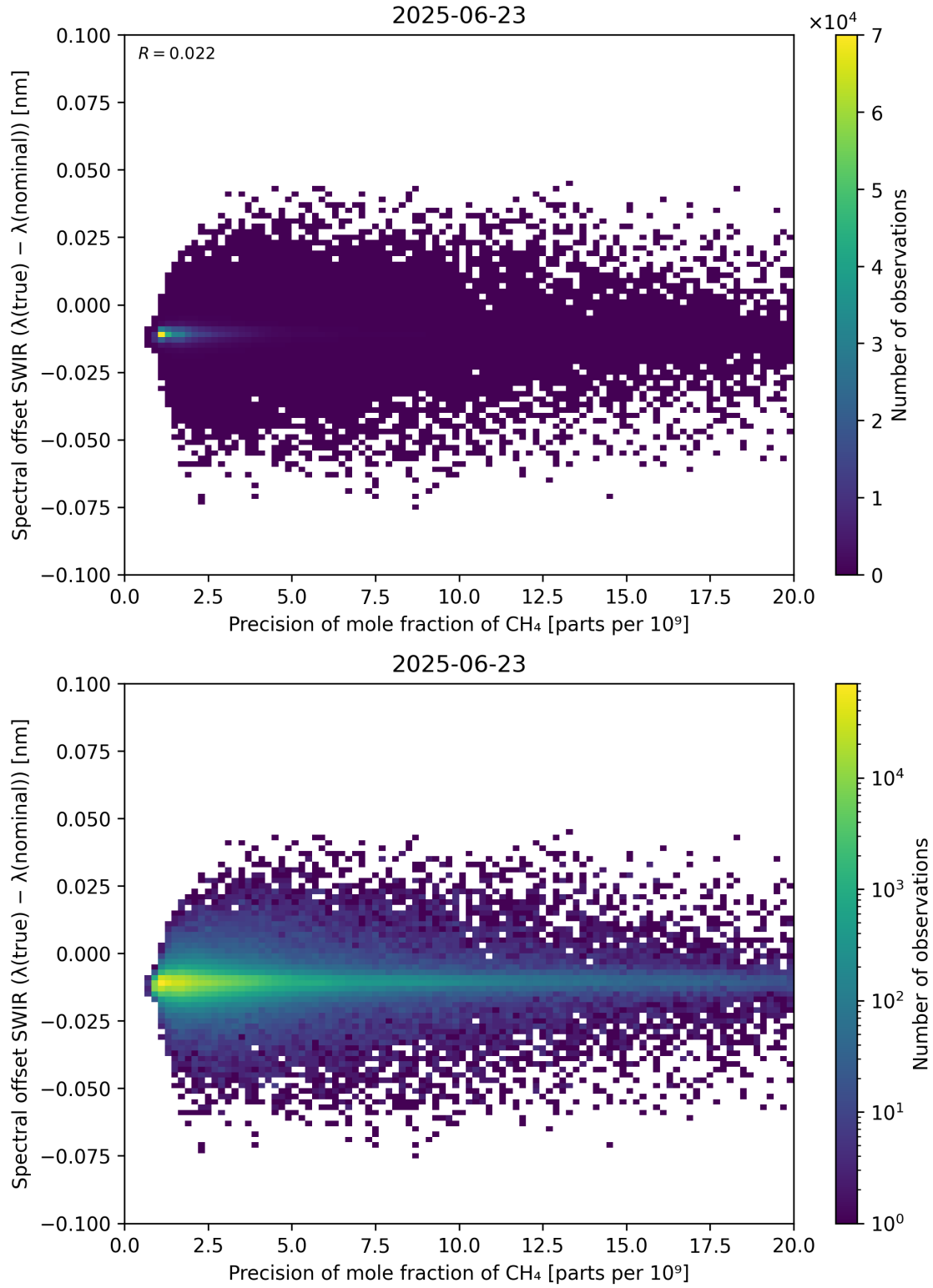
Figure 85: Scatter density plot of “Precision of mole fraction of CH 4 ” against “Spectral offset SWIR ( \lambda_{\text{true}} - \lambda_{\text{nominal}} )” for 2025-06-22 to 2025-06-24.
