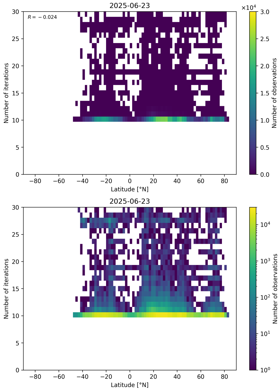
Figure 60: Scatter density plot of “Latitude” against “Number of iterations” for 2025-06-22 to 2025-06-24.
