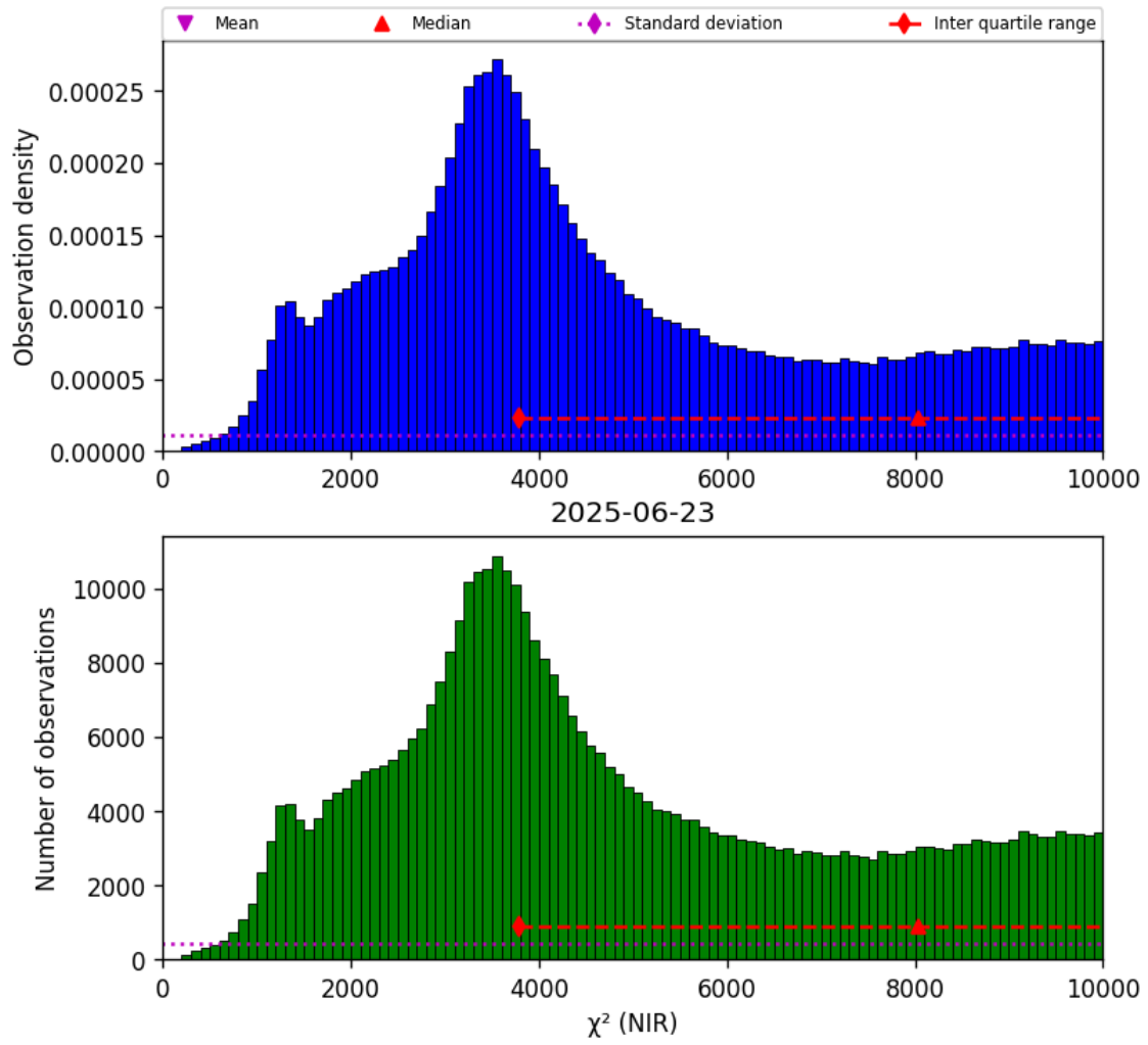
Figure 29: Histogram of “ \chi^2 (NIR)” for 2025-06-22 to 2025-06-24
