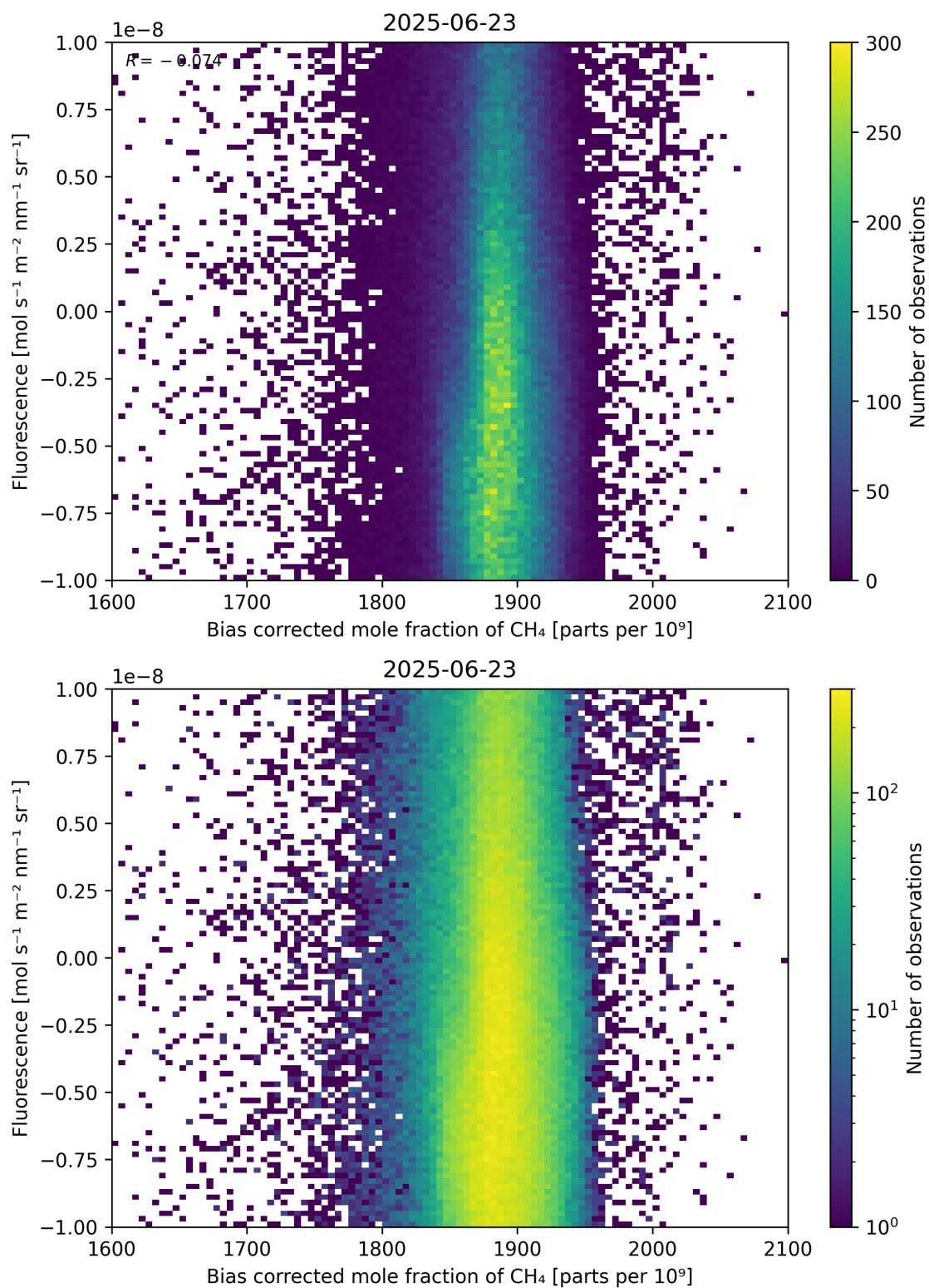
Figure 66: Scatter density plot of “Bias corrected mole fraction of \text{CH}_4 ” against “Fluorescence” for 2025-06-22 to 2025-06-24.
