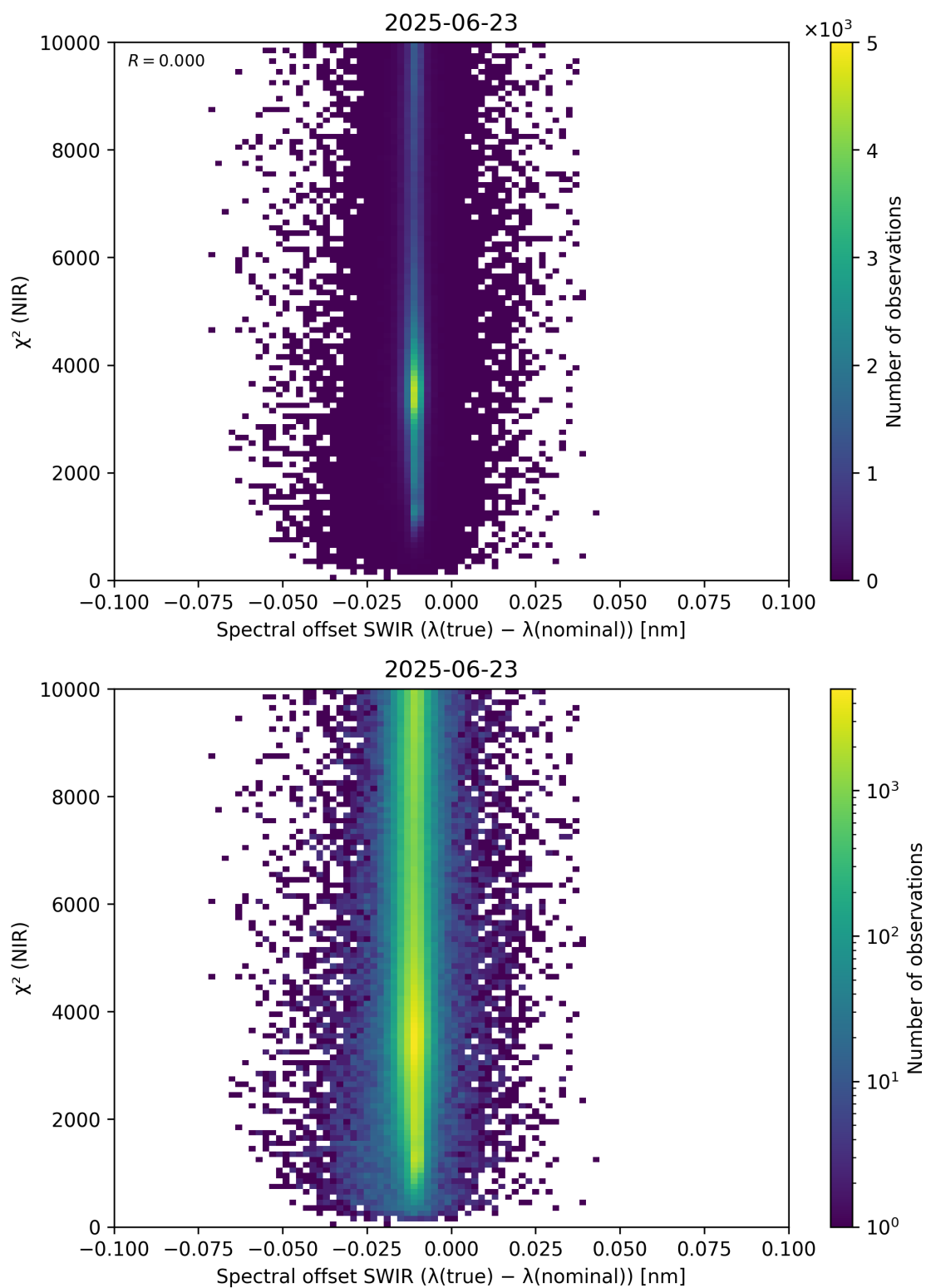
Figure 117: Scatter density plot of “Spectral offset SWIR ( \lambda_{\text{true}} - \lambda_{\text{nominal}} )” against “ \chi^2 (NIR)” for 2025-06-22 to 2025-06-24.
