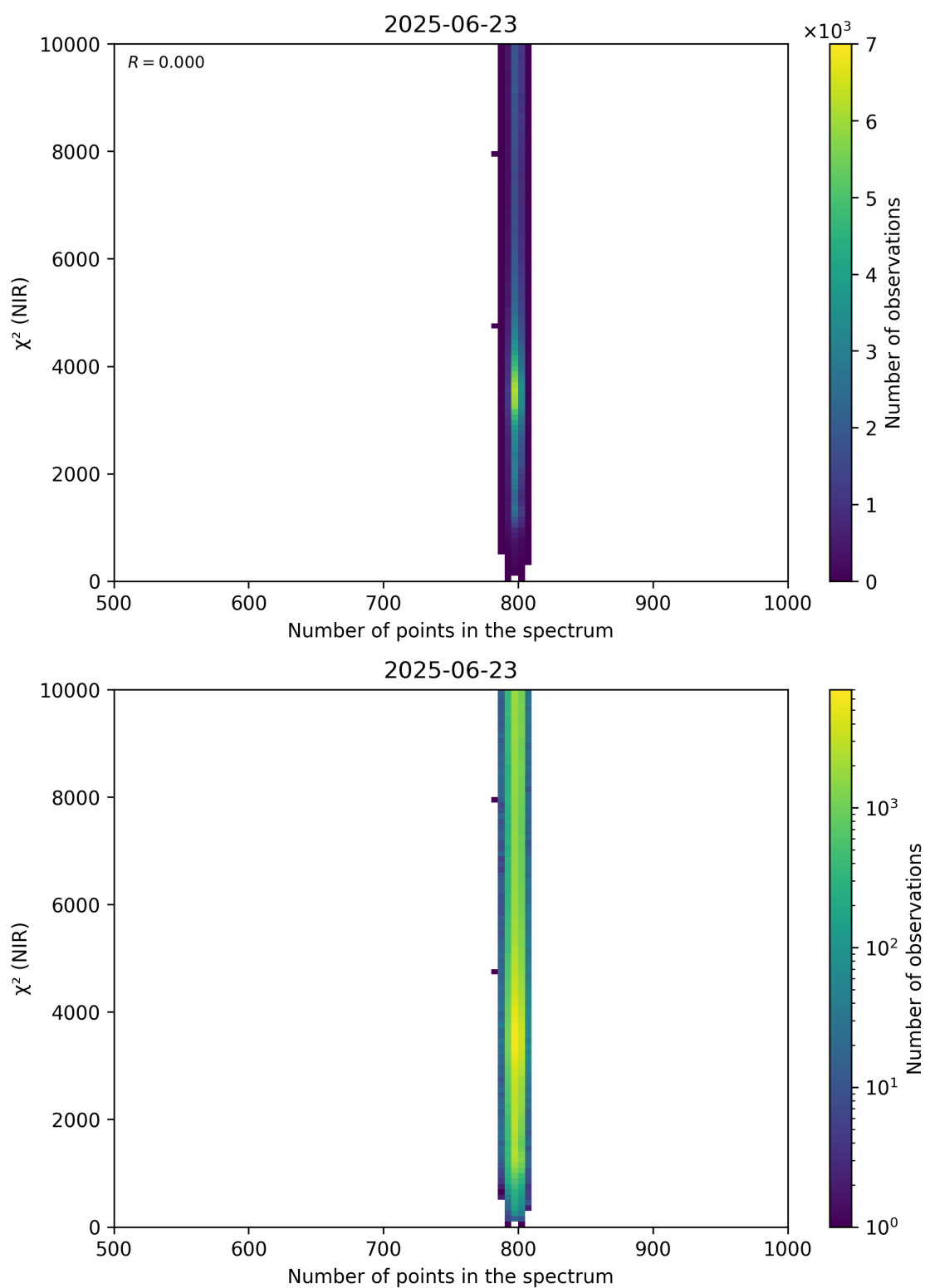
Figure 88: Scatter density plot of “Number of points in the spectrum” against “ \chi^2 (NIR)” for 2025-06-22 to 2025-06-24.
