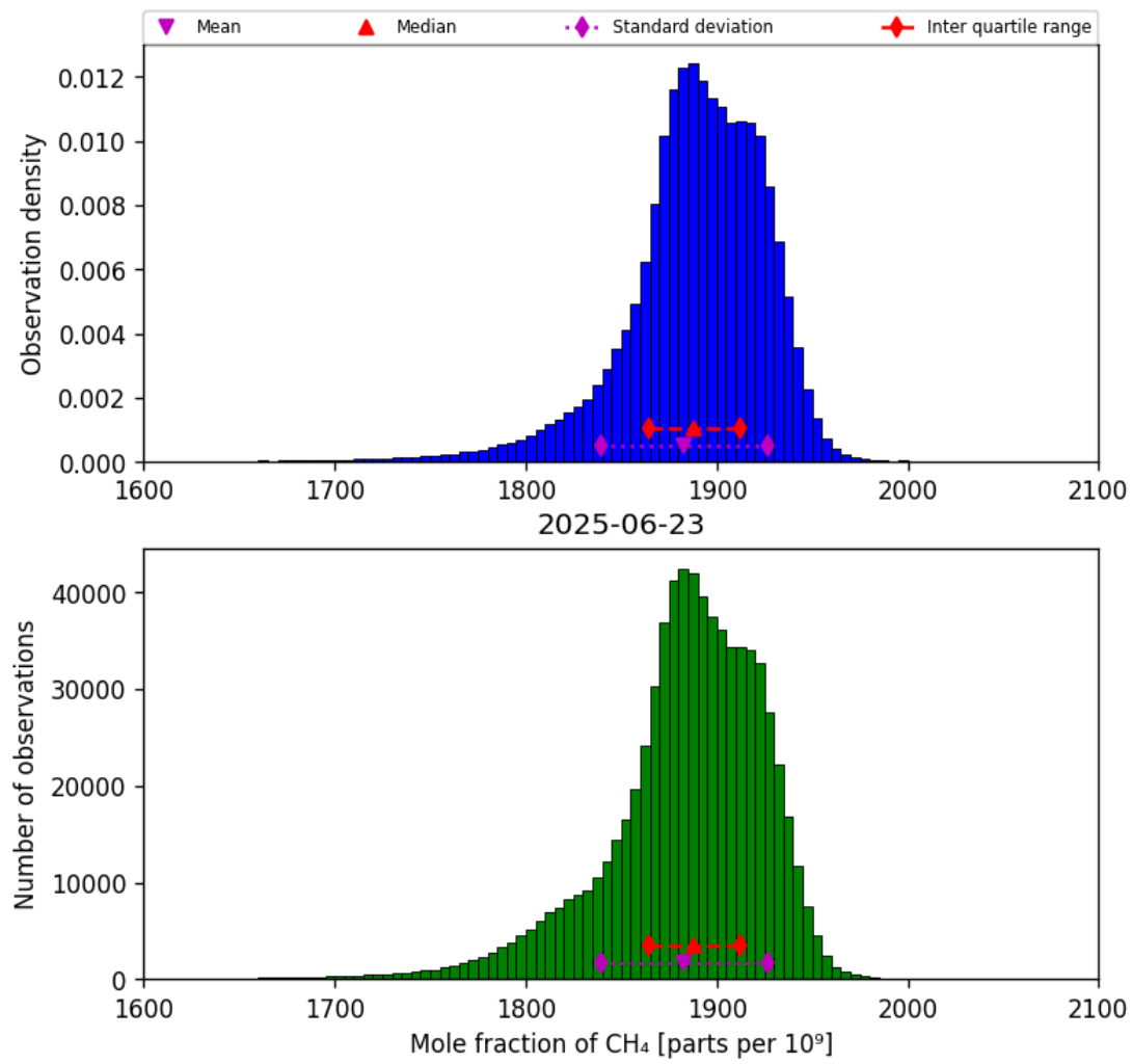
Figure 23: Histogram of “Mole fraction of CH 4 ” for 2025-06-22 to 2025-06-24
