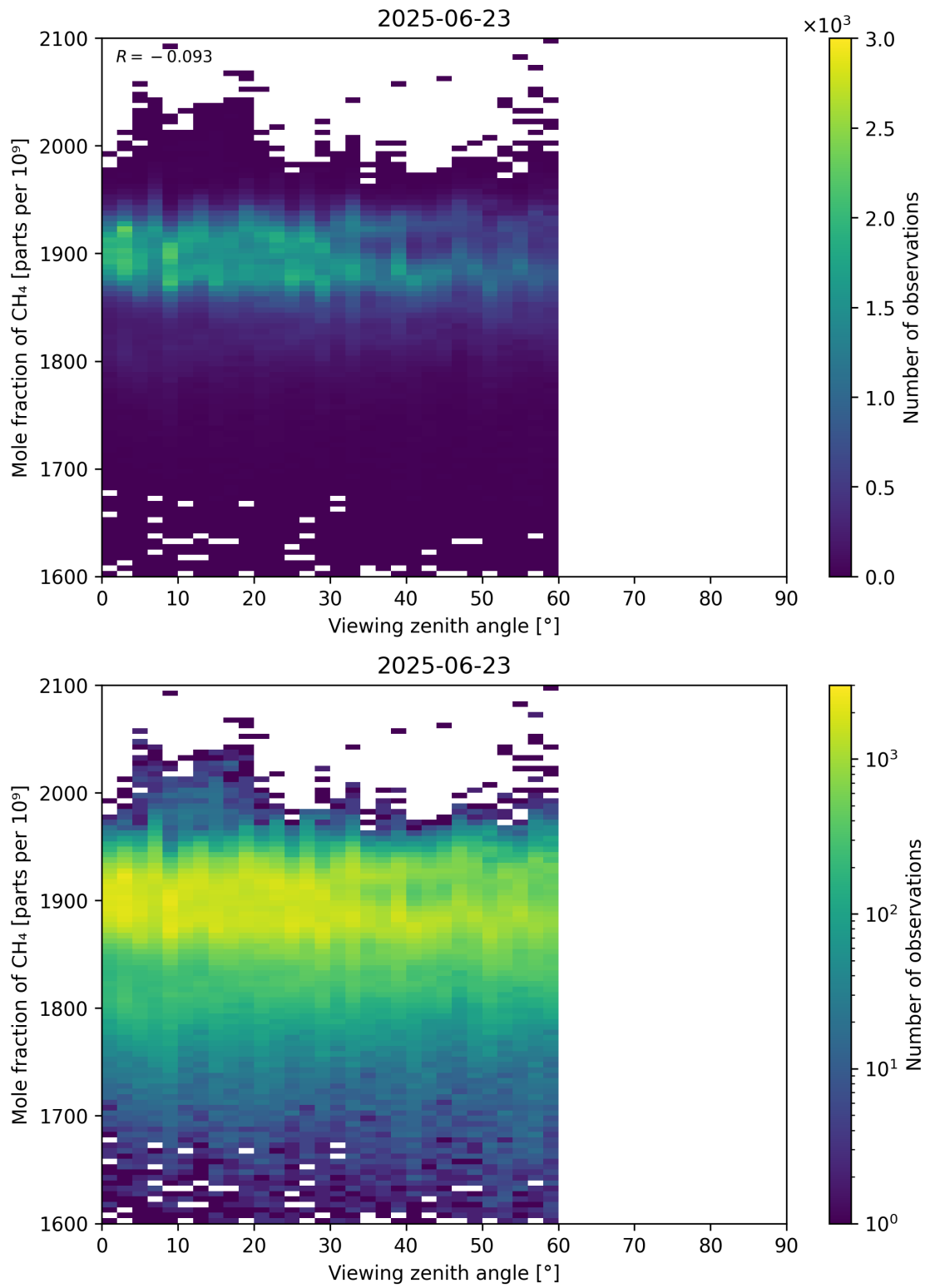
Figure 110: Scatter density plot of “Viewing zenith angle” against “Mole fraction of CH 4 ” for 2025-06-22 to 2025-06-24.
