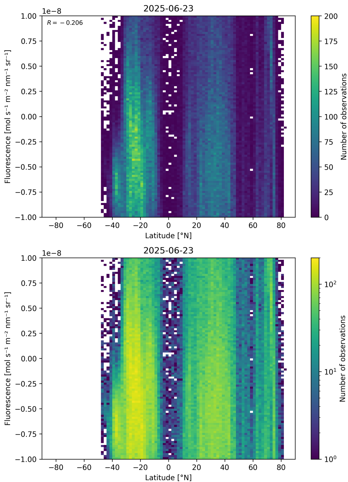
Figure 56: Scatter density plot of “Latitude” against “Fluorescence” for 2025-06-22 to 2025-06-24.
