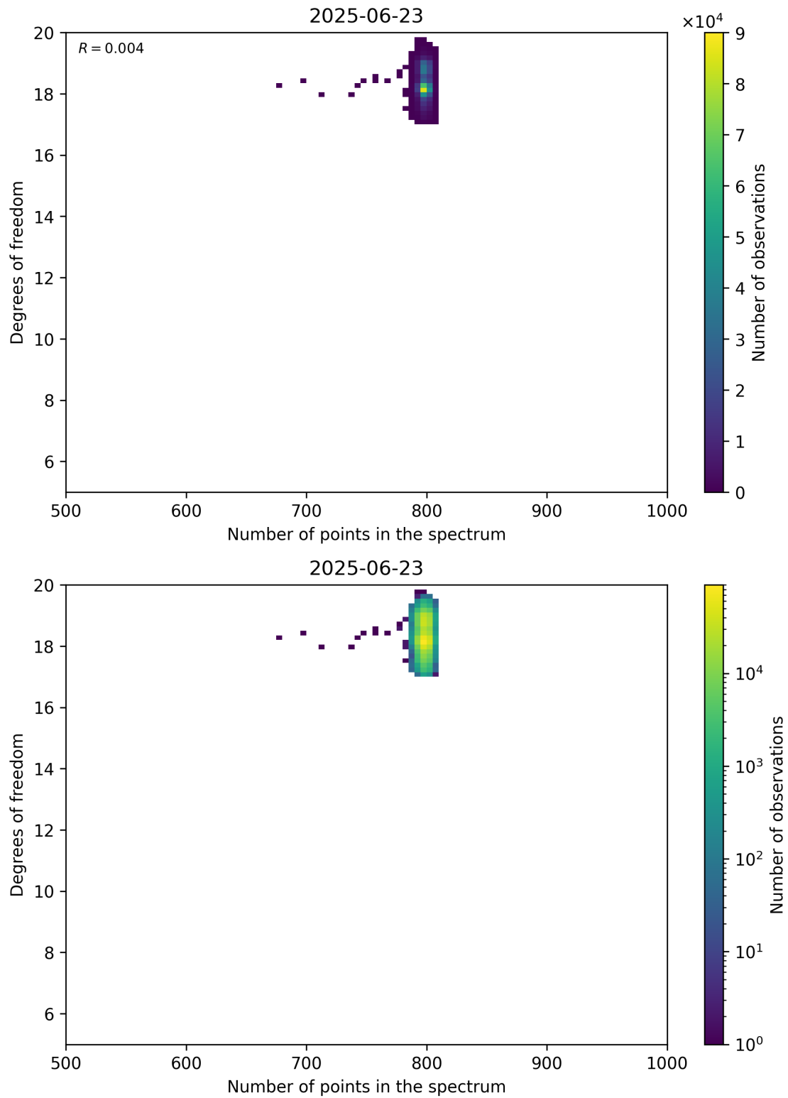
Figure 90: Scatter density plot of “Number of points in the spectrum” against “Degrees of freedom” for 2025-06-22 to 2025-06-24.
