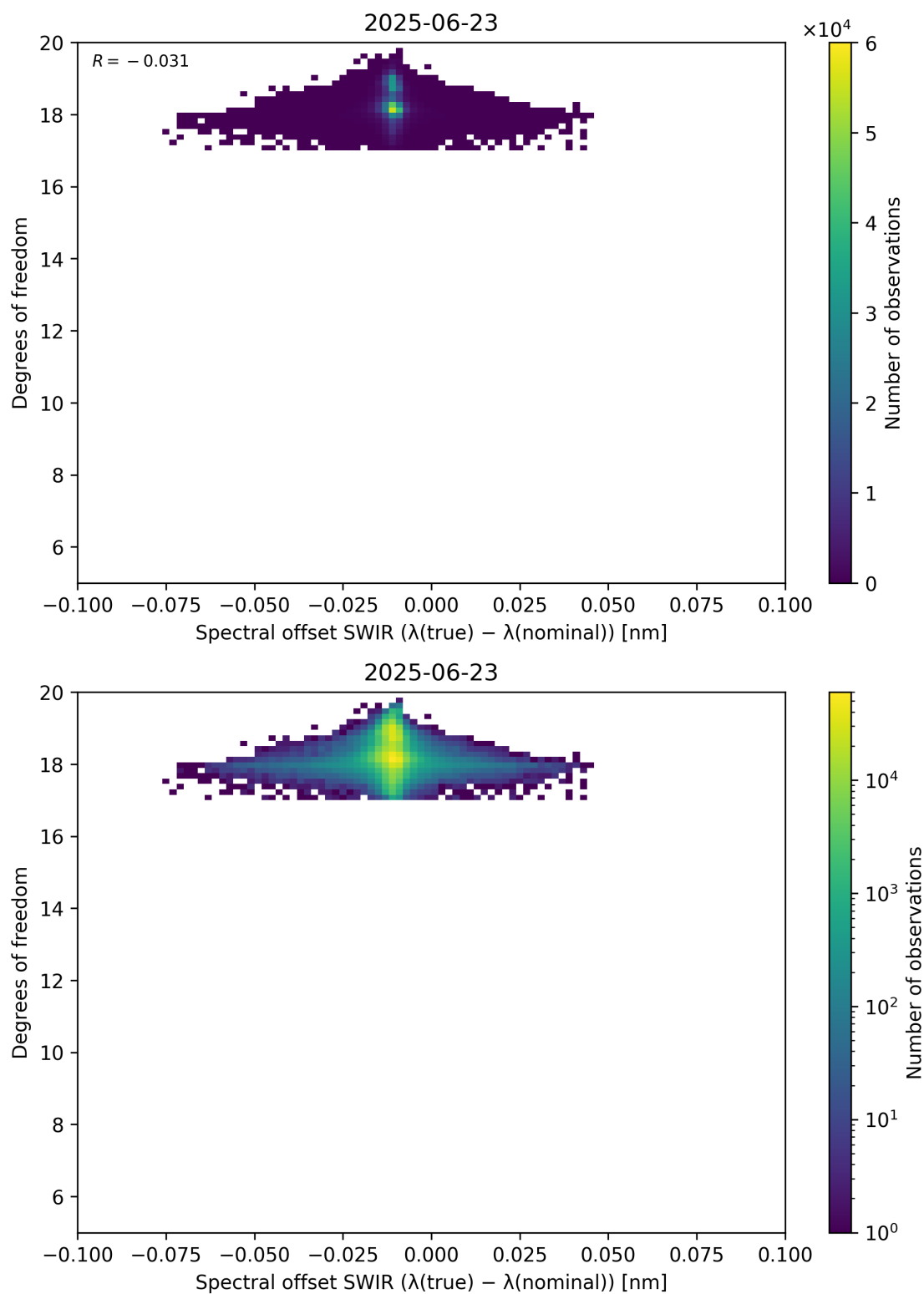
Figure 119: Scatter density plot of “Spectral offset SWIR ( \lambda_{\text{true}} - \lambda_{\text{nominal}} )” against “Degrees of freedom” for 2025-06-22 to 2025-06-24.
