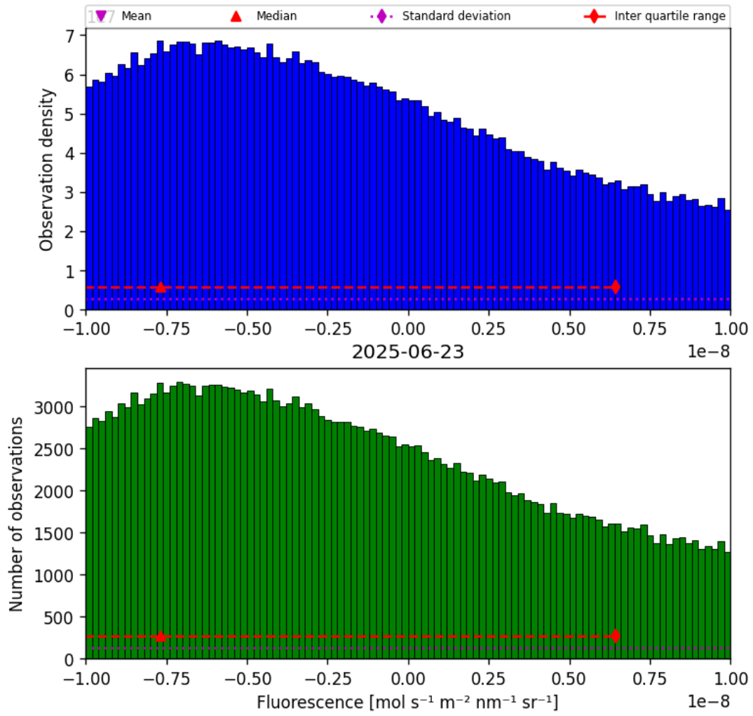
Figure 32: Histogram of “Fluorescence” for 2025-06-22 to 2025-06-24
