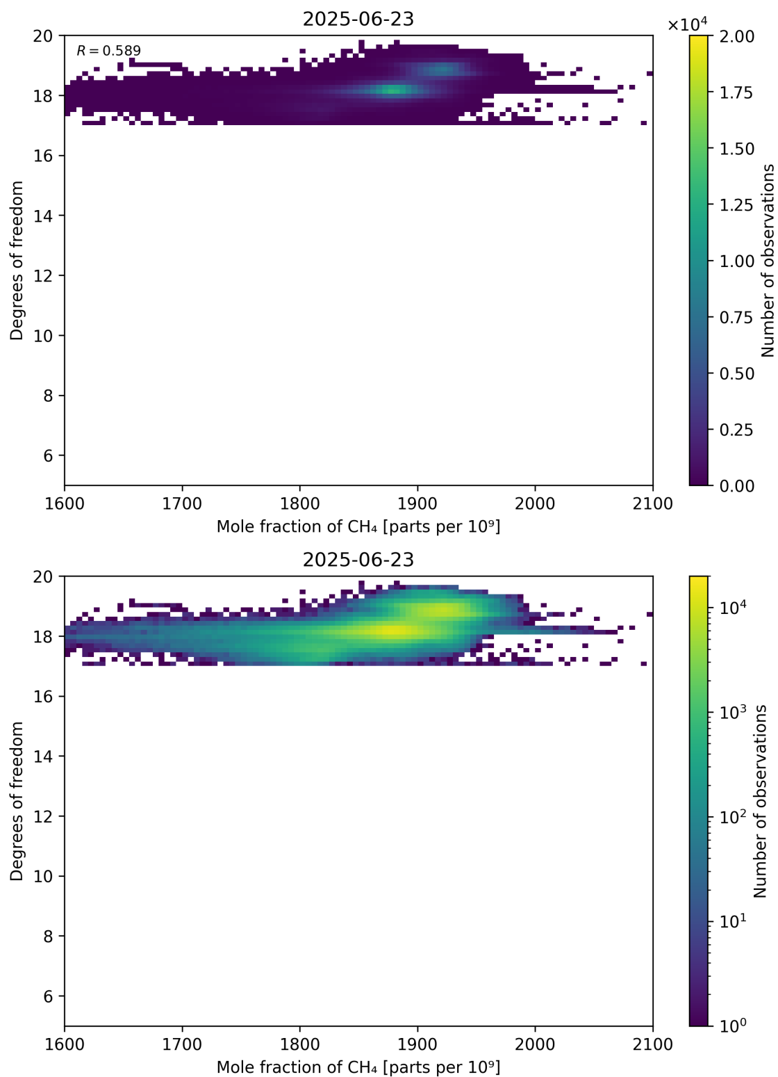
Figure 72: Scatter density plot of “Mole fraction of CH 4 ” against “Degrees of freedom” for 2025-06-22 to 2025-06-24.
