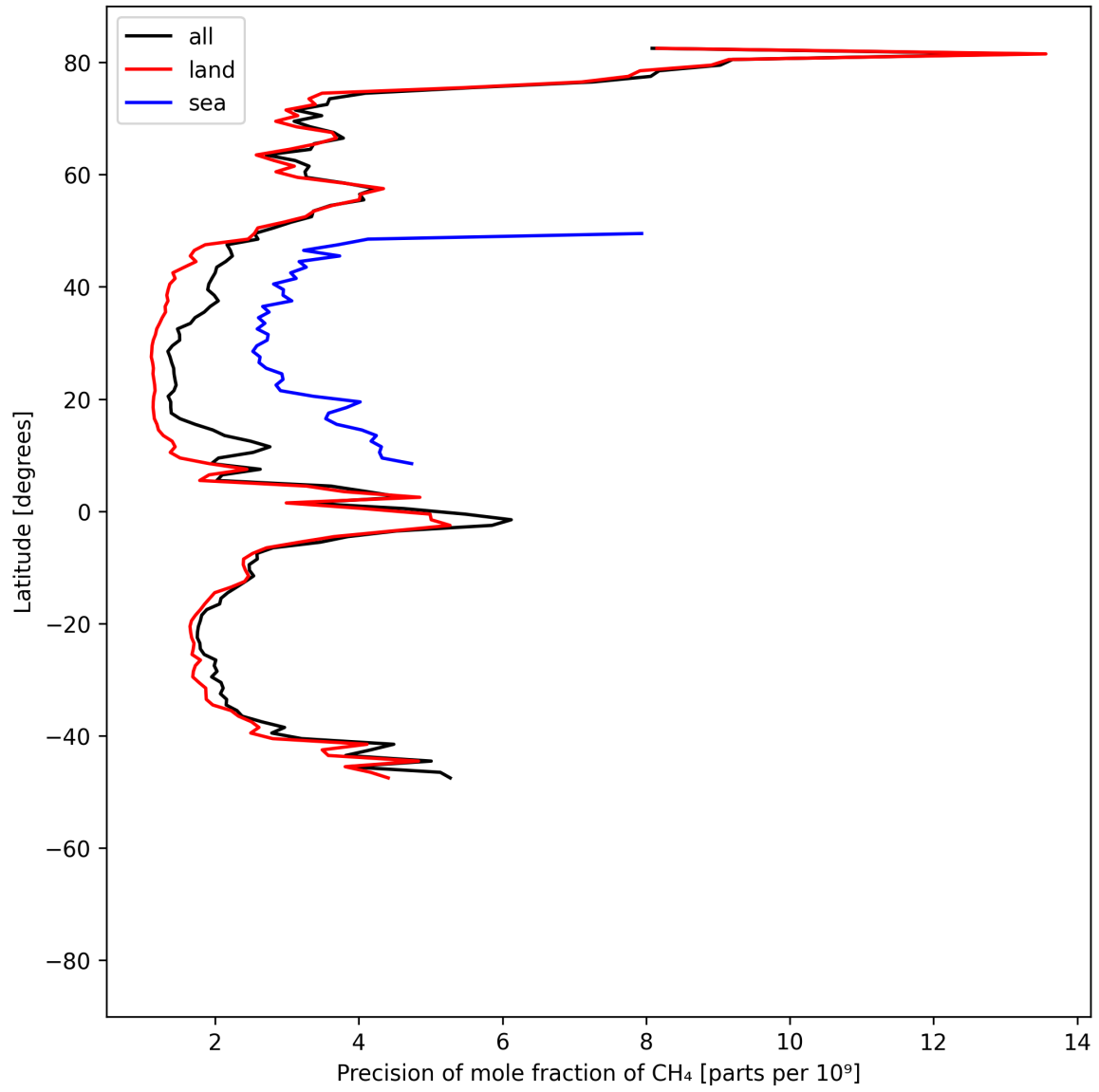
Figure 13: Zonal average of “Precision of mole fraction of CH 4 ” for 2025-06-22 to 2025-06-24.
