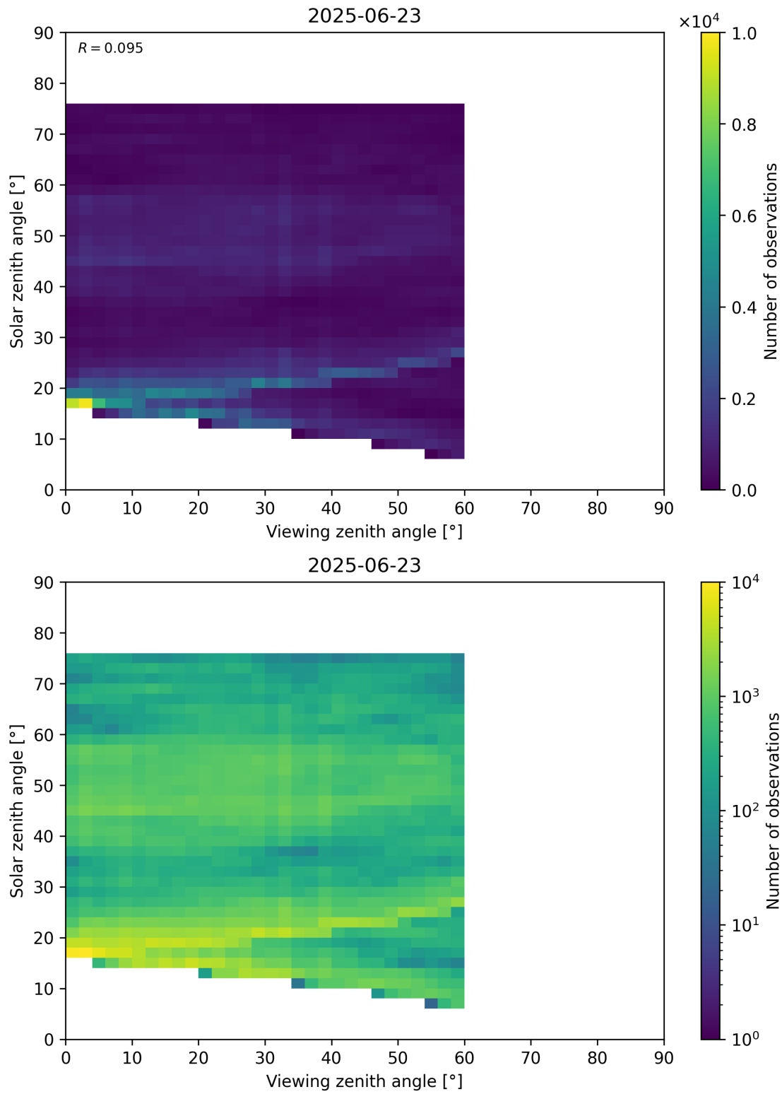
Figure 115: Scatter density plot of “Viewing zenith angle” against “Solar zenith angle” for 2025-06-22 to 2025-06-24.
