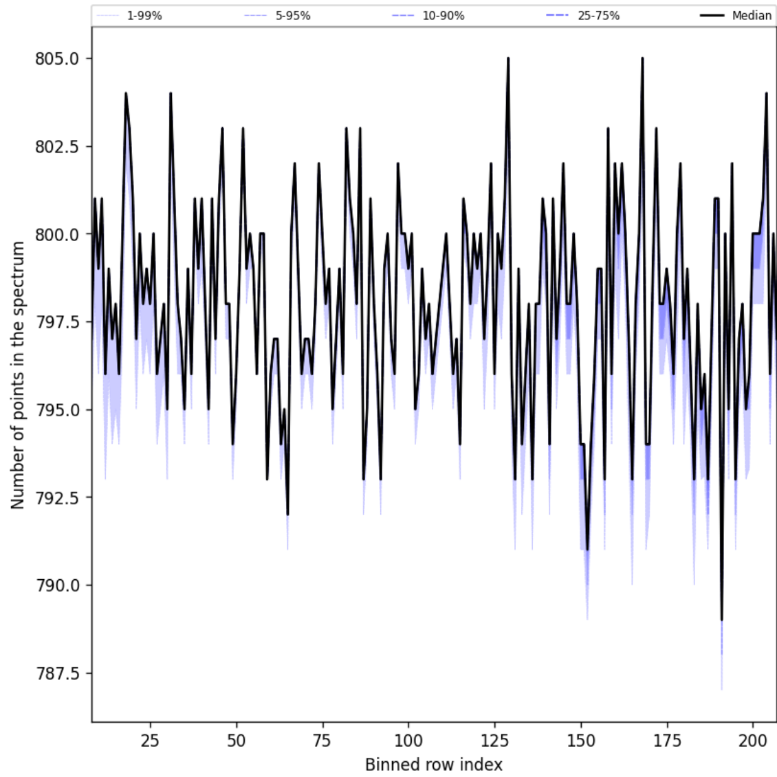
Figure 37: Along track statistics of “Number of points in the spectrum” for 2025-06-22 to 2025-06-24
