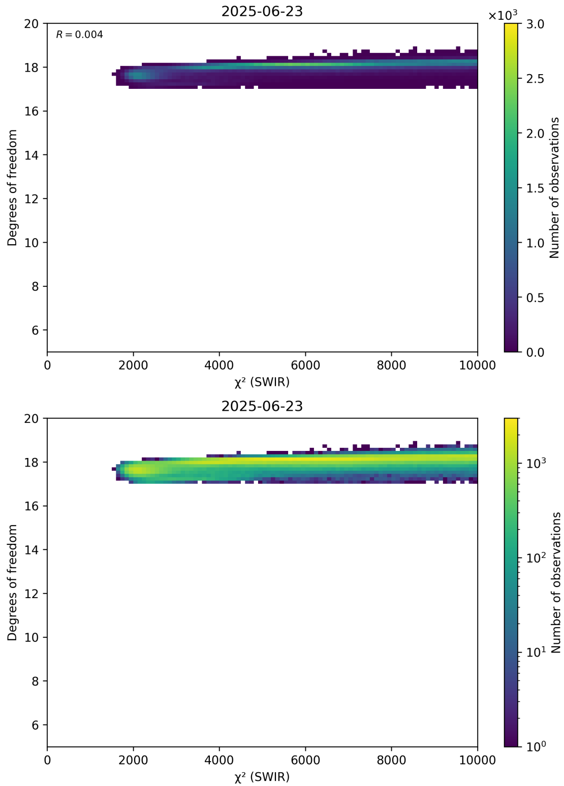
Figure 48: Scatter density plot of “ \chi^2 (SWIR)” against “Degrees of freedom” for 2025-06-22 to 2025-06-24.
