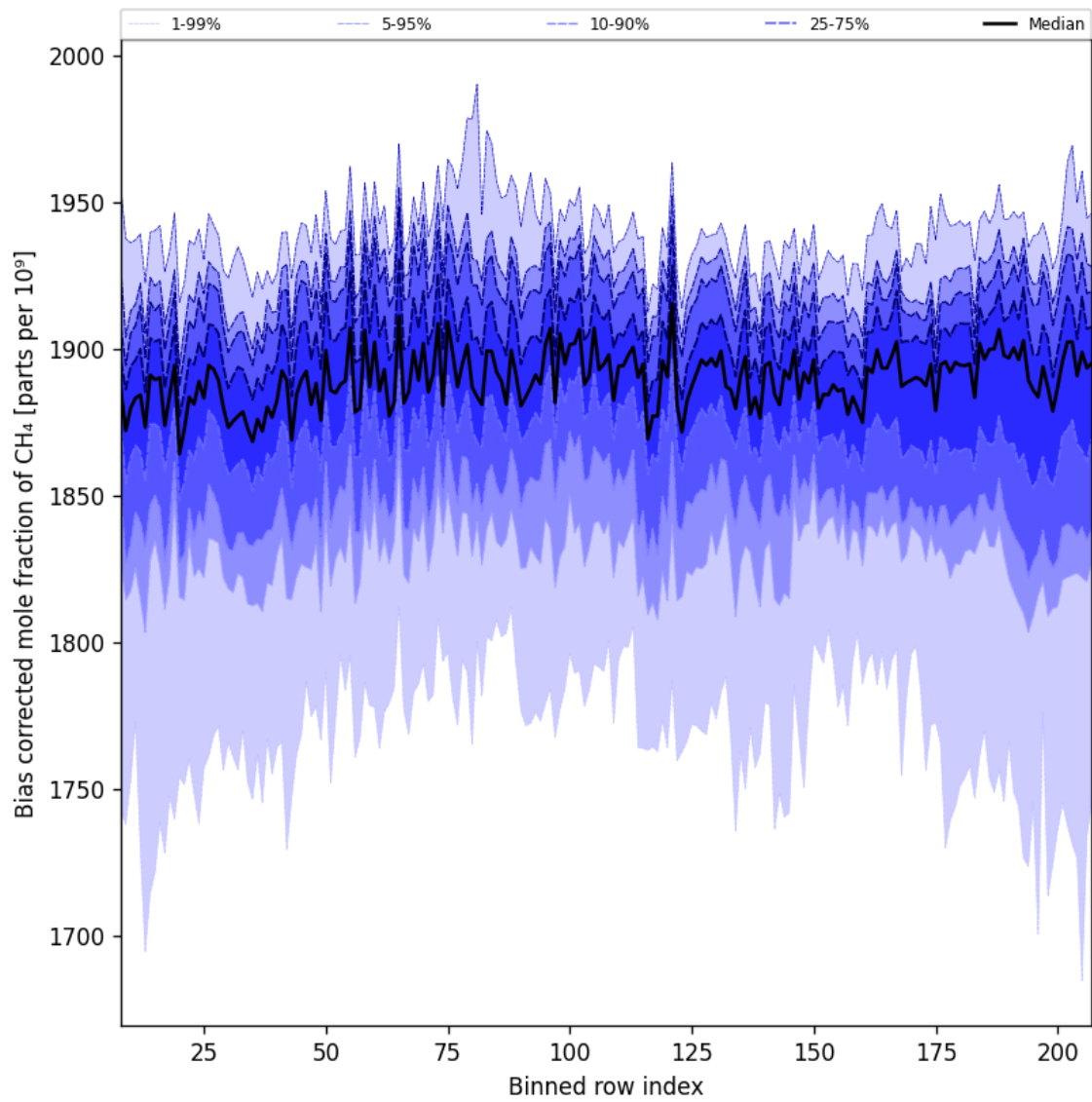
Figure 36: Along track statistics of “Bias corrected mole fraction of CH 4 ” for 2025-06-22 to 2025-06-24
