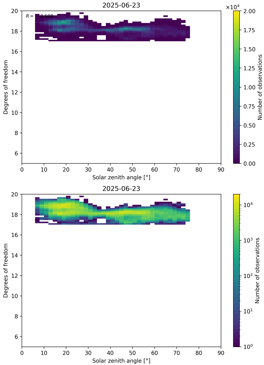
Figure 96: Scatter density plot of “Solar zenith angle” against “Degrees of freedom” for 2025-06-22 to 2025-06-24.
