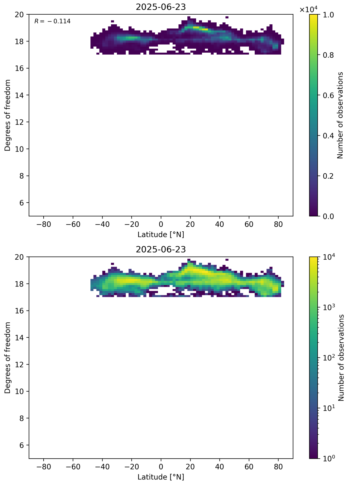
Figure 55: Scatter density plot of “Latitude” against “Degrees of freedom” for 2025-06-22 to 2025-06-24.
