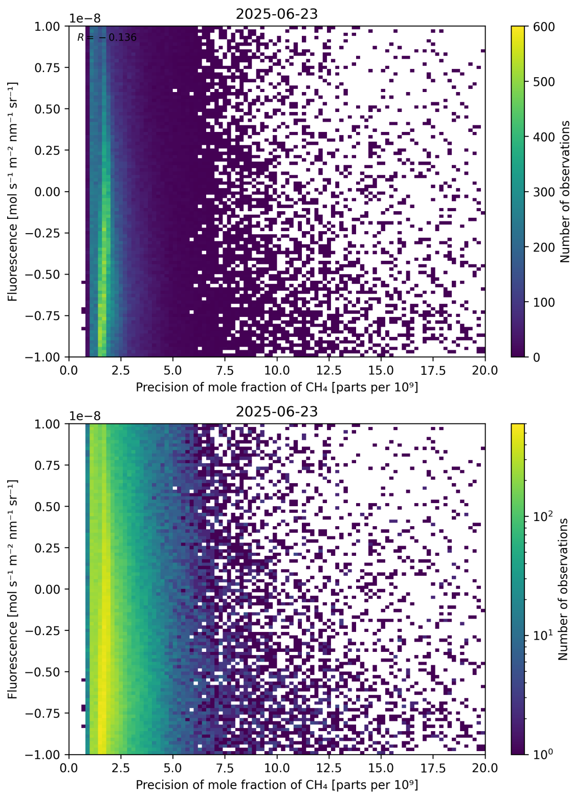
Figure 81: Scatter density plot of “Precision of mole fraction of CH 4 ” against “Fluorescence” for 2025-06-22 to 2025-06-24.
