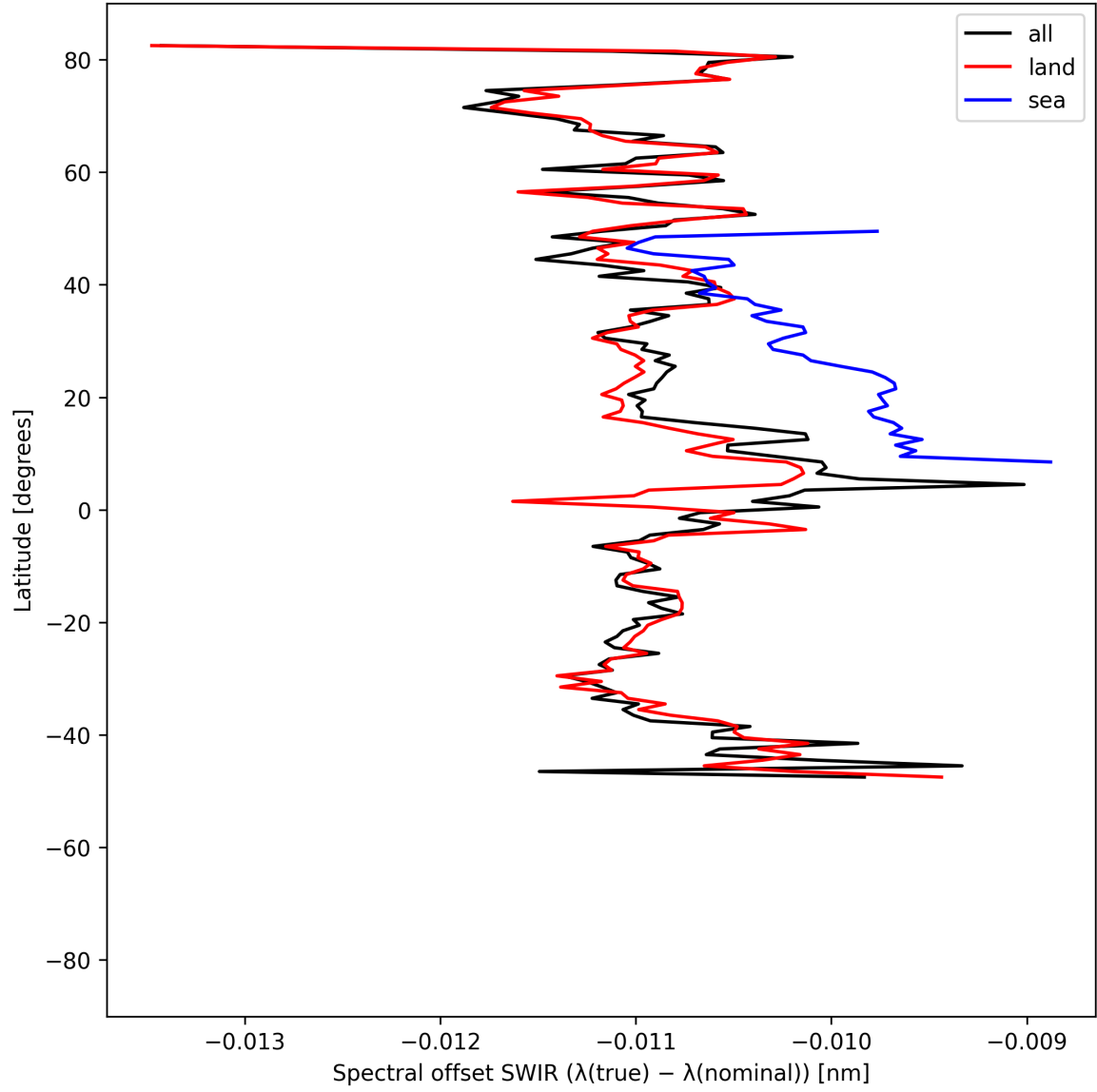
Figure 16: Zonal average of “Spectral offset SWIR ( \lambda_{\text{true}} - \lambda_{\text{nominal}} )” for 2025-06-22 to 2025-06-24.
