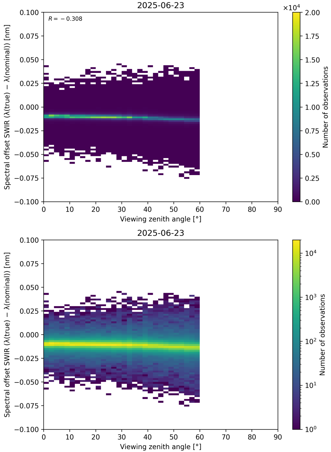
Figure 116: Scatter density plot of “Viewing zenith angle” against “Spectral offset SWIR ( \lambda_{\text{true}} - \lambda_{\text{nominal}} )” for 2025-06-22 to 2025-06-24.
