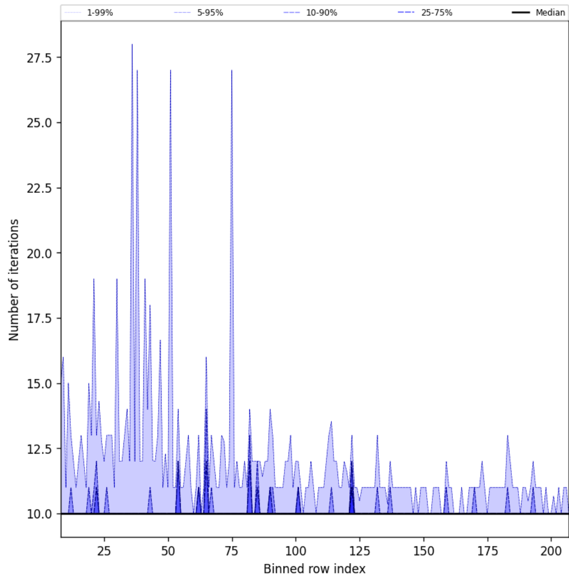
Figure 42: Along track statistics of “Number of iterations” for 2025-06-22 to 2025-06-24
