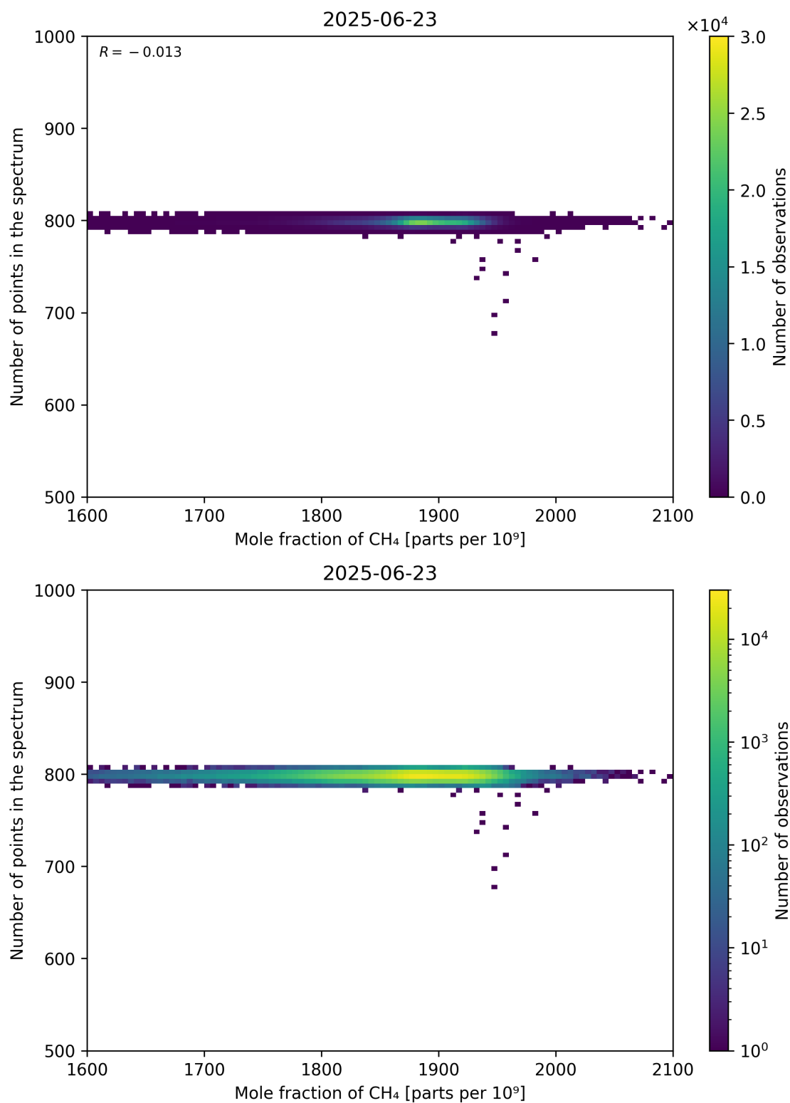
Figure 77: Scatter density plot of “Mole fraction of CH 4 ” against “Number of points in the spectrum” for 2025-06-22 to 2025-06-24.
