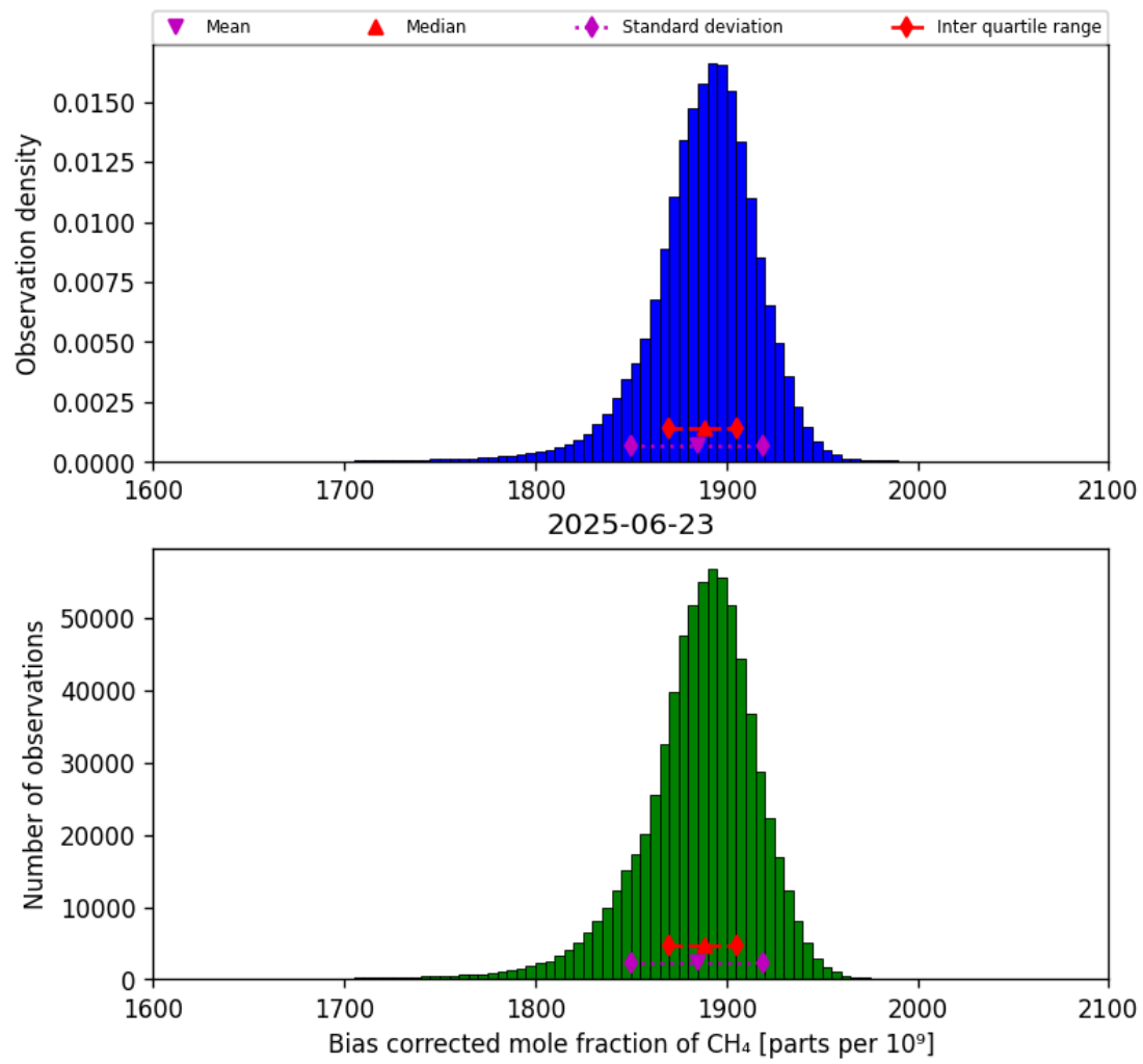
Figure 25: Histogram of “Bias corrected mole fraction of CH 4 ” for 2025-06-22 to 2025-06-24
