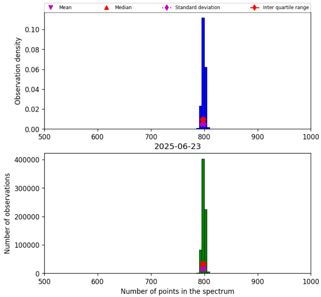
Figure 26: Histogram of “Number of points in the spectrum” for 2025-06-22 to 2025-06-24
