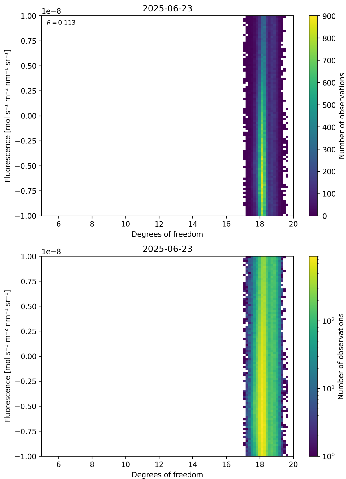
Figure 51: Scatter density plot of “Degrees of freedom” against “Fluorescence” for 2025-06-22 to 2025-06-24.
