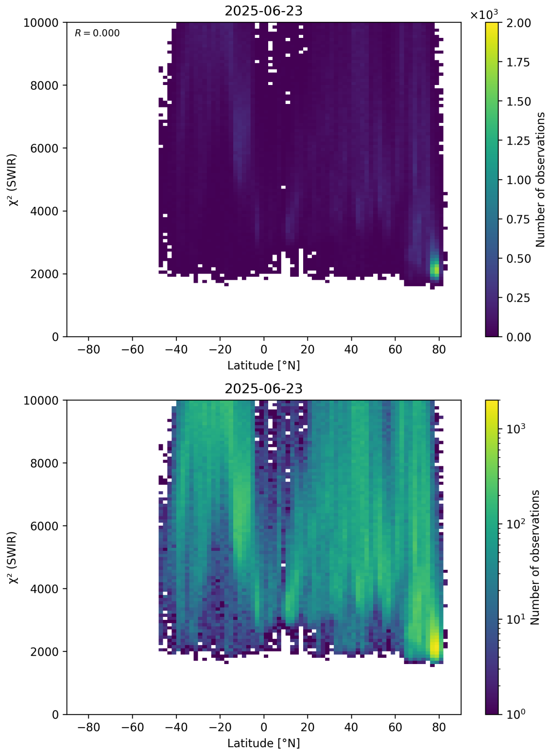
Figure 54: Scatter density plot of “Latitude” against “ \chi^2 (SWIR)” for 2025-06-22 to 2025-06-24.
