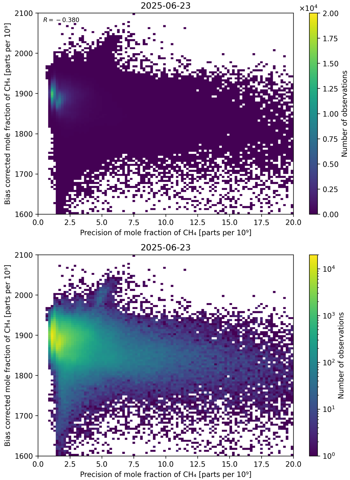
Figure 82: Scatter density plot of “Precision of mole fraction of \text{CH}_4 ” against “Bias corrected mole fraction of \text{CH}_4 ” for 2025-06-22 to 2025-06-24.
