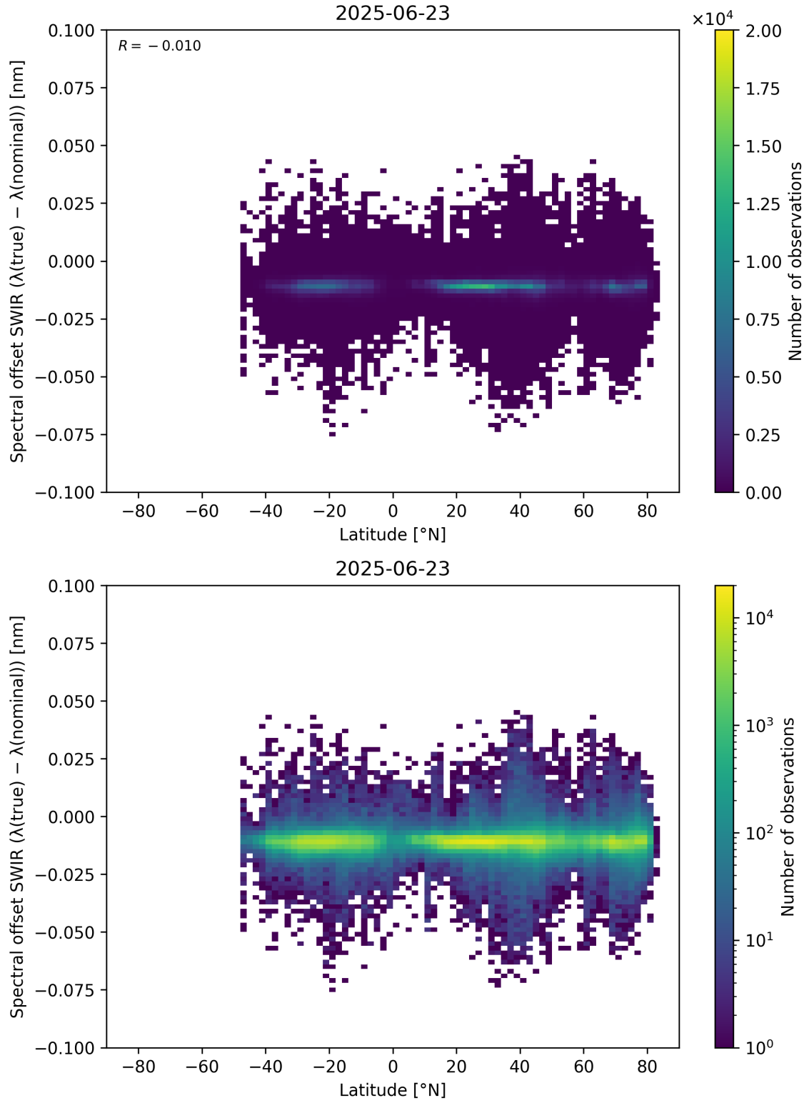
Figure 62: Scatter density plot of “Latitude” against “Spectral offset SWIR ( \lambda_{\text{true}} - \lambda_{\text{nominal}} )” for 2025-06-22 to 2025-06-24.
