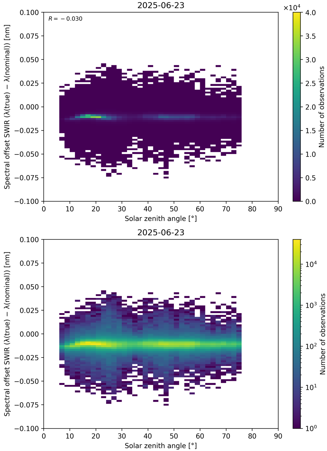
Figure 104: Scatter density plot of “Solar zenith angle” against “Spectral offset SWIR ( \lambda_{\text{true}} - \lambda_{\text{nominal}} )” for 2025-06-22 to 2025-06-24.
