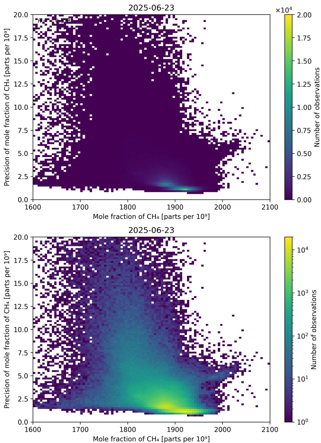
Figure 75: Scatter density plot of “Mole fraction of CH 4 ” against “Precision of mole fraction of CH 4 ” for 2025-06-22 to 2025-06-24.
