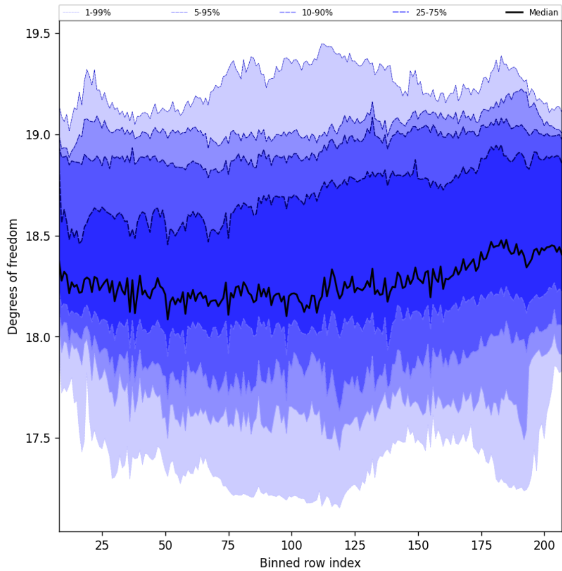
Figure 41: Along track statistics of “Degrees of freedom” for 2025-06-22 to 2025-06-24
