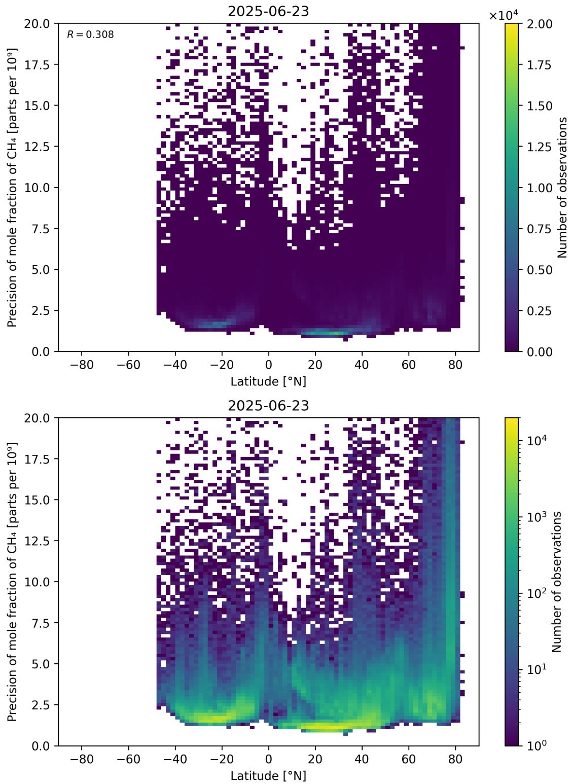
Figure 59: Scatter density plot of “Latitude” against “Precision of mole fraction of \text{CH}_4 ” for 2025-06-22 to 2025-06-24.
