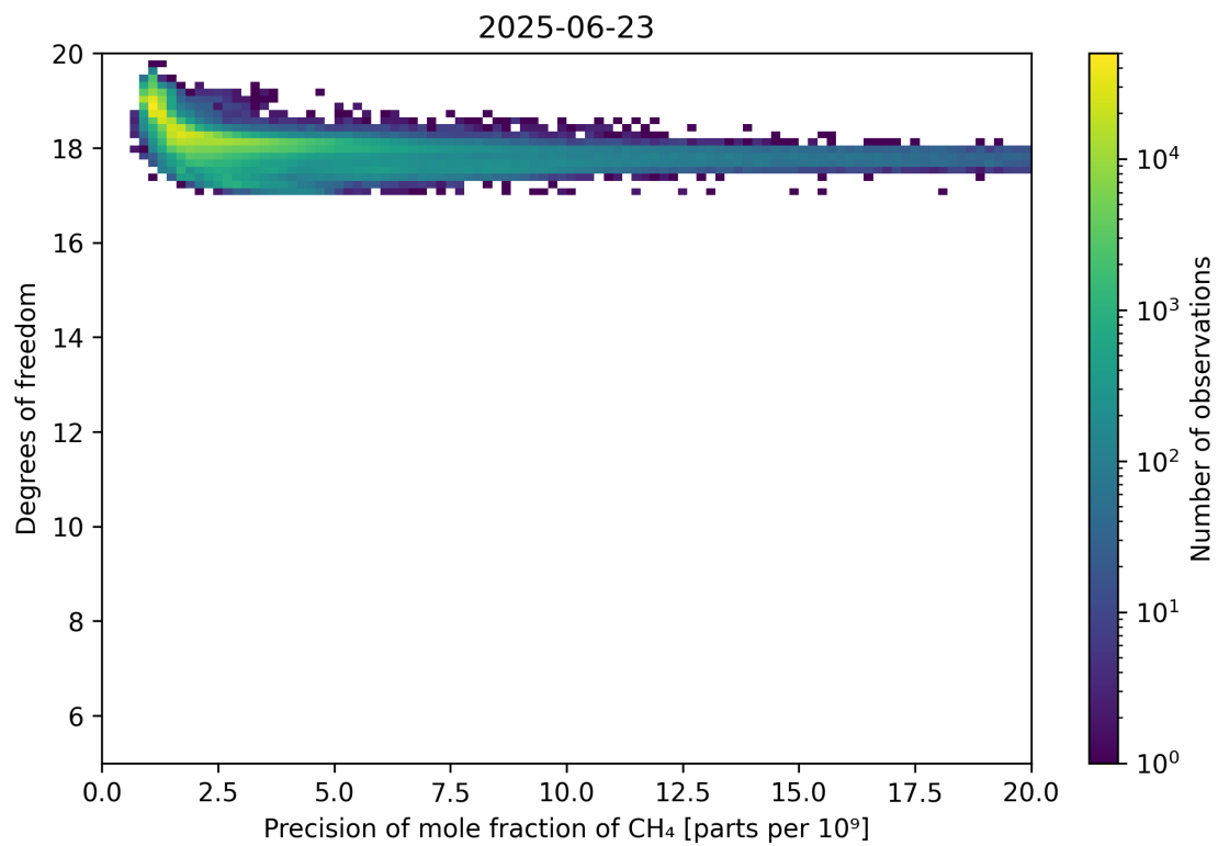
Figure 80: Scatter density plot of “Precision of mole fraction of CH 4 ” against “Degrees of freedom” for 2025-06-22 to 2025-06-24.
