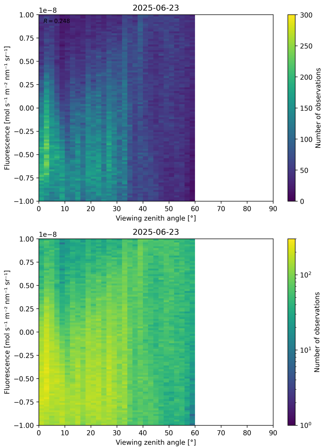
Figure 108: Scatter density plot of “Viewing zenith angle” against “Fluorescence” for 2025-06-22 to 2025-06-24.
