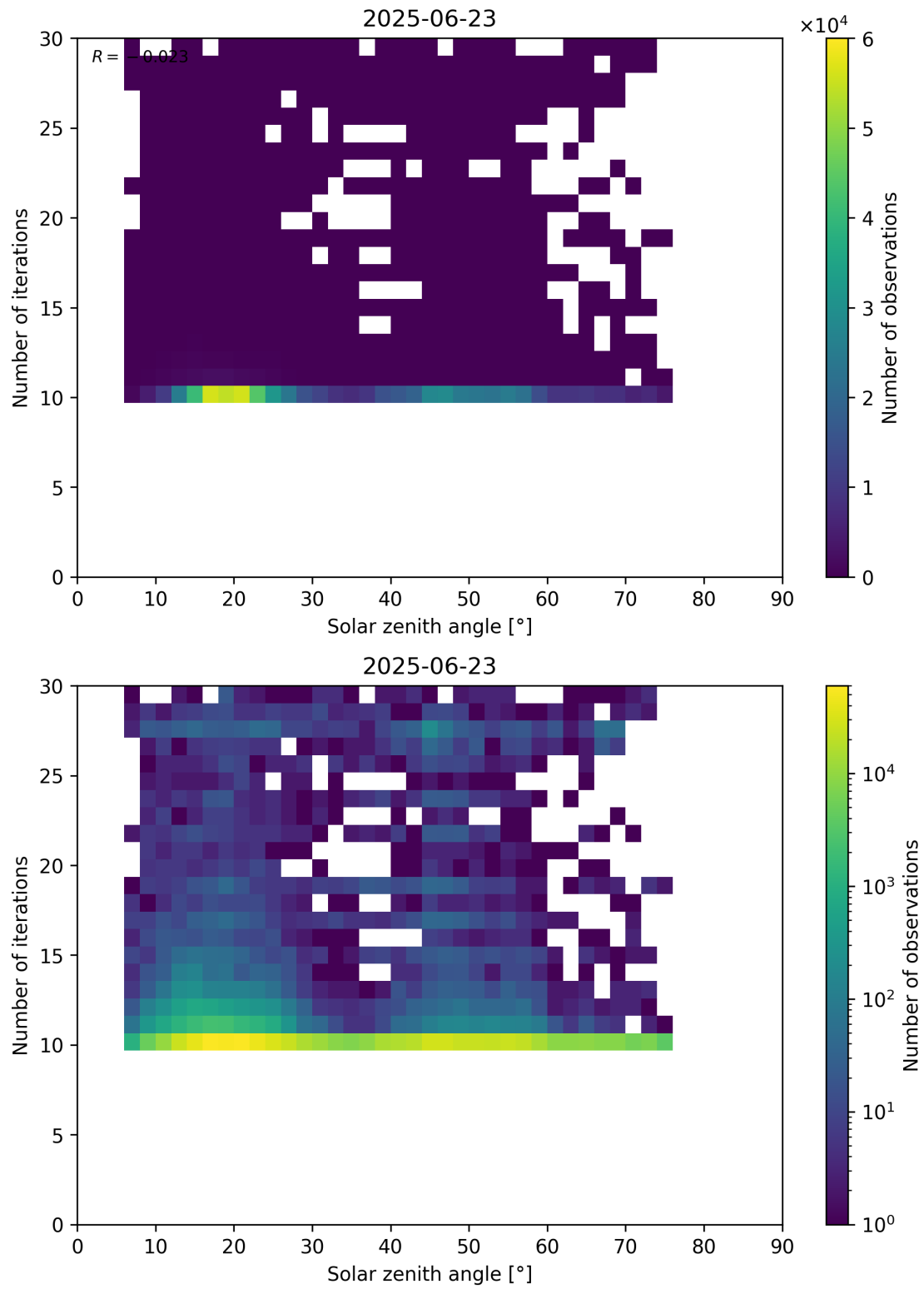
Figure 102: Scatter density plot of “Solar zenith angle” against “Number of iterations” for 2025-06-22 to 2025-06-24.
