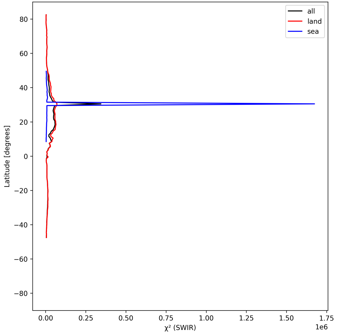
Figure 17: Zonal average of “ \chi^2 (SWIR)” for 2025-06-22 to 2025-06-24.
