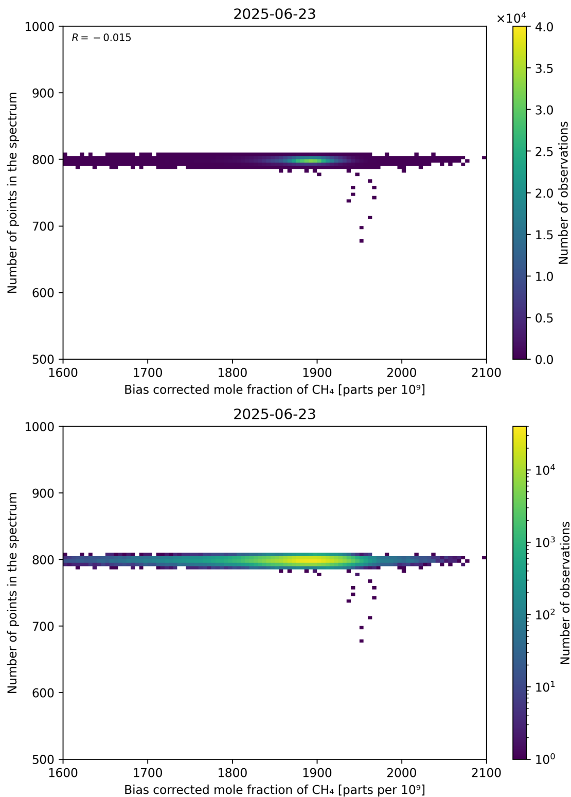
Figure 68: Scatter density plot of “Bias corrected mole fraction of CH 4 ” against “Number of points in the spectrum” for 2025-06-22 to 2025-06-24.
