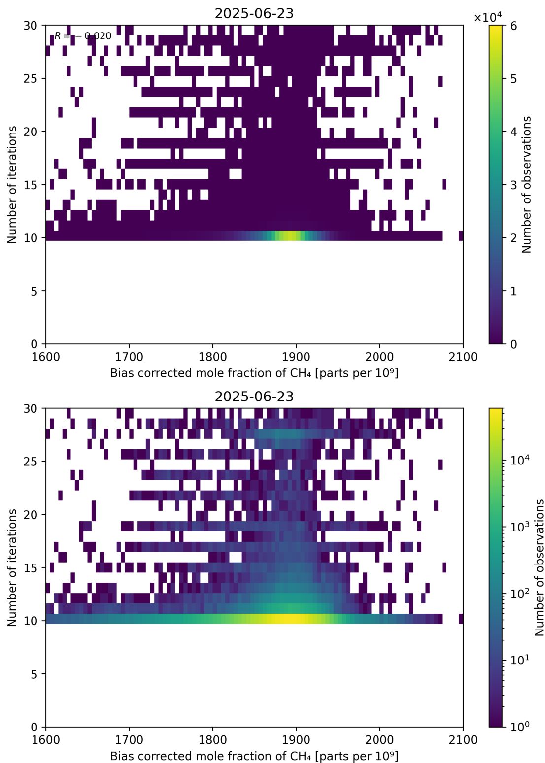
Figure 67: Scatter density plot of “Bias corrected mole fraction of CH 4 ” against “Number of iterations” for 2025-06-22 to 2025-06-24.
