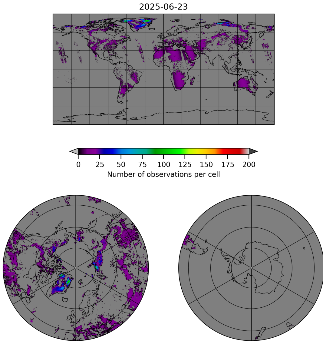
Figure 10: Map of the number of observations for 2025-06-22 to 2025-06-24
