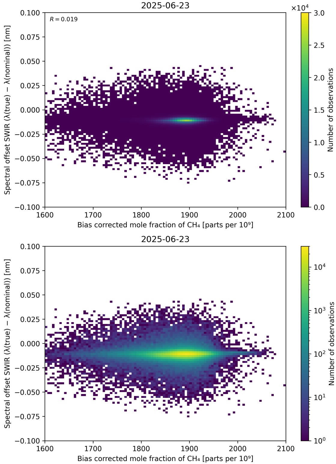
Figure 69: Scatter density plot of “Bias corrected mole fraction of \text{CH}_4 ” against “Spectral offset SWIR ( \lambda_{\text{true}} - \lambda_{\text{nominal}} )” for 2025-06-22 to 2025-06-24.
