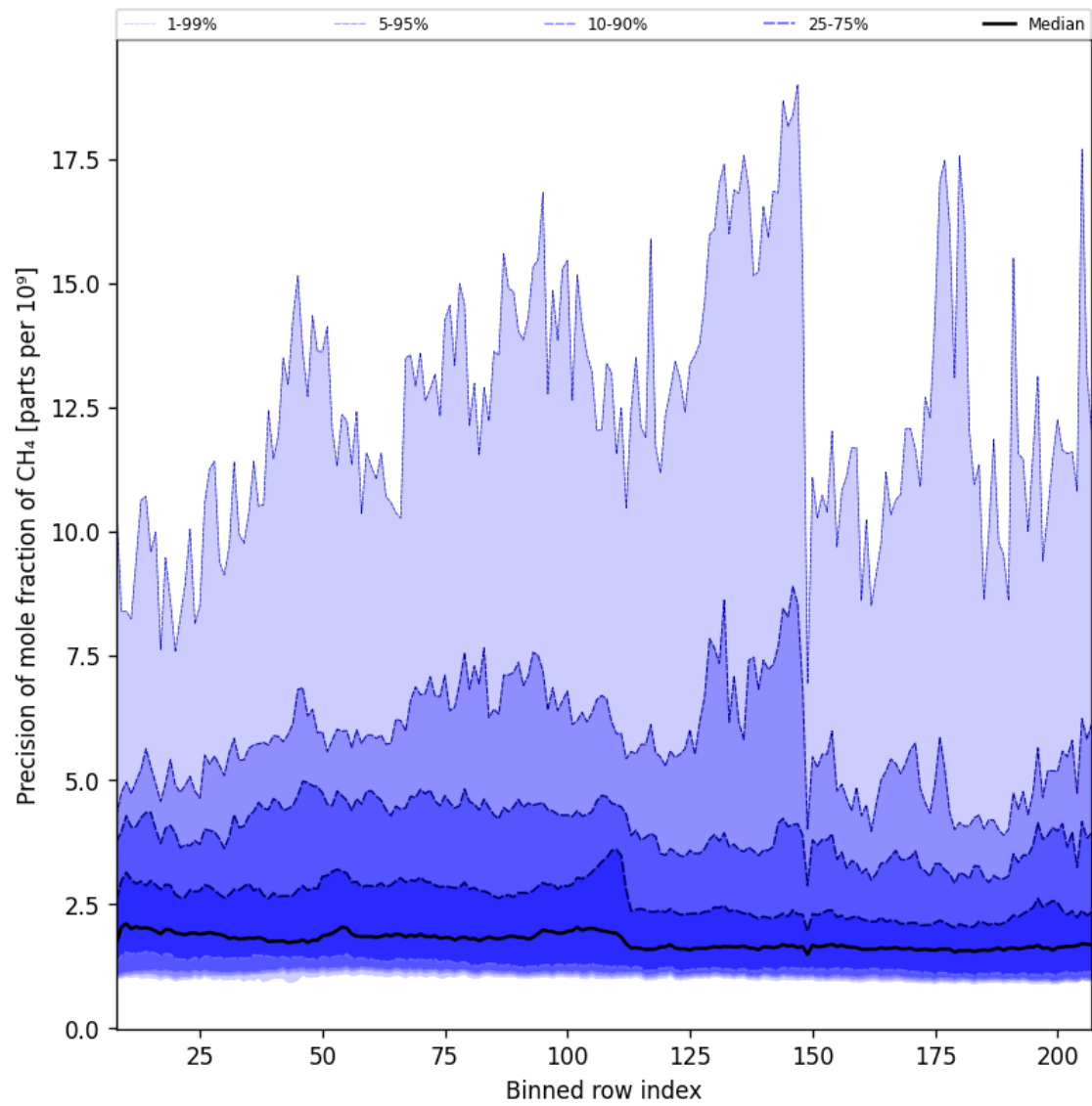
Figure 35: Along track statistics of “Precision of mole fraction of CH 4 ” for 2025-06-22 to 2025-06-24
