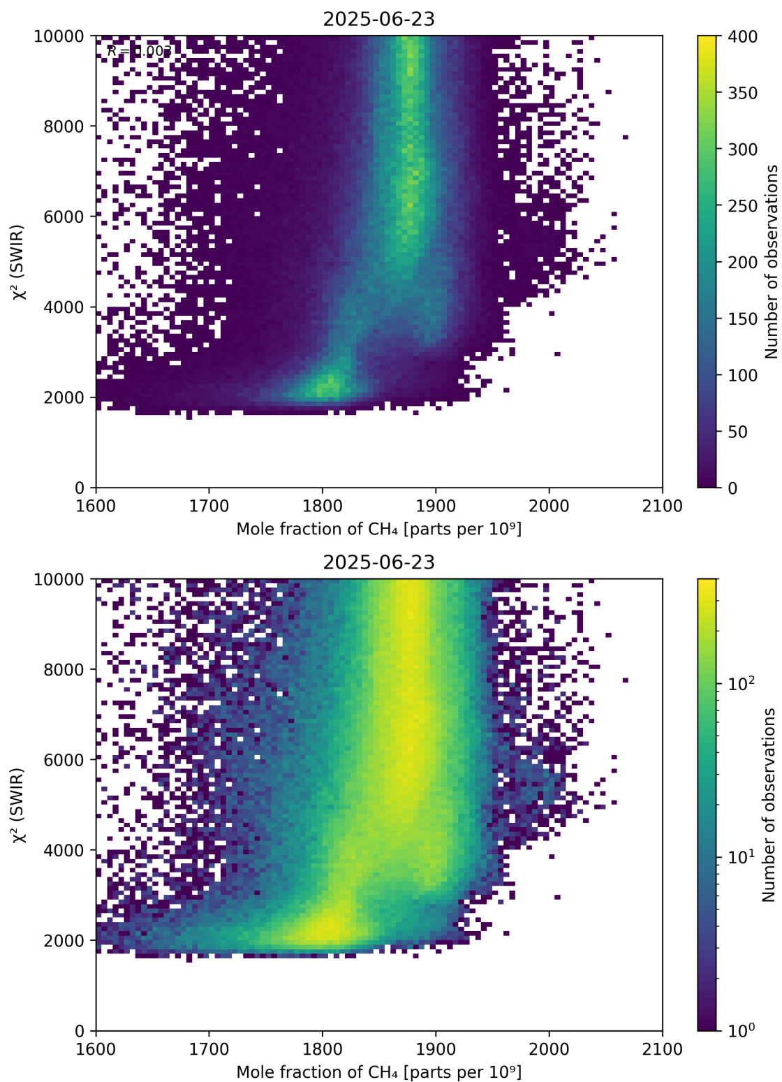
Figure 71: Scatter density plot of “Mole fraction of \text{CH}_4 ” against “ \chi^2 (SWIR)” for 2025-06-22 to 2025-06-24.
