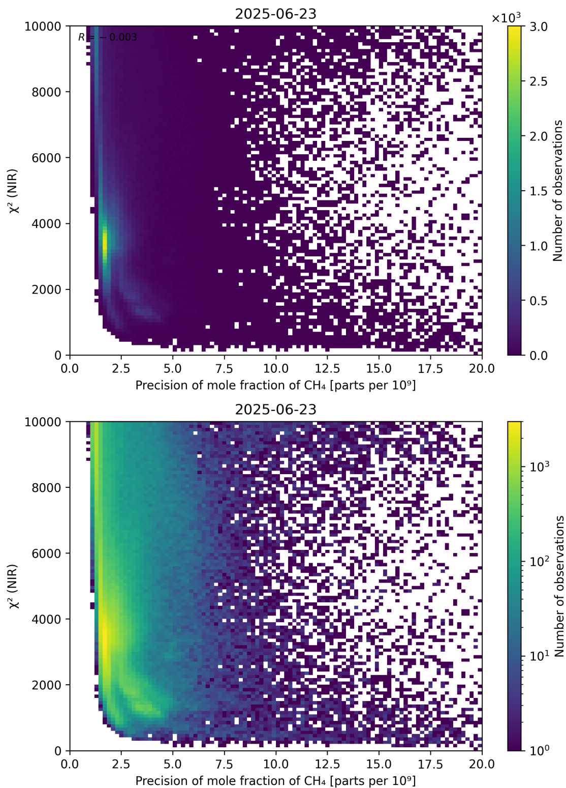
Figure 78: Scatter density plot of “Precision of mole fraction of CH 4 ” against “ \chi^2 (NIR)” for 2025-06-22 to 2025-06-24.
