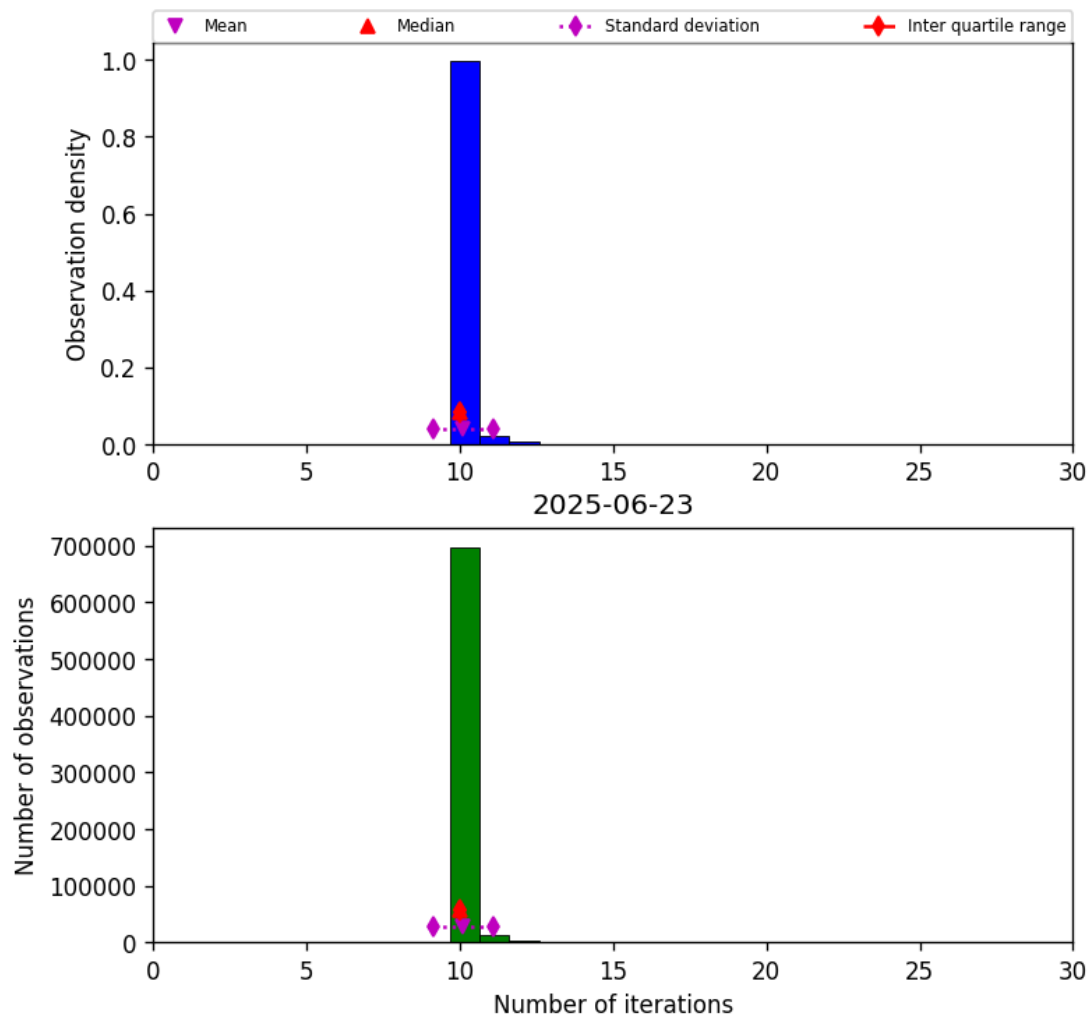
Figure 31: Histogram of “Number of iterations” for 2025-06-22 to 2025-06-24
