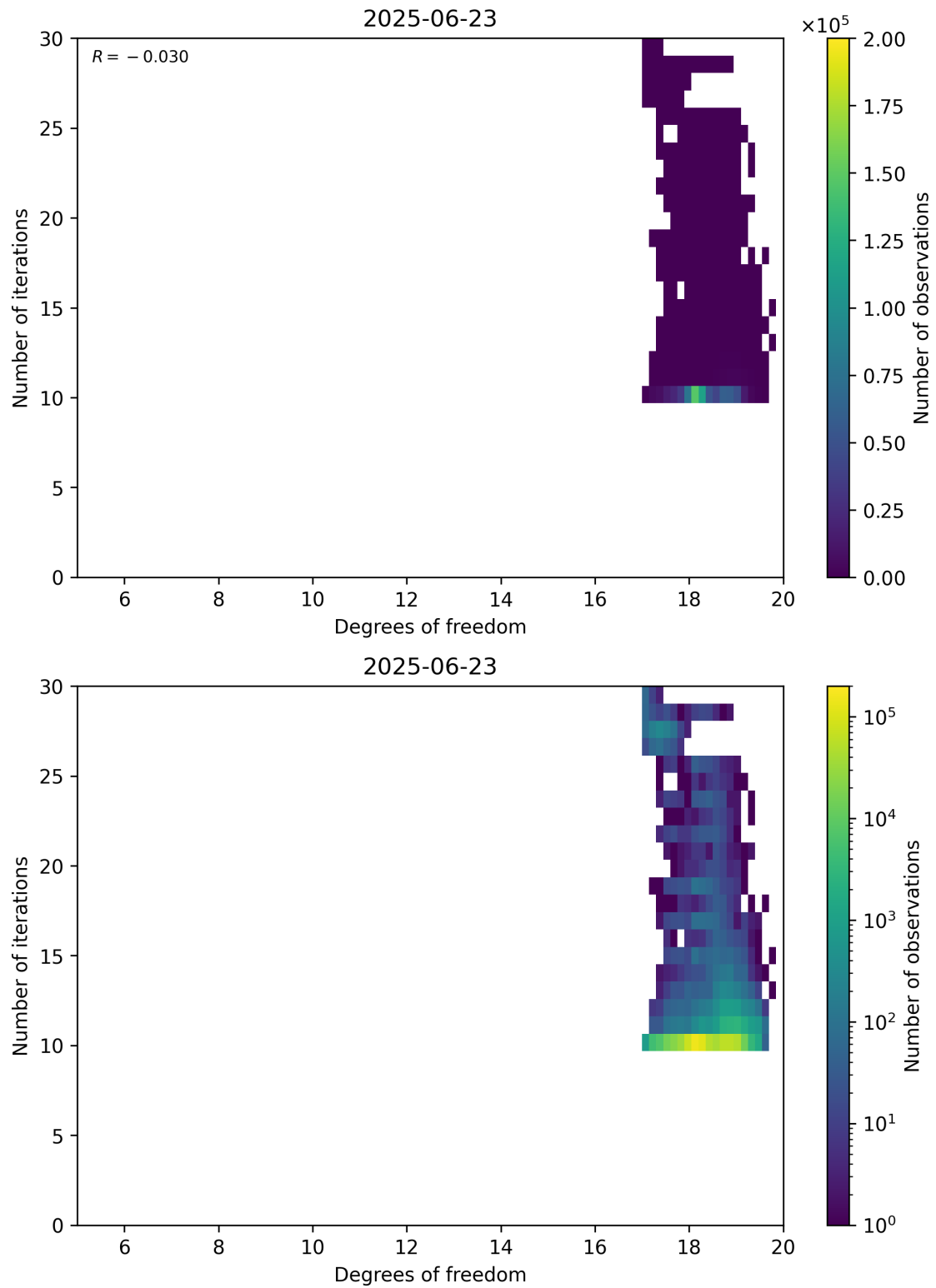
Figure 52: Scatter density plot of “Degrees of freedom” against “Number of iterations” for 2025-06-22 to 2025-06-24.
