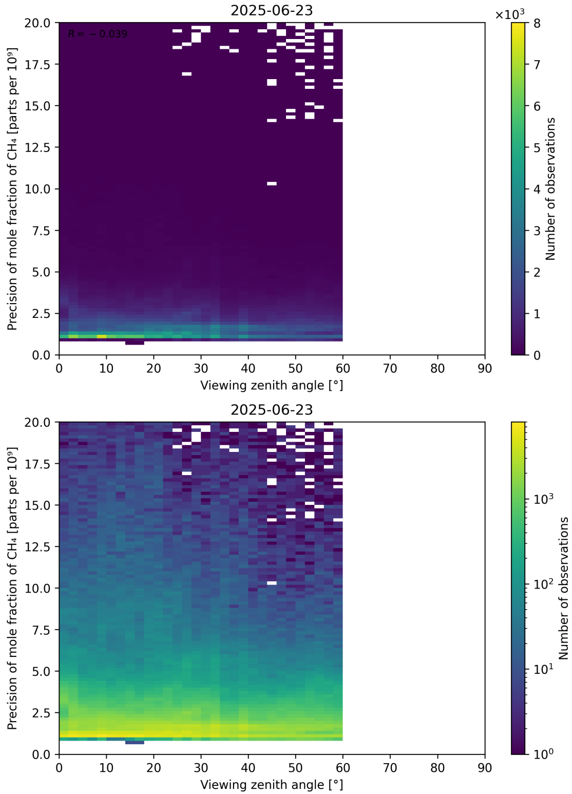
Figure 112: Scatter density plot of “Viewing zenith angle” against “Precision of mole fraction of \text{CH}_4 ” for 2025-06-22 to 2025-06-24.
