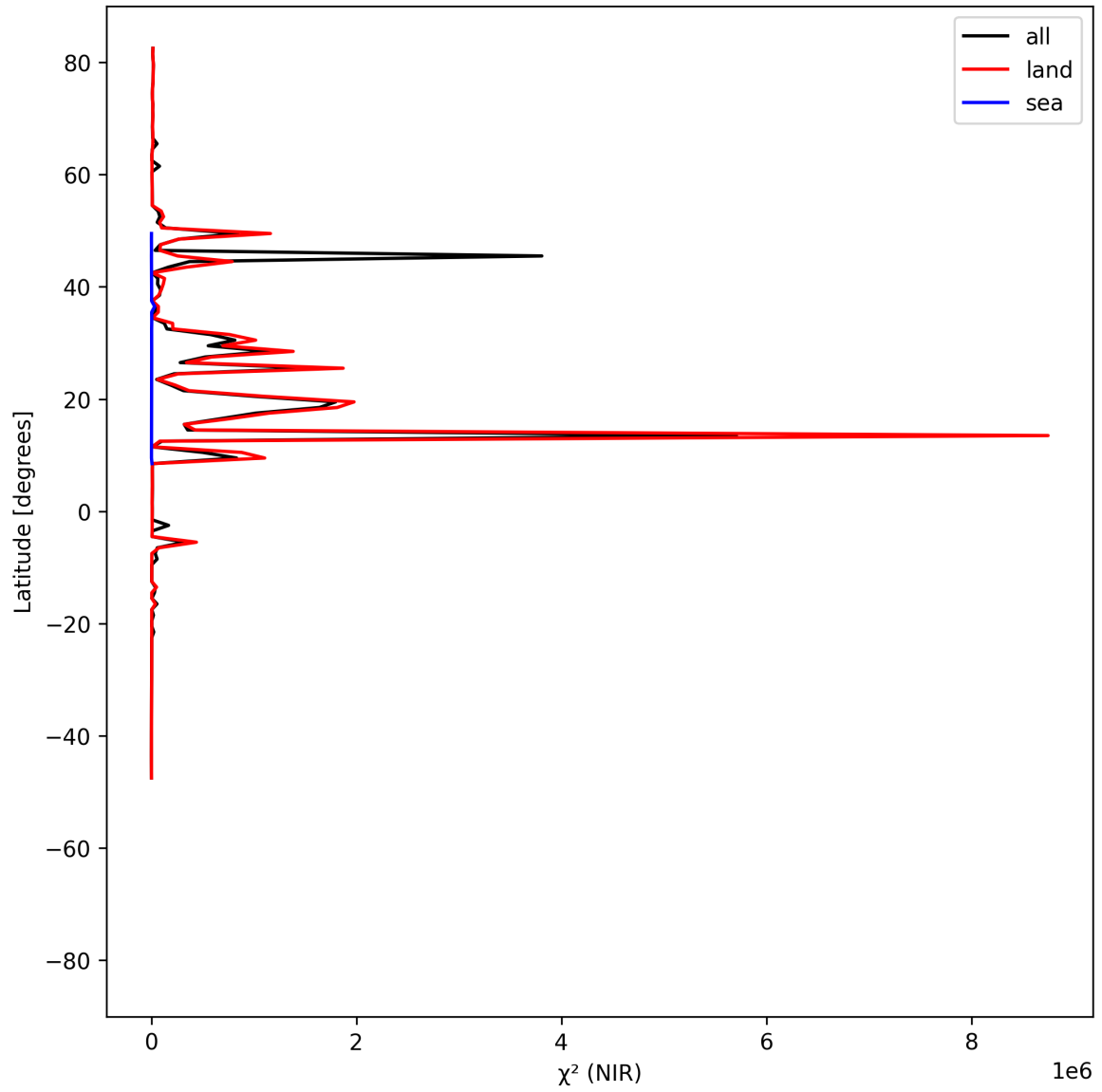
Figure 18: Zonal average of “ \chi^2 (NIR)” for 2025-06-22 to 2025-06-24.
