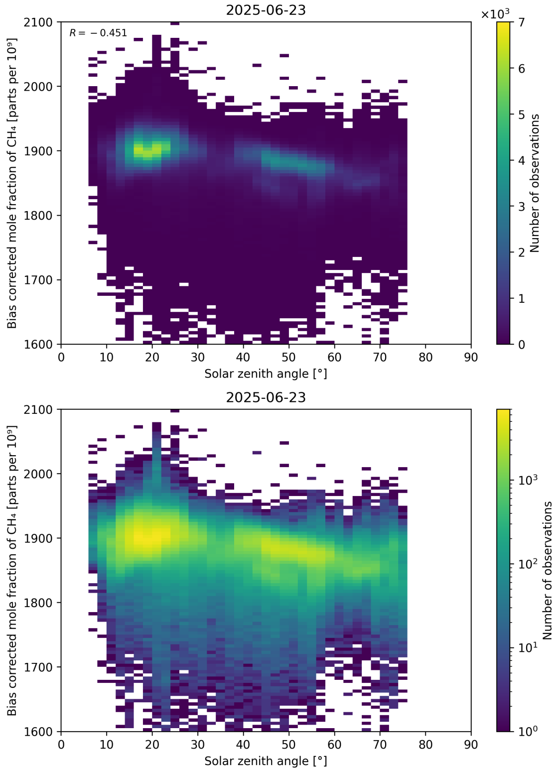
Figure 100: Scatter density plot of “Solar zenith angle” against “Bias corrected mole fraction of CH 4 ” for 2025-06-22 to 2025-06-24.
