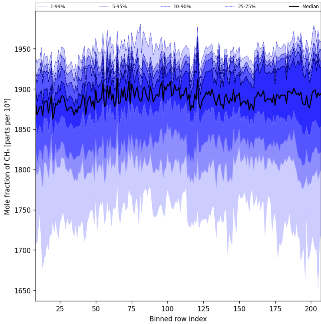
Figure 34: Along track statistics of “Mole fraction of CH 4 ” for 2025-06-22 to 2025-06-24
