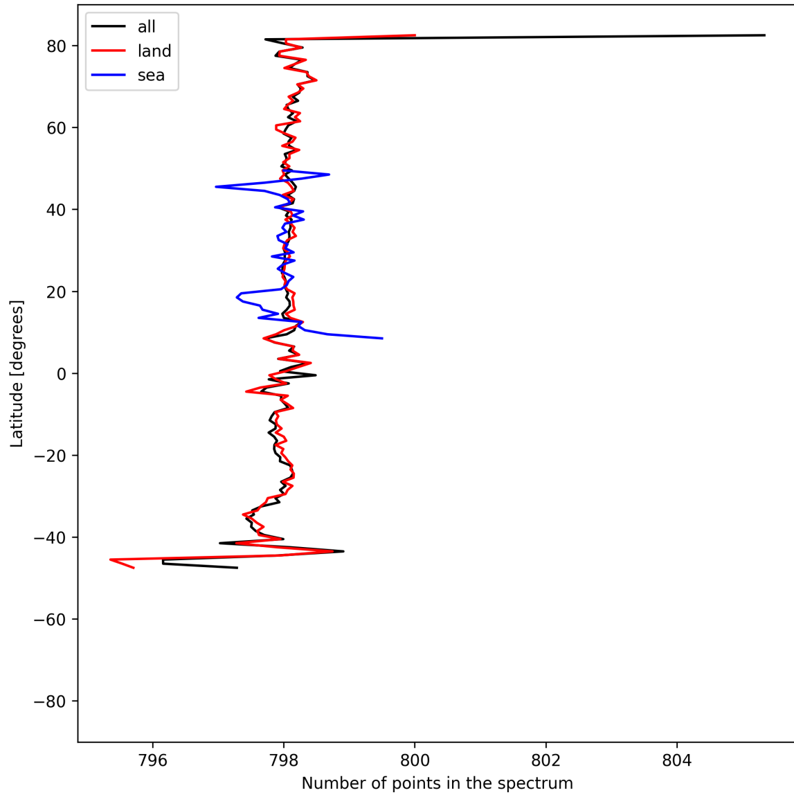
Figure 15: Zonal average of “Number of points in the spectrum” for 2025-06-22 to 2025-06-24.
