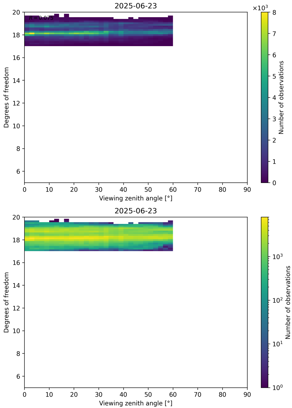
Figure 107: Scatter density plot of “Viewing zenith angle” against “Degrees of freedom” for 2025-06-22 to 2025-06-24.
