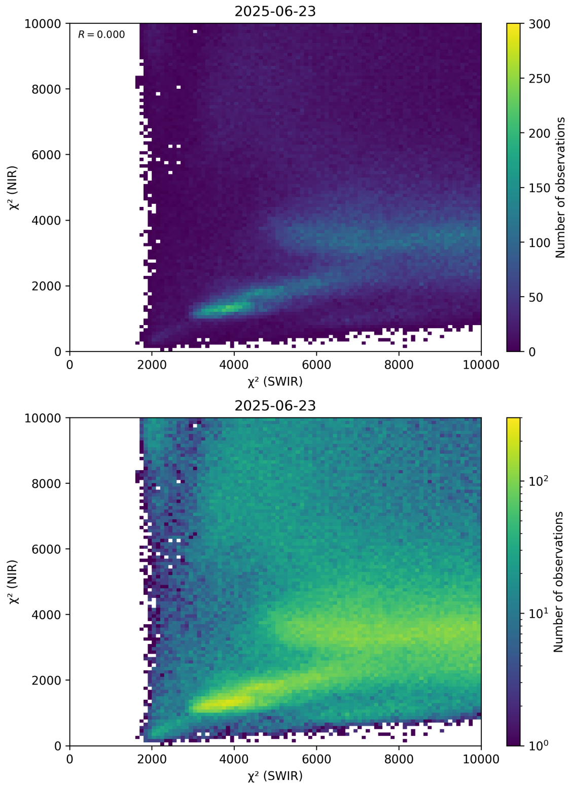
Figure 47: Scatter density plot of “ \chi^2 (SWIR)” against “ \chi^2 (NIR)” for 2025-06-22 to 2025-06-24.
