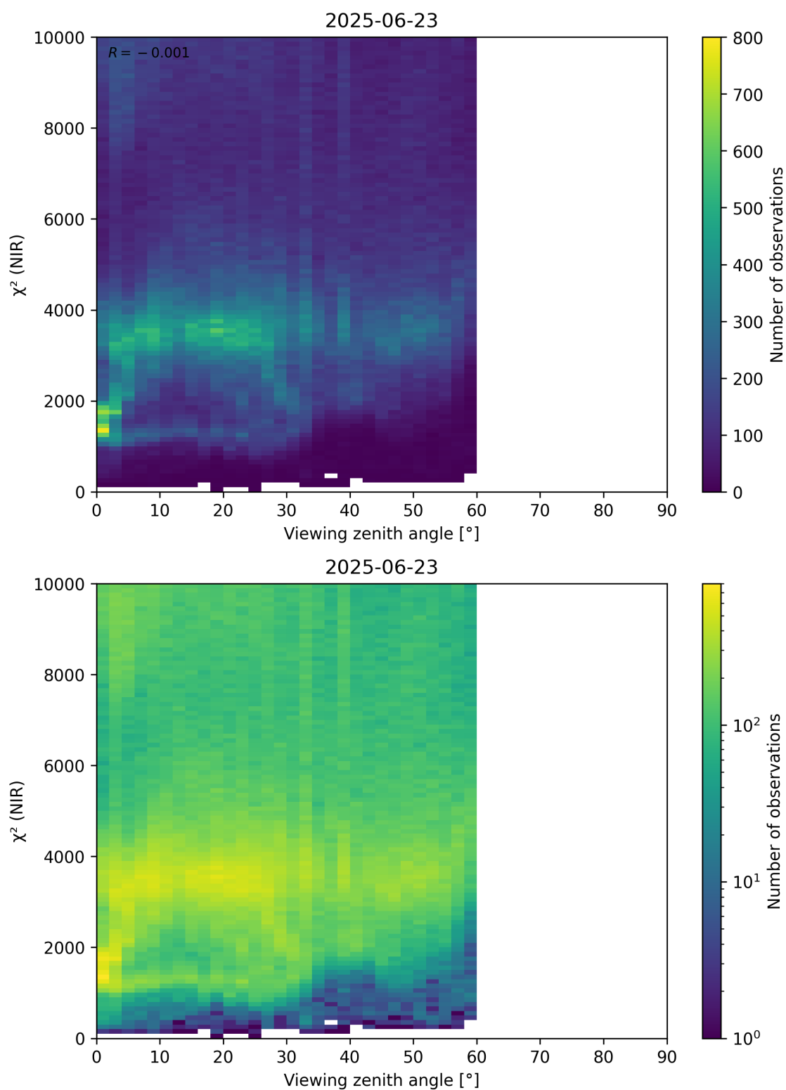
Figure 105: Scatter density plot of “Viewing zenith angle” against “ \chi^2 (NIR)” for 2025-06-22 to 2025-06-24.
