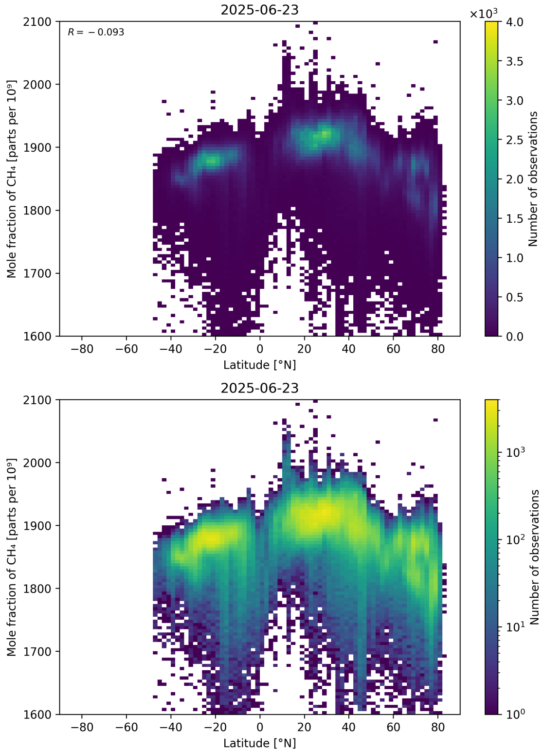
Figure 57: Scatter density plot of “Latitude” against “Mole fraction of CH 4 ” for 2025-06-22 to 2025-06-24.
