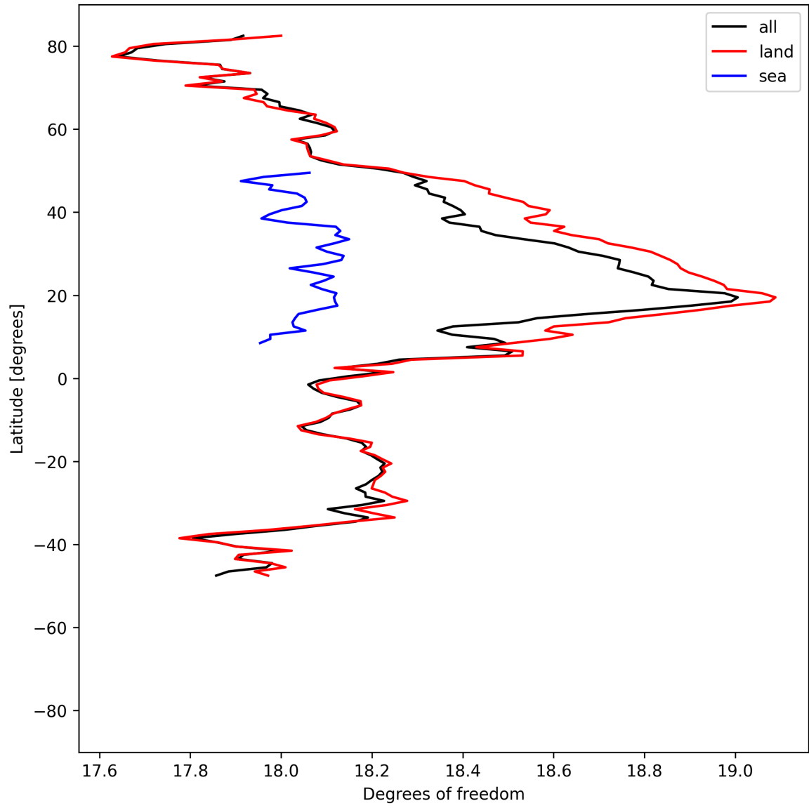
Figure 19: Zonal average of “Degrees of freedom” for 2025-06-22 to 2025-06-24.
