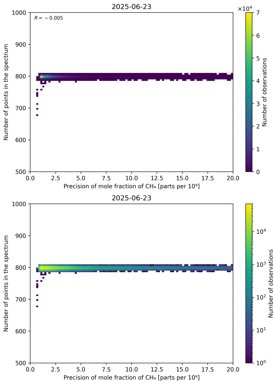
Figure 84: Scatter density plot of “Precision of mole fraction of CH 4 ” against “Number of points in the spectrum” for 2025-06-22 to 2025-06-24.
