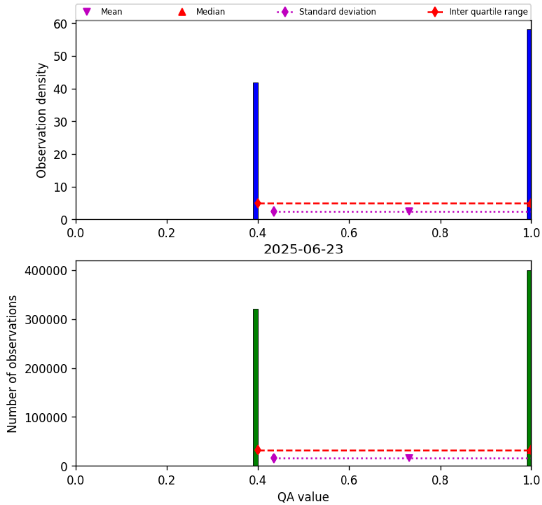
Figure 22: Histogram of “QA value” for 2025-06-22 to 2025-06-24
