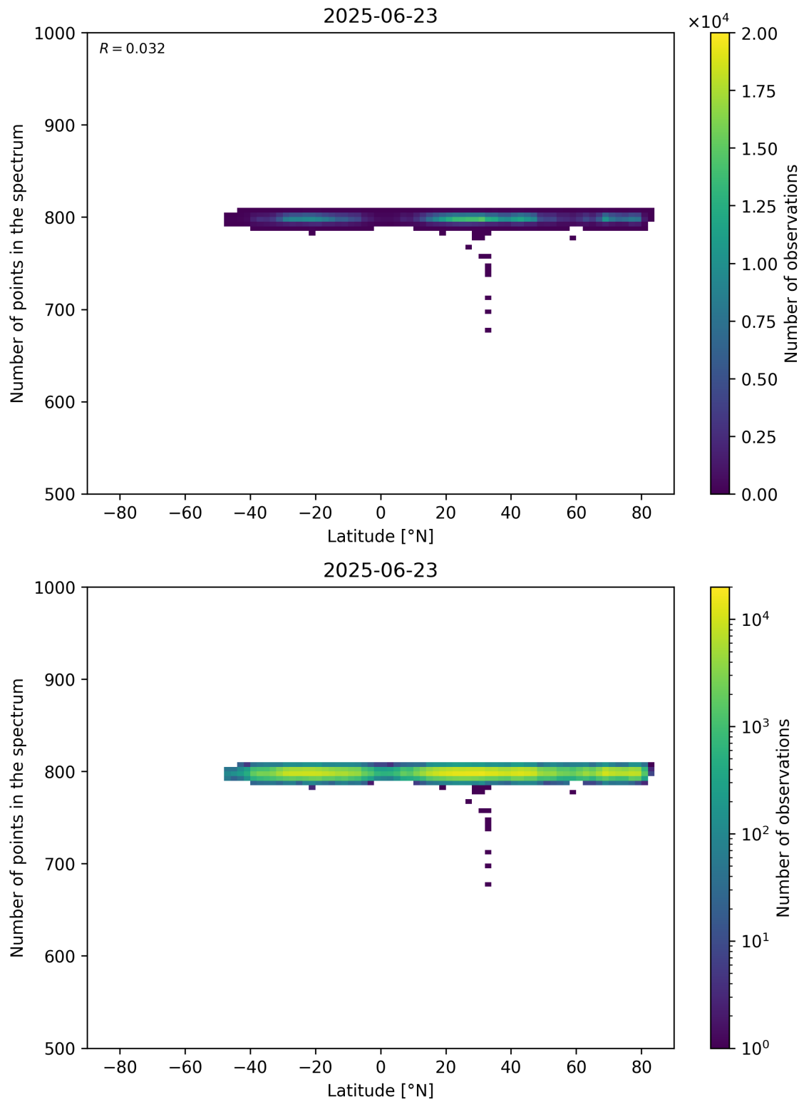
Figure 61: Scatter density plot of “Latitude” against “Number of points in the spectrum” for 2025-06-22 to 2025-06-24.
