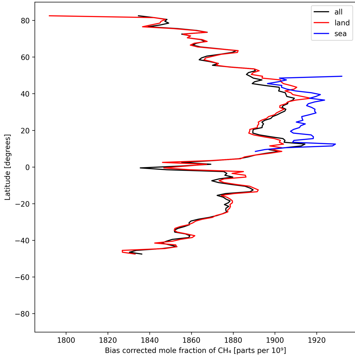
Figure 14: Zonal average of “Bias corrected mole fraction of \text{CH}_4 ” for 2025-06-22 to 2025-06-24.
