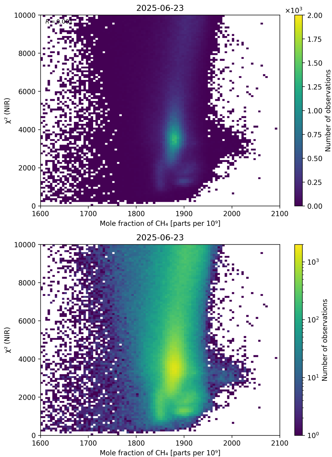
Figure 70: Scatter density plot of “Mole fraction of \text{CH}_4 ” against “ \chi^2 (NIR)” for 2025-06-22 to 2025-06-24.
