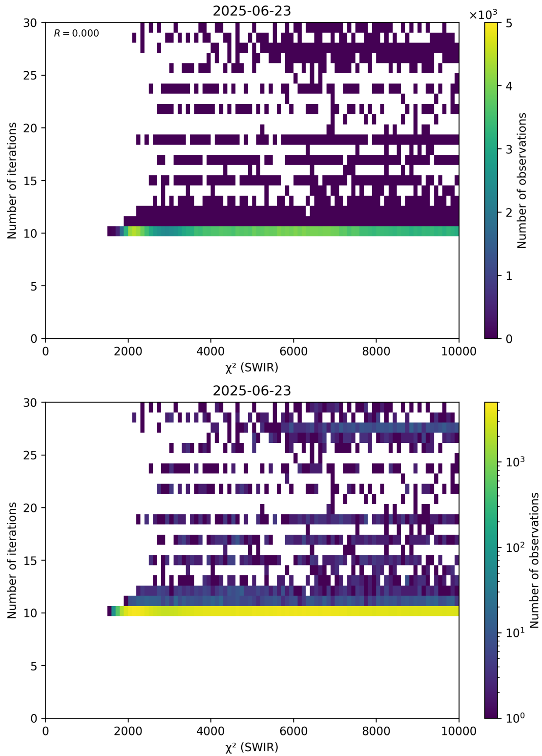
Figure 50: Scatter density plot of “ \chi^2 (SWIR)” against “Number of iterations” for 2025-06-22 to 2025-06-24.
