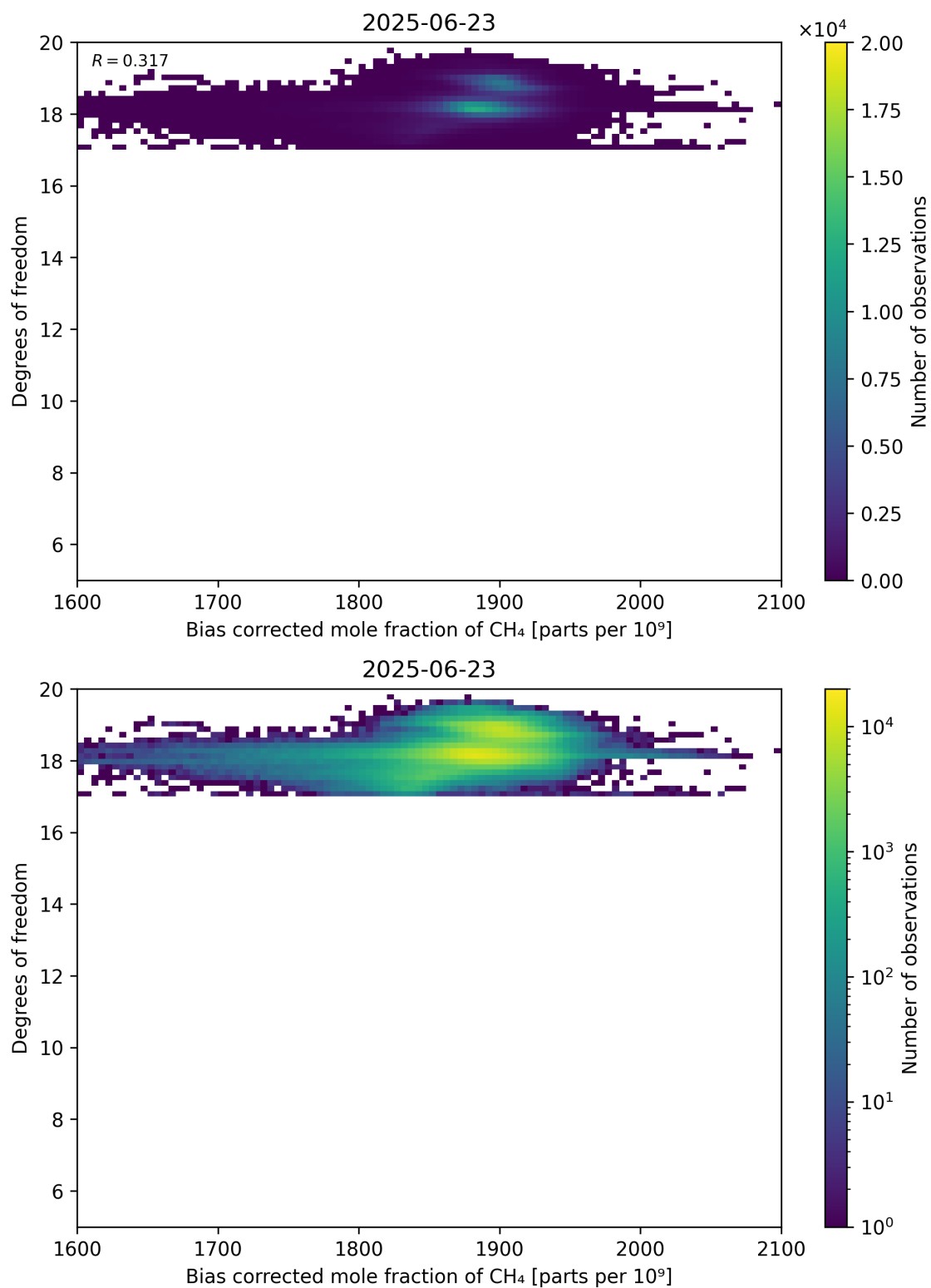
Figure 65: Scatter density plot of “Bias corrected mole fraction of CH 4 ” against “Degrees of freedom” for 2025-06-22 to 2025-06-24.
