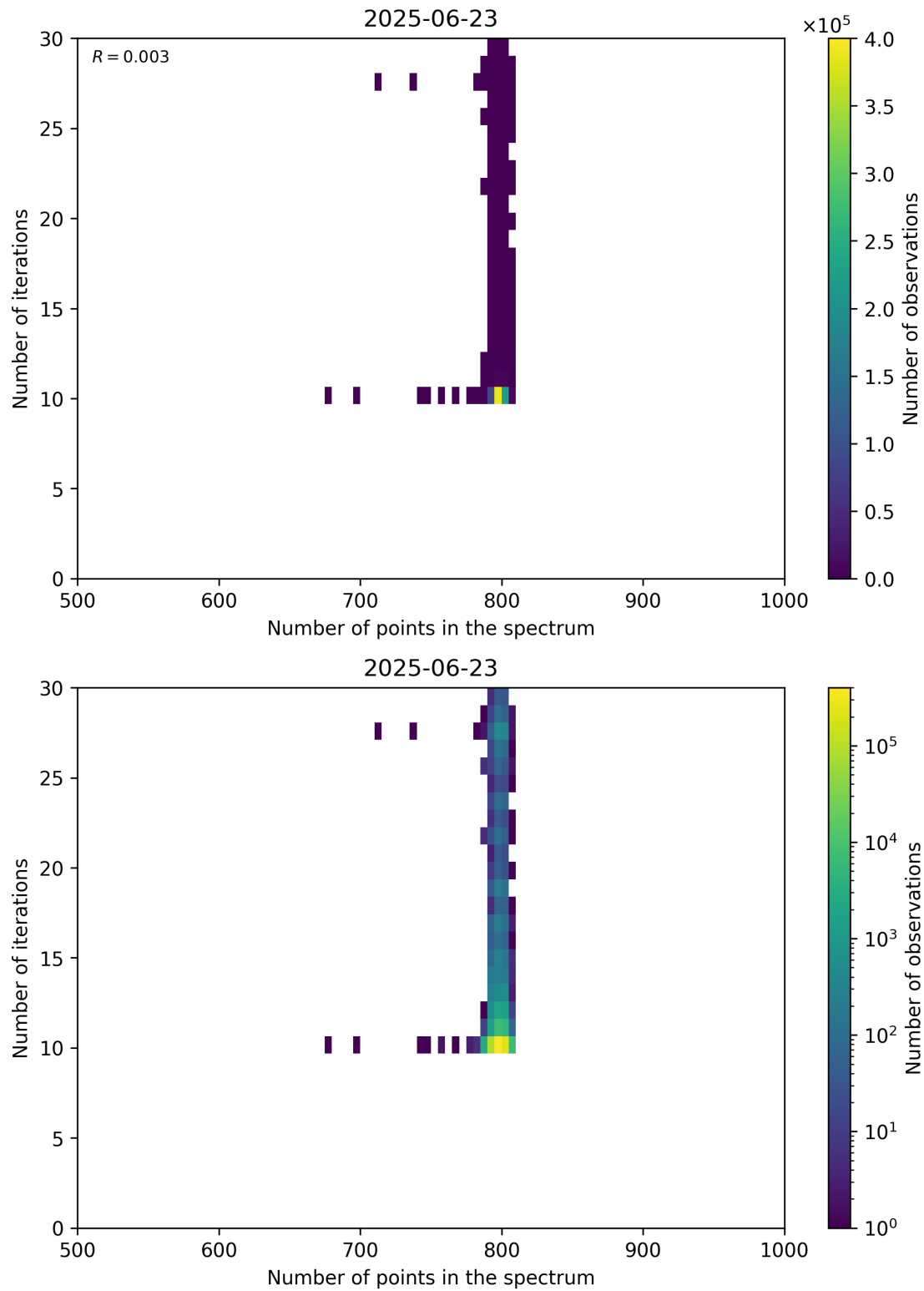
Figure 92: Scatter density plot of “Number of points in the spectrum” against “Number of iterations” for 2025-06-22 to 2025-06-24.
