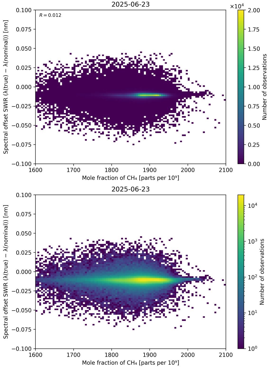
Figure 86: Scatter density plot of “Mole fraction of CH 4 ” against “Spectral offset SWIR ( \lambda_{\text{true}} - \lambda_{\text{nominal}} )” for 2025-06-22 to 2025-06-24.
