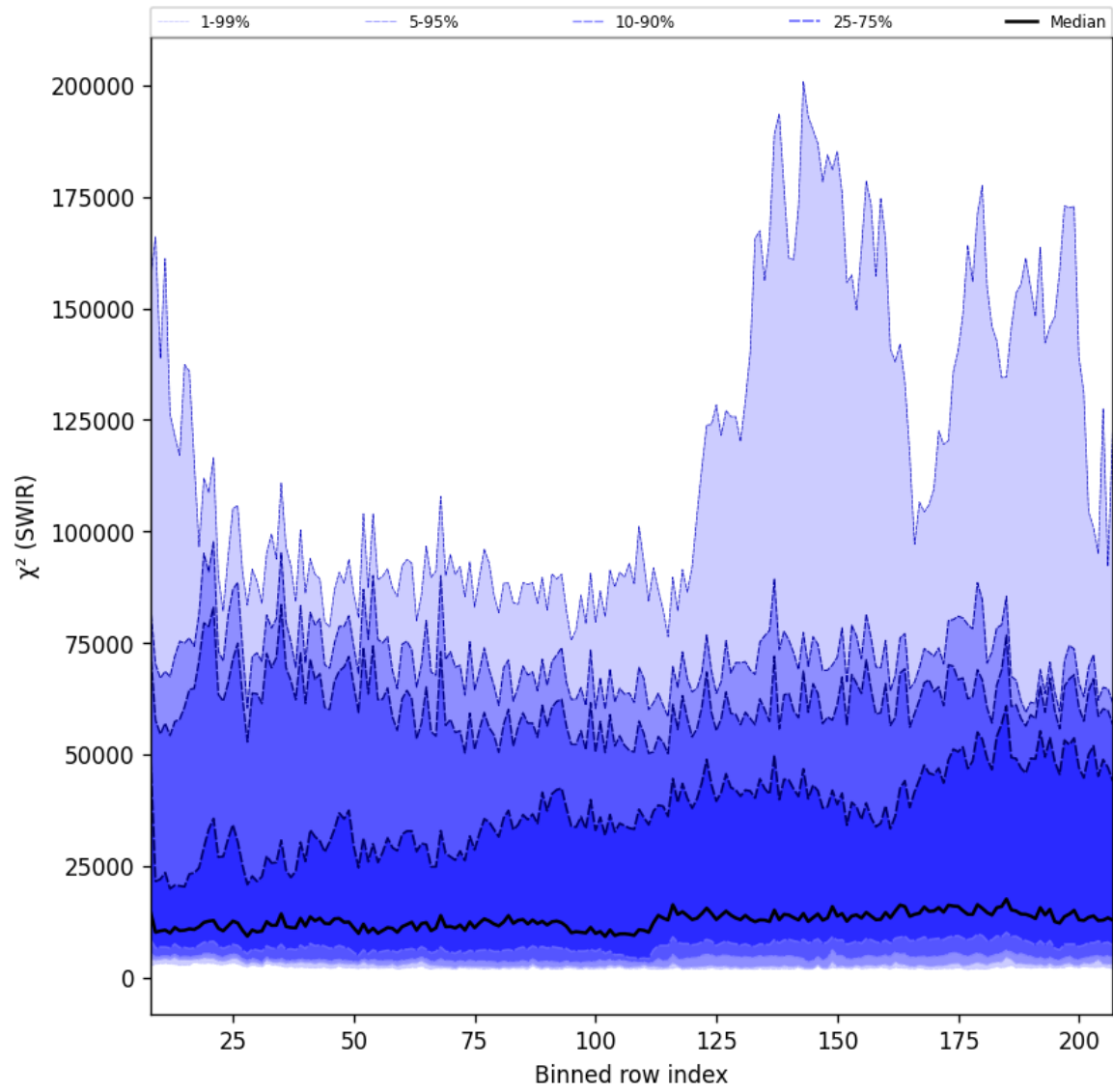
Figure 39: Along track statistics of “ \chi^2 (SWIR)” for 2025-06-22 to 2025-06-24
