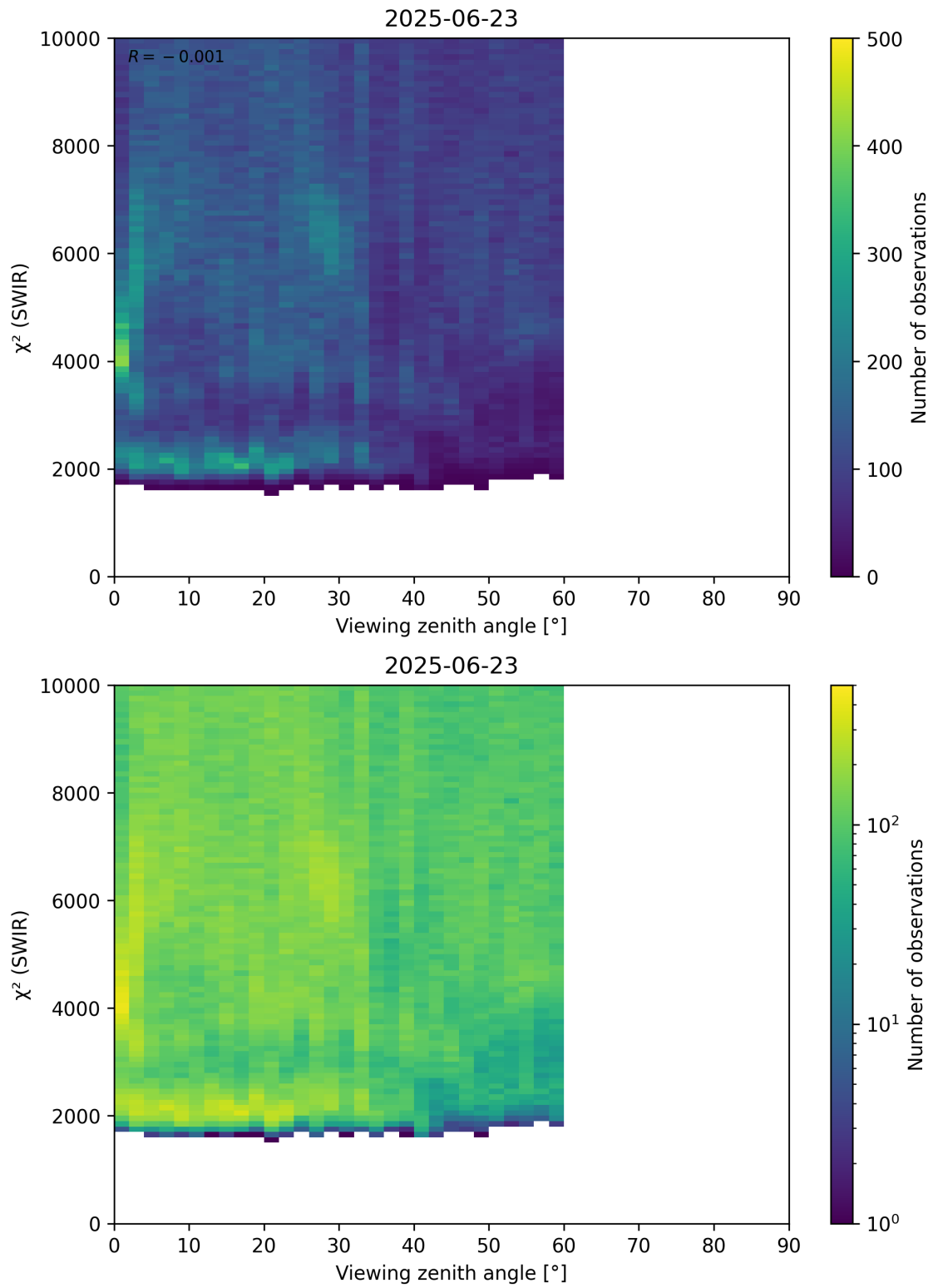
Figure 106: Scatter density plot of “Viewing zenith angle” against “ \chi^2 (SWIR)” for 2025-06-22 to 2025-06-24.
