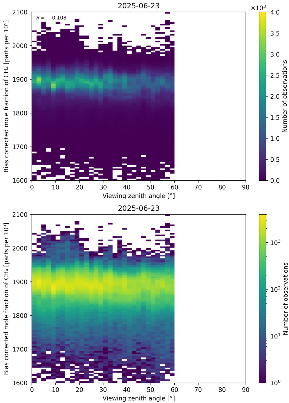
Figure 111: Scatter density plot of “Viewing zenith angle” against “Bias corrected mole fraction of CH 4 ” for 2025-06-22 to 2025-06-24.
