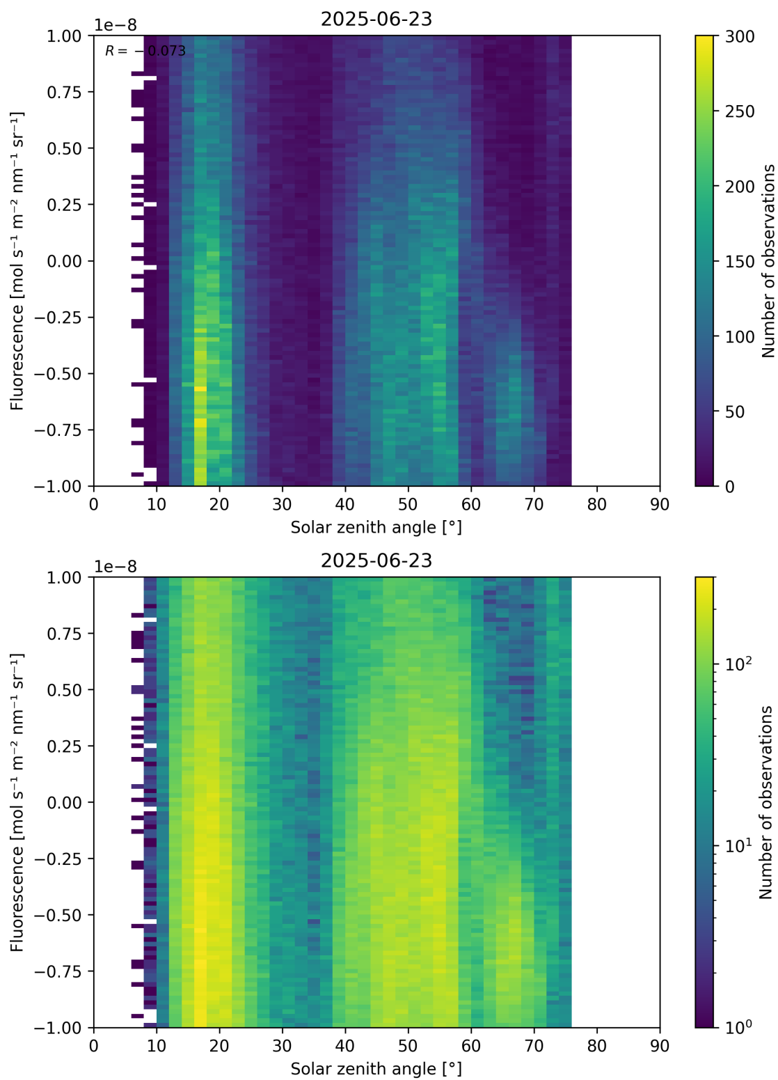
Figure 97: Scatter density plot of “Solar zenith angle” against “Fluorescence” for 2025-06-22 to 2025-06-24.
