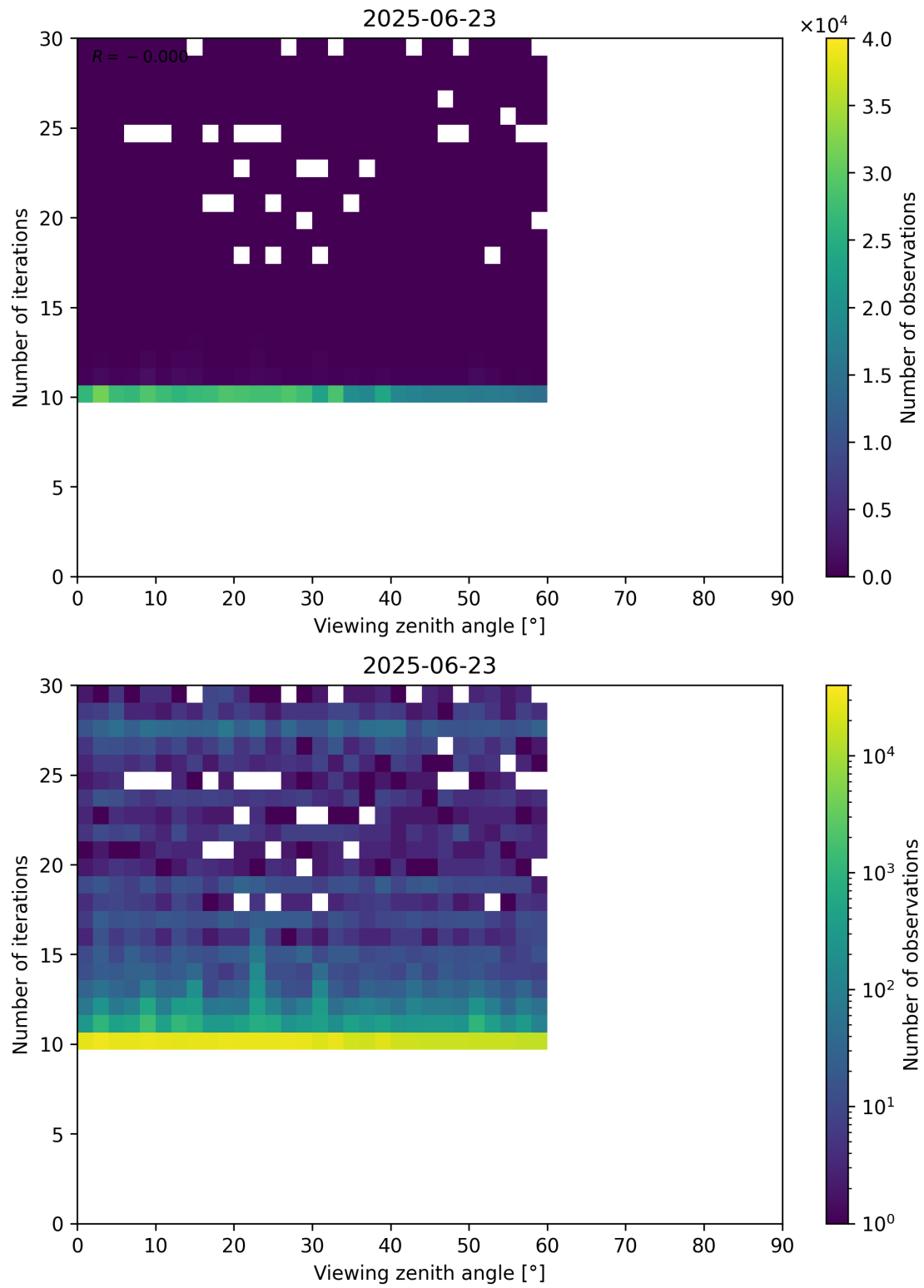
Figure 113: Scatter density plot of “Viewing zenith angle” against “Number of iterations” for 2025-06-22 to 2025-06-24.
