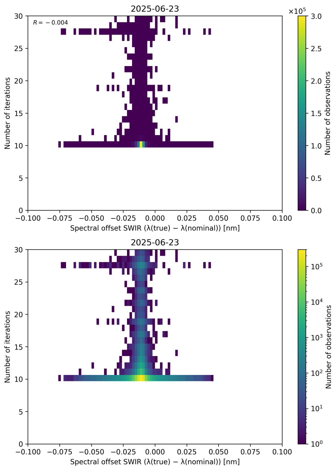
Figure 121: Scatter density plot of “Spectral offset SWIR ( \lambda_{\text{true}} - \lambda_{\text{nominal}} )” against “Number of iterations” for 2025-06-22 to 2025-06-24.
