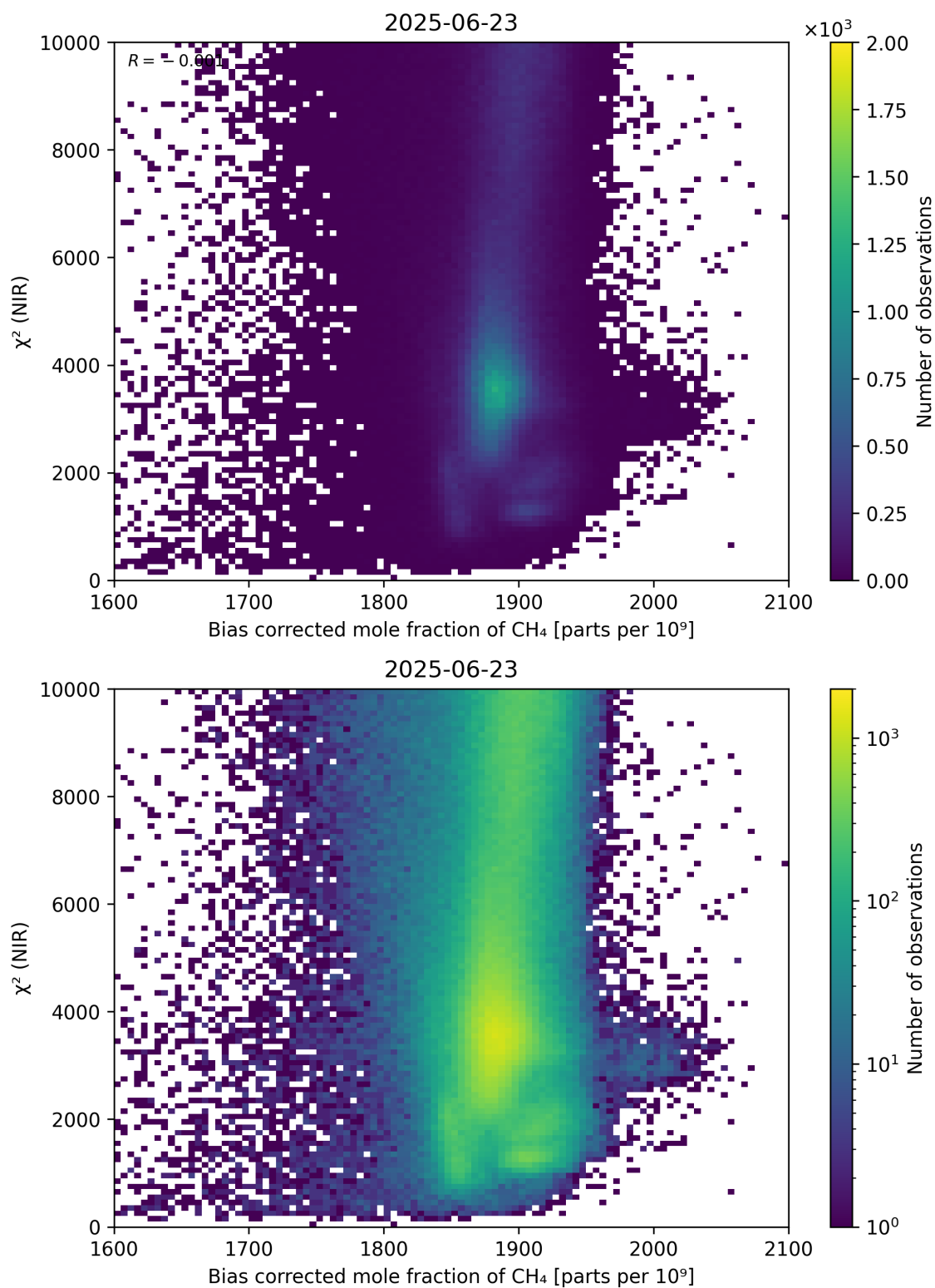
Figure 63: Scatter density plot of “Bias corrected mole fraction of \text{CH}_4 ” against “ \chi^2 (NIR)” for 2025-06-22 to 2025-06-24.
