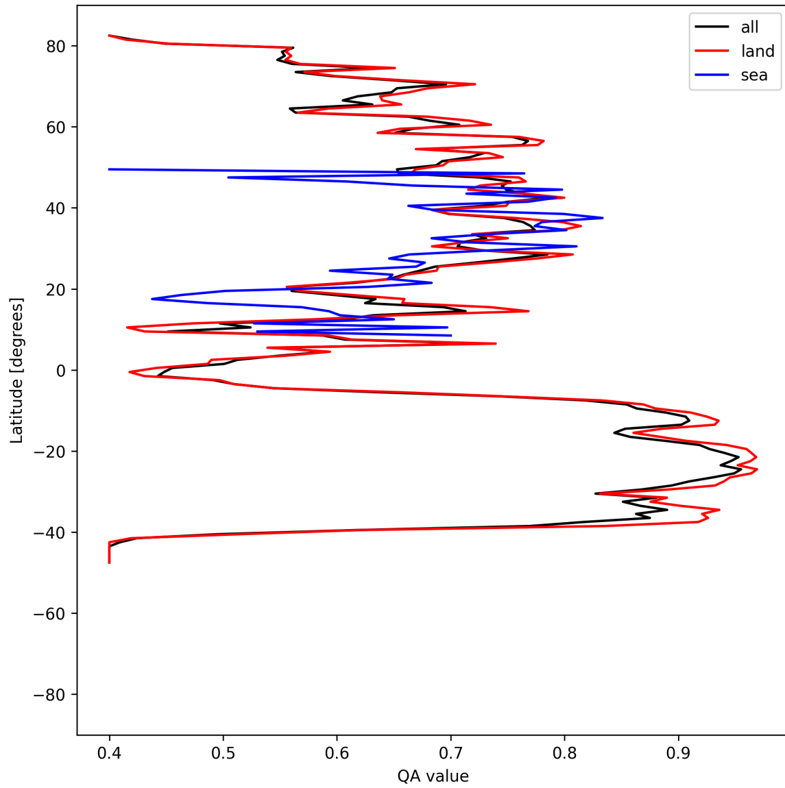
Figure 11: Zonal average of “QA value” for 2025-06-22 to 2025-06-24.
