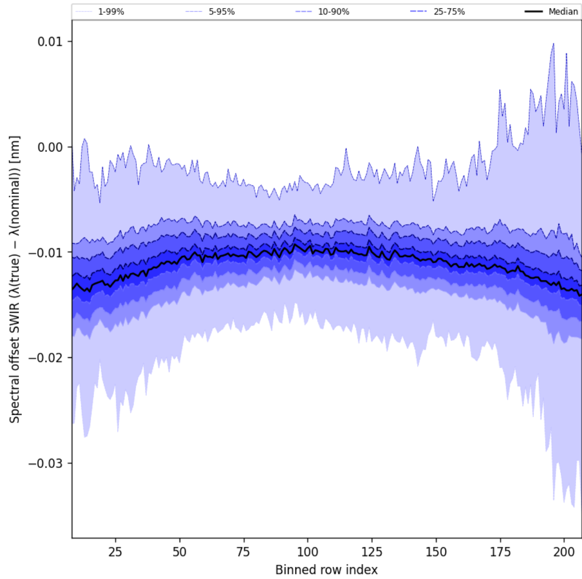
Figure 38: Along track statistics of “Spectral offset SWIR ( \lambda_{\text{true}} - \lambda_{\text{nominal}} )” for 2025-06-22 to 2025-06-24
