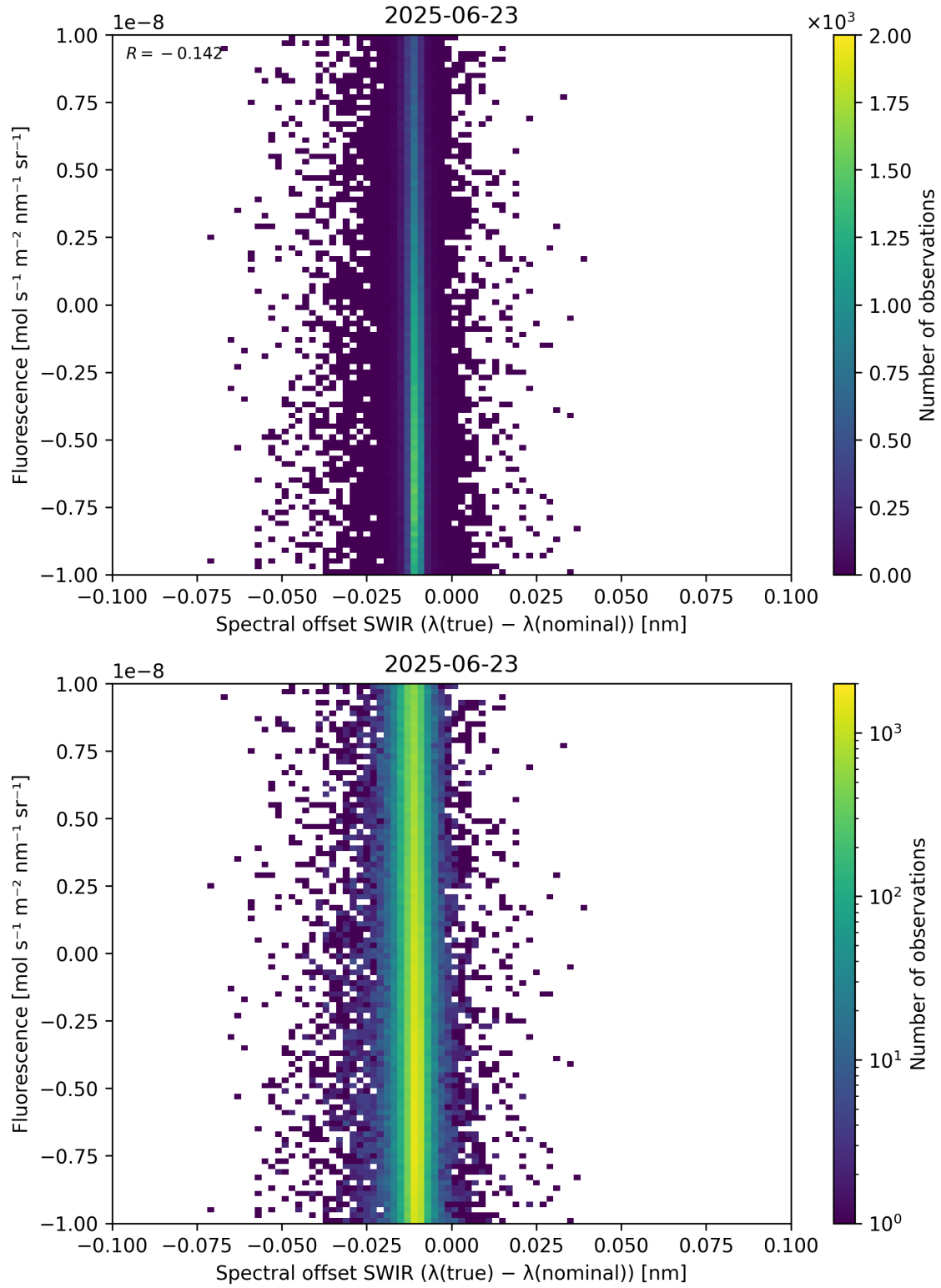
Figure 120: Scatter density plot of “Spectral offset SWIR ( \lambda_{\text{true}} - \lambda_{\text{nominal}} )” against “Fluorescence” for 2025-06-22 to 2025-06-24.
