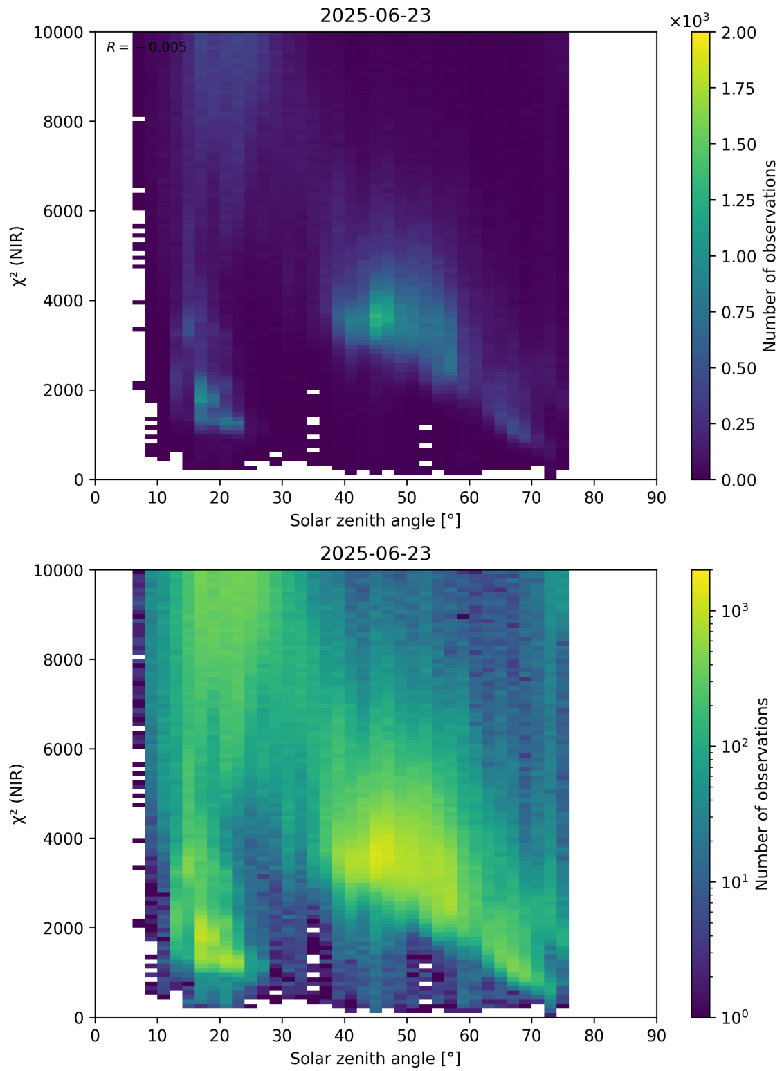
Figure 94: Scatter density plot of “Solar zenith angle” against “ \chi^2 (NIR)” for 2025-06-22 to 2025-06-24.
