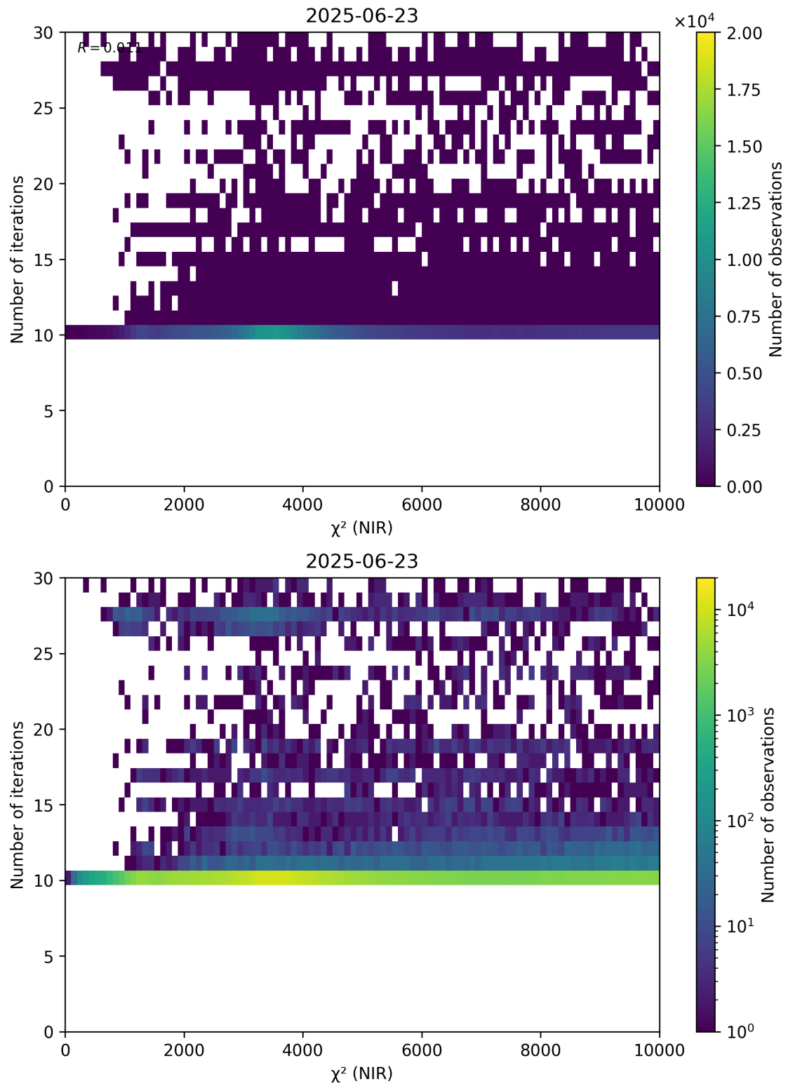
Figure 46: Scatter density plot of “ \chi^2 (NIR)” against “Number of iterations” for 2025-06-22 to 2025-06-24.
