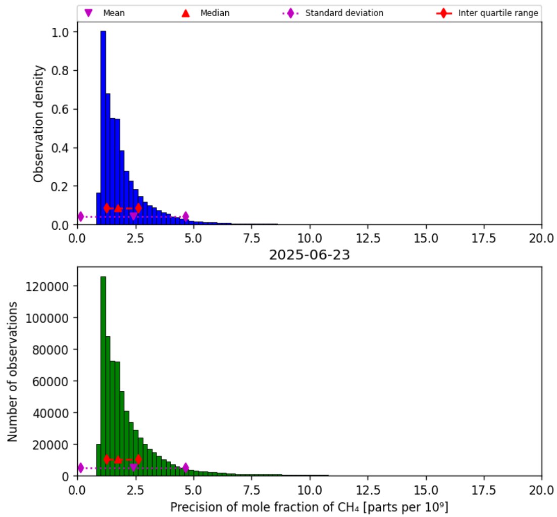
Figure 24: Histogram of “Precision of mole fraction of CH 4 ” for 2025-06-22 to 2025-06-24
