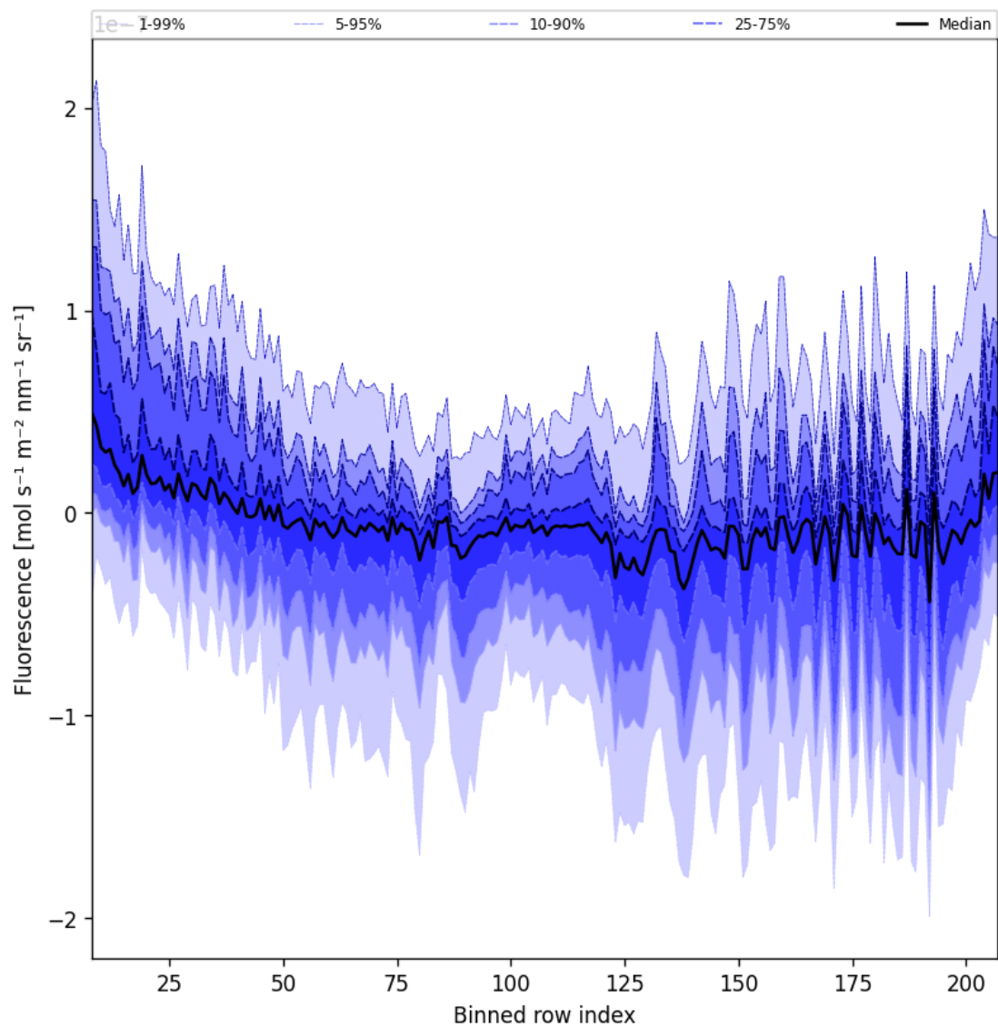
Figure 43: Along track statistics of “Fluorescence” for 2025-06-22 to 2025-06-24
