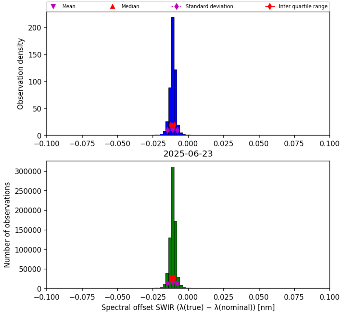
Figure 27: Histogram of “Spectral offset SWIR ( \lambda_{\text{true}} - \lambda_{\text{nominal}} )” for 2025-06-22 to 2025-06-24
