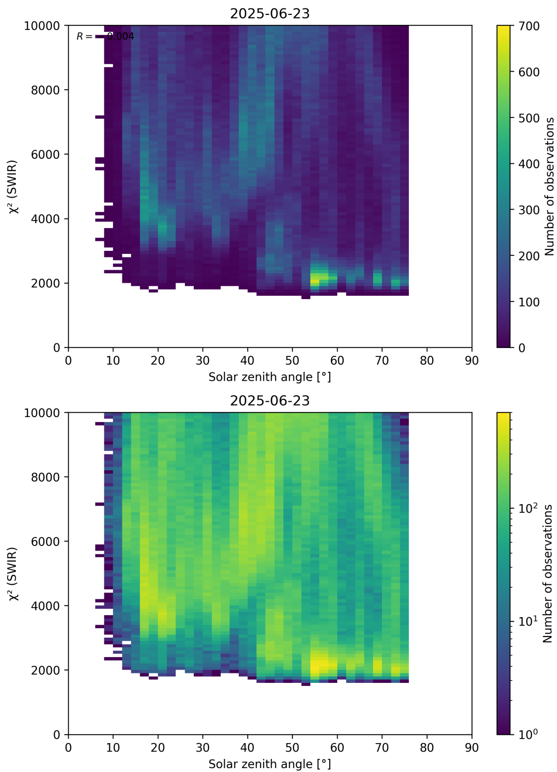
Figure 95: Scatter density plot of “Solar zenith angle” against “ \chi^2 (SWIR)” for 2025-06-22 to 2025-06-24.
