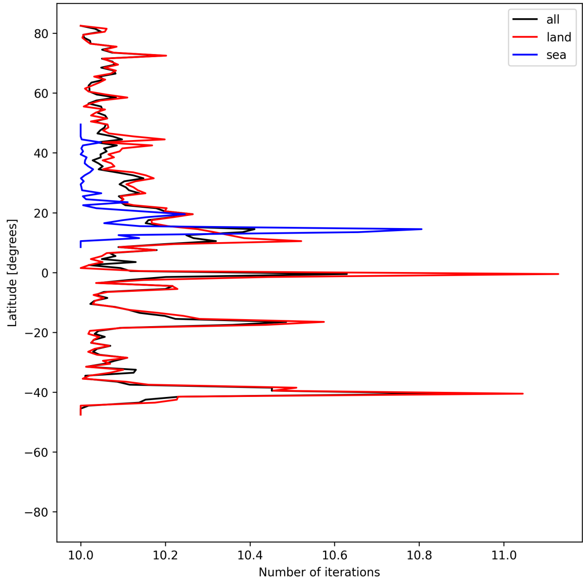
Figure 20: Zonal average of “Number of iterations” for 2025-06-22 to 2025-06-24.
