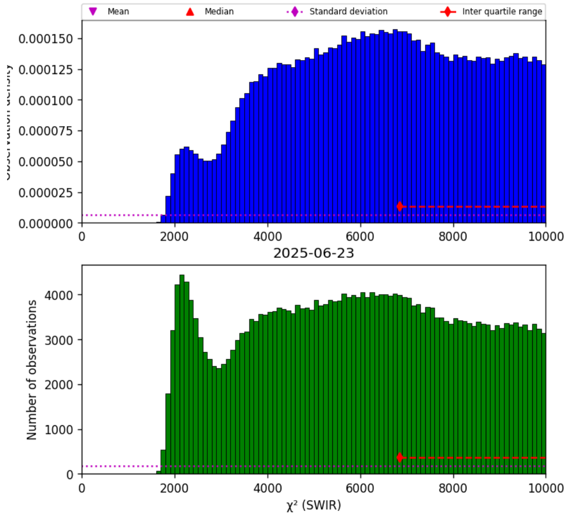
Figure 28: Histogram of “ \chi^2 (SWIR)” for 2025-06-22 to 2025-06-24
