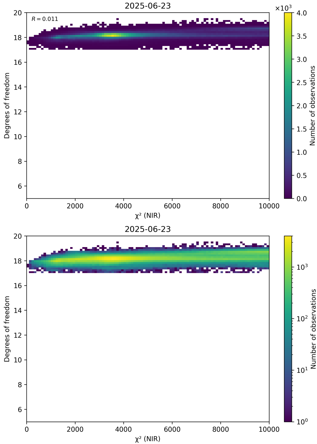
Figure 44: Scatter density plot of “ \chi^2 (NIR)” against “Degrees of freedom” for 2025-06-22 to 2025-06-24.
