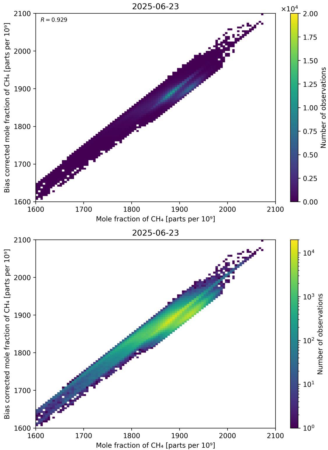
Figure 74: Scatter density plot of “Mole fraction of CH 4 ” against “Bias corrected mole fraction of CH 4 ” for 2025-06-22 to 2025-06-24.
