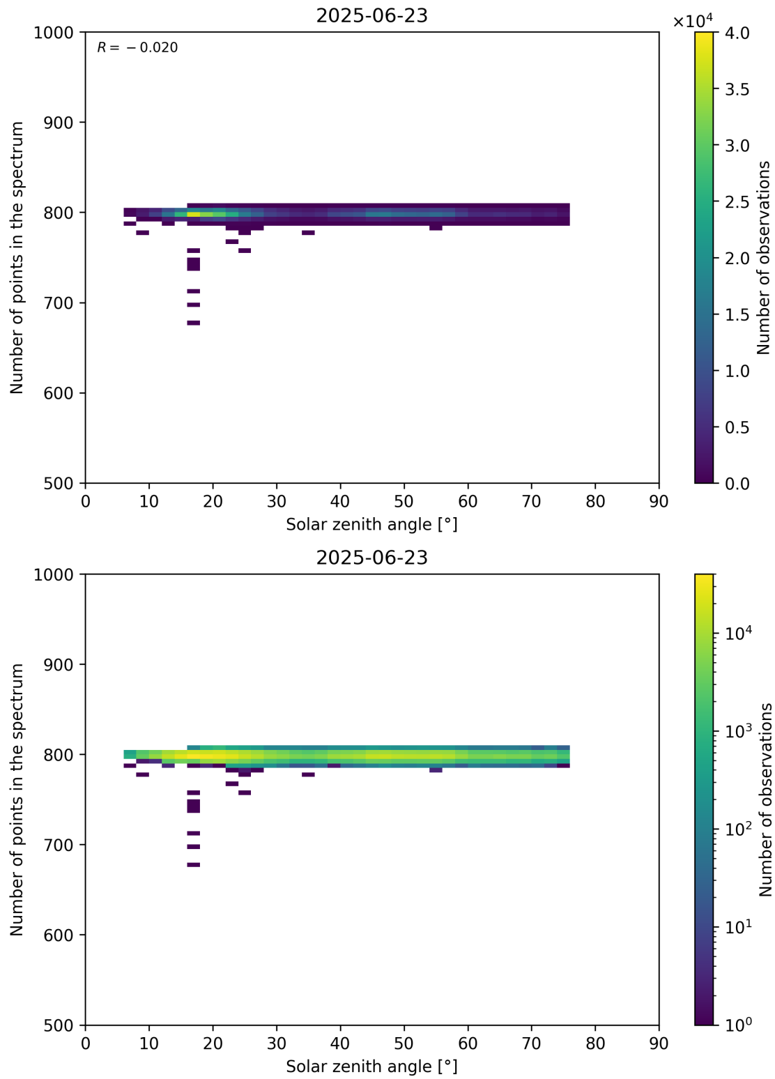
Figure 103: Scatter density plot of “Solar zenith angle” against “Number of points in the spectrum” for 2025-06-22 to 2025-06-24.
