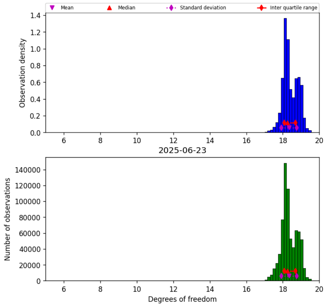
Figure 30: Histogram of “Degrees of freedom” for 2025-06-22 to 2025-06-24
