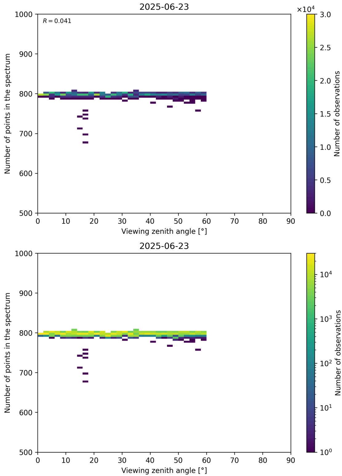
Figure 114: Scatter density plot of “Viewing zenith angle” against “Number of points in the spectrum” for 2025-06-22 to 2025-06-24.
