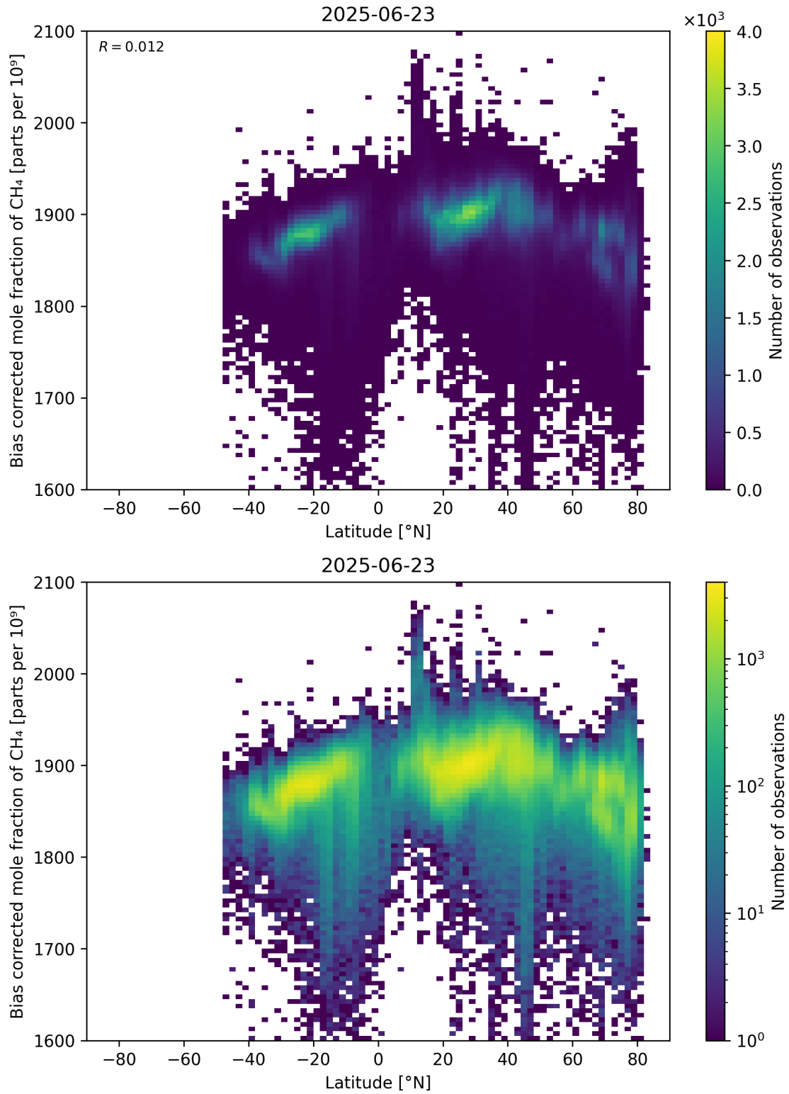
Figure 58: Scatter density plot of “Latitude” against “Bias corrected mole fraction of \text{CH}_4 ” for 2025-06-22 to 2025-06-24.
