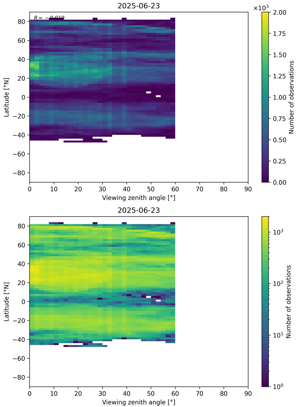
Figure 109: Scatter density plot of “Viewing zenith angle” against “Latitude” for 2025-06-22 to 2025-06-24.
