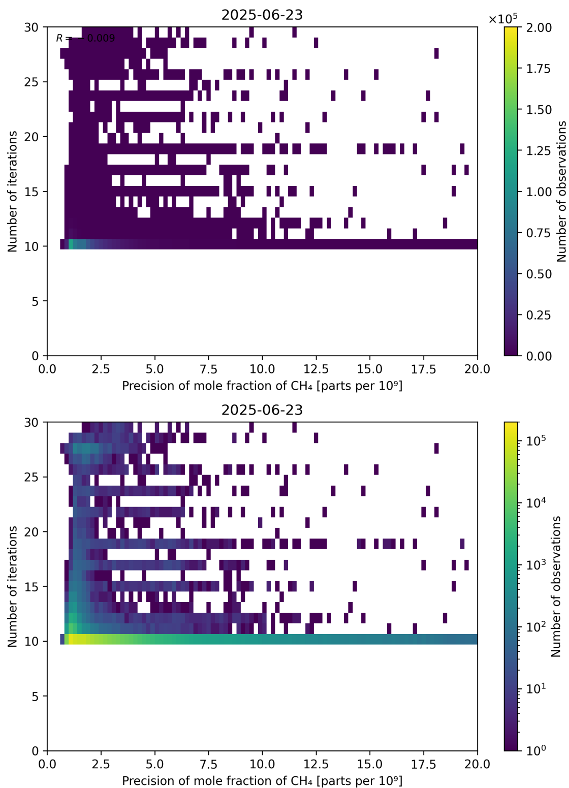
Figure 83: Scatter density plot of “Precision of mole fraction of CH 4 ” against “Number of iterations” for 2025-06-22 to 2025-06-24.
