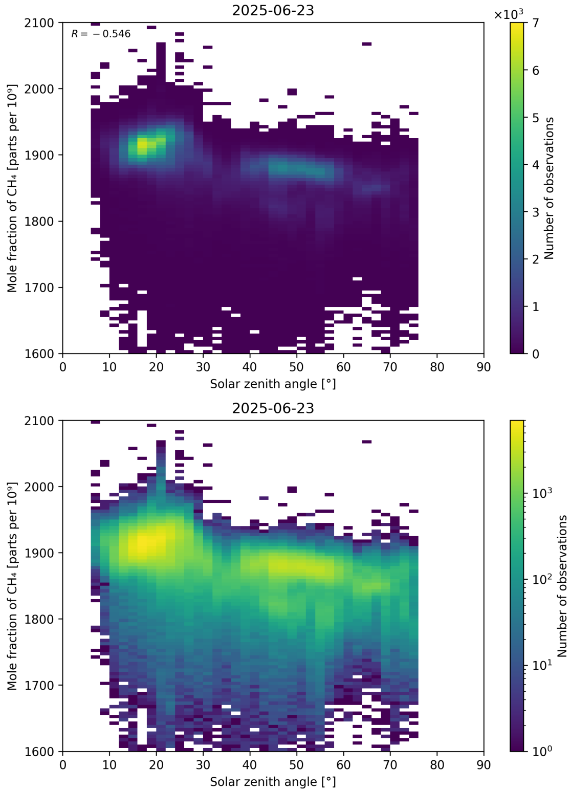
Figure 99: Scatter density plot of “Solar zenith angle” against “Mole fraction of CH 4 ” for 2025-06-22 to 2025-06-24.
