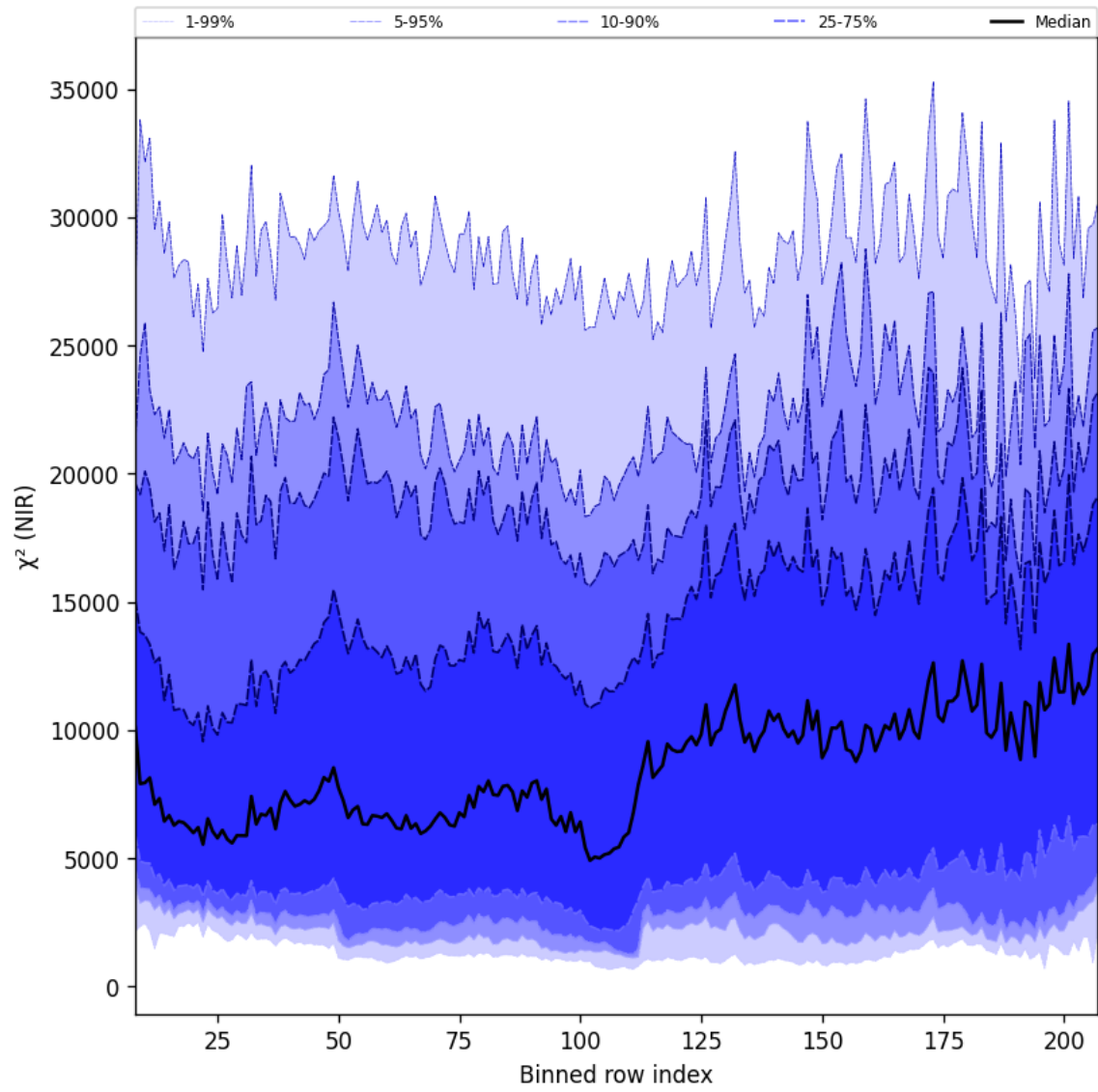
Figure 40: Along track statistics of “ \chi^2 (NIR)” for 2025-06-22 to 2025-06-24
