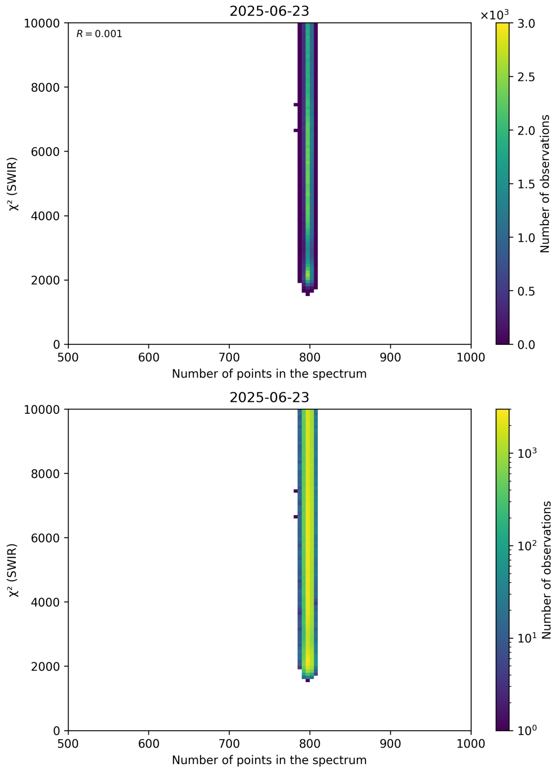
Figure 89: Scatter density plot of “Number of points in the spectrum” against “ \chi^2 (SWIR)” for 2025-06-22 to 2025-06-24.
