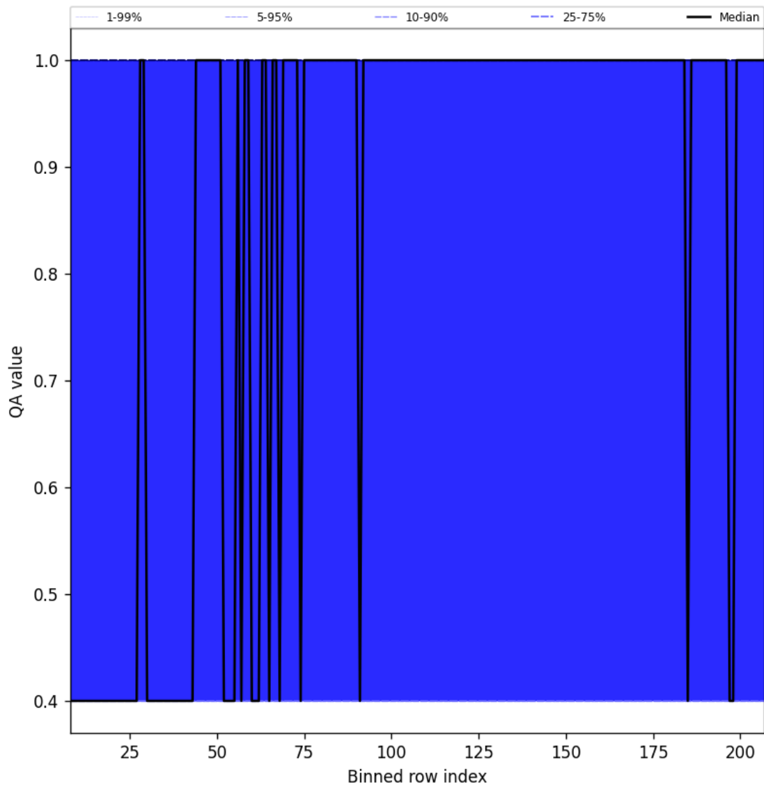
Figure 33: Along track statistics of “QA value” for 2025-06-22 to 2025-06-24
