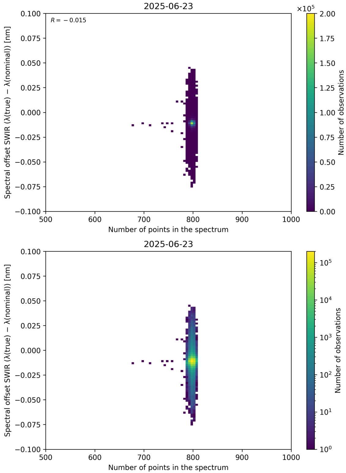
Figure 93: Scatter density plot of “Number of points in the spectrum” against “Spectral offset SWIR ( \lambda_{\text{true}} - \lambda_{\text{nominal}} )” for 2025-06-22 to 2025-06-24.
