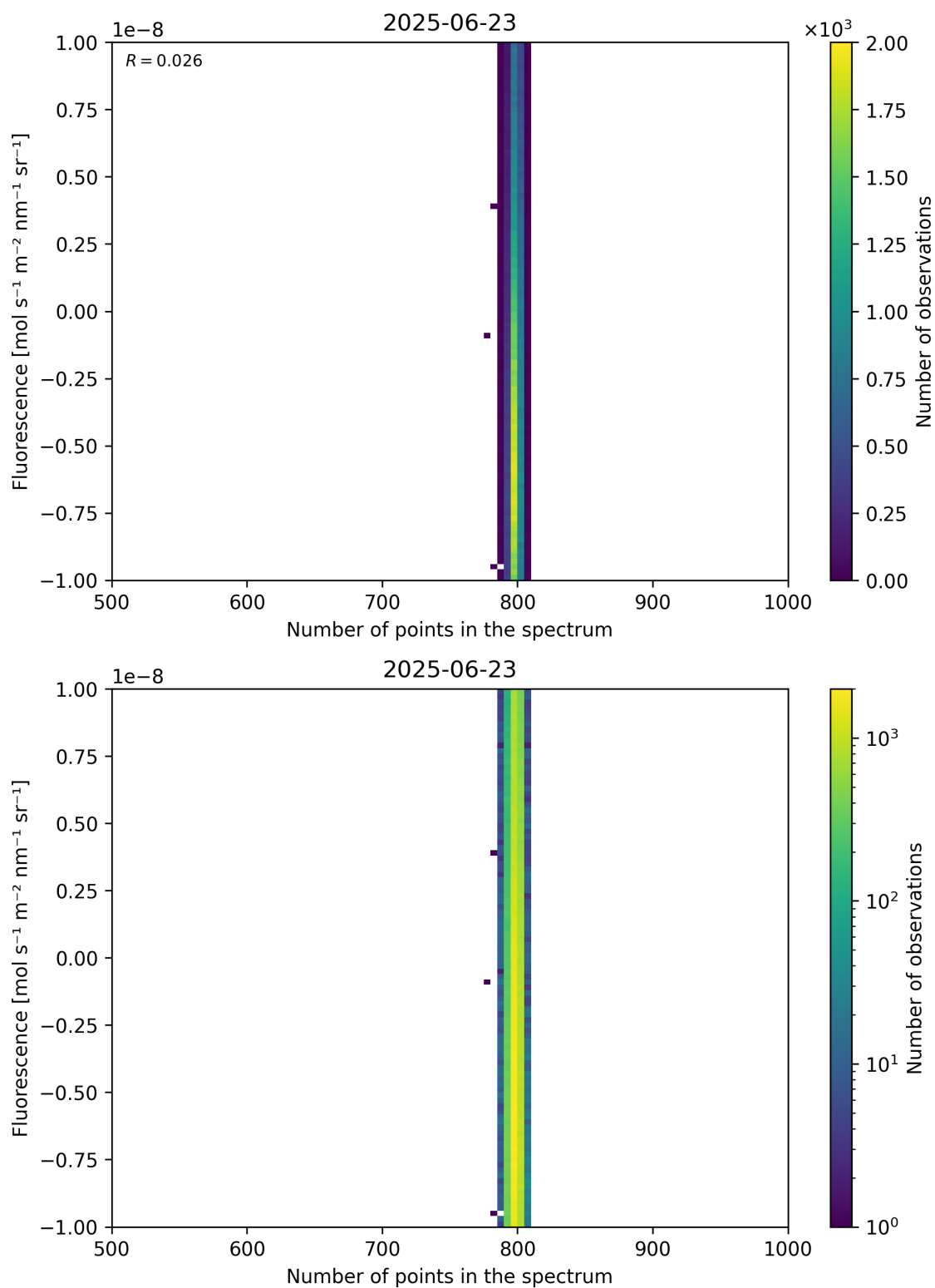
Figure 91: Scatter density plot of “Number of points in the spectrum” against “Fluorescence” for 2025-06-22 to 2025-06-24.
