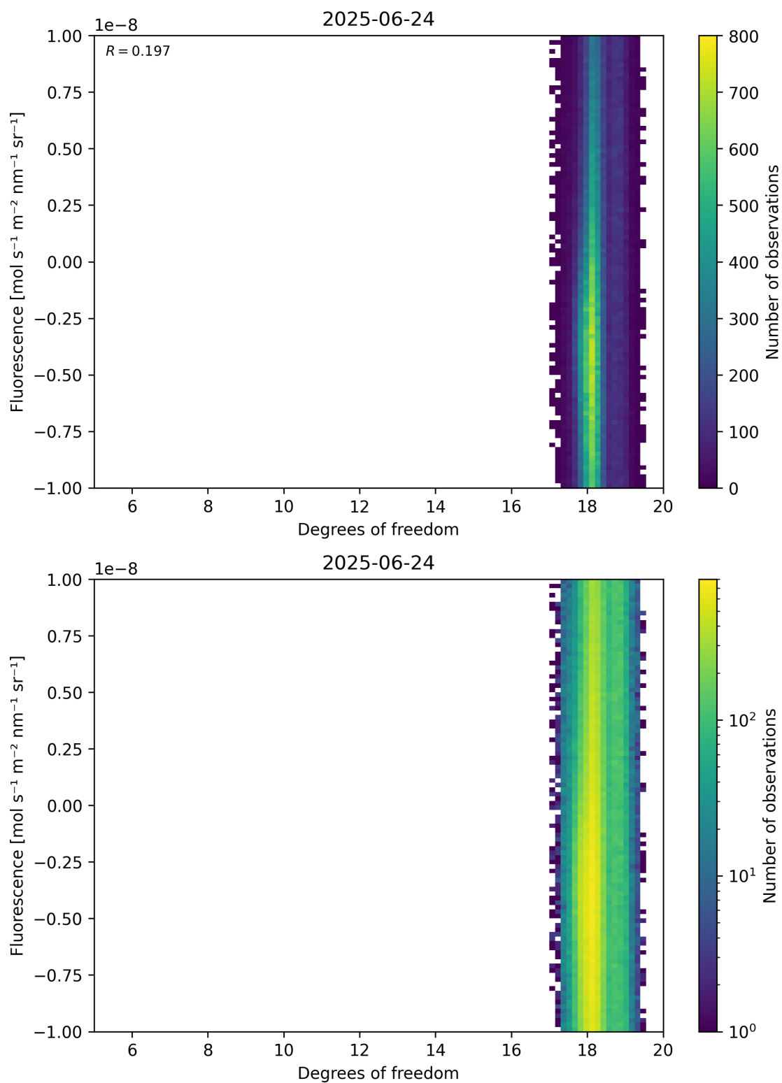
Figure 51: Scatter density plot of “Degrees of freedom” against “Fluorescence” for 2025-06-23 to 2025-06-25.
