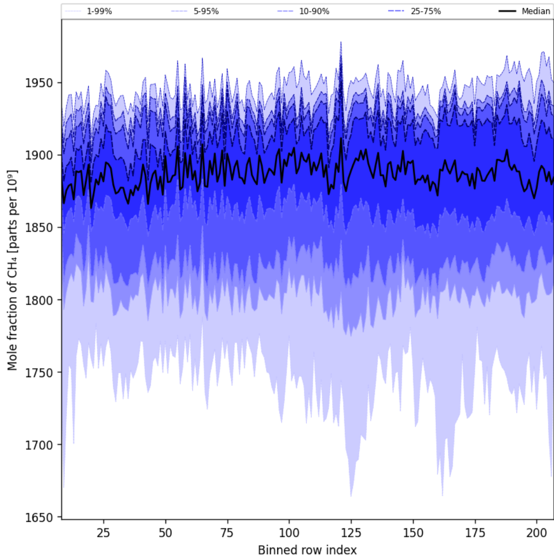
Figure 34: Along track statistics of “Mole fraction of CH 4 ” for 2025-06-23 to 2025-06-25
