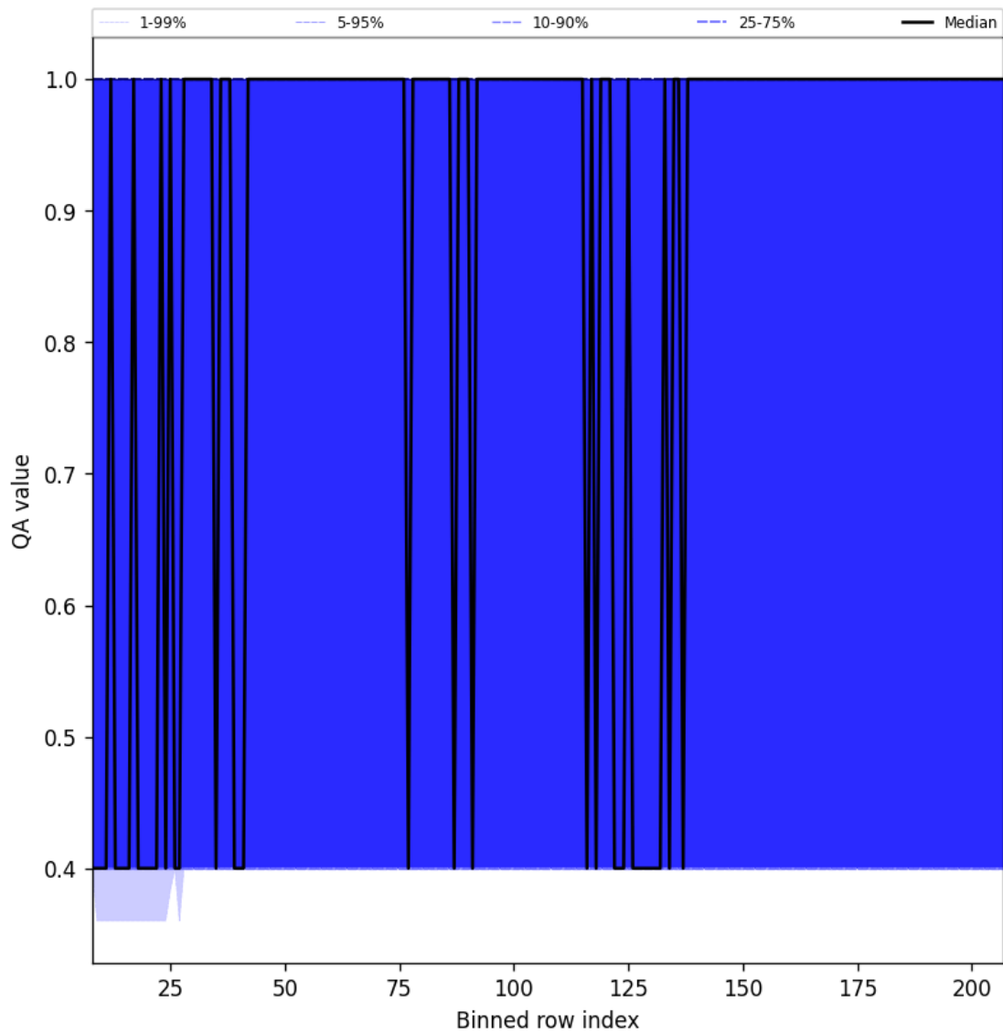
Figure 33: Along track statistics of “QA value” for 2025-06-23 to 2025-06-25
