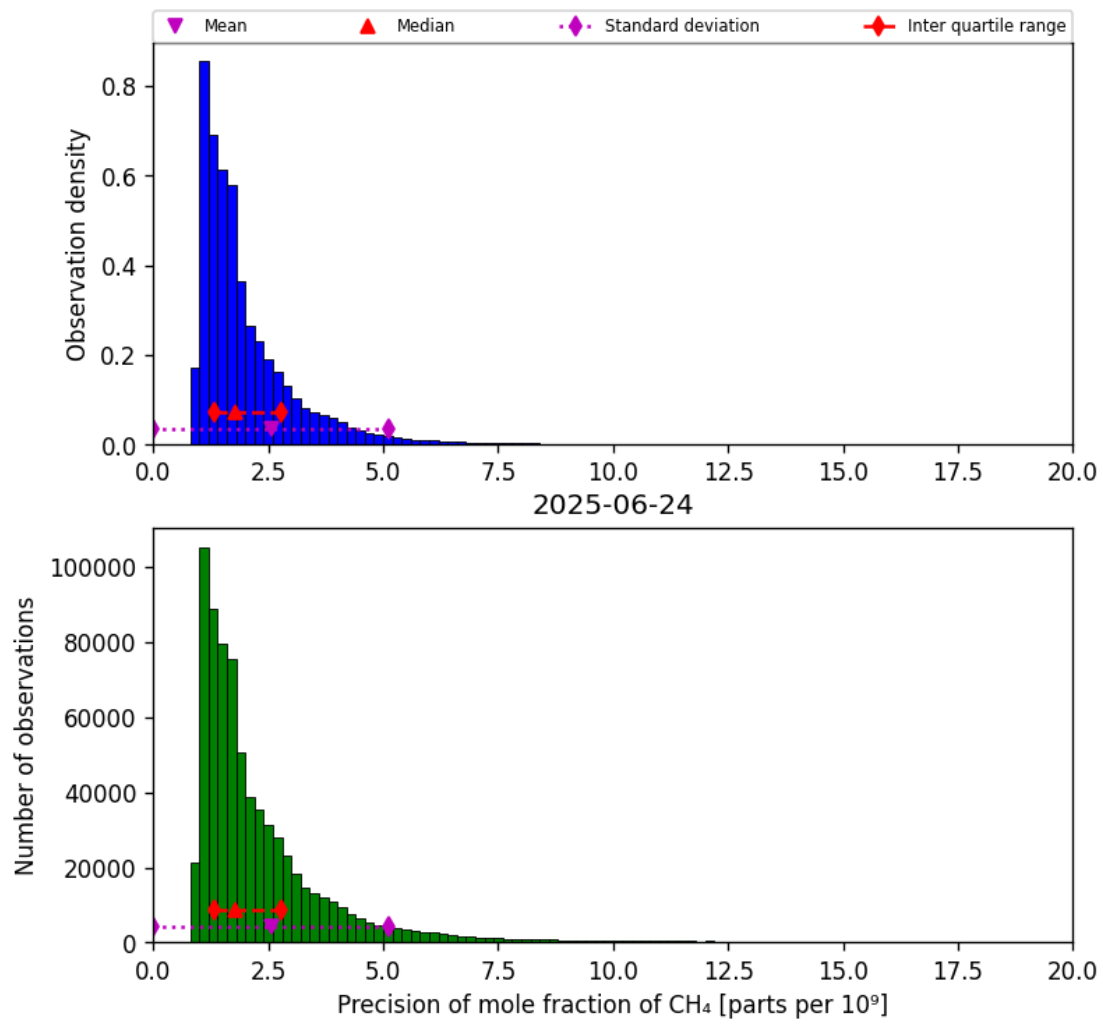
Figure 24: Histogram of “Precision of mole fraction of CH 4 ” for 2025-06-23 to 2025-06-25
