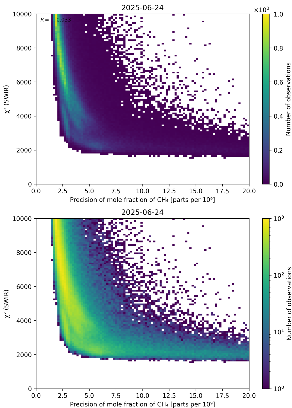
Figure 79: Scatter density plot of “Precision of mole fraction of \text{CH}_4 ” against “ \chi^2 (SWIR)” for 2025-06-23 to 2025-06-25.
