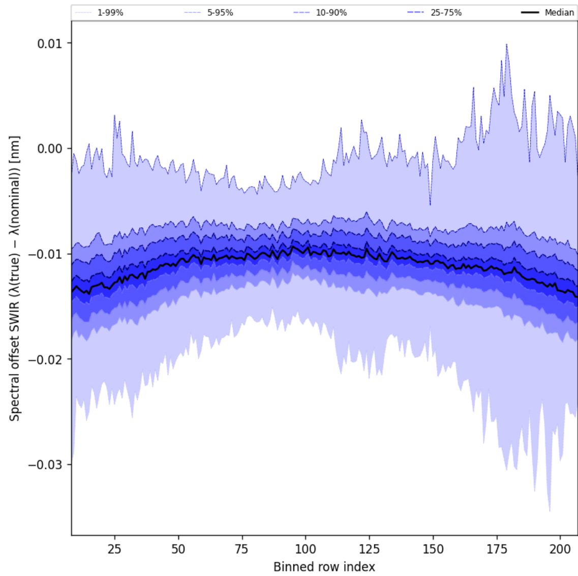
Figure 38: Along track statistics of “Spectral offset SWIR ( \lambda_{\text{true}} - \lambda_{\text{nominal}} )” for 2025-06-23 to 2025-06-25
