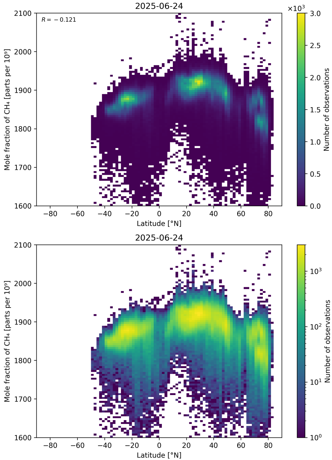
Figure 57: Scatter density plot of “Latitude” against “Mole fraction of \text{CH}_4 ” for 2025-06-23 to 2025-06-25.
