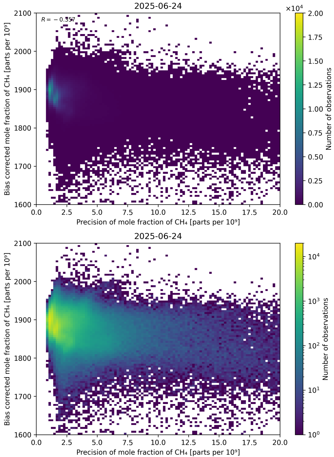
Figure 82: Scatter density plot of “Precision of mole fraction of CH 4 ” against “Bias corrected mole fraction of CH 4 ” for 2025-06-23 to 2025-06-25.
