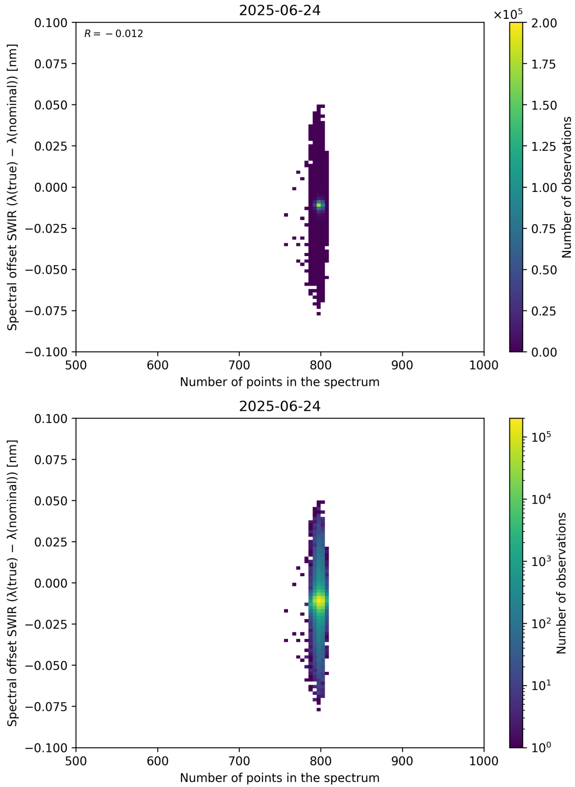
Figure 93: Scatter density plot of “Number of points in the spectrum” against “Spectral offset SWIR ( \lambda_{\text{true}} - \lambda_{\text{nominal}} )” for 2025-06-23 to 2025-06-25.
