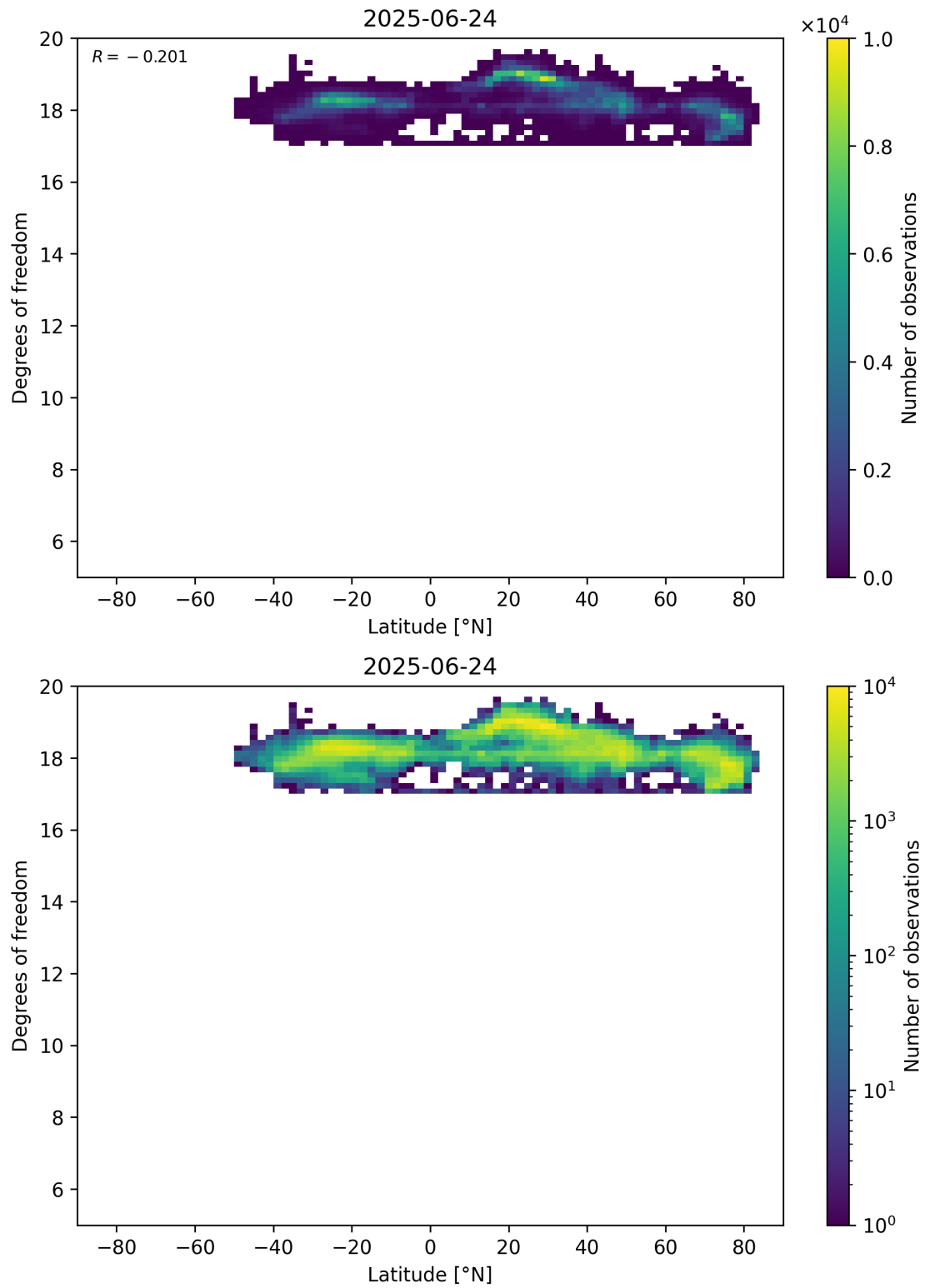
Figure 55: Scatter density plot of “Latitude” against “Degrees of freedom” for 2025-06-23 to 2025-06-25.
