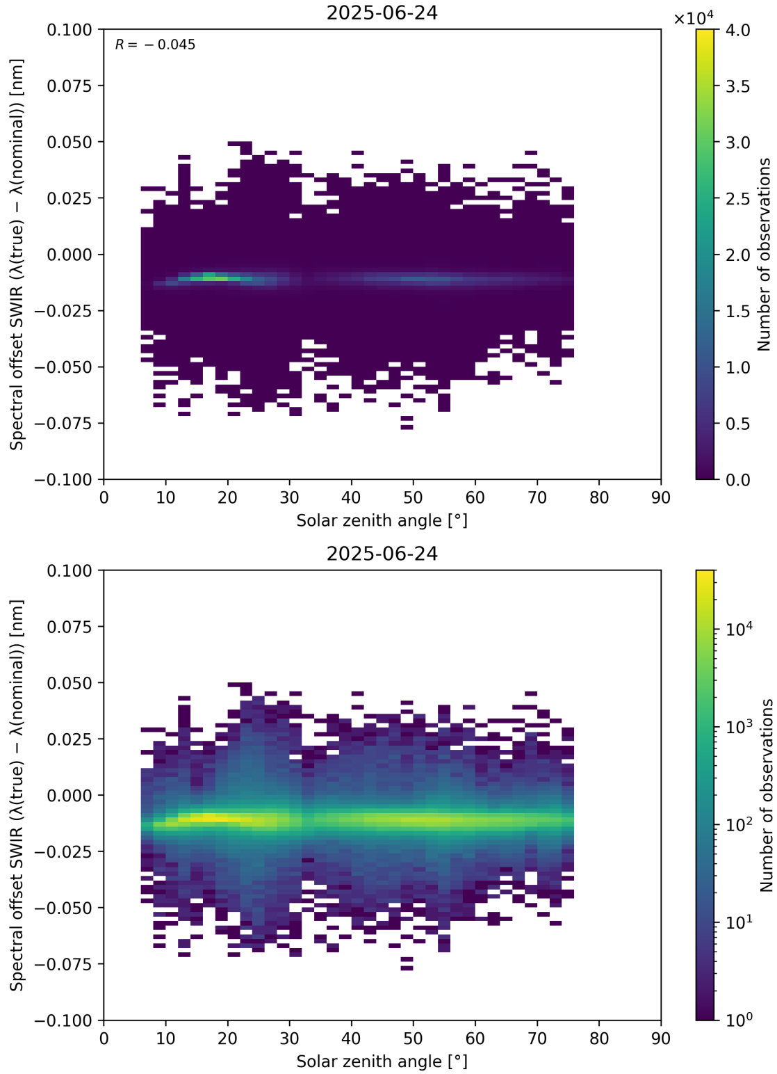
Figure 104: Scatter density plot of “Solar zenith angle” against “Spectral offset SWIR ( \lambda_{\text{true}} - \lambda_{\text{nominal}} )” for 2025-06-23 to 2025-06-25.
