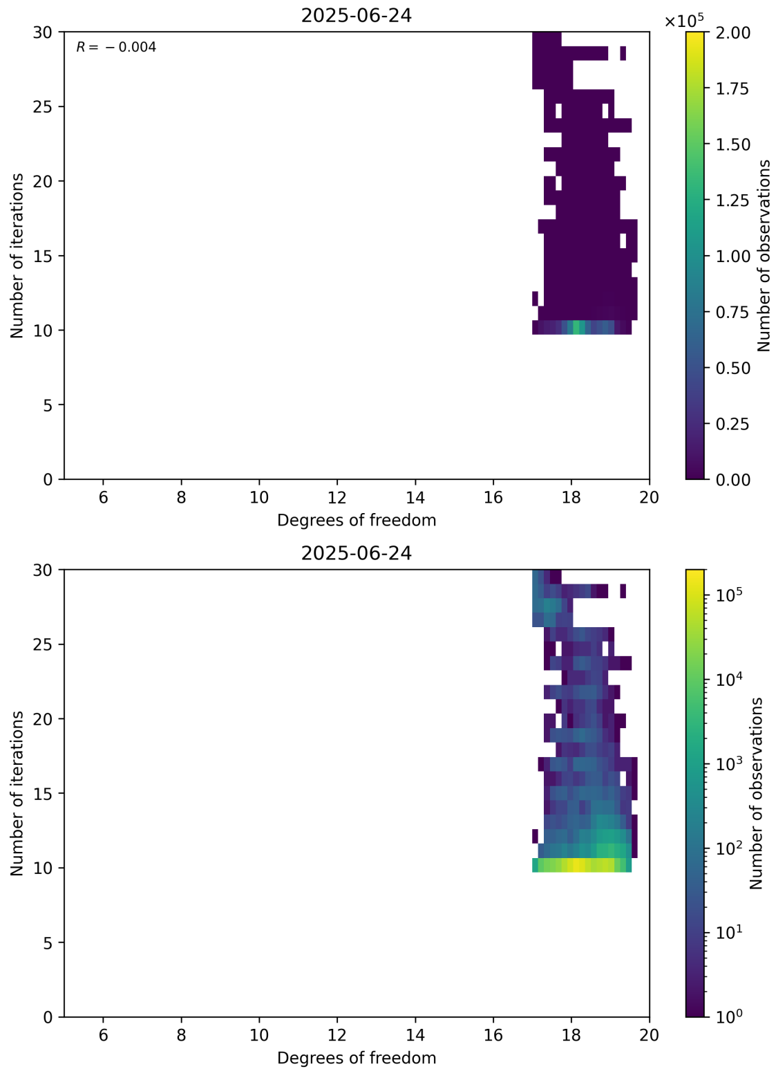
Figure 52: Scatter density plot of “Degrees of freedom” against “Number of iterations” for 2025-06-23 to 2025-06-25.
