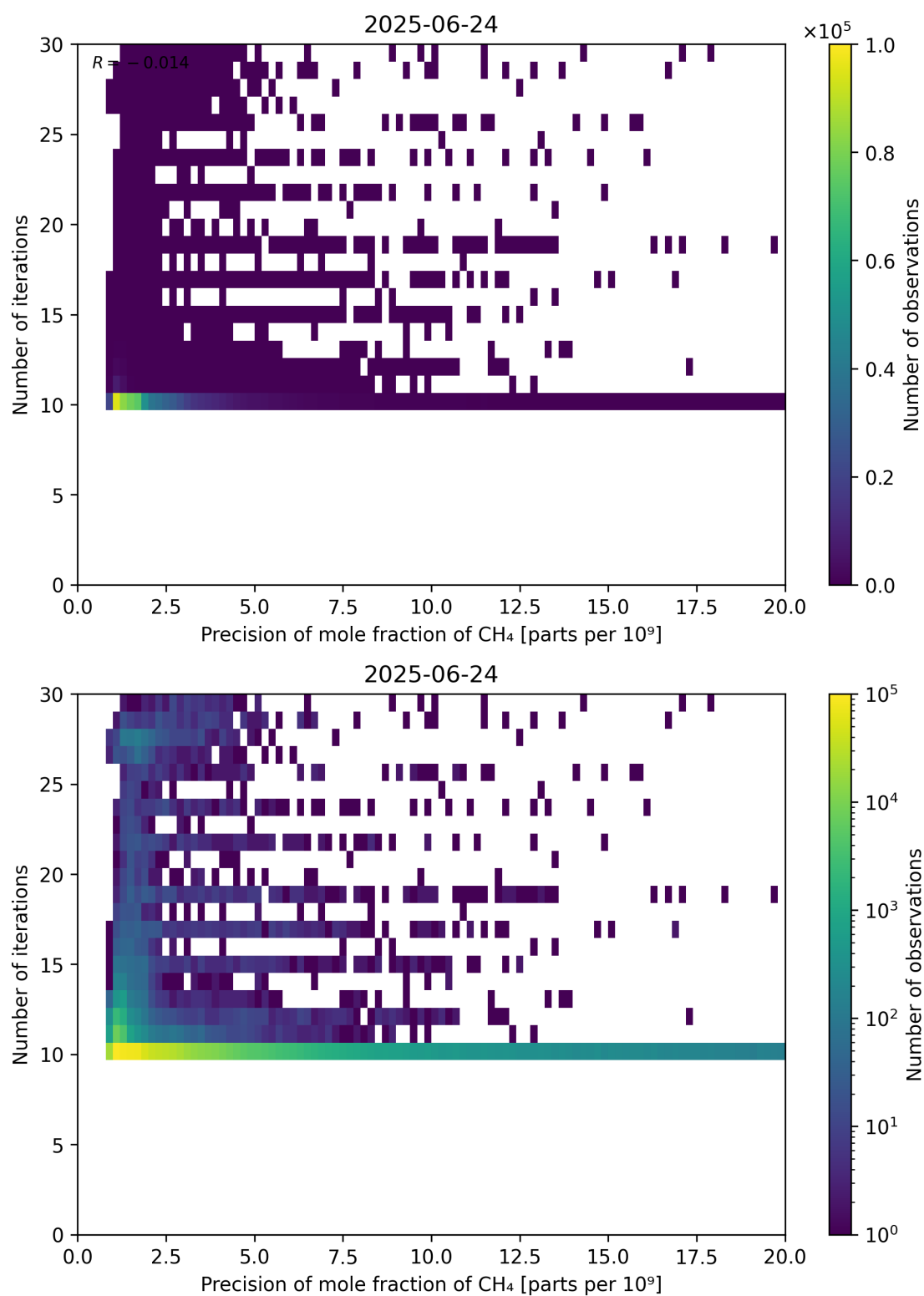
Figure 83: Scatter density plot of “Precision of mole fraction of CH 4 ” against “Number of iterations” for 2025-06-23 to 2025-06-25.
