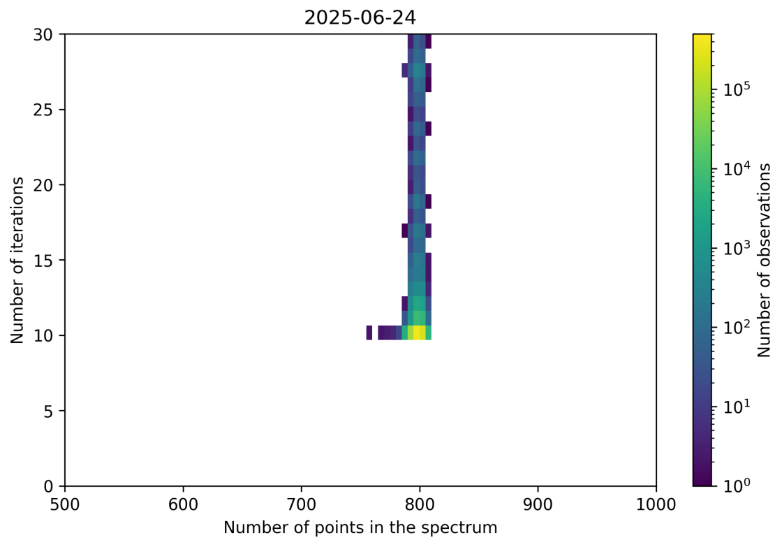
Figure 92: Scatter density plot of “Number of points in the spectrum” against “Number of iterations” for 2025-06-23 to 2025-06-25.
