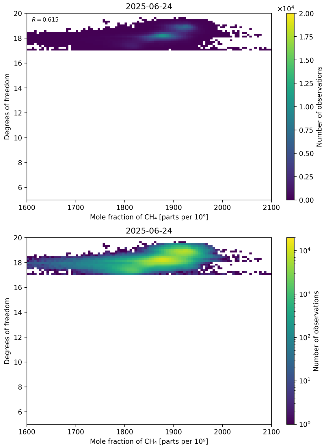
Figure 72: Scatter density plot of “Mole fraction of CH 4 ” against “Degrees of freedom” for 2025-06-23 to 2025-06-25.
