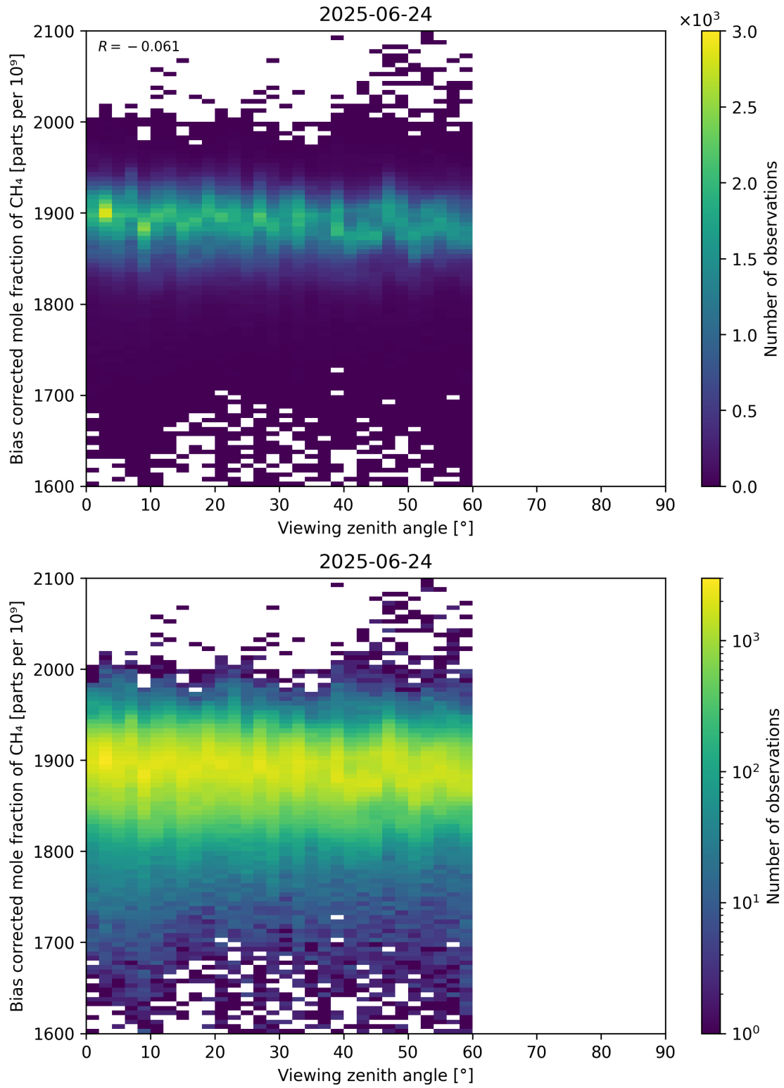
Figure 111: Scatter density plot of “Viewing zenith angle” against “Bias corrected mole fraction of CH 4 ” for 2025-06-23 to 2025-06-25.
