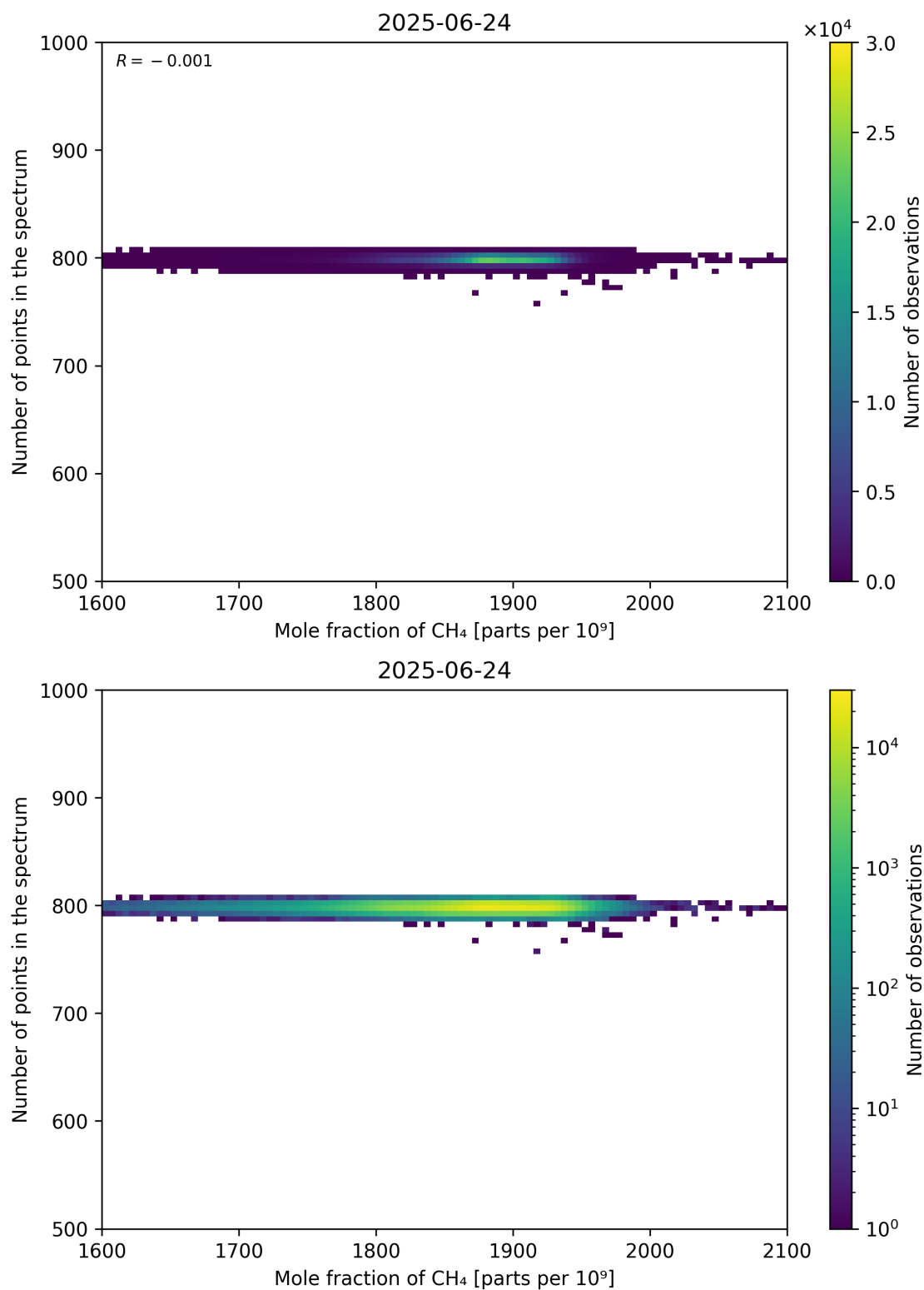
Figure 77: Scatter density plot of “Mole fraction of CH 4 ” against “Number of points in the spectrum” for 2025-06-23 to 2025-06-25.
