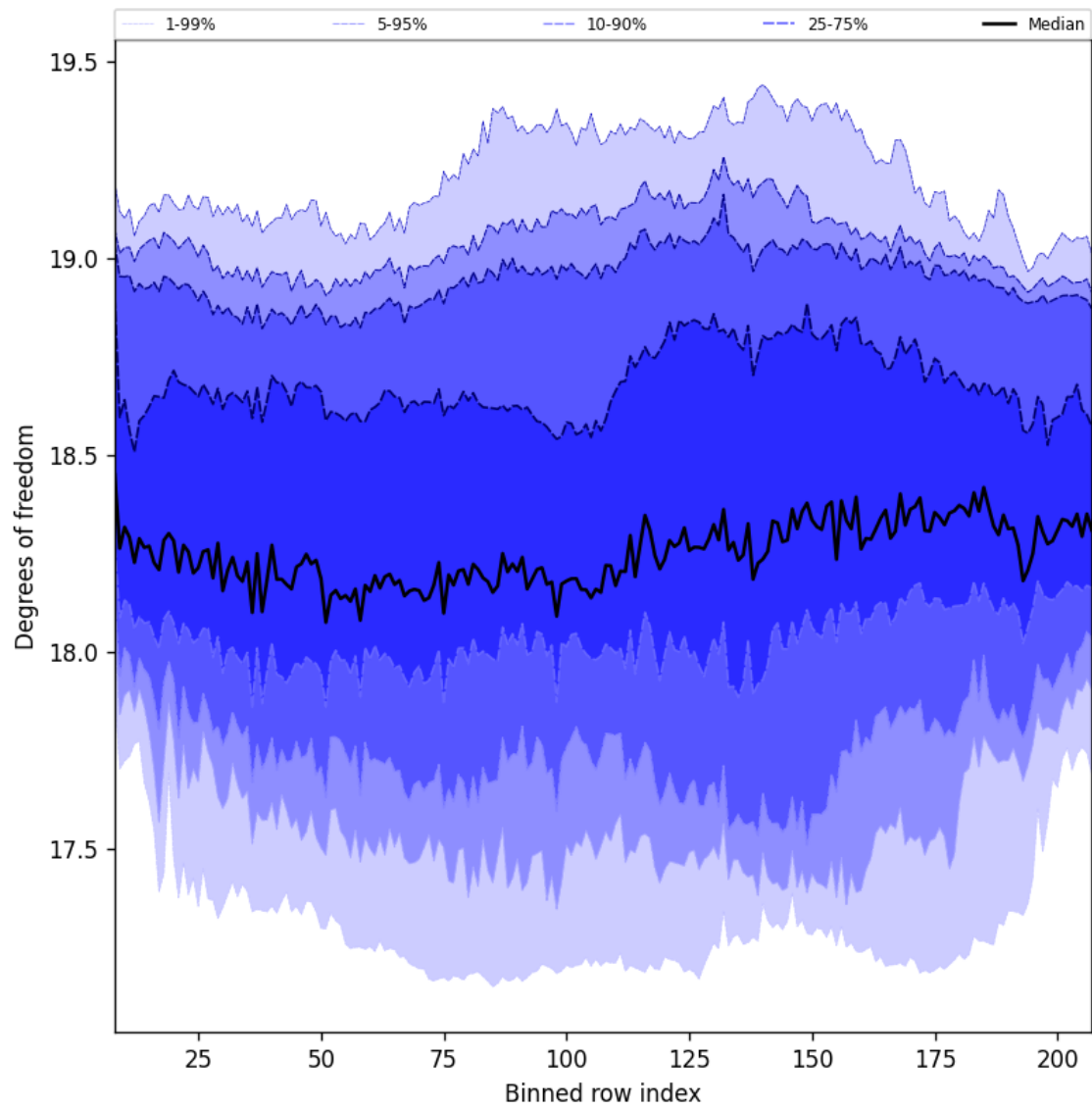
Figure 41: Along track statistics of “Degrees of freedom” for 2025-06-23 to 2025-06-25
