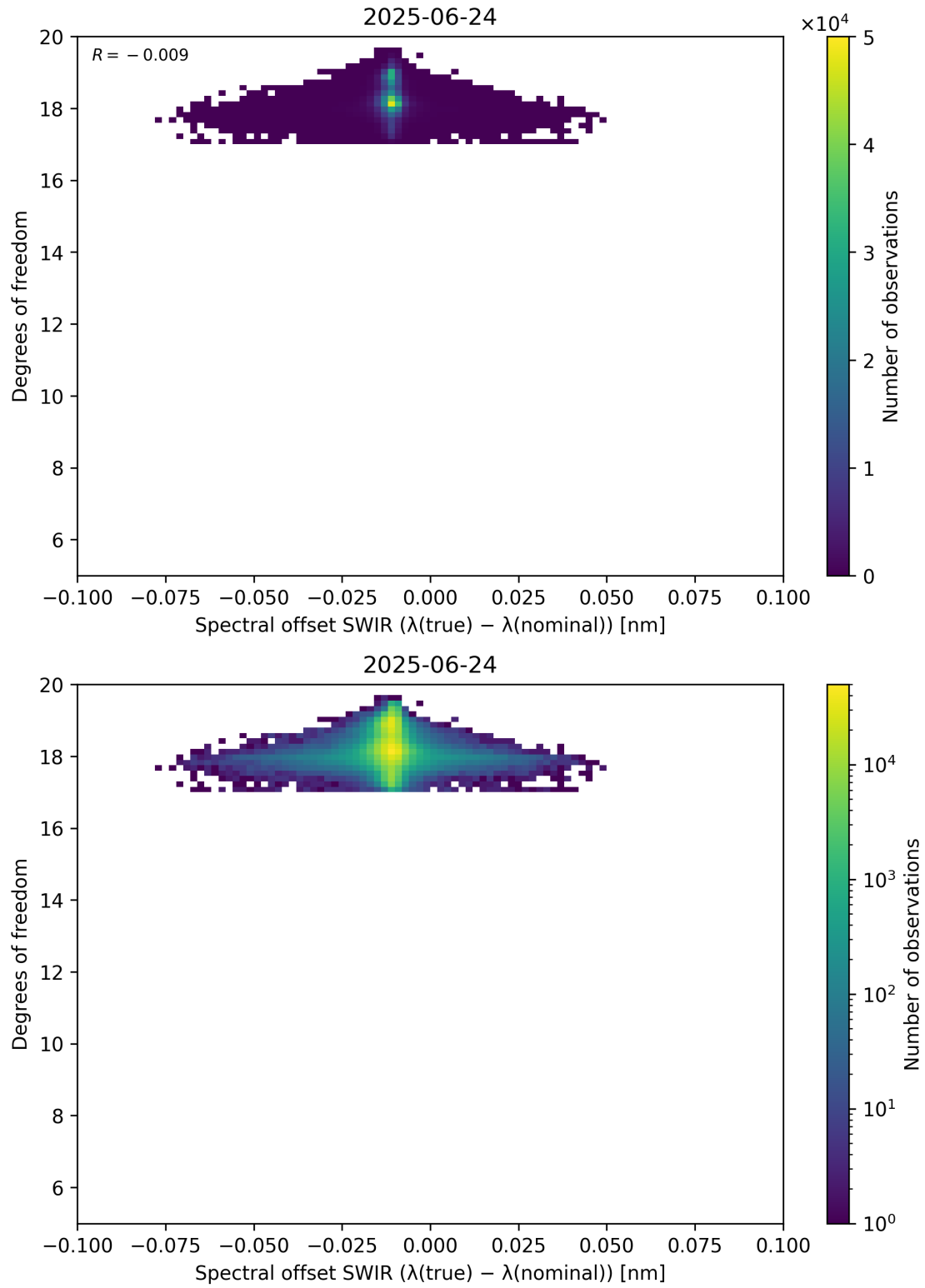
Figure 119: Scatter density plot of “Spectral offset SWIR ( \lambda_{\text{true}} - \lambda_{\text{nominal}} )” against “Degrees of freedom” for 2025-06-23 to 2025-06-25.
