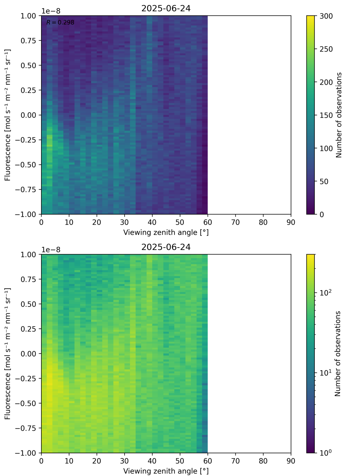
Figure 108: Scatter density plot of “Viewing zenith angle” against “Fluorescence” for 2025-06-23 to 2025-06-25.
