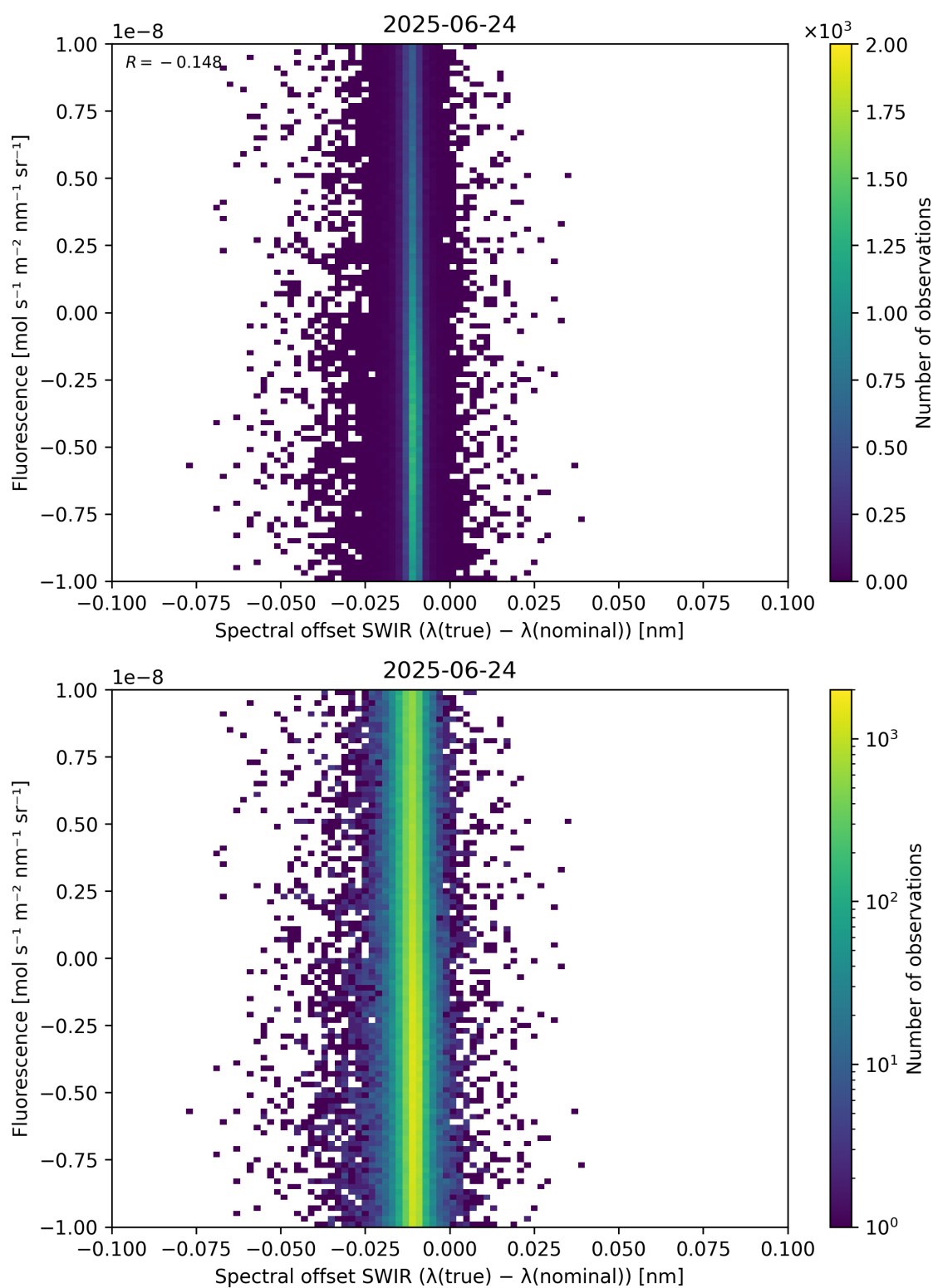
Figure 120: Scatter density plot of “Spectral offset SWIR ( \lambda_{\text{true}} - \lambda_{\text{nominal}} )” against “Fluorescence” for 2025-06-23 to 2025-06-25.
