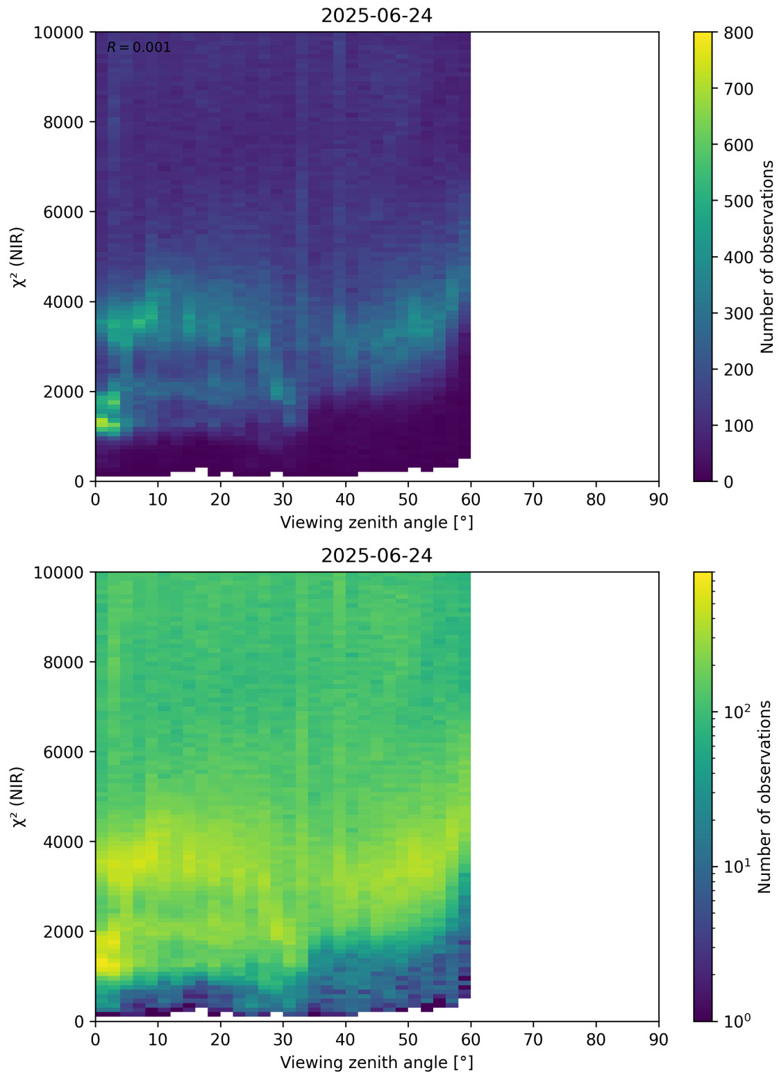
Figure 105: Scatter density plot of “Viewing zenith angle” against “ \chi^2 (NIR)” for 2025-06-23 to 2025-06-25.
