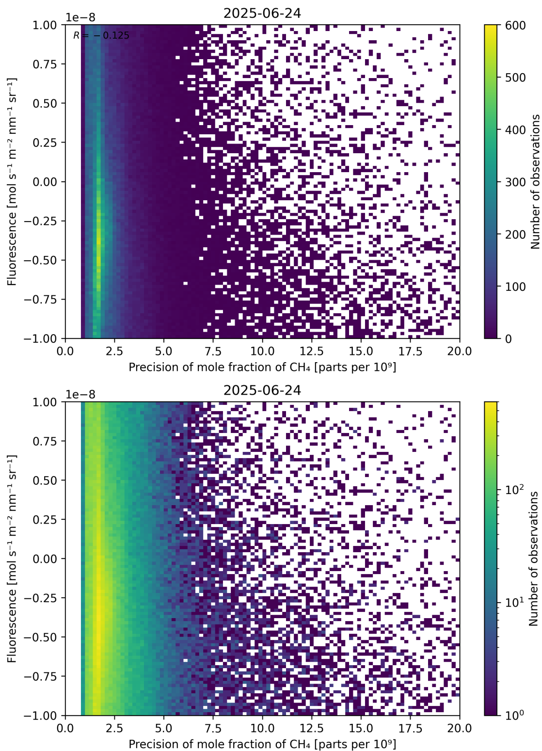
Figure 81: Scatter density plot of “Precision of mole fraction of \text{CH}_4 ” against “Fluorescence” for 2025-06-23 to 2025-06-25.
