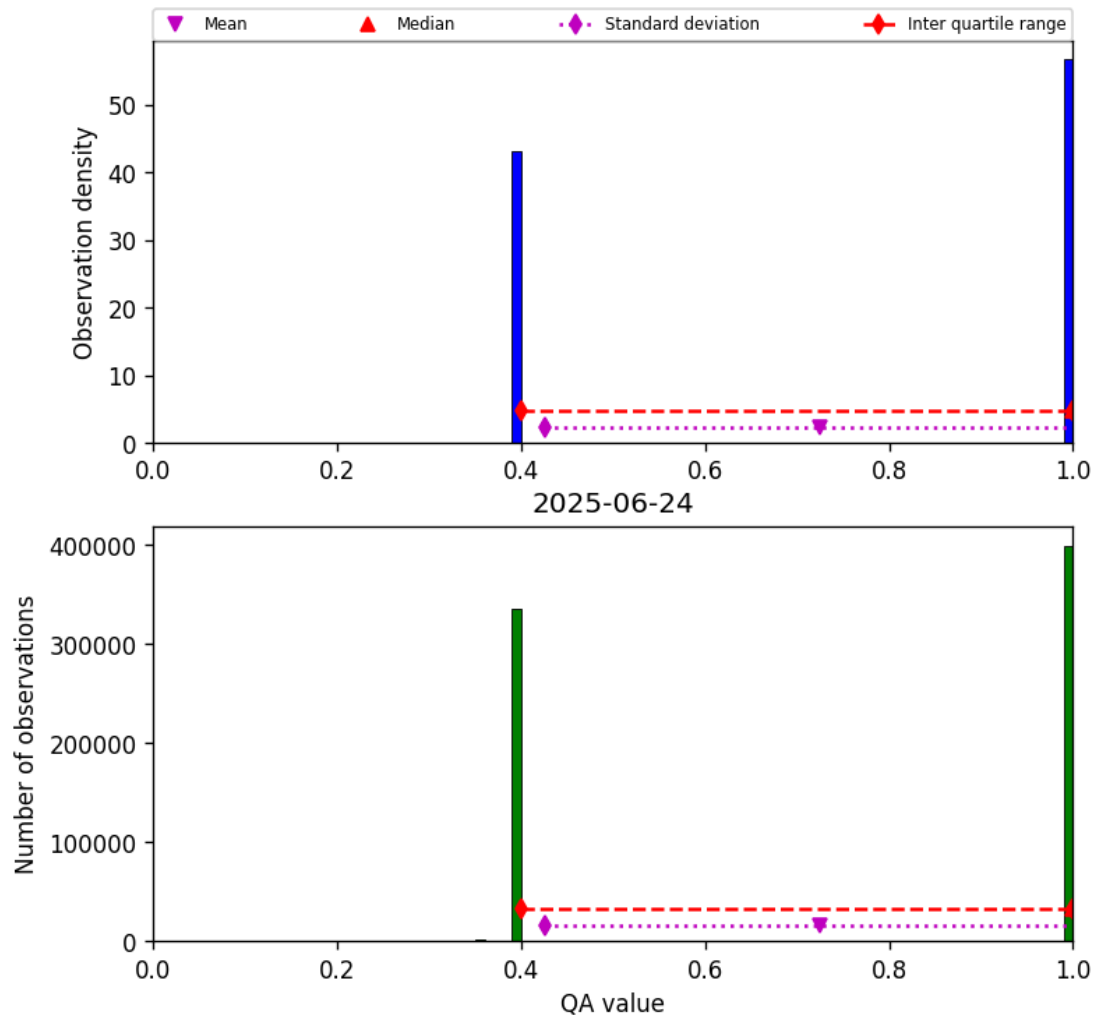
Figure 22: Histogram of “QA value” for 2025-06-23 to 2025-06-25
