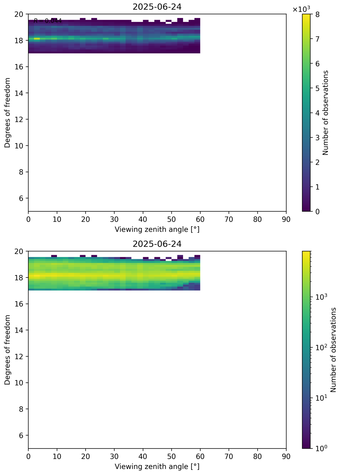
Figure 107: Scatter density plot of “Viewing zenith angle” against “Degrees of freedom” for 2025-06-23 to 2025-06-25.
