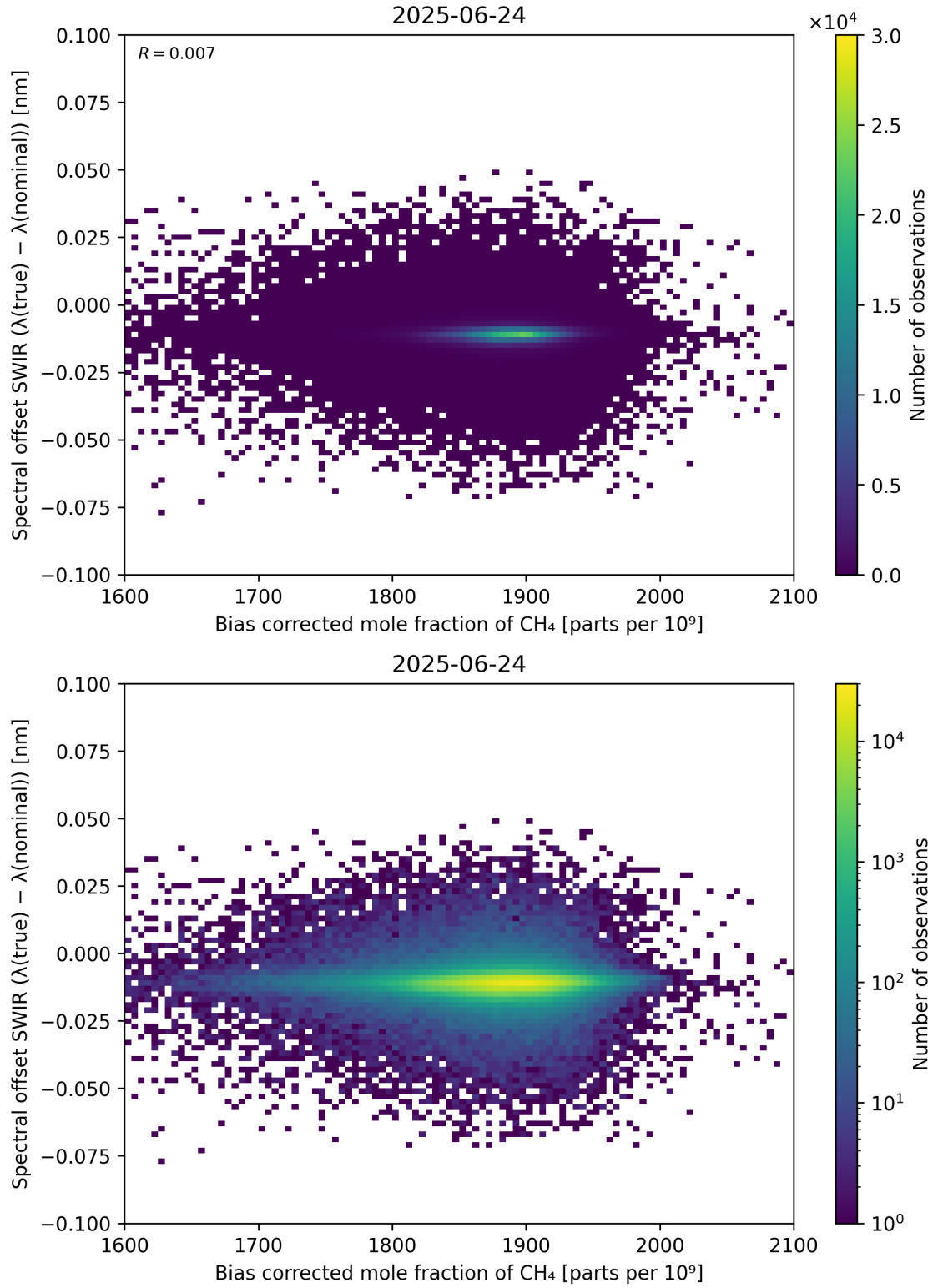
Figure 69: Scatter density plot of “Bias corrected mole fraction of CH 4 ” against “Spectral offset SWIR ( \lambda_{\text{true}} - \lambda_{\text{nominal}} )” for 2025-06-23 to 2025-06-25.
