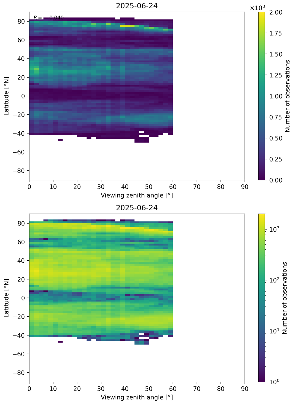
Figure 109: Scatter density plot of “Viewing zenith angle” against “Latitude” for 2025-06-23 to 2025-06-25.
