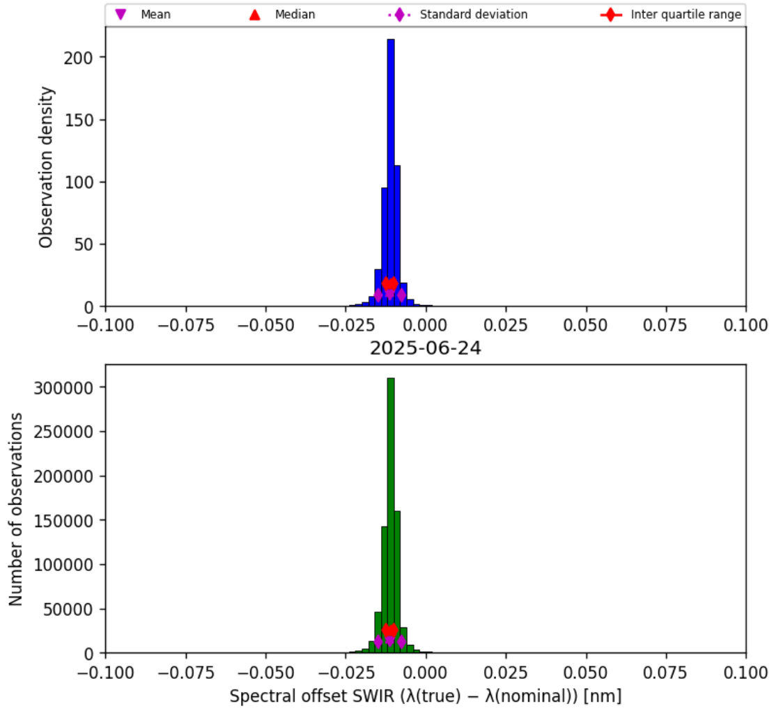
Figure 27: Histogram of “Spectral offset SWIR ( \lambda_{\text{true}} - \lambda_{\text{nominal}} )” for 2025-06-23 to 2025-06-25
