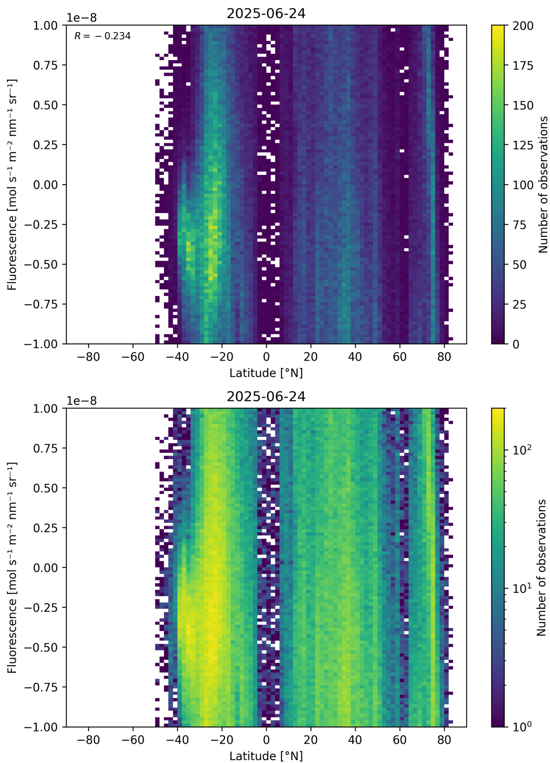
Figure 56: Scatter density plot of “Latitude” against “Fluorescence” for 2025-06-23 to 2025-06-25.
