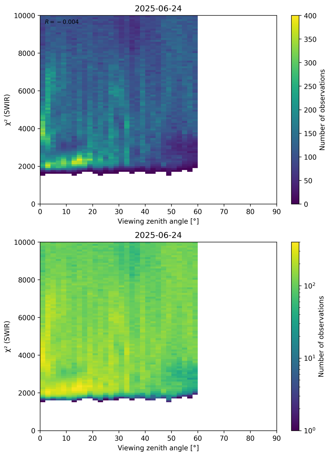
Figure 106: Scatter density plot of “Viewing zenith angle” against “ \chi^2 (SWIR)” for 2025-06-23 to 2025-06-25.
