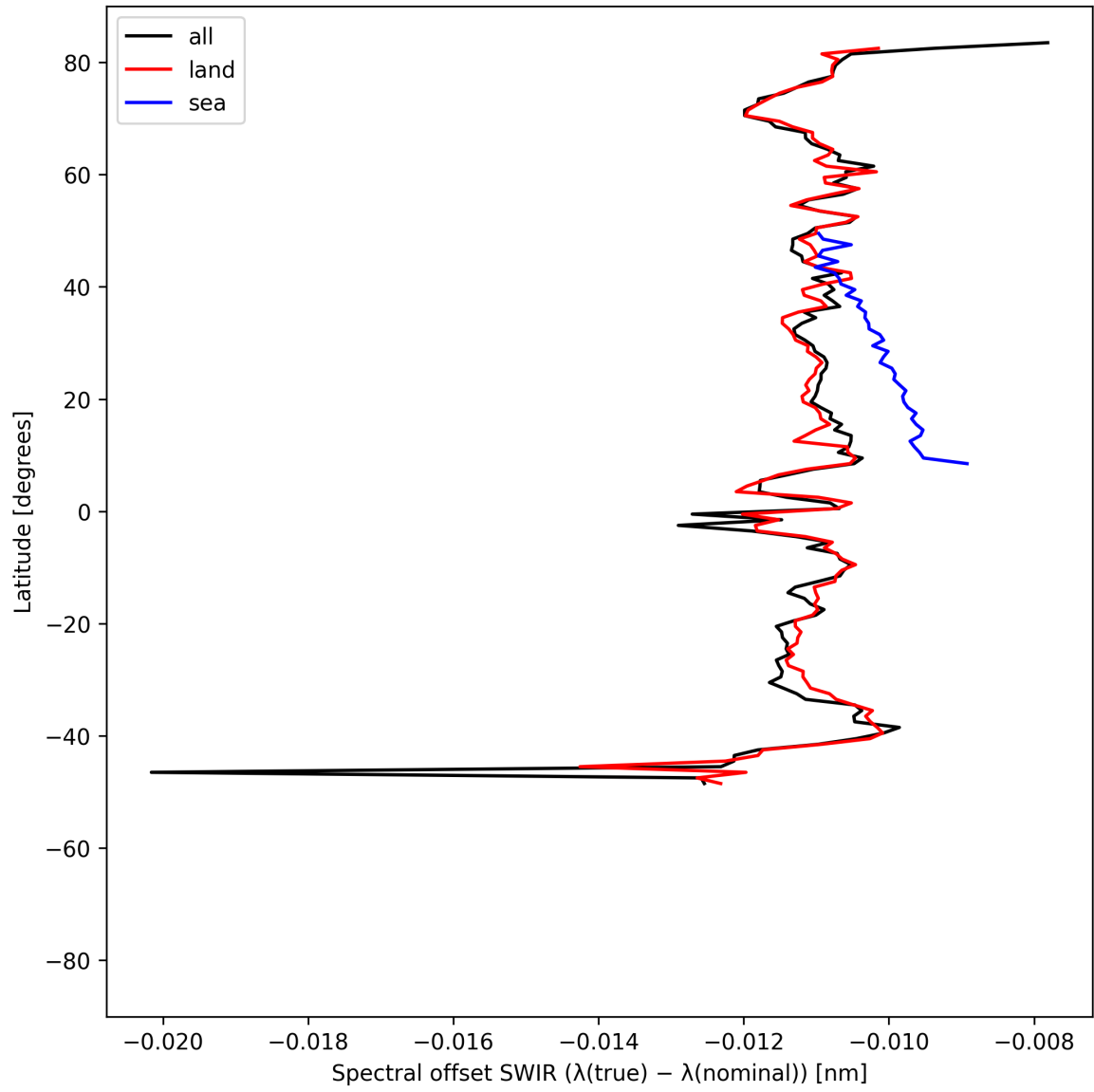
Figure 16: Zonal average of “Spectral offset SWIR ( \lambda_{\text{true}} - \lambda_{\text{nominal}} )” for 2025-06-23 to 2025-06-25.
