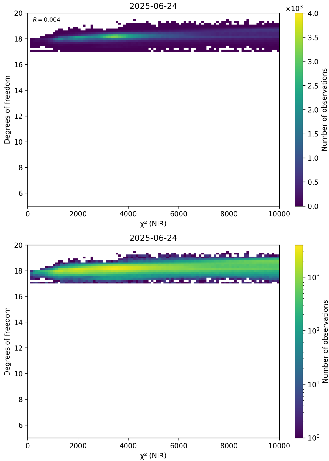
Figure 44: Scatter density plot of “ \chi^2 (NIR)” against “Degrees of freedom” for 2025-06-23 to 2025-06-25.
