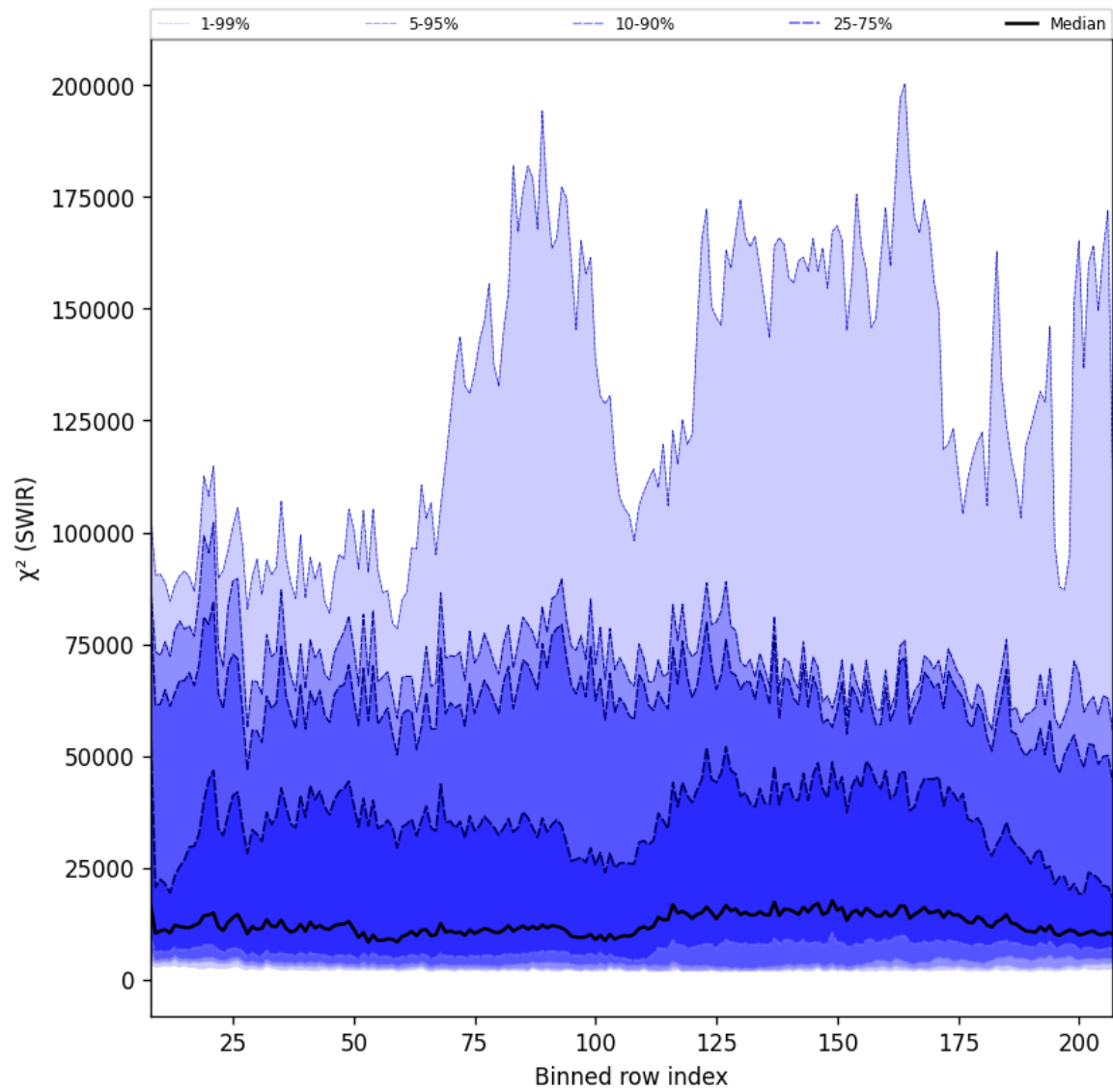
Figure 39: Along track statistics of " \chi^2 (SWIR)" for 2025-06-23 to 2025-06-25
