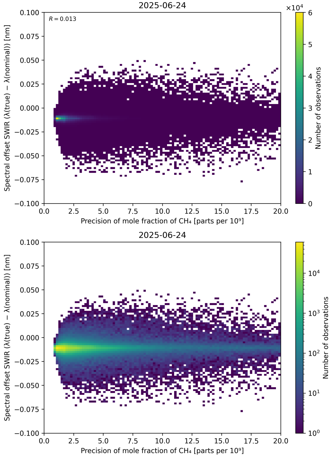
Figure 85: Scatter density plot of “Precision of mole fraction of \text{CH}_4 ” against “Spectral offset SWIR ( \lambda_{\text{true}} - \lambda_{\text{nominal}} )” for 2025-06-23 to 2025-06-25.
