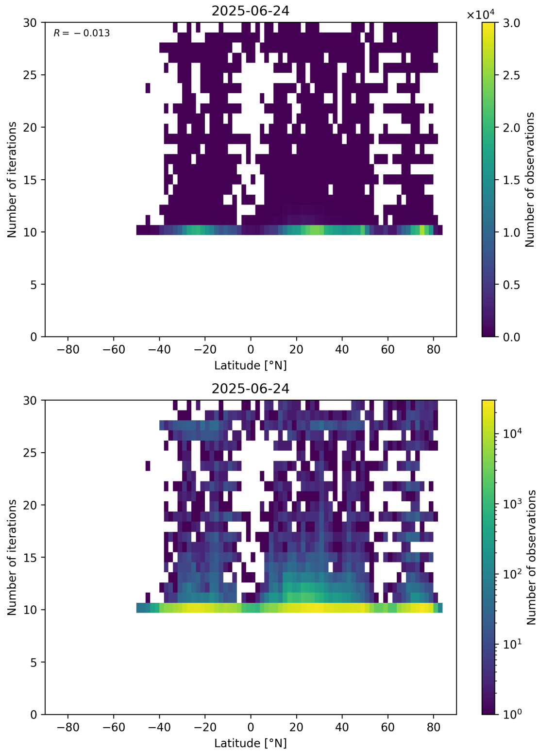
Figure 60: Scatter density plot of “Latitude” against “Number of iterations” for 2025-06-23 to 2025-06-25.
