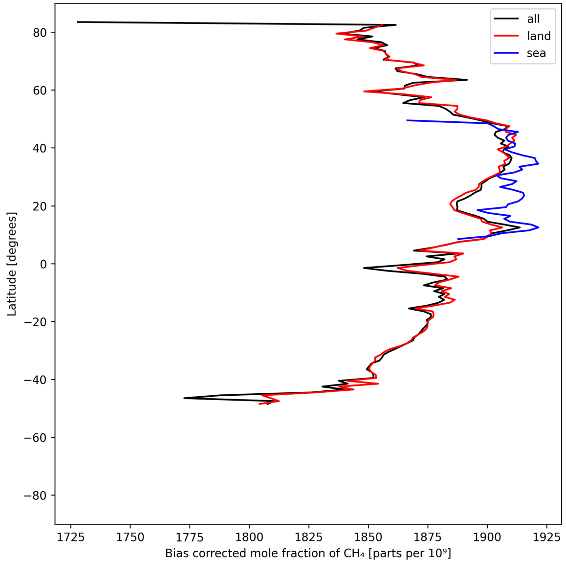
Figure 14: Zonal average of “Bias corrected mole fraction of \text{CH}_4 ” for 2025-06-23 to 2025-06-25.
