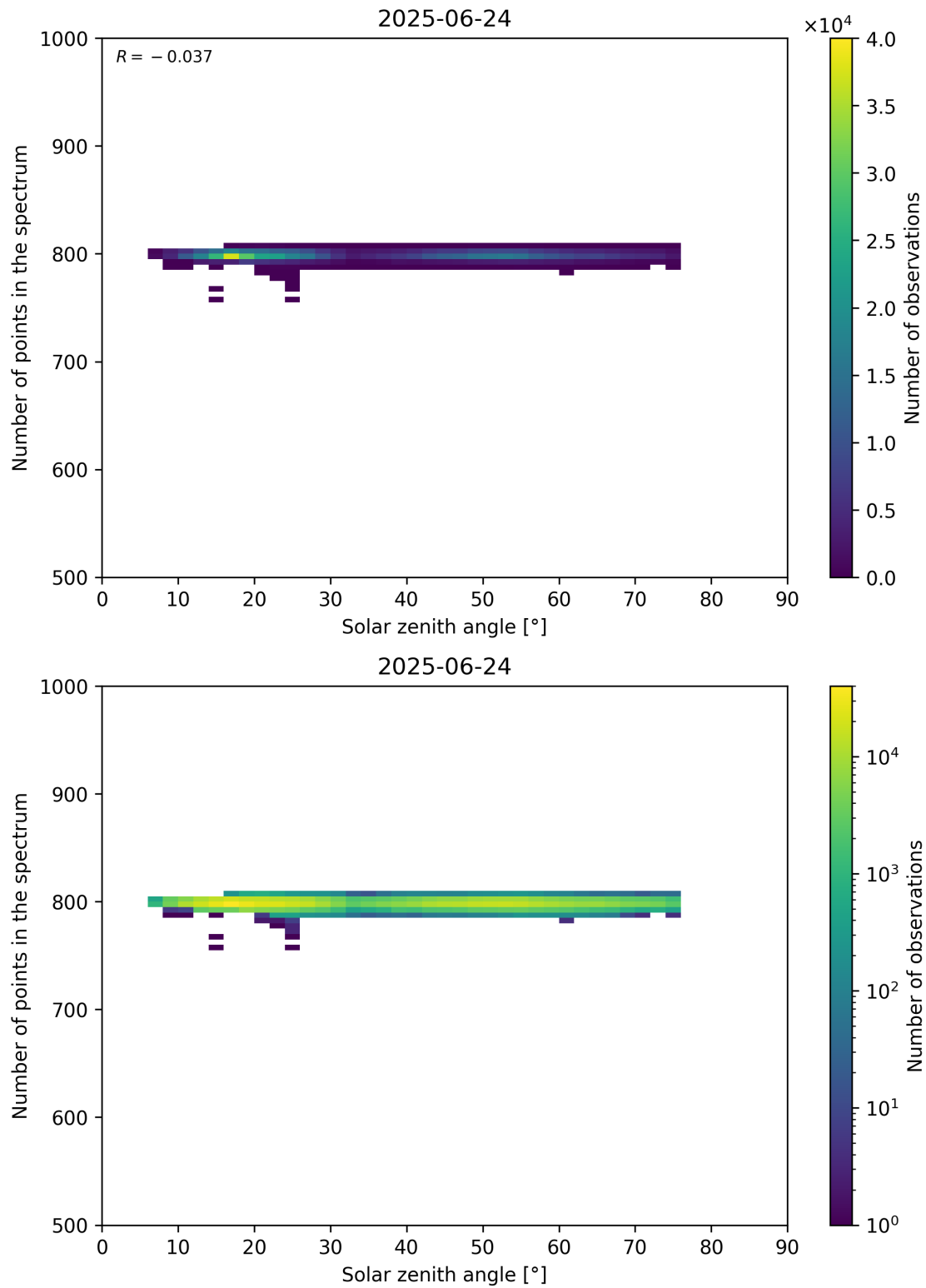
Figure 103: Scatter density plot of “Solar zenith angle” against “Number of points in the spectrum” for 2025-06-23 to 2025-06-25.
