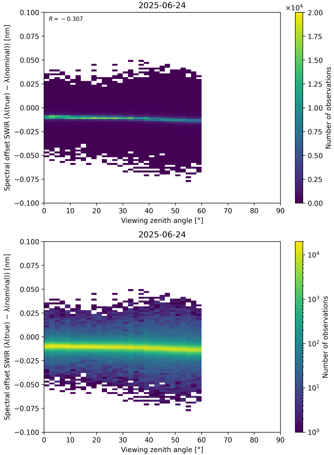
Figure 116: Scatter density plot of “Viewing zenith angle” against “Spectral offset SWIR ( \lambda_{\text{true}} - \lambda_{\text{nominal}} )” for 2025-06-23 to 2025-06-25.
