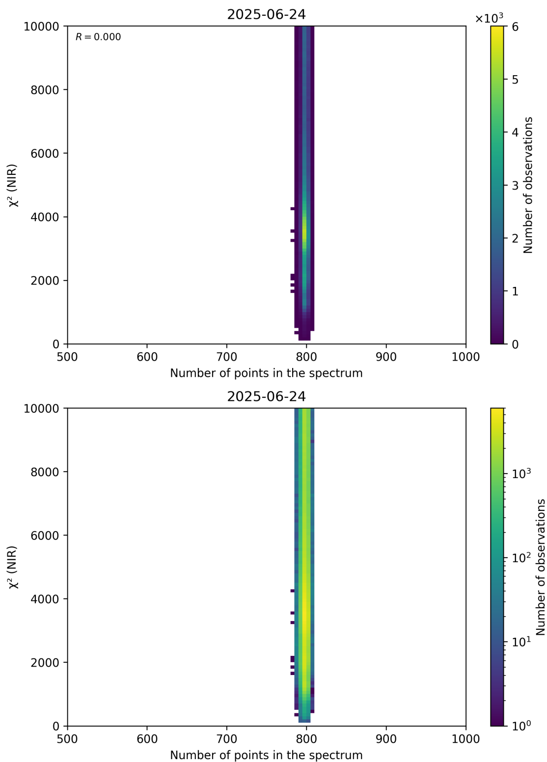
Figure 88: Scatter density plot of “Number of points in the spectrum” against “ \chi^2 (NIR)” for 2025-06-23 to 2025-06-25.
