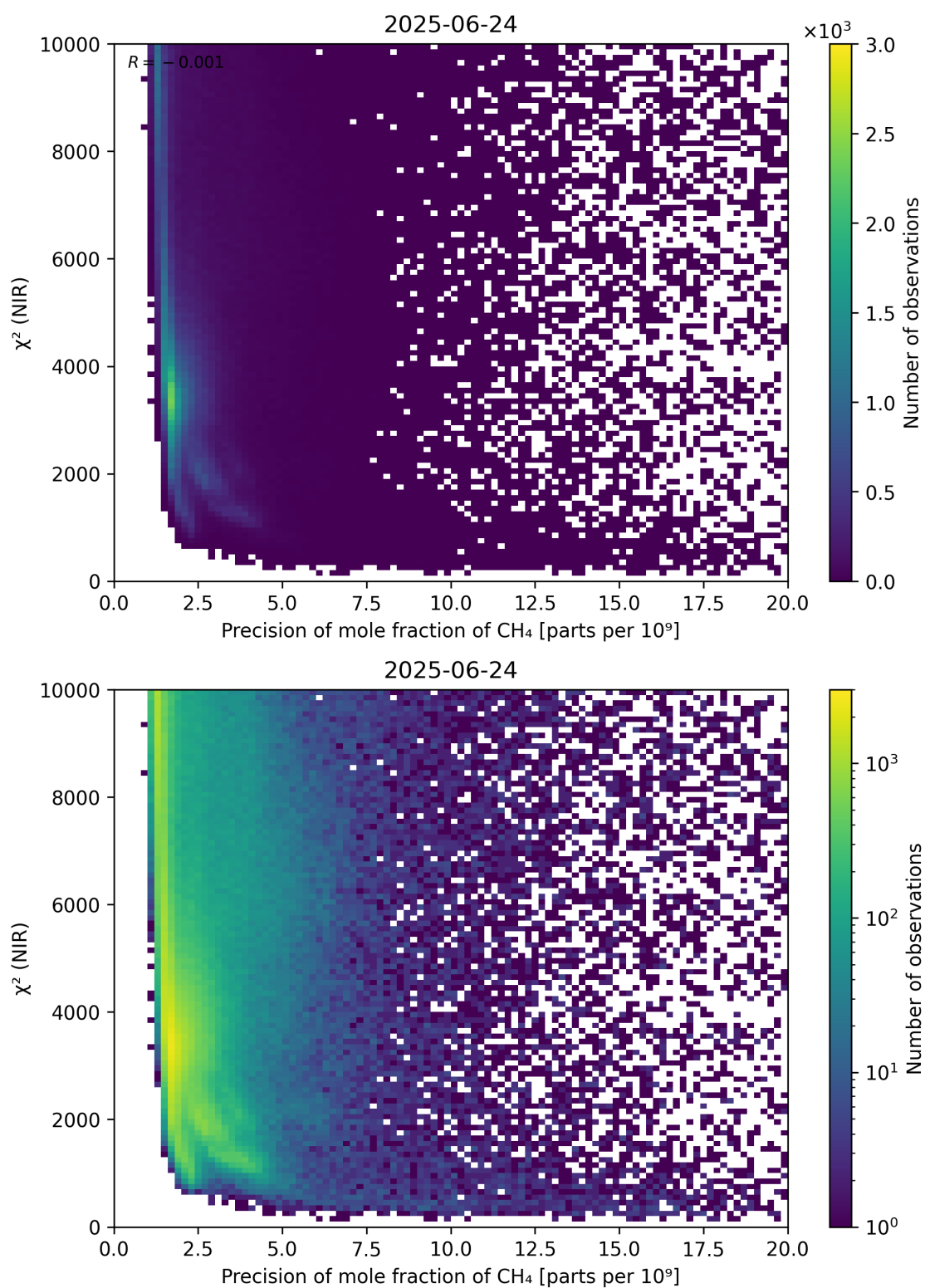
Figure 78: Scatter density plot of “Precision of mole fraction of \text{CH}_4 ” against “ \chi^2 (NIR)” for 2025-06-23 to 2025-06-25.
