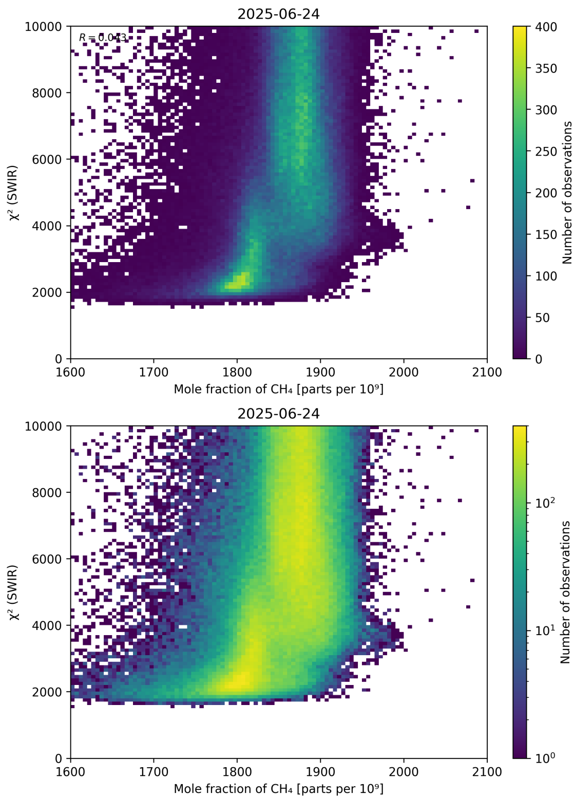
Figure 71: Scatter density plot of “Mole fraction of \text{CH}_4 ” against “ \chi^2 (SWIR)” for 2025-06-23 to 2025-06-25.
