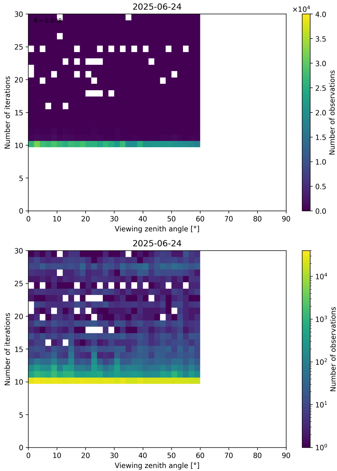
Figure 113: Scatter density plot of “Viewing zenith angle” against “Number of iterations” for 2025-06-23 to 2025-06-25.
