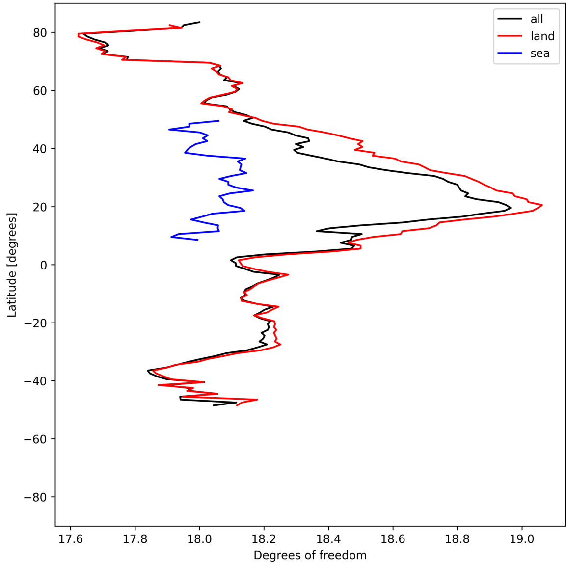
Figure 19: Zonal average of “Degrees of freedom” for 2025-06-23 to 2025-06-25.
