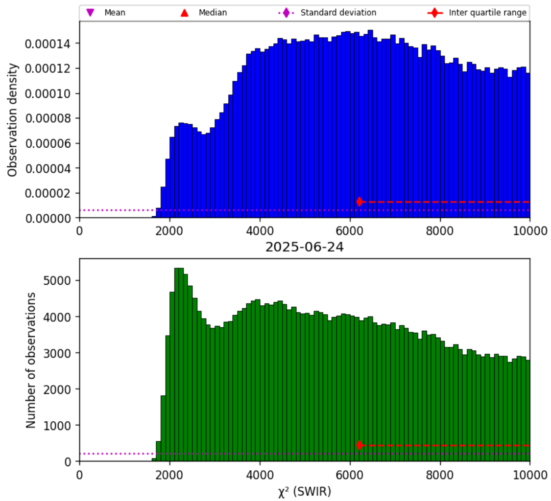
Figure 28: Histogram of “ \chi^2 (SWIR)” for 2025-06-23 to 2025-06-25
