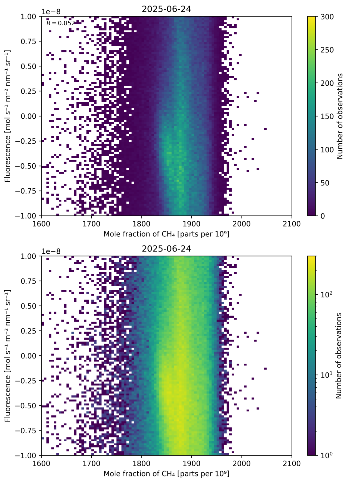
Figure 73: Scatter density plot of “Mole fraction of \text{CH}_4 ” against “Fluorescence” for 2025-06-23 to 2025-06-25.
