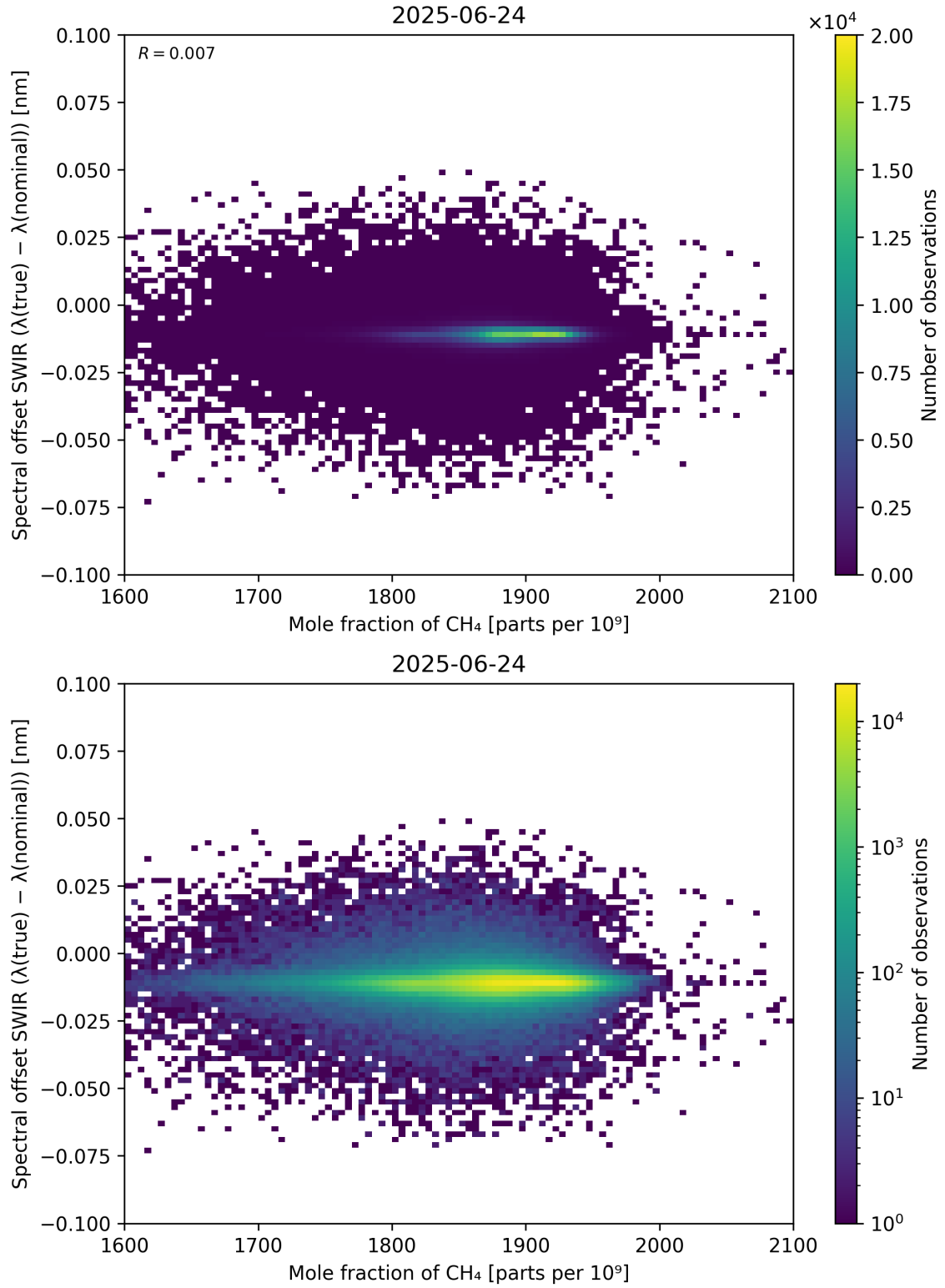
Figure 86: Scatter density plot of “Mole fraction of CH 4 ” against “Spectral offset SWIR ( \lambda_{\text{true}} - \lambda_{\text{nominal}} )” for 2025-06-23 to 2025-06-25.
