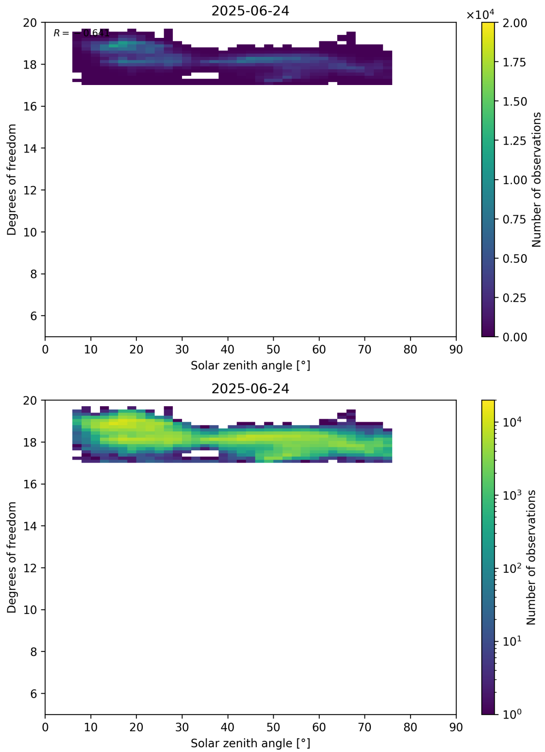
Figure 96: Scatter density plot of “Solar zenith angle” against “Degrees of freedom” for 2025-06-23 to 2025-06-25.
