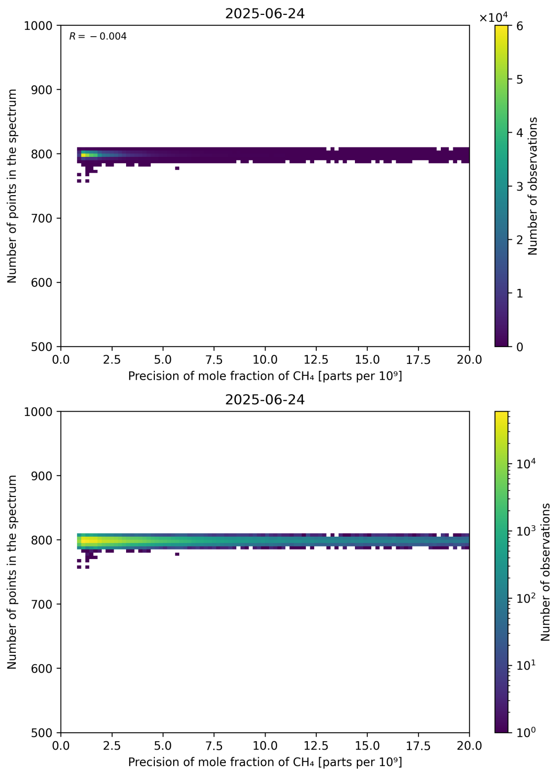
Figure 84: Scatter density plot of “Precision of mole fraction of CH 4 ” against “Number of points in the spectrum” for 2025-06-23 to 2025-06-25.
