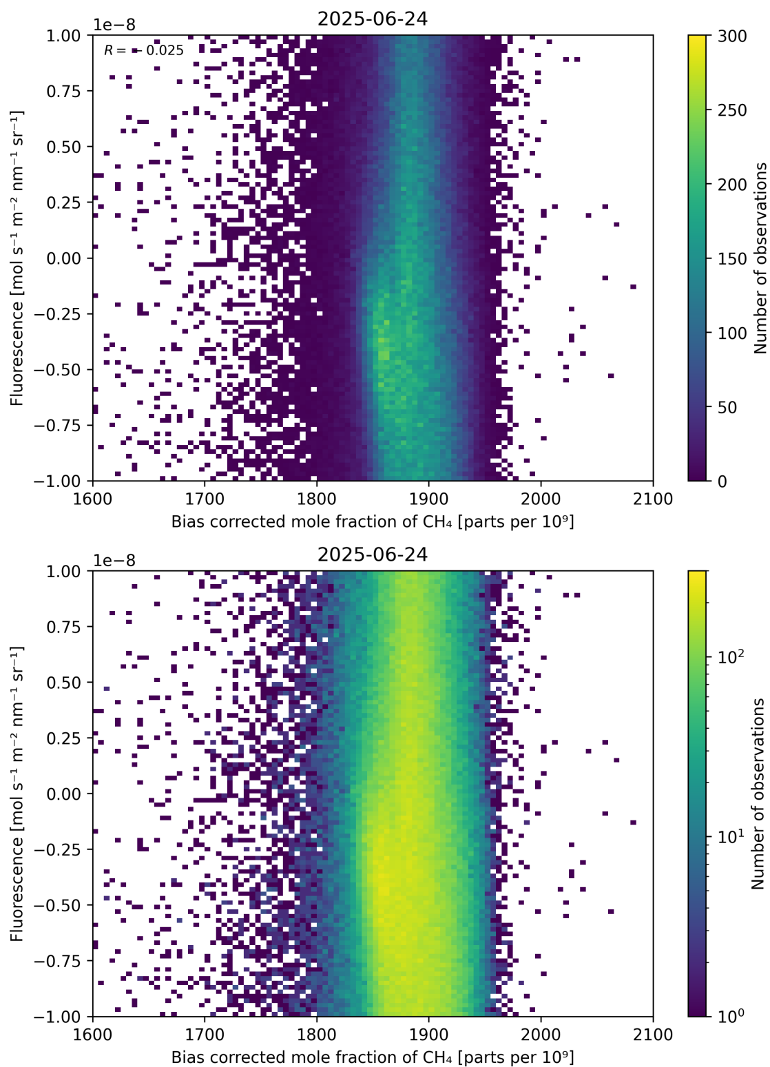
Figure 66: Scatter density plot of “Bias corrected mole fraction of \text{CH}_4 ” against “Fluorescence” for 2025-06-23 to 2025-06-25.
