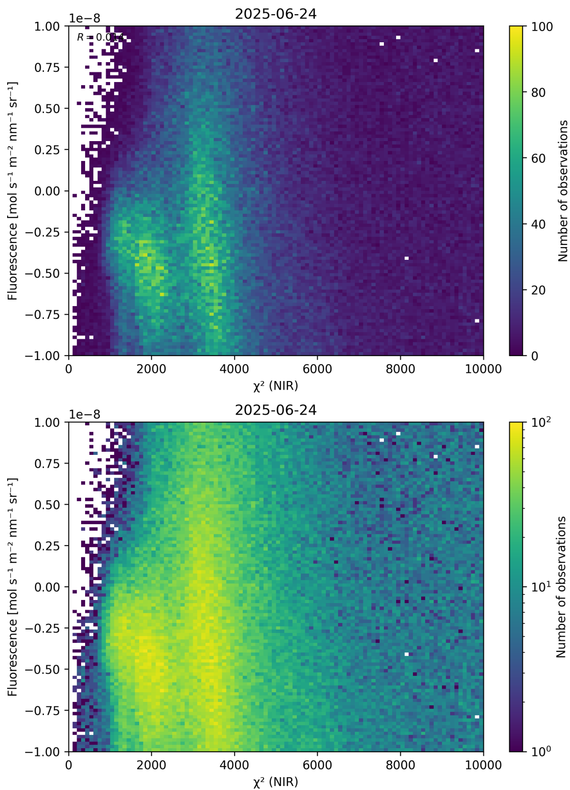
Figure 45: Scatter density plot of “ \chi^2 (NIR)” against “Fluorescence” for 2025-06-23 to 2025-06-25.
