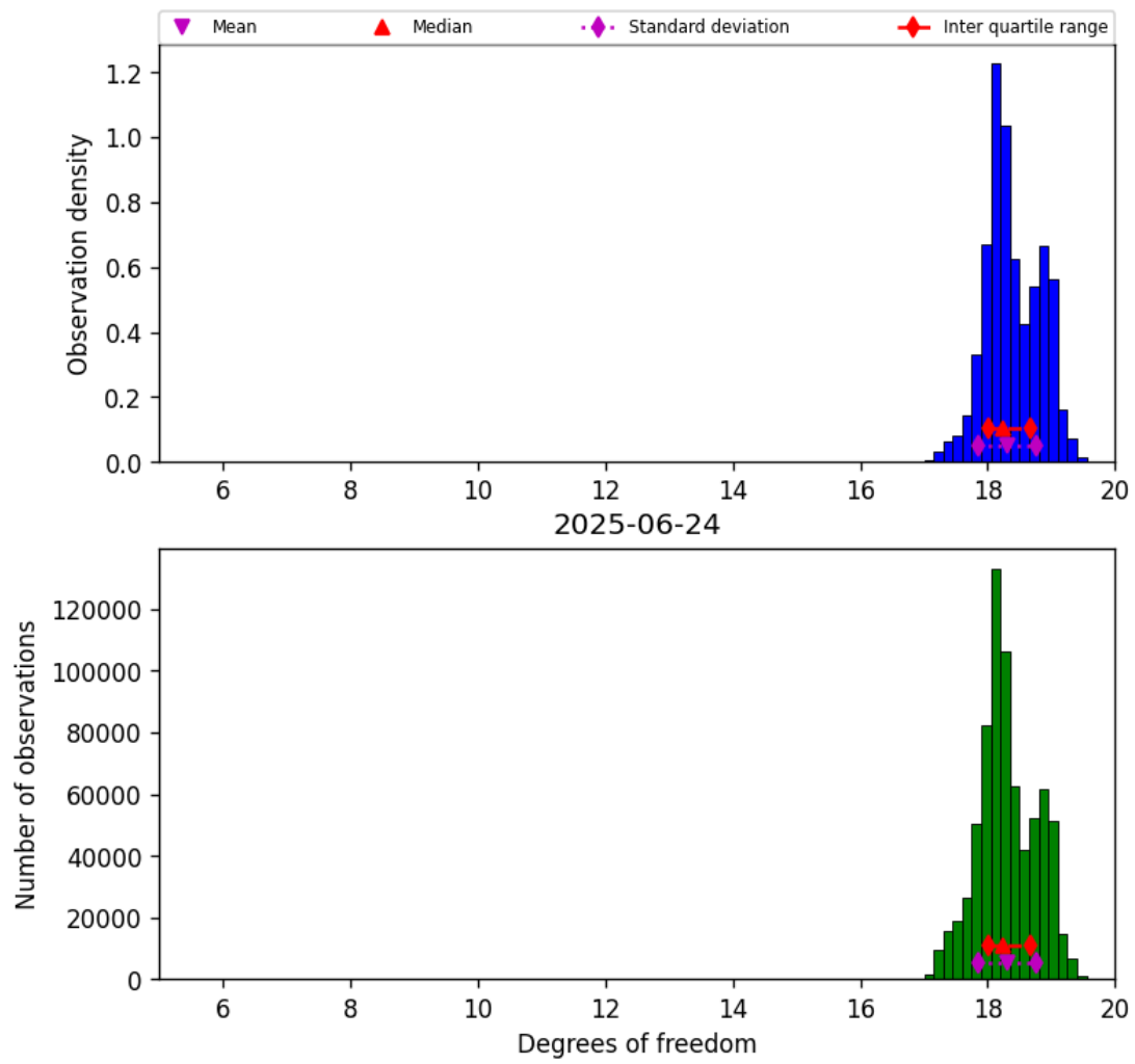
Figure 30: Histogram of “Degrees of freedom” for 2025-06-23 to 2025-06-25
