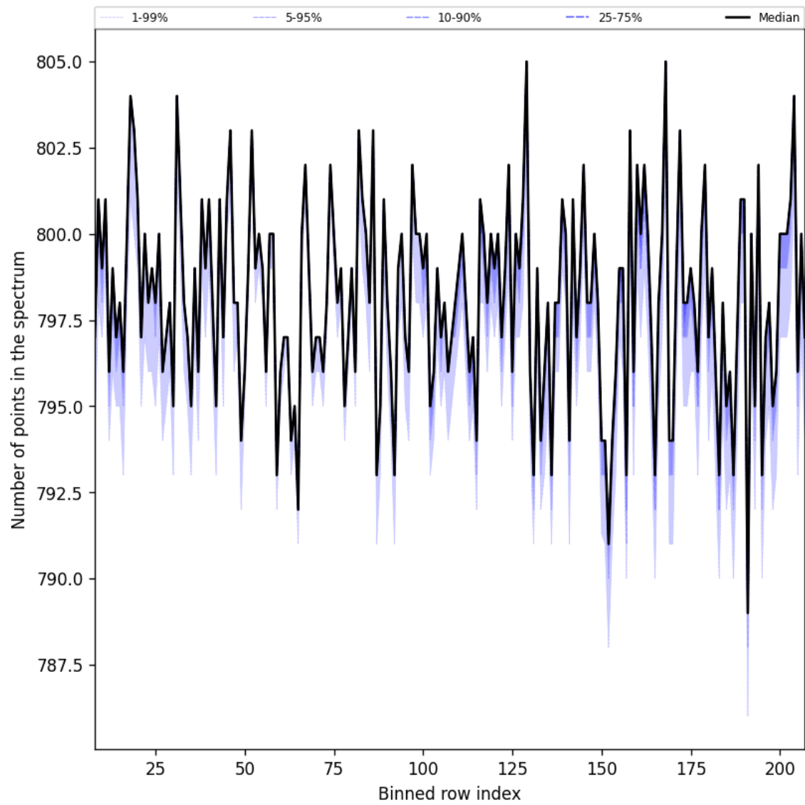
Figure 37: Along track statistics of “Number of points in the spectrum” for 2025-06-23 to 2025-06-25
