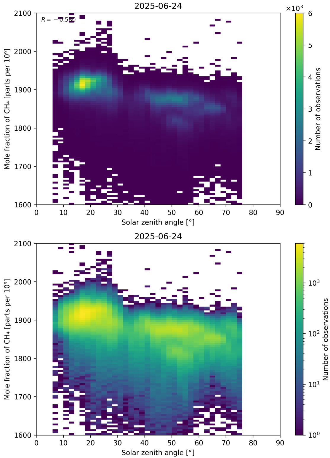
Figure 99: Scatter density plot of “Solar zenith angle” against “Mole fraction of CH 4 ” for 2025-06-23 to 2025-06-25.
