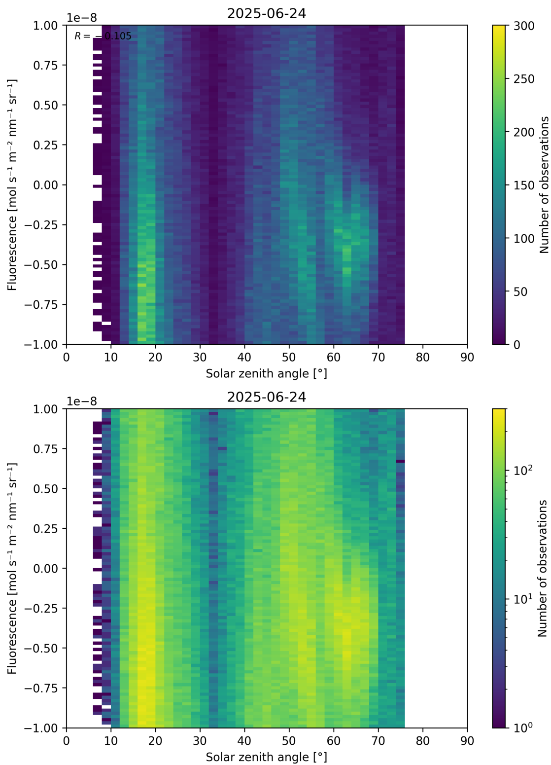
Figure 97: Scatter density plot of “Solar zenith angle” against “Fluorescence” for 2025-06-23 to 2025-06-25.
