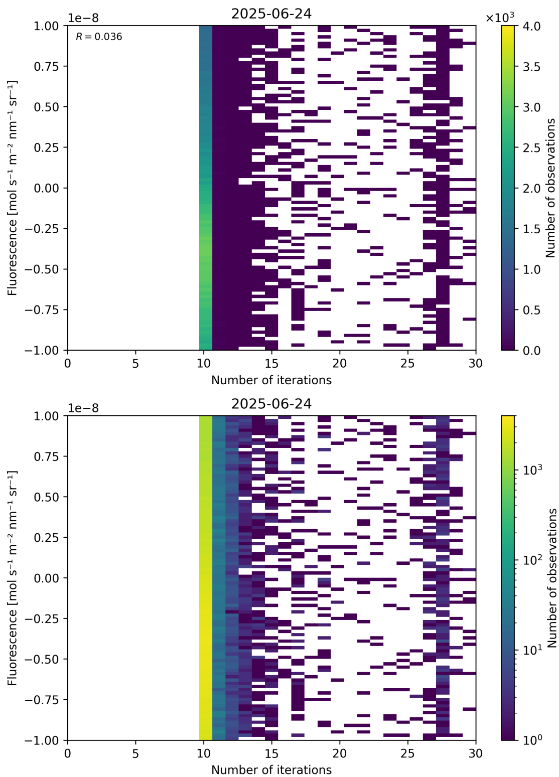
Figure 87: Scatter density plot of “Number of iterations” against “Fluorescence” for 2025-06-23 to 2025-06-25.
