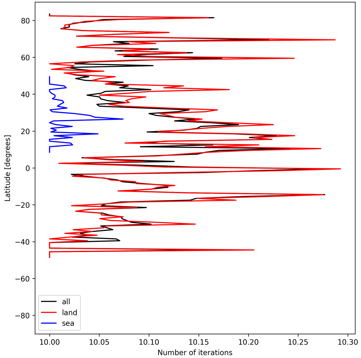
Figure 20: Zonal average of “Number of iterations” for 2025-06-23 to 2025-06-25.
