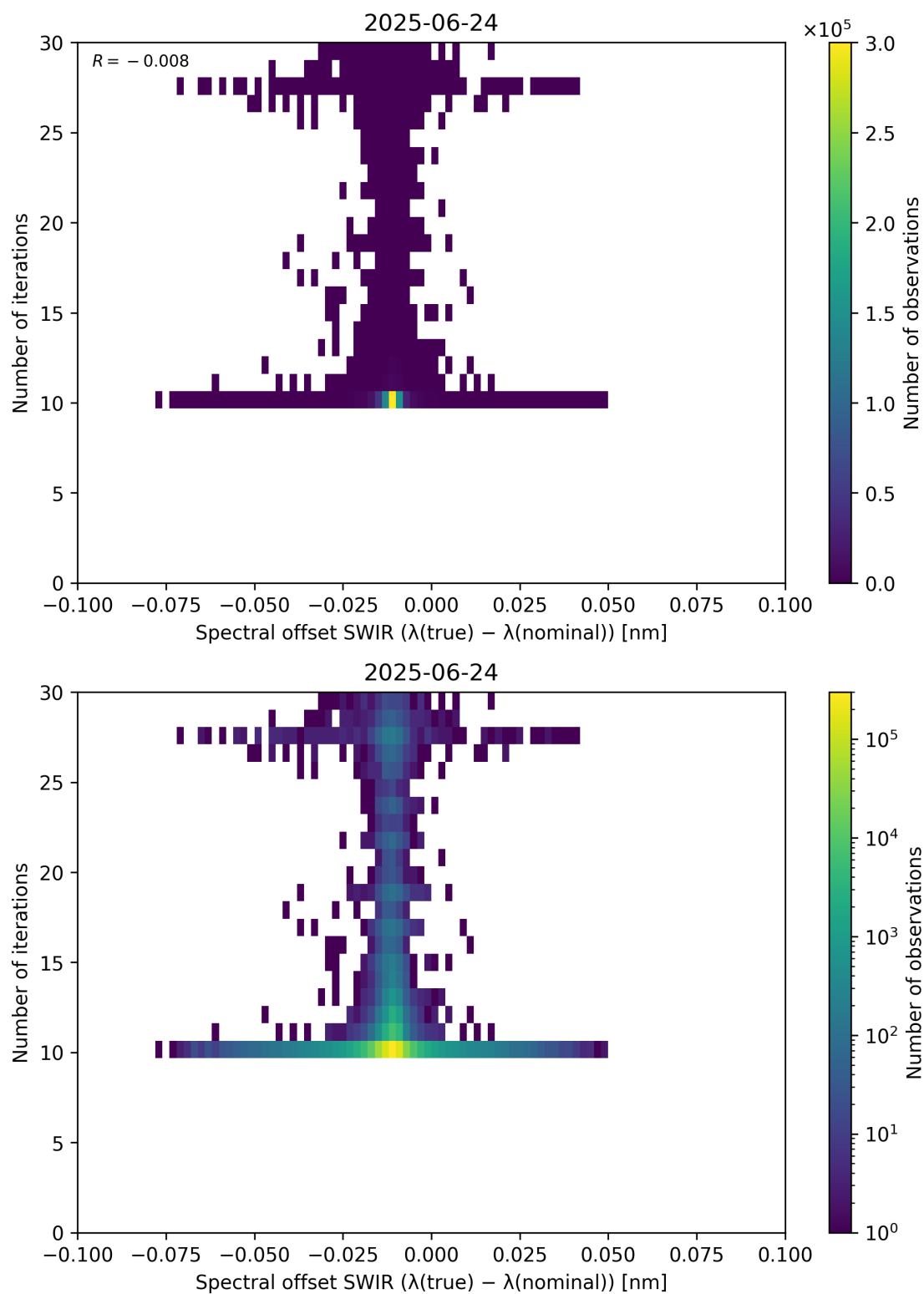
Figure 121: Scatter density plot of “Spectral offset SWIR ( \lambda_{\text{true}} - \lambda_{\text{nominal}} )” against “Number of iterations” for 2025-06-23 to 2025-06-25.
