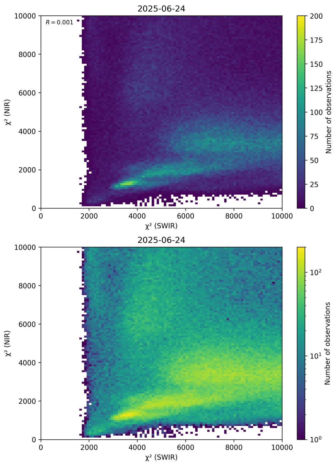
Figure 47: Scatter density plot of “ \chi^2 (SWIR)” against “ \chi^2 (NIR)” for 2025-06-23 to 2025-06-25.
