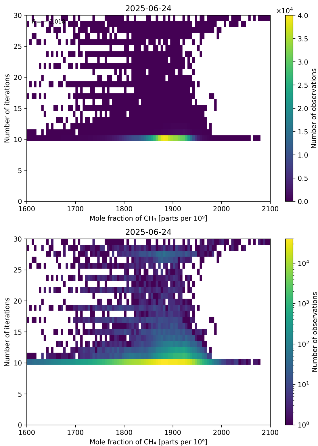
Figure 76: Scatter density plot of “Mole fraction of CH 4 ” against “Number of iterations” for 2025-06-23 to 2025-06-25.
