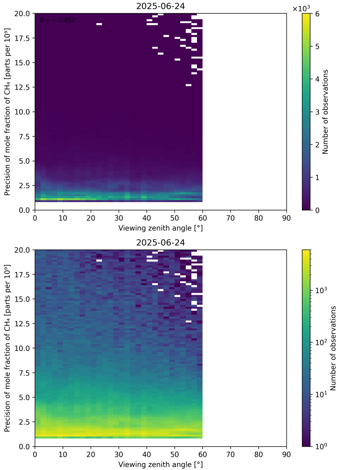
Figure 112: Scatter density plot of “Viewing zenith angle” against “Precision of mole fraction of \text{CH}_4 ” for 2025-06-23 to 2025-06-25.
