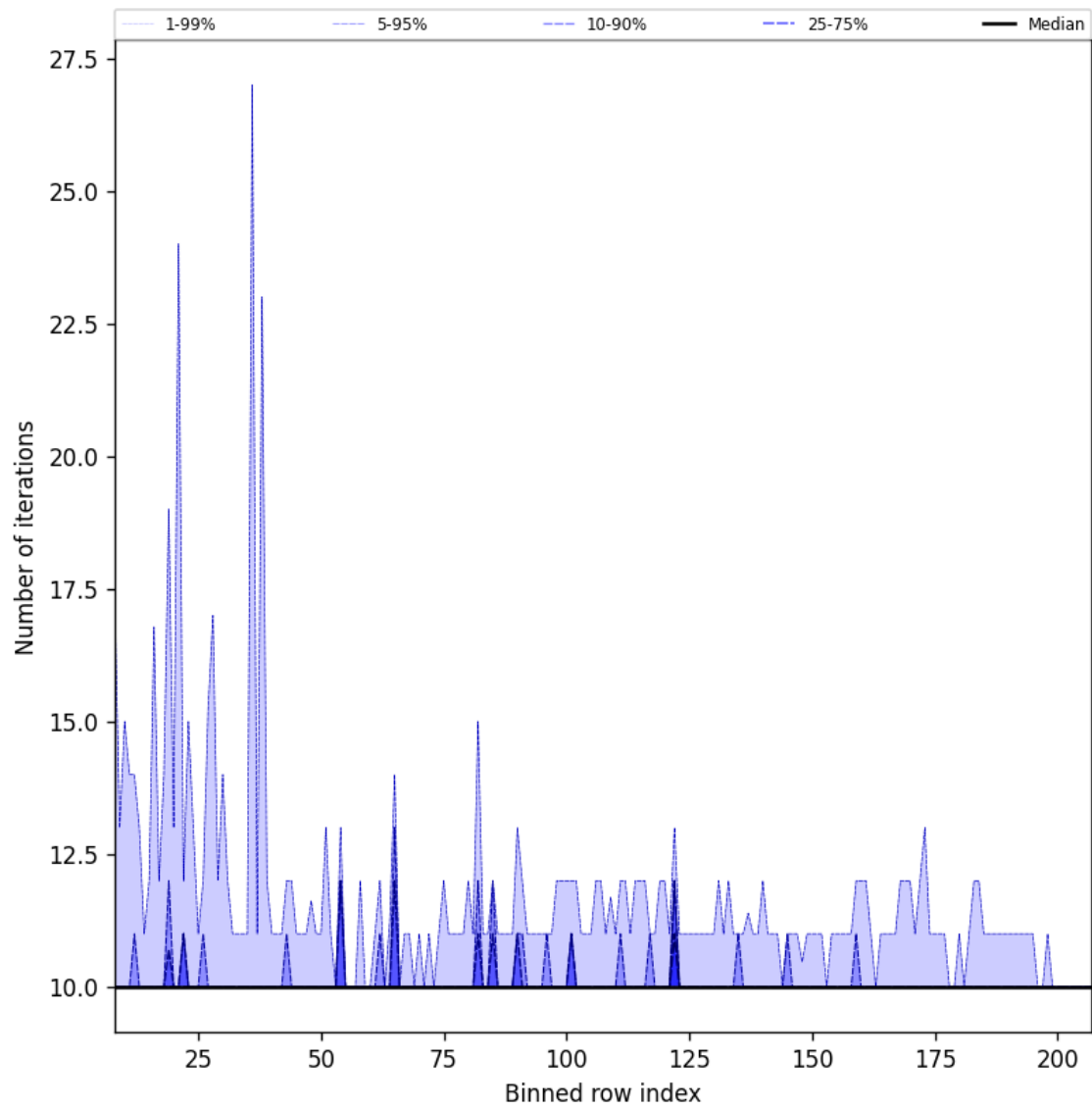
Figure 42: Along track statistics of “Number of iterations” for 2025-06-23 to 2025-06-25
