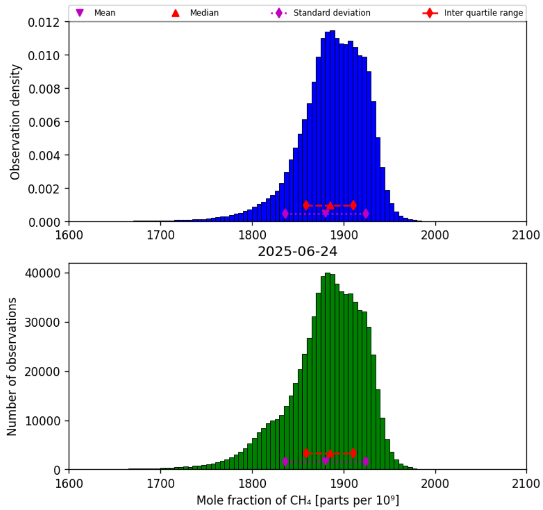
Figure 23: Histogram of “Mole fraction of CH 4 ” for 2025-06-23 to 2025-06-25
