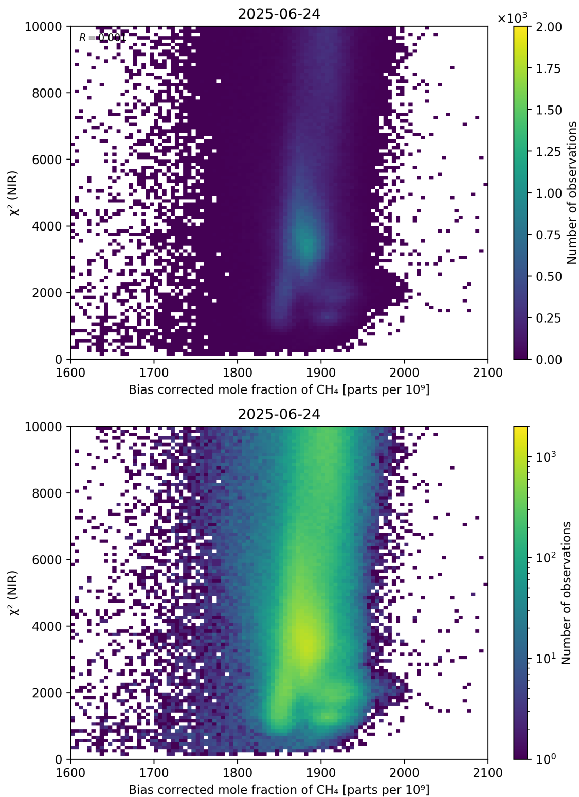
Figure 63: Scatter density plot of “Bias corrected mole fraction of \text{CH}_4 ” against “ \chi^2 (NIR)” for 2025-06-23 to 2025-06-25.
