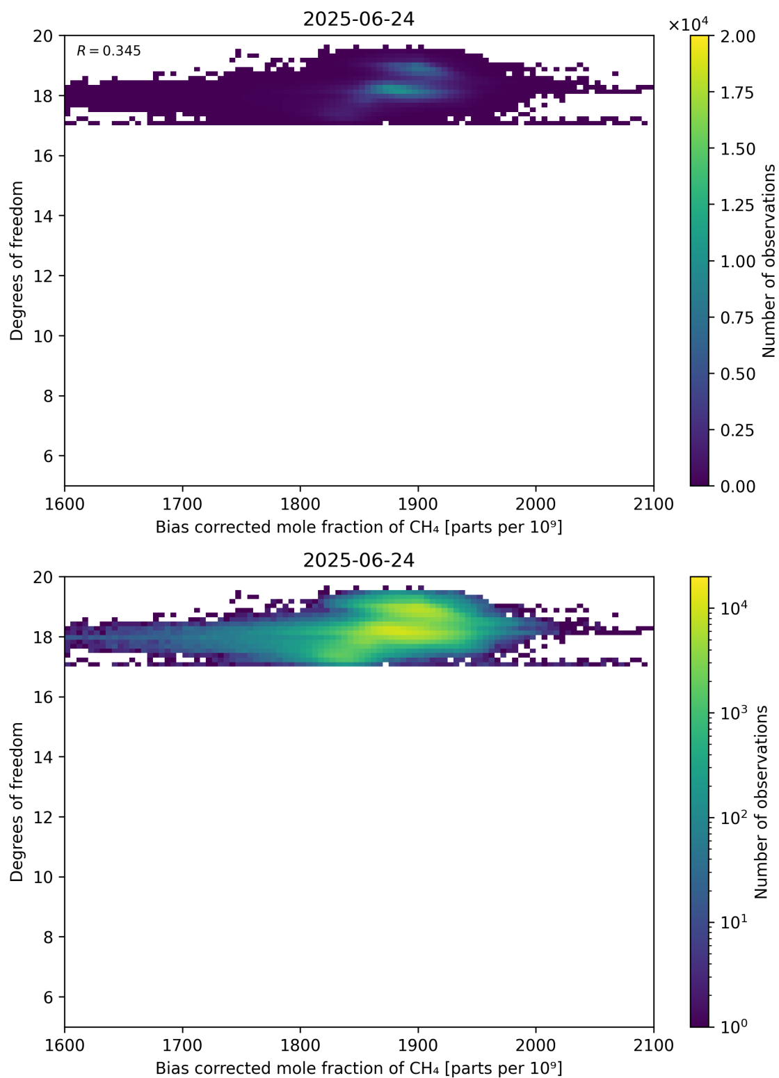
Figure 65: Scatter density plot of “Bias corrected mole fraction of CH 4 ” against “Degrees of freedom” for 2025-06-23 to 2025-06-25.
