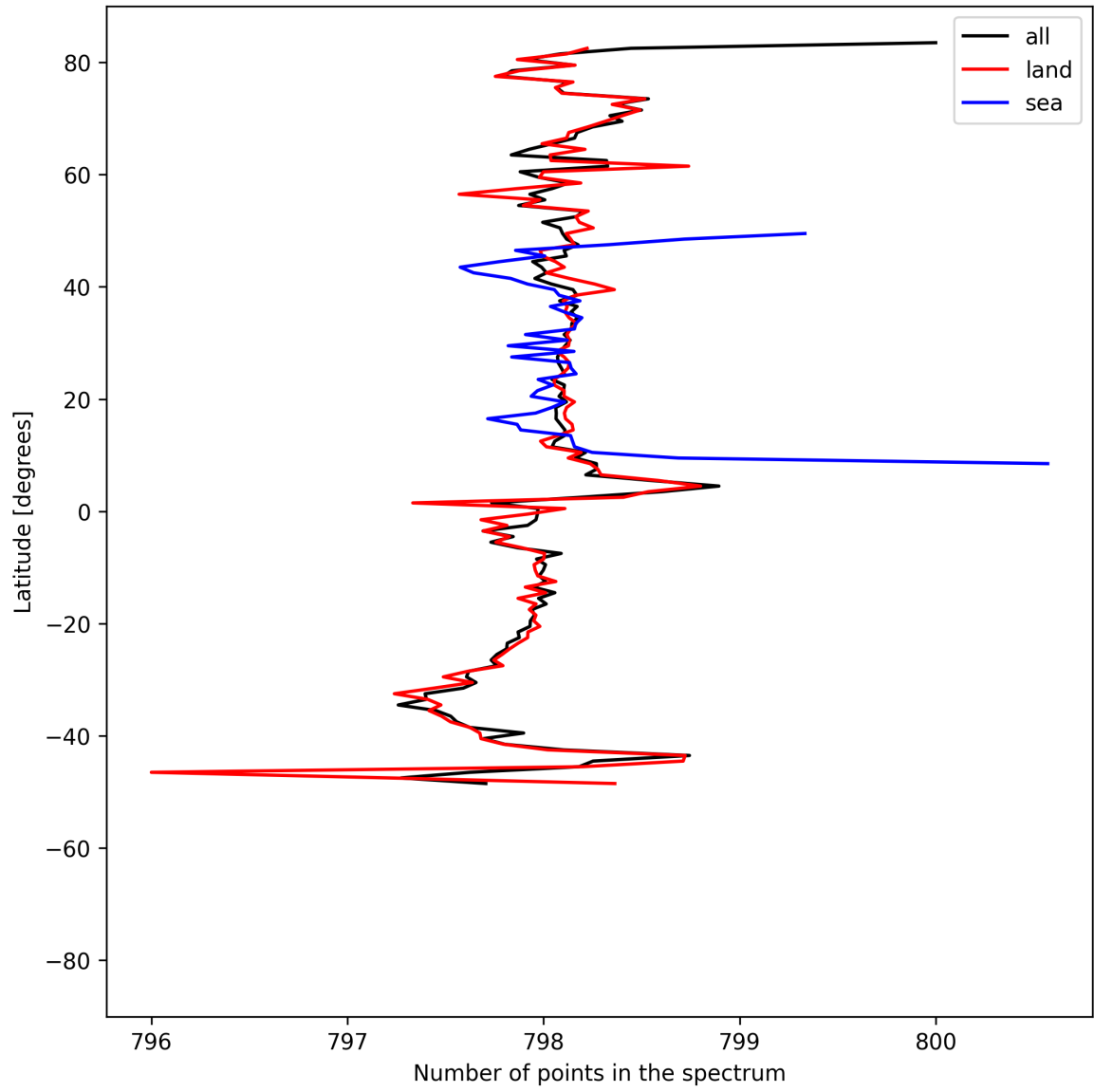
Figure 15: Zonal average of “Number of points in the spectrum” for 2025-06-23 to 2025-06-25.
