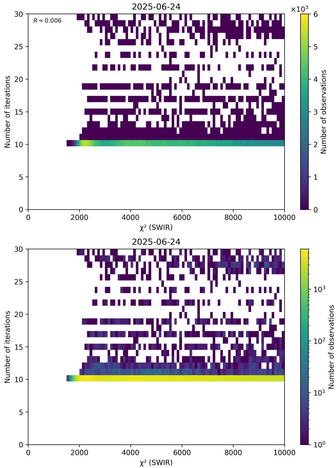
Figure 50: Scatter density plot of “ \chi^2 (SWIR)” against “Number of iterations” for 2025-06-23 to 2025-06-25.
