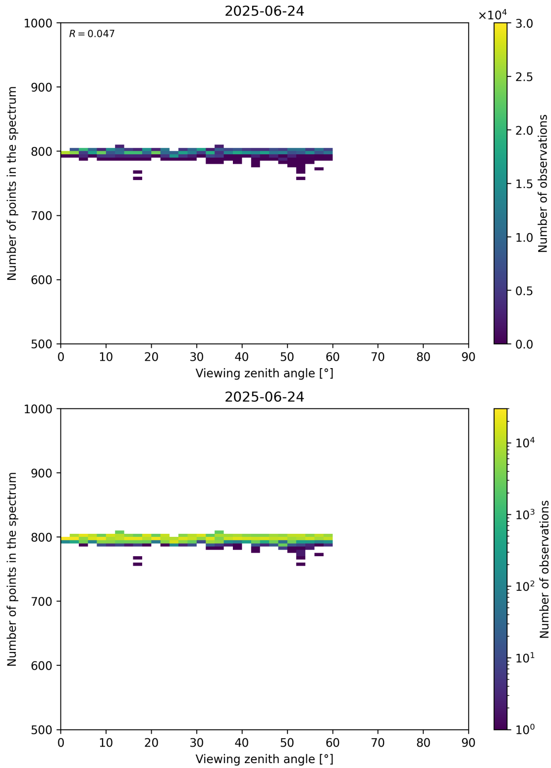
Figure 114: Scatter density plot of “Viewing zenith angle” against “Number of points in the spectrum” for 2025-06-23 to 2025-06-25.
