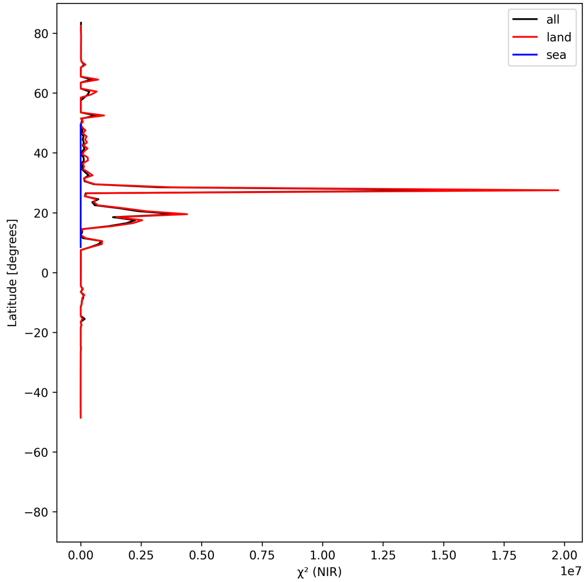
Figure 18: Zonal average of “ \chi^2 (NIR)” for 2025-06-23 to 2025-06-25.
