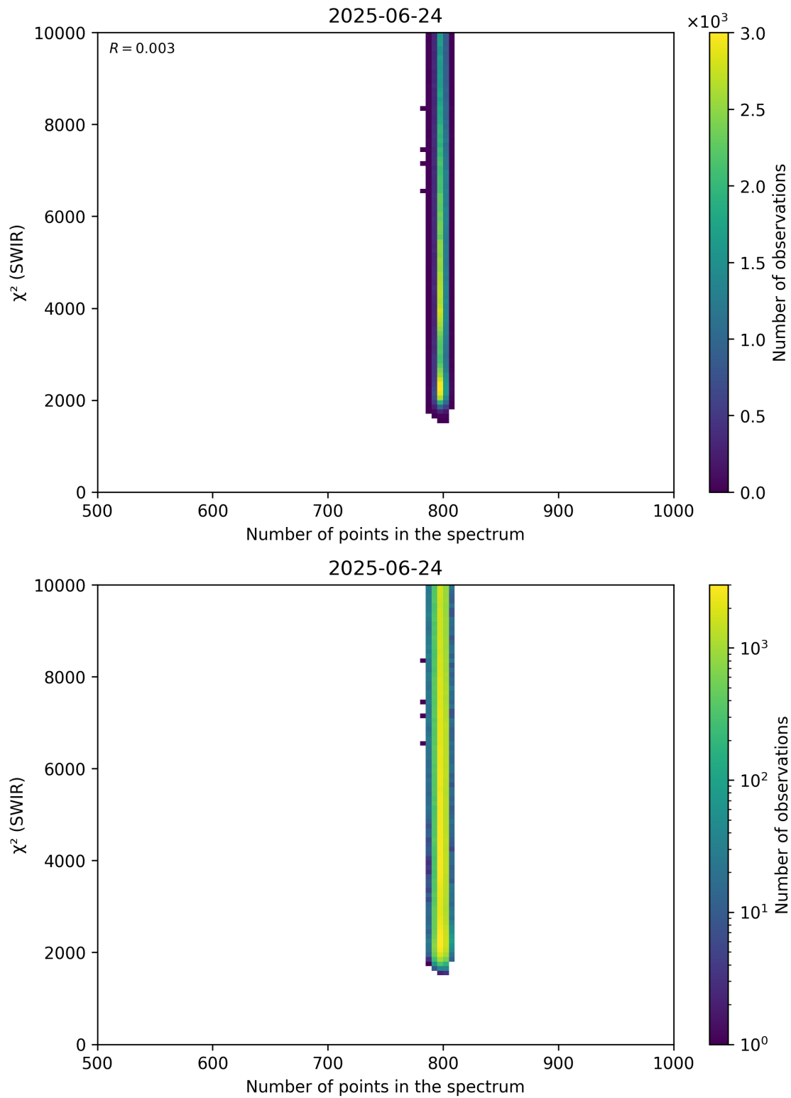
Figure 89: Scatter density plot of “Number of points in the spectrum” against “ \chi^2 (SWIR)” for 2025-06-23 to 2025-06-25.
