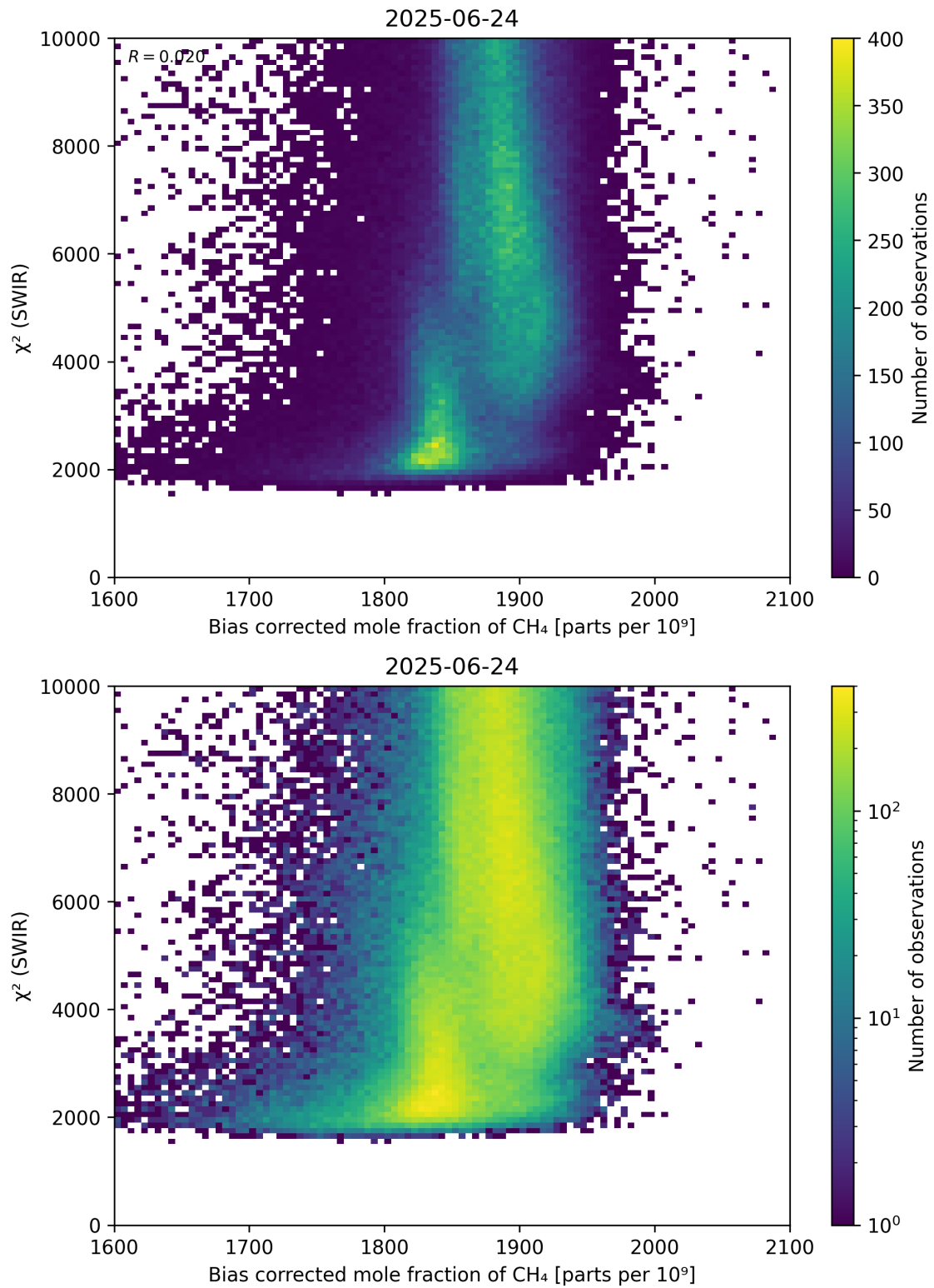
Figure 64: Scatter density plot of “Bias corrected mole fraction of \text{CH}_4 ” against “ \chi^2 (SWIR)” for 2025-06-23 to 2025-06-25.
