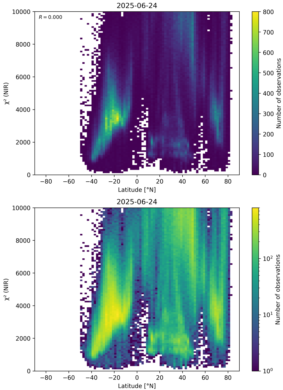
Figure 53: Scatter density plot of “Latitude” against “ \chi^2 (NIR)” for 2025-06-23 to 2025-06-25.
