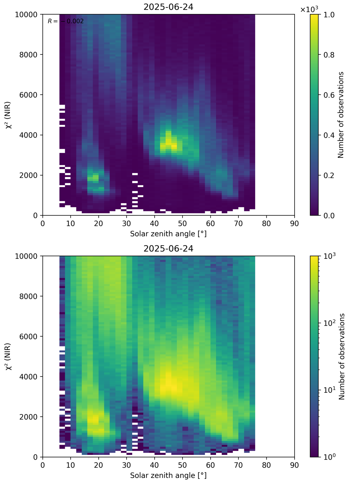
Figure 94: Scatter density plot of “Solar zenith angle” against “ \chi^2 (NIR)” for 2025-06-23 to 2025-06-25.
