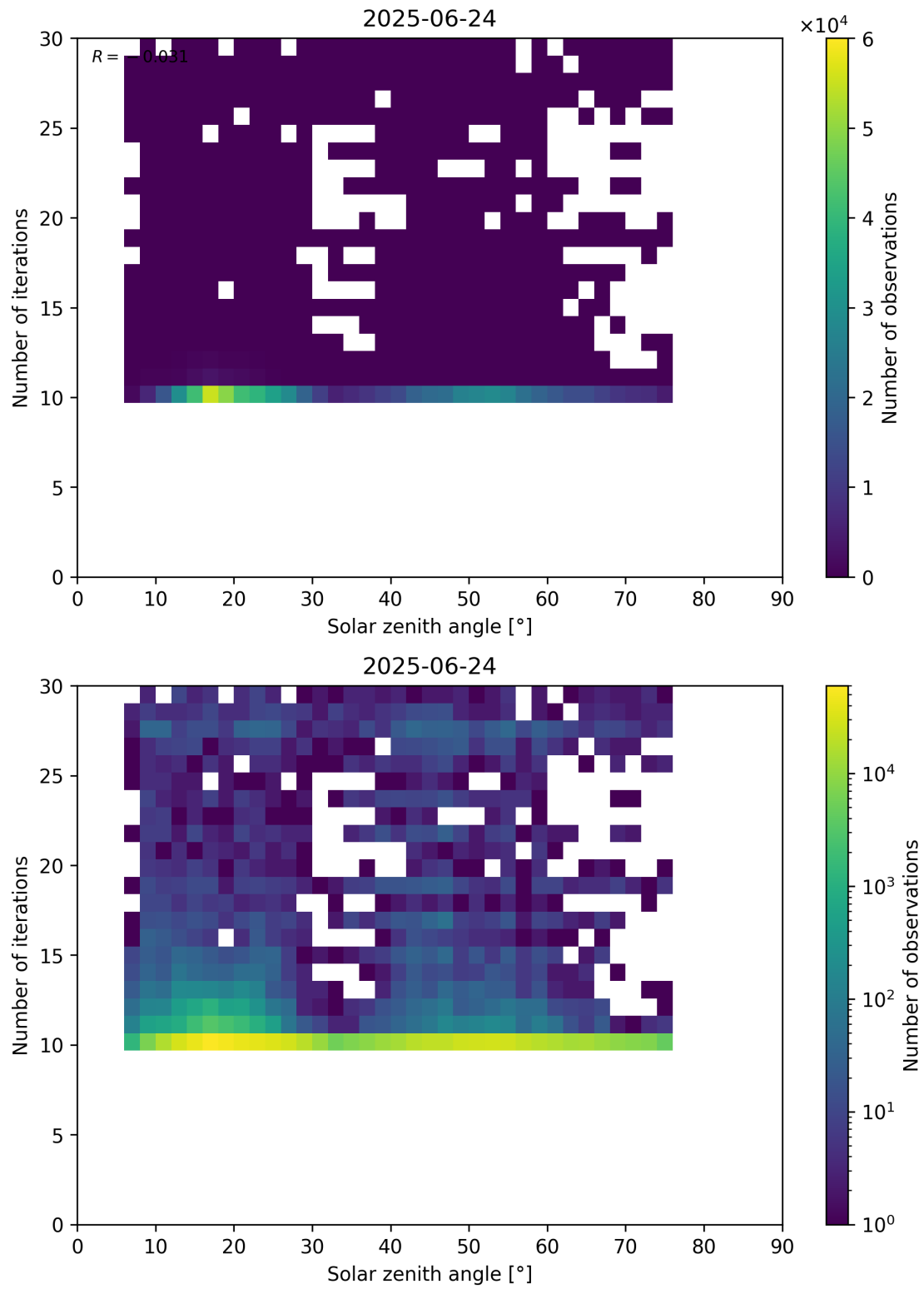
Figure 102: Scatter density plot of “Solar zenith angle” against “Number of iterations” for 2025-06-23 to 2025-06-25.
