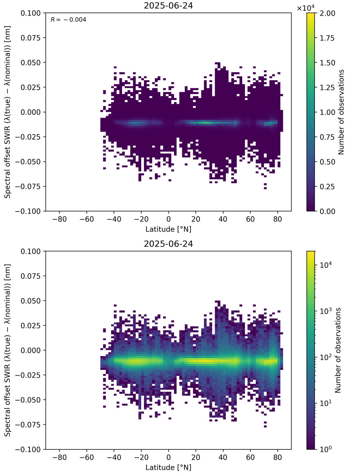
Figure 62: Scatter density plot of “Latitude” against “Spectral offset SWIR ( \lambda_{\text{true}} - \lambda_{\text{nominal}} )” for 2025-06-23 to 2025-06-25.
