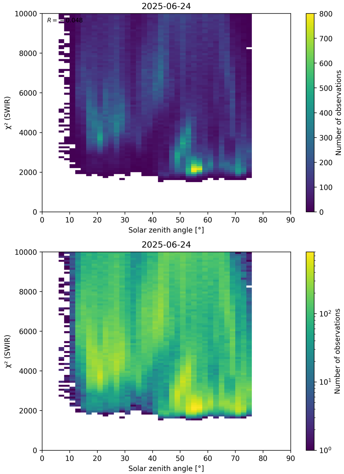
Figure 95: Scatter density plot of “Solar zenith angle” against “ \chi^2 (SWIR)” for 2025-06-23 to 2025-06-25.
