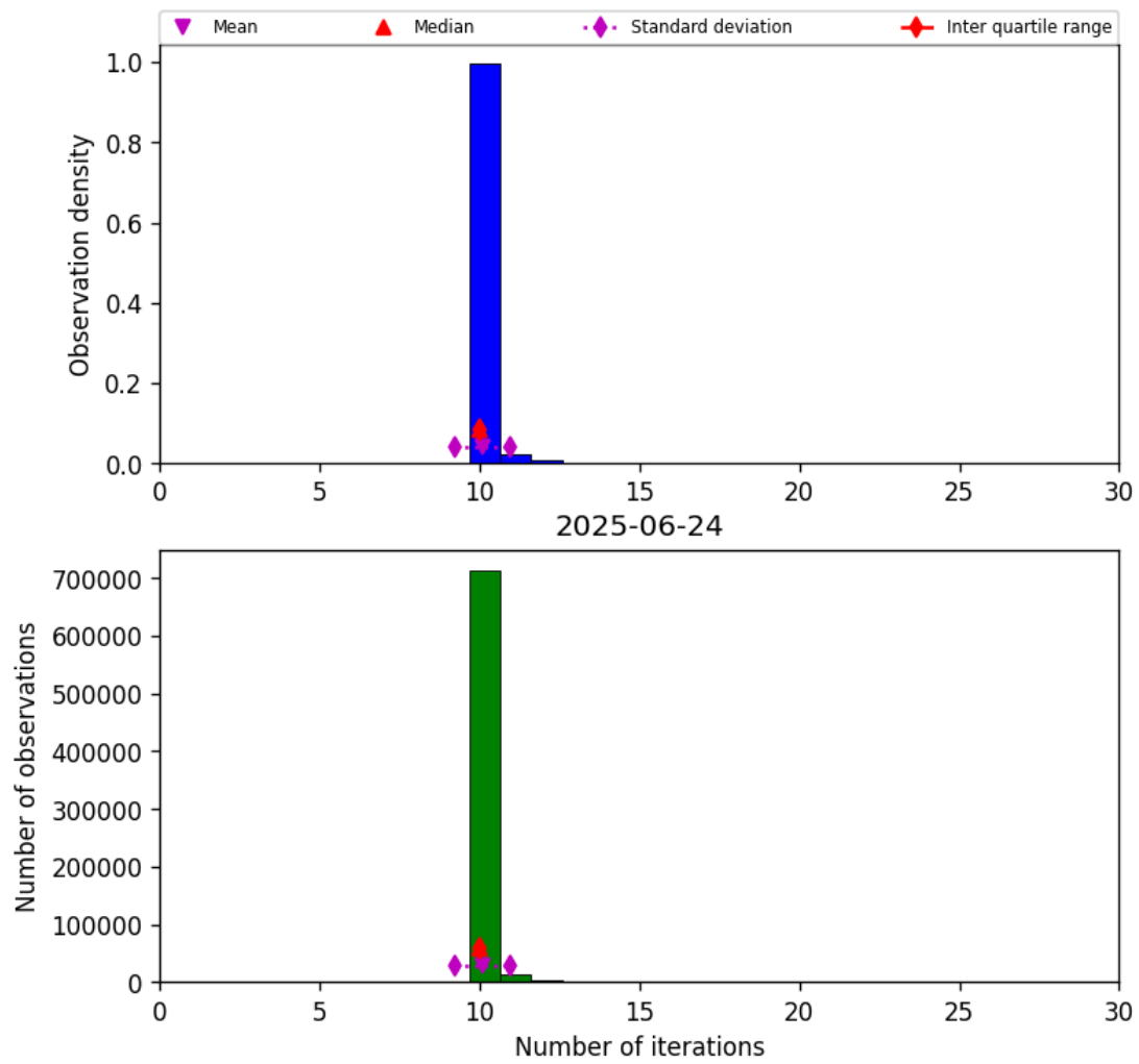
Figure 31: Histogram of “Number of iterations” for 2025-06-23 to 2025-06-25
