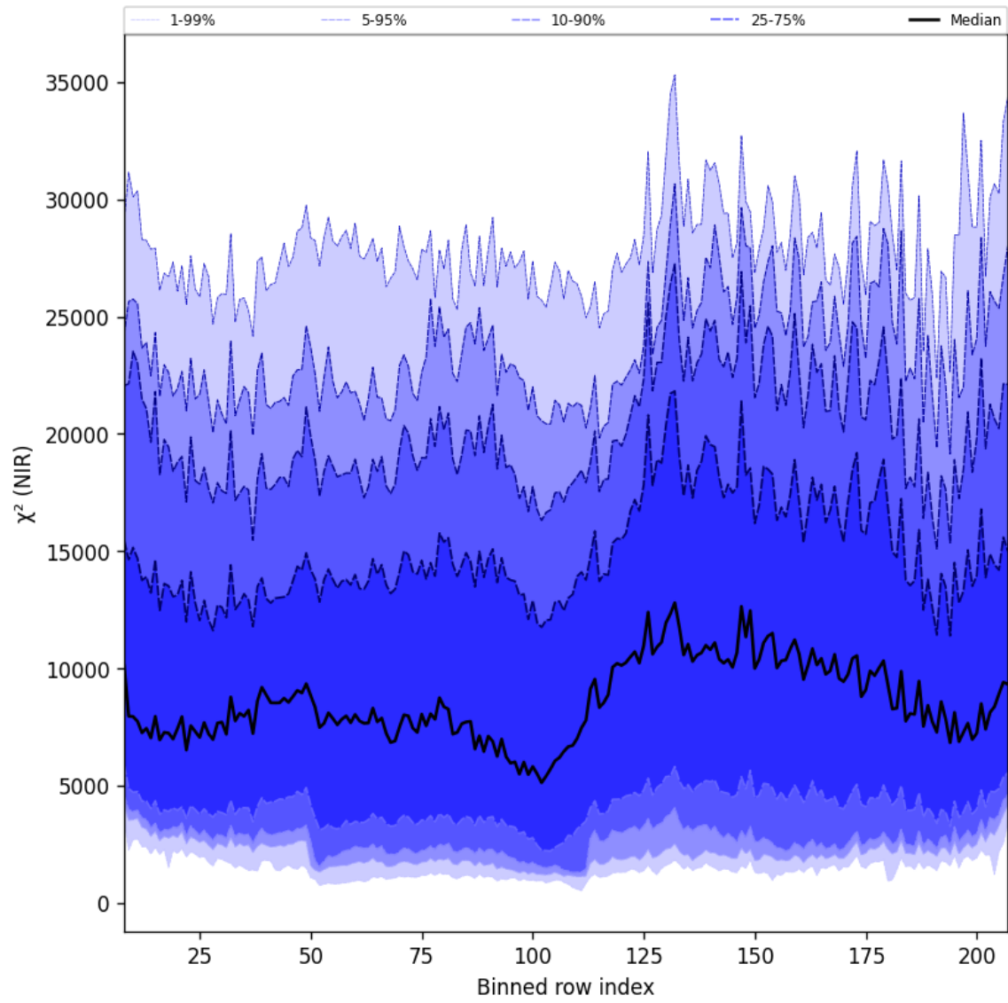
Figure 40: Along track statistics of “ \chi^2 (NIR)” for 2025-06-23 to 2025-06-25
