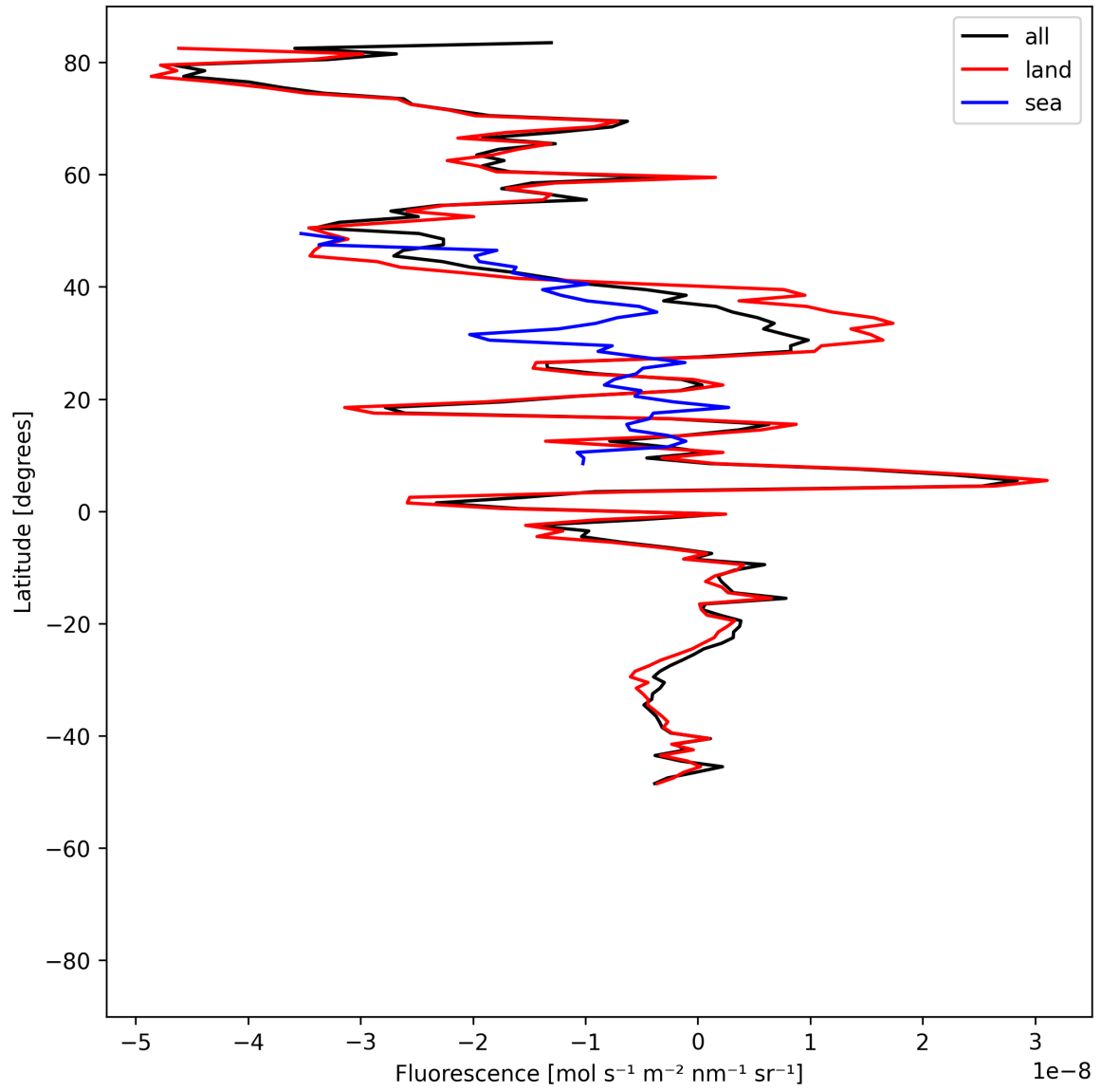
Figure 21: Zonal average of “Fluorescence” for 2025-06-23 to 2025-06-25.
