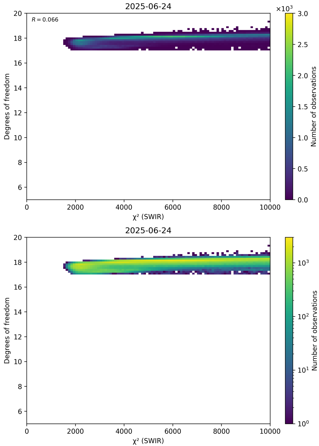
Figure 48: Scatter density plot of “ \chi^2 (SWIR)” against “Degrees of freedom” for 2025-06-23 to 2025-06-25.
