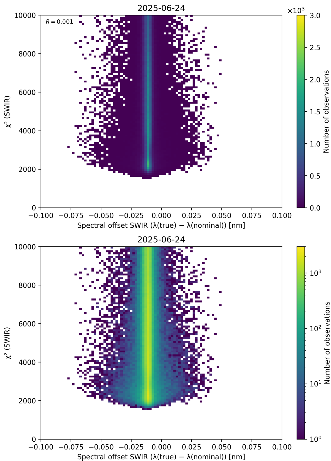
Figure 118: Scatter density plot of “Spectral offset SWIR ( \lambda_{\text{true}} - \lambda_{\text{nominal}} )” against “ \chi^2 (SWIR)” for 2025-06-23 to 2025-06-25.
