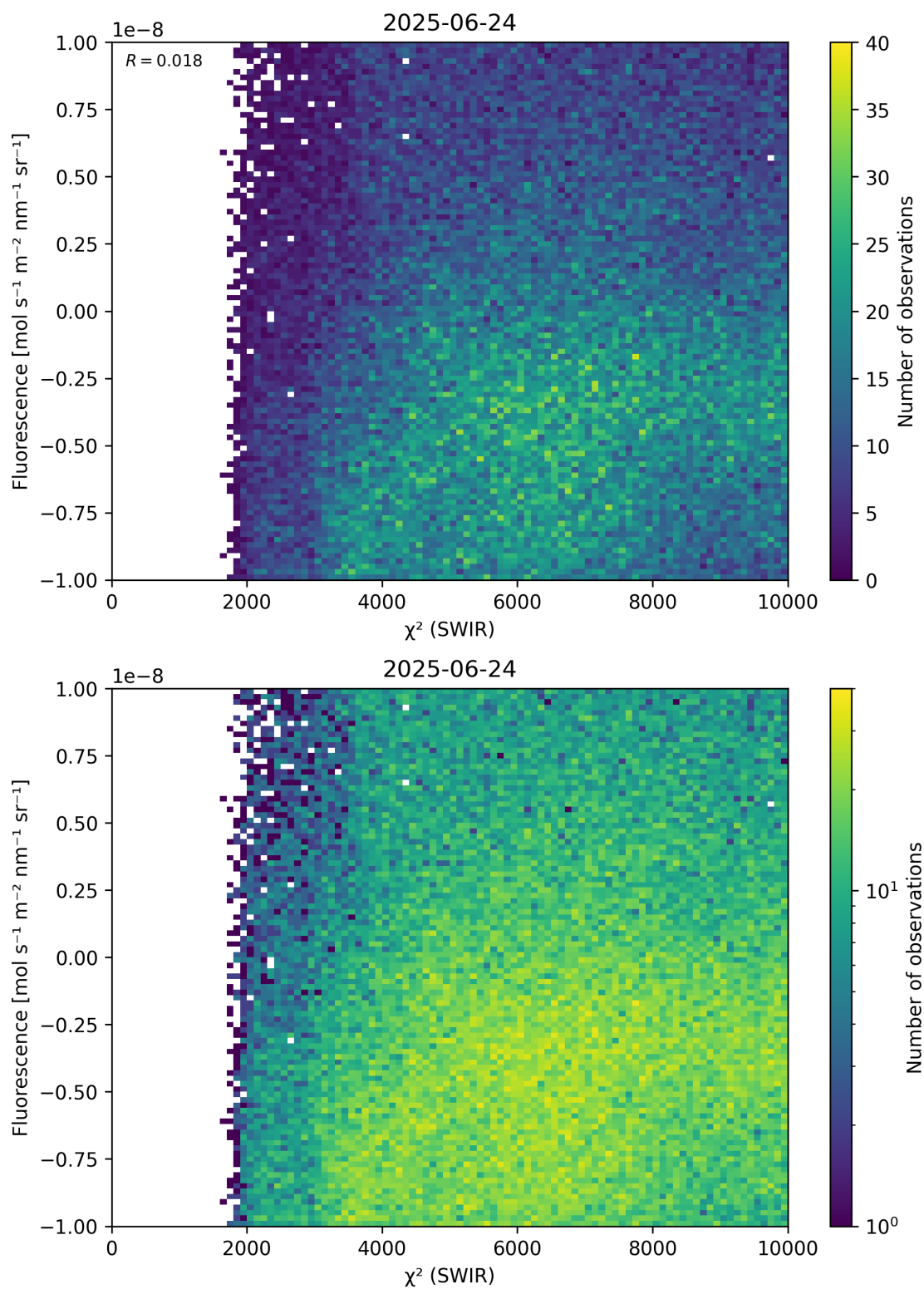
Figure 49: Scatter density plot of “ \chi^2 (SWIR)” against “Fluorescence” for 2025-06-23 to 2025-06-25.
