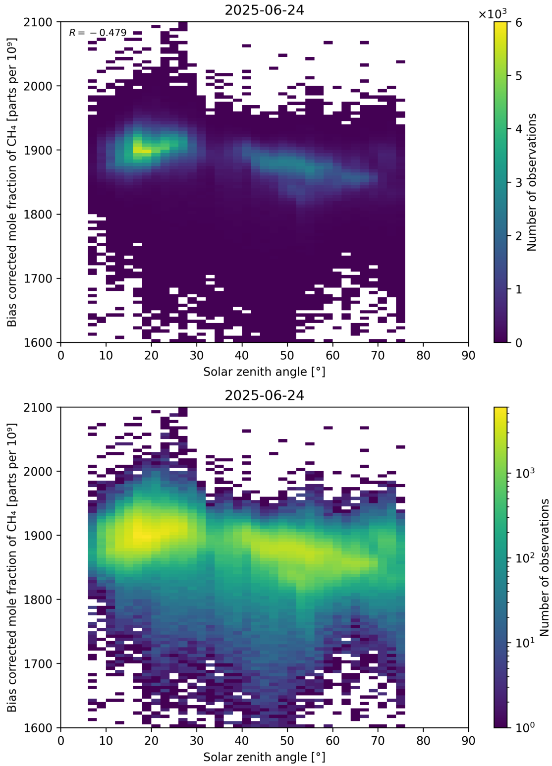
Figure 100: Scatter density plot of “Solar zenith angle” against “Bias corrected mole fraction of CH 4 ” for 2025-06-23 to 2025-06-25.
