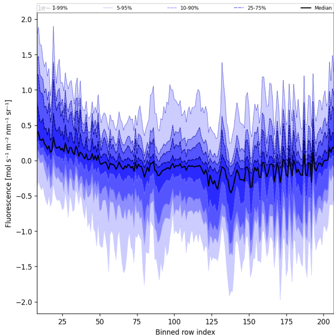
Figure 43: Along track statistics of “Fluorescence” for 2025-06-23 to 2025-06-25
