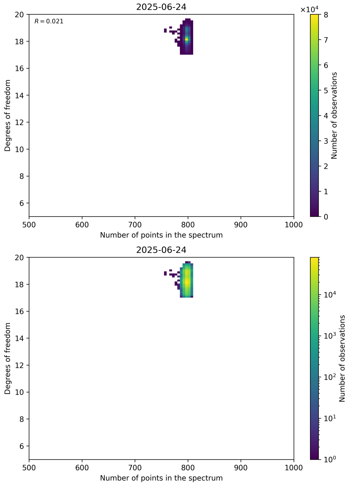
Figure 90: Scatter density plot of “Number of points in the spectrum” against “Degrees of freedom” for 2025-06-23 to 2025-06-25.
