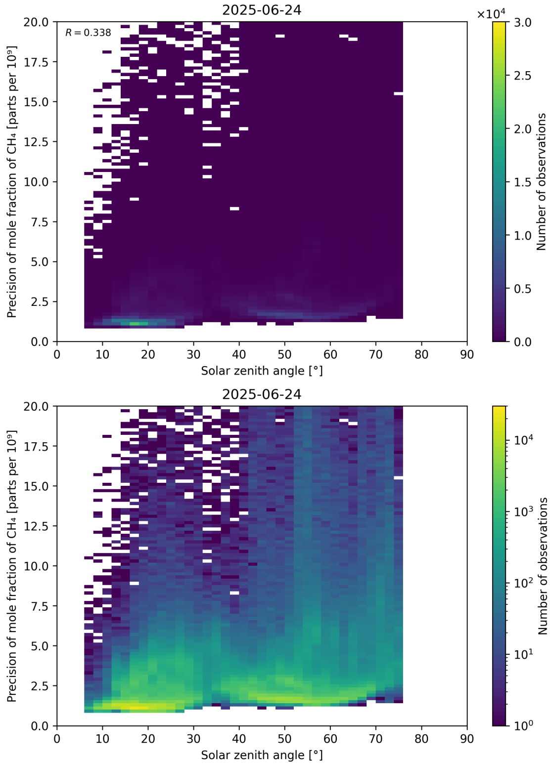
Figure 101: Scatter density plot of “Solar zenith angle” against “Precision of mole fraction of CH 4 ” for 2025-06-23 to 2025-06-25.
