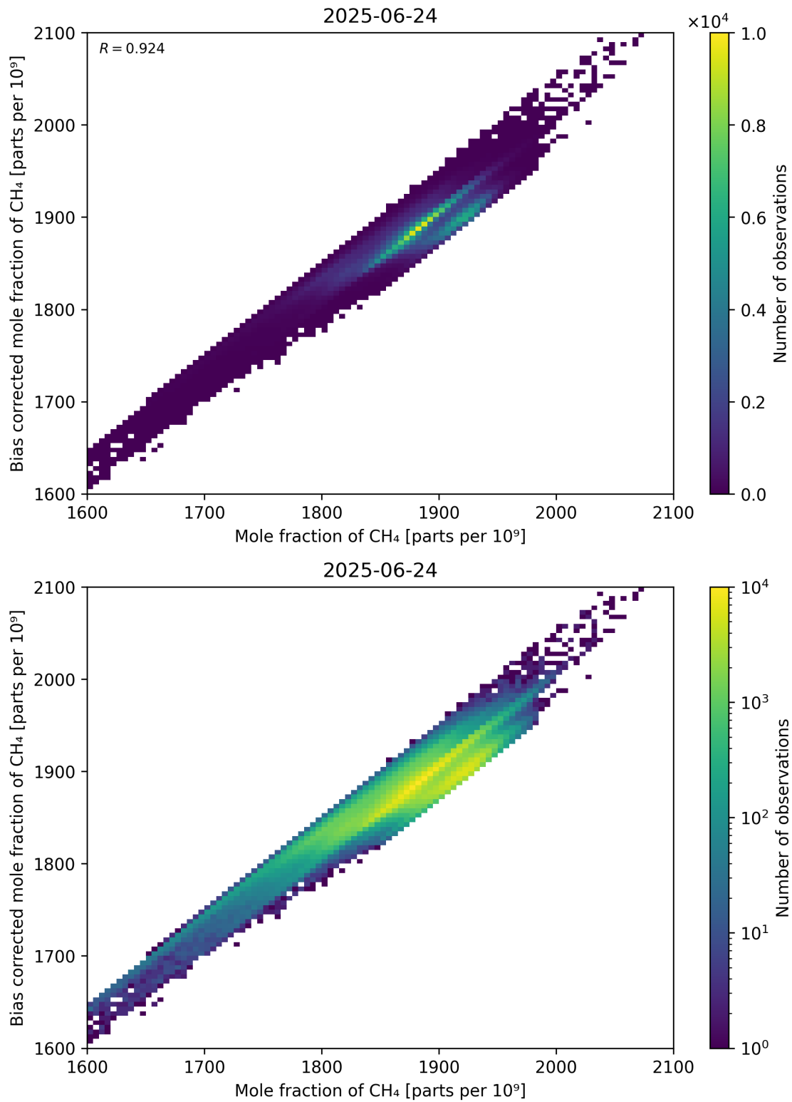
Figure 74: Scatter density plot of “Mole fraction of CH 4 ” against “Bias corrected mole fraction of CH 4 ” for 2025-06-23 to 2025-06-25.
