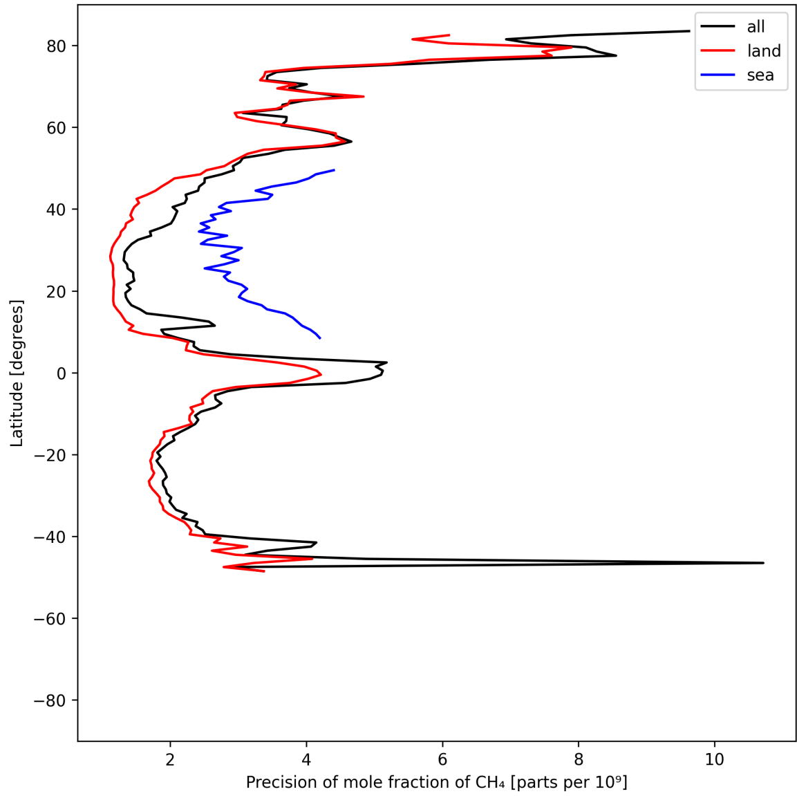
Figure 13: Zonal average of “Precision of mole fraction of CH 4 ” for 2025-06-23 to 2025-06-25.
