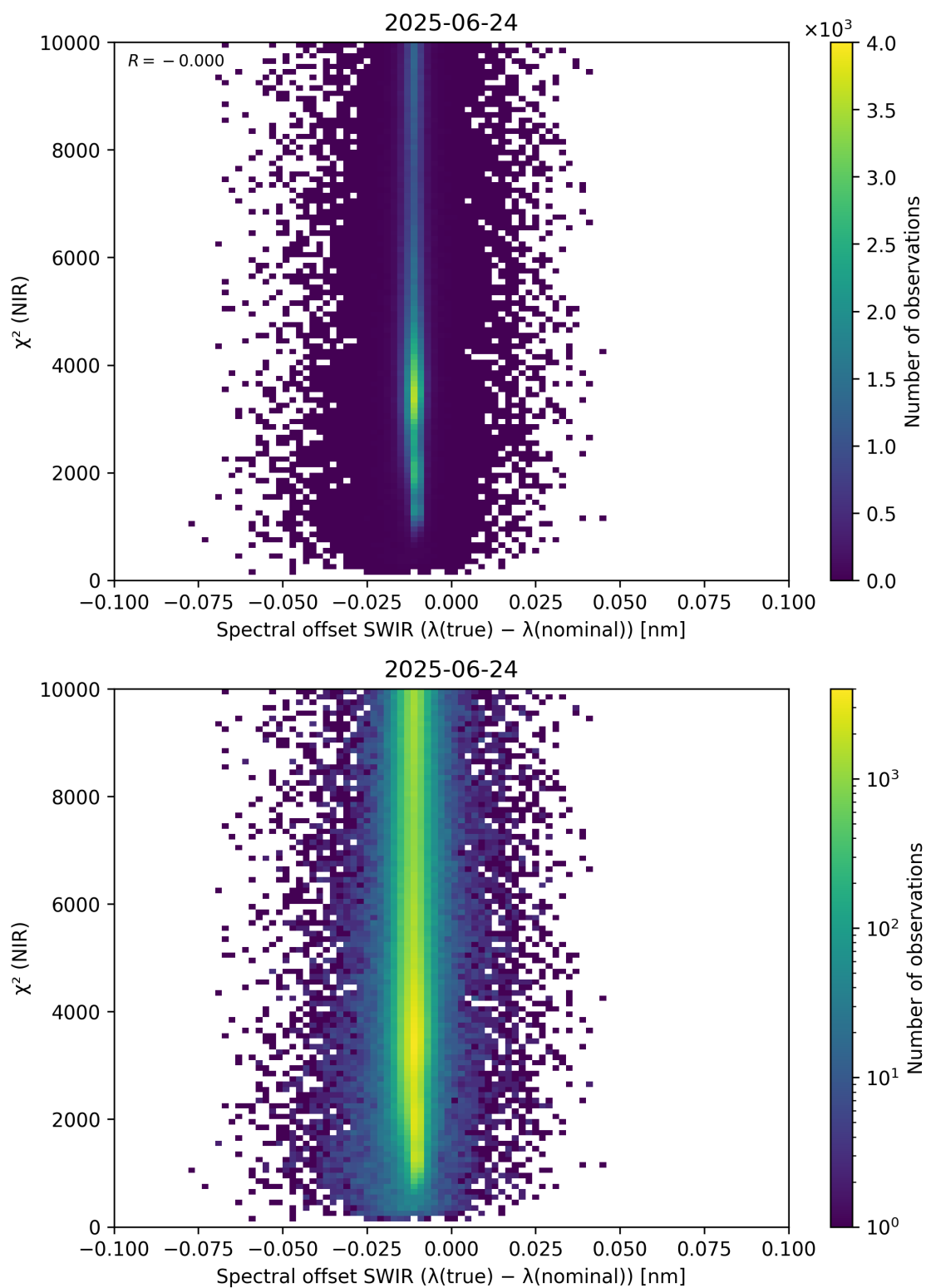
Figure 117: Scatter density plot of “Spectral offset SWIR ( \lambda_{\text{true}} - \lambda_{\text{nominal}} )” against “ \chi^2 (NIR)” for 2025-06-23 to 2025-06-25.
