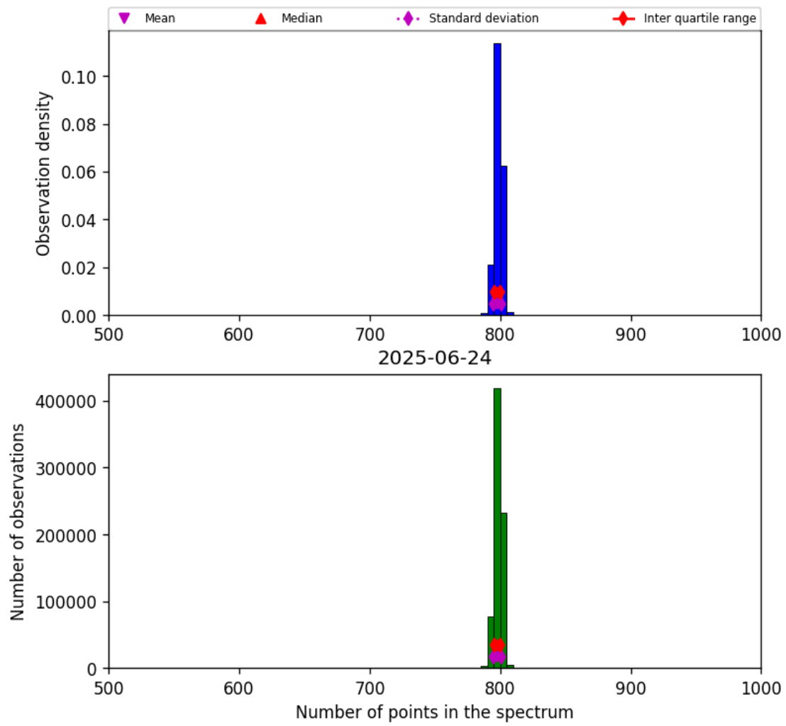
Figure 26: Histogram of “Number of points in the spectrum” for 2025-06-23 to 2025-06-25
