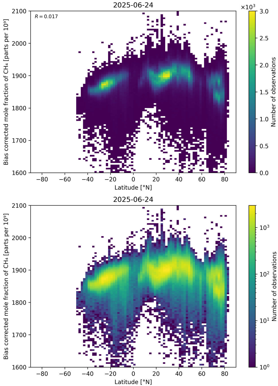
Figure 58: Scatter density plot of “Latitude” against “Bias corrected mole fraction of CH 4 ” for 2025-06-23 to 2025-06-25.
