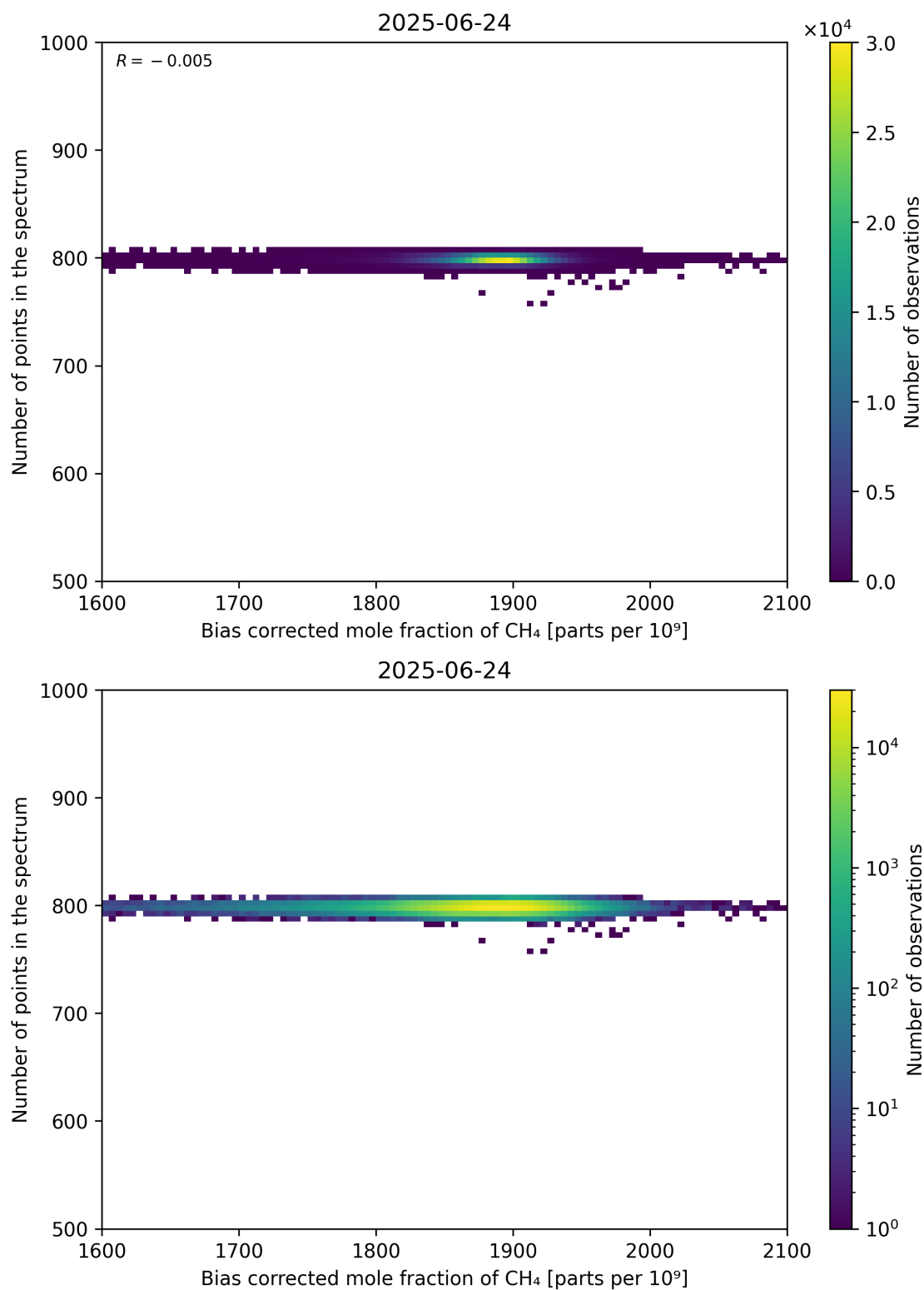
Figure 68: Scatter density plot of “Bias corrected mole fraction of CH 4 ” against “Number of points in the spectrum” for 2025-06-23 to 2025-06-25.
