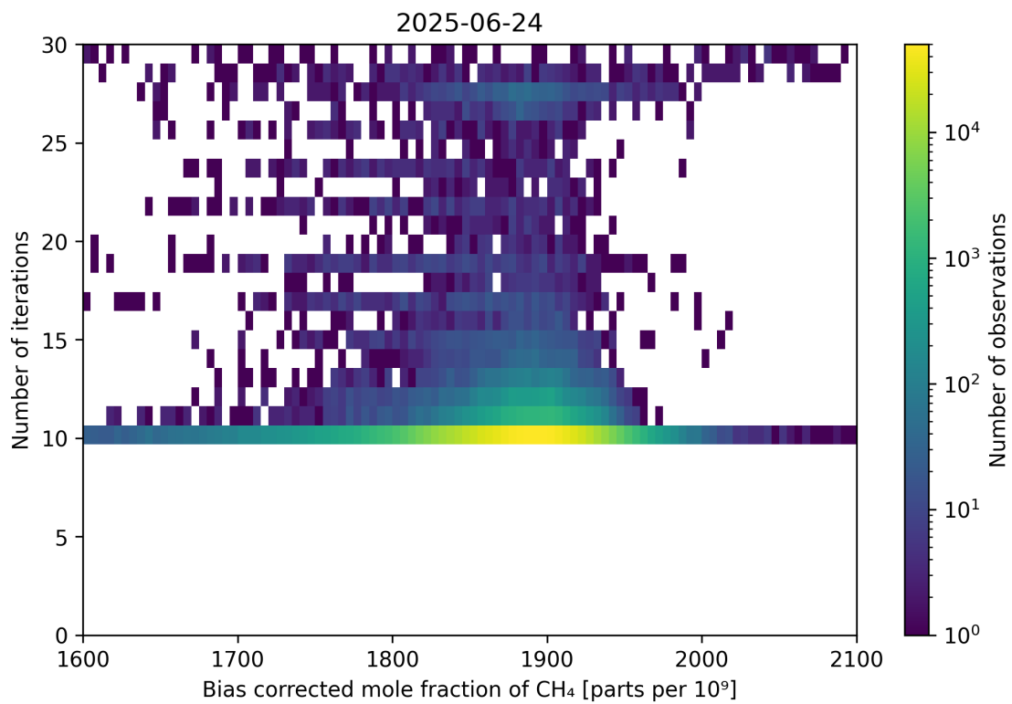
Figure 67: Scatter density plot of “Bias corrected mole fraction of CH 4 ” against “Number of iterations” for 2025-06-23 to 2025-06-25.
