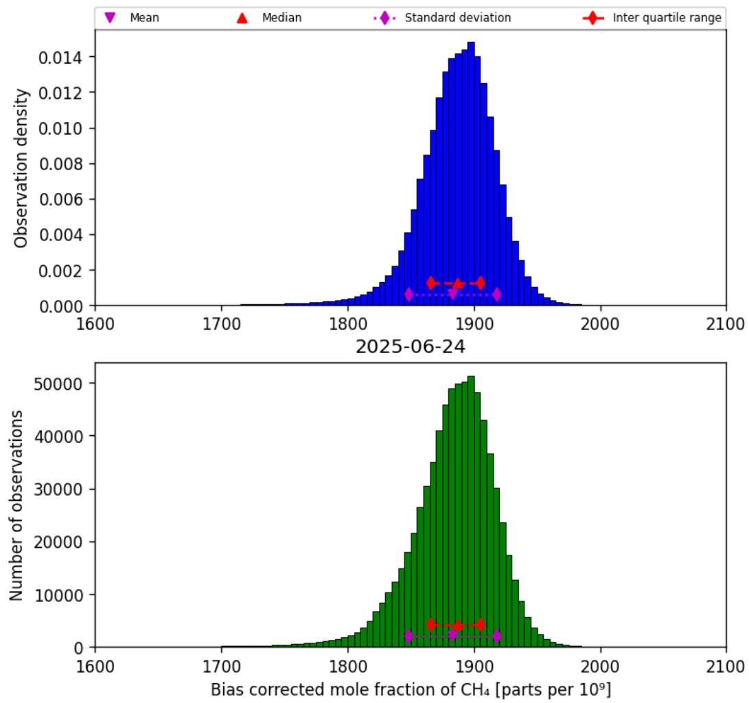
Figure 25: Histogram of “Bias corrected mole fraction of CH 4 ” for 2025-06-23 to 2025-06-25
