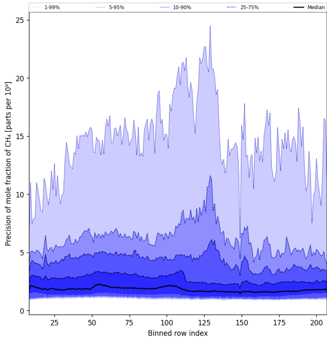
Figure 35: Along track statistics of “Precision of mole fraction of CH 4 ” for 2025-06-23 to 2025-06-25
