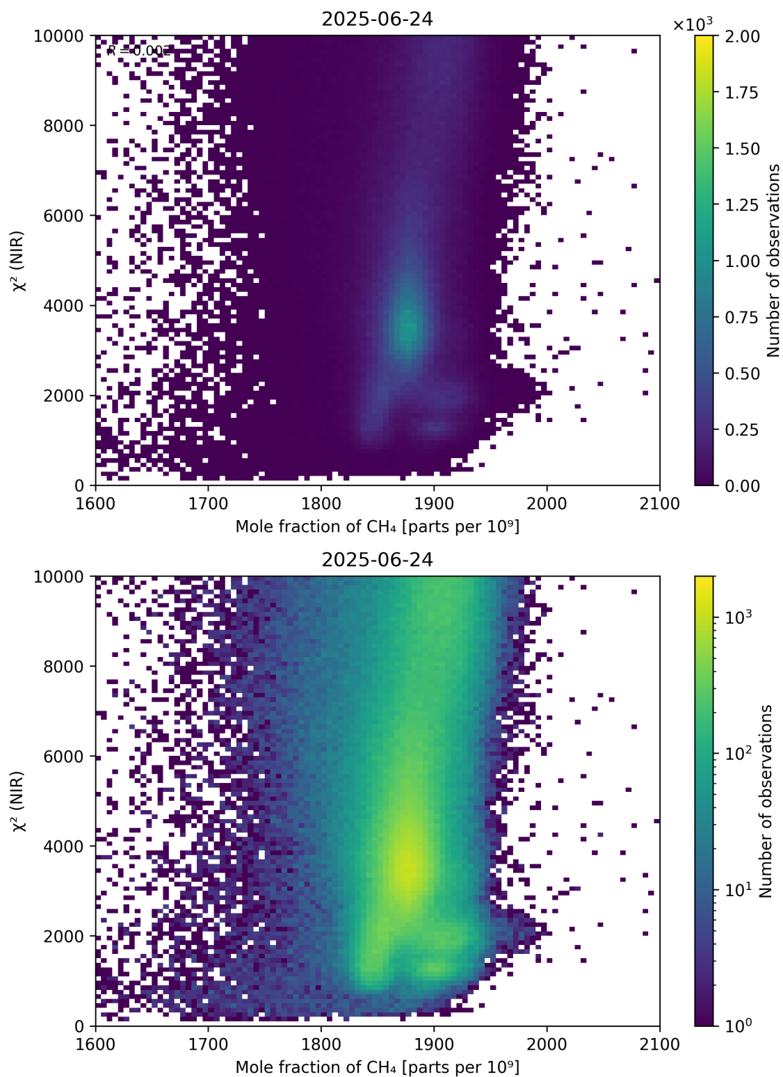
Figure 70: Scatter density plot of “Mole fraction of \text{CH}_4 ” against “ \chi^2 (NIR)” for 2025-06-23 to 2025-06-25.
