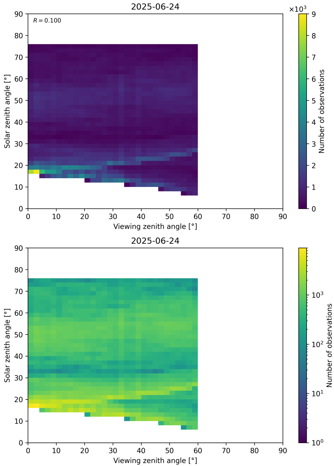
Figure 115: Scatter density plot of “Viewing zenith angle” against “Solar zenith angle” for 2025-06-23 to 2025-06-25.
