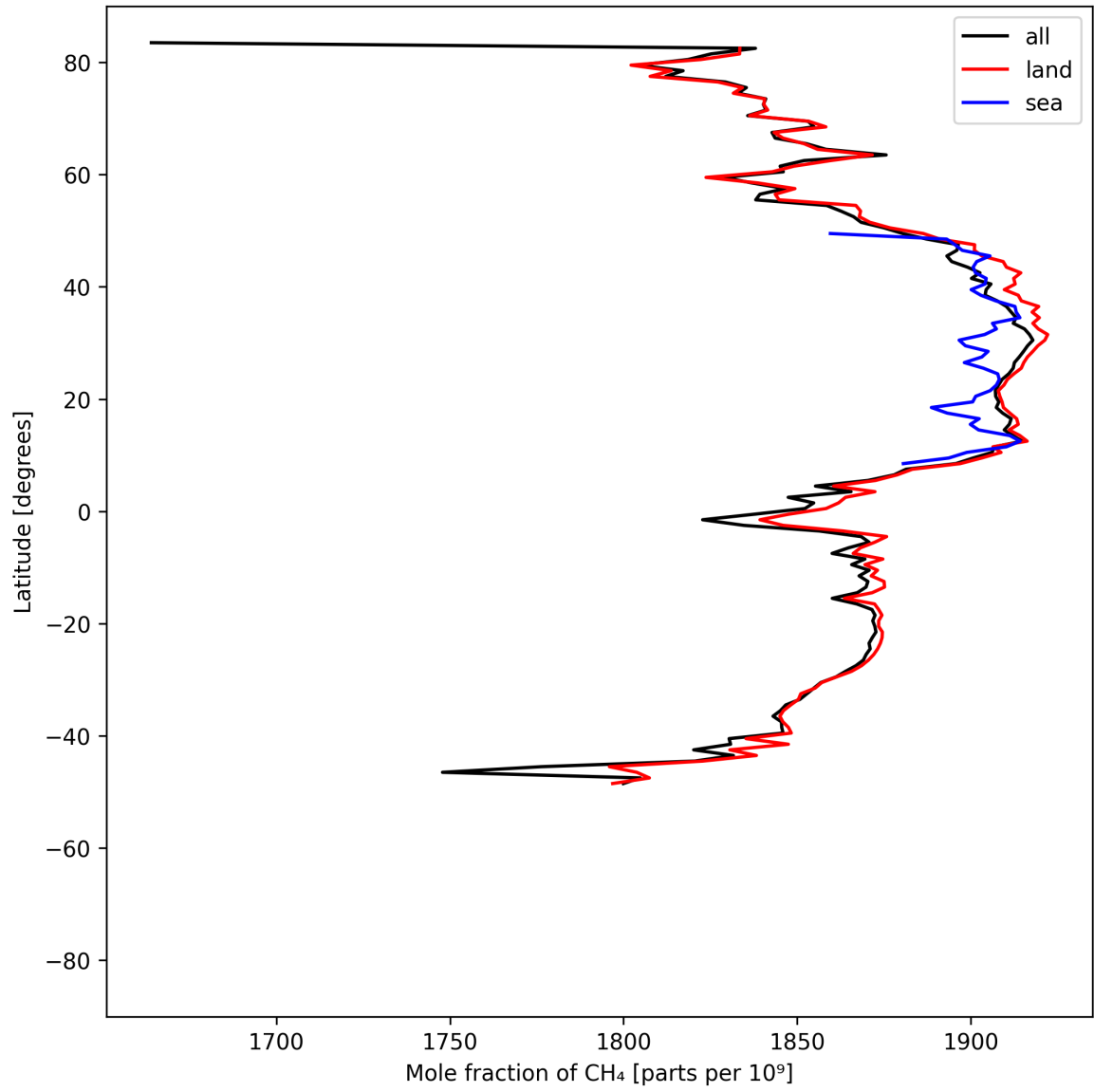
Figure 12: Zonal average of “Mole fraction of CH 4 ” for 2025-06-23 to 2025-06-25.
