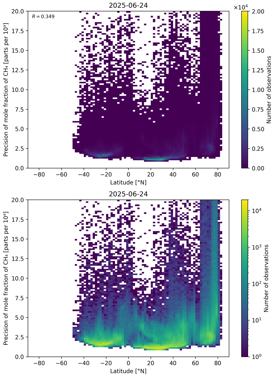
Figure 59: Scatter density plot of “Latitude” against “Precision of mole fraction of \text{CH}_4 ” for 2025-06-23 to 2025-06-25.
