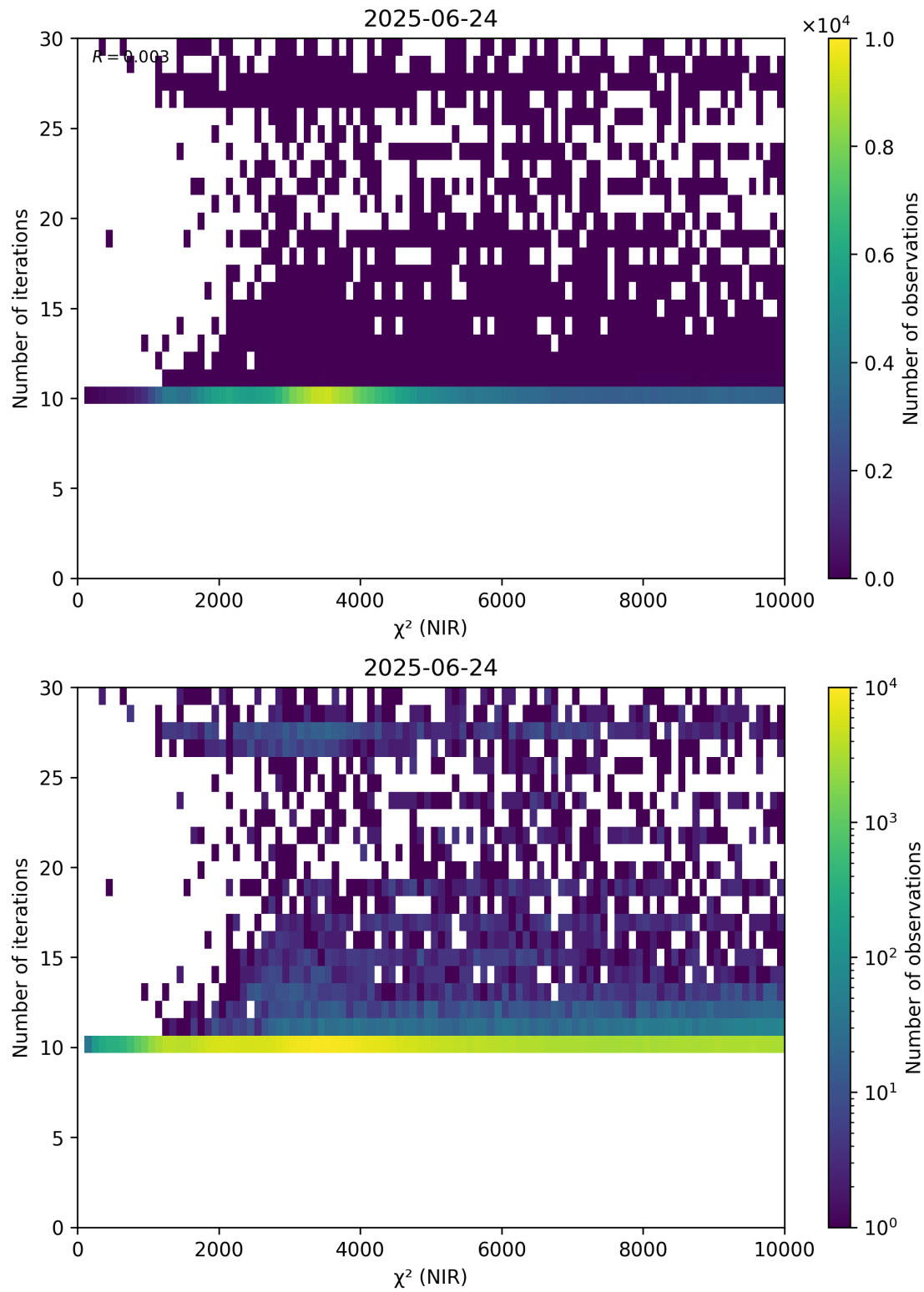
Figure 46: Scatter density plot of “ \chi^2 (NIR)” against “Number of iterations” for 2025-06-23 to 2025-06-25.
