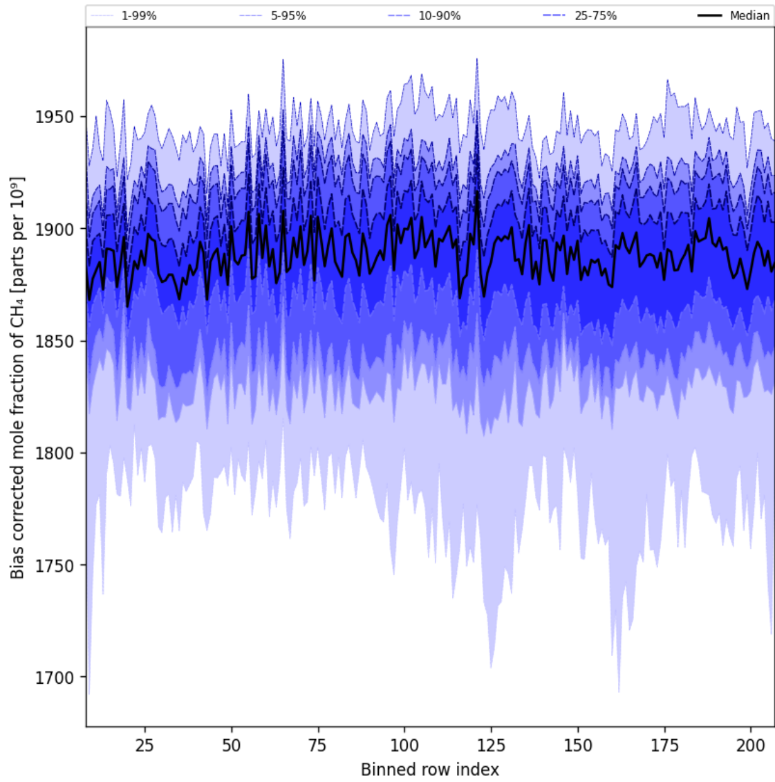
Figure 36: Along track statistics of “Bias corrected mole fraction of CH 4 ” for 2025-06-23 to 2025-06-25
