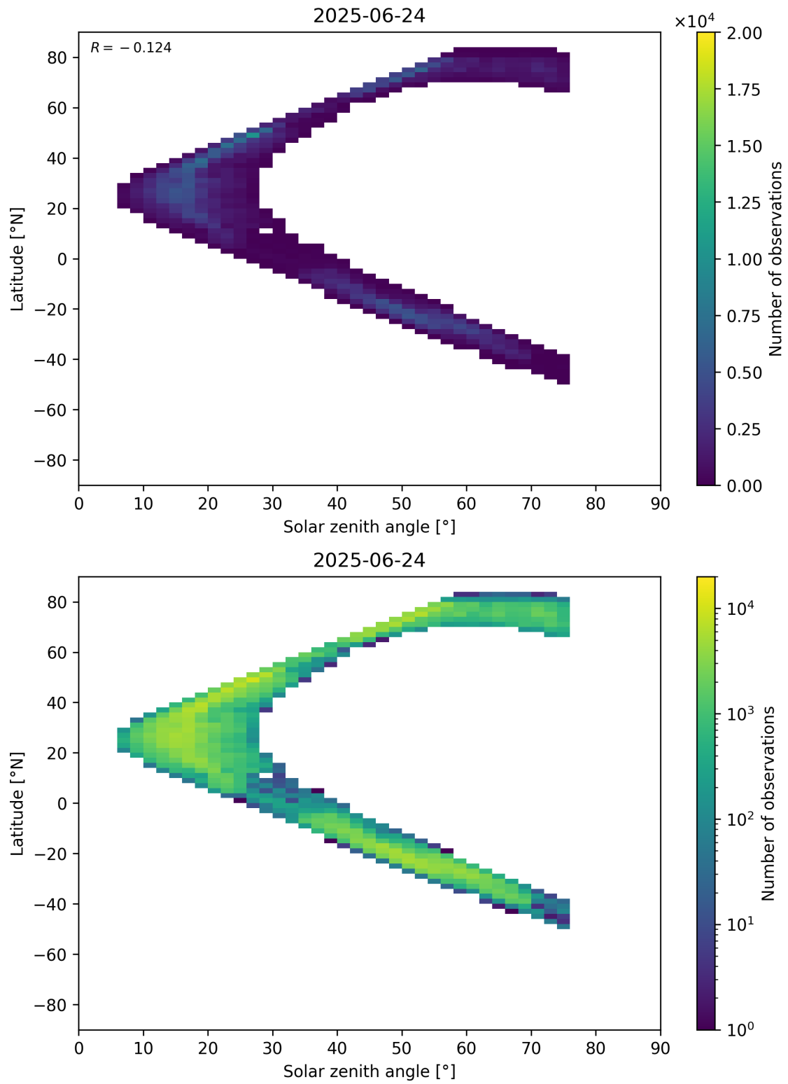
Figure 98: Scatter density plot of “Solar zenith angle” against “Latitude” for 2025-06-23 to 2025-06-25.
