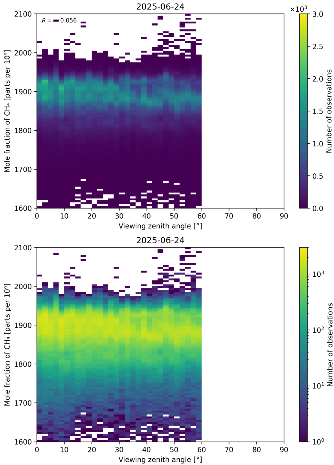
Figure 110: Scatter density plot of “Viewing zenith angle” against “Mole fraction of CH 4 ” for 2025-06-23 to 2025-06-25.
