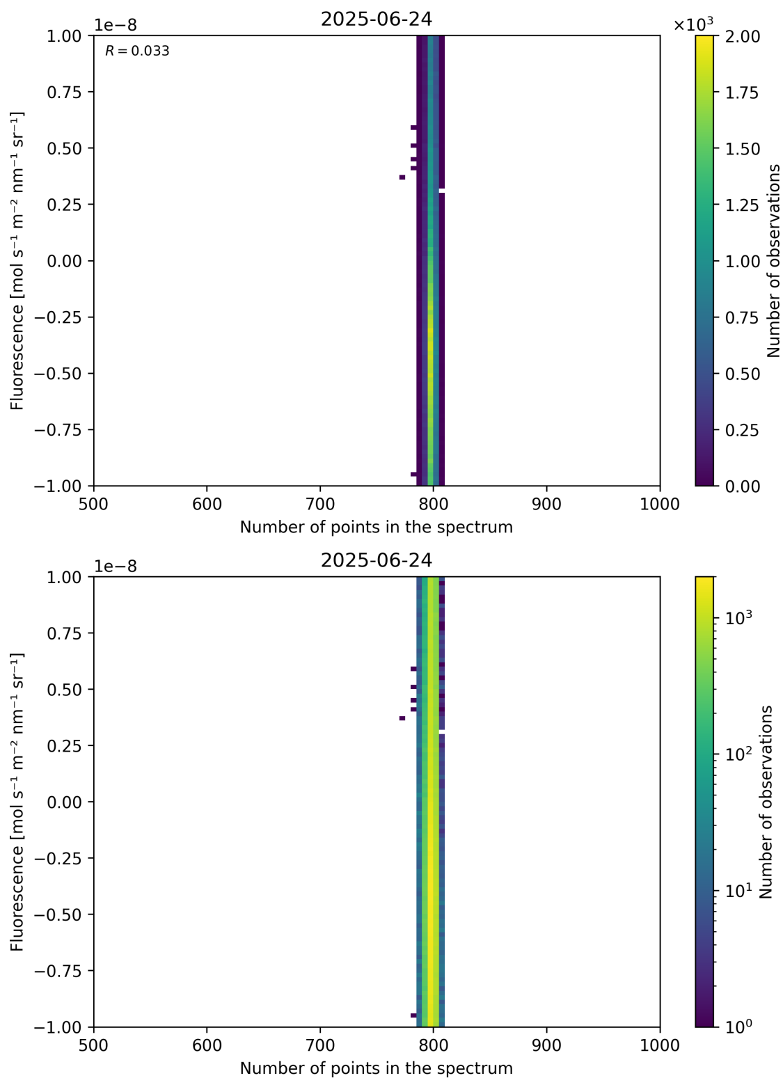
Figure 91: Scatter density plot of “Number of points in the spectrum” against “Fluorescence” for 2025-06-23 to 2025-06-25.
