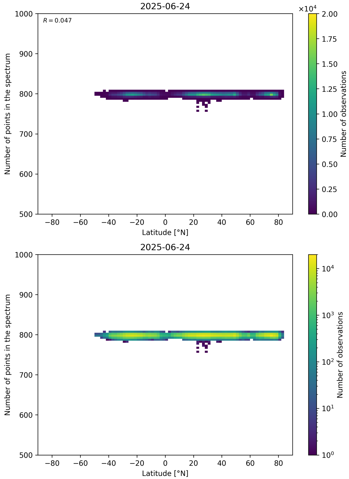
Figure 61: Scatter density plot of “Latitude” against “Number of points in the spectrum” for 2025-06-23 to 2025-06-25.
