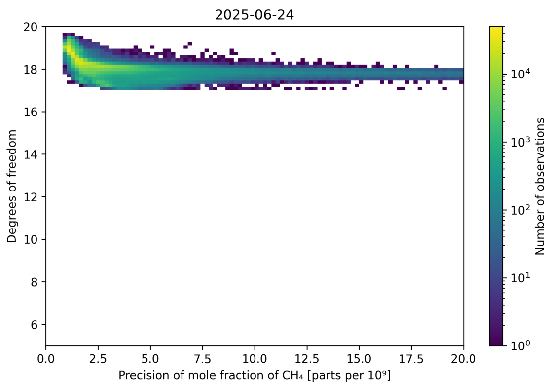
Figure 80: Scatter density plot of “Precision of mole fraction of CH 4 ” against “Degrees of freedom” for 2025-06-23 to 2025-06-25.
