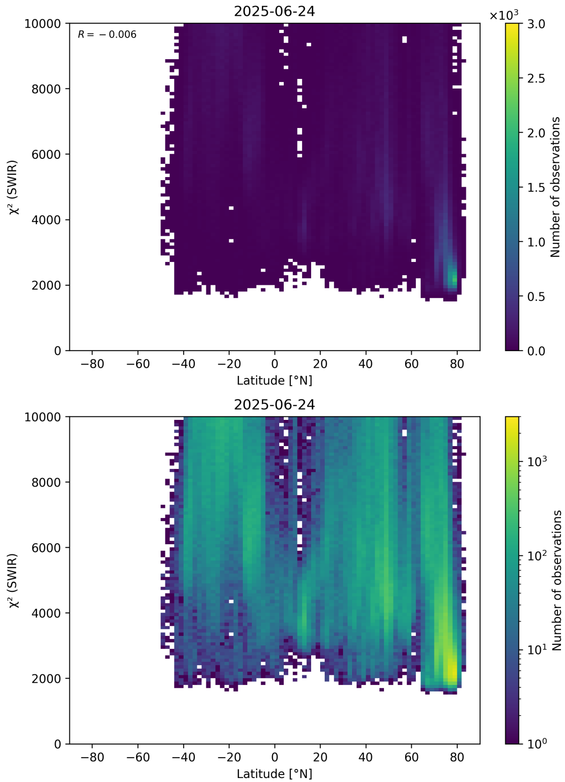
Figure 54: Scatter density plot of “Latitude” against “ \chi^2 (SWIR)” for 2025-06-23 to 2025-06-25.
