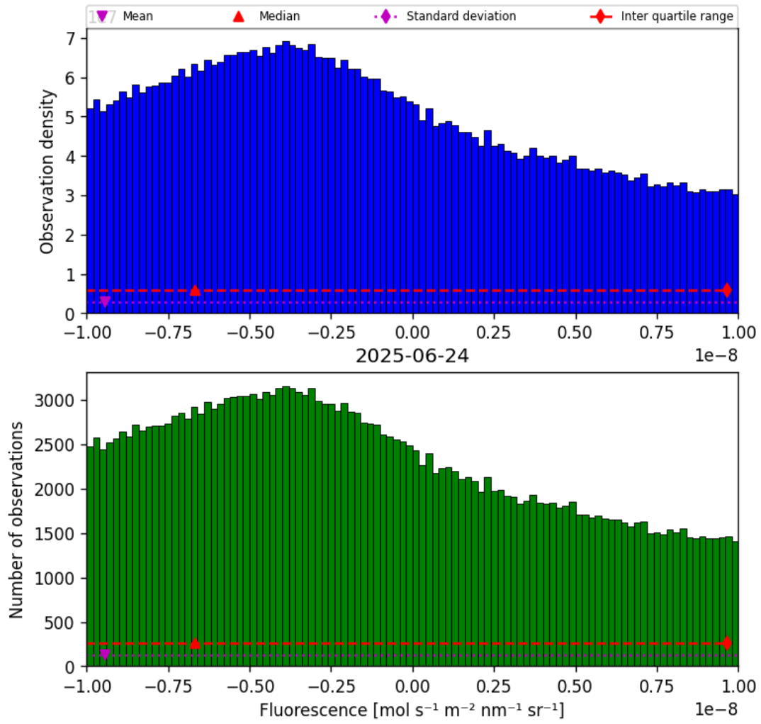
Figure 32: Histogram of “Fluorescence” for 2025-06-23 to 2025-06-25
