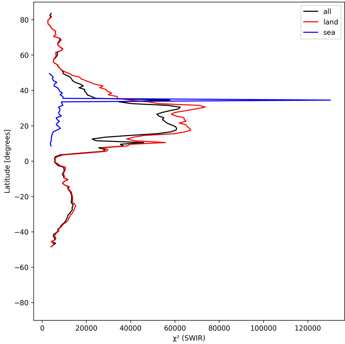
Figure 17: Zonal average of “ \chi^2 (SWIR)” for 2025-06-23 to 2025-06-25.
