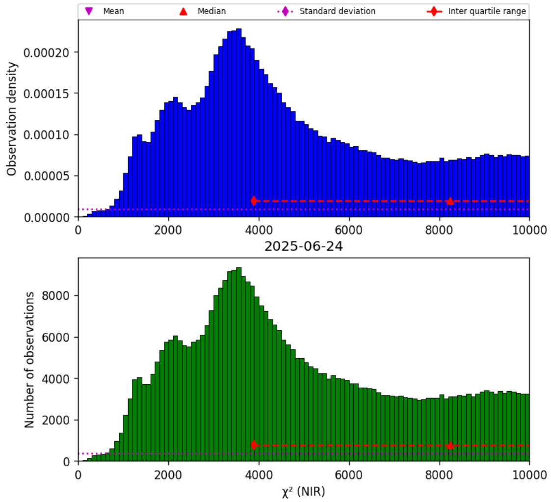
Figure 29: Histogram of " \chi^2 (NIR)" for 2025-06-23 to 2025-06-25
