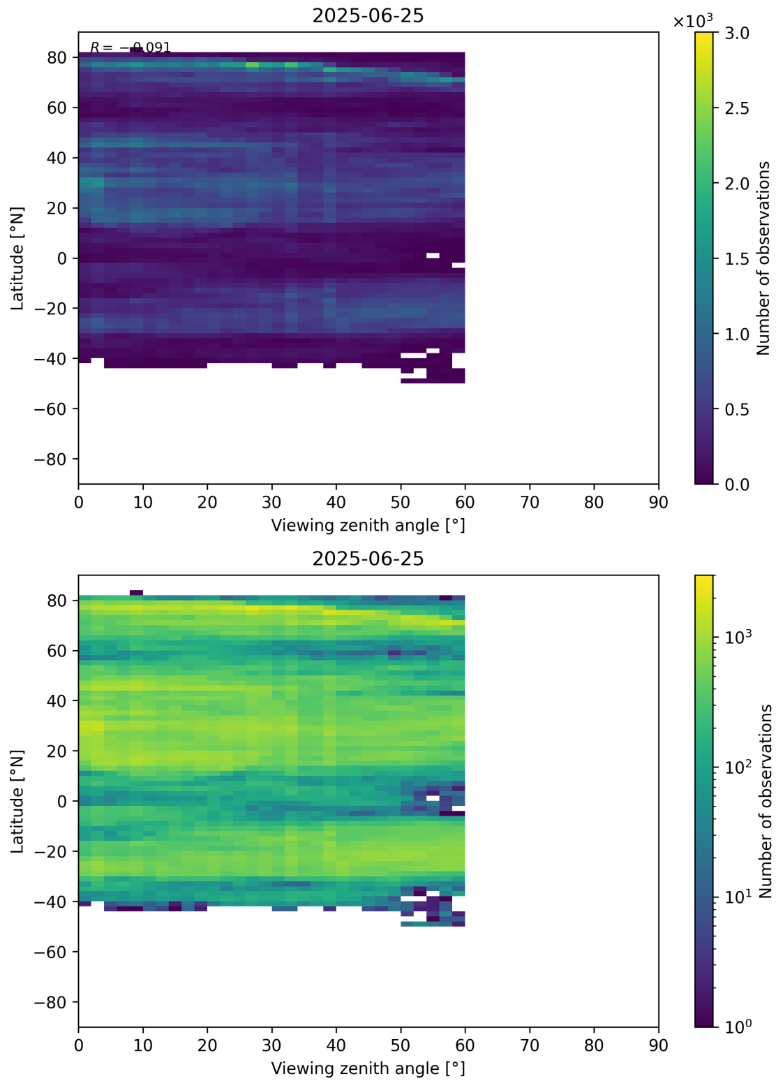
Figure 109: Scatter density plot of “Viewing zenith angle” against “Latitude” for 2025-06-24 to 2025-06-26.
