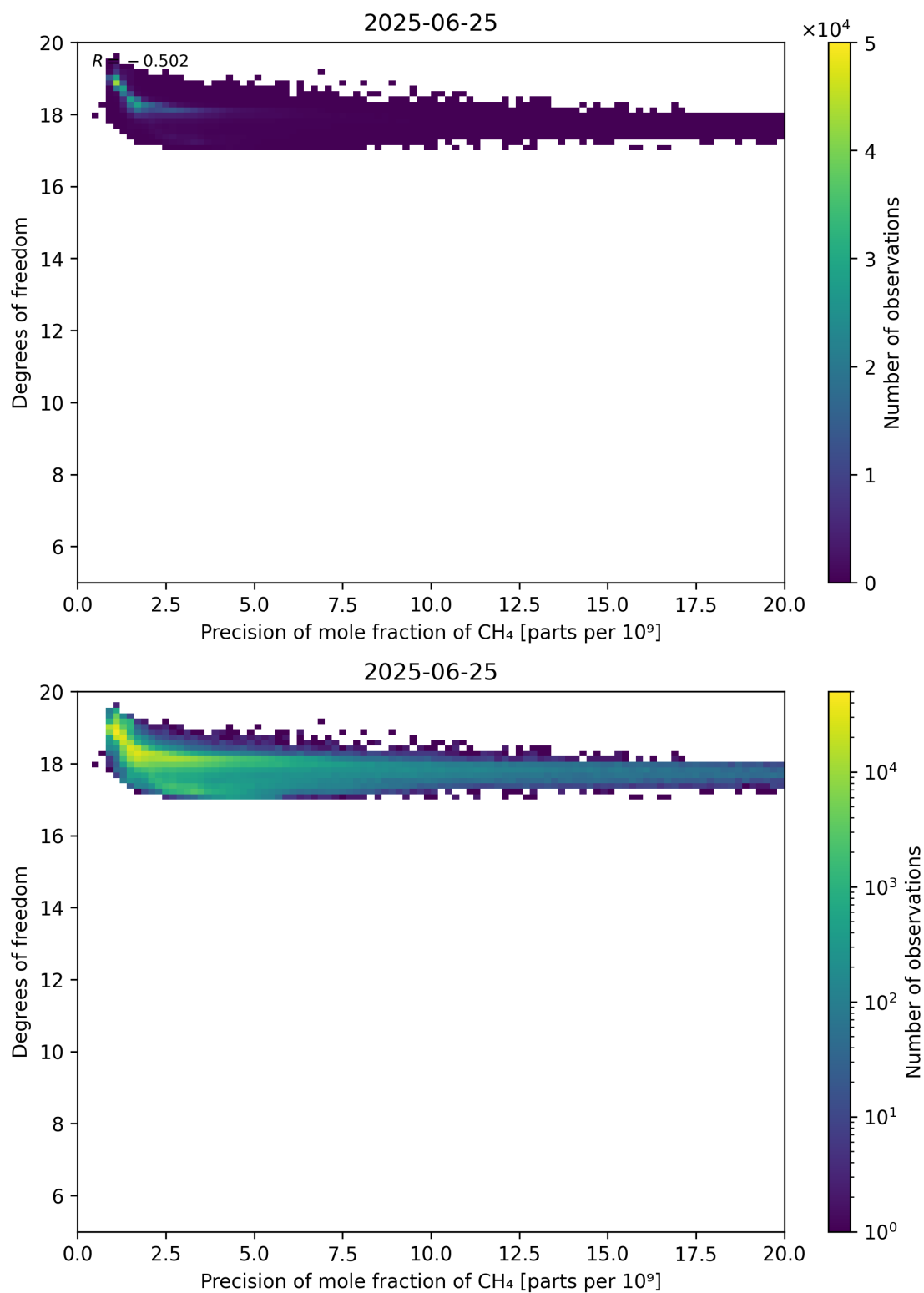
Figure 80: Scatter density plot of “Precision of mole fraction of CH 4 ” against “Degrees of freedom” for 2025-06-24 to 2025-06-26.
