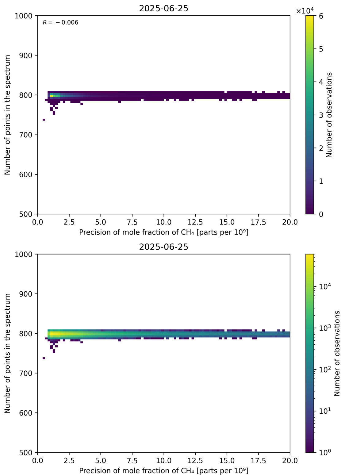
Figure 84: Scatter density plot of “Precision of mole fraction of CH 4 ” against “Number of points in the spectrum” for 2025-06-24 to 2025-06-26.
