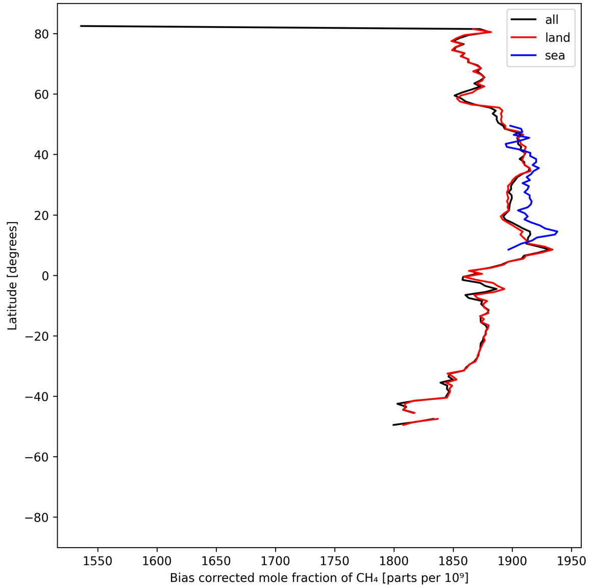
Figure 14: Zonal average of “Bias corrected mole fraction of CH 4 ” for 2025-06-24 to 2025-06-26.
