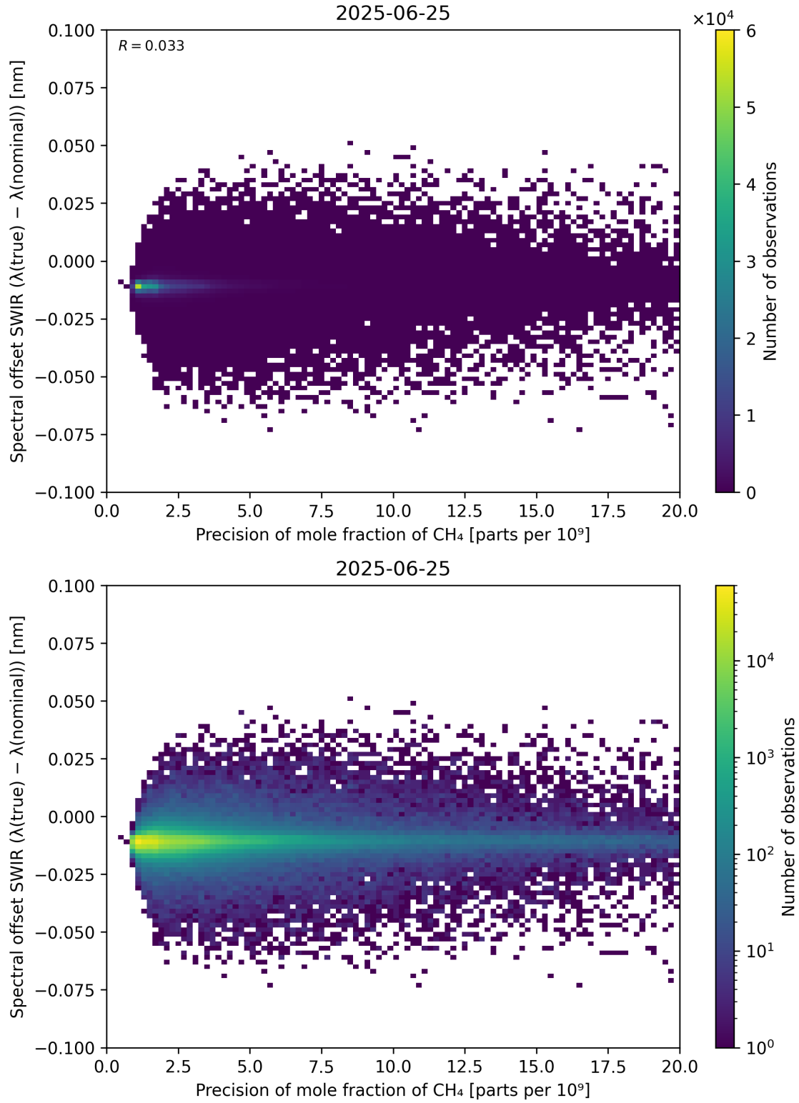
Figure 85: Scatter density plot of “Precision of mole fraction of CH 4 ” against “Spectral offset SWIR ( \lambda_{\text{true}} - \lambda_{\text{nominal}} )” for 2025-06-24 to 2025-06-26.
