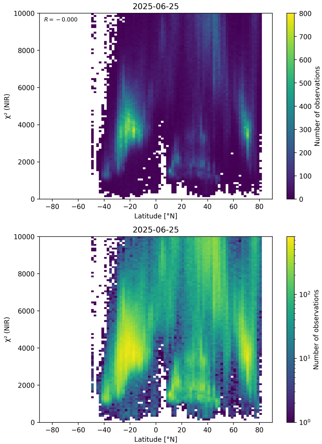
Figure 53: Scatter density plot of “Latitude” against “ \chi^2 (NIR)” for 2025-06-24 to 2025-06-26.
