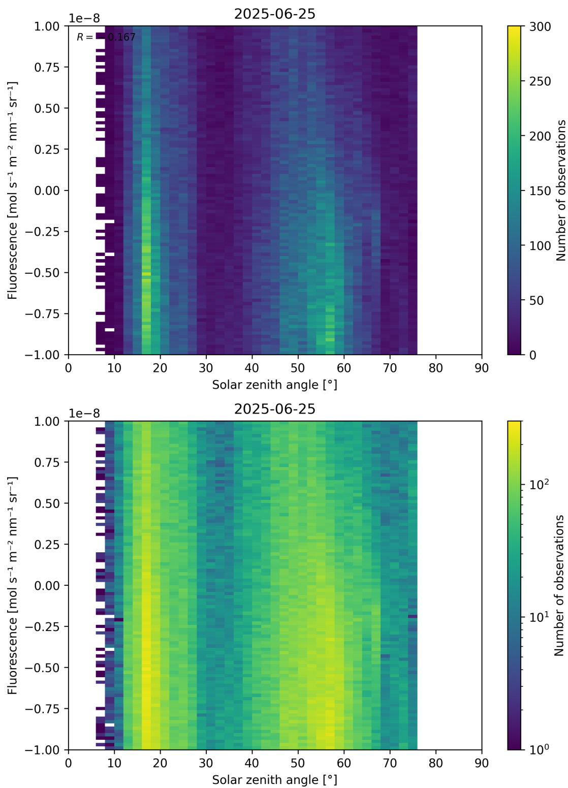
Figure 97: Scatter density plot of “Solar zenith angle” against “Fluorescence” for 2025-06-24 to 2025-06-26.
