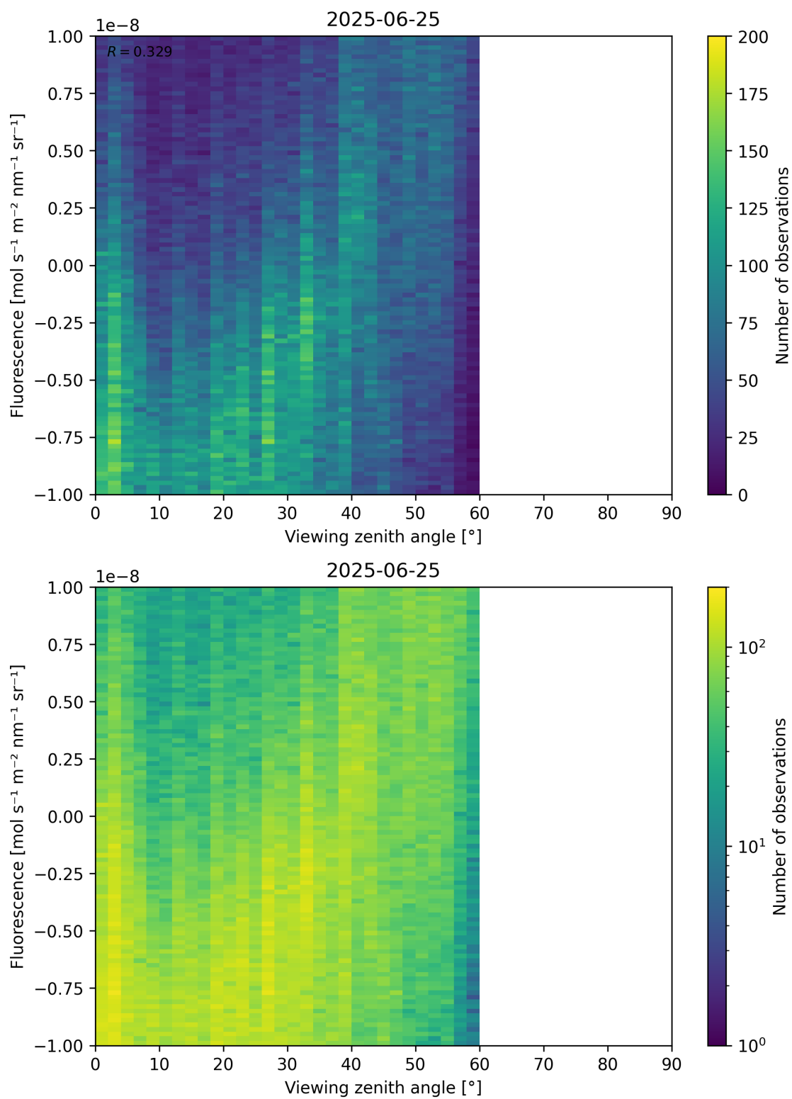
Figure 108: Scatter density plot of “Viewing zenith angle” against “Fluorescence” for 2025-06-24 to 2025-06-26.
