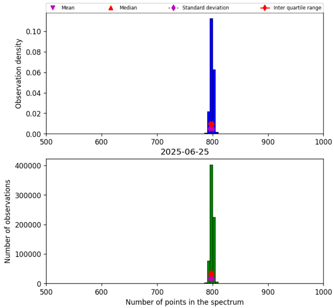
Figure 26: Histogram of “Number of points in the spectrum” for 2025-06-24 to 2025-06-26
