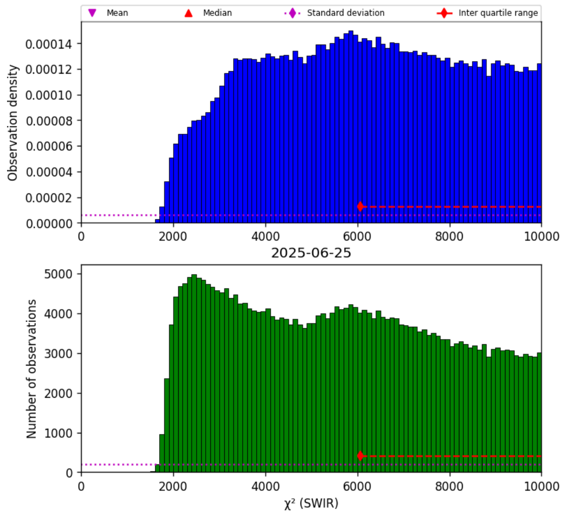
Figure 28: Histogram of “ \chi^2 (SWIR)” for 2025-06-24 to 2025-06-26
