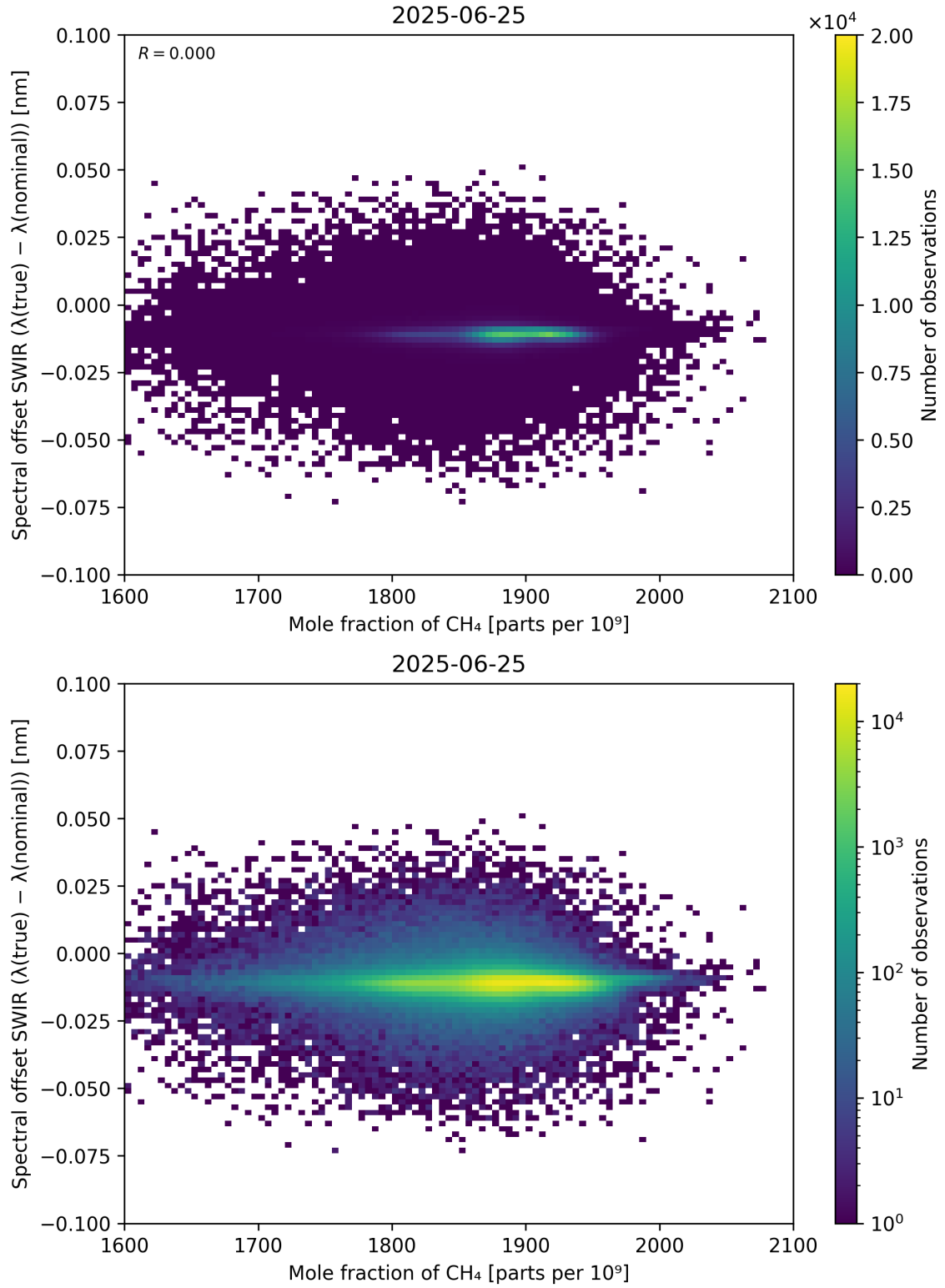
Figure 86: Scatter density plot of “Mole fraction of CH 4 ” against “Spectral offset SWIR ( \lambda_{\text{true}} - \lambda_{\text{nominal}} )” for 2025-06-24 to 2025-06-26.
