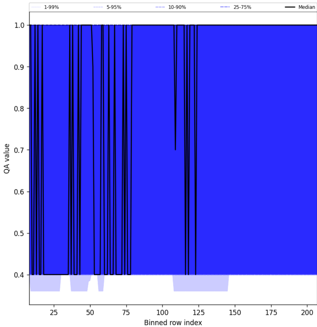
Figure 33: Along track statistics of “QA value” for 2025-06-24 to 2025-06-26
