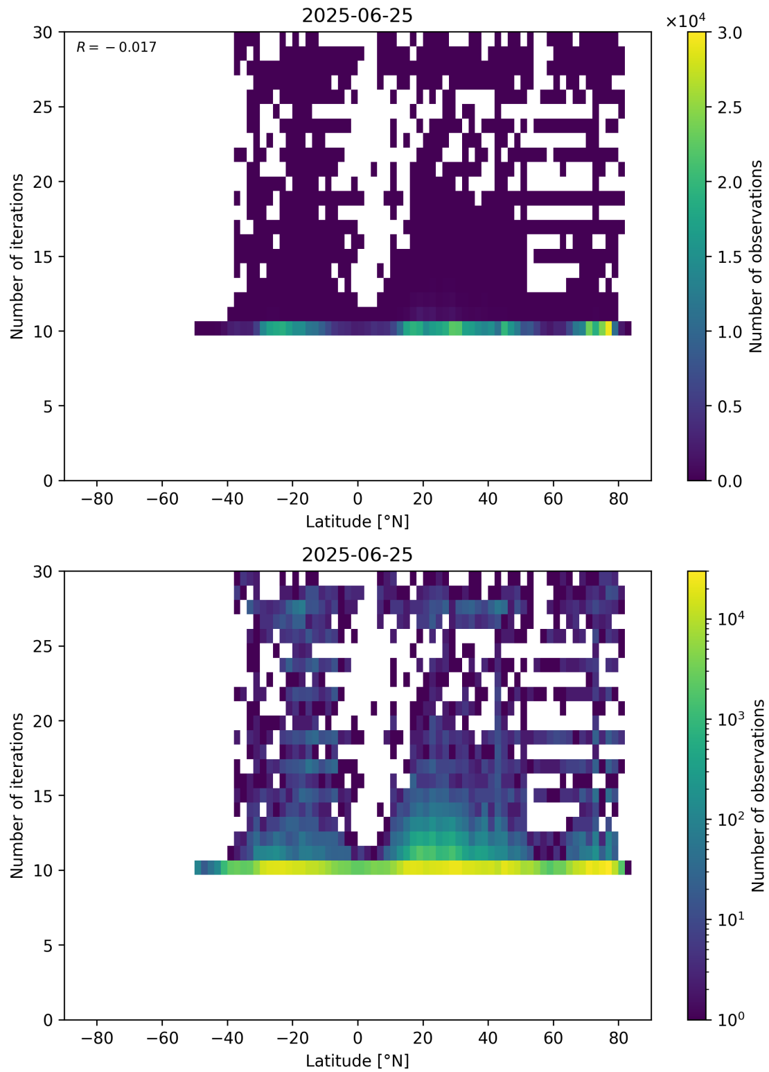
Figure 60: Scatter density plot of “Latitude” against “Number of iterations” for 2025-06-24 to 2025-06-26.
