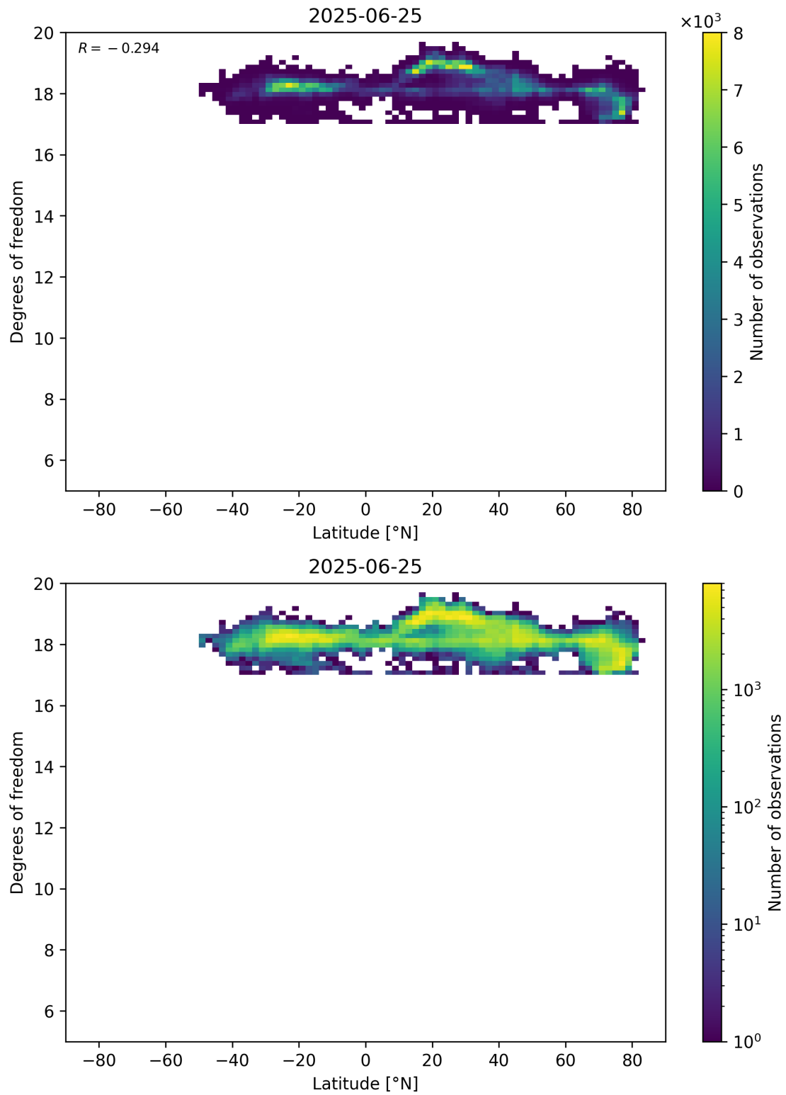
Figure 55: Scatter density plot of “Latitude” against “Degrees of freedom” for 2025-06-24 to 2025-06-26.
