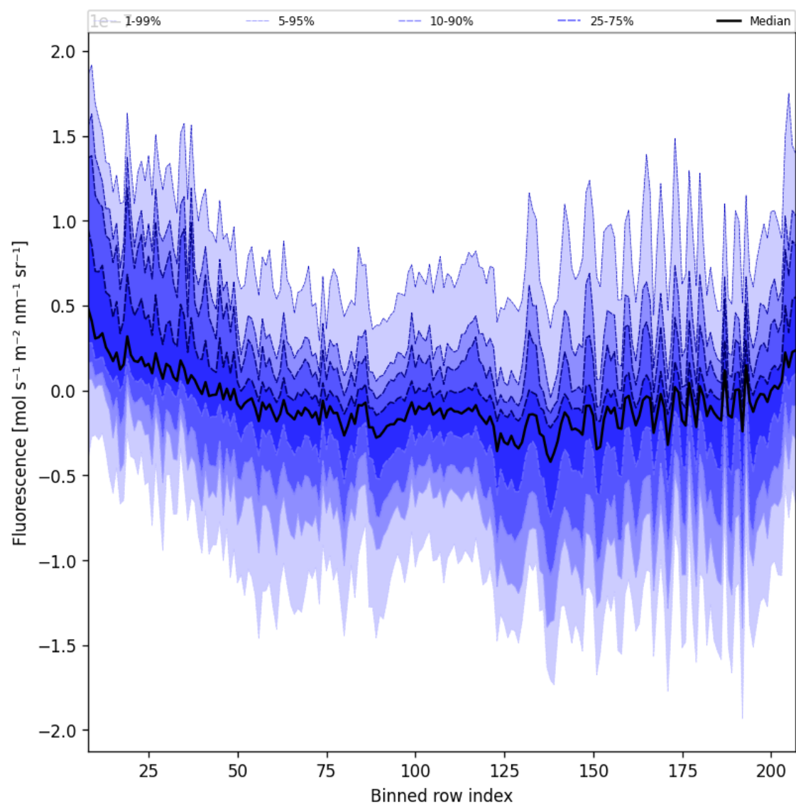
Figure 43: Along track statistics of “Fluorescence” for 2025-06-24 to 2025-06-26
