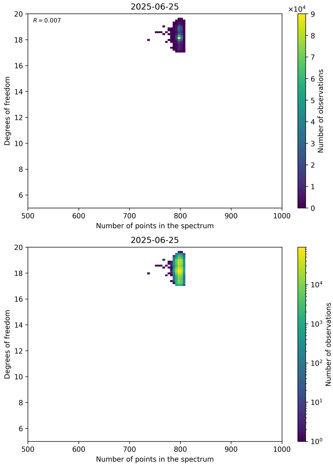
Figure 90: Scatter density plot of “Number of points in the spectrum” against “Degrees of freedom” for 2025-06-24 to 2025-06-26.
