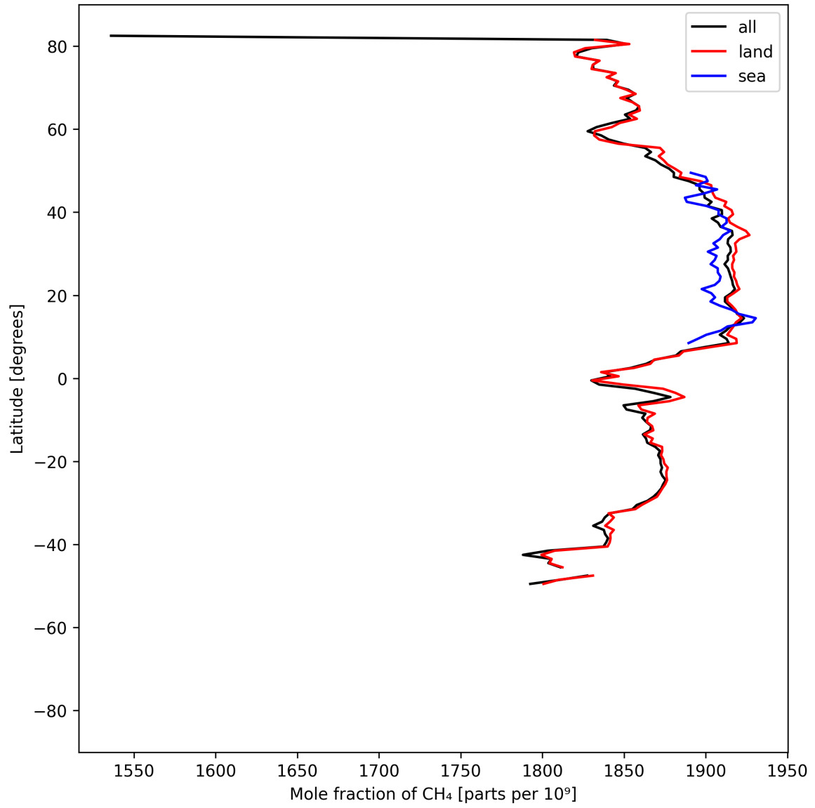
Figure 12: Zonal average of “Mole fraction of \text{CH}_4 ” for 2025-06-24 to 2025-06-26.
