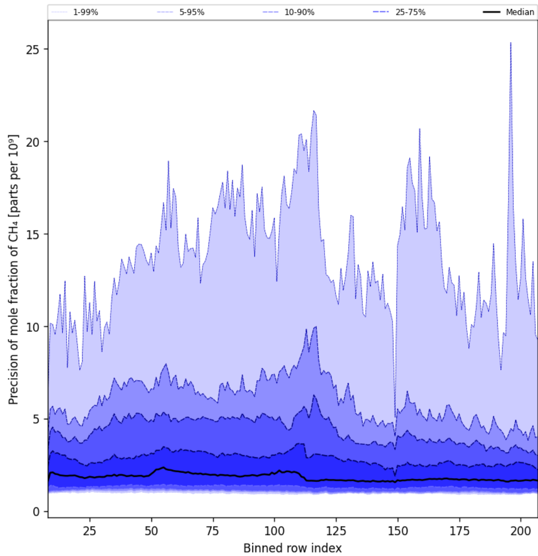
Figure 35: Along track statistics of “Precision of mole fraction of CH 4 ” for 2025-06-24 to 2025-06-26
