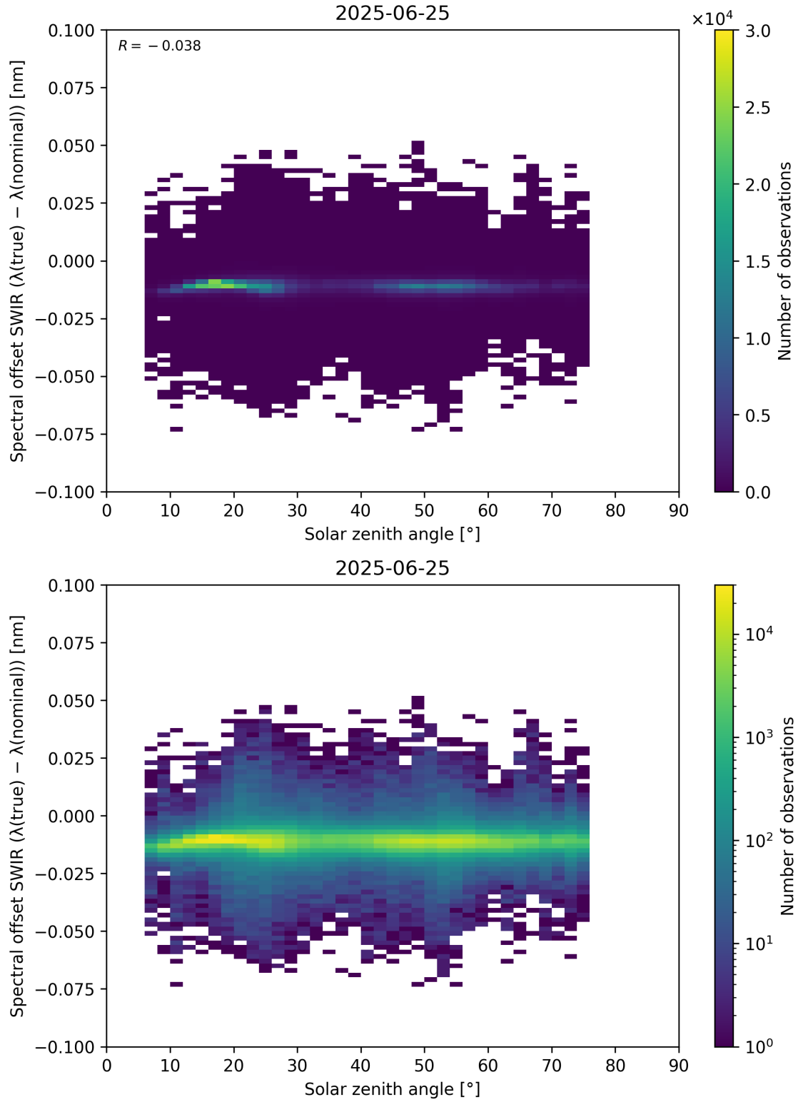
Figure 104: Scatter density plot of “Solar zenith angle” against “Spectral offset SWIR ( \lambda_{\text{true}} - \lambda_{\text{nominal}} )” for 2025-06-24 to 2025-06-26.
