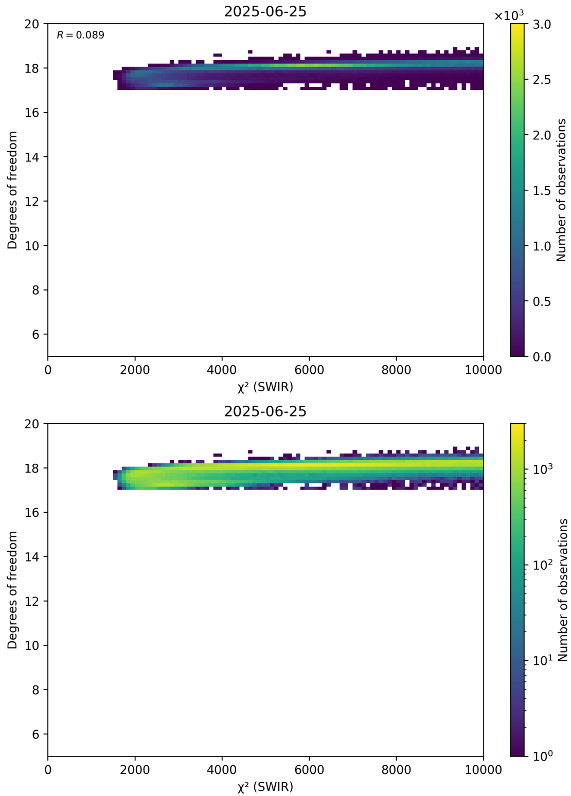
Figure 48: Scatter density plot of “ \chi^2 (SWIR)” against “Degrees of freedom” for 2025-06-24 to 2025-06-26.
