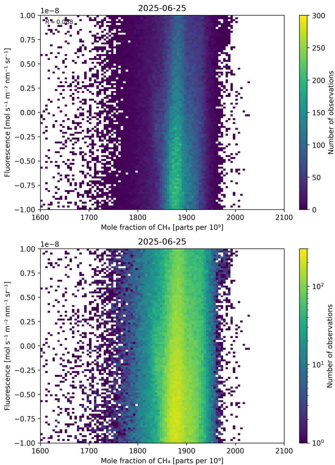
Figure 73: Scatter density plot of “Mole fraction of \text{CH}_4 ” against “Fluorescence” for 2025-06-24 to 2025-06-26.
