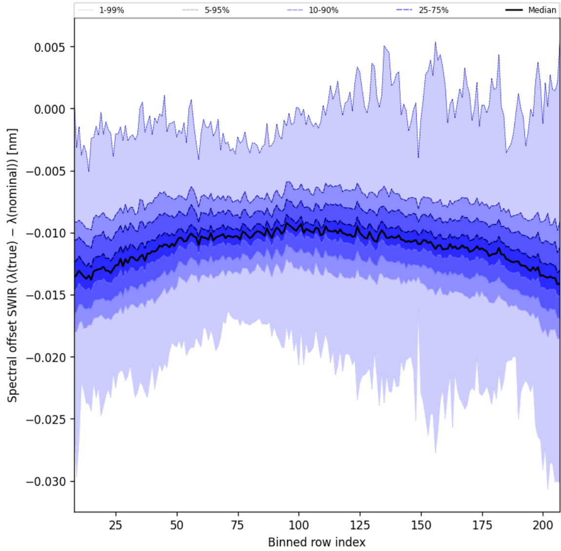
Figure 38: Along track statistics of “Spectral offset SWIR ( \lambda_{\text{true}} - \lambda_{\text{nominal}} )” for 2025-06-24 to 2025-06-26
