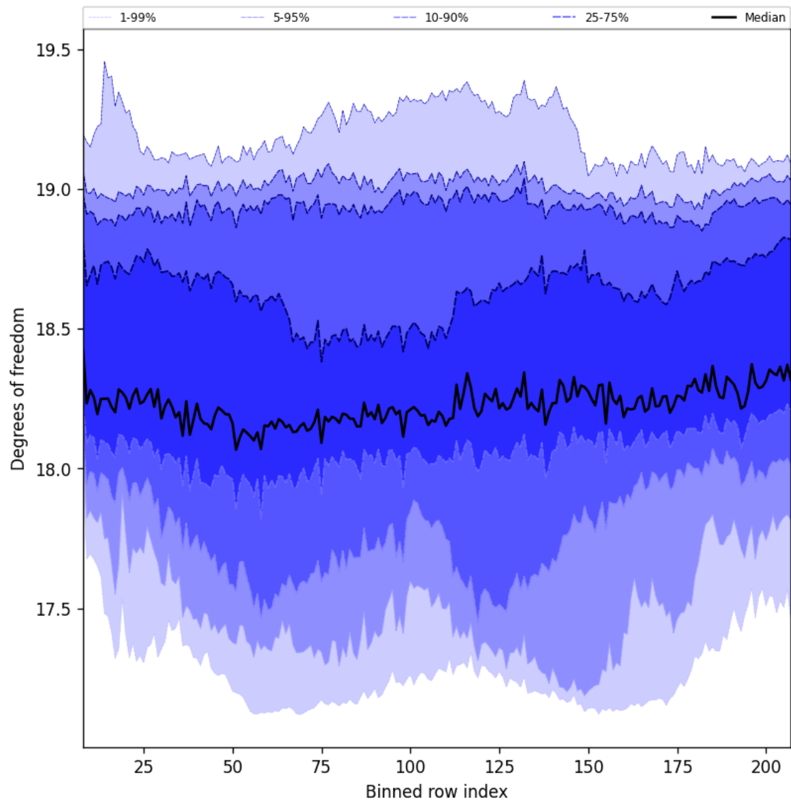
Figure 41: Along track statistics of “Degrees of freedom” for 2025-06-24 to 2025-06-26
