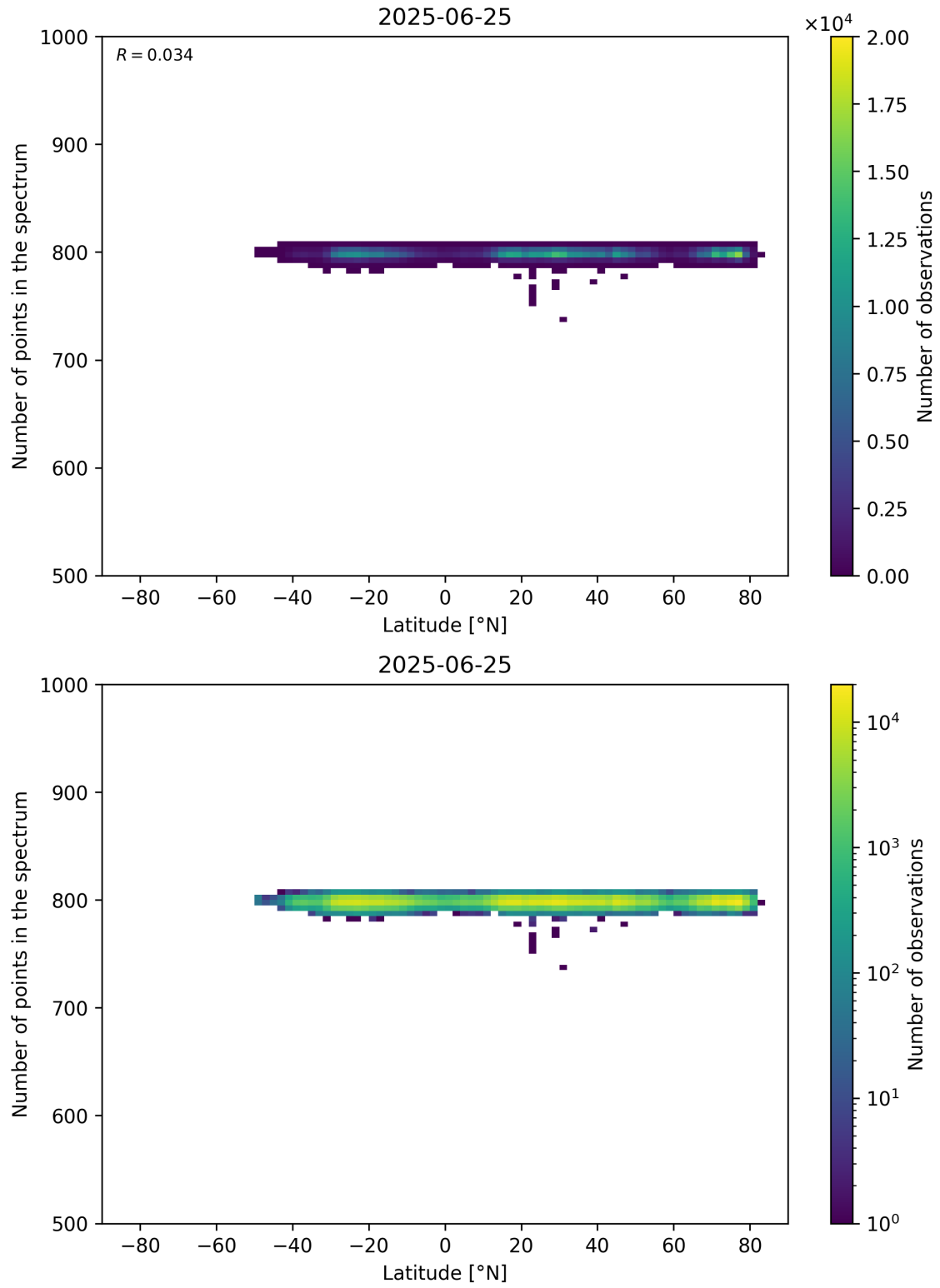
Figure 61: Scatter density plot of “Latitude” against “Number of points in the spectrum” for 2025-06-24 to 2025-06-26.
