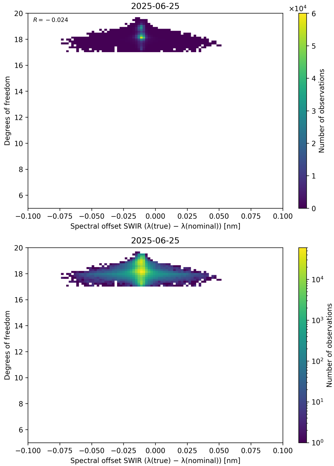
Figure 119: Scatter density plot of “Spectral offset SWIR ( \lambda_{\text{true}} - \lambda_{\text{nominal}} )” against “Degrees of freedom” for 2025-06-24 to 2025-06-26.
