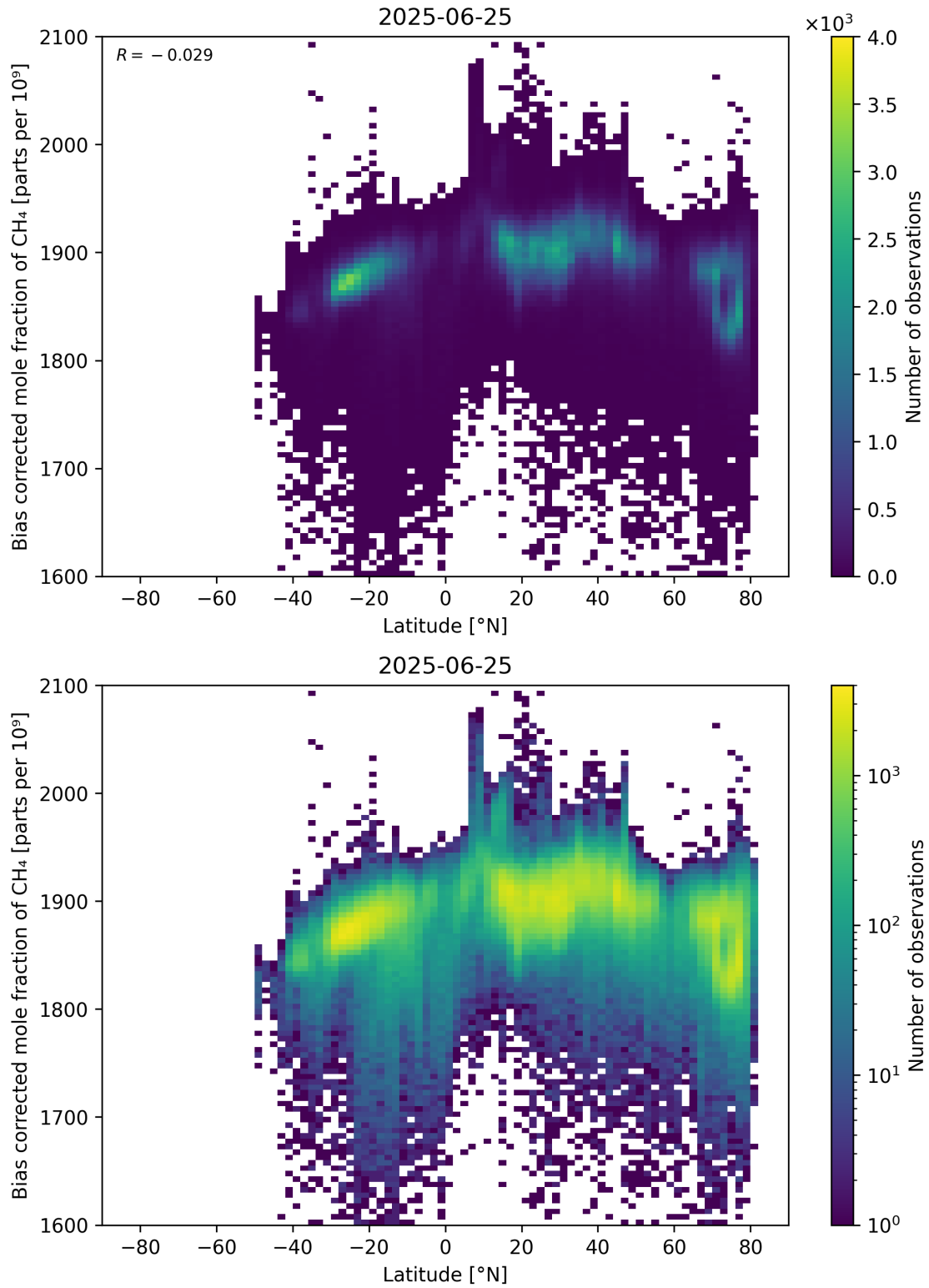
Figure 58: Scatter density plot of “Latitude” against “Bias corrected mole fraction of \text{CH}_4 ” for 2025-06-24 to 2025-06-26.
