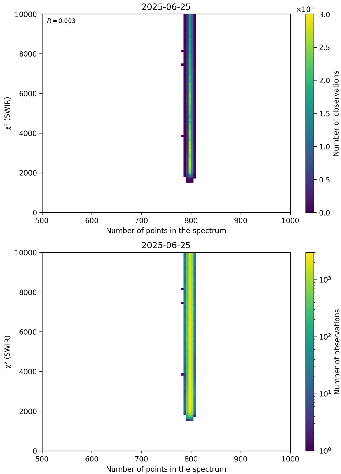
Figure 89: Scatter density plot of “Number of points in the spectrum” against “ \chi^2 (SWIR)” for 2025-06-24 to 2025-06-26.
