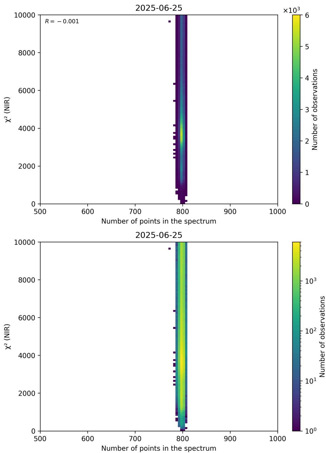
Figure 88: Scatter density plot of “Number of points in the spectrum” against “ \chi^2 (NIR)” for 2025-06-24 to 2025-06-26.
