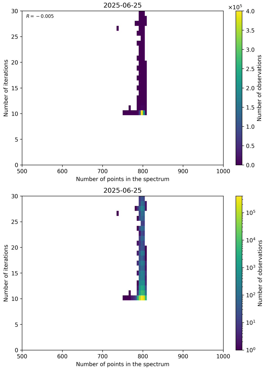
Figure 92: Scatter density plot of “Number of points in the spectrum” against “Number of iterations” for 2025-06-24 to 2025-06-26.
