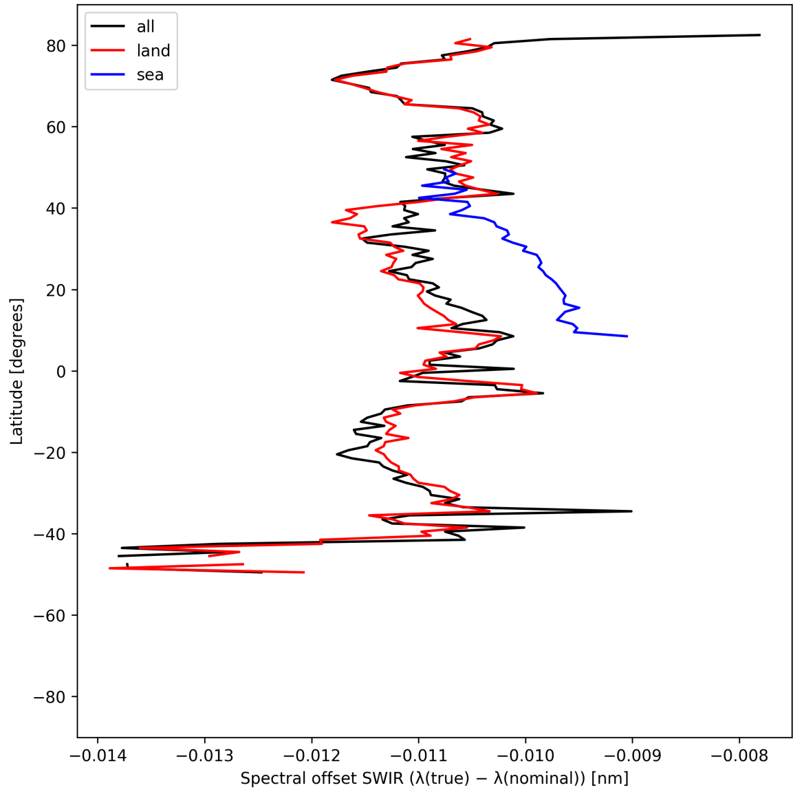
Figure 16: Zonal average of “Spectral offset SWIR ( \lambda_{\text{true}} - \lambda_{\text{nominal}} )” for 2025-06-24 to 2025-06-26.
