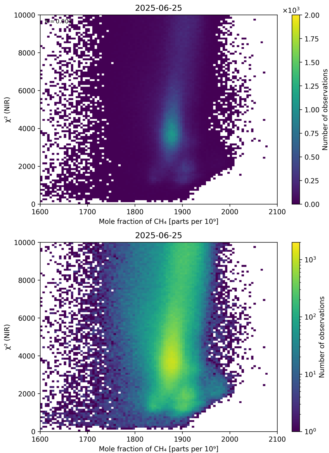
Figure 70: Scatter density plot of “Mole fraction of \text{CH}_4 ” against “ \chi^2 (NIR)” for 2025-06-24 to 2025-06-26.
