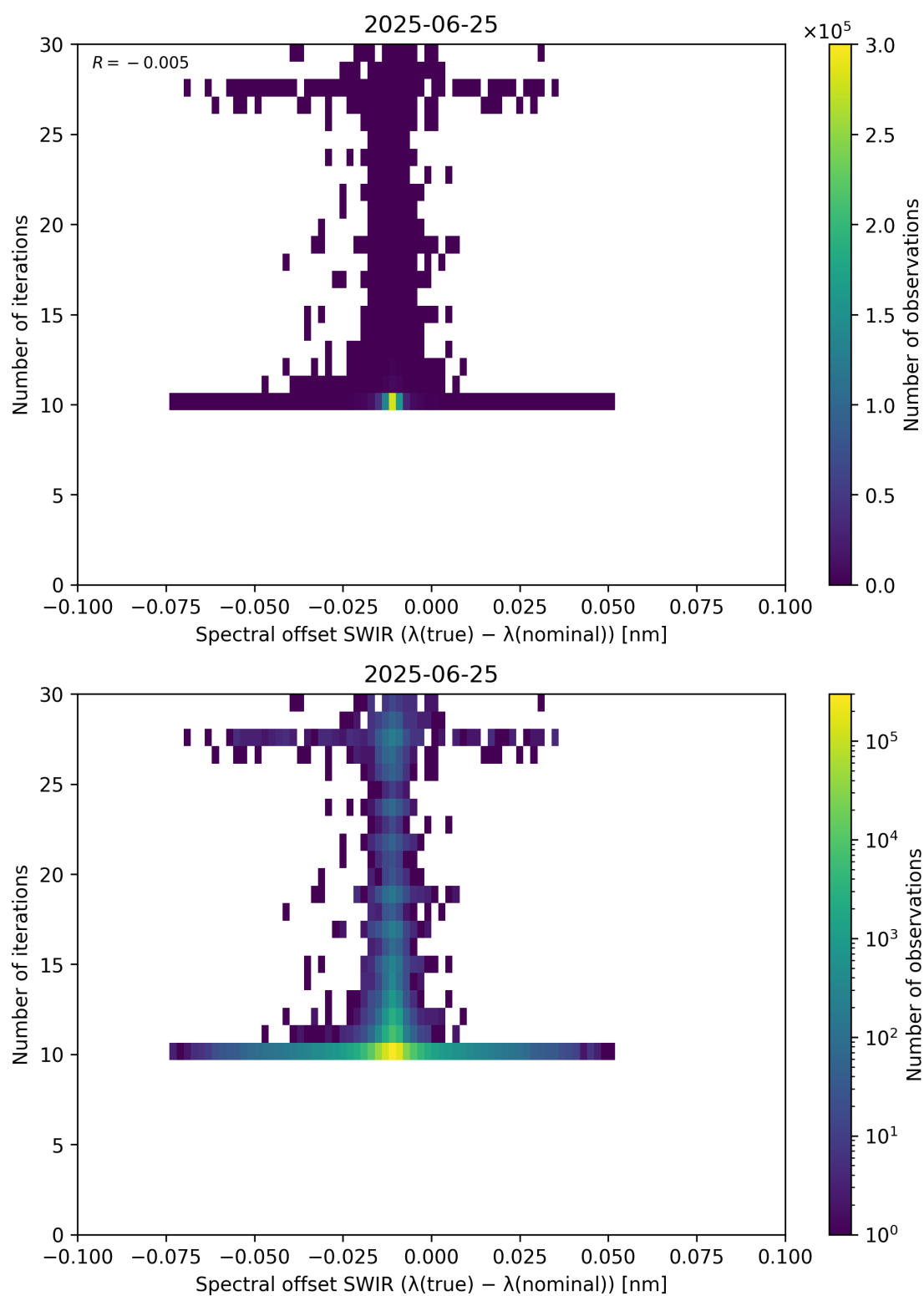
Figure 121: Scatter density plot of “Spectral offset SWIR ( \lambda_{\text{true}} - \lambda_{\text{nominal}} )” against “Number of iterations” for 2025-06-24 to 2025-06-26.
