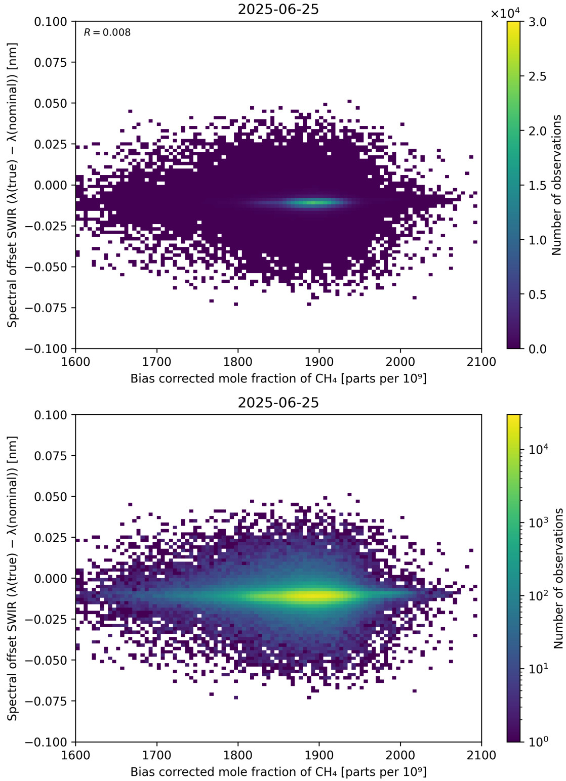
Figure 69: Scatter density plot of “Bias corrected mole fraction of \text{CH}_4 ” against “Spectral offset SWIR ( \lambda_{\text{true}} - \lambda_{\text{nominal}} )” for 2025-06-24 to 2025-06-26.
