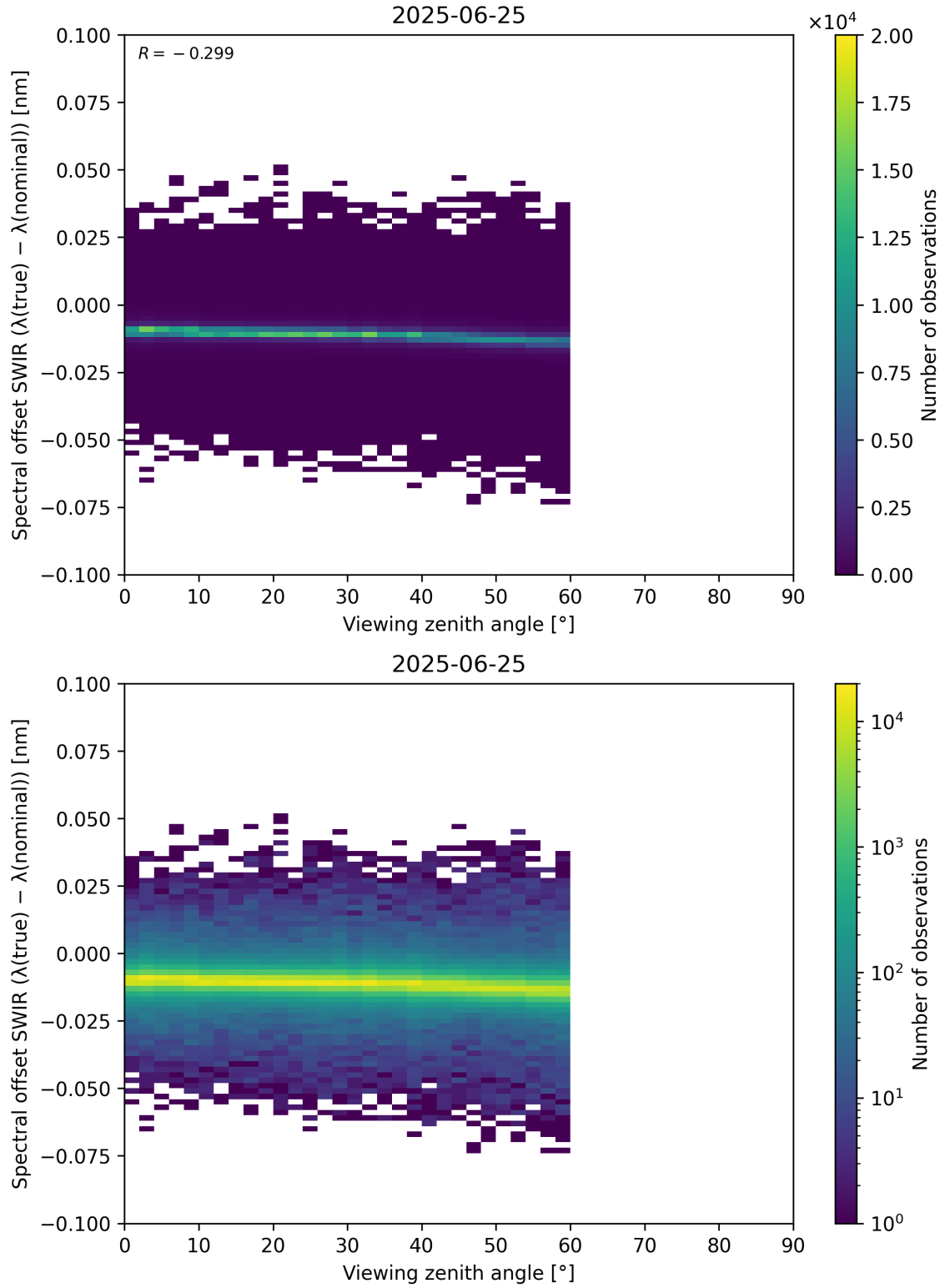
Figure 116: Scatter density plot of “Viewing zenith angle” against “Spectral offset SWIR ( \lambda_{\text{true}} - \lambda_{\text{nominal}} )” for 2025-06-24 to 2025-06-26.
