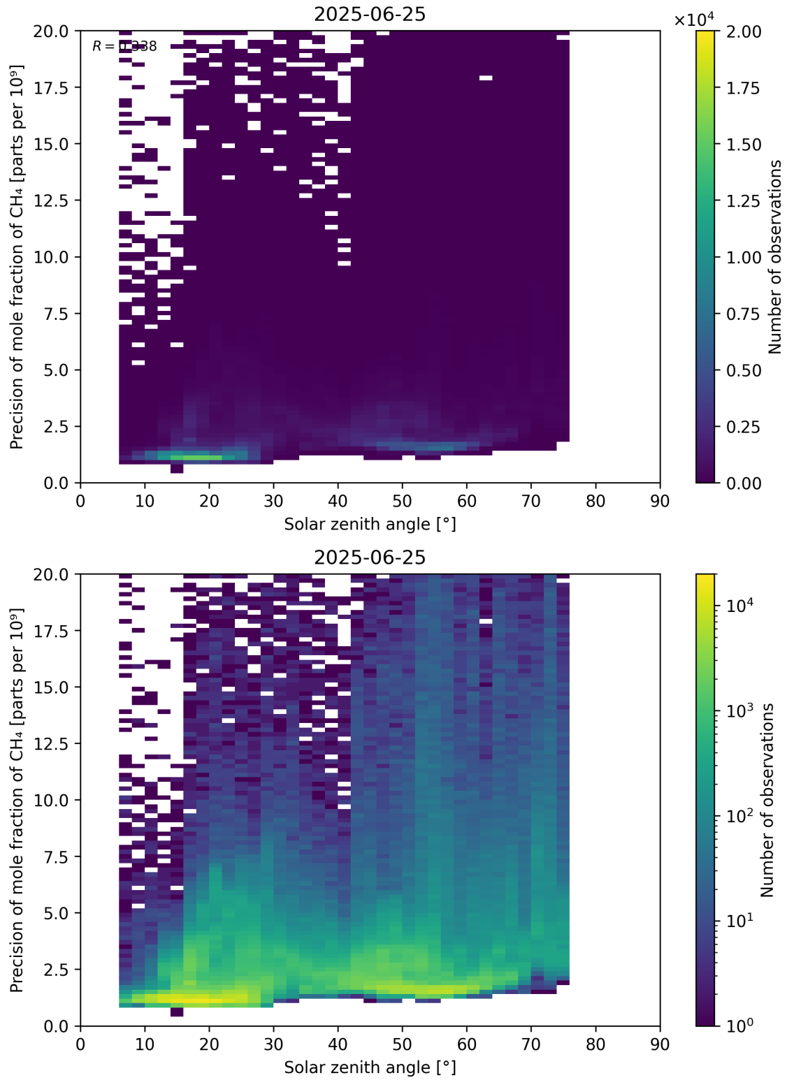
Figure 101: Scatter density plot of “Solar zenith angle” against “Precision of mole fraction of CH 4 ” for 2025-06-24 to 2025-06-26.
