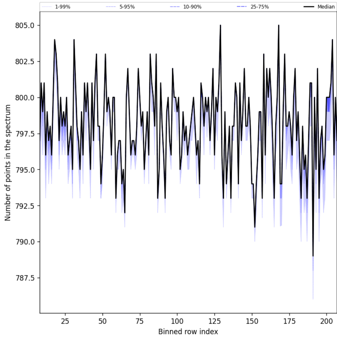
Figure 37: Along track statistics of “Number of points in the spectrum” for 2025-06-24 to 2025-06-26
