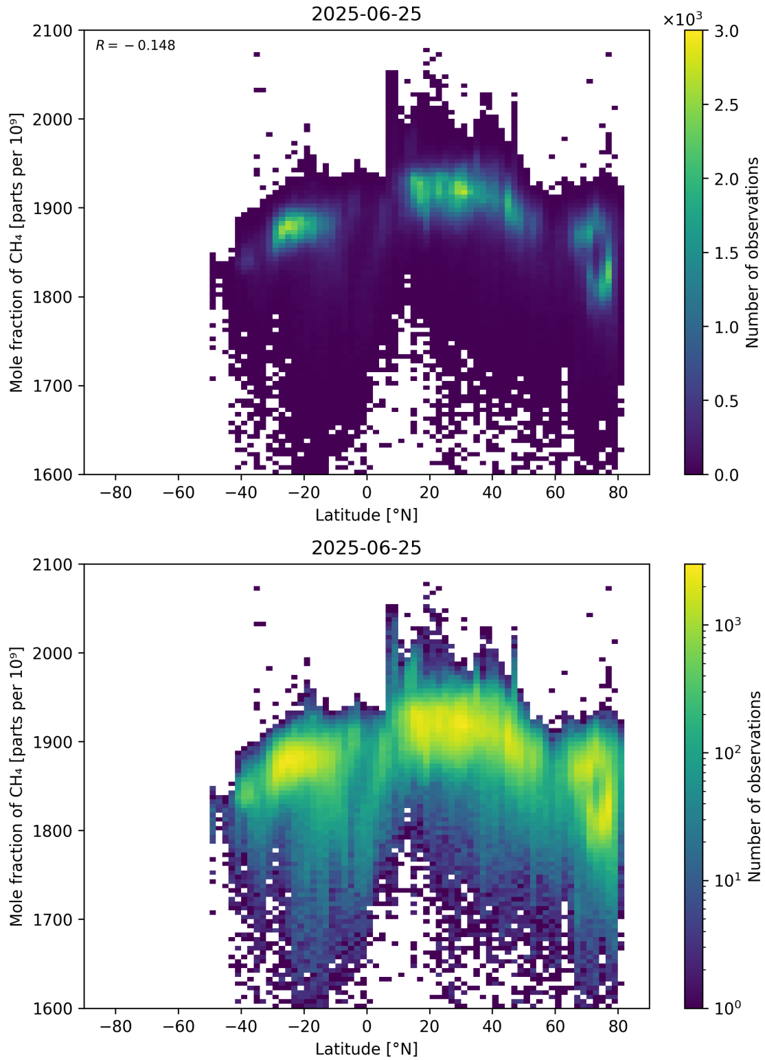
Figure 57: Scatter density plot of “Latitude” against “Mole fraction of CH 4 ” for 2025-06-24 to 2025-06-26.
