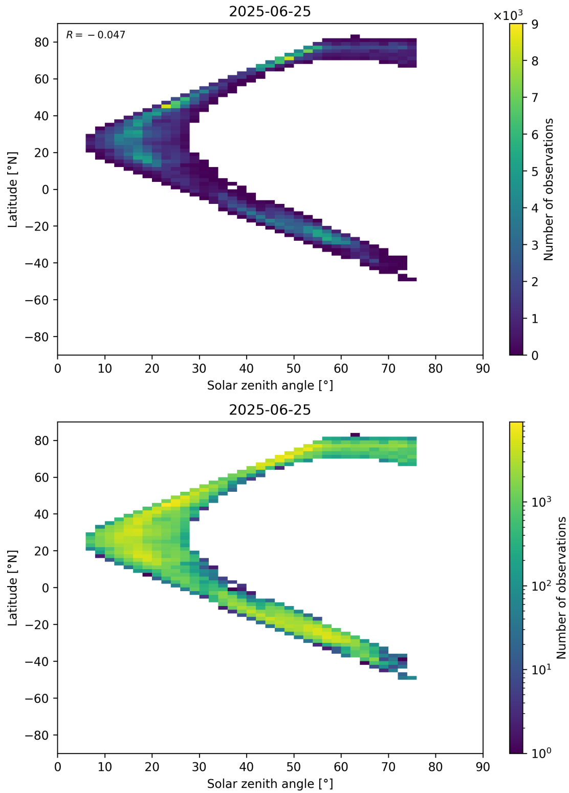
Figure 98: Scatter density plot of “Solar zenith angle” against “Latitude” for 2025-06-24 to 2025-06-26.
