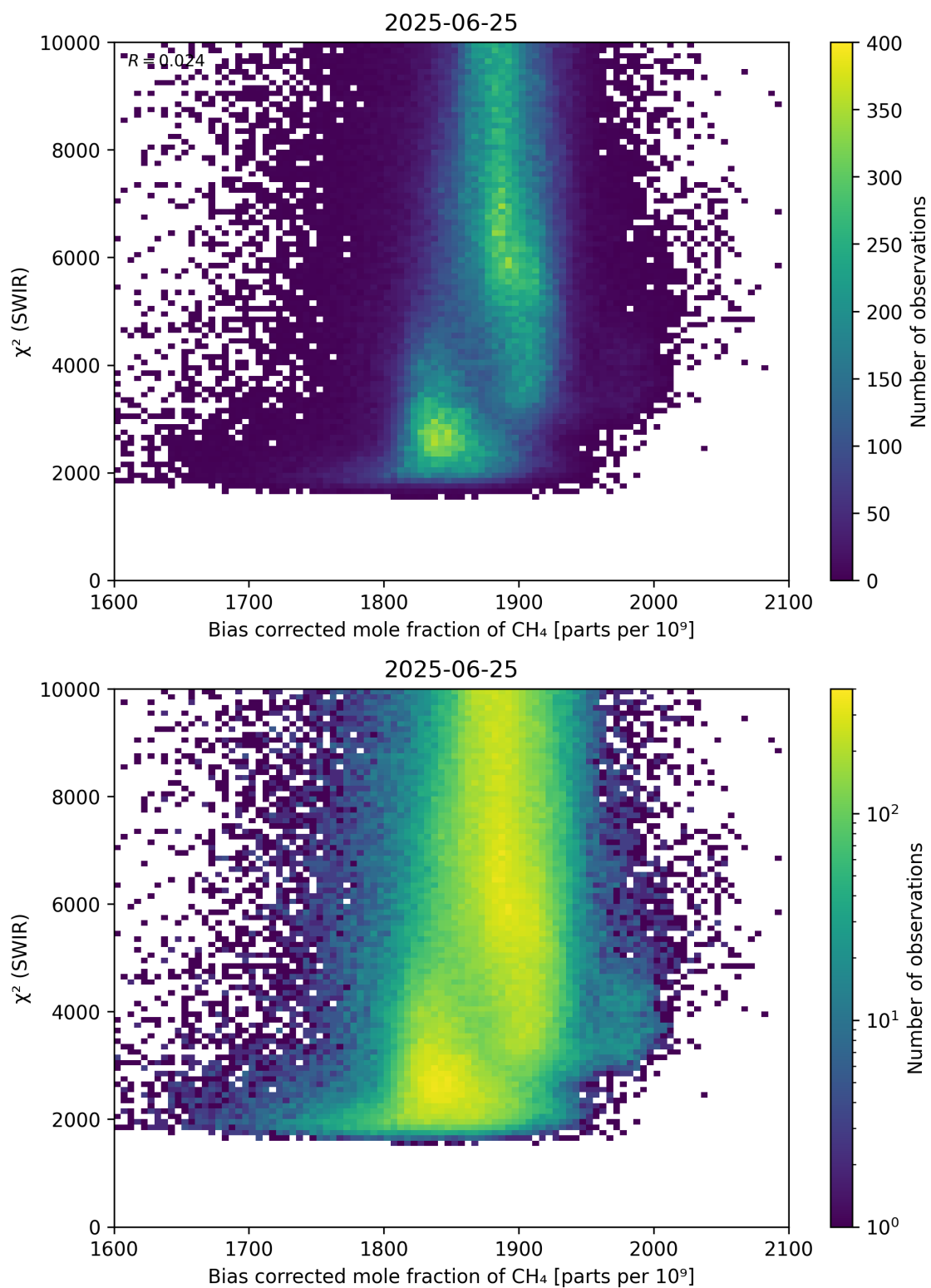
Figure 64: Scatter density plot of “Bias corrected mole fraction of \text{CH}_4 ” against “ \chi^2 (SWIR)” for 2025-06-24 to 2025-06-26.
