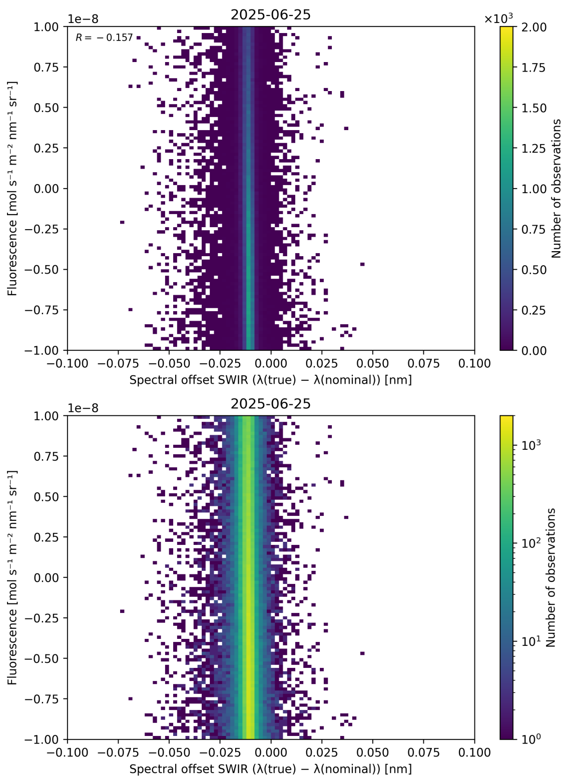
Figure 120: Scatter density plot of “Spectral offset SWIR ( \lambda_{\text{true}} - \lambda_{\text{nominal}} )” against “Fluorescence” for 2025-06-24 to 2025-06-26.
