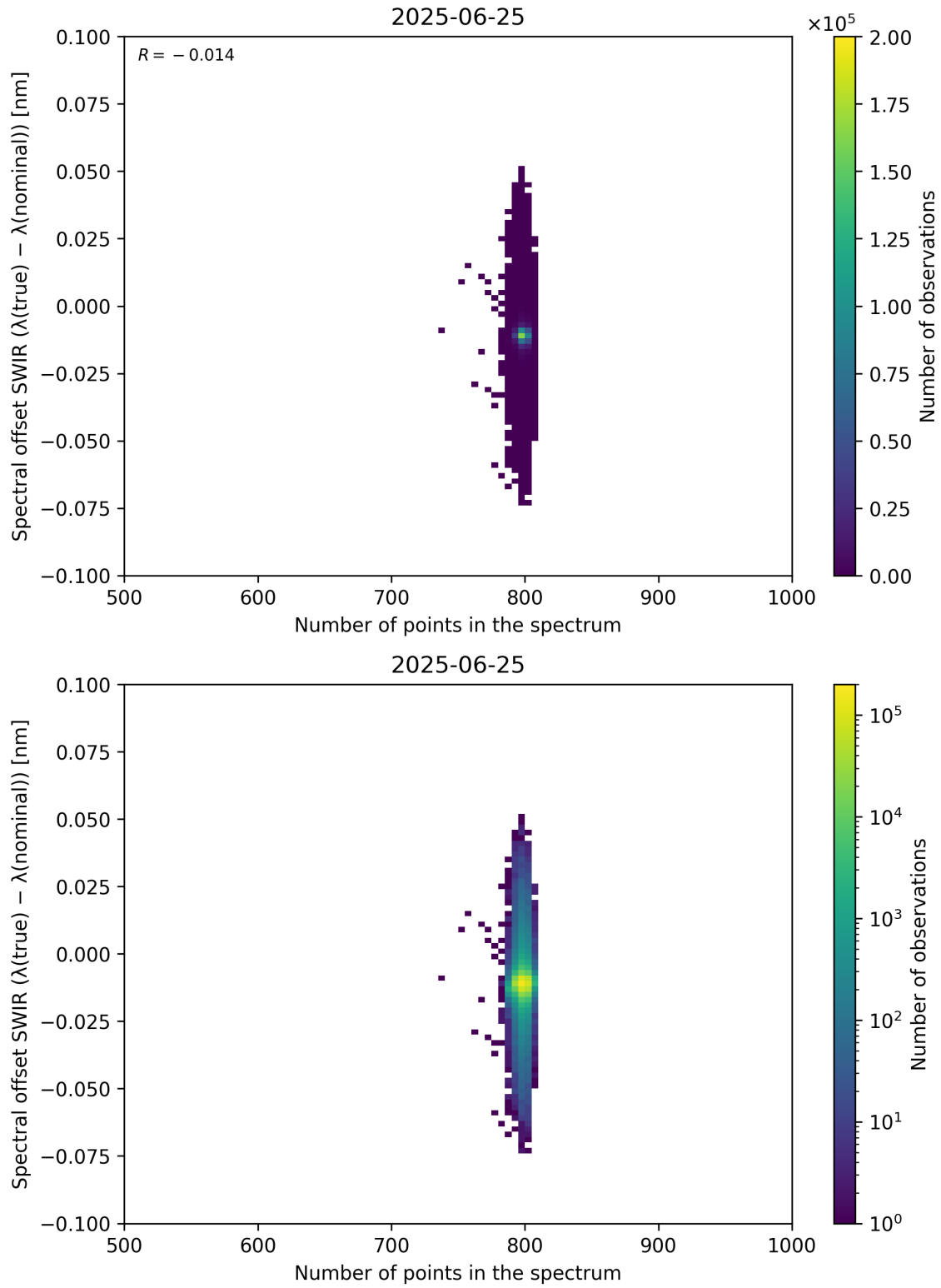
Figure 93: Scatter density plot of “Number of points in the spectrum” against “Spectral offset SWIR ( \lambda_{\text{true}} - \lambda_{\text{nominal}} )” for 2025-06-24 to 2025-06-26.
