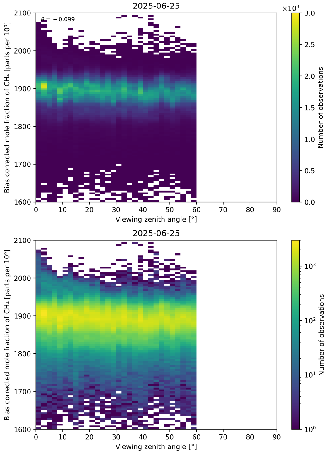
Figure 111: Scatter density plot of “Viewing zenith angle” against “Bias corrected mole fraction of CH 4 ” for 2025-06-24 to 2025-06-26.
