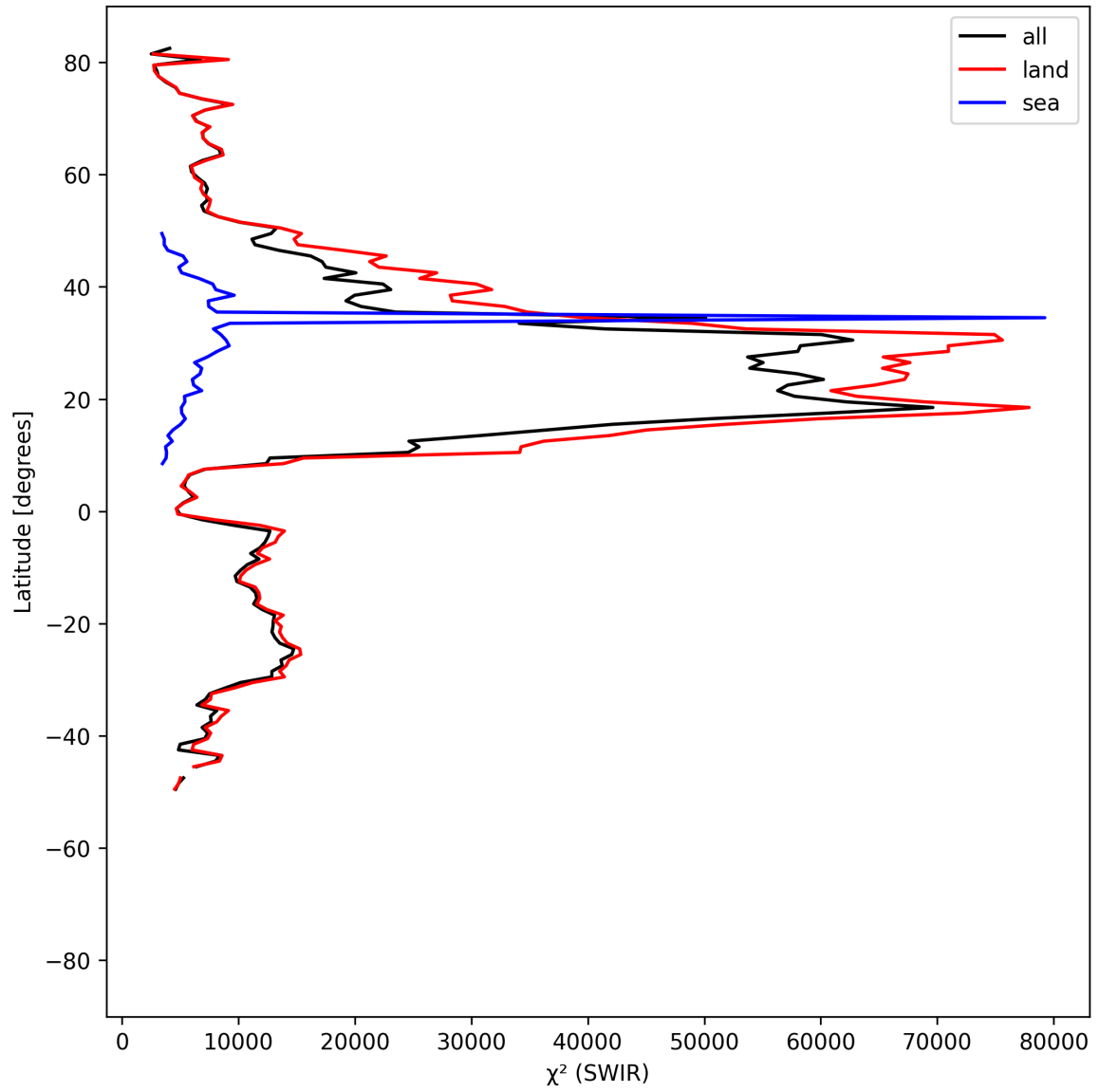
Figure 17: Zonal average of “ \chi^2 (SWIR)” for 2025-06-24 to 2025-06-26.
