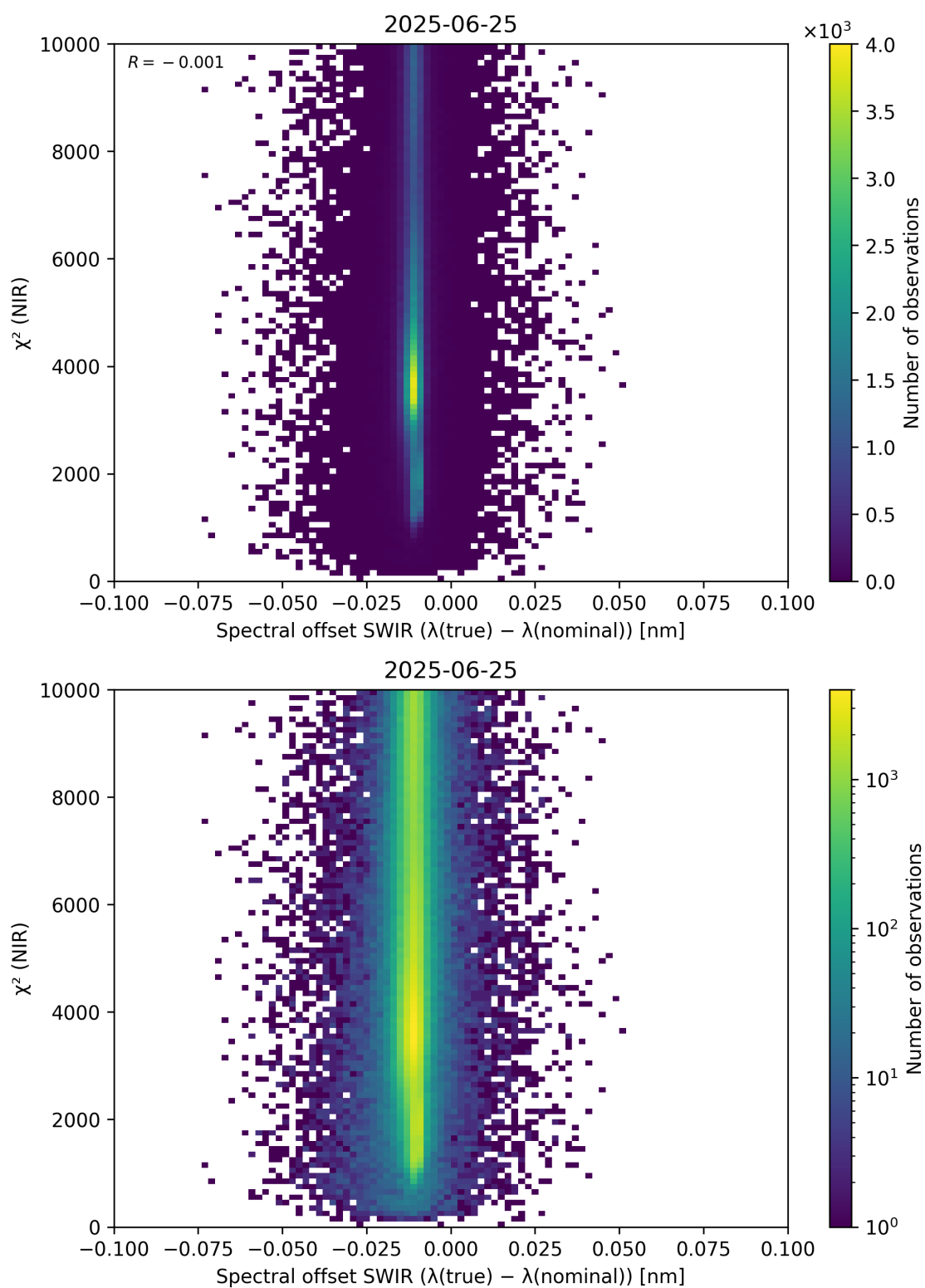
Figure 117: Scatter density plot of “Spectral offset SWIR ( \lambda_{\text{true}} - \lambda_{\text{nominal}} )” against “ \chi^2 (NIR)” for 2025-06-24 to 2025-06-26.
