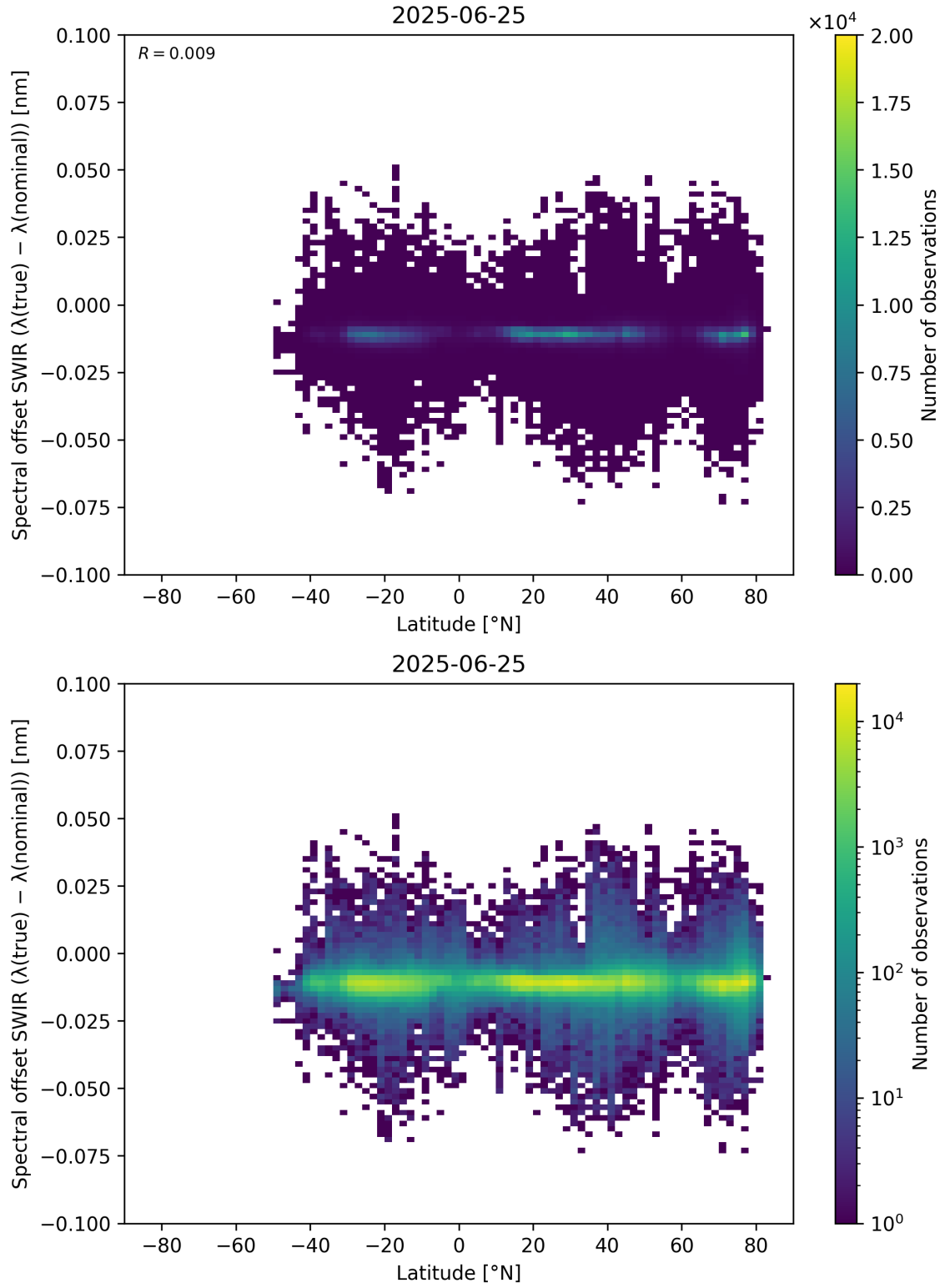
Figure 62: Scatter density plot of “Latitude” against “Spectral offset SWIR ( \lambda_{\text{true}} - \lambda_{\text{nominal}} )” for 2025-06-24 to 2025-06-26.
