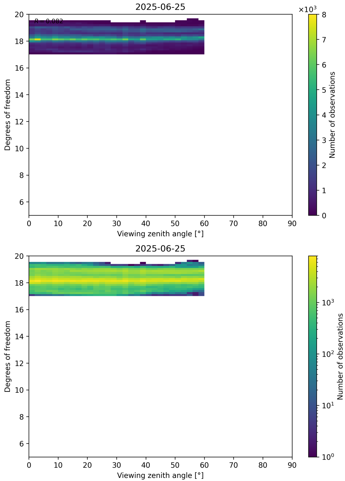
Figure 107: Scatter density plot of “Viewing zenith angle” against “Degrees of freedom” for 2025-06-24 to 2025-06-26.
