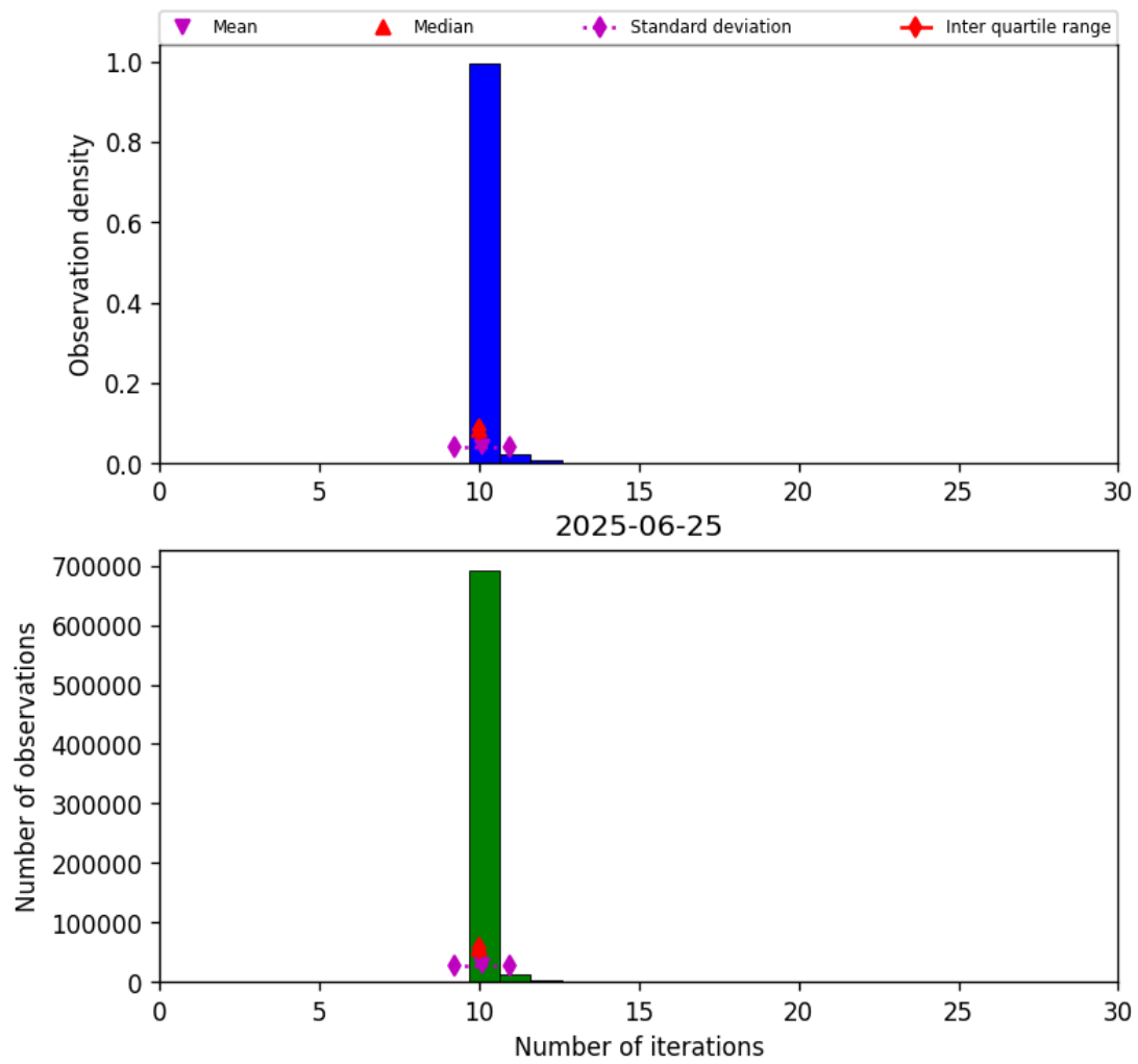
Figure 31: Histogram of “Number of iterations” for 2025-06-24 to 2025-06-26
