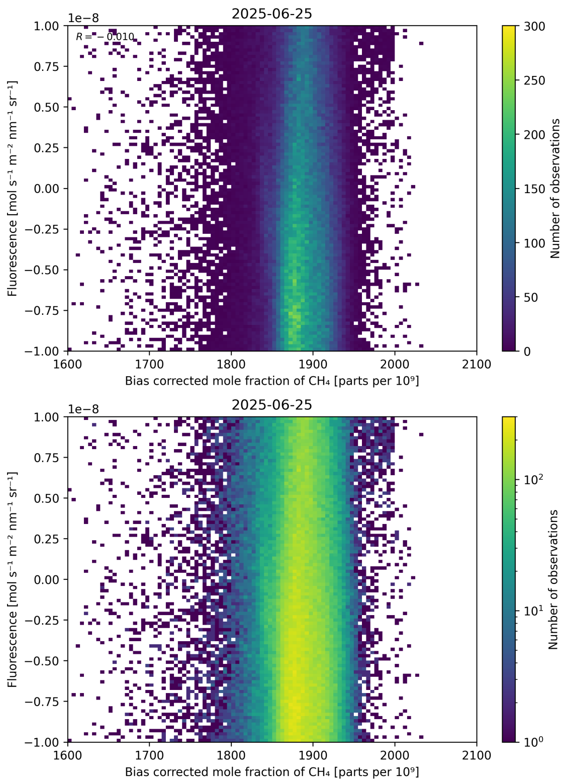
Figure 66: Scatter density plot of “Bias corrected mole fraction of \text{CH}_4 ” against “Fluorescence” for 2025-06-24 to 2025-06-26.
