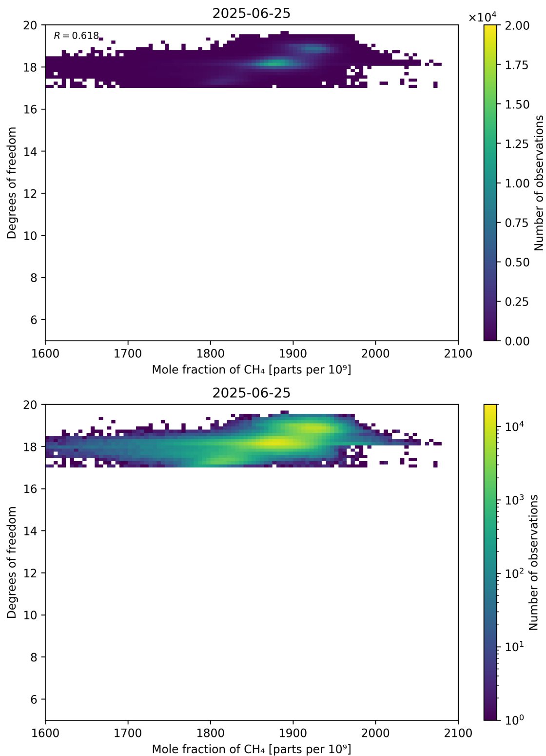
Figure 72: Scatter density plot of “Mole fraction of CH 4 ” against “Degrees of freedom” for 2025-06-24 to 2025-06-26.
