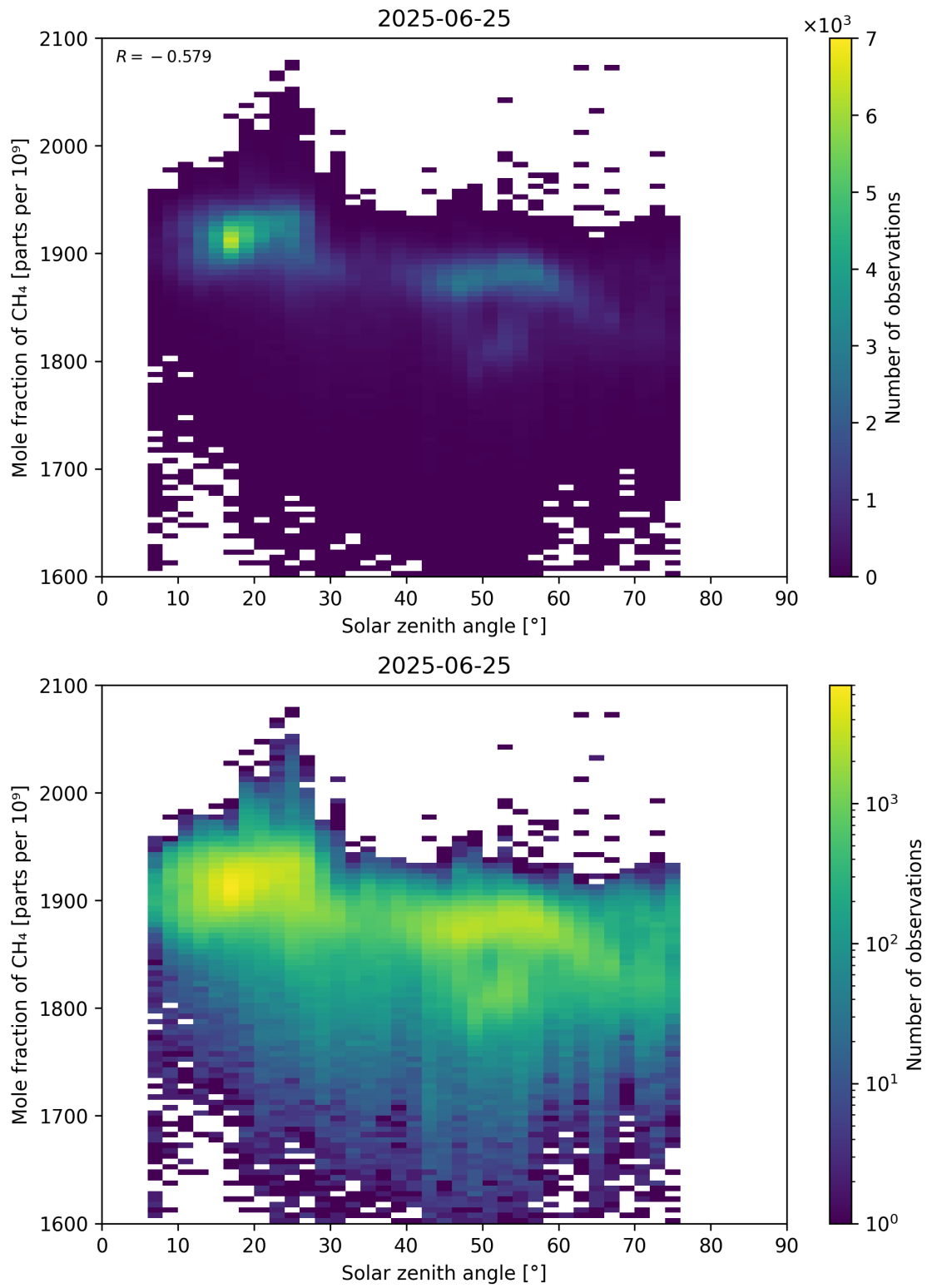
Figure 99: Scatter density plot of “Solar zenith angle” against “Mole fraction of \text{CH}_4 ” for 2025-06-24 to 2025-06-26.
