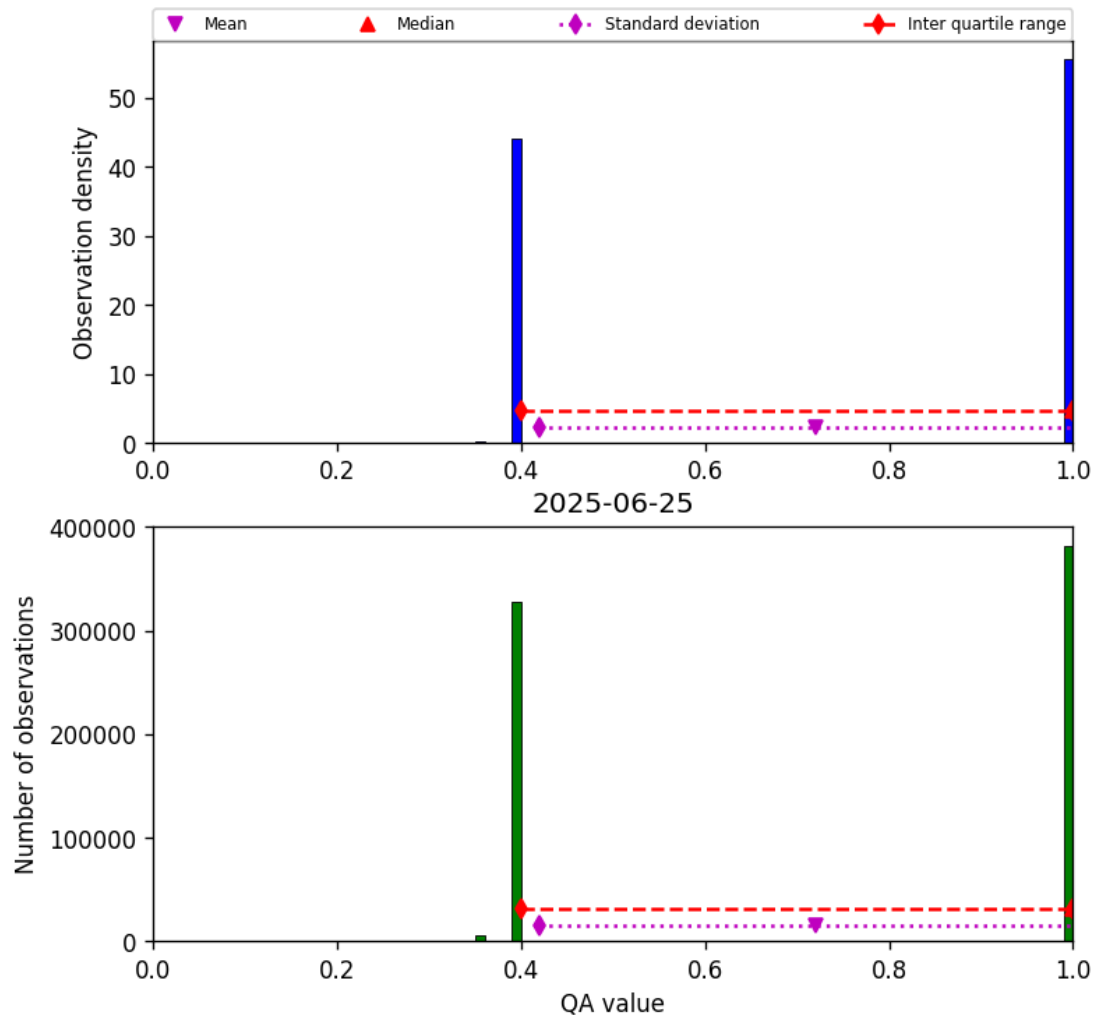
Figure 22: Histogram of “QA value” for 2025-06-24 to 2025-06-26
