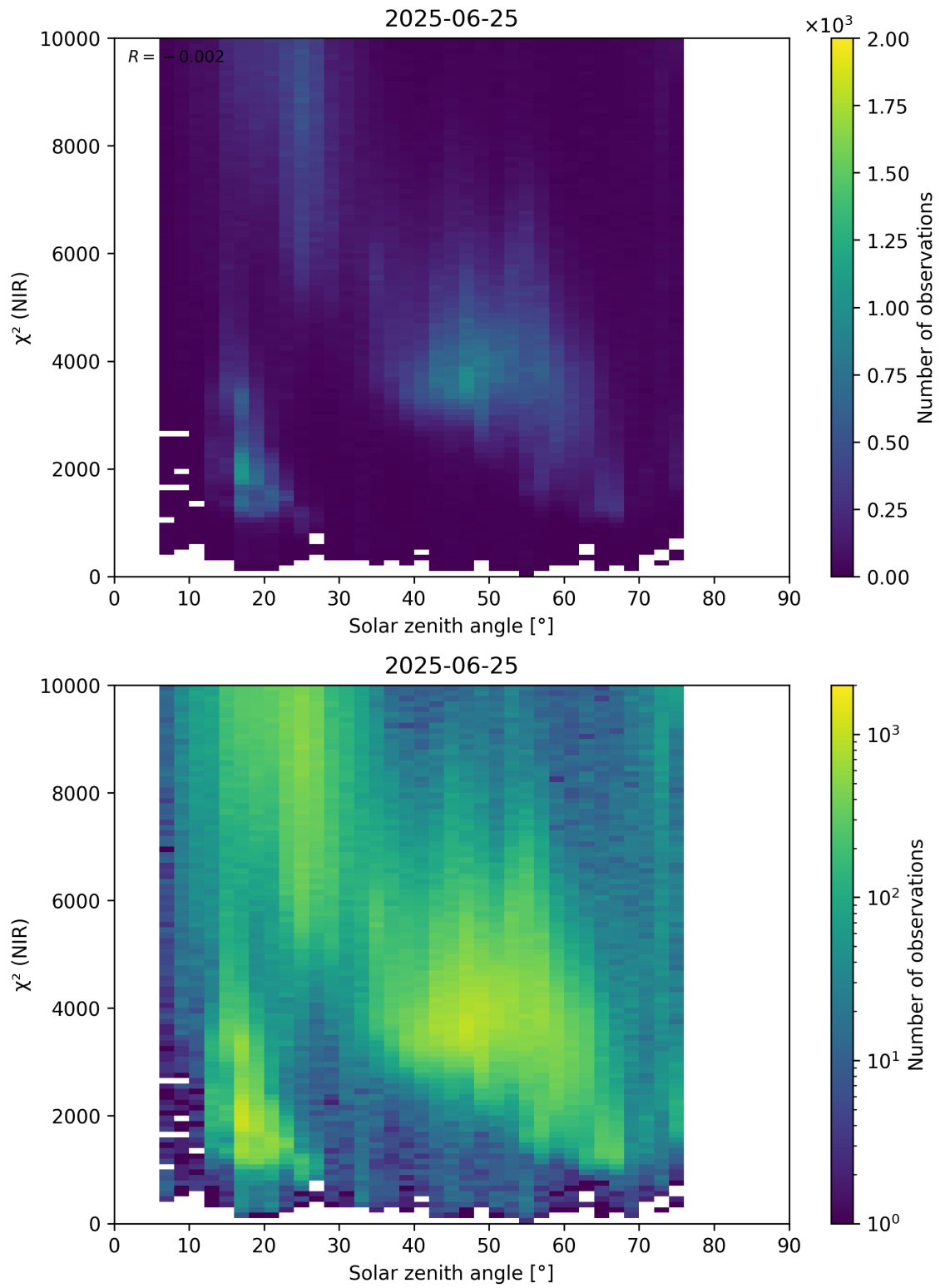
Figure 94: Scatter density plot of “Solar zenith angle” against “ \chi^2 (NIR)” for 2025-06-24 to 2025-06-26.
