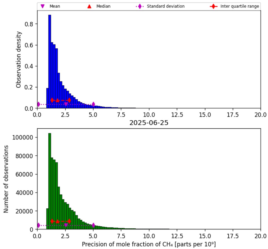
Figure 24: Histogram of “Precision of mole fraction of CH 4 ” for 2025-06-24 to 2025-06-26
