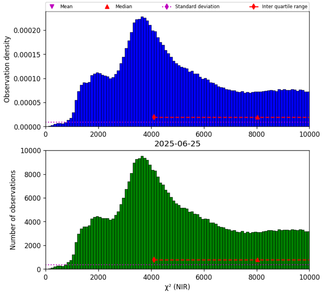
Figure 29: Histogram of " \chi^2 (NIR)" for 2025-06-24 to 2025-06-26
