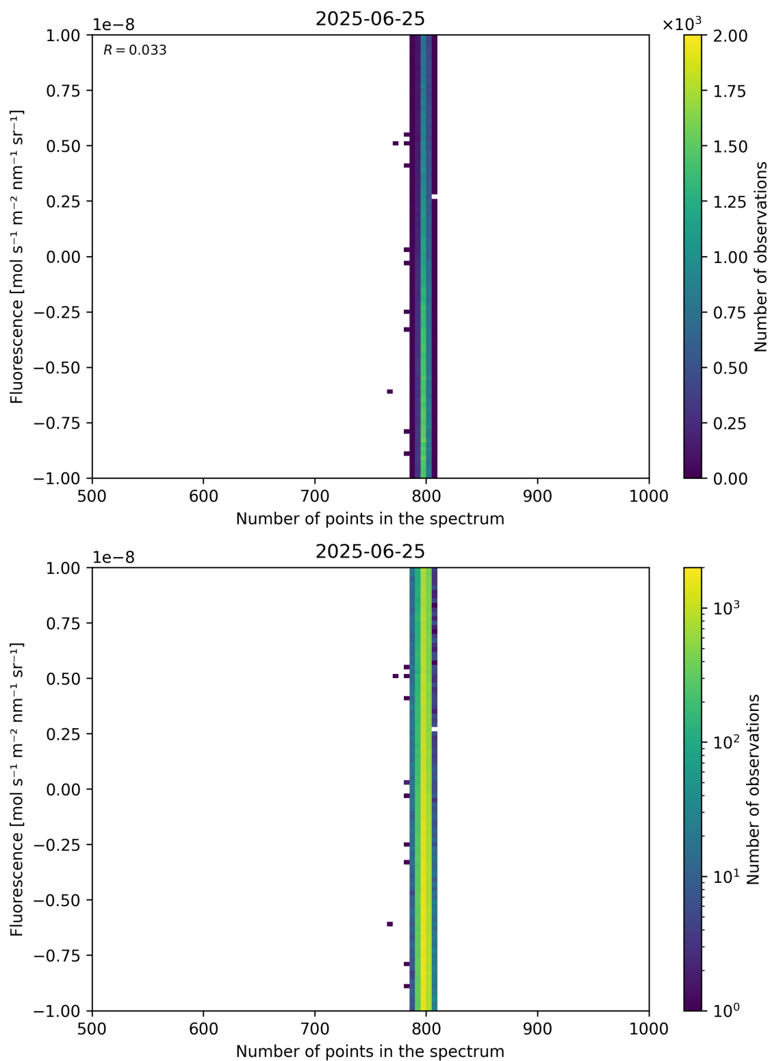
Figure 91: Scatter density plot of “Number of points in the spectrum” against “Fluorescence” for 2025-06-24 to 2025-06-26.
