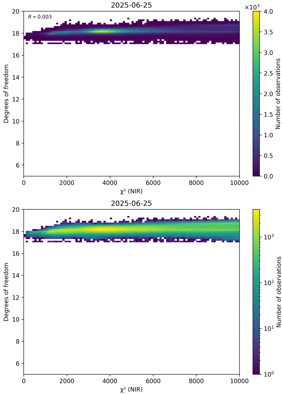
Figure 44: Scatter density plot of “ \chi^2 (NIR)” against “Degrees of freedom” for 2025-06-24 to 2025-06-26.
