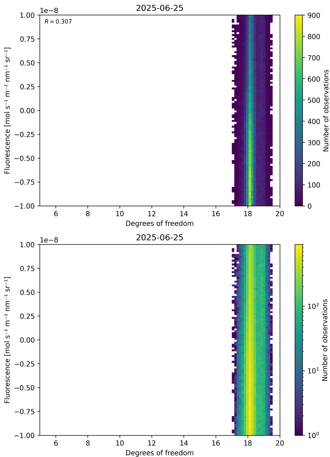
Figure 51: Scatter density plot of “Degrees of freedom” against “Fluorescence” for 2025-06-24 to 2025-06-26.
