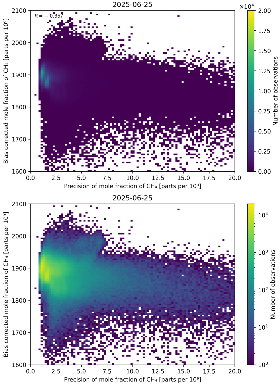
Figure 82: Scatter density plot of “Precision of mole fraction of CH 4 ” against “Bias corrected mole fraction of CH 4 ” for 2025-06-24 to 2025-06-26.
