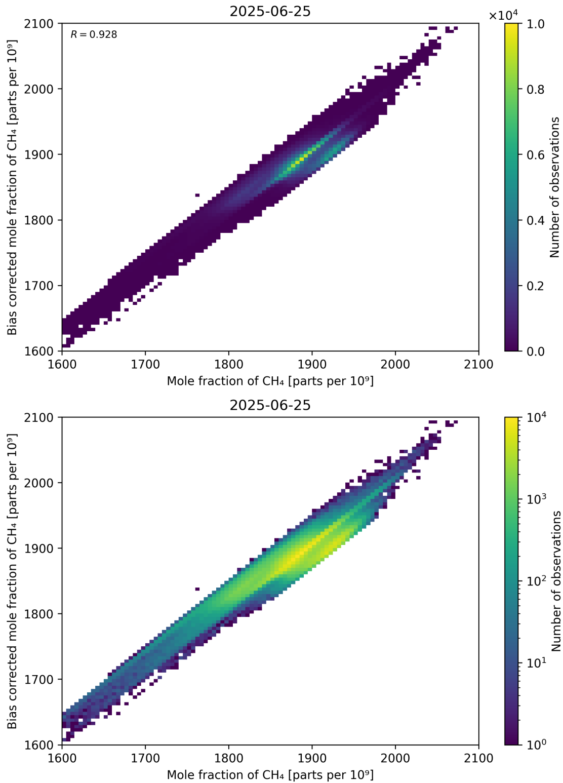
Figure 74: Scatter density plot of “Mole fraction of CH 4 ” against “Bias corrected mole fraction of CH 4 ” for 2025-06-24 to 2025-06-26.
