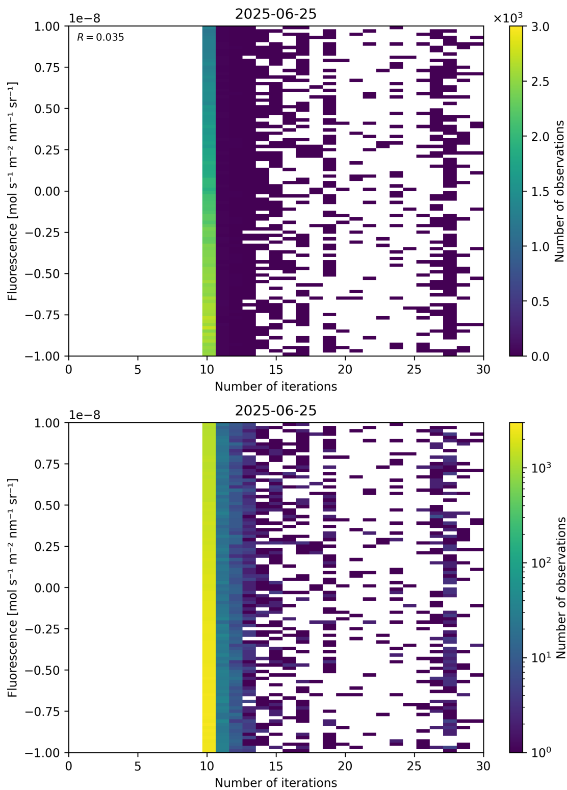
Figure 87: Scatter density plot of “Number of iterations” against “Fluorescence” for 2025-06-24 to 2025-06-26.
