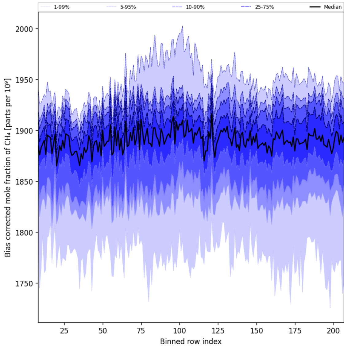
Figure 36: Along track statistics of “Bias corrected mole fraction of CH 4 ” for 2025-06-24 to 2025-06-26
