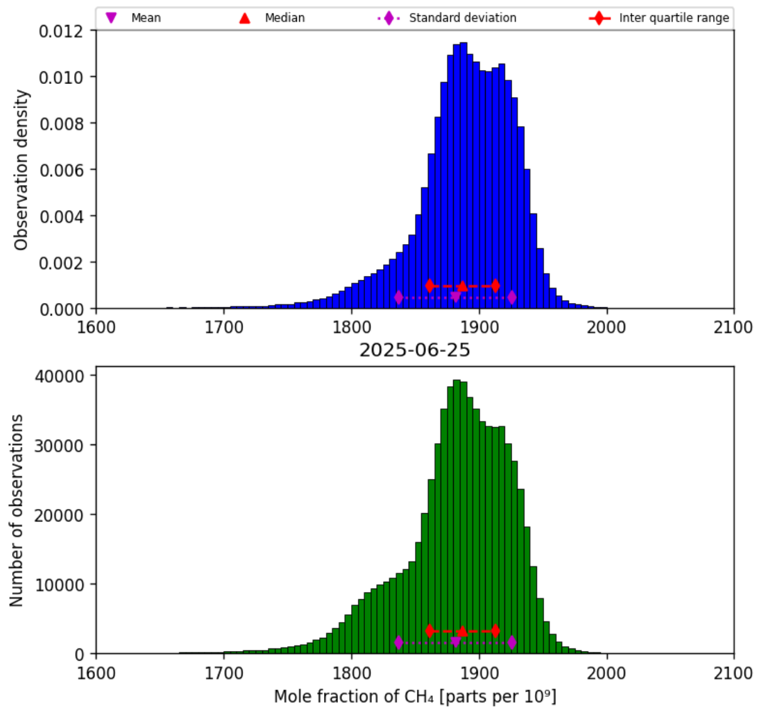
Figure 23: Histogram of “Mole fraction of CH 4 ” for 2025-06-24 to 2025-06-26
