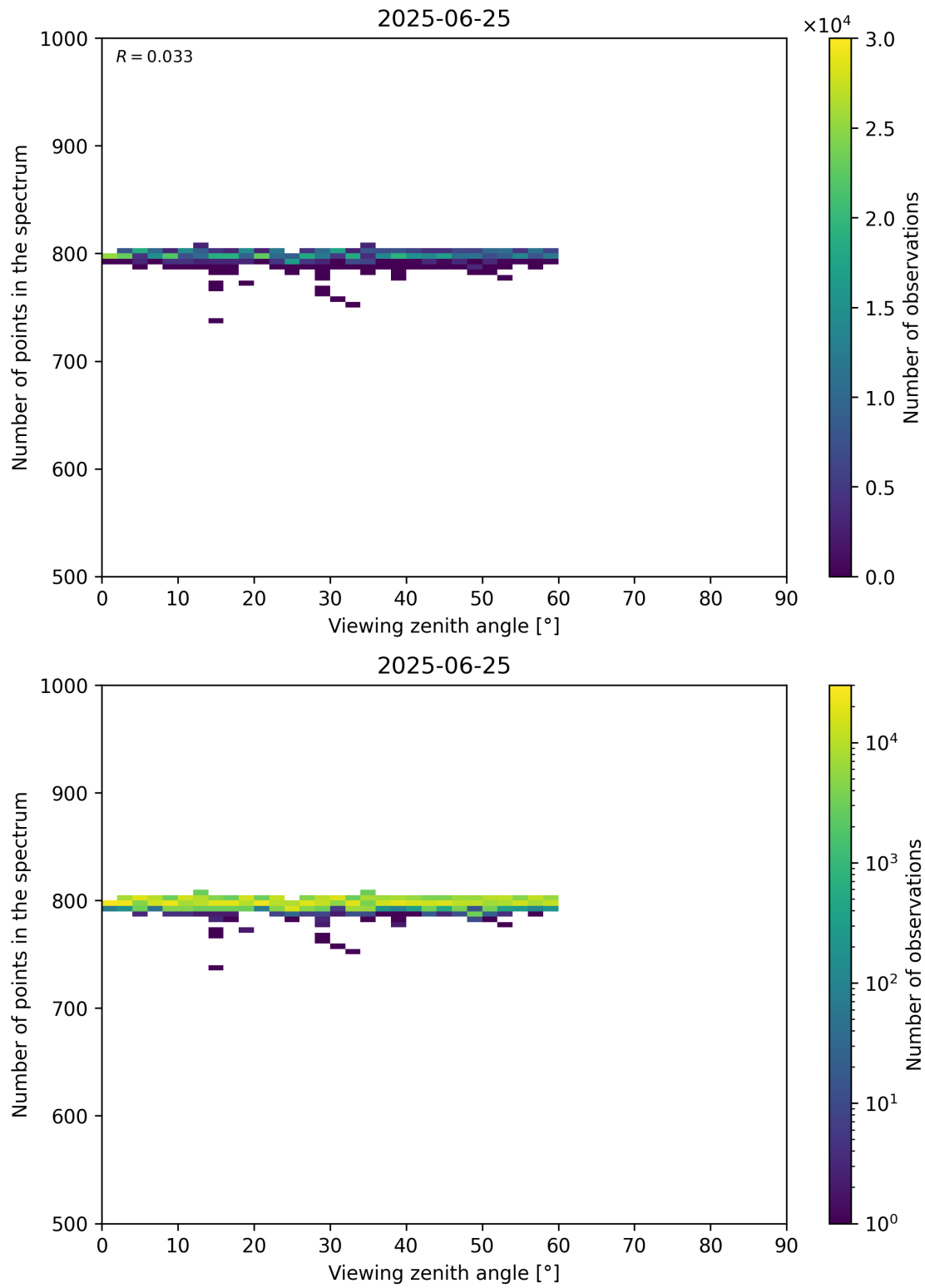
Figure 114: Scatter density plot of “Viewing zenith angle” against “Number of points in the spectrum” for 2025-06-24 to 2025-06-26.
