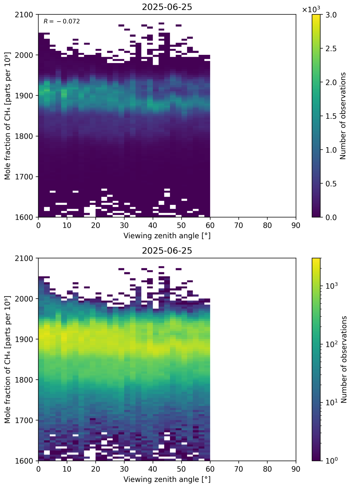
Figure 110: Scatter density plot of “Viewing zenith angle” against “Mole fraction of \text{CH}_4 ” for 2025-06-24 to 2025-06-26.
