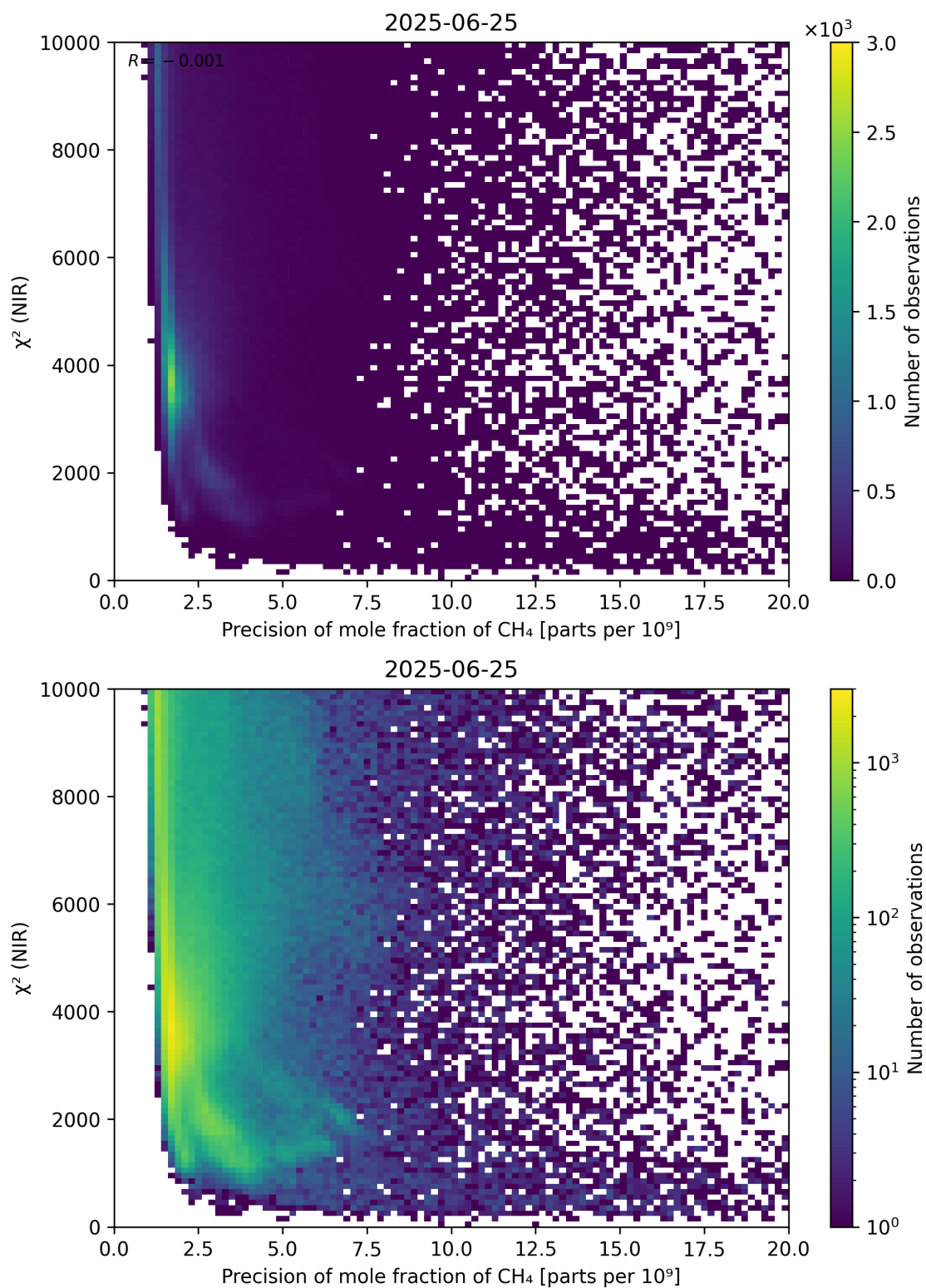
Figure 78: Scatter density plot of “Precision of mole fraction of CH 4 ” against “ \chi^2 (NIR)” for 2025-06-24 to 2025-06-26.
