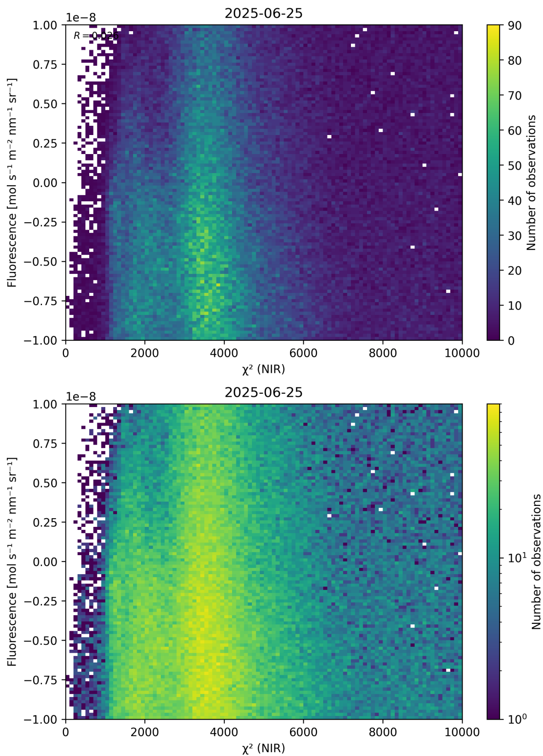
Figure 45: Scatter density plot of “ \chi^2 (NIR)” against “Fluorescence” for 2025-06-24 to 2025-06-26.
