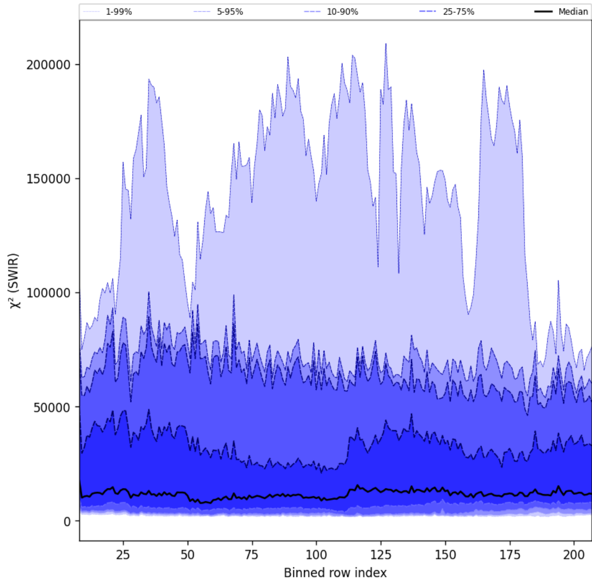
Figure 39: Along track statistics of " \chi^2 (SWIR)" for 2025-06-24 to 2025-06-26
