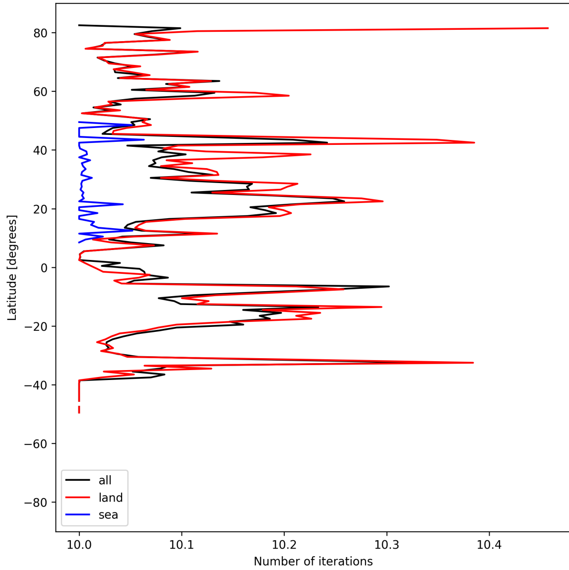
Figure 20: Zonal average of “Number of iterations” for 2025-06-24 to 2025-06-26.
