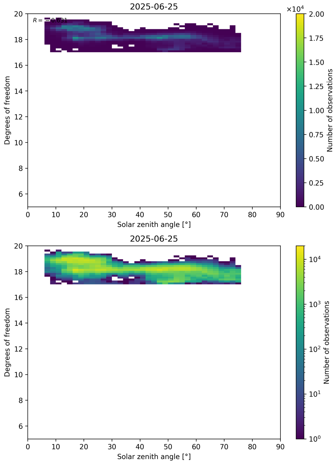
Figure 96: Scatter density plot of “Solar zenith angle” against “Degrees of freedom” for 2025-06-24 to 2025-06-26.
