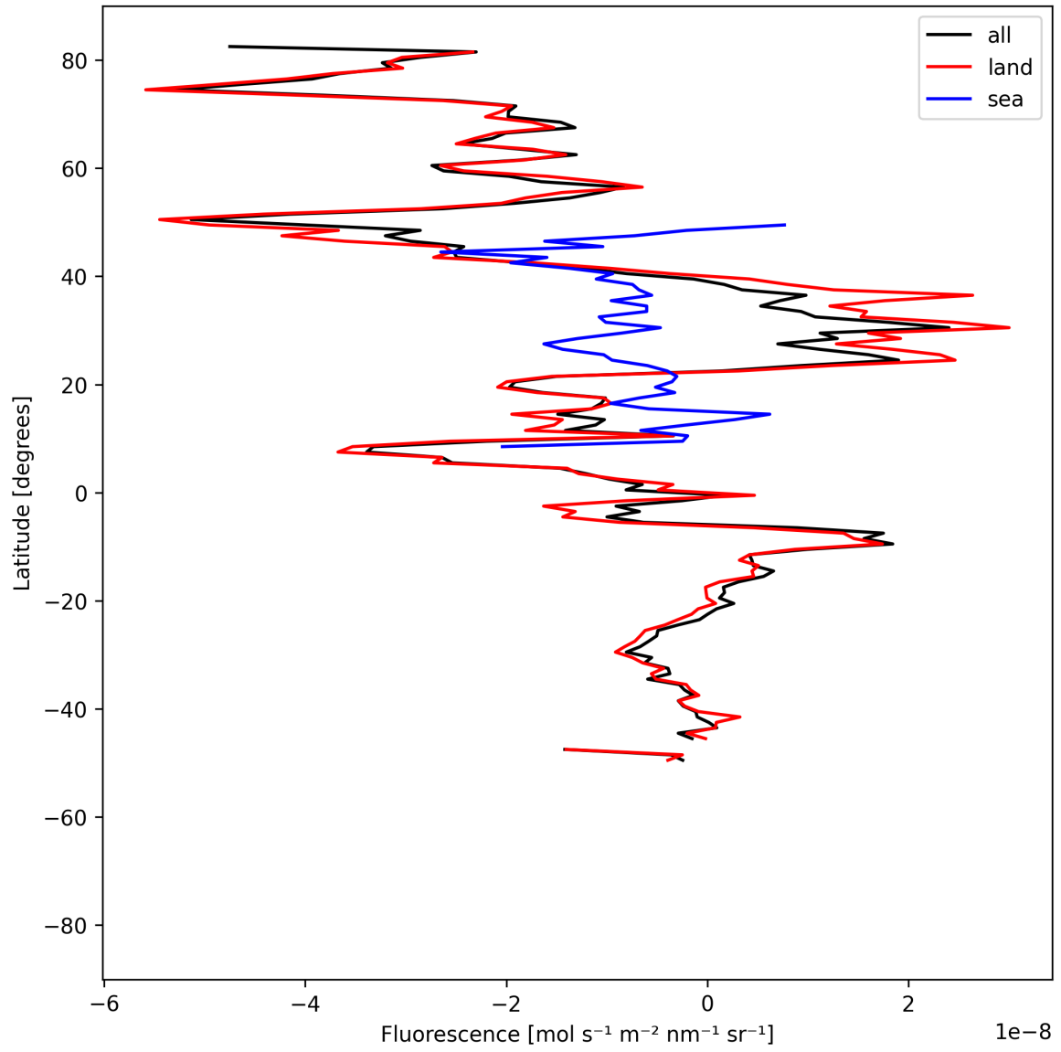
Figure 21: Zonal average of “Fluorescence” for 2025-06-24 to 2025-06-26.
