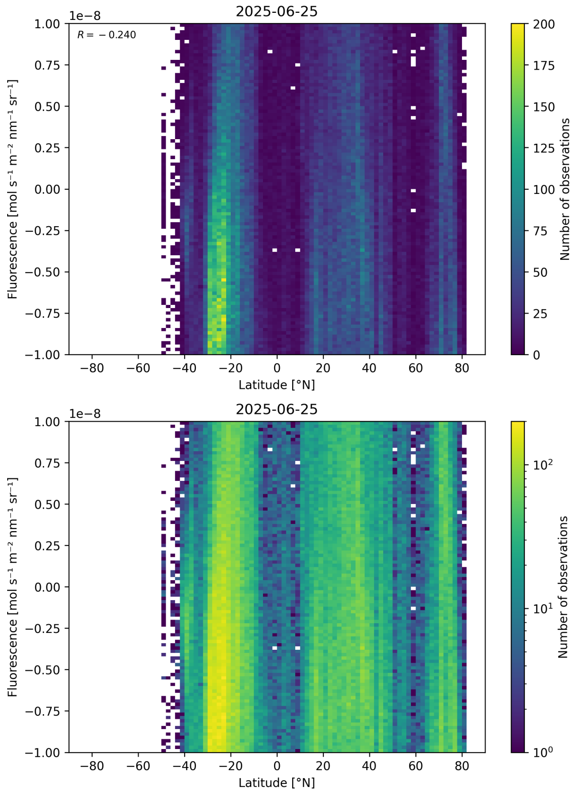
Figure 56: Scatter density plot of “Latitude” against “Fluorescence” for 2025-06-24 to 2025-06-26.
