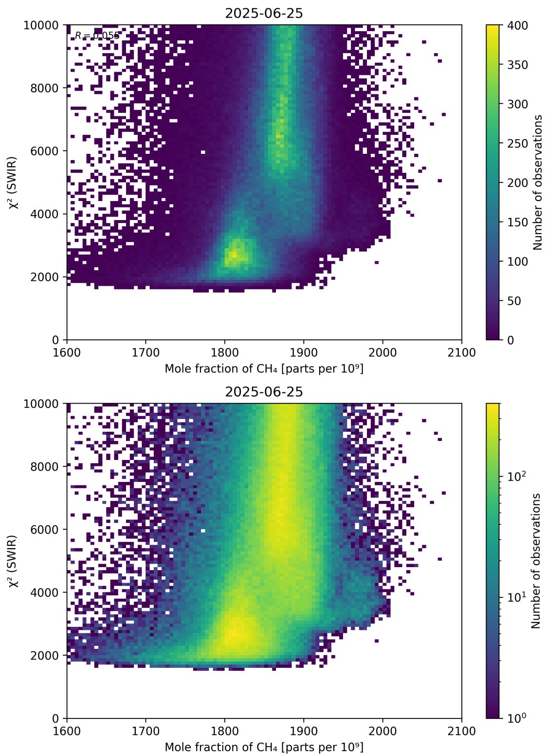
Figure 71: Scatter density plot of “Mole fraction of \text{CH}_4 ” against “ \chi^2 (SWIR)” for 2025-06-24 to 2025-06-26.
