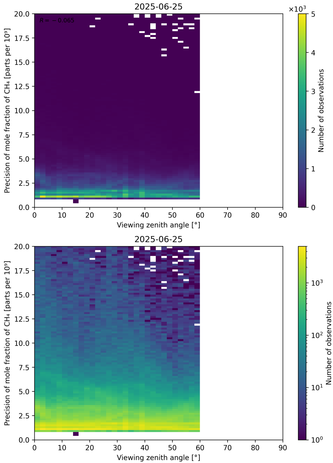
Figure 112: Scatter density plot of “Viewing zenith angle” against “Precision of mole fraction of CH 4 ” for 2025-06-24 to 2025-06-26.
