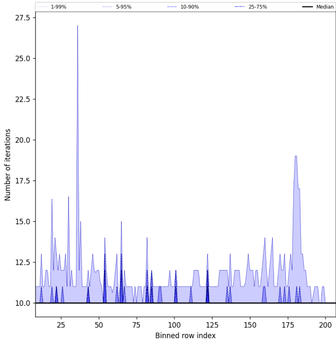
Figure 42: Along track statistics of “Number of iterations” for 2025-06-24 to 2025-06-26
