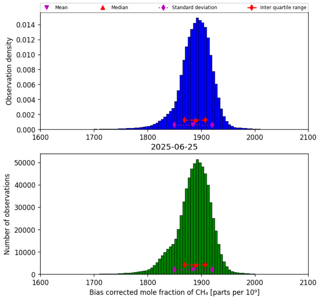
Figure 25: Histogram of “Bias corrected mole fraction of CH 4 ” for 2025-06-24 to 2025-06-26
