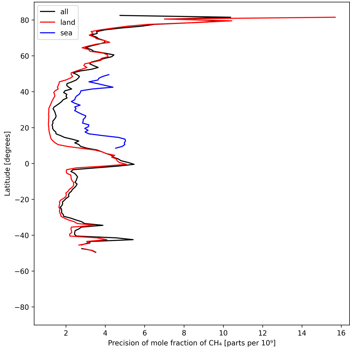
Figure 13: Zonal average of “Precision of mole fraction of CH 4 ” for 2025-06-24 to 2025-06-26.
