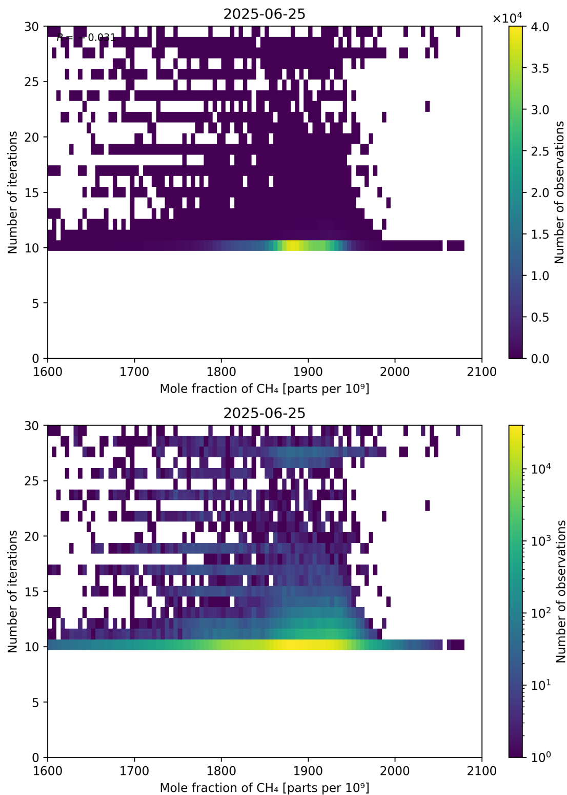
Figure 76: Scatter density plot of “Mole fraction of CH 4 ” against “Number of iterations” for 2025-06-24 to 2025-06-26.
