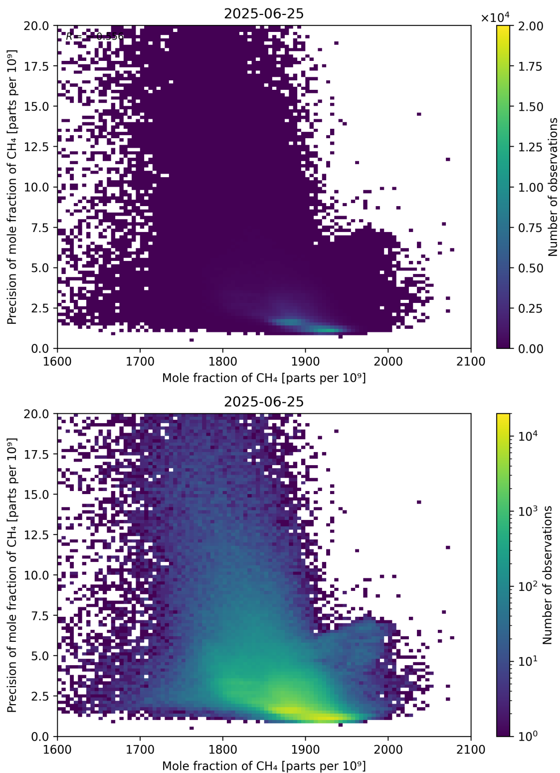
Figure 75: Scatter density plot of “Mole fraction of CH 4 ” against “Precision of mole fraction of CH 4 ” for 2025-06-24 to 2025-06-26.
