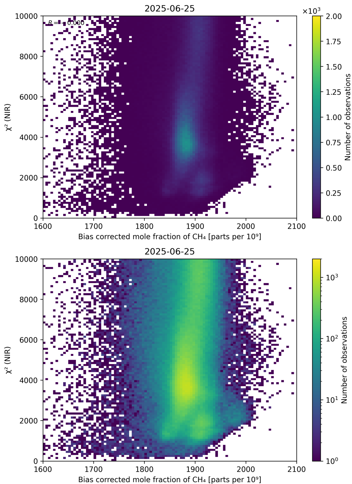
Figure 63: Scatter density plot of “Bias corrected mole fraction of CH 4 ” against “ \chi^2 (NIR)” for 2025-06-24 to 2025-06-26.
