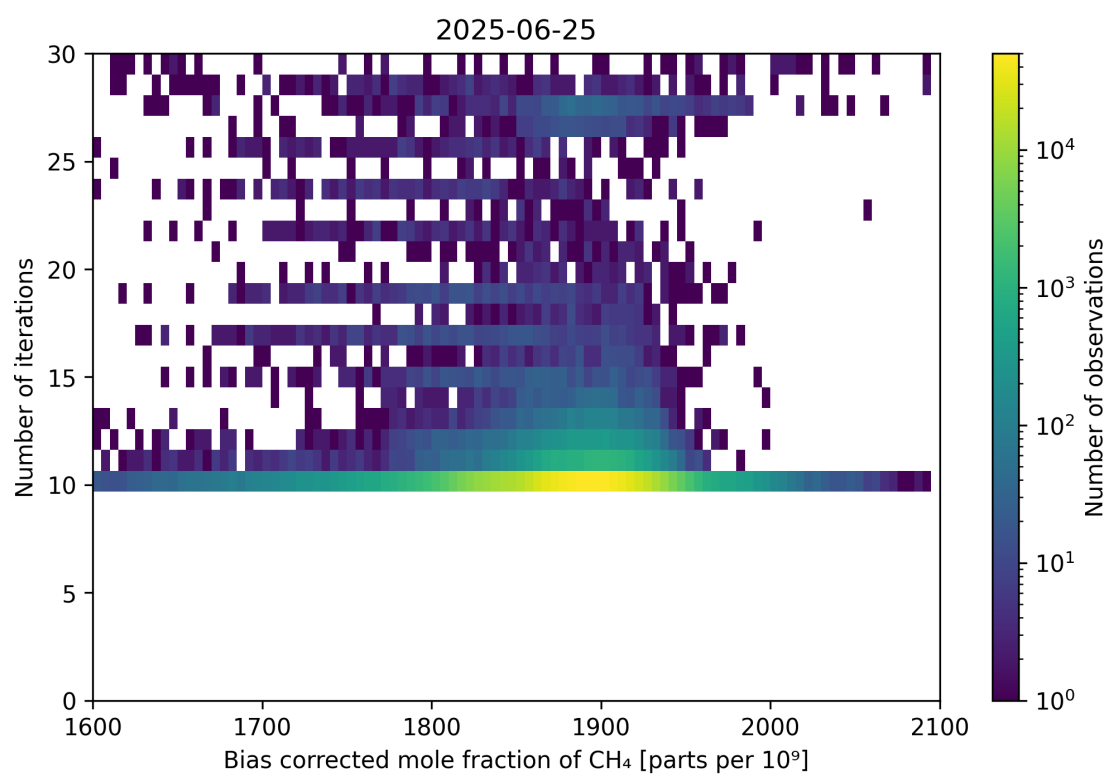
Figure 67: Scatter density plot of “Bias corrected mole fraction of CH 4 ” against “Number of iterations” for 2025-06-24 to 2025-06-26.
