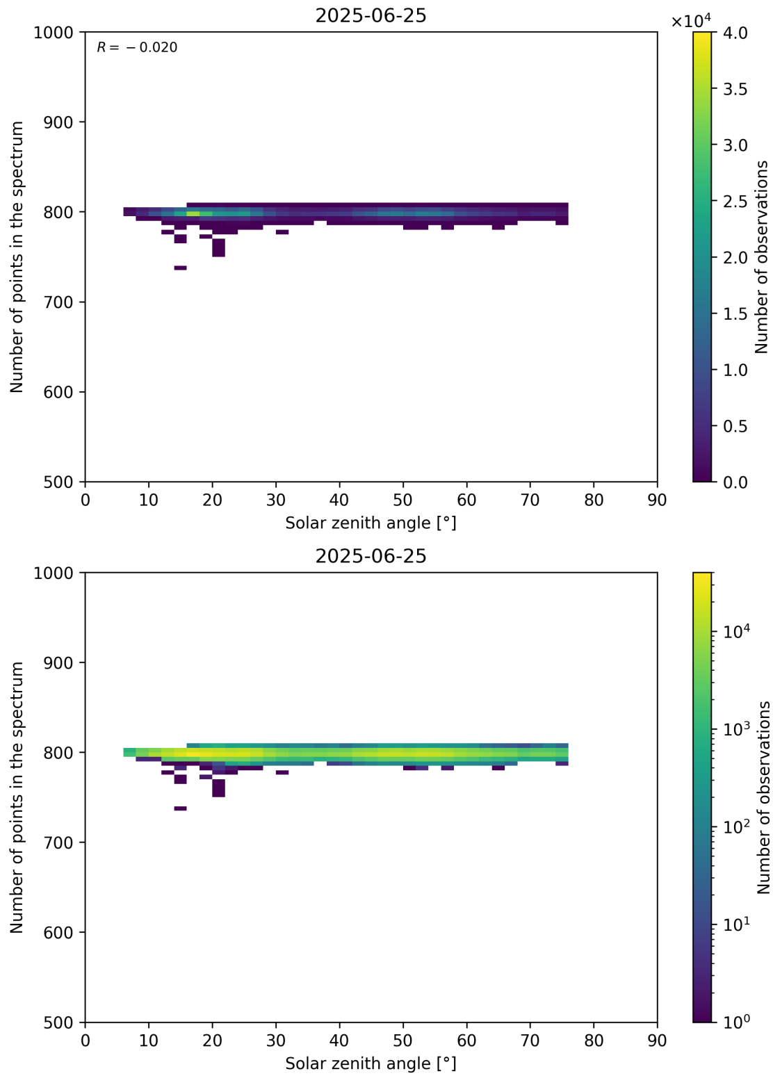
Figure 103: Scatter density plot of “Solar zenith angle” against “Number of points in the spectrum” for 2025-06-24 to 2025-06-26.
