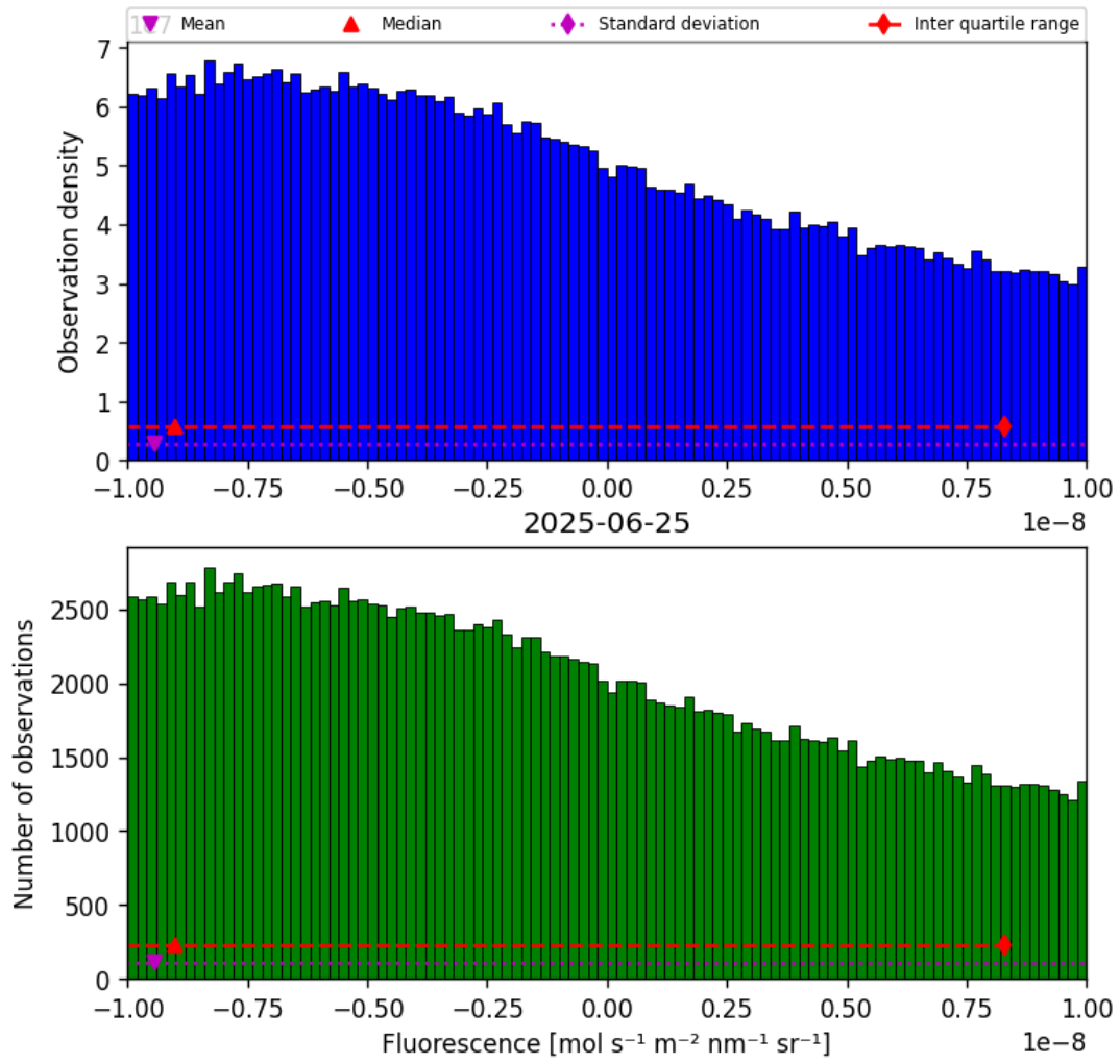
Figure 32: Histogram of “Fluorescence” for 2025-06-24 to 2025-06-26
