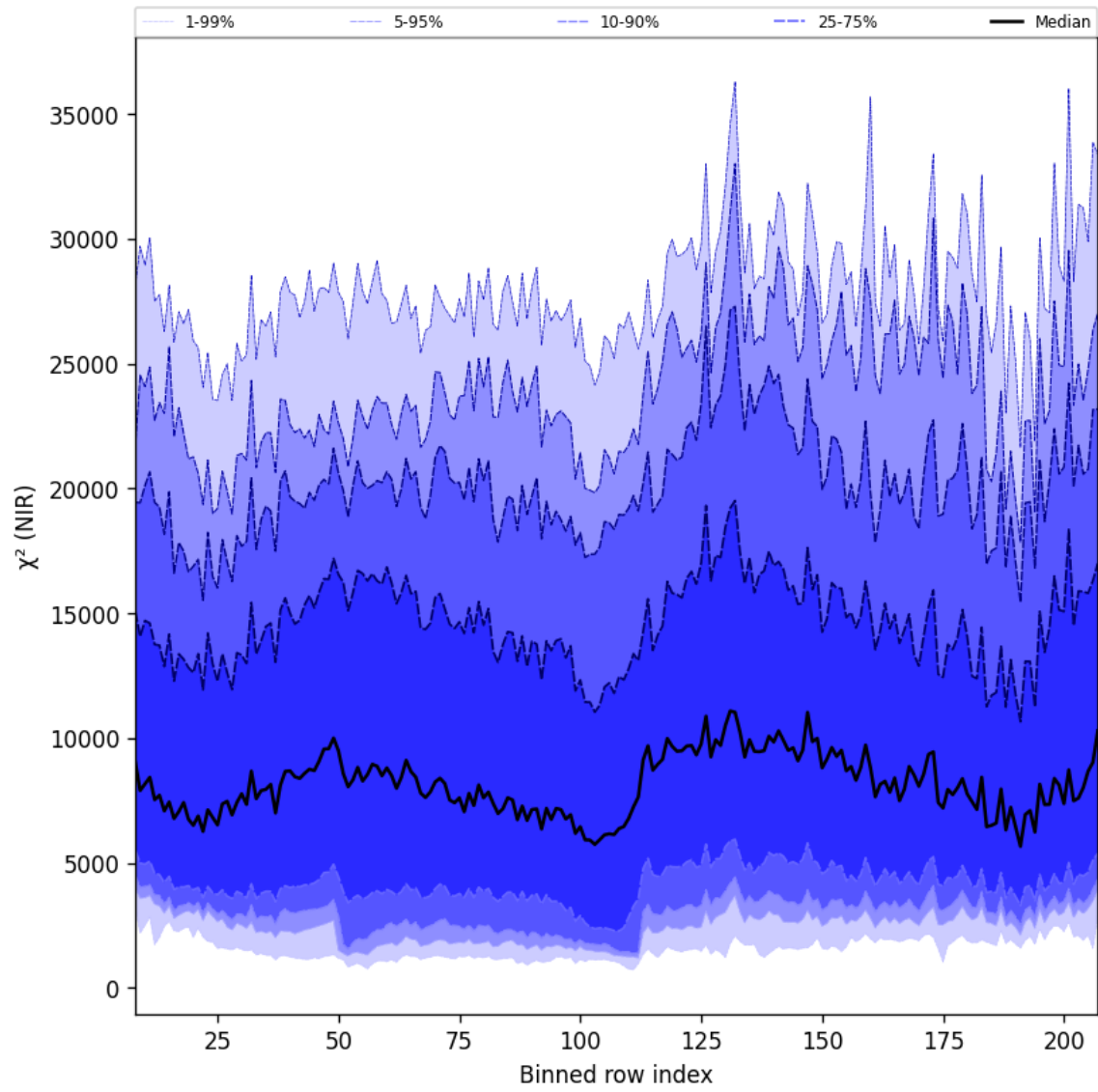
Figure 40: Along track statistics of “ \chi^2 (NIR)” for 2025-06-24 to 2025-06-26
