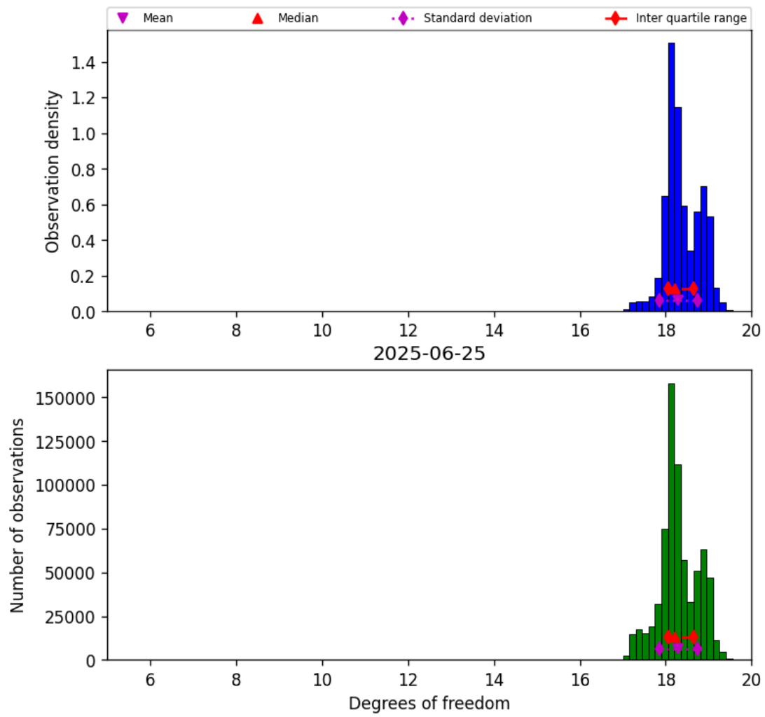
Figure 30: Histogram of “Degrees of freedom” for 2025-06-24 to 2025-06-26
