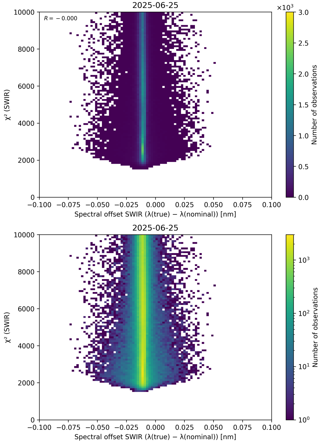
Figure 118: Scatter density plot of “Spectral offset SWIR ( \lambda_{\text{true}} - \lambda_{\text{nominal}} )” against “ \chi^2 (SWIR)” for 2025-06-24 to 2025-06-26.
