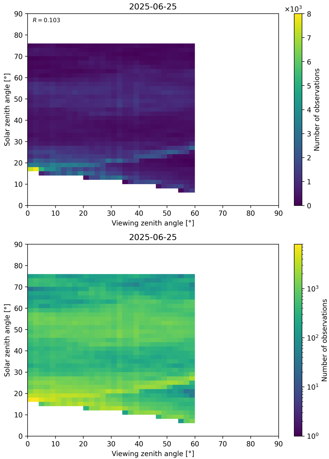
Figure 115: Scatter density plot of “Viewing zenith angle” against “Solar zenith angle” for 2025-06-24 to 2025-06-26.
