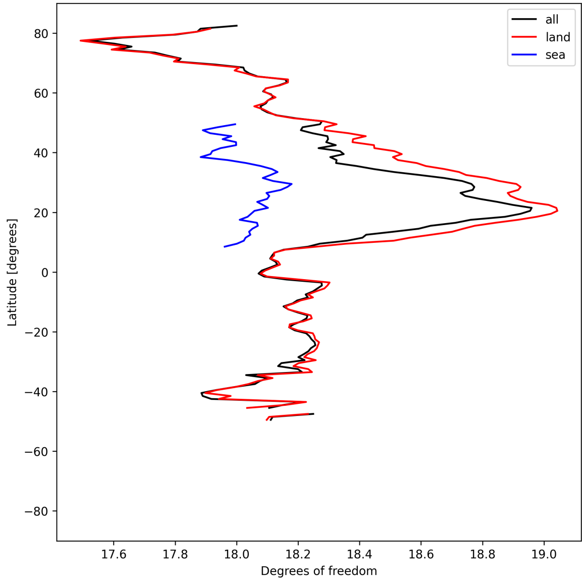
Figure 19: Zonal average of “Degrees of freedom” for 2025-06-24 to 2025-06-26.
