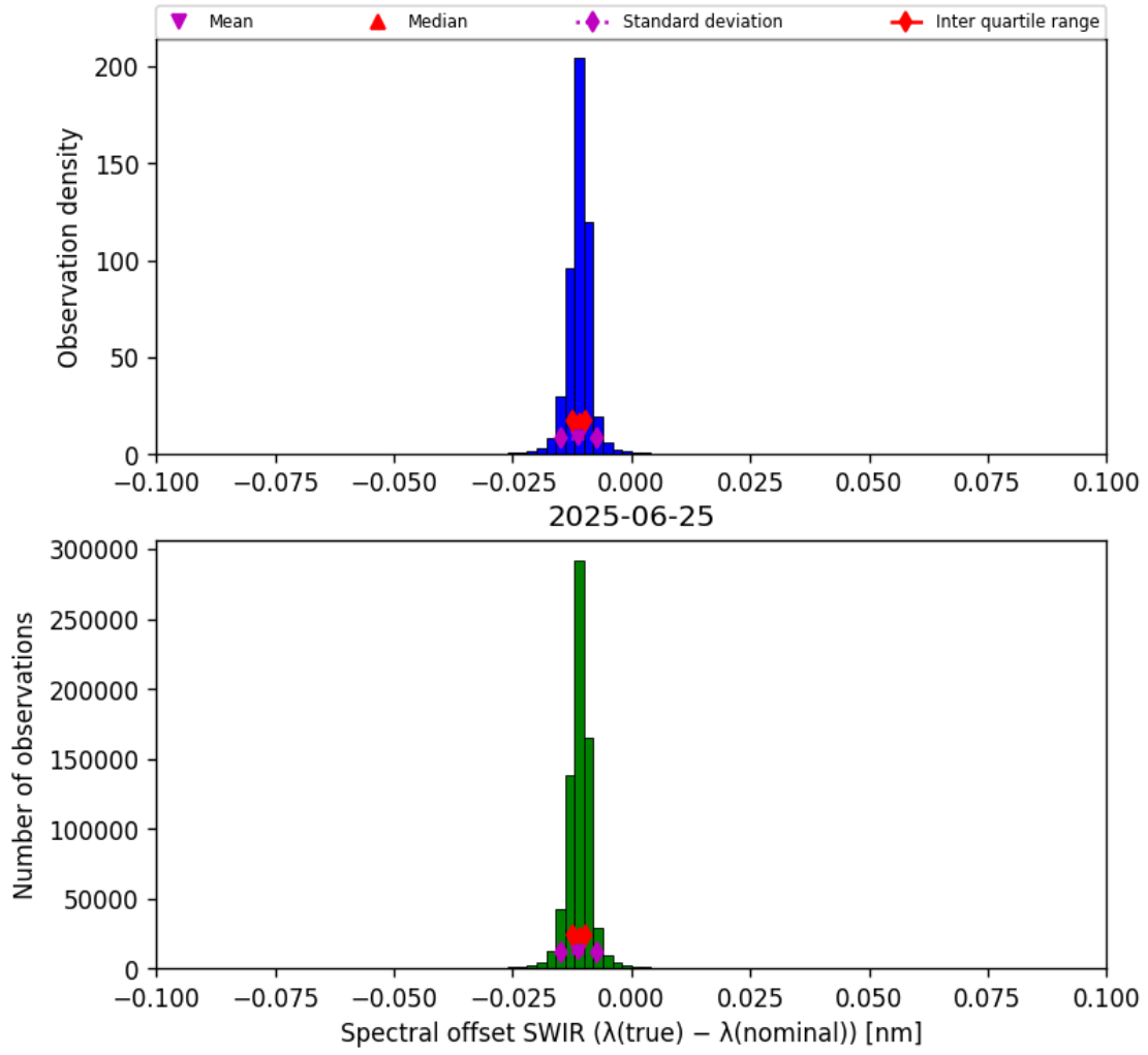
Figure 27: Histogram of “Spectral offset SWIR ( \lambda_{\text{true}} - \lambda_{\text{nominal}} )” for 2025-06-24 to 2025-06-26
