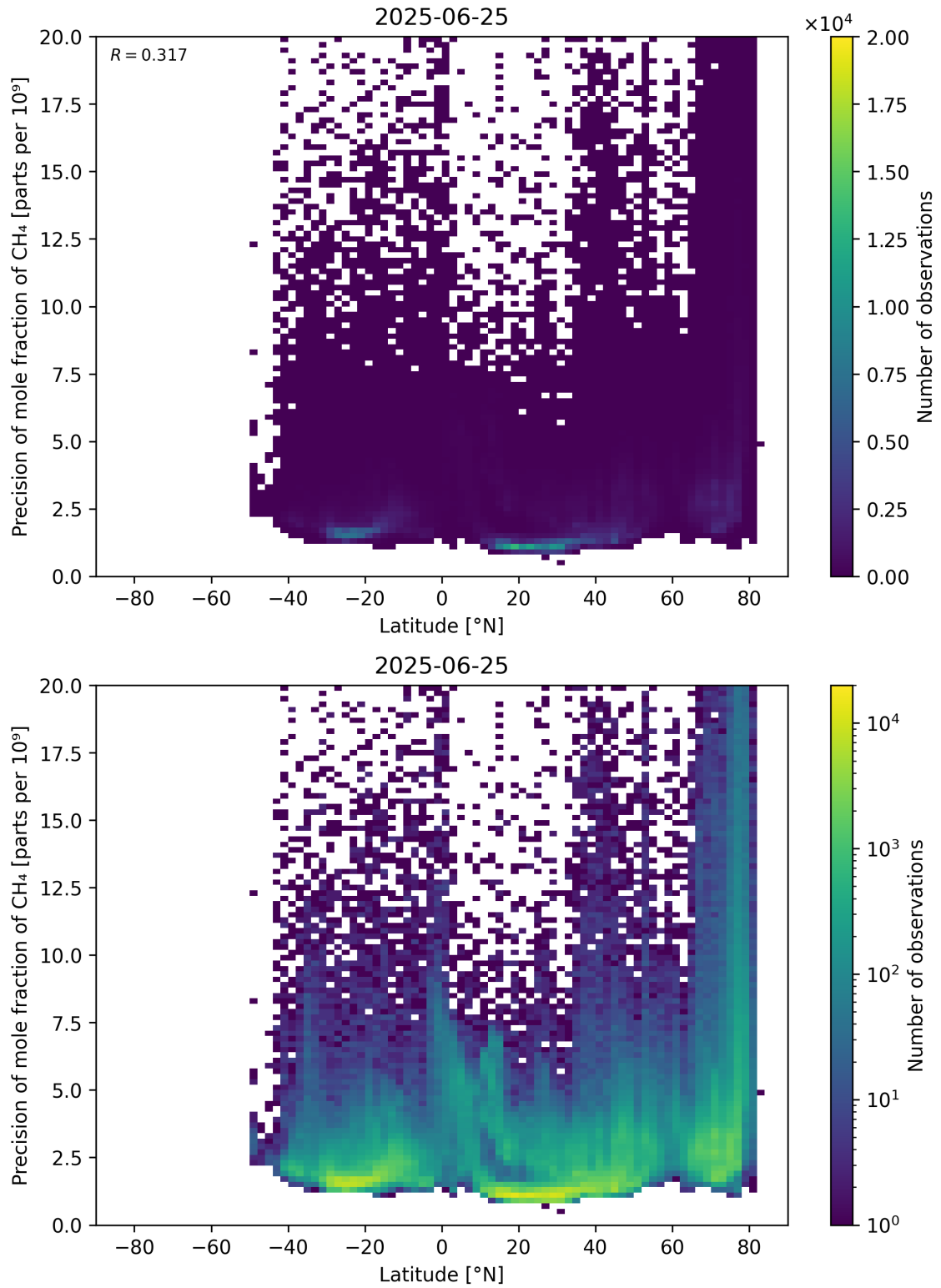
Figure 59: Scatter density plot of “Latitude” against “Precision of mole fraction of CH 4 ” for 2025-06-24 to 2025-06-26.
