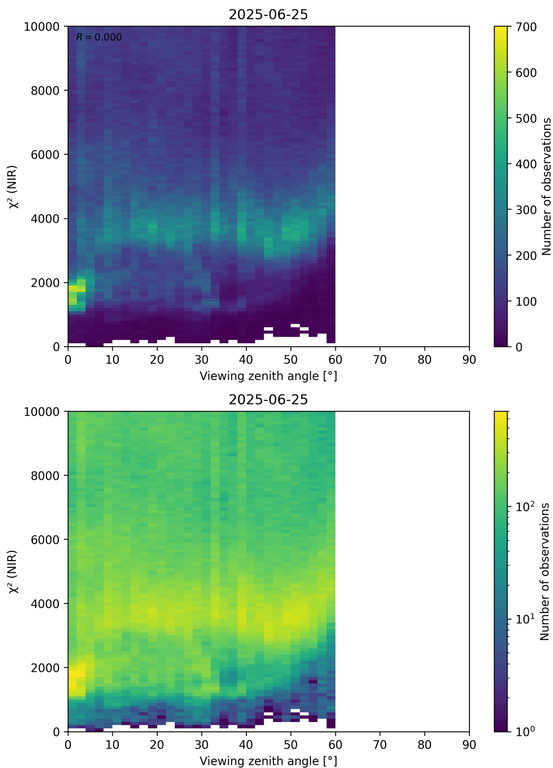
Figure 105: Scatter density plot of “Viewing zenith angle” against “ \chi^2 (NIR)” for 2025-06-24 to 2025-06-26.
