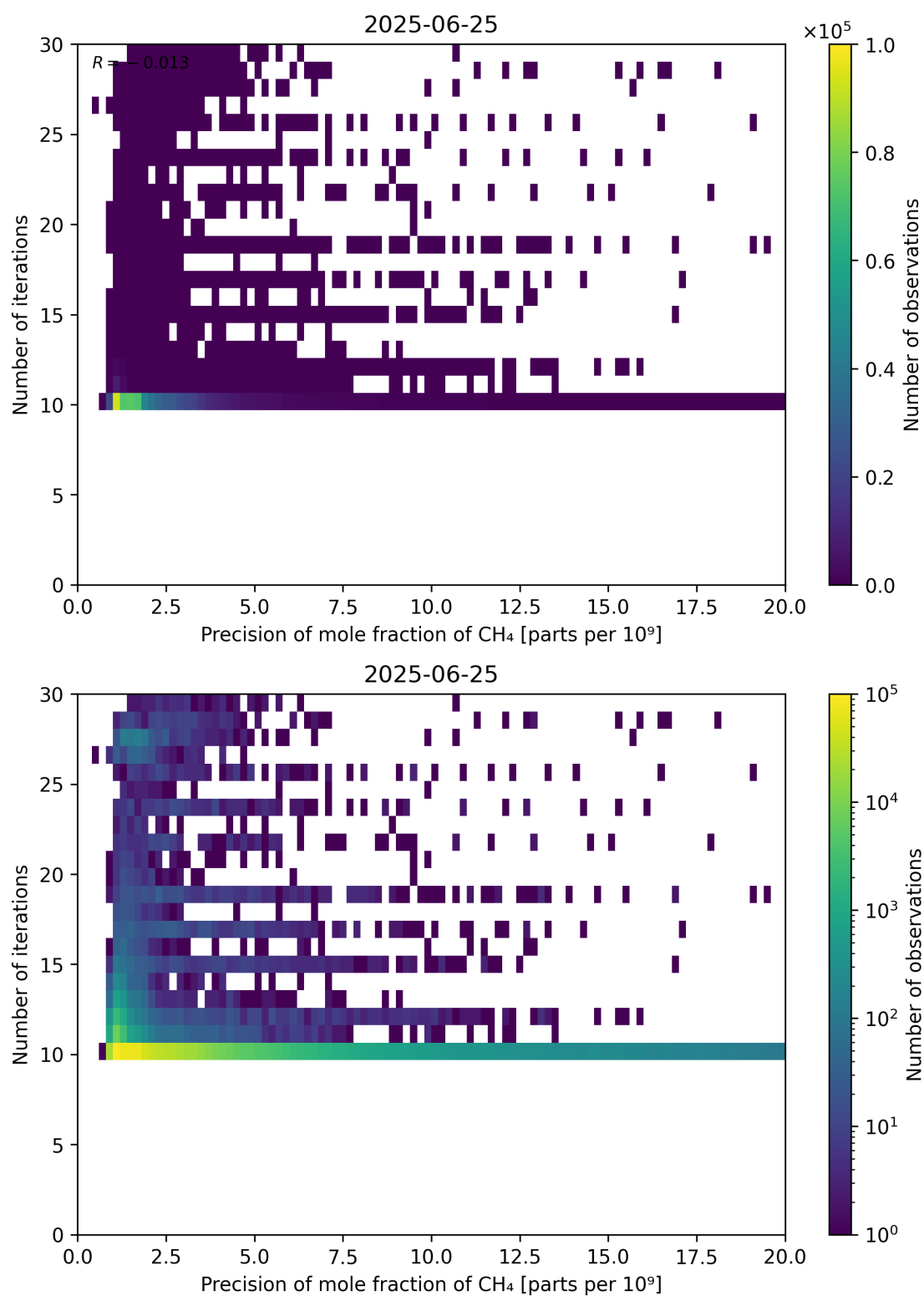
Figure 83: Scatter density plot of “Precision of mole fraction of CH 4 ” against “Number of iterations” for 2025-06-24 to 2025-06-26.
