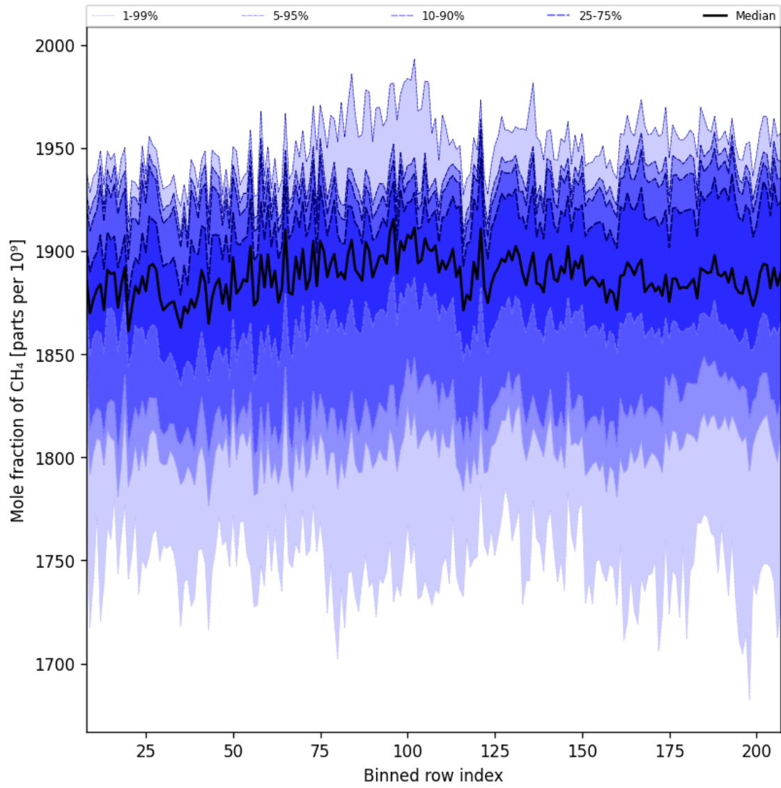
Figure 34: Along track statistics of “Mole fraction of CH 4 ” for 2025-06-24 to 2025-06-26
