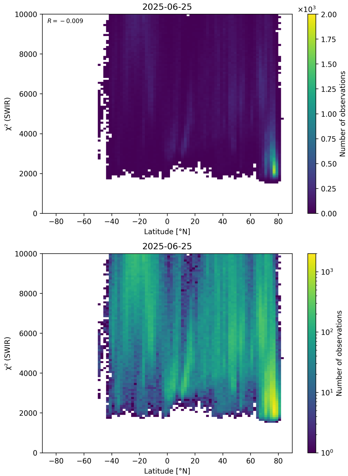
Figure 54: Scatter density plot of “Latitude” against “ \chi^2 (SWIR)” for 2025-06-24 to 2025-06-26.
