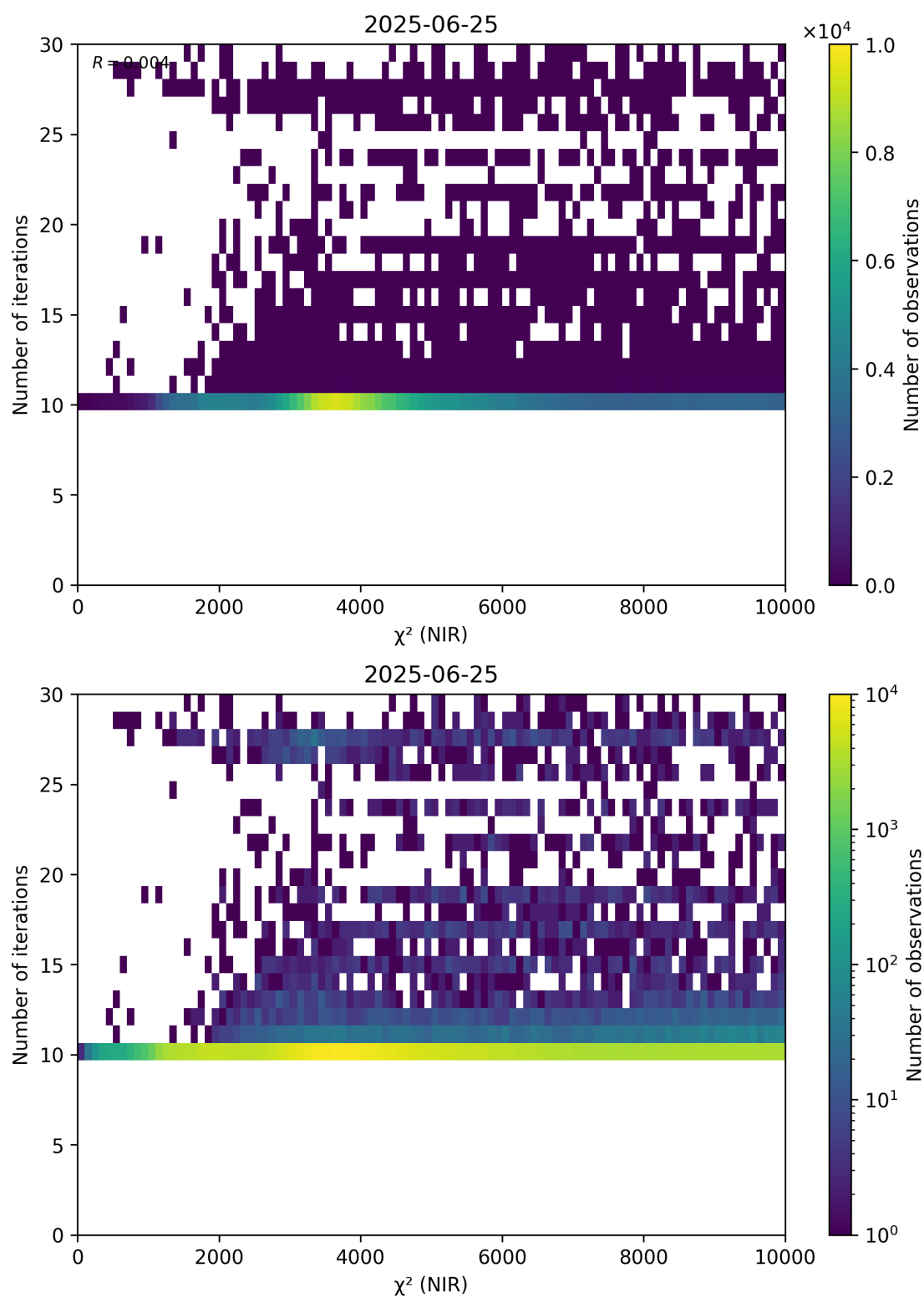
Figure 46: Scatter density plot of “ \chi^2 (NIR)” against “Number of iterations” for 2025-06-24 to 2025-06-26.
