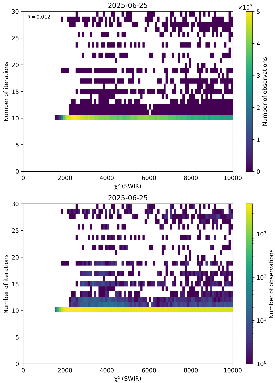
Figure 50: Scatter density plot of “ \chi^2 (SWIR)” against “Number of iterations” for 2025-06-24 to 2025-06-26.
