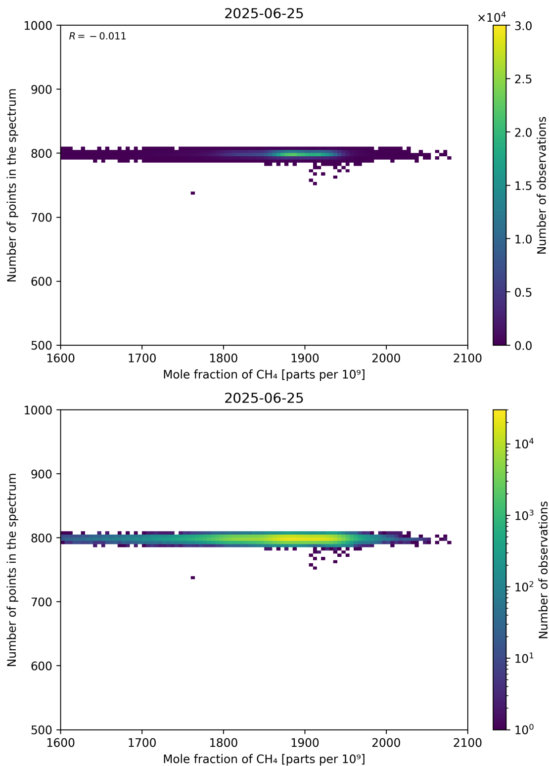
Figure 77: Scatter density plot of “Mole fraction of CH 4 ” against “Number of points in the spectrum” for 2025-06-24 to 2025-06-26.
