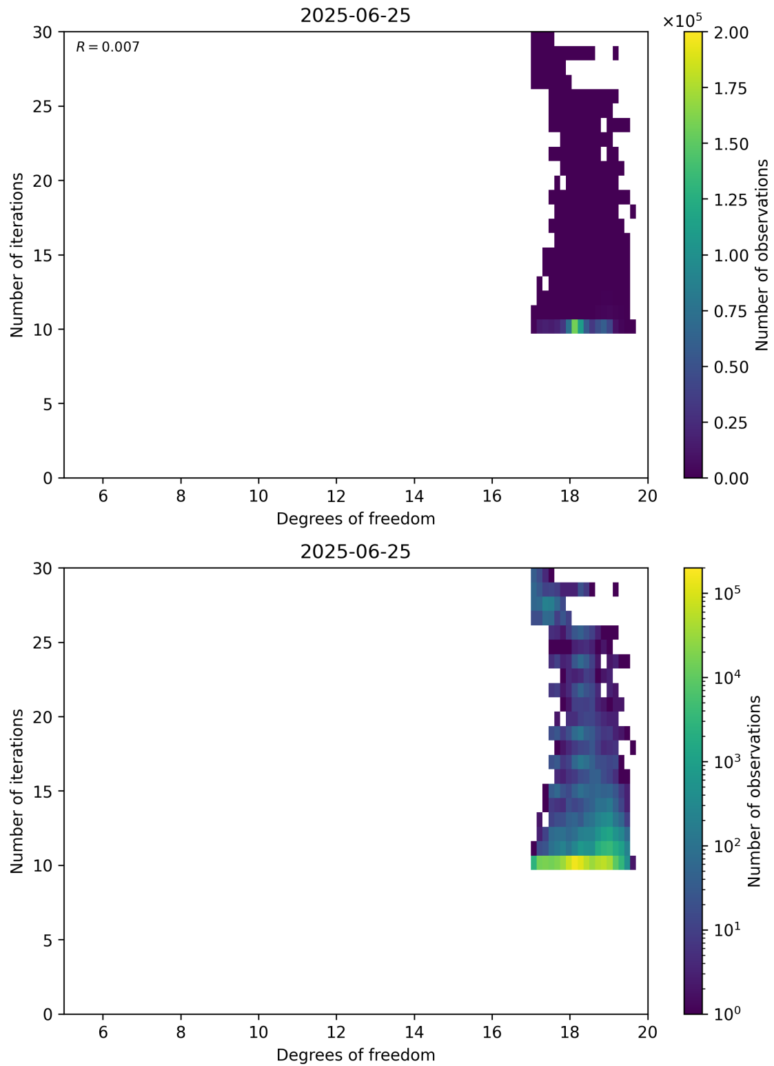
Figure 52: Scatter density plot of “Degrees of freedom” against “Number of iterations” for 2025-06-24 to 2025-06-26.
