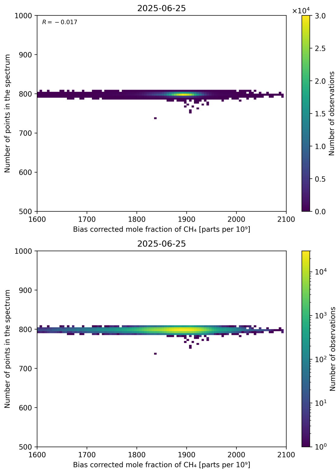
Figure 68: Scatter density plot of “Bias corrected mole fraction of CH 4 ” against “Number of points in the spectrum” for 2025-06-24 to 2025-06-26.
