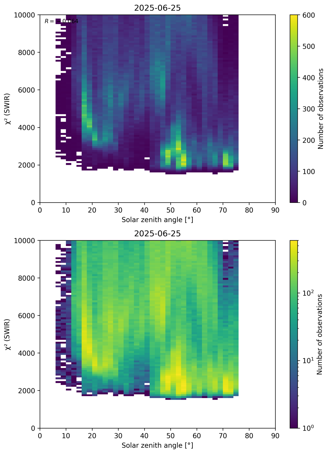
Figure 95: Scatter density plot of “Solar zenith angle” against “ \chi^2 (SWIR)” for 2025-06-24 to 2025-06-26.
