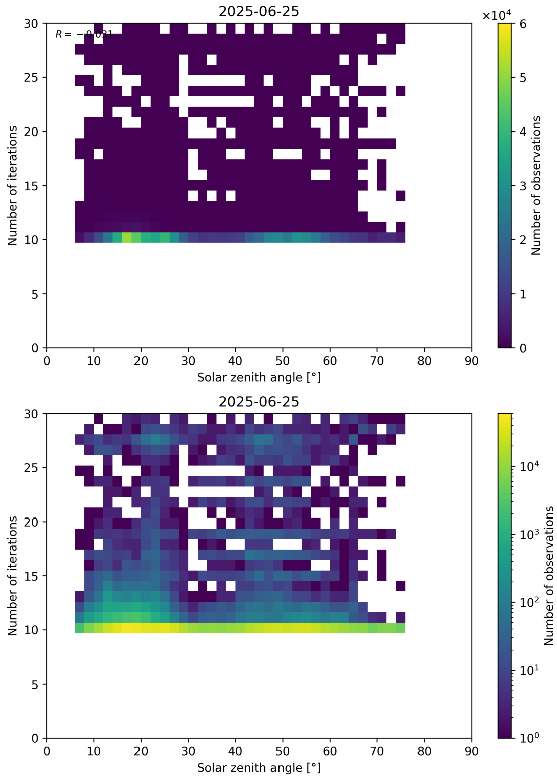
Figure 102: Scatter density plot of “Solar zenith angle” against “Number of iterations” for 2025-06-24 to 2025-06-26.
