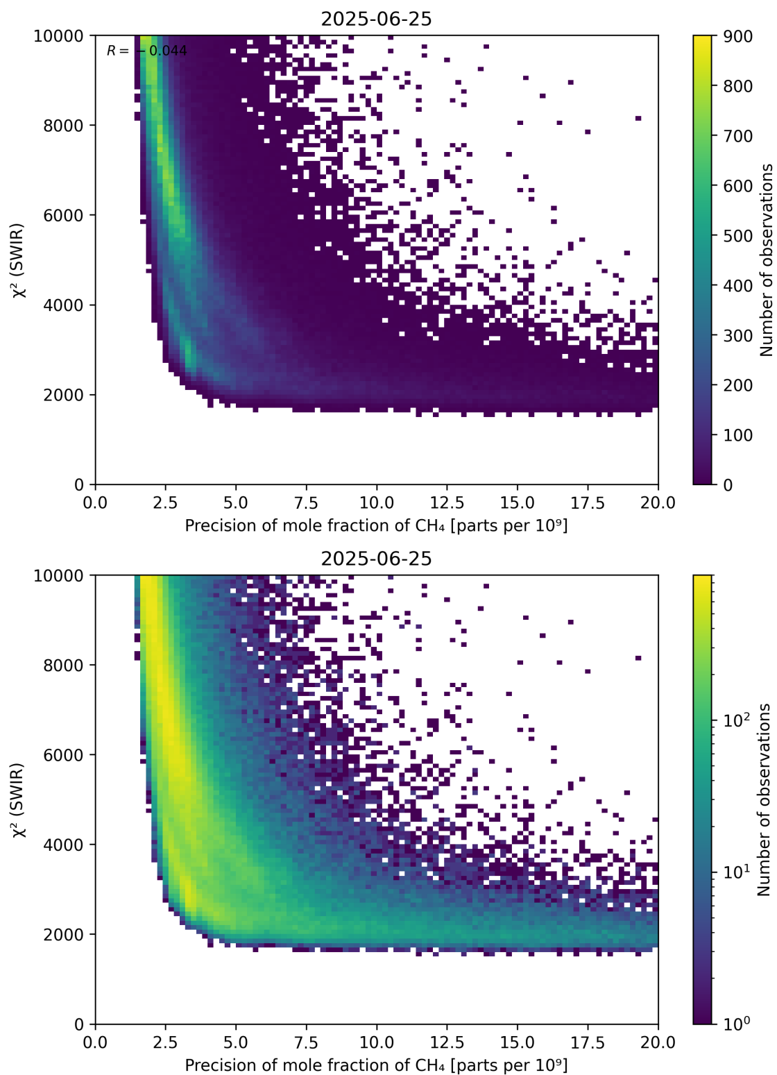
Figure 79: Scatter density plot of “Precision of mole fraction of CH 4 ” against “ \chi^2 (SWIR)” for 2025-06-24 to 2025-06-26.
