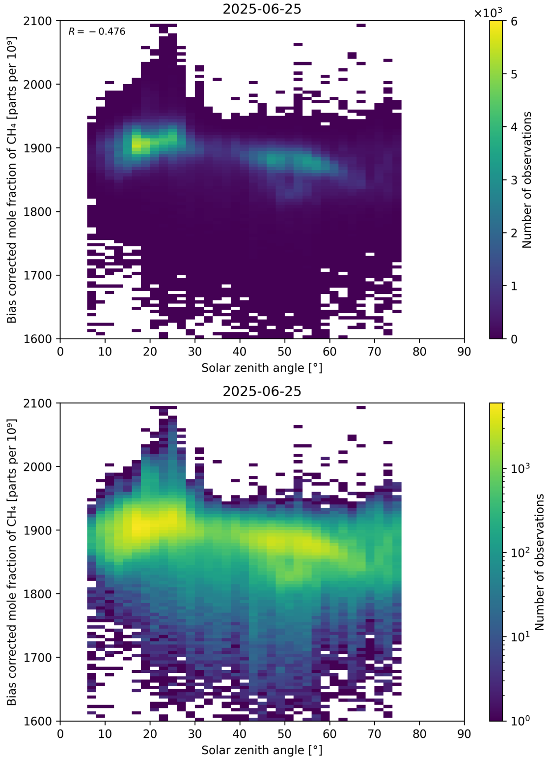
Figure 100: Scatter density plot of “Solar zenith angle” against “Bias corrected mole fraction of \text{CH}_4 ” for 2025-06-24 to 2025-06-26.
