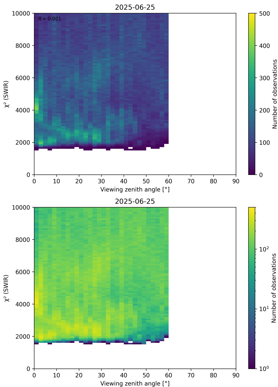
Figure 106: Scatter density plot of “Viewing zenith angle” against “ \chi^2 (SWIR)” for 2025-06-24 to 2025-06-26.
