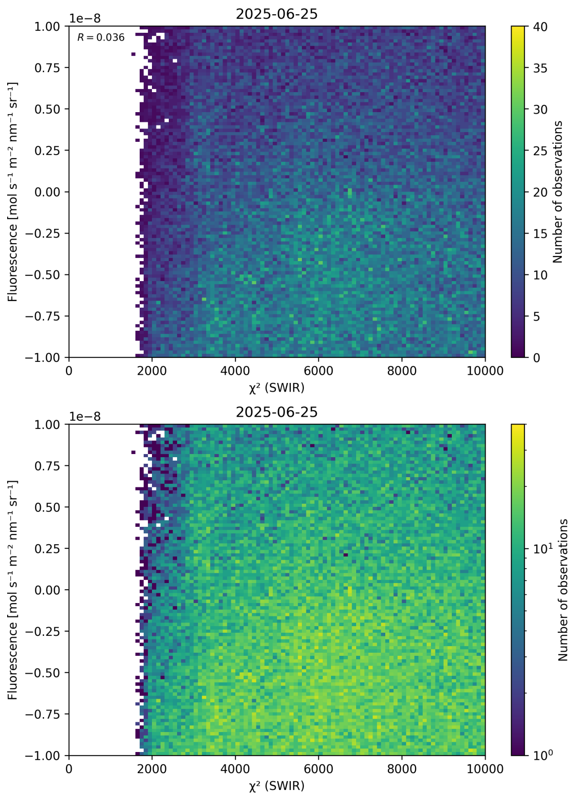
Figure 49: Scatter density plot of “ \chi^2 (SWIR)” against “Fluorescence” for 2025-06-24 to 2025-06-26.
