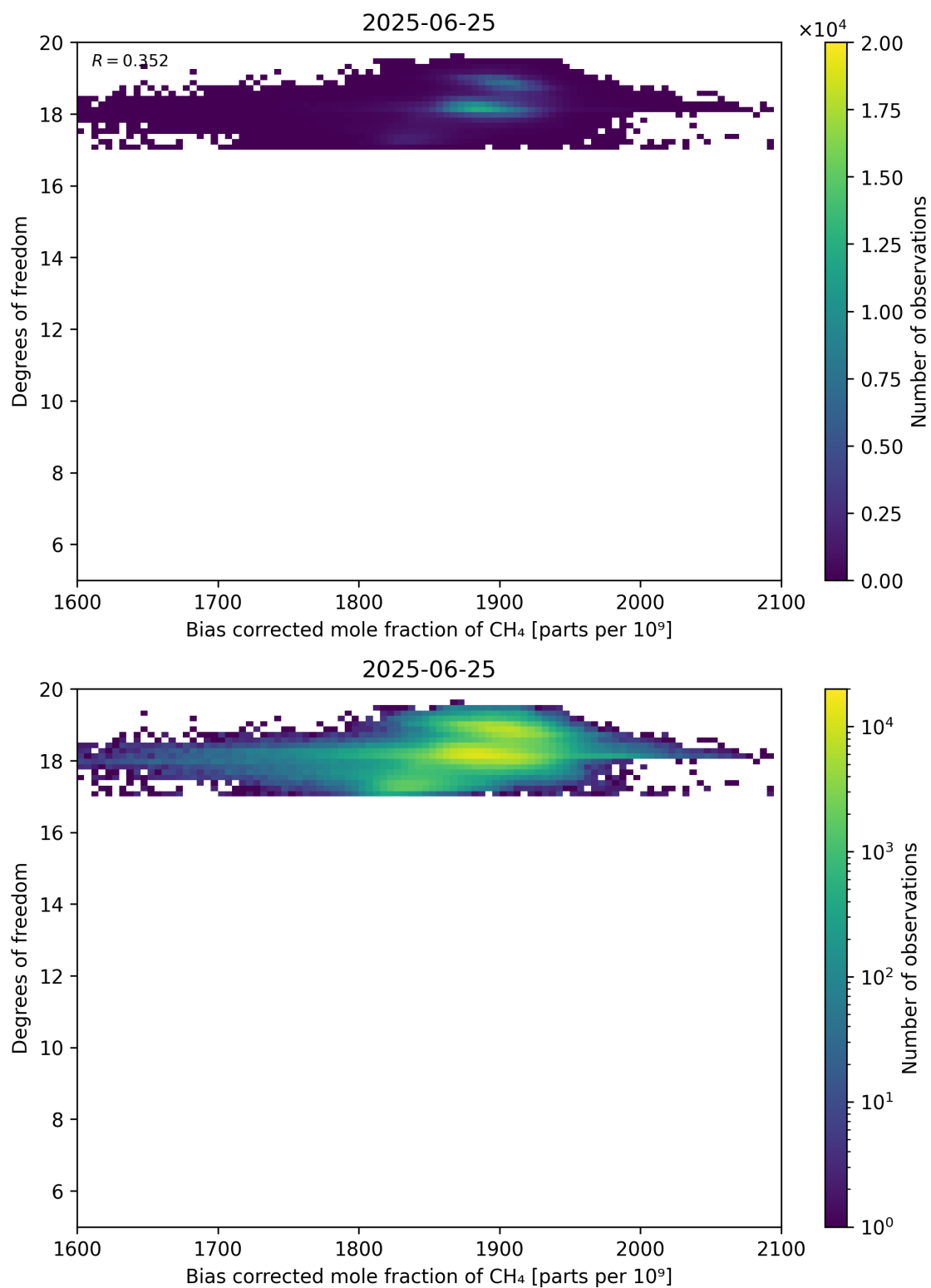
Figure 65: Scatter density plot of “Bias corrected mole fraction of CH 4 ” against “Degrees of freedom” for 2025-06-24 to 2025-06-26.
