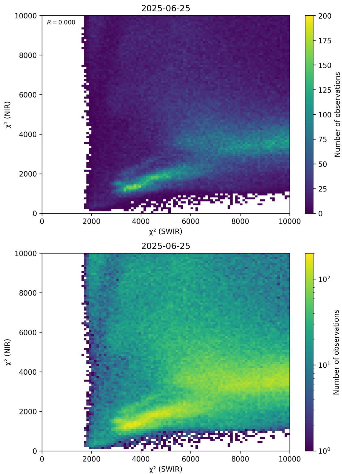
Figure 47: Scatter density plot of “ \chi^2 (SWIR)” against “ \chi^2 (NIR)” for 2025-06-24 to 2025-06-26.
