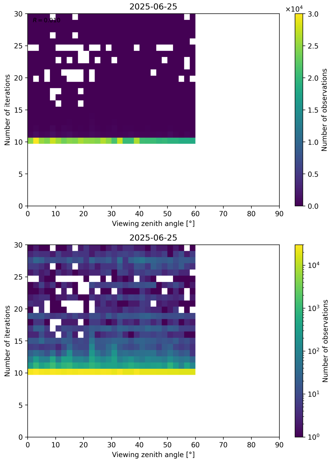
Figure 113: Scatter density plot of “Viewing zenith angle” against “Number of iterations” for 2025-06-24 to 2025-06-26.
