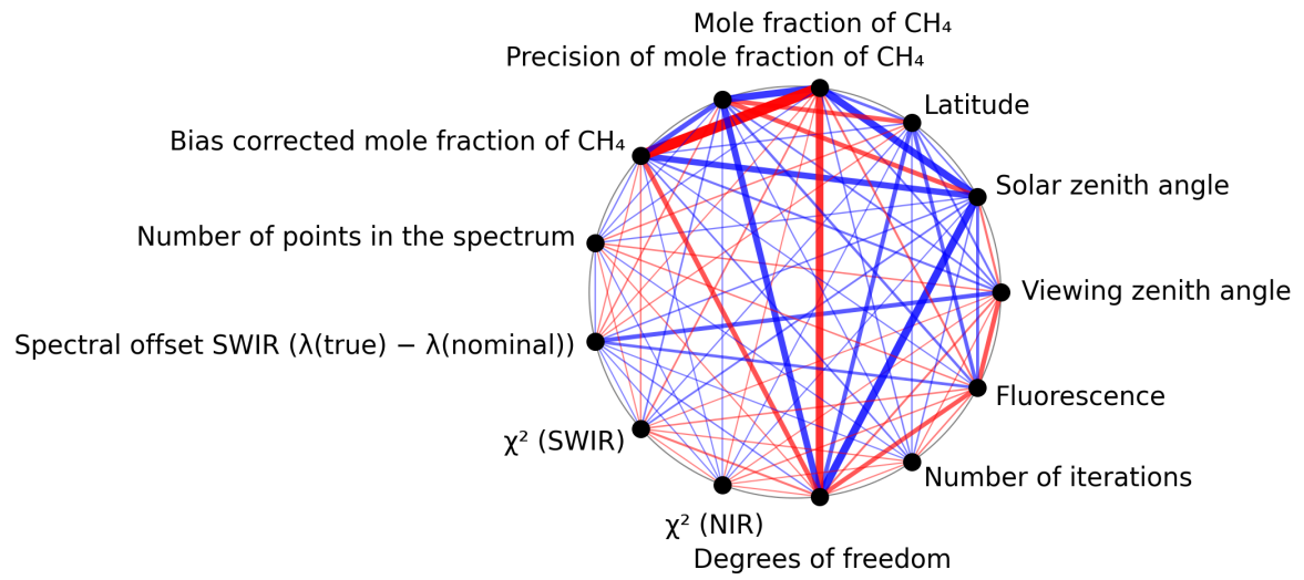
Figure 1: Map of correlation graph for 2025-06-24 to 2025-06-26.
