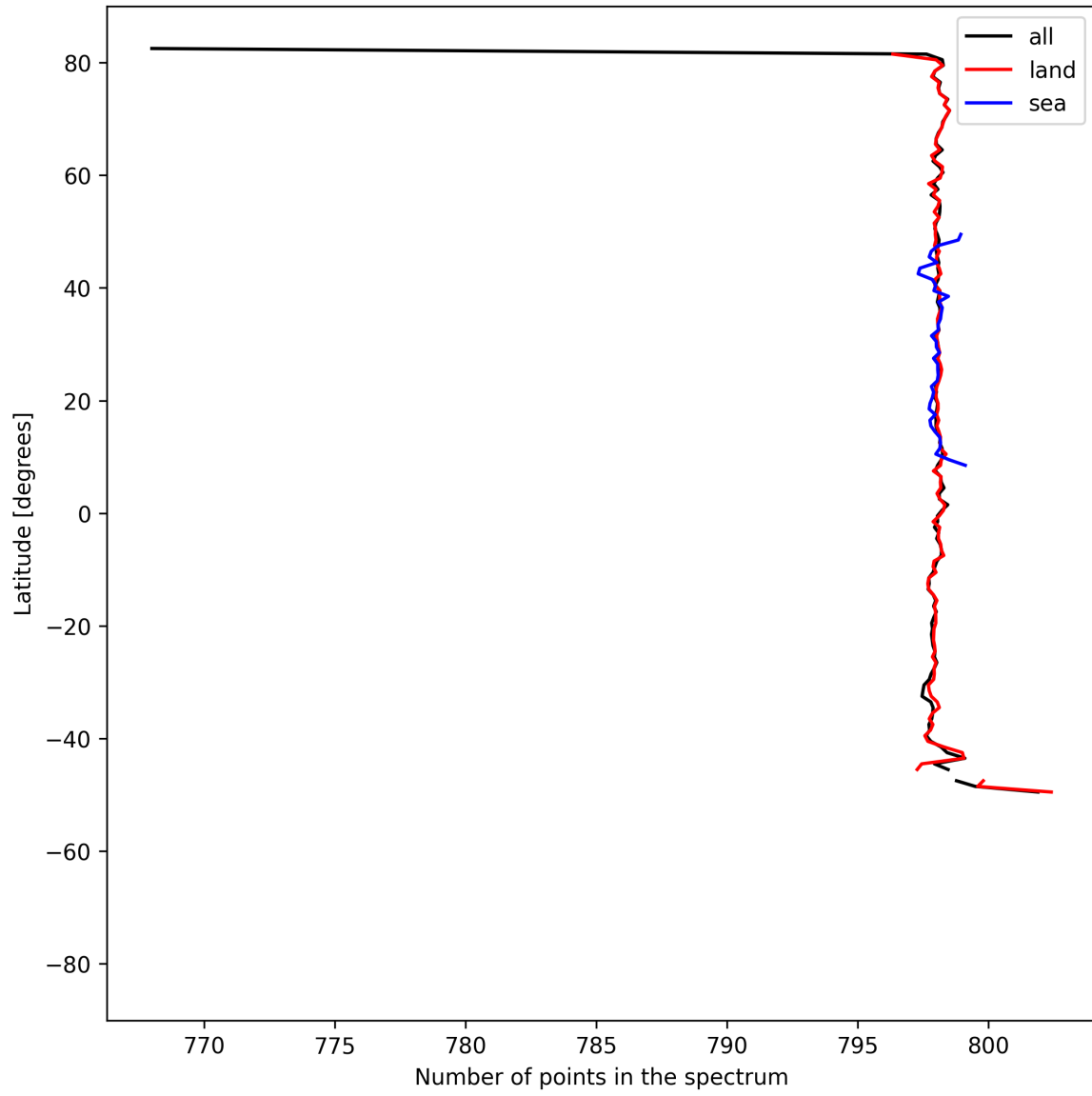
Figure 15: Zonal average of “Number of points in the spectrum” for 2025-06-24 to 2025-06-26.
