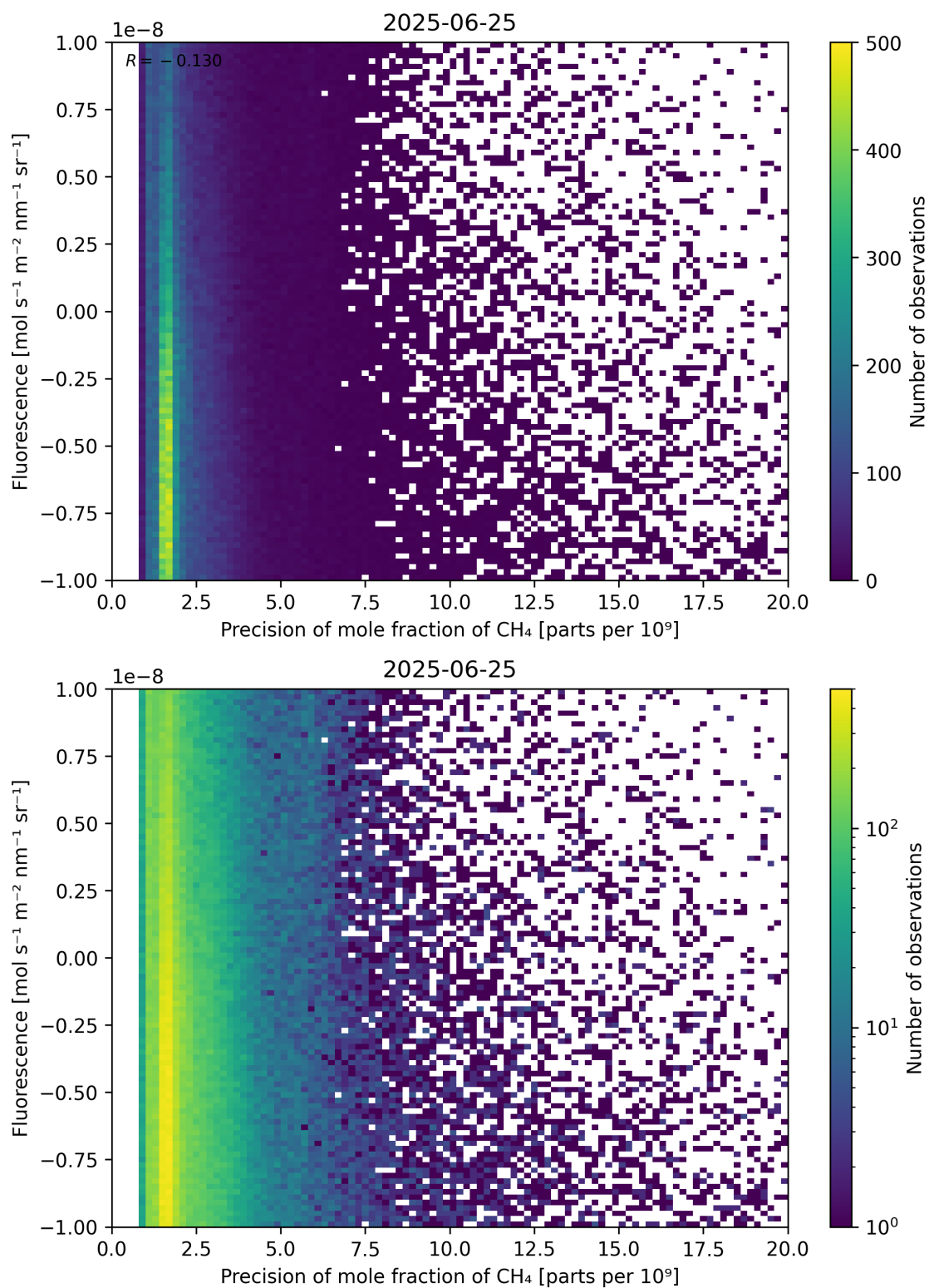
Figure 81: Scatter density plot of “Precision of mole fraction of \text{CH}_4 ” against “Fluorescence” for 2025-06-24 to 2025-06-26.
