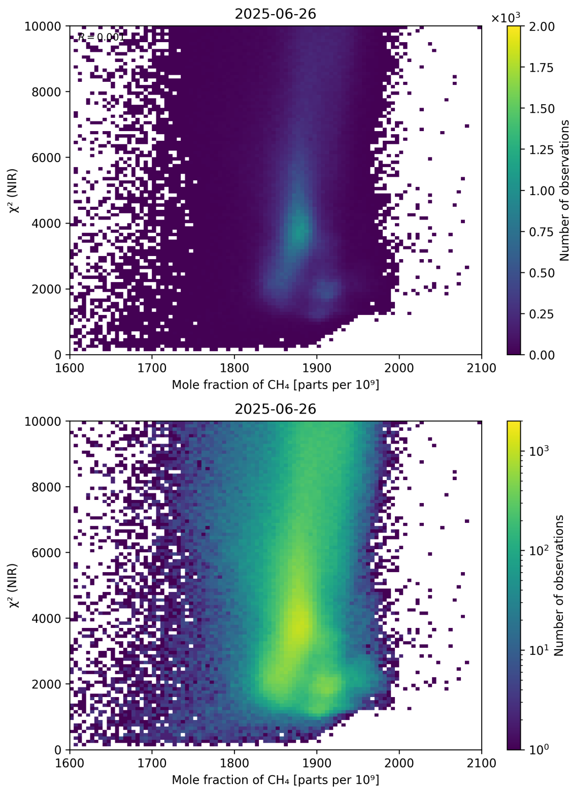
Figure 70: Scatter density plot of “Mole fraction of \text{CH}_4 ” against “ \chi^2 (NIR)” for 2025-06-25 to 2025-06-27.
