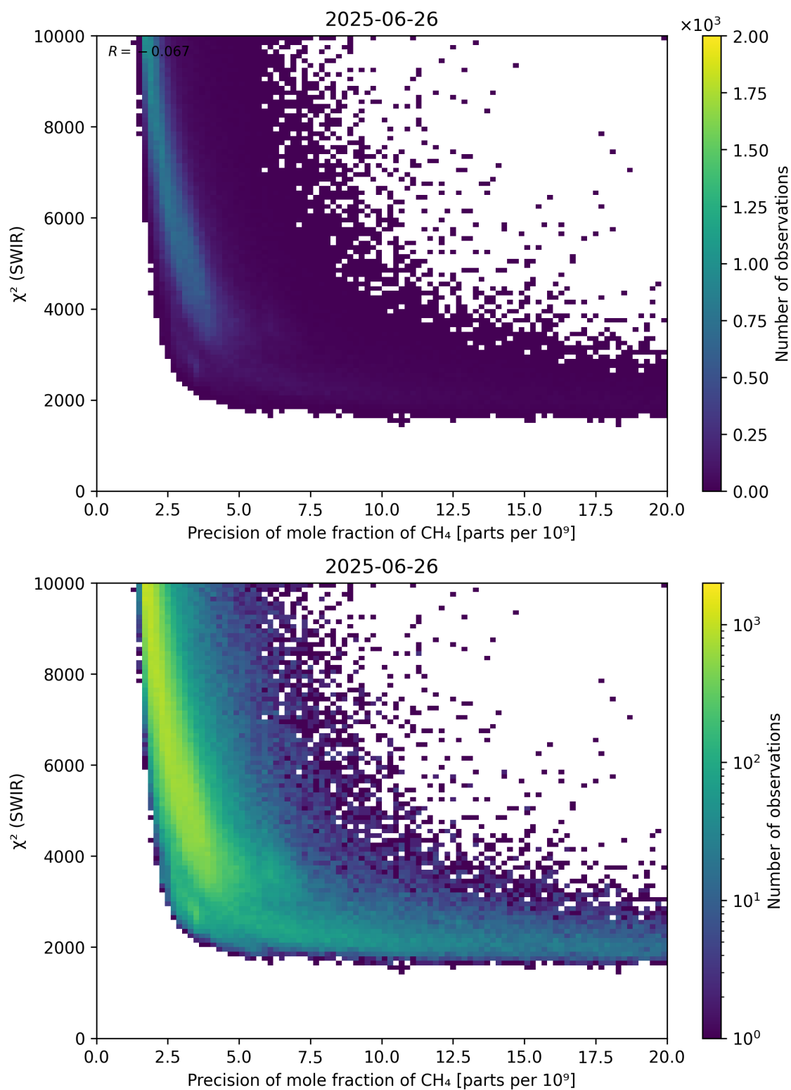
Figure 79: Scatter density plot of “Precision of mole fraction of \text{CH}_4 ” against “ \chi^2 (SWIR)” for 2025-06-25 to 2025-06-27.
