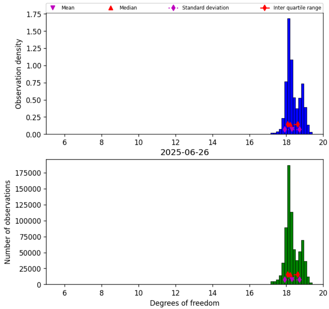
Figure 30: Histogram of “Degrees of freedom” for 2025-06-25 to 2025-06-27
