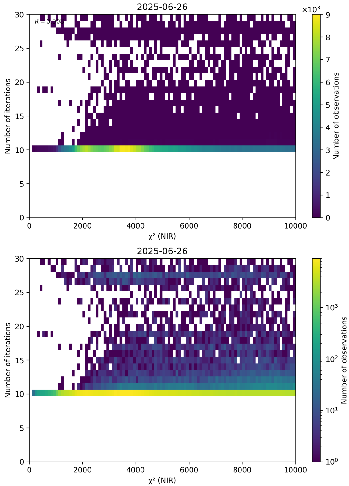
Figure 46: Scatter density plot of “ \chi^2 (NIR)” against “Number of iterations” for 2025-06-25 to 2025-06-27.
