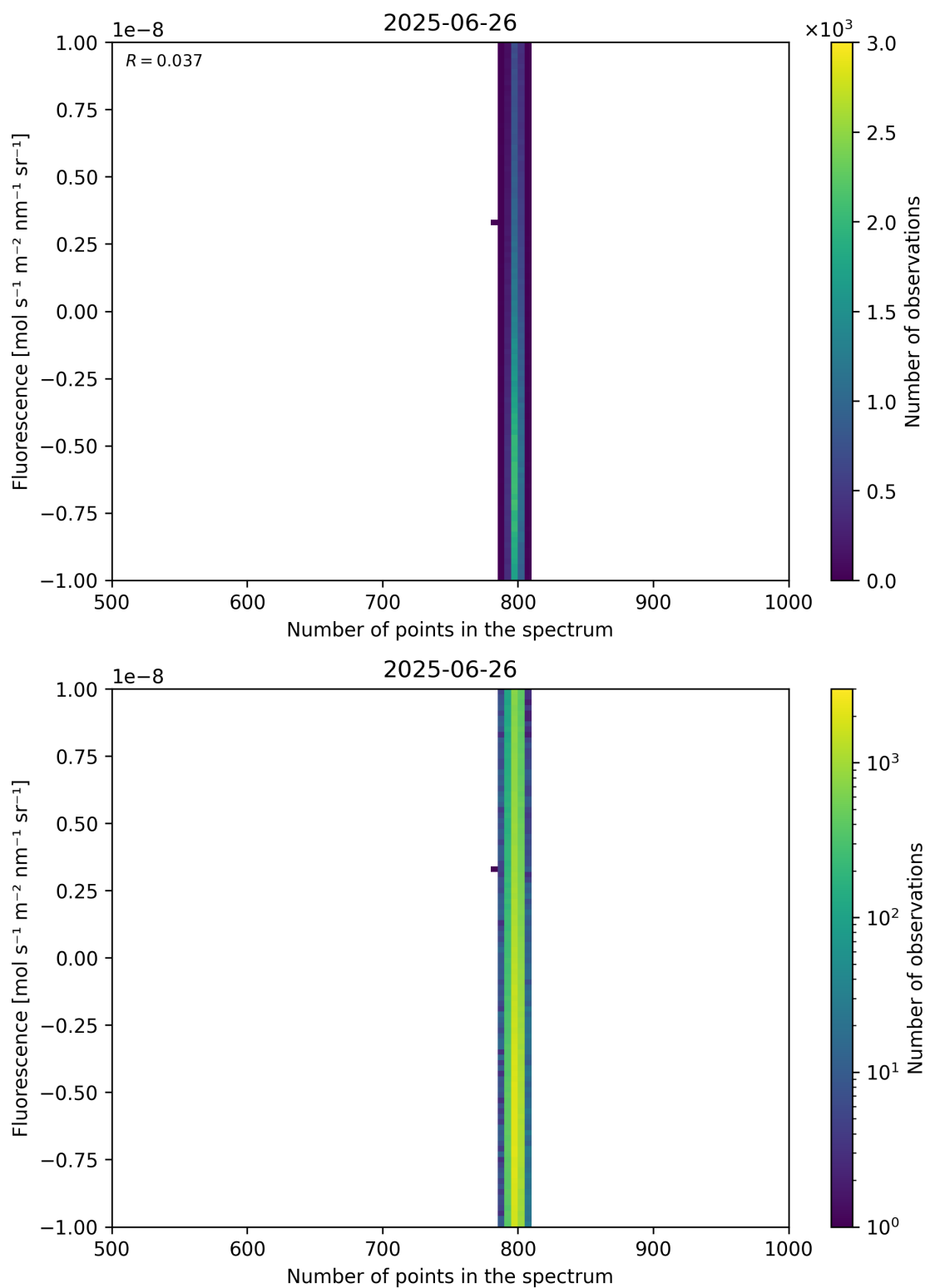
Figure 91: Scatter density plot of “Number of points in the spectrum” against “Fluorescence” for 2025-06-25 to 2025-06-27.
