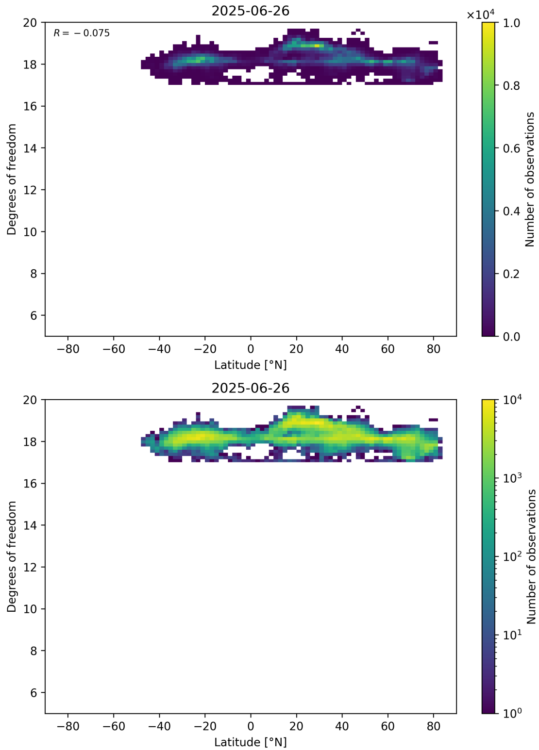
Figure 55: Scatter density plot of “Latitude” against “Degrees of freedom” for 2025-06-25 to 2025-06-27.
