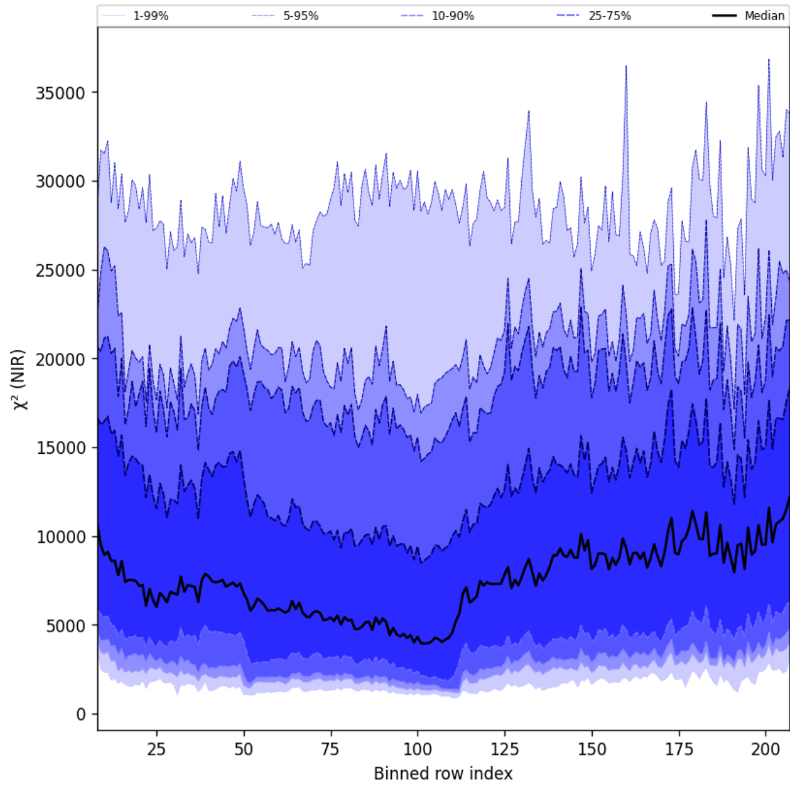
Figure 40: Along track statistics of “ \chi^2 (NIR)” for 2025-06-25 to 2025-06-27
