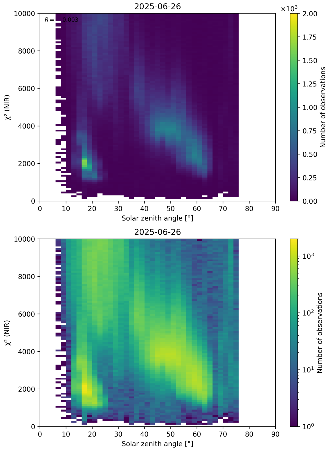
Figure 94: Scatter density plot of “Solar zenith angle” against “ \chi^2 (NIR)” for 2025-06-25 to 2025-06-27.
