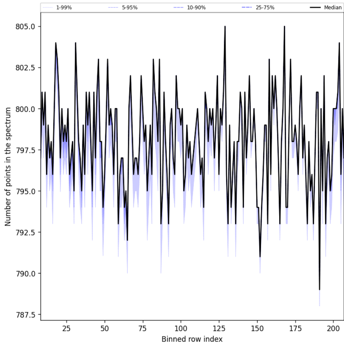
Figure 37: Along track statistics of “Number of points in the spectrum” for 2025-06-25 to 2025-06-27
