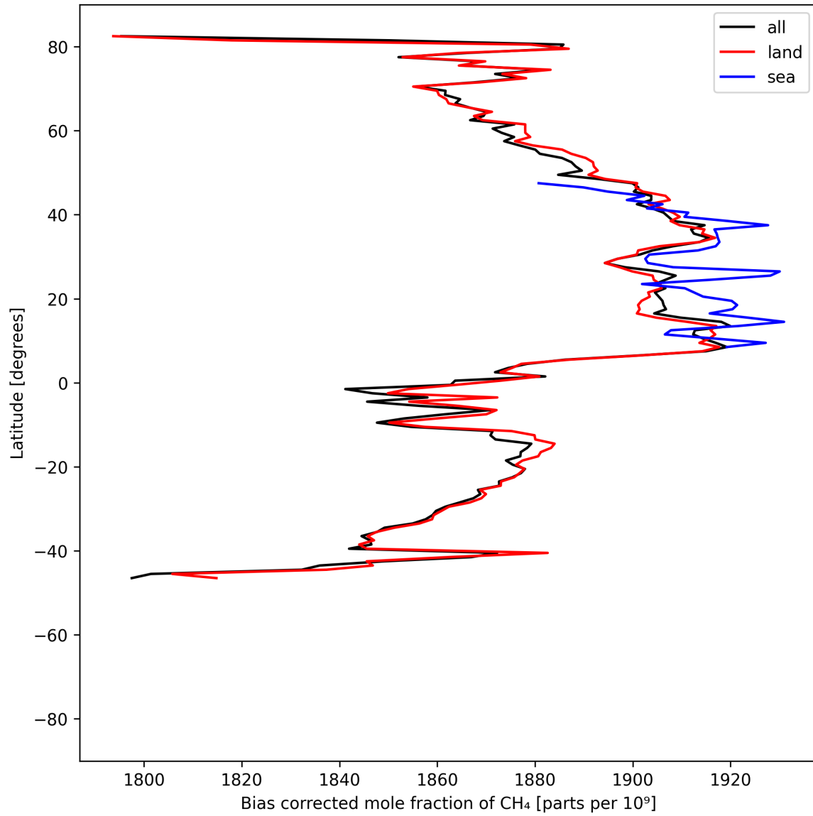
Figure 14: Zonal average of “Bias corrected mole fraction of CH 4 ” for 2025-06-25 to 2025-06-27.
