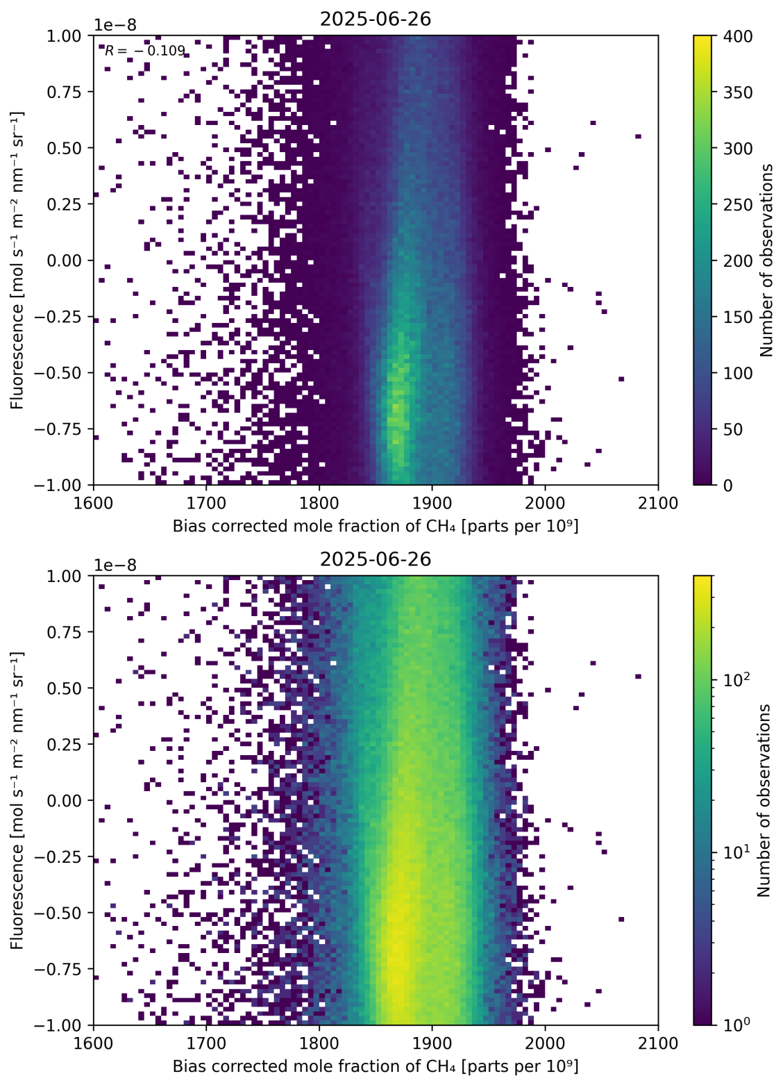
Figure 66: Scatter density plot of “Bias corrected mole fraction of \text{CH}_4 ” against “Fluorescence” for 2025-06-25 to 2025-06-27.
