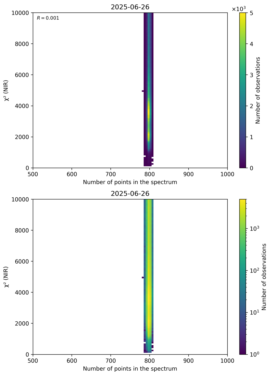
Figure 88: Scatter density plot of “Number of points in the spectrum” against “ \chi^2 (NIR)” for 2025-06-25 to 2025-06-27.
