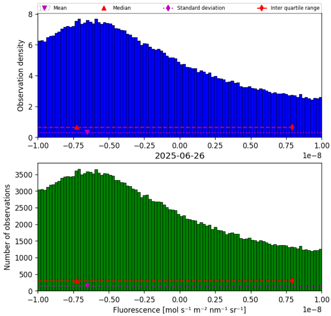
Figure 32: Histogram of “Fluorescence” for 2025-06-25 to 2025-06-27
