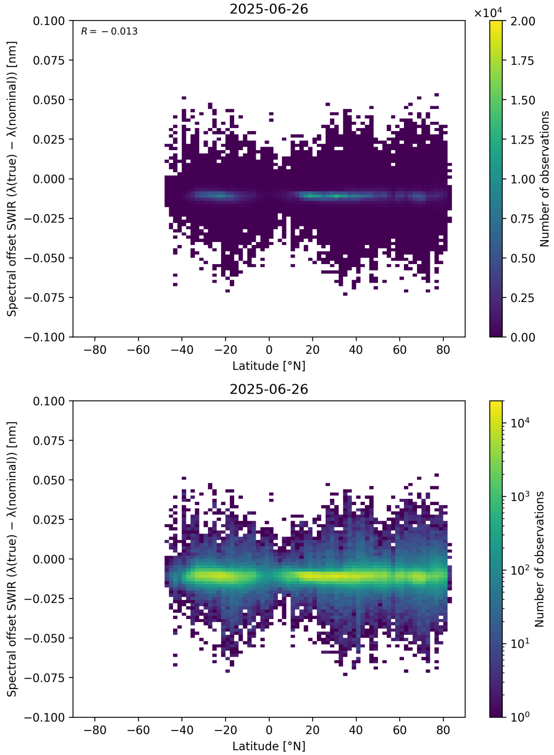
Figure 62: Scatter density plot of “Latitude” against “Spectral offset SWIR ( \lambda_{\text{true}} - \lambda_{\text{nominal}} )” for 2025-06-25 to 2025-06-27.
