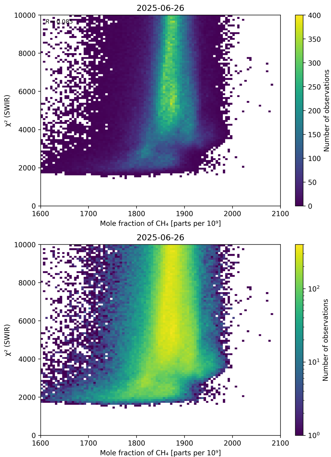
Figure 71: Scatter density plot of “Mole fraction of \text{CH}_4 ” against “ \chi^2 (SWIR)” for 2025-06-25 to 2025-06-27.
