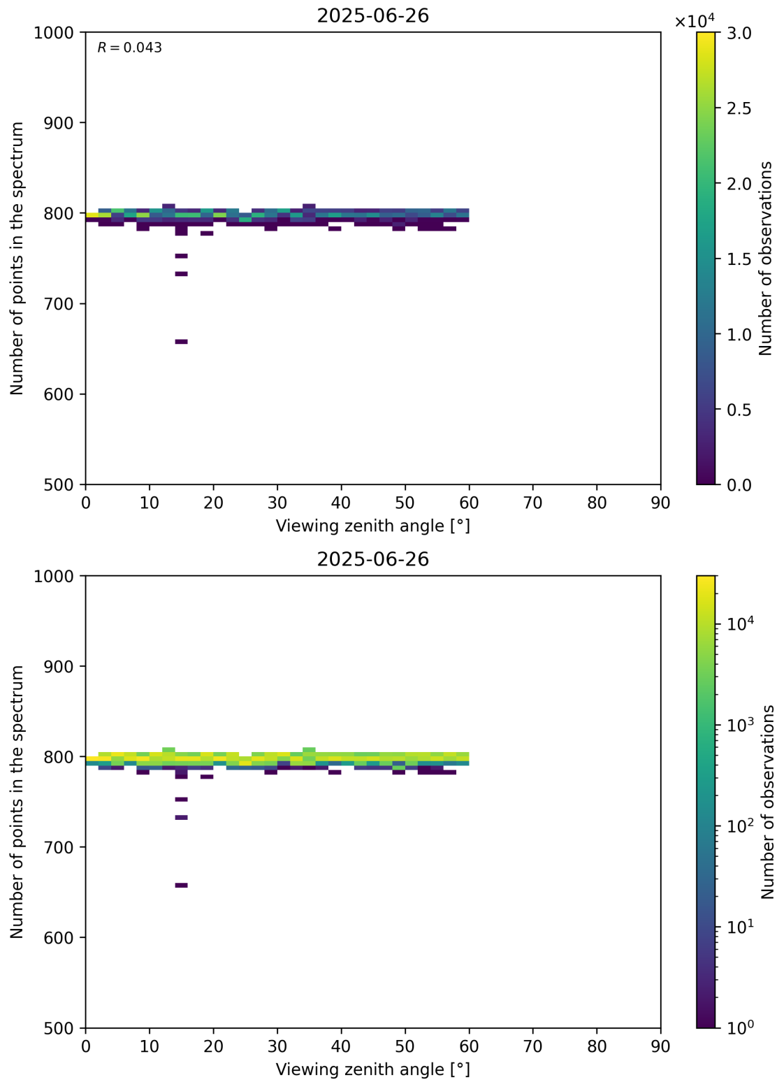
Figure 114: Scatter density plot of “Viewing zenith angle” against “Number of points in the spectrum” for 2025-06-25 to 2025-06-27.
