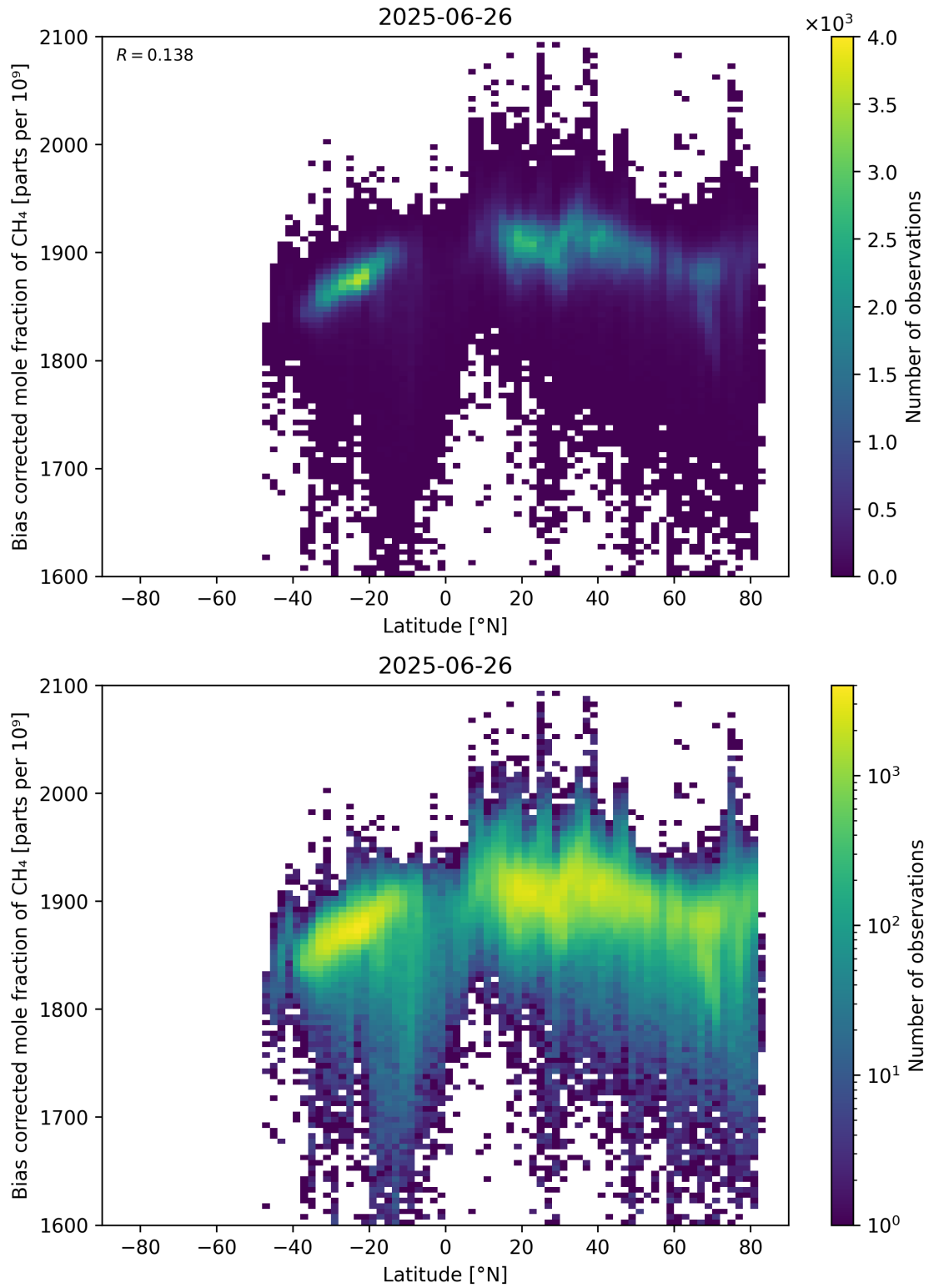
Figure 58: Scatter density plot of “Latitude” against “Bias corrected mole fraction of CH 4 ” for 2025-06-25 to 2025-06-27.
