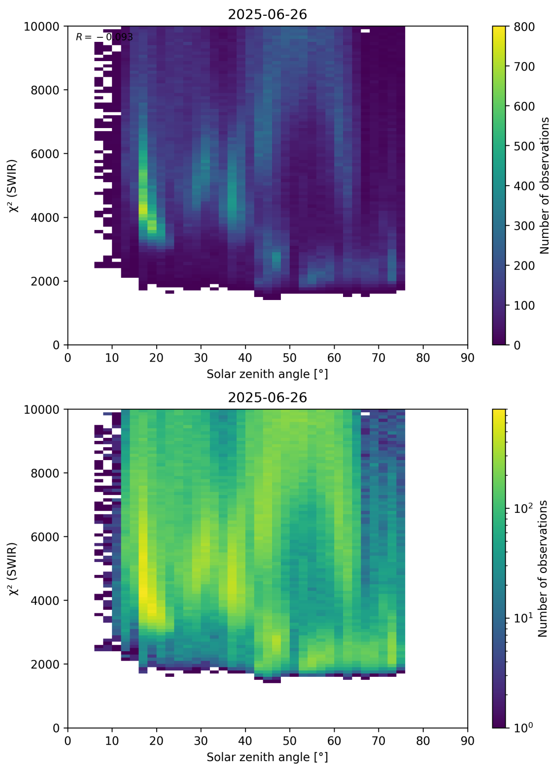
Figure 95: Scatter density plot of “Solar zenith angle” against “ \chi^2 (SWIR)” for 2025-06-25 to 2025-06-27.
