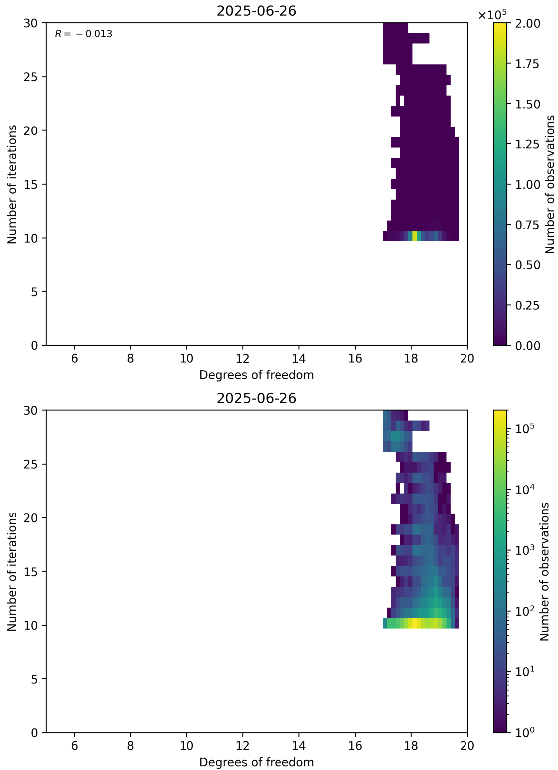
Figure 52: Scatter density plot of “Degrees of freedom” against “Number of iterations” for 2025-06-25 to 2025-06-27.
