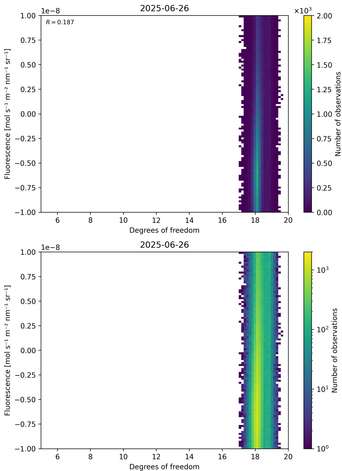
Figure 51: Scatter density plot of “Degrees of freedom” against “Fluorescence” for 2025-06-25 to 2025-06-27.
