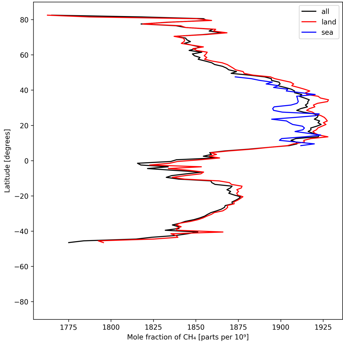
Figure 12: Zonal average of “Mole fraction of \text{CH}_4 ” for 2025-06-25 to 2025-06-27.
