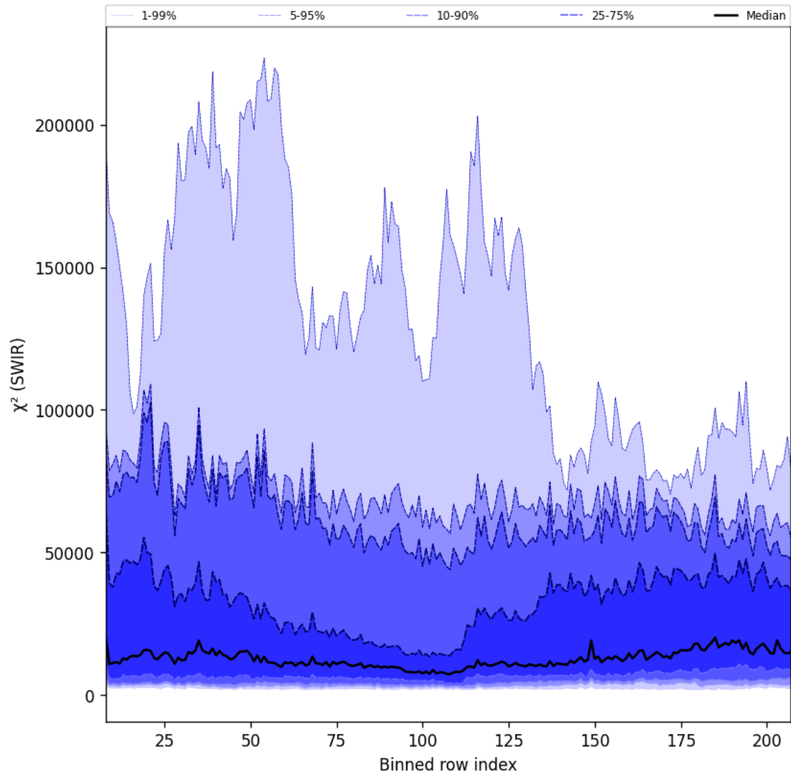
Figure 39: Along track statistics of “ \chi^2 (SWIR)” for 2025-06-25 to 2025-06-27
