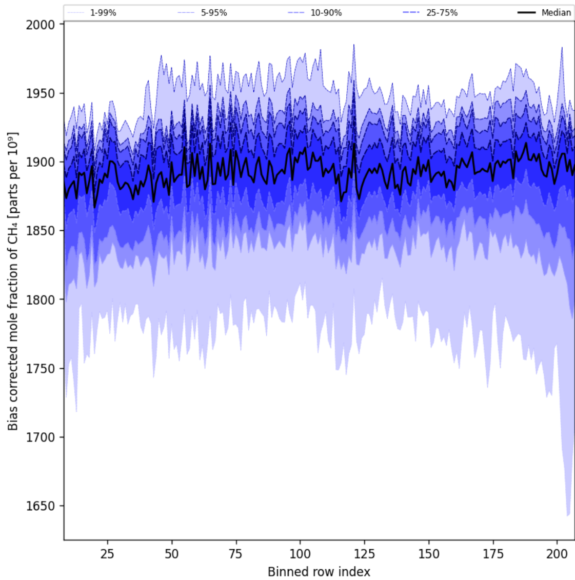
Figure 36: Along track statistics of “Bias corrected mole fraction of CH 4 ” for 2025-06-25 to 2025-06-27
