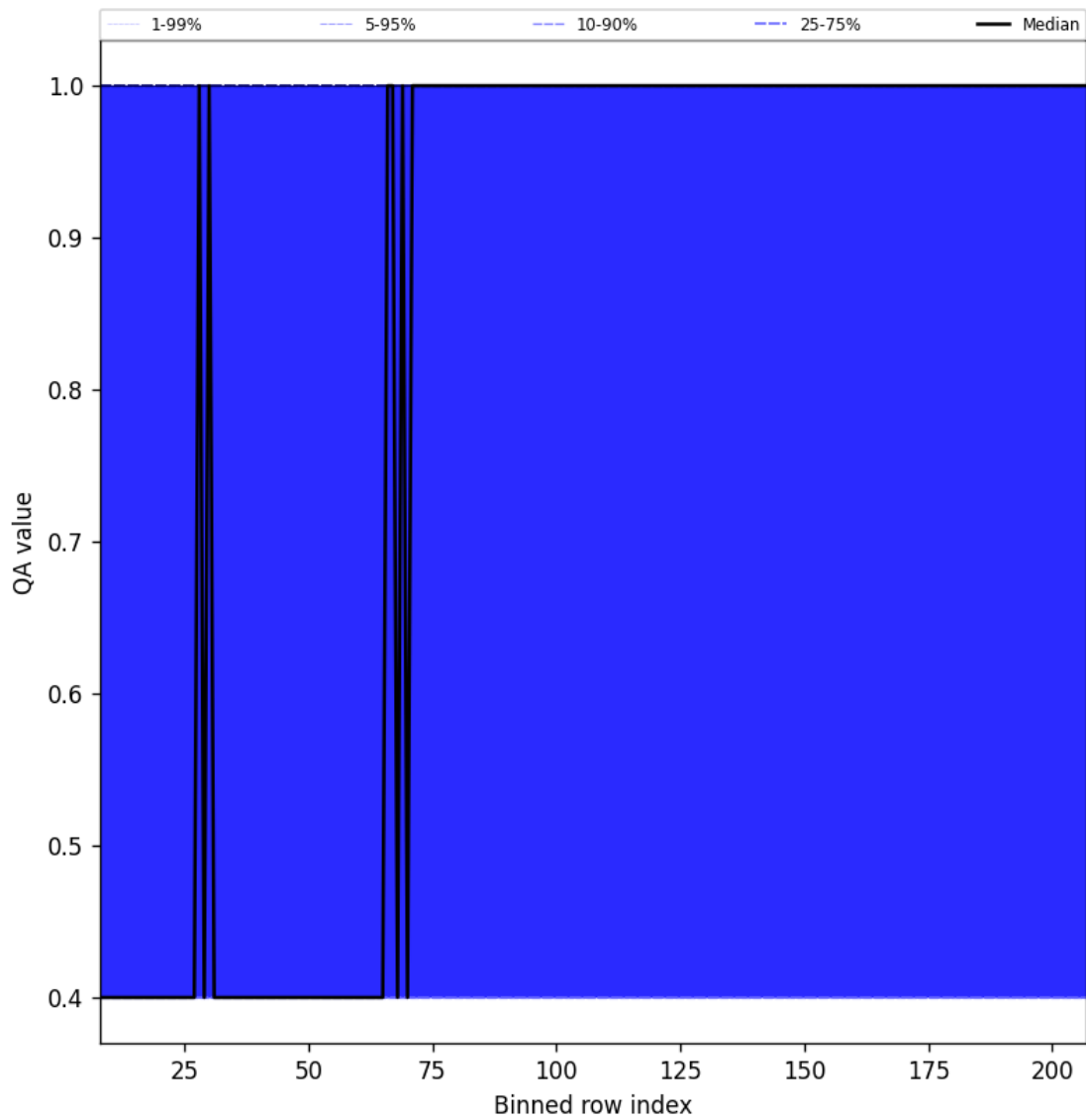
Figure 33: Along track statistics of “QA value” for 2025-06-25 to 2025-06-27
