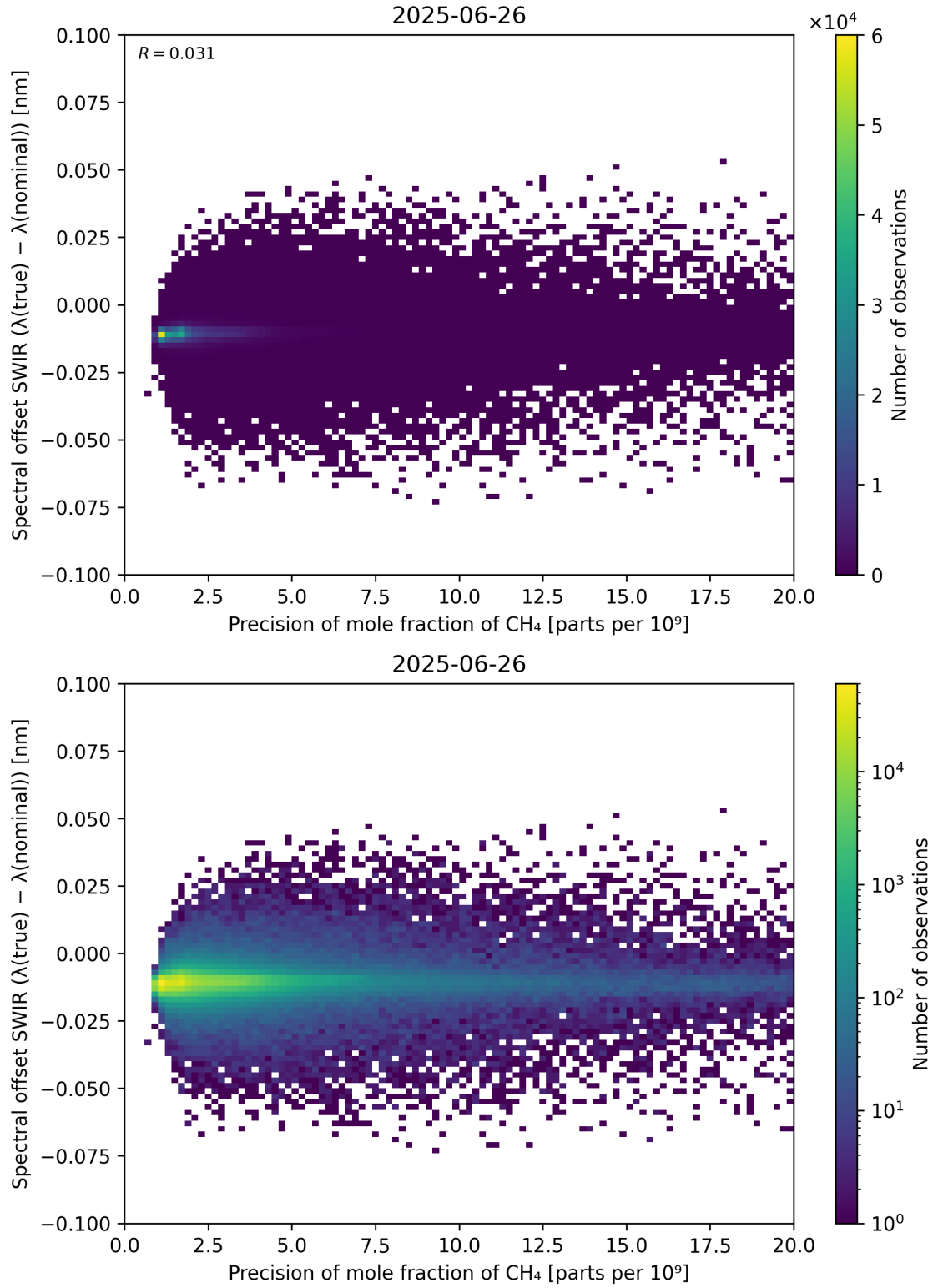
Figure 85: Scatter density plot of “Precision of mole fraction of CH 4 ” against “Spectral offset SWIR ( \lambda_{\text{true}} - \lambda_{\text{nominal}} )” for 2025-06-25 to 2025-06-27.
