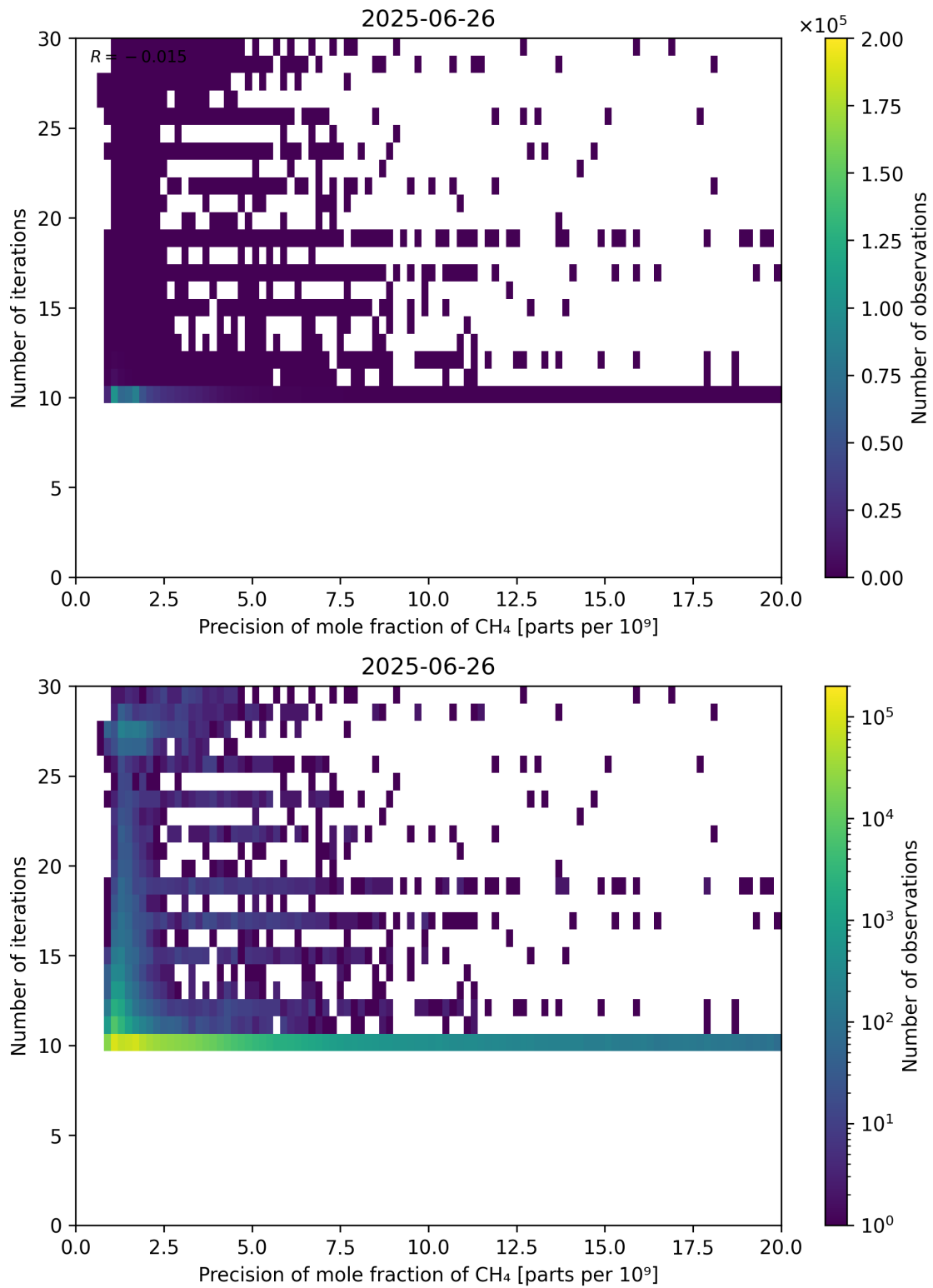
Figure 83: Scatter density plot of “Precision of mole fraction of CH 4 ” against “Number of iterations” for 2025-06-25 to 2025-06-27.
