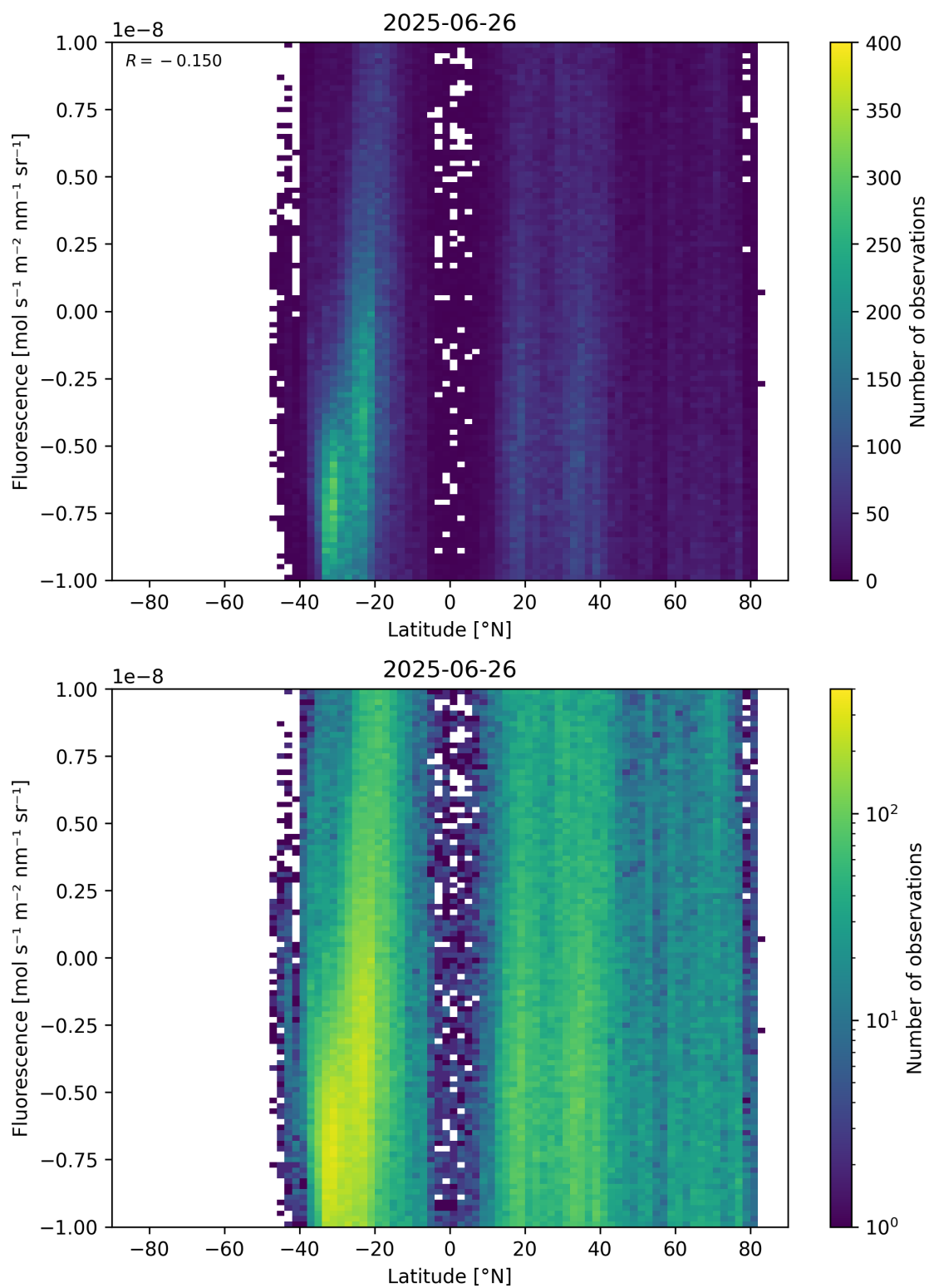
Figure 56: Scatter density plot of “Latitude” against “Fluorescence” for 2025-06-25 to 2025-06-27.
