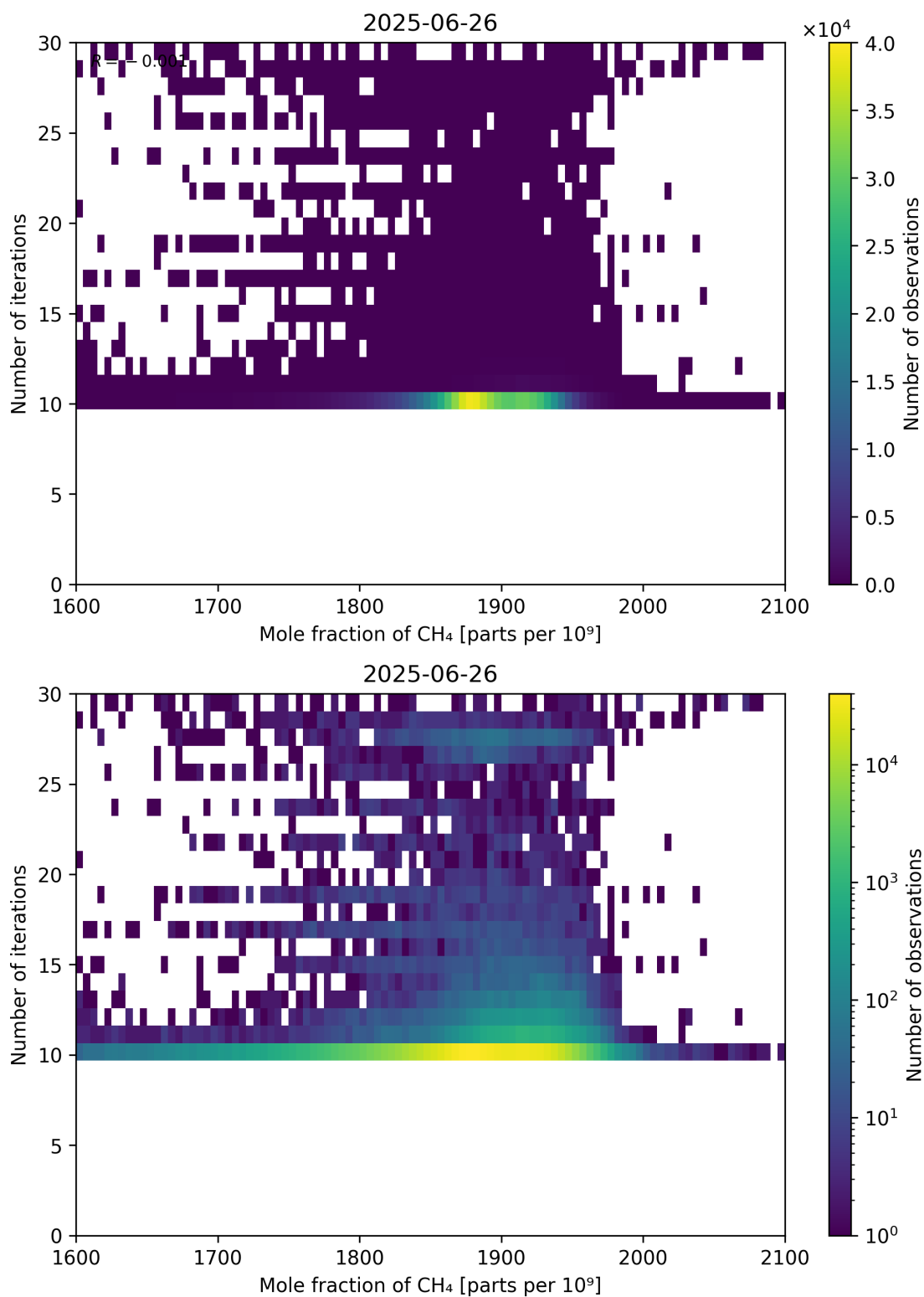
Figure 76: Scatter density plot of “Mole fraction of CH 4 ” against “Number of iterations” for 2025-06-25 to 2025-06-27.
