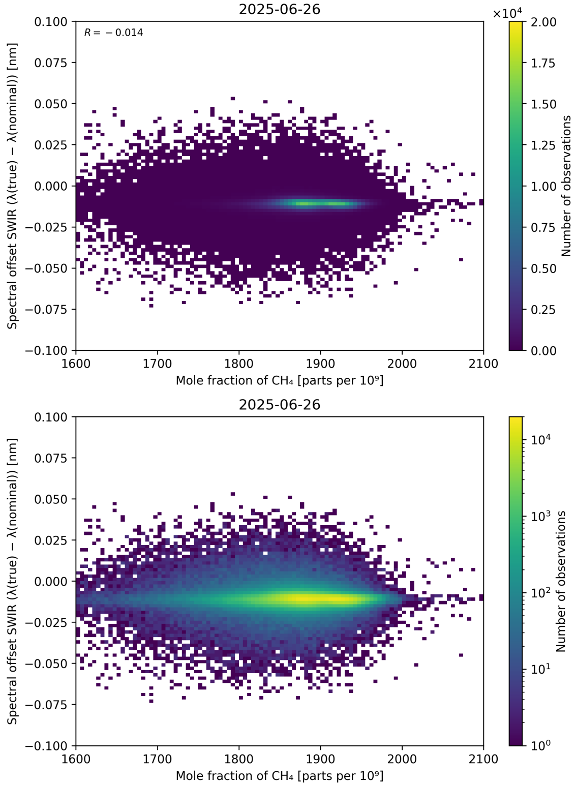
Figure 86: Scatter density plot of “Mole fraction of CH 4 ” against “Spectral offset SWIR ( \lambda_{\text{true}} - \lambda_{\text{nominal}} )” for 2025-06-25 to 2025-06-27.
