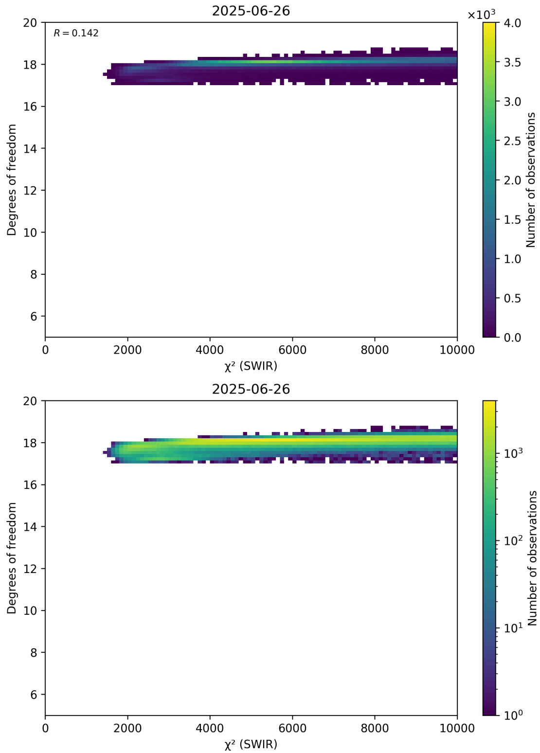
Figure 48: Scatter density plot of “ \chi^2 (SWIR)” against “Degrees of freedom” for 2025-06-25 to 2025-06-27.
