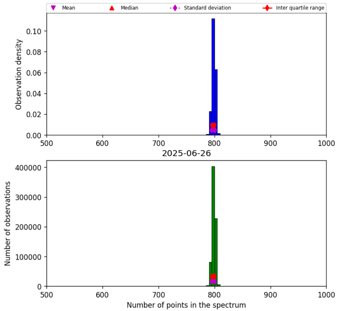
Figure 26: Histogram of “Number of points in the spectrum” for 2025-06-25 to 2025-06-27
