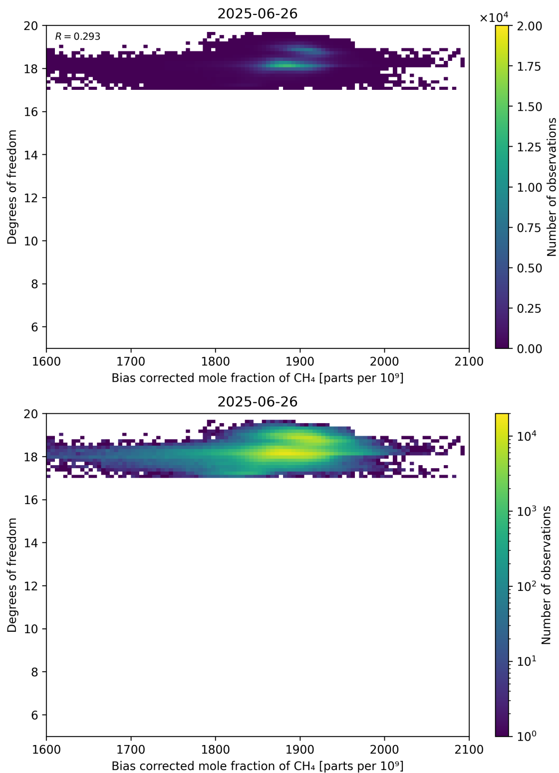
Figure 65: Scatter density plot of “Bias corrected mole fraction of CH 4 ” against “Degrees of freedom” for 2025-06-25 to 2025-06-27.
