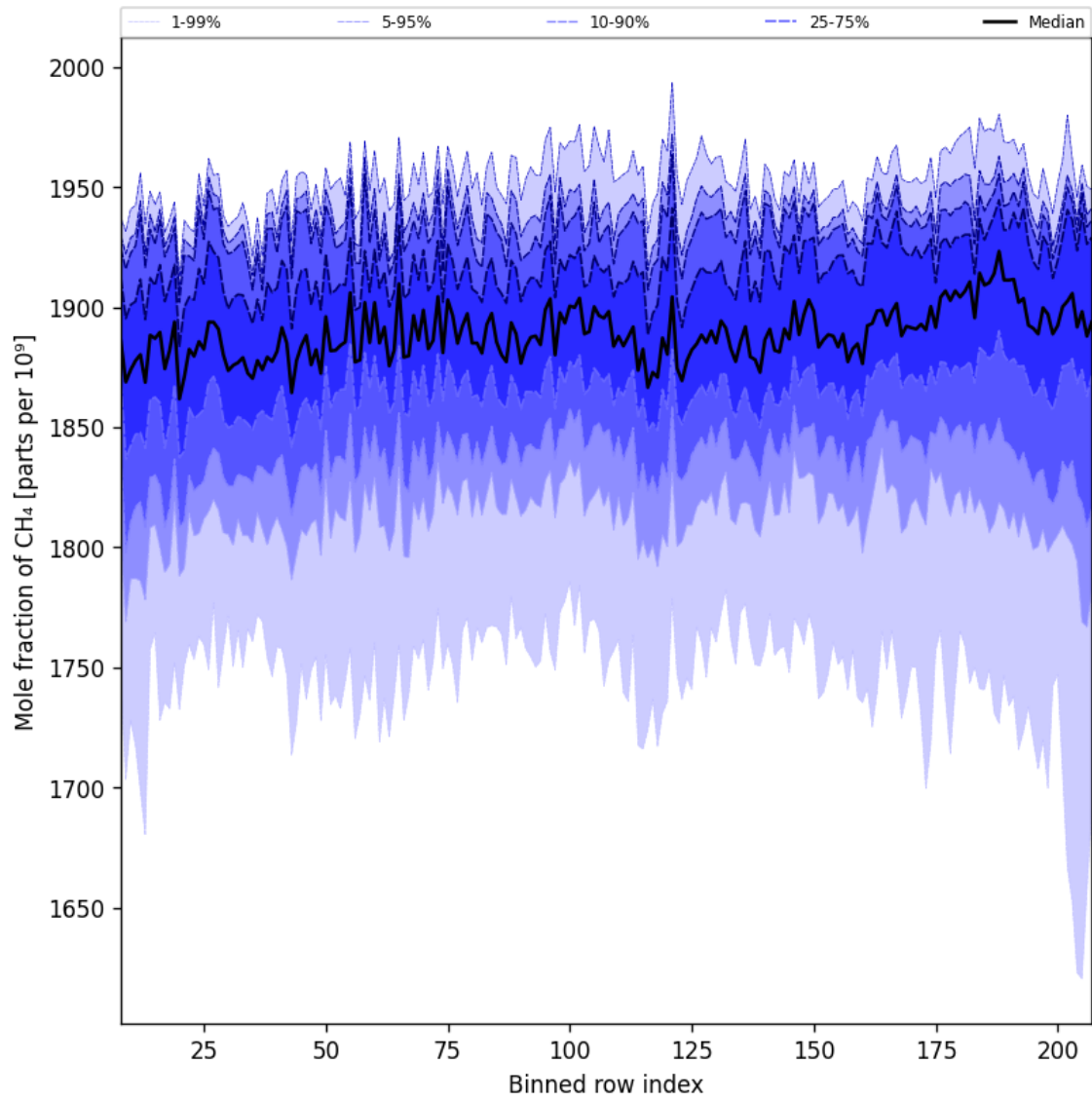
Figure 34: Along track statistics of “Mole fraction of CH 4 ” for 2025-06-25 to 2025-06-27
