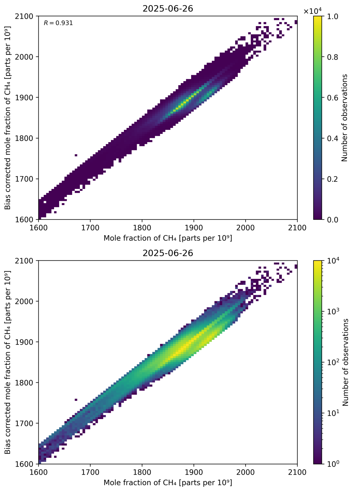
Figure 74: Scatter density plot of “Mole fraction of CH 4 ” against “Bias corrected mole fraction of CH 4 ” for 2025-06-25 to 2025-06-27.
