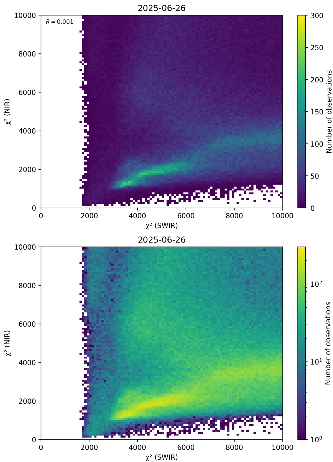
Figure 47: Scatter density plot of “ \chi^2 (SWIR)” against “ \chi^2 (NIR)” for 2025-06-25 to 2025-06-27.
