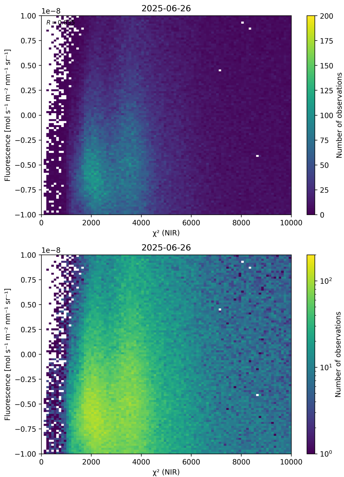
Figure 45: Scatter density plot of “ \chi^2 (NIR)” against “Fluorescence” for 2025-06-25 to 2025-06-27.
