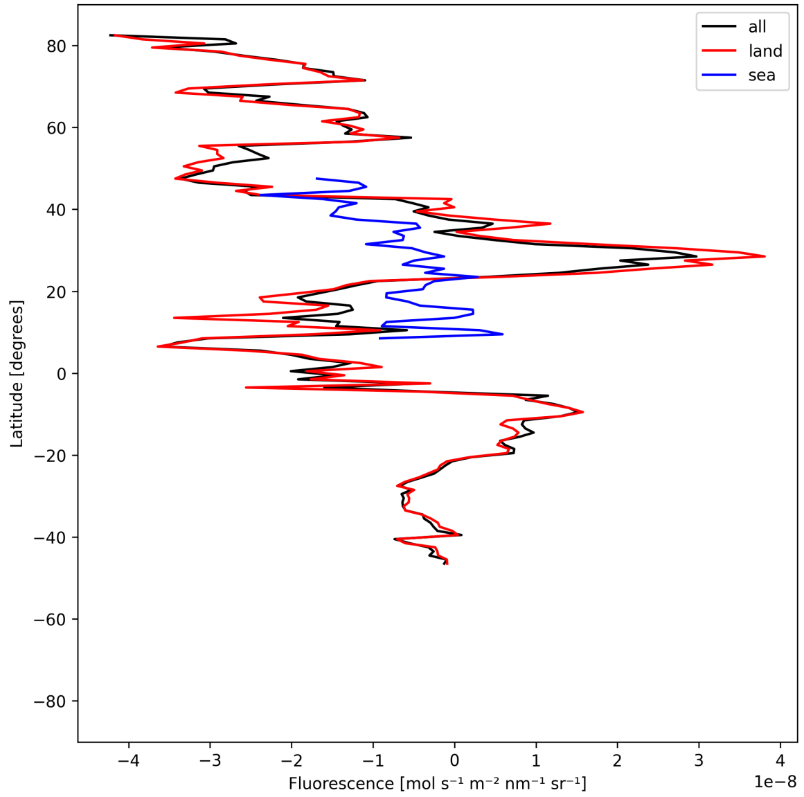
Figure 21: Zonal average of “Fluorescence” for 2025-06-25 to 2025-06-27.
