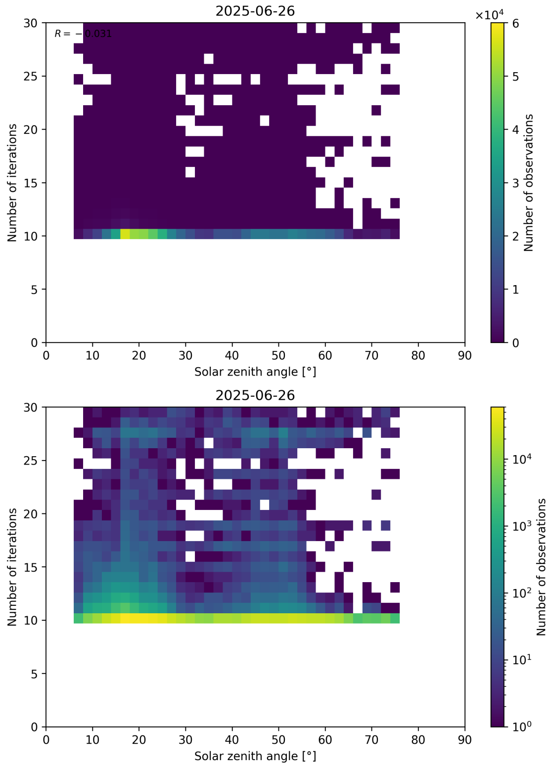
Figure 102: Scatter density plot of “Solar zenith angle” against “Number of iterations” for 2025-06-25 to 2025-06-27.
