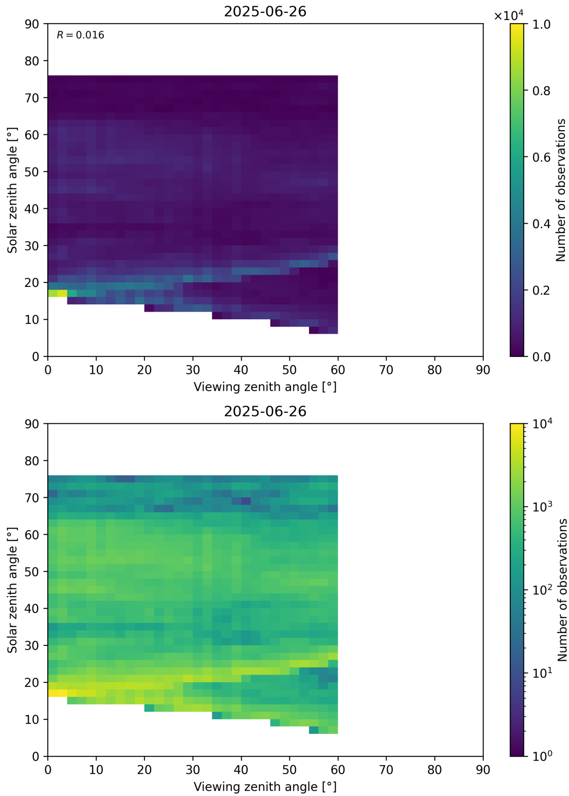
Figure 115: Scatter density plot of “Viewing zenith angle” against “Solar zenith angle” for 2025-06-25 to 2025-06-27.
