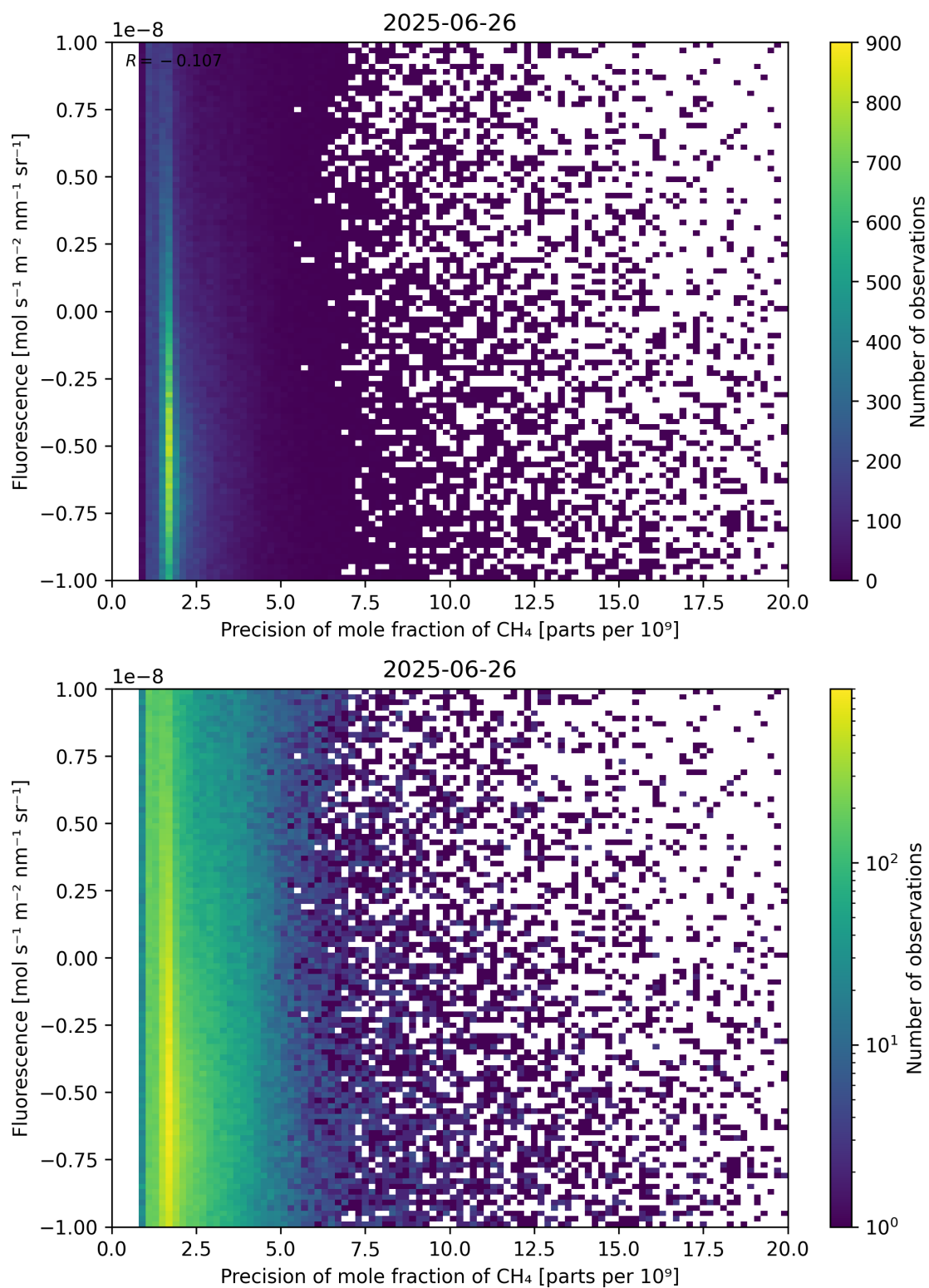
Figure 81: Scatter density plot of “Precision of mole fraction of \text{CH}_4 ” against “Fluorescence” for 2025-06-25 to 2025-06-27.
