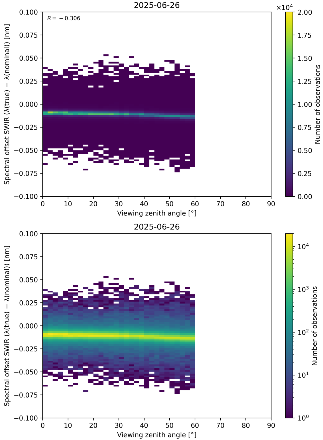
Figure 116: Scatter density plot of “Viewing zenith angle” against “Spectral offset SWIR ( \lambda_{\text{true}} - \lambda_{\text{nominal}} )” for 2025-06-25 to 2025-06-27.
