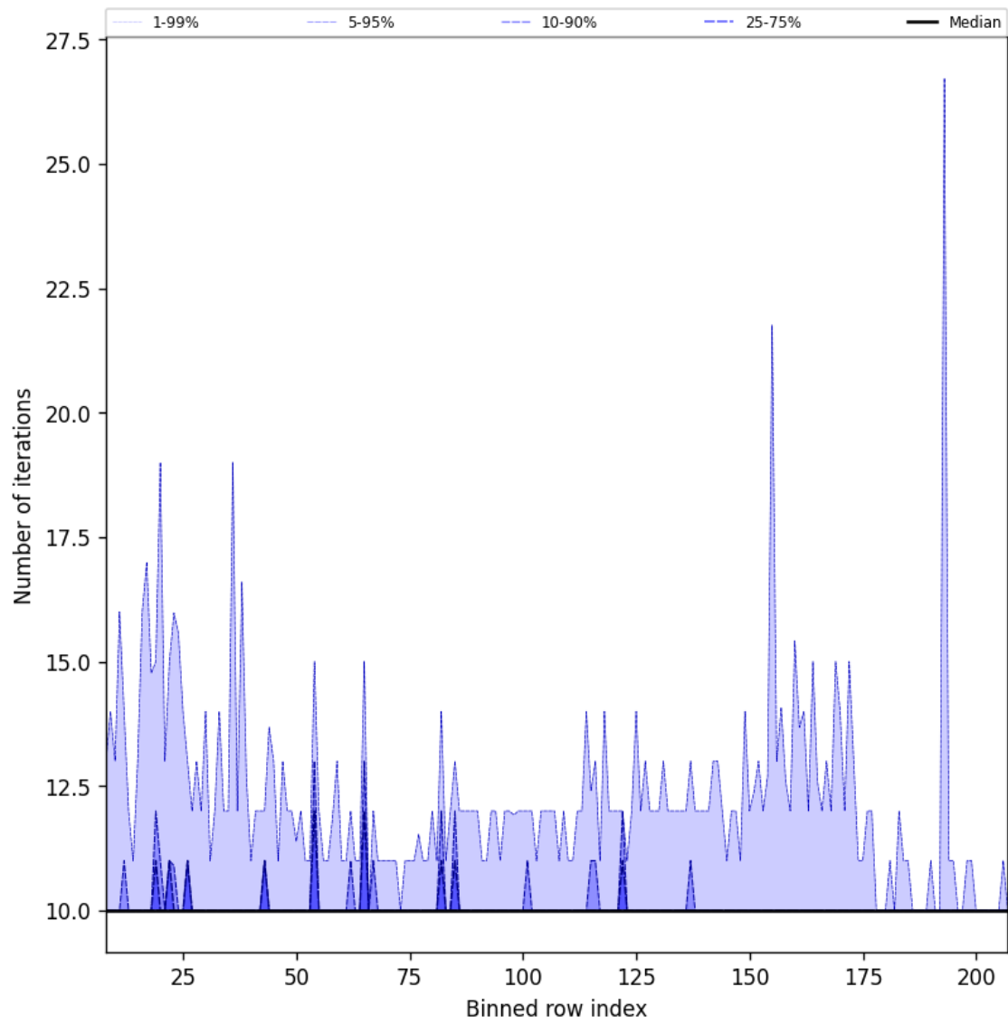
Figure 42: Along track statistics of “Number of iterations” for 2025-06-25 to 2025-06-27
