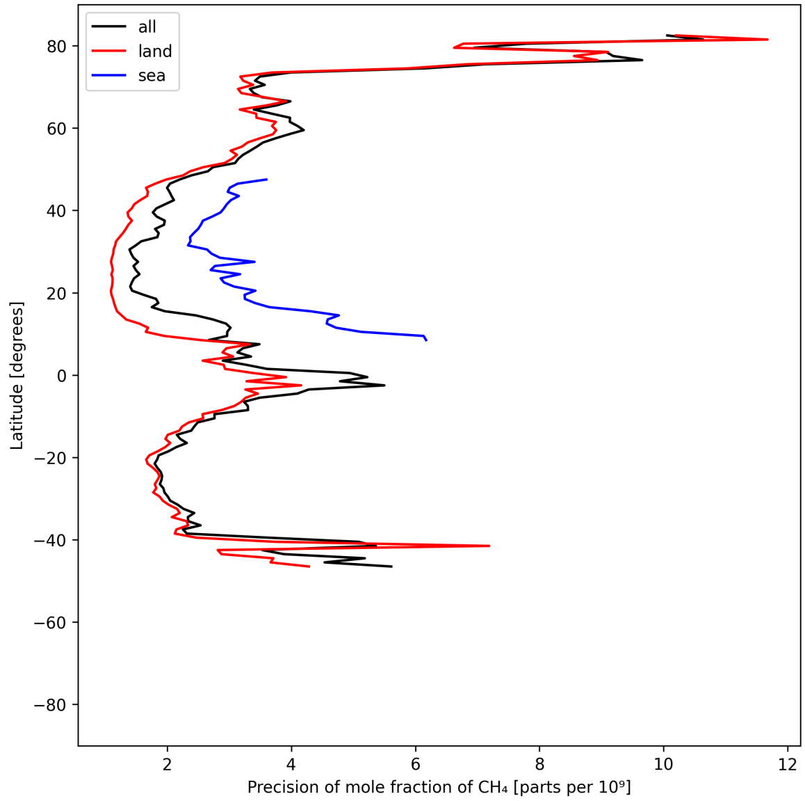
Figure 13: Zonal average of “Precision of mole fraction of CH 4 ” for 2025-06-25 to 2025-06-27.
