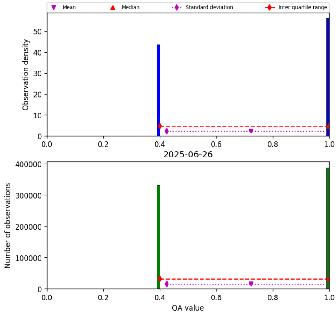
Figure 22: Histogram of “QA value” for 2025-06-25 to 2025-06-27
