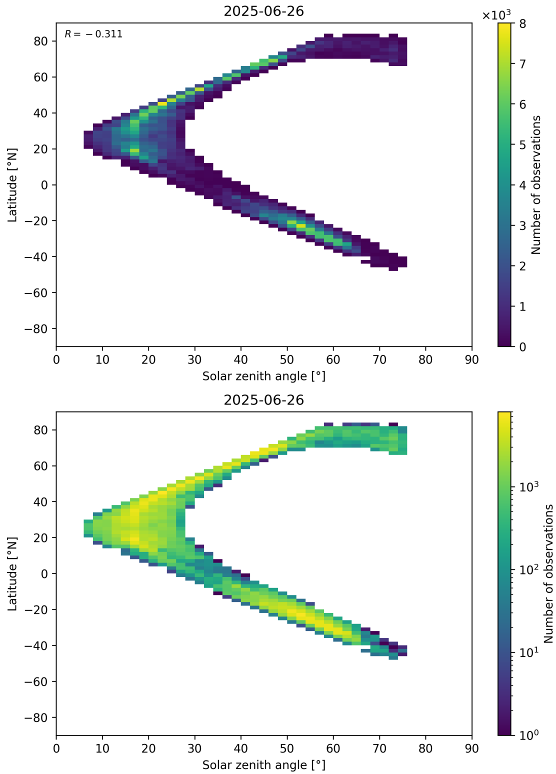
Figure 98: Scatter density plot of “Solar zenith angle” against “Latitude” for 2025-06-25 to 2025-06-27.
