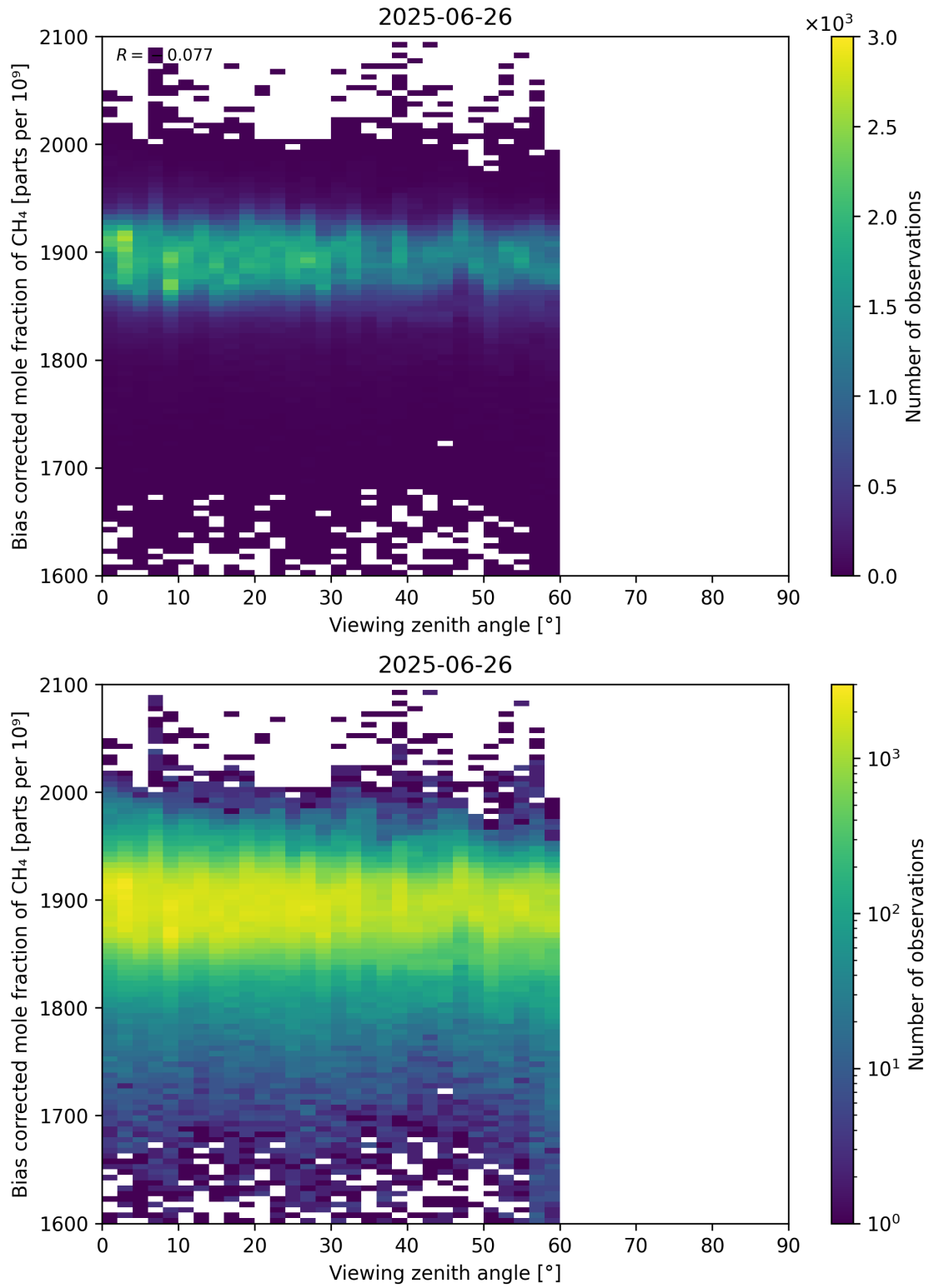
Figure 111: Scatter density plot of “Viewing zenith angle” against “Bias corrected mole fraction of CH 4 ” for 2025-06-25 to 2025-06-27.
