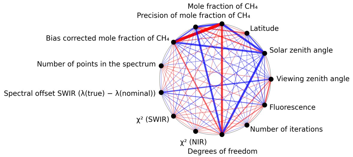
Figure 1: Map of correlation graph for 2025-06-25 to 2025-06-27.
