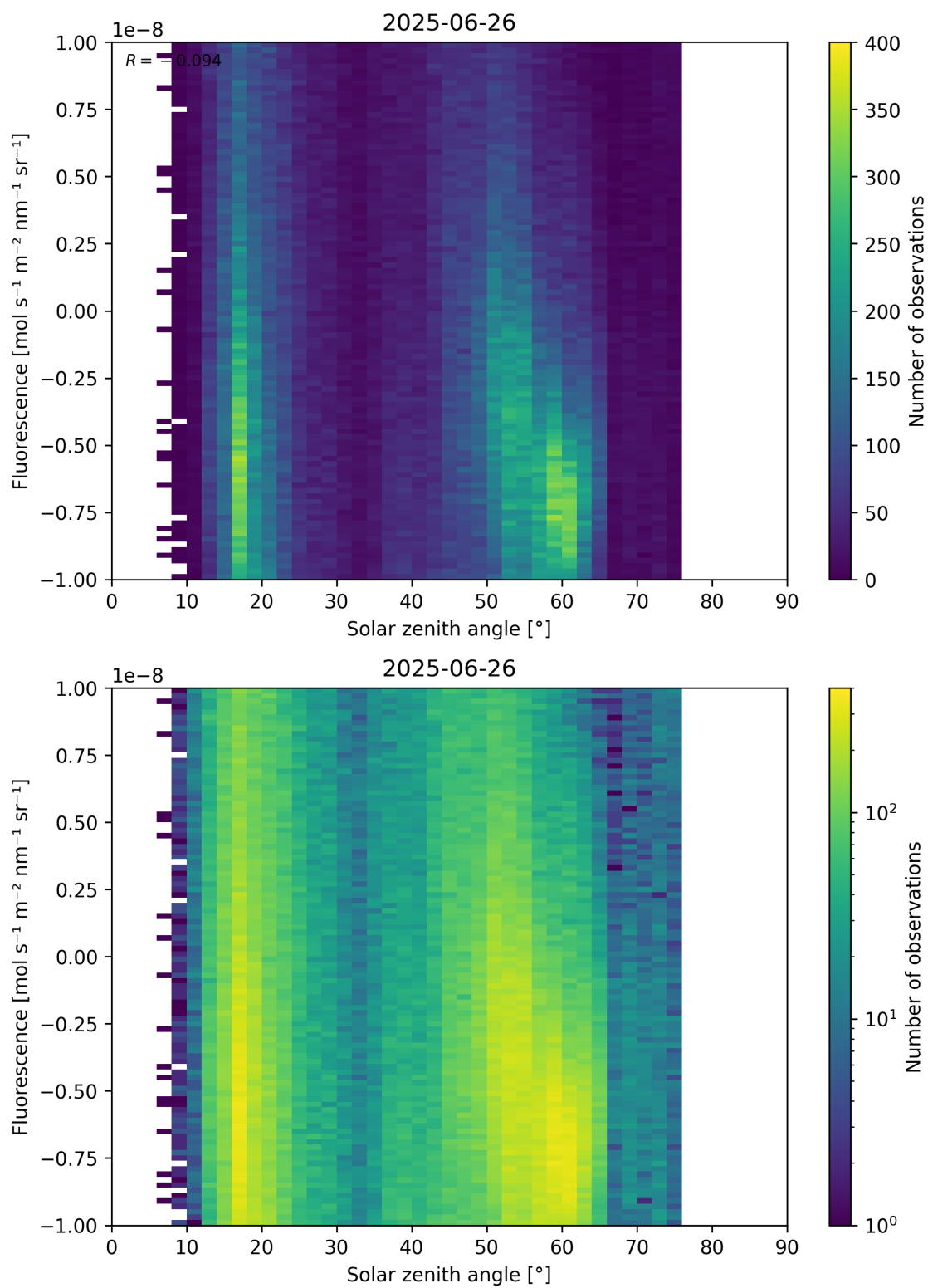
Figure 97: Scatter density plot of “Solar zenith angle” against “Fluorescence” for 2025-06-25 to 2025-06-27.
