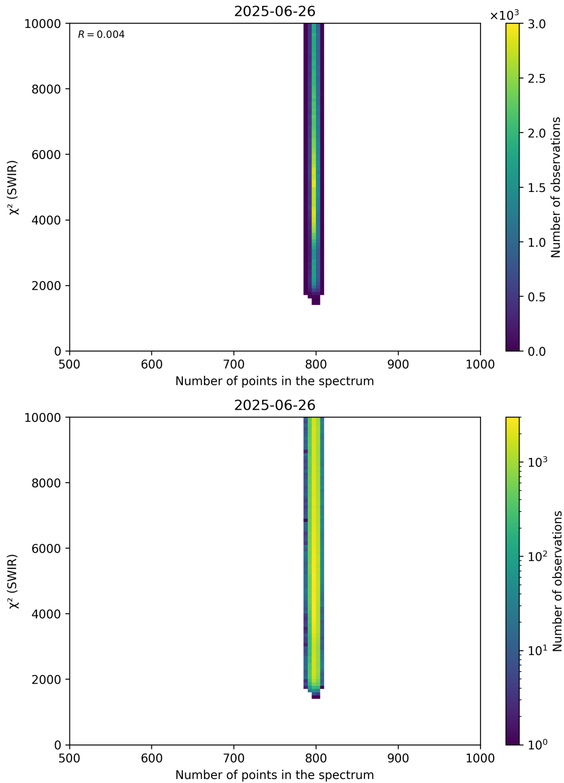
Figure 89: Scatter density plot of “Number of points in the spectrum” against “ \chi^2 (SWIR)” for 2025-06-25 to 2025-06-27.
