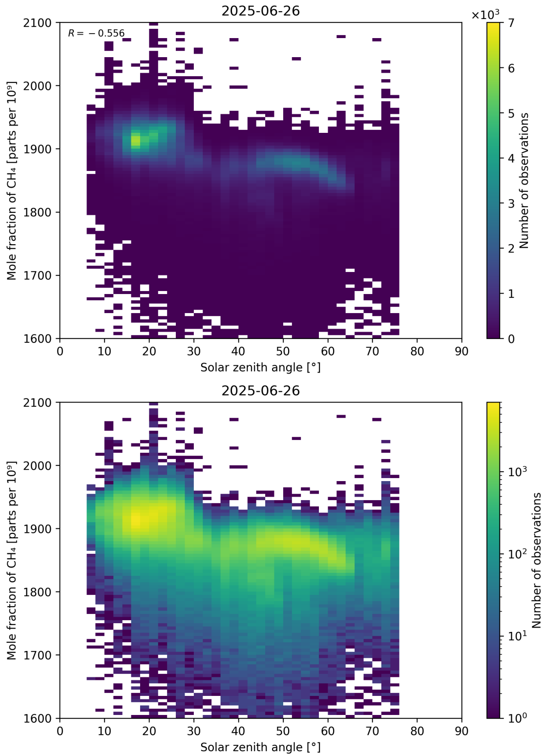
Figure 99: Scatter density plot of “Solar zenith angle” against “Mole fraction of \text{CH}_4 ” for 2025-06-25 to 2025-06-27.
