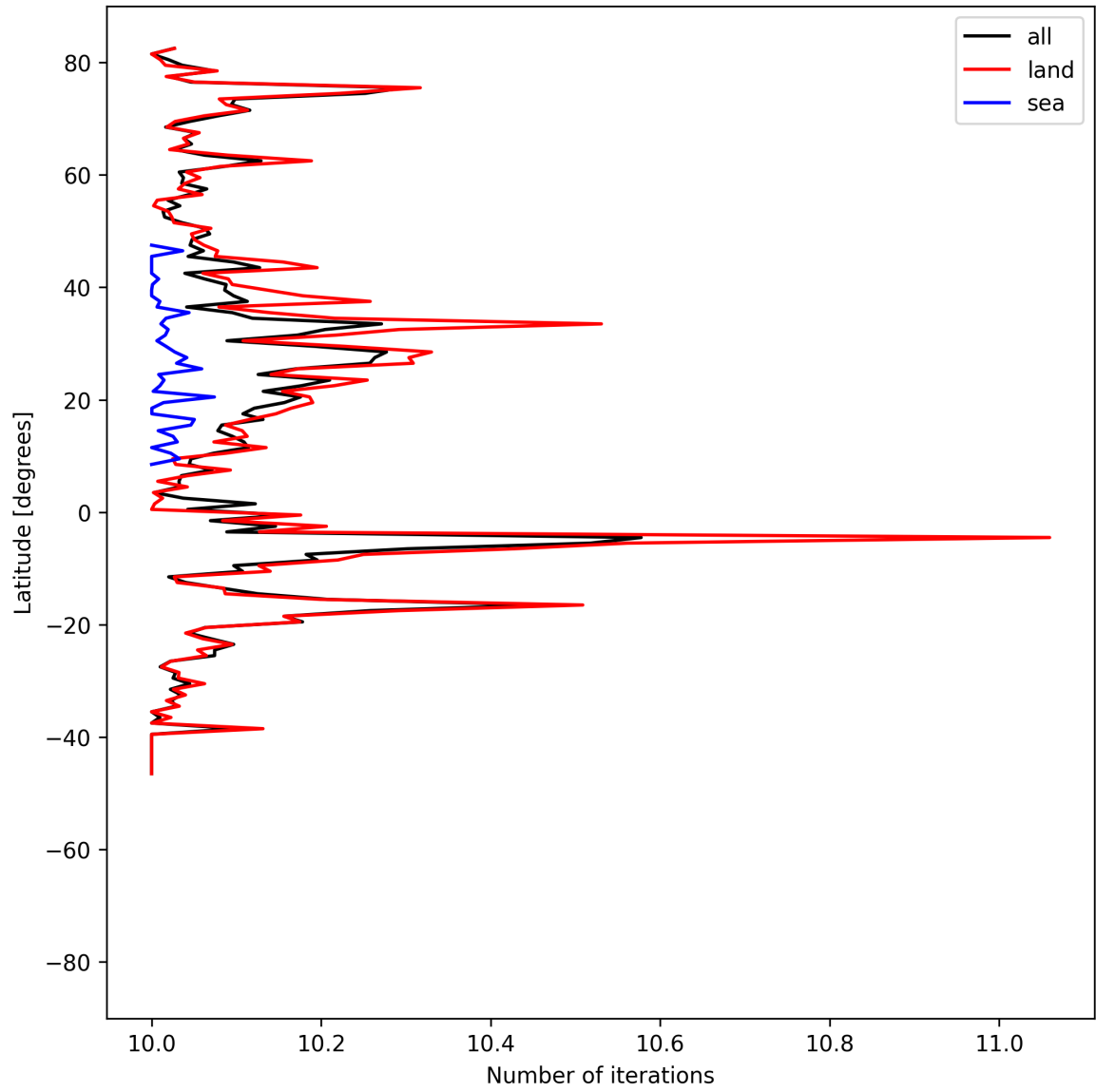
Figure 20: Zonal average of “Number of iterations” for 2025-06-25 to 2025-06-27.
