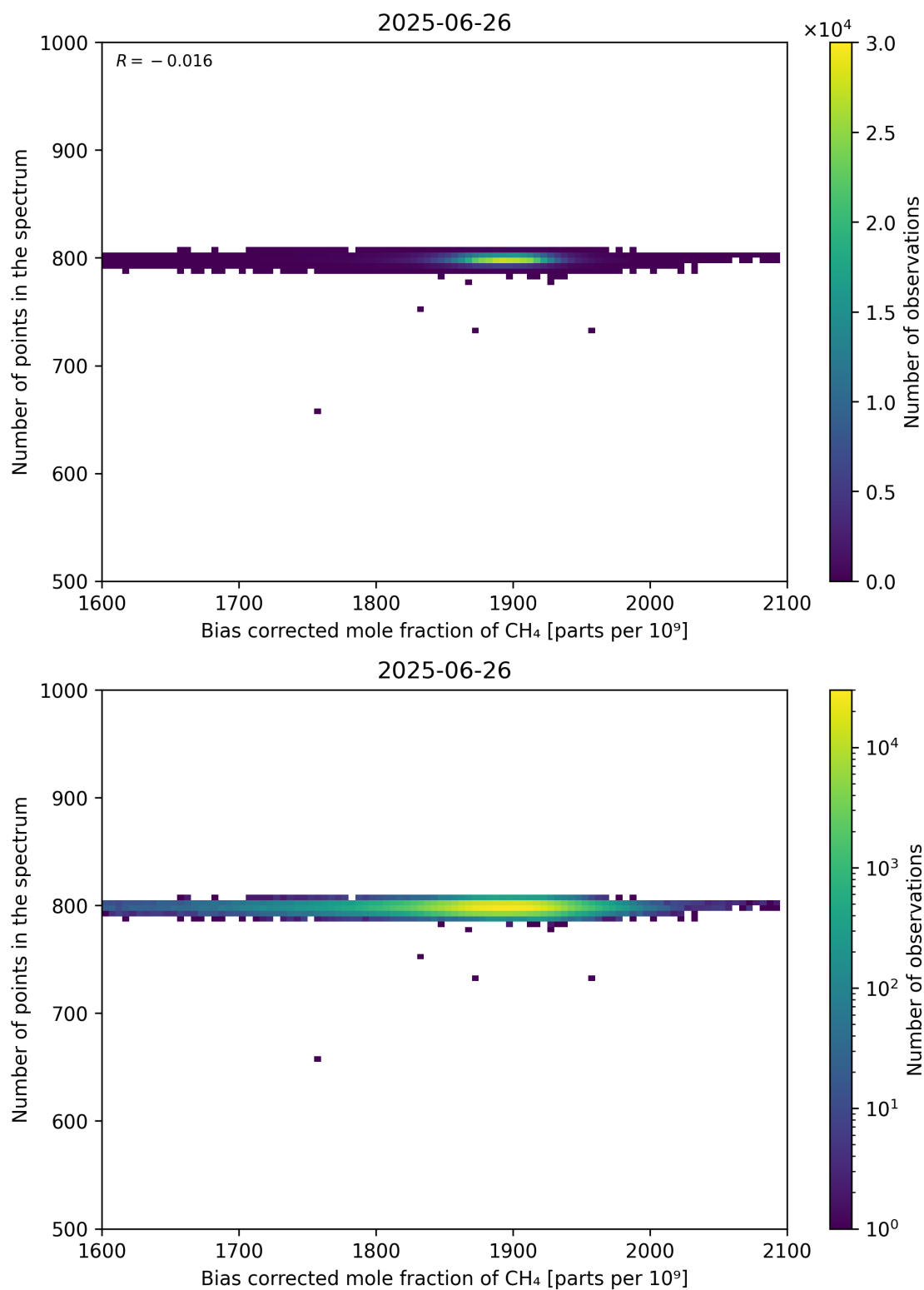
Figure 68: Scatter density plot of “Bias corrected mole fraction of CH 4 ” against “Number of points in the spectrum” for 2025-06-25 to 2025-06-27.
