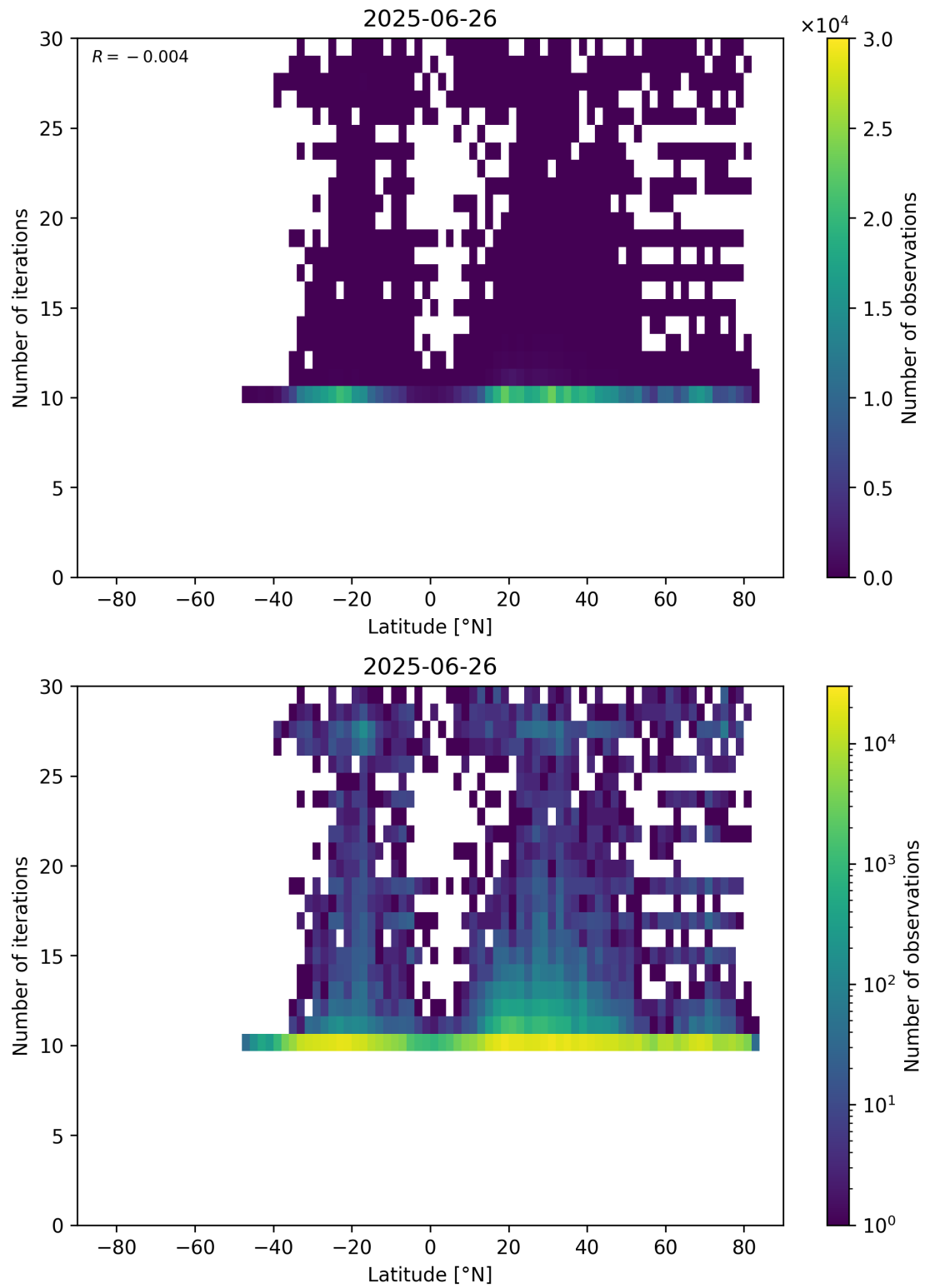
Figure 60: Scatter density plot of “Latitude” against “Number of iterations” for 2025-06-25 to 2025-06-27.
