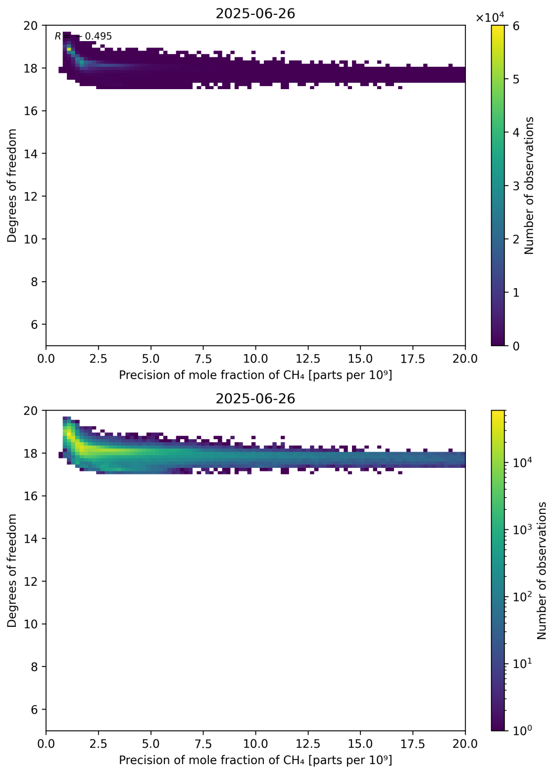
Figure 80: Scatter density plot of “Precision of mole fraction of CH 4 ” against “Degrees of freedom” for 2025-06-25 to 2025-06-27.
