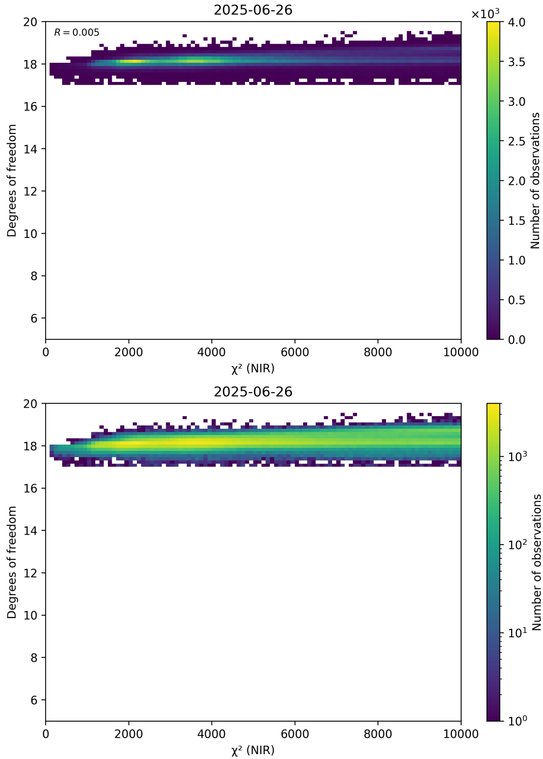
Figure 44: Scatter density plot of “ \chi^2 (NIR)” against “Degrees of freedom” for 2025-06-25 to 2025-06-27.
