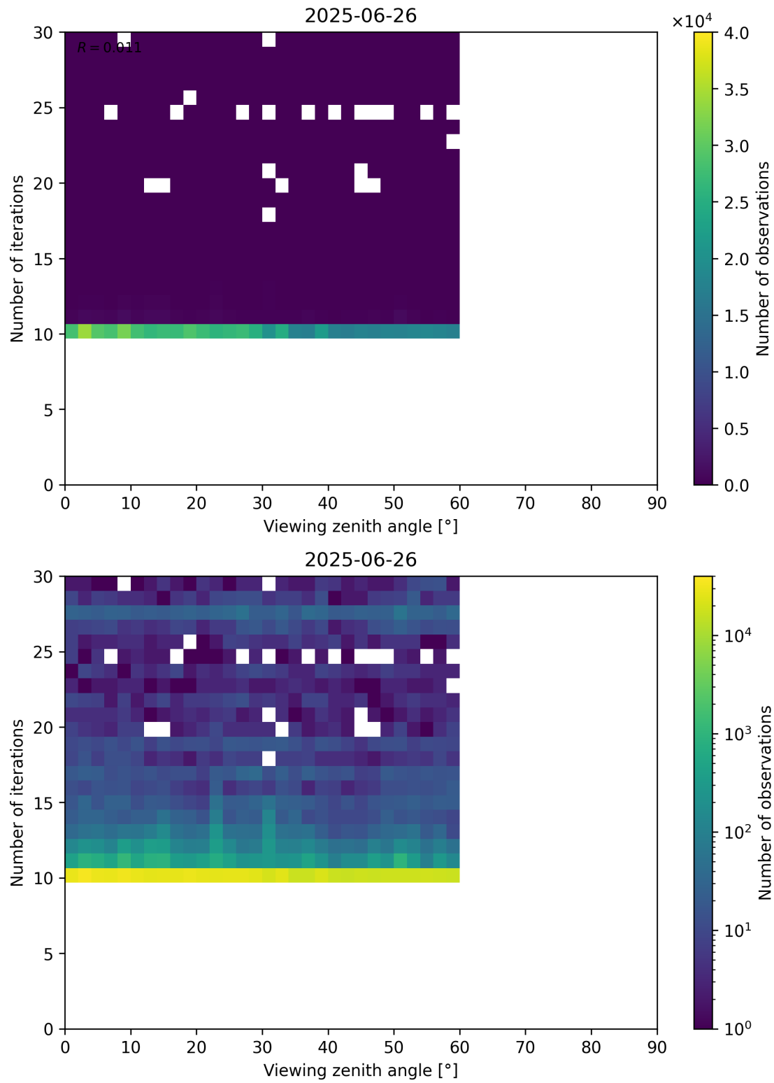
Figure 113: Scatter density plot of “Viewing zenith angle” against “Number of iterations” for 2025-06-25 to 2025-06-27.
