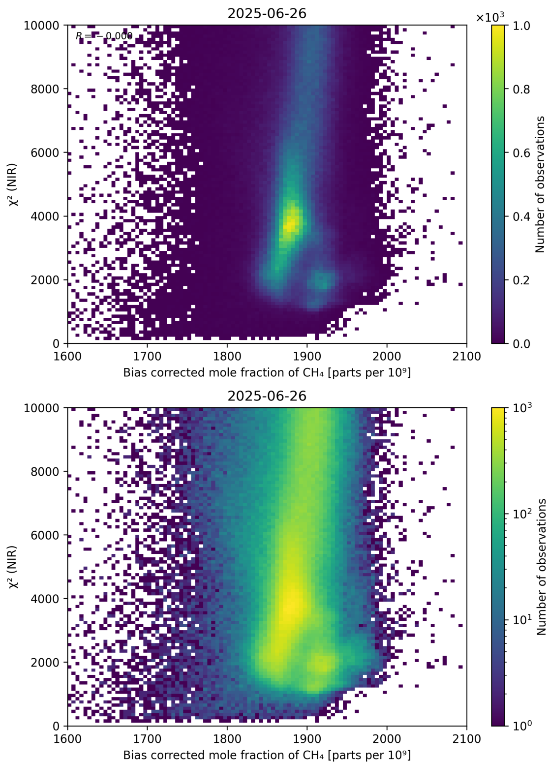
Figure 63: Scatter density plot of “Bias corrected mole fraction of \text{CH}_4 ” against “ \chi^2 (NIR)” for 2025-06-25 to 2025-06-27.
