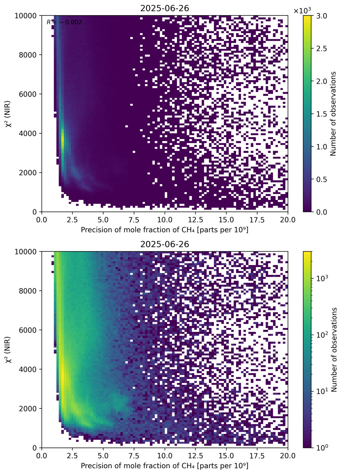
Figure 78: Scatter density plot of “Precision of mole fraction of \text{CH}_4 ” against “ \chi^2 (NIR)” for 2025-06-25 to 2025-06-27.
