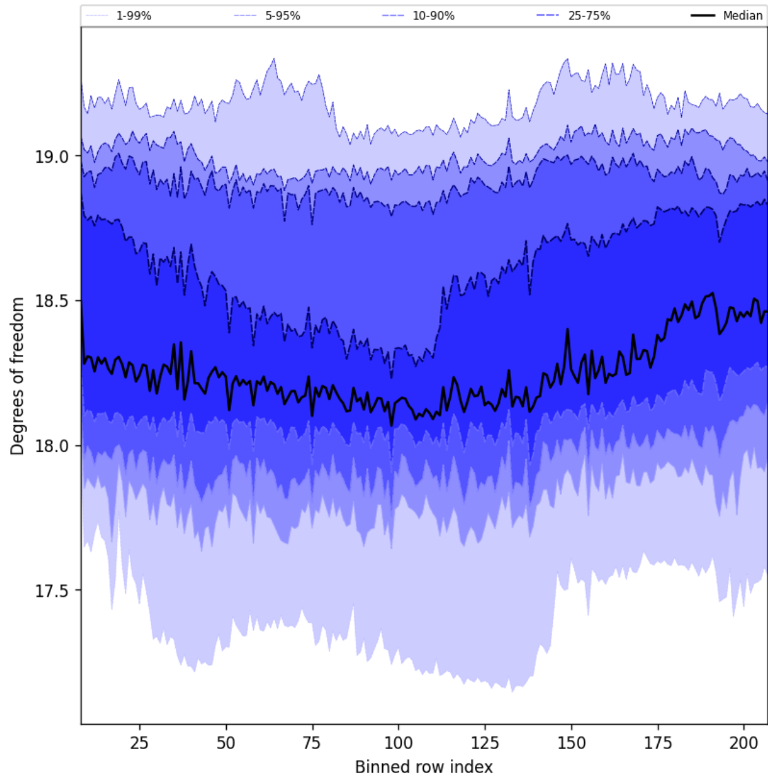
Figure 41: Along track statistics of “Degrees of freedom” for 2025-06-25 to 2025-06-27
