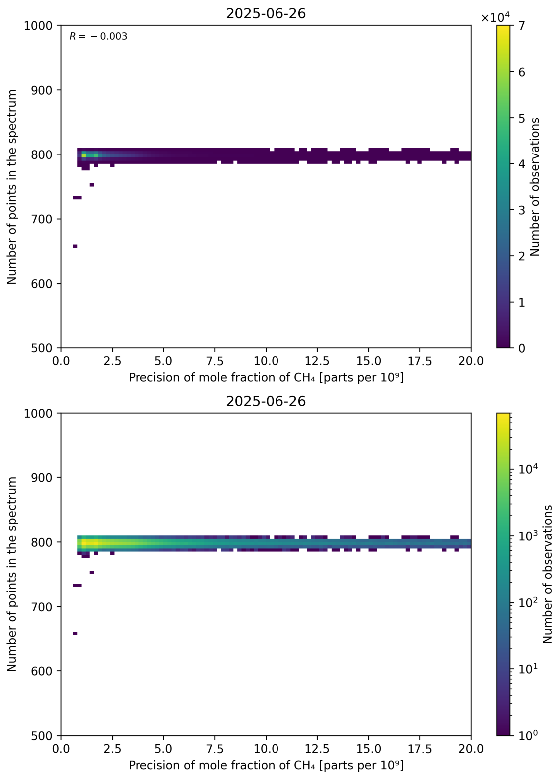
Figure 84: Scatter density plot of “Precision of mole fraction of CH 4 ” against “Number of points in the spectrum” for 2025-06-25 to 2025-06-27.
