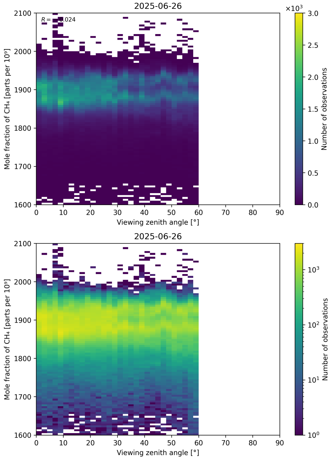
Figure 110: Scatter density plot of “Viewing zenith angle” against “Mole fraction of CH 4 ” for 2025-06-25 to 2025-06-27.
