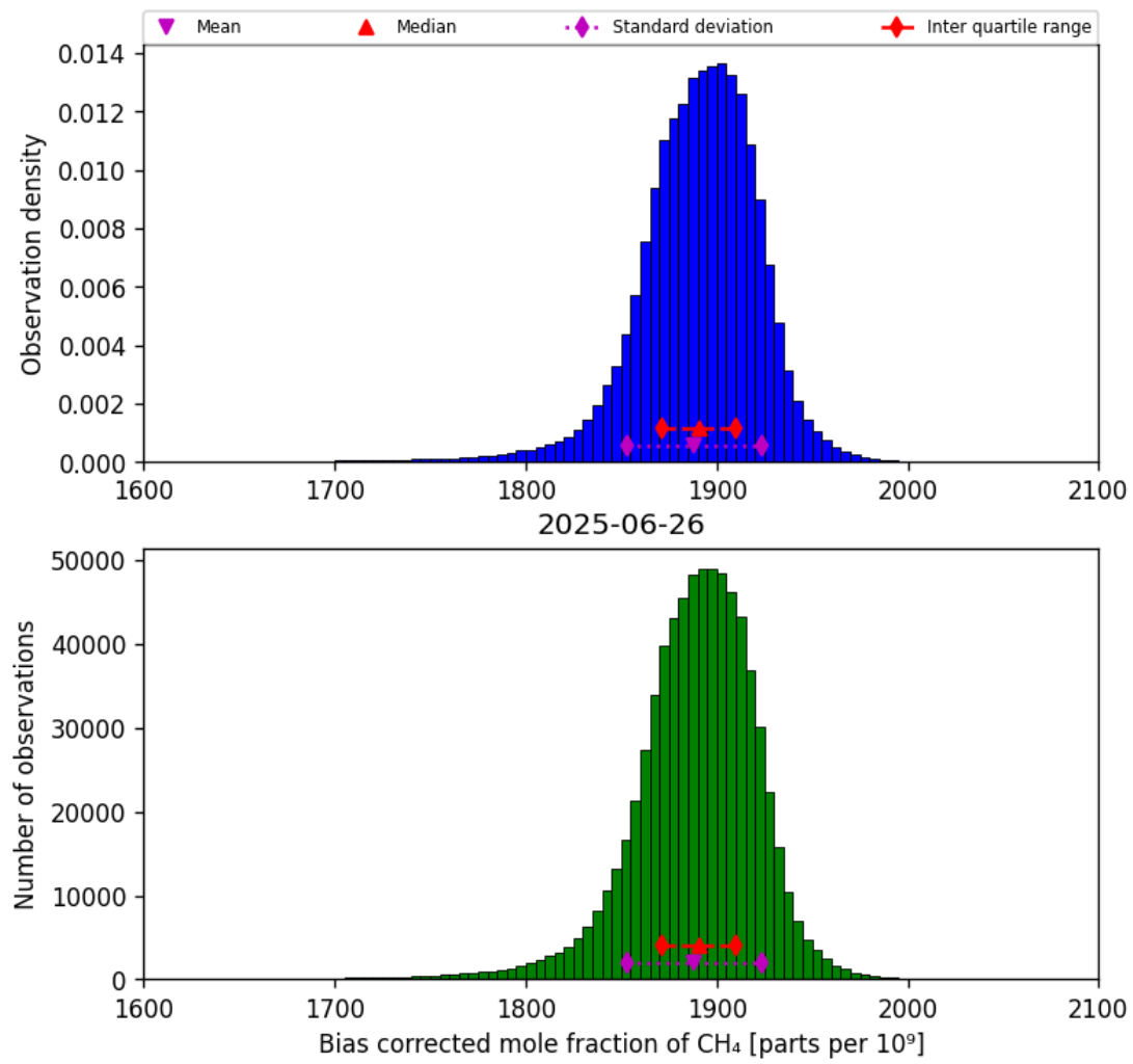
Figure 25: Histogram of “Bias corrected mole fraction of CH 4 ” for 2025-06-25 to 2025-06-27
