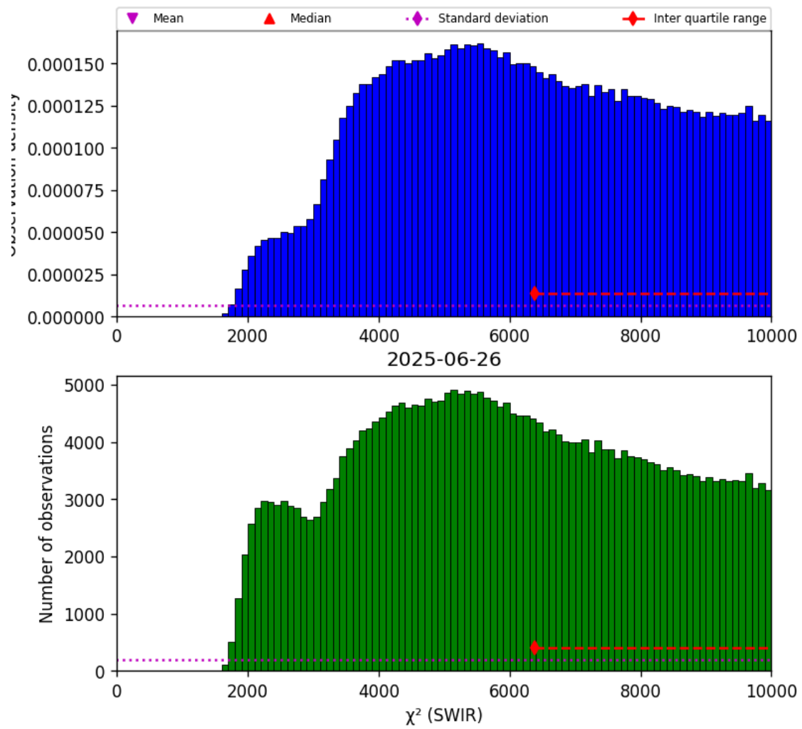
Figure 28: Histogram of “ \chi^2 (SWIR)” for 2025-06-25 to 2025-06-27
