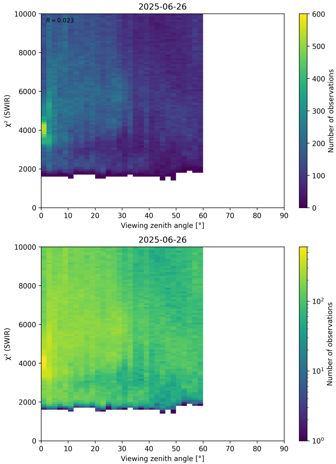
Figure 106: Scatter density plot of “Viewing zenith angle” against “ \chi^2 (SWIR)” for 2025-06-25 to 2025-06-27.
