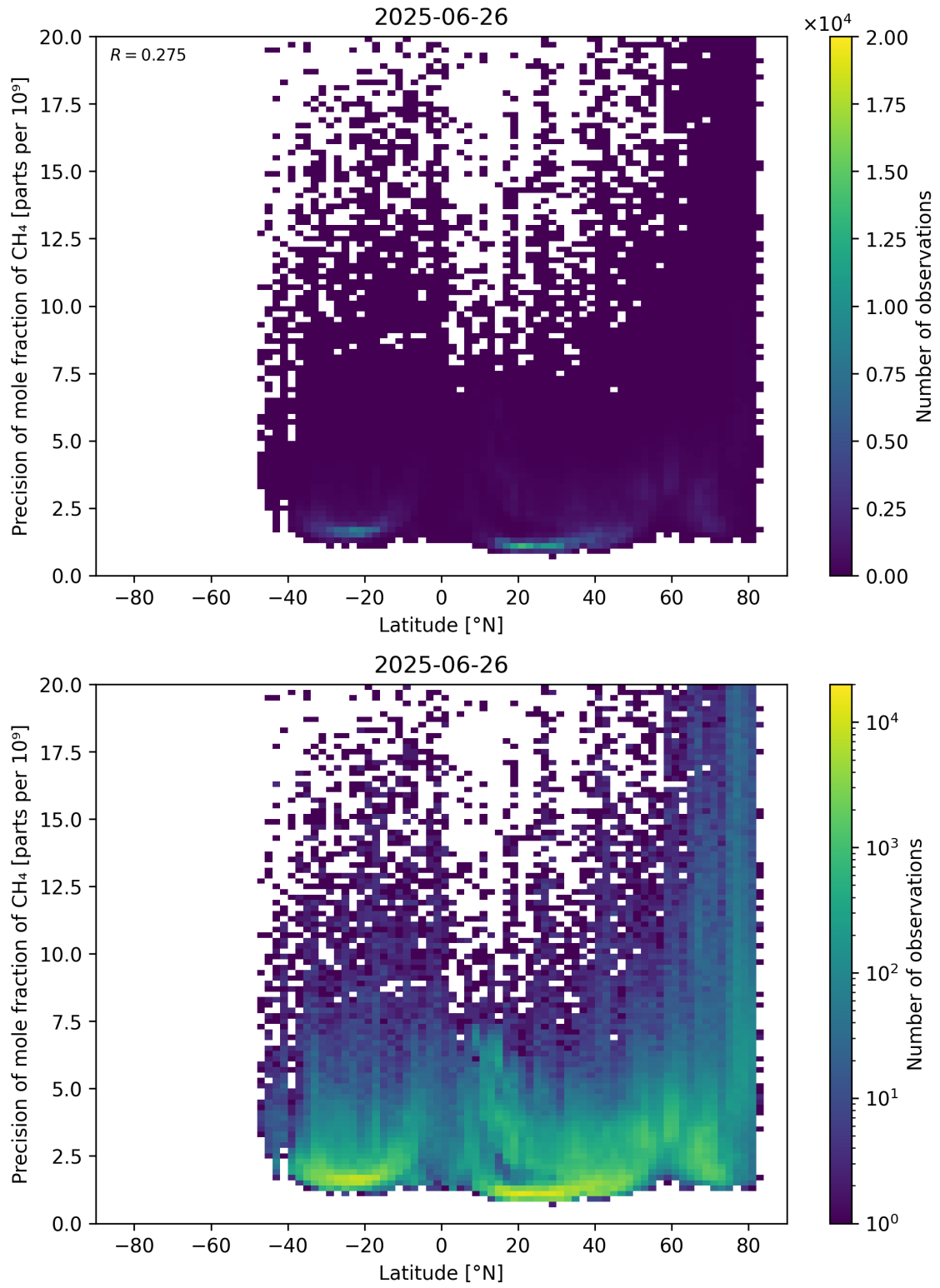
Figure 59: Scatter density plot of “Latitude” against “Precision of mole fraction of \text{CH}_4 ” for 2025-06-25 to 2025-06-27.
