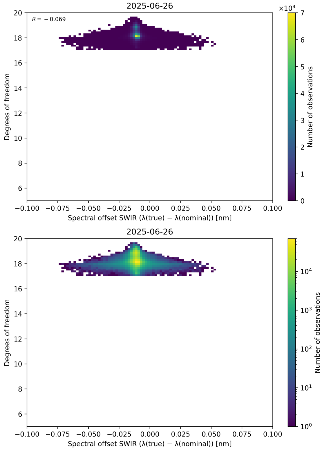
Figure 119: Scatter density plot of “Spectral offset SWIR ( \lambda_{\text{true}} - \lambda_{\text{nominal}} )” against “Degrees of freedom” for 2025-06-25 to 2025-06-27.
