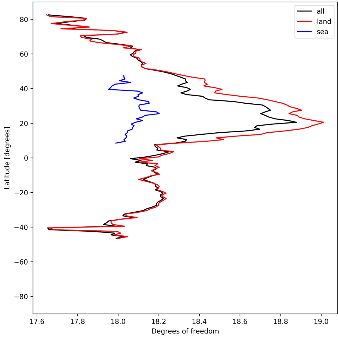
Figure 19: Zonal average of “Degrees of freedom” for 2025-06-25 to 2025-06-27.
