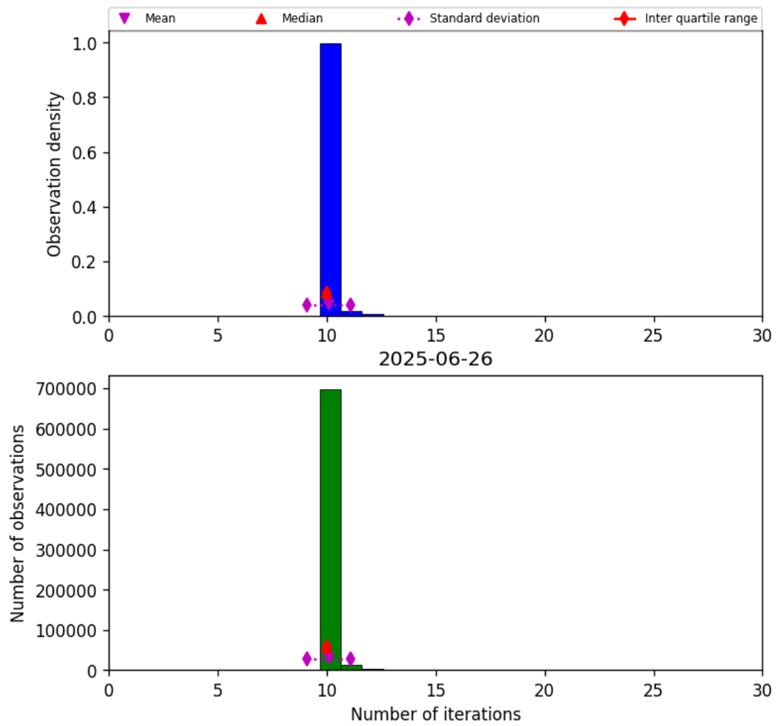
Figure 31: Histogram of “Number of iterations” for 2025-06-25 to 2025-06-27
