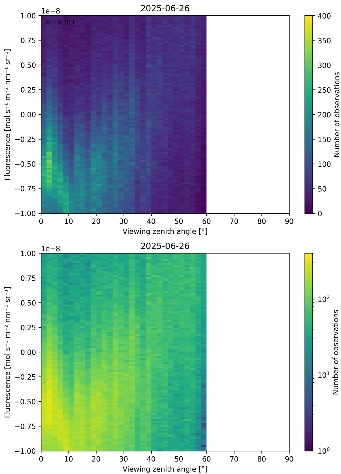
Figure 108: Scatter density plot of “Viewing zenith angle” against “Fluorescence” for 2025-06-25 to 2025-06-27.
