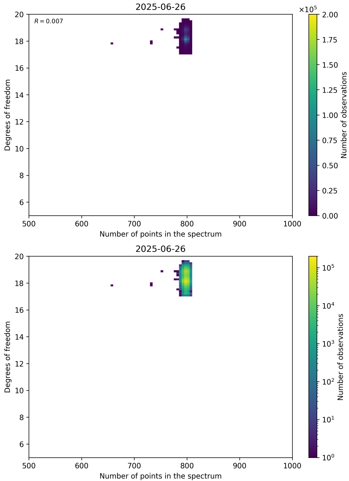
Figure 90: Scatter density plot of “Number of points in the spectrum” against “Degrees of freedom” for 2025-06-25 to 2025-06-27.
