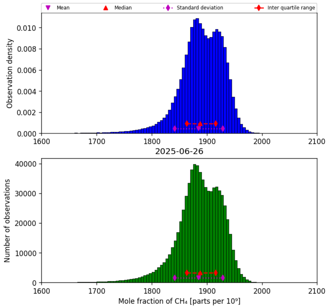
Figure 23: Histogram of “Mole fraction of CH 4 ” for 2025-06-25 to 2025-06-27
