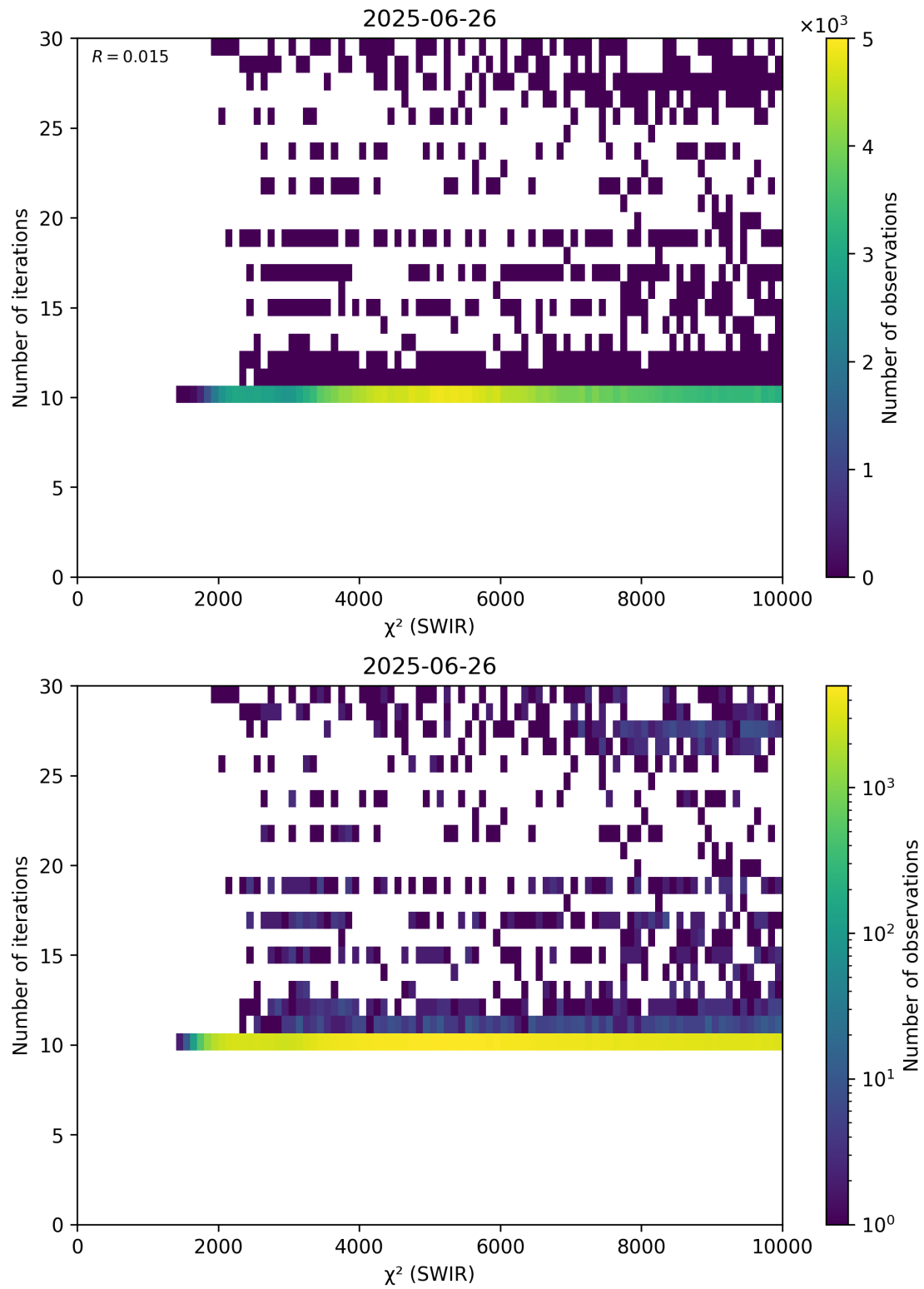
Figure 50: Scatter density plot of “ \chi^2 (SWIR)” against “Number of iterations” for 2025-06-25 to 2025-06-27.
