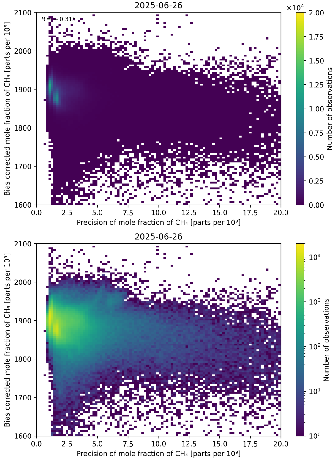
Figure 82: Scatter density plot of “Precision of mole fraction of CH 4 ” against “Bias corrected mole fraction of CH 4 ” for 2025-06-25 to 2025-06-27.
