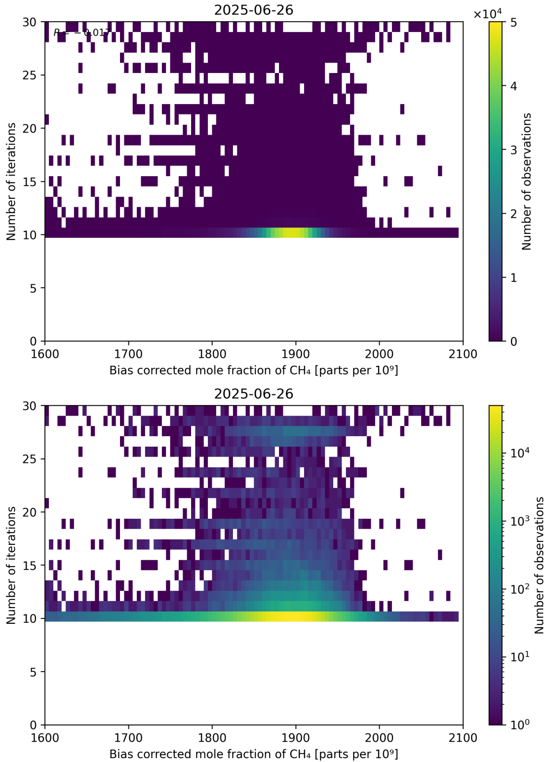
Figure 67: Scatter density plot of “Bias corrected mole fraction of CH 4 ” against “Number of iterations” for 2025-06-25 to 2025-06-27.
