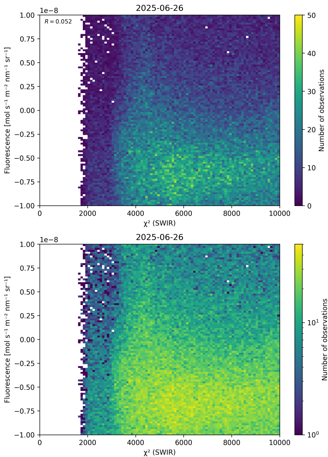
Figure 49: Scatter density plot of “ \chi^2 (SWIR)” against “Fluorescence” for 2025-06-25 to 2025-06-27.
