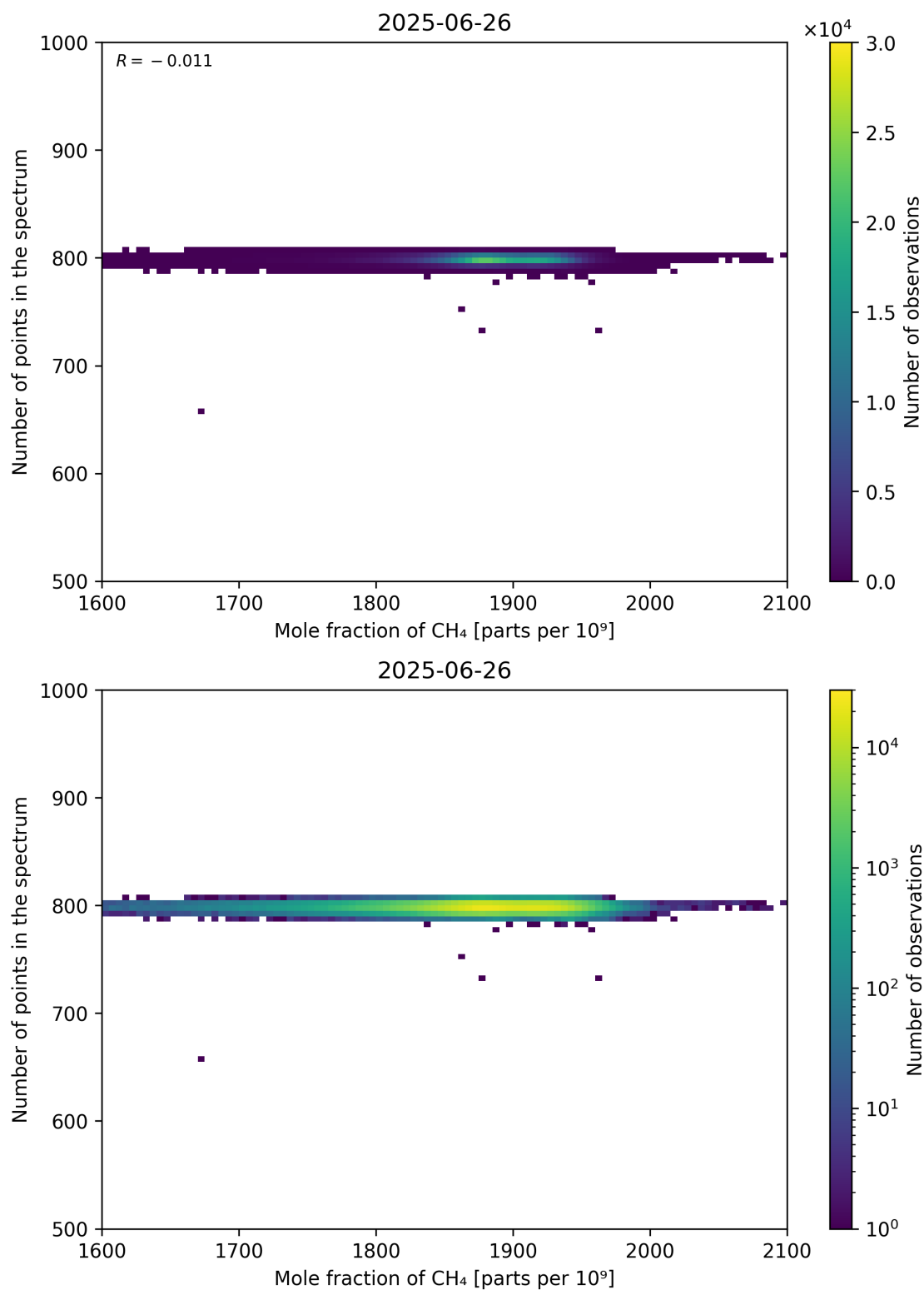
Figure 77: Scatter density plot of “Mole fraction of CH 4 ” against “Number of points in the spectrum” for 2025-06-25 to 2025-06-27.
