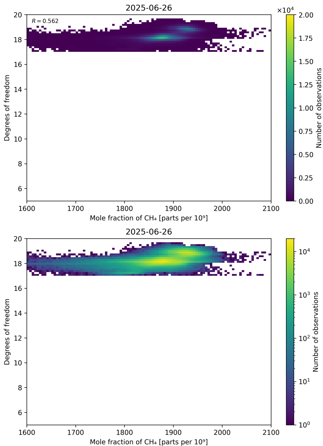
Figure 72: Scatter density plot of “Mole fraction of CH 4 ” against “Degrees of freedom” for 2025-06-25 to 2025-06-27.
