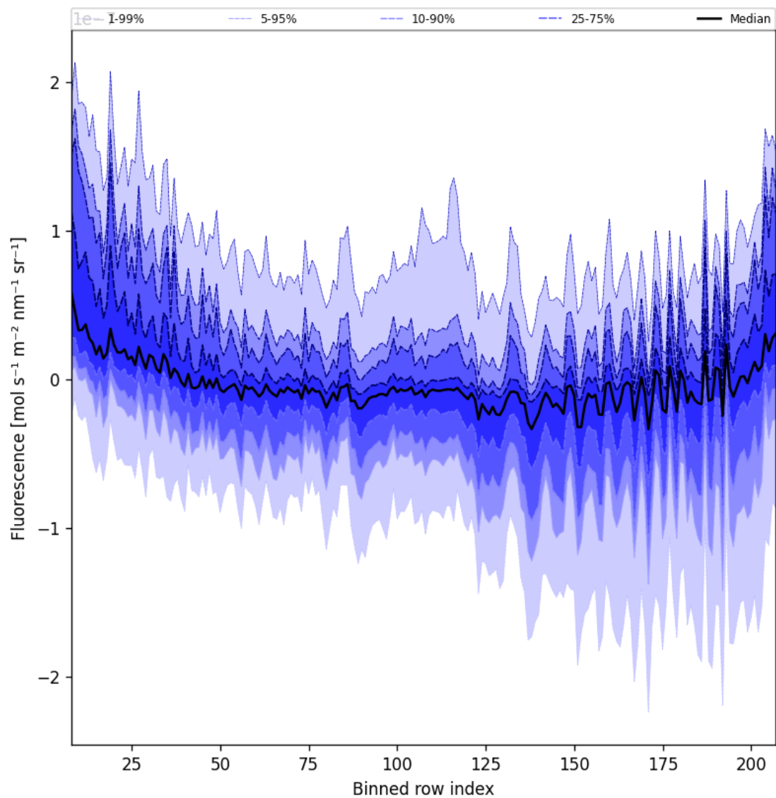
Figure 43: Along track statistics of “Fluorescence” for 2025-06-25 to 2025-06-27
