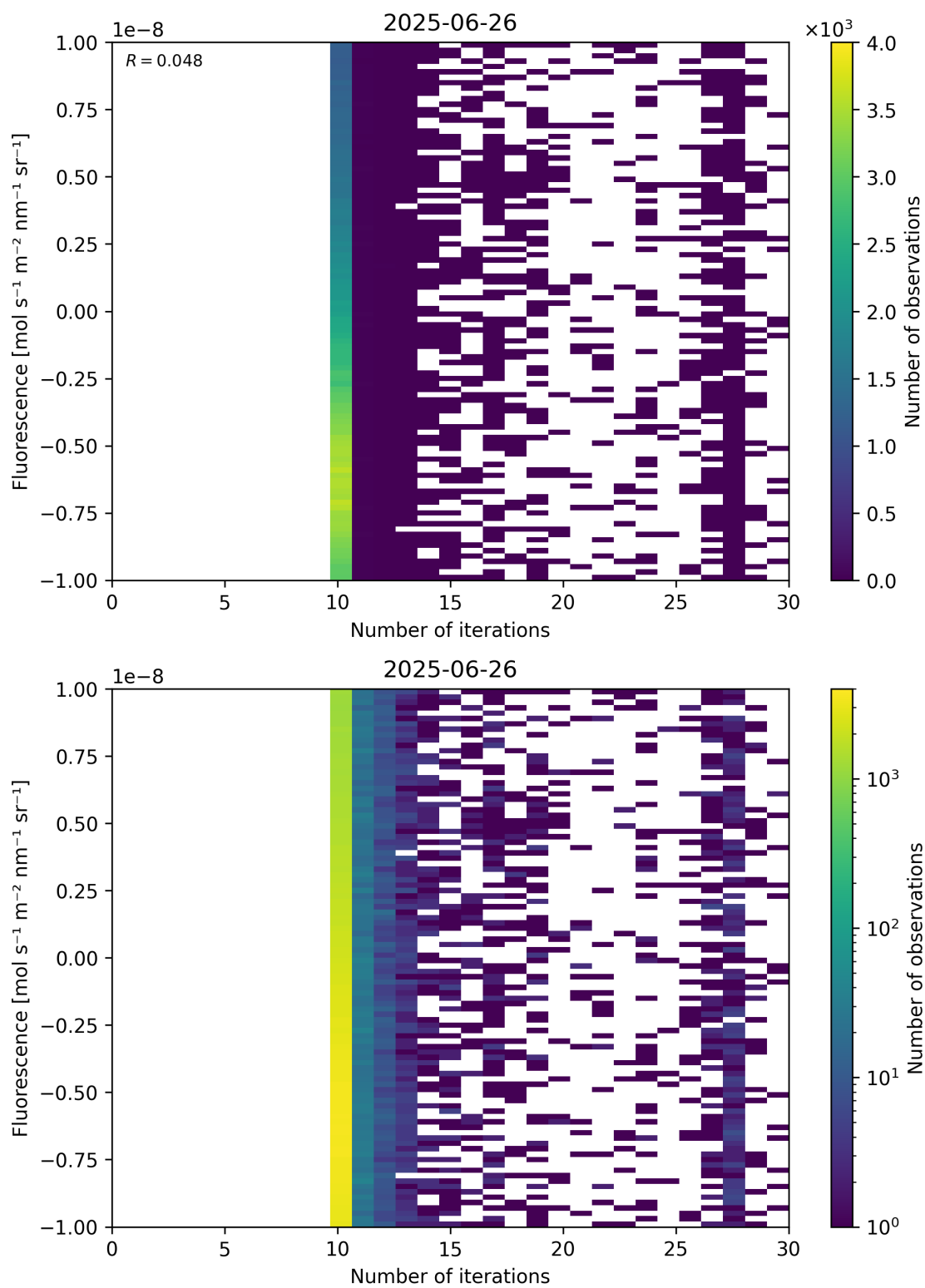
Figure 87: Scatter density plot of “Number of iterations” against “Fluorescence” for 2025-06-25 to 2025-06-27.
