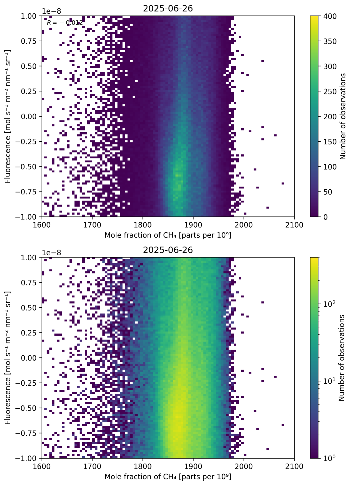
Figure 73: Scatter density plot of “Mole fraction of \text{CH}_4 ” against “Fluorescence” for 2025-06-25 to 2025-06-27.
