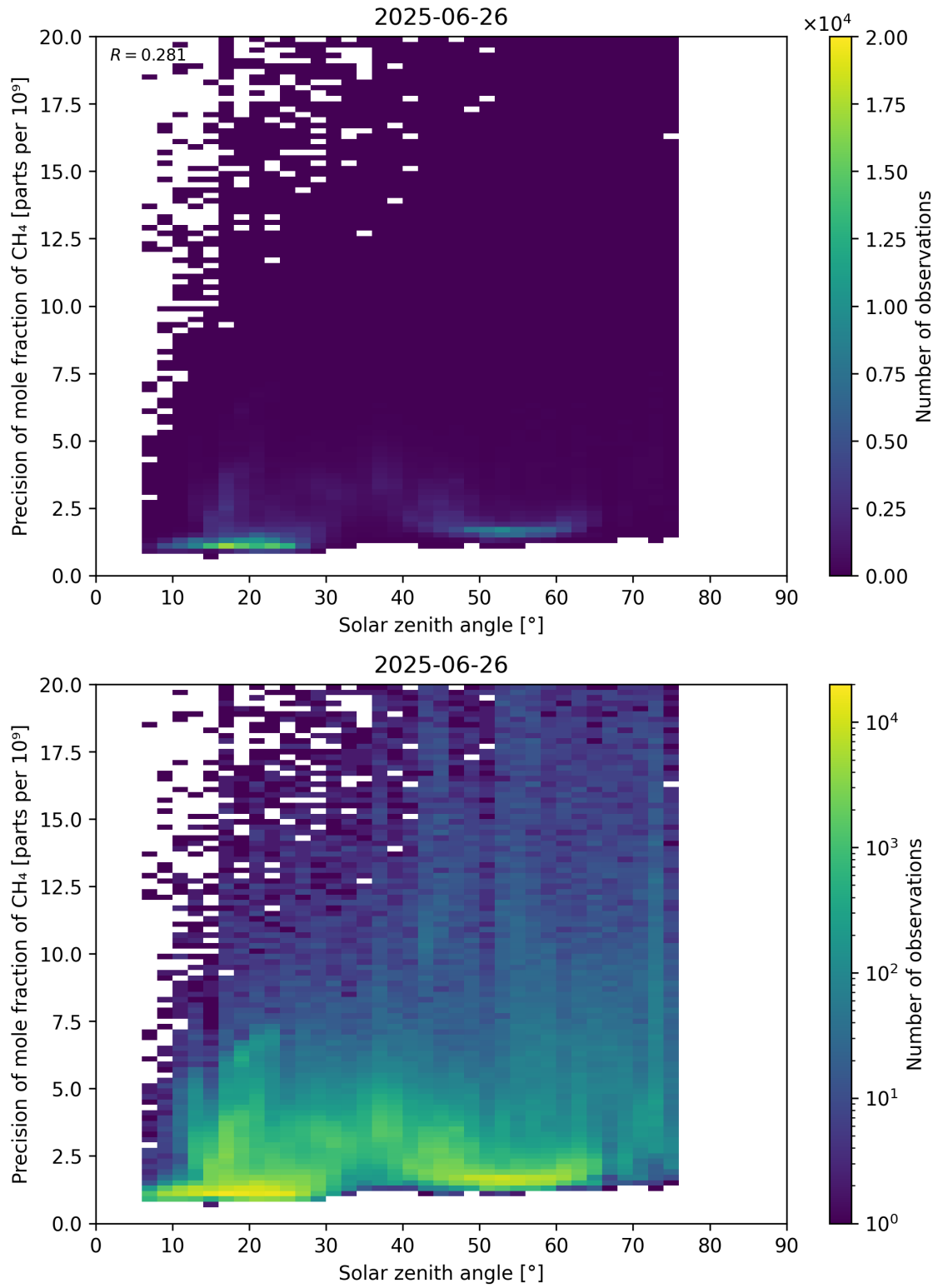
Figure 101: Scatter density plot of “Solar zenith angle” against “Precision of mole fraction of \text{CH}_4 ” for 2025-06-25 to 2025-06-27.
