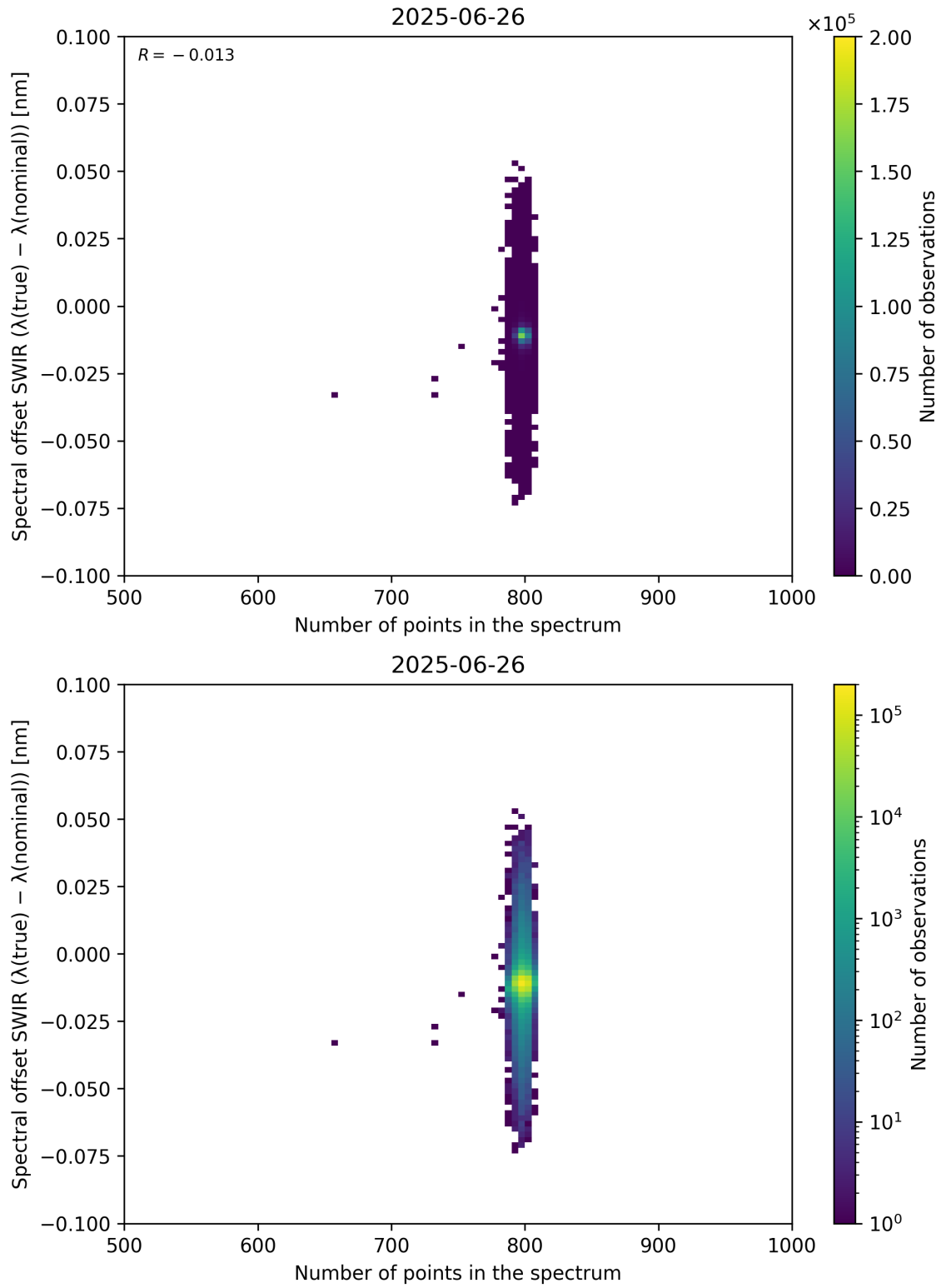
Figure 93: Scatter density plot of “Number of points in the spectrum” against “Spectral offset SWIR ( \lambda_{\text{true}} - \lambda_{\text{nominal}} )” for 2025-06-25 to 2025-06-27.
