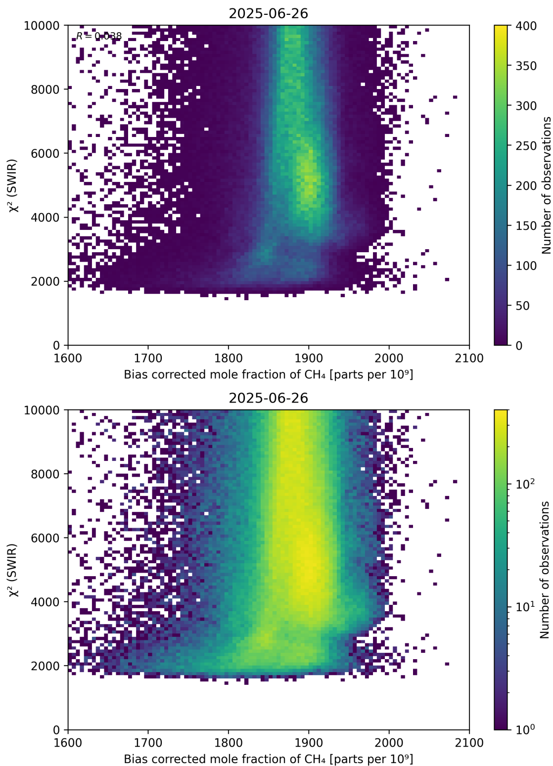
Figure 64: Scatter density plot of “Bias corrected mole fraction of \text{CH}_4 ” against “ \chi^2 (SWIR)” for 2025-06-25 to 2025-06-27.
