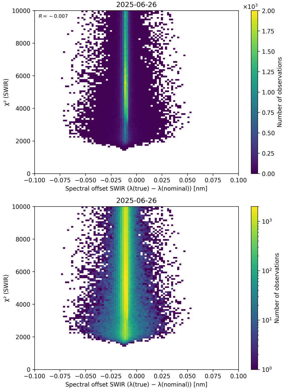
Figure 118: Scatter density plot of “Spectral offset SWIR ( \lambda_{\text{true}} - \lambda_{\text{nominal}} )” against “ \chi^2 (SWIR)” for 2025-06-25 to 2025-06-27.
