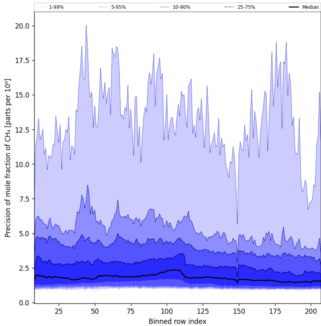
Figure 35: Along track statistics of “Precision of mole fraction of CH 4 ” for 2025-06-25 to 2025-06-27
