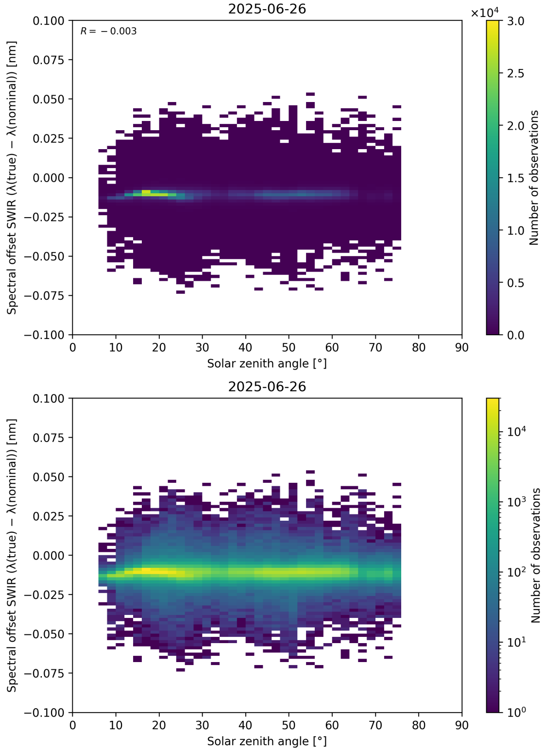
Figure 104: Scatter density plot of “Solar zenith angle” against “Spectral offset SWIR ( \lambda_{\text{true}} - \lambda_{\text{nominal}} )” for 2025-06-25 to 2025-06-27.
