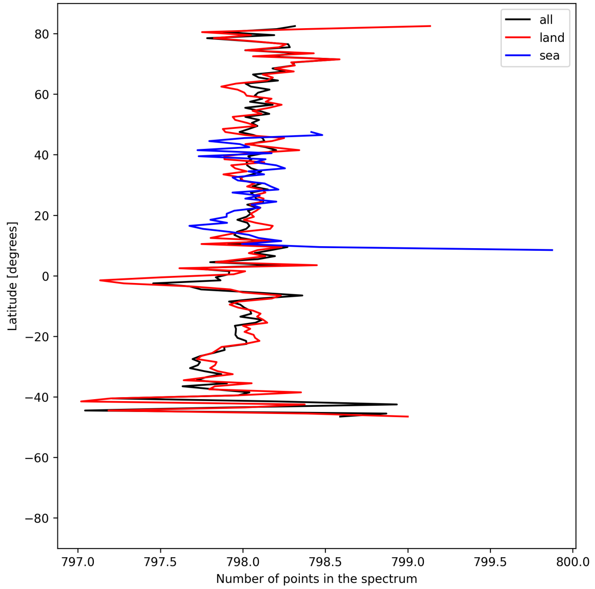
Figure 15: Zonal average of “Number of points in the spectrum” for 2025-06-25 to 2025-06-27.
