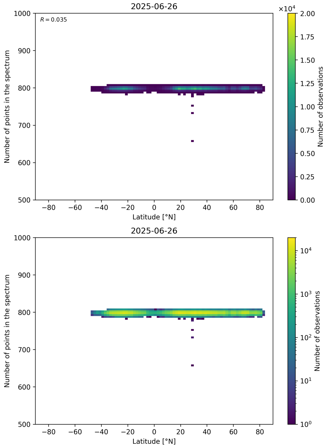
Figure 61: Scatter density plot of “Latitude” against “Number of points in the spectrum” for 2025-06-25 to 2025-06-27.
