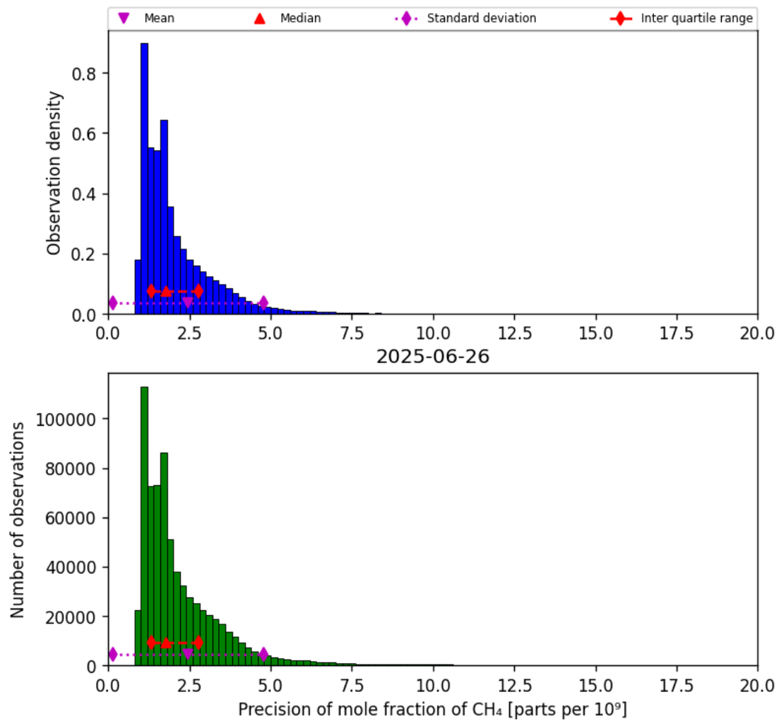
Figure 24: Histogram of “Precision of mole fraction of CH 4 ” for 2025-06-25 to 2025-06-27
