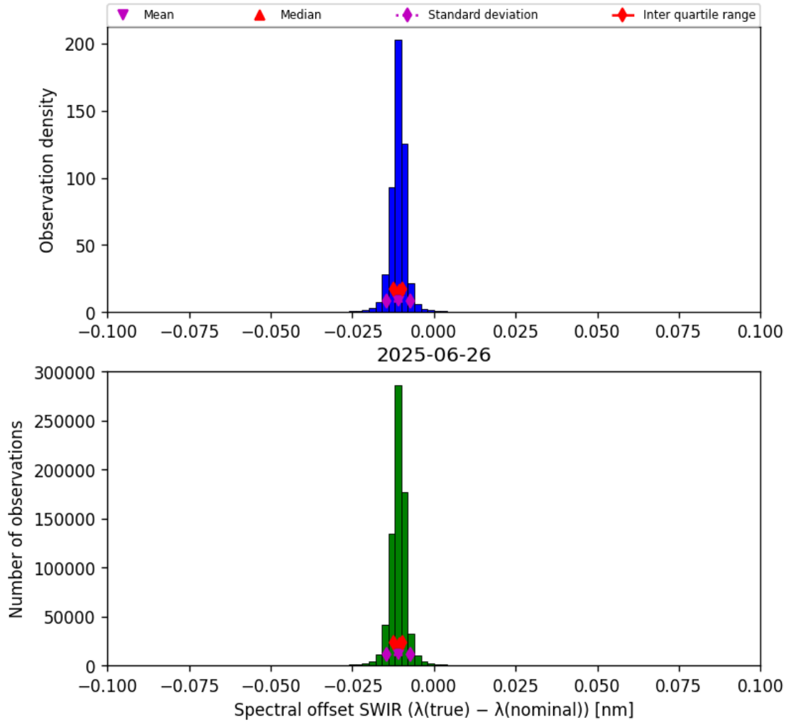
Figure 27: Histogram of “Spectral offset SWIR ( \lambda_{\text{true}} - \lambda_{\text{nominal}} )” for 2025-06-25 to 2025-06-27
