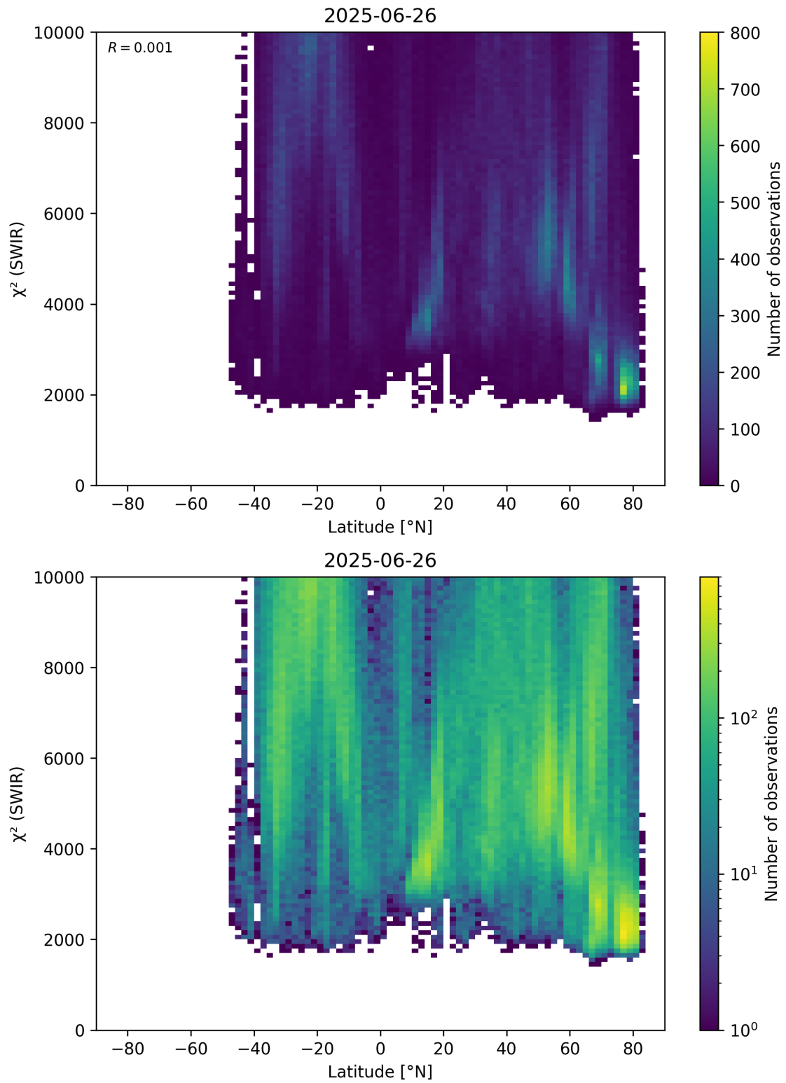
Figure 54: Scatter density plot of “Latitude” against “ \chi^2 (SWIR)” for 2025-06-25 to 2025-06-27.
