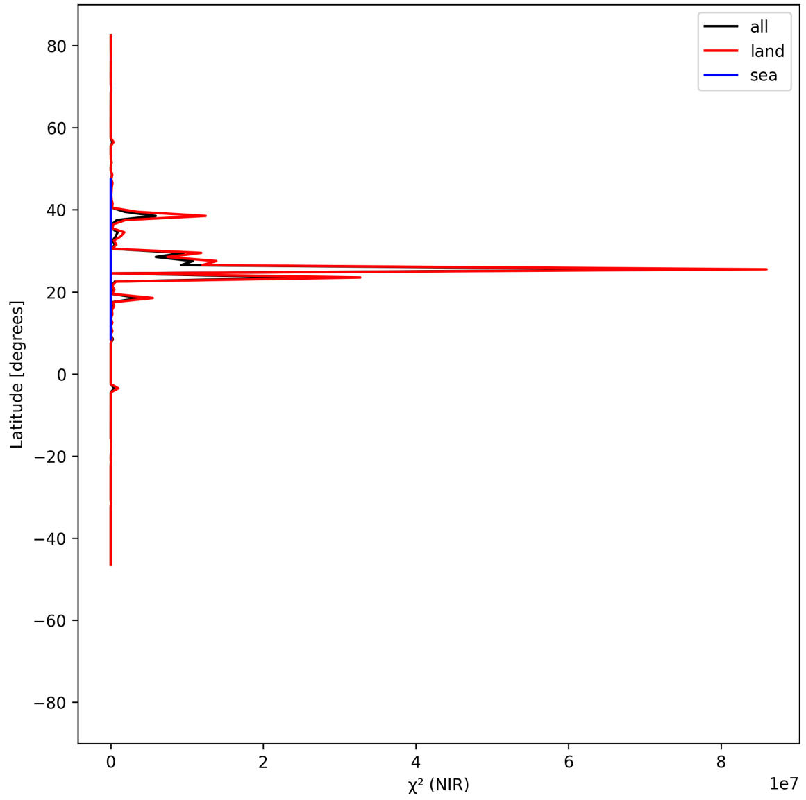
Figure 18: Zonal average of “ \chi^2 (NIR)” for 2025-06-25 to 2025-06-27.
