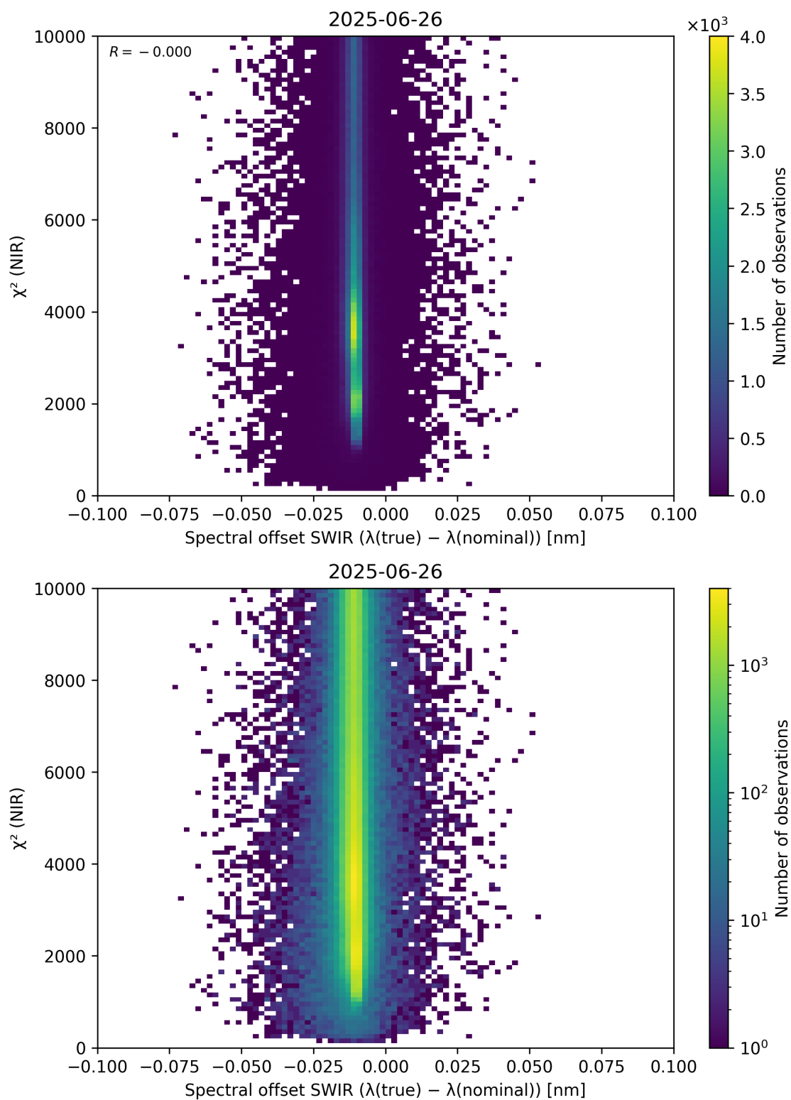
Figure 117: Scatter density plot of “Spectral offset SWIR ( \lambda_{\text{true}} - \lambda_{\text{nominal}} )” against “ \chi^2 (NIR)” for 2025-06-25 to 2025-06-27.
