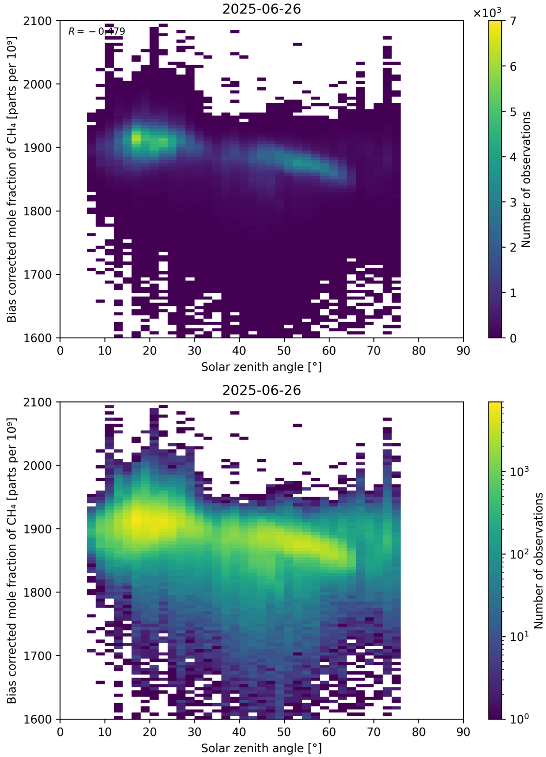
Figure 100: Scatter density plot of “Solar zenith angle” against “Bias corrected mole fraction of CH 4 ” for 2025-06-25 to 2025-06-27.
