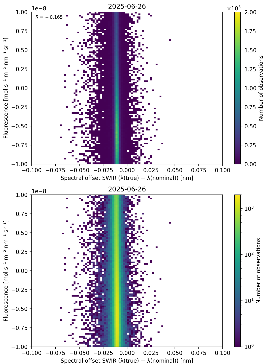
Figure 120: Scatter density plot of “Spectral offset SWIR ( \lambda_{\text{true}} - \lambda_{\text{nominal}} )” against “Fluorescence” for 2025-06-25 to 2025-06-27.
