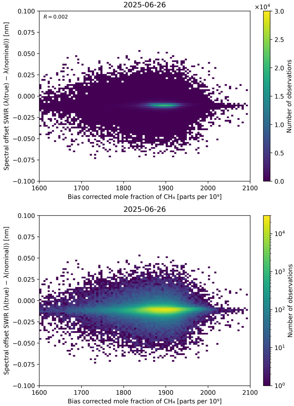
Figure 69: Scatter density plot of “Bias corrected mole fraction of \text{CH}_4 ” against “Spectral offset SWIR ( \lambda_{\text{true}} - \lambda_{\text{nominal}} )” for 2025-06-25 to 2025-06-27.
