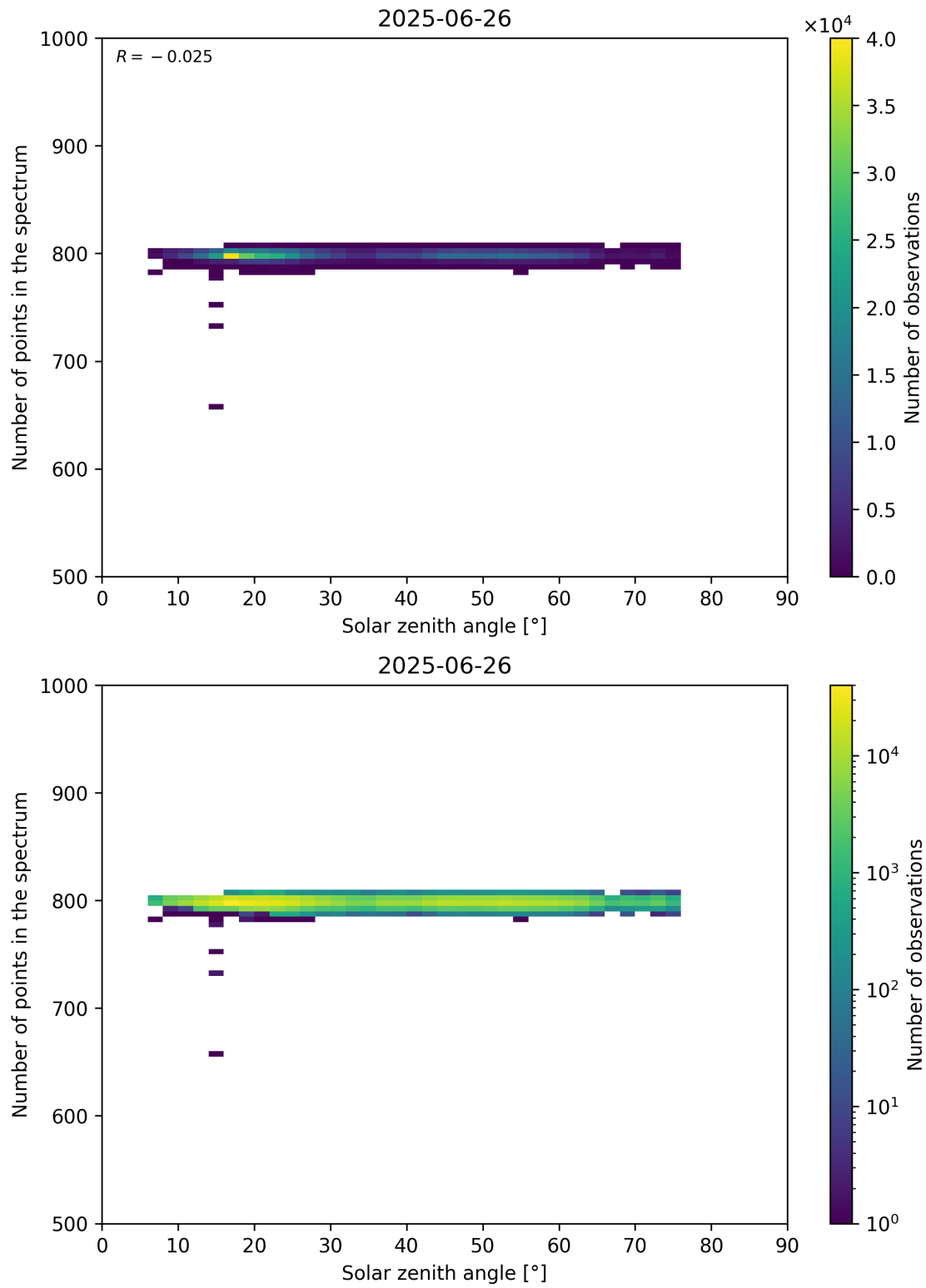
Figure 103: Scatter density plot of “Solar zenith angle” against “Number of points in the spectrum” for 2025-06-25 to 2025-06-27.
