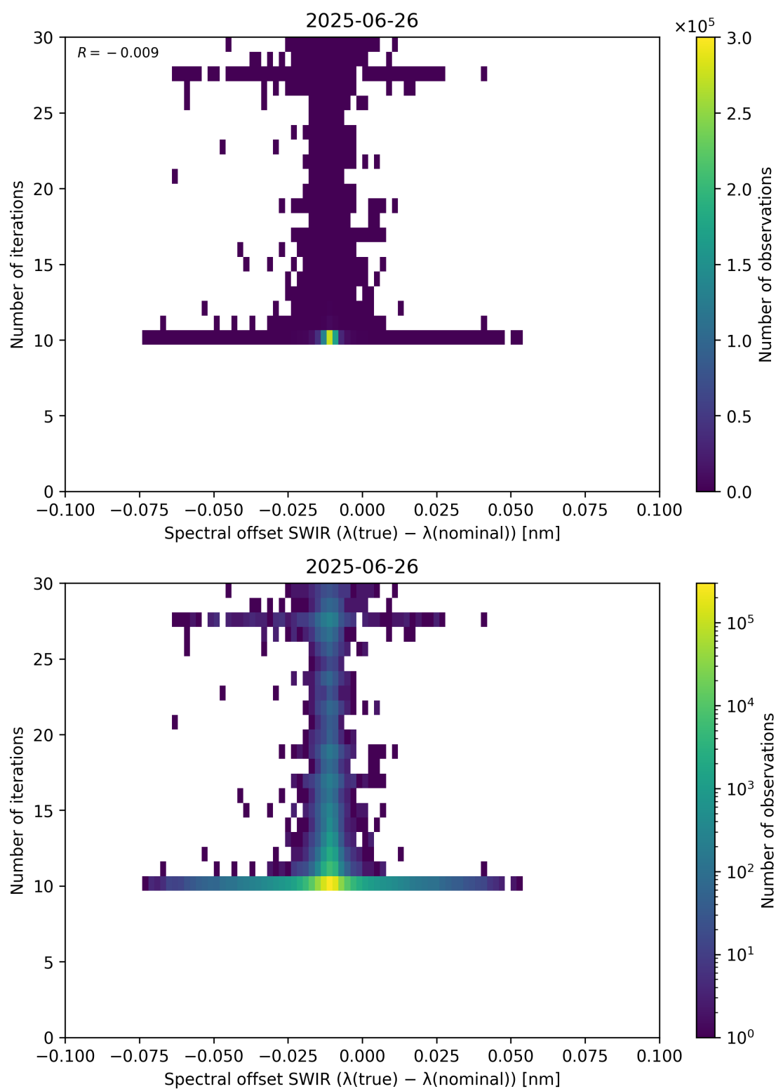
Figure 121: Scatter density plot of “Spectral offset SWIR ( \lambda_{\text{true}} - \lambda_{\text{nominal}} )” against “Number of iterations” for 2025-06-25 to 2025-06-27.
