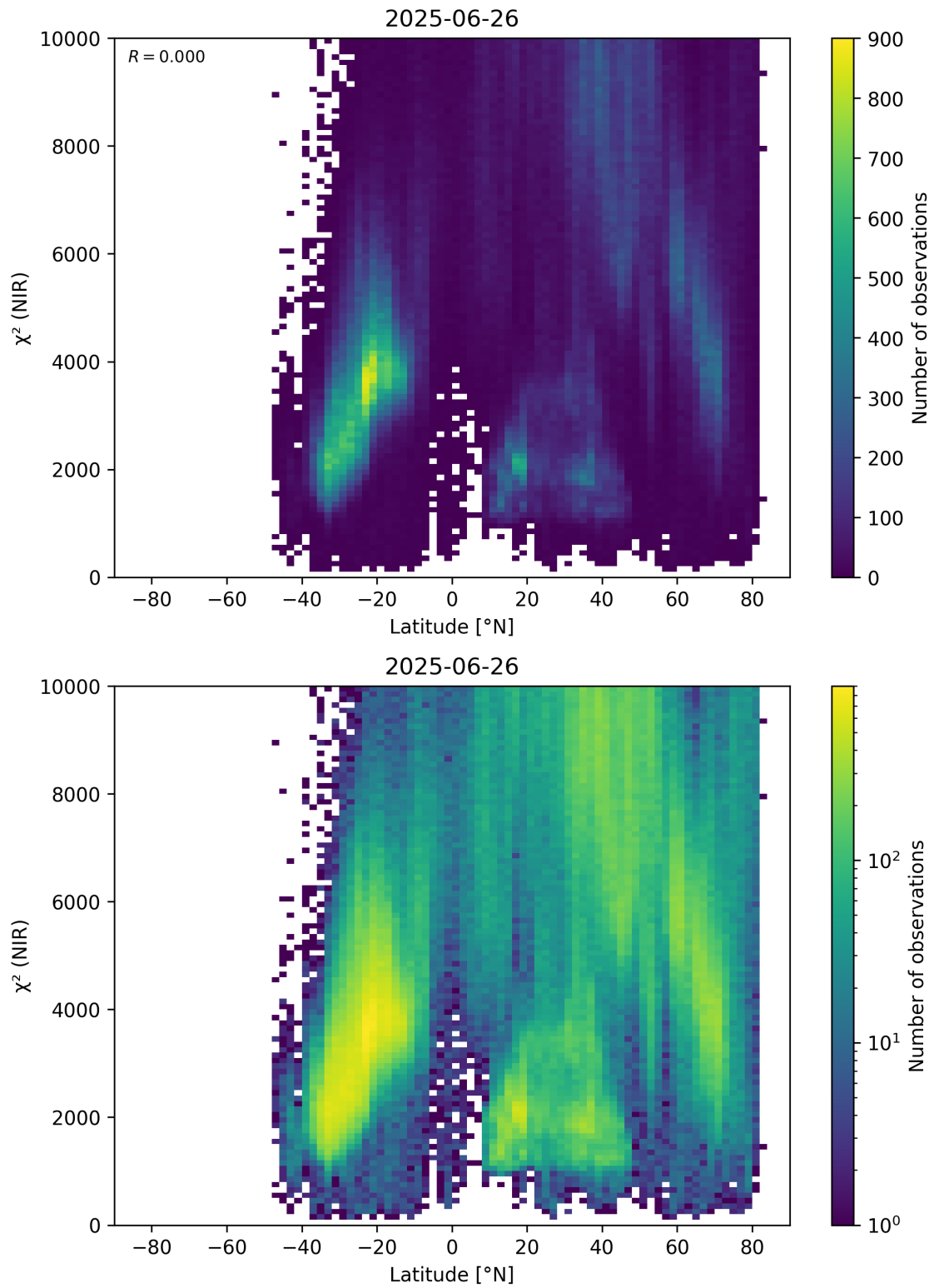
Figure 53: Scatter density plot of “Latitude” against “ \chi^2 (NIR)” for 2025-06-25 to 2025-06-27.
