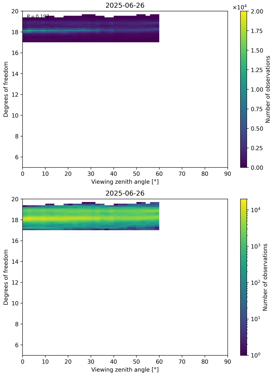
Figure 107: Scatter density plot of “Viewing zenith angle” against “Degrees of freedom” for 2025-06-25 to 2025-06-27.
