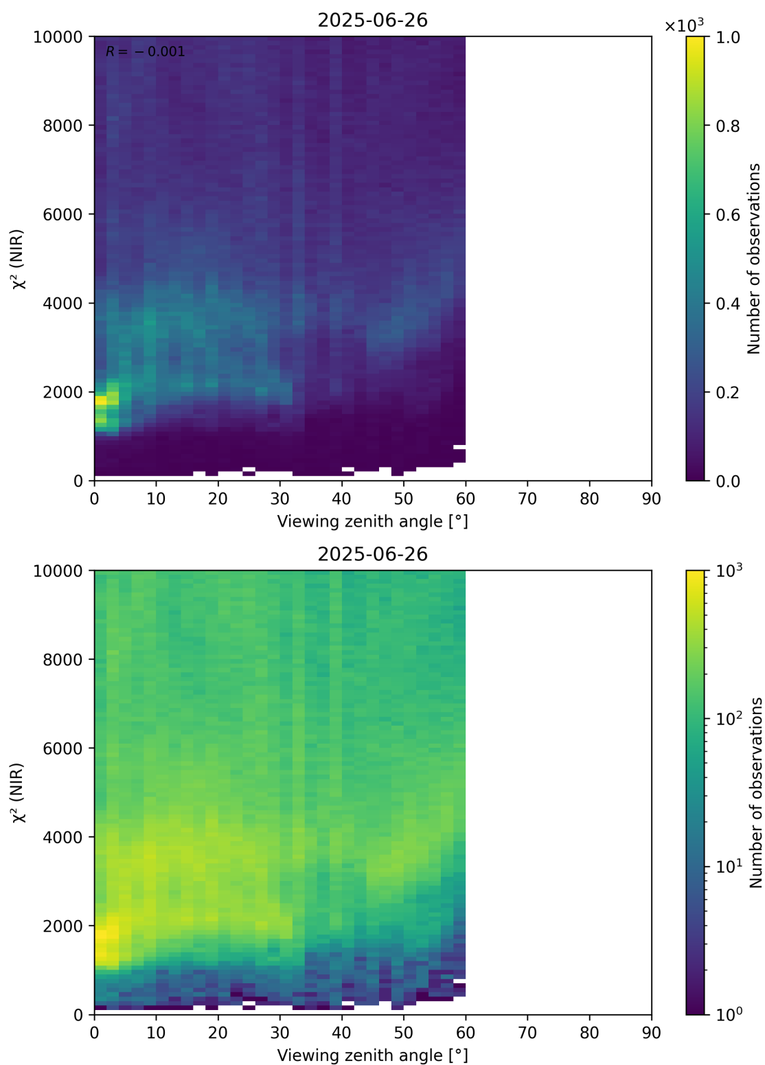
Figure 105: Scatter density plot of “Viewing zenith angle” against “ \chi^2 (NIR)” for 2025-06-25 to 2025-06-27.
