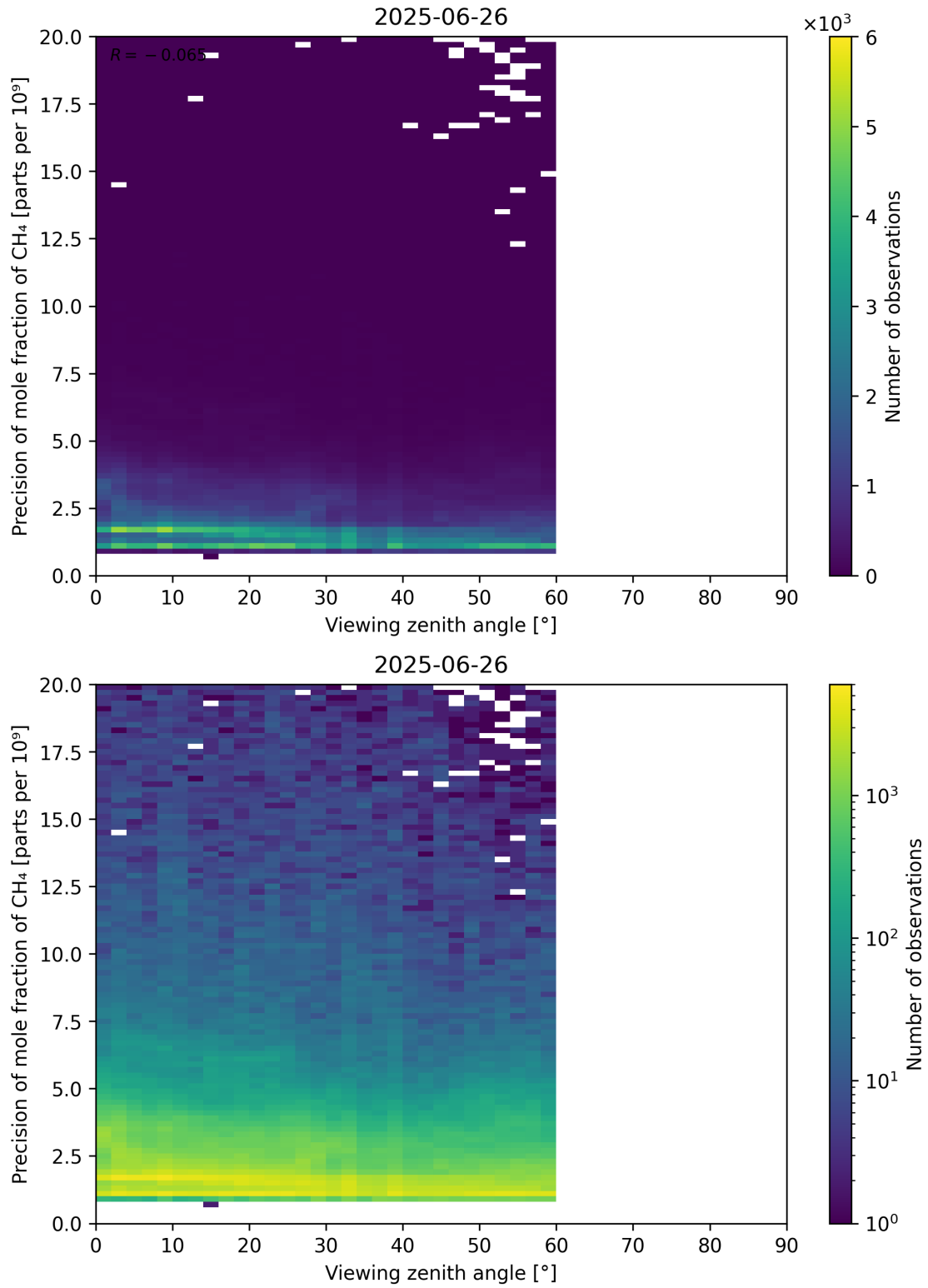
Figure 112: Scatter density plot of “Viewing zenith angle” against “Precision of mole fraction of CH 4 ” for 2025-06-25 to 2025-06-27.
