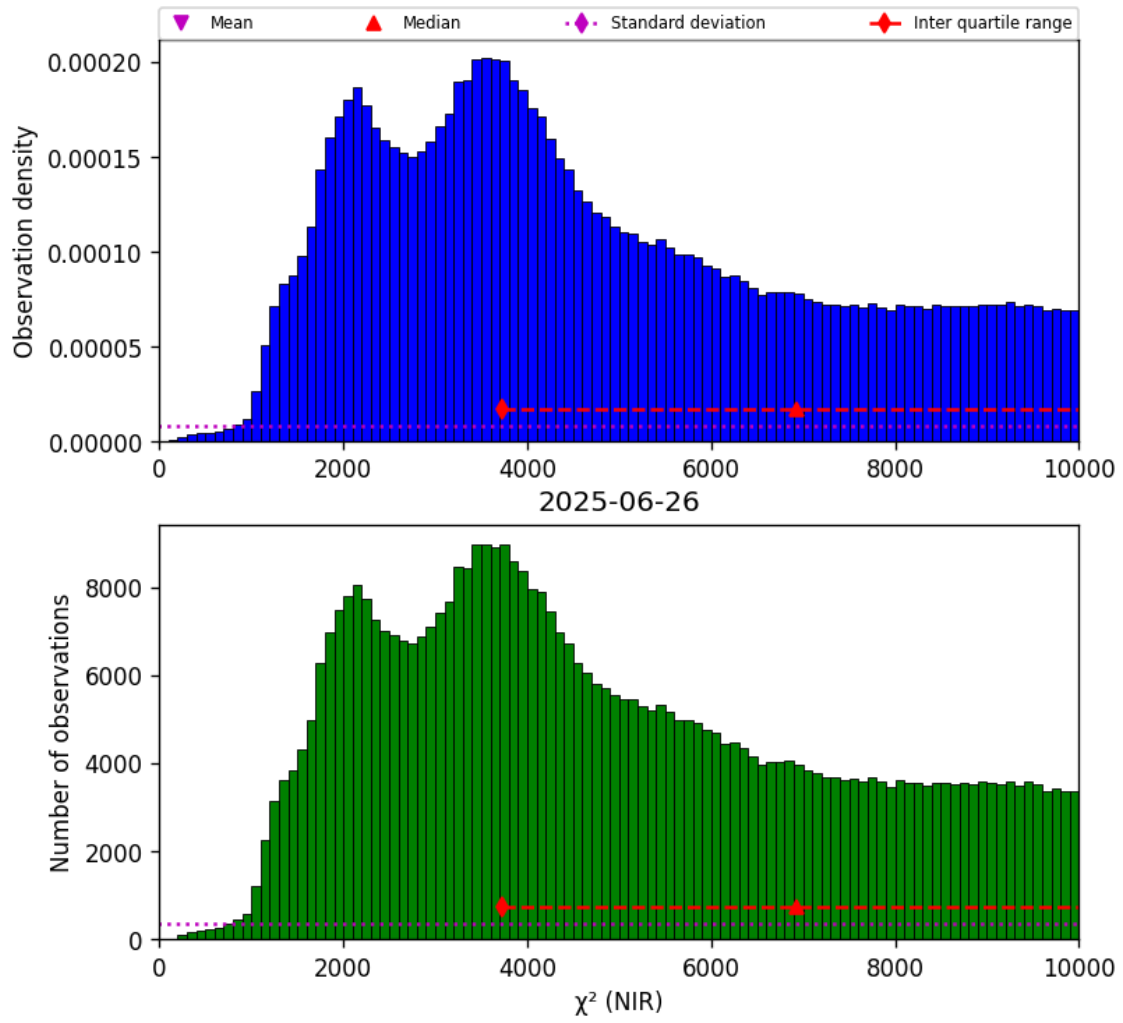
Figure 29: Histogram of “ \chi^2 (NIR)” for 2025-06-25 to 2025-06-27
