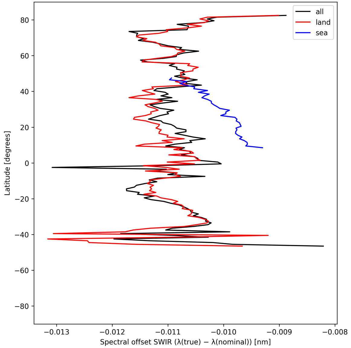
Figure 16: Zonal average of “Spectral offset SWIR ( \lambda_{\text{true}} - \lambda_{\text{nominal}} )” for 2025-06-25 to 2025-06-27.
