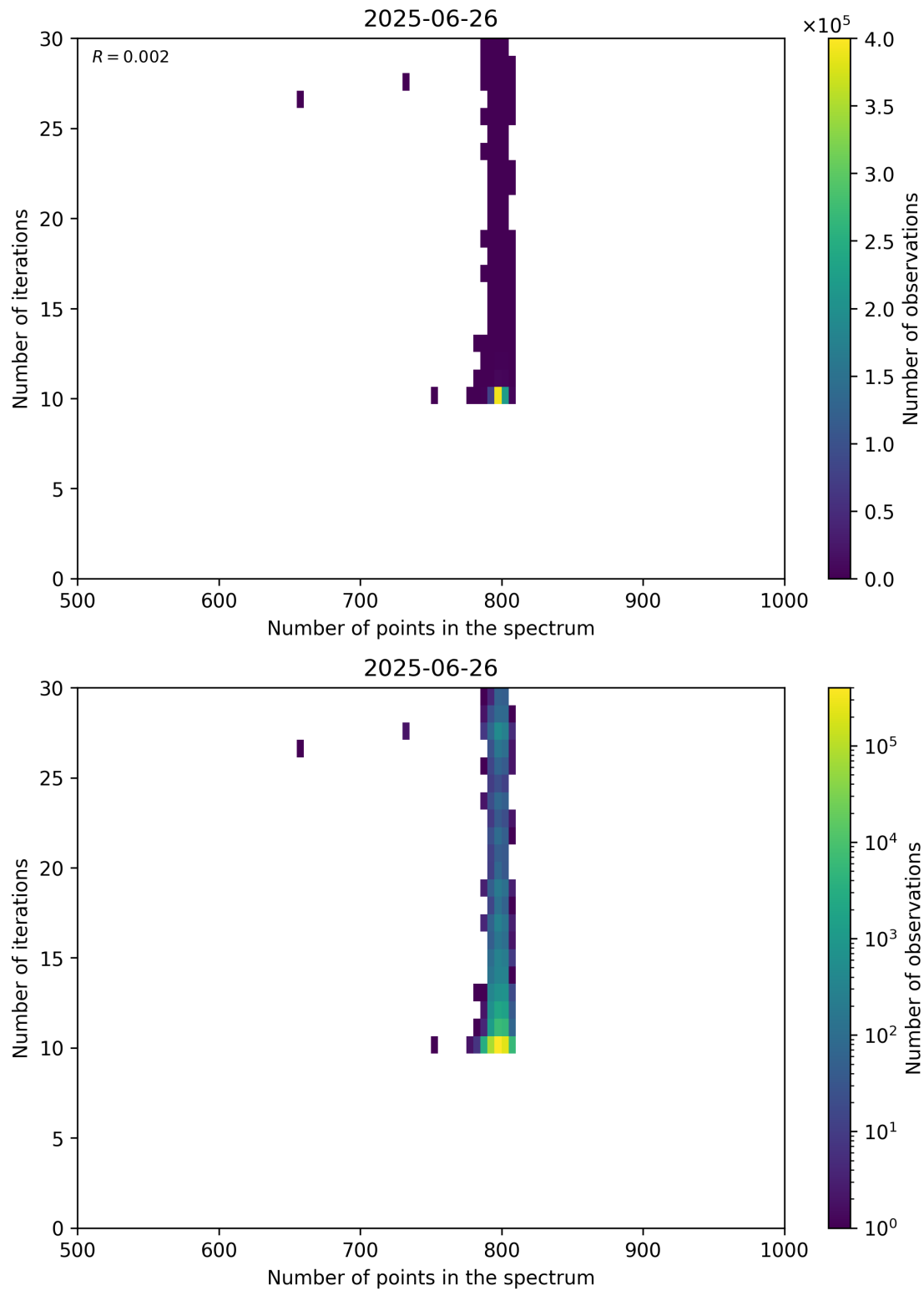
Figure 92: Scatter density plot of “Number of points in the spectrum” against “Number of iterations” for 2025-06-25 to 2025-06-27.
