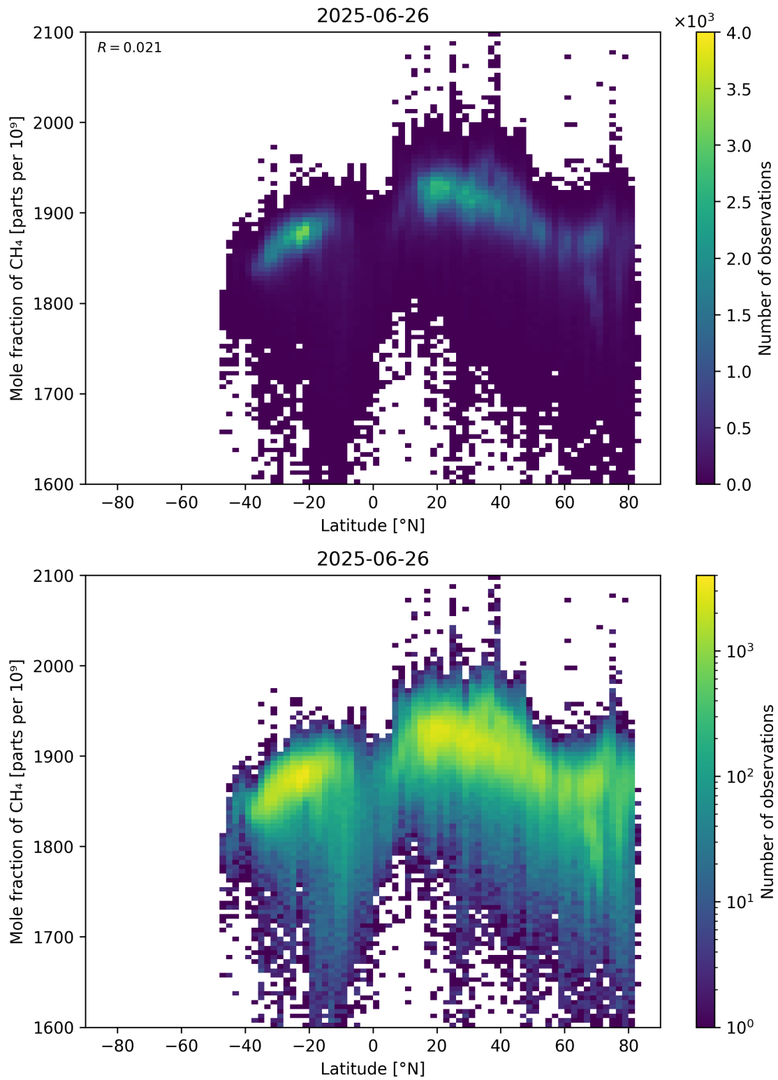
Figure 57: Scatter density plot of “Latitude” against “Mole fraction of \text{CH}_4 ” for 2025-06-25 to 2025-06-27.
