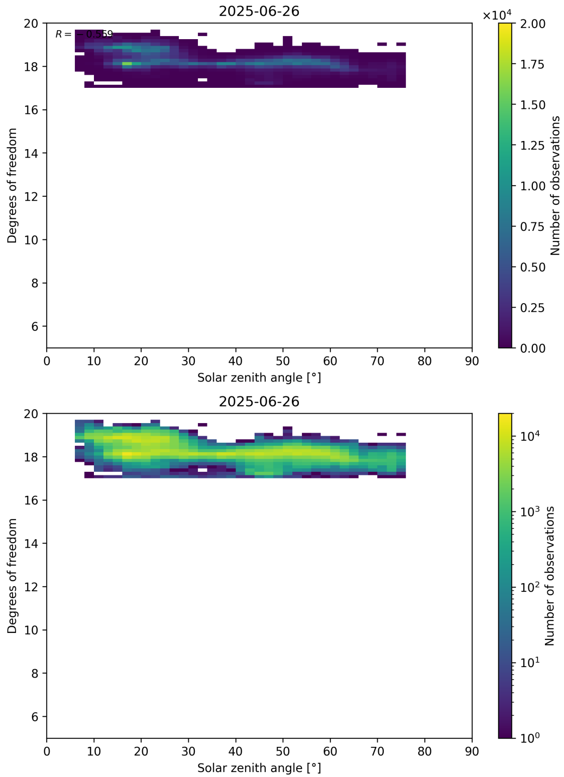
Figure 96: Scatter density plot of “Solar zenith angle” against “Degrees of freedom” for 2025-06-25 to 2025-06-27.
