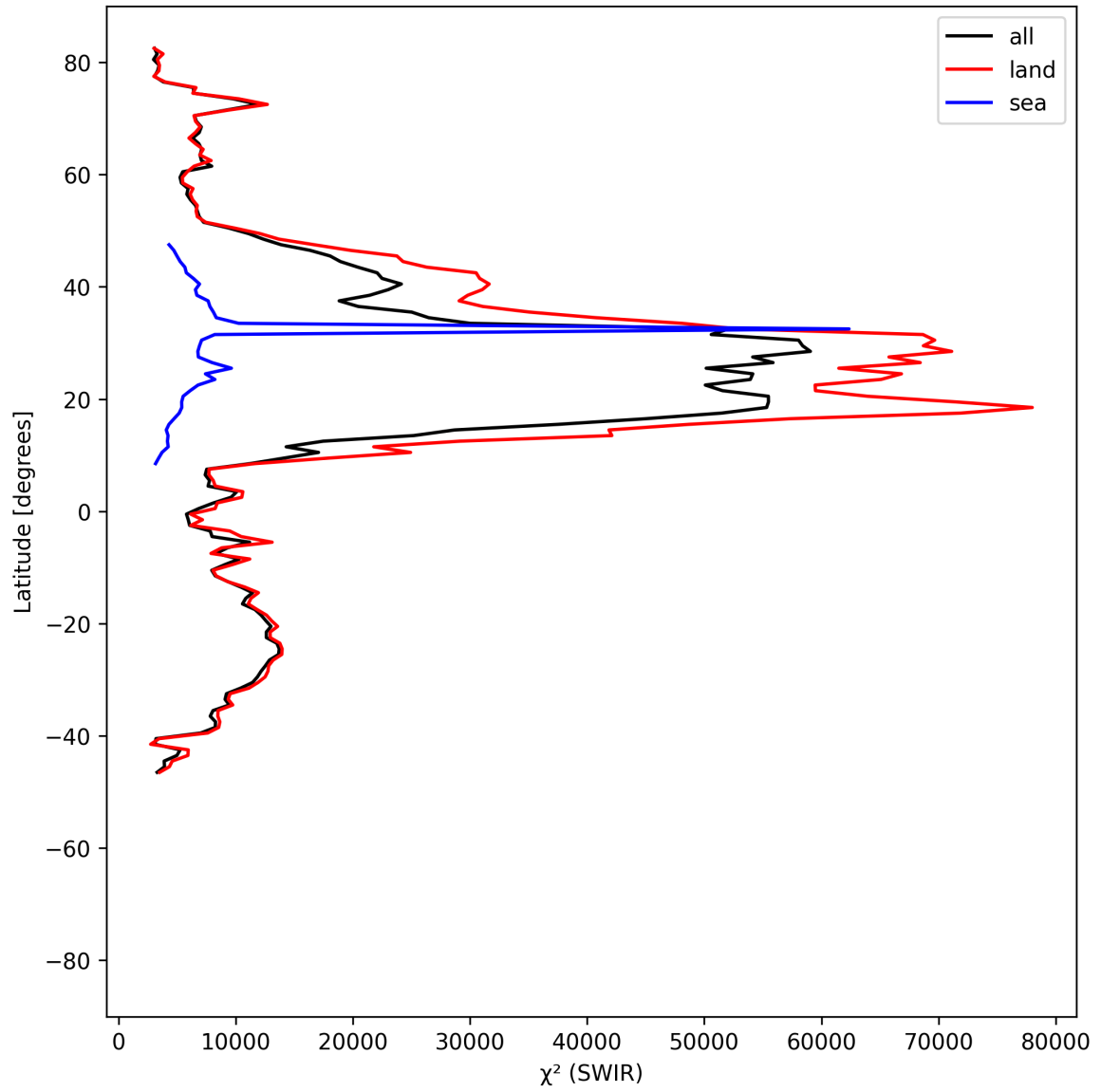
Figure 17: Zonal average of “ \chi^2 (SWIR)” for 2025-06-25 to 2025-06-27.
