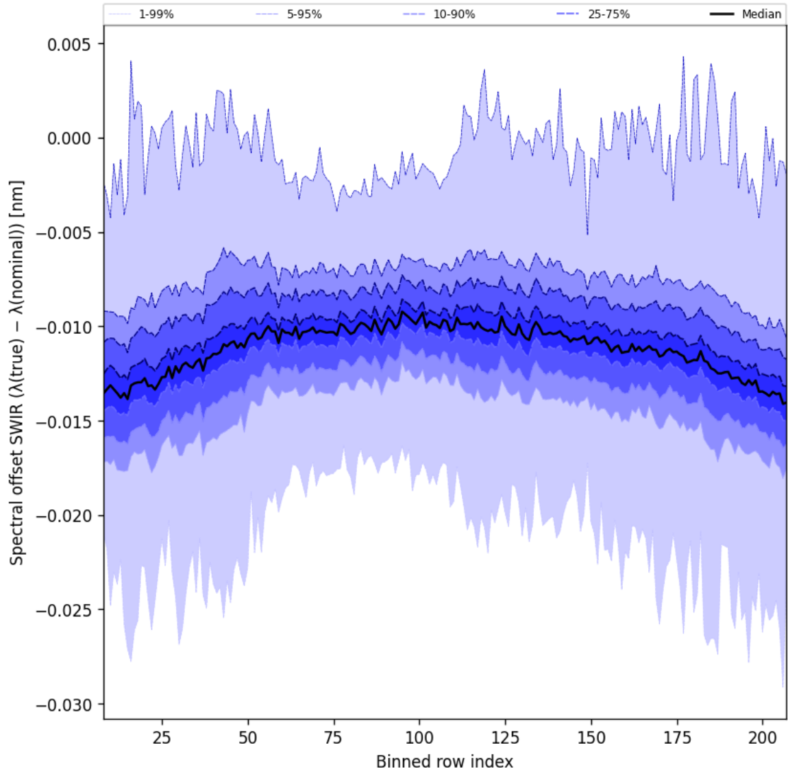
Figure 38: Along track statistics of “Spectral offset SWIR ( \lambda_{\text{true}} - \lambda_{\text{nominal}} )” for 2025-06-25 to 2025-06-27
