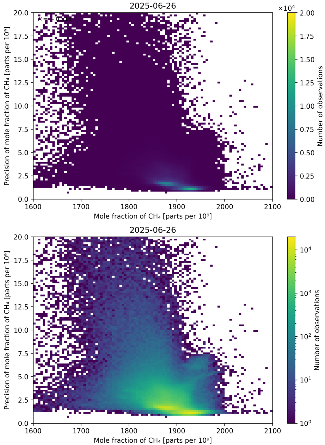
Figure 75: Scatter density plot of “Mole fraction of CH 4 ” against “Precision of mole fraction of CH 4 ” for 2025-06-25 to 2025-06-27.
