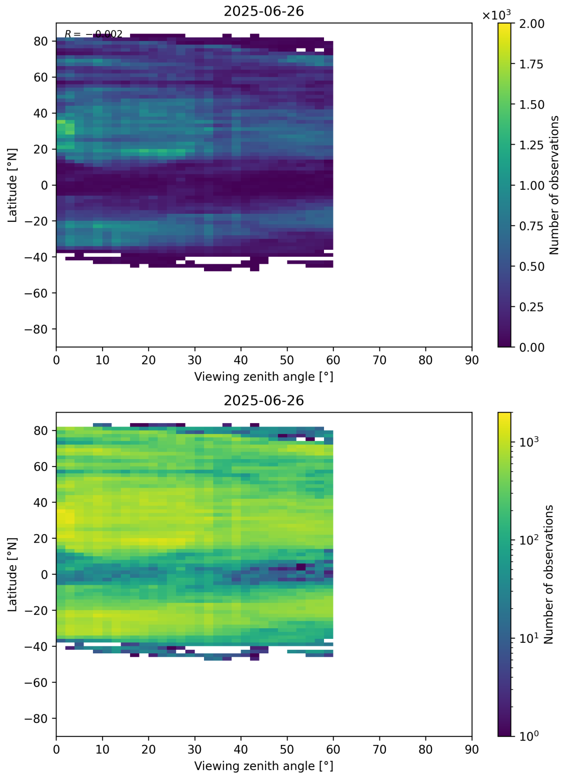
Figure 109: Scatter density plot of “Viewing zenith angle” against “Latitude” for 2025-06-25 to 2025-06-27.
