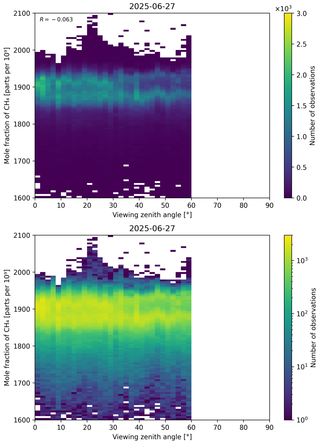
Figure 110: Scatter density plot of “Viewing zenith angle” against “Mole fraction of CH 4 ” for 2025-06-27 to 2025-06-28.
