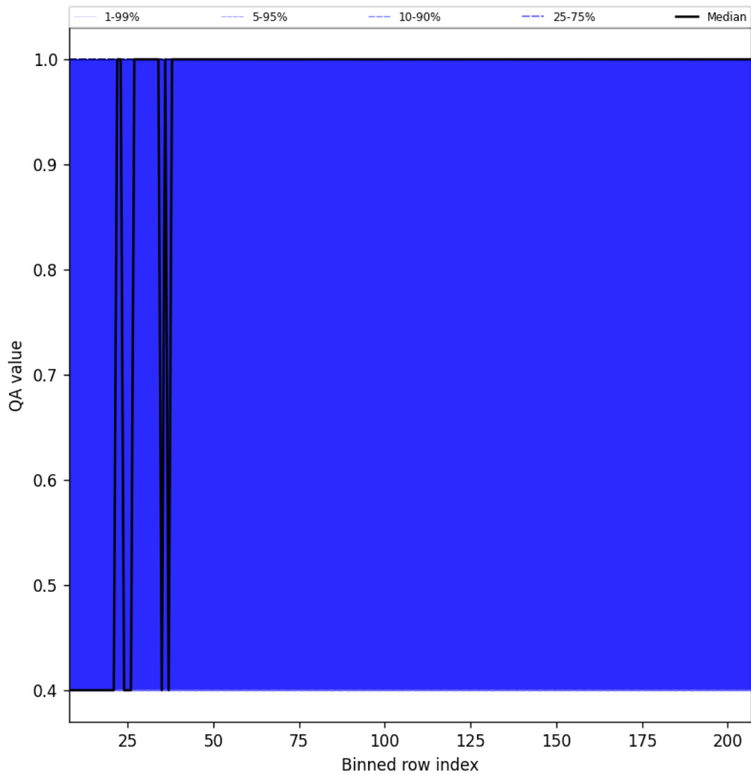
Figure 33: Along track statistics of “QA value” for 2025-06-27 to 2025-06-28
