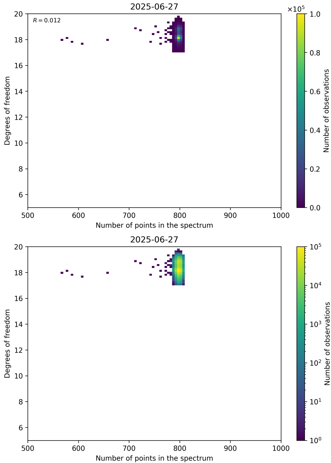
Figure 90: Scatter density plot of “Number of points in the spectrum” against “Degrees of freedom” for 2025-06-27 to 2025-06-28.
