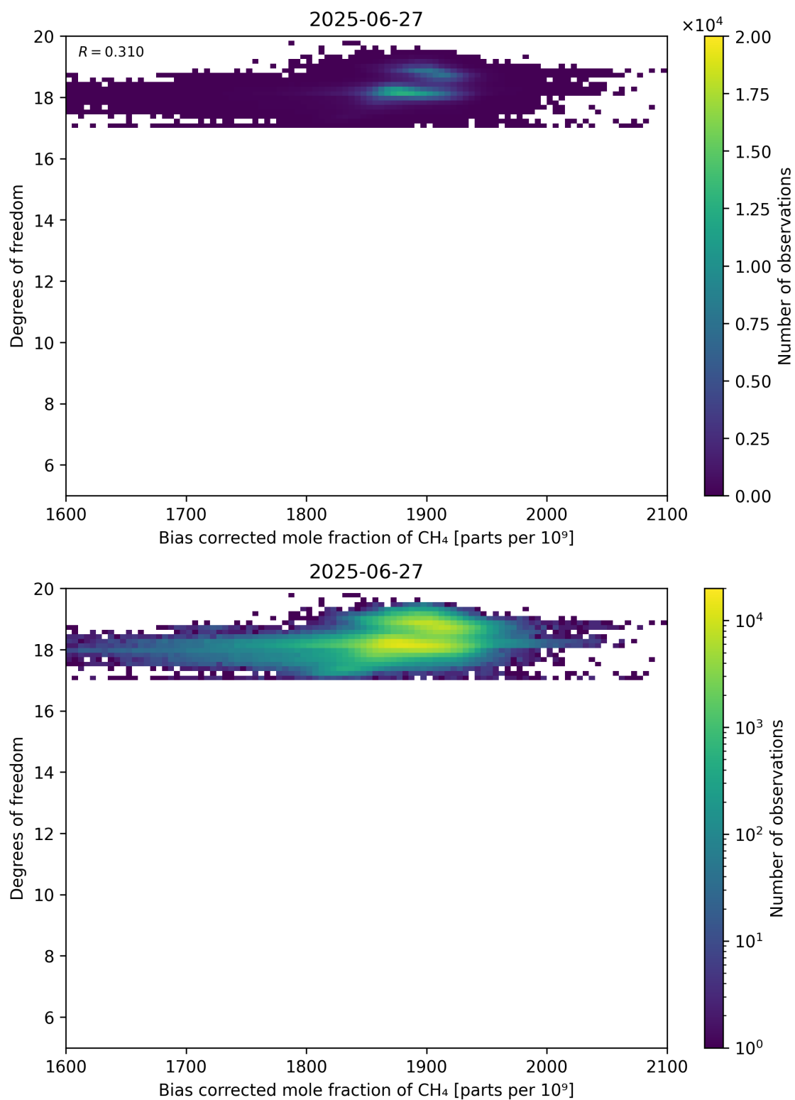
Figure 65: Scatter density plot of “Bias corrected mole fraction of \text{CH}_4 ” against “Degrees of freedom” for 2025-06-27 to 2025-06-28.
