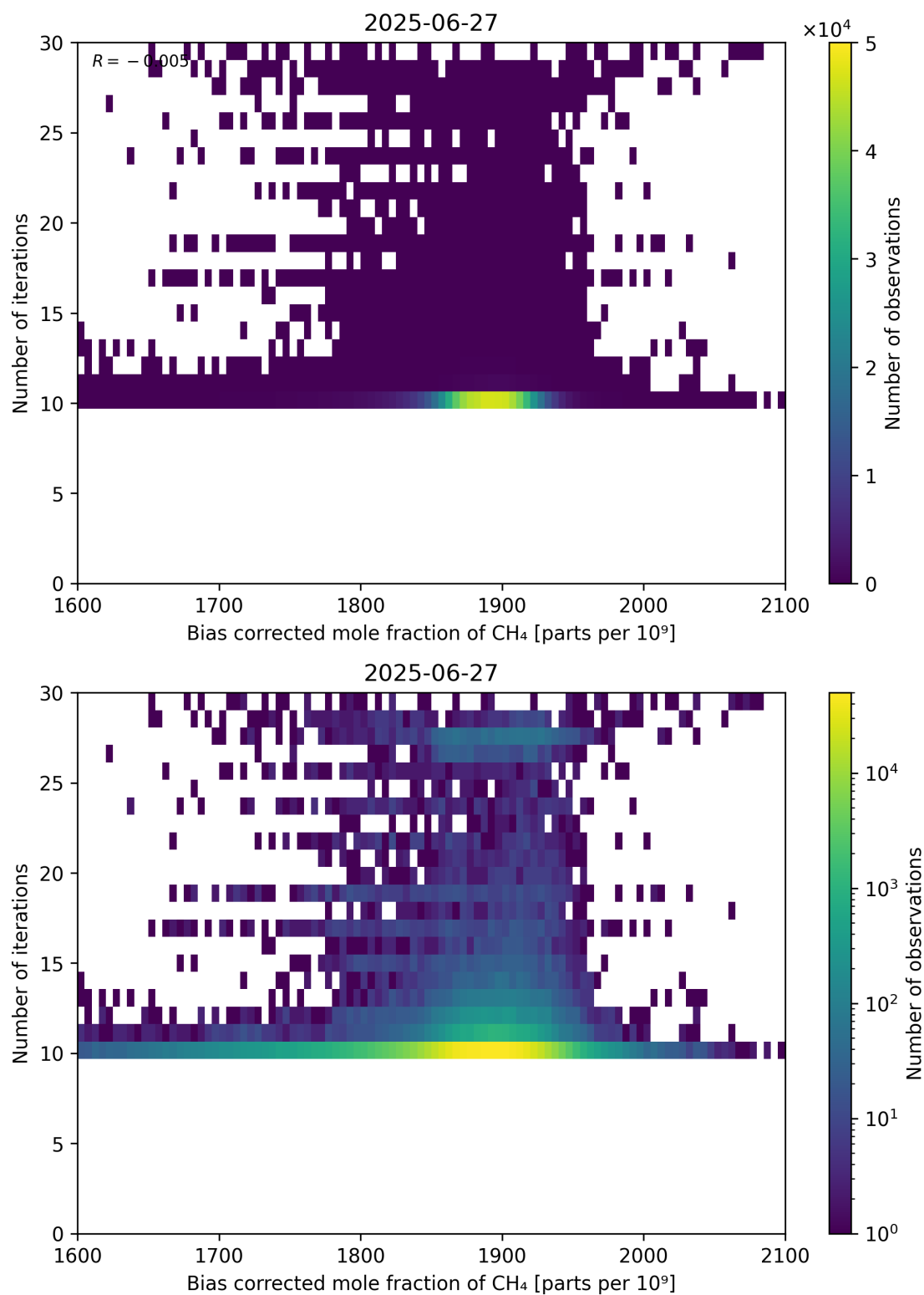
Figure 67: Scatter density plot of “Bias corrected mole fraction of CH 4 ” against “Number of iterations” for 2025-06-27 to 2025-06-28.
