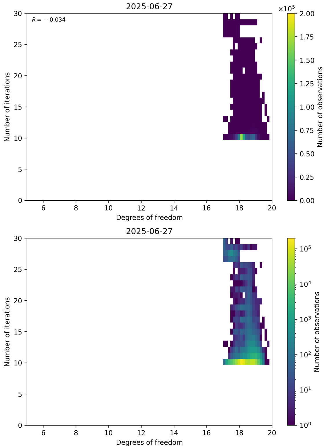
Figure 52: Scatter density plot of “Degrees of freedom” against “Number of iterations” for 2025-06-27 to 2025-06-28.
