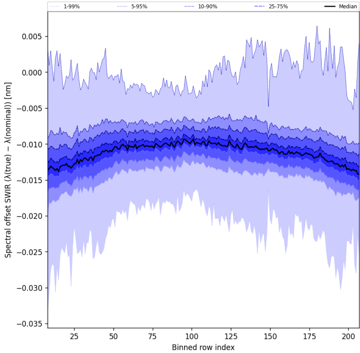
Figure 38: Along track statistics of “Spectral offset SWIR ( \lambda_{\text{true}} - \lambda_{\text{nominal}} )” for 2025-06-27 to 2025-06-28
