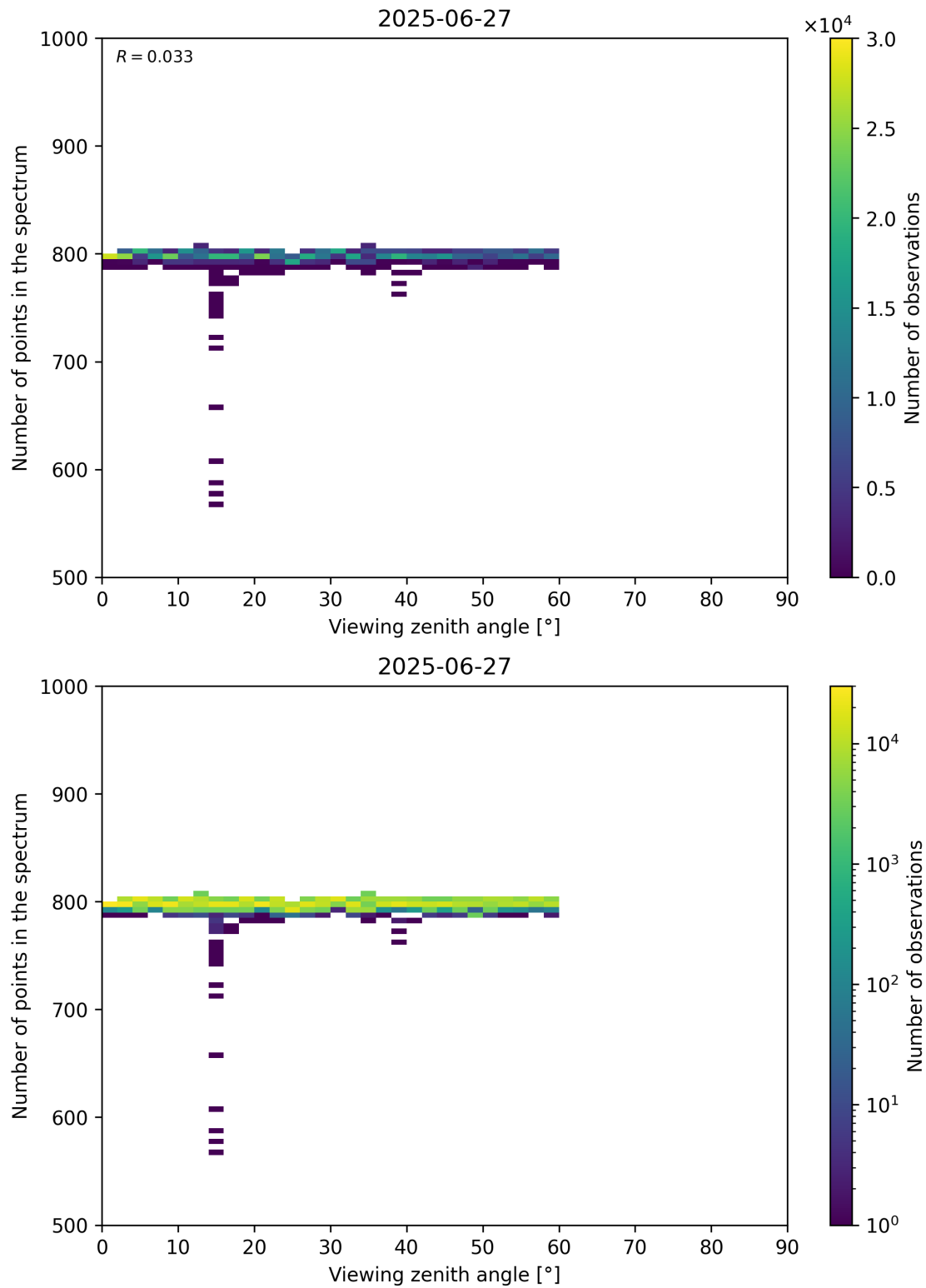
Figure 114: Scatter density plot of “Viewing zenith angle” against “Number of points in the spectrum” for 2025-06-27 to 2025-06-28.
