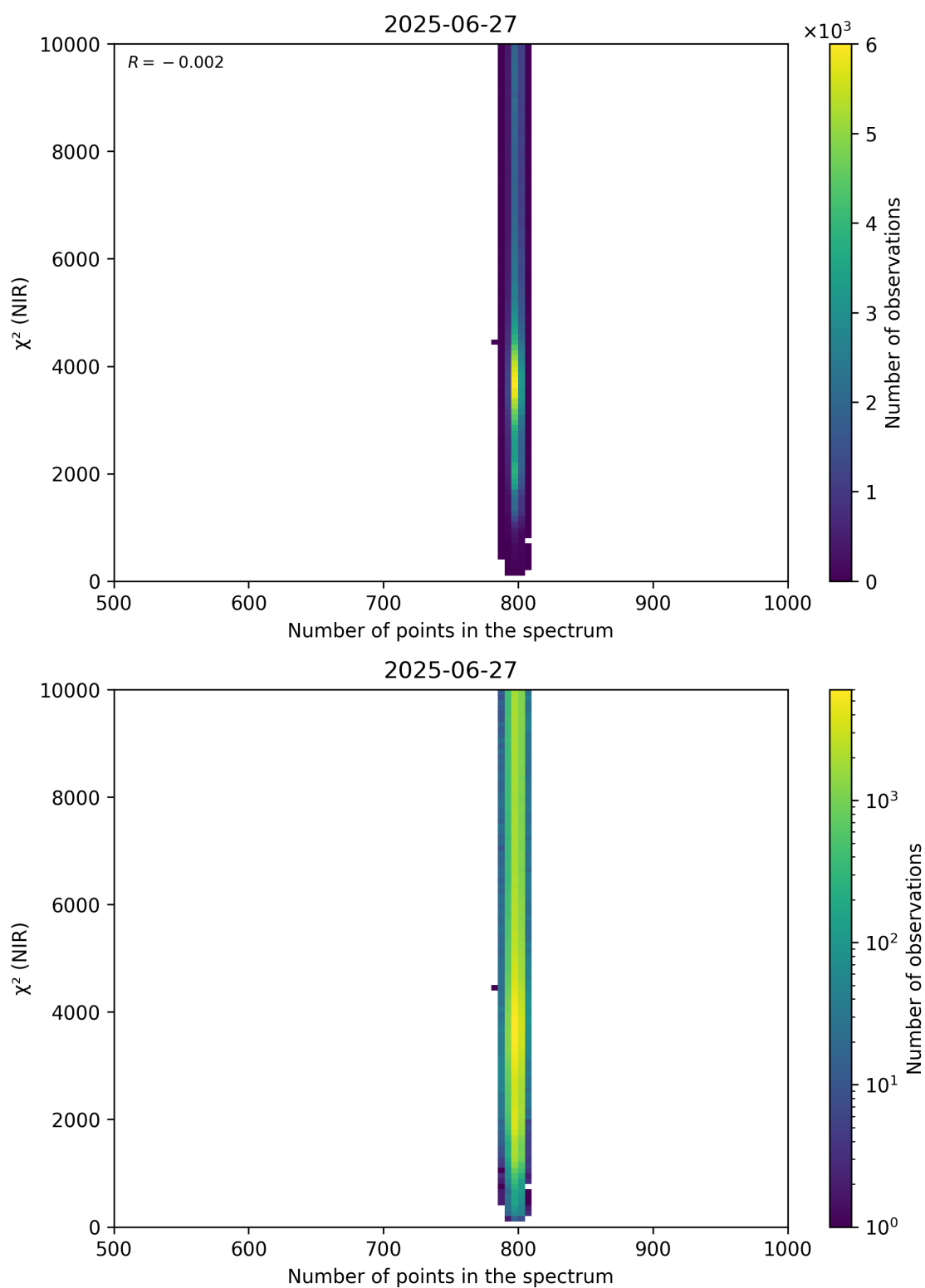
Figure 88: Scatter density plot of “Number of points in the spectrum” against “ \chi^2 (NIR)” for 2025-06-27 to 2025-06-28.
