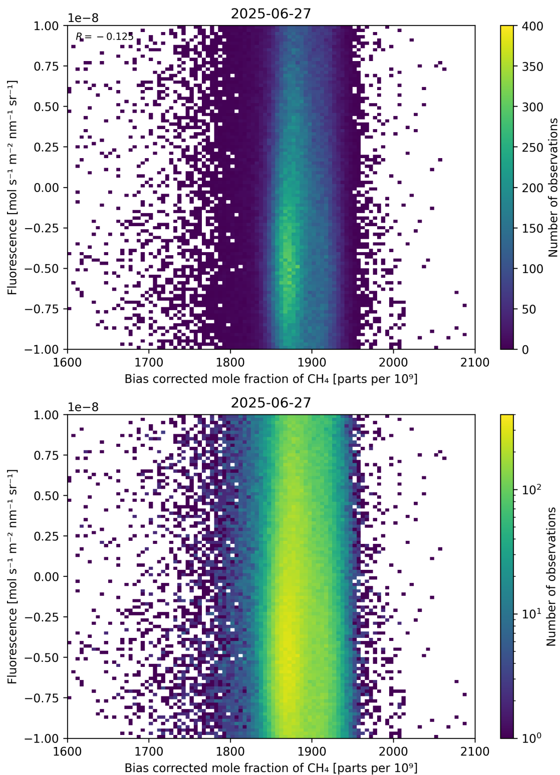
Figure 66: Scatter density plot of “Bias corrected mole fraction of \text{CH}_4 ” against “Fluorescence” for 2025-06-27 to 2025-06-28.
