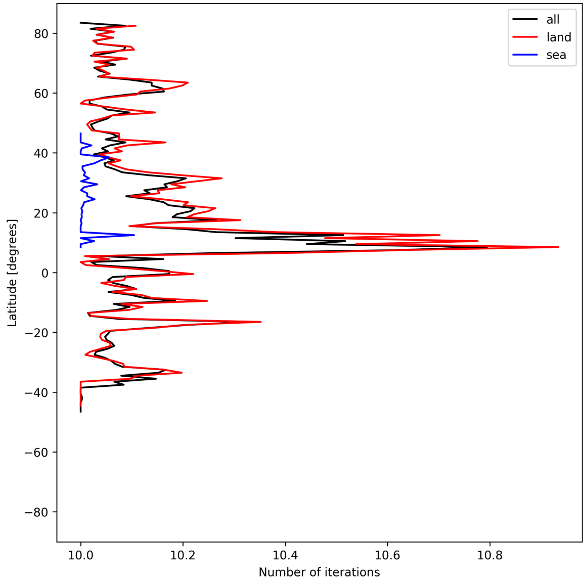
Figure 20: Zonal average of “Number of iterations” for 2025-06-27 to 2025-06-28.
