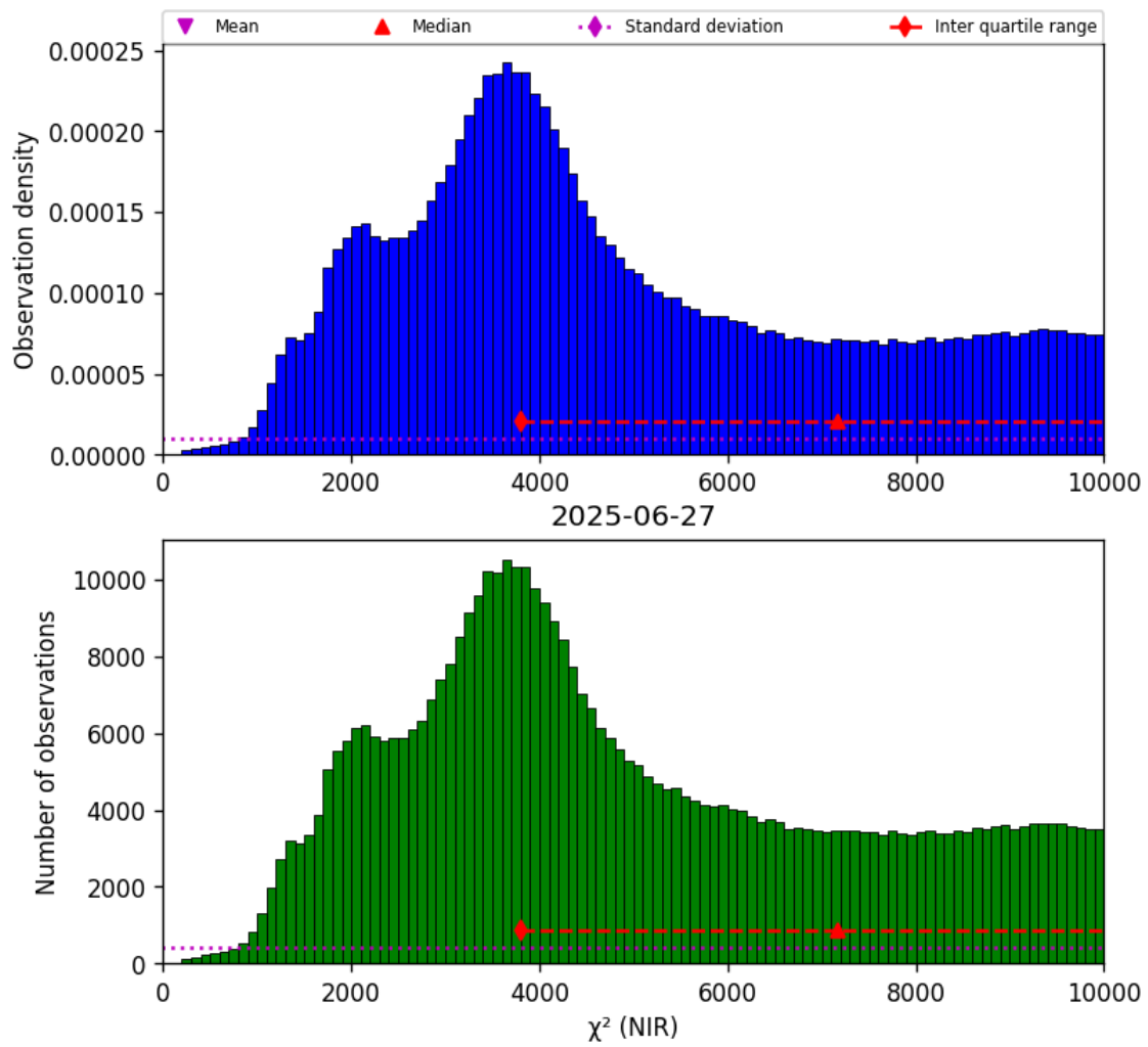
Figure 29: Histogram of “ \chi^2 (NIR)” for 2025-06-27 to 2025-06-28
