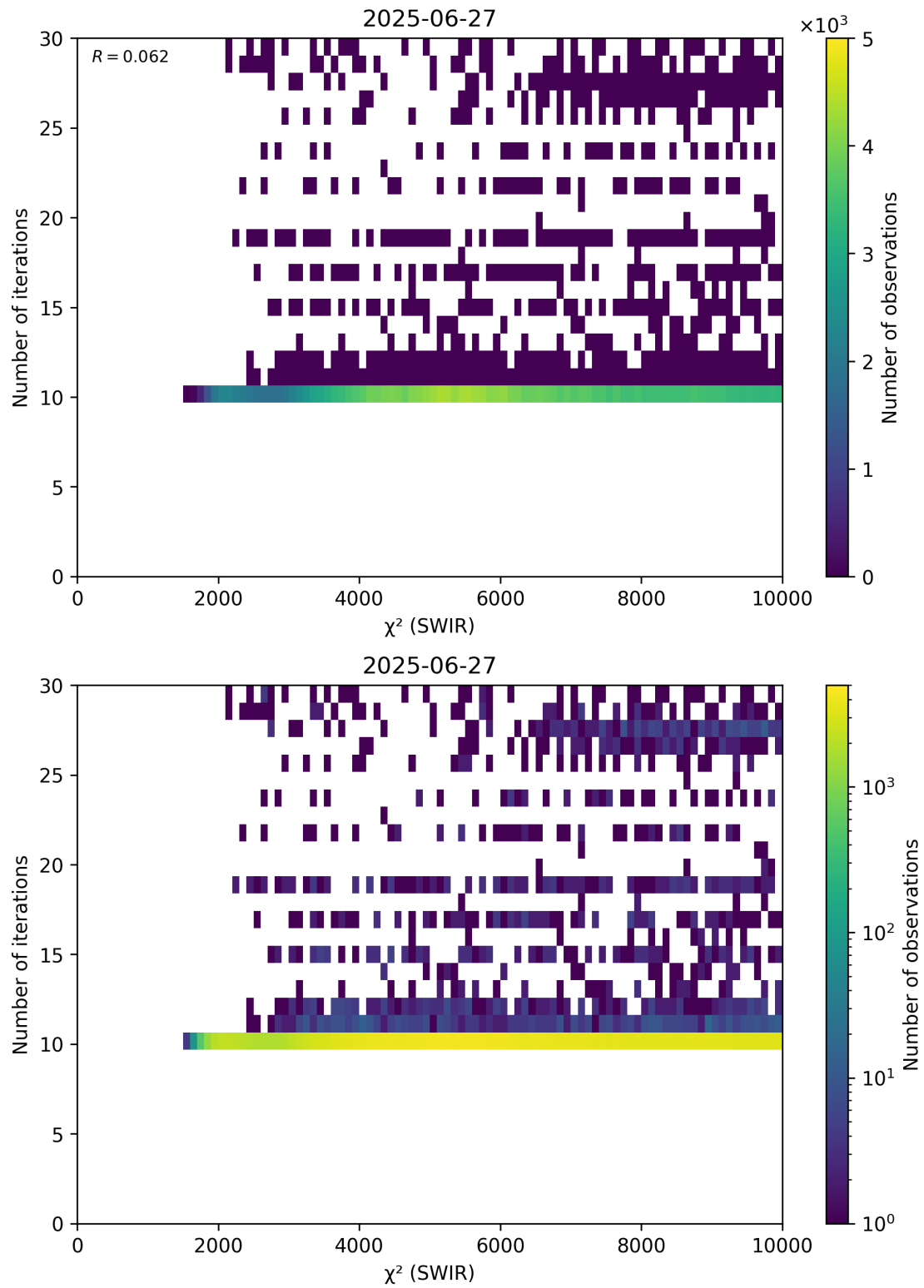
Figure 50: Scatter density plot of “ \chi^2 (SWIR)” against “Number of iterations” for 2025-06-27 to 2025-06-28.
