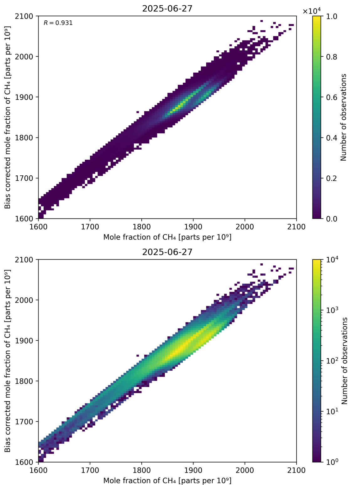
Figure 74: Scatter density plot of “Mole fraction of CH 4 ” against “Bias corrected mole fraction of CH 4 ” for 2025-06-27 to 2025-06-28.
