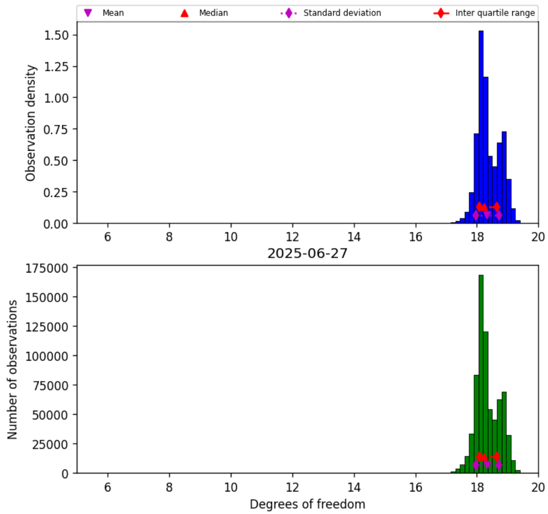
Figure 30: Histogram of “Degrees of freedom” for 2025-06-27 to 2025-06-28
