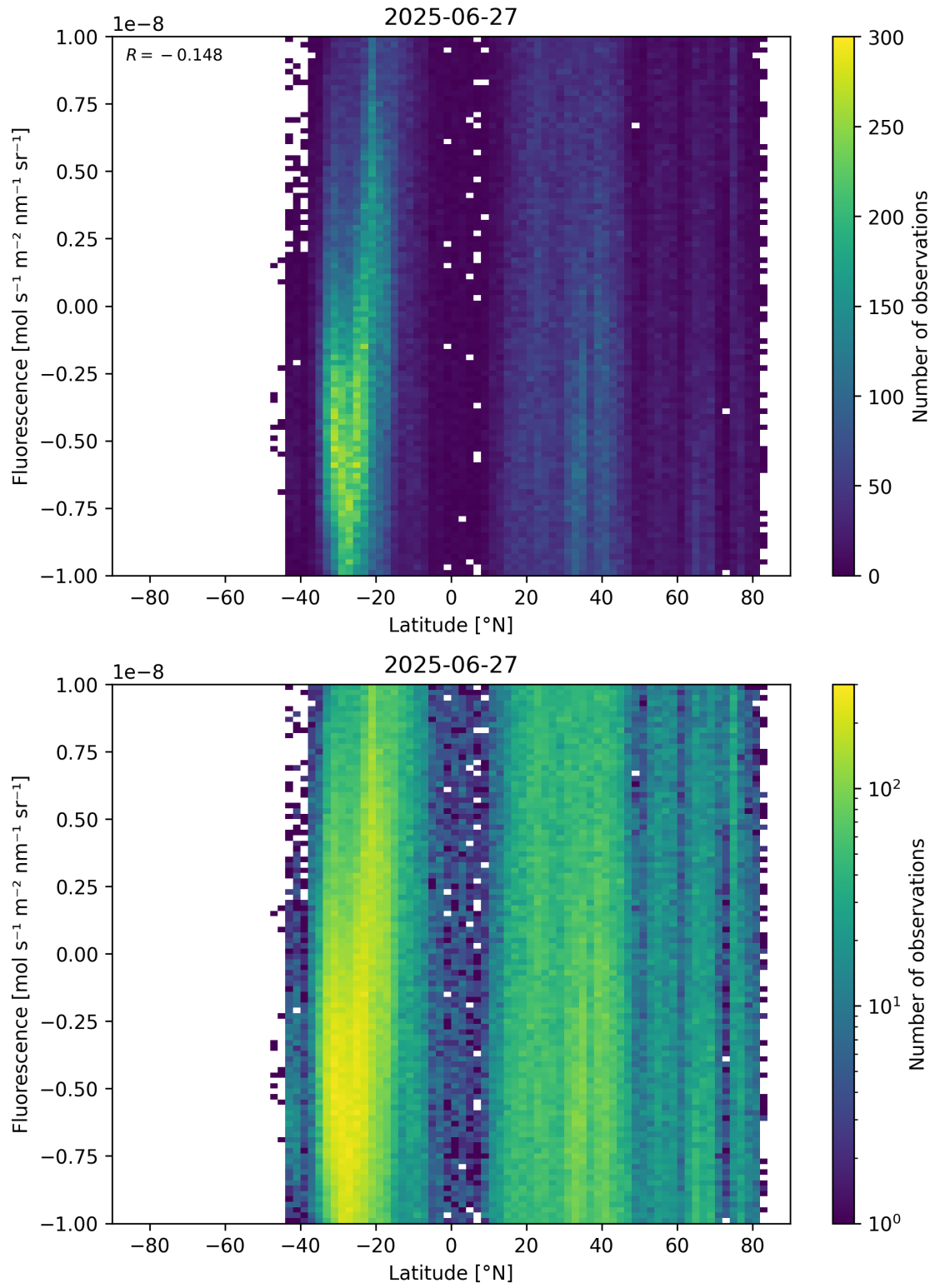
Figure 56: Scatter density plot of “Latitude” against “Fluorescence” for 2025-06-27 to 2025-06-28.
