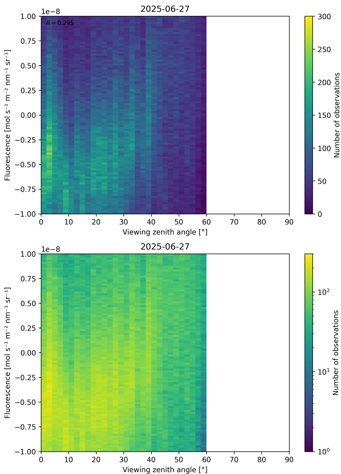
Figure 108: Scatter density plot of “Viewing zenith angle” against “Fluorescence” for 2025-06-27 to 2025-06-28.
