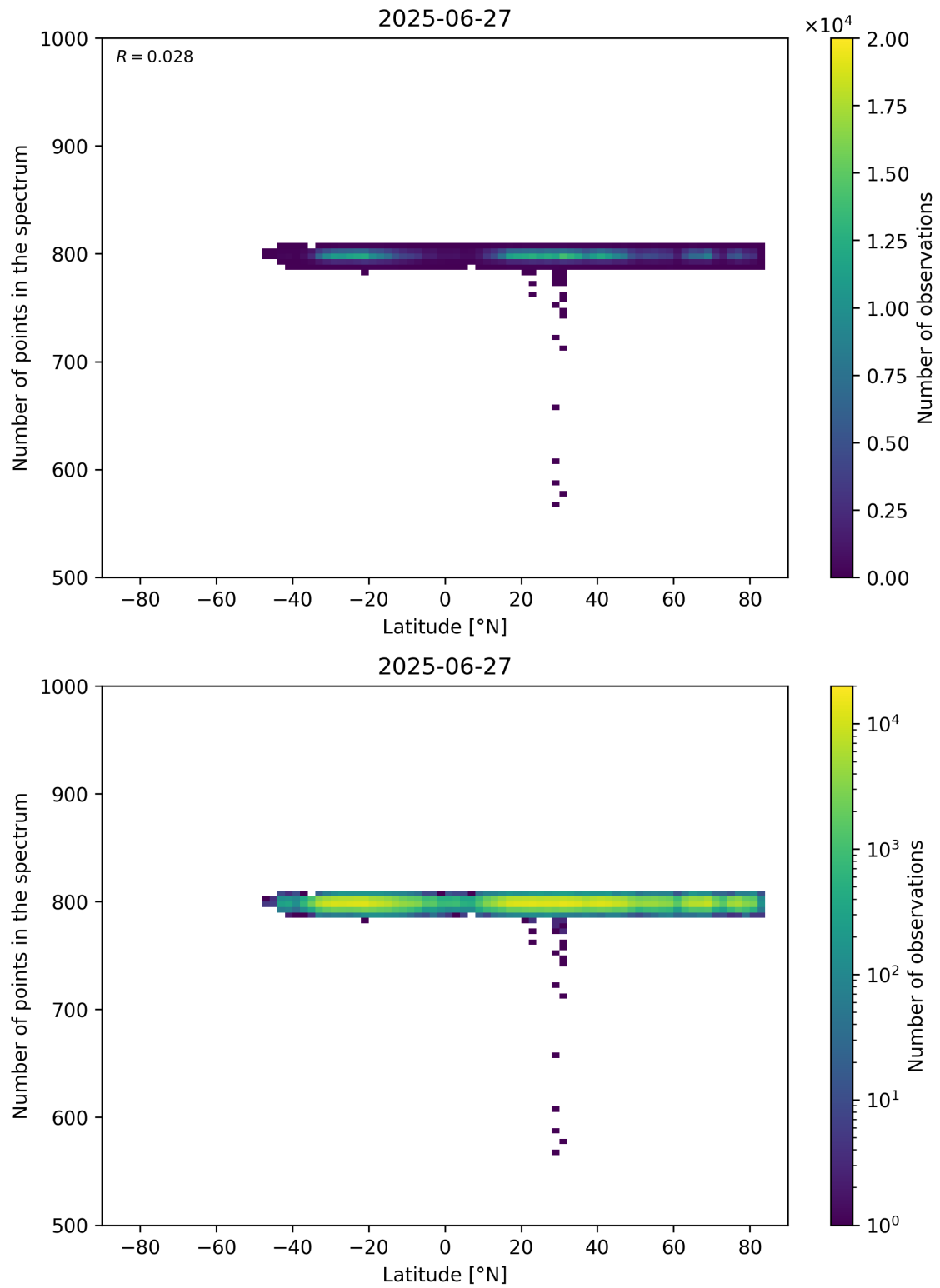
Figure 61: Scatter density plot of “Latitude” against “Number of points in the spectrum” for 2025-06-27 to 2025-06-28.
