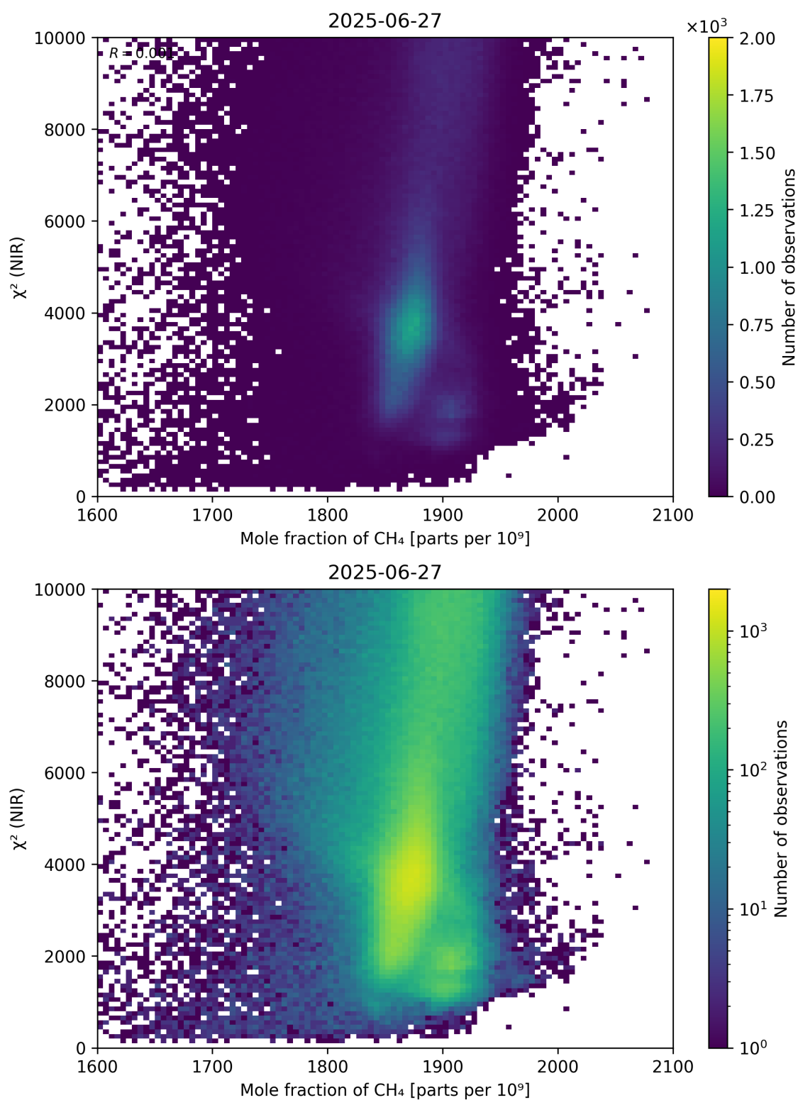
Figure 70: Scatter density plot of “Mole fraction of \text{CH}_4 ” against “ \chi^2 (NIR)” for 2025-06-27 to 2025-06-28.
