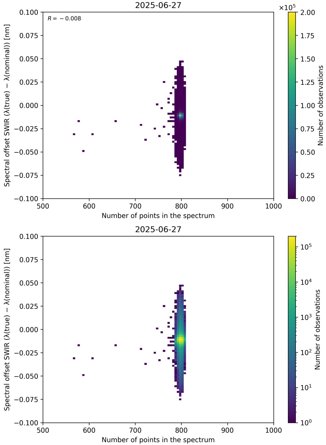
Figure 93: Scatter density plot of “Number of points in the spectrum” against “Spectral offset SWIR ( \lambda_{\text{true}} - \lambda_{\text{nominal}} )” for 2025-06-27 to 2025-06-28.
