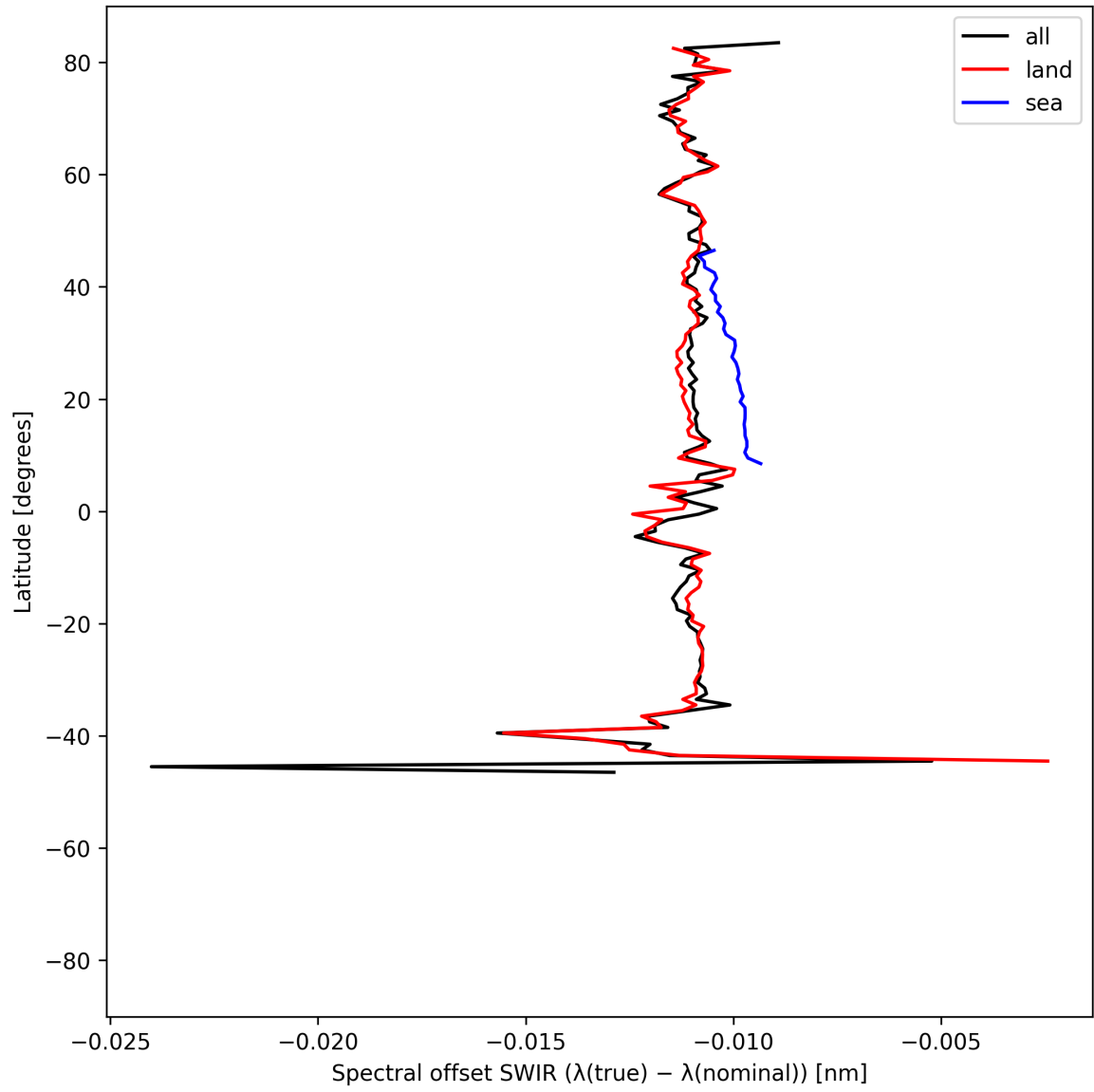
Figure 16: Zonal average of “Spectral offset SWIR ( \lambda_{\text{true}} - \lambda_{\text{nominal}} )” for 2025-06-27 to 2025-06-28.
