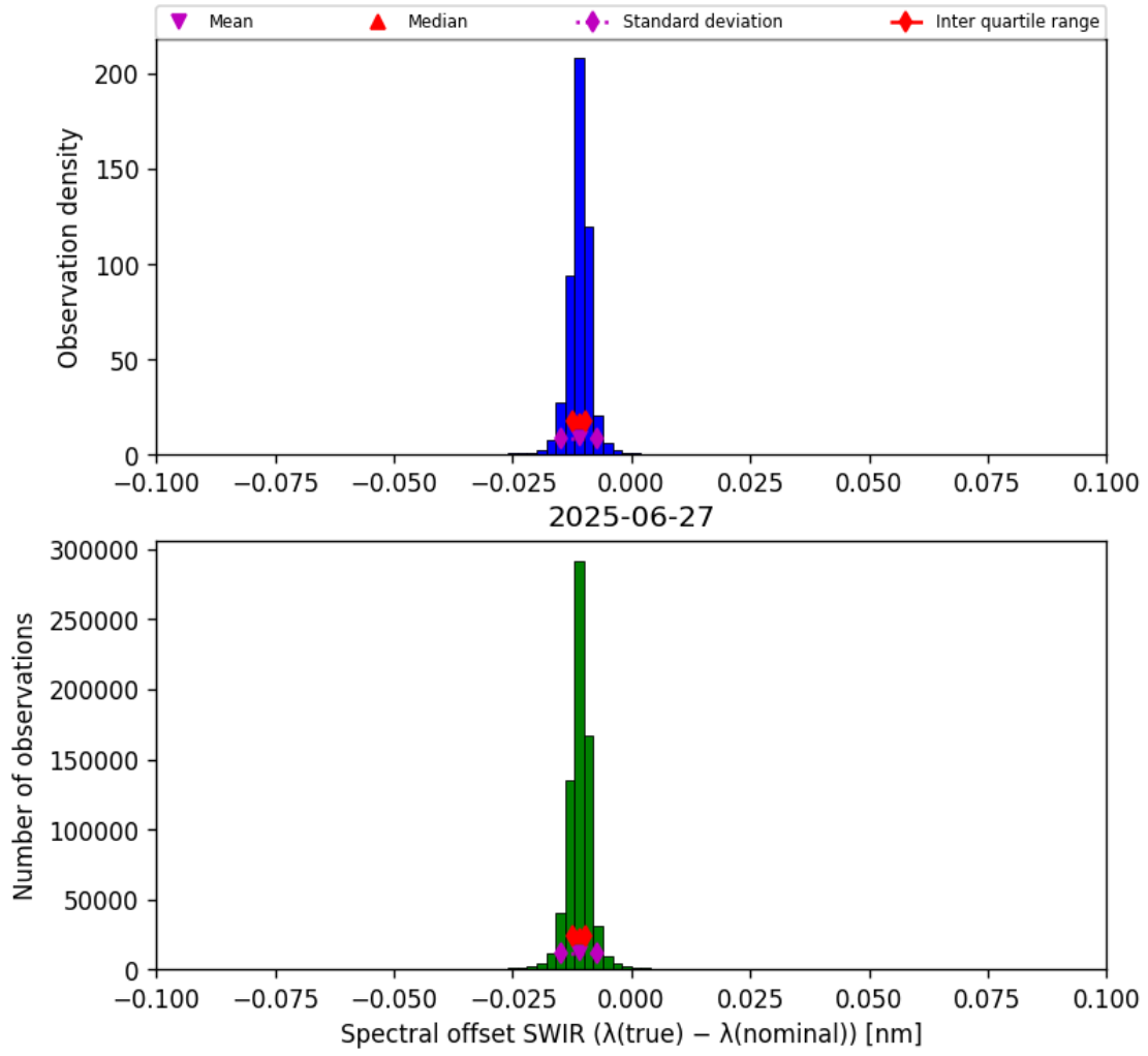
Figure 27: Histogram of “Spectral offset SWIR ( \lambda_{\text{true}} - \lambda_{\text{nominal}} )” for 2025-06-27 to 2025-06-28
