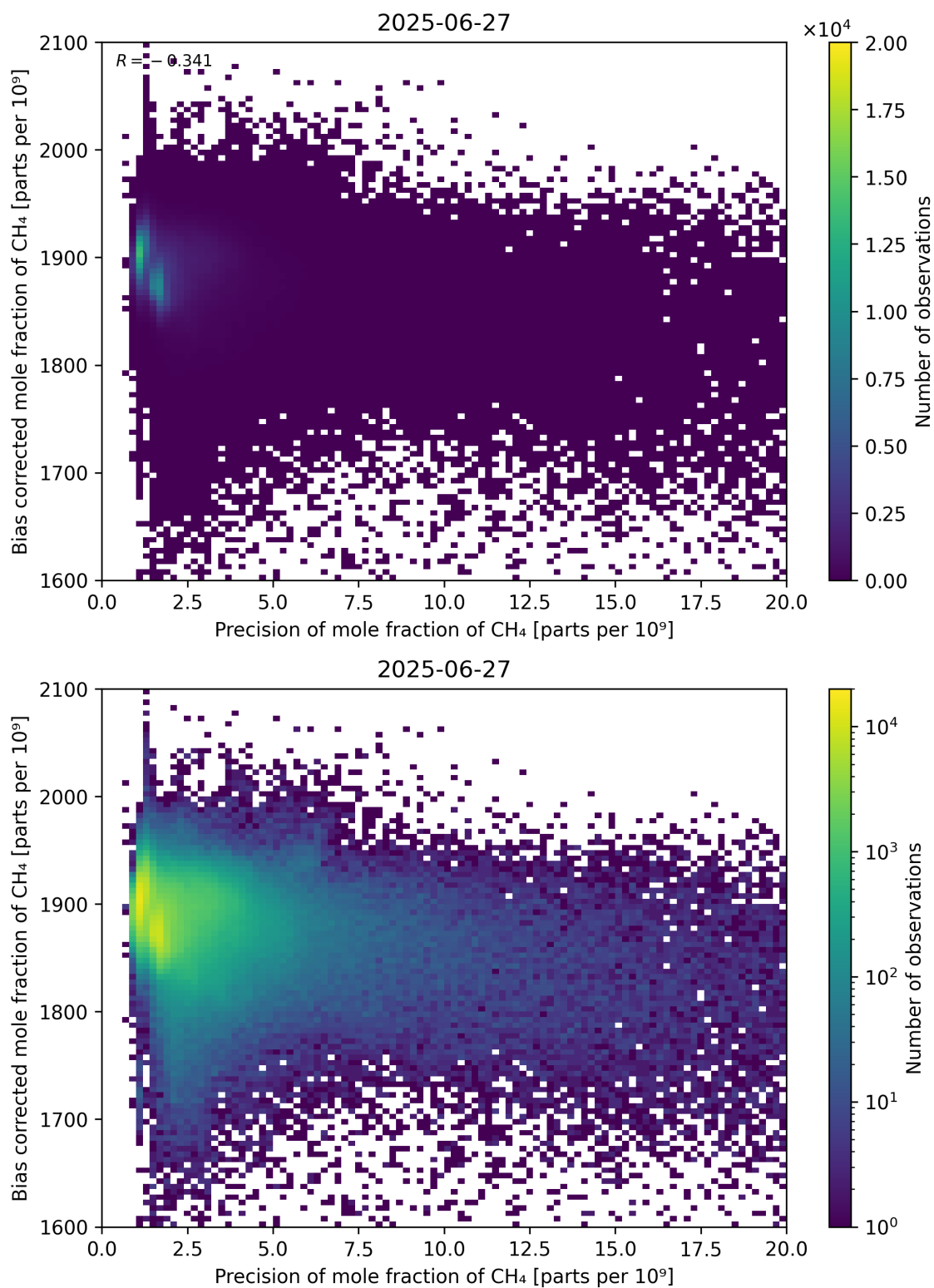
Figure 82: Scatter density plot of “Precision of mole fraction of CH 4 ” against “Bias corrected mole fraction of CH 4 ” for 2025-06-27 to 2025-06-28.
