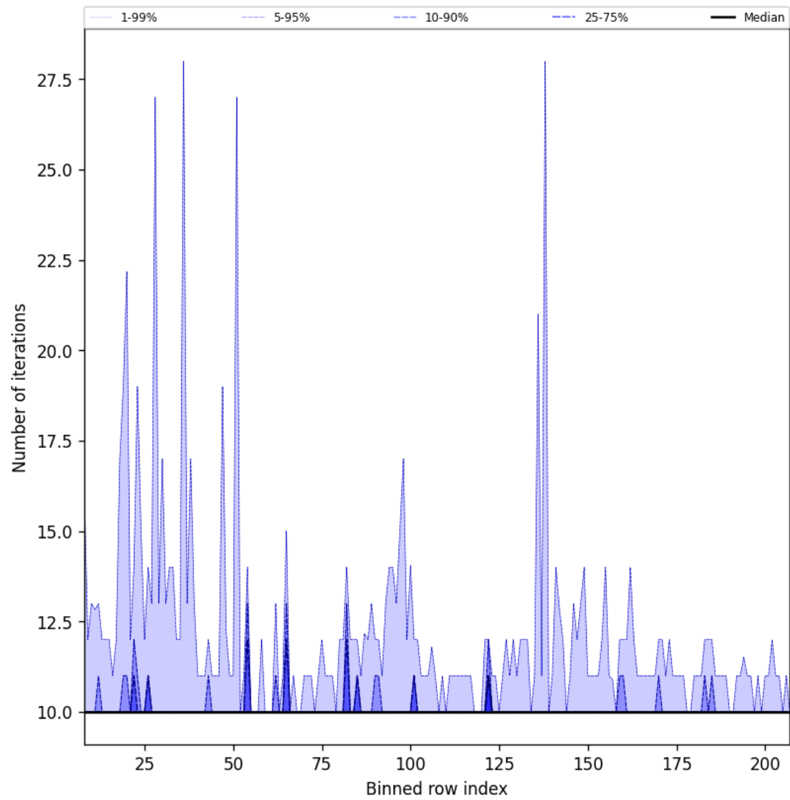
Figure 42: Along track statistics of “Number of iterations” for 2025-06-27 to 2025-06-28
