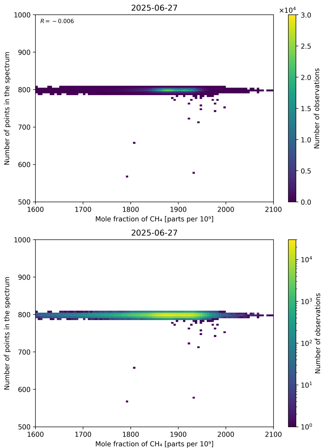
Figure 77: Scatter density plot of “Mole fraction of CH 4 ” against “Number of points in the spectrum” for 2025-06-27 to 2025-06-28.
