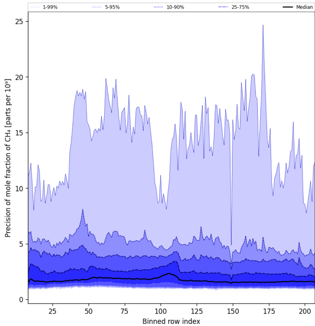
Figure 35: Along track statistics of “Precision of mole fraction of CH 4 ” for 2025-06-27 to 2025-06-28
