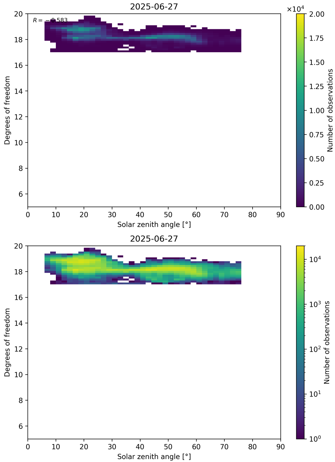
Figure 96: Scatter density plot of “Solar zenith angle” against “Degrees of freedom” for 2025-06-27 to 2025-06-28.
