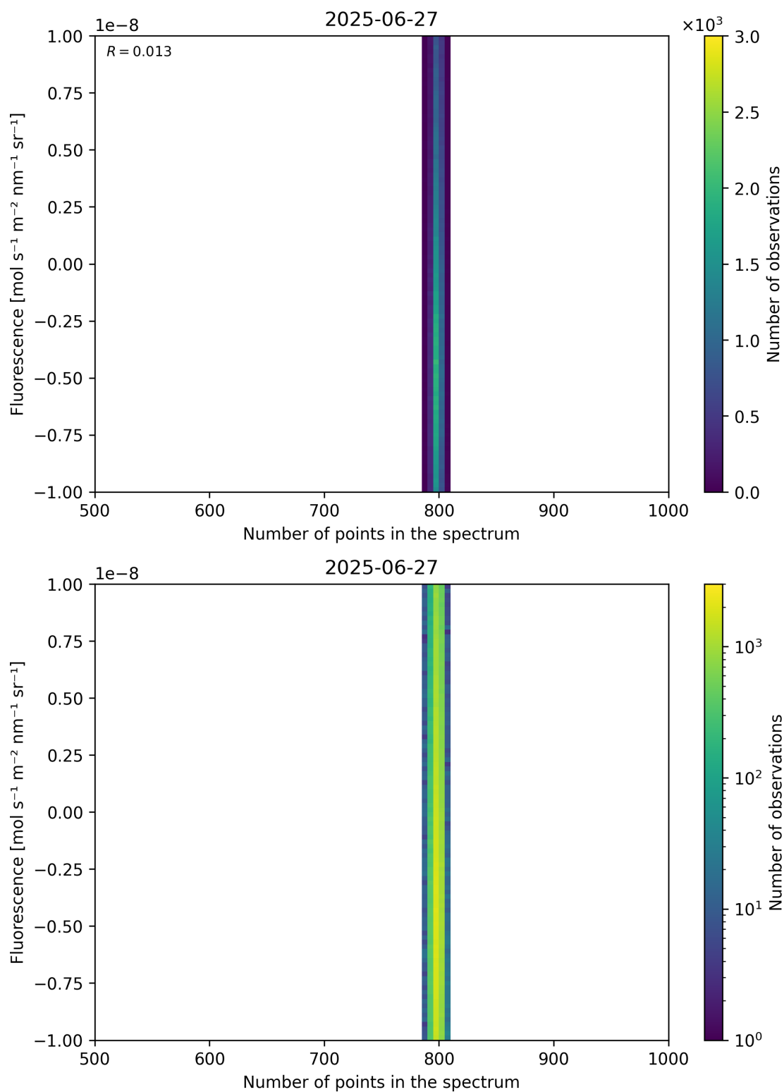
Figure 91: Scatter density plot of “Number of points in the spectrum” against “Fluorescence” for 2025-06-27 to 2025-06-28.
