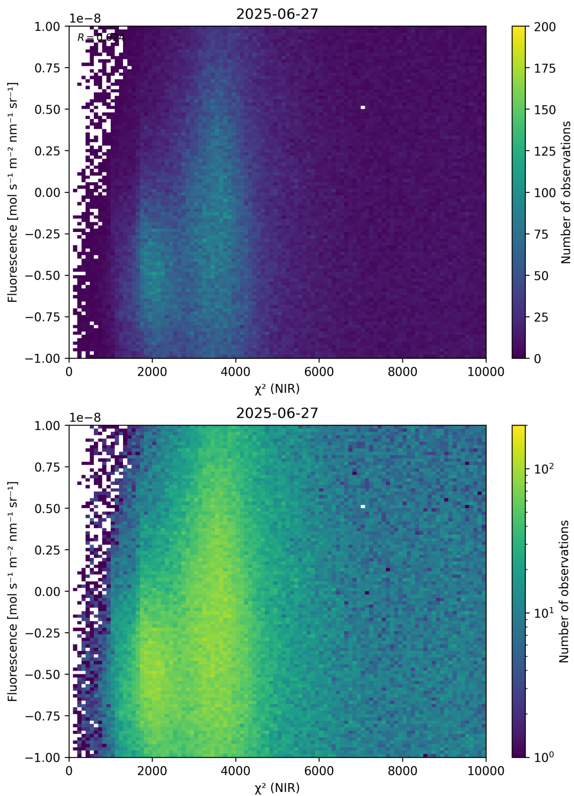
Figure 45: Scatter density plot of “ \chi^2 (NIR)” against “Fluorescence” for 2025-06-27 to 2025-06-28.
