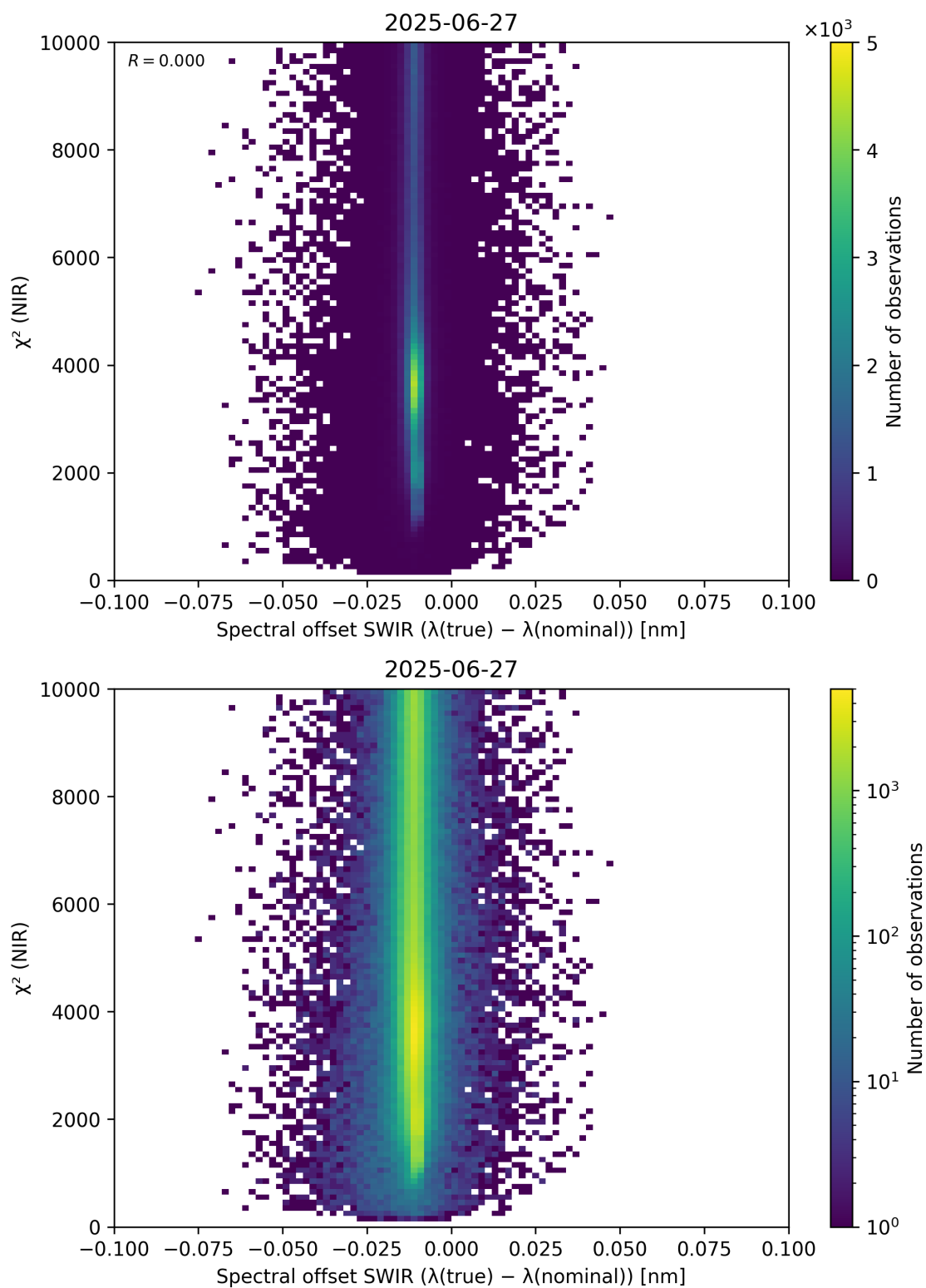
Figure 117: Scatter density plot of “Spectral offset SWIR ( \lambda_{\text{true}} - \lambda_{\text{nominal}} )” against “ \chi^2 (NIR)” for 2025-06-27 to 2025-06-28.
