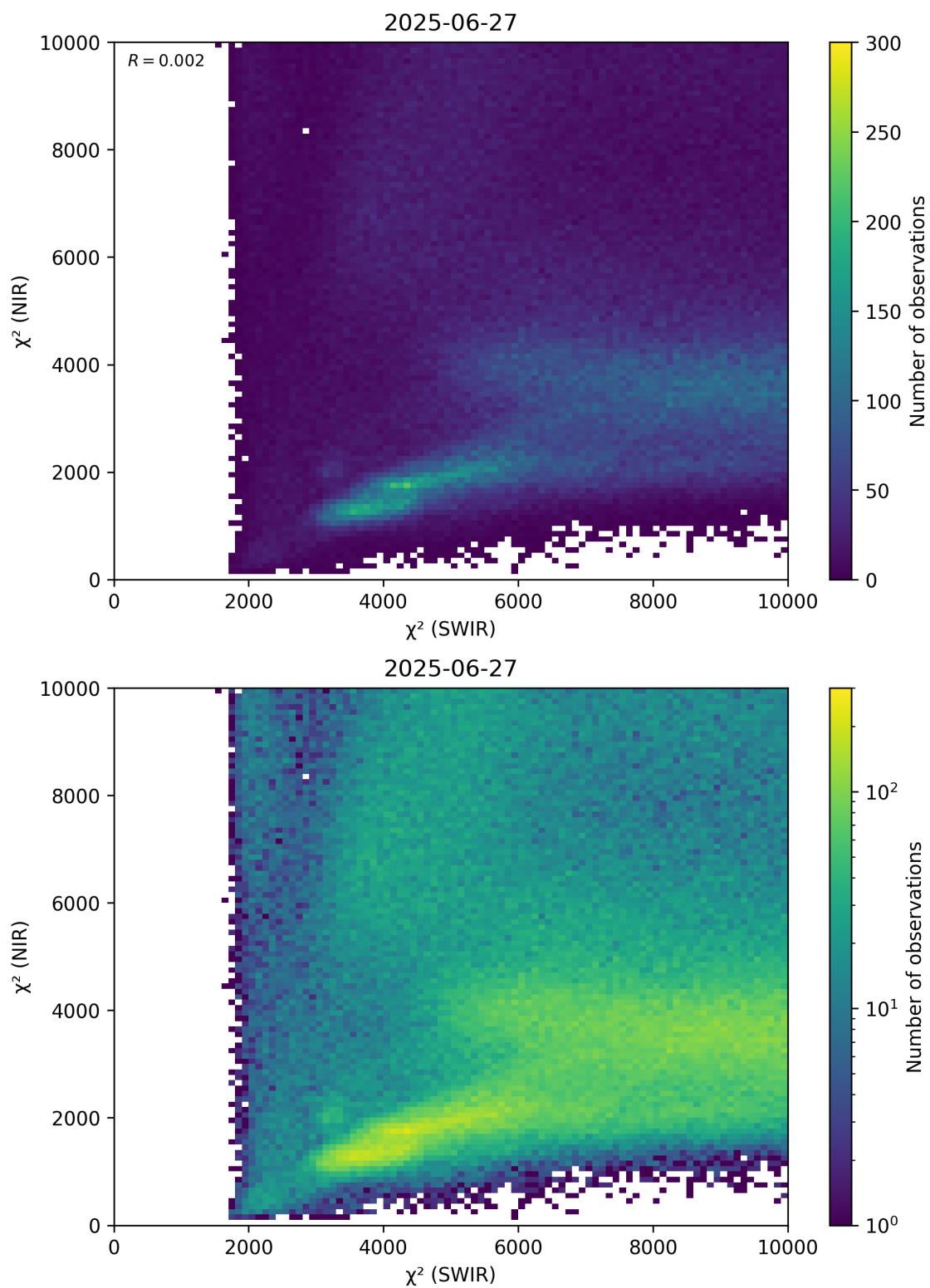
Figure 47: Scatter density plot of “ \chi^2 (SWIR)” against “ \chi^2 (NIR)” for 2025-06-27 to 2025-06-28.
