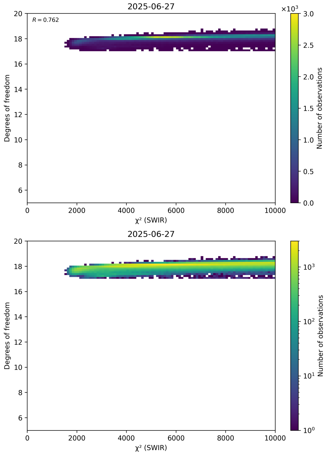
Figure 48: Scatter density plot of “ \chi^2 (SWIR)” against “Degrees of freedom” for 2025-06-27 to 2025-06-28.
