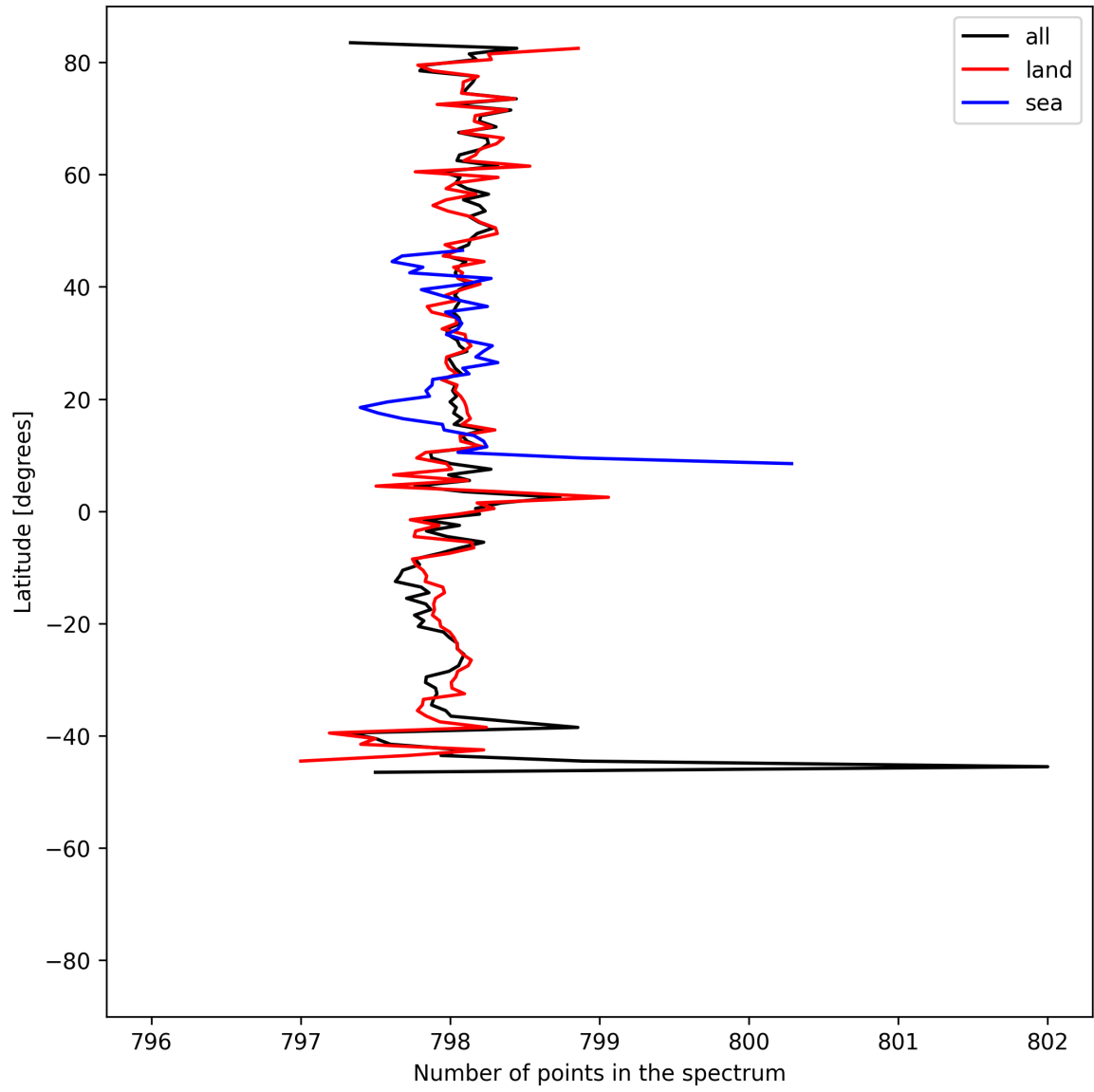
Figure 15: Zonal average of “Number of points in the spectrum” for 2025-06-27 to 2025-06-28.
