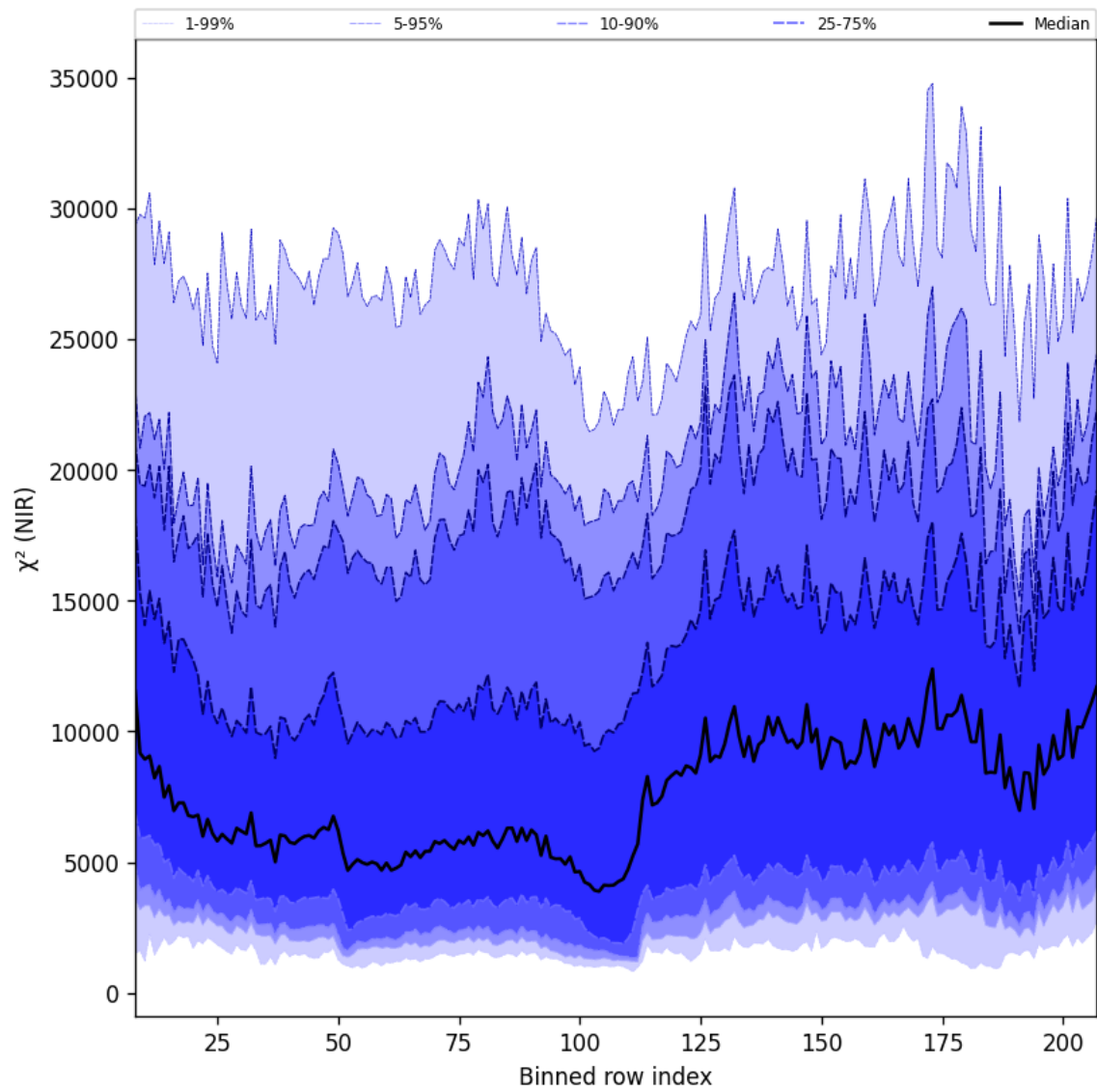
Figure 40: Along track statistics of “ \chi^2 (NIR)” for 2025-06-27 to 2025-06-28
