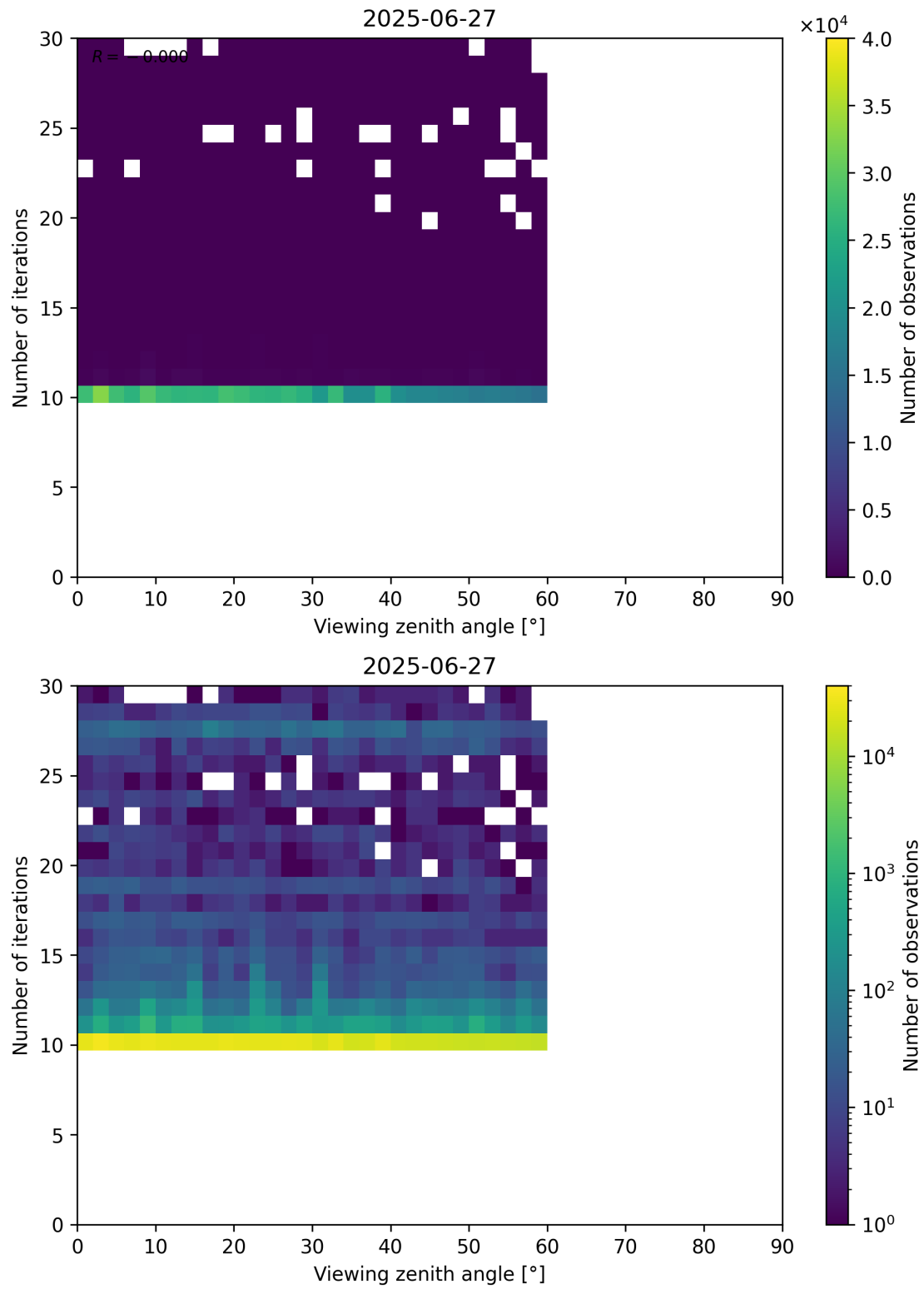
Figure 113: Scatter density plot of “Viewing zenith angle” against “Number of iterations” for 2025-06-27 to 2025-06-28.
