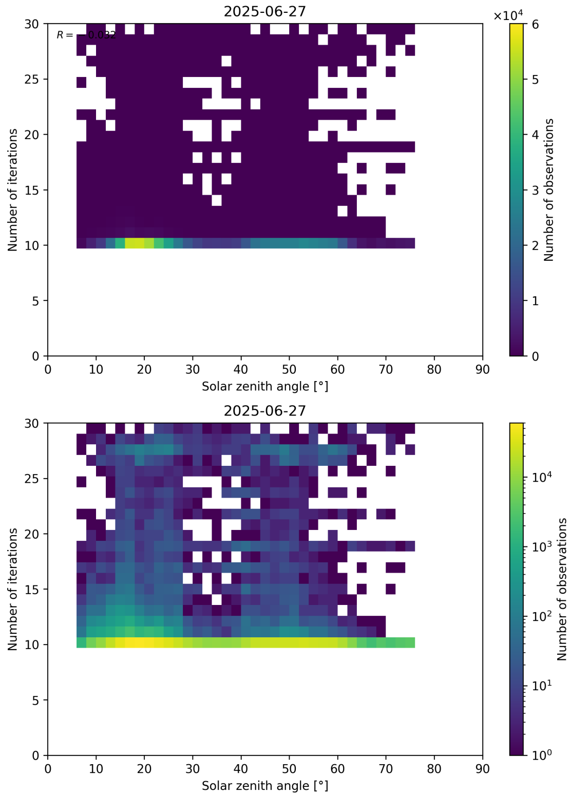
Figure 102: Scatter density plot of “Solar zenith angle” against “Number of iterations” for 2025-06-27 to 2025-06-28.
