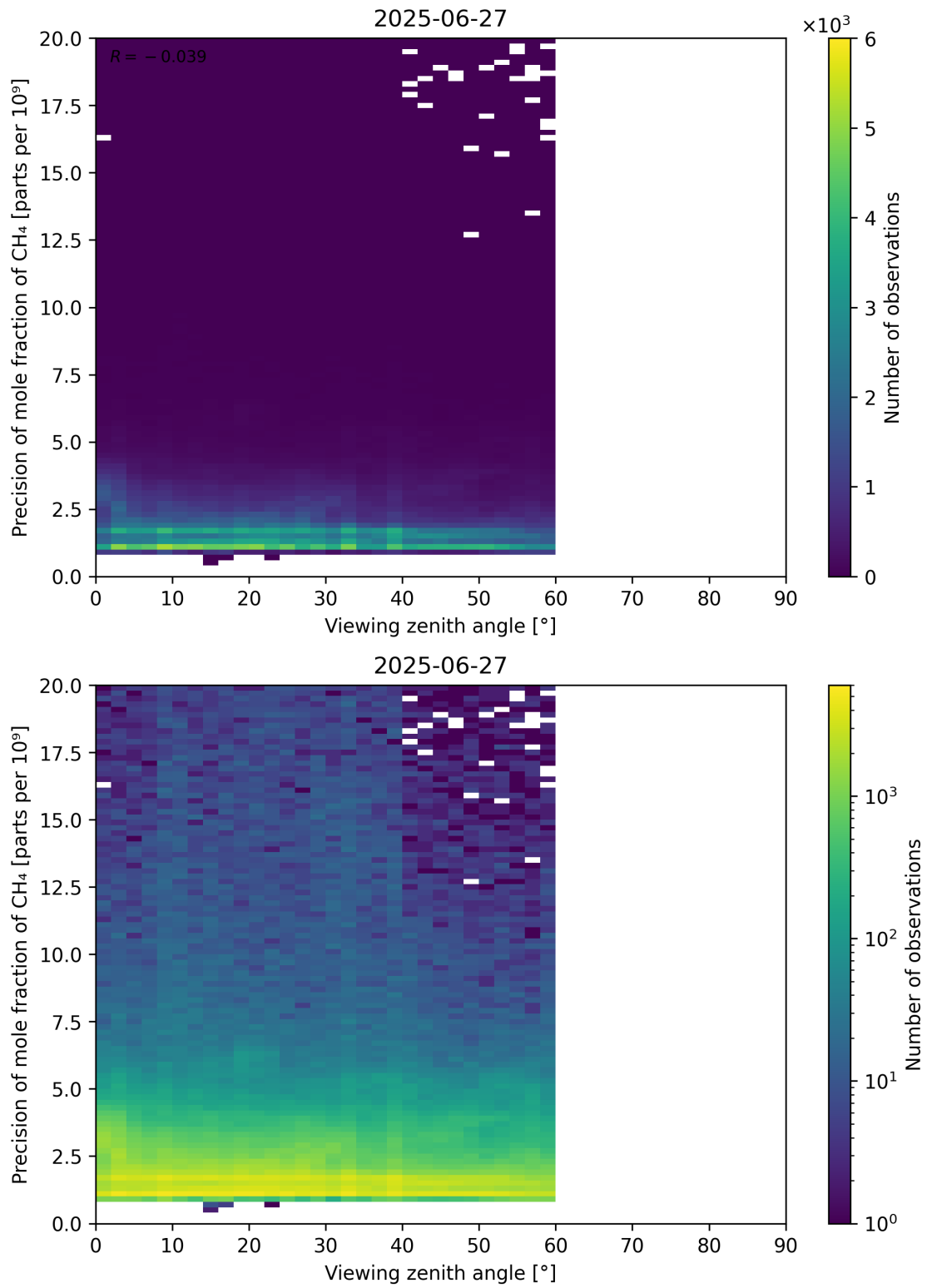
Figure 112: Scatter density plot of “Viewing zenith angle” against “Precision of mole fraction of CH 4 ” for 2025-06-27 to 2025-06-28.
