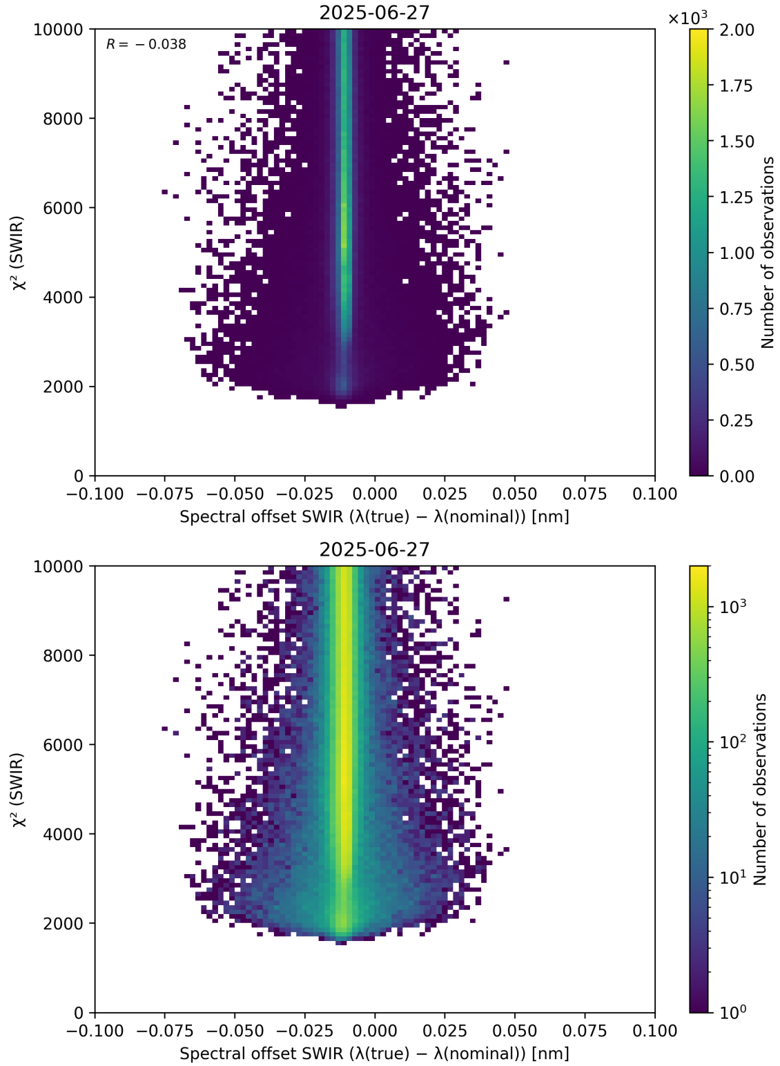
Figure 118: Scatter density plot of “Spectral offset SWIR ( \lambda_{\text{true}} - \lambda_{\text{nominal}} )” against “ \chi^2 (SWIR)” for 2025-06-27 to 2025-06-28.
