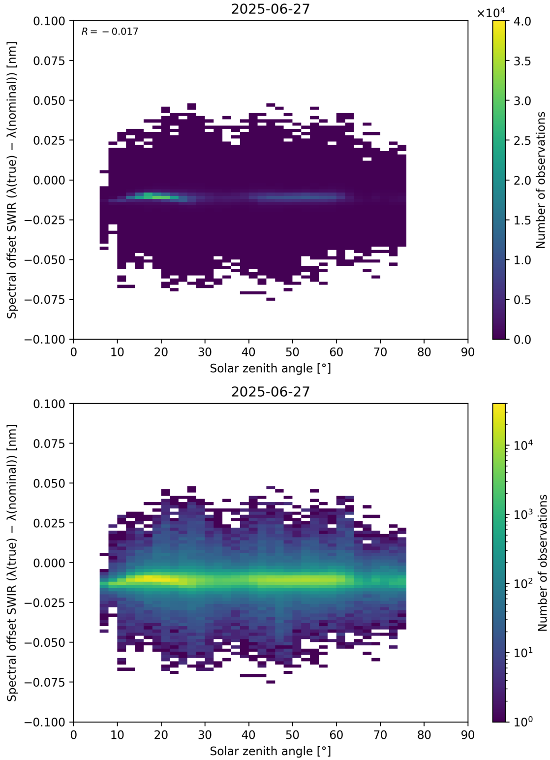
Figure 104: Scatter density plot of “Solar zenith angle” against “Spectral offset SWIR ( \lambda_{\text{true}} - \lambda_{\text{nominal}} )” for 2025-06-27 to 2025-06-28.
