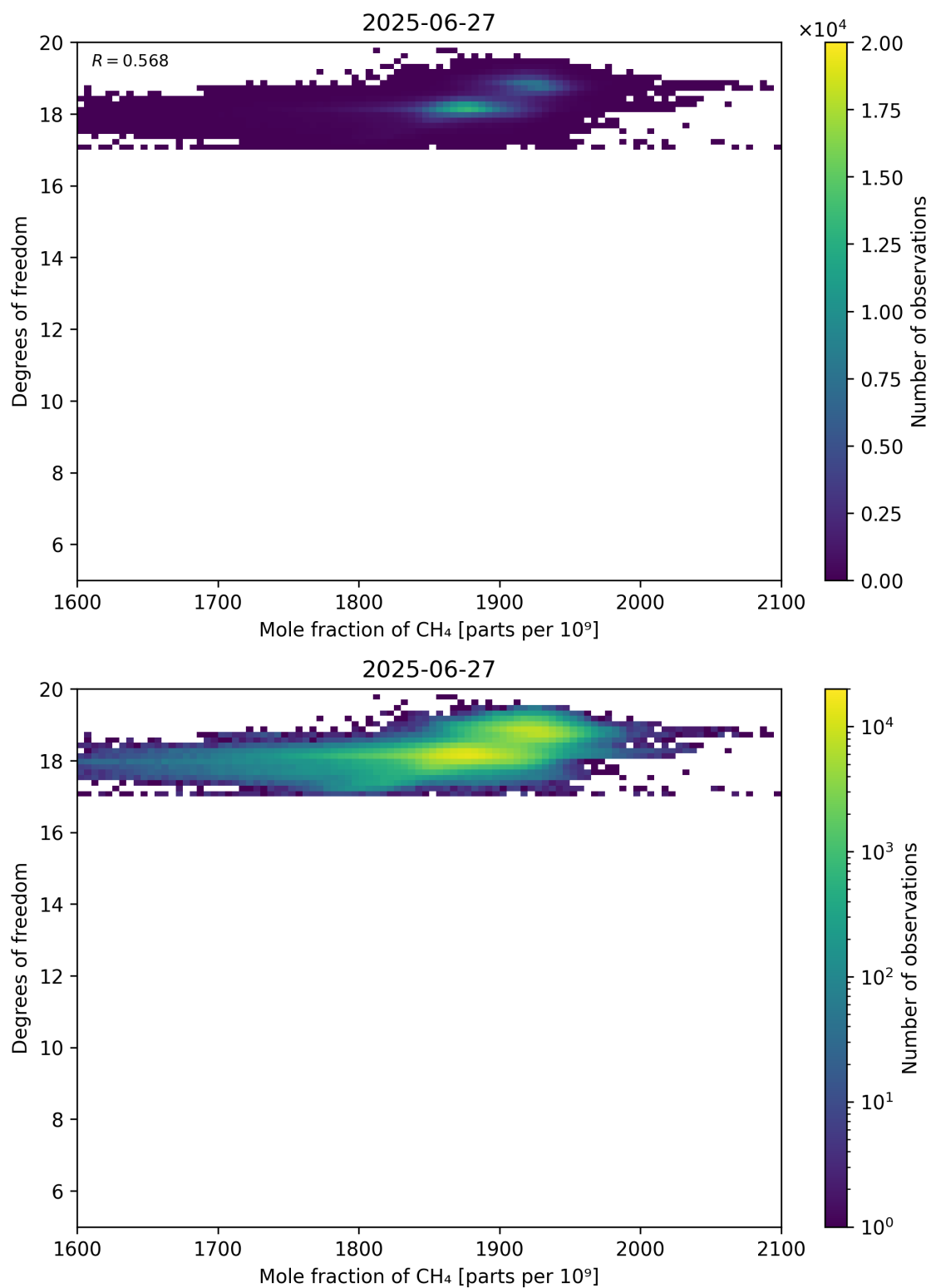
Figure 72: Scatter density plot of “Mole fraction of CH 4 ” against “Degrees of freedom” for 2025-06-27 to 2025-06-28.
