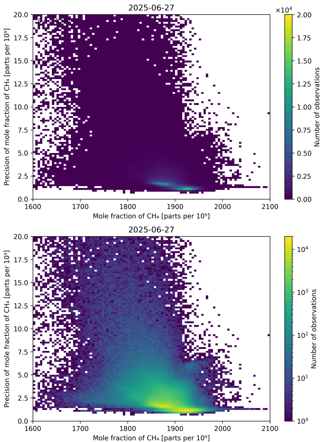
Figure 75: Scatter density plot of “Mole fraction of CH 4 ” against “Precision of mole fraction of CH 4 ” for 2025-06-27 to 2025-06-28.
