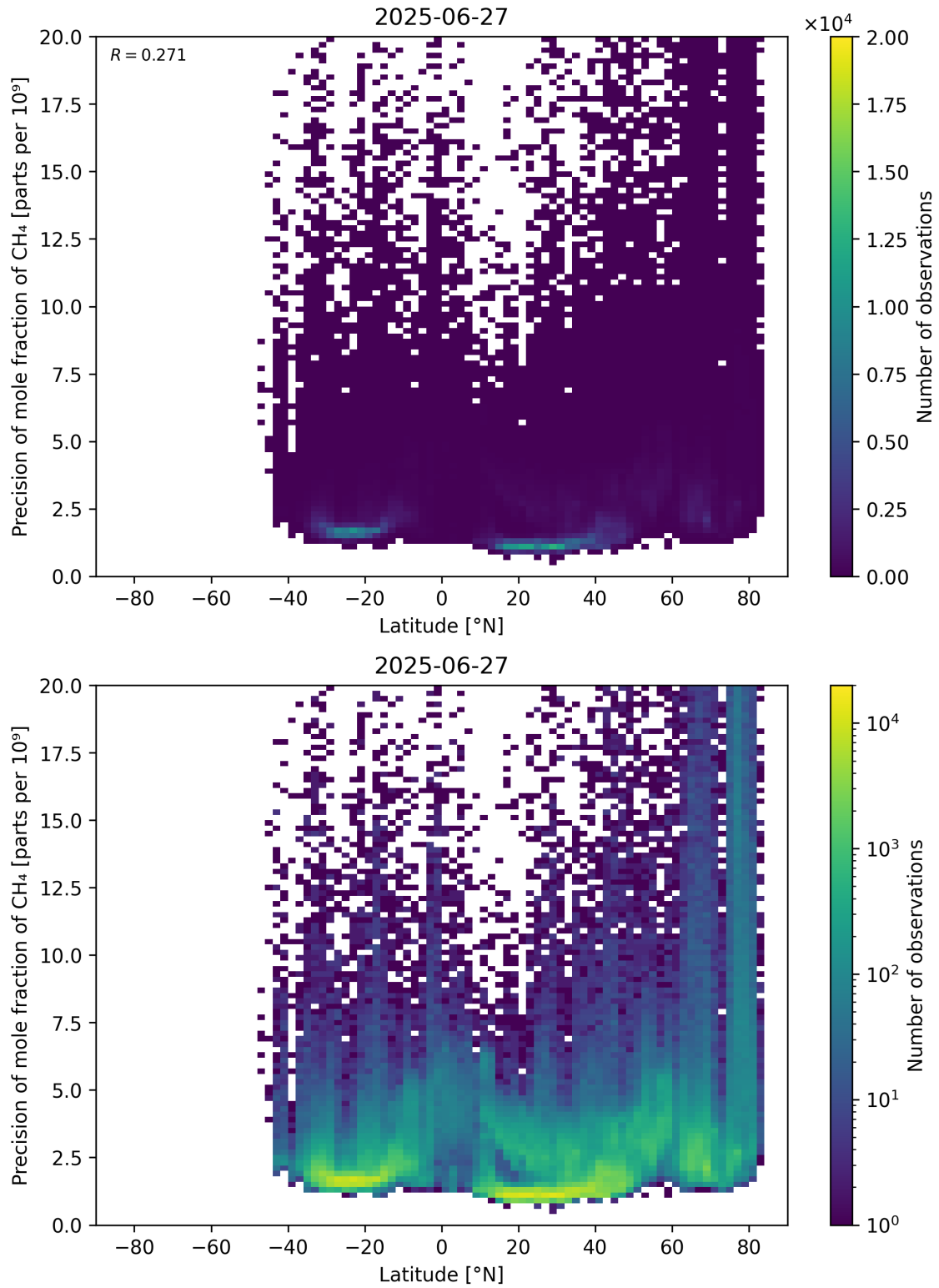
Figure 59: Scatter density plot of “Latitude” against “Precision of mole fraction of \text{CH}_4 ” for 2025-06-27 to 2025-06-28.
