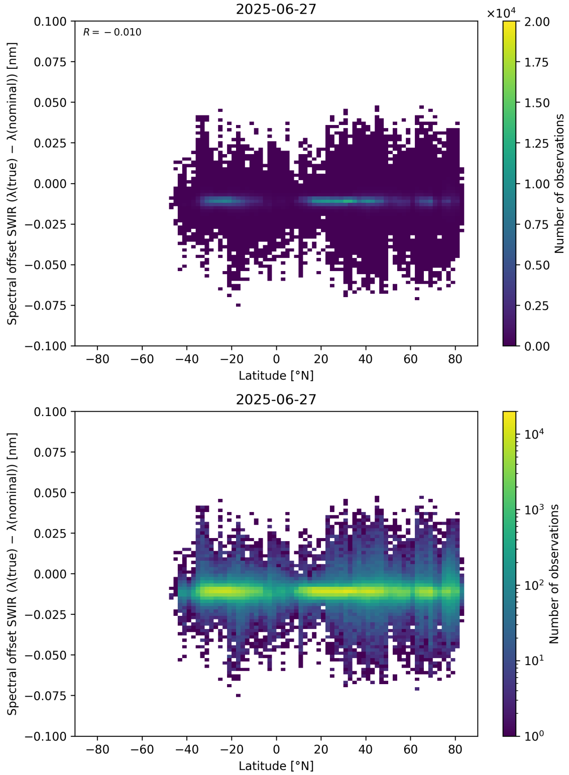
Figure 62: Scatter density plot of “Latitude” against “Spectral offset SWIR ( \lambda_{\text{true}} - \lambda_{\text{nominal}} )” for 2025-06-27 to 2025-06-28.
