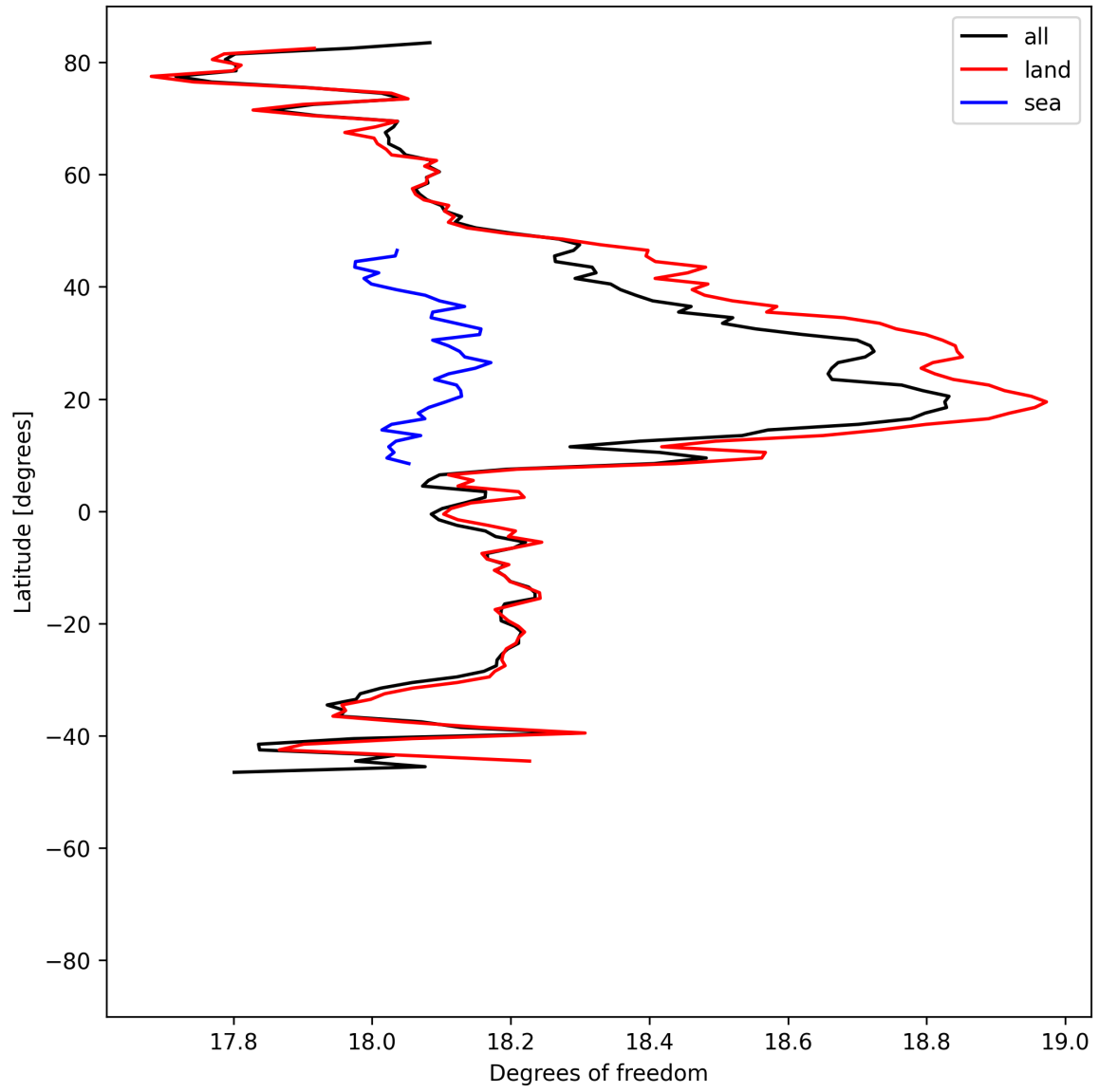
Figure 19: Zonal average of “Degrees of freedom” for 2025-06-27 to 2025-06-28.
