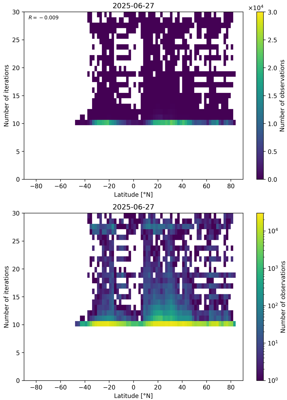
Figure 60: Scatter density plot of “Latitude” against “Number of iterations” for 2025-06-27 to 2025-06-28.
