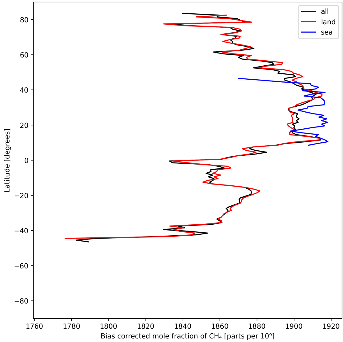
Figure 14: Zonal average of “Bias corrected mole fraction of \text{CH}_4 ” for 2025-06-27 to 2025-06-28.
