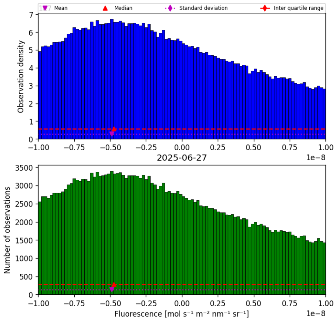
Figure 32: Histogram of “Fluorescence” for 2025-06-27 to 2025-06-28
