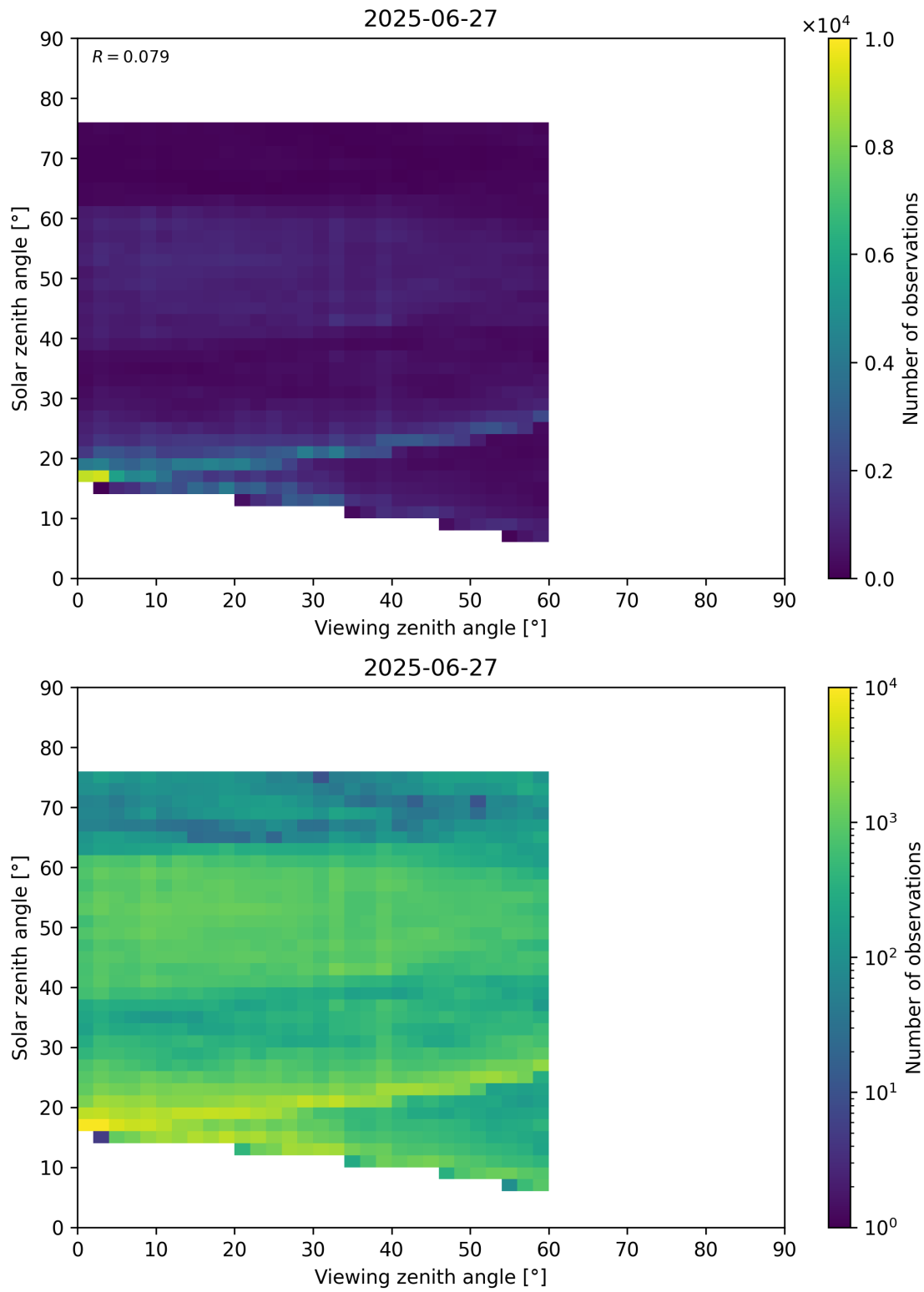
Figure 115: Scatter density plot of “Viewing zenith angle” against “Solar zenith angle” for 2025-06-27 to 2025-06-28.
