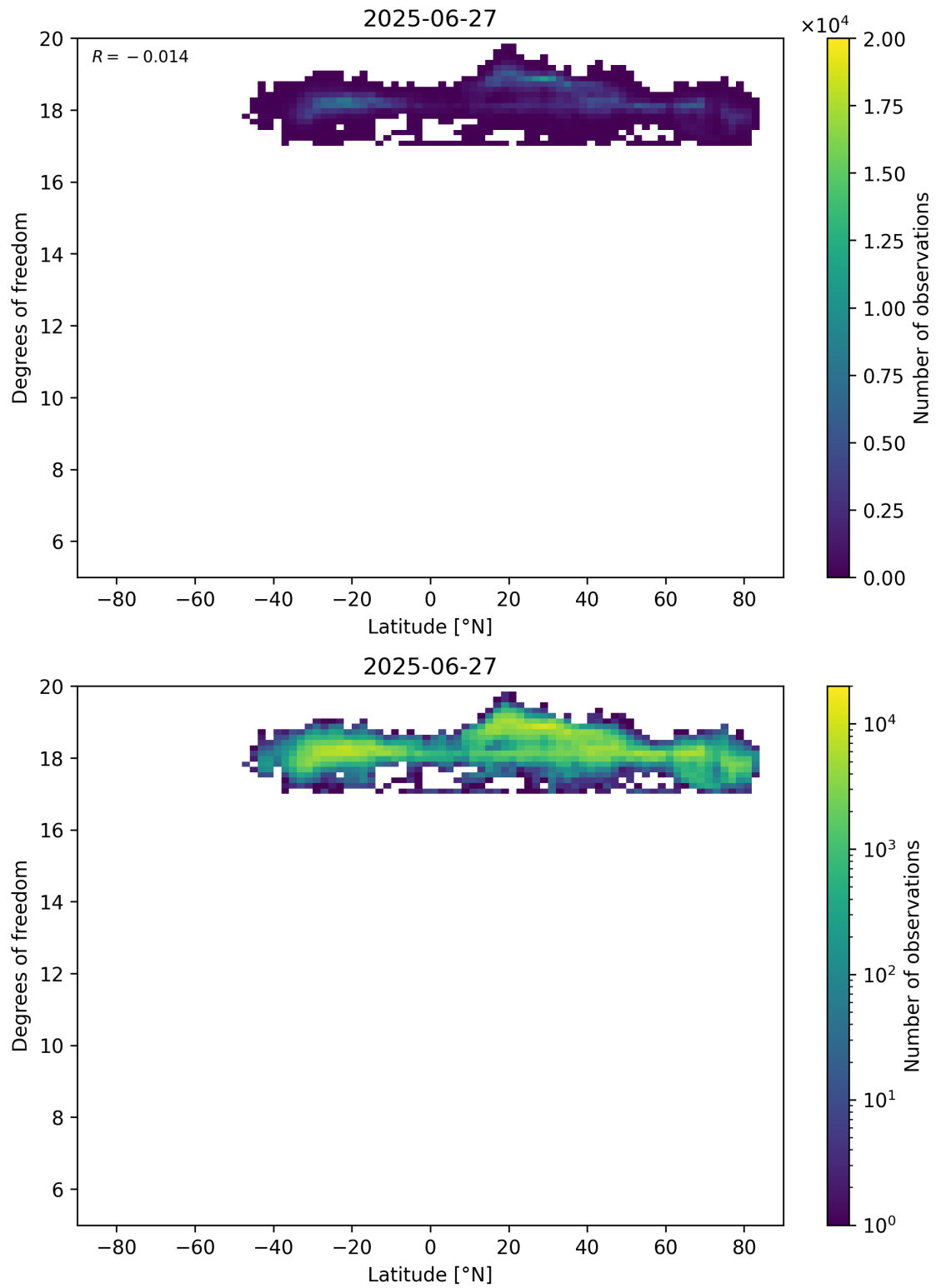
Figure 55: Scatter density plot of “Latitude” against “Degrees of freedom” for 2025-06-27 to 2025-06-28.
