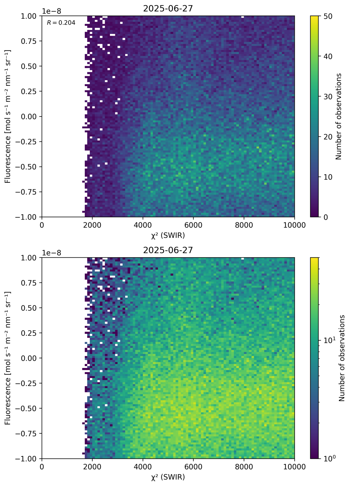
Figure 49: Scatter density plot of “ \chi^2 (SWIR)” against “Fluorescence” for 2025-06-27 to 2025-06-28.
