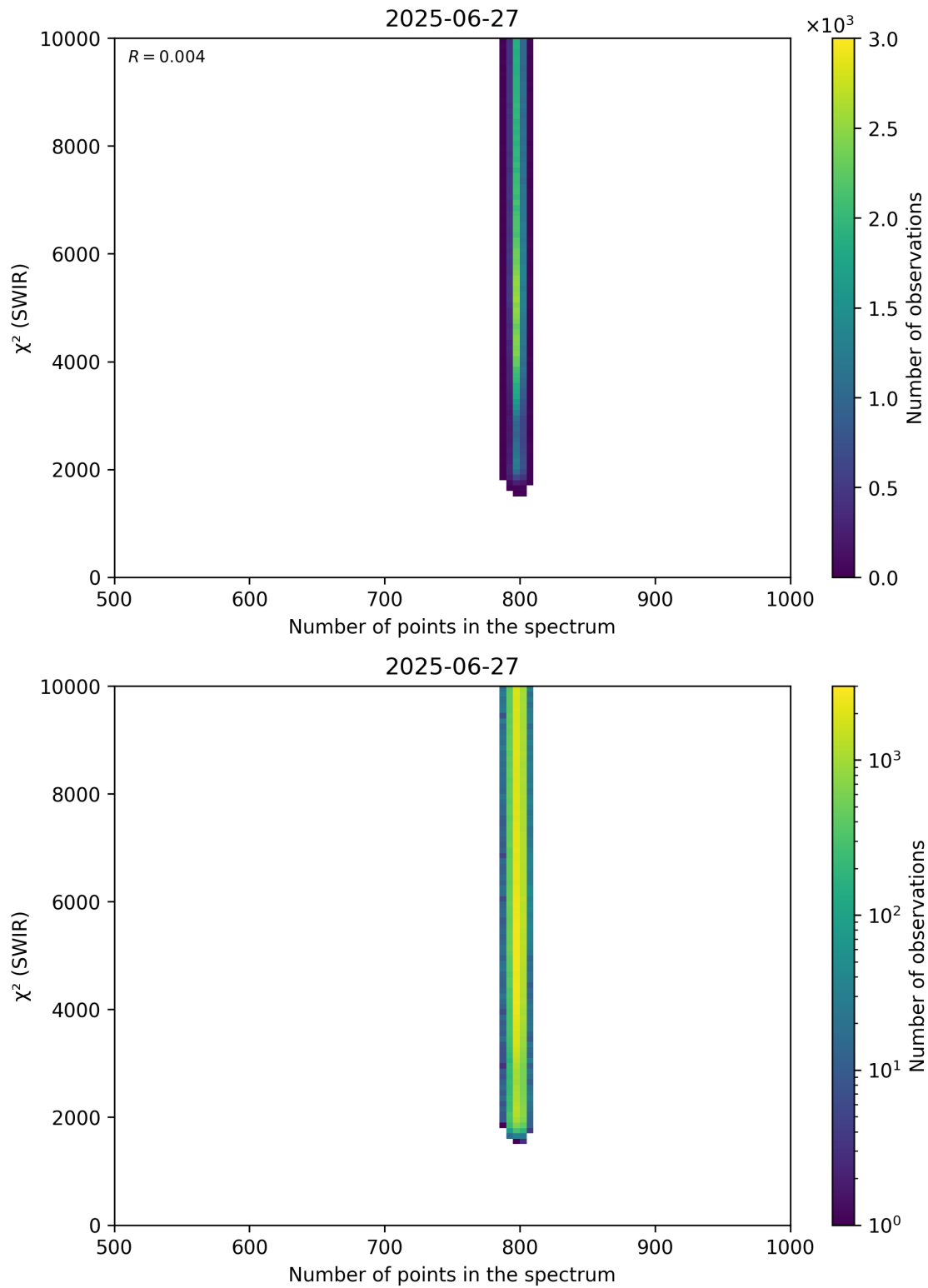
Figure 89: Scatter density plot of “Number of points in the spectrum” against “ \chi^2 (SWIR)” for 2025-06-27 to 2025-06-28.
