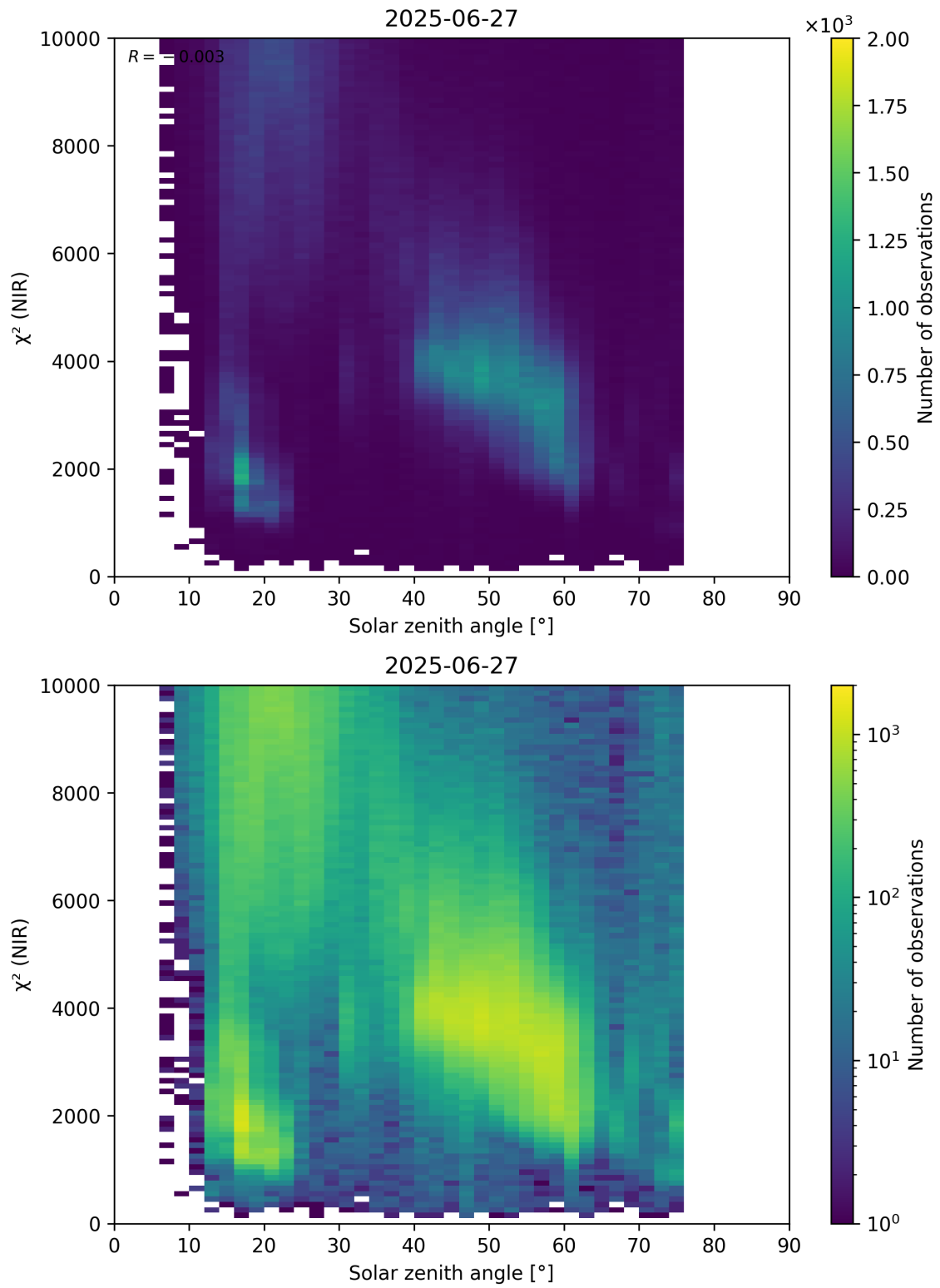
Figure 94: Scatter density plot of “Solar zenith angle” against “ \chi^2 (NIR)” for 2025-06-27 to 2025-06-28.
