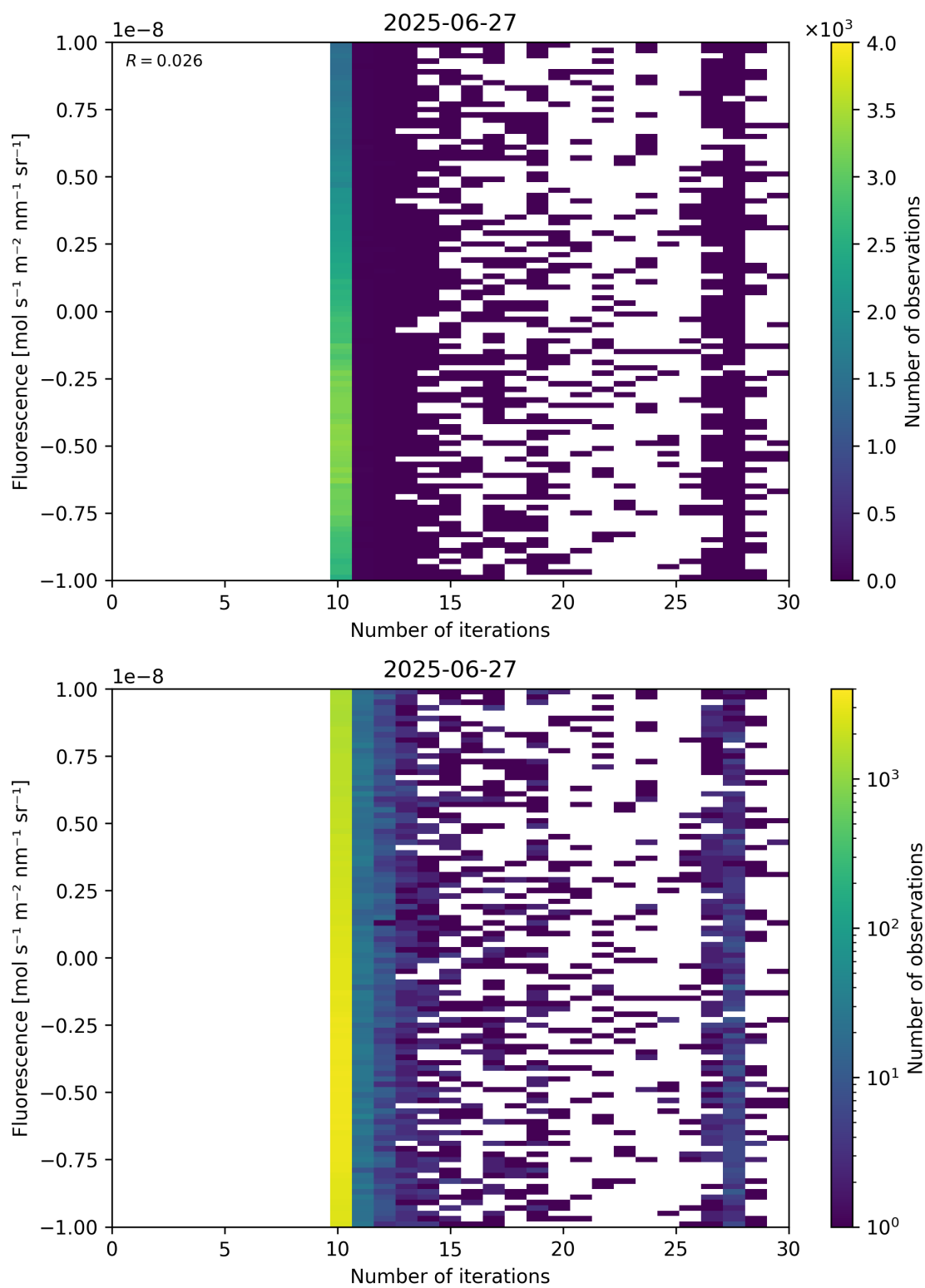
Figure 87: Scatter density plot of “Number of iterations” against “Fluorescence” for 2025-06-27 to 2025-06-28.
