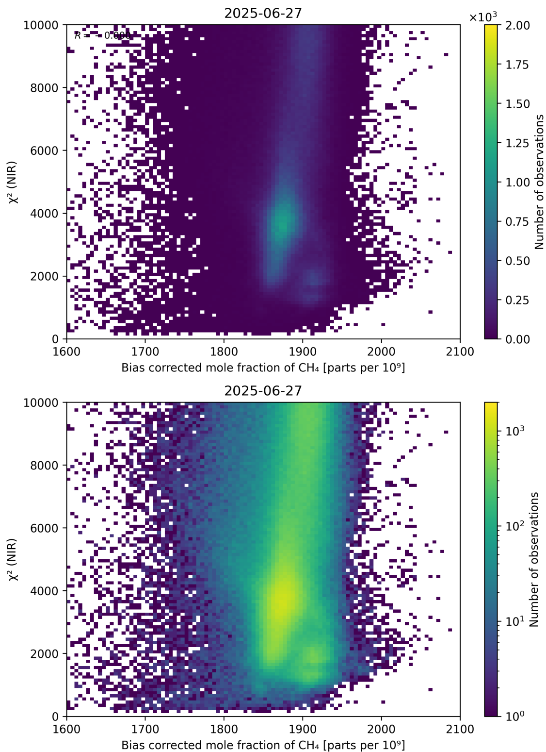
Figure 63: Scatter density plot of “Bias corrected mole fraction of \text{CH}_4 ” against “ \chi^2 (NIR)” for 2025-06-27 to 2025-06-28.
