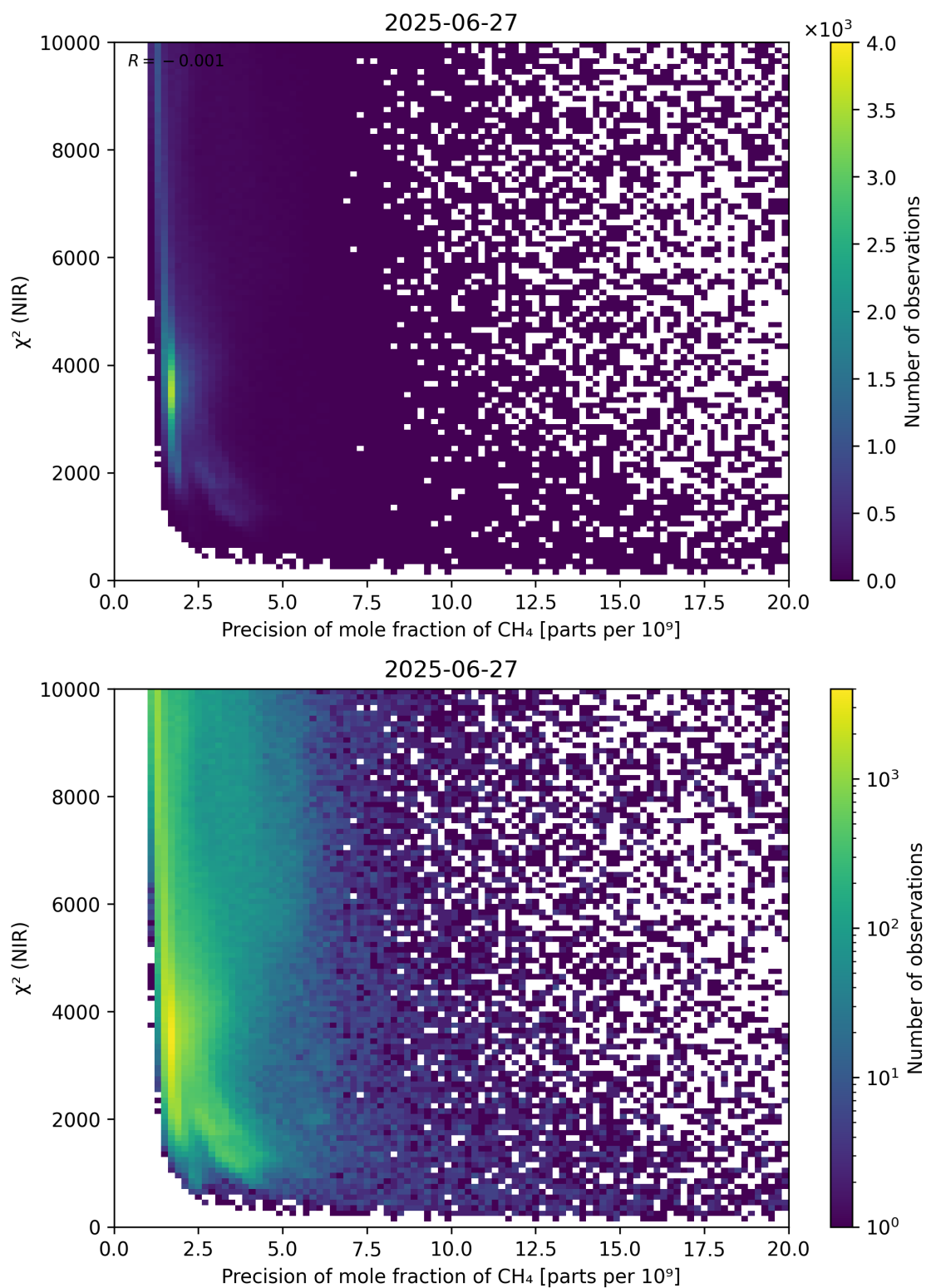
Figure 78: Scatter density plot of “Precision of mole fraction of CH 4 ” against “ \chi^2 (NIR)” for 2025-06-27 to 2025-06-28.
