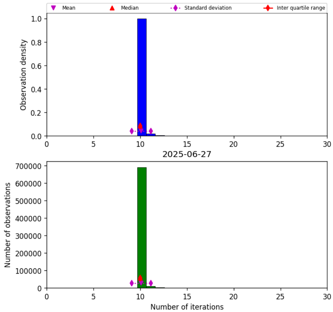
Figure 31: Histogram of “Number of iterations” for 2025-06-27 to 2025-06-28
