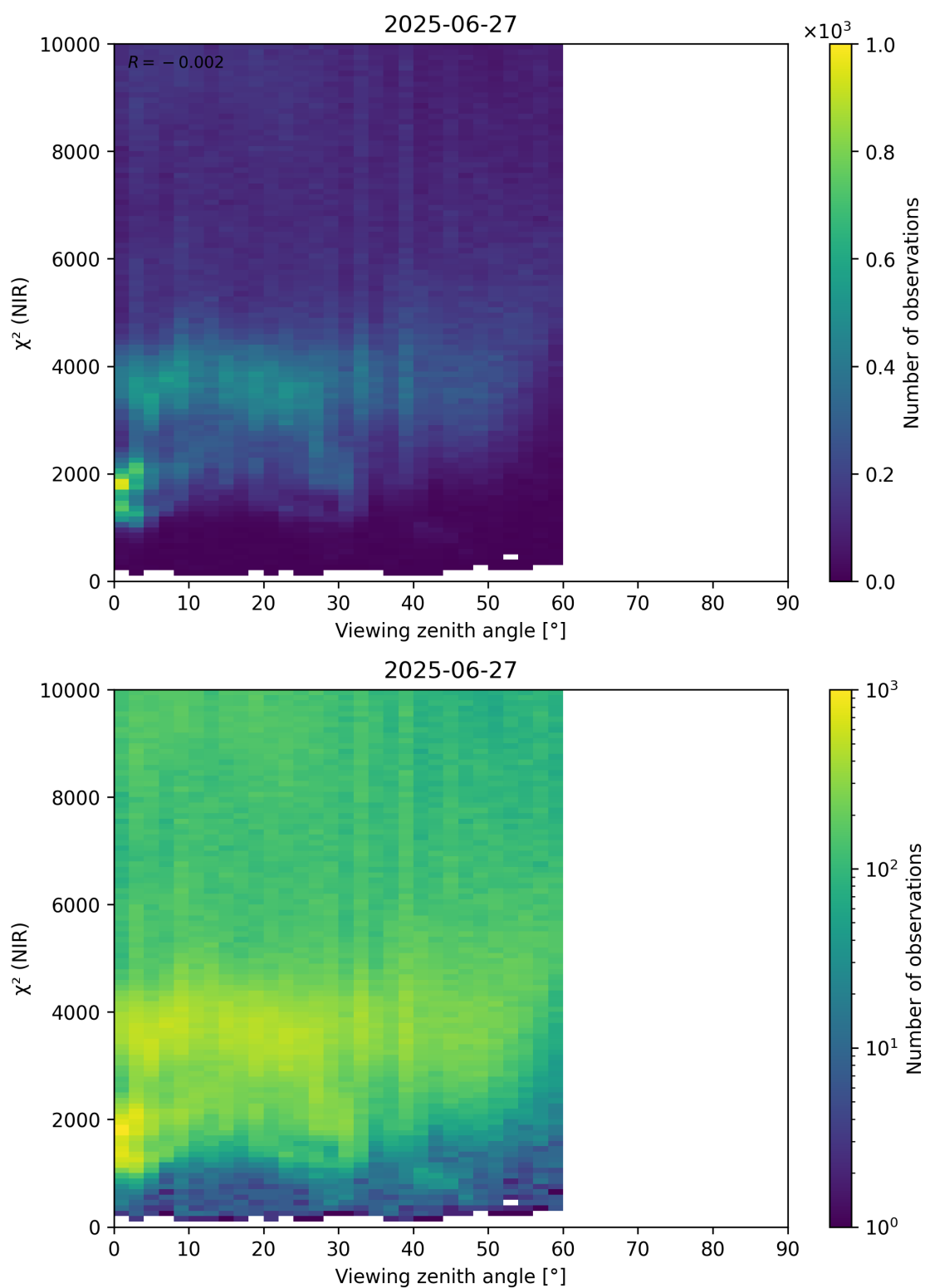
Figure 105: Scatter density plot of “Viewing zenith angle” against “ \chi^2 (NIR)” for 2025-06-27 to 2025-06-28.
