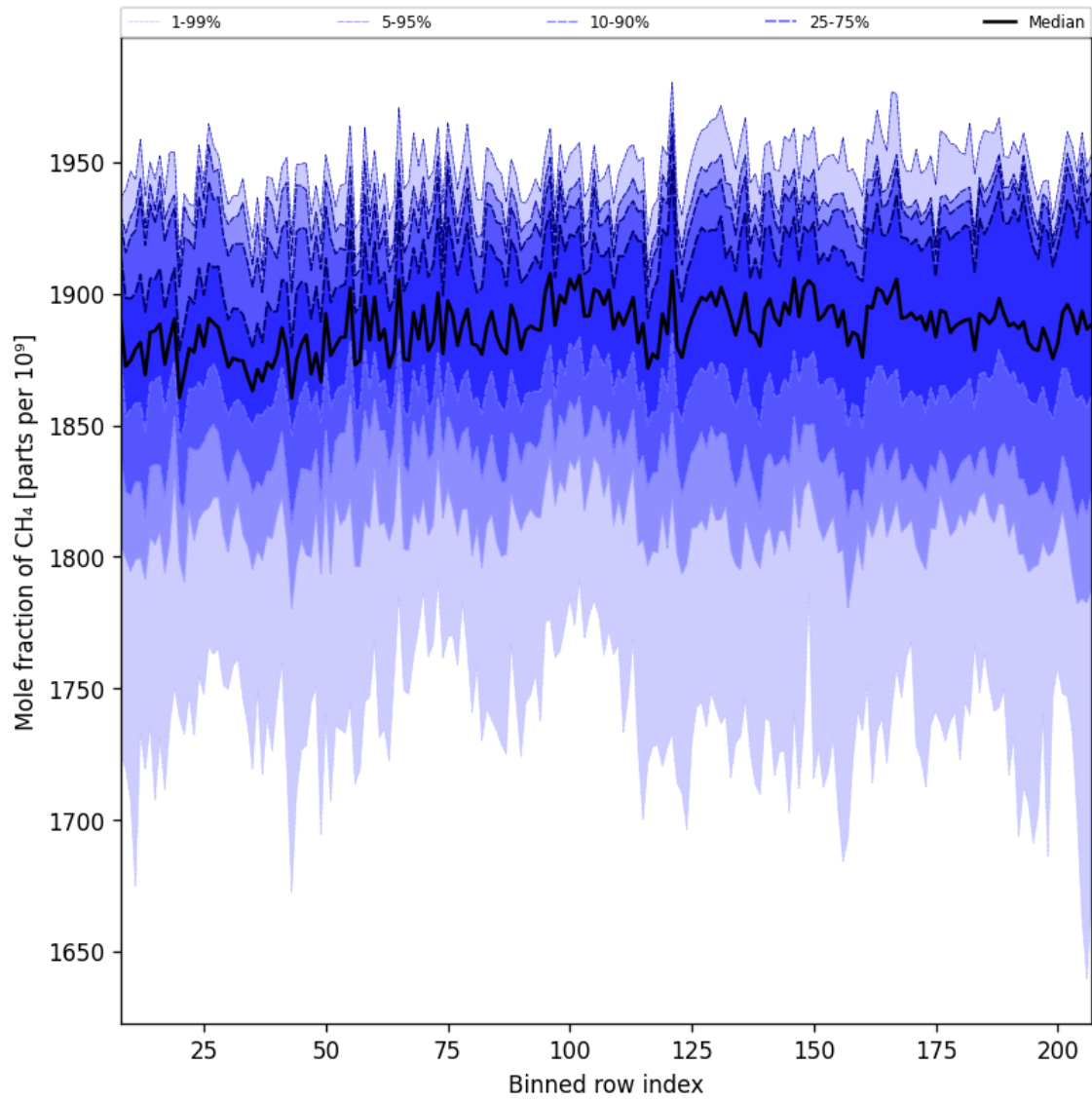
Figure 34: Along track statistics of “Mole fraction of CH 4 ” for 2025-06-27 to 2025-06-28
