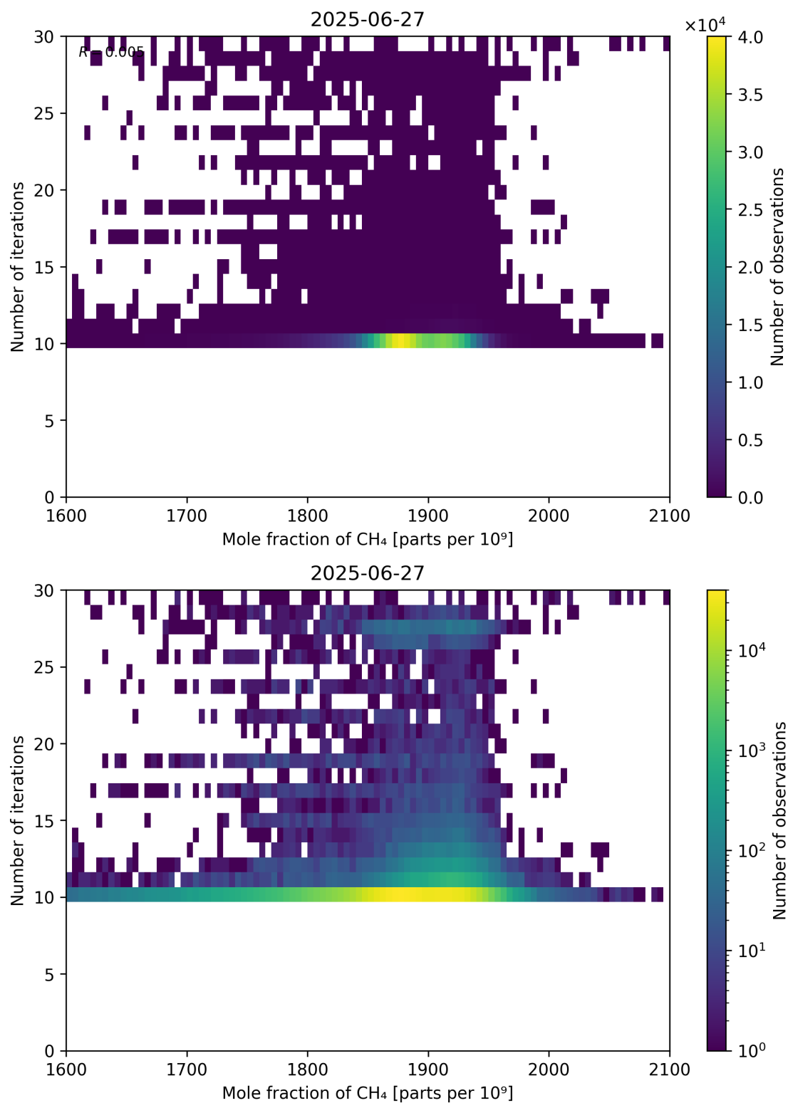
Figure 76: Scatter density plot of “Mole fraction of CH 4 ” against “Number of iterations” for 2025-06-27 to 2025-06-28.
