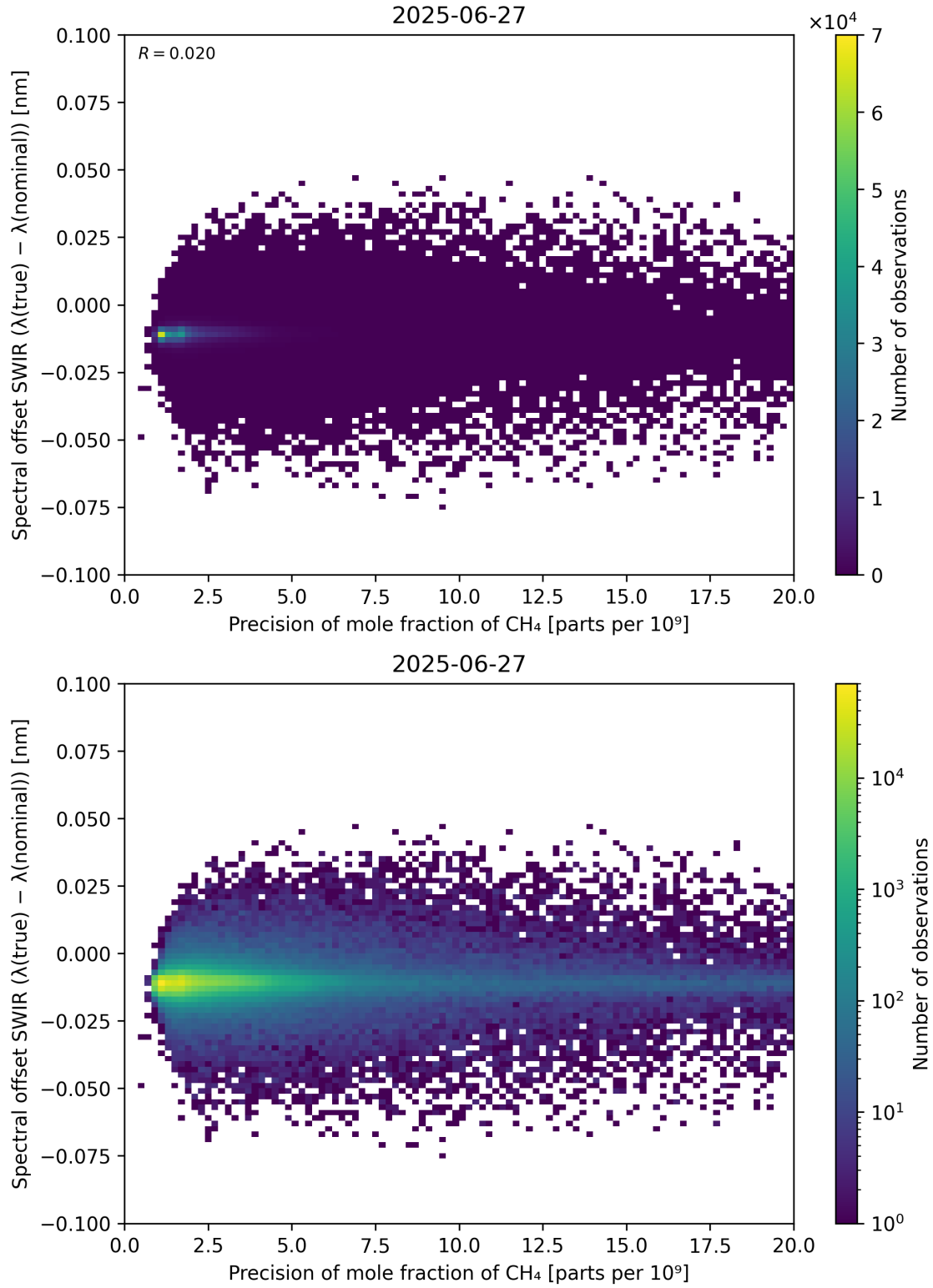
Figure 85: Scatter density plot of “Precision of mole fraction of \text{CH}_4 ” against “Spectral offset SWIR ( \lambda_{\text{true}} - \lambda_{\text{nominal}} )” for 2025-06-27 to 2025-06-28.
