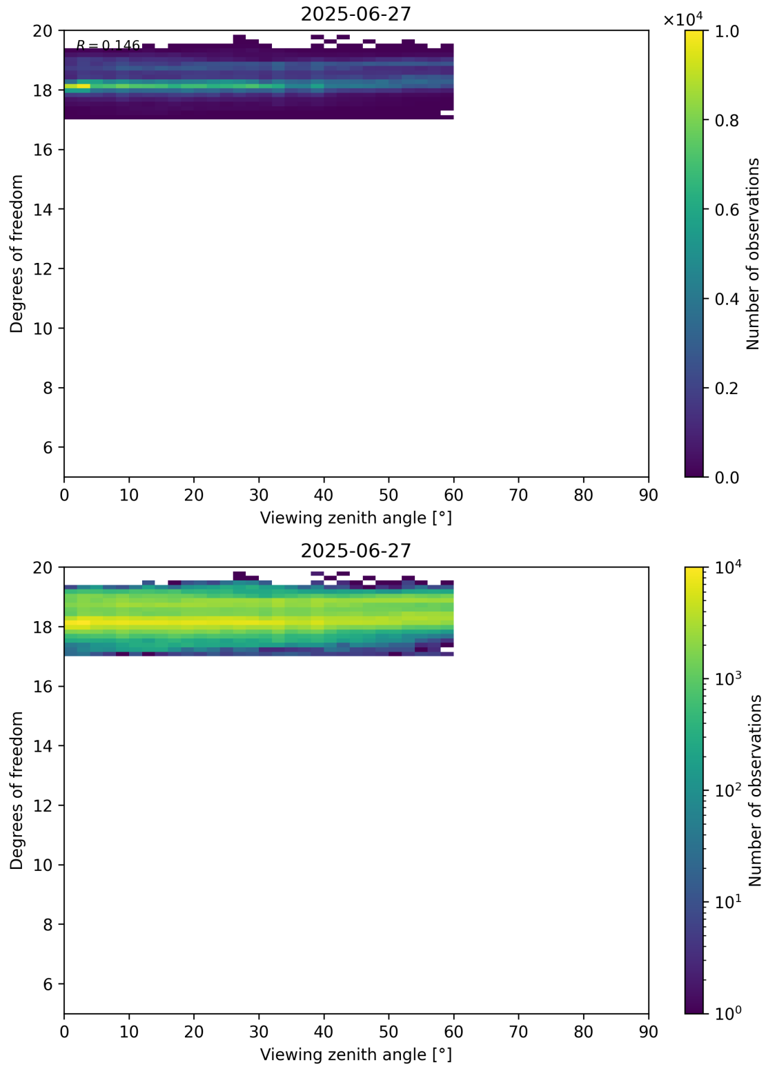
Figure 107: Scatter density plot of “Viewing zenith angle” against “Degrees of freedom” for 2025-06-27 to 2025-06-28.
