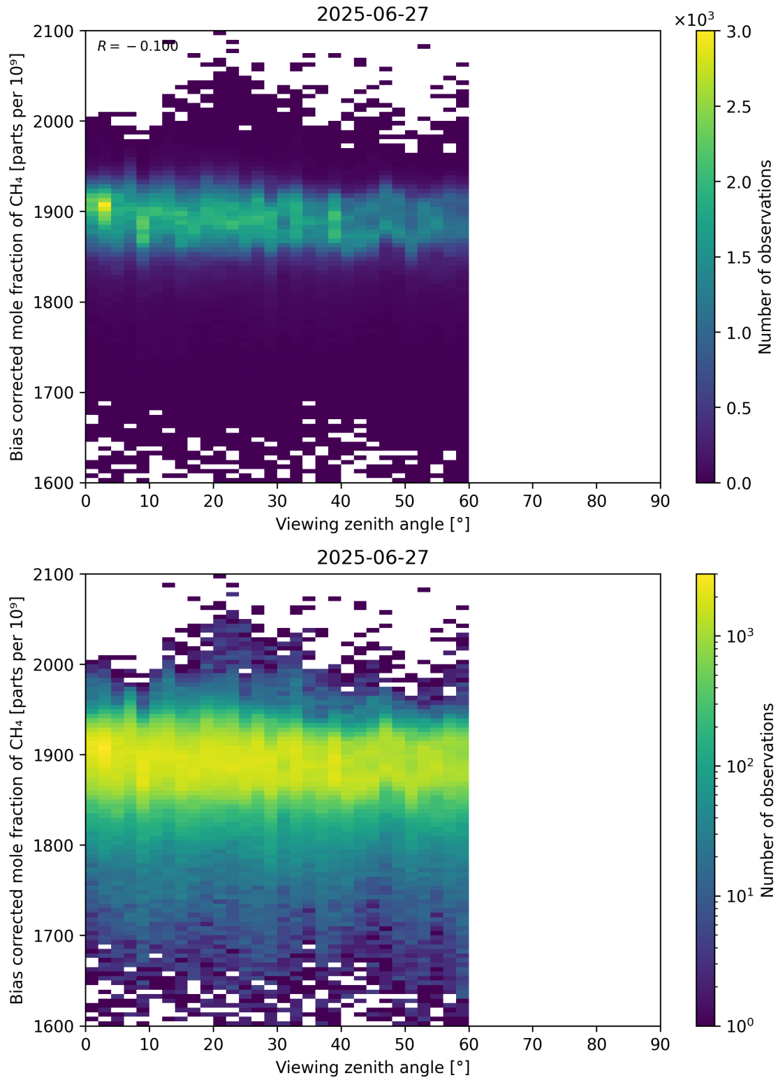
Figure 111: Scatter density plot of “Viewing zenith angle” against “Bias corrected mole fraction of CH 4 ” for 2025-06-27 to 2025-06-28.
