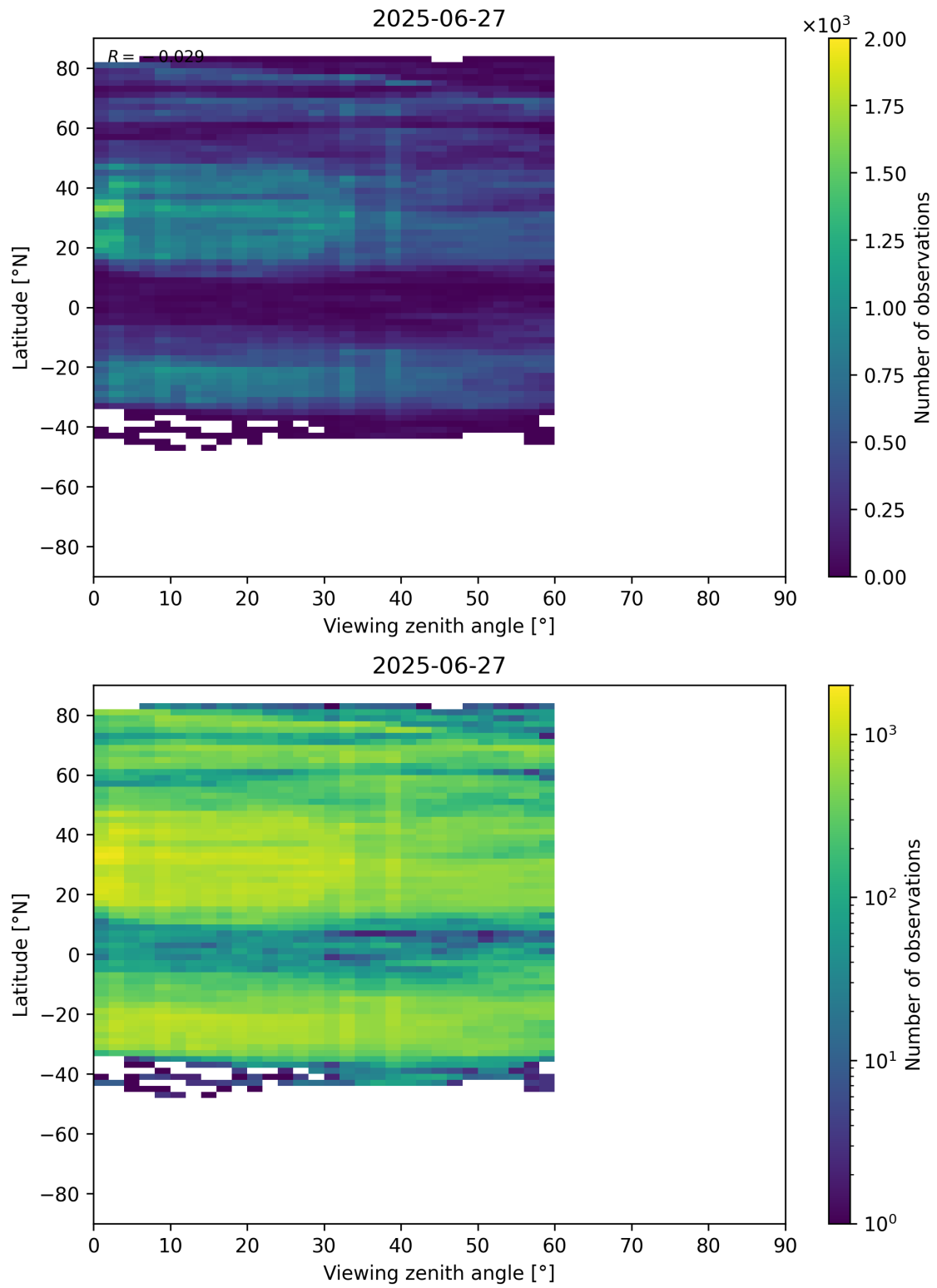
Figure 109: Scatter density plot of “Viewing zenith angle” against “Latitude” for 2025-06-27 to 2025-06-28.
