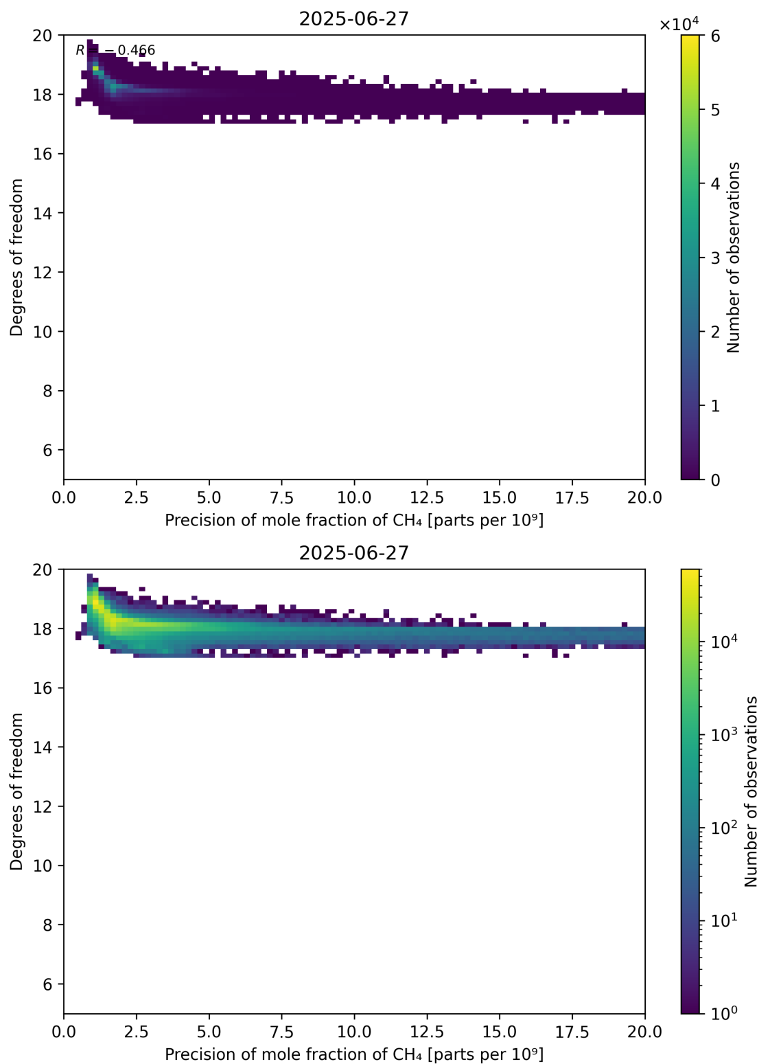
Figure 80: Scatter density plot of “Precision of mole fraction of CH 4 ” against “Degrees of freedom” for 2025-06-27 to 2025-06-28.
