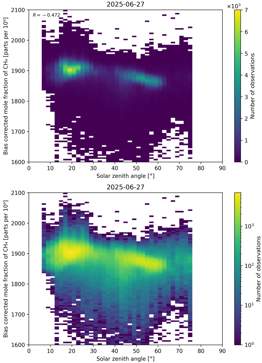
Figure 100: Scatter density plot of “Solar zenith angle” against “Bias corrected mole fraction of CH 4 ” for 2025-06-27 to 2025-06-28.
