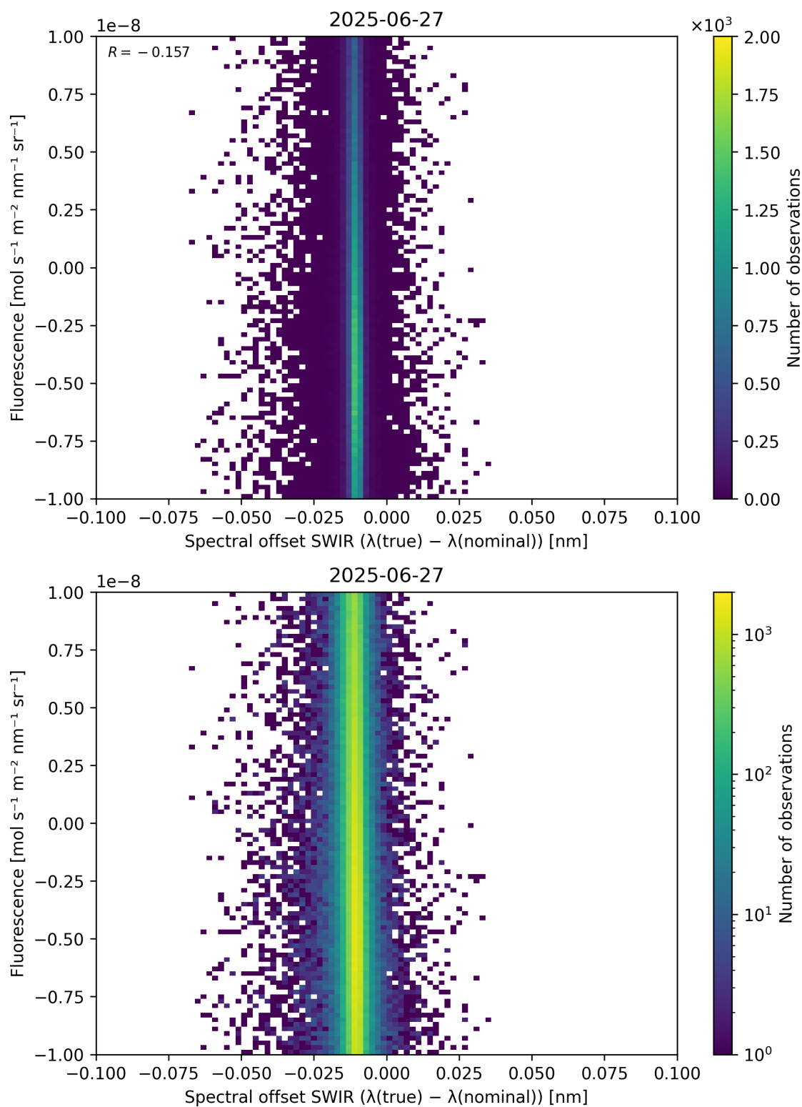
Figure 120: Scatter density plot of “Spectral offset SWIR ( \lambda_{\text{true}} - \lambda_{\text{nominal}} )” against “Fluorescence” for 2025-06-27 to 2025-06-28.
