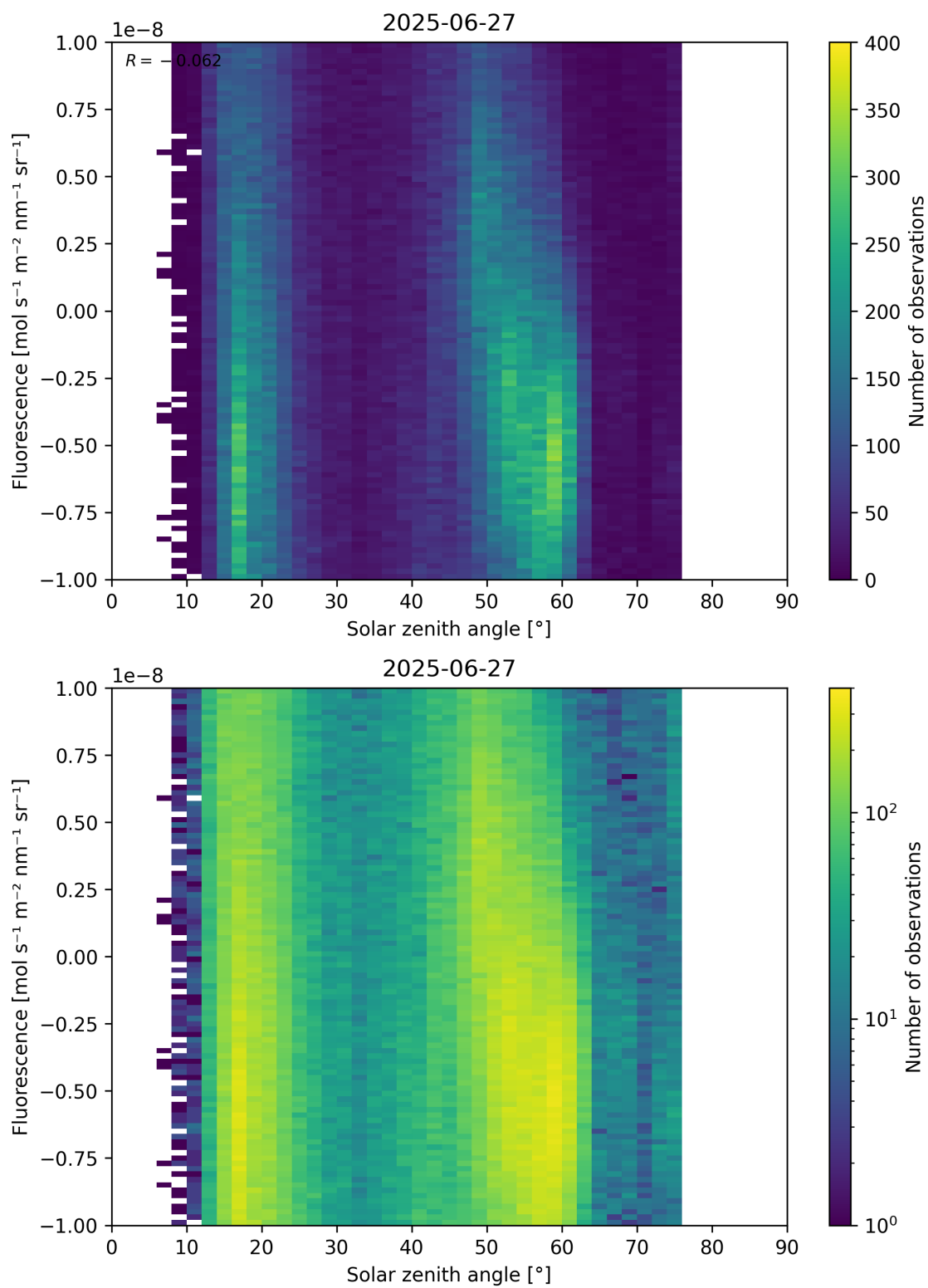
Figure 97: Scatter density plot of “Solar zenith angle” against “Fluorescence” for 2025-06-27 to 2025-06-28.
