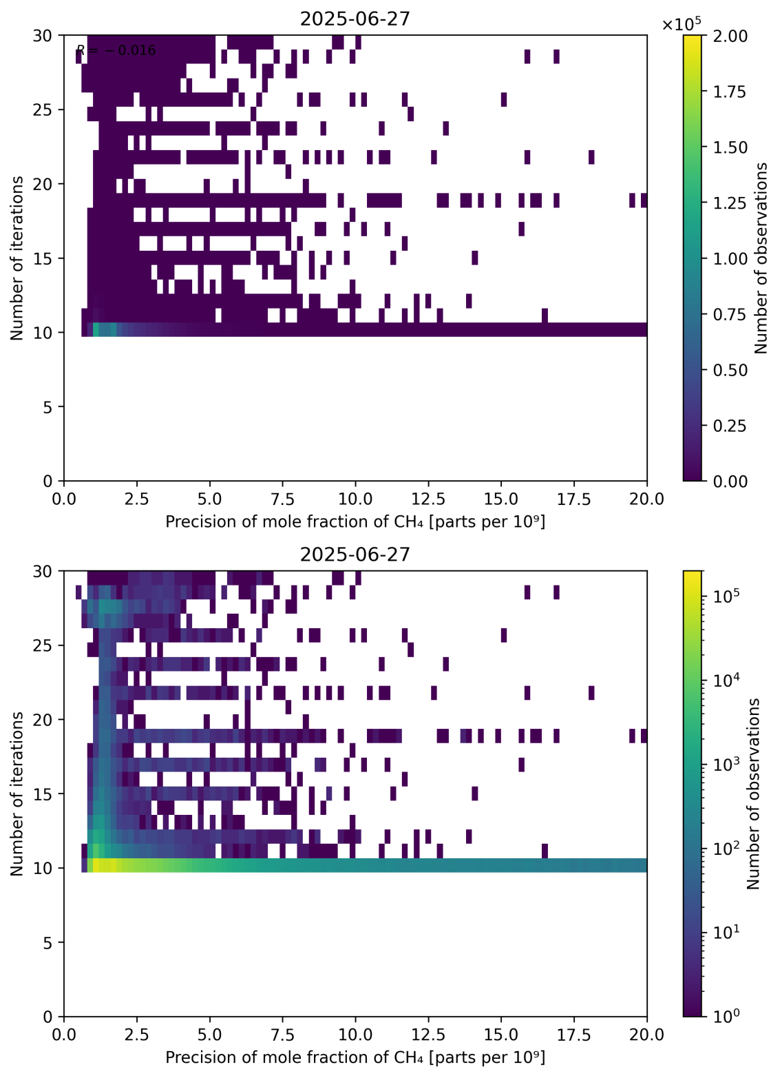
Figure 83: Scatter density plot of “Precision of mole fraction of CH 4 ” against “Number of iterations” for 2025-06-27 to 2025-06-28.
