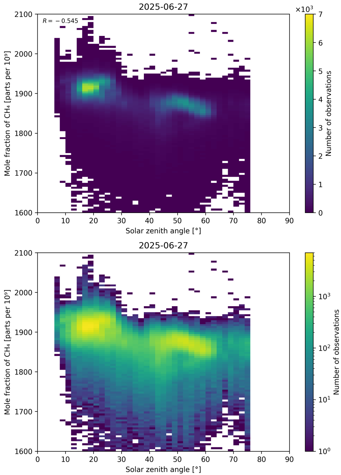
Figure 99: Scatter density plot of “Solar zenith angle” against “Mole fraction of CH 4 ” for 2025-06-27 to 2025-06-28.
