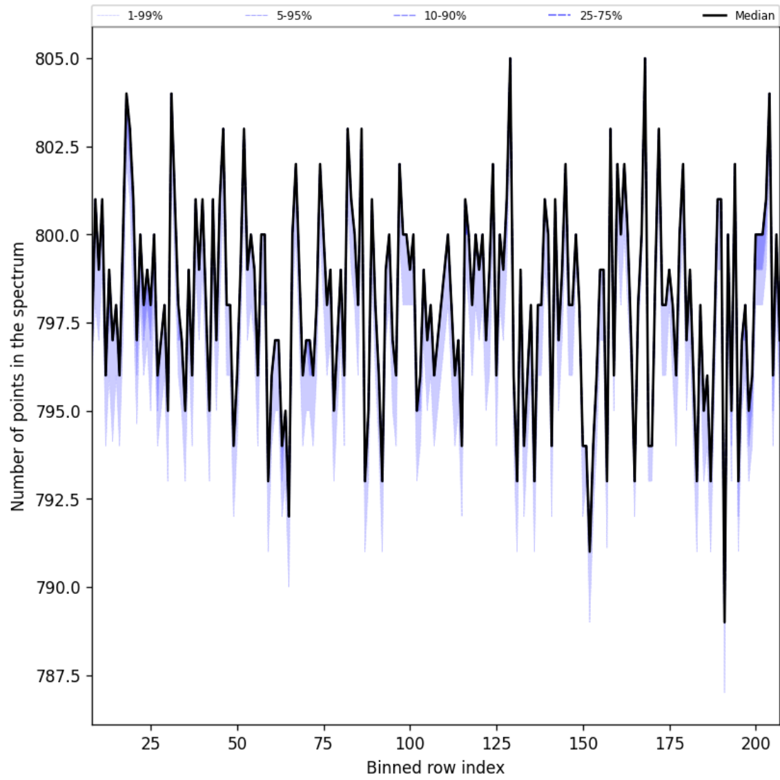
Figure 37: Along track statistics of “Number of points in the spectrum” for 2025-06-27 to 2025-06-28
