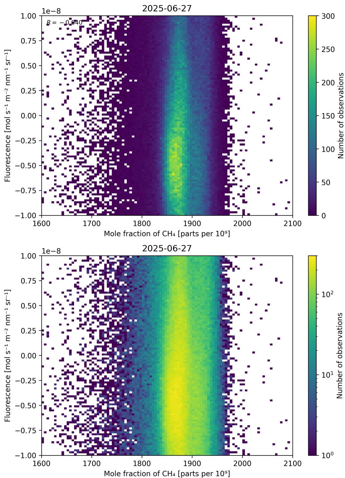
Figure 73: Scatter density plot of “Mole fraction of \text{CH}_4 ” against “Fluorescence” for 2025-06-27 to 2025-06-28.
