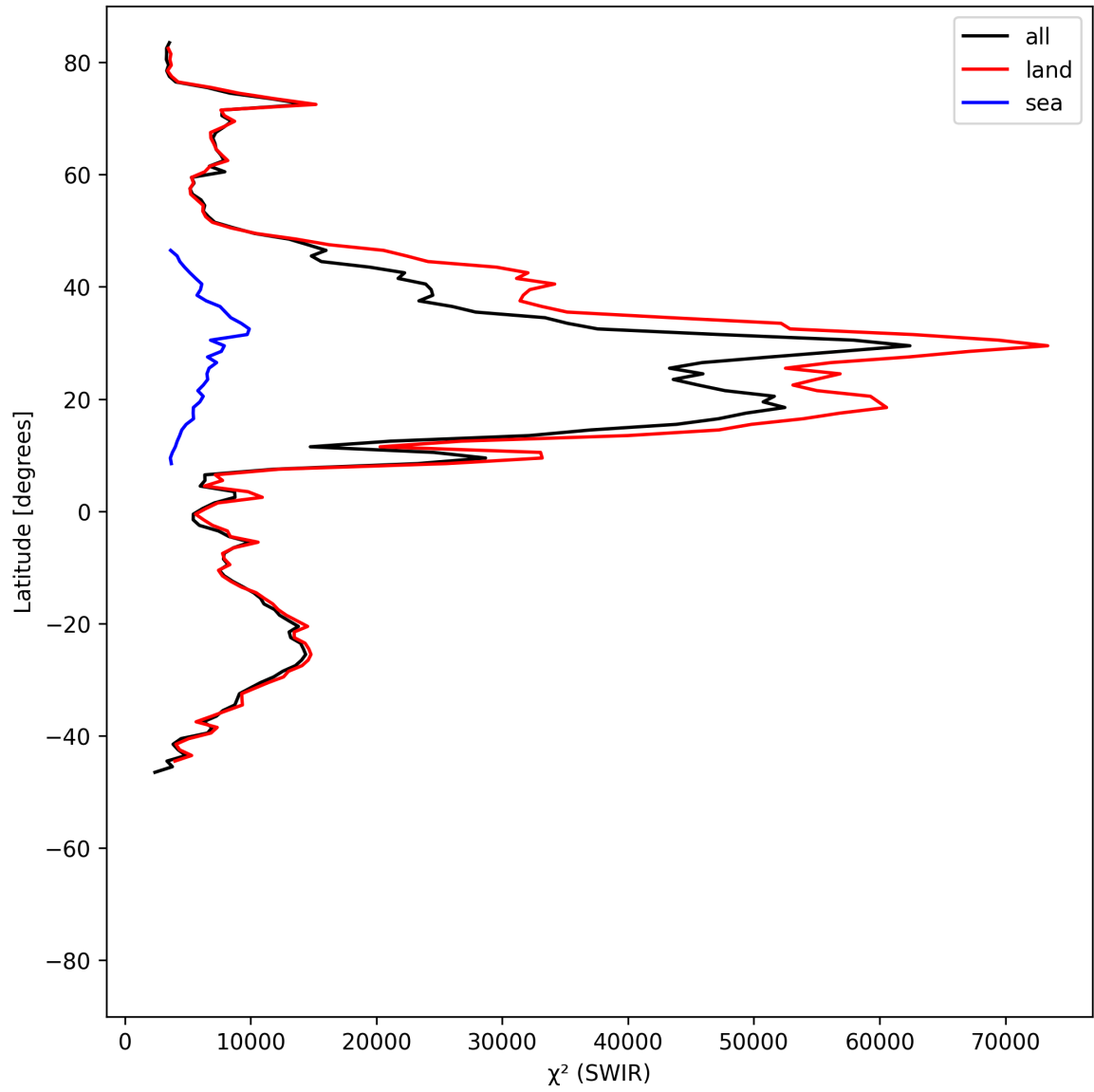
Figure 17: Zonal average of “ \chi^2 (SWIR)” for 2025-06-27 to 2025-06-28.
