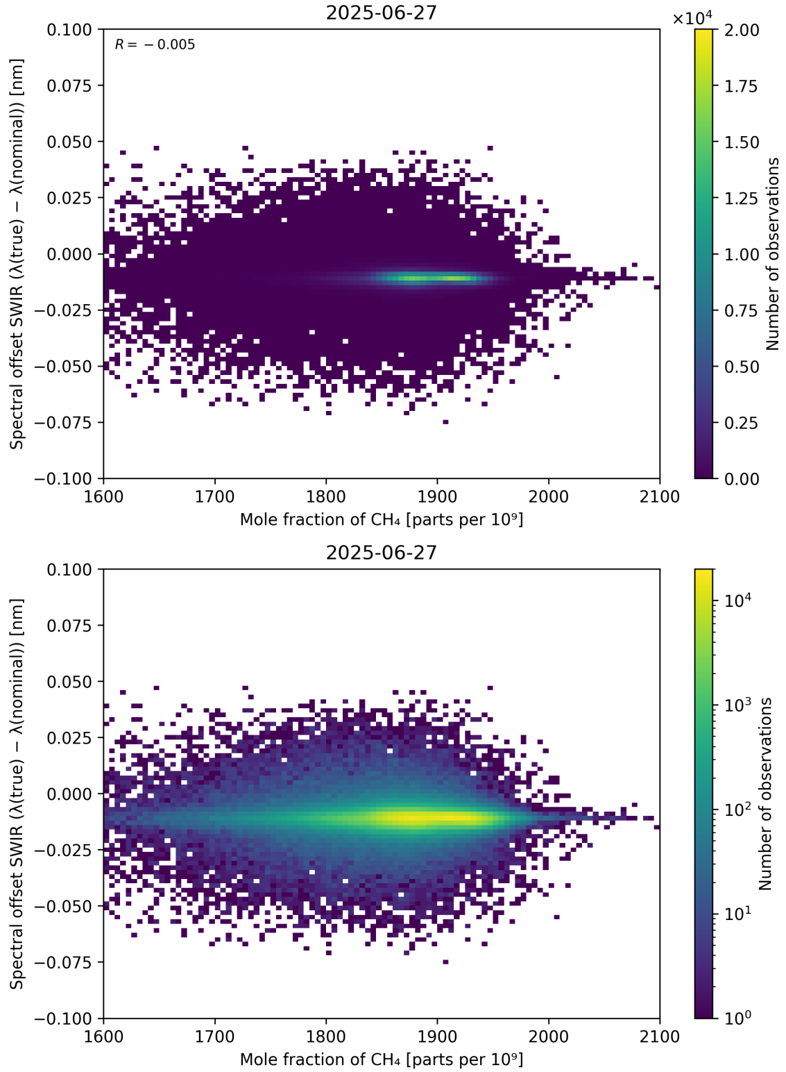
Figure 86: Scatter density plot of “Mole fraction of CH 4 ” against “Spectral offset SWIR ( \lambda_{\text{true}} - \lambda_{\text{nominal}} )” for 2025-06-27 to 2025-06-28.
