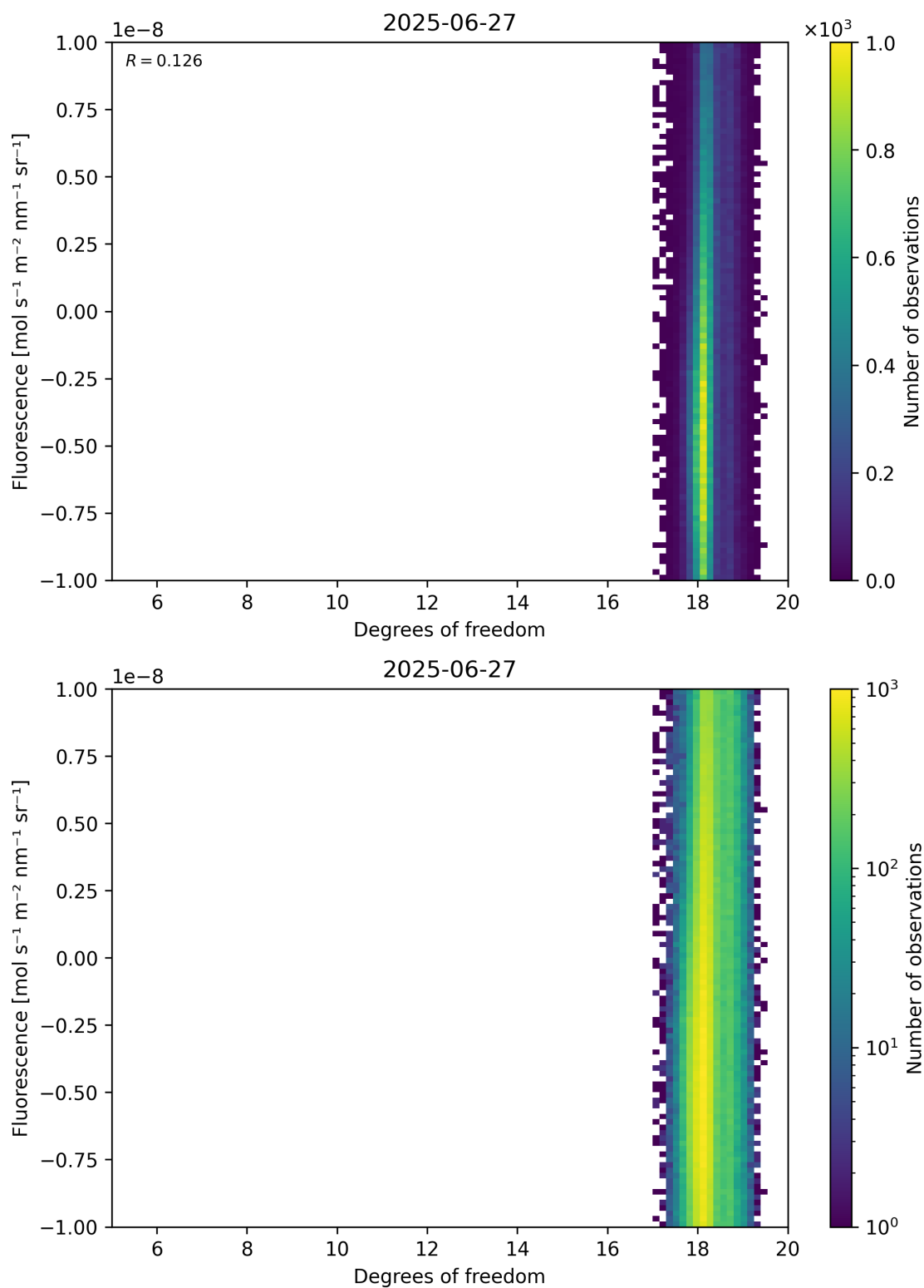
Figure 51: Scatter density plot of “Degrees of freedom” against “Fluorescence” for 2025-06-27 to 2025-06-28.
