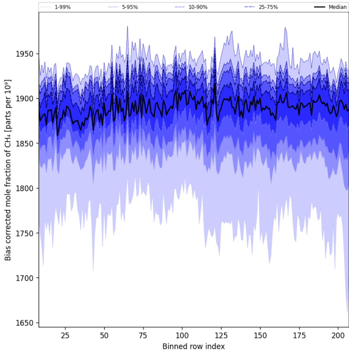
Figure 36: Along track statistics of “Bias corrected mole fraction of CH 4 ” for 2025-06-27 to 2025-06-28
