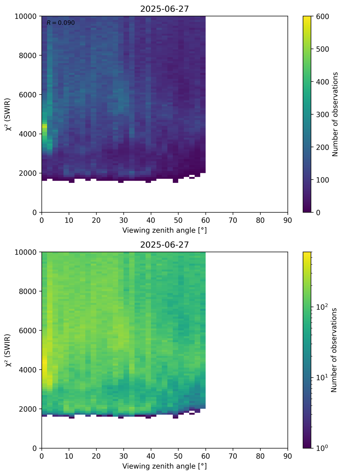
Figure 106: Scatter density plot of “Viewing zenith angle” against “ \chi^2 (SWIR)” for 2025-06-27 to 2025-06-28.
