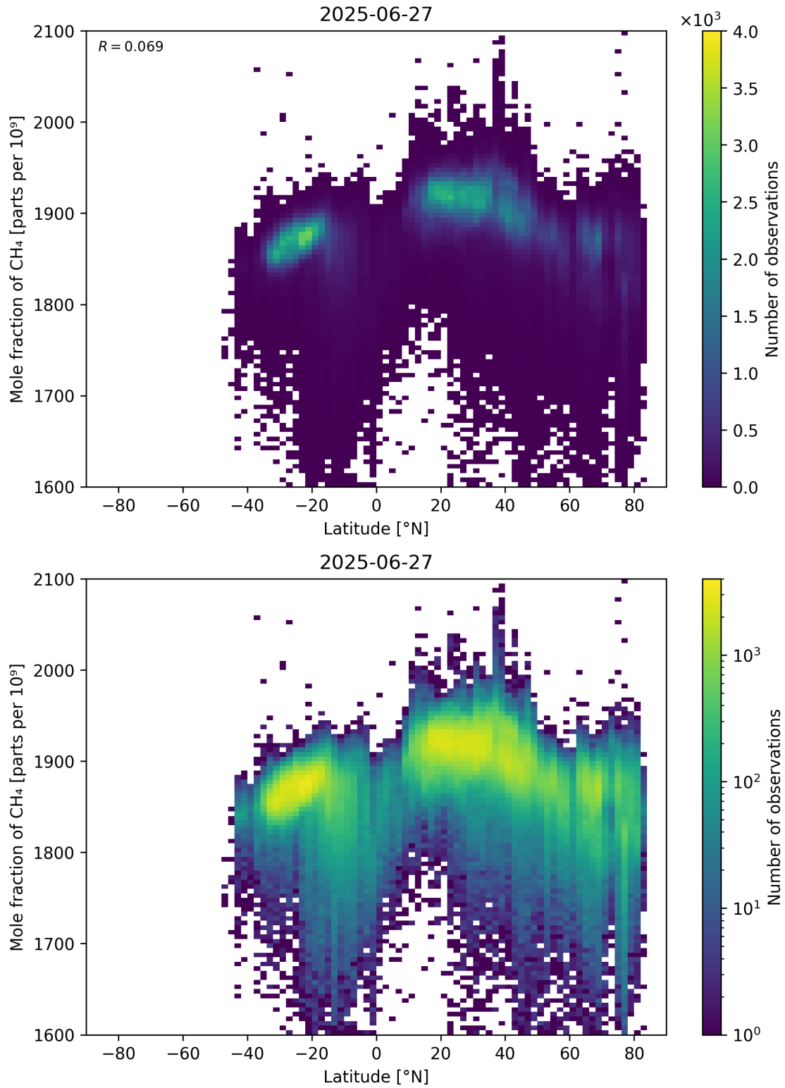
Figure 57: Scatter density plot of “Latitude” against “Mole fraction of \text{CH}_4 ” for 2025-06-27 to 2025-06-28.
