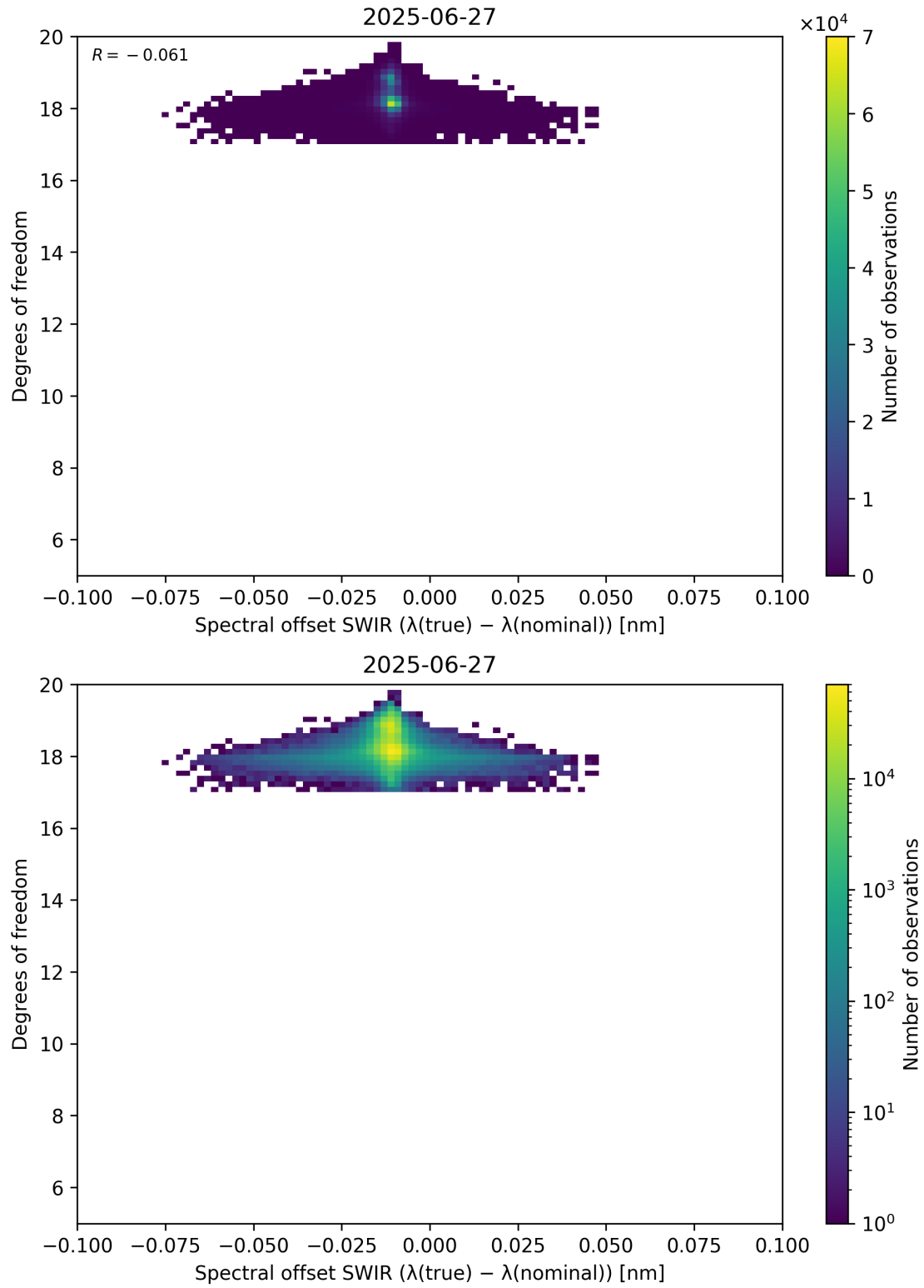
Figure 119: Scatter density plot of “Spectral offset SWIR ( \lambda_{\text{true}} - \lambda_{\text{nominal}} )” against “Degrees of freedom” for 2025-06-27 to 2025-06-28.
