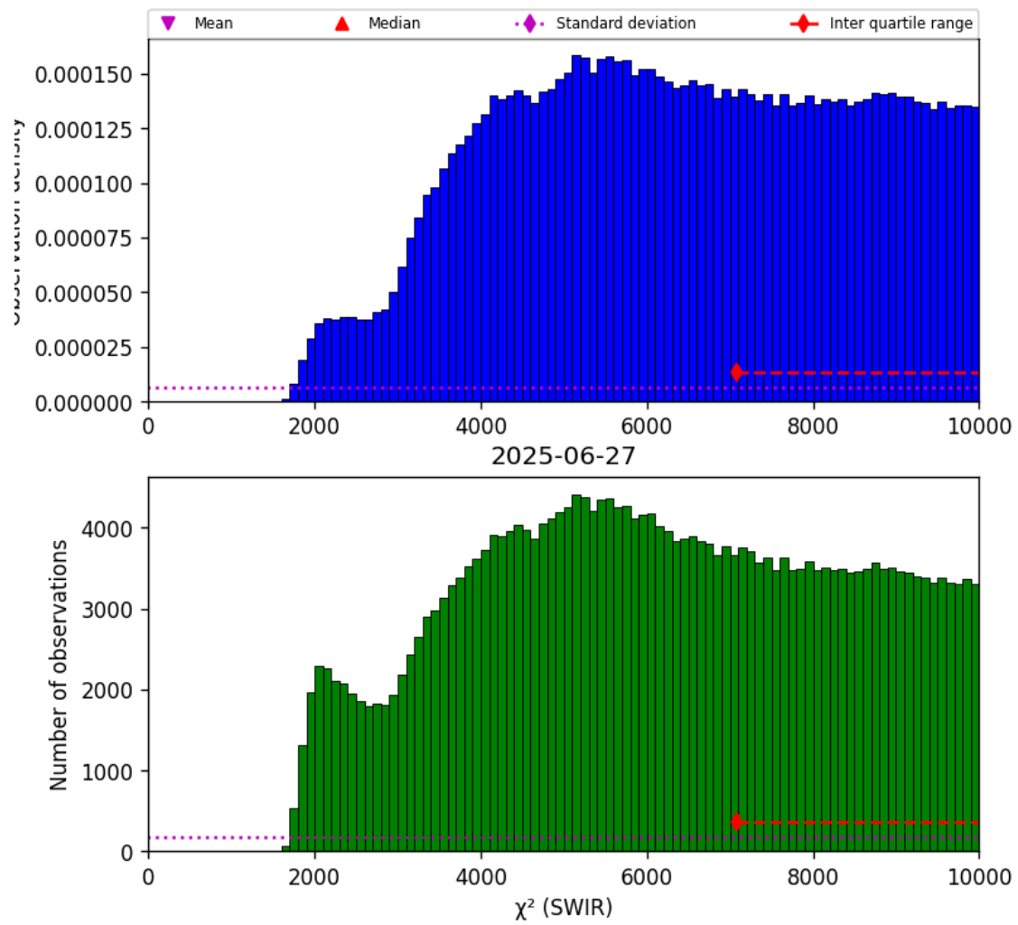
Figure 28: Histogram of “ \chi^2 (SWIR)” for 2025-06-27 to 2025-06-28
