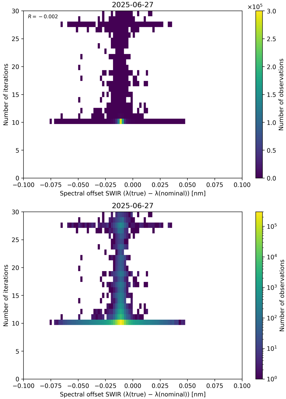
Figure 121: Scatter density plot of “Spectral offset SWIR ( \lambda_{\text{true}} - \lambda_{\text{nominal}} )” against “Number of iterations” for 2025-06-27 to 2025-06-28.
