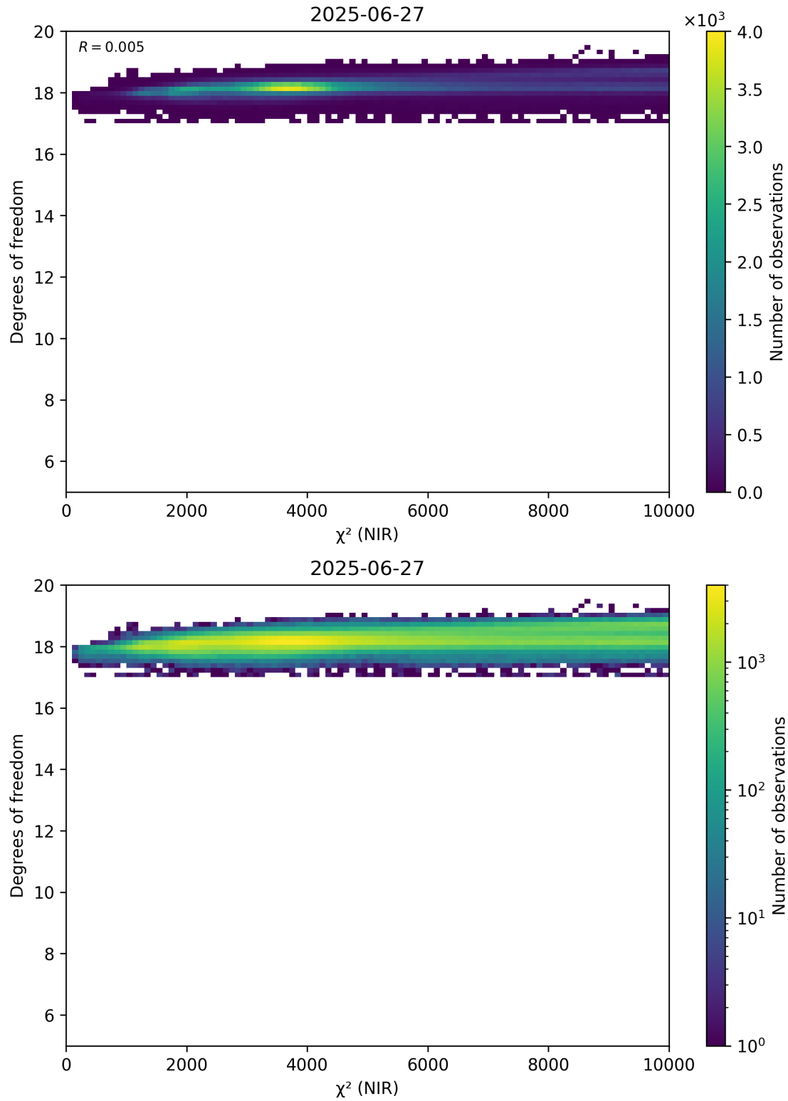
Figure 44: Scatter density plot of “ \chi^2 (NIR)” against “Degrees of freedom” for 2025-06-27 to 2025-06-28.
