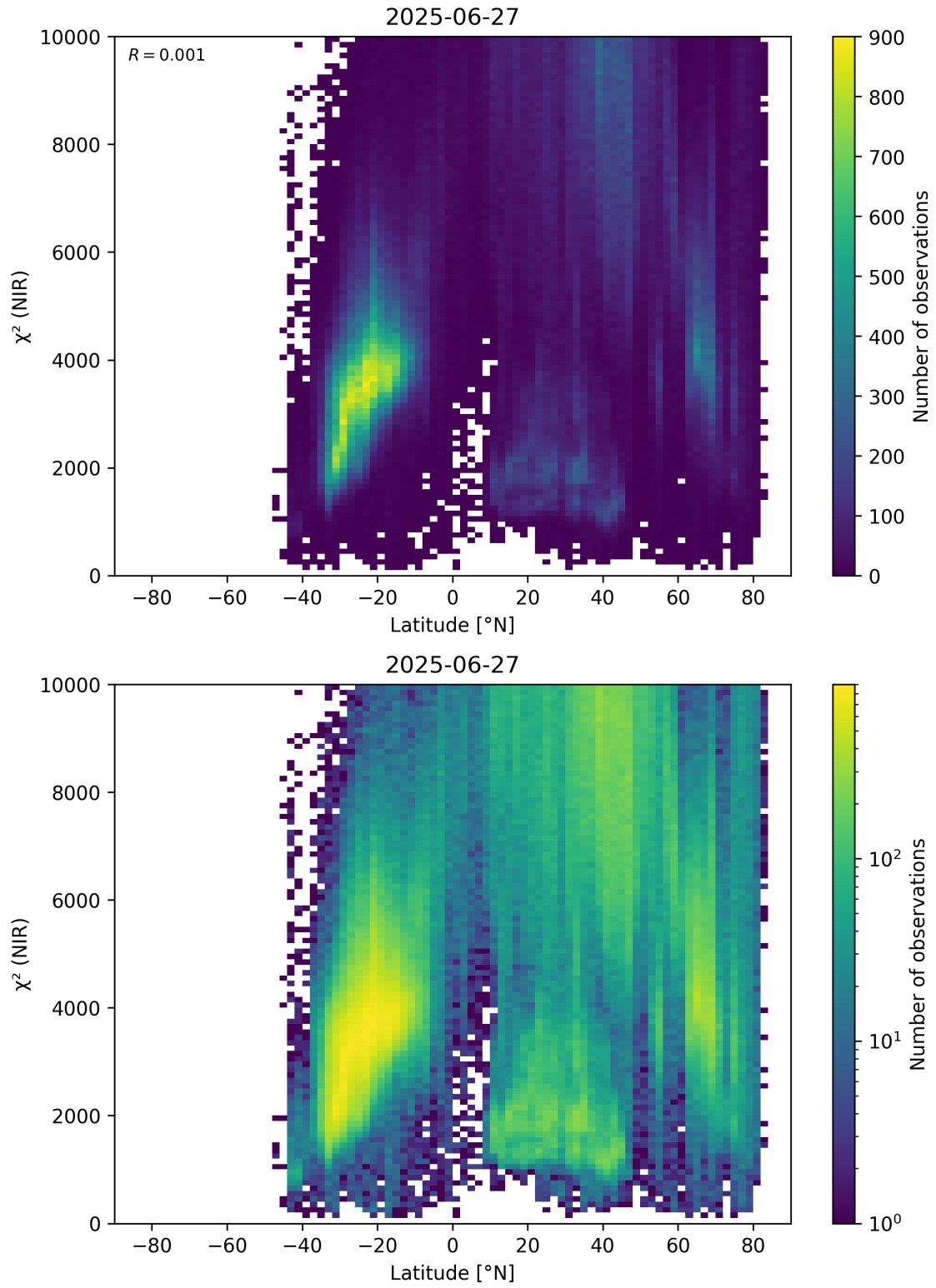
Figure 53: Scatter density plot of “Latitude” against “ \chi^2 (NIR)” for 2025-06-27 to 2025-06-28.
