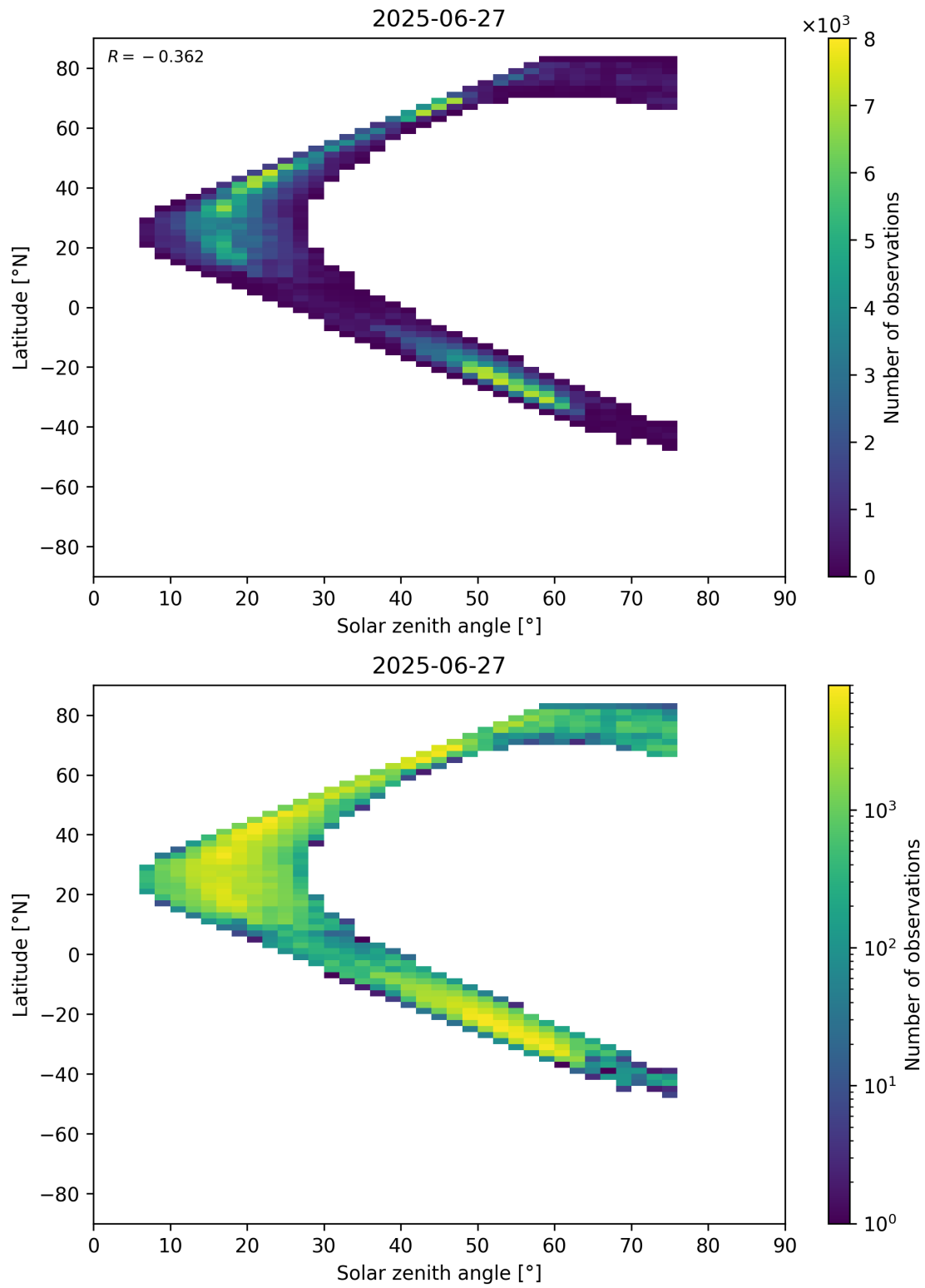
Figure 98: Scatter density plot of “Solar zenith angle” against “Latitude” for 2025-06-27 to 2025-06-28.
