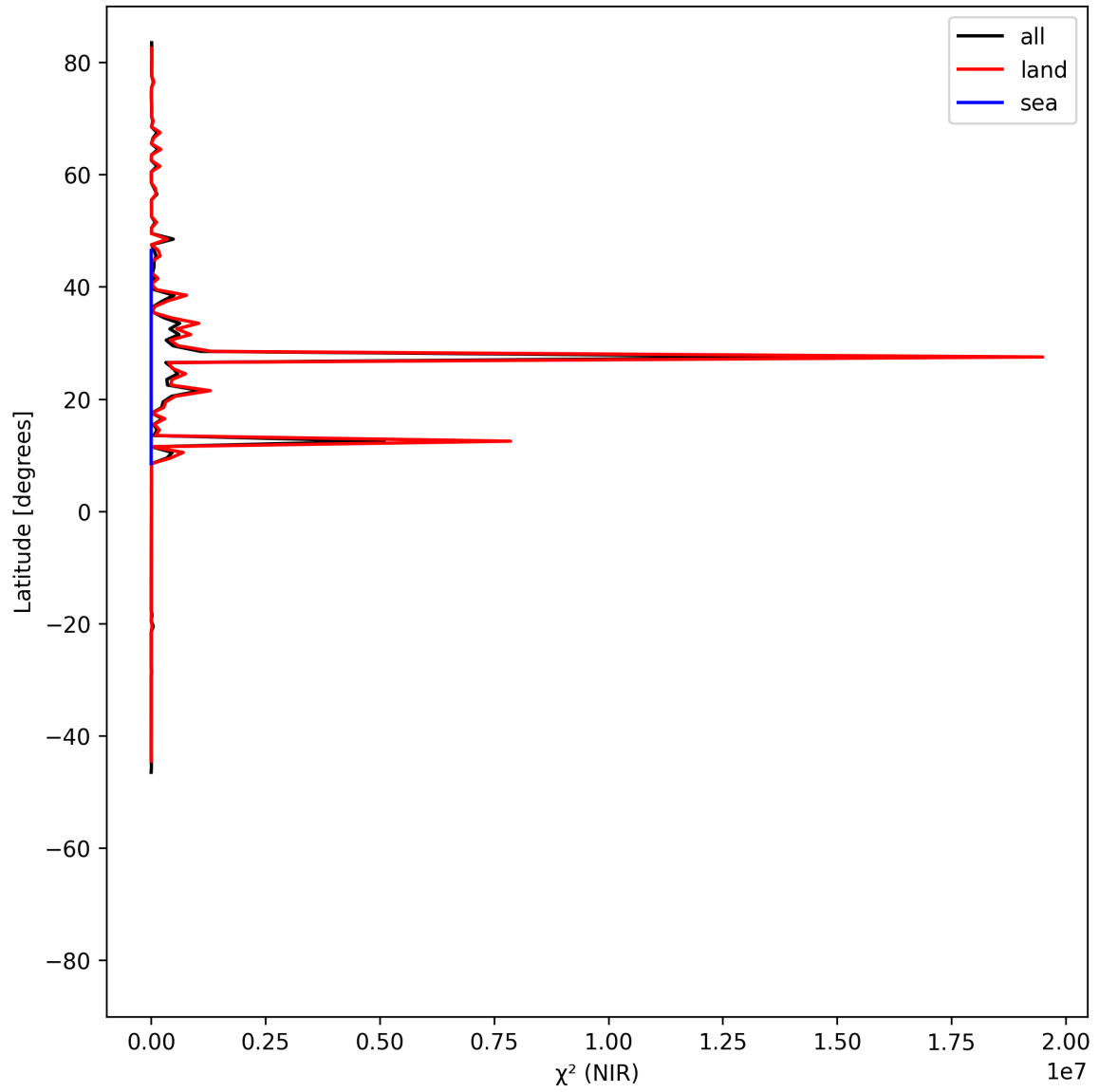
Figure 18: Zonal average of “ \chi^2 (NIR)” for 2025-06-27 to 2025-06-28.
