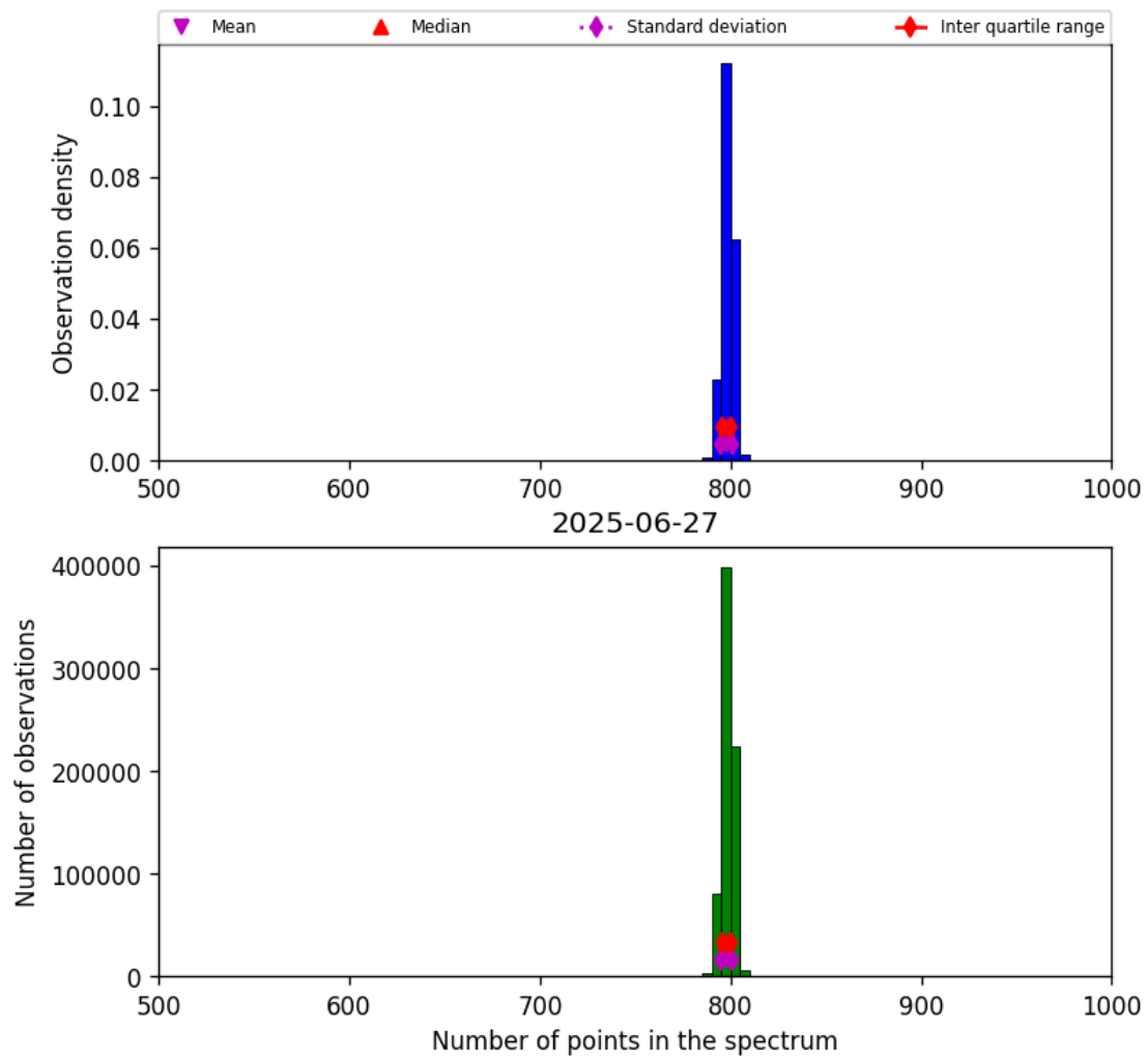
Figure 26: Histogram of “Number of points in the spectrum” for 2025-06-27 to 2025-06-28
