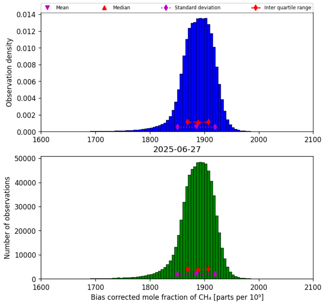
Figure 25: Histogram of “Bias corrected mole fraction of CH 4 ” for 2025-06-27 to 2025-06-28
