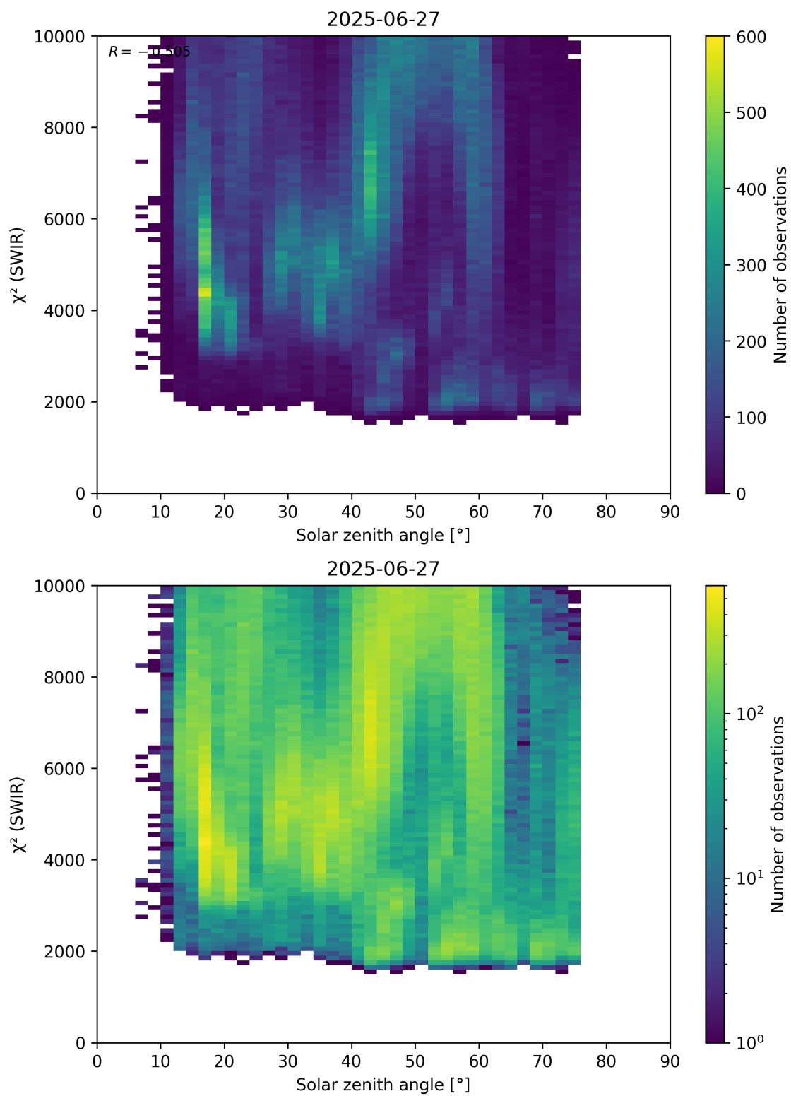
Figure 95: Scatter density plot of “Solar zenith angle” against “ \chi^2 (SWIR)” for 2025-06-27 to 2025-06-28.
