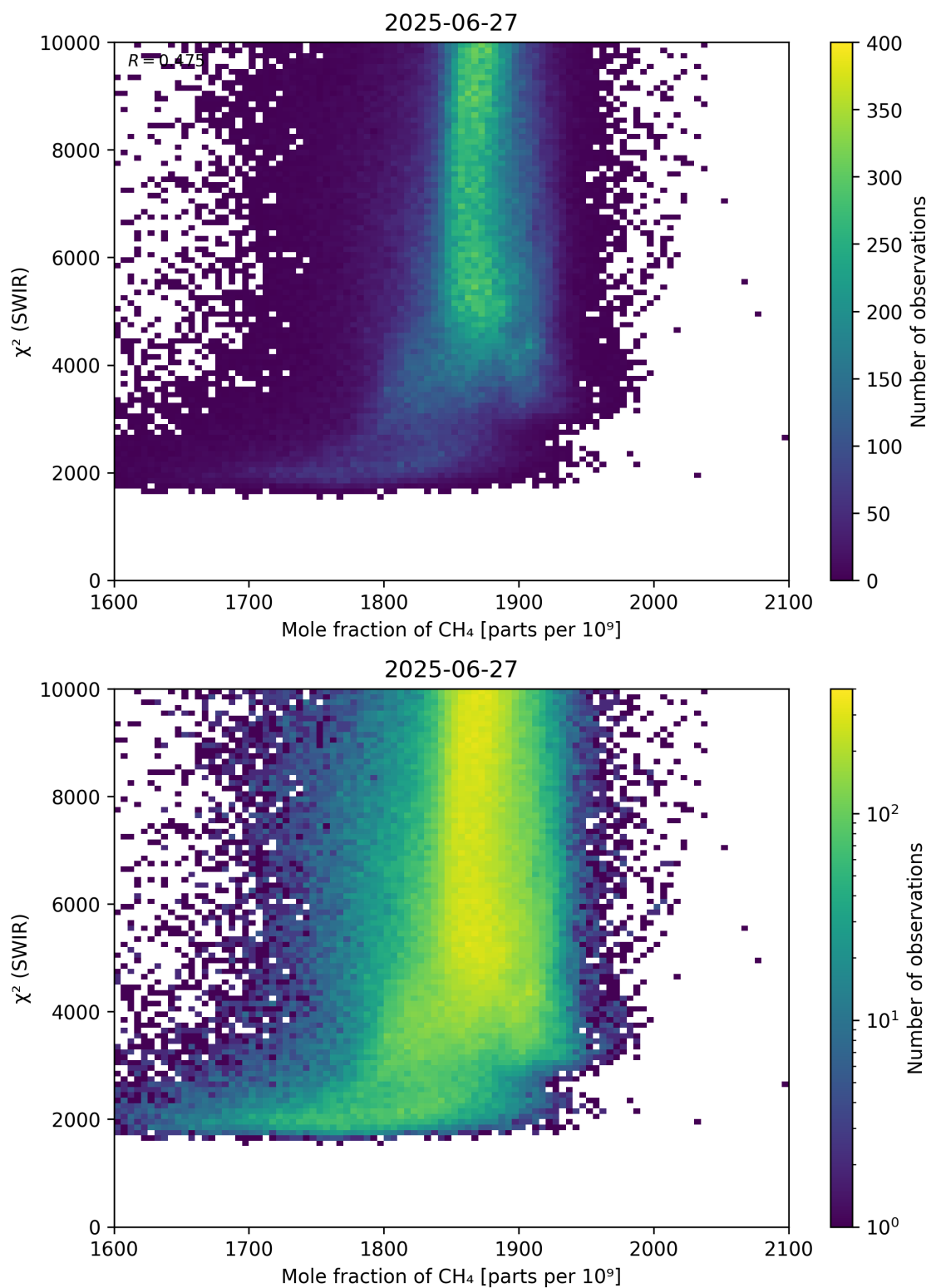
Figure 71: Scatter density plot of “Mole fraction of \text{CH}_4 ” against “ \chi^2 (SWIR)” for 2025-06-27 to 2025-06-28.
