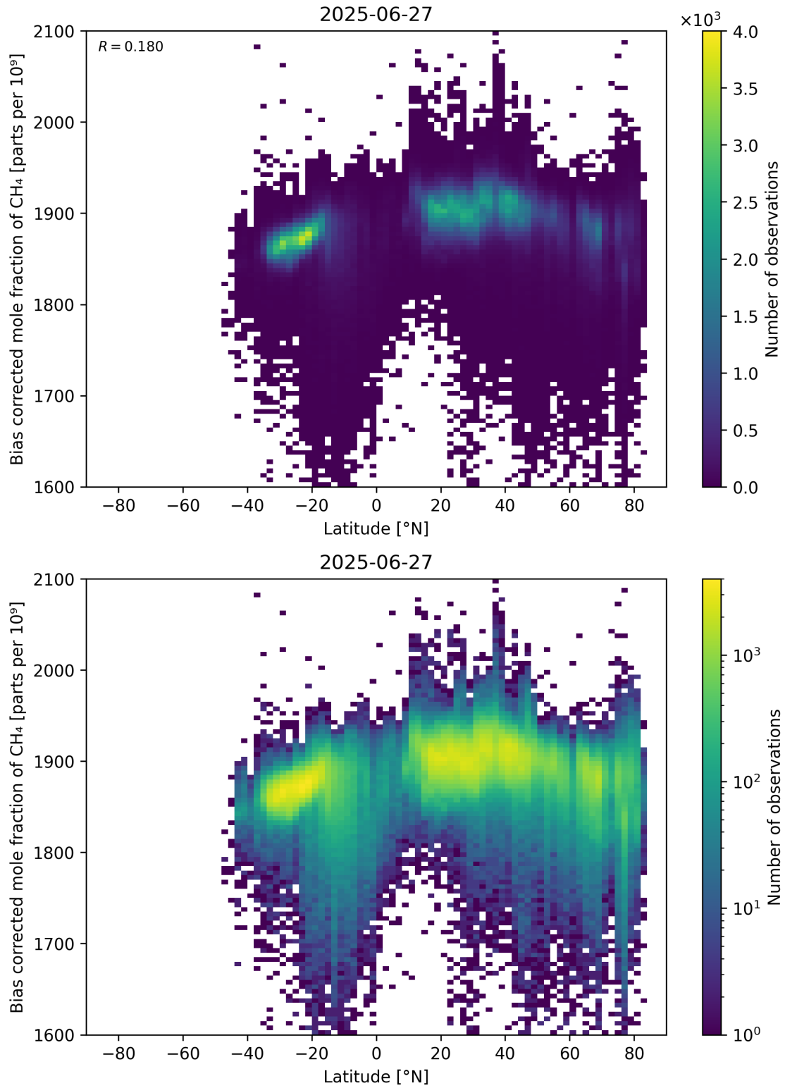
Figure 58: Scatter density plot of “Latitude” against “Bias corrected mole fraction of \text{CH}_4 ” for 2025-06-27 to 2025-06-28.
