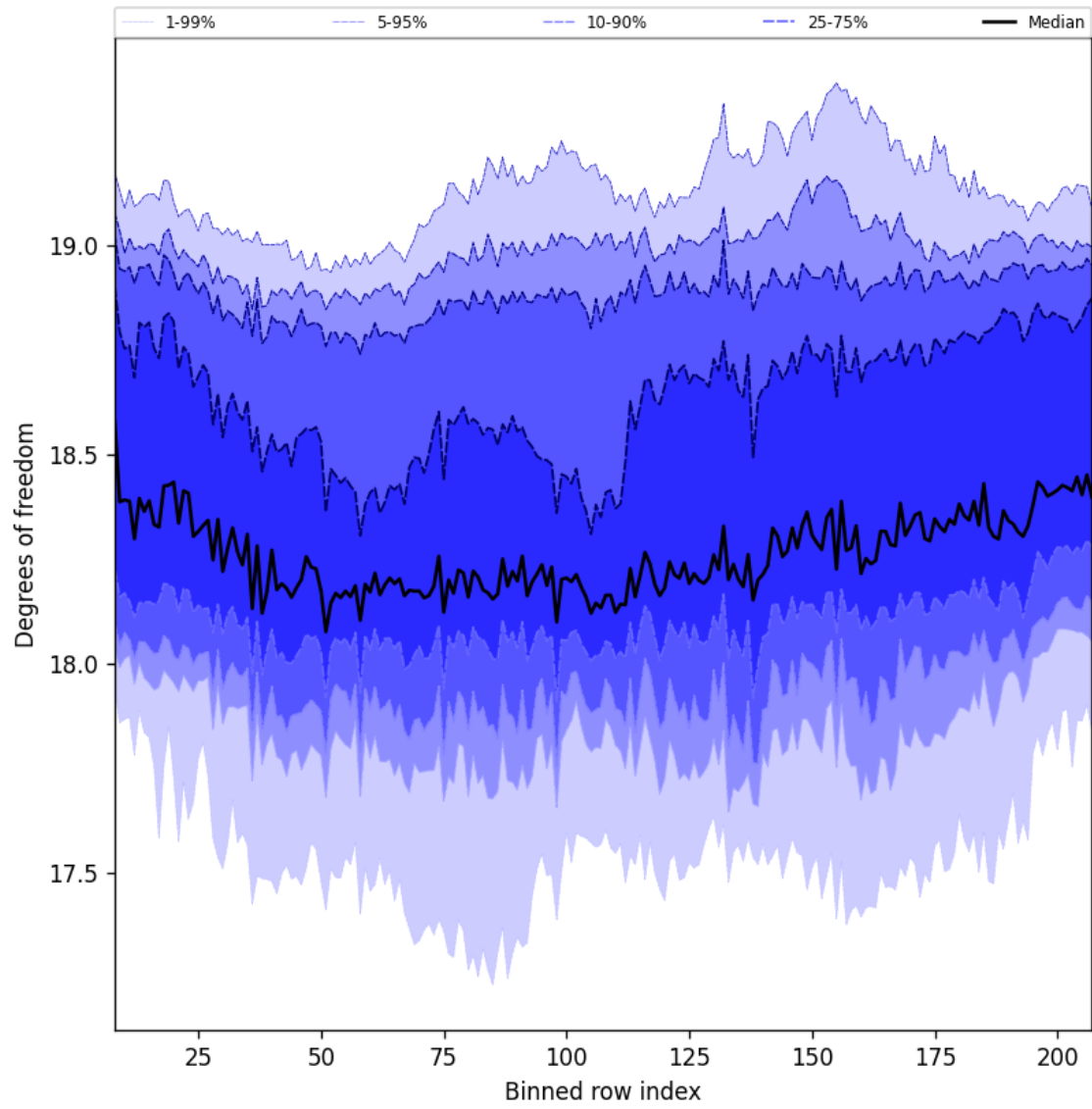
Figure 41: Along track statistics of “Degrees of freedom” for 2025-06-27 to 2025-06-28
