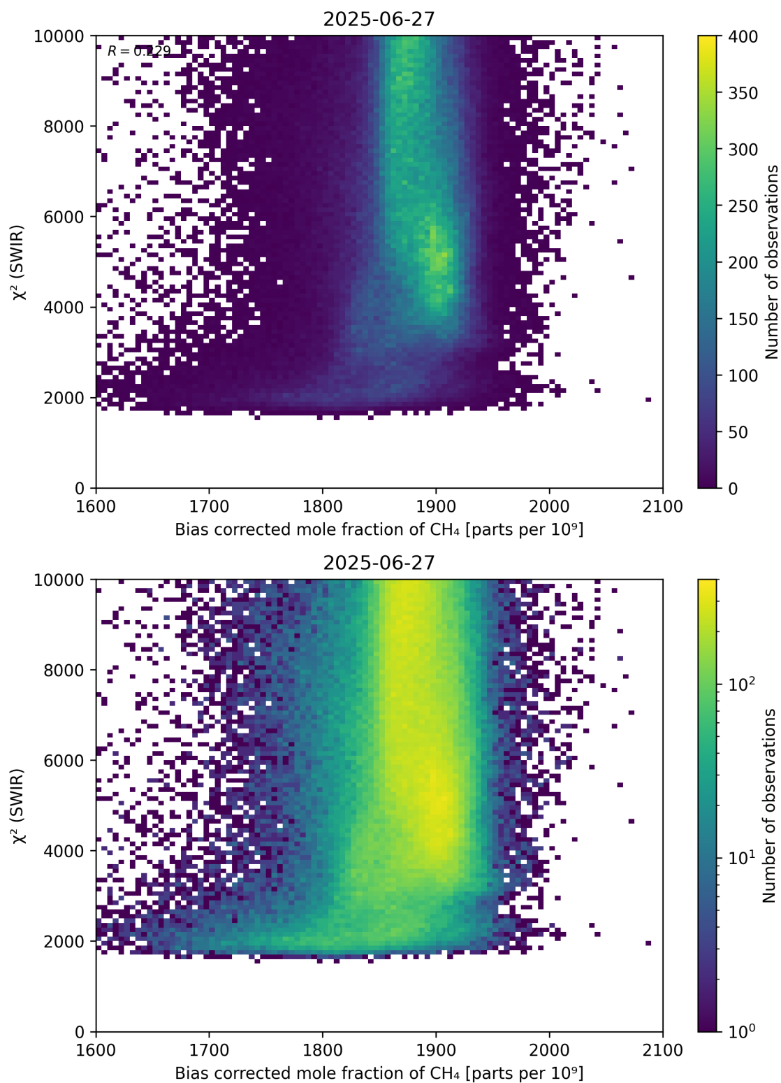
Figure 64: Scatter density plot of “Bias corrected mole fraction of \text{CH}_4 ” against “ \chi^2 (SWIR)” for 2025-06-27 to 2025-06-28.
