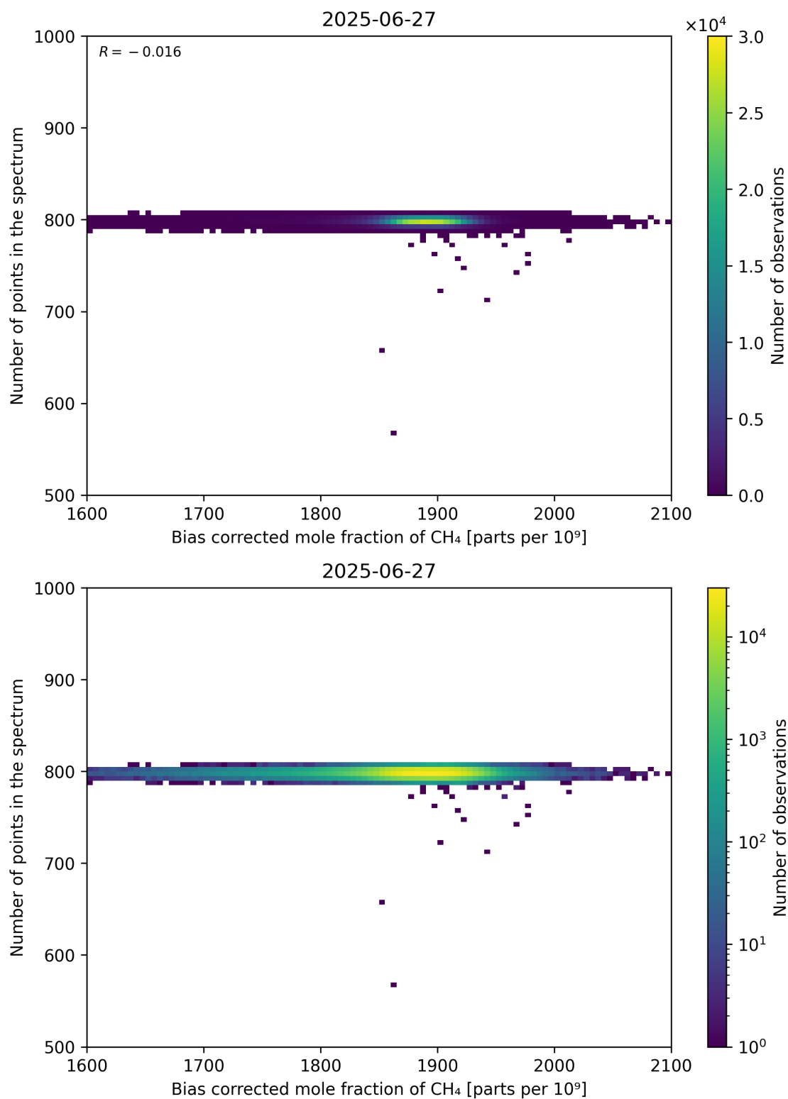
Figure 68: Scatter density plot of “Bias corrected mole fraction of CH 4 ” against “Number of points in the spectrum” for 2025-06-27 to 2025-06-28.
