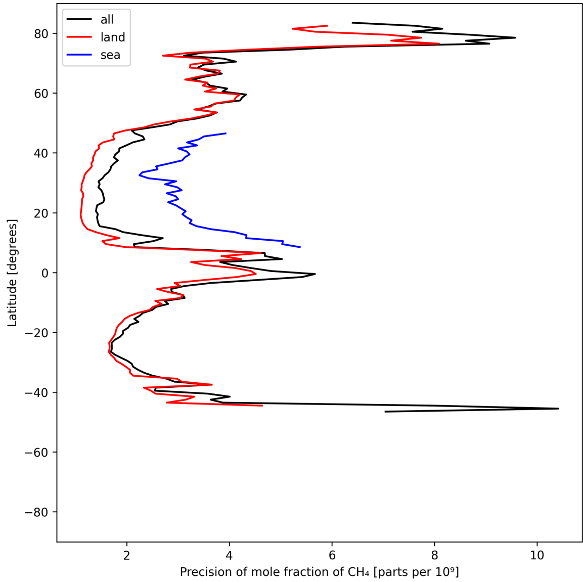
Figure 13: Zonal average of “Precision of mole fraction of \text{CH}_4 ” for 2025-06-27 to 2025-06-28.
