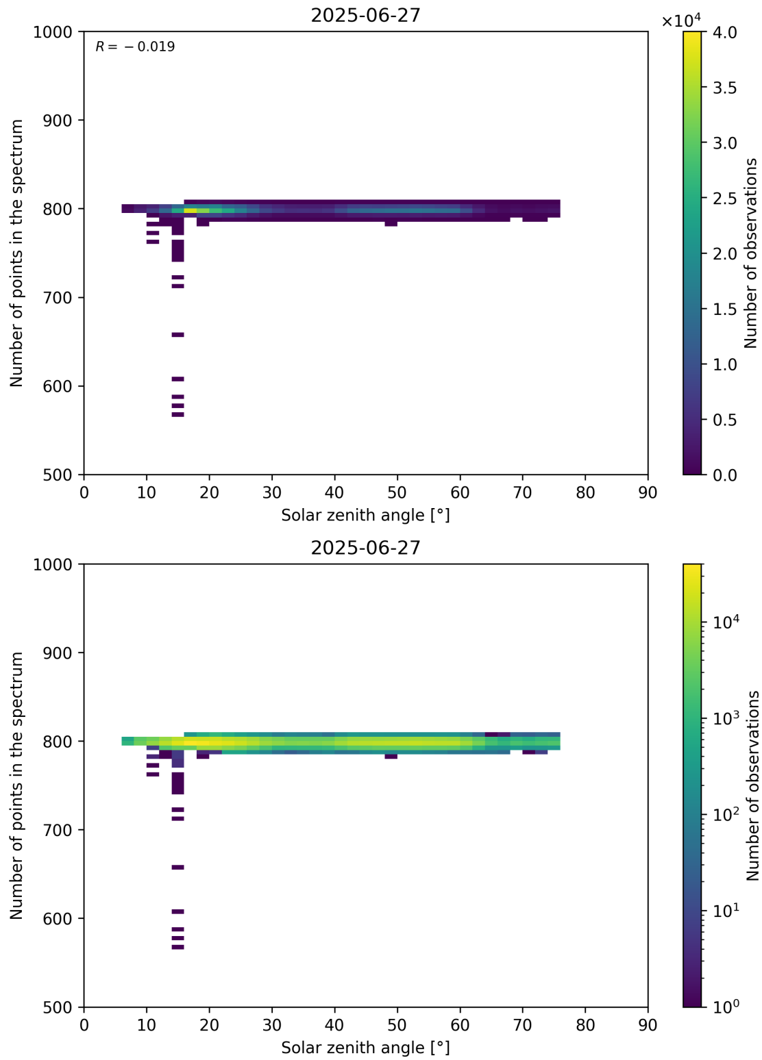
Figure 103: Scatter density plot of “Solar zenith angle” against “Number of points in the spectrum” for 2025-06-27 to 2025-06-28.
