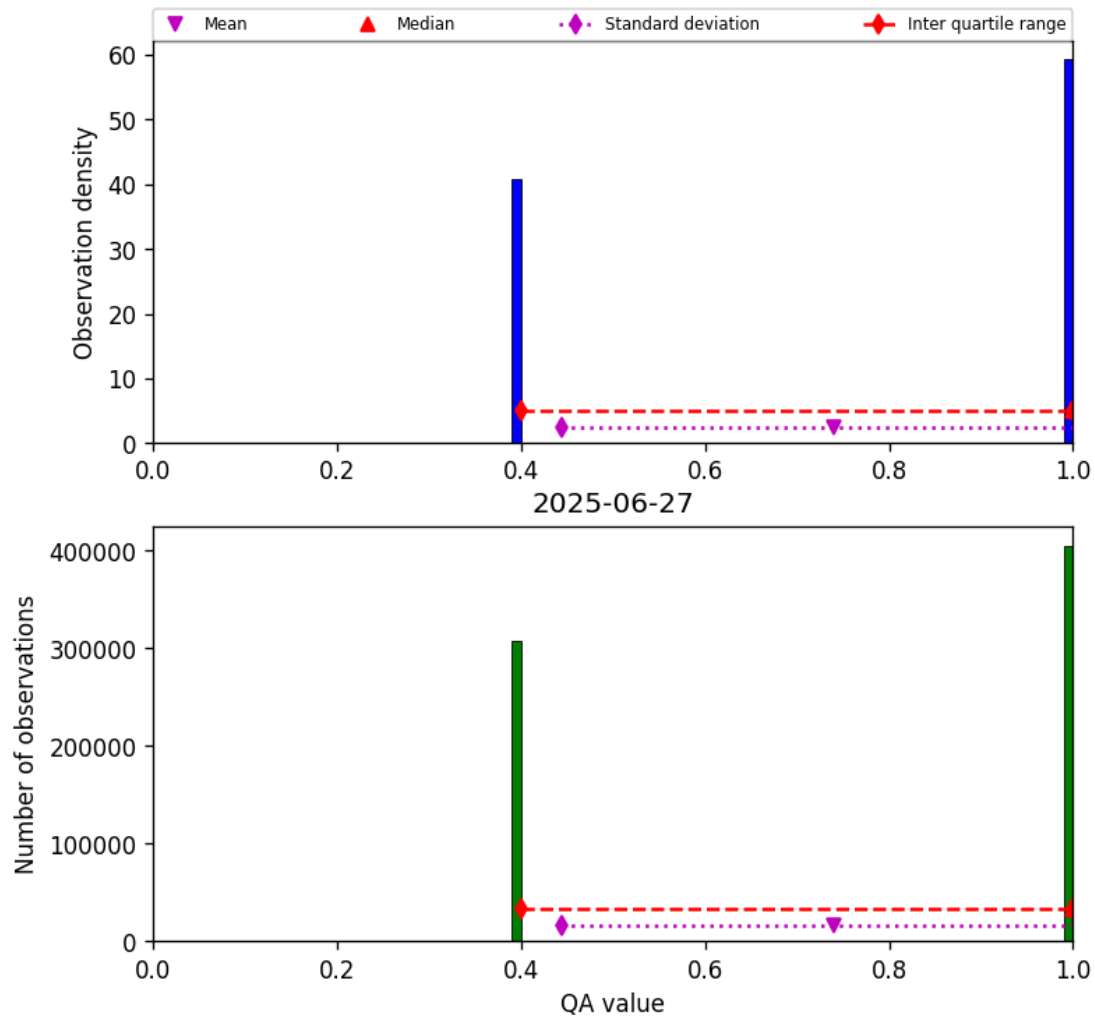
Figure 22: Histogram of “QA value” for 2025-06-27 to 2025-06-28
