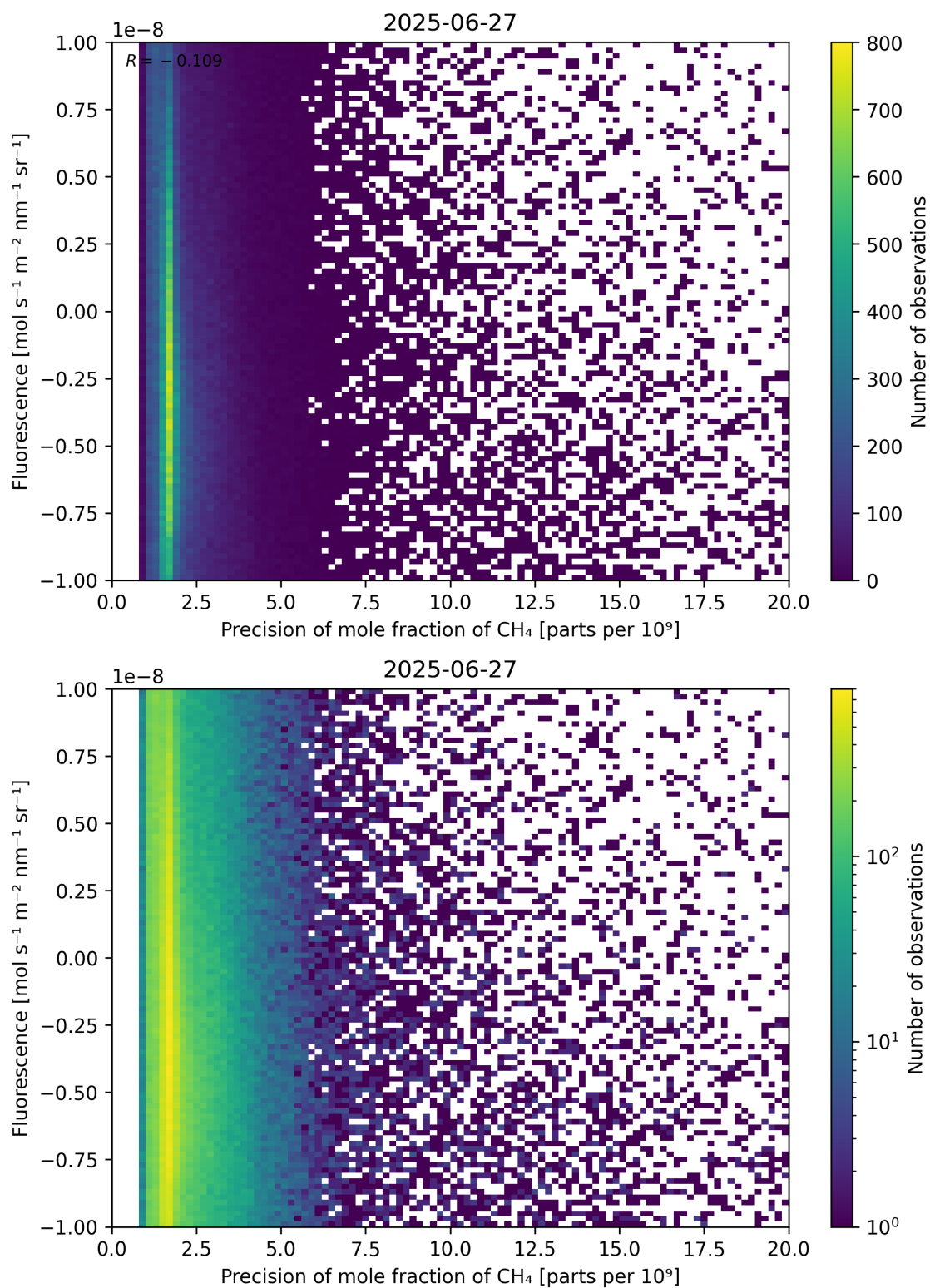
Figure 81: Scatter density plot of “Precision of mole fraction of CH 4 ” against “Fluorescence” for 2025-06-27 to 2025-06-28.
