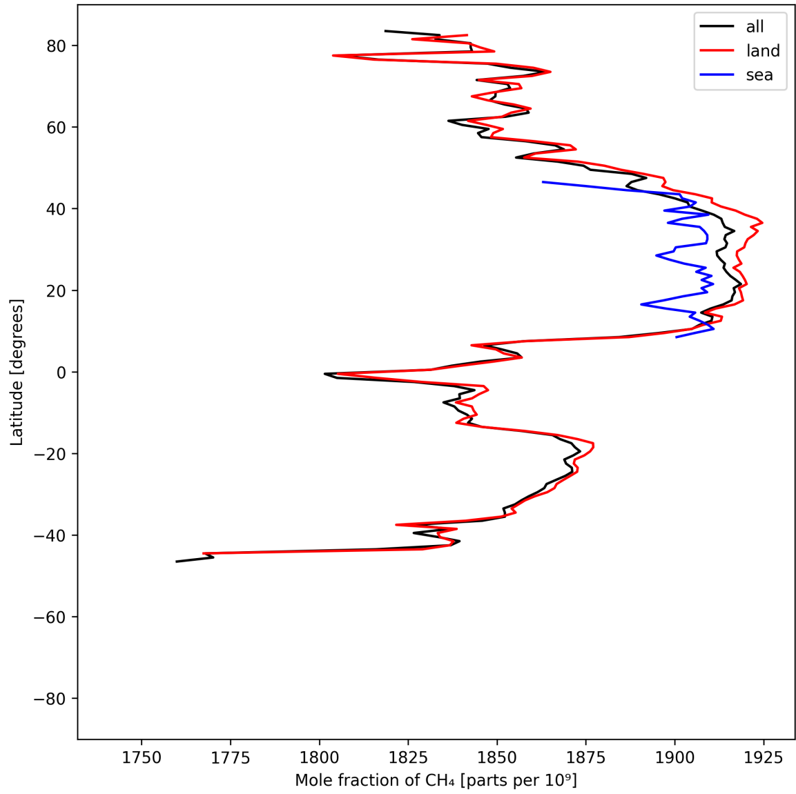
Figure 12: Zonal average of “Mole fraction of CH 4 ” for 2025-06-27 to 2025-06-28.
