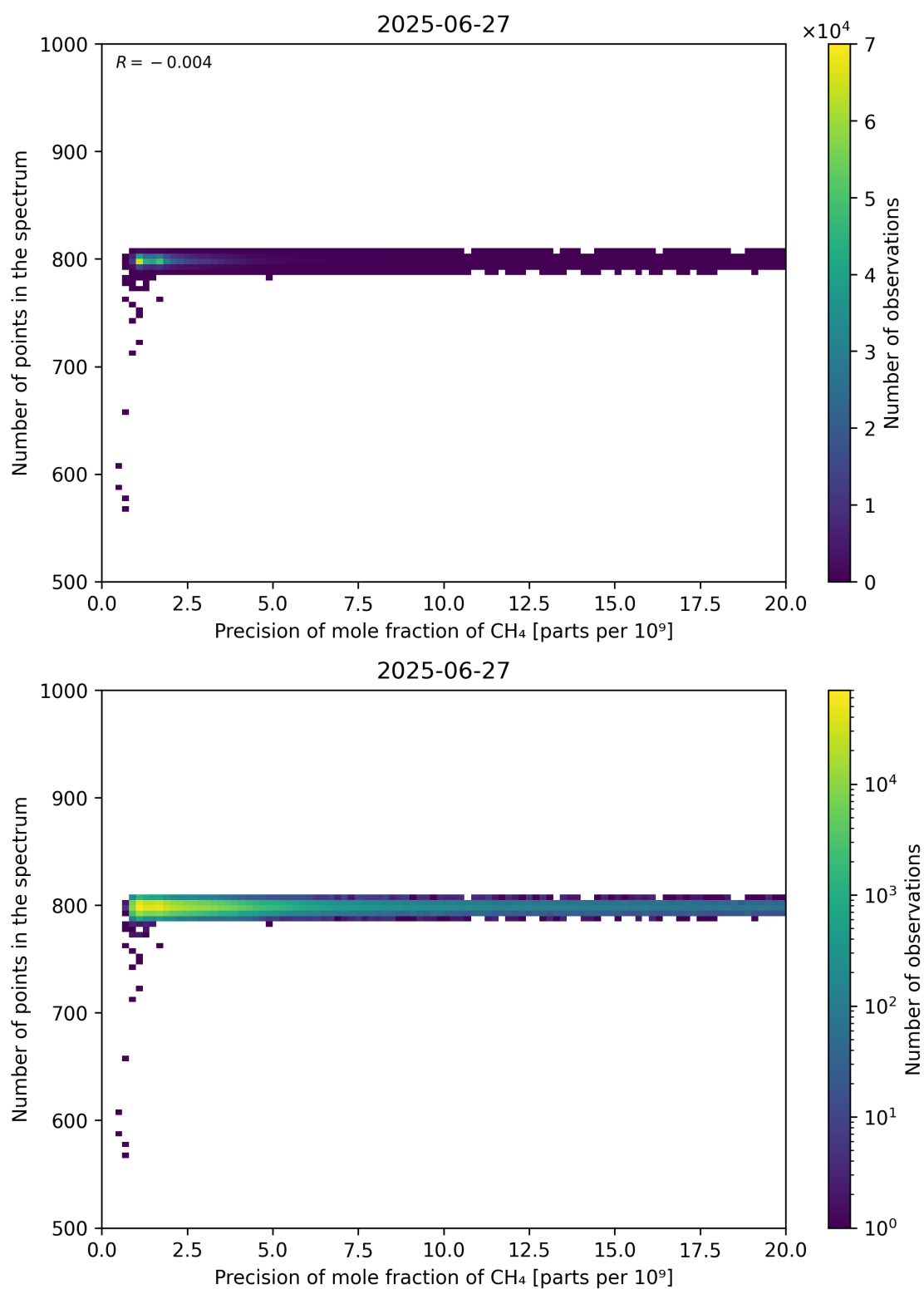
Figure 84: Scatter density plot of “Precision of mole fraction of CH 4 ” against “Number of points in the spectrum” for 2025-06-27 to 2025-06-28.
