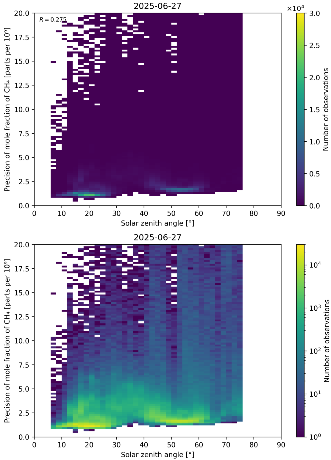
Figure 101: Scatter density plot of “Solar zenith angle” against “Precision of mole fraction of CH 4 ” for 2025-06-27 to 2025-06-28.
