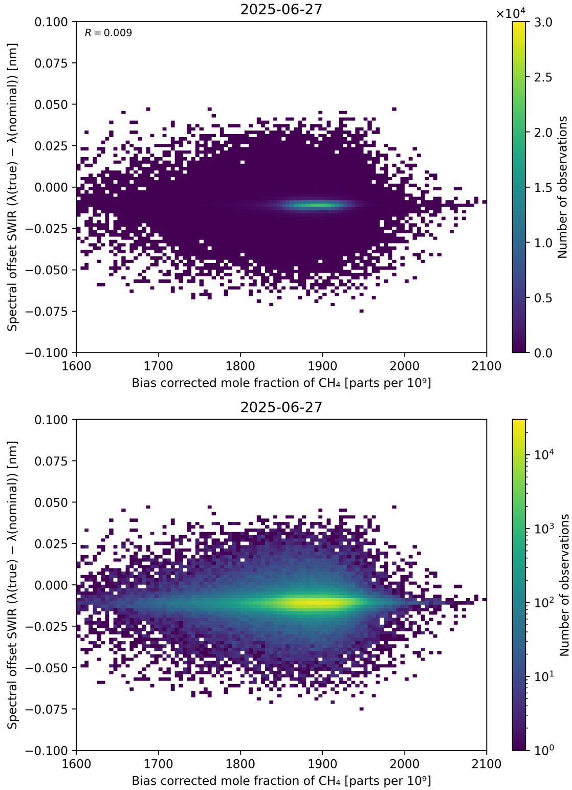
Figure 69: Scatter density plot of “Bias corrected mole fraction of \text{CH}_4 ” against “Spectral offset SWIR ( \lambda_{\text{true}} - \lambda_{\text{nominal}} )” for 2025-06-27 to 2025-06-28.
