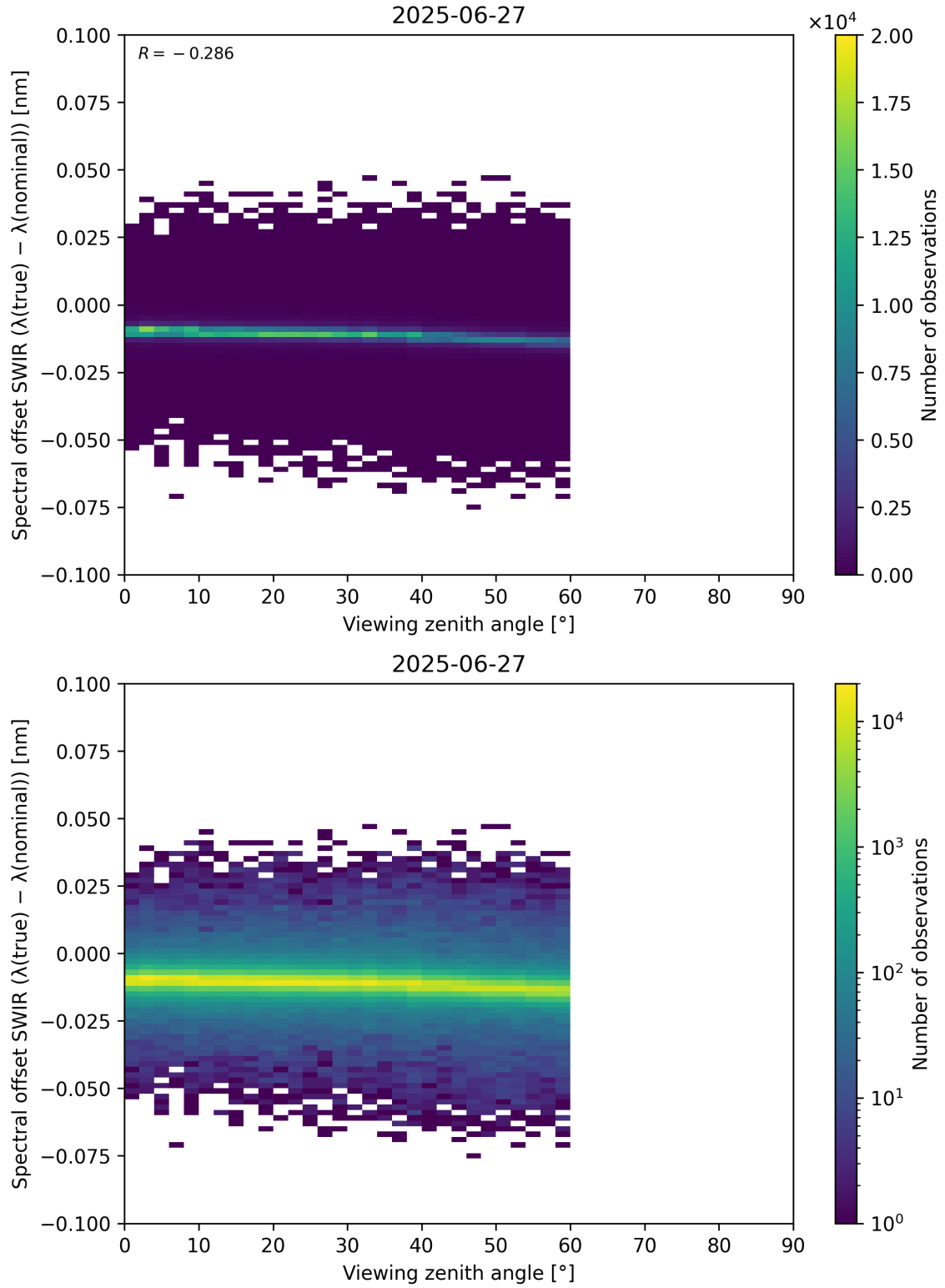
Figure 116: Scatter density plot of “Viewing zenith angle” against “Spectral offset SWIR ( \lambda_{\text{true}} - \lambda_{\text{nominal}} )” for 2025-06-27 to 2025-06-28.
