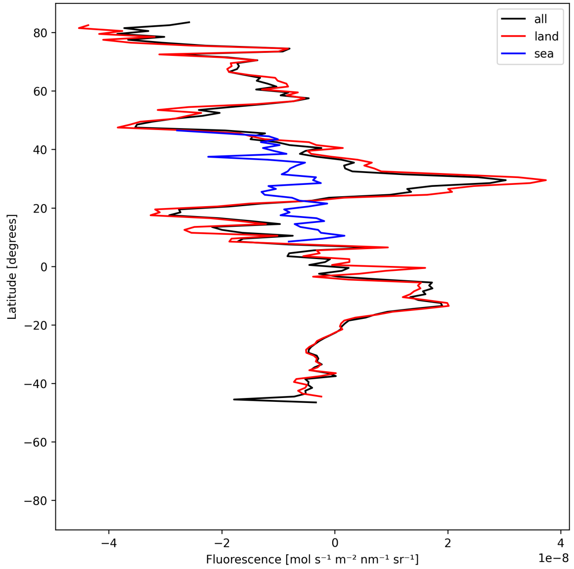
Figure 21: Zonal average of “Fluorescence” for 2025-06-27 to 2025-06-28.
