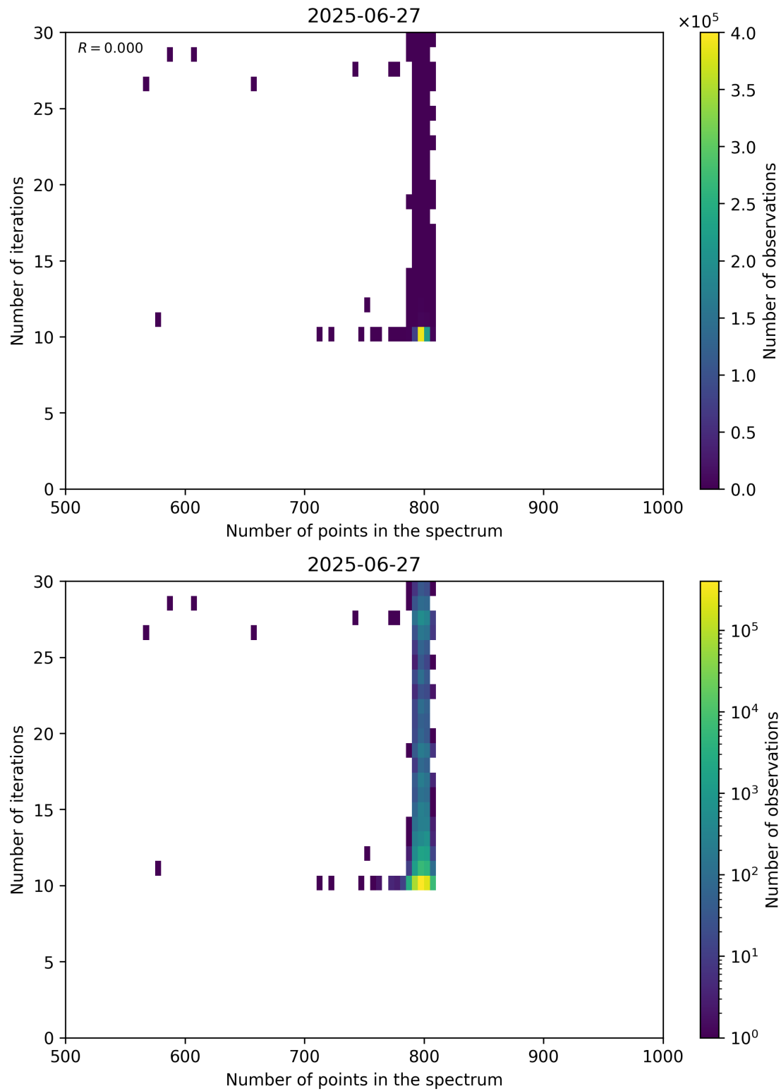
Figure 92: Scatter density plot of “Number of points in the spectrum” against “Number of iterations” for 2025-06-27 to 2025-06-28.
