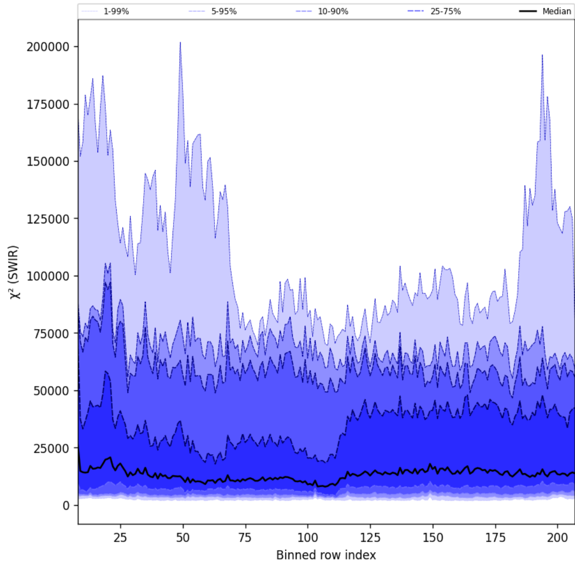
Figure 39: Along track statistics of “ \chi^2 (SWIR)” for 2025-06-27 to 2025-06-28
