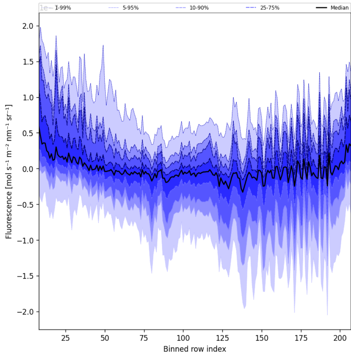
Figure 43: Along track statistics of “Fluorescence” for 2025-06-27 to 2025-06-28
