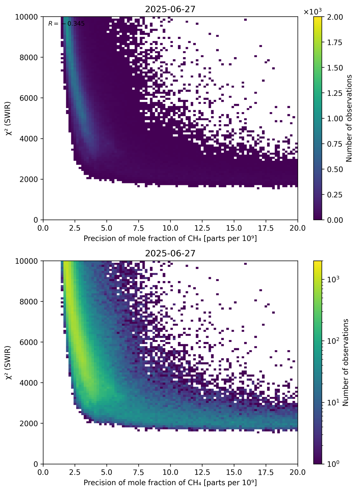
Figure 79: Scatter density plot of “Precision of mole fraction of \text{CH}_4 ” against “ \chi^2 (SWIR)” for 2025-06-27 to 2025-06-28.
