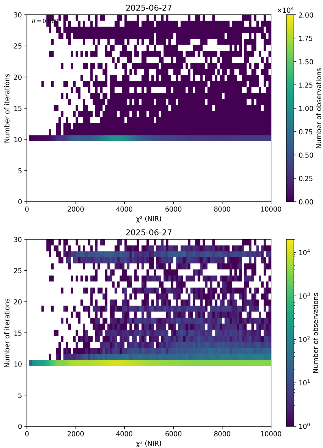
Figure 46: Scatter density plot of “ \chi^2 (NIR)” against “Number of iterations” for 2025-06-27 to 2025-06-28.
