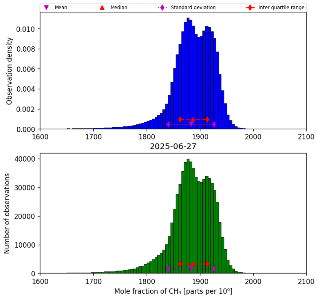
Figure 23: Histogram of “Mole fraction of CH 4 ” for 2025-06-27 to 2025-06-28
