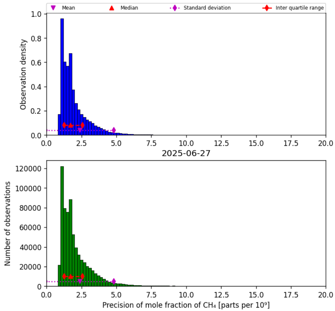
Figure 24: Histogram of “Precision of mole fraction of CH 4 ” for 2025-06-27 to 2025-06-28
