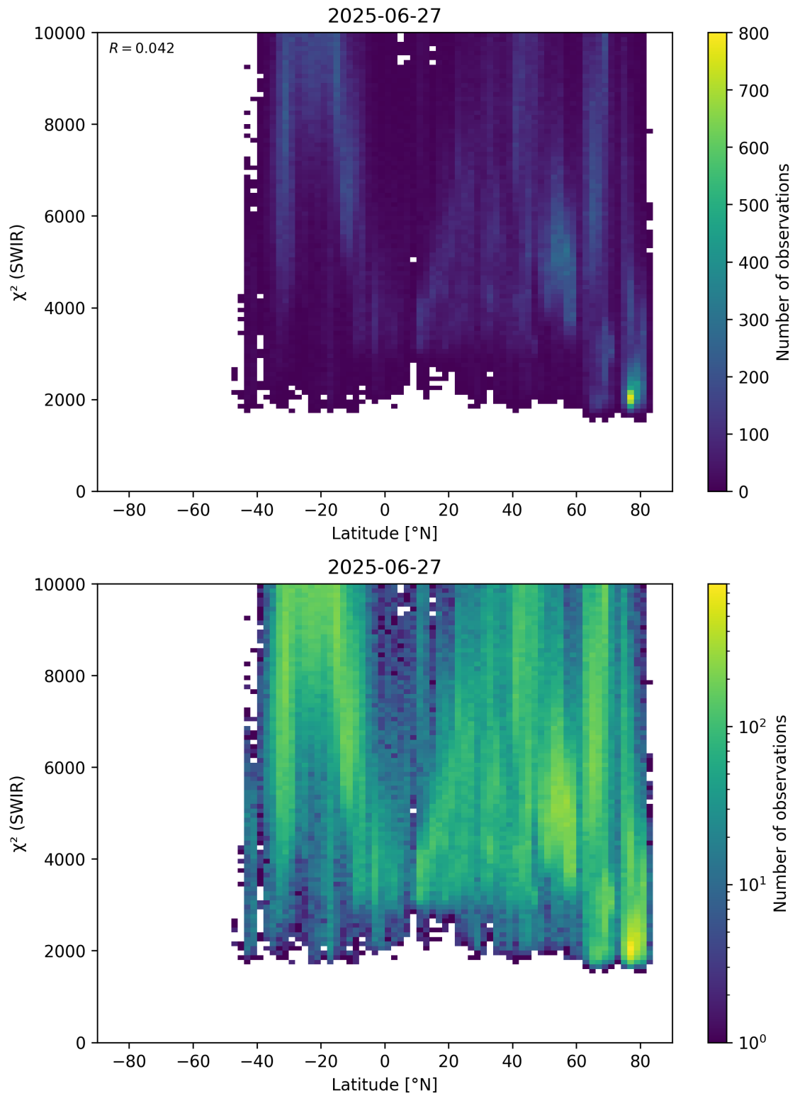
Figure 54: Scatter density plot of “Latitude” against “ \chi^2 (SWIR)” for 2025-06-27 to 2025-06-28.
