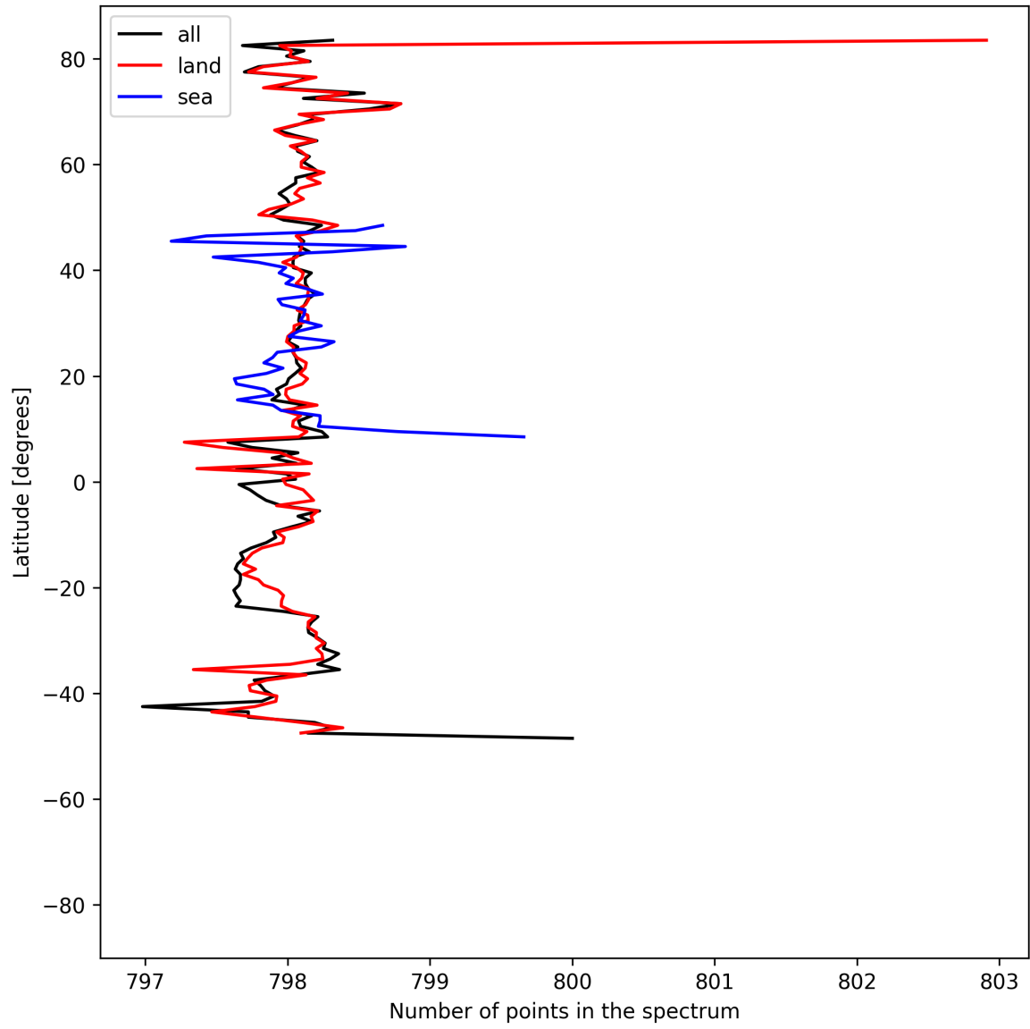
Figure 15: Zonal average of “Number of points in the spectrum” for 2025-06-27 to 2025-06-29.
