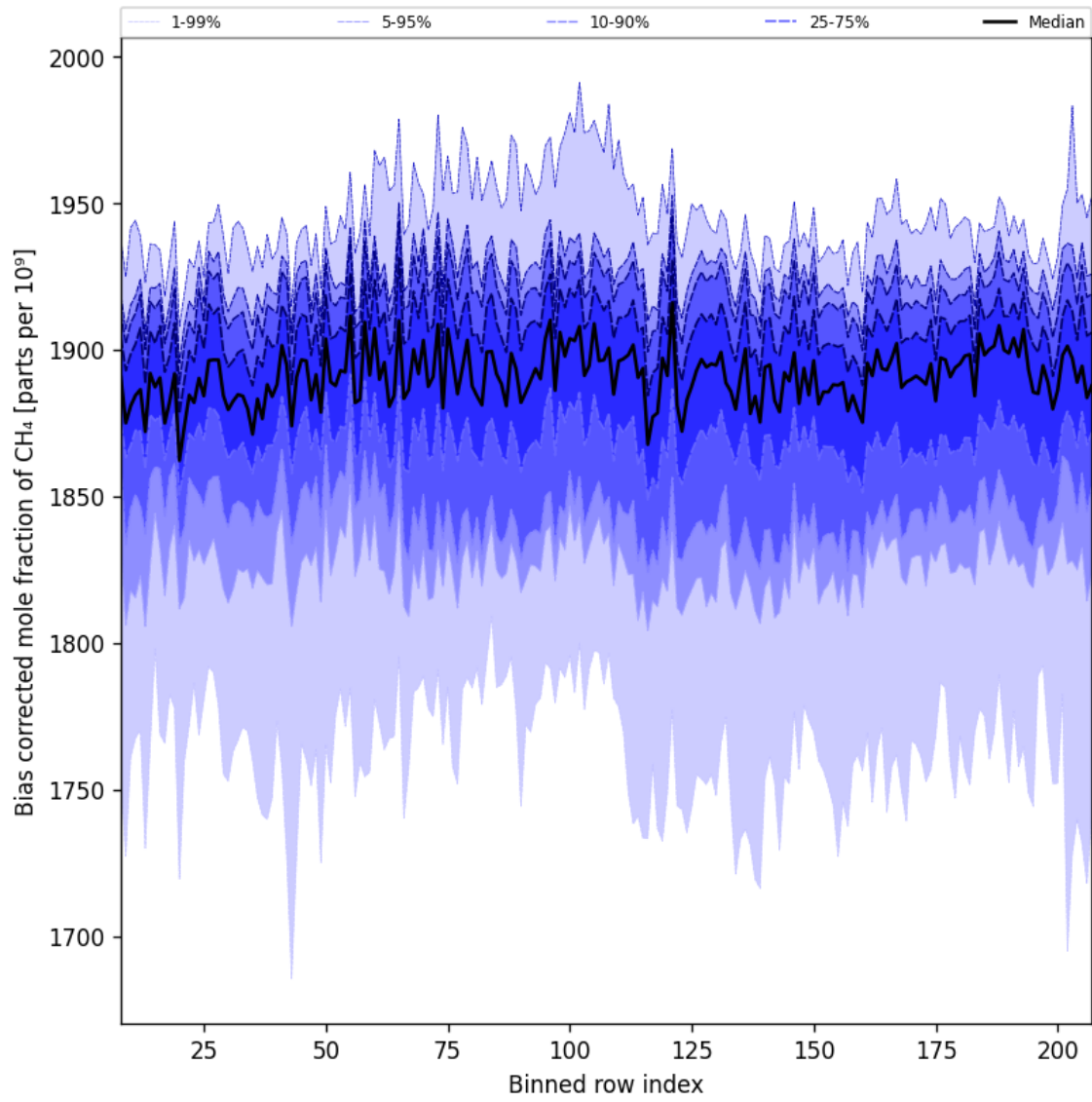
Figure 36: Along track statistics of “Bias corrected mole fraction of CH 4 ” for 2025-06-27 to 2025-06-29
