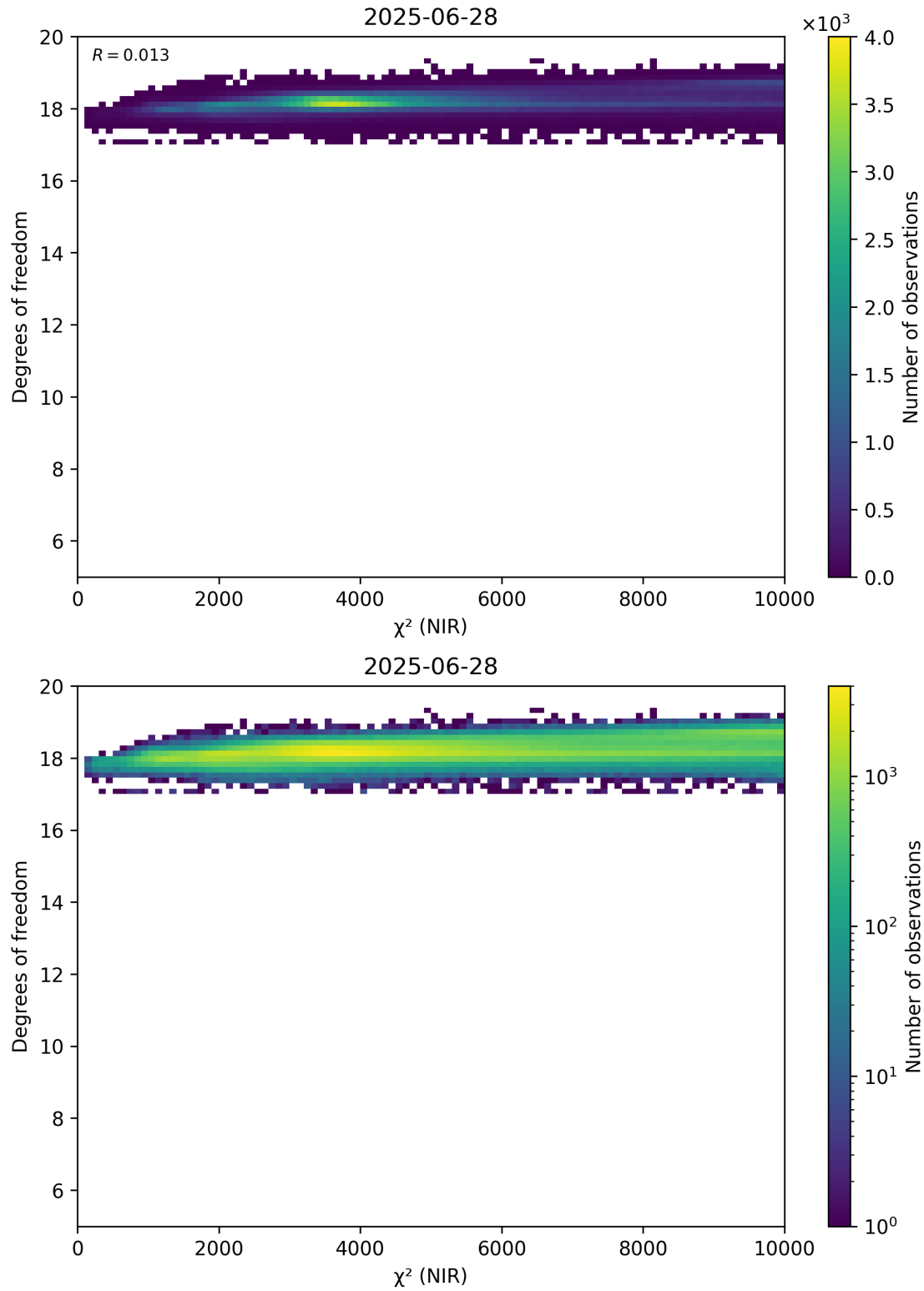
Figure 44: Scatter density plot of “ \chi^2 (NIR)” against “Degrees of freedom” for 2025-06-27 to 2025-06-29.
