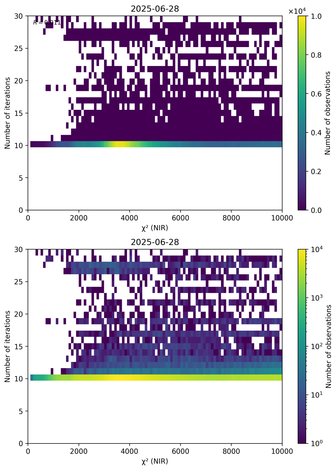
Figure 46: Scatter density plot of “ \chi^2 (NIR)” against “Number of iterations” for 2025-06-27 to 2025-06-29.
