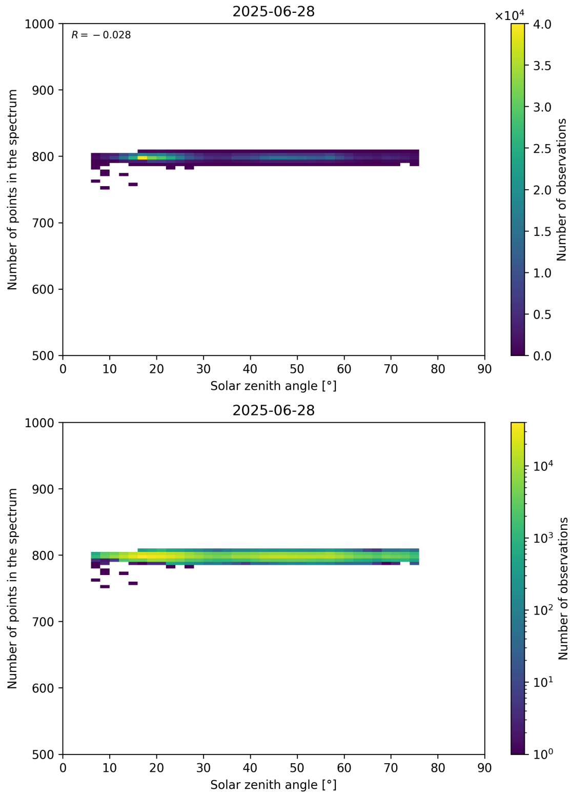
Figure 103: Scatter density plot of “Solar zenith angle” against “Number of points in the spectrum” for 2025-06-27 to 2025-06-29.
