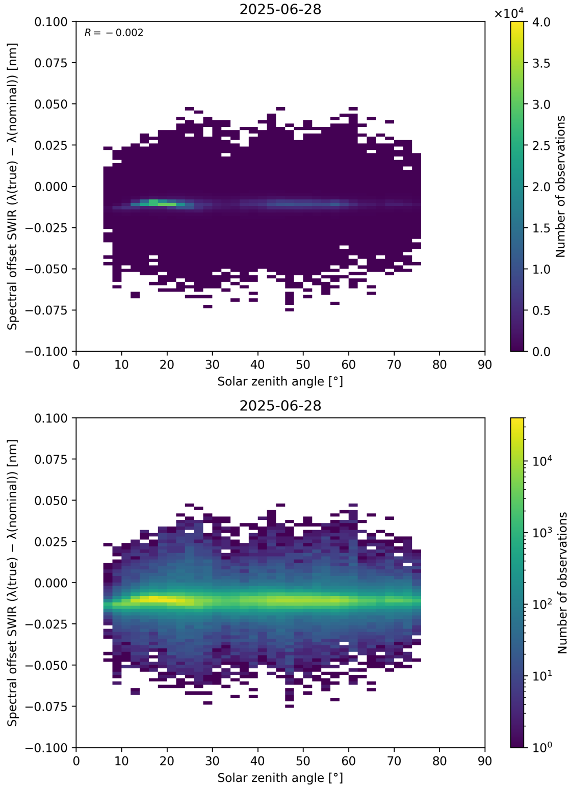
Figure 104: Scatter density plot of “Solar zenith angle” against “Spectral offset SWIR ( \lambda_{\text{true}} - \lambda_{\text{nominal}} )” for 2025-06-27 to 2025-06-29.
