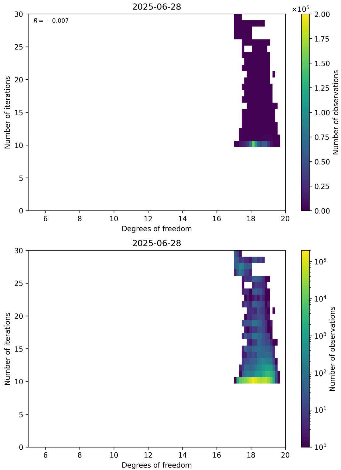
Figure 52: Scatter density plot of “Degrees of freedom” against “Number of iterations” for 2025-06-27 to 2025-06-29.
