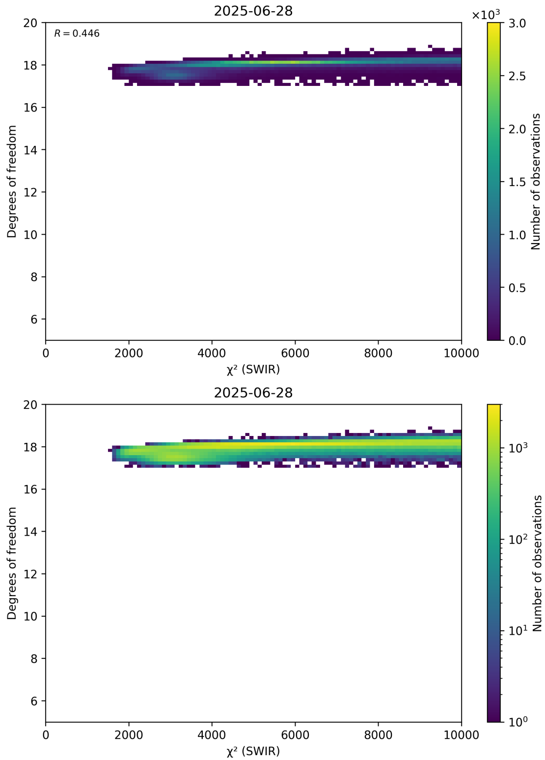
Figure 48: Scatter density plot of “ \chi^2 (SWIR)” against “Degrees of freedom” for 2025-06-27 to 2025-06-29.
