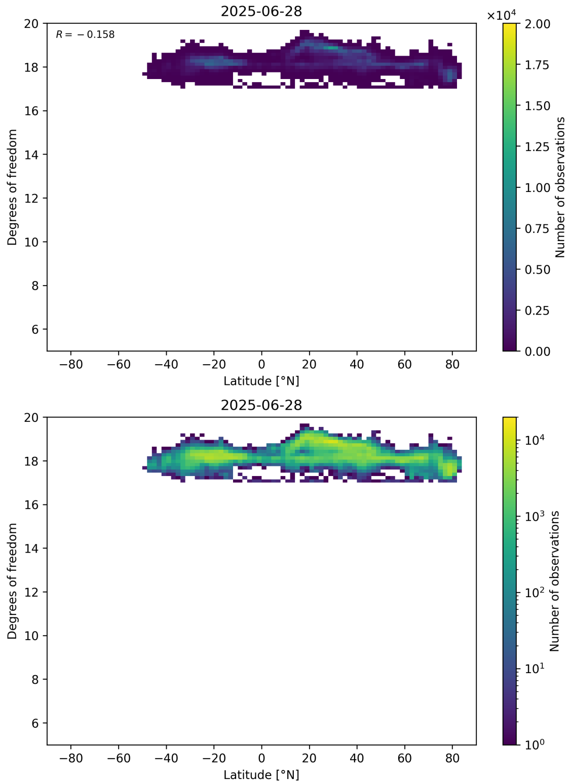
Figure 55: Scatter density plot of “Latitude” against “Degrees of freedom” for 2025-06-27 to 2025-06-29.
