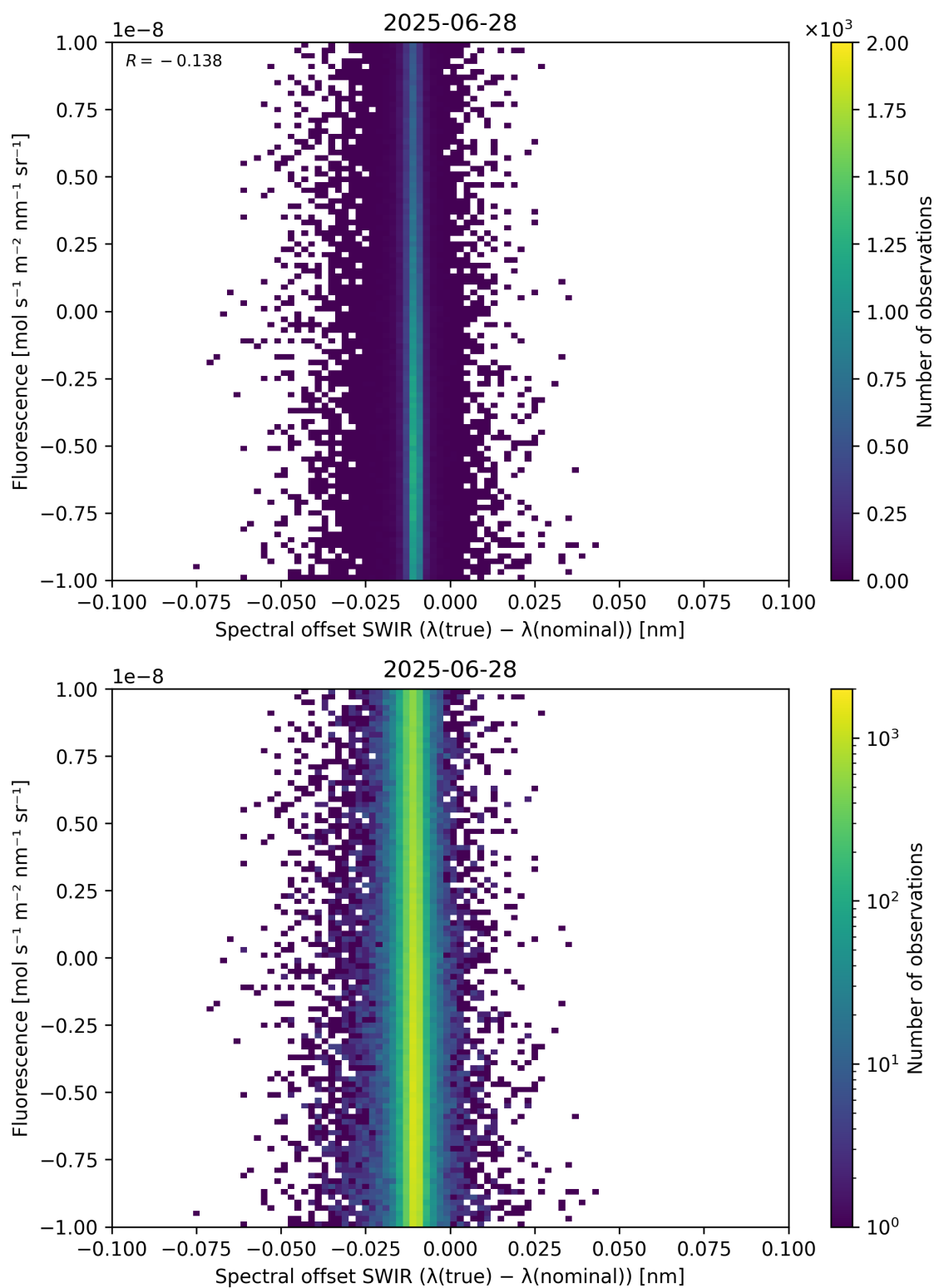
Figure 120: Scatter density plot of “Spectral offset SWIR ( \lambda_{\text{true}} - \lambda_{\text{nominal}} )” against “Fluorescence” for 2025-06-27 to 2025-06-29.
