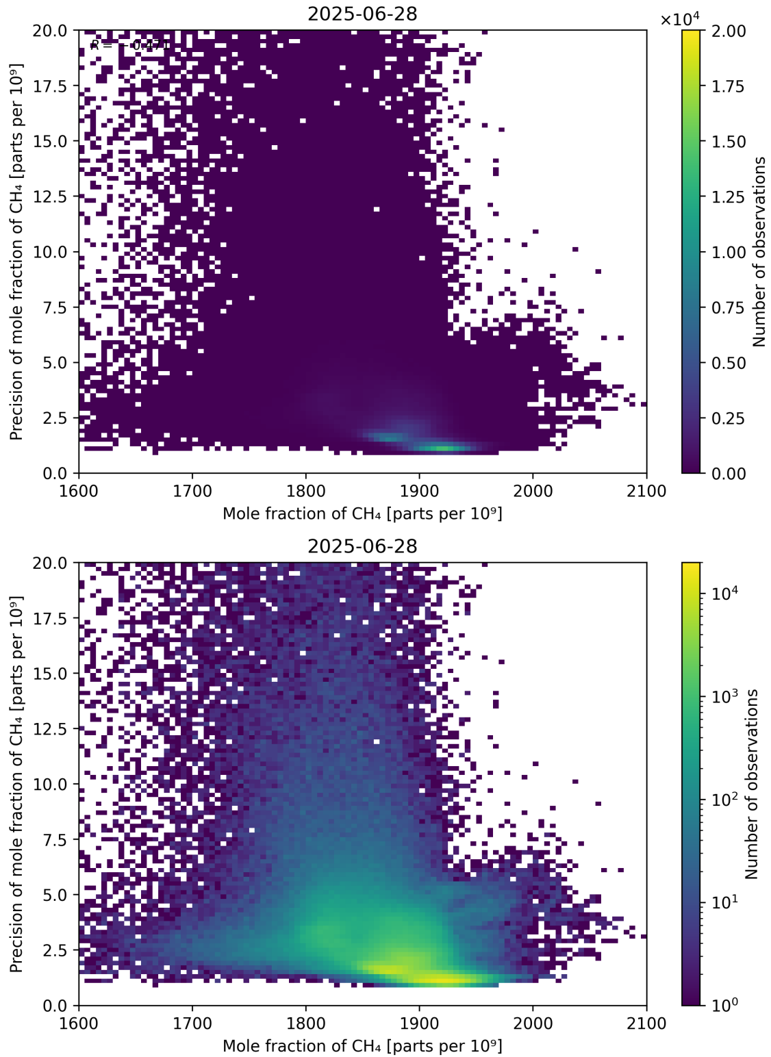
Figure 75: Scatter density plot of “Mole fraction of CH 4 ” against “Precision of mole fraction of CH 4 ” for 2025-06-27 to 2025-06-29.
