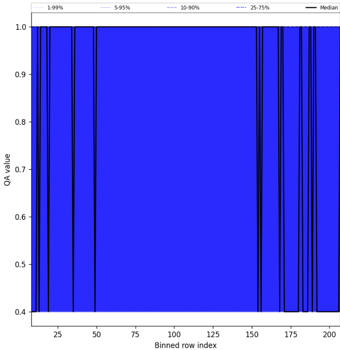
Figure 33: Along track statistics of “QA value” for 2025-06-27 to 2025-06-29
