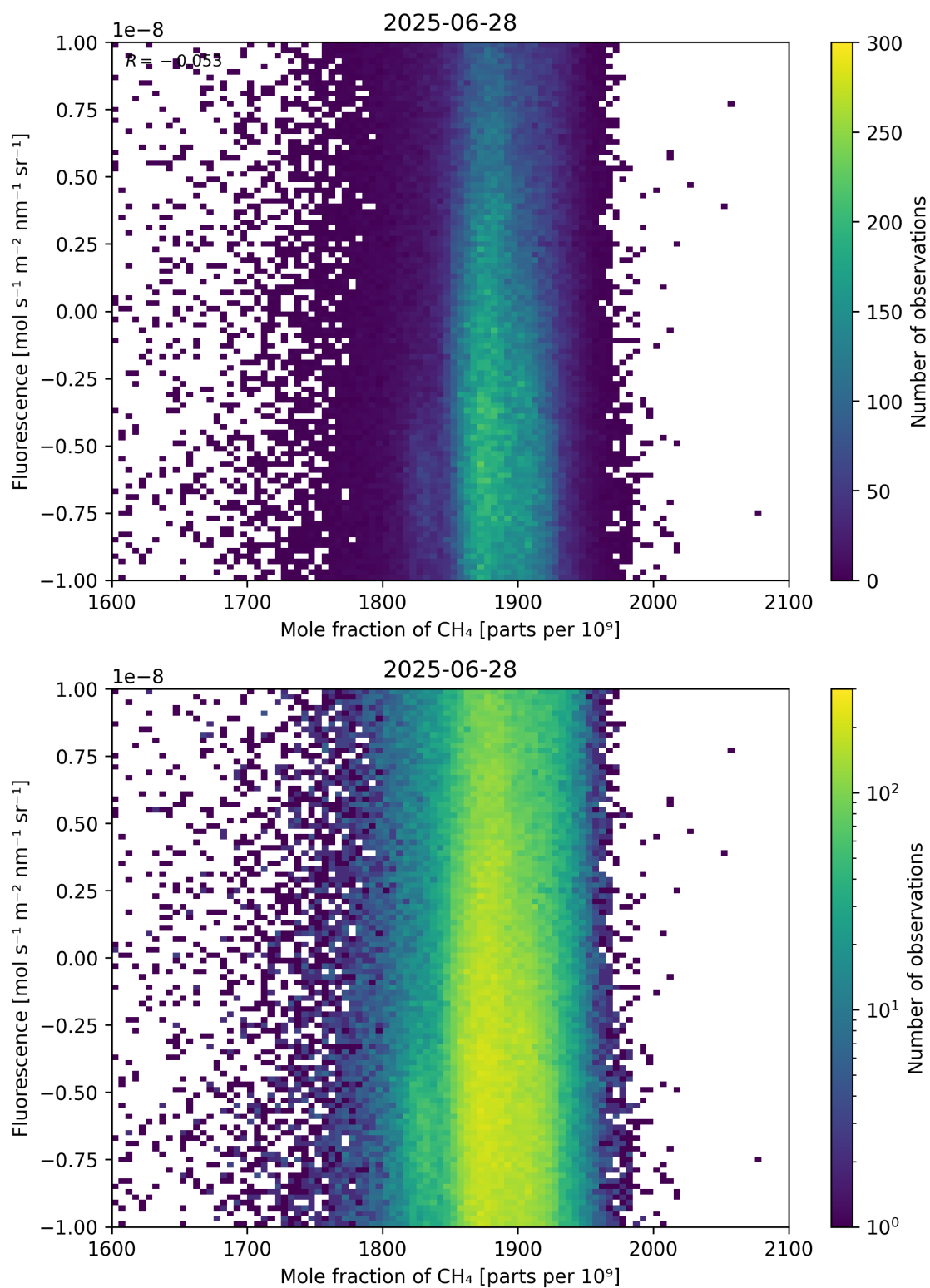
Figure 73: Scatter density plot of “Mole fraction of \text{CH}_4 ” against “Fluorescence” for 2025-06-27 to 2025-06-29.
