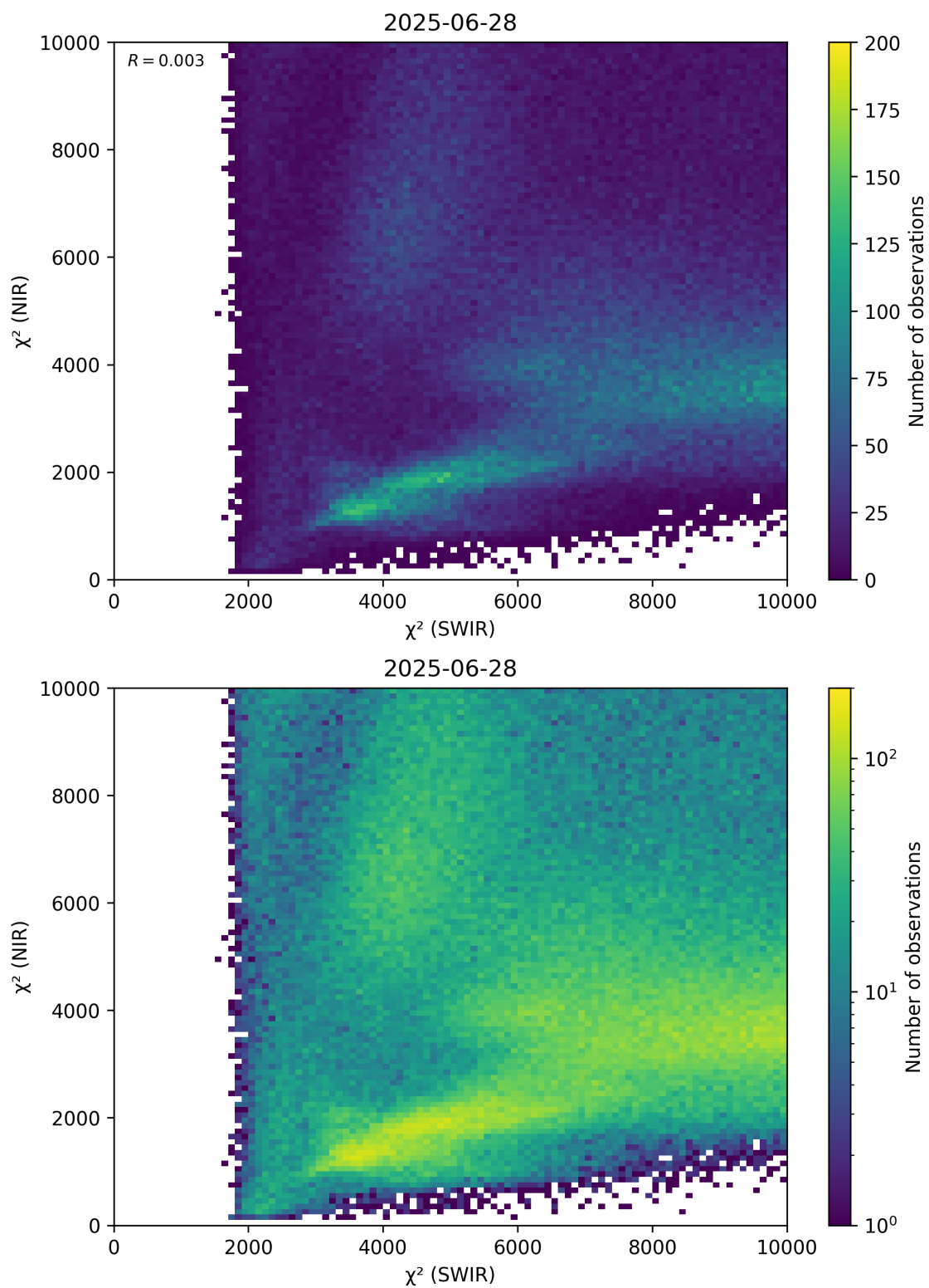
Figure 47: Scatter density plot of “ \chi^2 (SWIR)” against “ \chi^2 (NIR)” for 2025-06-27 to 2025-06-29.
