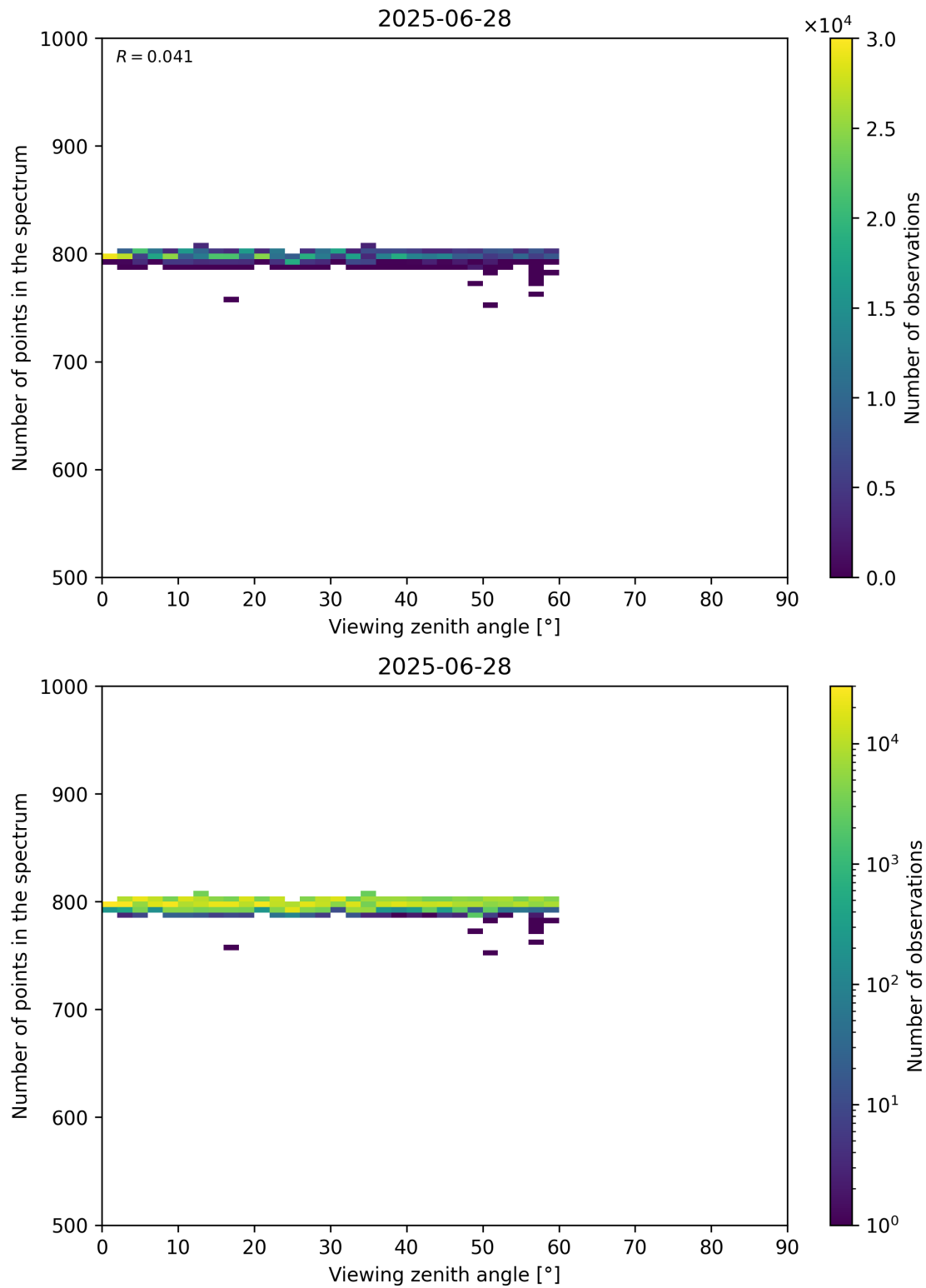
Figure 114: Scatter density plot of “Viewing zenith angle” against “Number of points in the spectrum” for 2025-06-27 to 2025-06-29.
