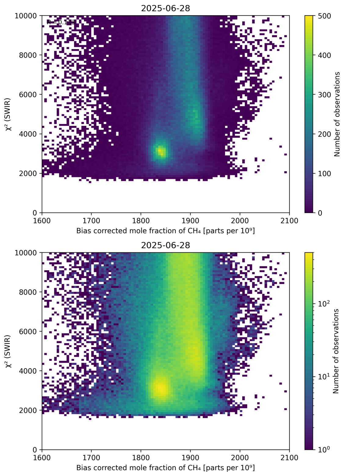
Figure 64: Scatter density plot of “Bias corrected mole fraction of CH 4 ” against “ \chi^2 (SWIR)” for 2025-06-27 to 2025-06-29.
