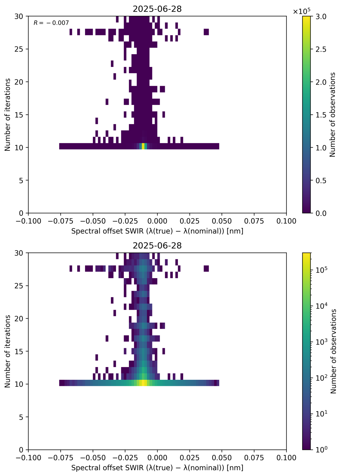
Figure 121: Scatter density plot of “Spectral offset SWIR ( \lambda_{\text{true}} - \lambda_{\text{nominal}} )” against “Number of iterations” for 2025-06-27 to 2025-06-29.
