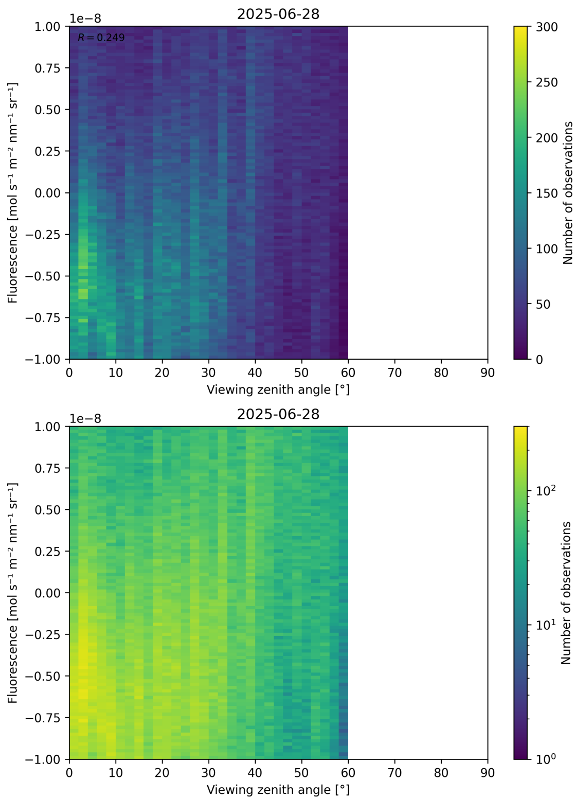
Figure 108: Scatter density plot of “Viewing zenith angle” against “Fluorescence” for 2025-06-27 to 2025-06-29.
