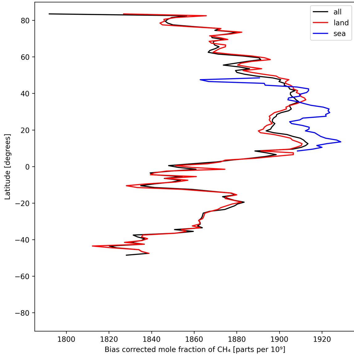
Figure 14: Zonal average of “Bias corrected mole fraction of CH 4 ” for 2025-06-27 to 2025-06-29.
