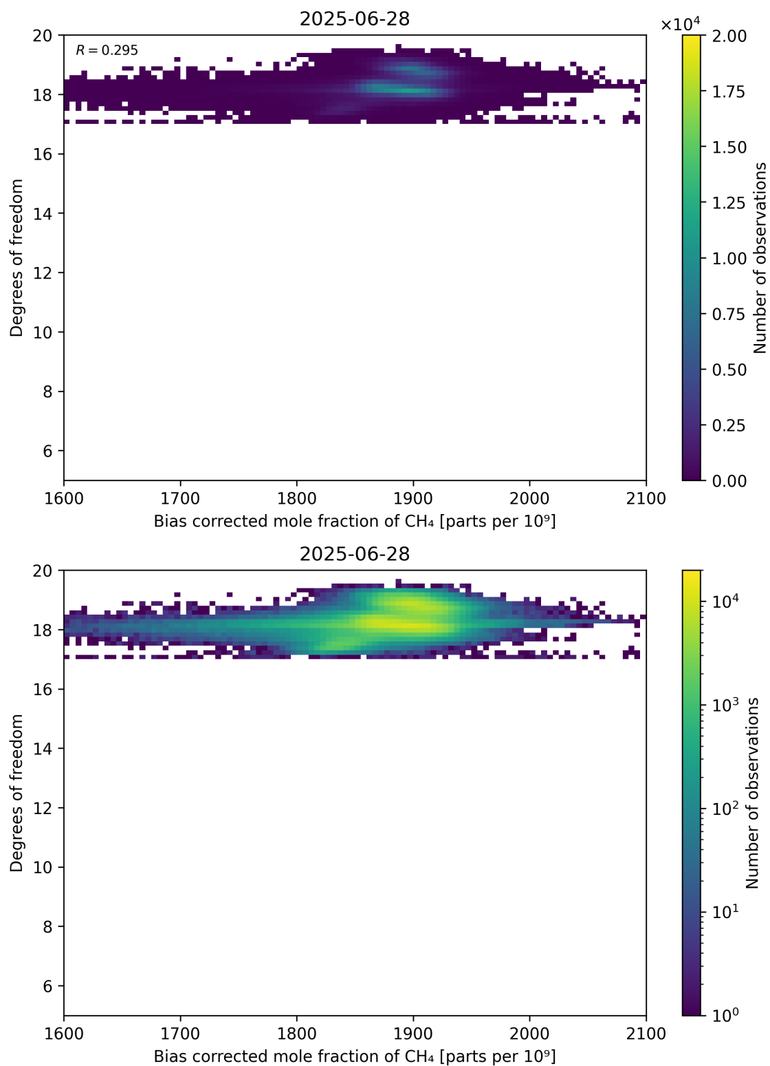
Figure 65: Scatter density plot of “Bias corrected mole fraction of CH 4 ” against “Degrees of freedom” for 2025-06-27 to 2025-06-29.
