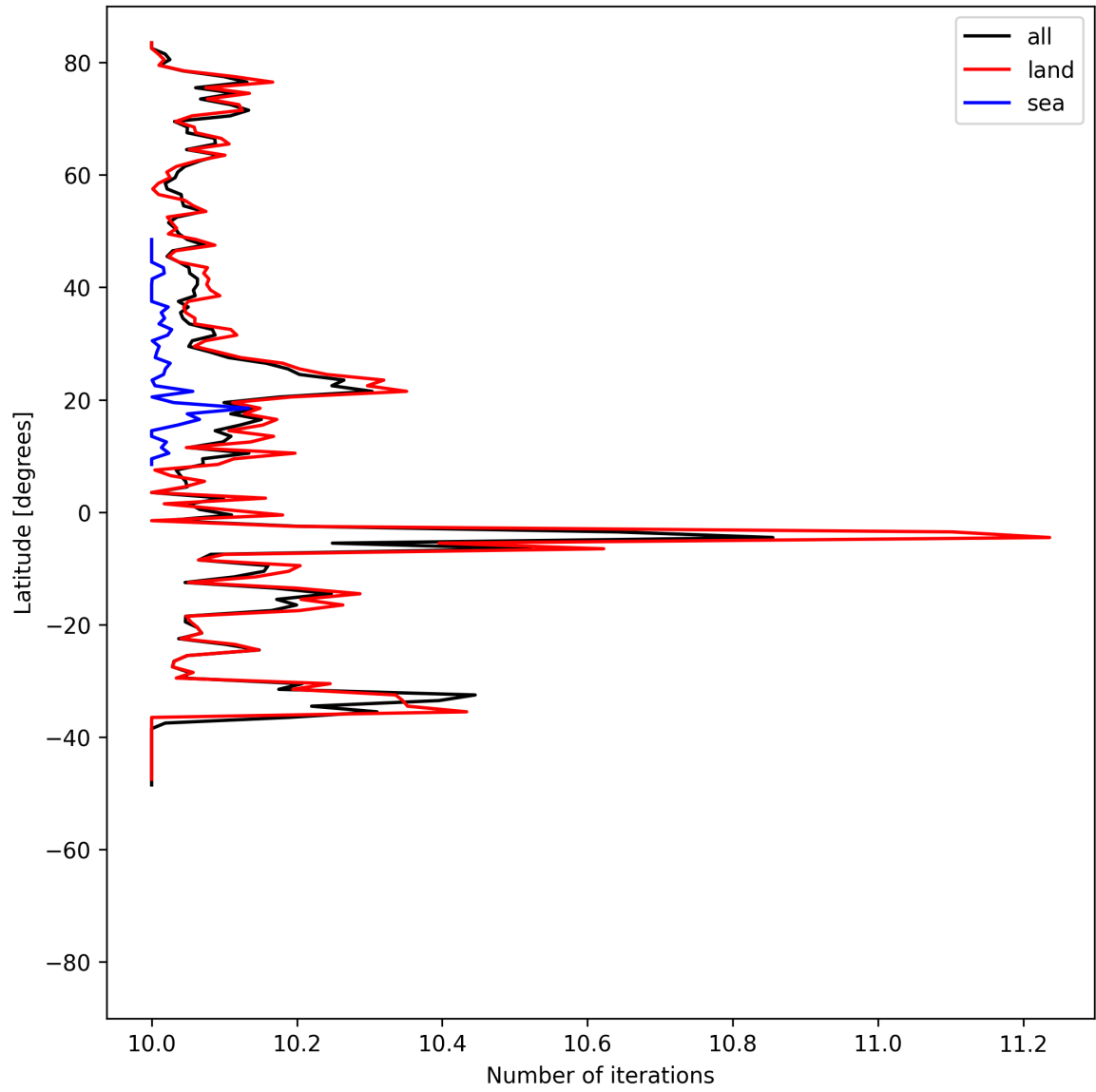
Figure 20: Zonal average of “Number of iterations” for 2025-06-27 to 2025-06-29.
