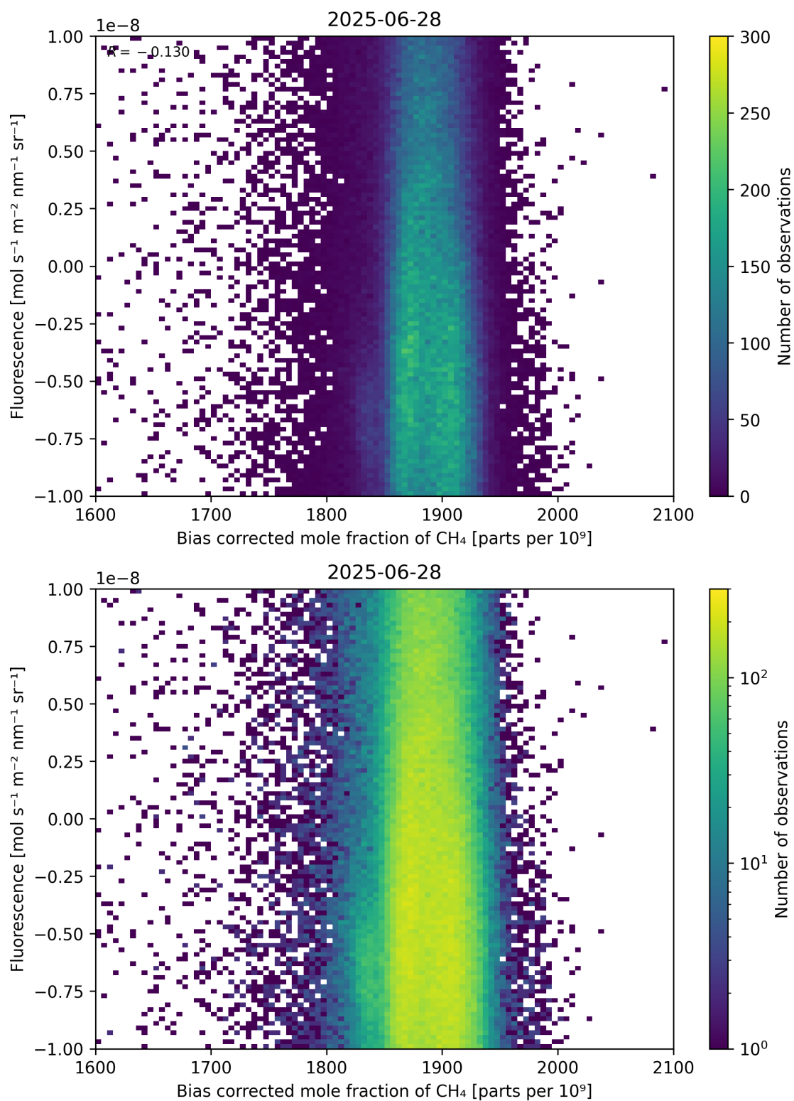
Figure 66: Scatter density plot of “Bias corrected mole fraction of \text{CH}_4 ” against “Fluorescence” for 2025-06-27 to 2025-06-29.
