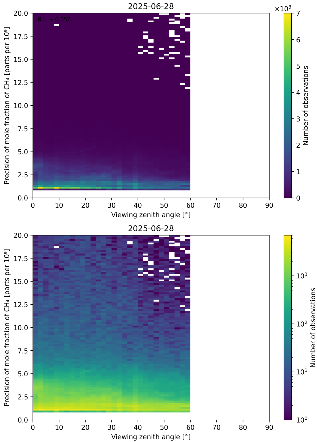
Figure 112: Scatter density plot of “Viewing zenith angle” against “Precision of mole fraction of CH 4 ” for 2025-06-27 to 2025-06-29.
