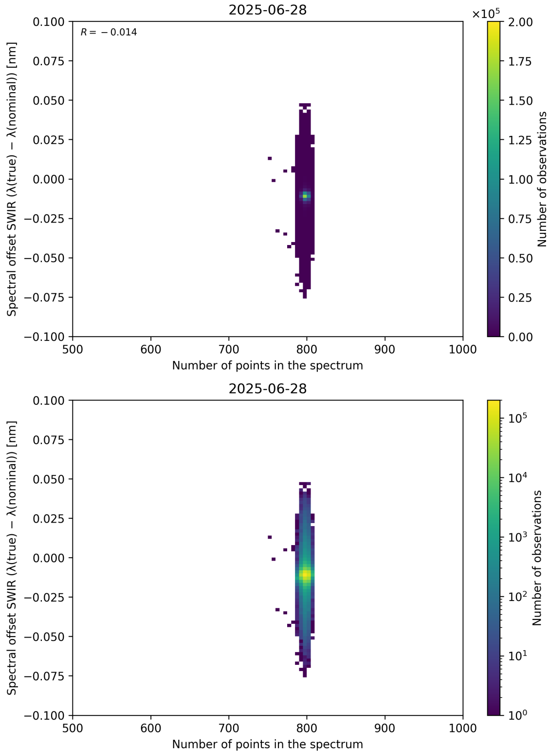
Figure 93: Scatter density plot of “Number of points in the spectrum” against “Spectral offset SWIR ( \lambda_{\text{true}} - \lambda_{\text{nominal}} )” for 2025-06-27 to 2025-06-29.
