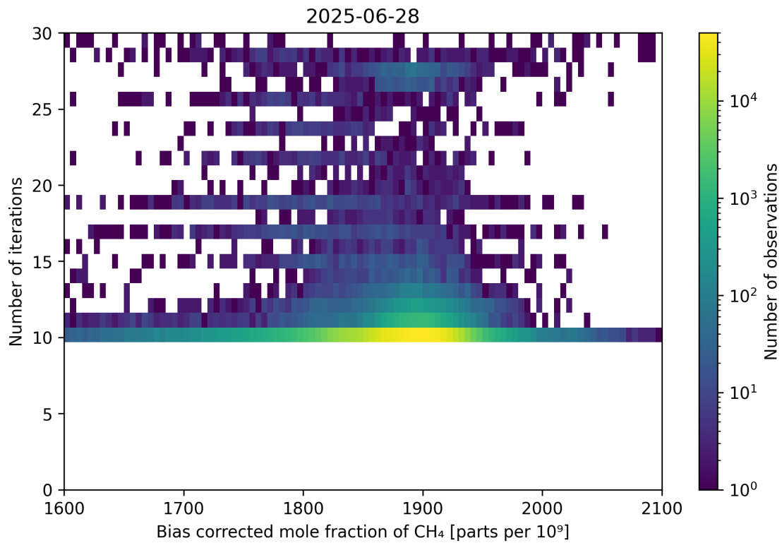
Figure 67: Scatter density plot of “Bias corrected mole fraction of \text{CH}_4 ” against “Number of iterations” for 2025-06-27 to 2025-06-29.
