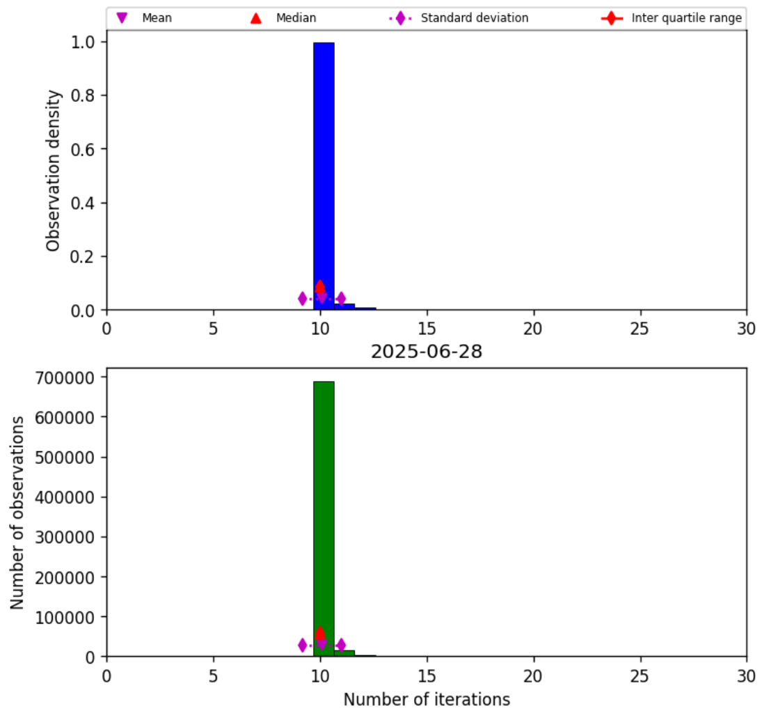
Figure 31: Histogram of “Number of iterations” for 2025-06-27 to 2025-06-29
