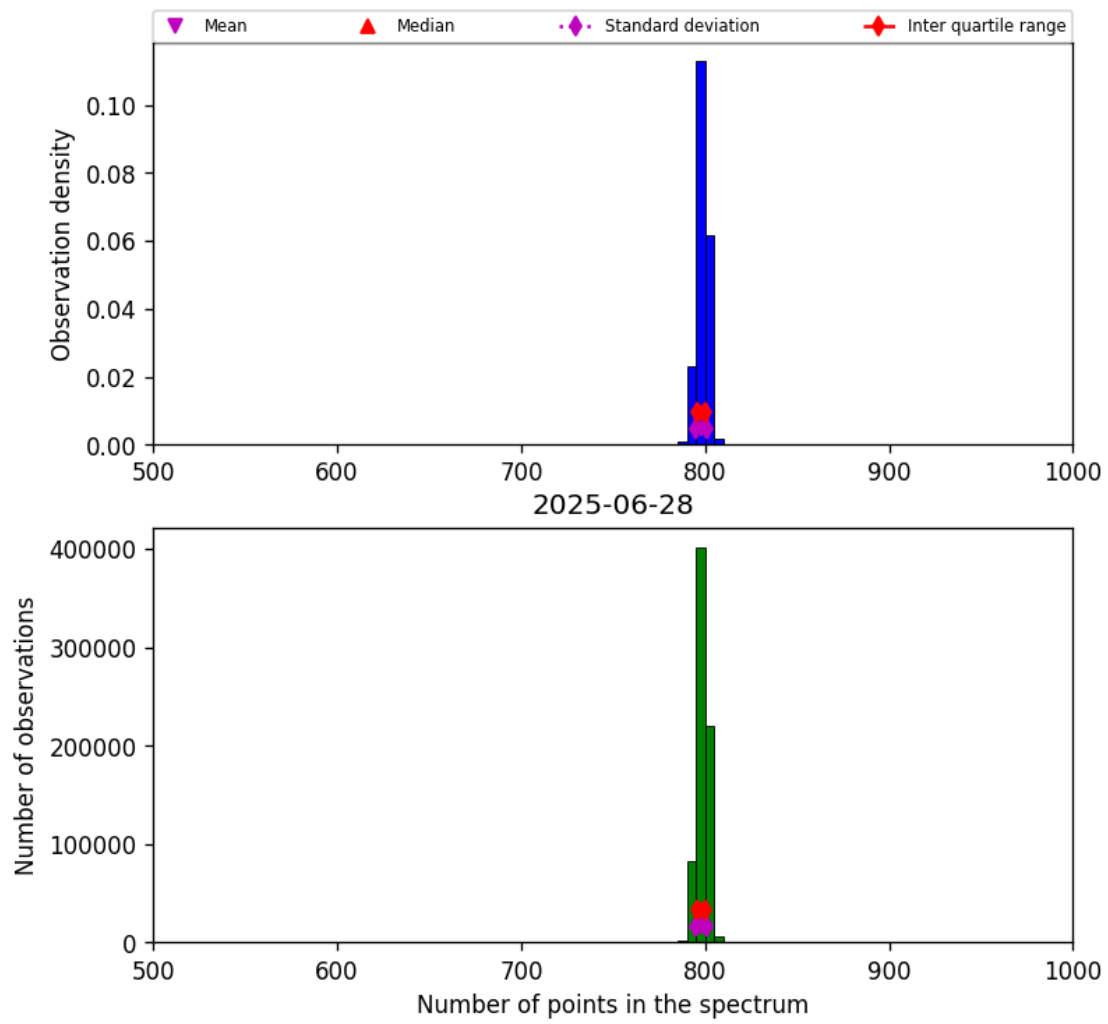
Figure 26: Histogram of “Number of points in the spectrum” for 2025-06-27 to 2025-06-29
