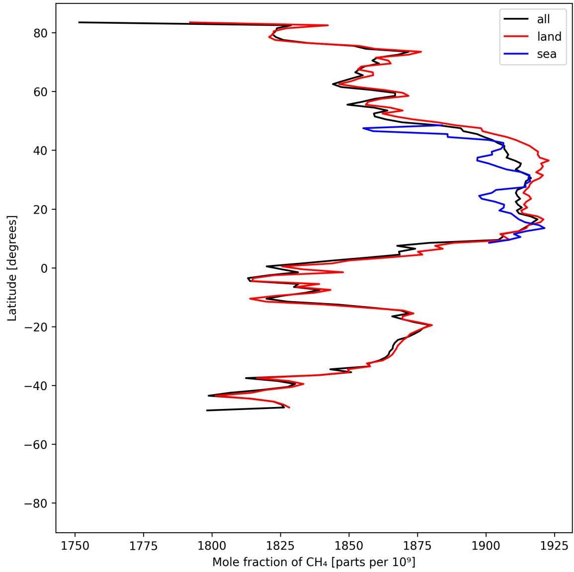
Figure 12: Zonal average of “Mole fraction of \text{CH}_4 ” for 2025-06-27 to 2025-06-29.
