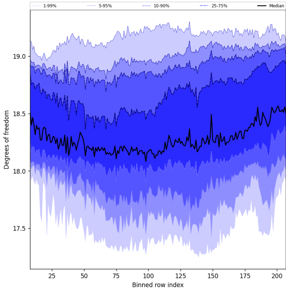
Figure 41: Along track statistics of “Degrees of freedom” for 2025-06-27 to 2025-06-29
