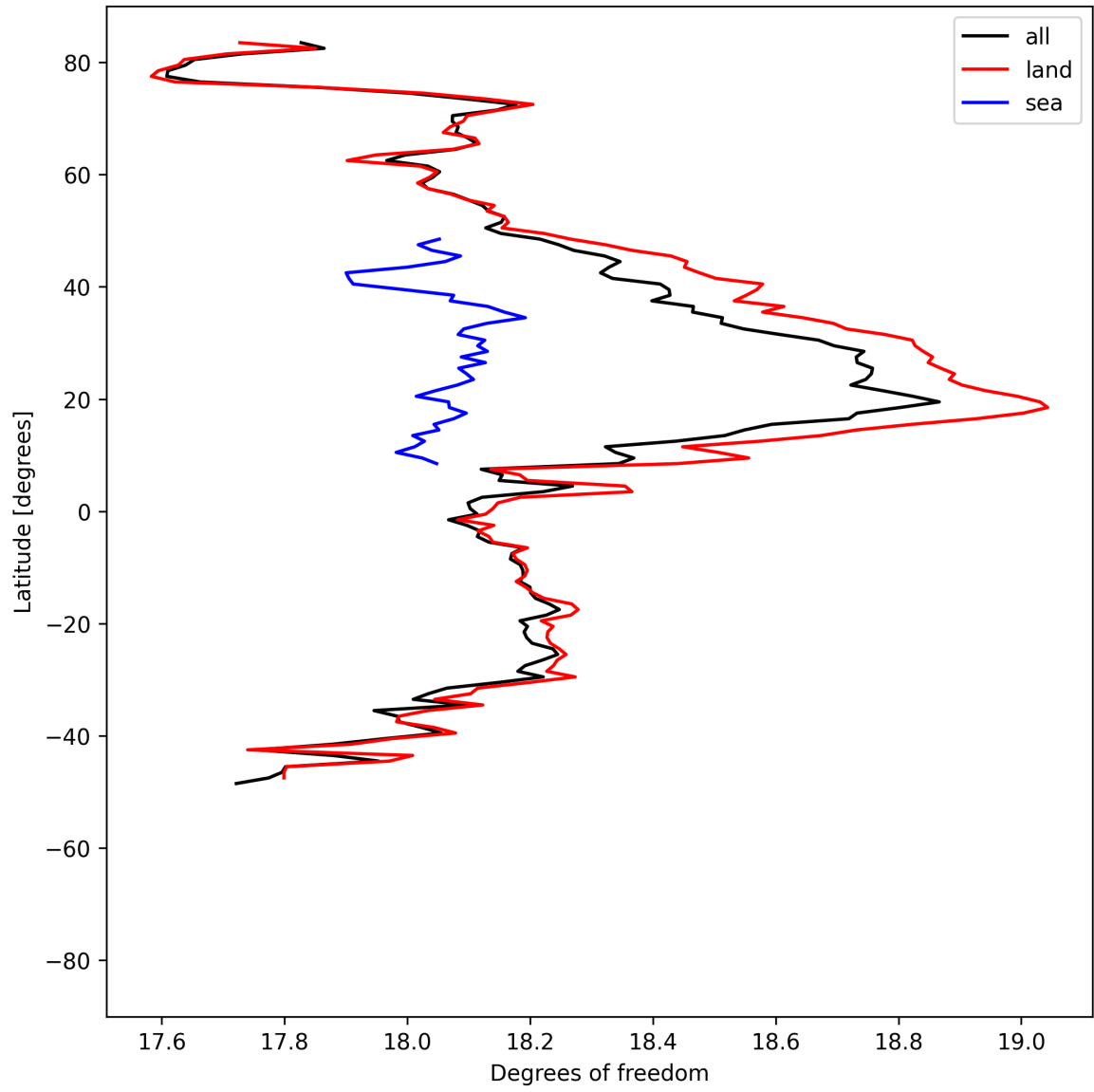
Figure 19: Zonal average of “Degrees of freedom” for 2025-06-27 to 2025-06-29.
