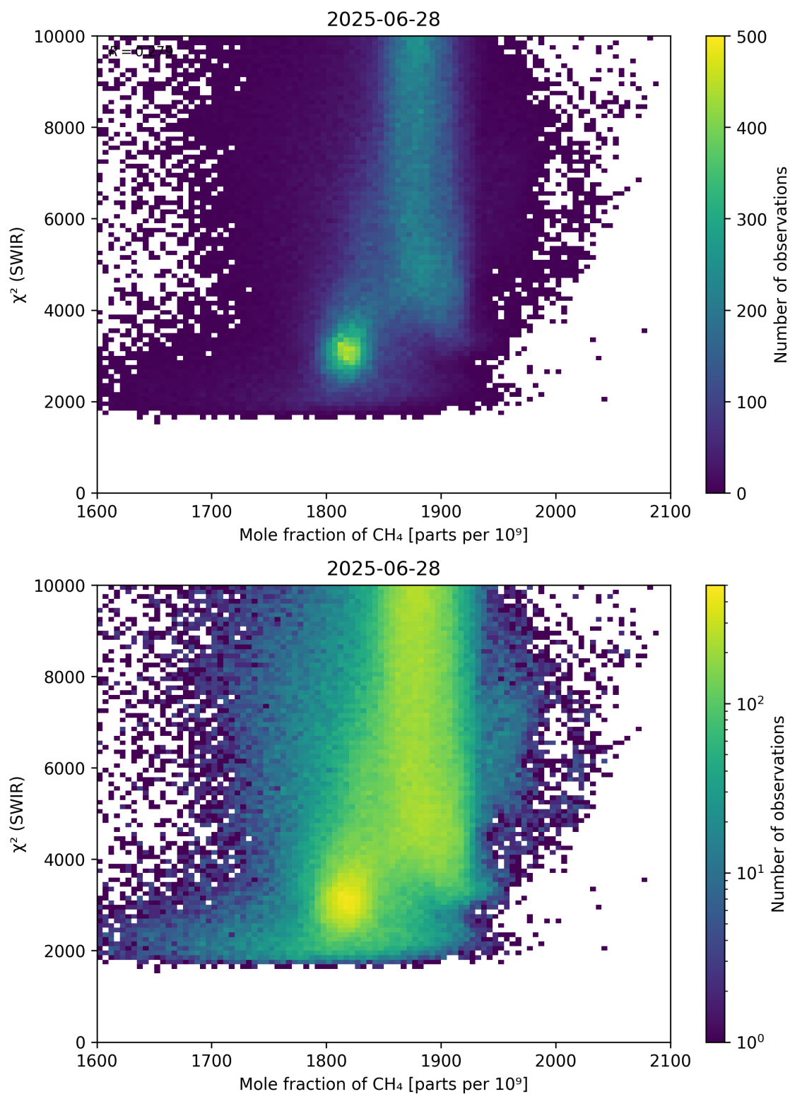
Figure 71: Scatter density plot of “Mole fraction of CH 4 ” against “ \chi^2 (SWIR)” for 2025-06-27 to 2025-06-29.
