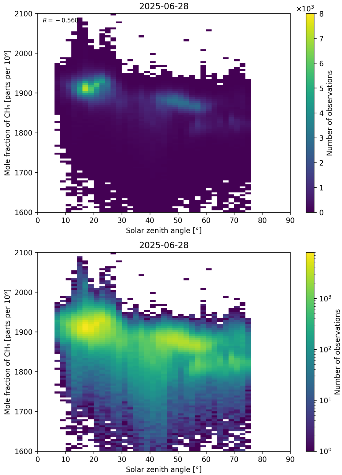
Figure 99: Scatter density plot of “Solar zenith angle” against “Mole fraction of CH 4 ” for 2025-06-27 to 2025-06-29.
