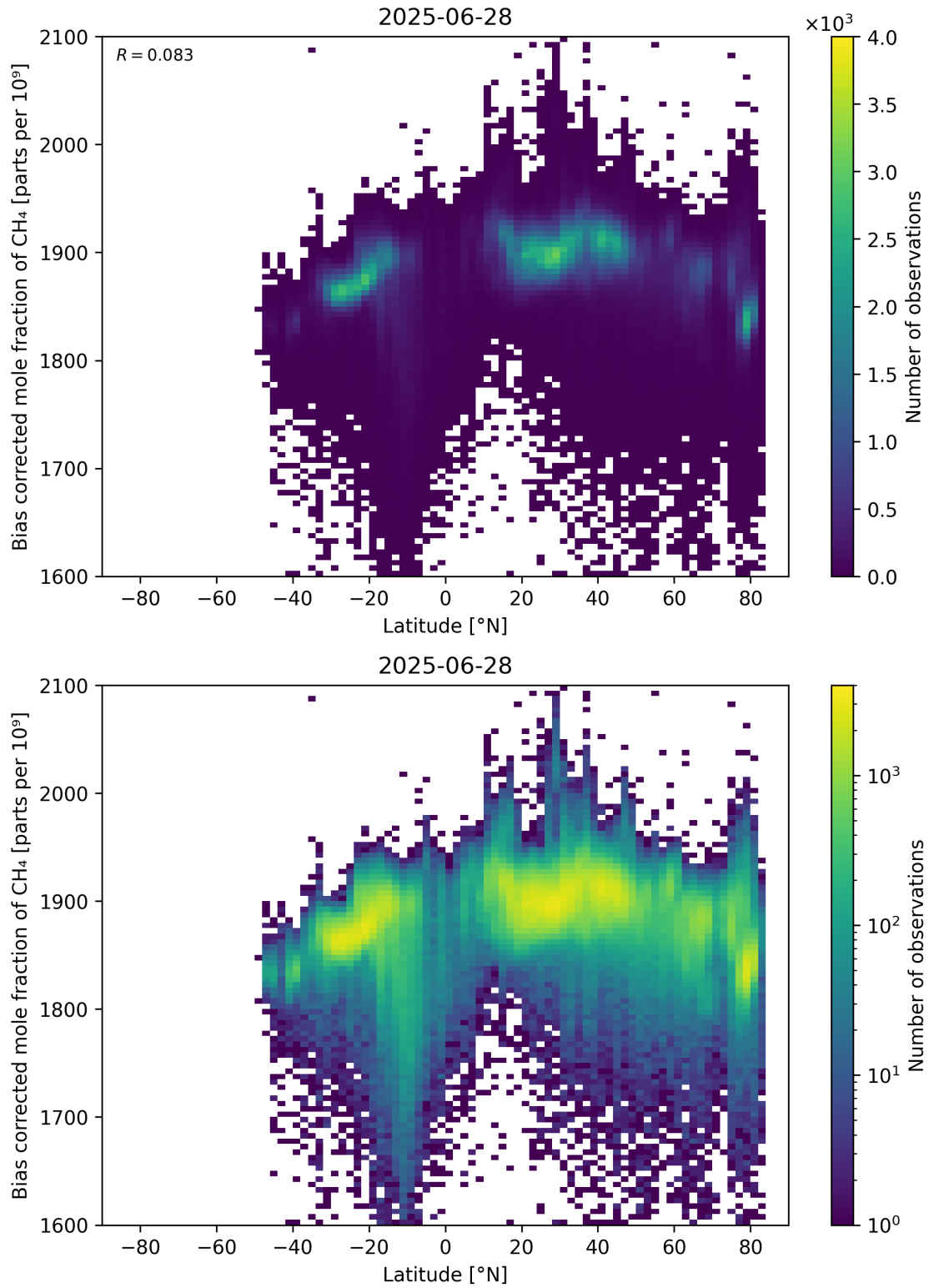
Figure 58: Scatter density plot of “Latitude” against “Bias corrected mole fraction of CH 4 ” for 2025-06-27 to 2025-06-29.
