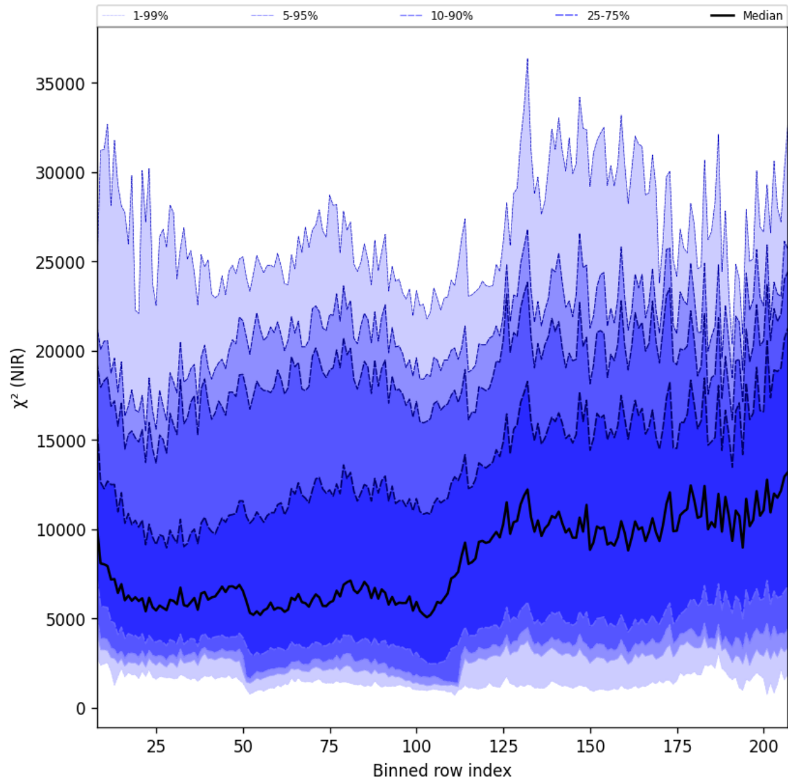
Figure 40: Along track statistics of " \chi^2 (NIR)" for 2025-06-27 to 2025-06-29
