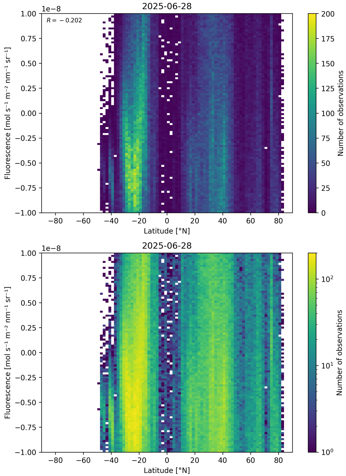
Figure 56: Scatter density plot of “Latitude” against “Fluorescence” for 2025-06-27 to 2025-06-29.
