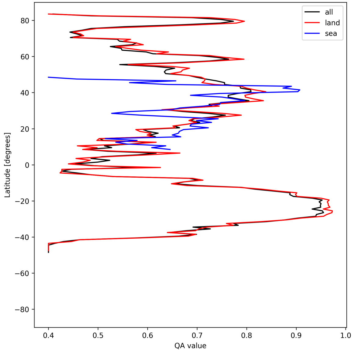
Figure 11: Zonal average of “QA value” for 2025-06-27 to 2025-06-29.
