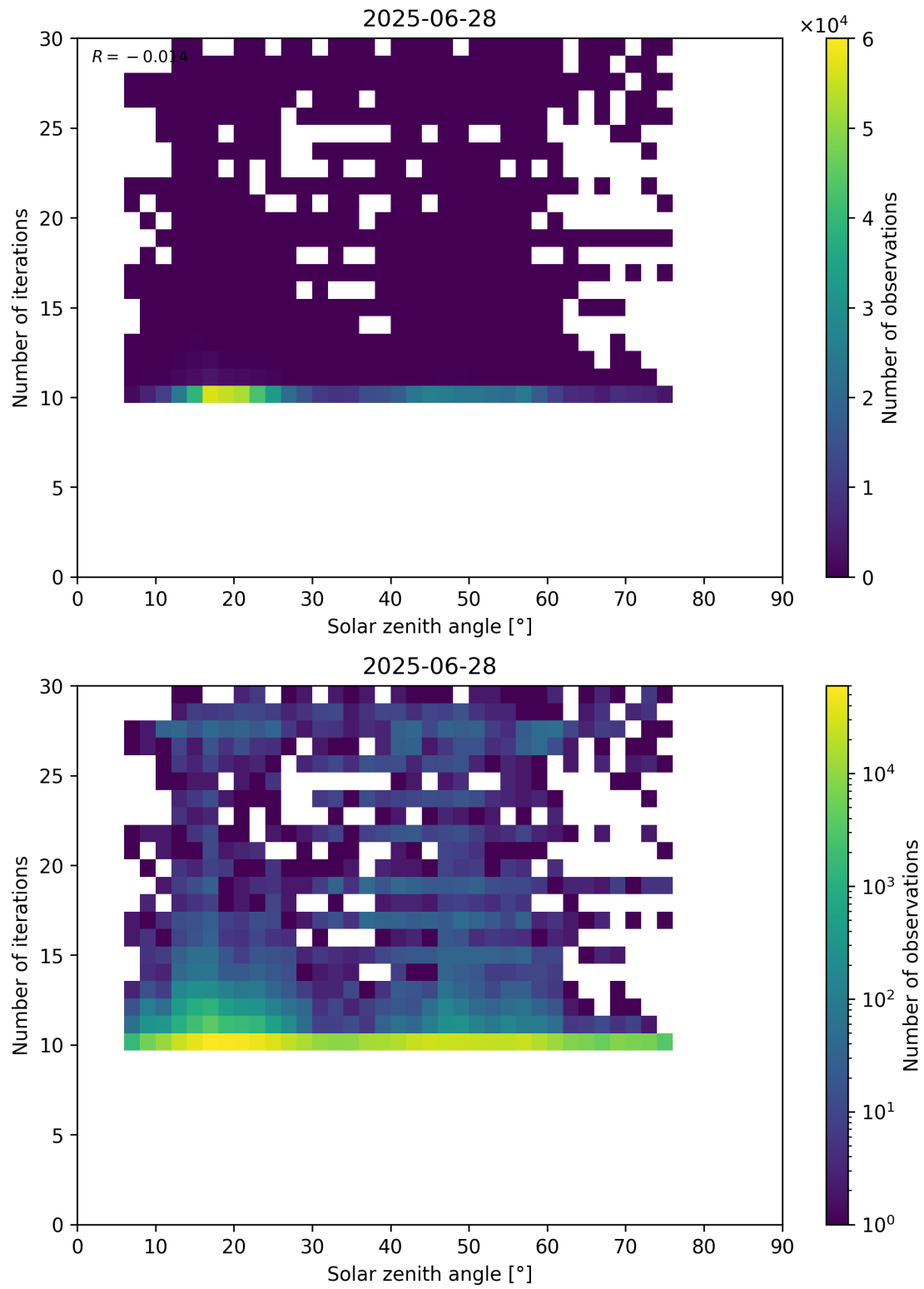
Figure 102: Scatter density plot of “Solar zenith angle” against “Number of iterations” for 2025-06-27 to 2025-06-29.
