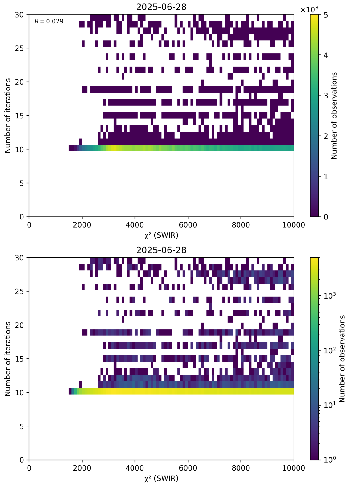
Figure 50: Scatter density plot of “ \chi^2 (SWIR)” against “Number of iterations” for 2025-06-27 to 2025-06-29.
