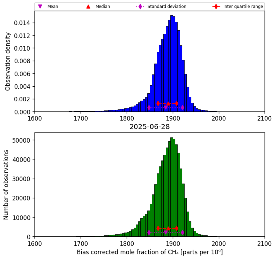
Figure 25: Histogram of “Bias corrected mole fraction of CH 4 ” for 2025-06-27 to 2025-06-29
