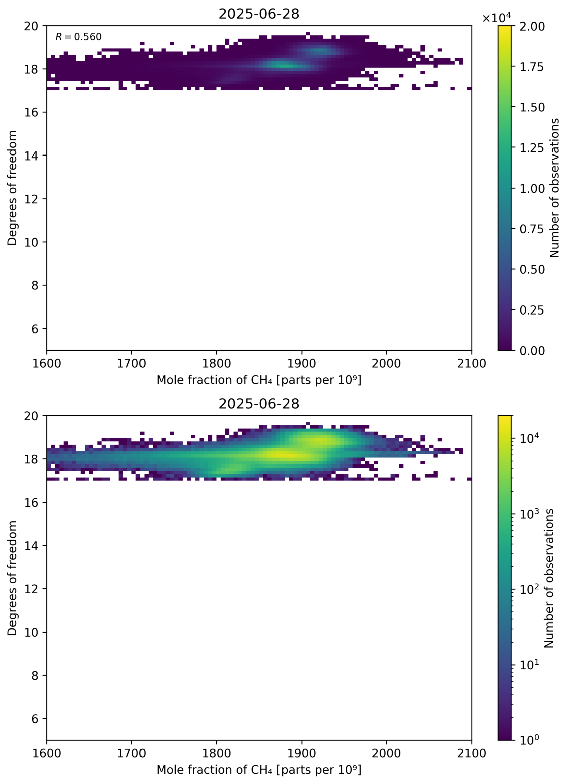
Figure 72: Scatter density plot of “Mole fraction of CH 4 ” against “Degrees of freedom” for 2025-06-27 to 2025-06-29.
