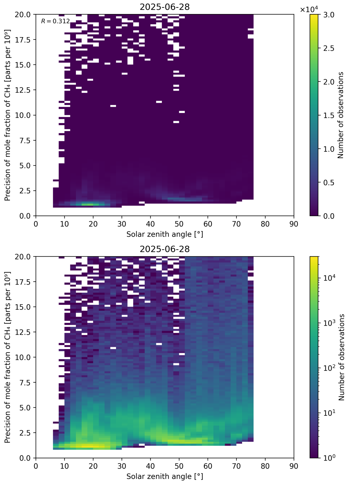
Figure 101: Scatter density plot of “Solar zenith angle” against “Precision of mole fraction of CH 4 ” for 2025-06-27 to 2025-06-29.
