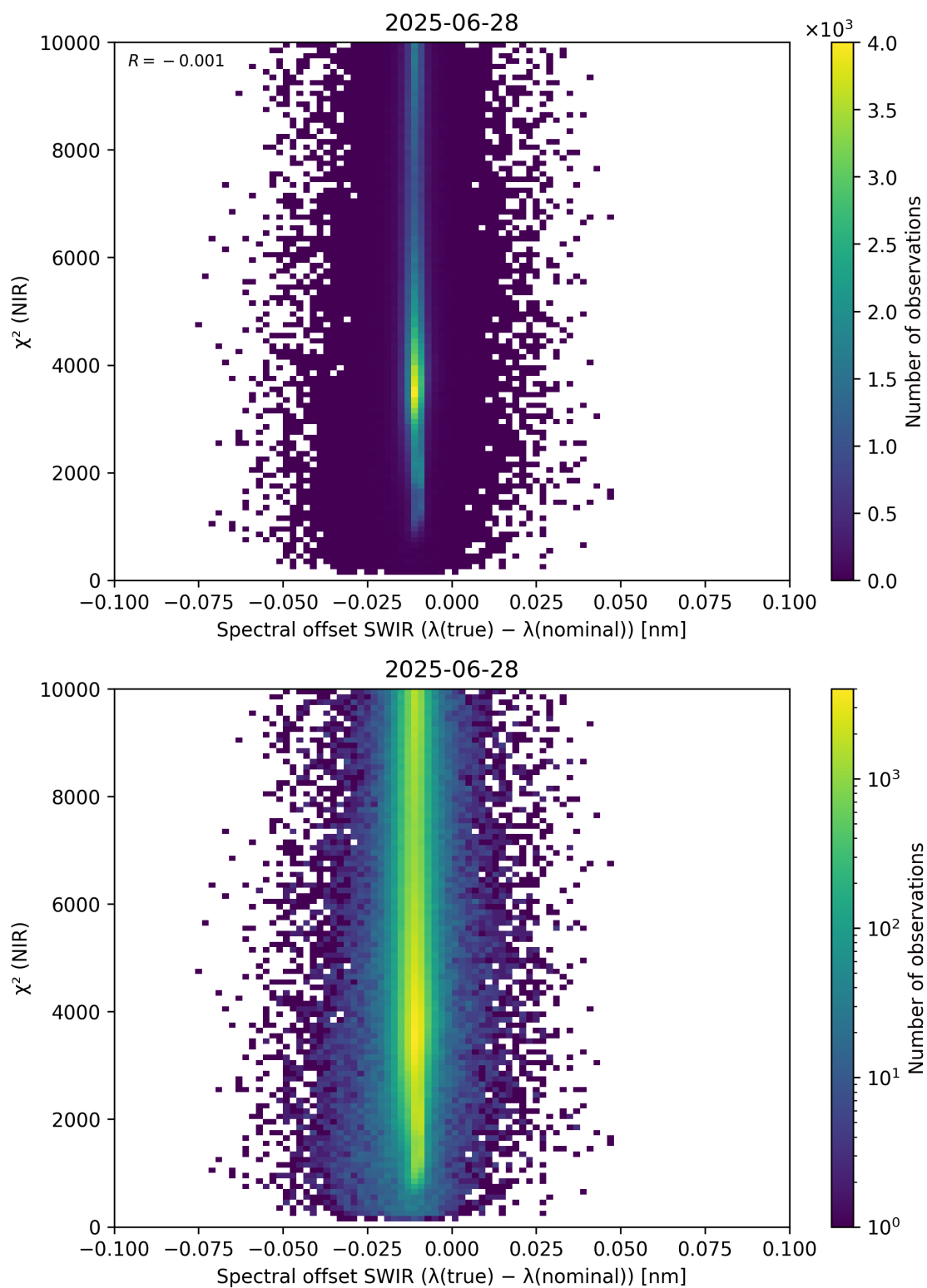
Figure 117: Scatter density plot of “Spectral offset SWIR ( \lambda_{\text{true}} - \lambda_{\text{nominal}} )” against “ \chi^2 (NIR)” for 2025-06-27 to 2025-06-29.
