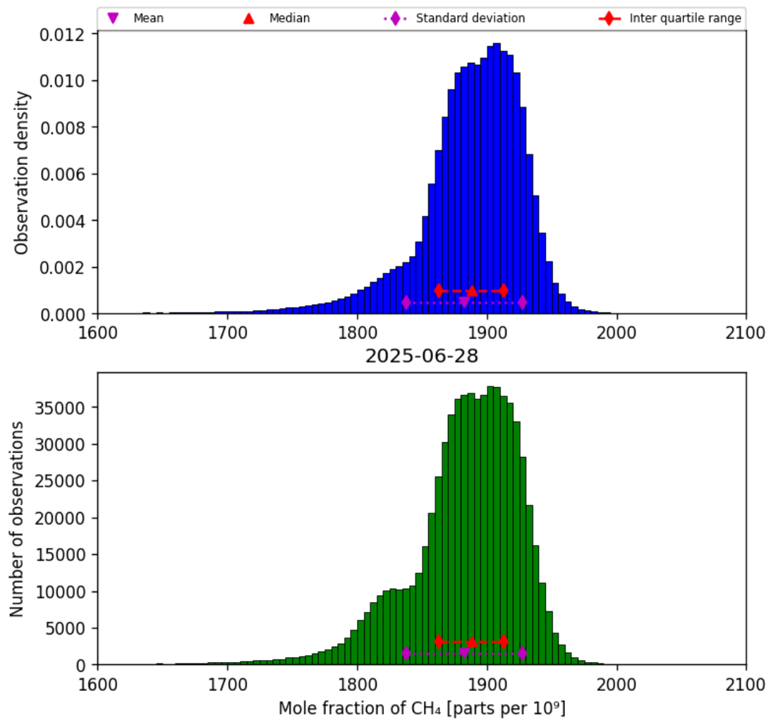
Figure 23: Histogram of “Mole fraction of CH 4 ” for 2025-06-27 to 2025-06-29
