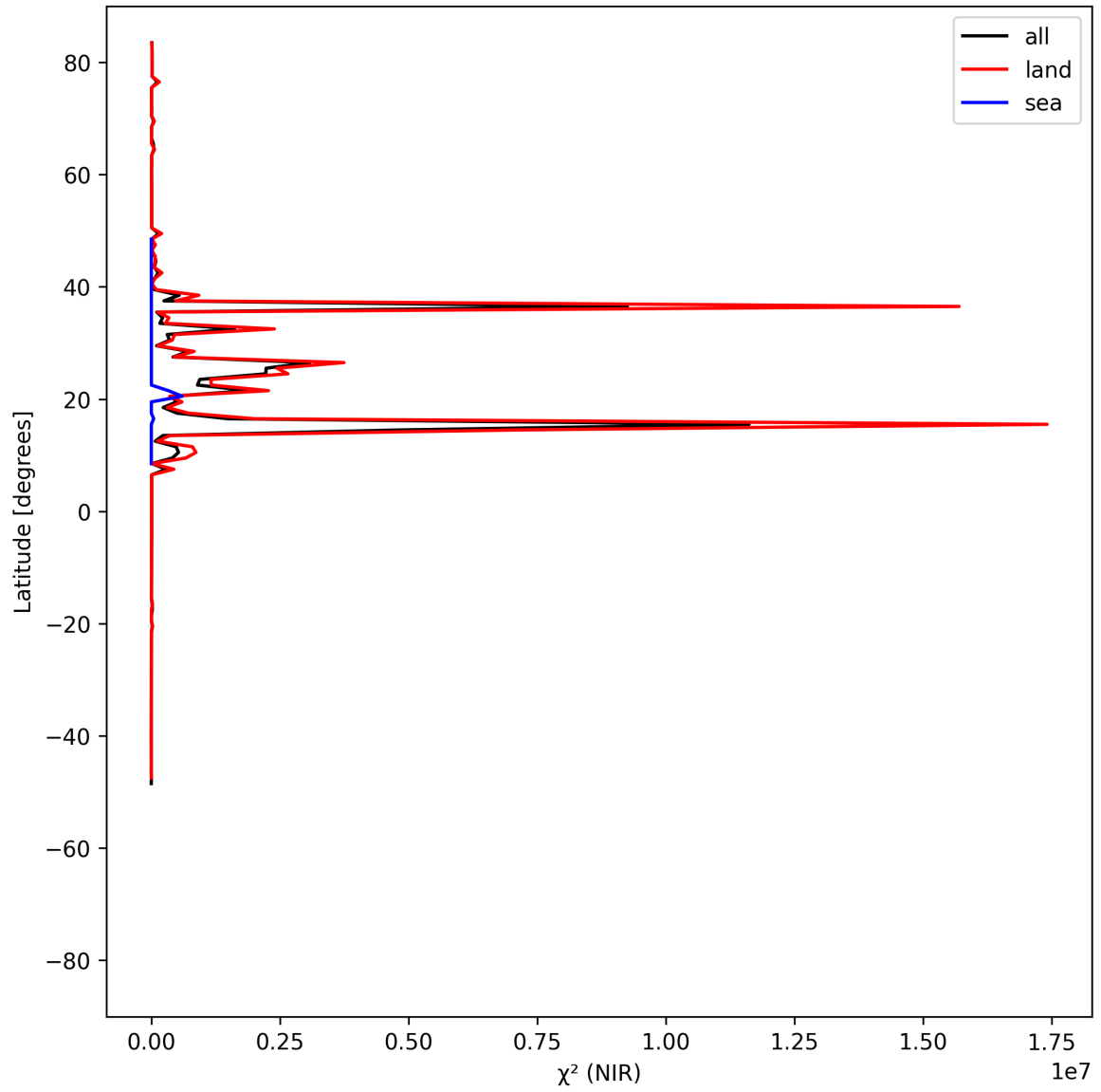
Figure 18: Zonal average of “ \chi^2 (NIR)” for 2025-06-27 to 2025-06-29.
