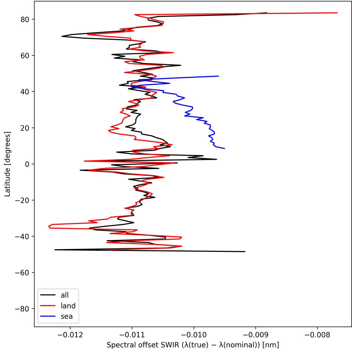
Figure 16: Zonal average of “Spectral offset SWIR ( \lambda_{\text{true}} - \lambda_{\text{nominal}} )” for 2025-06-27 to 2025-06-29.
