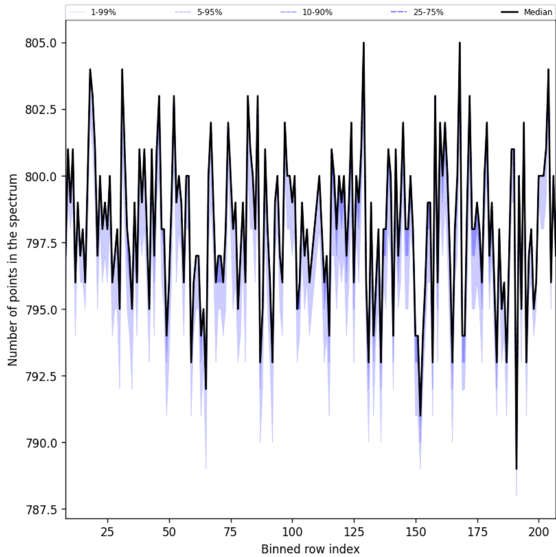
Figure 37: Along track statistics of “Number of points in the spectrum” for 2025-06-27 to 2025-06-29
