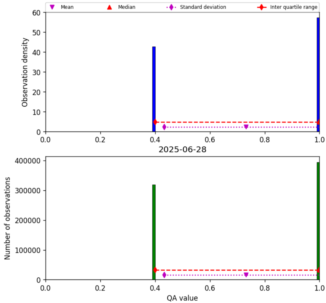
Figure 22: Histogram of “QA value” for 2025-06-27 to 2025-06-29
