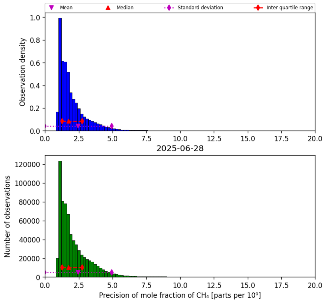
Figure 24: Histogram of “Precision of mole fraction of CH 4 ” for 2025-06-27 to 2025-06-29
