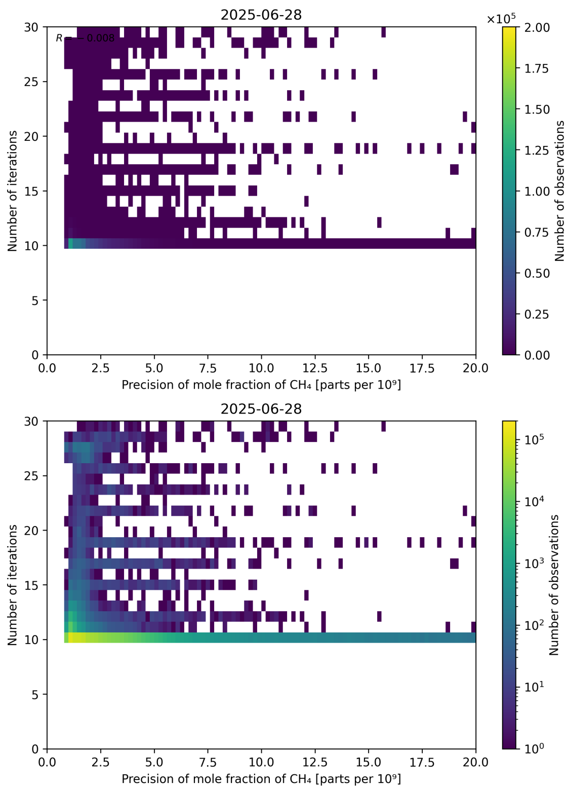
Figure 83: Scatter density plot of “Precision of mole fraction of CH 4 ” against “Number of iterations” for 2025-06-27 to 2025-06-29.
