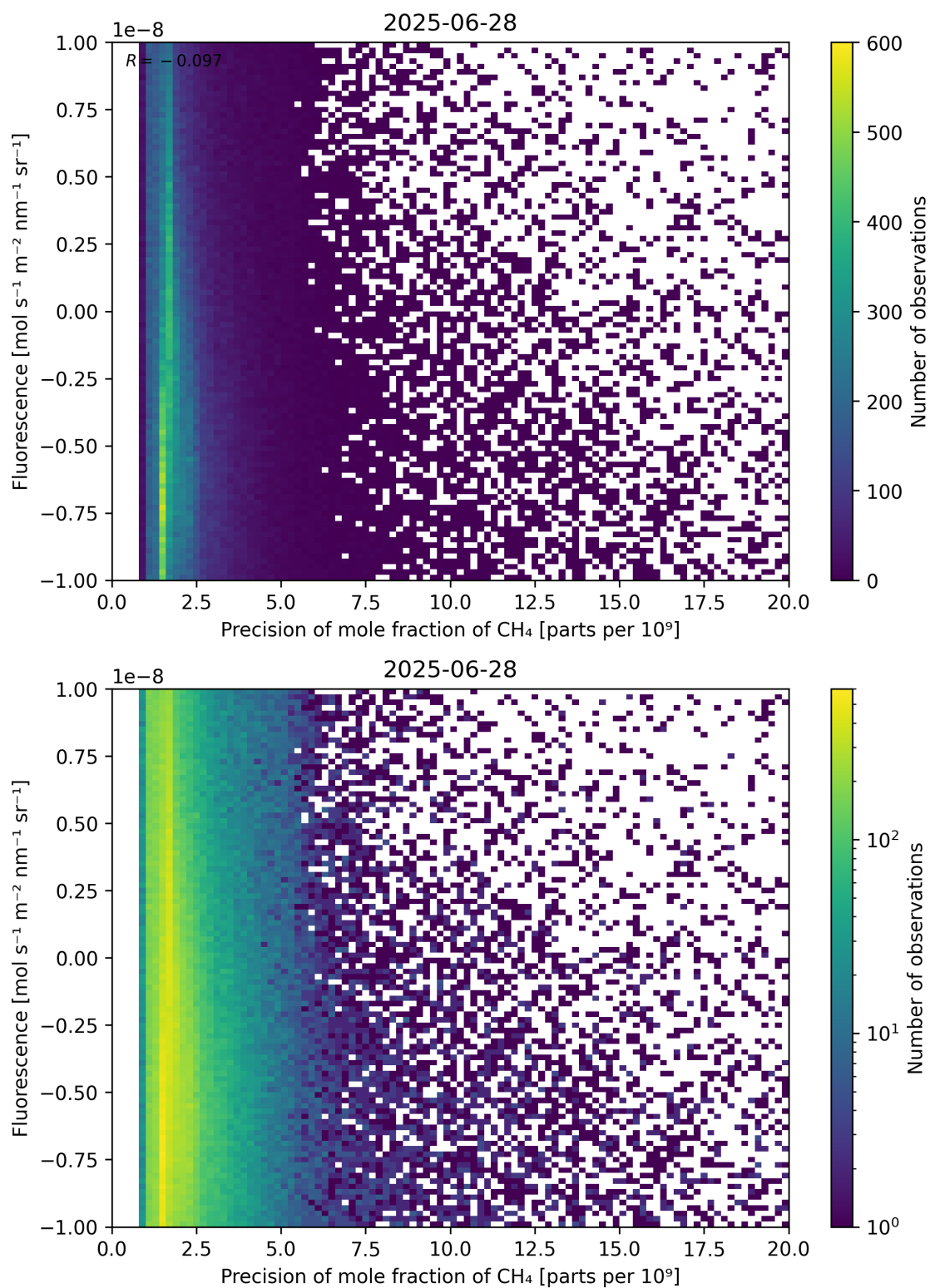
Figure 81: Scatter density plot of “Precision of mole fraction of \text{CH}_4 ” against “Fluorescence” for 2025-06-27 to 2025-06-29.
