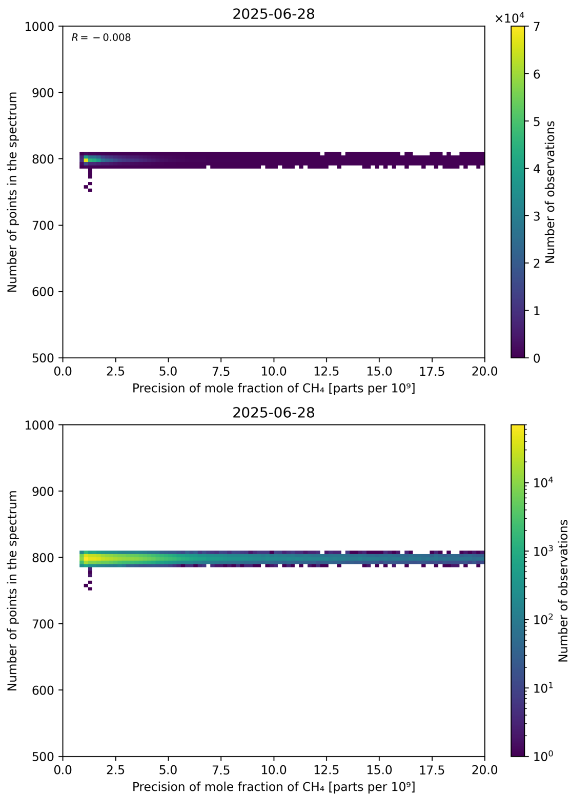
Figure 84: Scatter density plot of “Precision of mole fraction of CH 4 ” against “Number of points in the spectrum” for 2025-06-27 to 2025-06-29.
