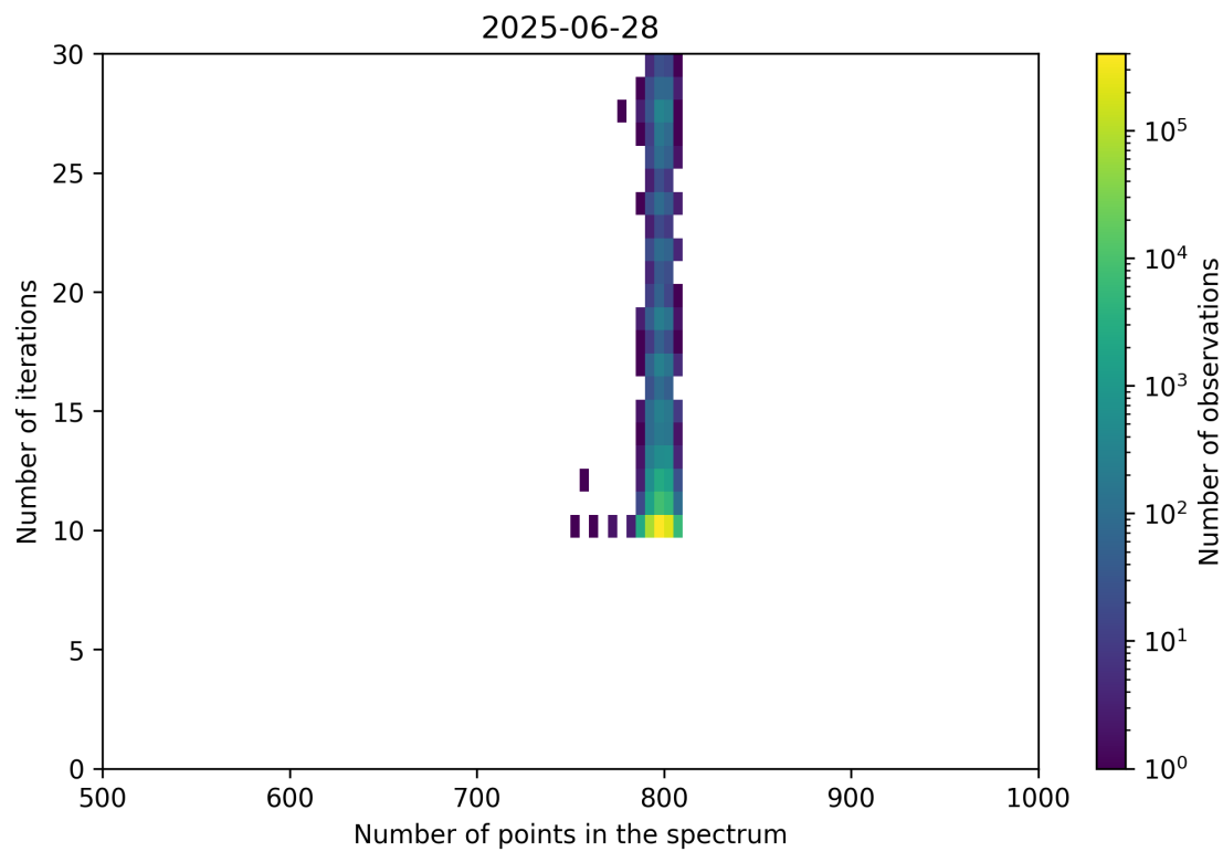
Figure 92: Scatter density plot of “Number of points in the spectrum” against “Number of iterations” for 2025-06-27 to 2025-06-29.
