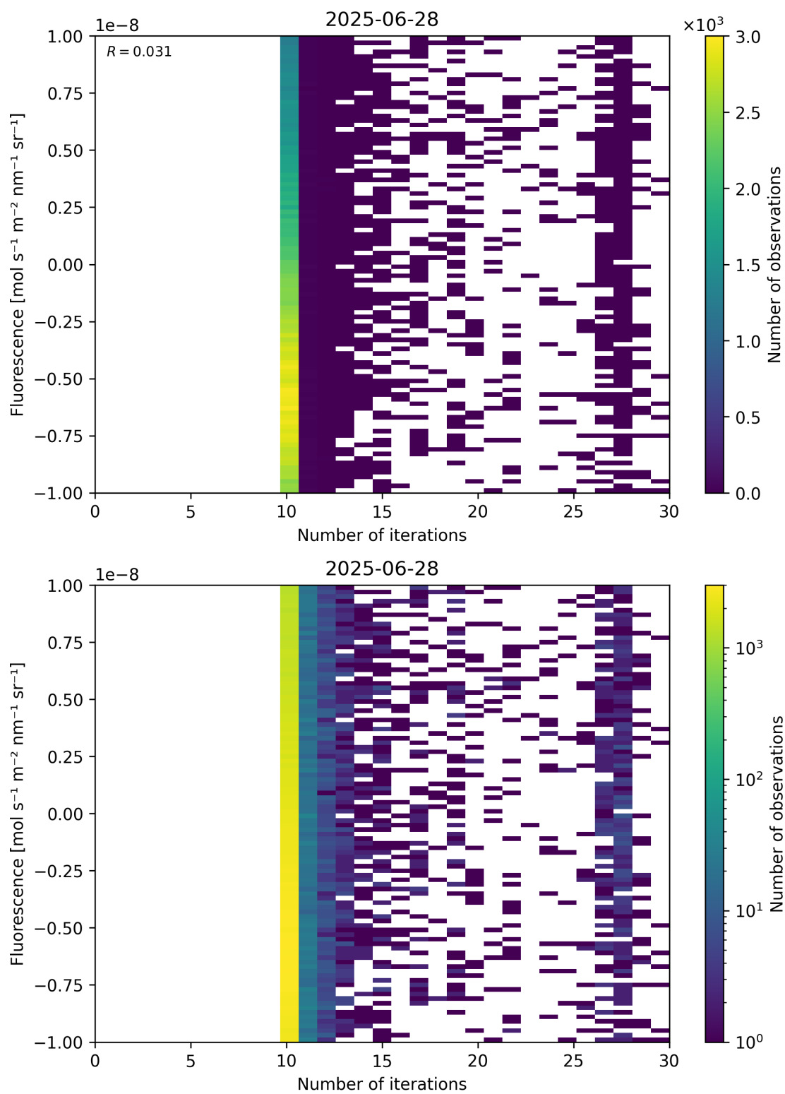
Figure 87: Scatter density plot of “Number of iterations” against “Fluorescence” for 2025-06-27 to 2025-06-29.
