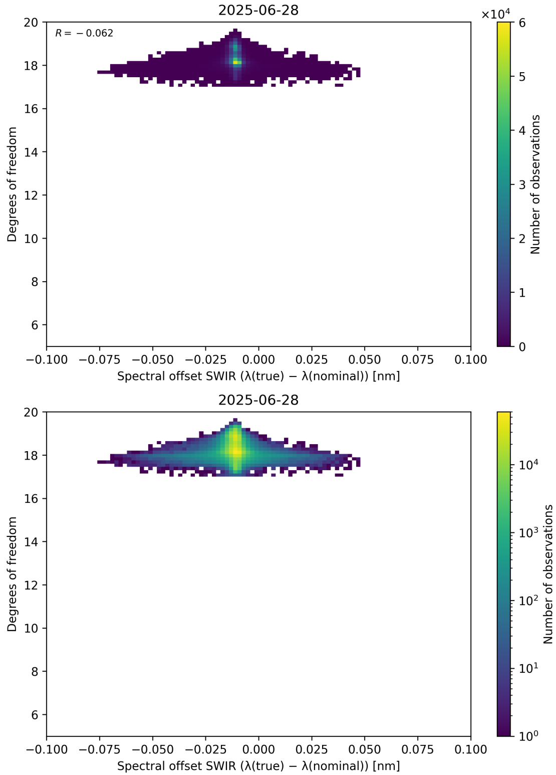
Figure 119: Scatter density plot of “Spectral offset SWIR ( \lambda_{\text{true}} - \lambda_{\text{nominal}} )” against “Degrees of freedom” for 2025-06-27 to 2025-06-29.
