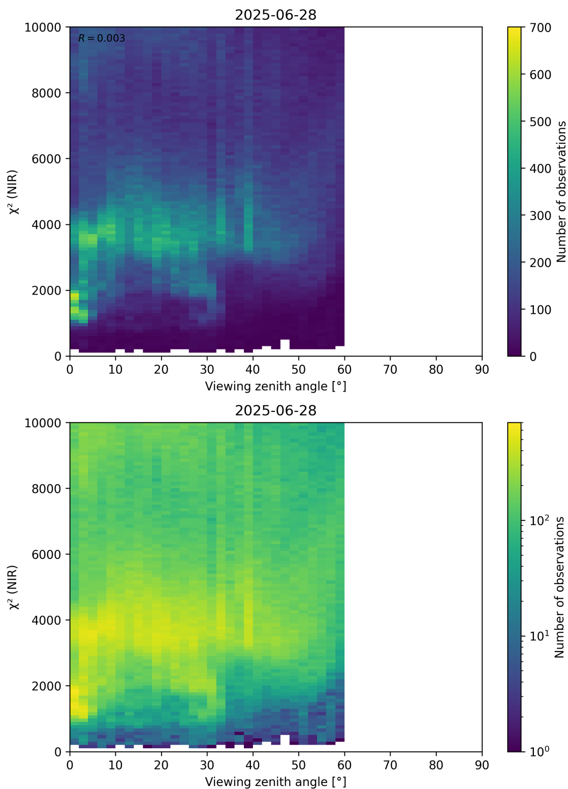
Figure 105: Scatter density plot of “Viewing zenith angle” against “ \chi^2 (NIR)” for 2025-06-27 to 2025-06-29.
