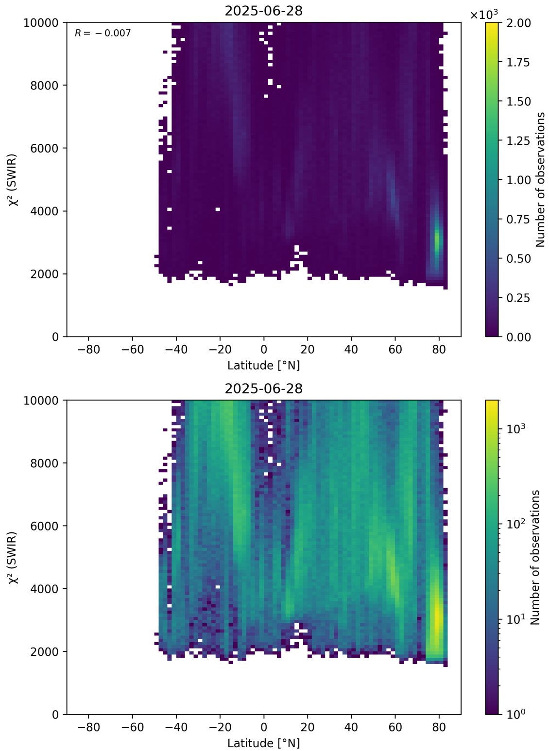
Figure 54: Scatter density plot of “Latitude” against “ \chi^2 (SWIR)” for 2025-06-27 to 2025-06-29.
