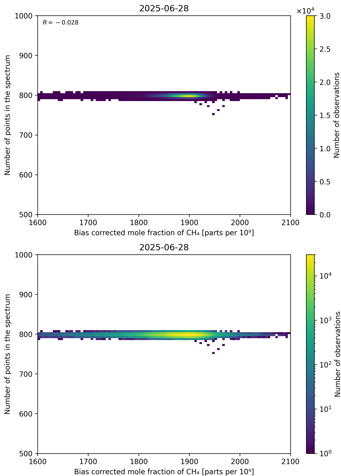
Figure 68: Scatter density plot of “Bias corrected mole fraction of CH 4 ” against “Number of points in the spectrum” for 2025-06-27 to 2025-06-29.
