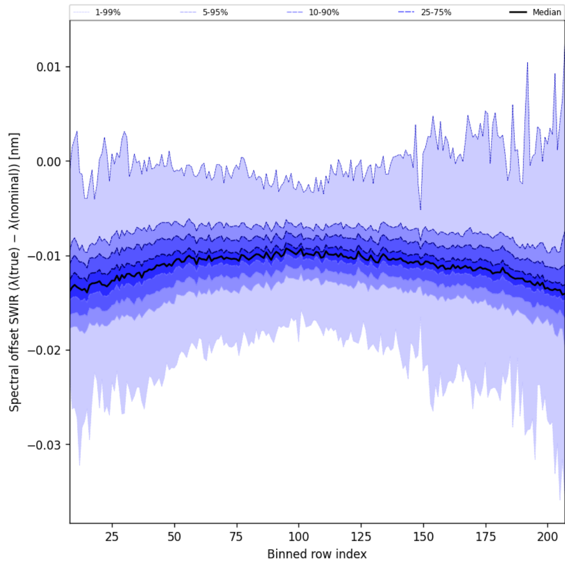
Figure 38: Along track statistics of “Spectral offset SWIR ( \lambda_{\text{true}} - \lambda_{\text{nominal}} )” for 2025-06-27 to 2025-06-29
