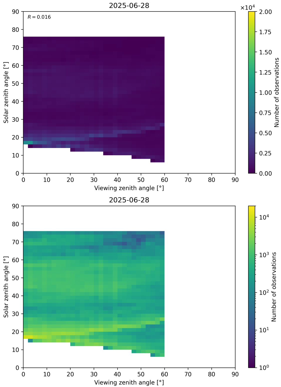
Figure 115: Scatter density plot of “Viewing zenith angle” against “Solar zenith angle” for 2025-06-27 to 2025-06-29.
