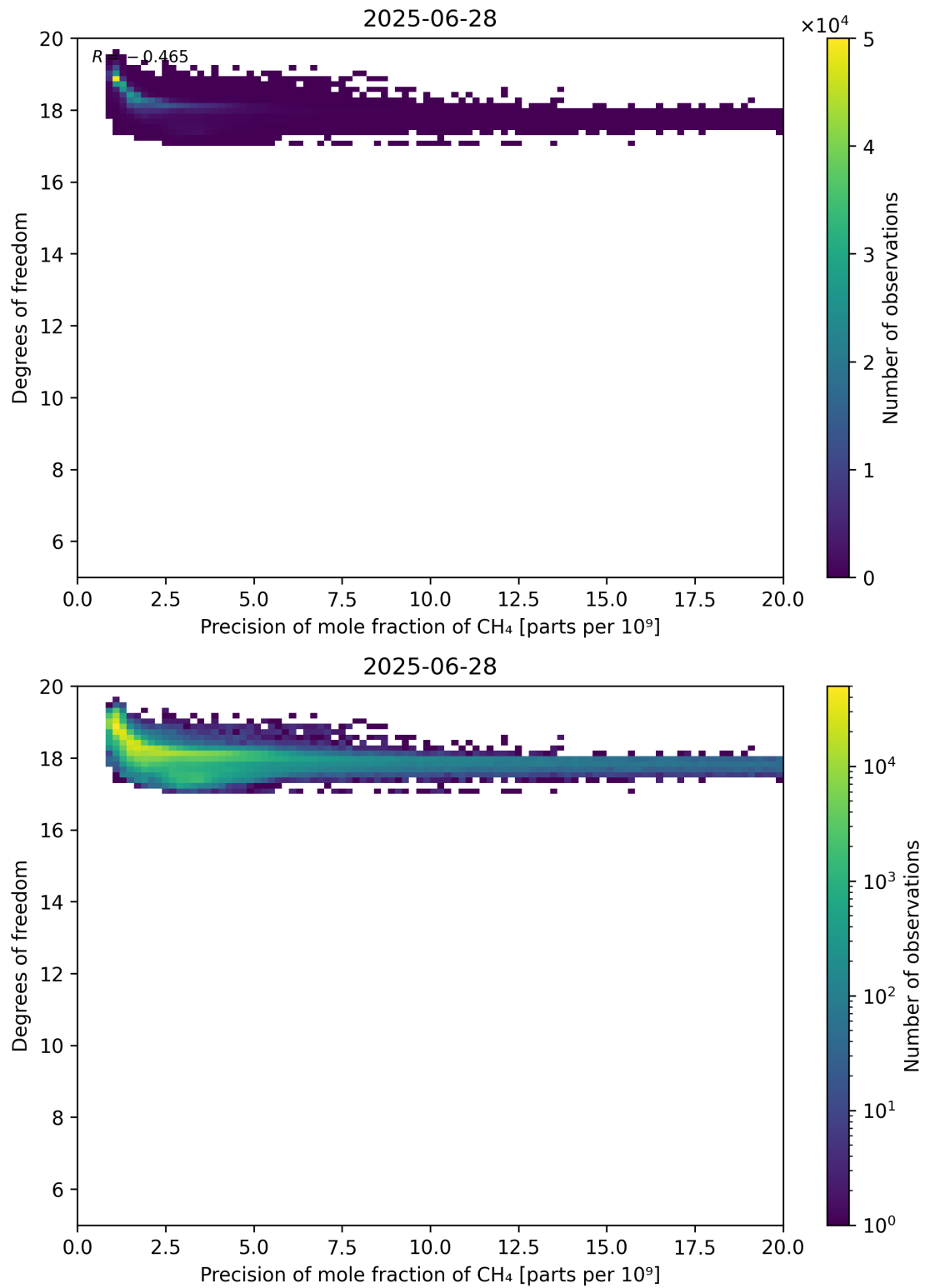
Figure 80: Scatter density plot of “Precision of mole fraction of CH 4 ” against “Degrees of freedom” for 2025-06-27 to 2025-06-29.
