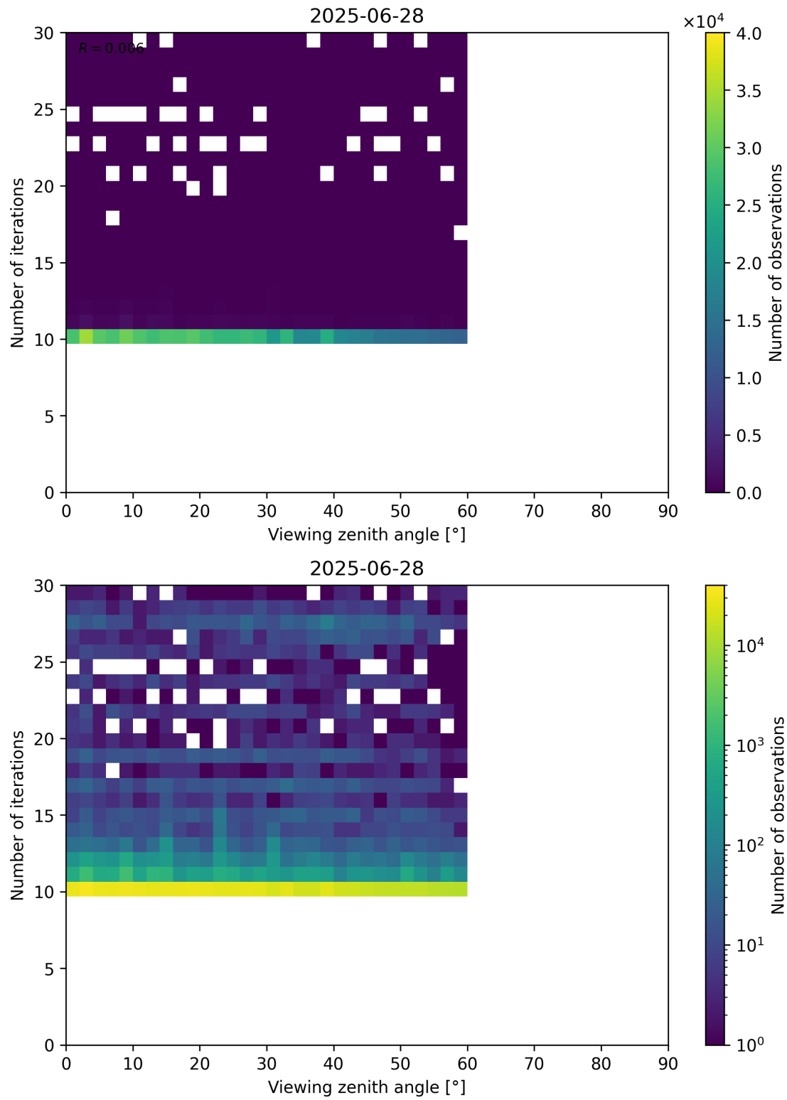
Figure 113: Scatter density plot of “Viewing zenith angle” against “Number of iterations” for 2025-06-27 to 2025-06-29.
