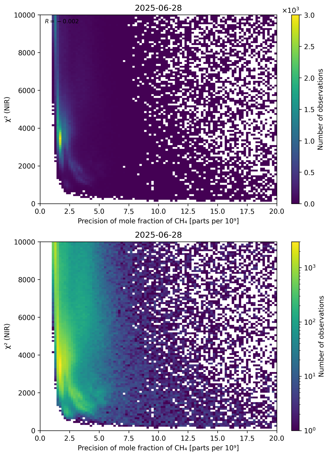
Figure 78: Scatter density plot of “Precision of mole fraction of CH 4 ” against “ \chi^2 (NIR)” for 2025-06-27 to 2025-06-29.
