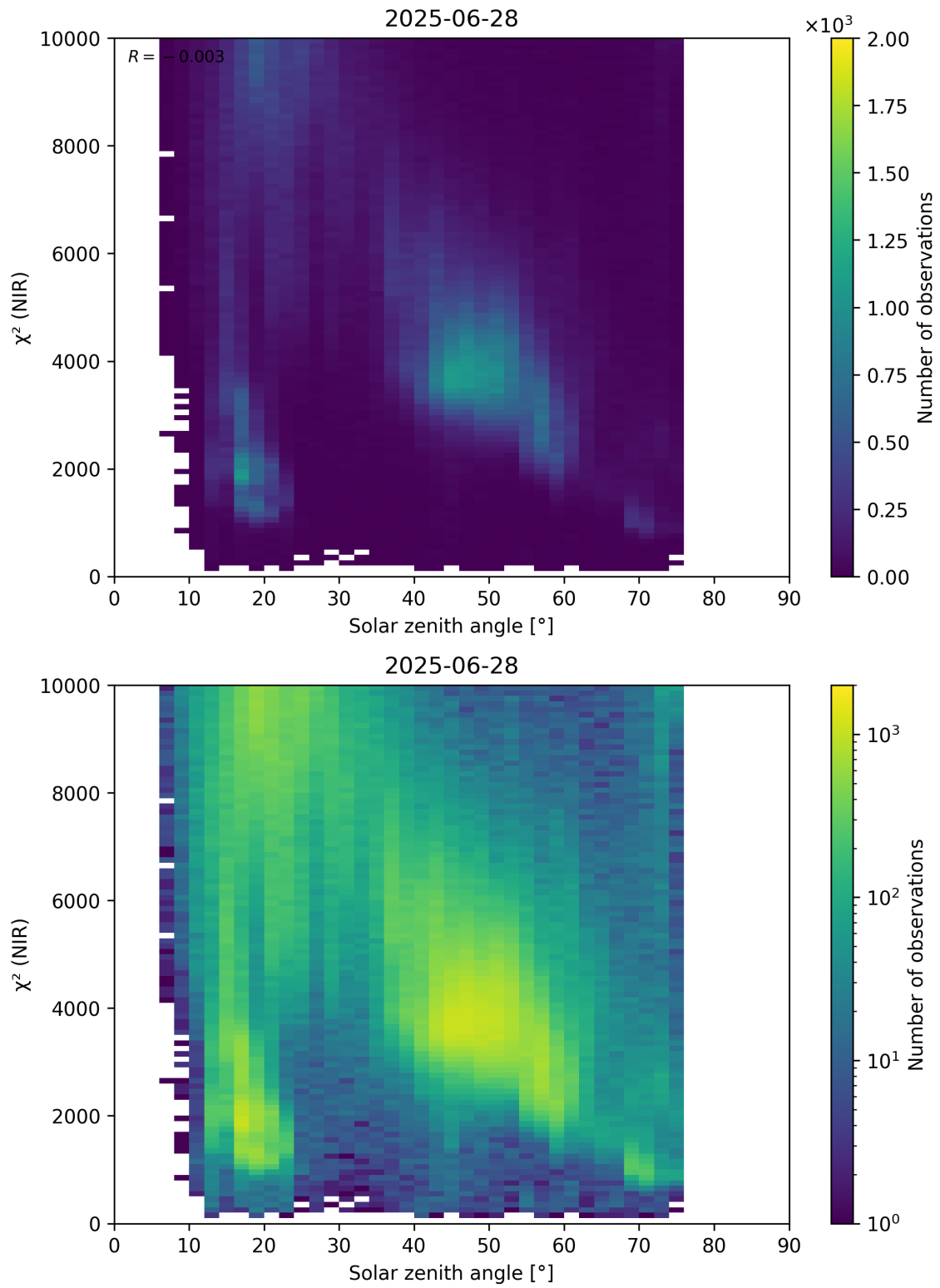
Figure 94: Scatter density plot of “Solar zenith angle” against “ \chi^2 (NIR)” for 2025-06-27 to 2025-06-29.
