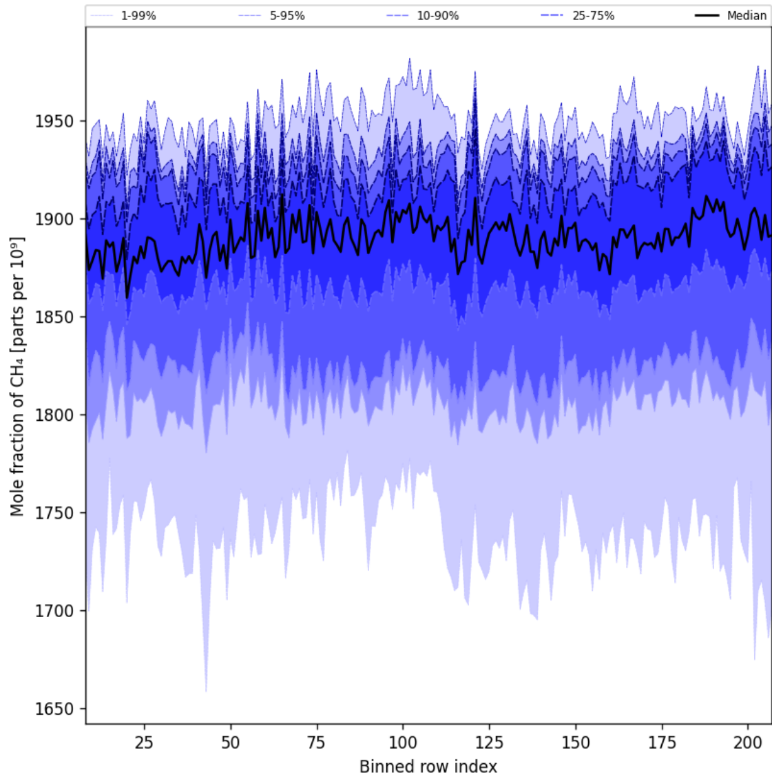
Figure 34: Along track statistics of “Mole fraction of CH 4 ” for 2025-06-27 to 2025-06-29
