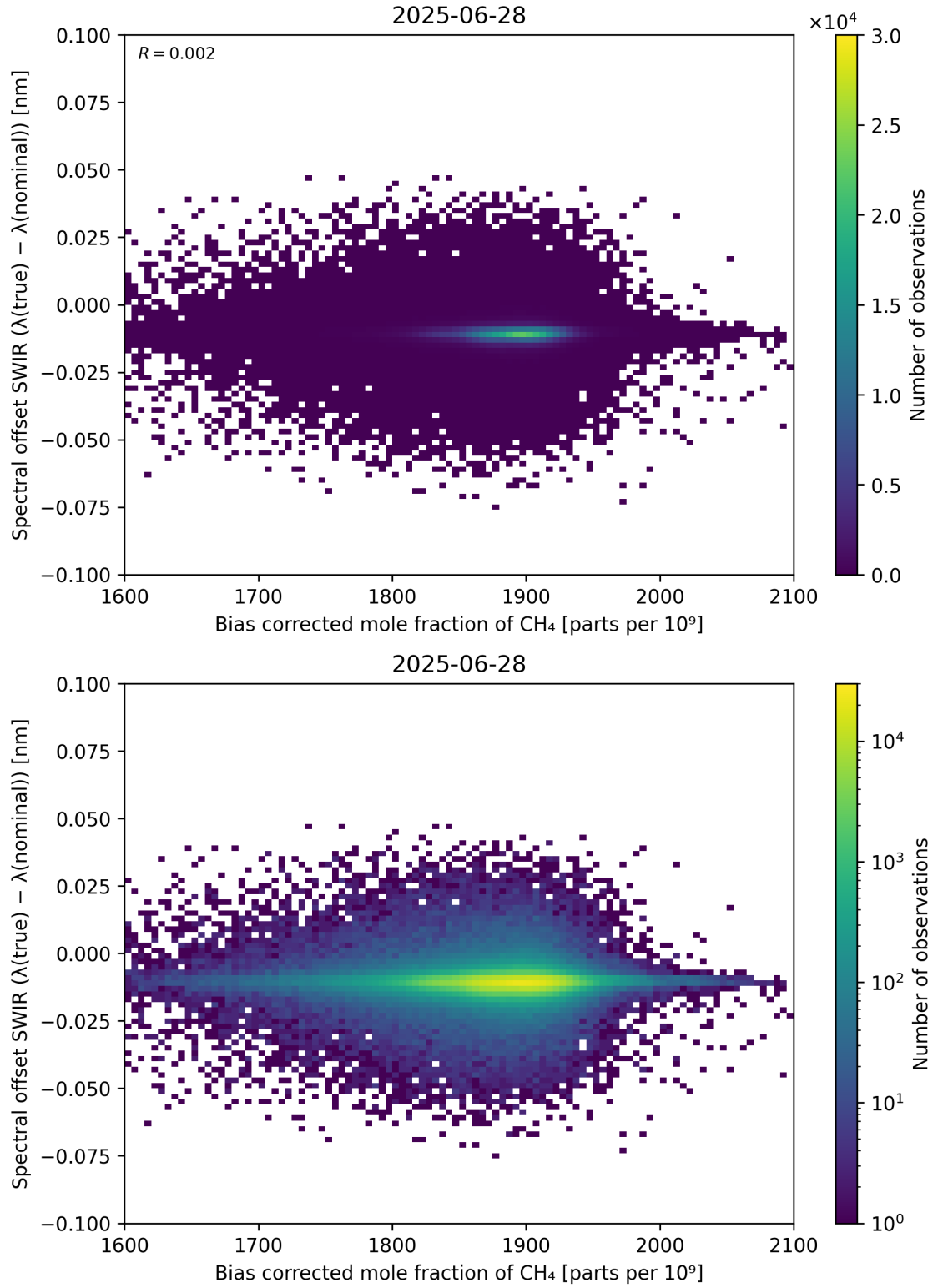
Figure 69: Scatter density plot of “Bias corrected mole fraction of \text{CH}_4 ” against “Spectral offset SWIR ( \lambda_{\text{true}} - \lambda_{\text{nominal}} )” for 2025-06-27 to 2025-06-29.
