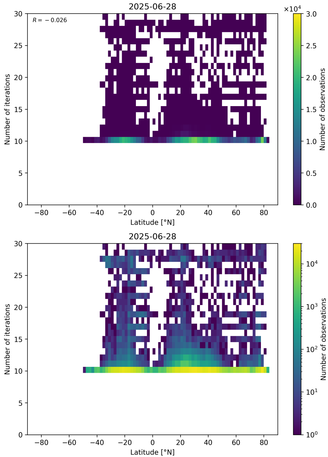
Figure 60: Scatter density plot of “Latitude” against “Number of iterations” for 2025-06-27 to 2025-06-29.
