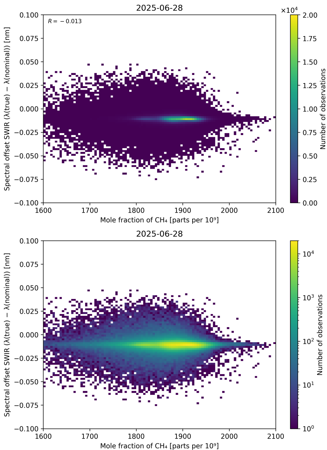
Figure 86: Scatter density plot of “Mole fraction of CH 4 ” against “Spectral offset SWIR ( \lambda_{\text{true}} - \lambda_{\text{nominal}} )” for 2025-06-27 to 2025-06-29.
