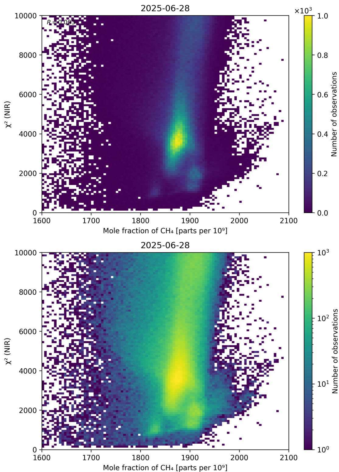
Figure 70: Scatter density plot of “Mole fraction of \text{CH}_4 ” against “ \chi^2 (NIR)” for 2025-06-27 to 2025-06-29.
