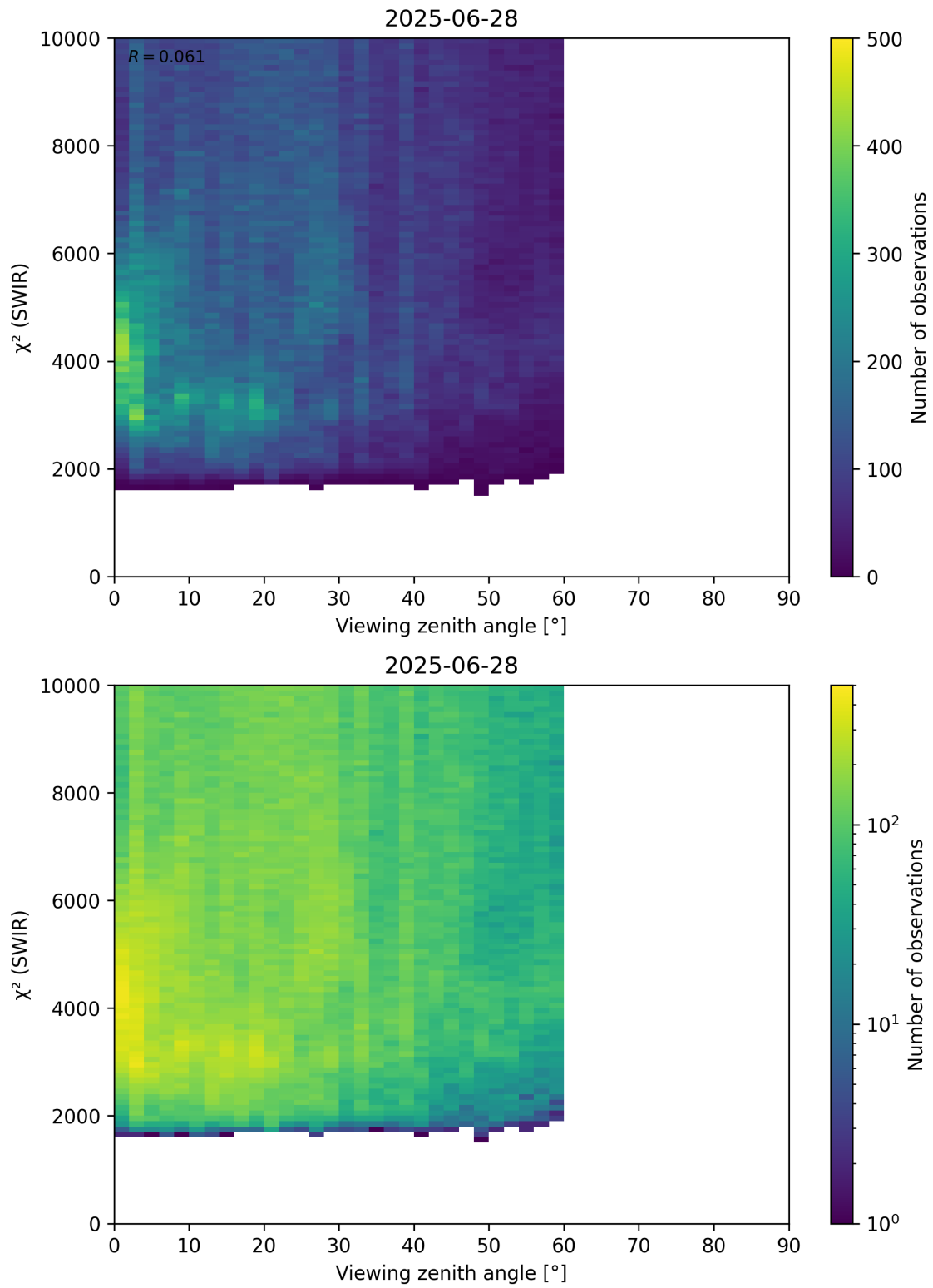
Figure 106: Scatter density plot of “Viewing zenith angle” against “ \chi^2 (SWIR)” for 2025-06-27 to 2025-06-29.
