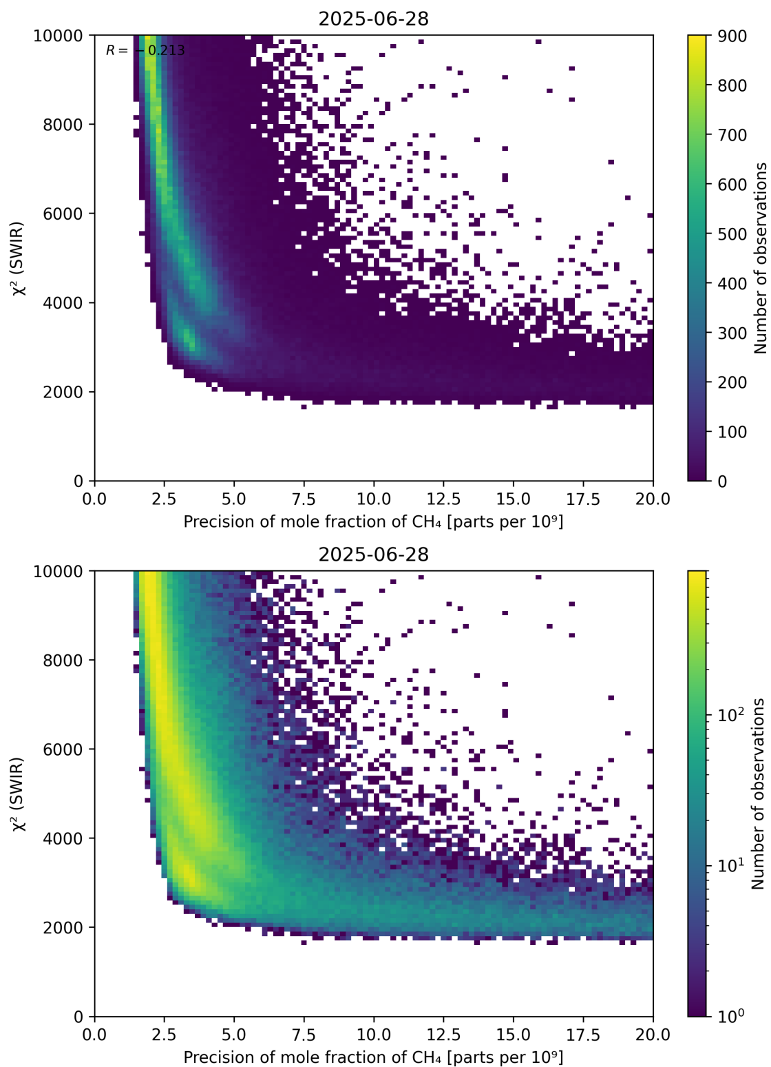
Figure 79: Scatter density plot of “Precision of mole fraction of \text{CH}_4 ” against “ \chi^2 (SWIR)” for 2025-06-27 to 2025-06-29.
