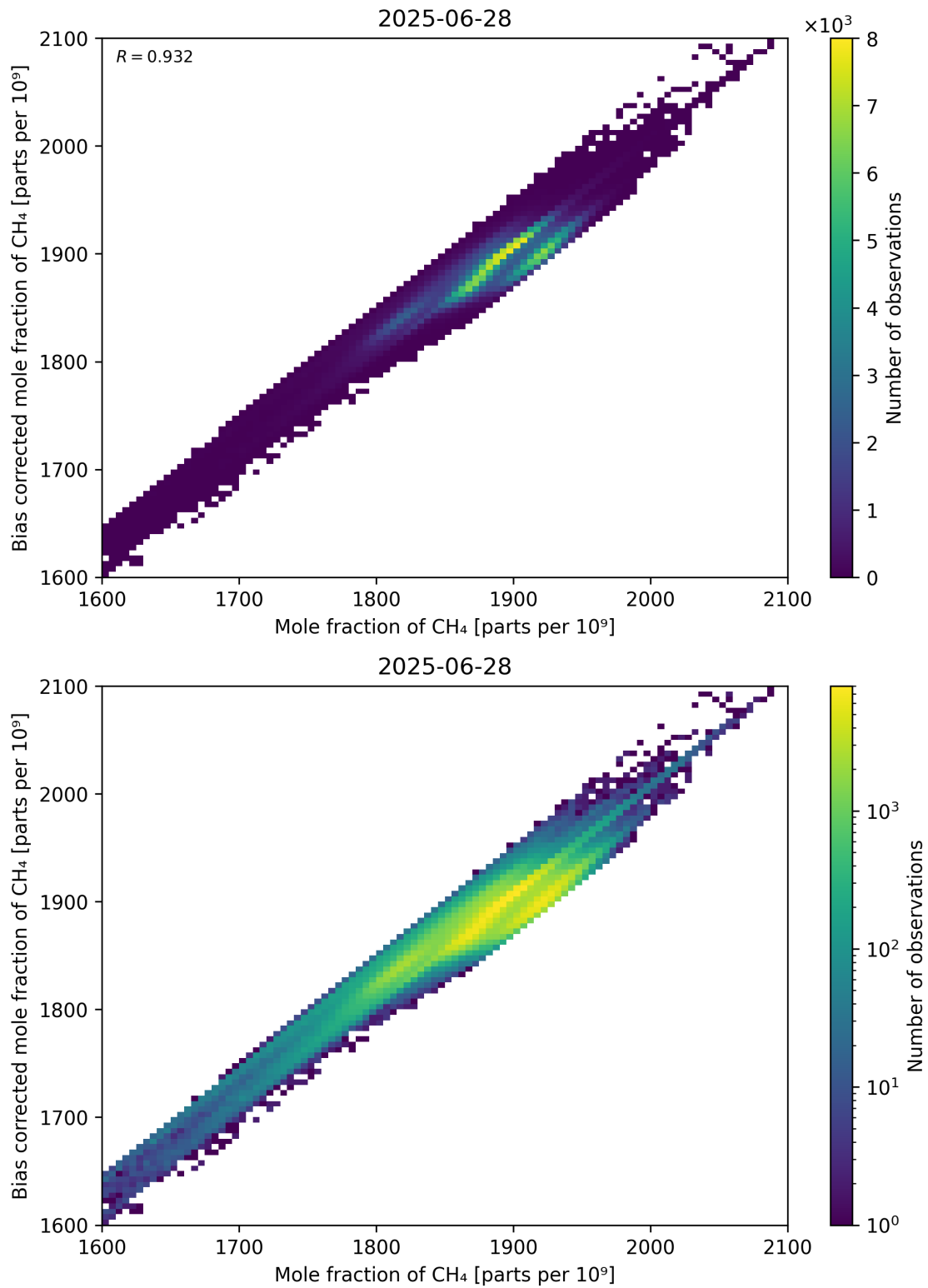
Figure 74: Scatter density plot of “Mole fraction of CH 4 ” against “Bias corrected mole fraction of CH 4 ” for 2025-06-27 to 2025-06-29.
