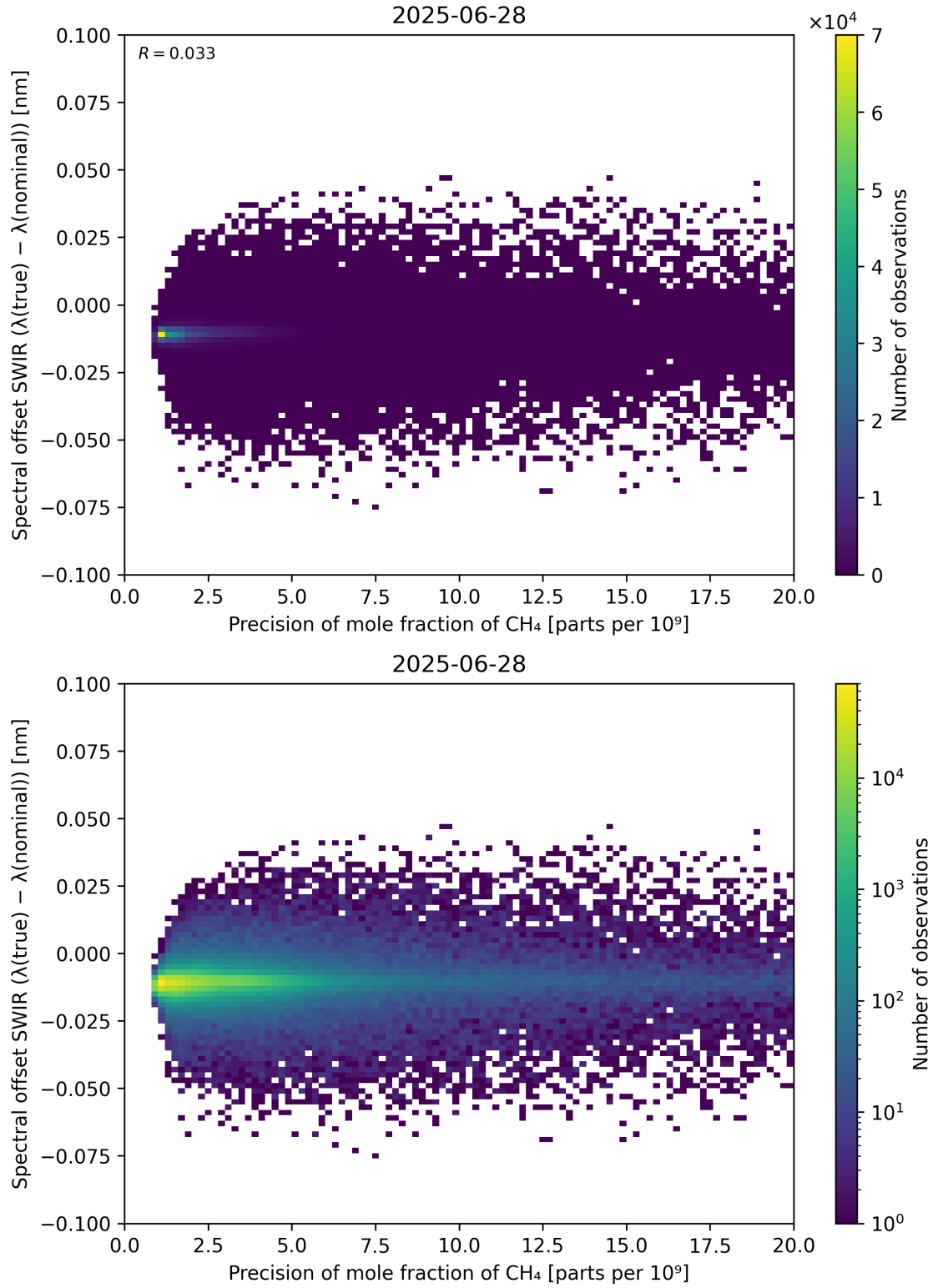
Figure 85: Scatter density plot of “Precision of mole fraction of \text{CH}_4 ” against “Spectral offset SWIR ( \lambda_{\text{true}} - \lambda_{\text{nominal}} )” for 2025-06-27 to 2025-06-29.
