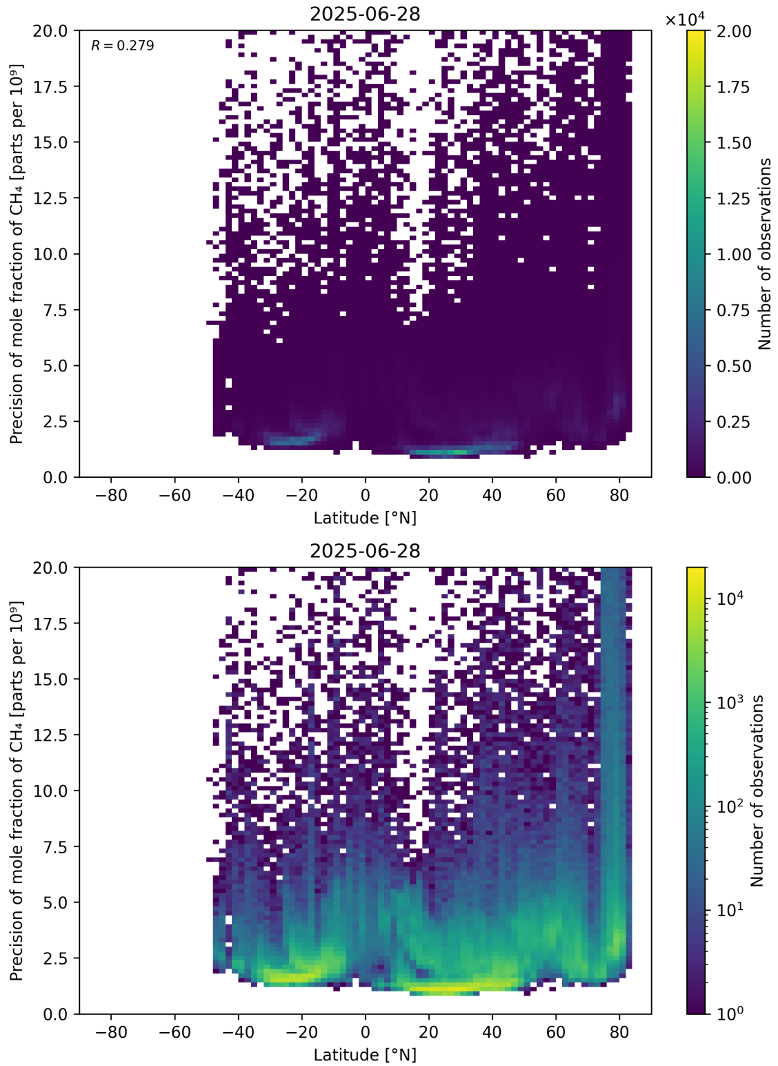
Figure 59: Scatter density plot of “Latitude” against “Precision of mole fraction of \text{CH}_4 ” for 2025-06-27 to 2025-06-29.
