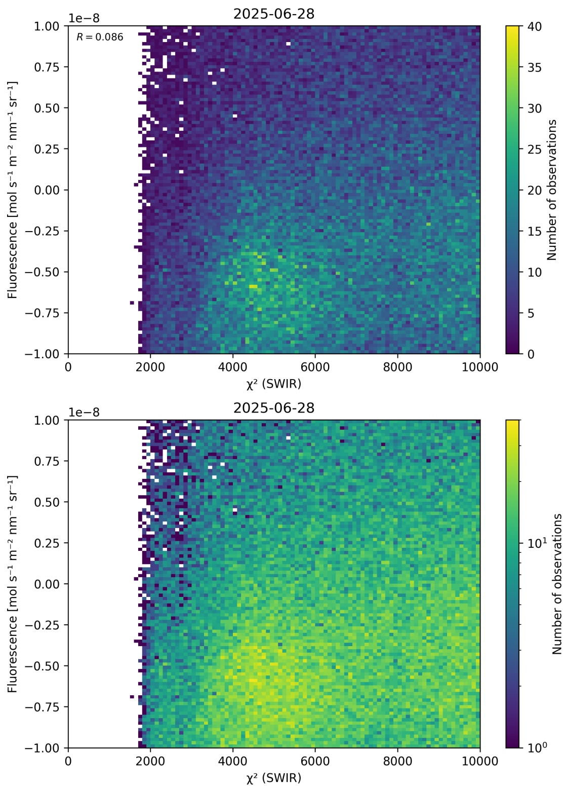
Figure 49: Scatter density plot of “ \chi^2 (SWIR)” against “Fluorescence” for 2025-06-27 to 2025-06-29.
