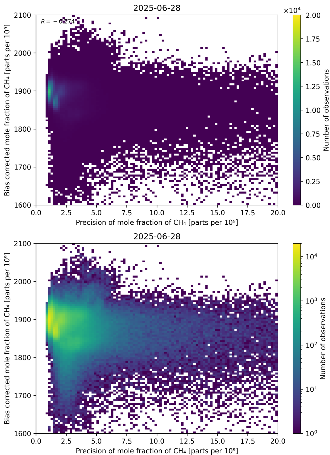
Figure 82: Scatter density plot of “Precision of mole fraction of \text{CH}_4 ” against “Bias corrected mole fraction of \text{CH}_4 ” for 2025-06-27 to 2025-06-29.
