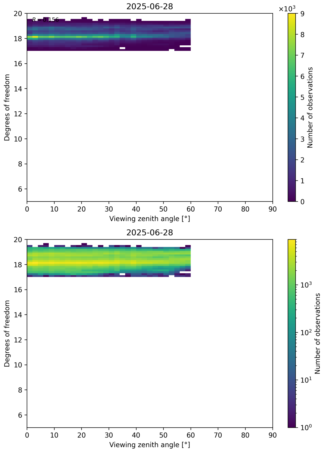
Figure 107: Scatter density plot of “Viewing zenith angle” against “Degrees of freedom” for 2025-06-27 to 2025-06-29.
