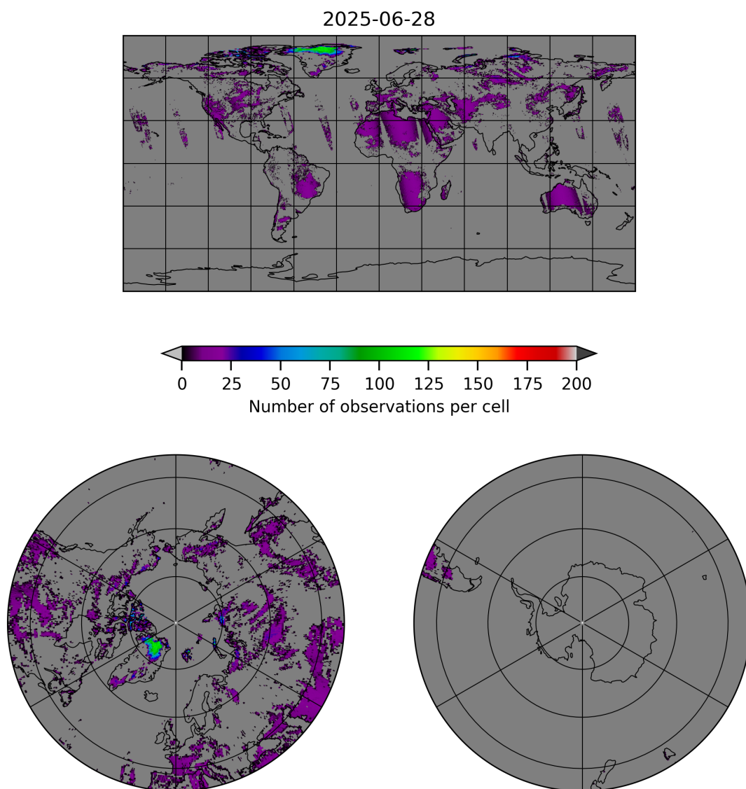
Figure 10: Map of the number of observations for 2025-06-27 to 2025-06-29
