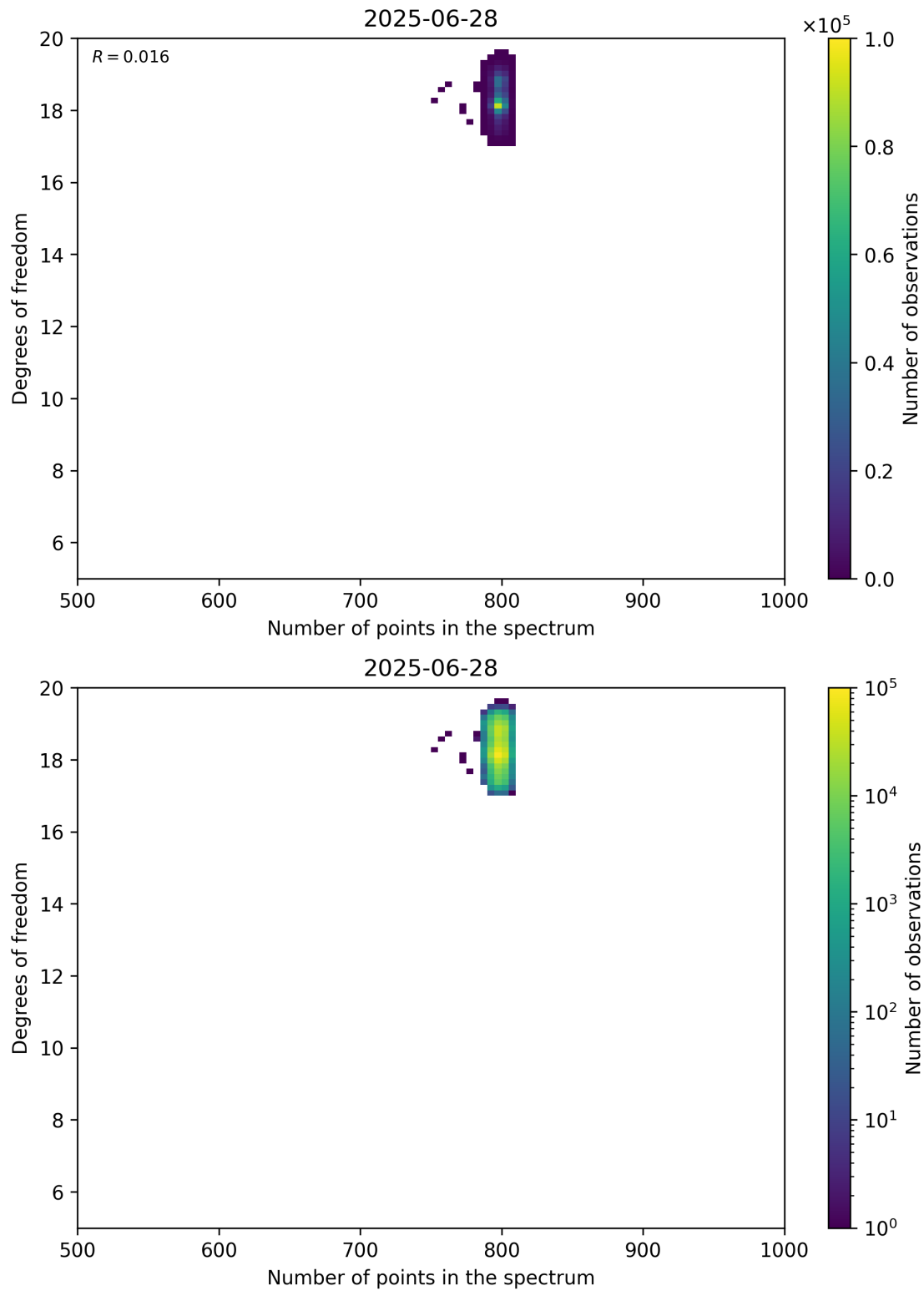
Figure 90: Scatter density plot of “Number of points in the spectrum” against “Degrees of freedom” for 2025-06-27 to 2025-06-29.
