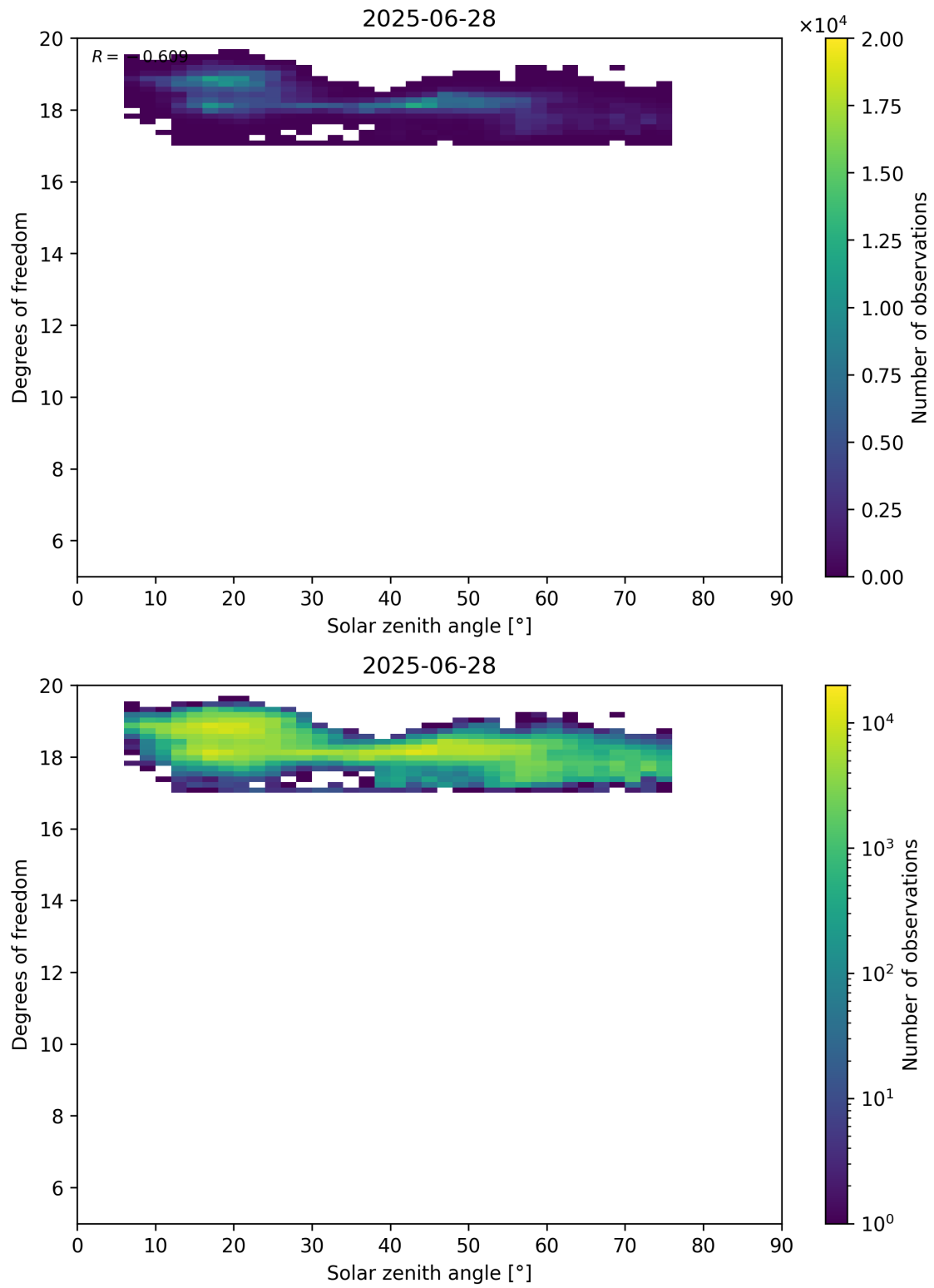
Figure 96: Scatter density plot of “Solar zenith angle” against “Degrees of freedom” for 2025-06-27 to 2025-06-29.
