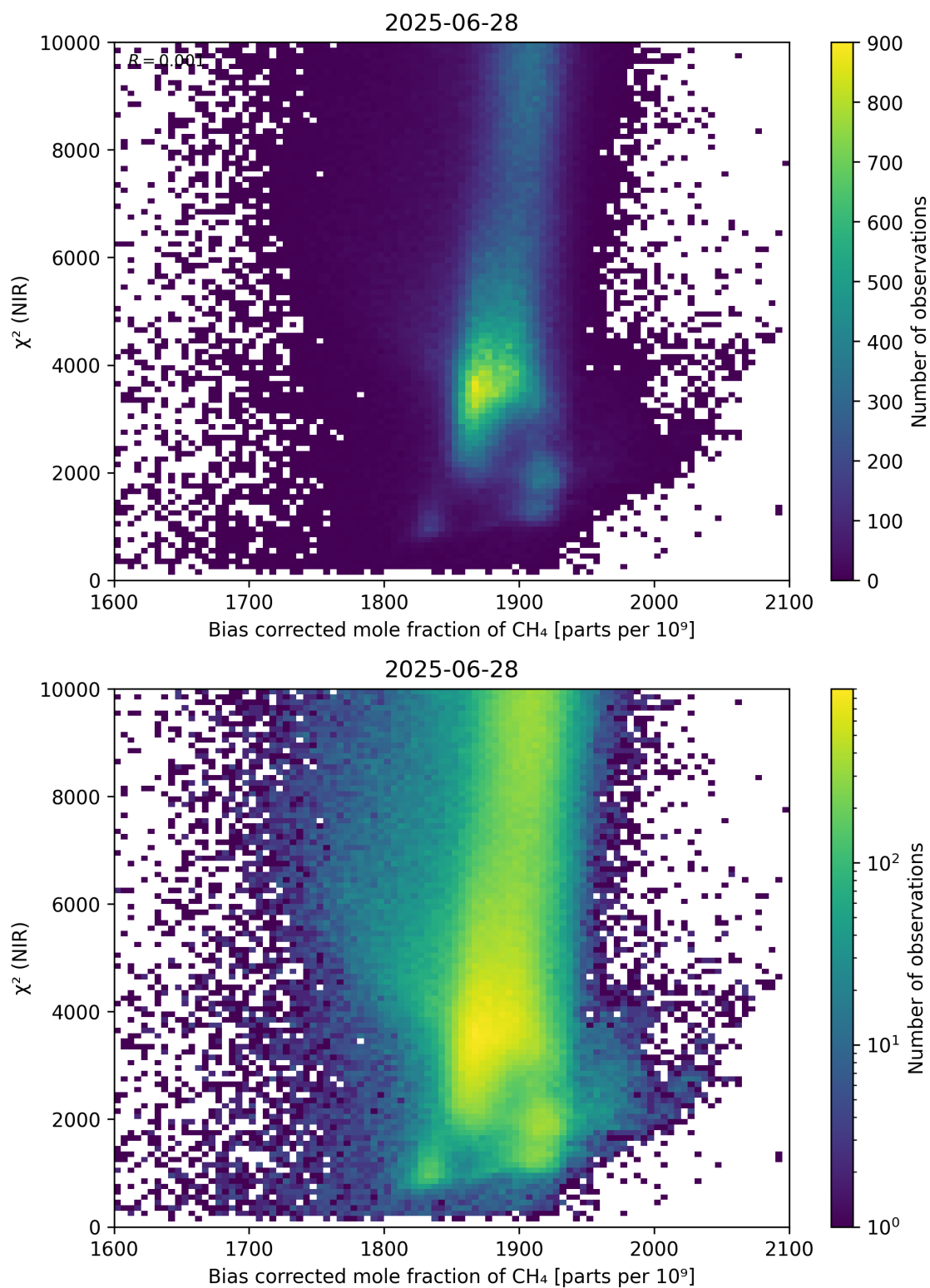
Figure 63: Scatter density plot of “Bias corrected mole fraction of \text{CH}_4 ” against “ \chi^2 (NIR)” for 2025-06-27 to 2025-06-29.
