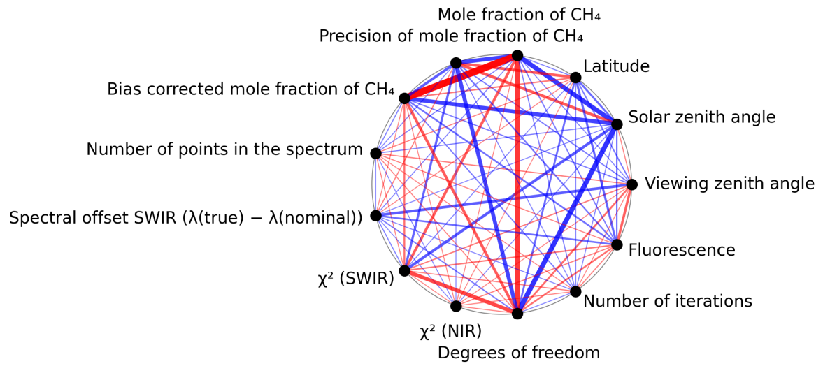
Figure 1: Map of correlation graph for 2025-06-27 to 2025-06-29.
