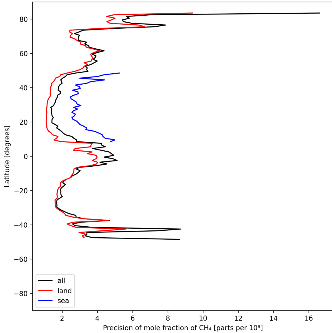
Figure 13: Zonal average of “Precision of mole fraction of CH 4 ” for 2025-06-27 to 2025-06-29.
