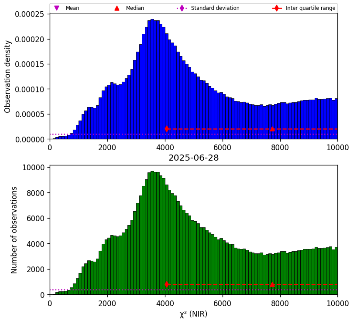
Figure 29: Histogram of “ \chi^2 (NIR)” for 2025-06-27 to 2025-06-29
