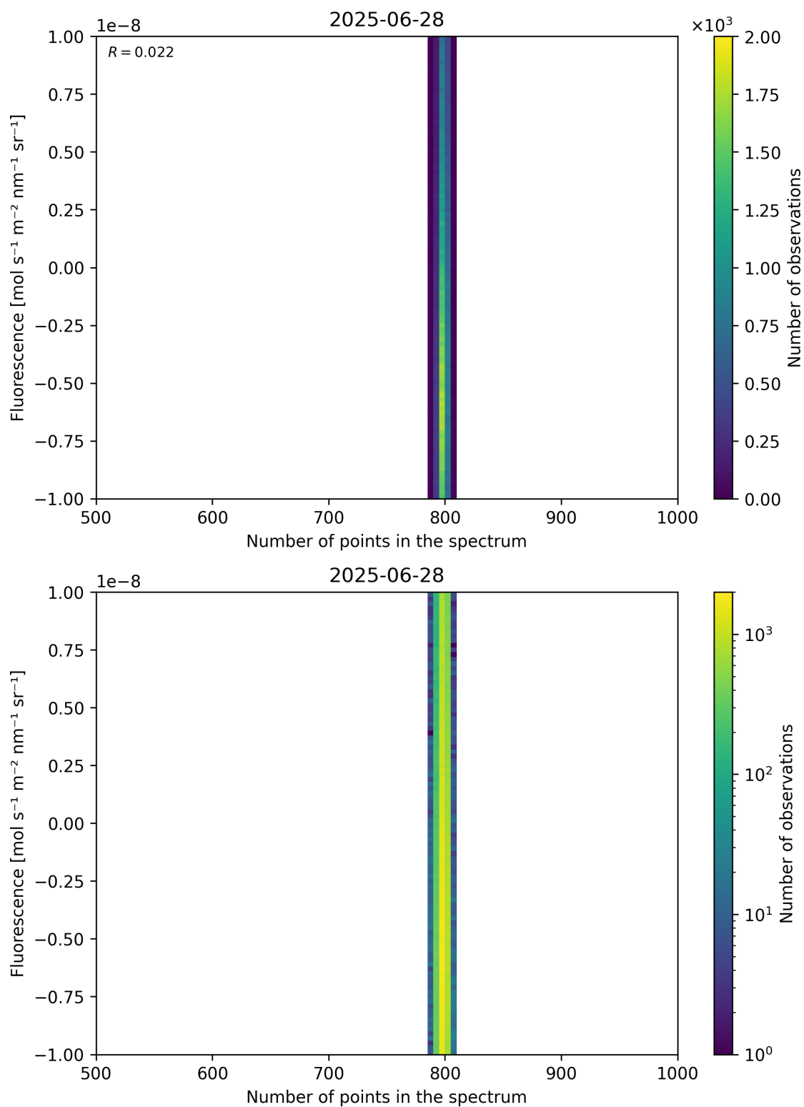
Figure 91: Scatter density plot of “Number of points in the spectrum” against “Fluorescence” for 2025-06-27 to 2025-06-29.
