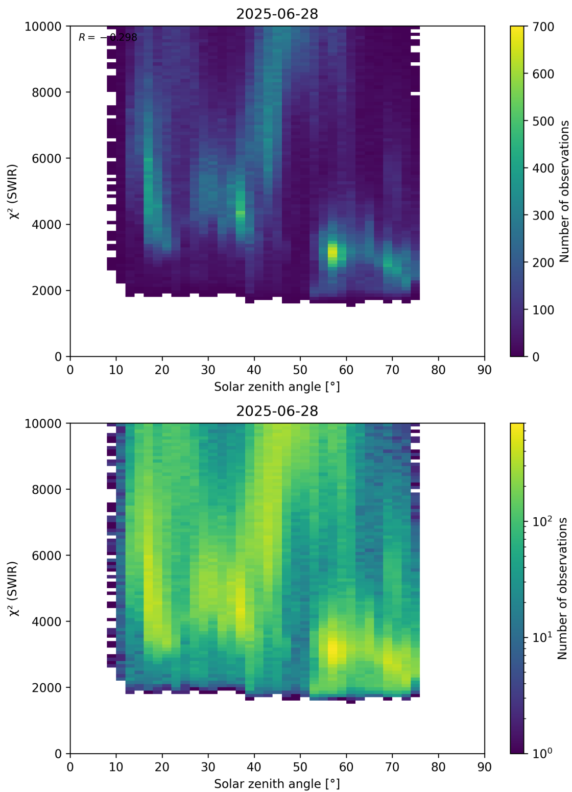
Figure 95: Scatter density plot of “Solar zenith angle” against “ \chi^2 (SWIR)” for 2025-06-27 to 2025-06-29.
