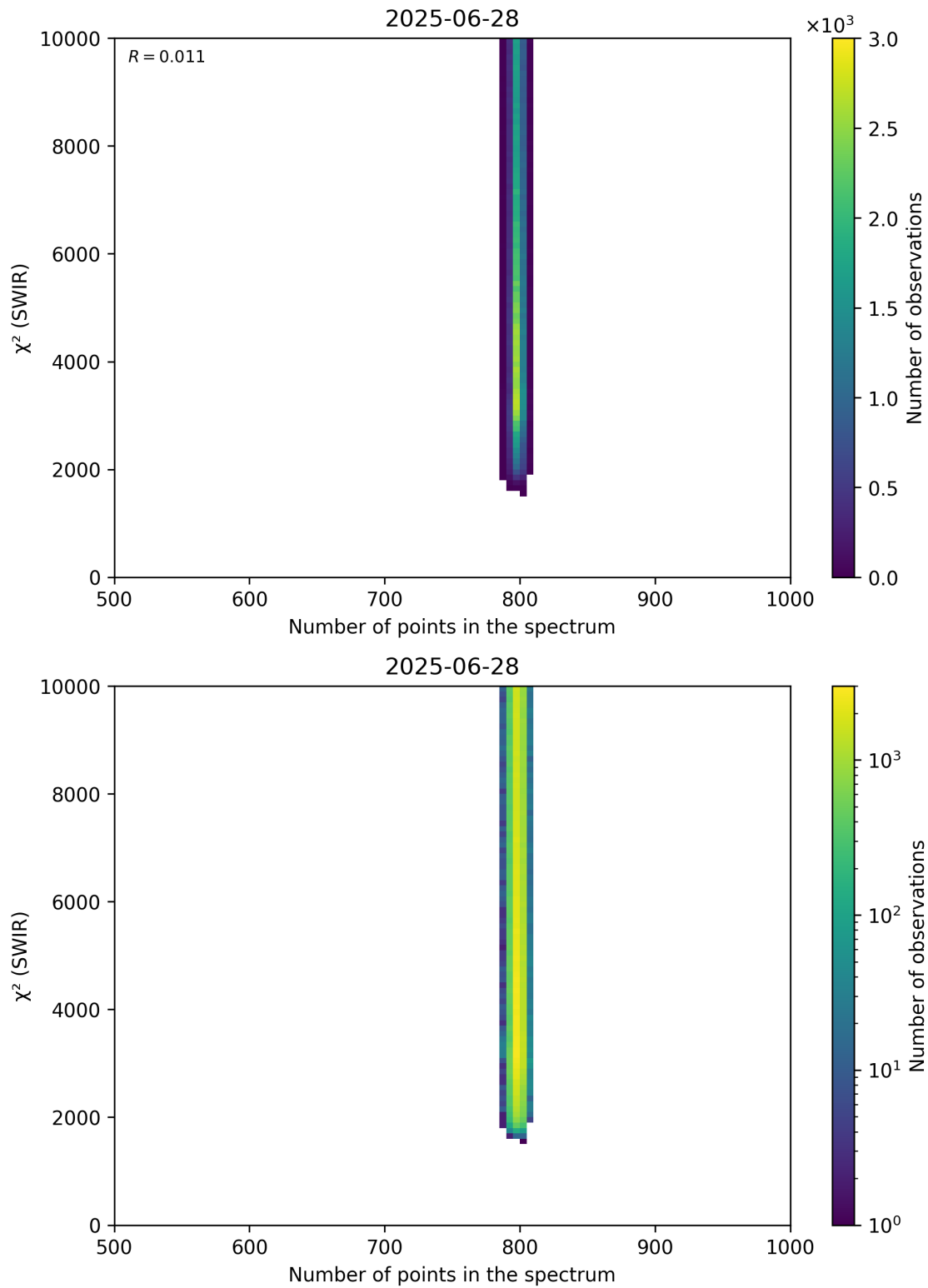
Figure 89: Scatter density plot of “Number of points in the spectrum” against “ \chi^2 (SWIR)” for 2025-06-27 to 2025-06-29.
