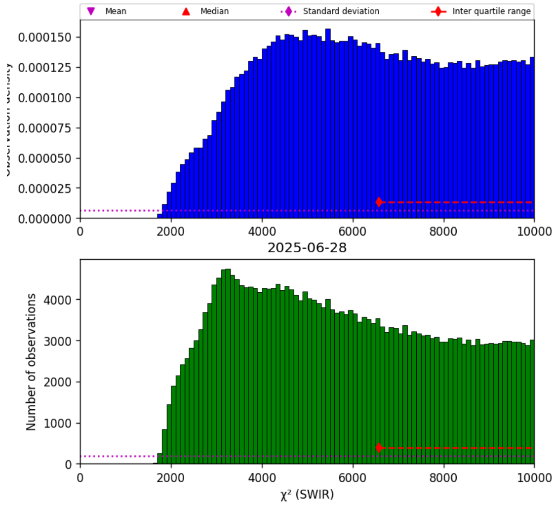
Figure 28: Histogram of “ \chi^2 (SWIR)” for 2025-06-27 to 2025-06-29
