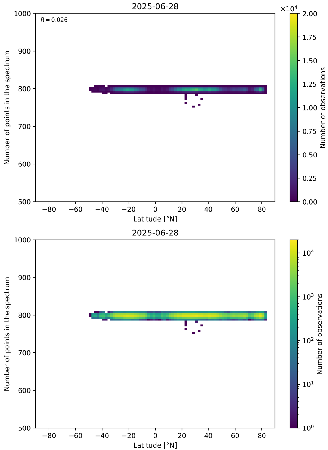
Figure 61: Scatter density plot of “Latitude” against “Number of points in the spectrum” for 2025-06-27 to 2025-06-29.
