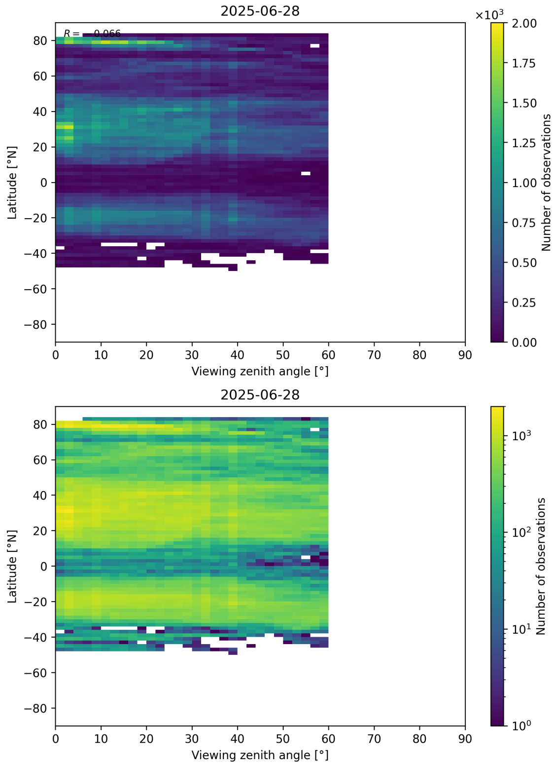
Figure 109: Scatter density plot of “Viewing zenith angle” against “Latitude” for 2025-06-27 to 2025-06-29.
