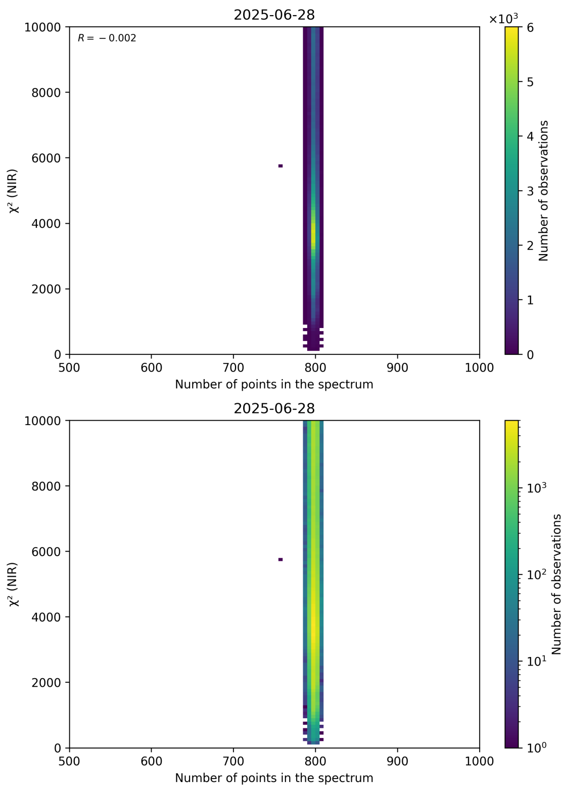
Figure 88: Scatter density plot of “Number of points in the spectrum” against “ \chi^2 (NIR)” for 2025-06-27 to 2025-06-29.
