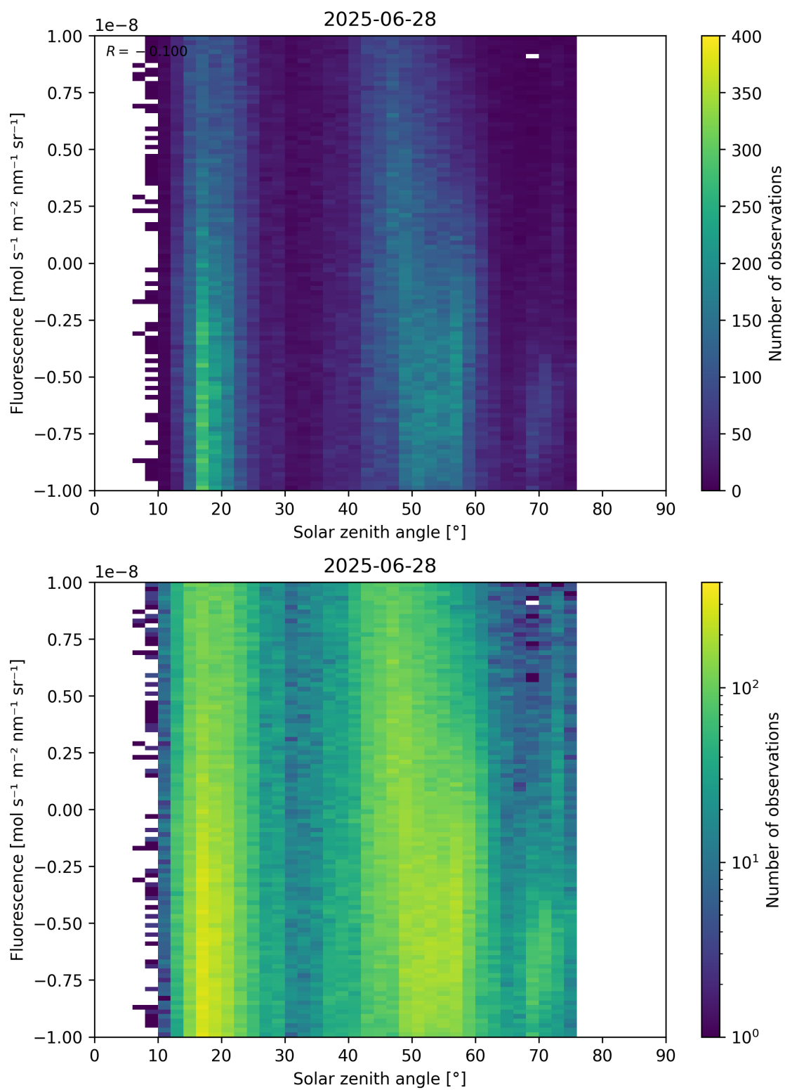
Figure 97: Scatter density plot of “Solar zenith angle” against “Fluorescence” for 2025-06-27 to 2025-06-29.
