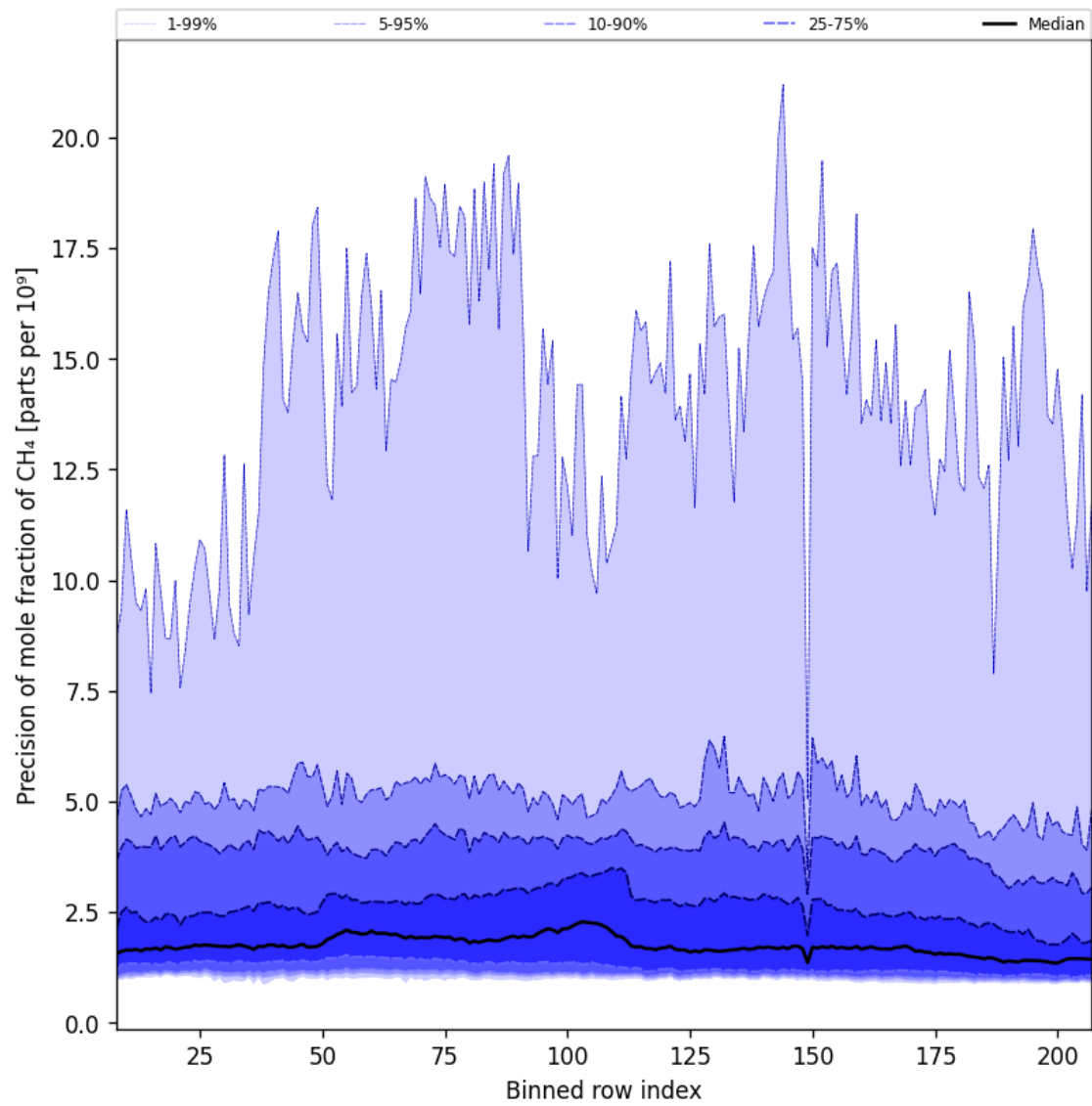
Figure 35: Along track statistics of “Precision of mole fraction of CH 4 ” for 2025-06-27 to 2025-06-29
