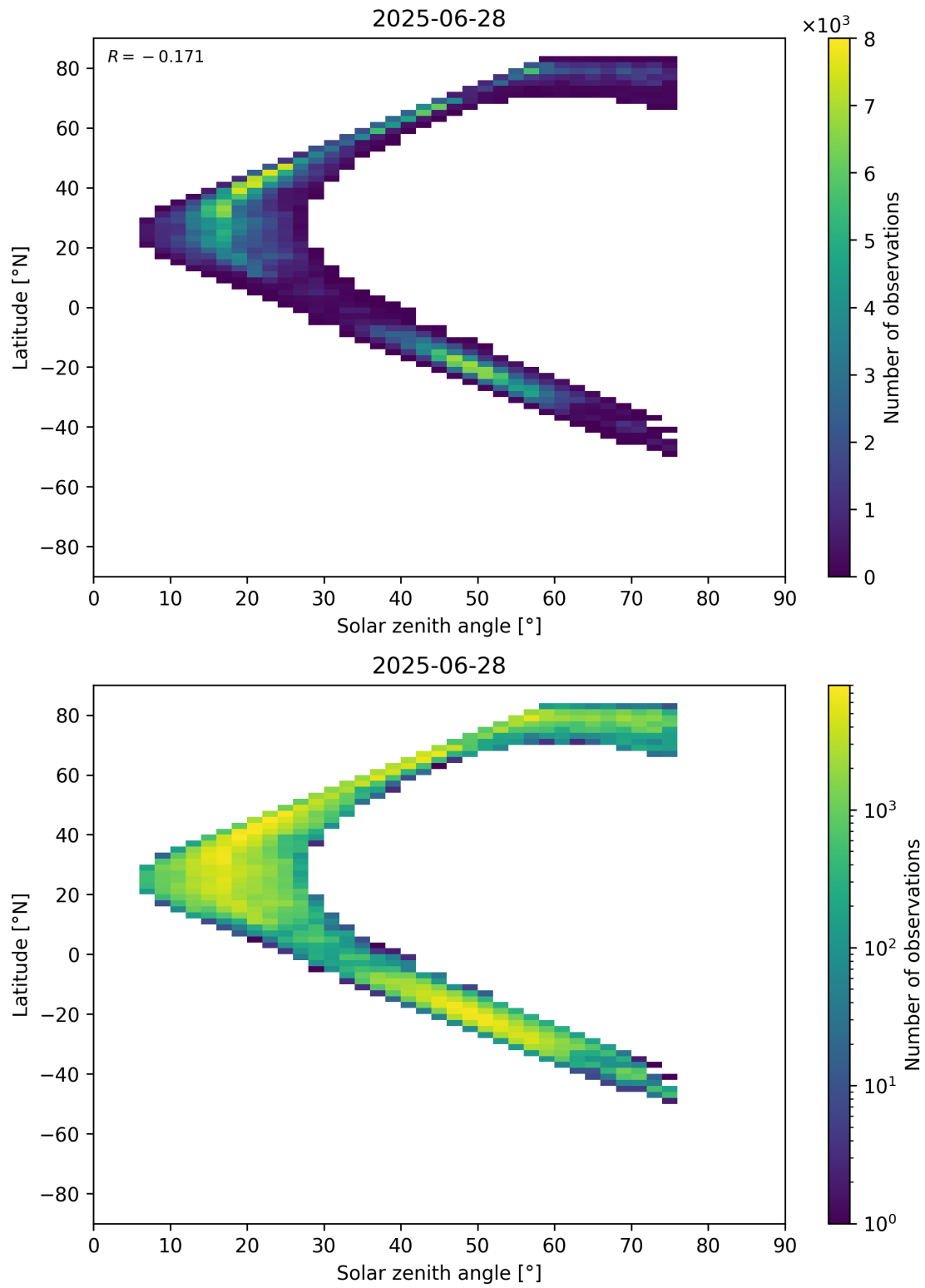
Figure 98: Scatter density plot of “Solar zenith angle” against “Latitude” for 2025-06-27 to 2025-06-29.
