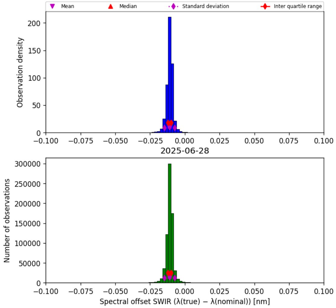
Figure 27: Histogram of “Spectral offset SWIR ( \lambda_{\text{true}} - \lambda_{\text{nominal}} )” for 2025-06-27 to 2025-06-29
