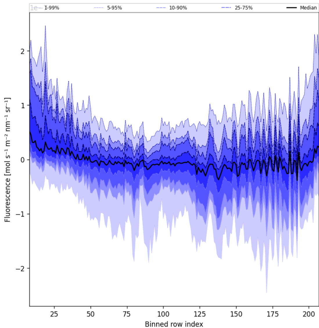
Figure 43: Along track statistics of “Fluorescence” for 2025-06-27 to 2025-06-29
