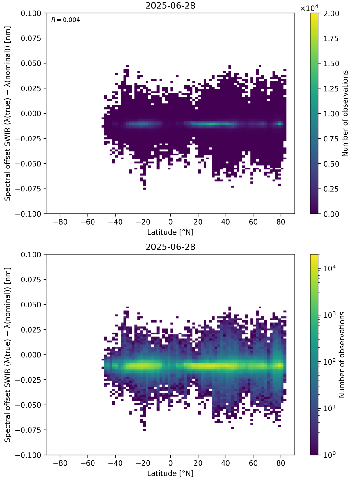
Figure 62: Scatter density plot of “Latitude” against “Spectral offset SWIR ( \lambda_{\text{true}} - \lambda_{\text{nominal}} )” for 2025-06-27 to 2025-06-29.
