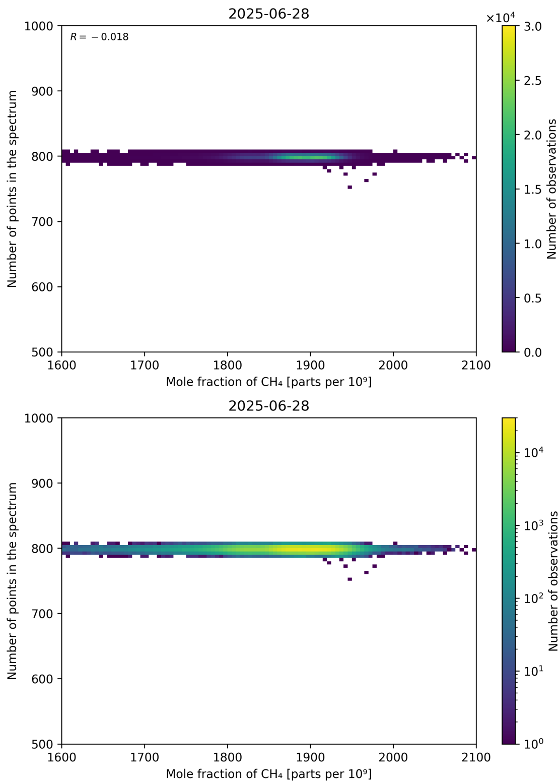
Figure 77: Scatter density plot of “Mole fraction of CH 4 ” against “Number of points in the spectrum” for 2025-06-27 to 2025-06-29.
