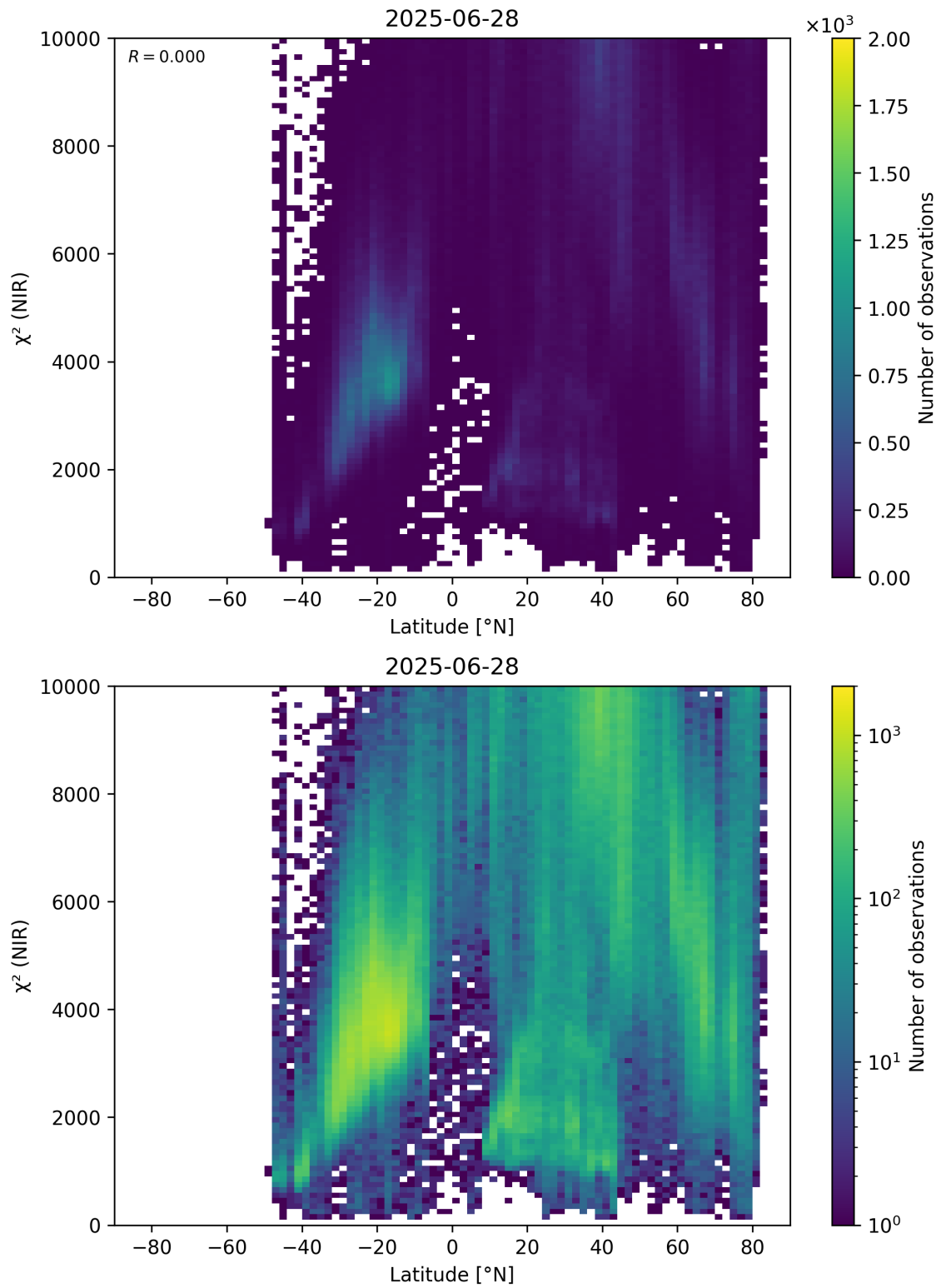
Figure 53: Scatter density plot of “Latitude” against “ \chi^2 (NIR)” for 2025-06-27 to 2025-06-29.
