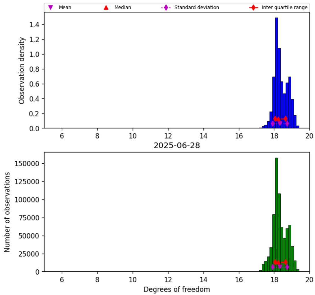
Figure 30: Histogram of “Degrees of freedom” for 2025-06-27 to 2025-06-29
