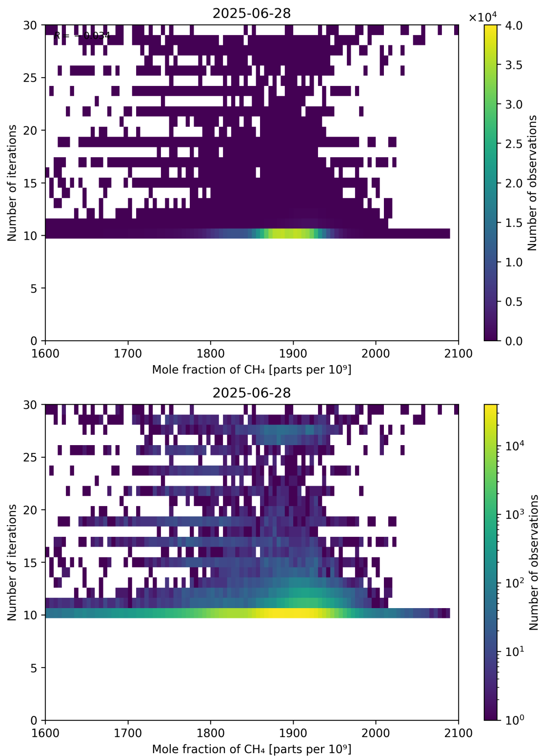
Figure 76: Scatter density plot of “Mole fraction of CH 4 ” against “Number of iterations” for 2025-06-27 to 2025-06-29.
