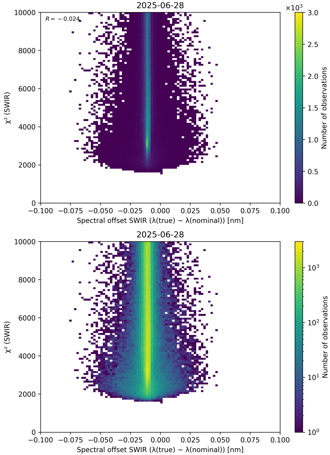
Figure 118: Scatter density plot of “Spectral offset SWIR ( \lambda_{\text{true}} - \lambda_{\text{nominal}} )” against “ \chi^2 (SWIR)” for 2025-06-27 to 2025-06-29.
