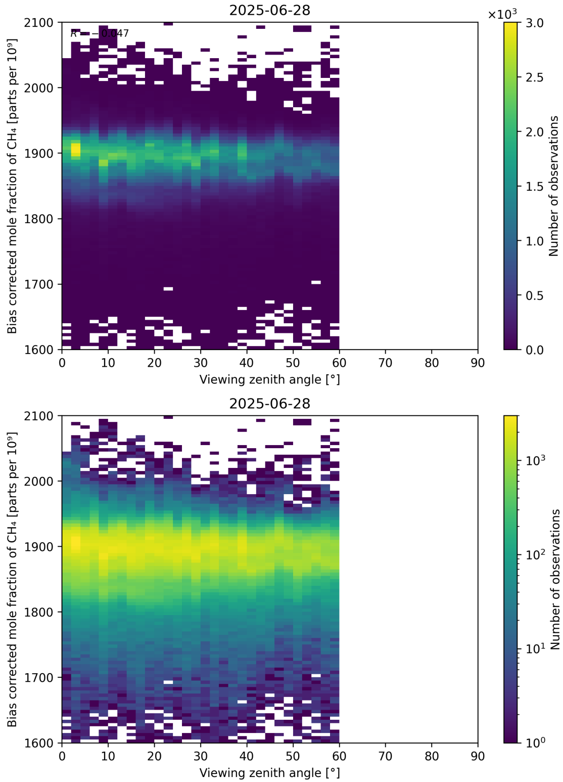
Figure 111: Scatter density plot of “Viewing zenith angle” against “Bias corrected mole fraction of CH 4 ” for 2025-06-27 to 2025-06-29.
