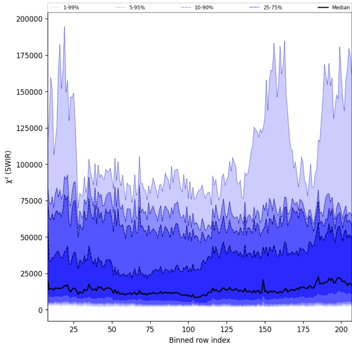
Figure 39: Along track statistics of “ \chi^2 (SWIR)” for 2025-06-27 to 2025-06-29
