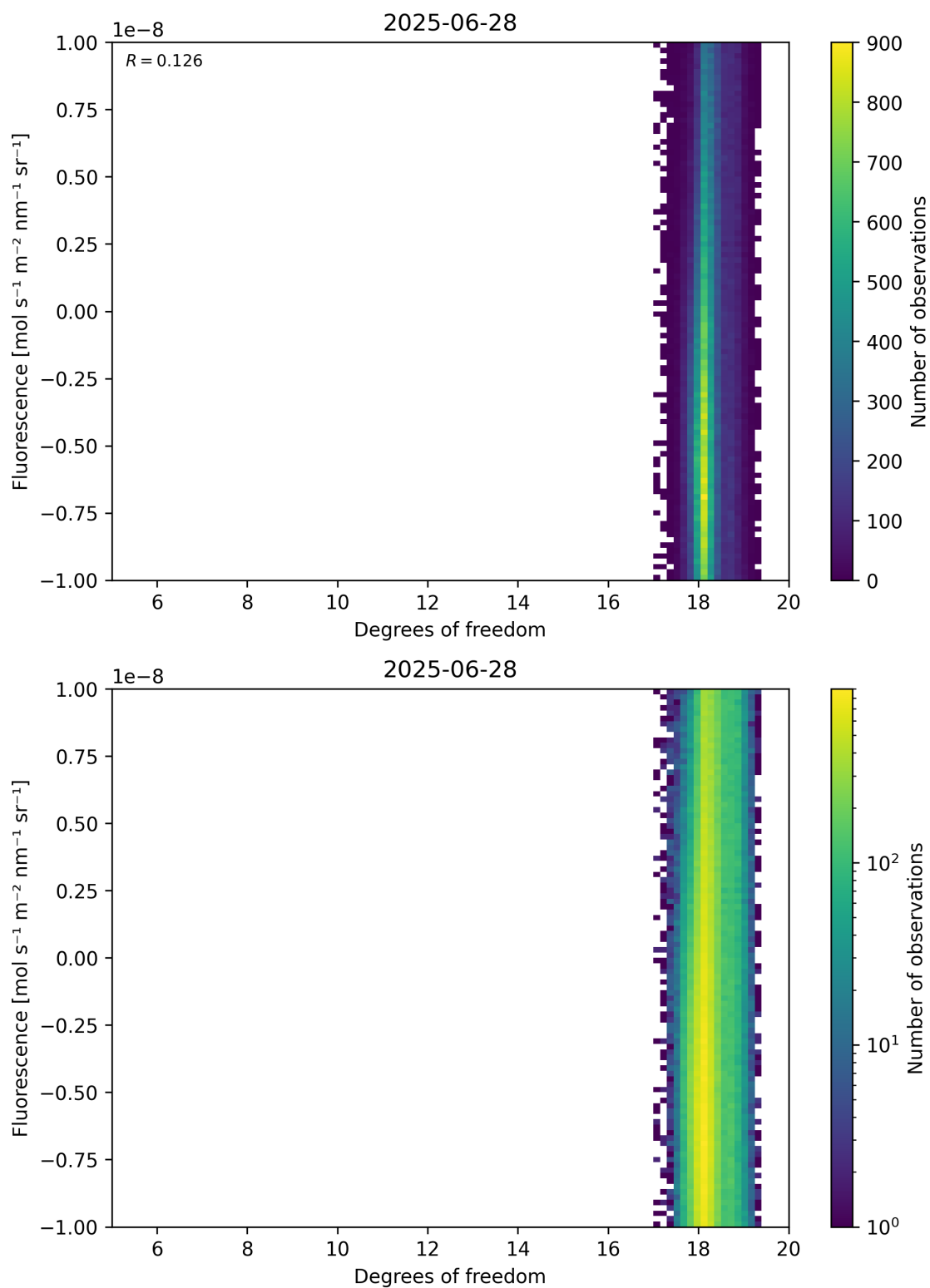
Figure 51: Scatter density plot of “Degrees of freedom” against “Fluorescence” for 2025-06-27 to 2025-06-29.
