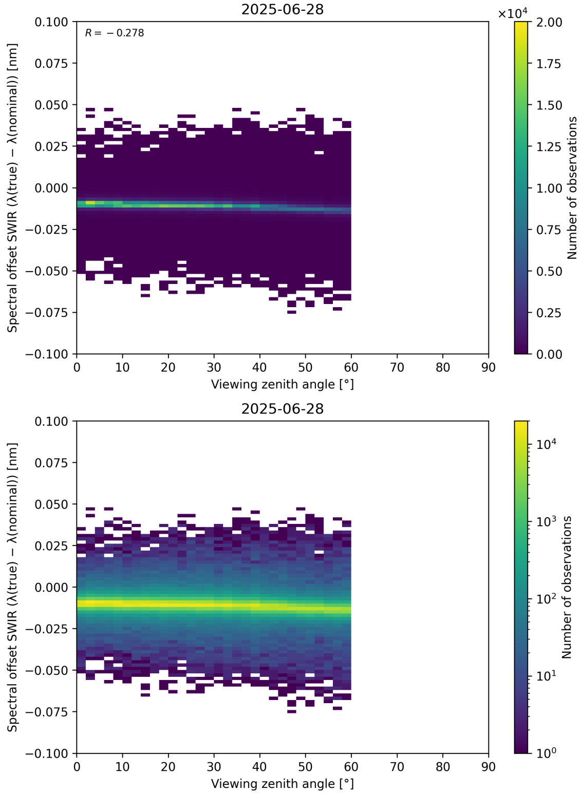
Figure 116: Scatter density plot of “Viewing zenith angle” against “Spectral offset SWIR ( \lambda_{\text{true}} - \lambda_{\text{nominal}} )” for 2025-06-27 to 2025-06-29.
