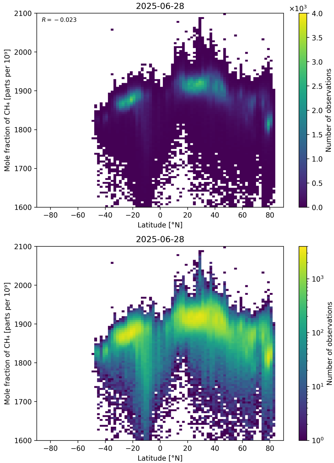
Figure 57: Scatter density plot of “Latitude” against “Mole fraction of CH 4 ” for 2025-06-27 to 2025-06-29.
