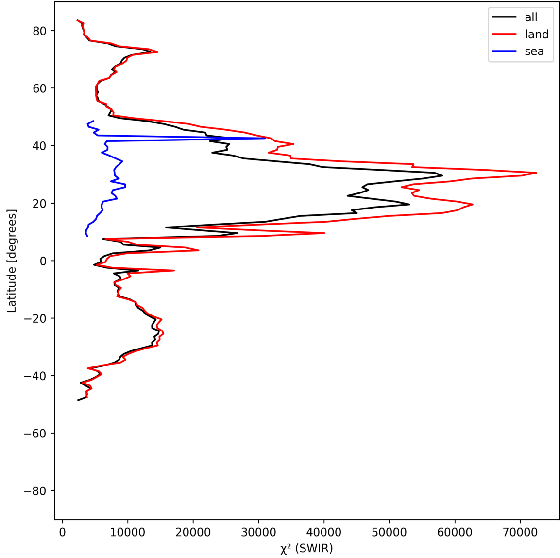
Figure 17: Zonal average of “ \chi^2 (SWIR)” for 2025-06-27 to 2025-06-29.
