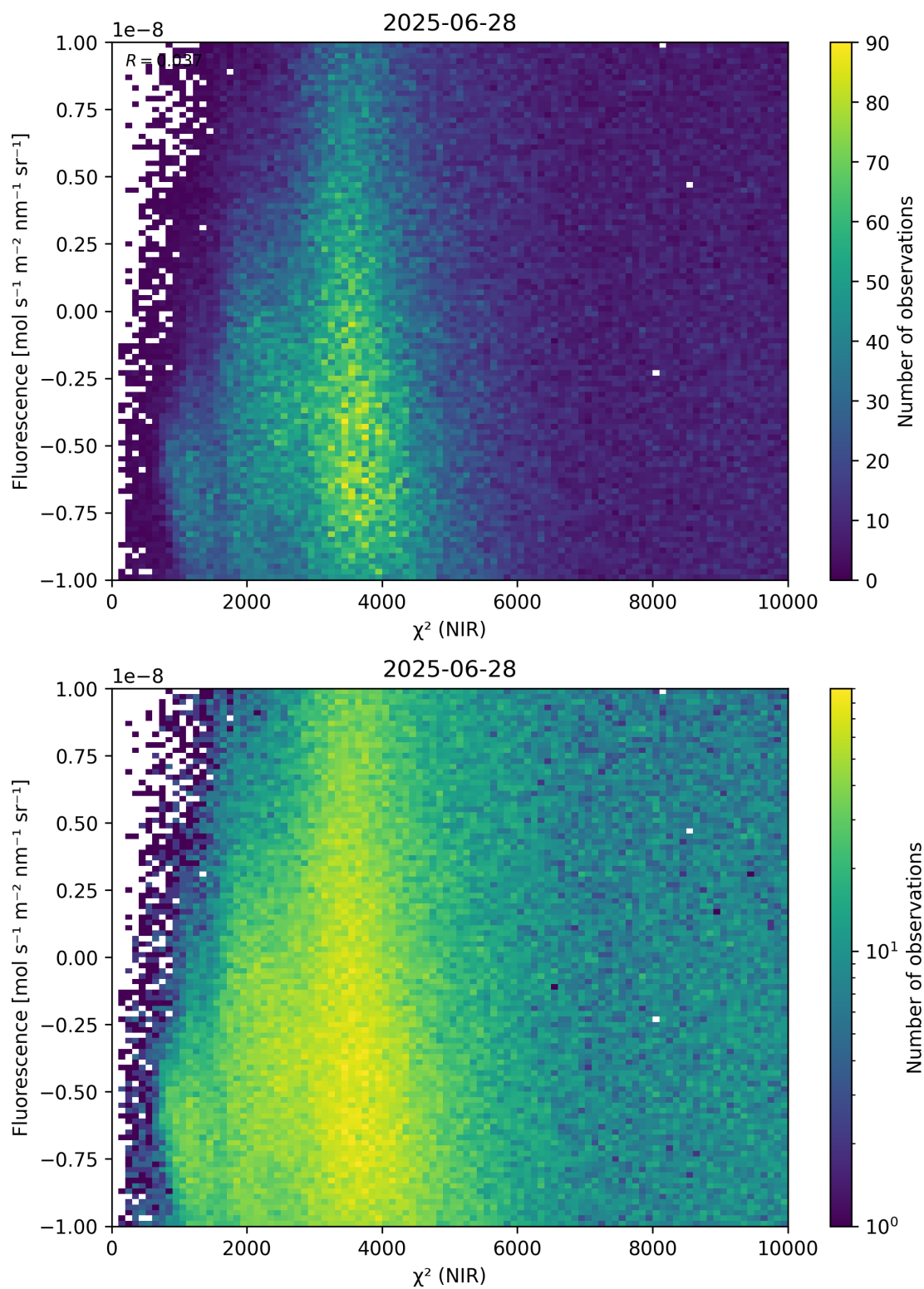
Figure 45: Scatter density plot of “ \chi^2 (NIR)” against “Fluorescence” for 2025-06-27 to 2025-06-29.
