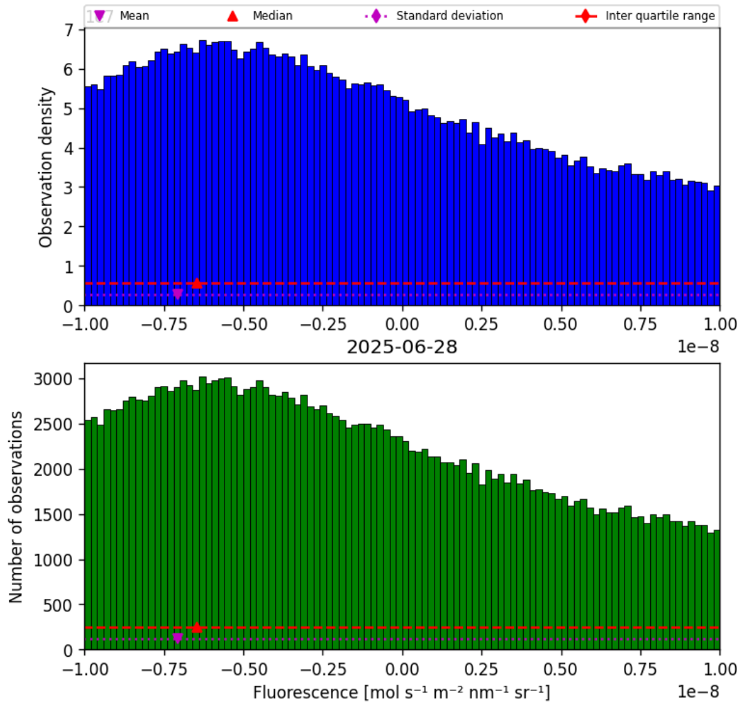
Figure 32: Histogram of “Fluorescence” for 2025-06-27 to 2025-06-29
