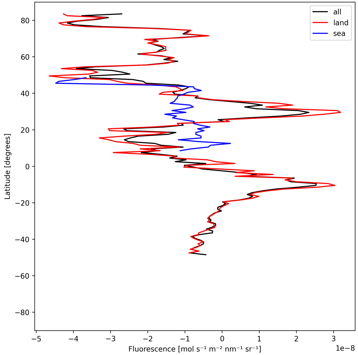
Figure 21: Zonal average of “Fluorescence” for 2025-06-27 to 2025-06-29.
