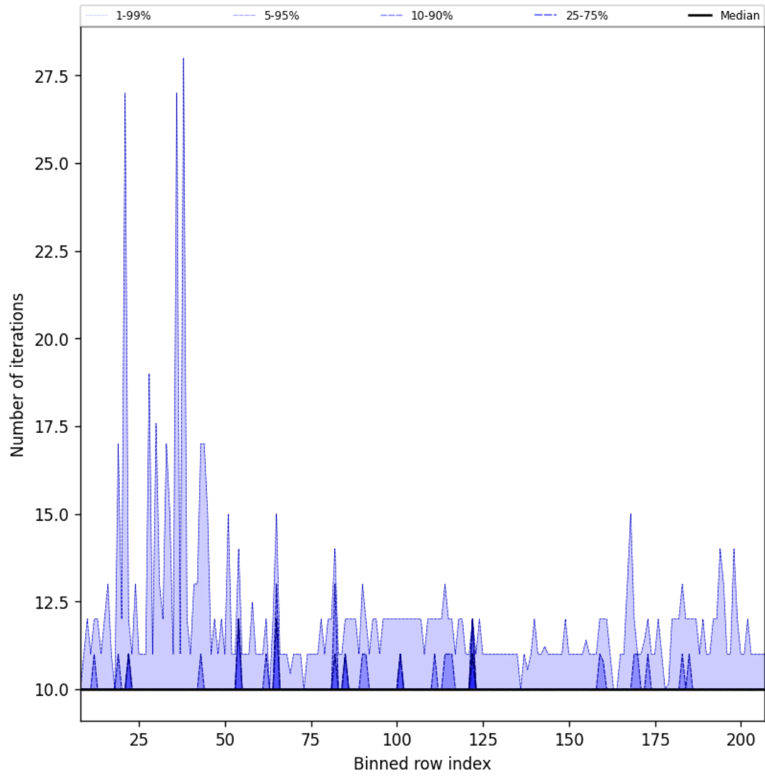
Figure 42: Along track statistics of “Number of iterations” for 2025-06-27 to 2025-06-29
