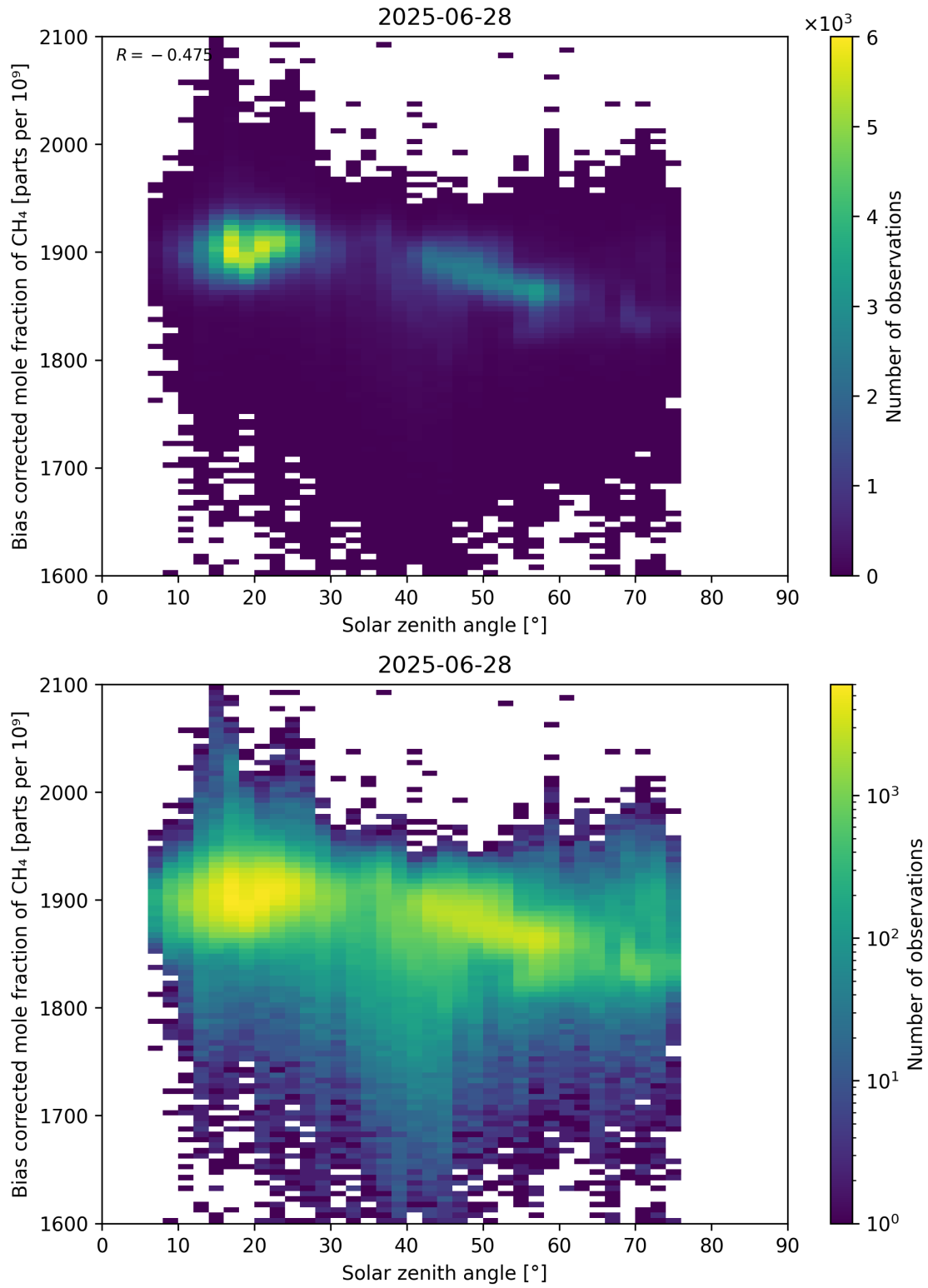
Figure 100: Scatter density plot of “Solar zenith angle” against “Bias corrected mole fraction of CH 4 ” for 2025-06-27 to 2025-06-29.
