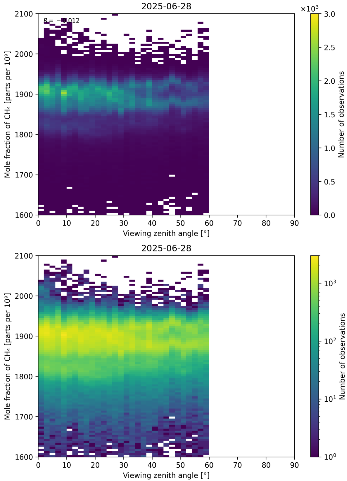
Figure 110: Scatter density plot of “Viewing zenith angle” against “Mole fraction of CH 4 ” for 2025-06-27 to 2025-06-29.
