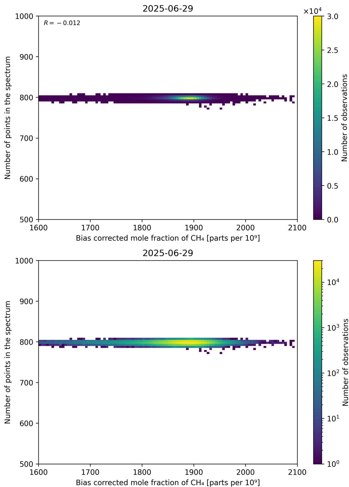
Figure 68: Scatter density plot of “Bias corrected mole fraction of CH 4 ” against “Number of points in the spectrum” for 2025-06-28 to 2025-06-30.
