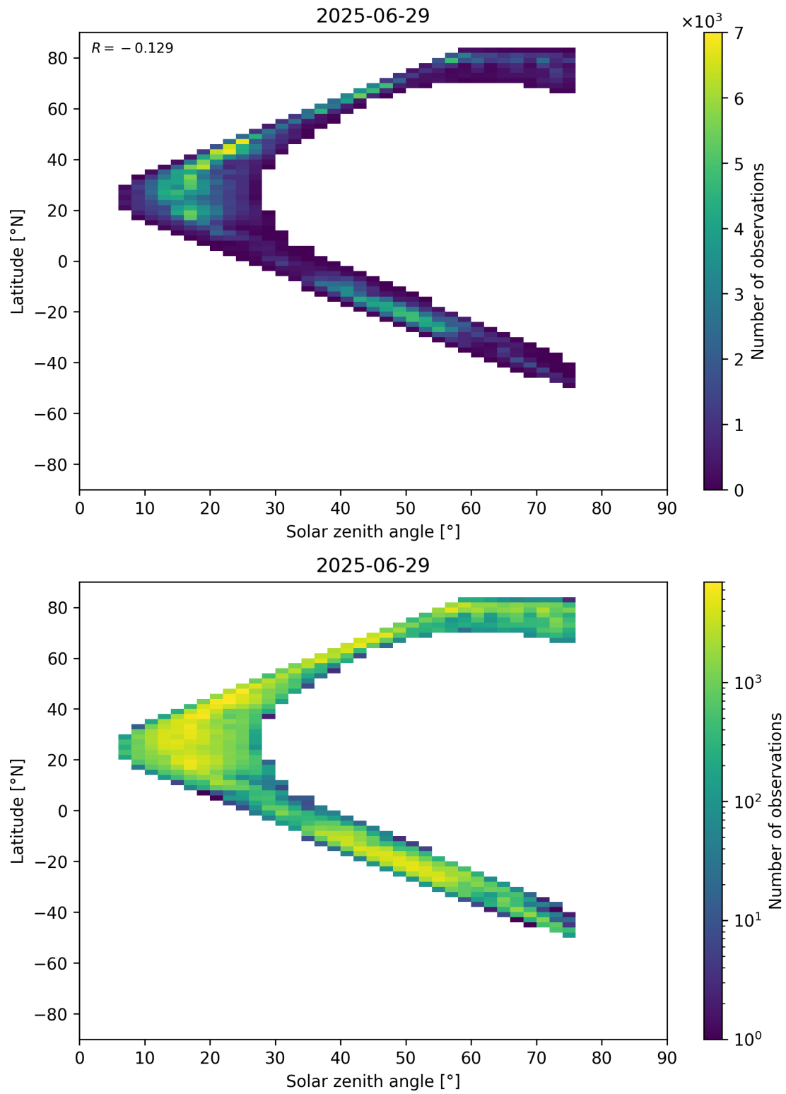
Figure 98: Scatter density plot of “Solar zenith angle” against “Latitude” for 2025-06-28 to 2025-06-30.
