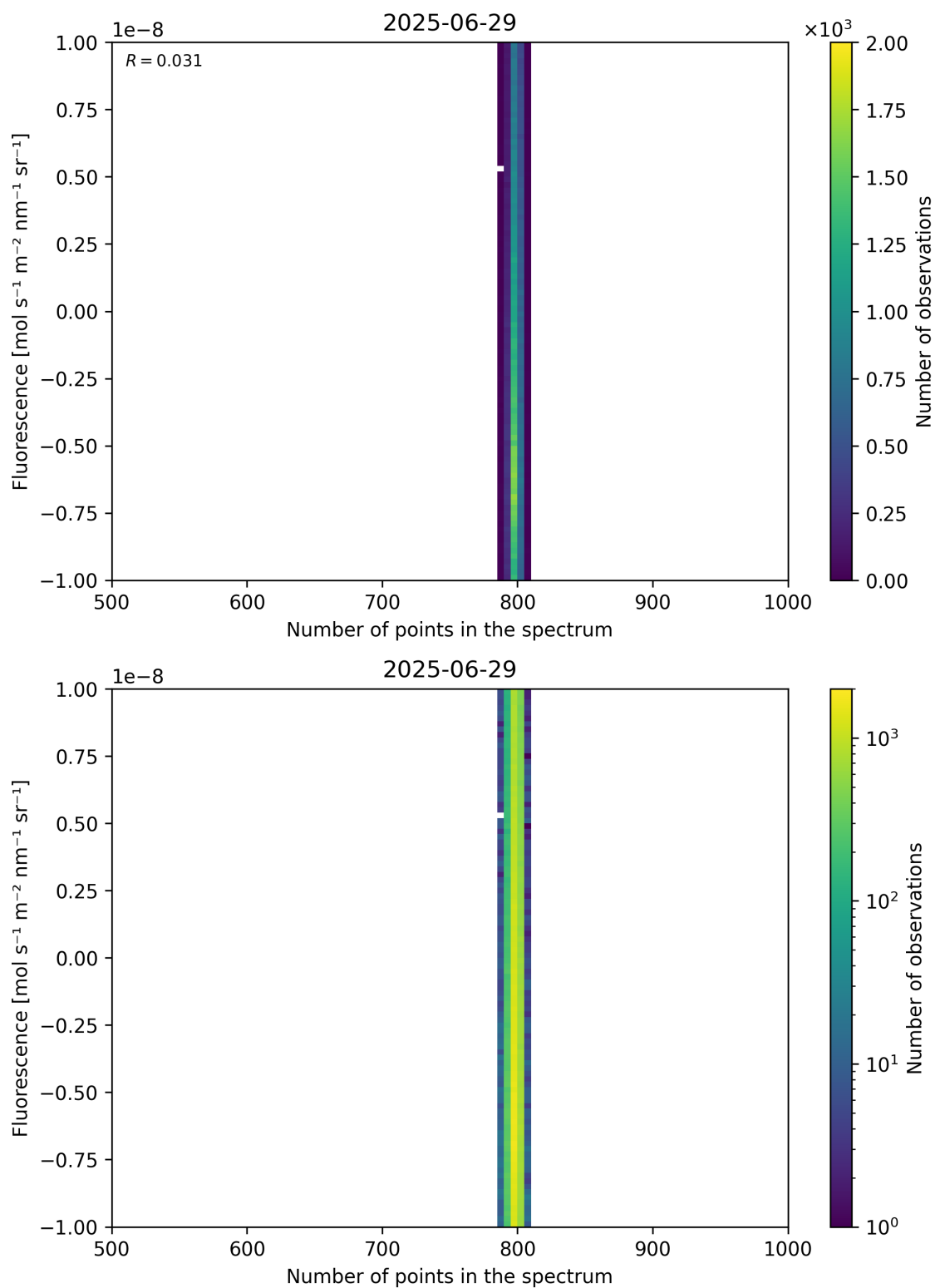
Figure 91: Scatter density plot of “Number of points in the spectrum” against “Fluorescence” for 2025-06-28 to 2025-06-30.
