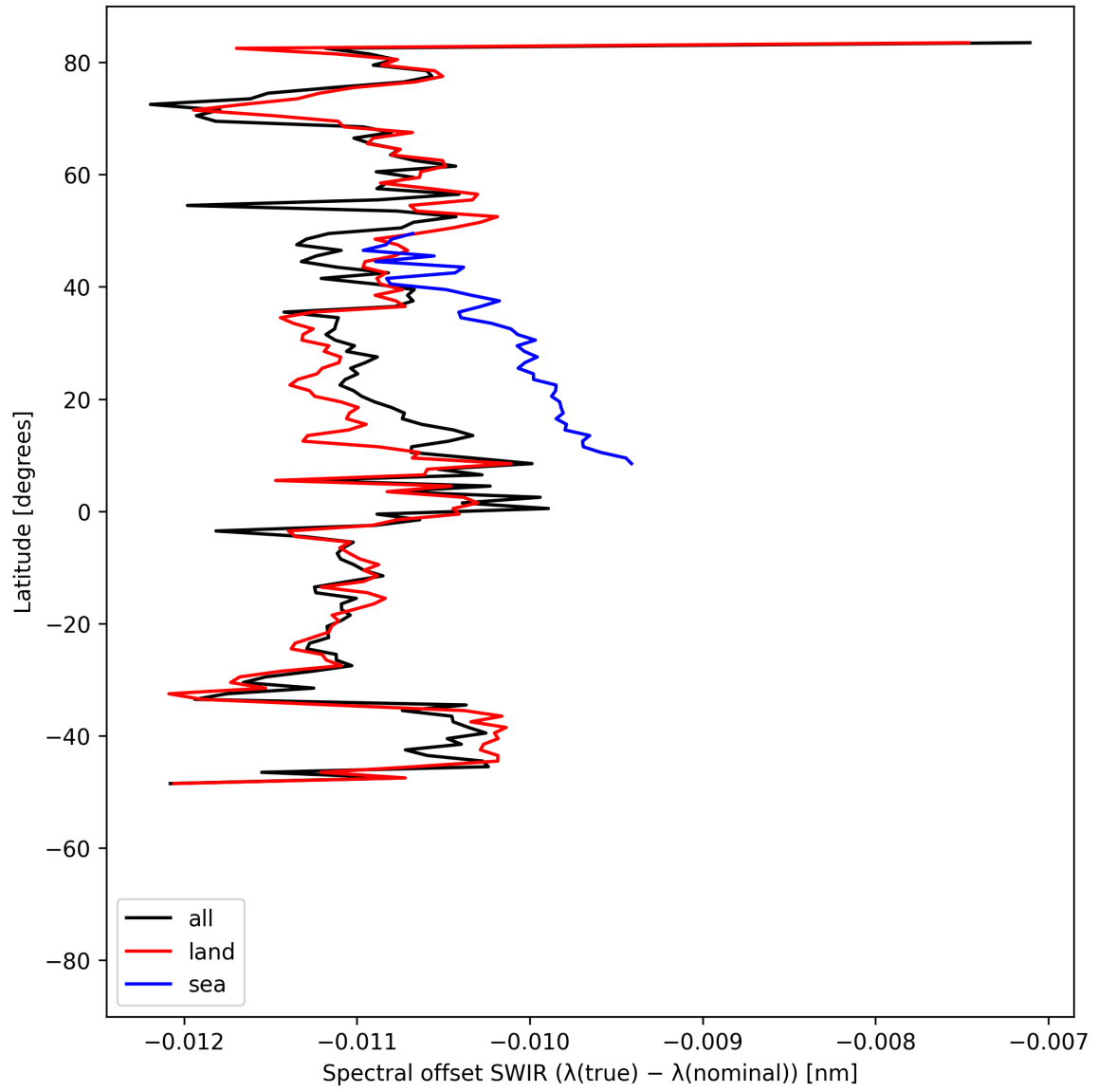
Figure 16: Zonal average of “Spectral offset SWIR ( \lambda_{\text{true}} - \lambda_{\text{nominal}} )” for 2025-06-28 to 2025-06-30.
