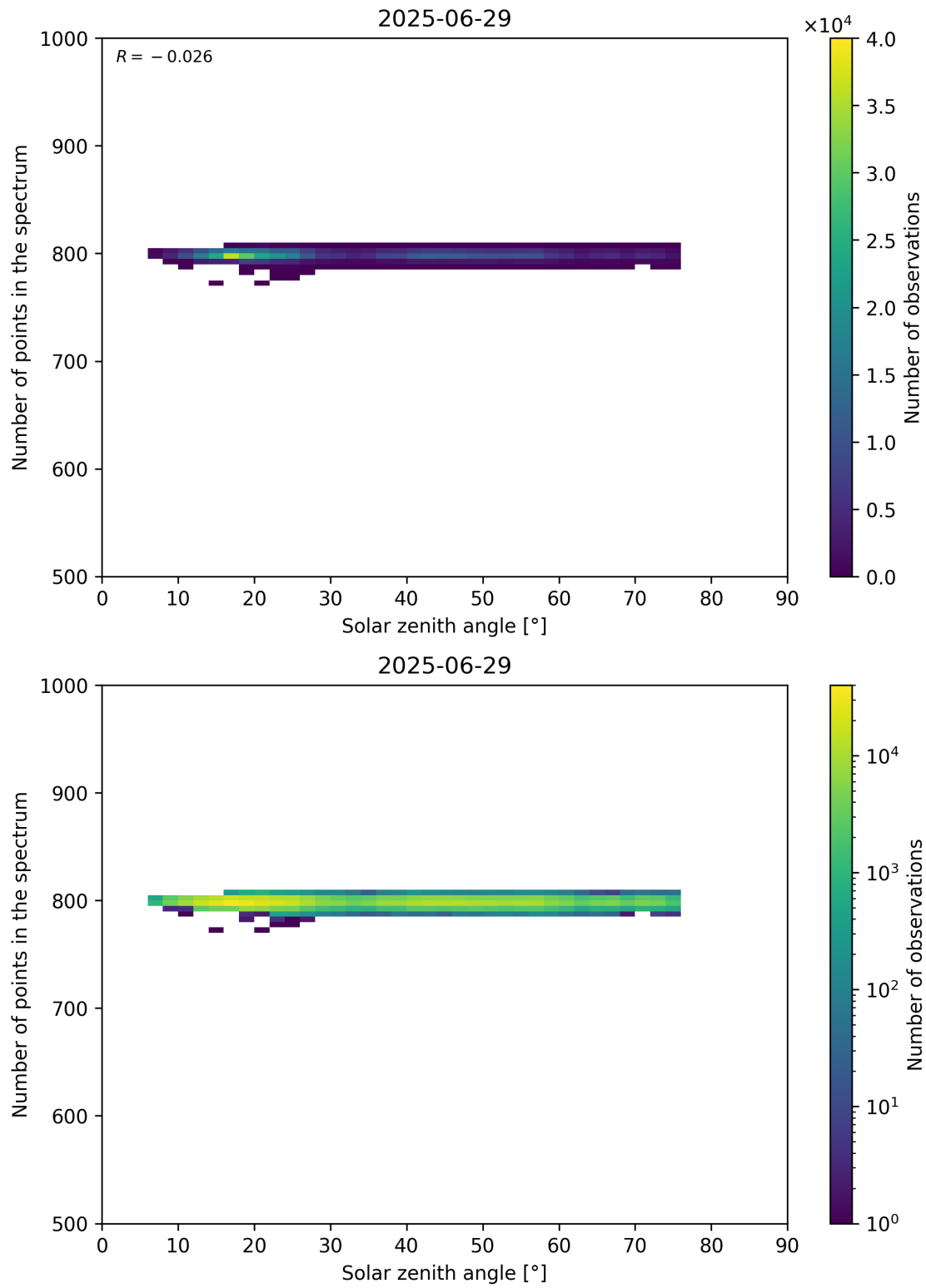
Figure 103: Scatter density plot of “Solar zenith angle” against “Number of points in the spectrum” for 2025-06-28 to 2025-06-30.
