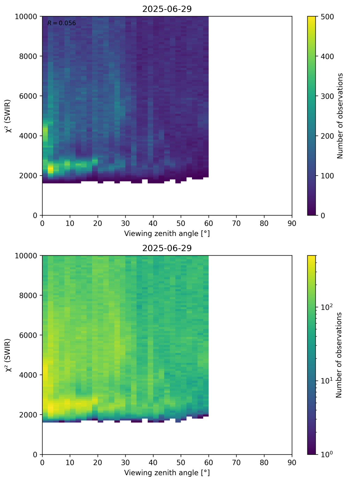
Figure 106: Scatter density plot of “Viewing zenith angle” against “ \chi^2 (SWIR)” for 2025-06-28 to 2025-06-30.
