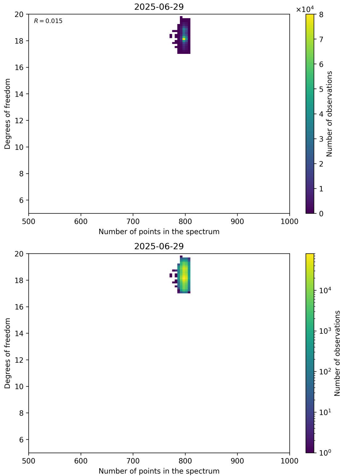
Figure 90: Scatter density plot of “Number of points in the spectrum” against “Degrees of freedom” for 2025-06-28 to 2025-06-30.
