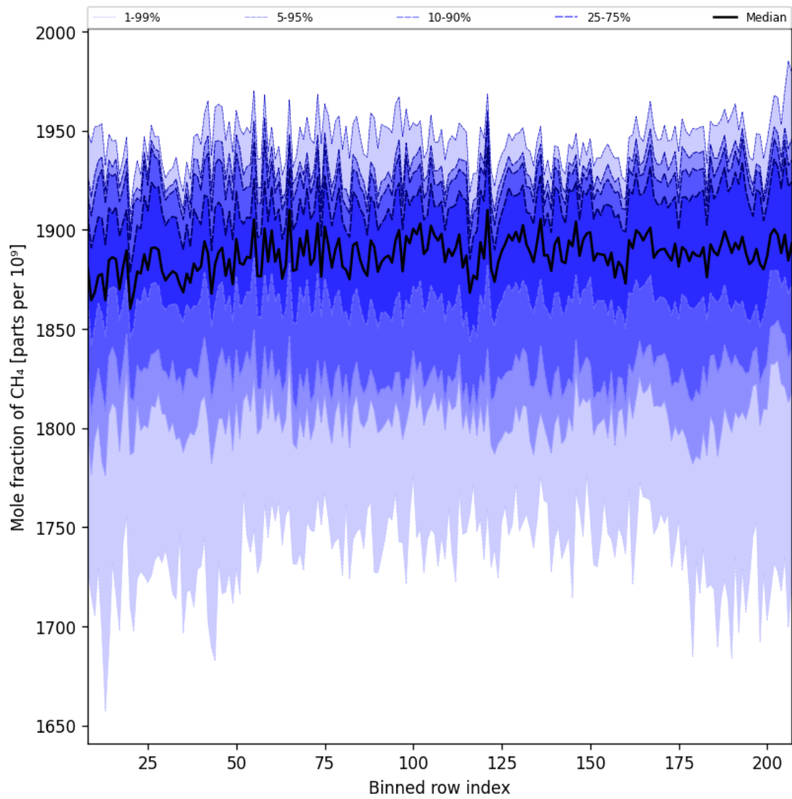
Figure 34: Along track statistics of “Mole fraction of CH 4 ” for 2025-06-28 to 2025-06-30
