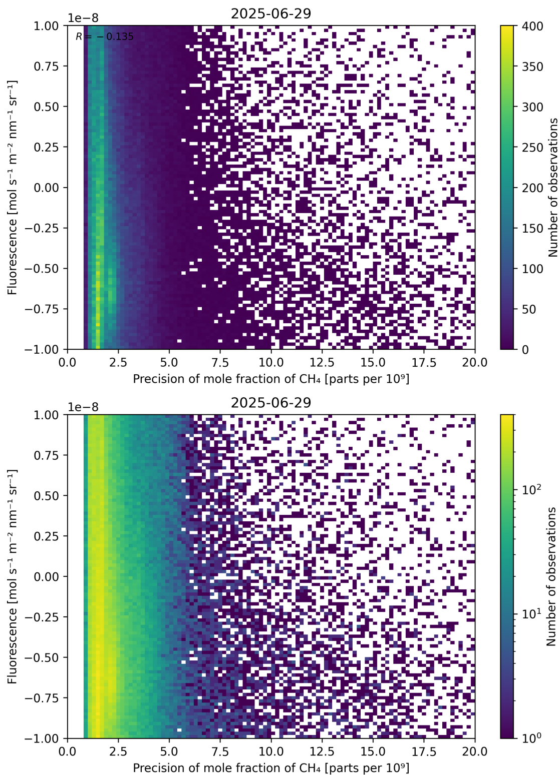
Figure 81: Scatter density plot of “Precision of mole fraction of \text{CH}_4 ” against “Fluorescence” for 2025-06-28 to 2025-06-30.
