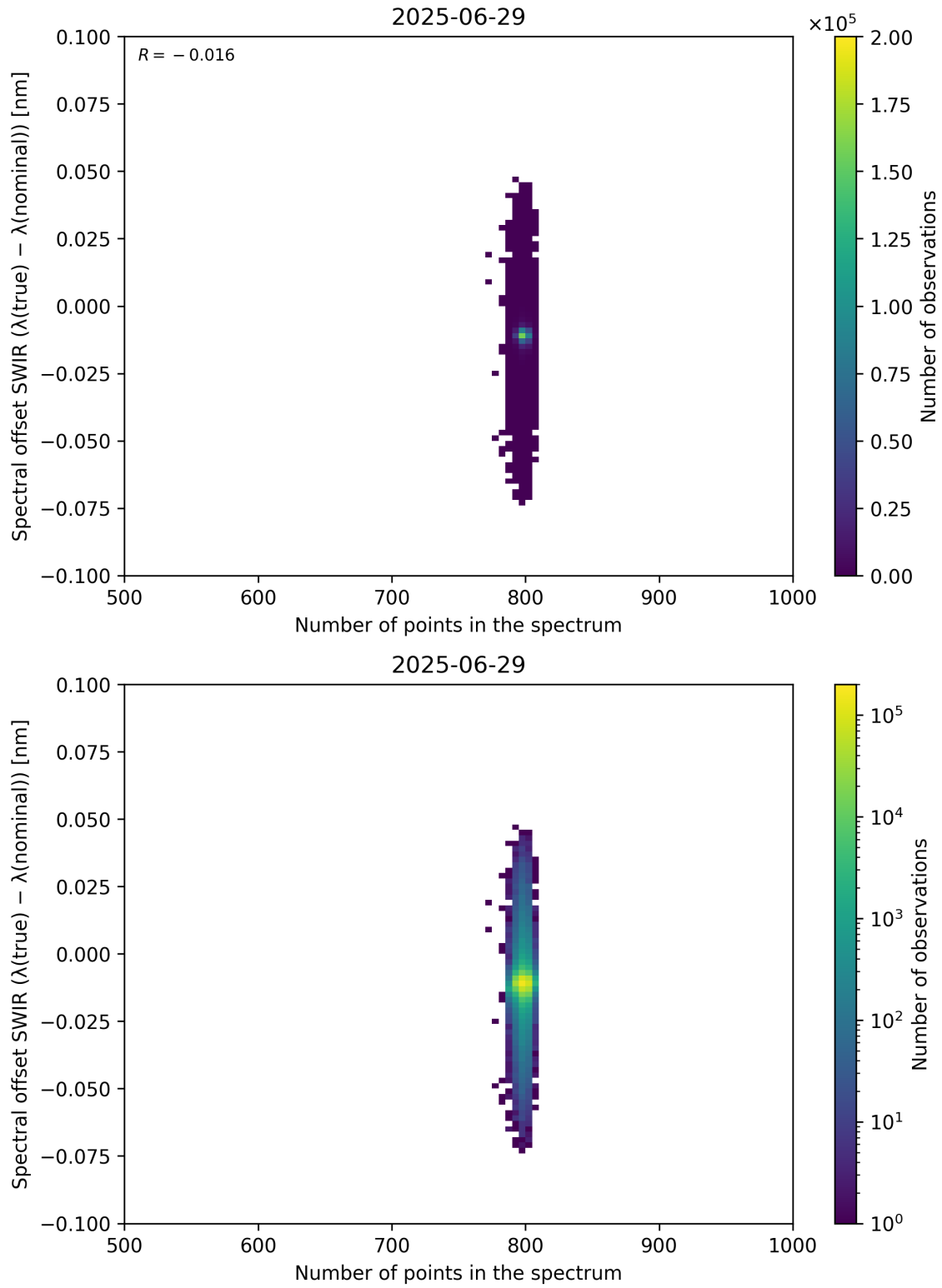
Figure 93: Scatter density plot of “Number of points in the spectrum” against “Spectral offset SWIR ( \lambda_{\text{true}} - \lambda_{\text{nominal}} )” for 2025-06-28 to 2025-06-30.
