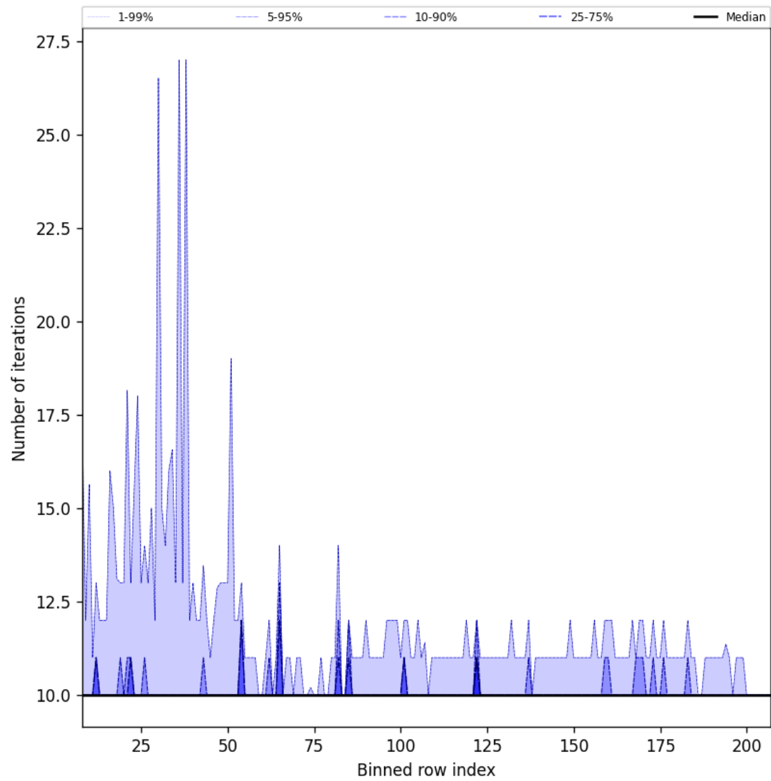
Figure 42: Along track statistics of “Number of iterations” for 2025-06-28 to 2025-06-30
