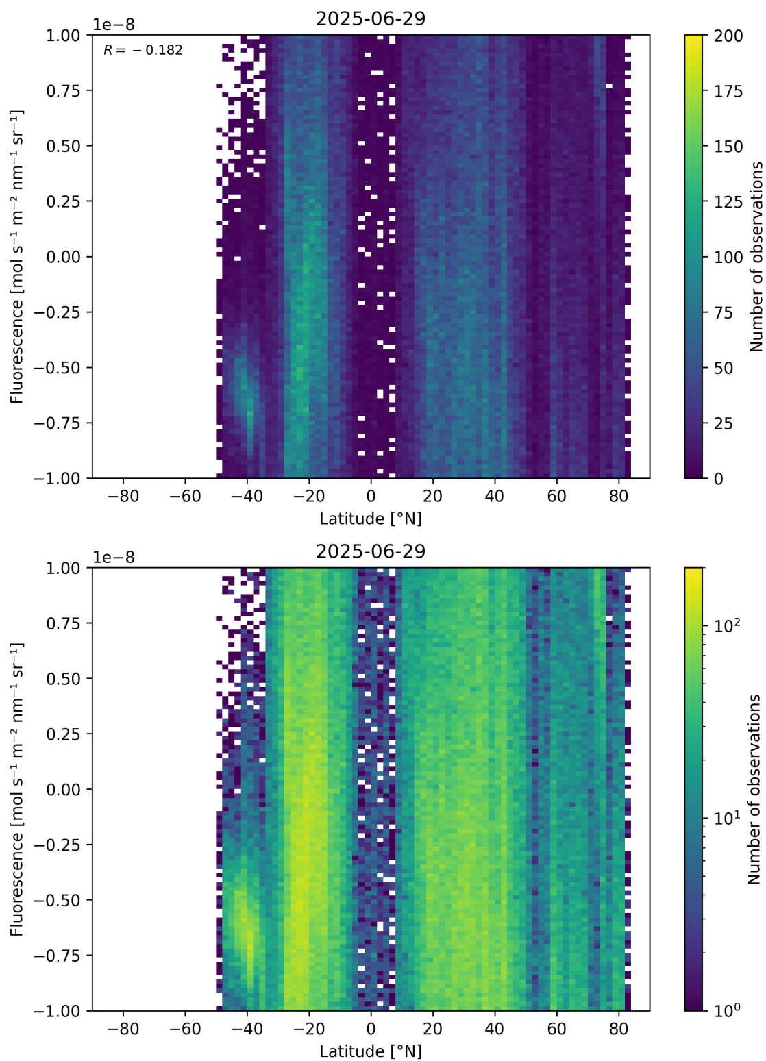
Figure 56: Scatter density plot of “Latitude” against “Fluorescence” for 2025-06-28 to 2025-06-30.
