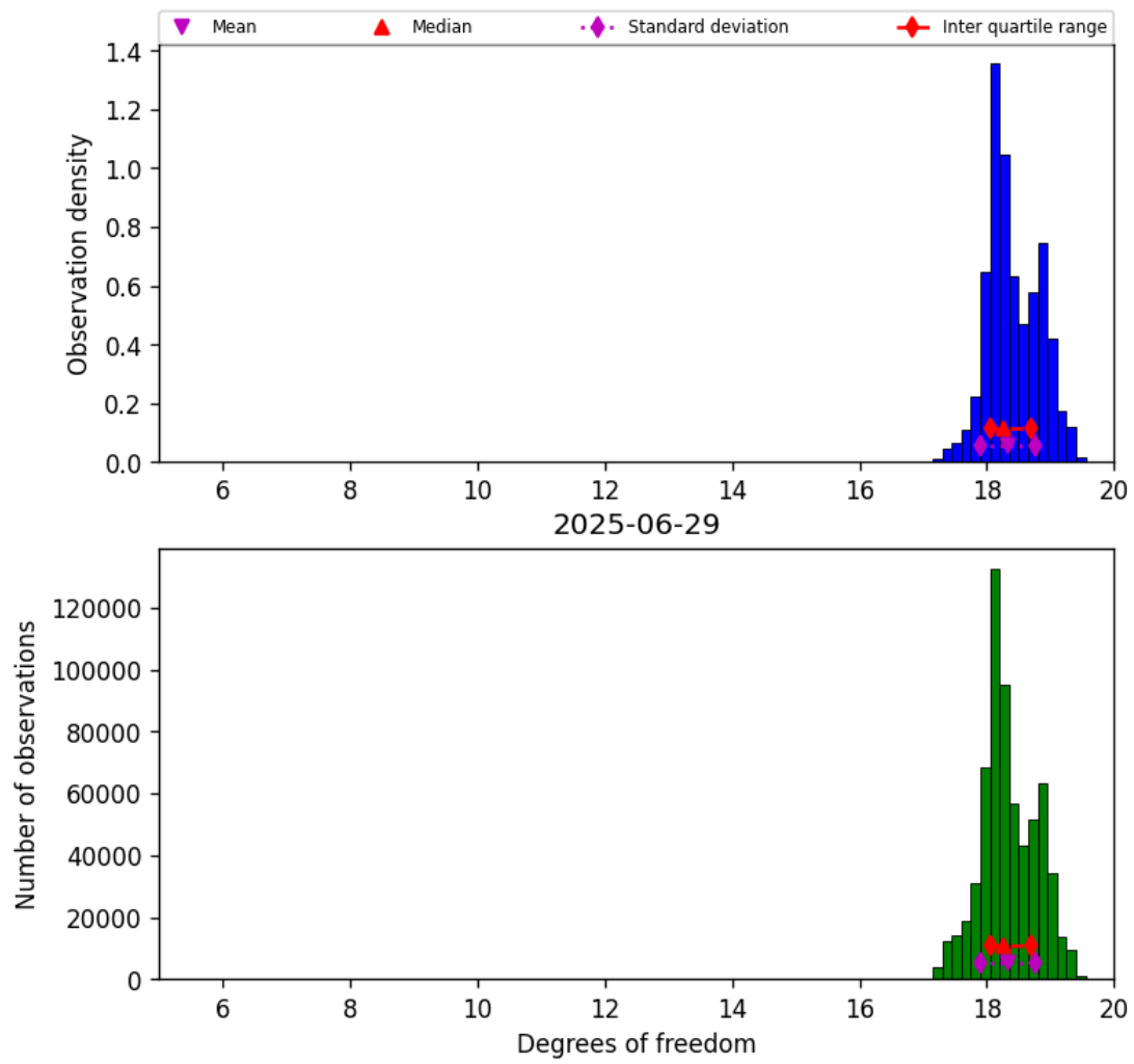
Figure 30: Histogram of “Degrees of freedom” for 2025-06-28 to 2025-06-30
