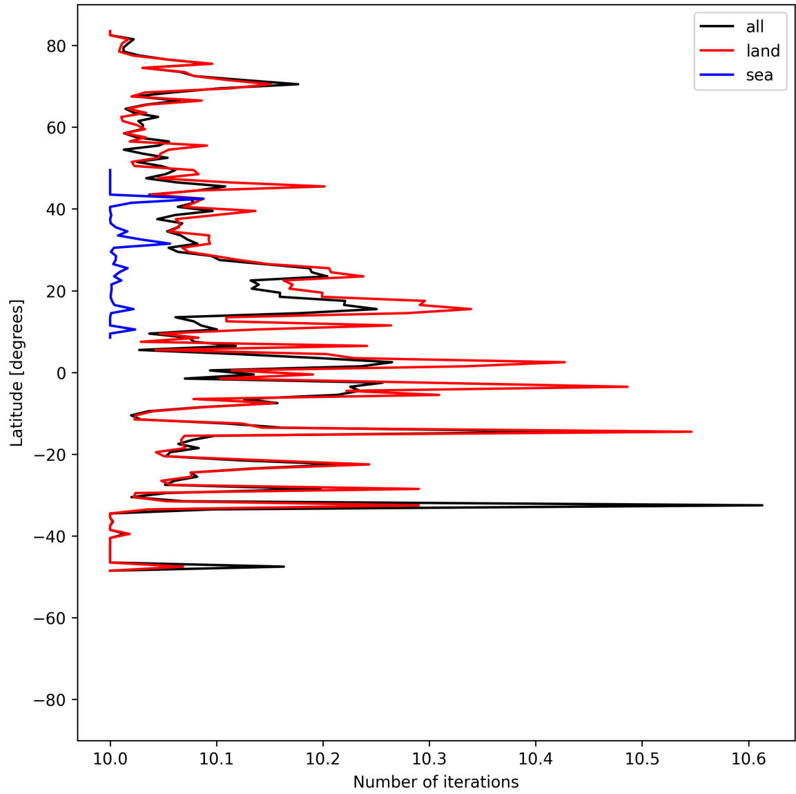
Figure 20: Zonal average of “Number of iterations” for 2025-06-28 to 2025-06-30.
