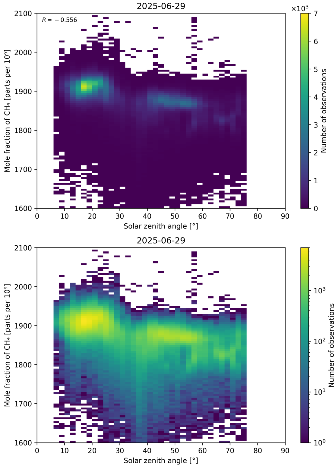
Figure 99: Scatter density plot of “Solar zenith angle” against “Mole fraction of \text{CH}_4 ” for 2025-06-28 to 2025-06-30.
