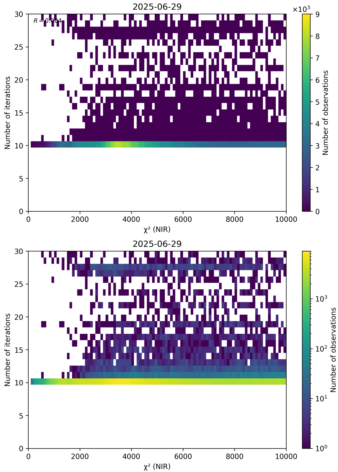
Figure 46: Scatter density plot of “ \chi^2 (NIR)” against “Number of iterations” for 2025-06-28 to 2025-06-30.
