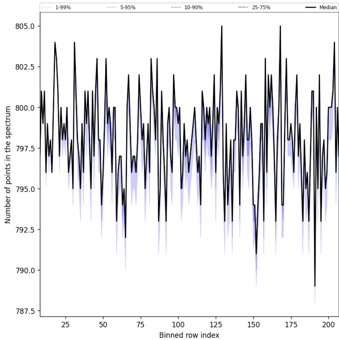
Figure 37: Along track statistics of “Number of points in the spectrum” for 2025-06-28 to 2025-06-30
