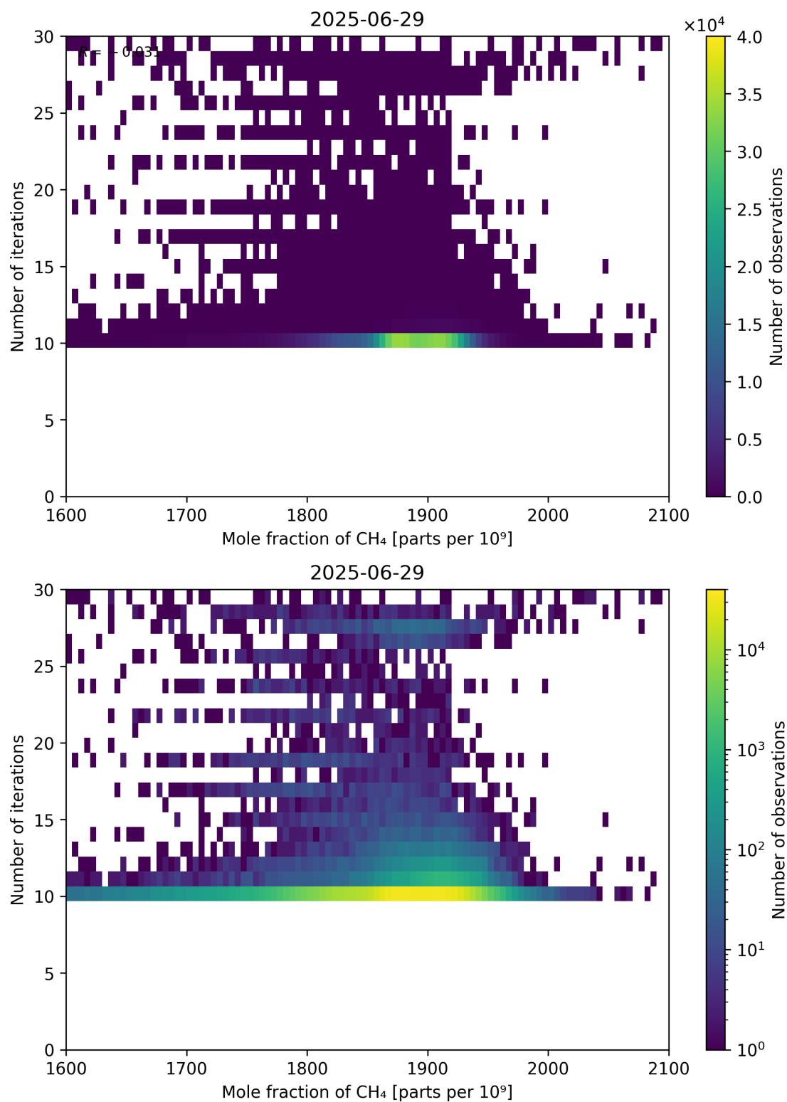
Figure 76: Scatter density plot of “Mole fraction of CH 4 ” against “Number of iterations” for 2025-06-28 to 2025-06-30.
