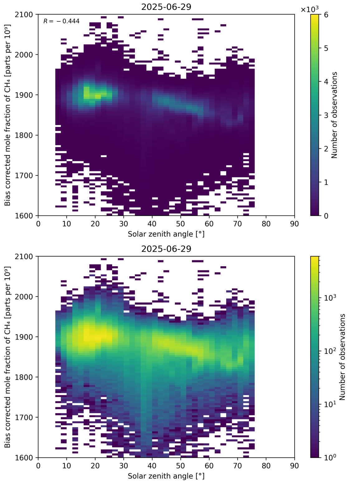
Figure 100: Scatter density plot of “Solar zenith angle” against “Bias corrected mole fraction of CH 4 ” for 2025-06-28 to 2025-06-30.
