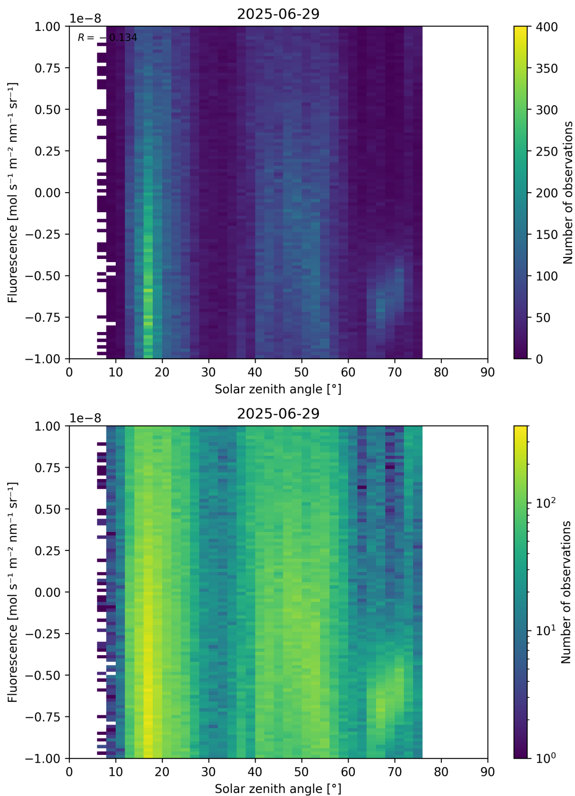
Figure 97: Scatter density plot of “Solar zenith angle” against “Fluorescence” for 2025-06-28 to 2025-06-30.
