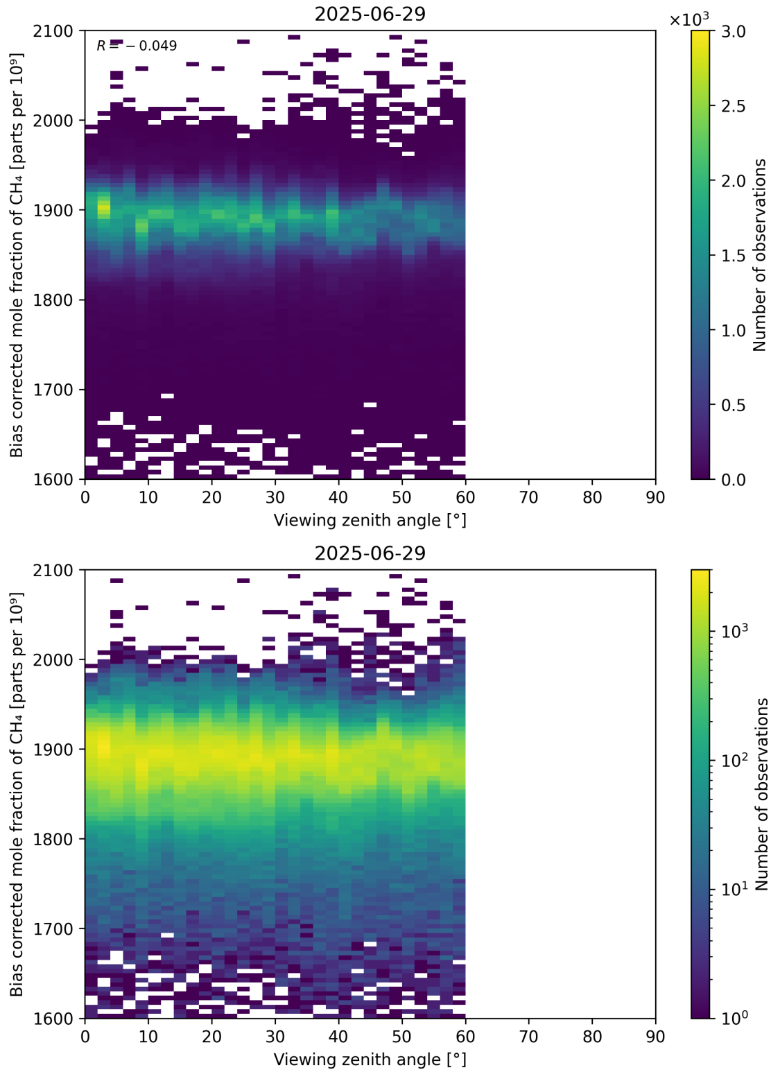
Figure 111: Scatter density plot of “Viewing zenith angle” against “Bias corrected mole fraction of CH 4 ” for 2025-06-28 to 2025-06-30.
