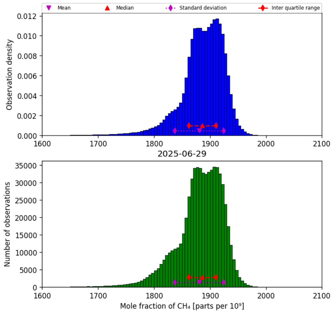
Figure 23: Histogram of “Mole fraction of CH 4 ” for 2025-06-28 to 2025-06-30
