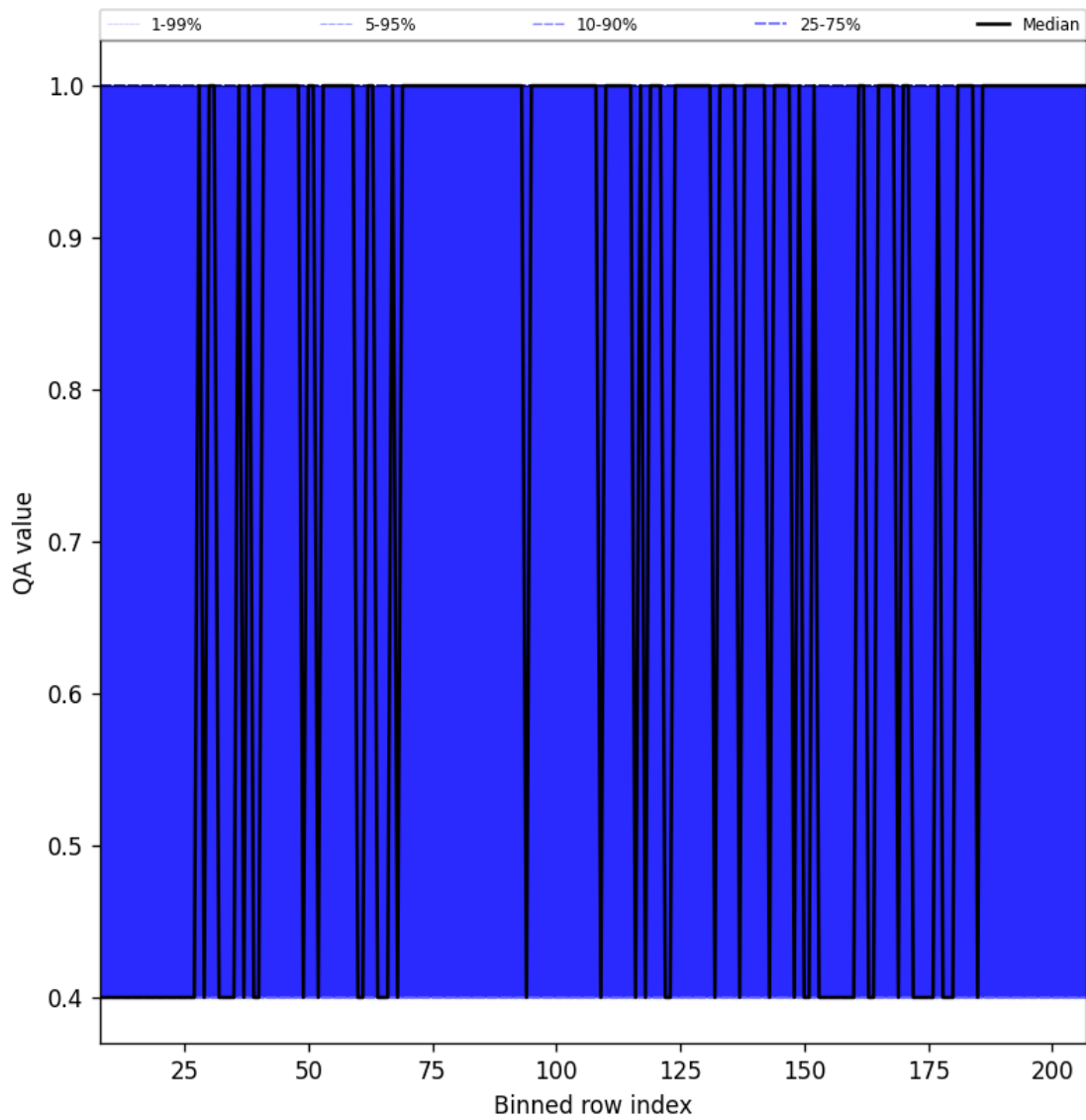
Figure 33: Along track statistics of “QA value” for 2025-06-28 to 2025-06-30
