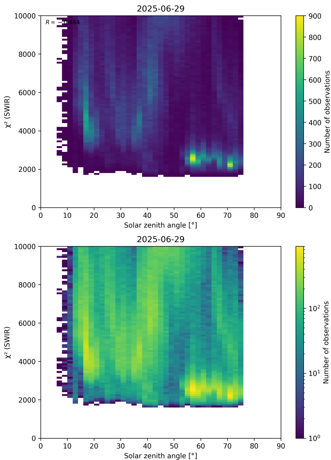
Figure 95: Scatter density plot of “Solar zenith angle” against “ \chi^2 (SWIR)” for 2025-06-28 to 2025-06-30.
