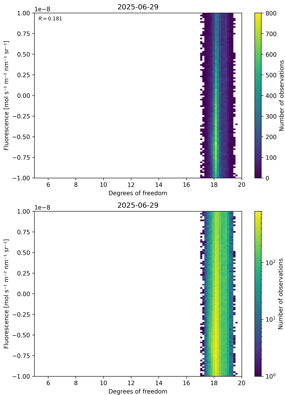
Figure 51: Scatter density plot of “Degrees of freedom” against “Fluorescence” for 2025-06-28 to 2025-06-30.
