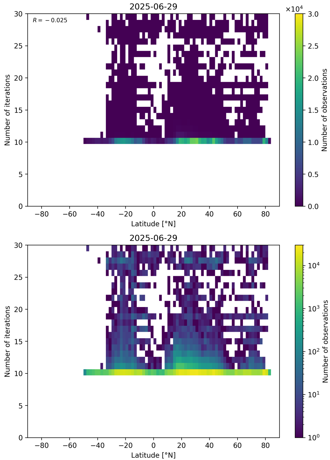
Figure 60: Scatter density plot of “Latitude” against “Number of iterations” for 2025-06-28 to 2025-06-30.
