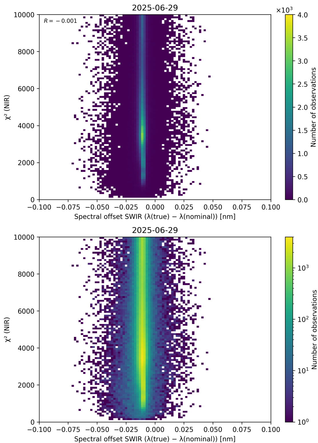
Figure 117: Scatter density plot of “Spectral offset SWIR ( \lambda_{\text{true}} - \lambda_{\text{nominal}} )” against “ \chi^2 (NIR)” for 2025-06-28 to 2025-06-30.
