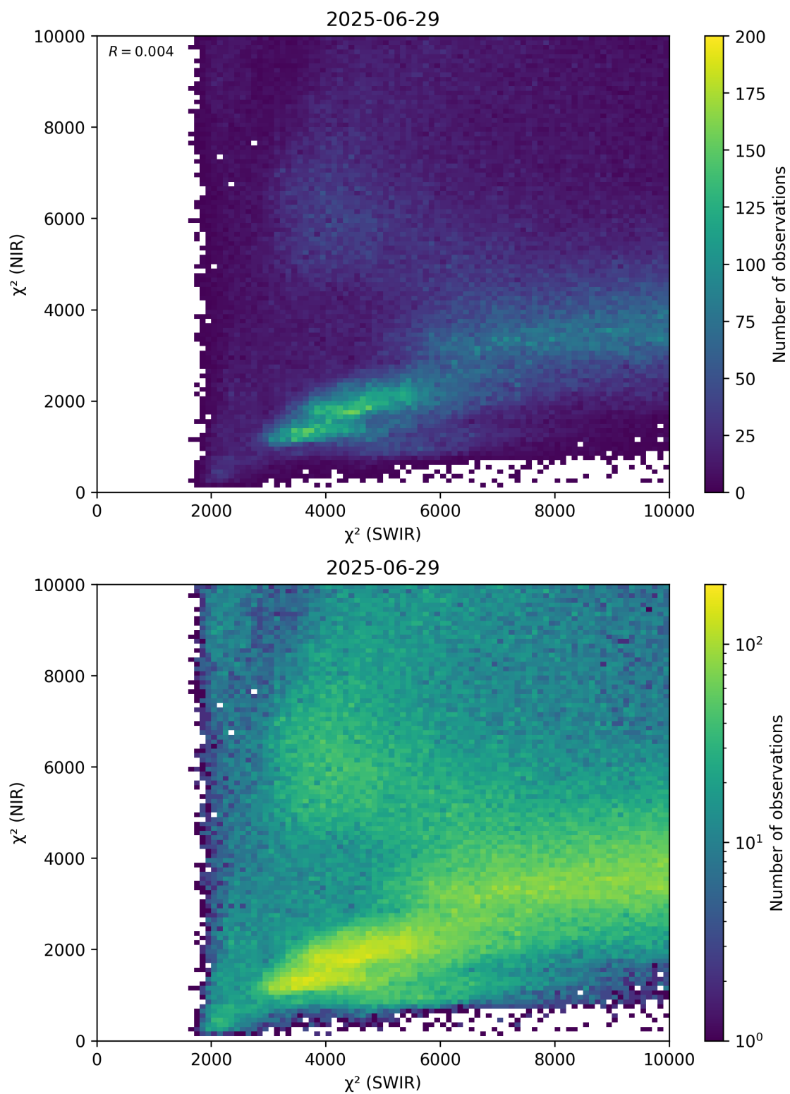
Figure 47: Scatter density plot of “ \chi^2 (SWIR)” against “ \chi^2 (NIR)” for 2025-06-28 to 2025-06-30.
