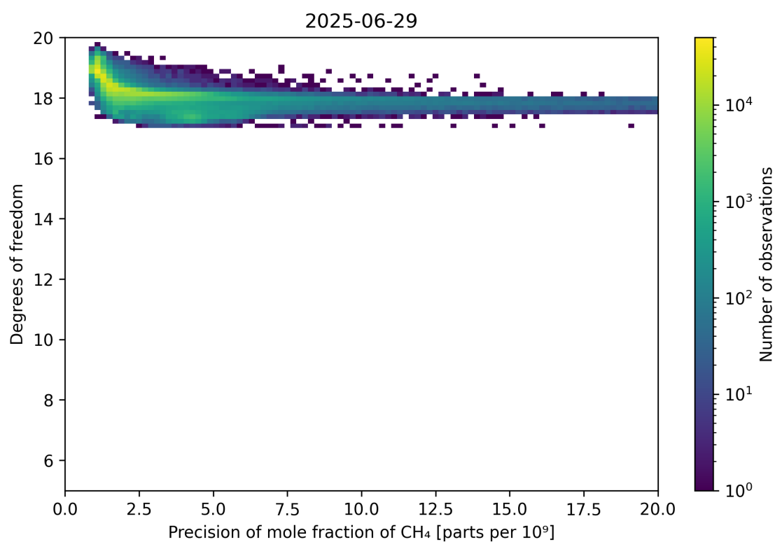
Figure 80: Scatter density plot of “Precision of mole fraction of CH 4 ” against “Degrees of freedom” for 2025-06-28 to 2025-06-30.
