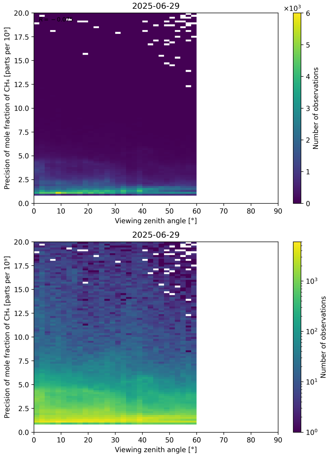
Figure 112: Scatter density plot of “Viewing zenith angle” against “Precision of mole fraction of CH 4 ” for 2025-06-28 to 2025-06-30.
