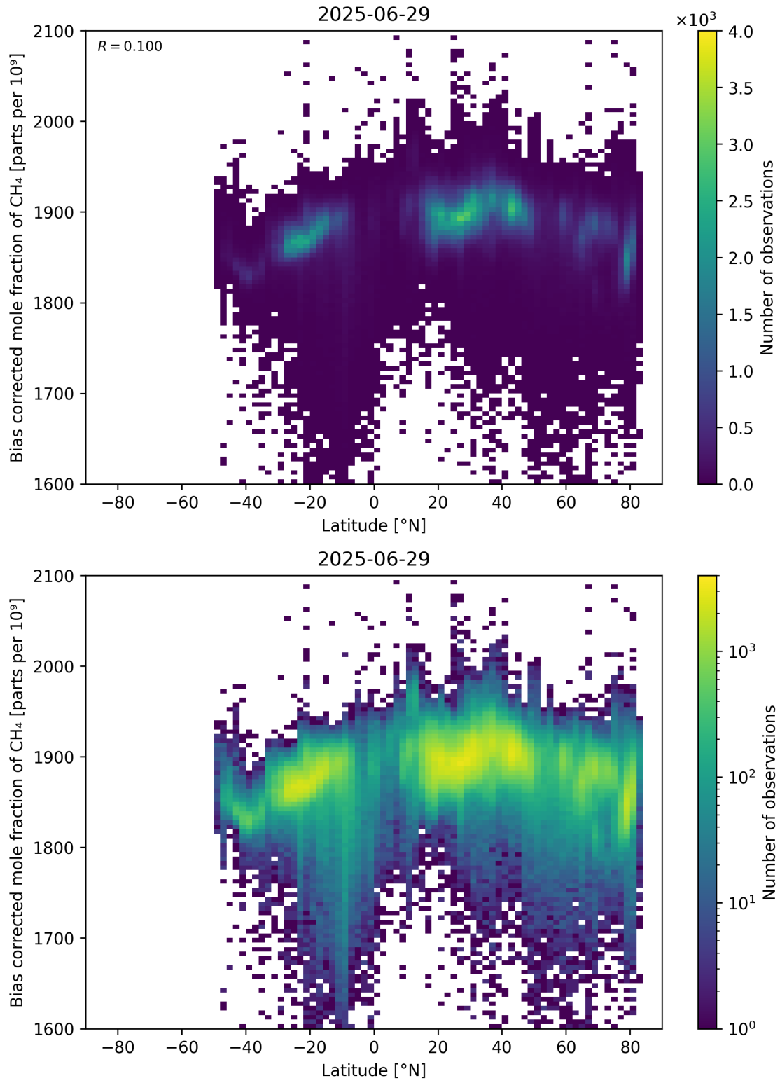
Figure 58: Scatter density plot of “Latitude” against “Bias corrected mole fraction of CH 4 ” for 2025-06-28 to 2025-06-30.
