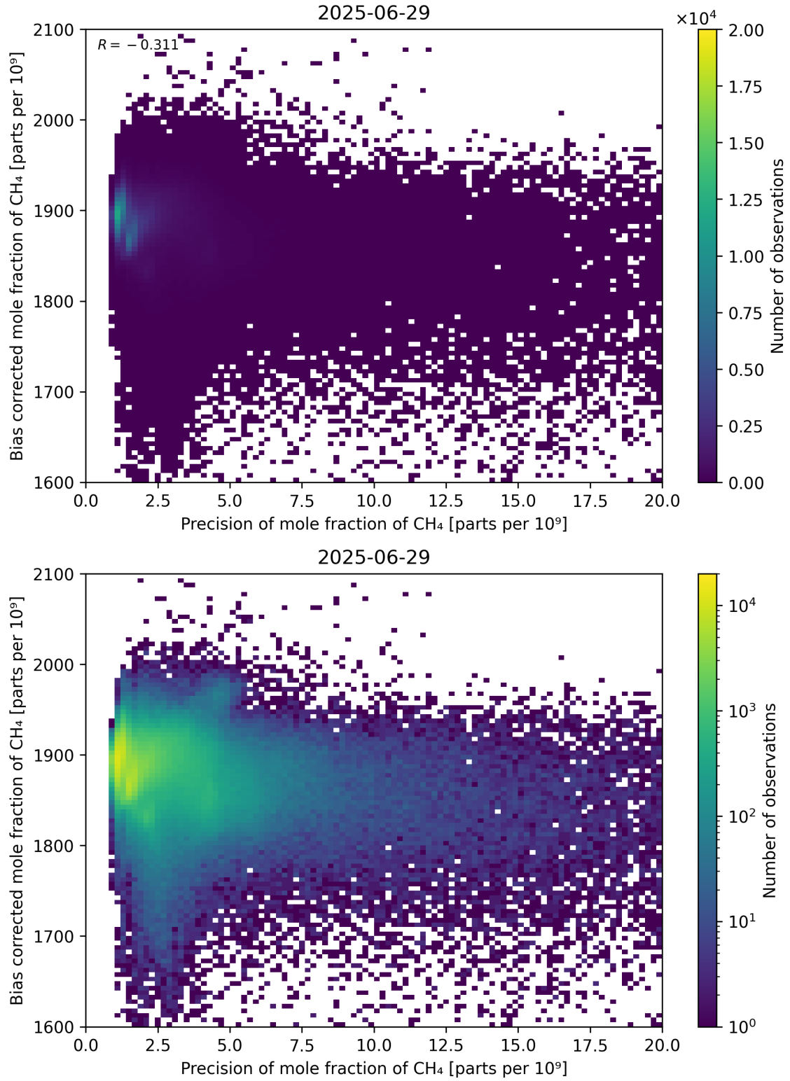
Figure 82: Scatter density plot of “Precision of mole fraction of \text{CH}_4 ” against “Bias corrected mole fraction of \text{CH}_4 ” for 2025-06-28 to 2025-06-30.
