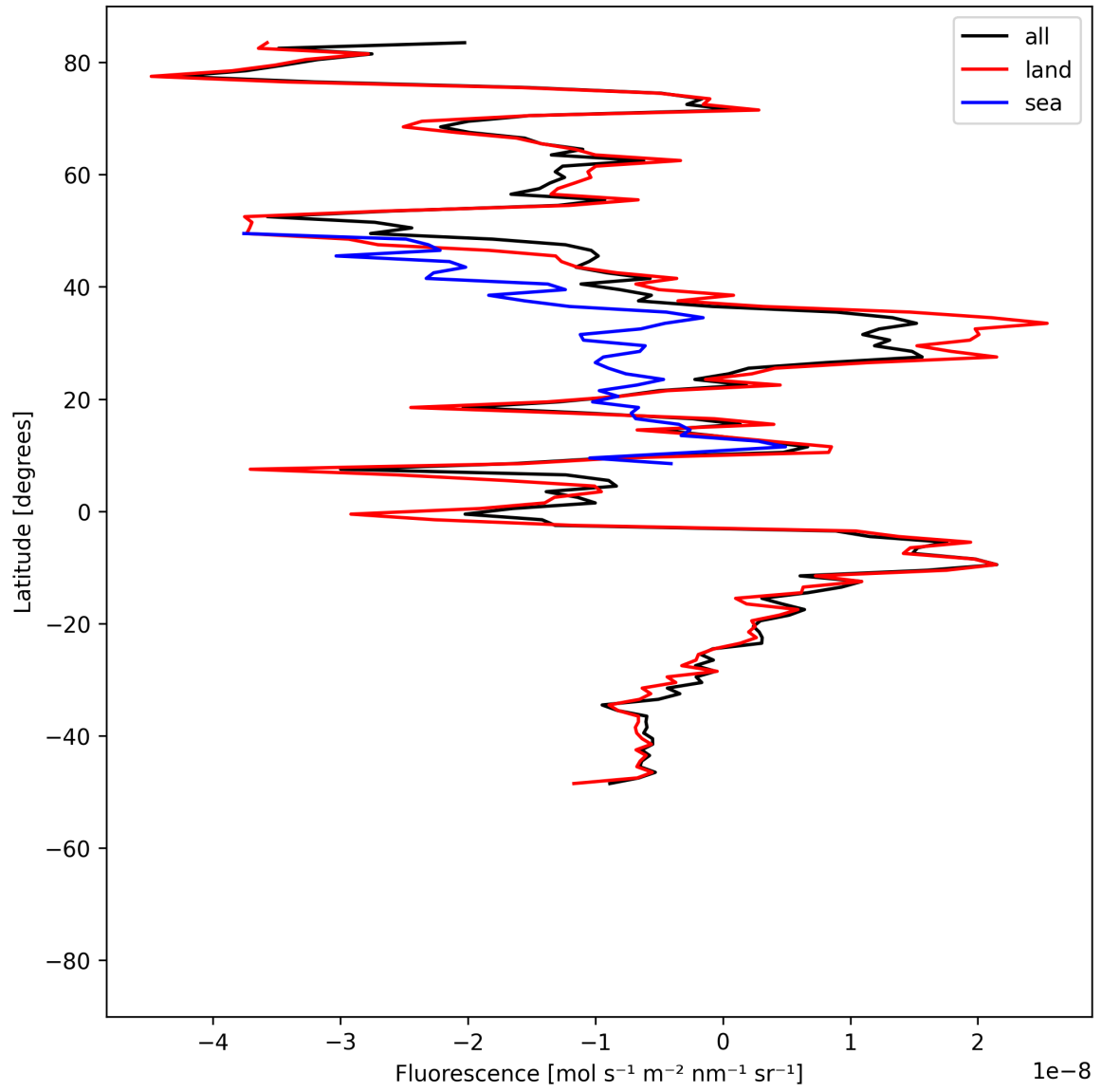
Figure 21: Zonal average of “Fluorescence” for 2025-06-28 to 2025-06-30.
