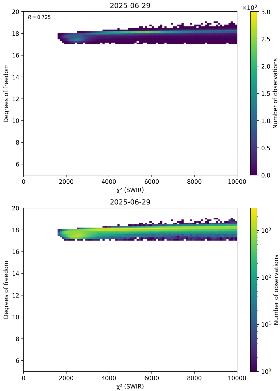
Figure 48: Scatter density plot of “ \chi^2 (SWIR)” against “Degrees of freedom” for 2025-06-28 to 2025-06-30.
