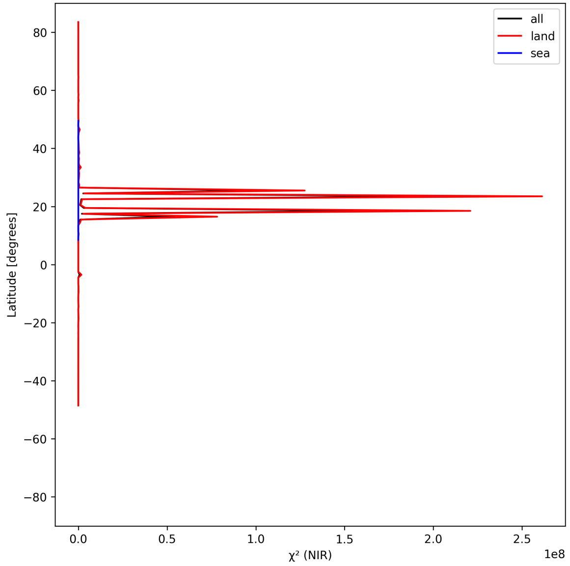
Figure 18: Zonal average of “ \chi^2 (NIR)” for 2025-06-28 to 2025-06-30.
