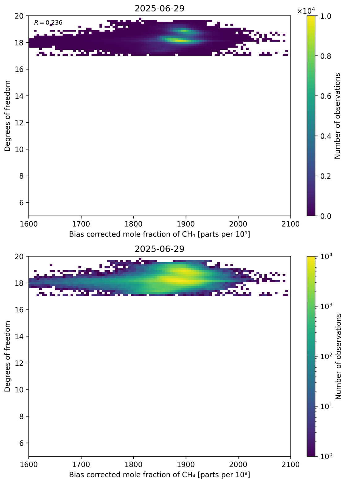
Figure 65: Scatter density plot of “Bias corrected mole fraction of CH 4 ” against “Degrees of freedom” for 2025-06-28 to 2025-06-30.
