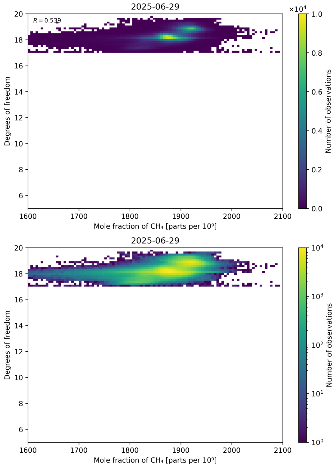
Figure 72: Scatter density plot of “Mole fraction of CH 4 ” against “Degrees of freedom” for 2025-06-28 to 2025-06-30.
