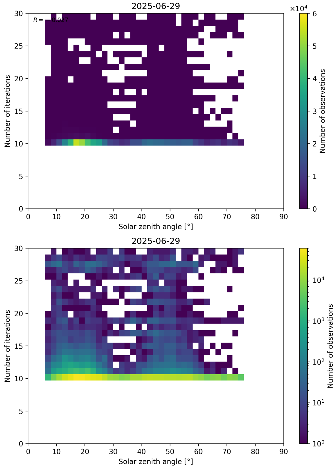
Figure 102: Scatter density plot of “Solar zenith angle” against “Number of iterations” for 2025-06-28 to 2025-06-30.
