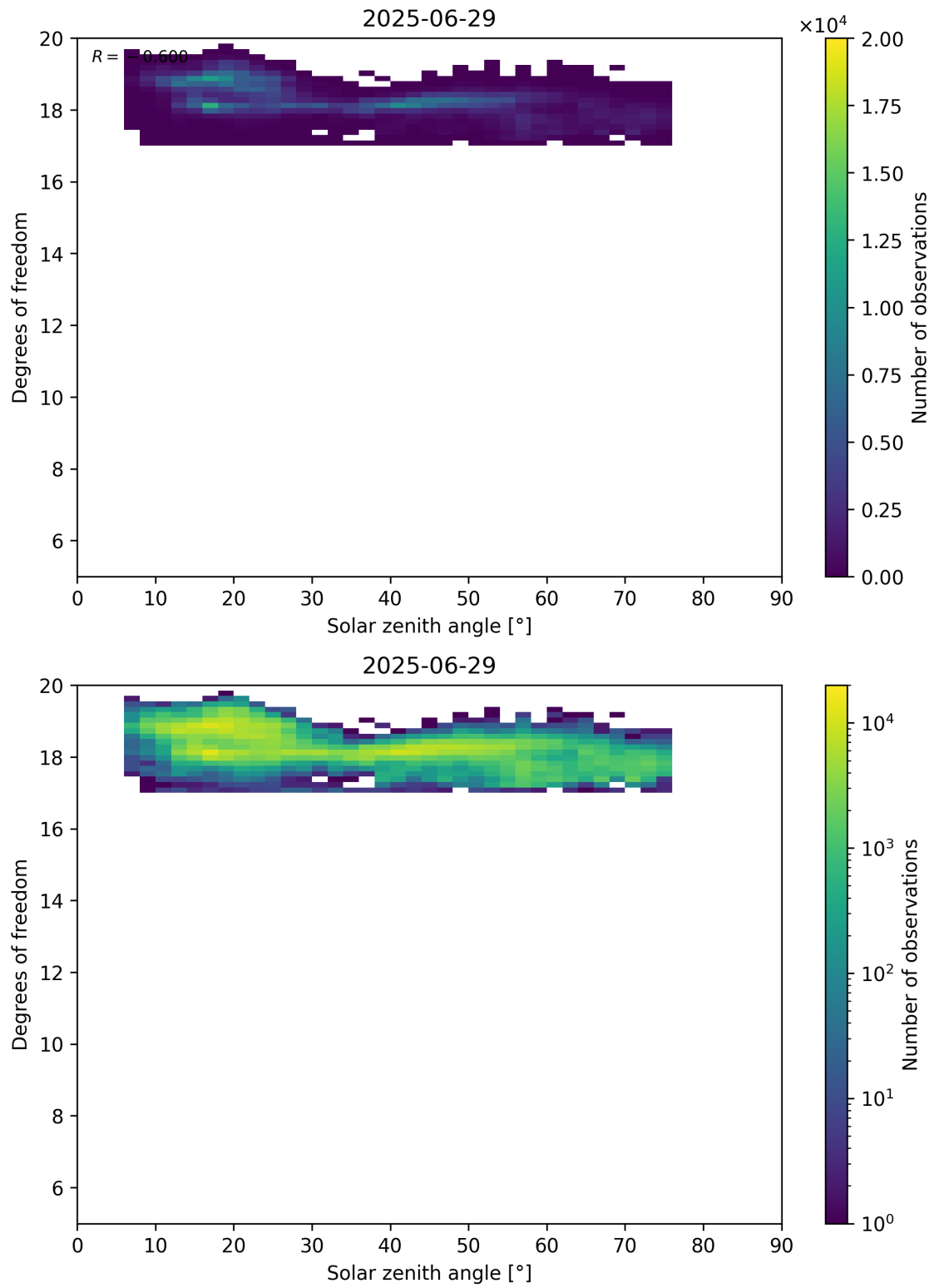
Figure 96: Scatter density plot of “Solar zenith angle” against “Degrees of freedom” for 2025-06-28 to 2025-06-30.
