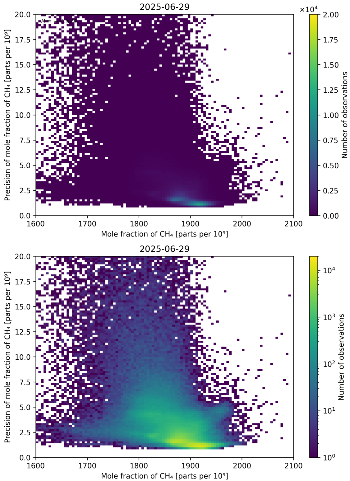
Figure 75: Scatter density plot of “Mole fraction of CH 4 ” against “Precision of mole fraction of CH 4 ” for 2025-06-28 to 2025-06-30.
