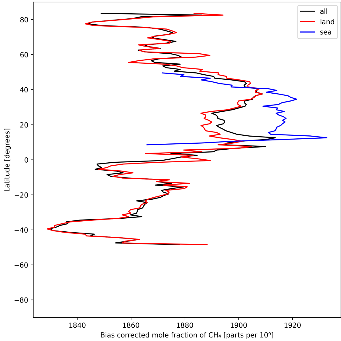
Figure 14: Zonal average of “Bias corrected mole fraction of CH 4 ” for 2025-06-28 to 2025-06-30.
