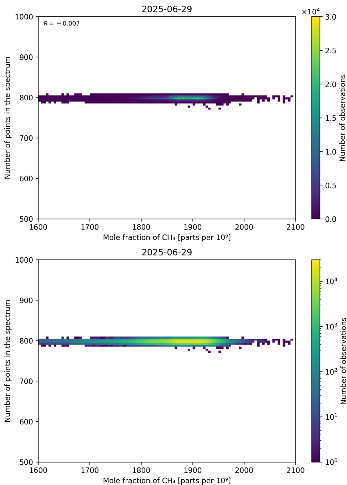
Figure 77: Scatter density plot of “Mole fraction of CH 4 ” against “Number of points in the spectrum” for 2025-06-28 to 2025-06-30.
