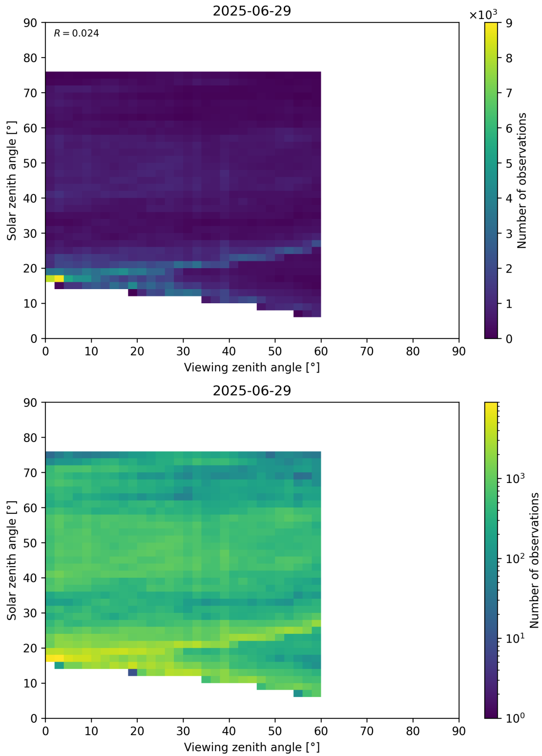
Figure 115: Scatter density plot of “Viewing zenith angle” against “Solar zenith angle” for 2025-06-28 to 2025-06-30.
