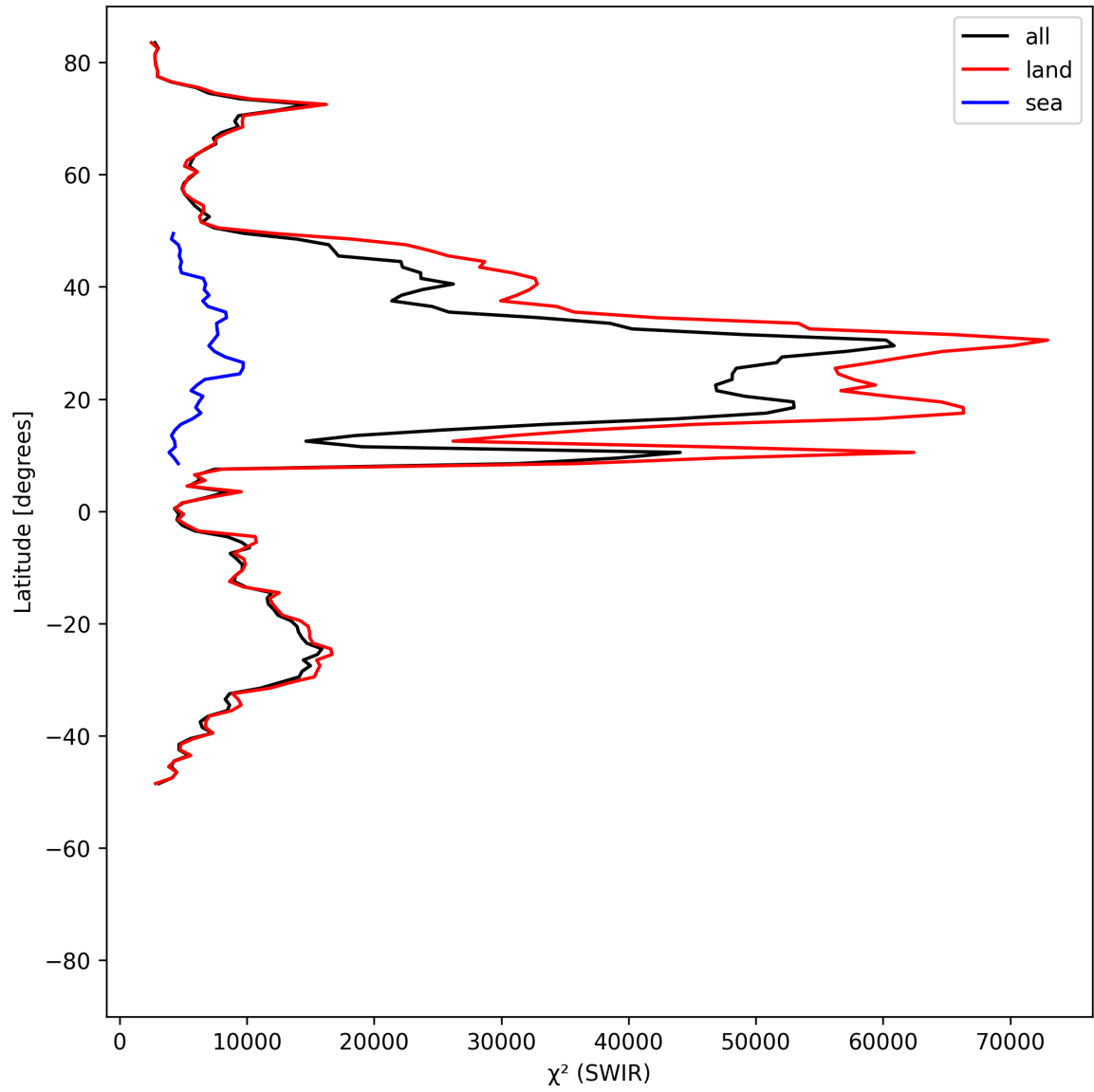
Figure 17: Zonal average of “ \chi^2 (SWIR)” for 2025-06-28 to 2025-06-30.
