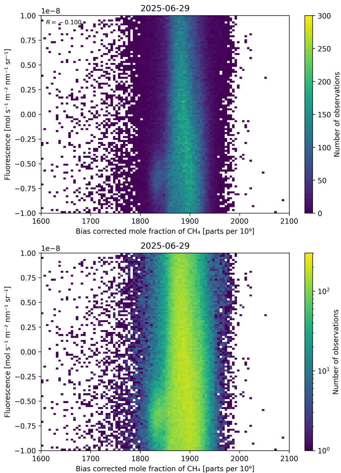
Figure 66: Scatter density plot of “Bias corrected mole fraction of \text{CH}_4 ” against “Fluorescence” for 2025-06-28 to 2025-06-30.
