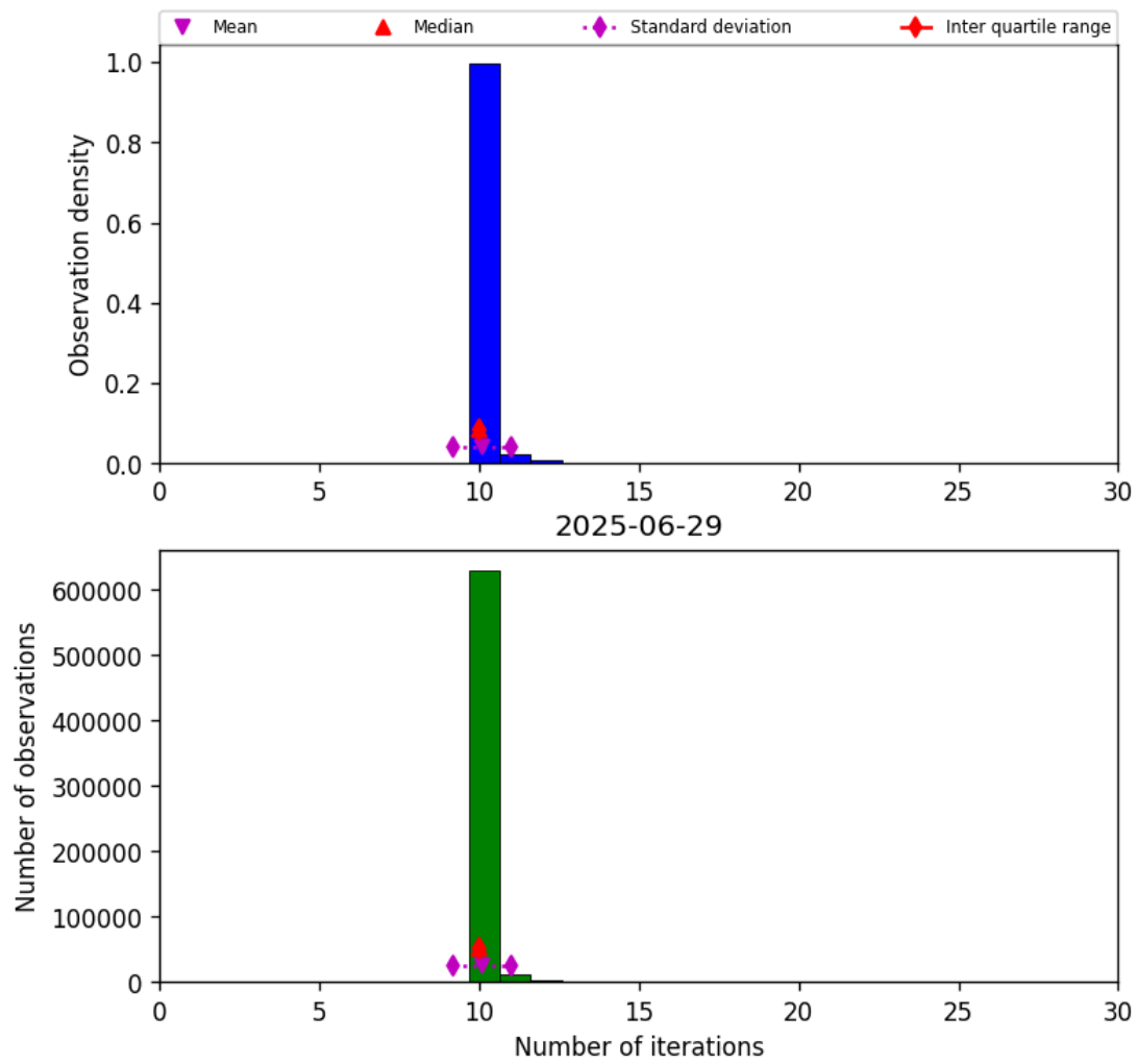
Figure 31: Histogram of “Number of iterations” for 2025-06-28 to 2025-06-30
