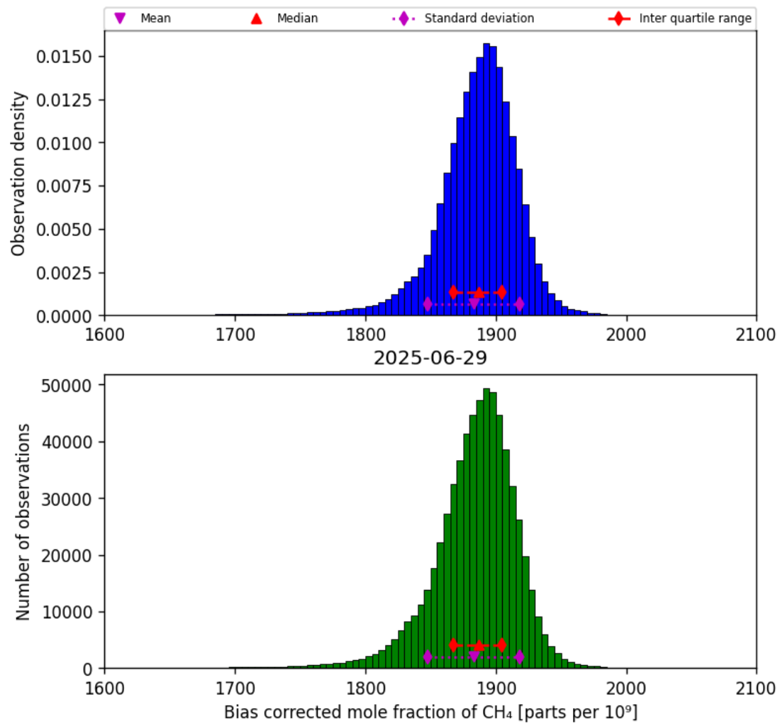
Figure 25: Histogram of “Bias corrected mole fraction of CH 4 ” for 2025-06-28 to 2025-06-30
