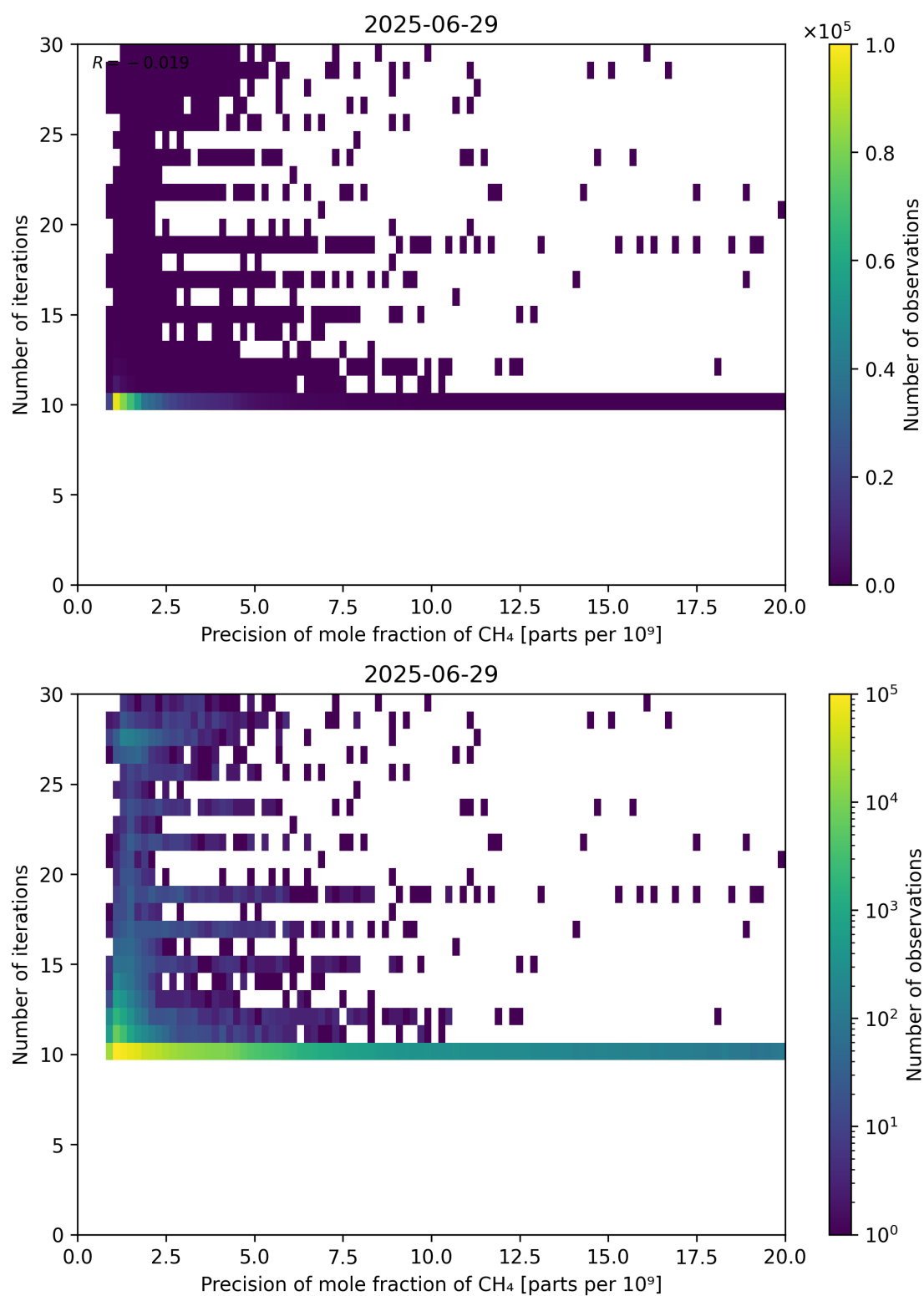
Figure 83: Scatter density plot of “Precision of mole fraction of CH 4 ” against “Number of iterations” for 2025-06-28 to 2025-06-30.
