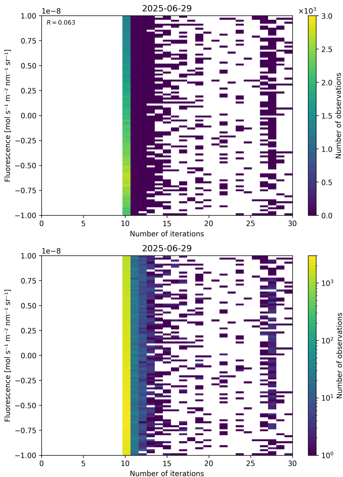
Figure 87: Scatter density plot of “Number of iterations” against “Fluorescence” for 2025-06-28 to 2025-06-30.
