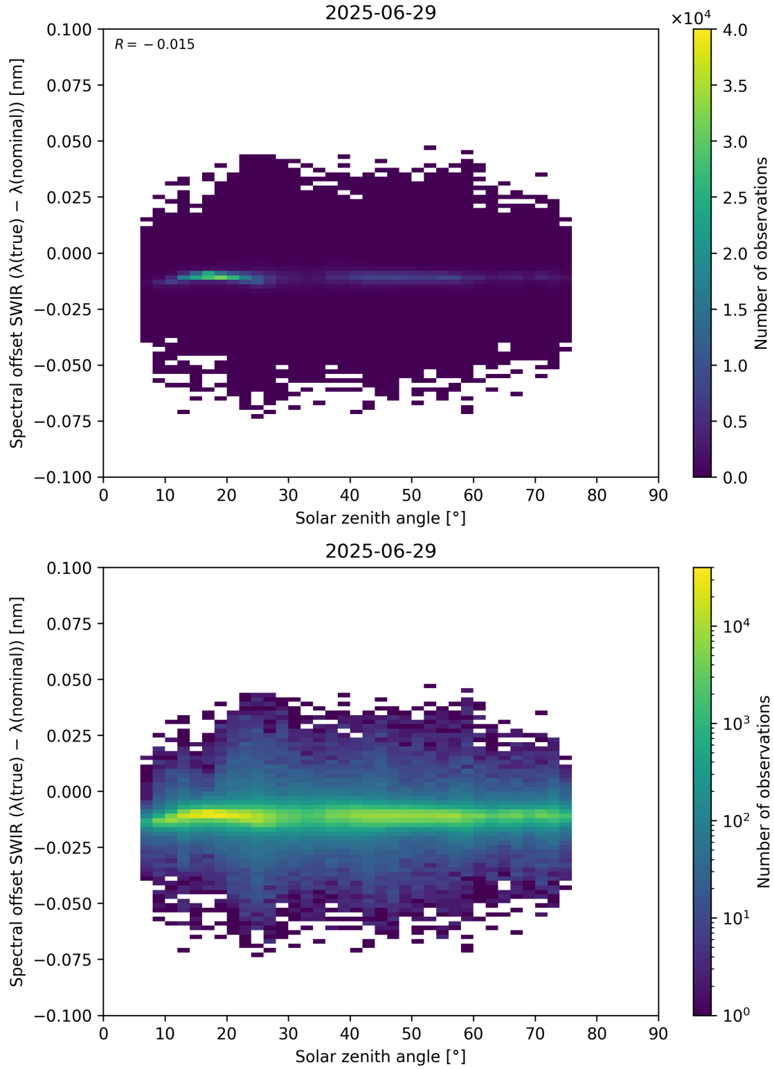
Figure 104: Scatter density plot of “Solar zenith angle” against “Spectral offset SWIR ( \lambda_{\text{true}} - \lambda_{\text{nominal}} )” for 2025-06-28 to 2025-06-30.
