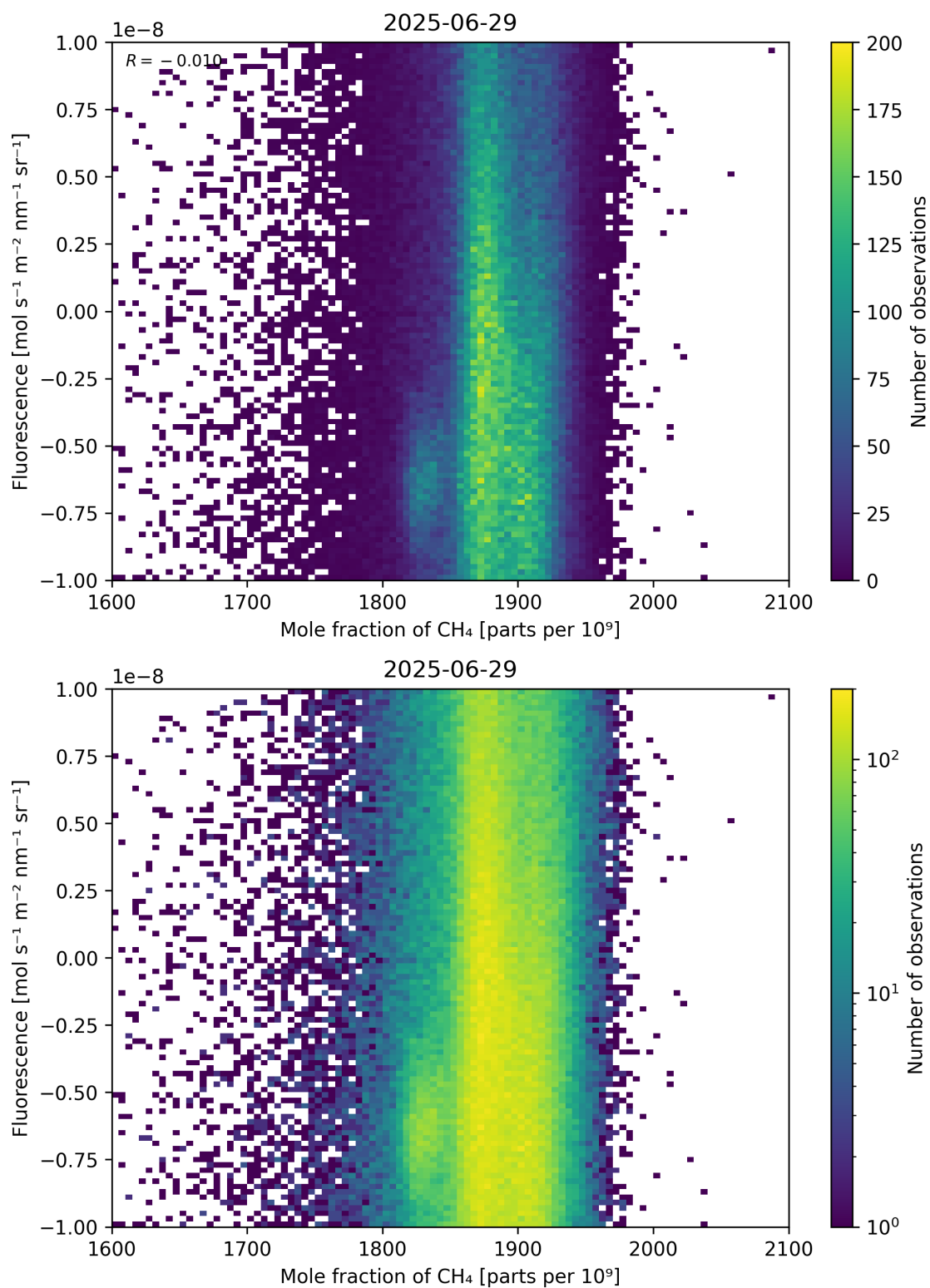
Figure 73: Scatter density plot of “Mole fraction of \text{CH}_4 ” against “Fluorescence” for 2025-06-28 to 2025-06-30.
