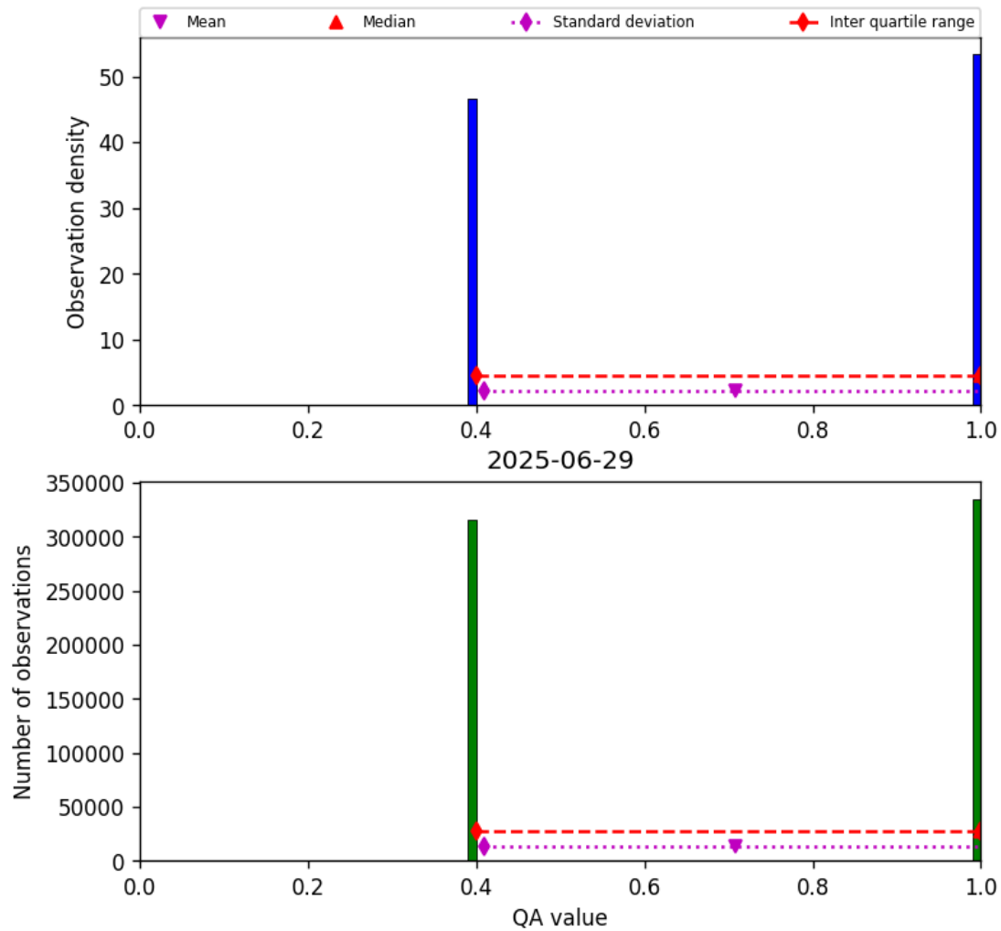
Figure 22: Histogram of “QA value” for 2025-06-28 to 2025-06-30
