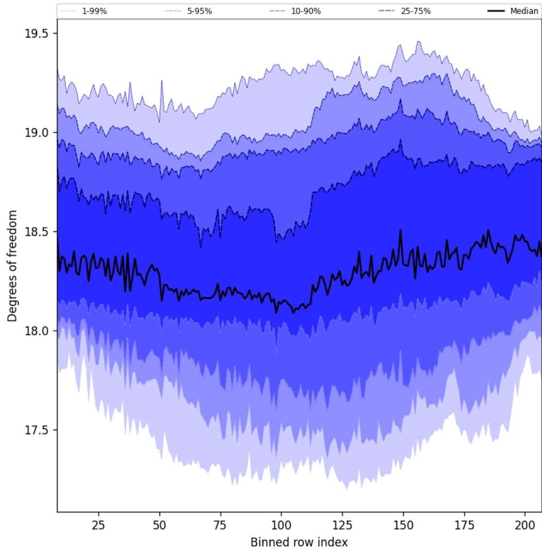
Figure 41: Along track statistics of “Degrees of freedom” for 2025-06-28 to 2025-06-30
