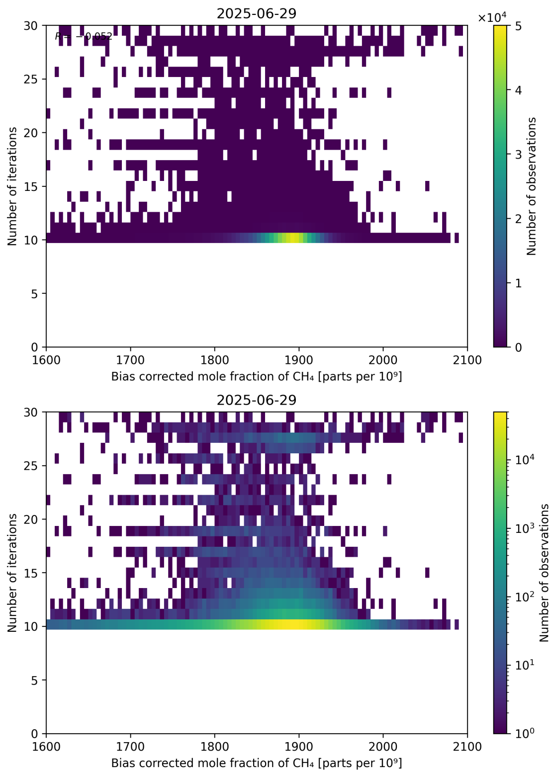
Figure 67: Scatter density plot of “Bias corrected mole fraction of CH 4 ” against “Number of iterations” for 2025-06-28 to 2025-06-30.
