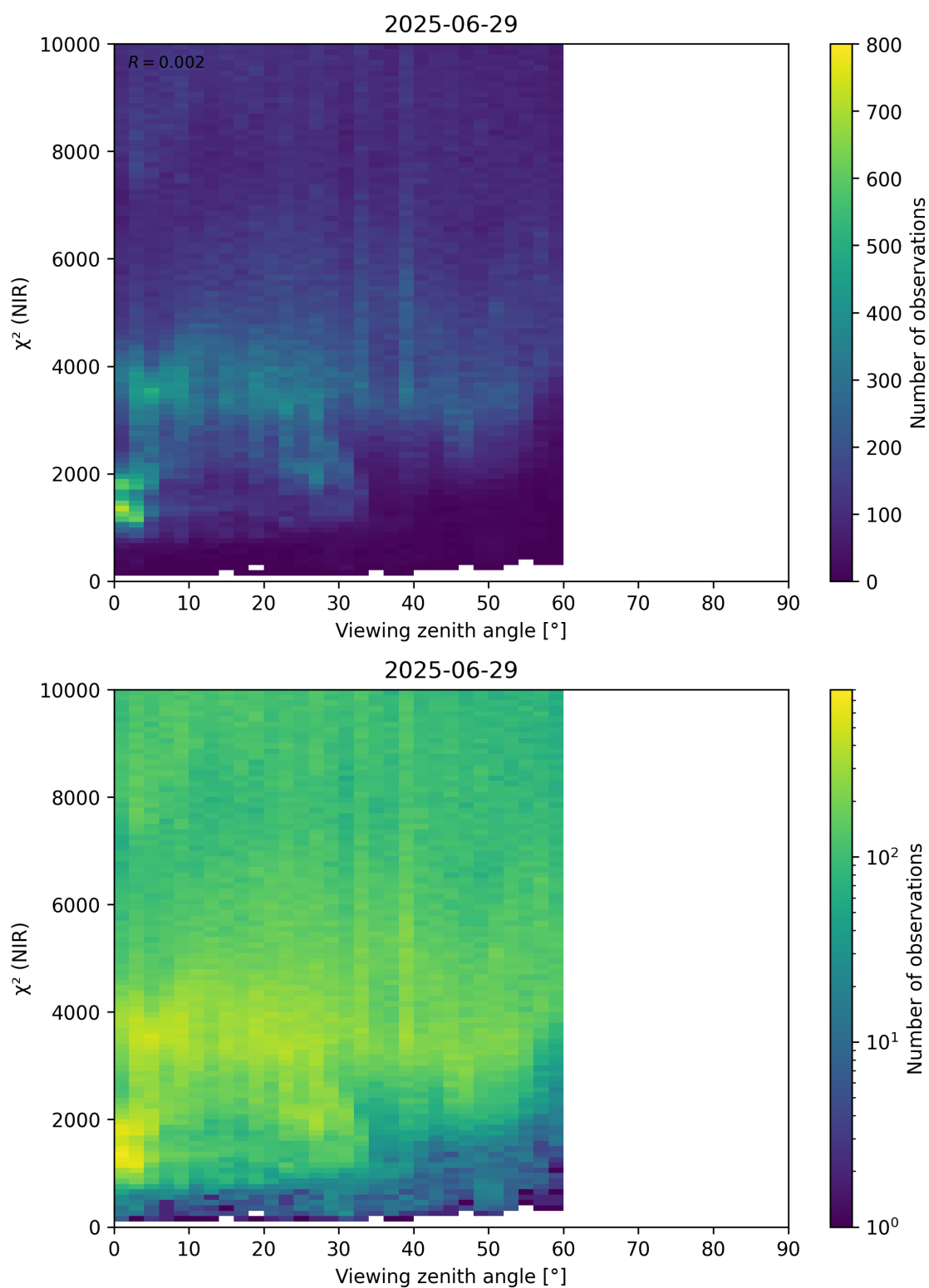
Figure 105: Scatter density plot of “Viewing zenith angle” against “ \chi^2 (NIR)” for 2025-06-28 to 2025-06-30.
