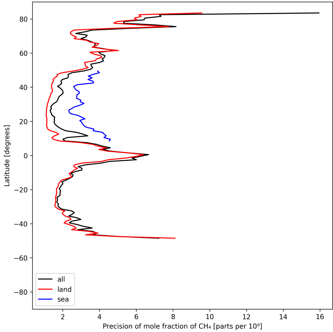
Figure 13: Zonal average of “Precision of mole fraction of CH 4 ” for 2025-06-28 to 2025-06-30.
