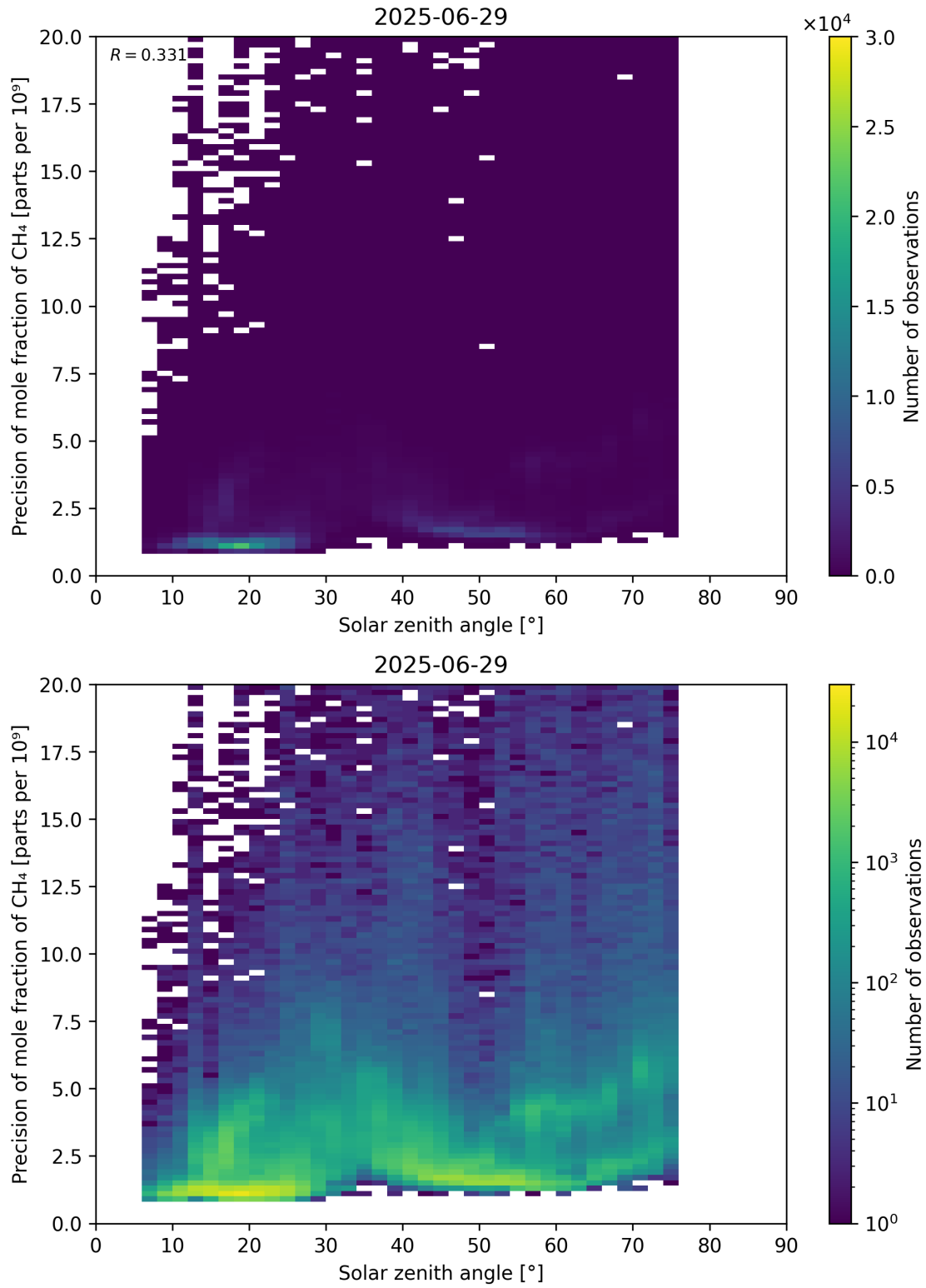
Figure 101: Scatter density plot of “Solar zenith angle” against “Precision of mole fraction of CH 4 ” for 2025-06-28 to 2025-06-30.
