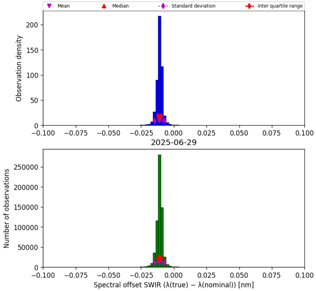
Figure 27: Histogram of “Spectral offset SWIR ( \lambda_{\text{true}} - \lambda_{\text{nominal}} )” for 2025-06-28 to 2025-06-30
