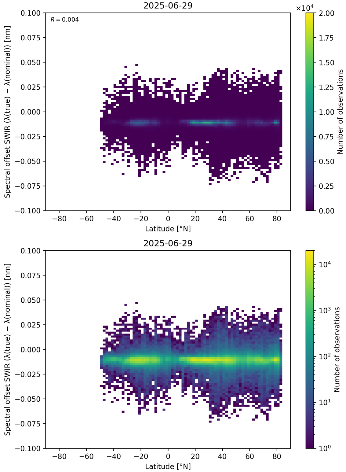
Figure 62: Scatter density plot of “Latitude” against “Spectral offset SWIR ( \lambda_{\text{true}} - \lambda_{\text{nominal}} )” for 2025-06-28 to 2025-06-30.
