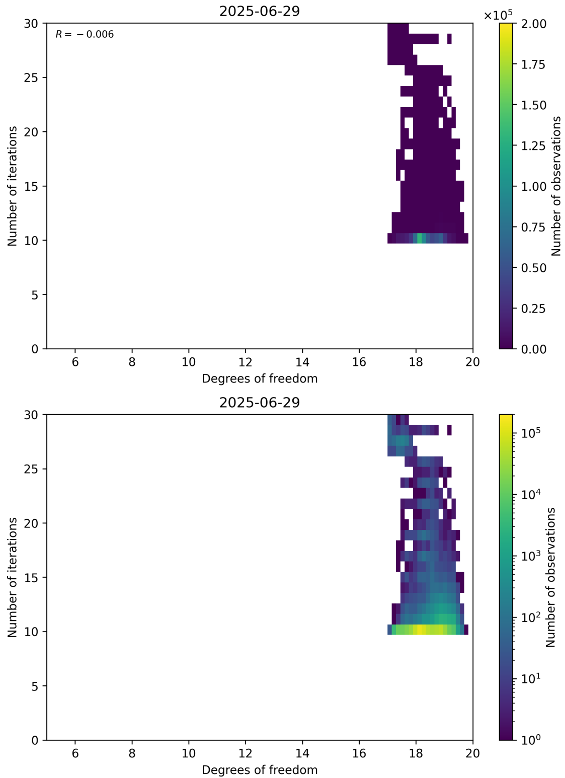
Figure 52: Scatter density plot of “Degrees of freedom” against “Number of iterations” for 2025-06-28 to 2025-06-30.
