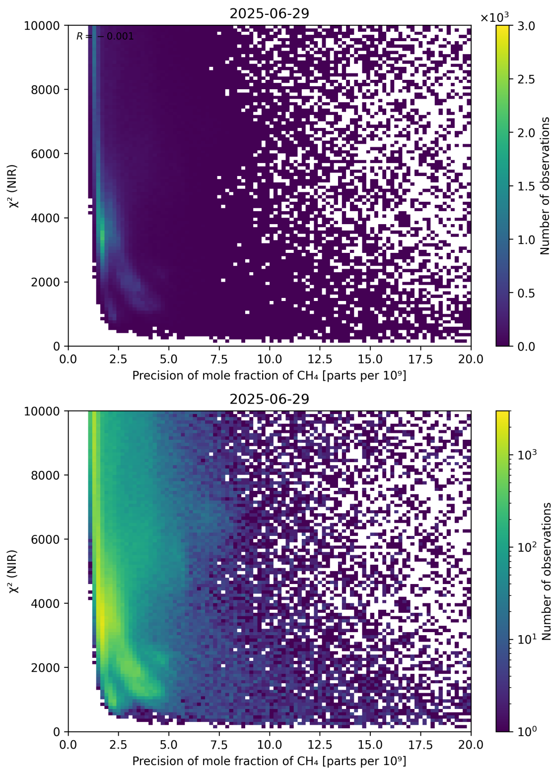
Figure 78: Scatter density plot of “Precision of mole fraction of CH 4 ” against “ \chi^2 (NIR)” for 2025-06-28 to 2025-06-30.
