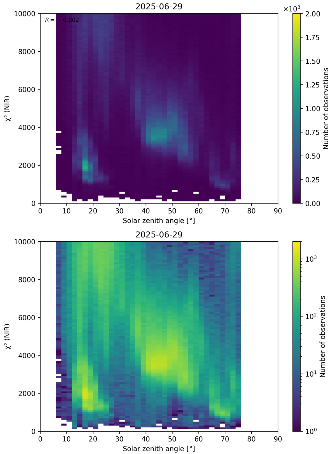
Figure 94: Scatter density plot of “Solar zenith angle” against “ \chi^2 (NIR)” for 2025-06-28 to 2025-06-30.
