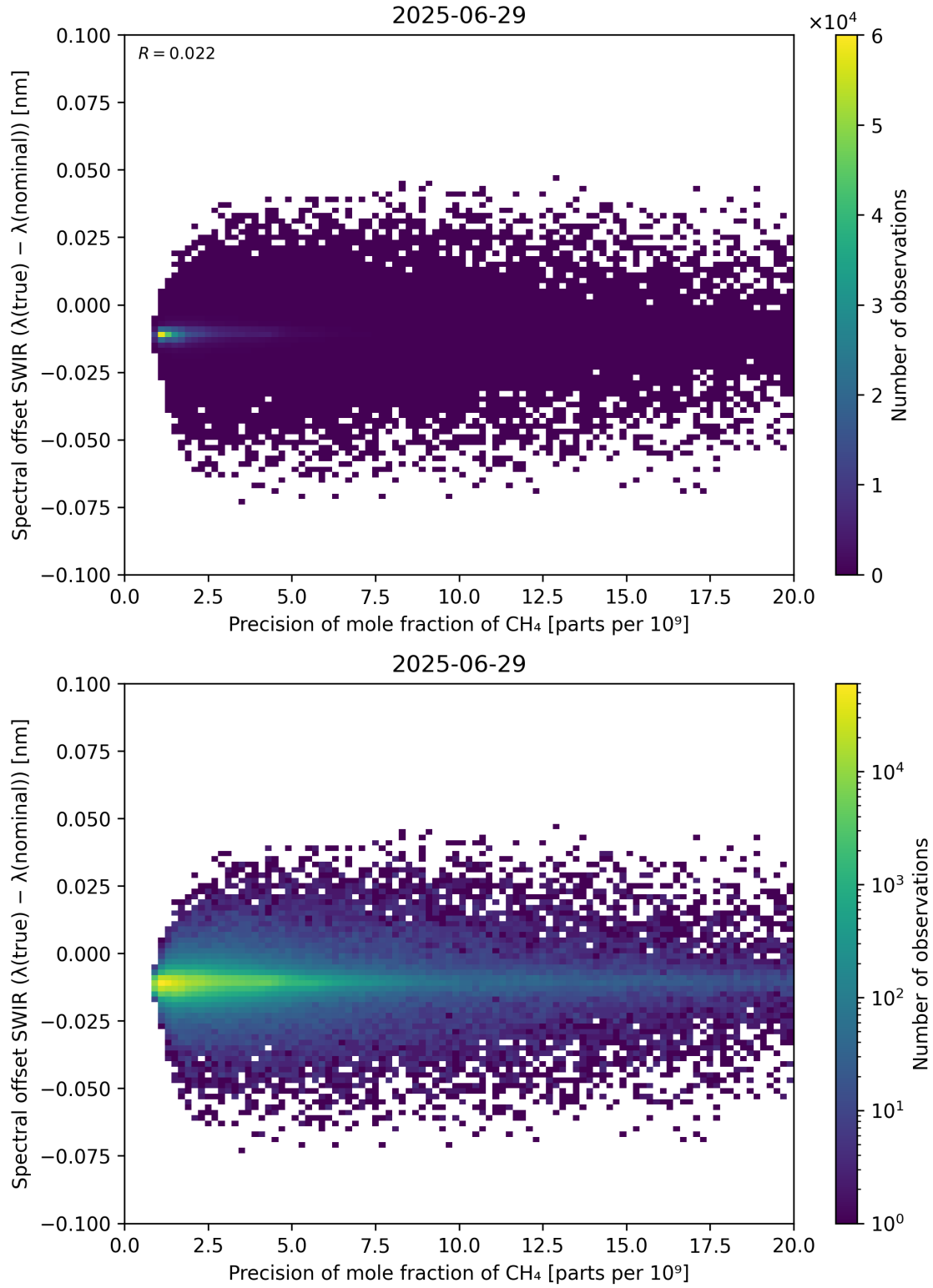
Figure 85: Scatter density plot of “Precision of mole fraction of CH 4 ” against “Spectral offset SWIR ( \lambda_{\text{true}} - \lambda_{\text{nominal}} )” for 2025-06-28 to 2025-06-30.
