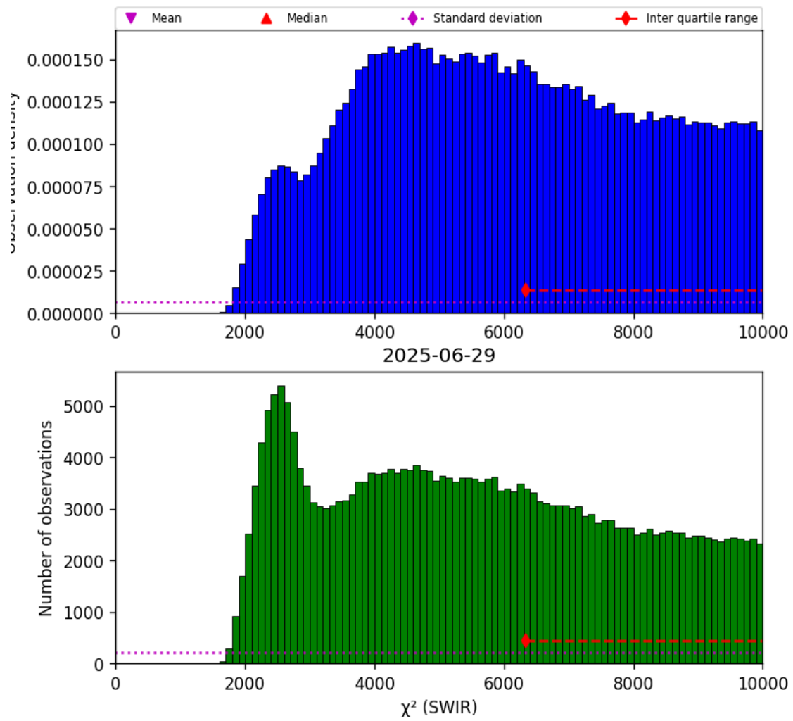
Figure 28: Histogram of “ \chi^2 (SWIR)” for 2025-06-28 to 2025-06-30
