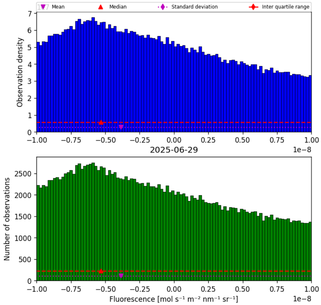
Figure 32: Histogram of “Fluorescence” for 2025-06-28 to 2025-06-30
