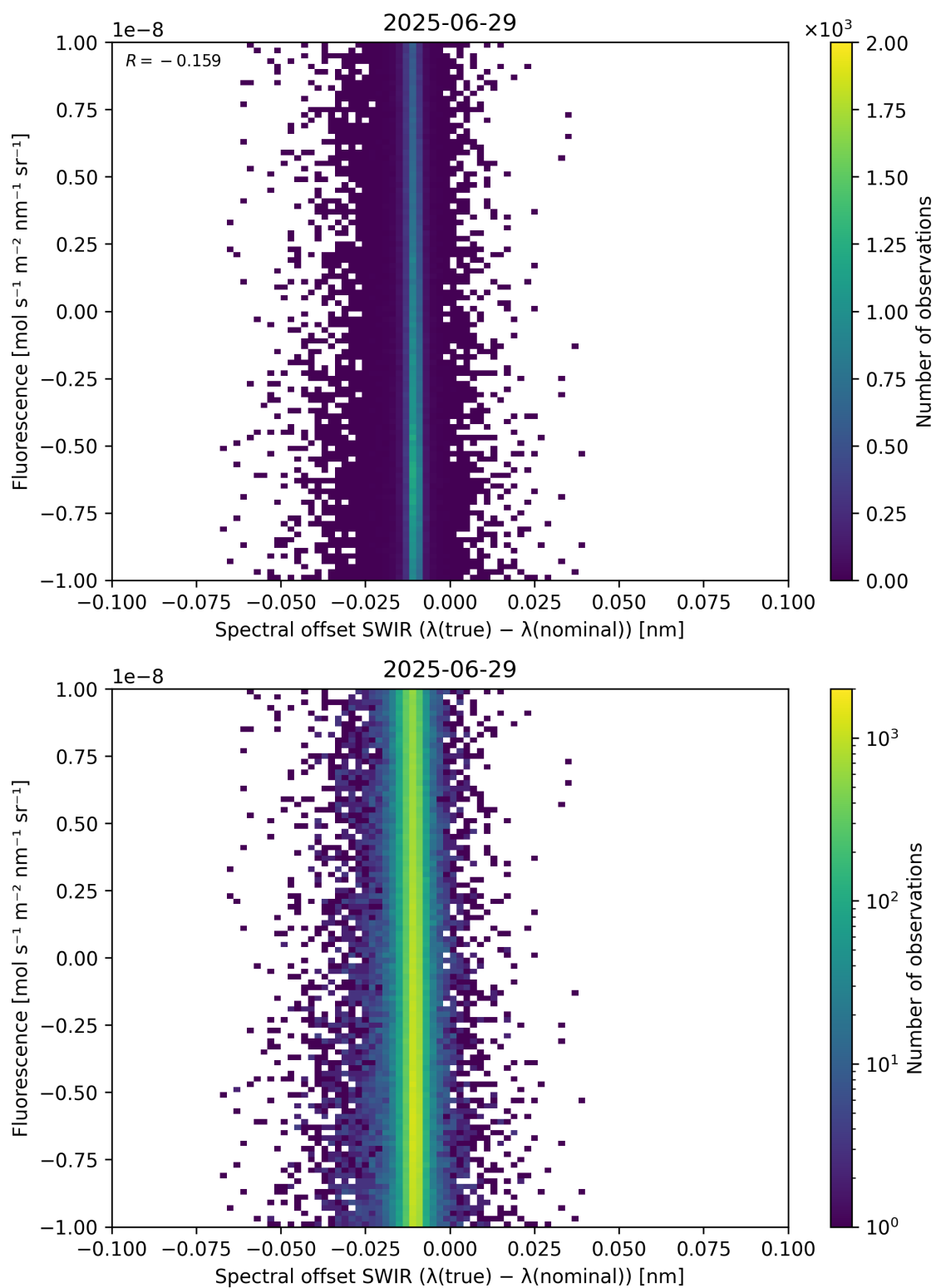
Figure 120: Scatter density plot of “Spectral offset SWIR ( \lambda_{\text{true}} - \lambda_{\text{nominal}} )” against “Fluorescence” for 2025-06-28 to 2025-06-30.
