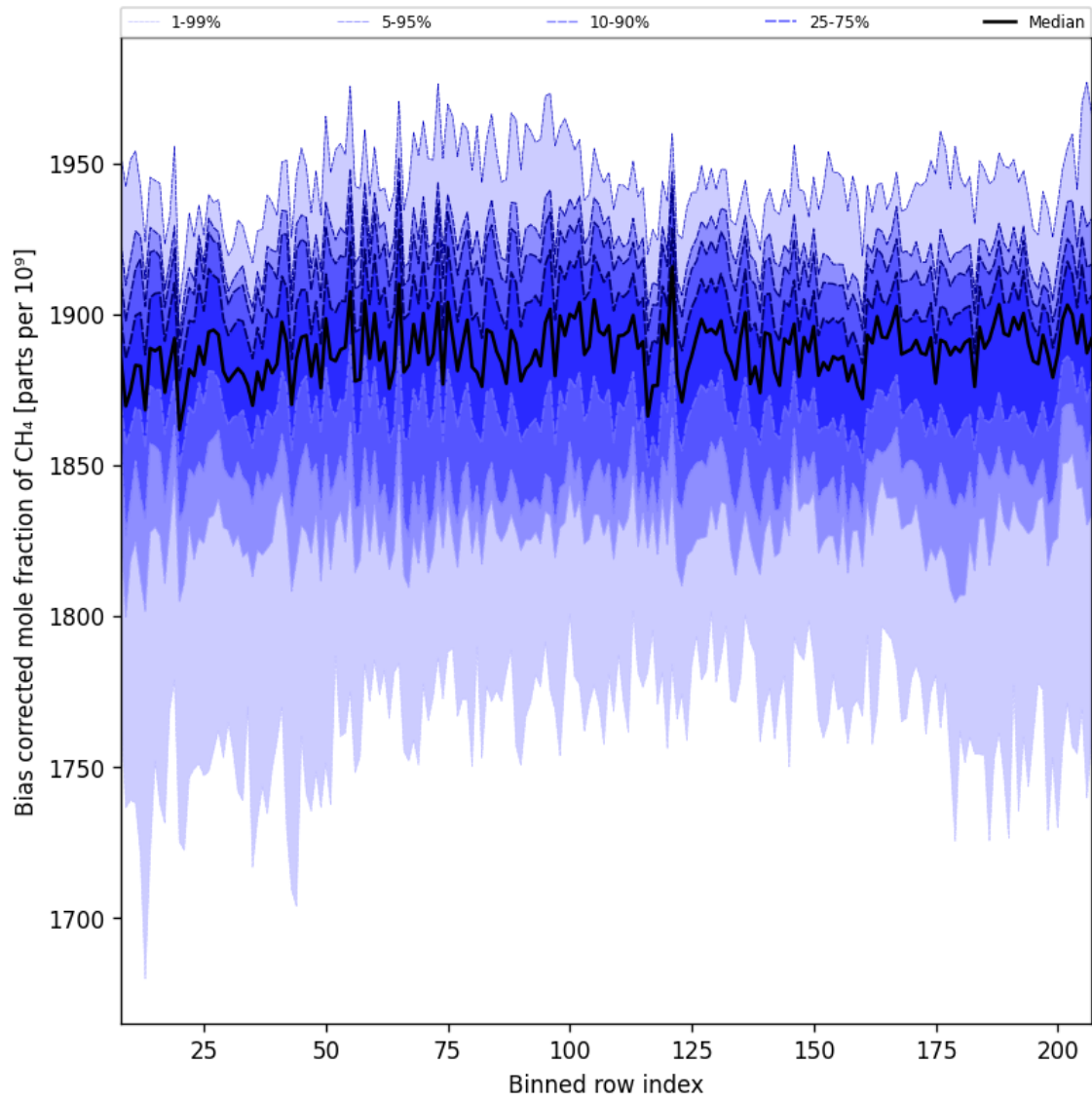
Figure 36: Along track statistics of “Bias corrected mole fraction of CH 4 ” for 2025-06-28 to 2025-06-30
