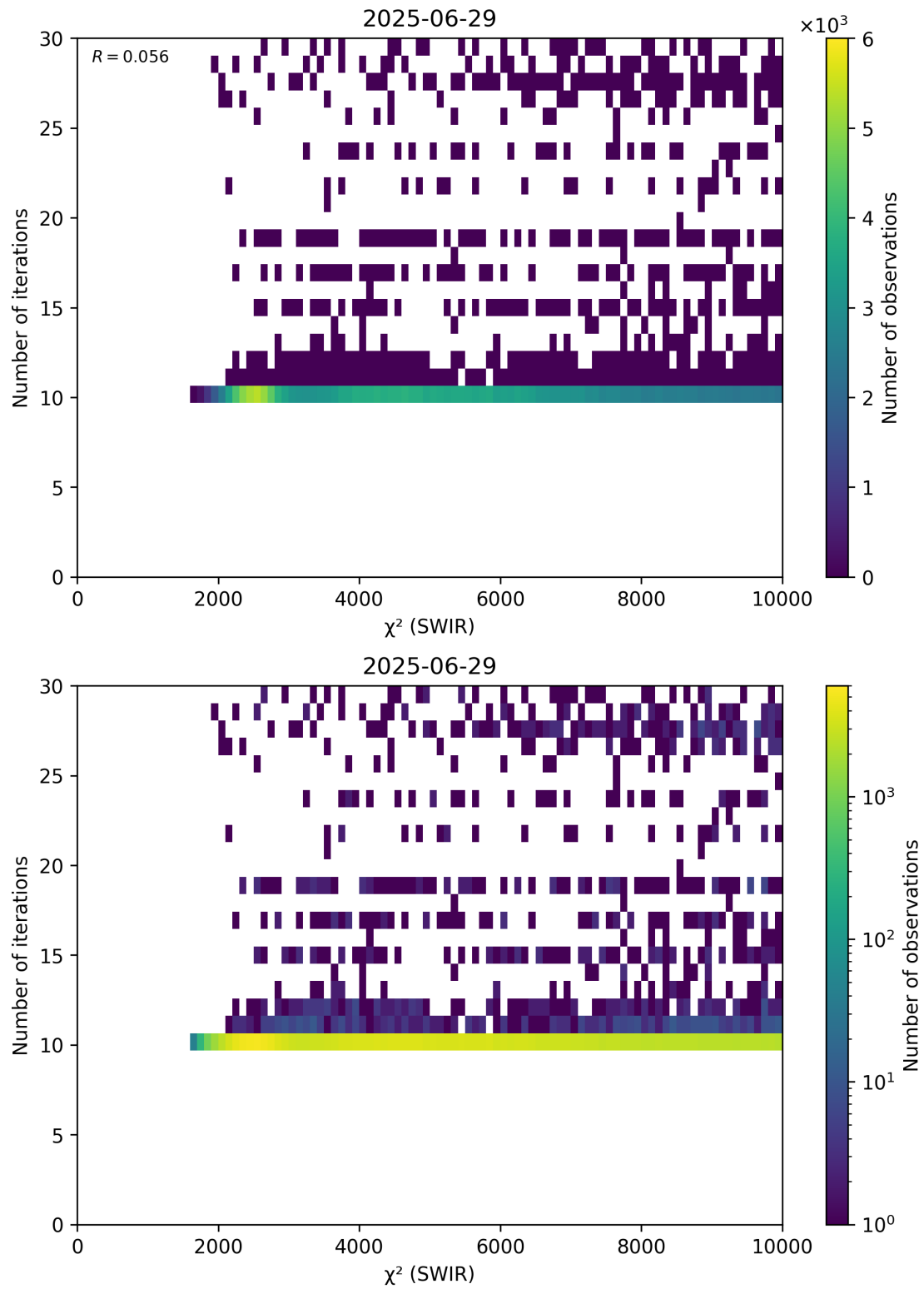
Figure 50: Scatter density plot of “ \chi^2 (SWIR)” against “Number of iterations” for 2025-06-28 to 2025-06-30.
