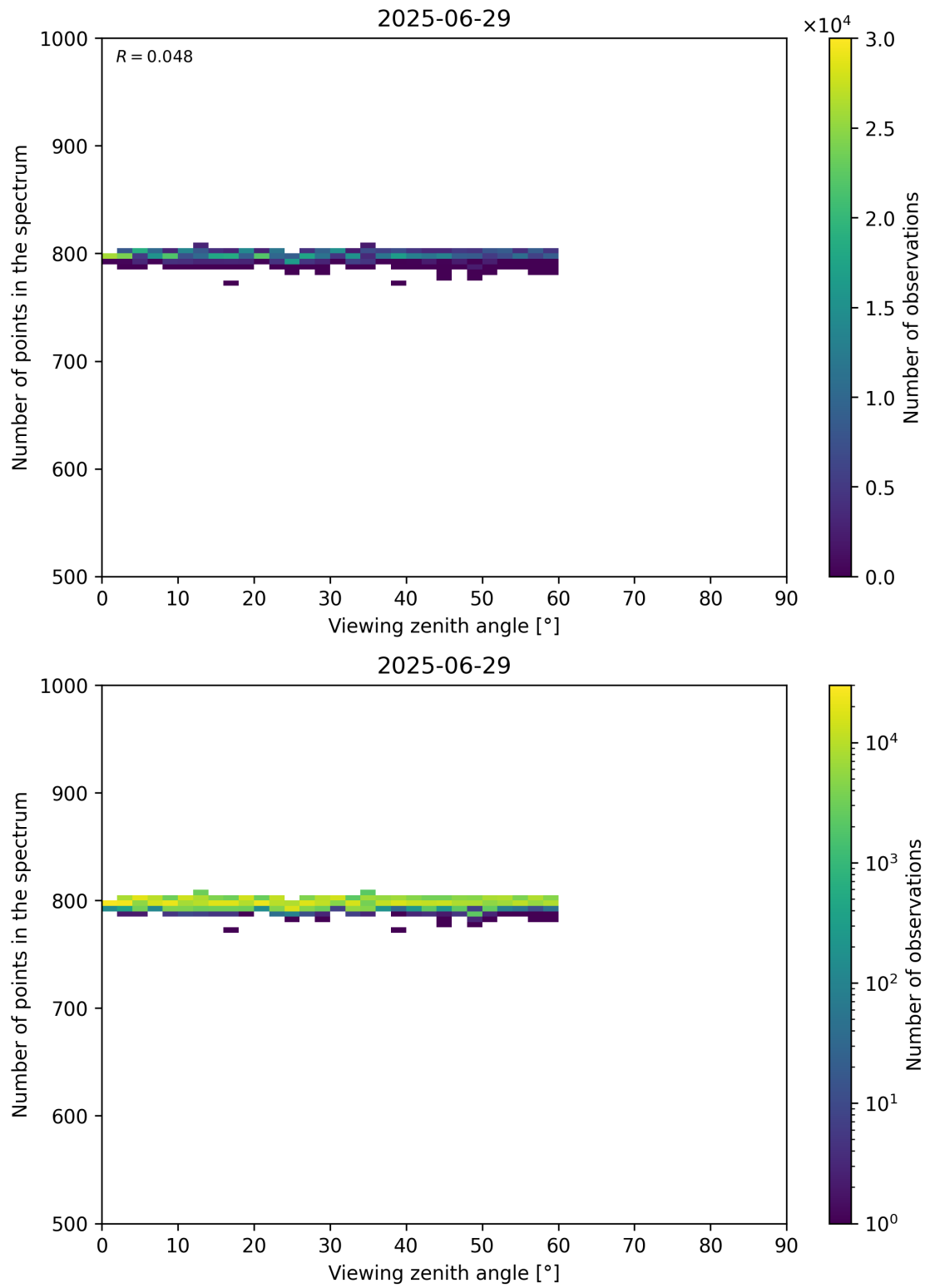
Figure 114: Scatter density plot of “Viewing zenith angle” against “Number of points in the spectrum” for 2025-06-28 to 2025-06-30.
