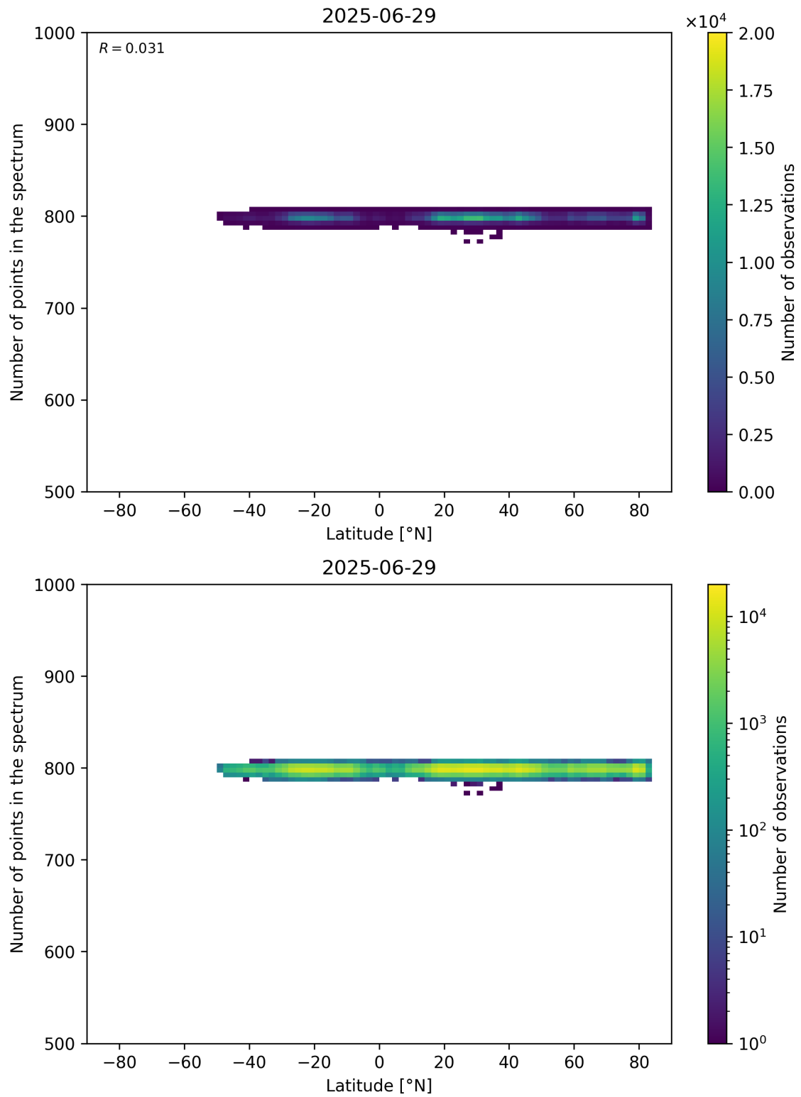
Figure 61: Scatter density plot of “Latitude” against “Number of points in the spectrum” for 2025-06-28 to 2025-06-30.
