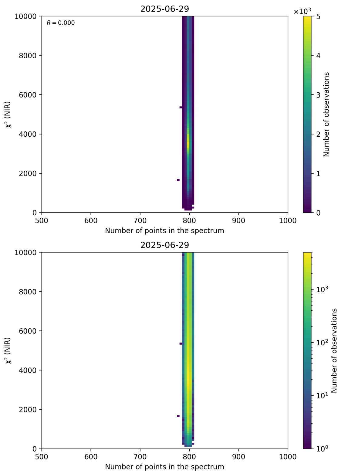
Figure 88: Scatter density plot of “Number of points in the spectrum” against “ \chi^2 (NIR)” for 2025-06-28 to 2025-06-30.
