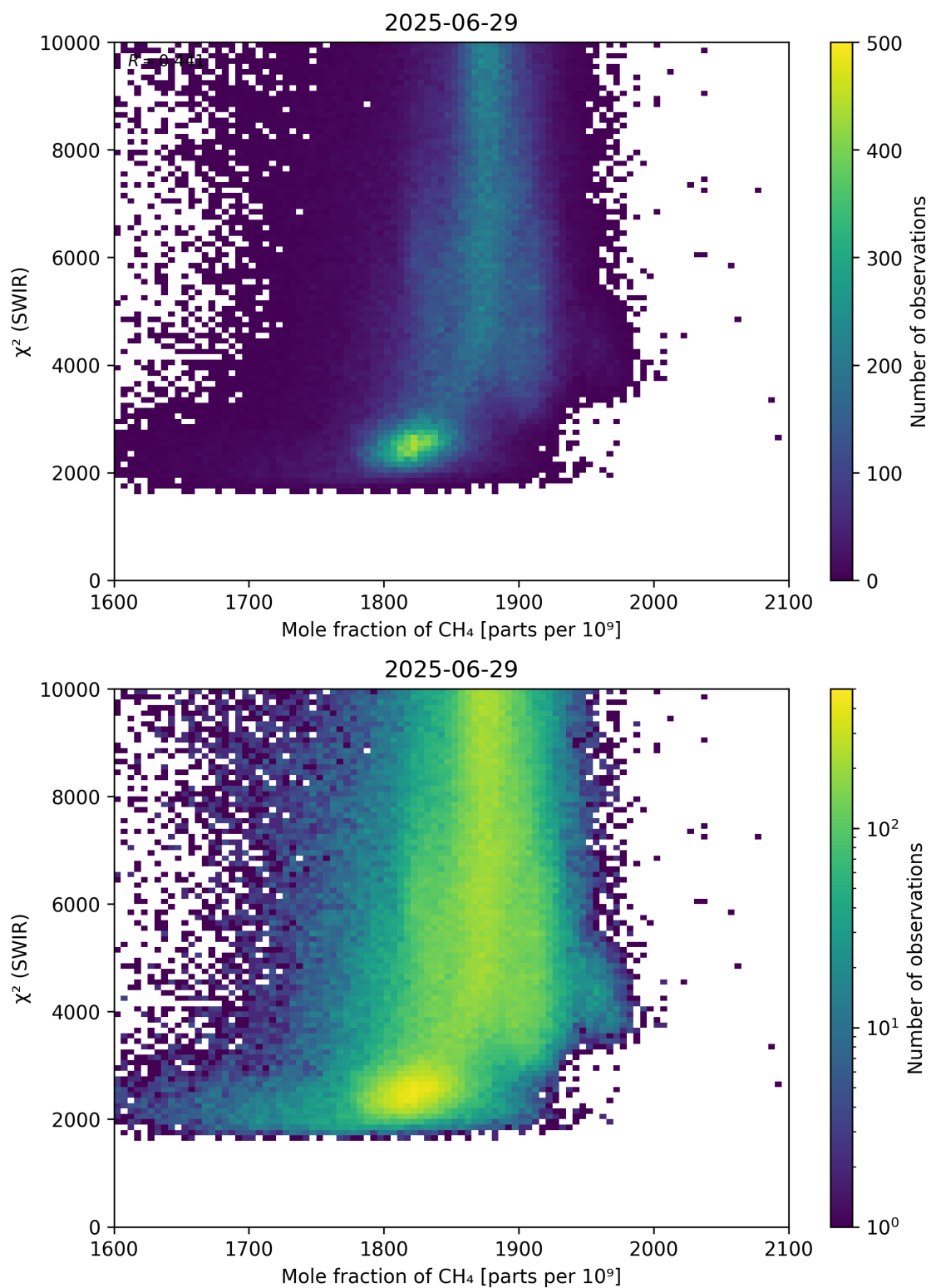
Figure 71: Scatter density plot of “Mole fraction of CH 4 ” against “ \chi^2 (SWIR)” for 2025-06-28 to 2025-06-30.
