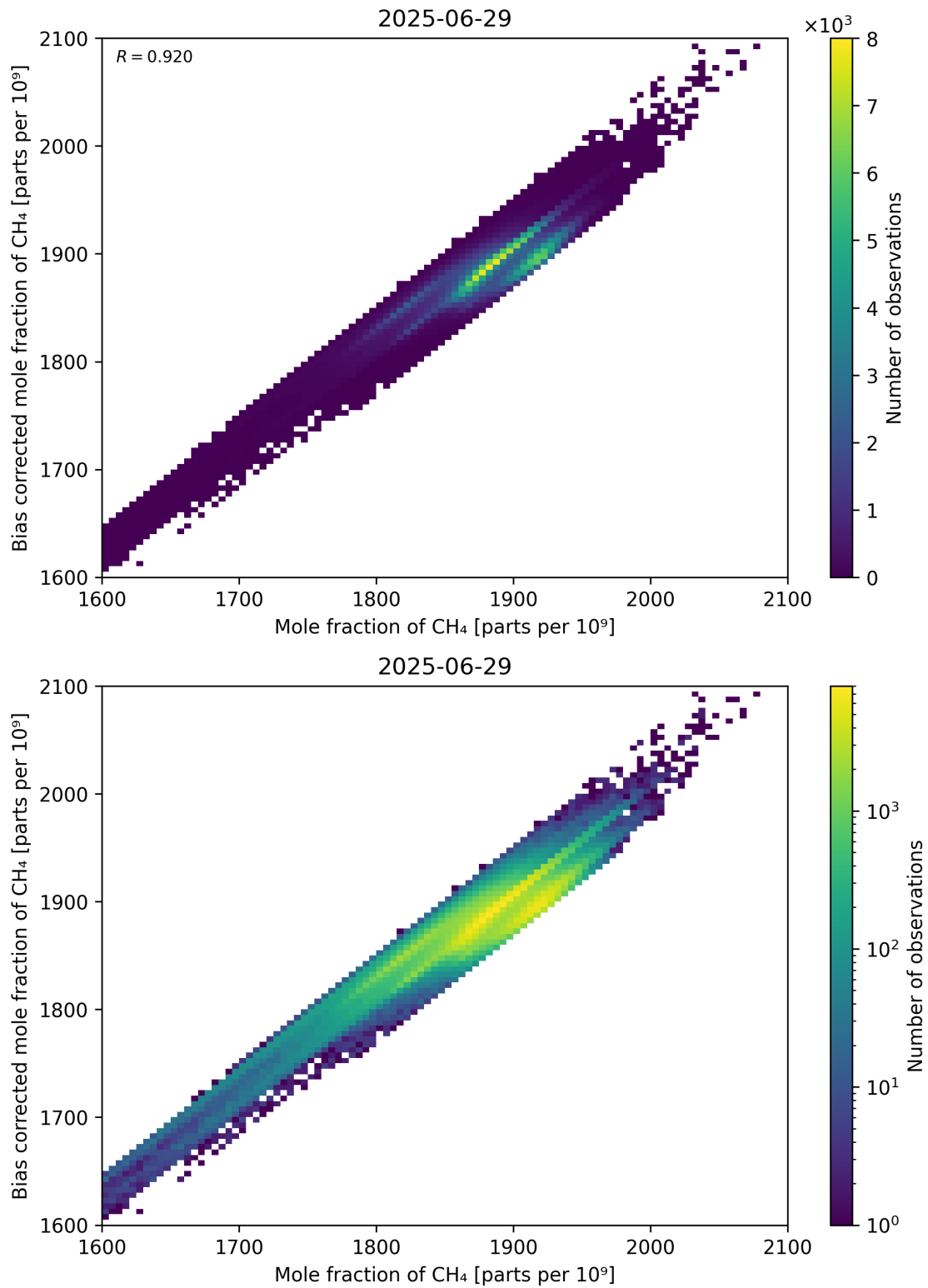
Figure 74: Scatter density plot of “Mole fraction of CH 4 ” against “Bias corrected mole fraction of CH 4 ” for 2025-06-28 to 2025-06-30.
