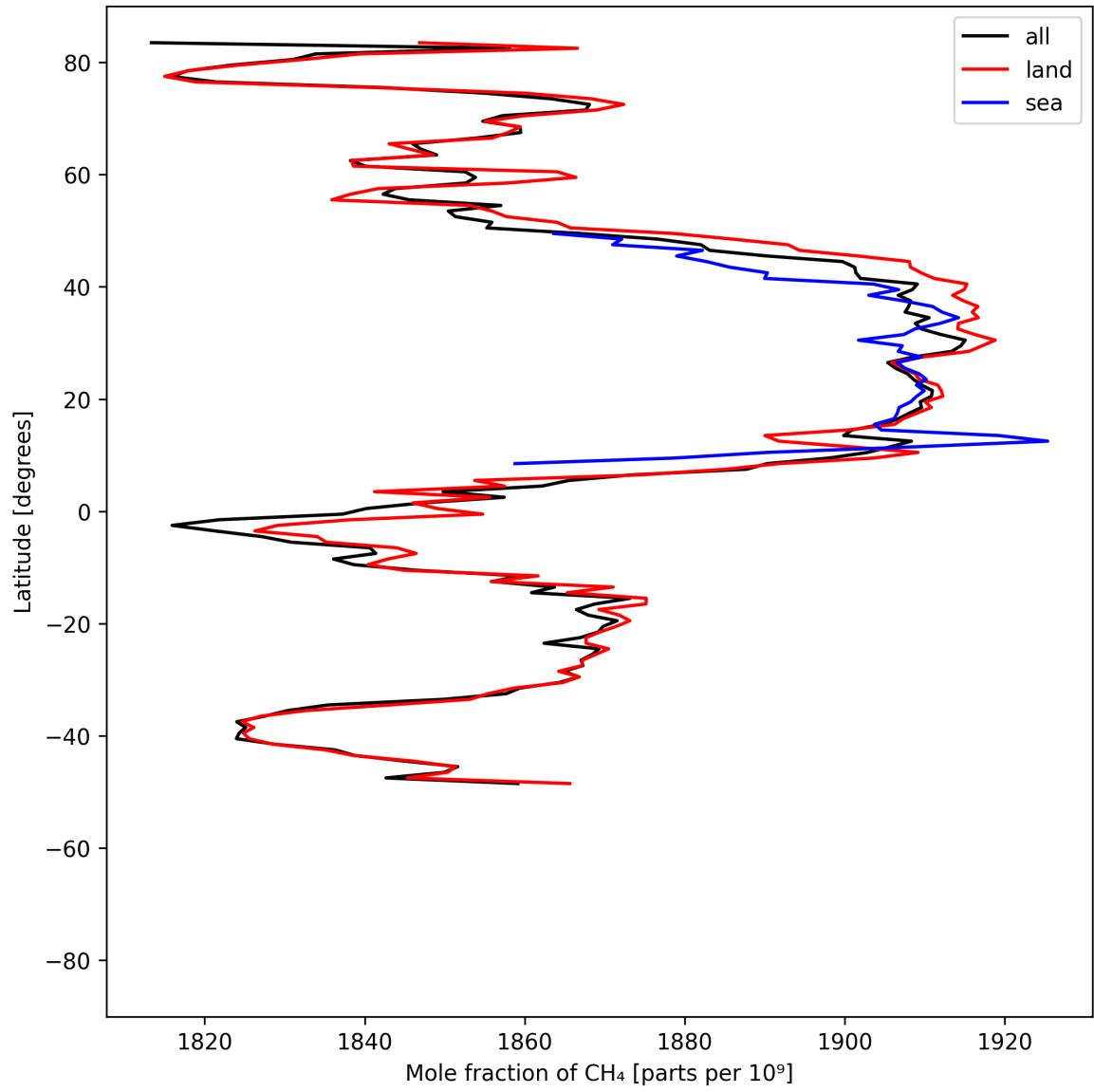
Figure 12: Zonal average of “Mole fraction of \text{CH}_4 ” for 2025-06-28 to 2025-06-30.
