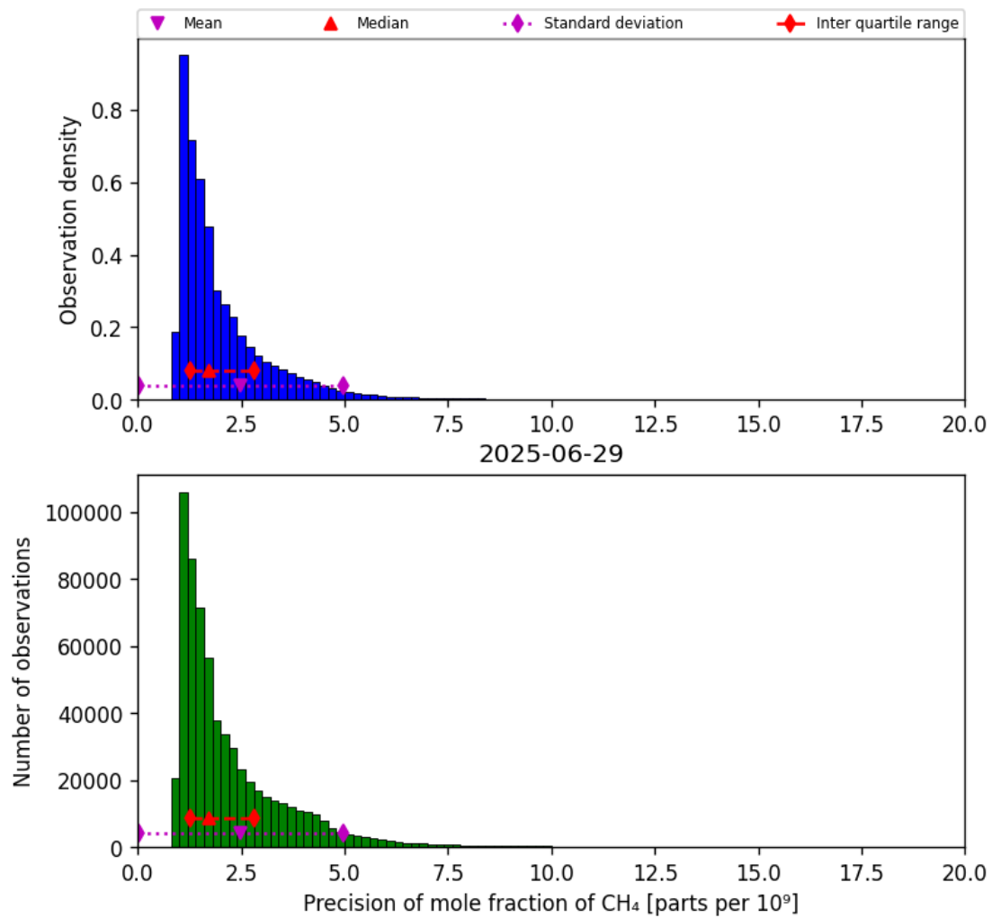
Figure 24: Histogram of “Precision of mole fraction of CH 4 ” for 2025-06-28 to 2025-06-30
