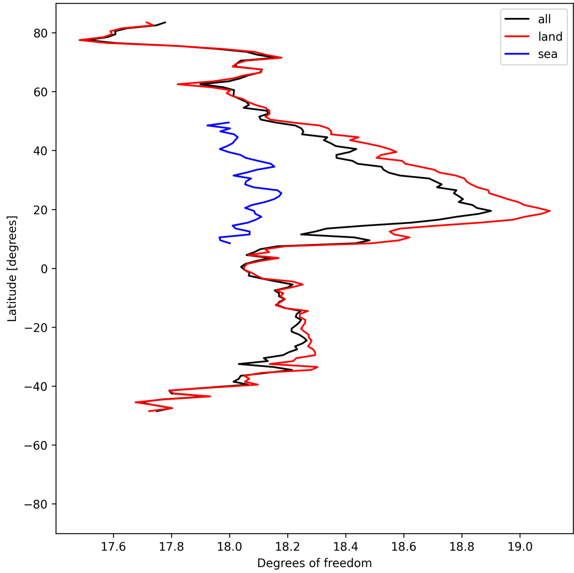
Figure 19: Zonal average of “Degrees of freedom” for 2025-06-28 to 2025-06-30.
