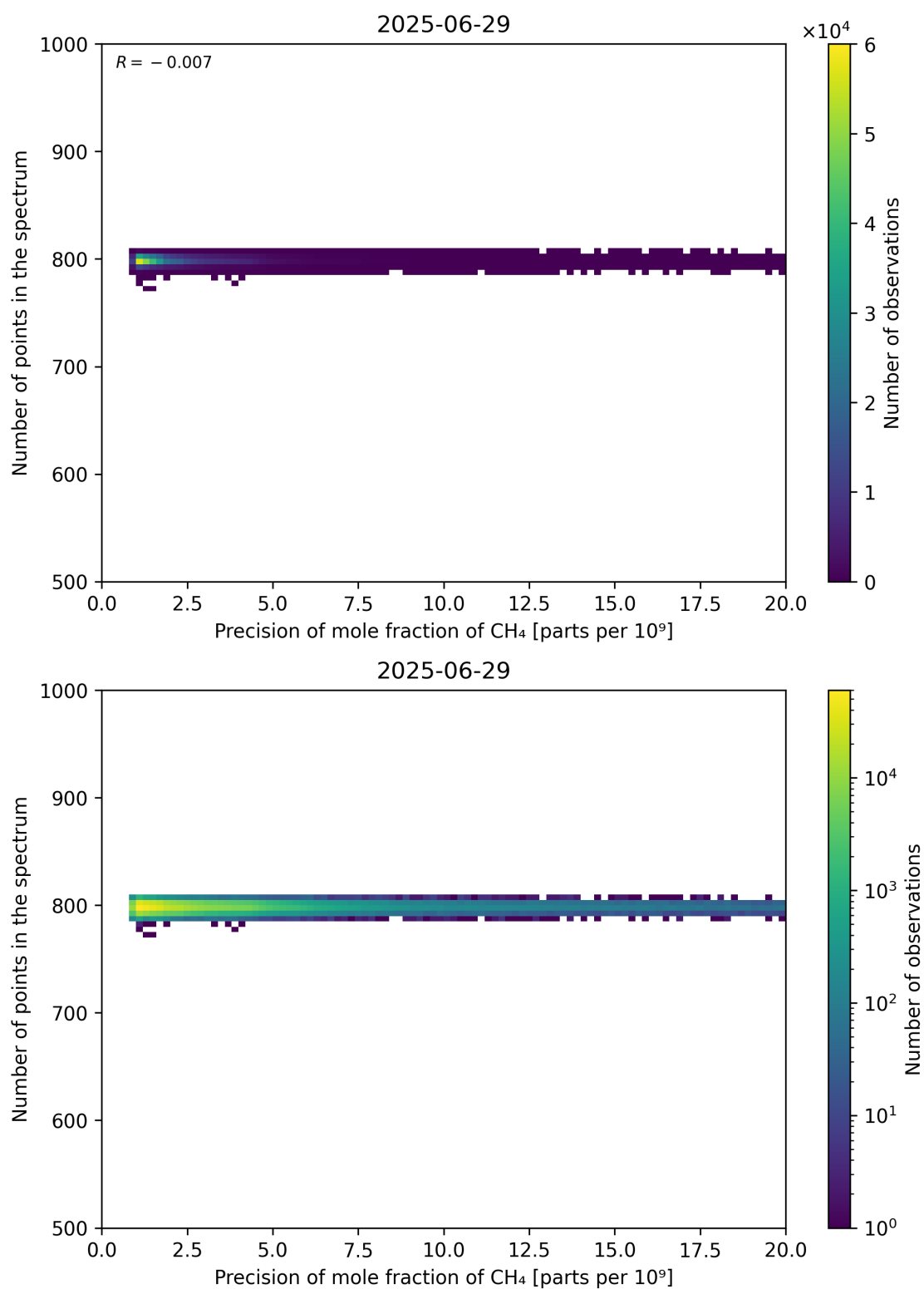
Figure 84: Scatter density plot of “Precision of mole fraction of CH 4 ” against “Number of points in the spectrum” for 2025-06-28 to 2025-06-30.
