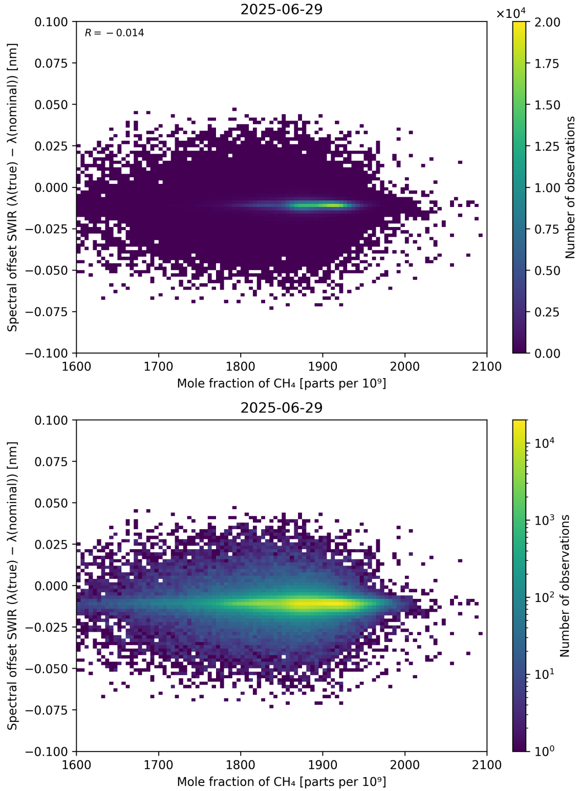
Figure 86: Scatter density plot of “Mole fraction of CH 4 ” against “Spectral offset SWIR ( \lambda_{\text{true}} - \lambda_{\text{nominal}} )” for 2025-06-28 to 2025-06-30.
