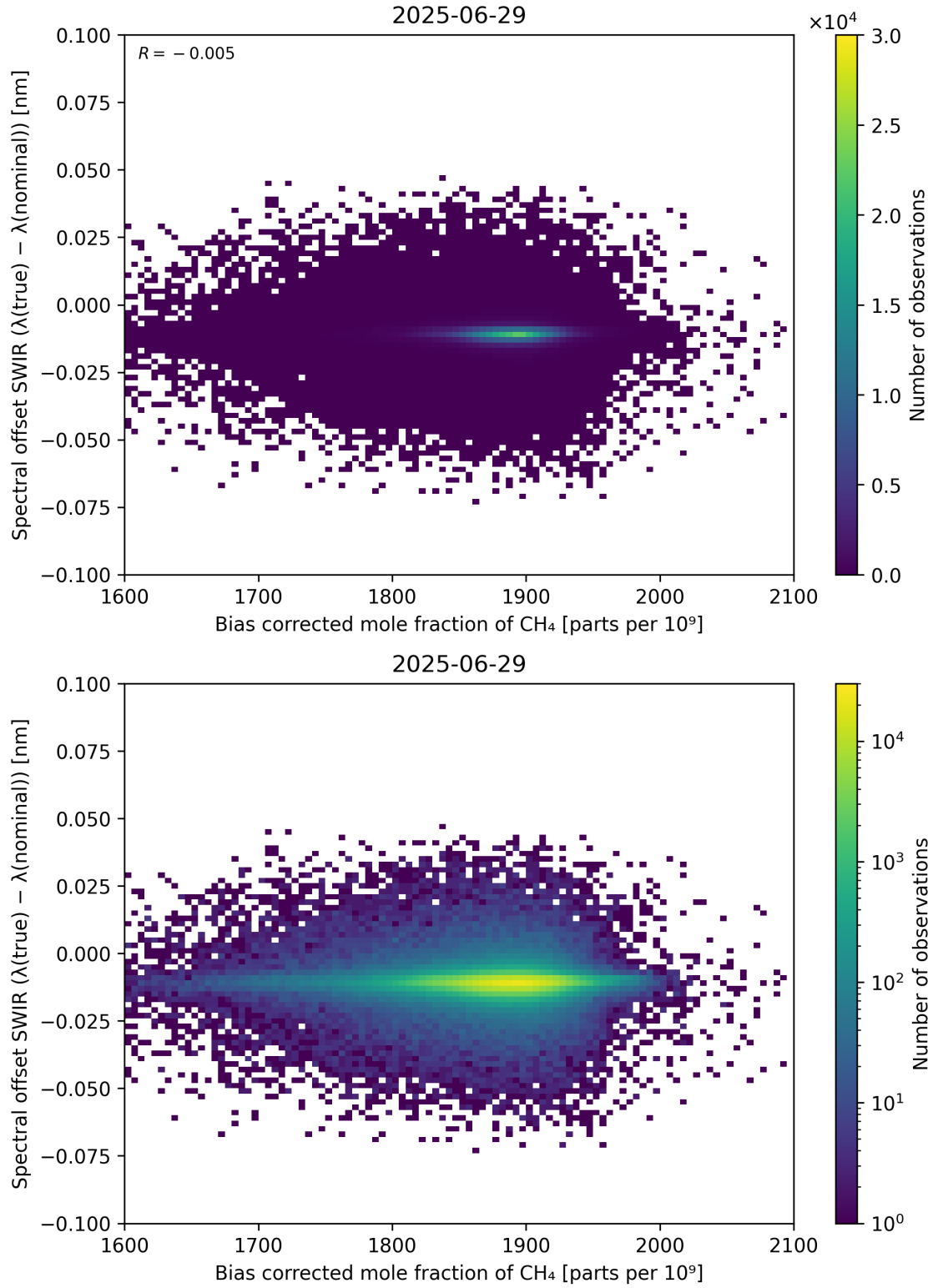
Figure 69: Scatter density plot of “Bias corrected mole fraction of \text{CH}_4 ” against “Spectral offset SWIR ( \lambda_{\text{true}} - \lambda_{\text{nominal}} )” for 2025-06-28 to 2025-06-30.
