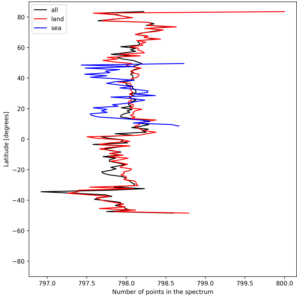
Figure 15: Zonal average of “Number of points in the spectrum” for 2025-06-28 to 2025-06-30.
