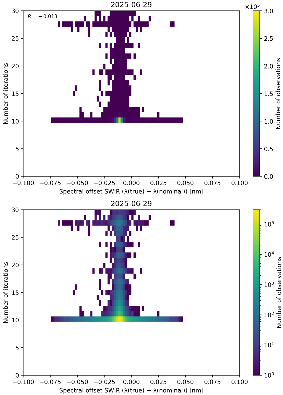
Figure 121: Scatter density plot of “Spectral offset SWIR ( \lambda_{\text{true}} - \lambda_{\text{nominal}} )” against “Number of iterations” for 2025-06-28 to 2025-06-30.
