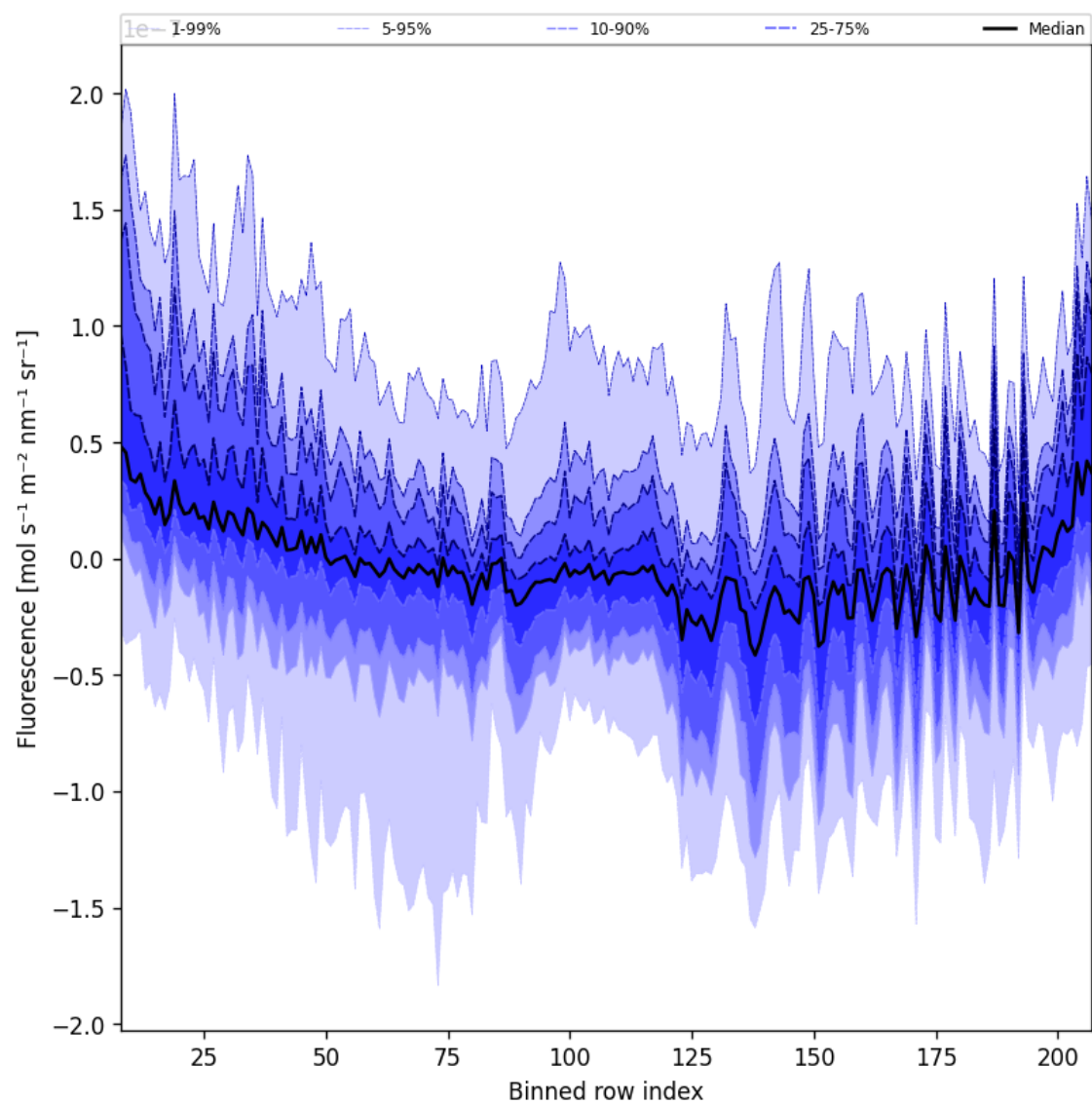
Figure 43: Along track statistics of “Fluorescence” for 2025-06-28 to 2025-06-30
