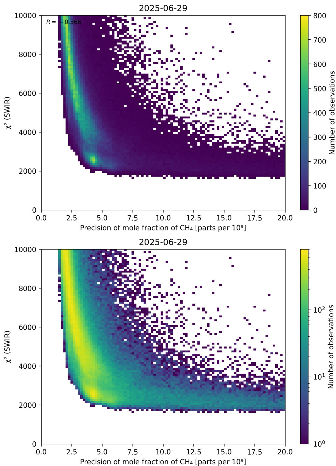
Figure 79: Scatter density plot of “Precision of mole fraction of CH 4 ” against “ \chi^2 (SWIR)” for 2025-06-28 to 2025-06-30.
