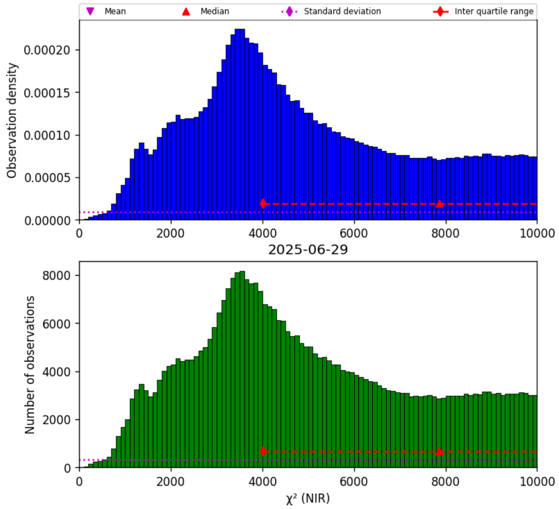
Figure 29: Histogram of " \chi^2 (NIR)" for 2025-06-28 to 2025-06-30
