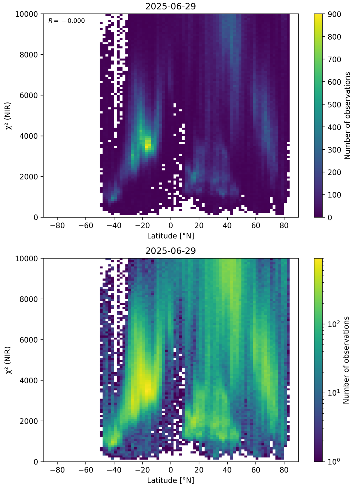
Figure 53: Scatter density plot of “Latitude” against “ \chi^2 (NIR)” for 2025-06-28 to 2025-06-30.
