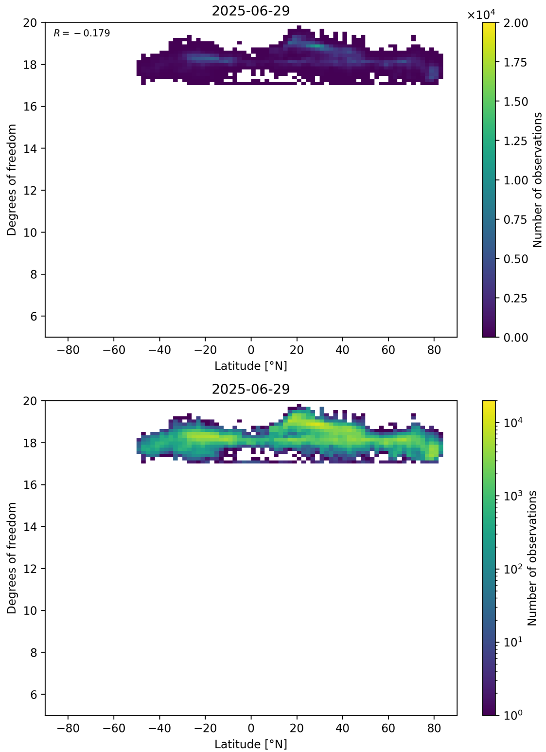
Figure 55: Scatter density plot of “Latitude” against “Degrees of freedom” for 2025-06-28 to 2025-06-30.
