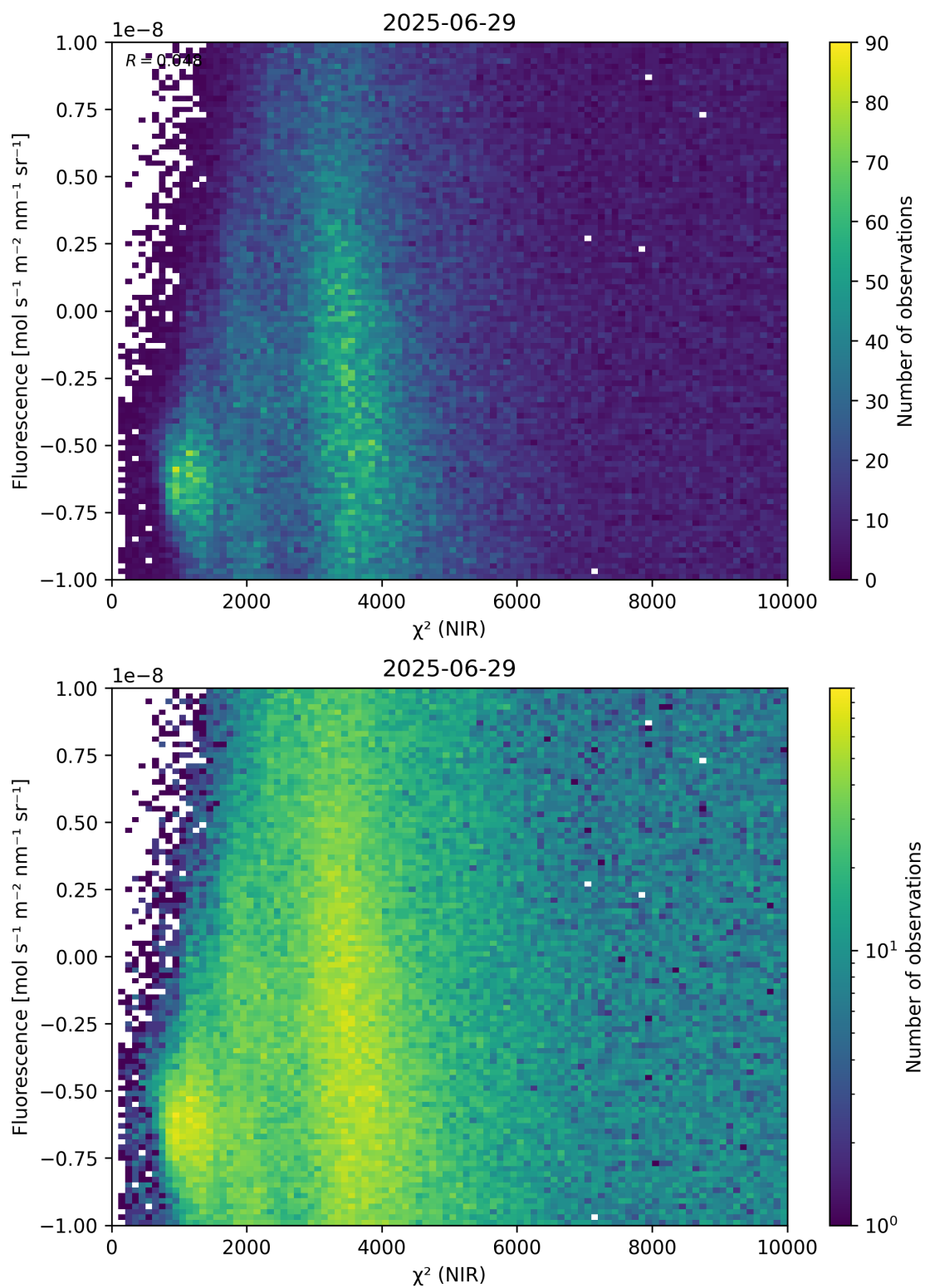
Figure 45: Scatter density plot of “ \chi^2 (NIR)” against “Fluorescence” for 2025-06-28 to 2025-06-30.
