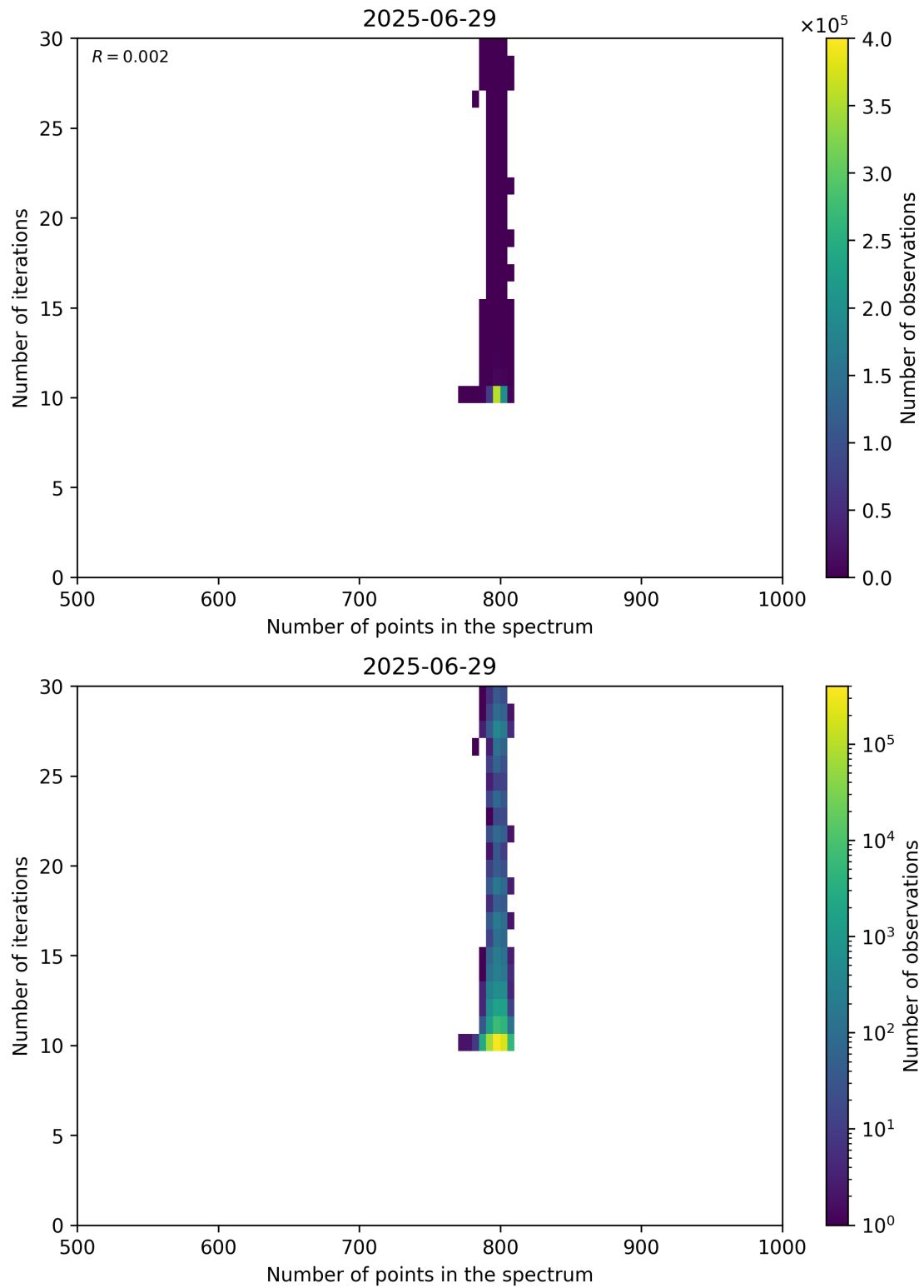
Figure 92: Scatter density plot of “Number of points in the spectrum” against “Number of iterations” for 2025-06-28 to 2025-06-30.
