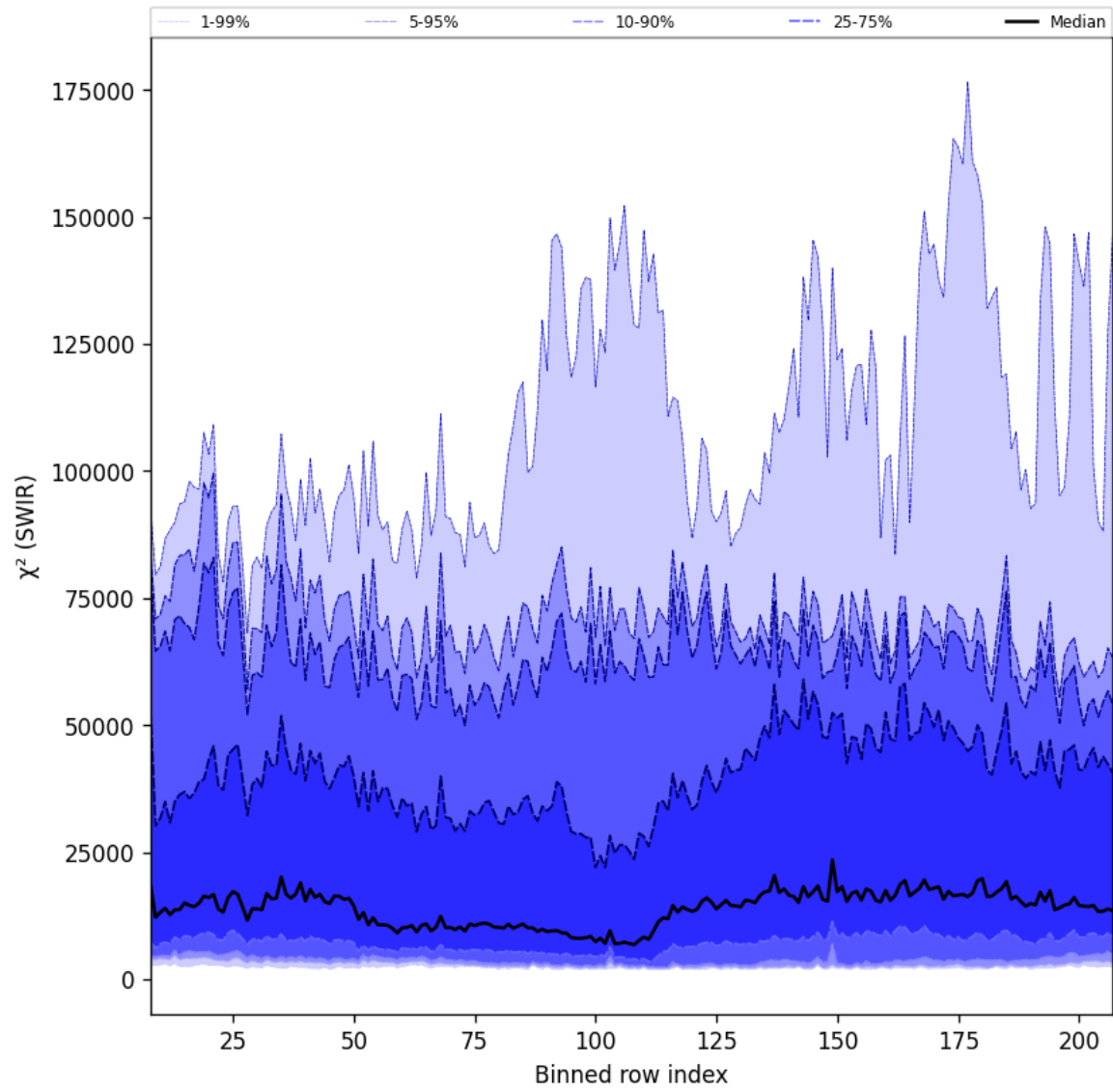
Figure 39: Along track statistics of " \chi^2 (SWIR)" for 2025-06-28 to 2025-06-30
