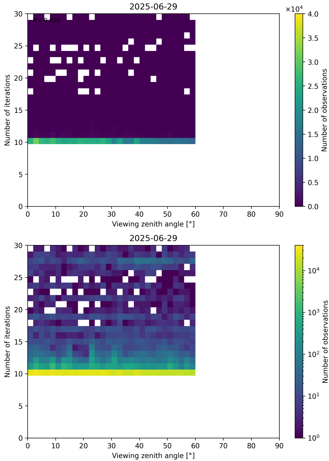
Figure 113: Scatter density plot of “Viewing zenith angle” against “Number of iterations” for 2025-06-28 to 2025-06-30.
