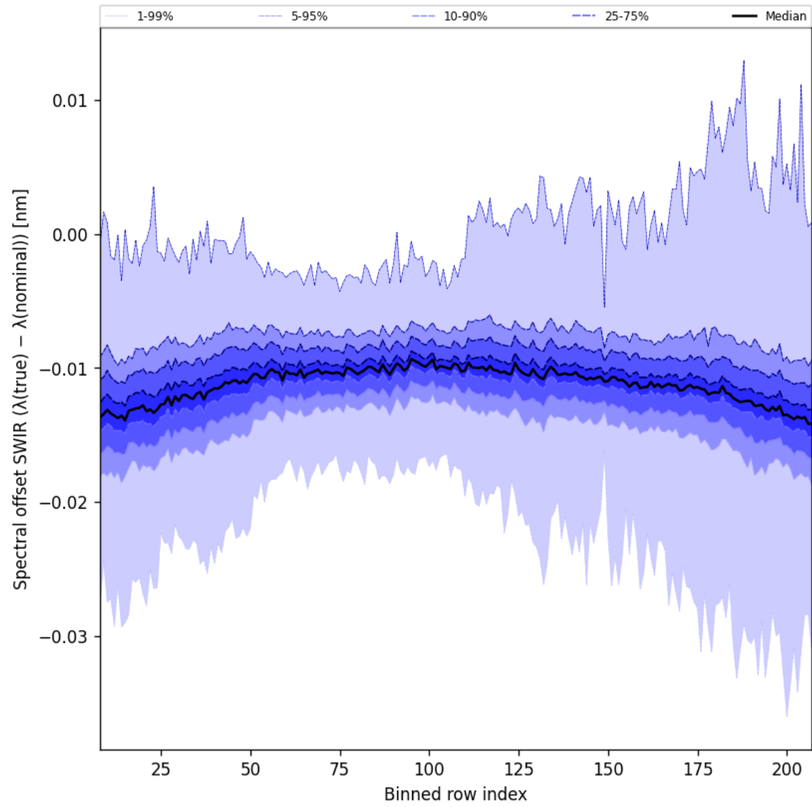
Figure 38: Along track statistics of “Spectral offset SWIR ( \lambda_{\text{true}} - \lambda_{\text{nominal}} )” for 2025-06-28 to 2025-06-30
