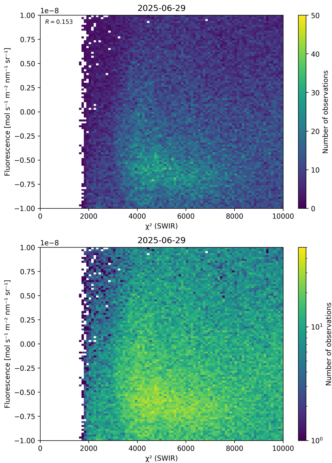
Figure 49: Scatter density plot of “ \chi^2 (SWIR)” against “Fluorescence” for 2025-06-28 to 2025-06-30.
