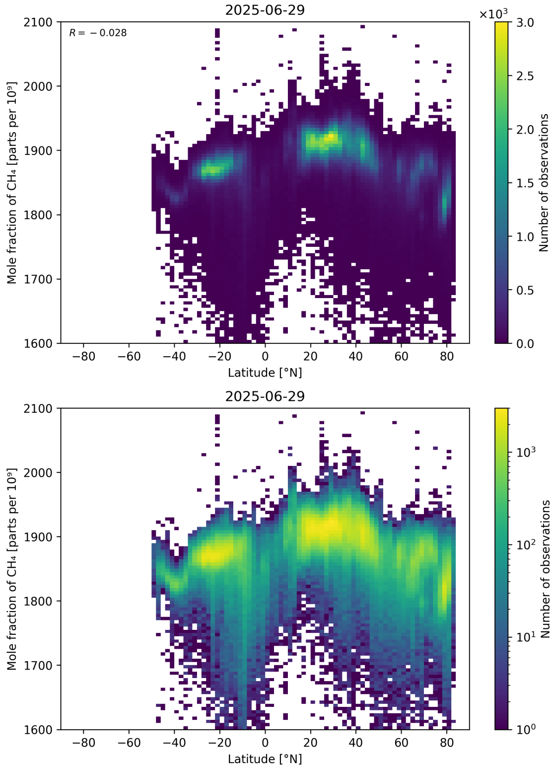
Figure 57: Scatter density plot of “Latitude” against “Mole fraction of \text{CH}_4 ” for 2025-06-28 to 2025-06-30.
