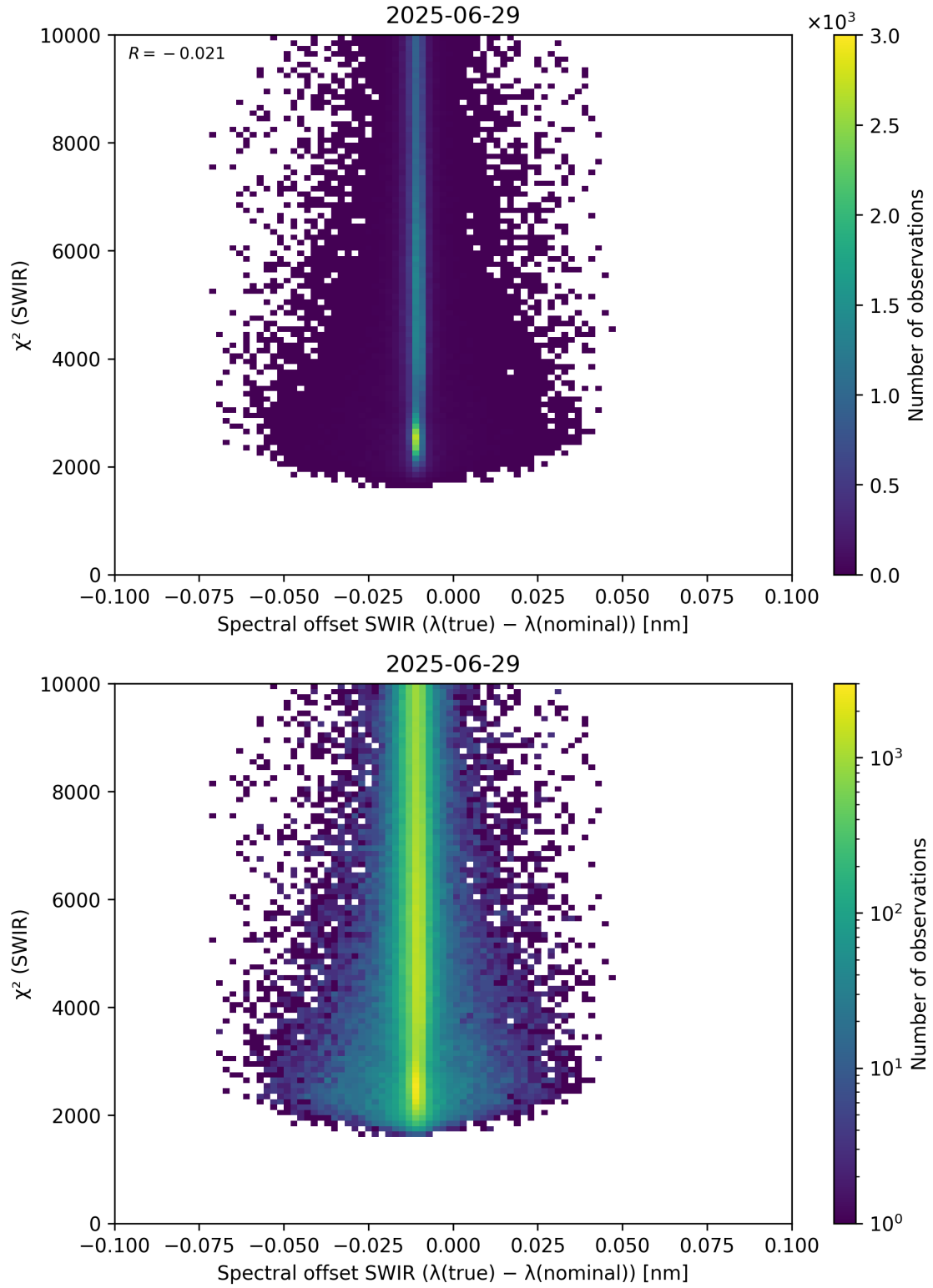
Figure 118: Scatter density plot of “Spectral offset SWIR ( \lambda_{\text{true}} - \lambda_{\text{nominal}} )” against “ \chi^2 (SWIR)” for 2025-06-28 to 2025-06-30.
