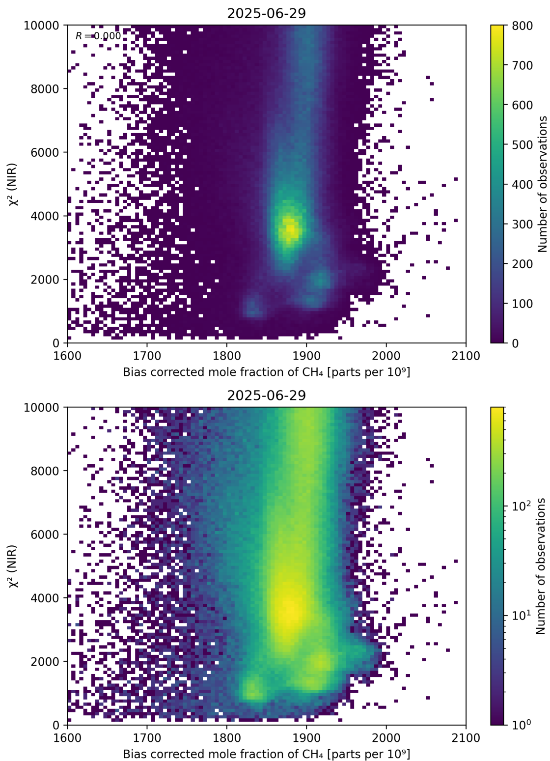
Figure 63: Scatter density plot of “Bias corrected mole fraction of CH 4 ” against “ \chi^2 (NIR)” for 2025-06-28 to 2025-06-30.
