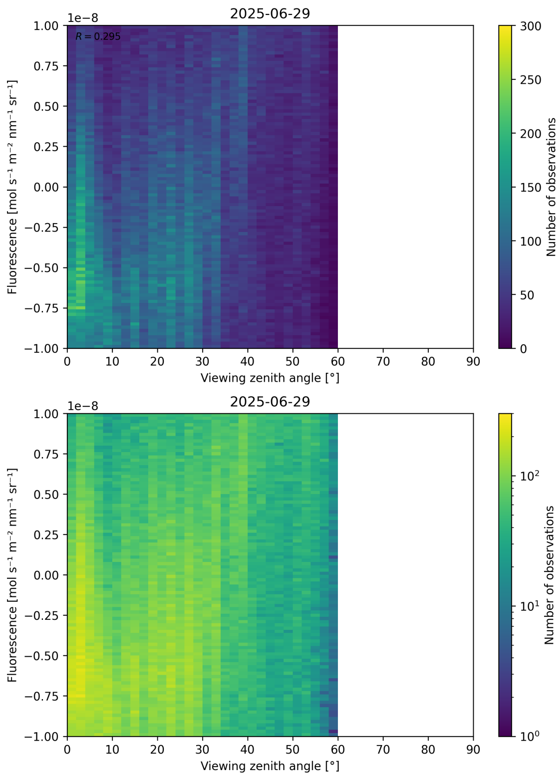
Figure 108: Scatter density plot of “Viewing zenith angle” against “Fluorescence” for 2025-06-28 to 2025-06-30.
