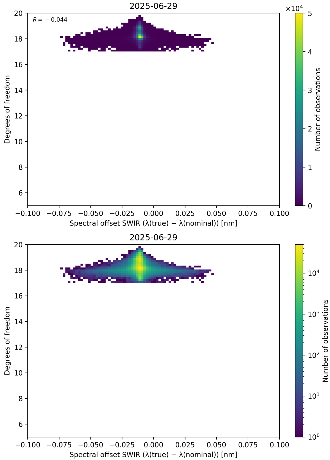
Figure 119: Scatter density plot of “Spectral offset SWIR ( \lambda_{\text{true}} - \lambda_{\text{nominal}} )” against “Degrees of freedom” for 2025-06-28 to 2025-06-30.
