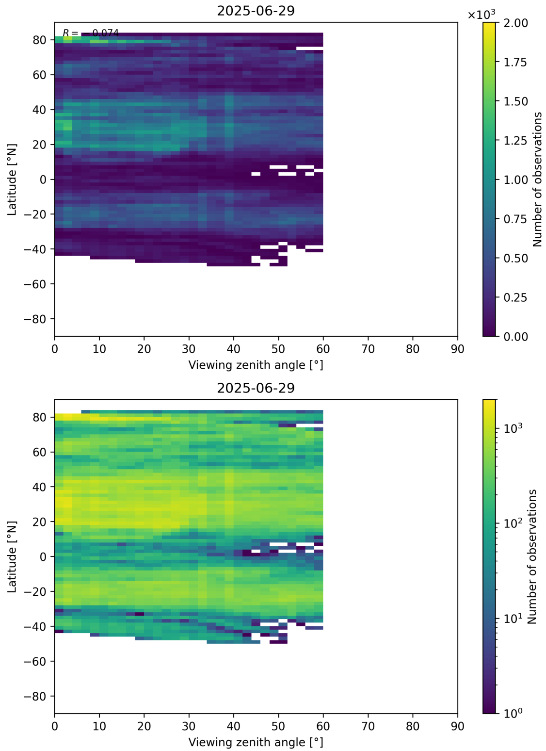
Figure 109: Scatter density plot of “Viewing zenith angle” against “Latitude” for 2025-06-28 to 2025-06-30.
