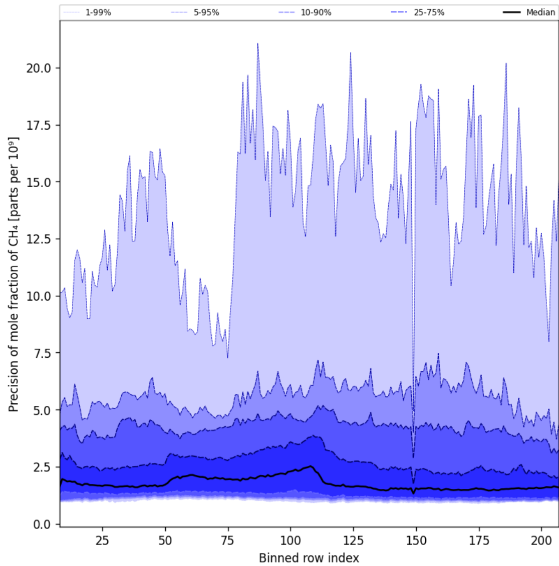
Figure 35: Along track statistics of “Precision of mole fraction of CH 4 ” for 2025-06-28 to 2025-06-30
