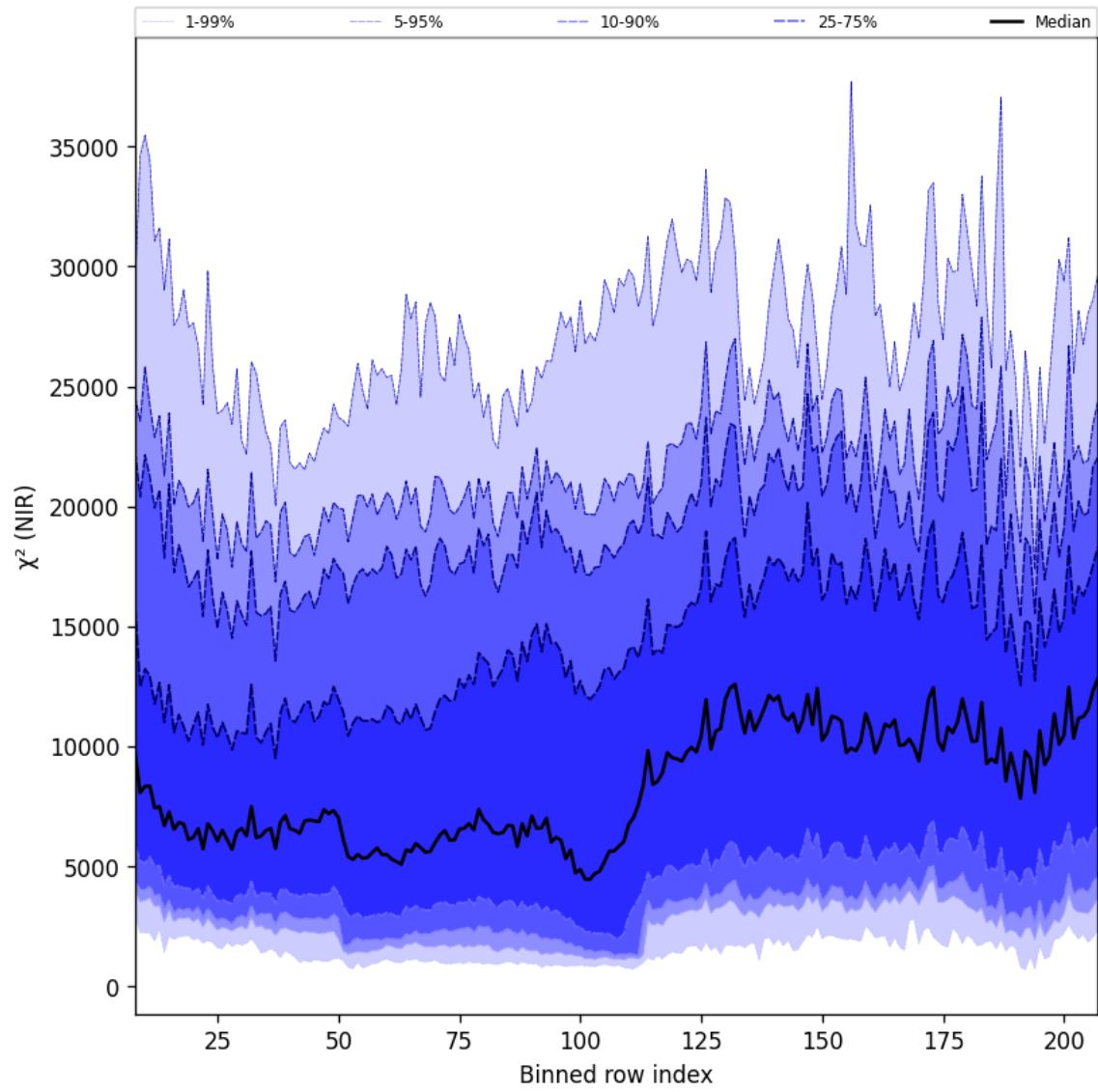
Figure 40: Along track statistics of " \chi^2 (NIR)" for 2025-06-28 to 2025-06-30
