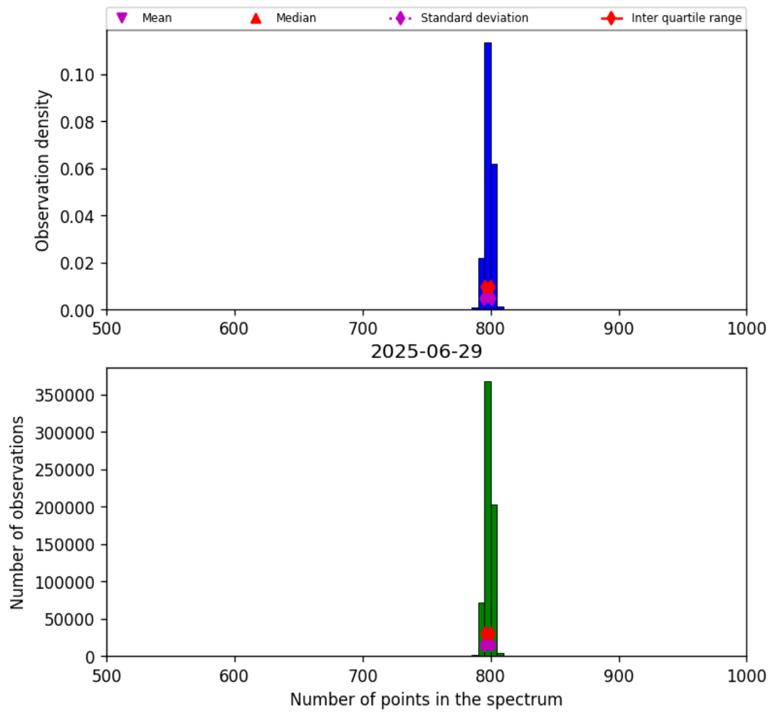
Figure 26: Histogram of “Number of points in the spectrum” for 2025-06-28 to 2025-06-30
