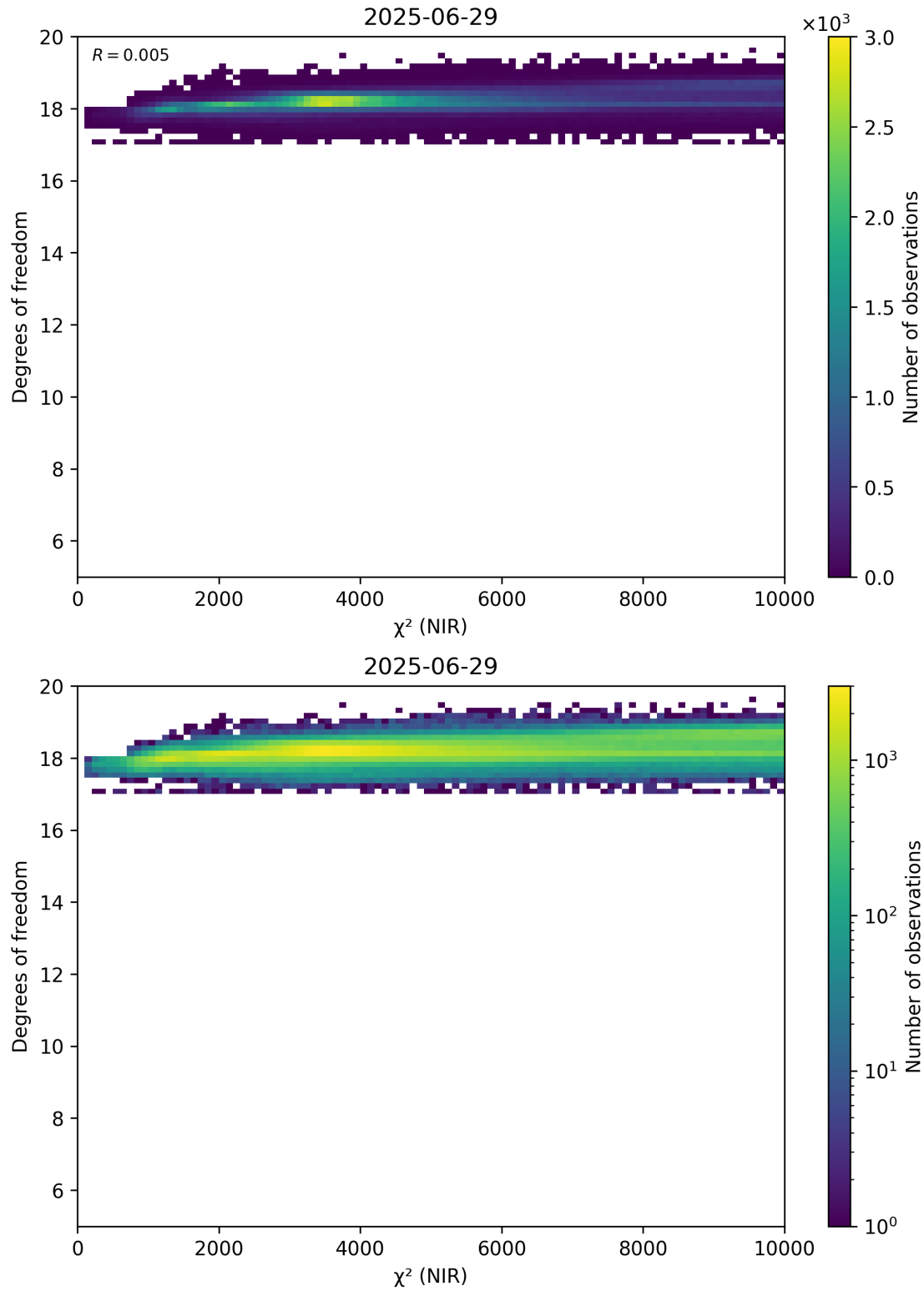
Figure 44: Scatter density plot of “ \chi^2 (NIR)” against “Degrees of freedom” for 2025-06-28 to 2025-06-30.
