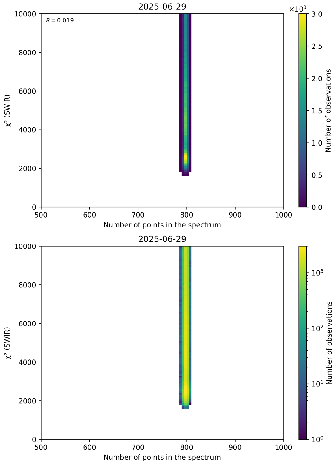
Figure 89: Scatter density plot of “Number of points in the spectrum” against “ \chi^2 (SWIR)” for 2025-06-28 to 2025-06-30.
