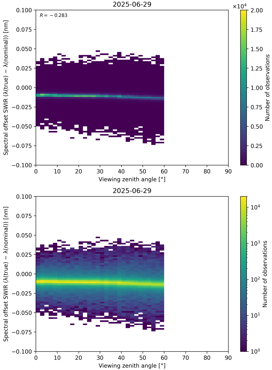
Figure 116: Scatter density plot of “Viewing zenith angle” against “Spectral offset SWIR ( \lambda_{\text{true}} - \lambda_{\text{nominal}} )” for 2025-06-28 to 2025-06-30.
