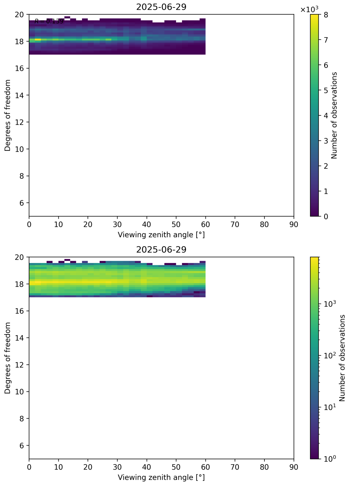
Figure 107: Scatter density plot of “Viewing zenith angle” against “Degrees of freedom” for 2025-06-28 to 2025-06-30.
