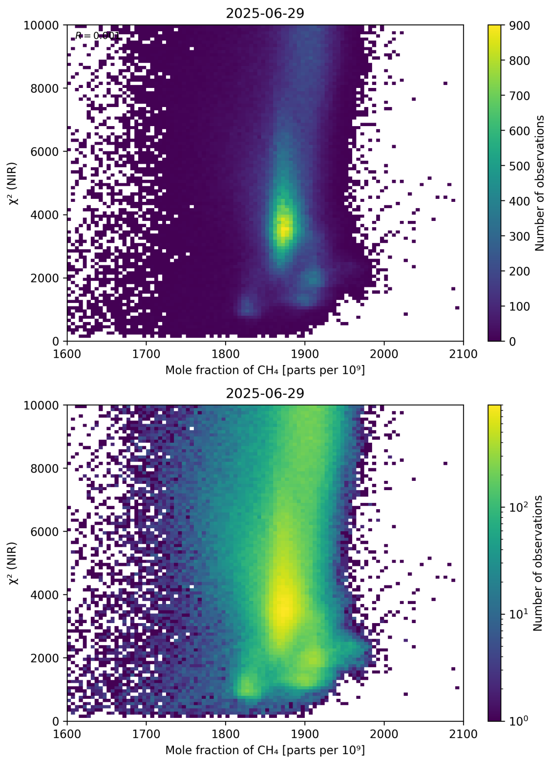
Figure 70: Scatter density plot of “Mole fraction of \text{CH}_4 ” against “ \chi^2 (NIR)” for 2025-06-28 to 2025-06-30.
