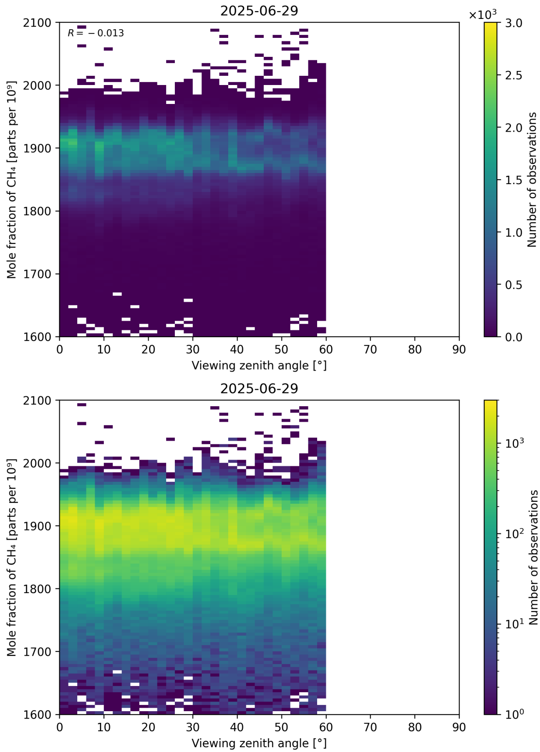
Figure 110: Scatter density plot of “Viewing zenith angle” against “Mole fraction of CH 4 ” for 2025-06-28 to 2025-06-30.
