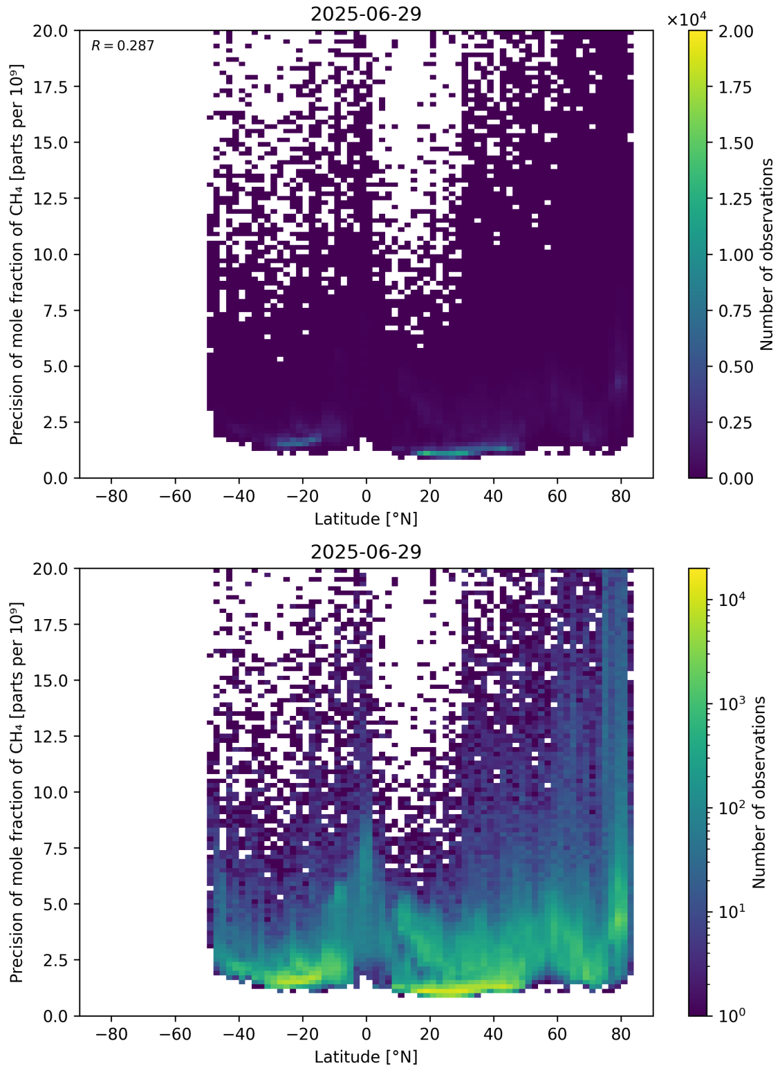
Figure 59: Scatter density plot of “Latitude” against “Precision of mole fraction of \text{CH}_4 ” for 2025-06-28 to 2025-06-30.
