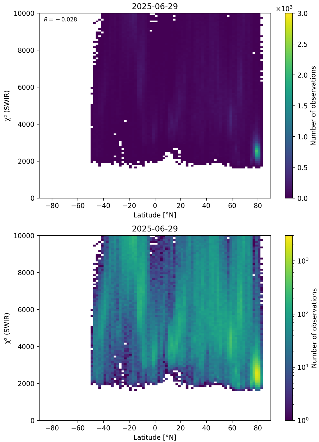
Figure 54: Scatter density plot of “Latitude” against “ \chi^2 (SWIR)” for 2025-06-28 to 2025-06-30.
