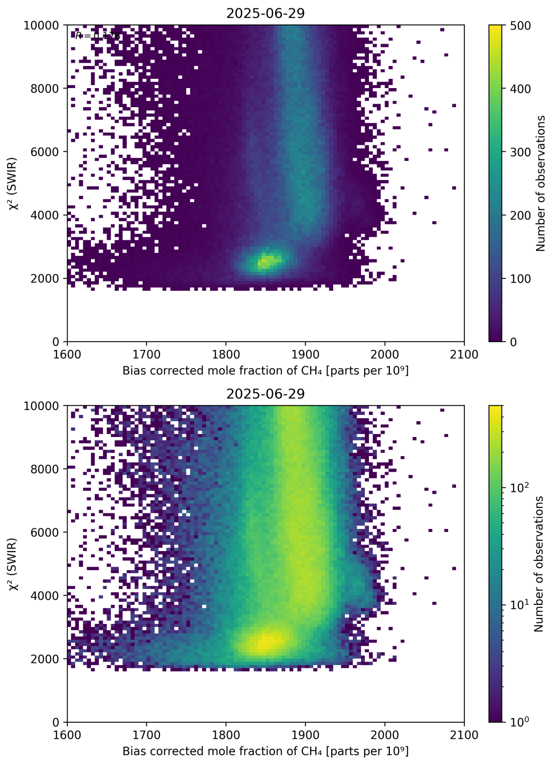
Figure 64: Scatter density plot of “Bias corrected mole fraction of CH 4 ” against “ \chi^2 (SWIR)” for 2025-06-28 to 2025-06-30.
