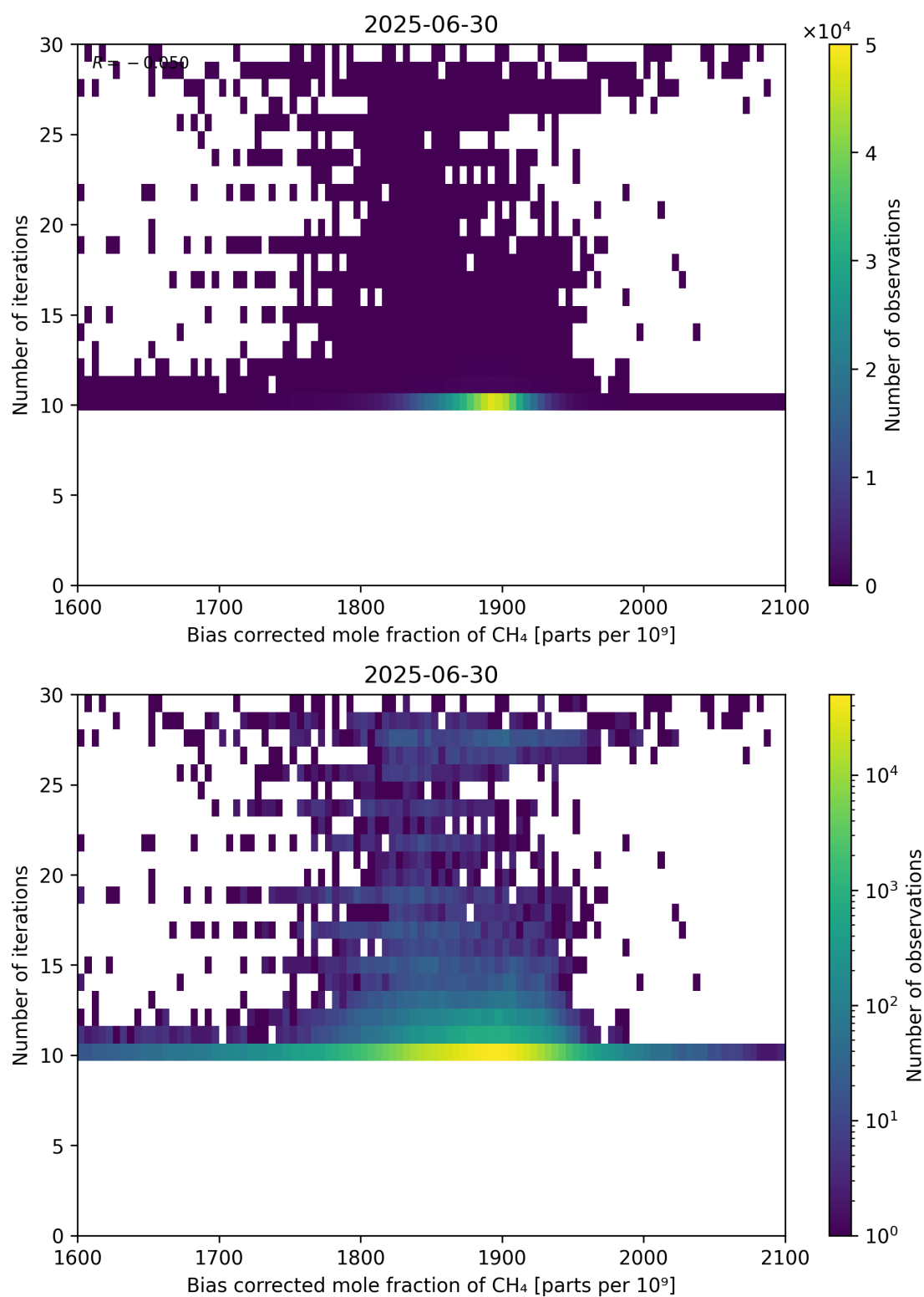
Figure 67: Scatter density plot of “Bias corrected mole fraction of CH 4 ” against “Number of iterations” for 2025-06-29 to 2025-07-01.
