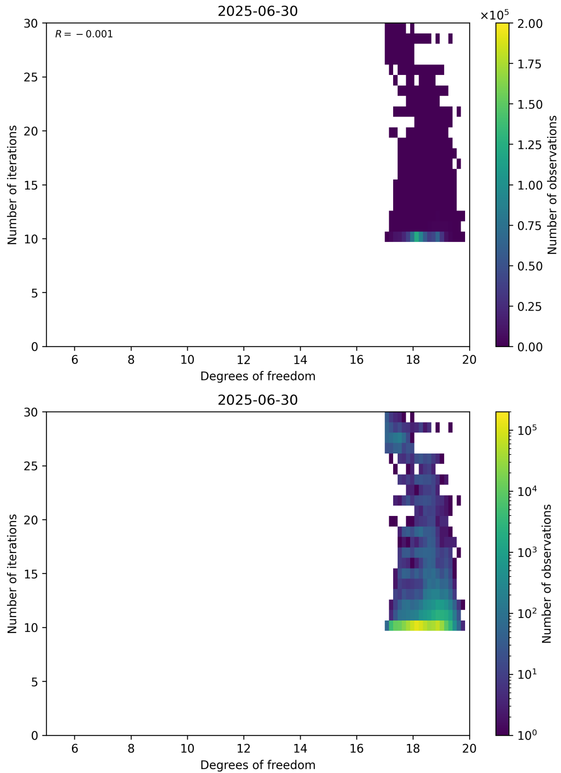
Figure 52: Scatter density plot of “Degrees of freedom” against “Number of iterations” for 2025-06-29 to 2025-07-01.
