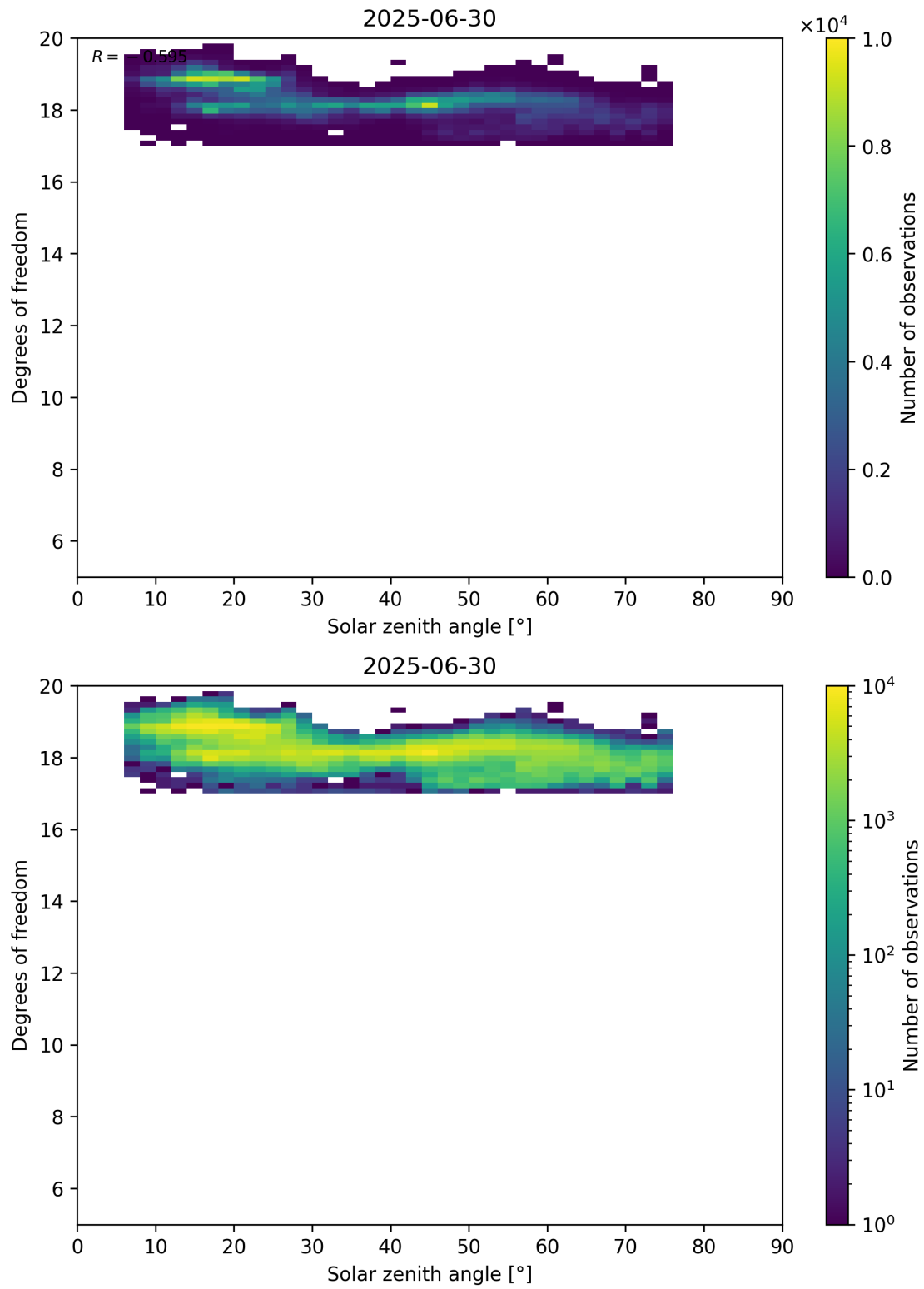
Figure 96: Scatter density plot of “Solar zenith angle” against “Degrees of freedom” for 2025-06-29 to 2025-07-01.
