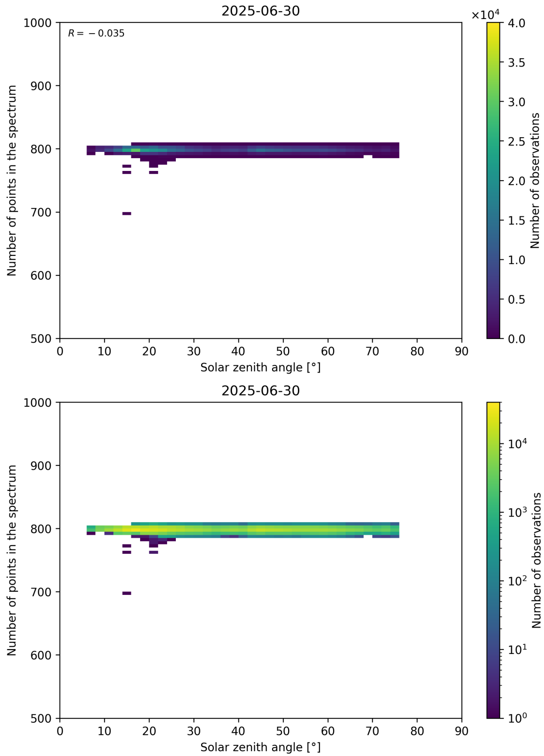
Figure 103: Scatter density plot of “Solar zenith angle” against “Number of points in the spectrum” for 2025-06-29 to 2025-07-01.
