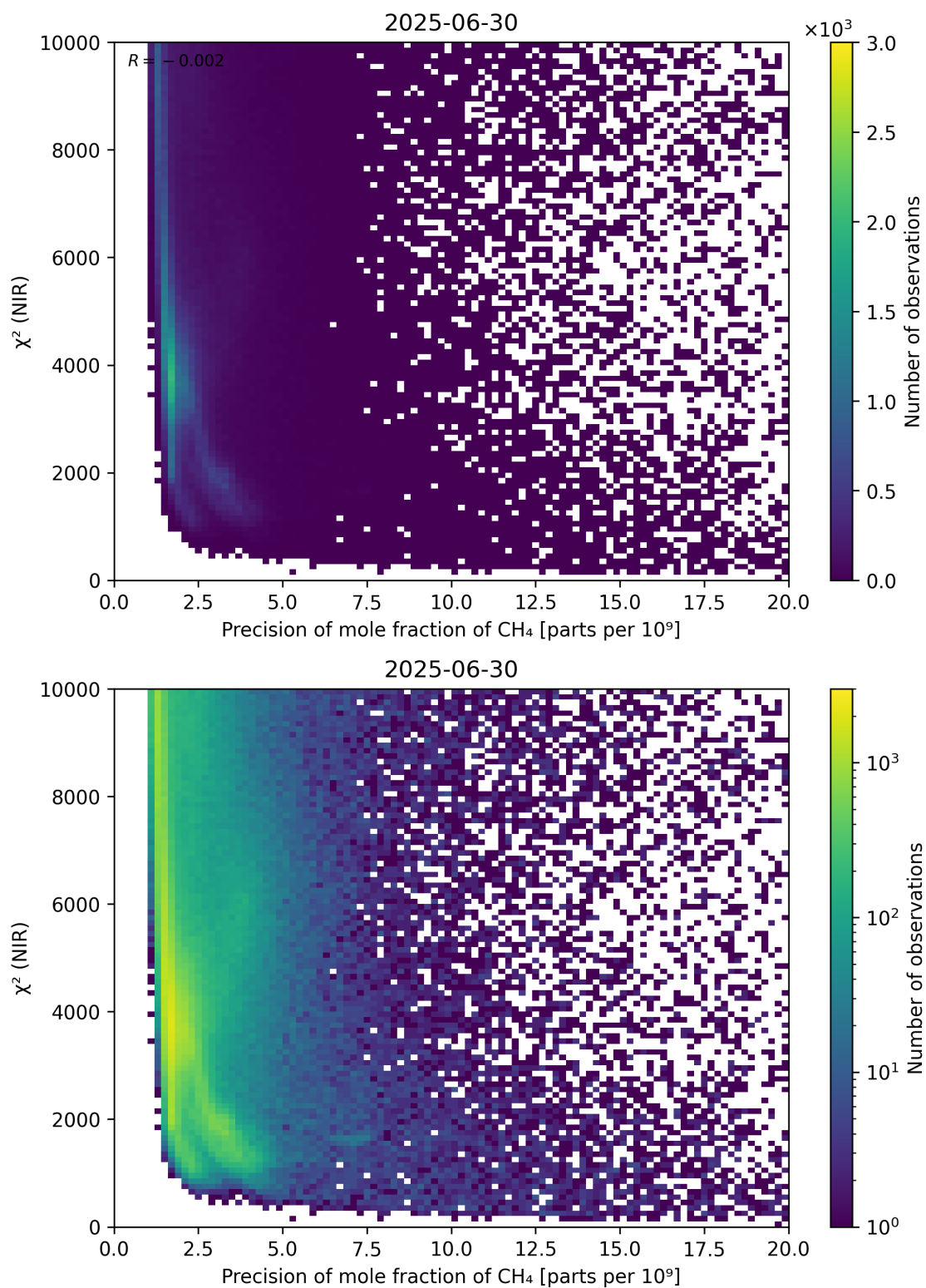
Figure 78: Scatter density plot of “Precision of mole fraction of CH 4 ” against “ \chi^2 (NIR)” for 2025-06-29 to 2025-07-01.
