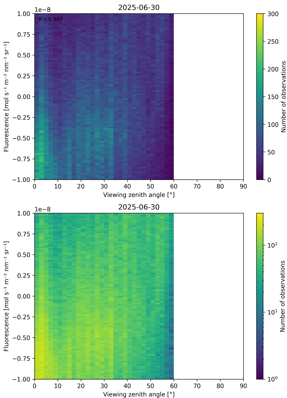
Figure 108: Scatter density plot of “Viewing zenith angle” against “Fluorescence” for 2025-06-29 to 2025-07-01.
