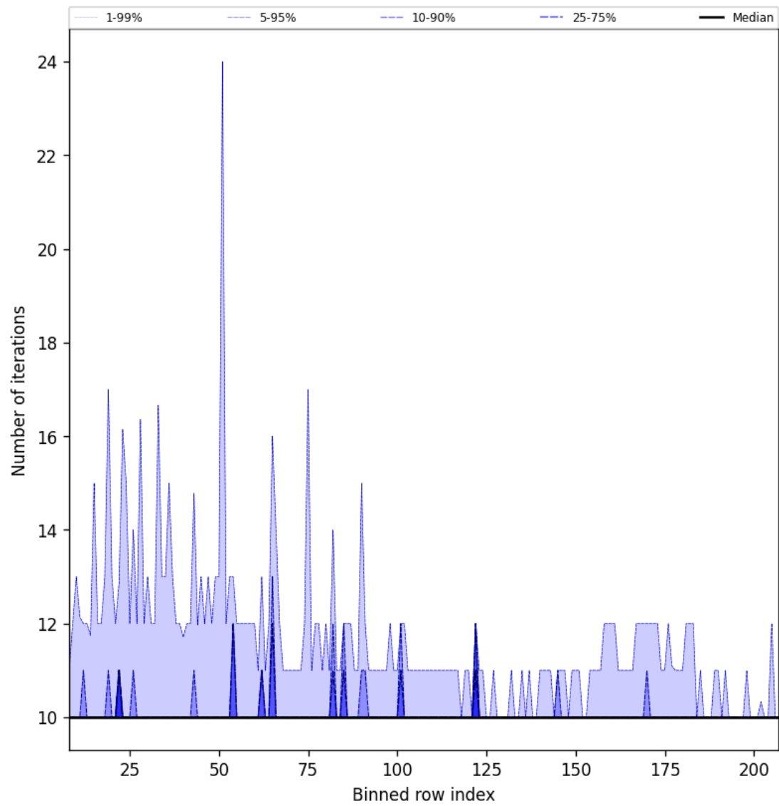
Figure 42: Along track statistics of “Number of iterations” for 2025-06-29 to 2025-07-01
