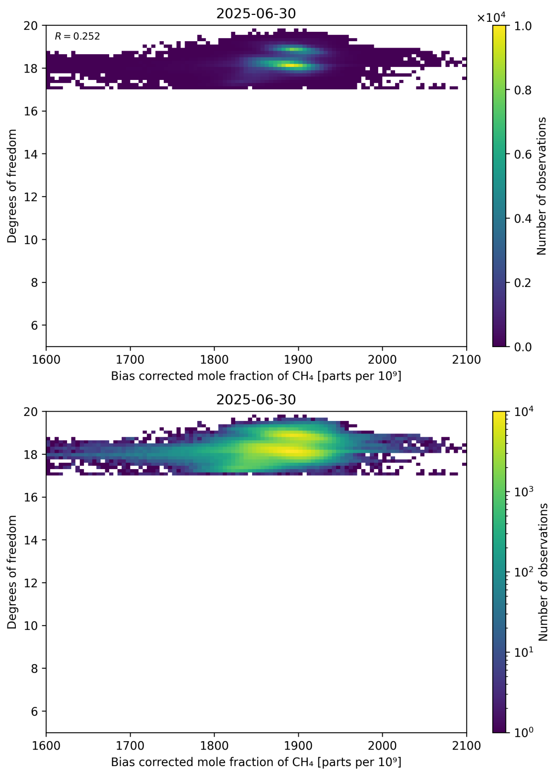
Figure 65: Scatter density plot of “Bias corrected mole fraction of CH 4 ” against “Degrees of freedom” for 2025-06-29 to 2025-07-01.
