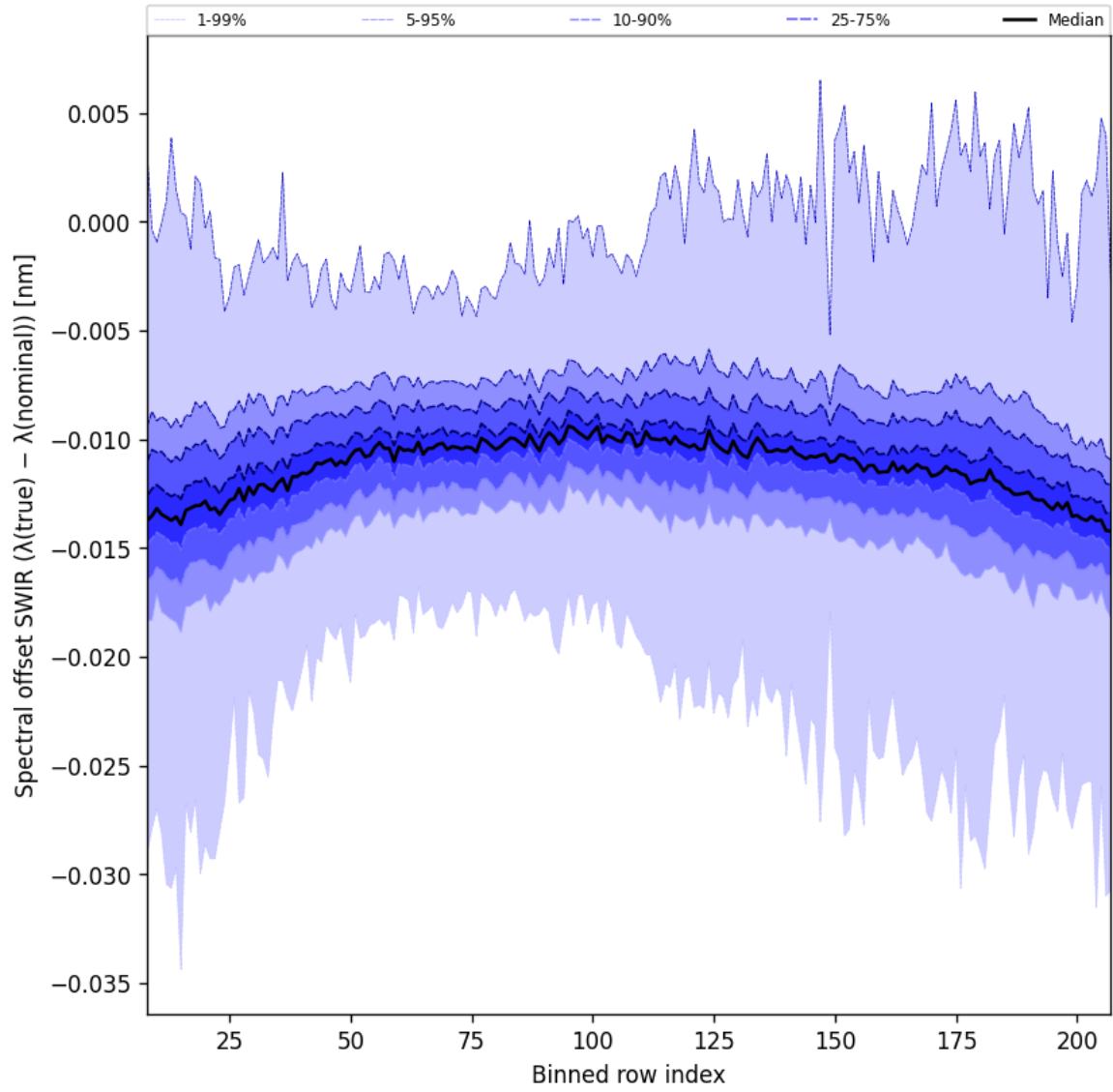
Figure 38: Along track statistics of “Spectral offset SWIR ( \lambda_{\text{true}} - \lambda_{\text{nominal}} )” for 2025-06-29 to 2025-07-01
