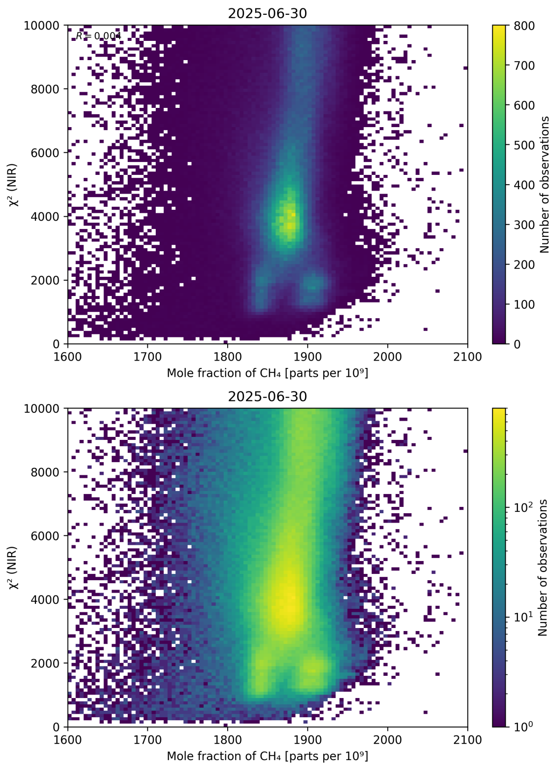
Figure 70: Scatter density plot of “Mole fraction of \text{CH}_4 ” against “ \chi^2 (NIR)” for 2025-06-29 to 2025-07-01.
