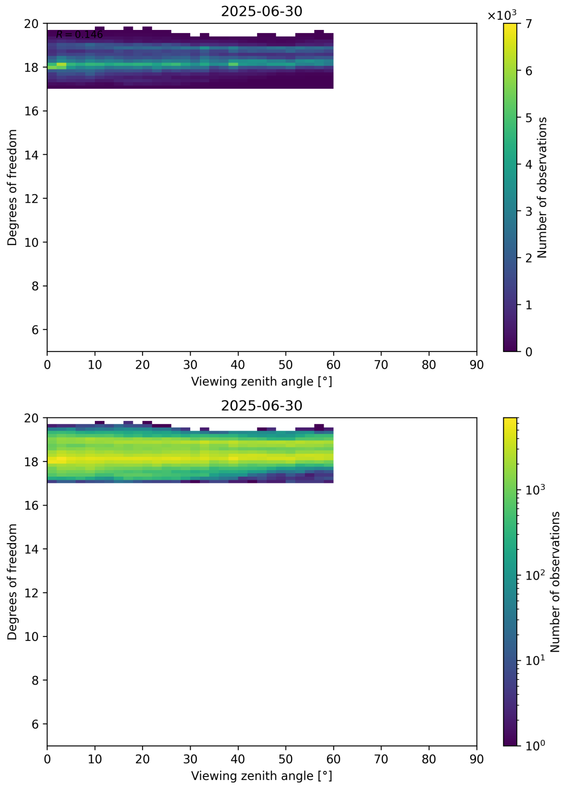
Figure 107: Scatter density plot of “Viewing zenith angle” against “Degrees of freedom” for 2025-06-29 to 2025-07-01.
