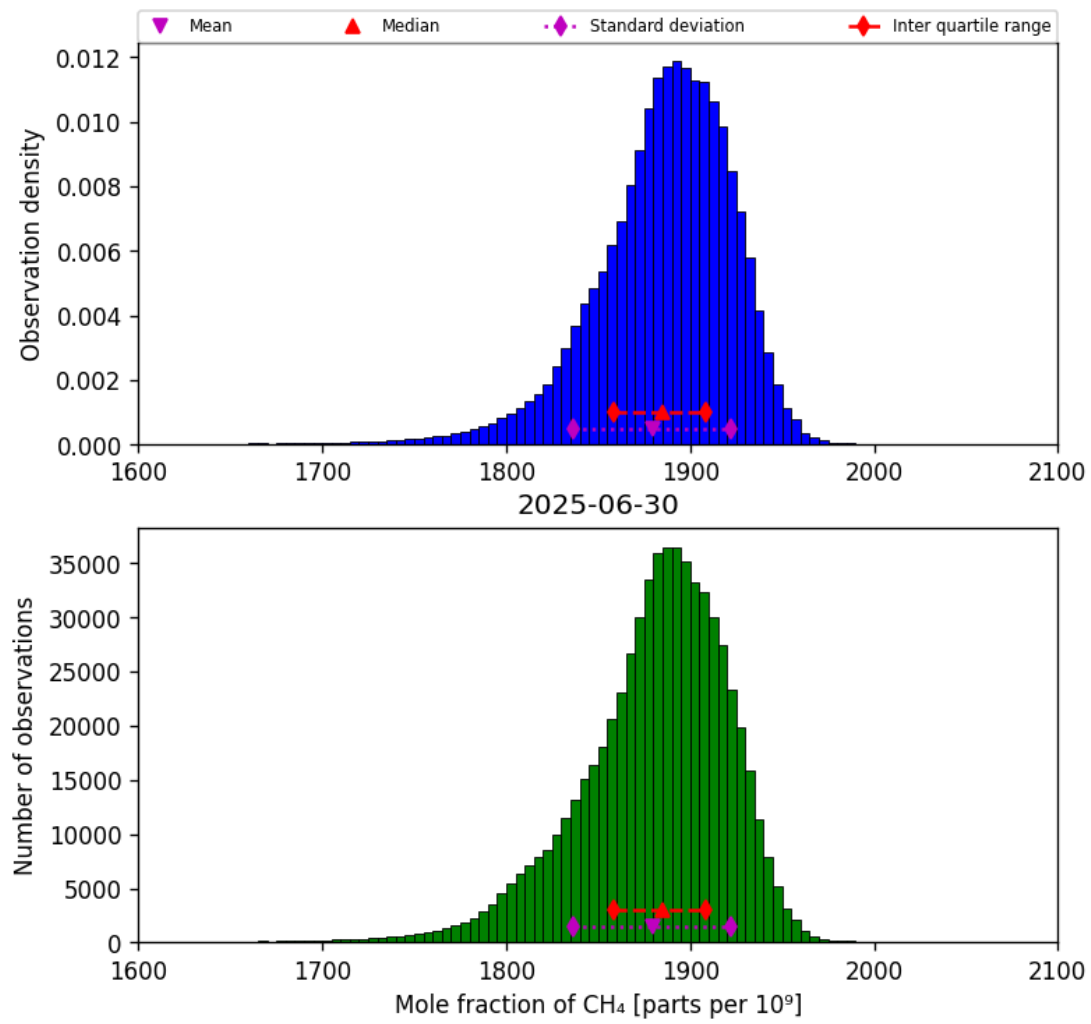
Figure 23: Histogram of “Mole fraction of CH 4 ” for 2025-06-29 to 2025-07-01
