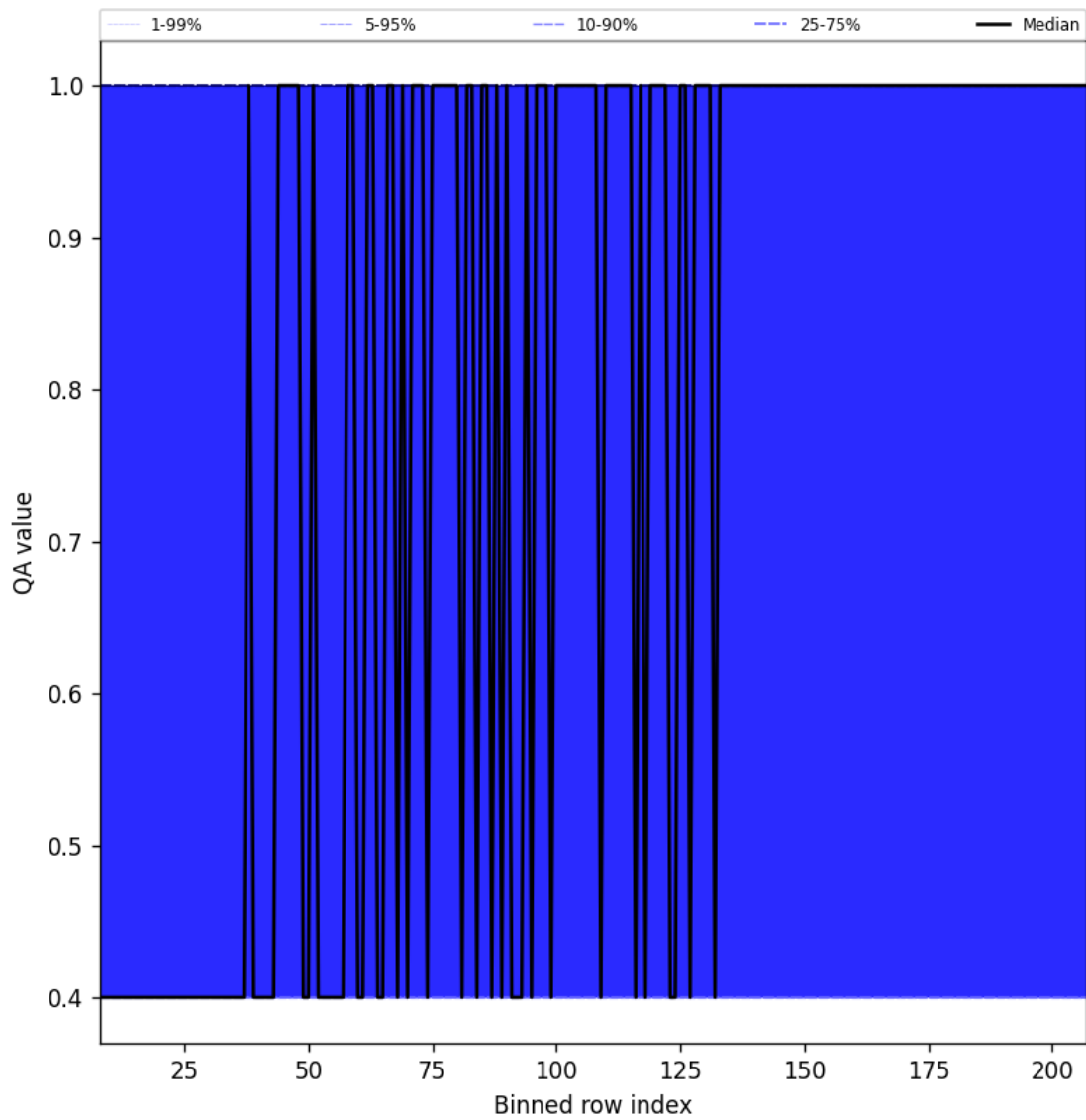
Figure 33: Along track statistics of “QA value” for 2025-06-29 to 2025-07-01
