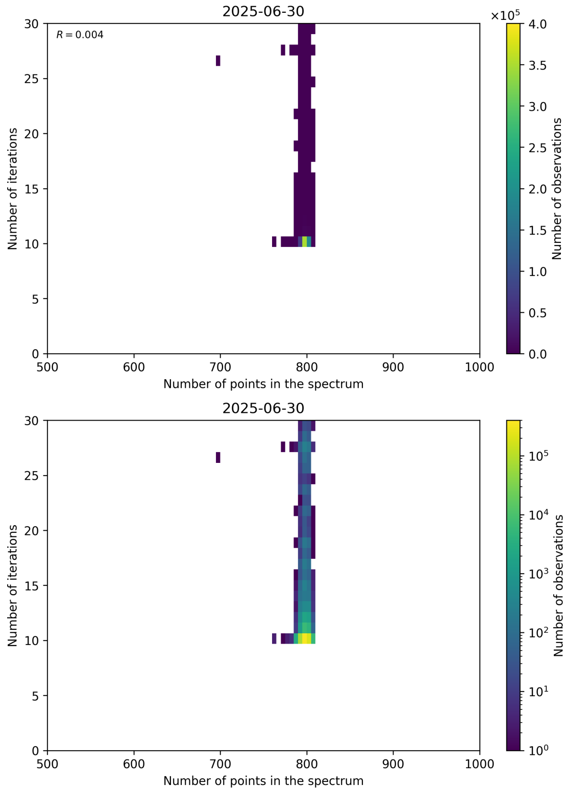
Figure 92: Scatter density plot of “Number of points in the spectrum” against “Number of iterations” for 2025-06-29 to 2025-07-01.
