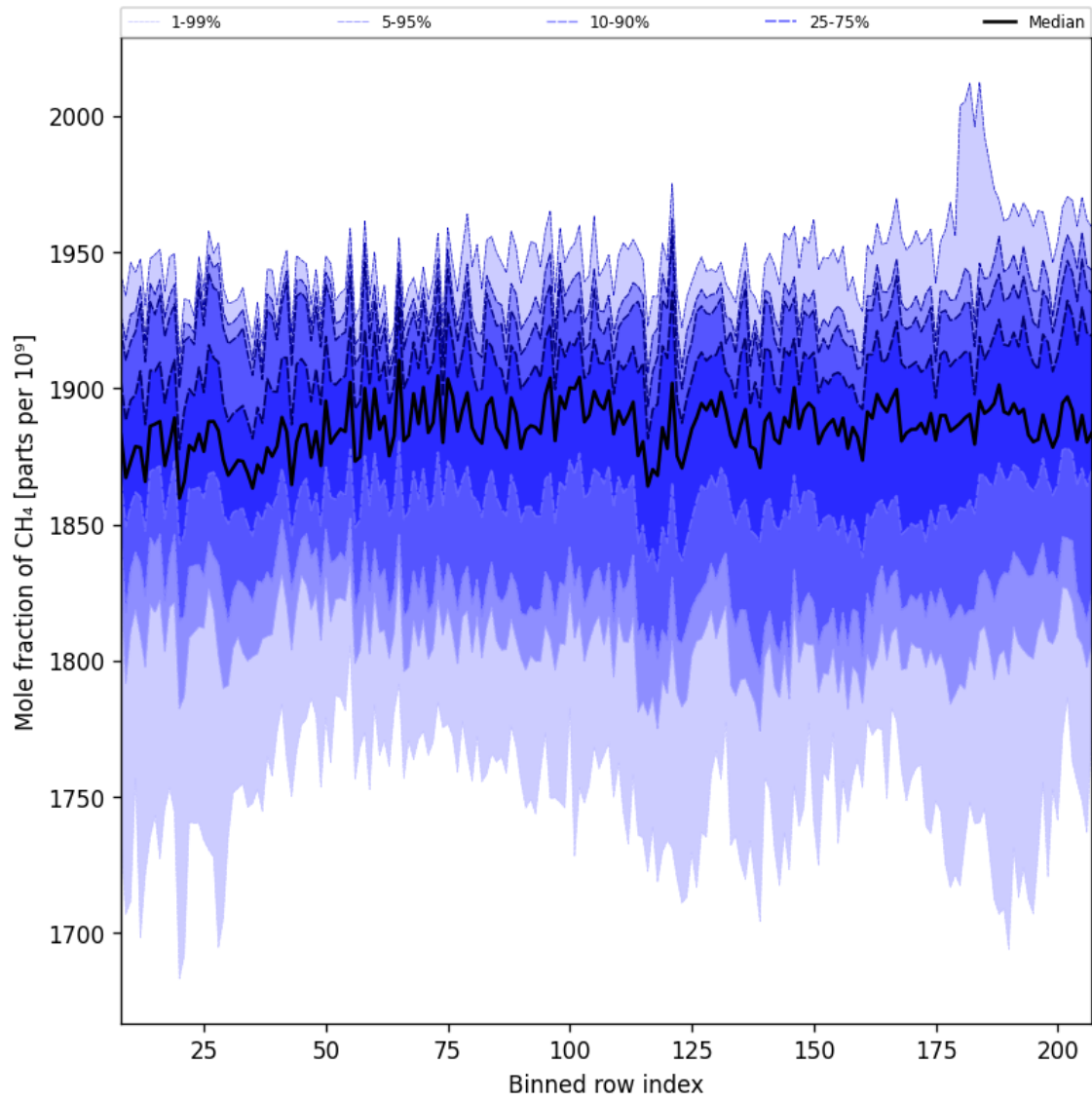
Figure 34: Along track statistics of “Mole fraction of CH 4 ” for 2025-06-29 to 2025-07-01
