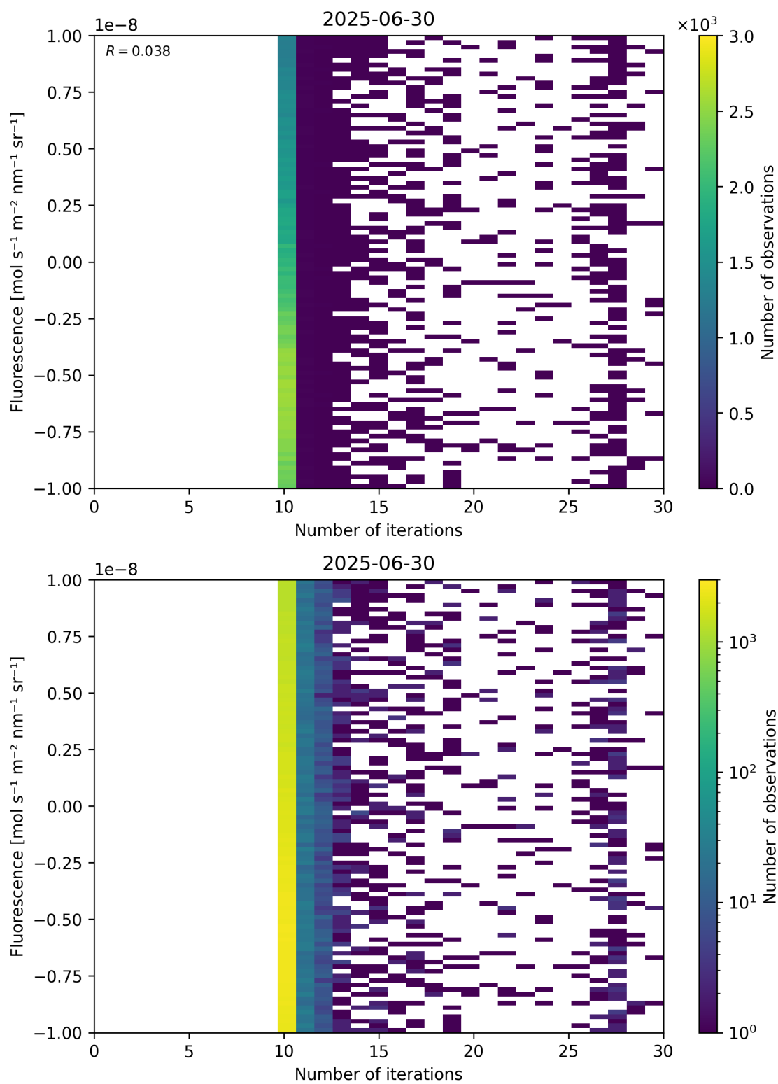
Figure 87: Scatter density plot of “Number of iterations” against “Fluorescence” for 2025-06-29 to 2025-07-01.
