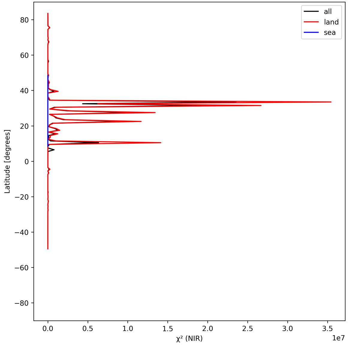
Figure 18: Zonal average of “ \chi^2 (NIR)” for 2025-06-29 to 2025-07-01.
