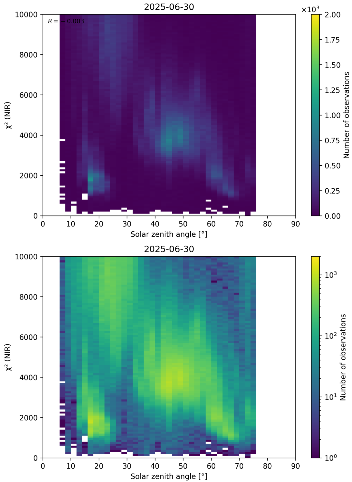
Figure 94: Scatter density plot of “Solar zenith angle” against “ \chi^2 (NIR)” for 2025-06-29 to 2025-07-01.
