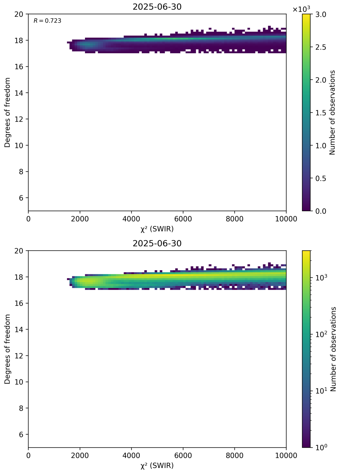
Figure 48: Scatter density plot of “ \chi^2 (SWIR)” against “Degrees of freedom” for 2025-06-29 to 2025-07-01.
