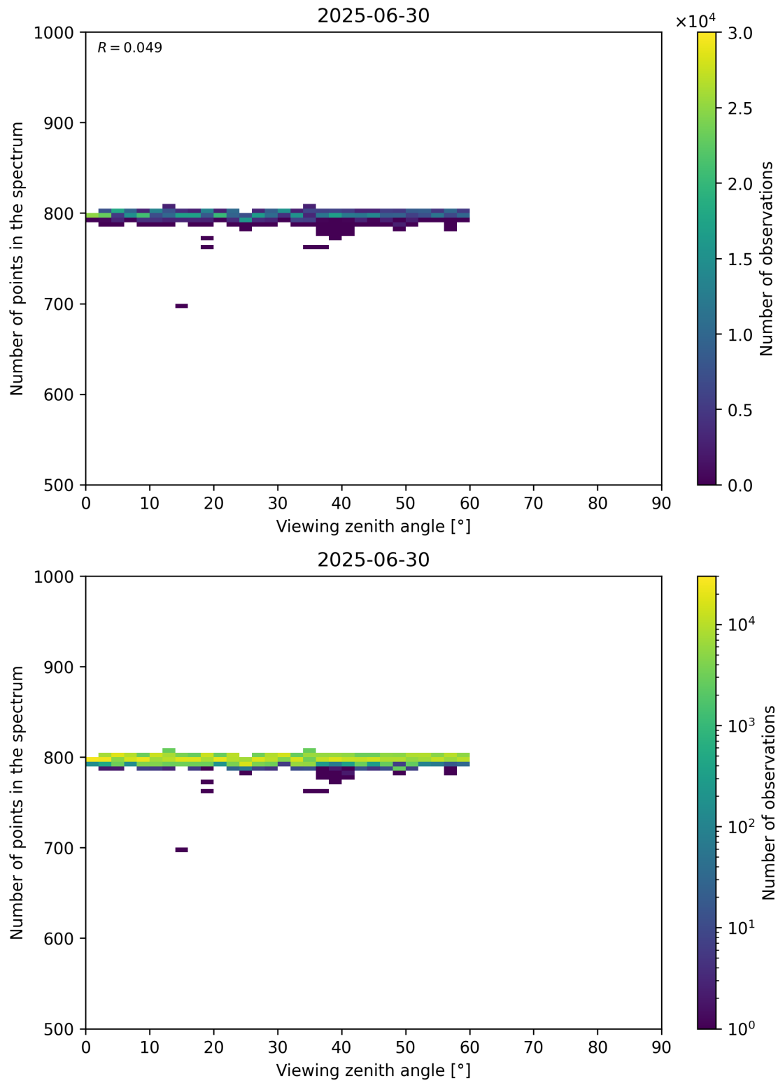
Figure 114: Scatter density plot of “Viewing zenith angle” against “Number of points in the spectrum” for 2025-06-29 to 2025-07-01.
