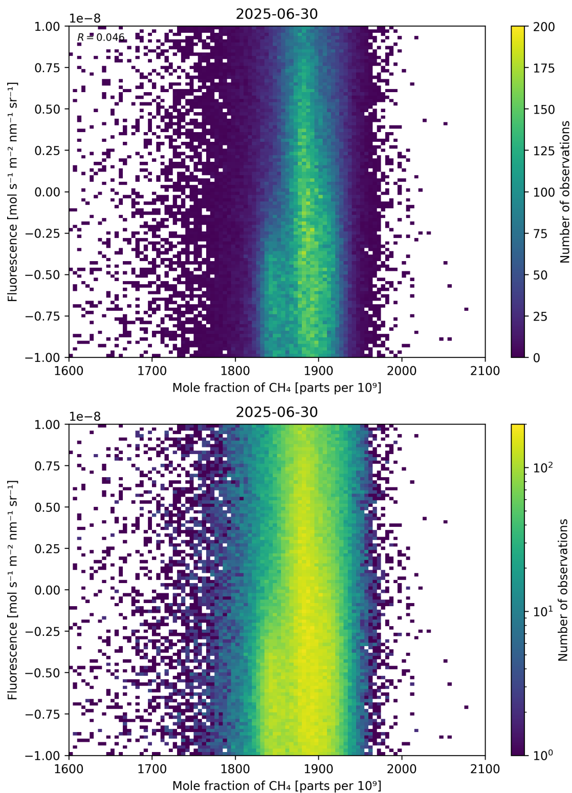
Figure 73: Scatter density plot of “Mole fraction of \text{CH}_4 ” against “Fluorescence” for 2025-06-29 to 2025-07-01.
