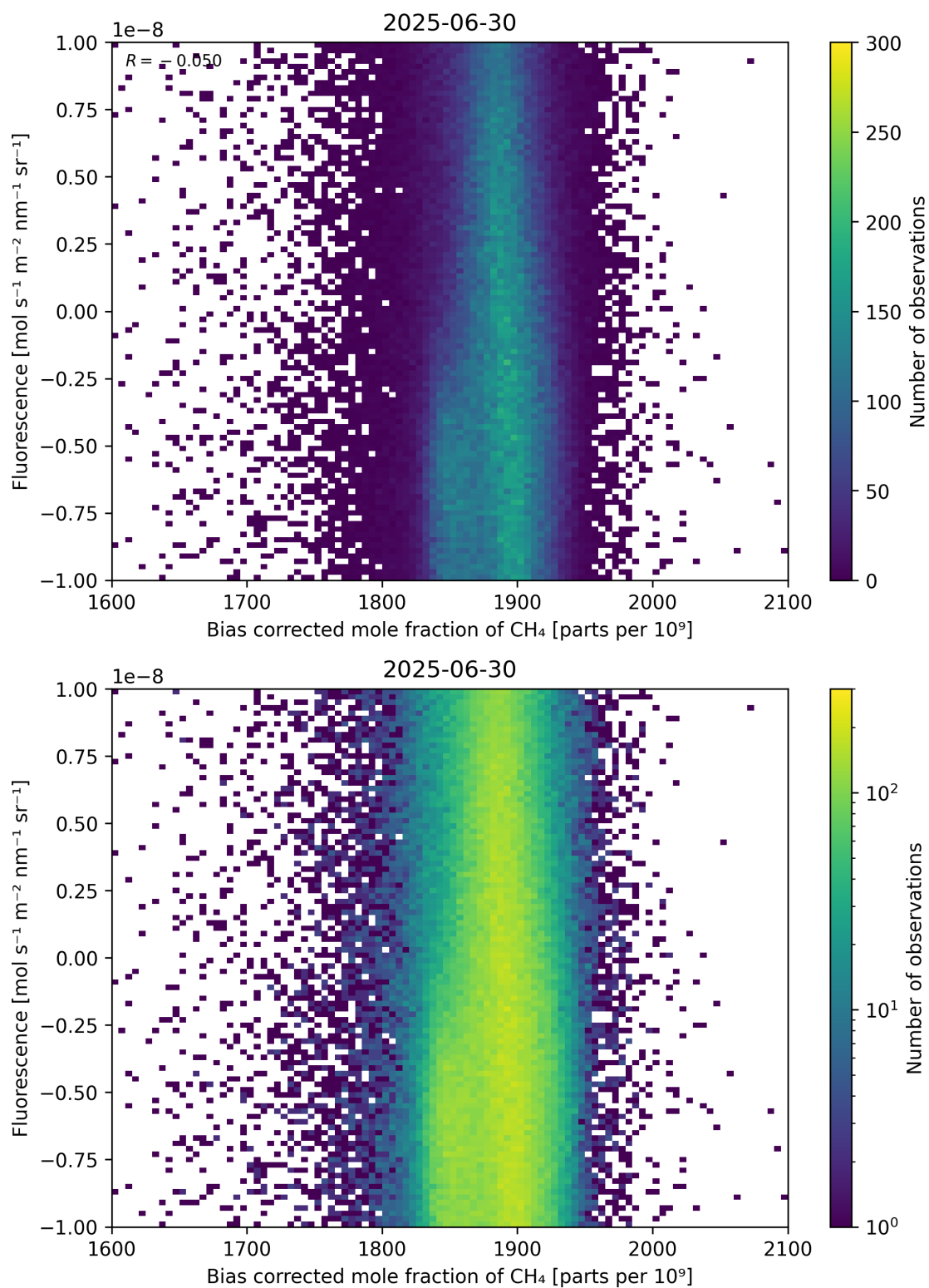
Figure 66: Scatter density plot of “Bias corrected mole fraction of \text{CH}_4 ” against “Fluorescence” for 2025-06-29 to 2025-07-01.
