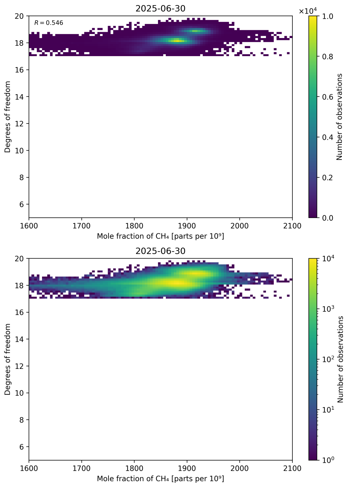
Figure 72: Scatter density plot of “Mole fraction of CH 4 ” against “Degrees of freedom” for 2025-06-29 to 2025-07-01.
