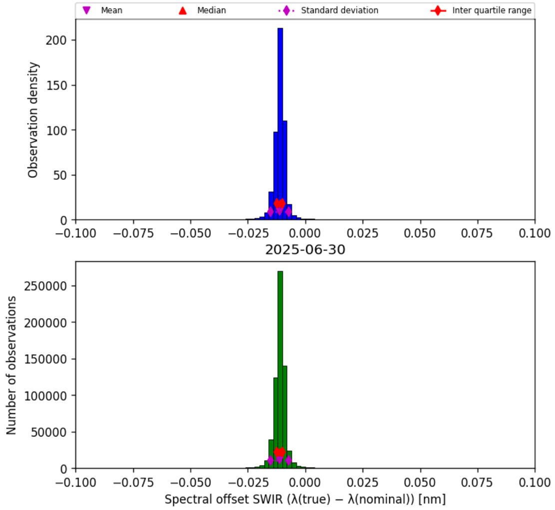
Figure 27: Histogram of “Spectral offset SWIR ( \lambda_{\text{true}} - \lambda_{\text{nominal}} )” for 2025-06-29 to 2025-07-01
