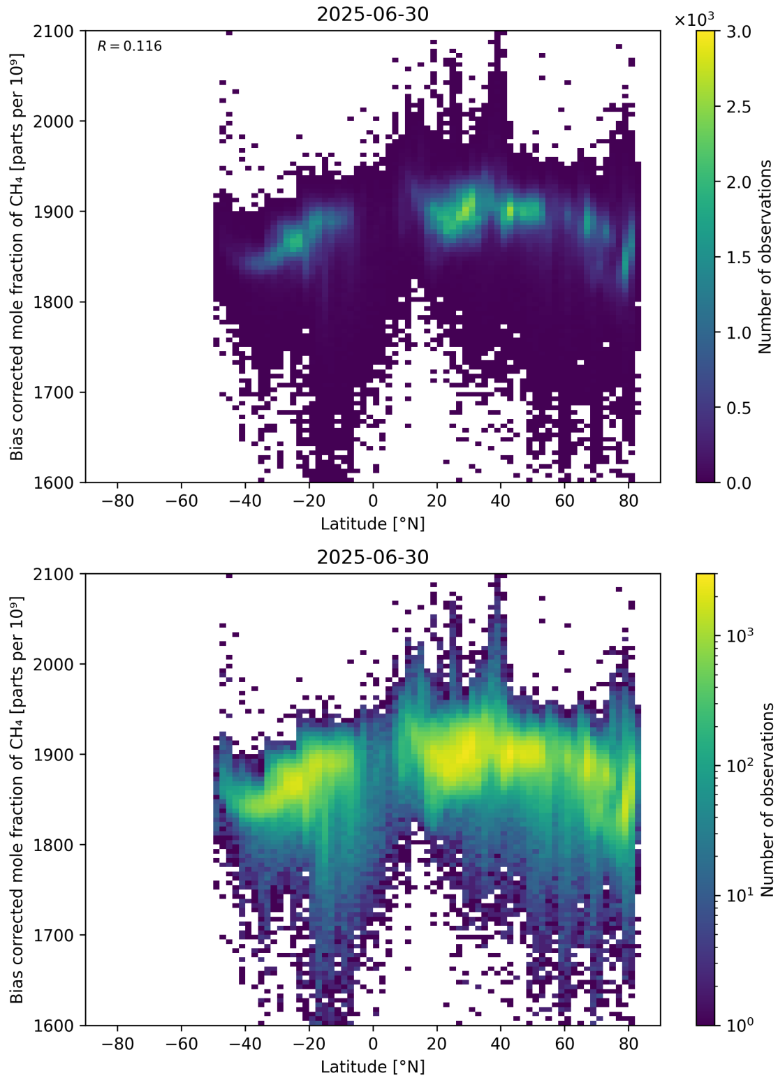
Figure 58: Scatter density plot of “Latitude” against “Bias corrected mole fraction of CH 4 ” for 2025-06-29 to 2025-07-01.
