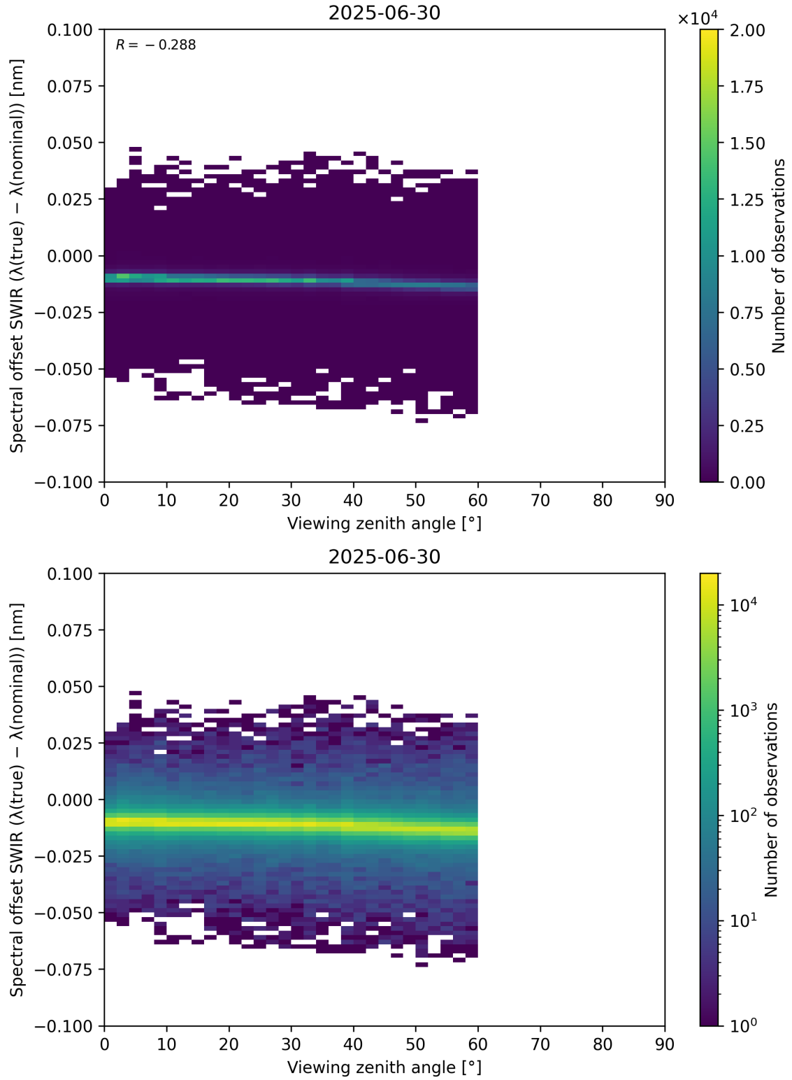
Figure 116: Scatter density plot of “Viewing zenith angle” against “Spectral offset SWIR ( \lambda_{\text{true}} - \lambda_{\text{nominal}} )” for 2025-06-29 to 2025-07-01.
