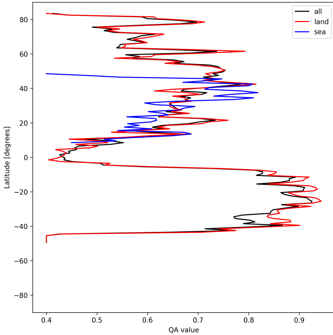
Figure 11: Zonal average of “QA value” for 2025-06-29 to 2025-07-01.
