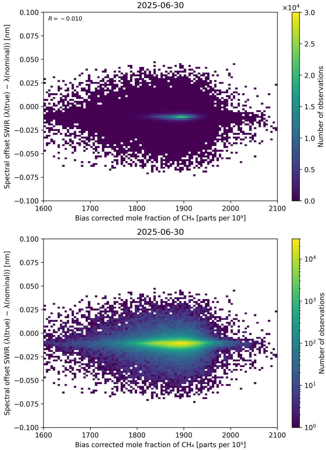
Figure 69: Scatter density plot of “Bias corrected mole fraction of \text{CH}_4 ” against “Spectral offset SWIR ( \lambda_{\text{true}} - \lambda_{\text{nominal}} )” for 2025-06-29 to 2025-07-01.
