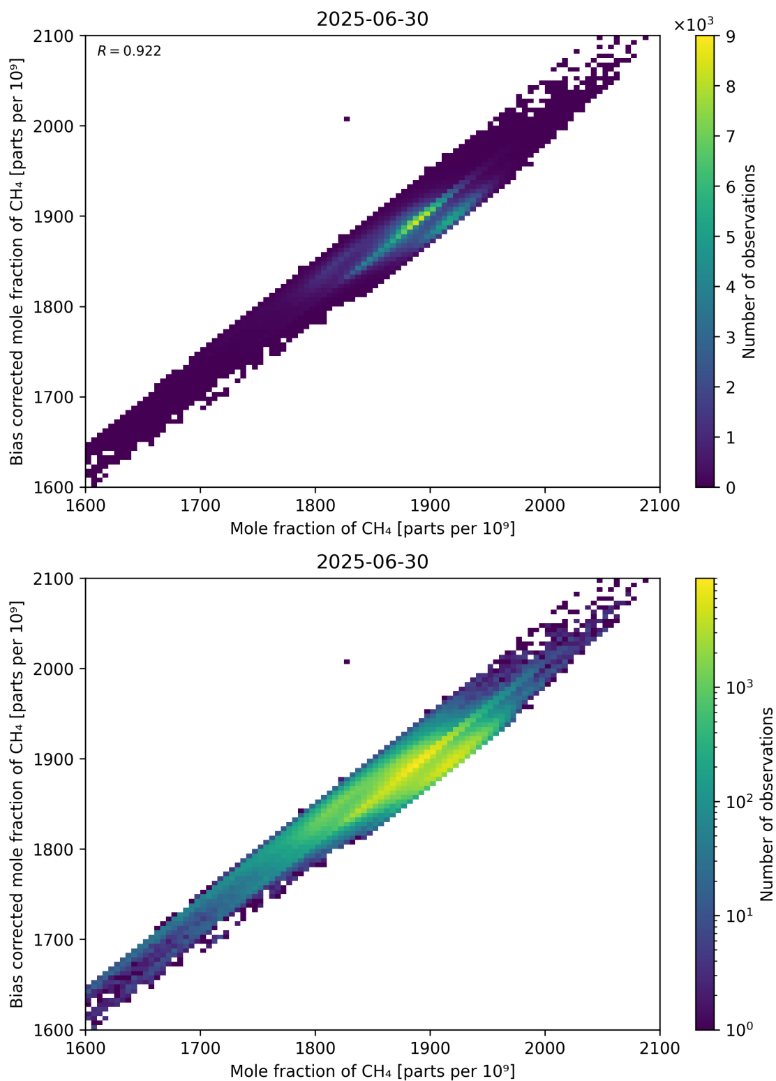
Figure 74: Scatter density plot of “Mole fraction of CH 4 ” against “Bias corrected mole fraction of CH 4 ” for 2025-06-29 to 2025-07-01.
