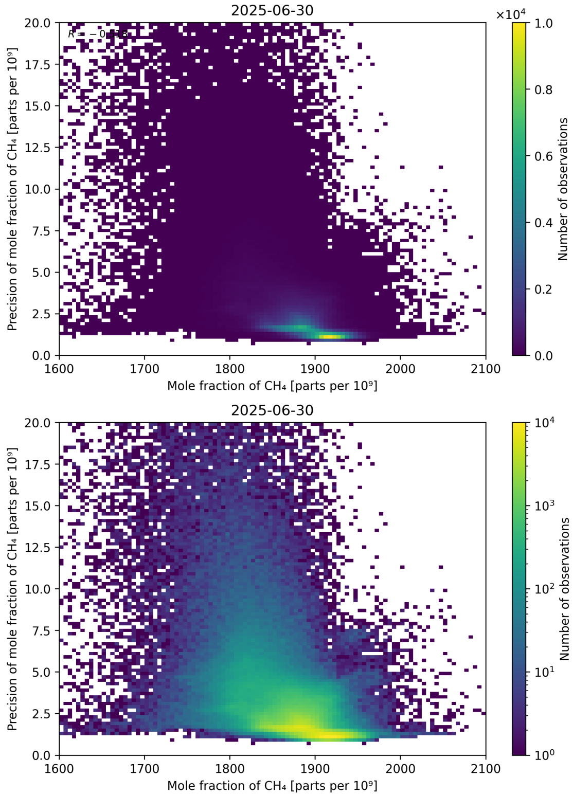
Figure 75: Scatter density plot of “Mole fraction of CH 4 ” against “Precision of mole fraction of CH 4 ” for 2025-06-29 to 2025-07-01.
