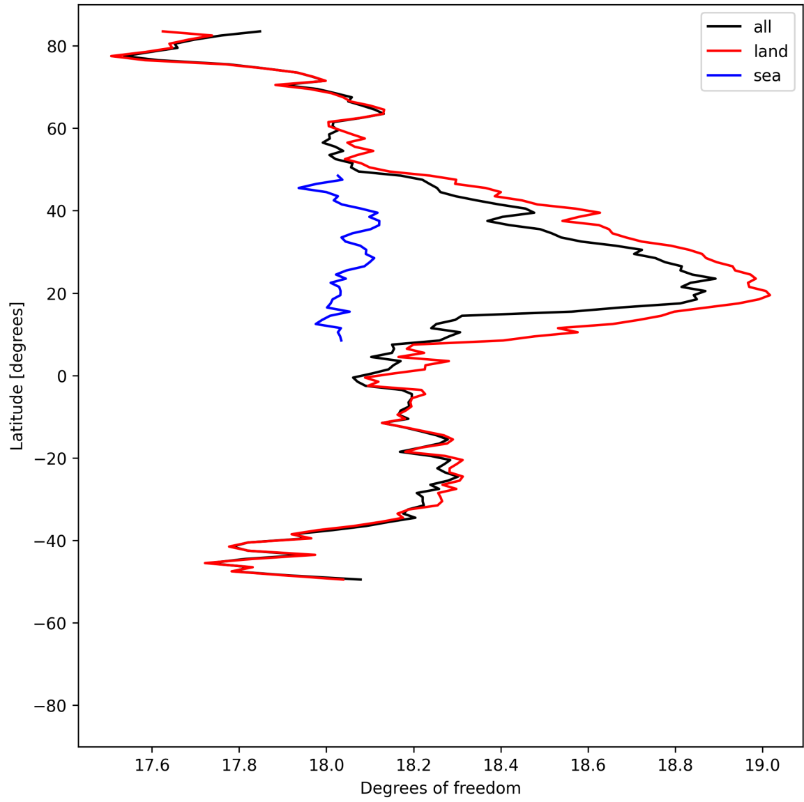
Figure 19: Zonal average of “Degrees of freedom” for 2025-06-29 to 2025-07-01.
