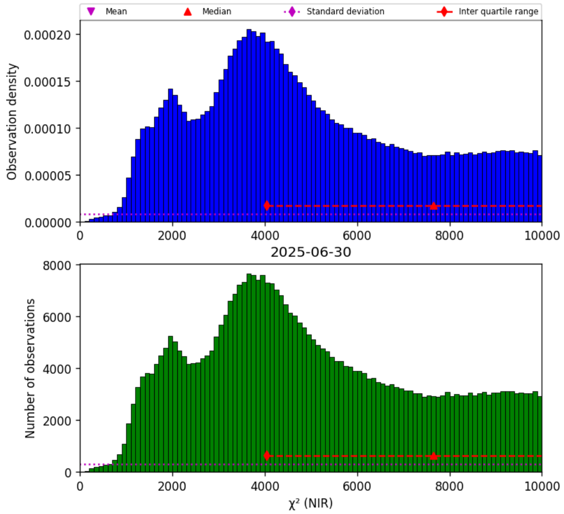
Figure 29: Histogram of “ \chi^2 (NIR)” for 2025-06-29 to 2025-07-01
