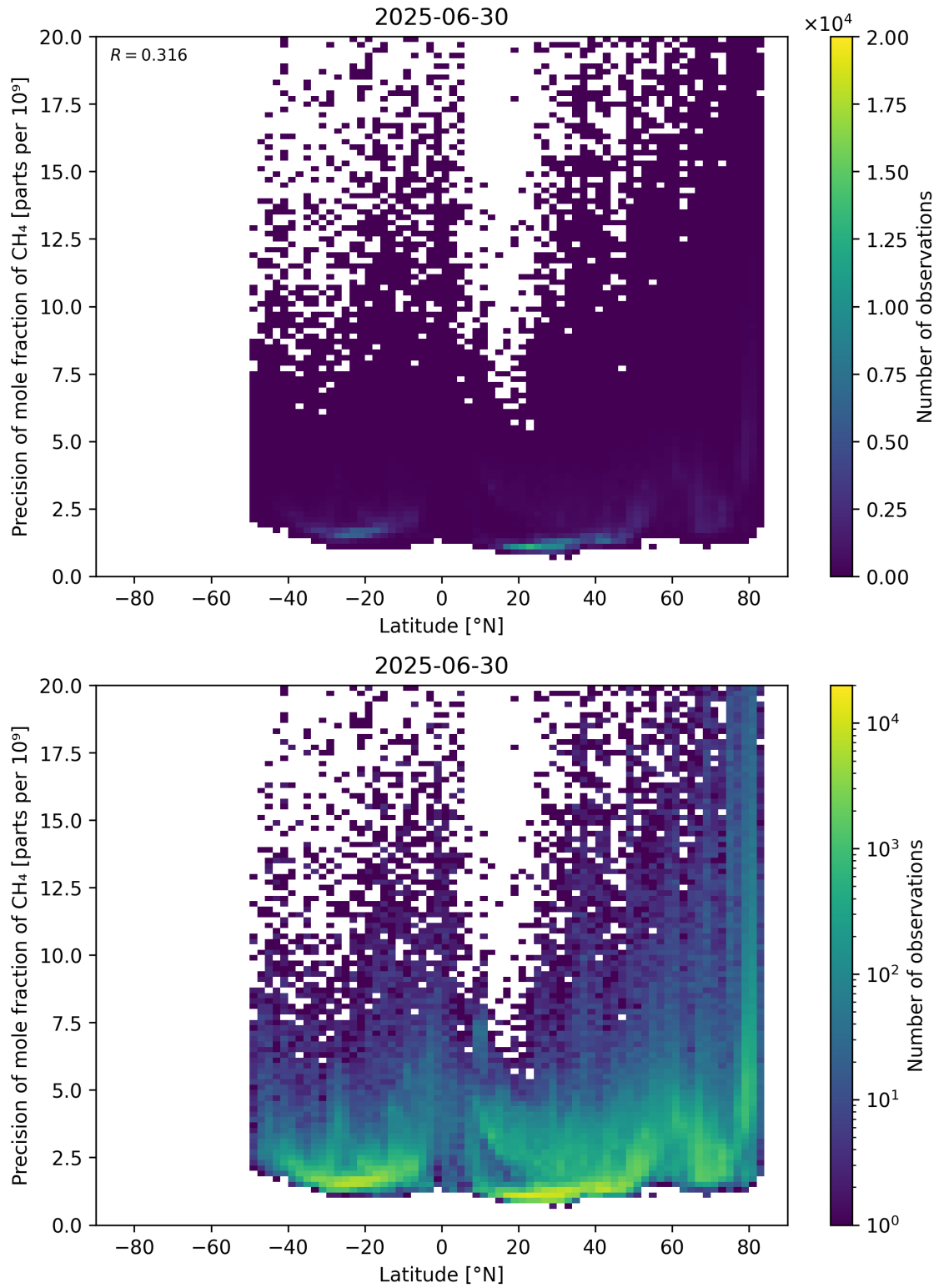
Figure 59: Scatter density plot of “Latitude” against “Precision of mole fraction of \text{CH}_4 ” for 2025-06-29 to 2025-07-01.
