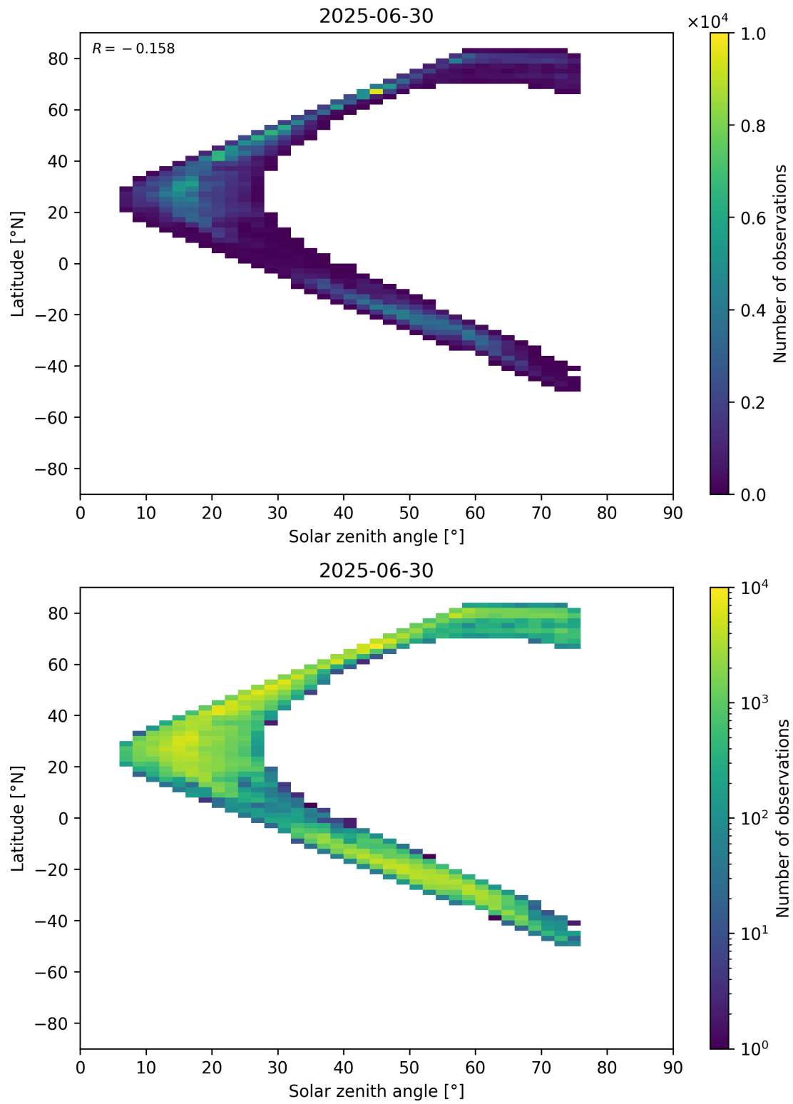
Figure 98: Scatter density plot of “Solar zenith angle” against “Latitude” for 2025-06-29 to 2025-07-01.
