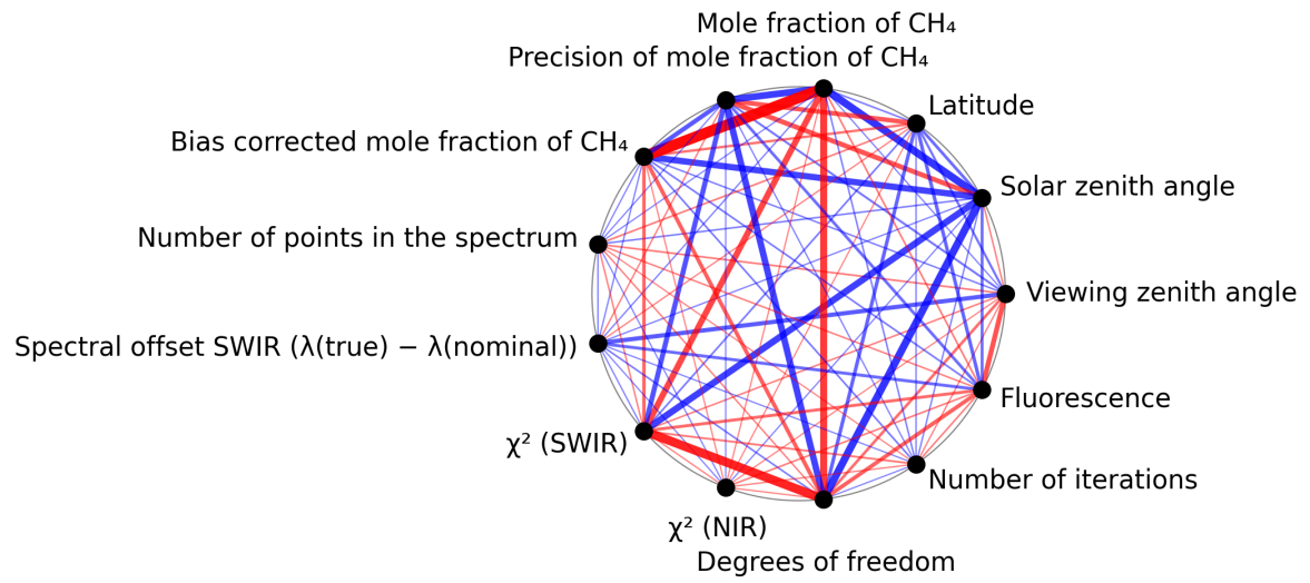
Figure 1: Map of correlation graph for 2025-06-29 to 2025-07-01.
