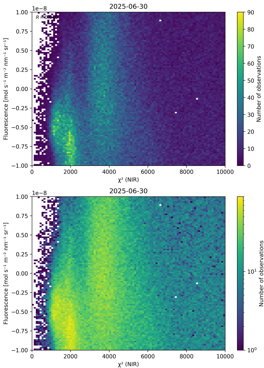
Figure 45: Scatter density plot of “ \chi^2 (NIR)” against “Fluorescence” for 2025-06-29 to 2025-07-01.
