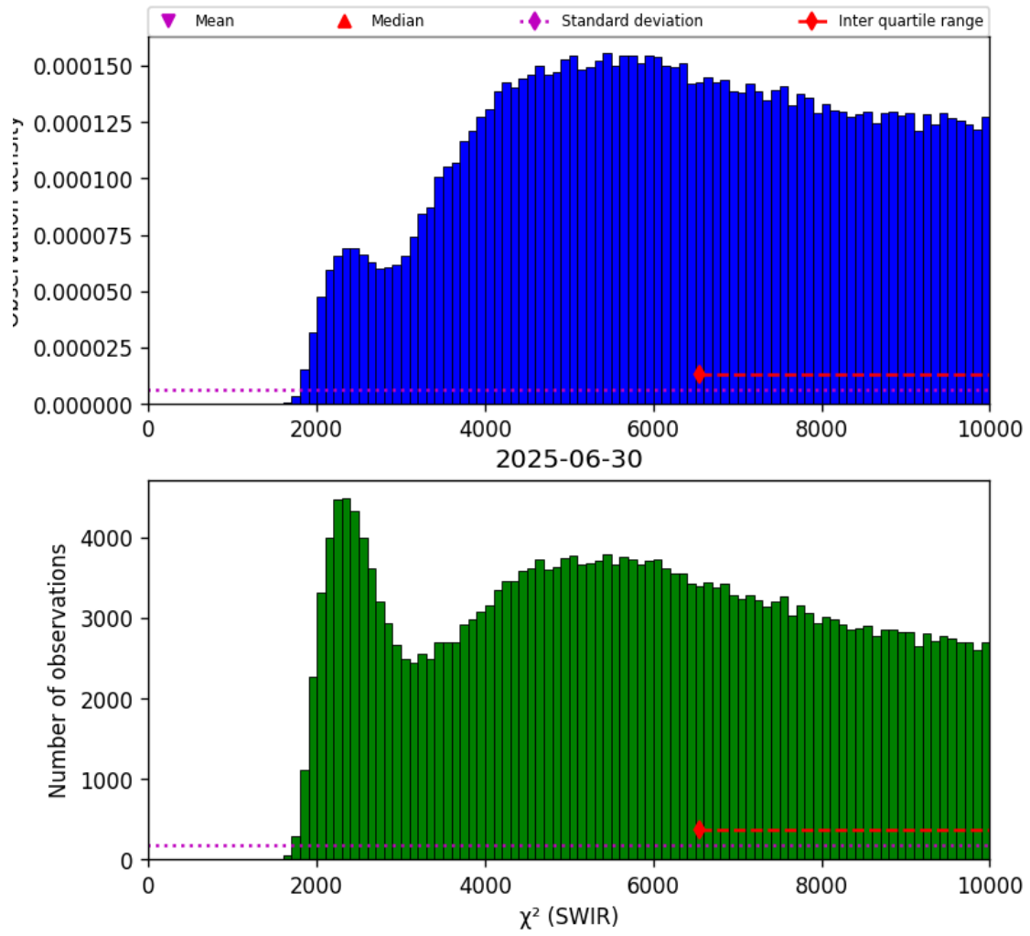
Figure 28: Histogram of “ \chi^2 (SWIR)” for 2025-06-29 to 2025-07-01
