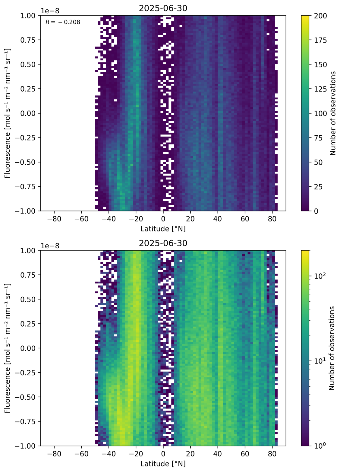
Figure 56: Scatter density plot of “Latitude” against “Fluorescence” for 2025-06-29 to 2025-07-01.
