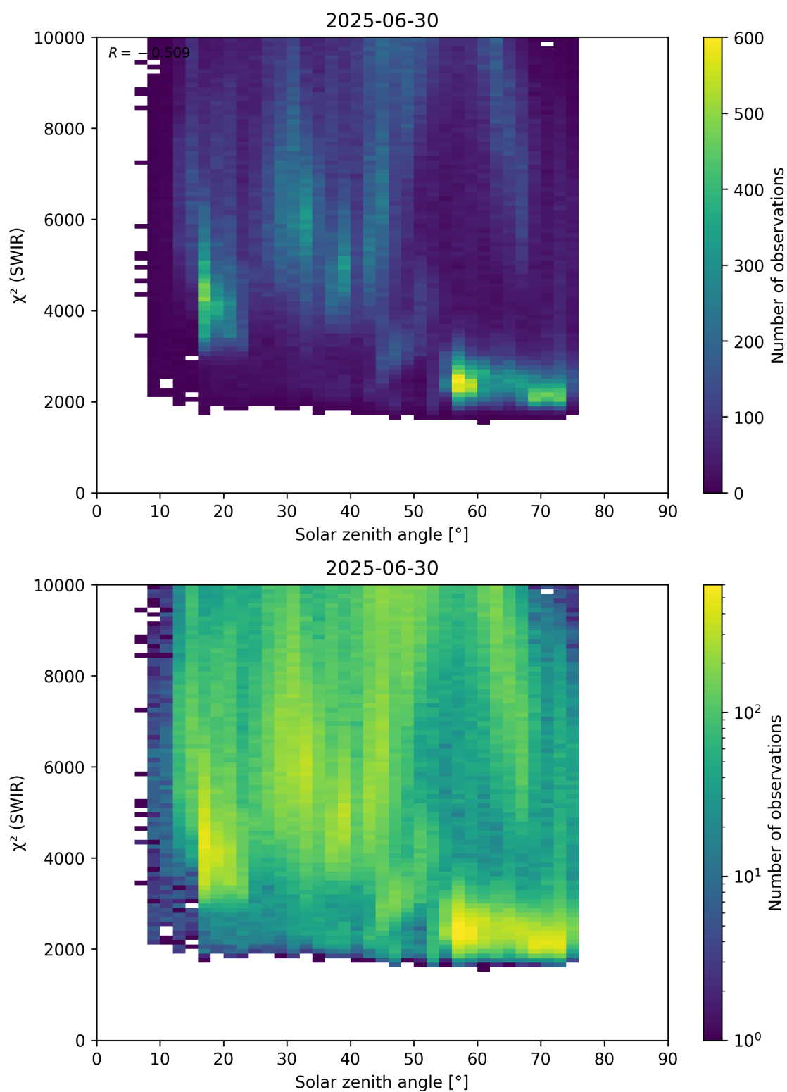
Figure 95: Scatter density plot of “Solar zenith angle” against “ \chi^2 (SWIR)” for 2025-06-29 to 2025-07-01.
