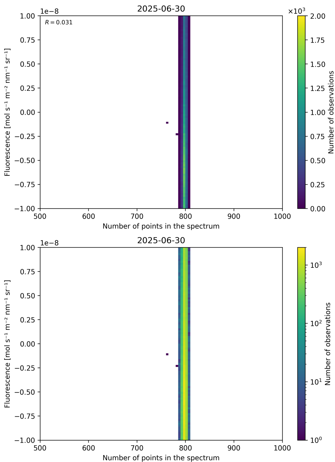
Figure 91: Scatter density plot of “Number of points in the spectrum” against “Fluorescence” for 2025-06-29 to 2025-07-01.
