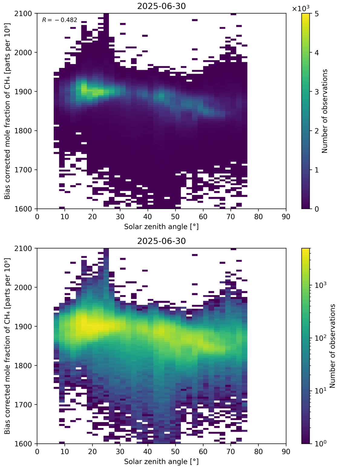
Figure 100: Scatter density plot of “Solar zenith angle” against “Bias corrected mole fraction of CH 4 ” for 2025-06-29 to 2025-07-01.
