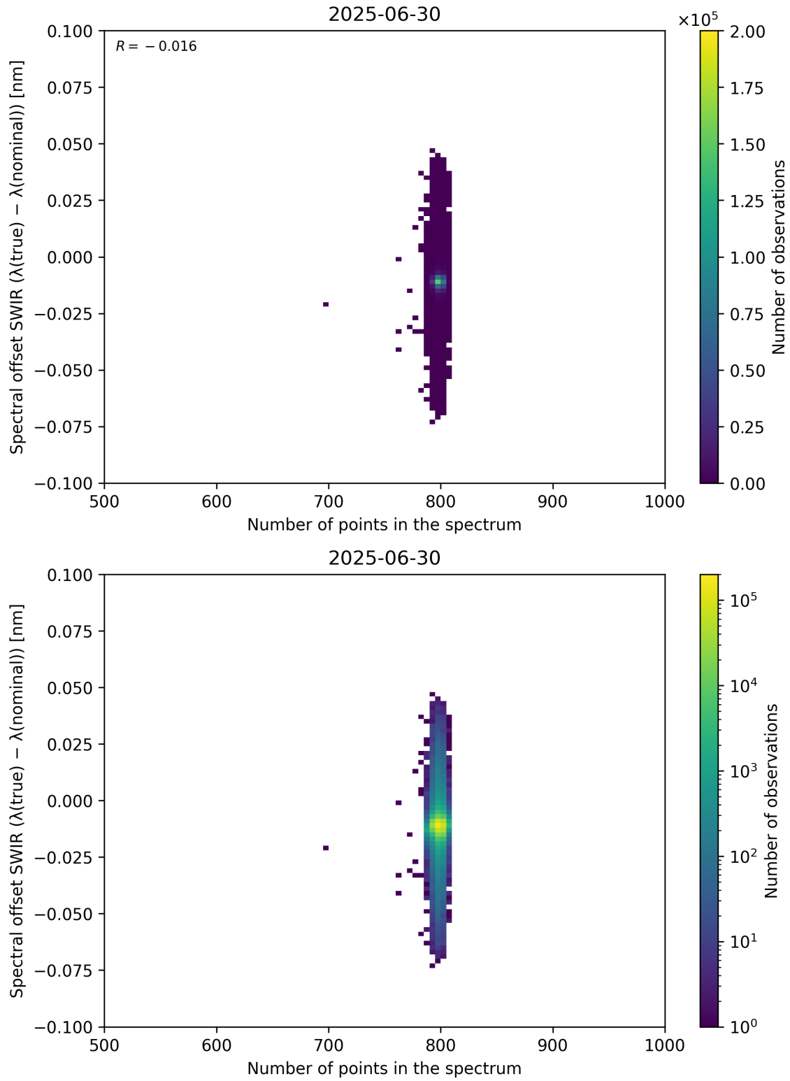
Figure 93: Scatter density plot of “Number of points in the spectrum” against “Spectral offset SWIR ( \lambda_{\text{true}} - \lambda_{\text{nominal}} )” for 2025-06-29 to 2025-07-01.
