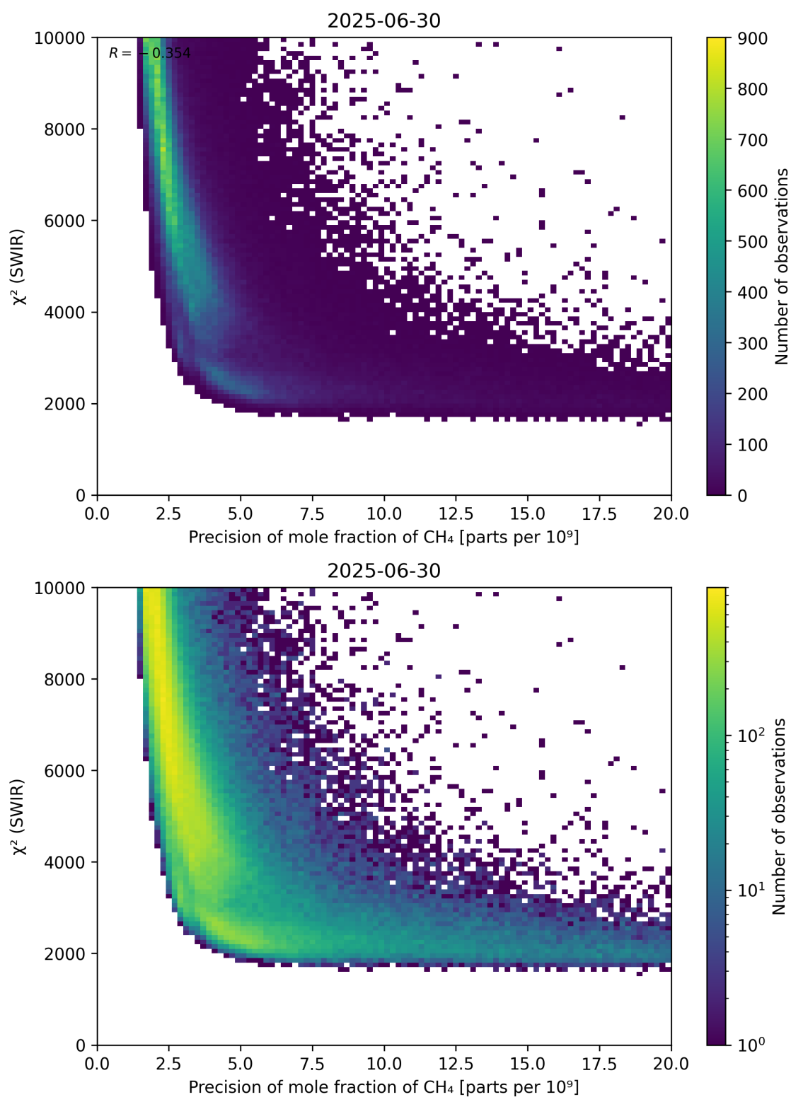
Figure 79: Scatter density plot of “Precision of mole fraction of \text{CH}_4 ” against “ \chi^2 (SWIR)” for 2025-06-29 to 2025-07-01.
