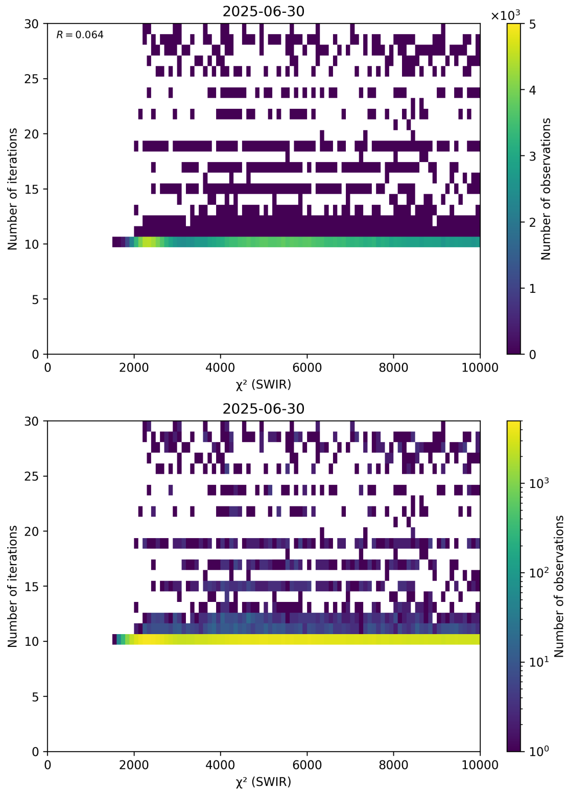
Figure 50: Scatter density plot of “ \chi^2 (SWIR)” against “Number of iterations” for 2025-06-29 to 2025-07-01.
