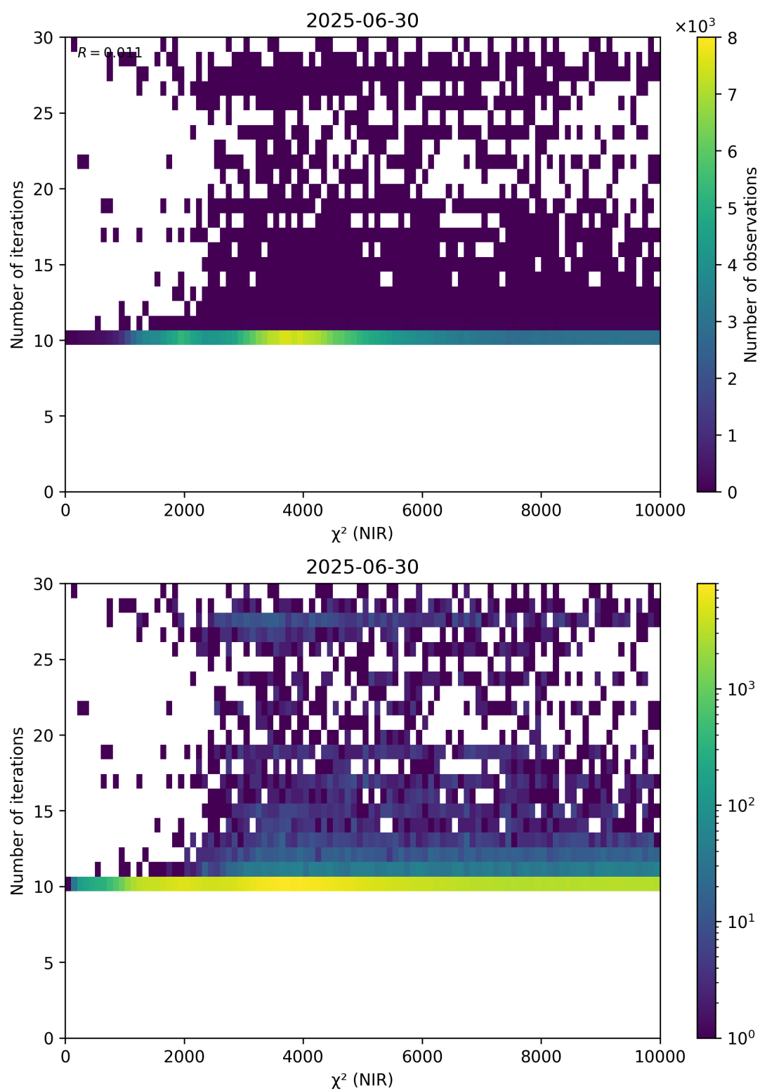
Figure 46: Scatter density plot of “ \chi^2 (NIR)” against “Number of iterations” for 2025-06-29 to 2025-07-01.
