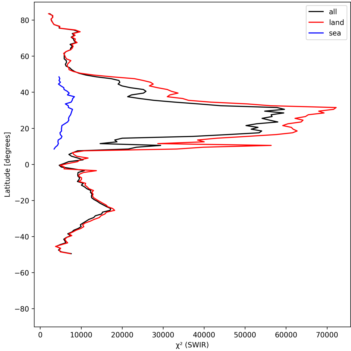
Figure 17: Zonal average of “ \chi^2 (SWIR)” for 2025-06-29 to 2025-07-01.
