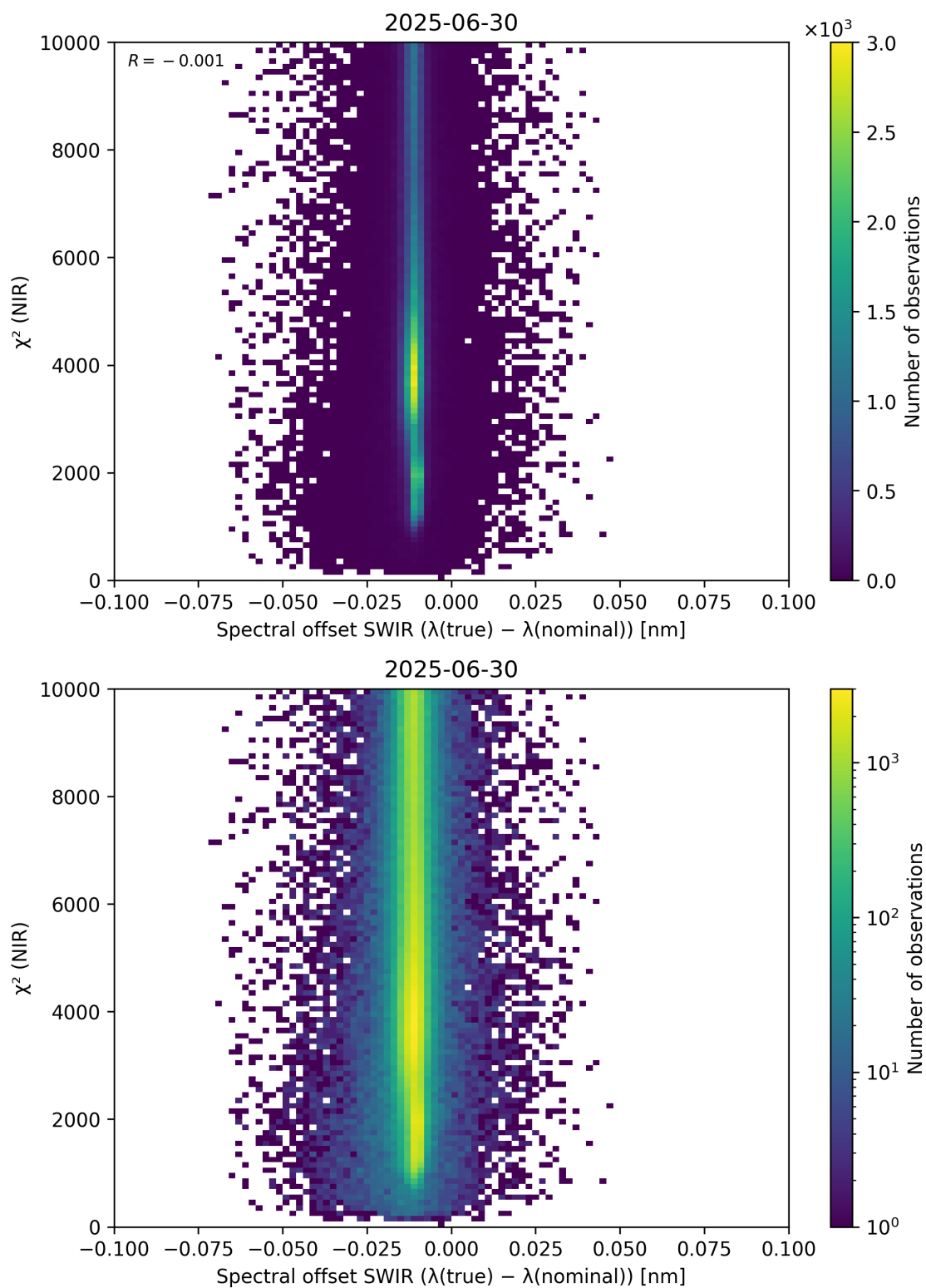
Figure 117: Scatter density plot of “Spectral offset SWIR ( \lambda_{\text{true}} - \lambda_{\text{nominal}} )” against “ \chi^2 (NIR)” for 2025-06-29 to 2025-07-01.
