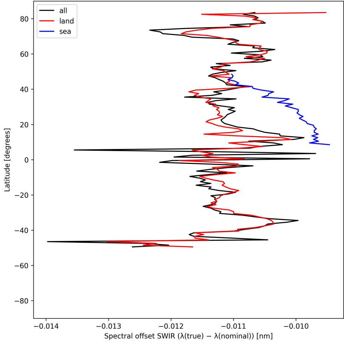
Figure 16: Zonal average of “Spectral offset SWIR ( \lambda_{\text{true}} - \lambda_{\text{nominal}} )” for 2025-06-29 to 2025-07-01.
