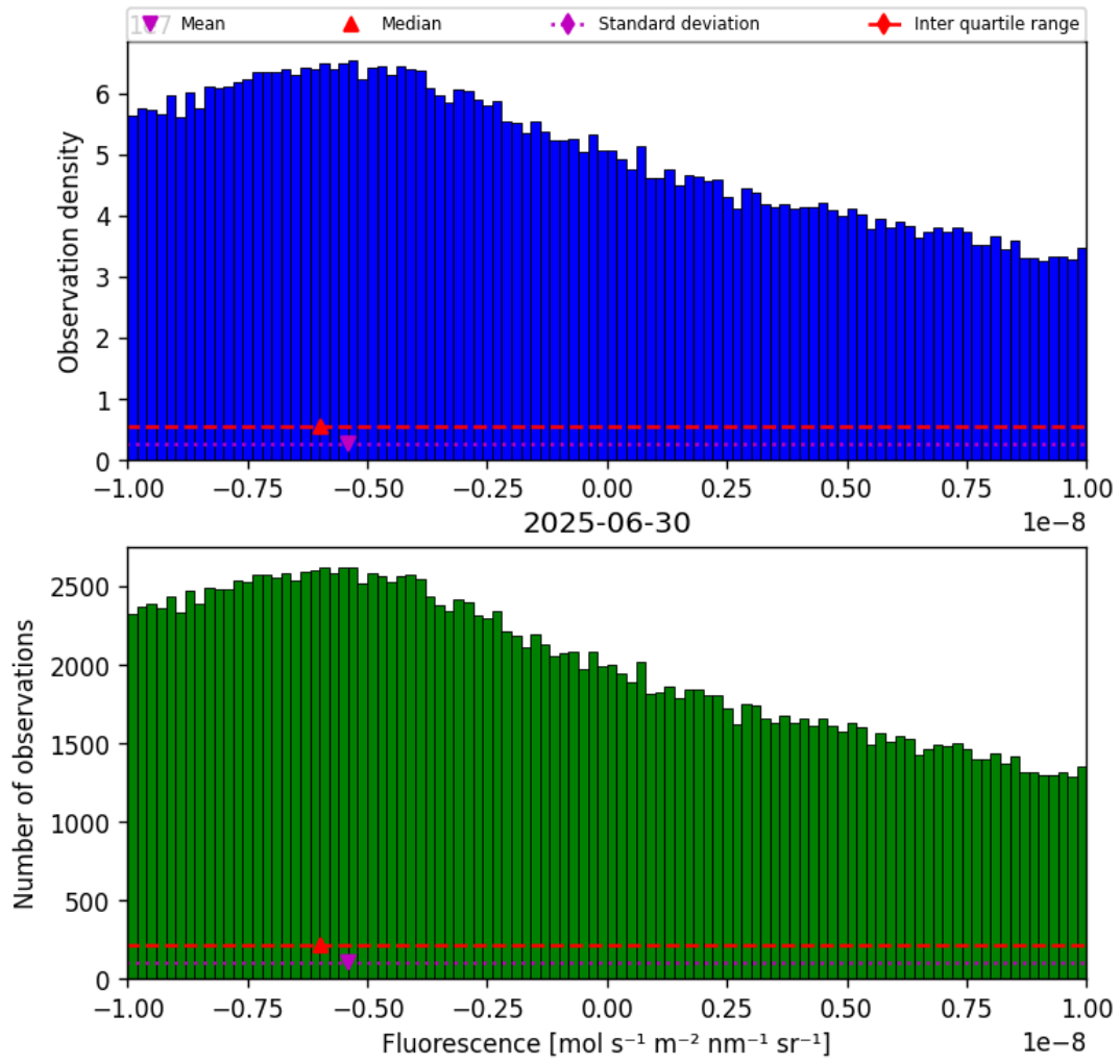
Figure 32: Histogram of “Fluorescence” for 2025-06-29 to 2025-07-01
