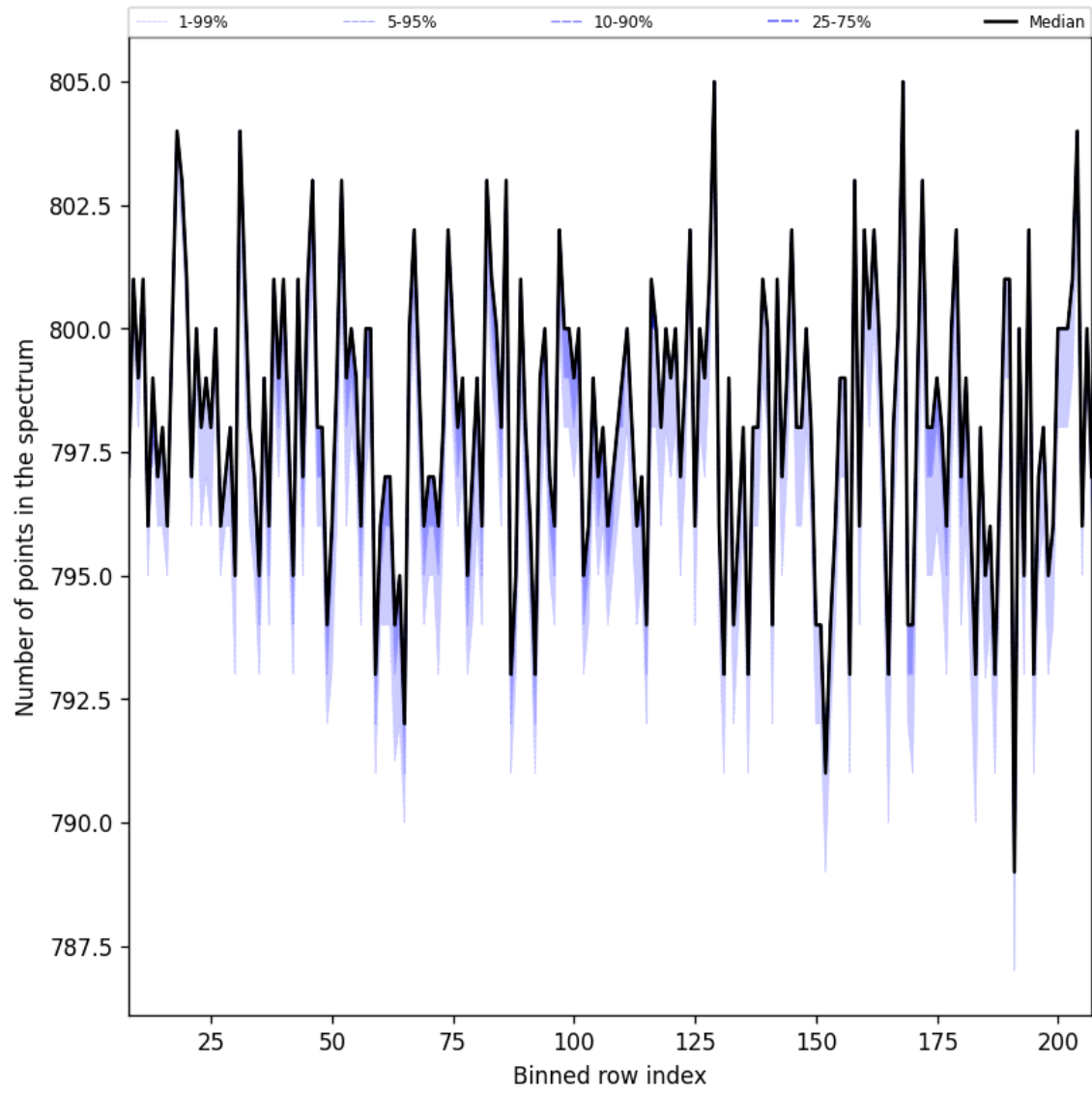
Figure 37: Along track statistics of “Number of points in the spectrum” for 2025-06-29 to 2025-07-01
