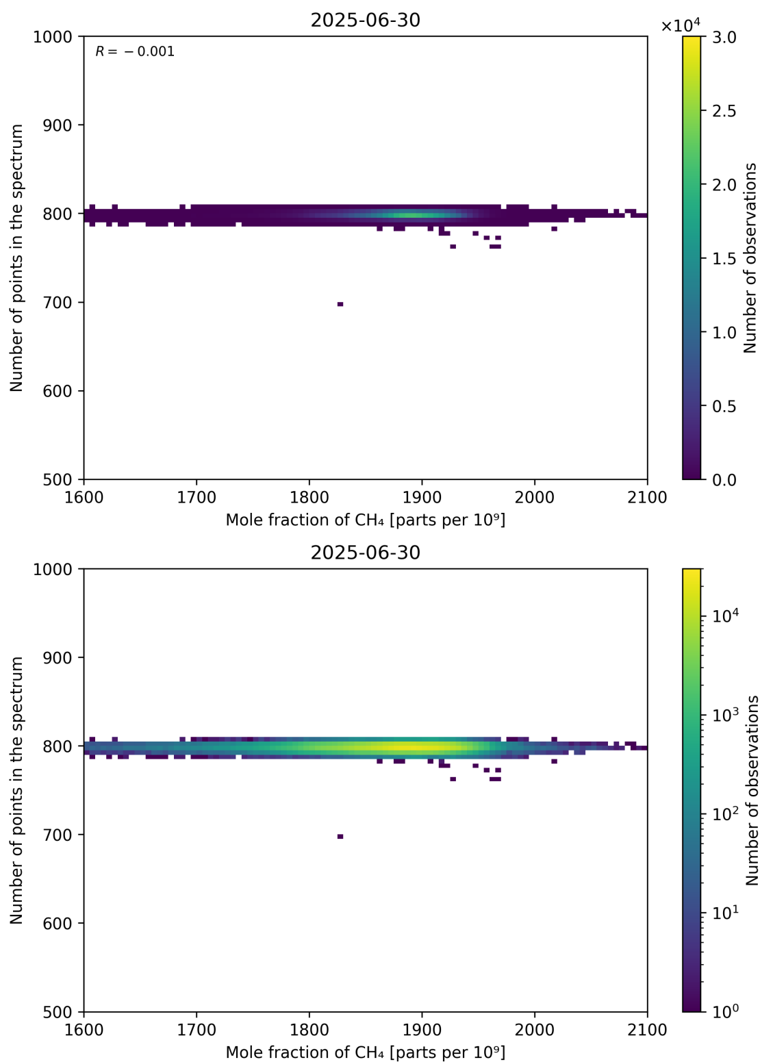
Figure 77: Scatter density plot of “Mole fraction of CH 4 ” against “Number of points in the spectrum” for 2025-06-29 to 2025-07-01.
