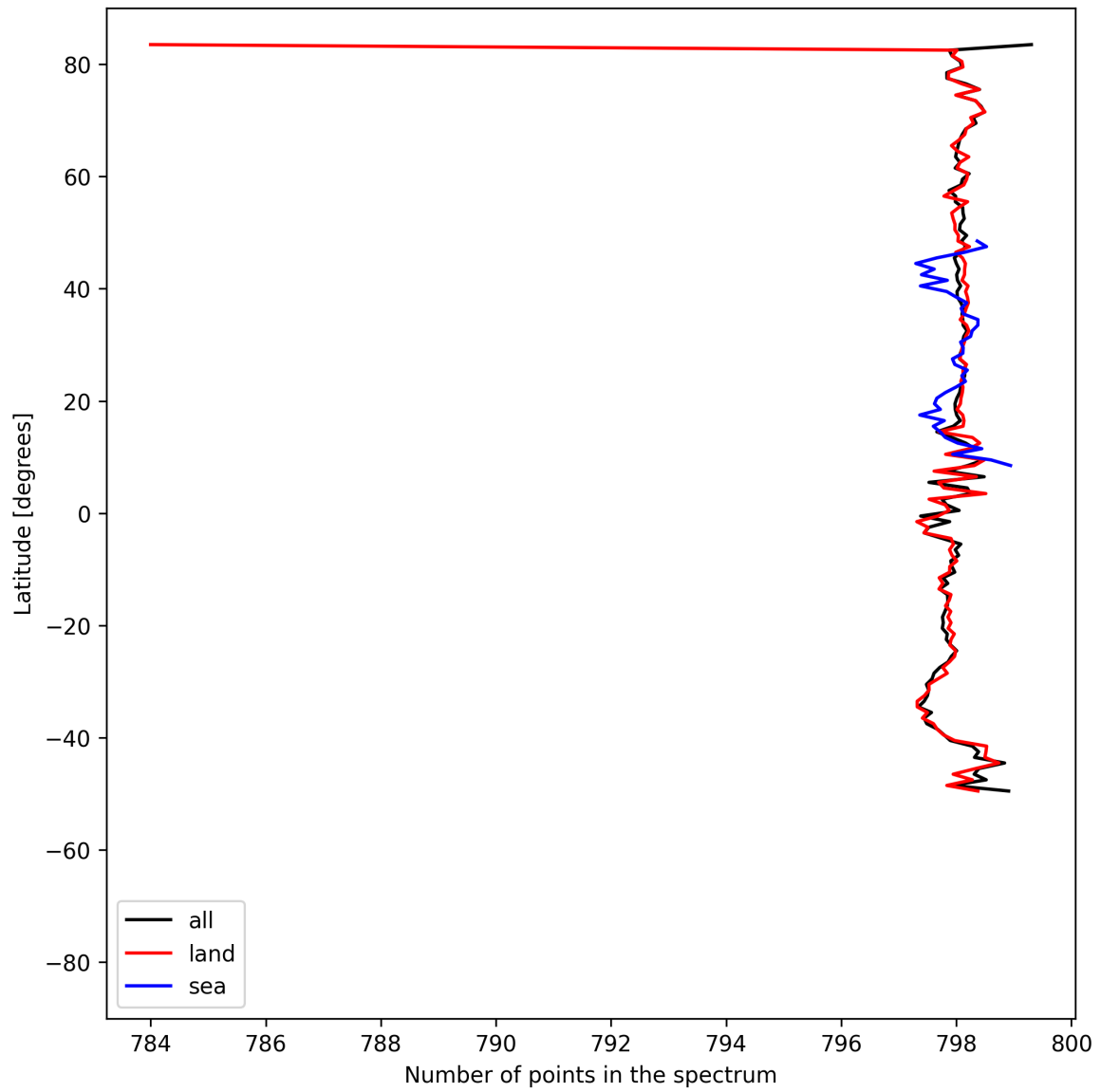
Figure 15: Zonal average of “Number of points in the spectrum” for 2025-06-29 to 2025-07-01.
