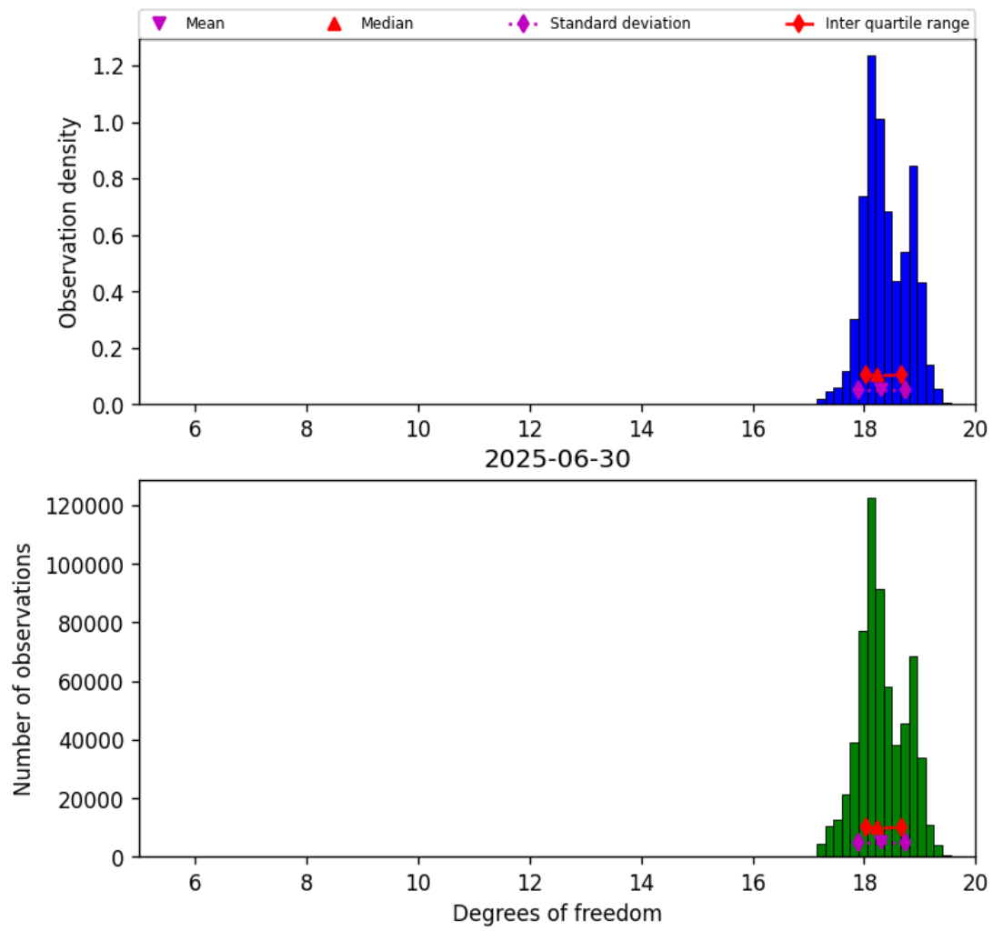
Figure 30: Histogram of “Degrees of freedom” for 2025-06-29 to 2025-07-01
