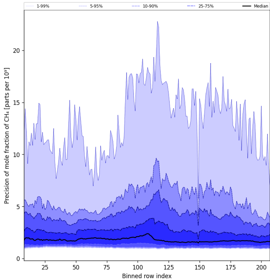
Figure 35: Along track statistics of “Precision of mole fraction of CH 4 ” for 2025-06-29 to 2025-07-01
