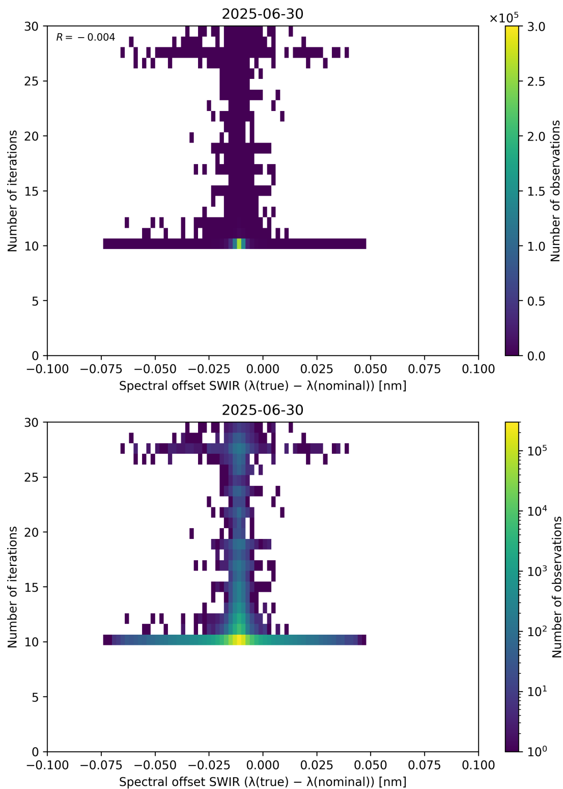
Figure 121: Scatter density plot of “Spectral offset SWIR ( \lambda_{\text{true}} - \lambda_{\text{nominal}} )” against “Number of iterations” for 2025-06-29 to 2025-07-01.
