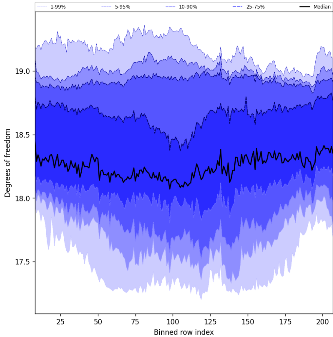
Figure 41: Along track statistics of “Degrees of freedom” for 2025-06-29 to 2025-07-01
