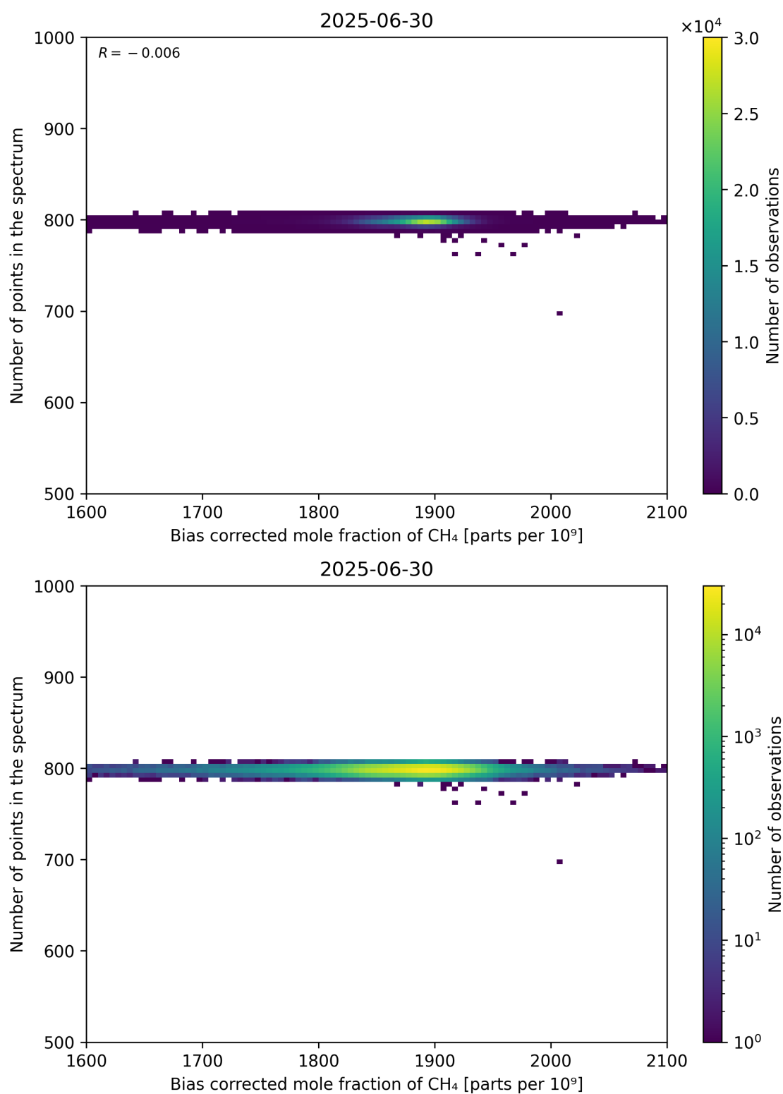
Figure 68: Scatter density plot of “Bias corrected mole fraction of CH 4 ” against “Number of points in the spectrum” for 2025-06-29 to 2025-07-01.
