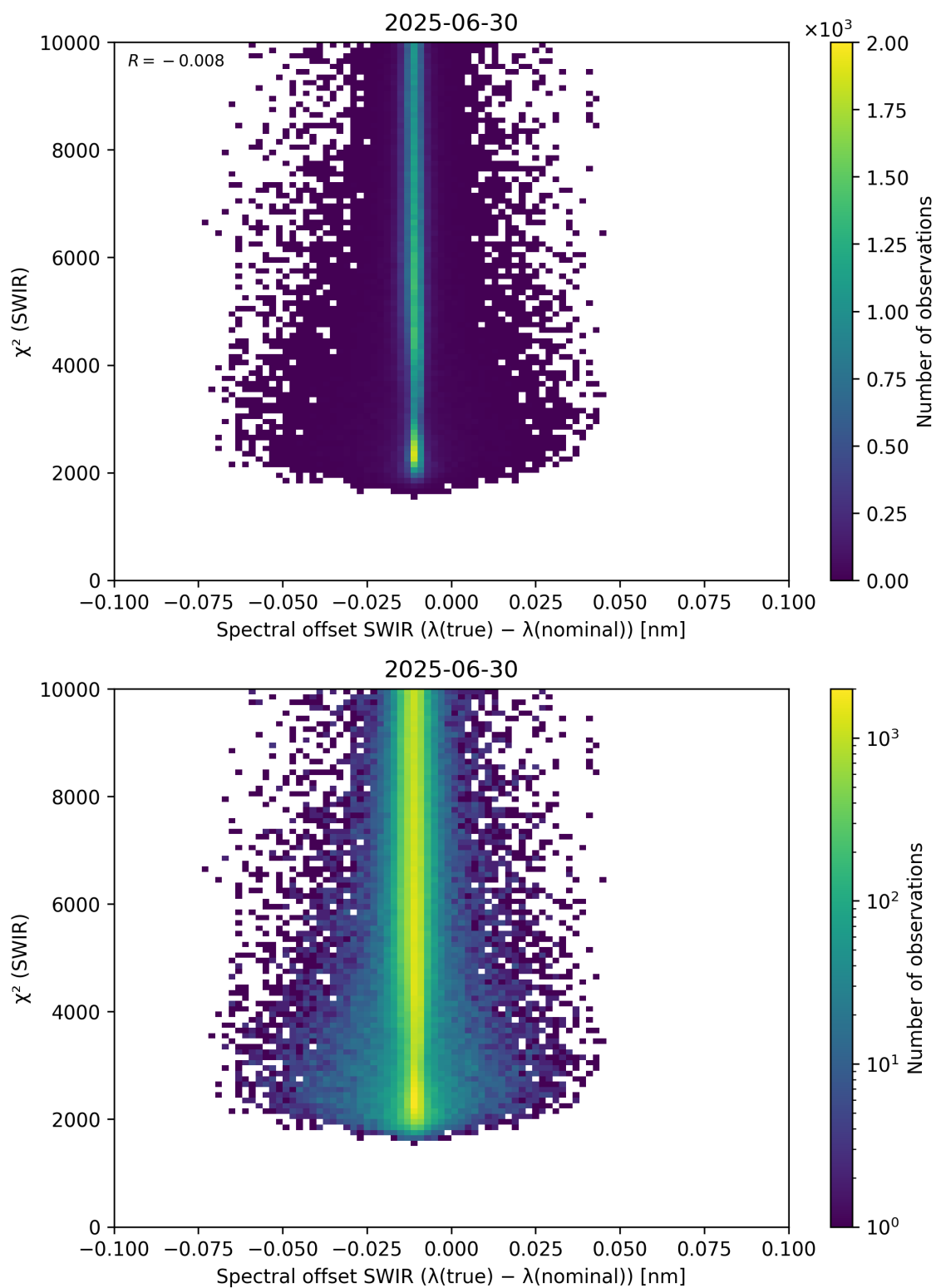
Figure 118: Scatter density plot of “Spectral offset SWIR ( \lambda_{\text{true}} - \lambda_{\text{nominal}} )” against “ \chi^2 (SWIR)” for 2025-06-29 to 2025-07-01.
