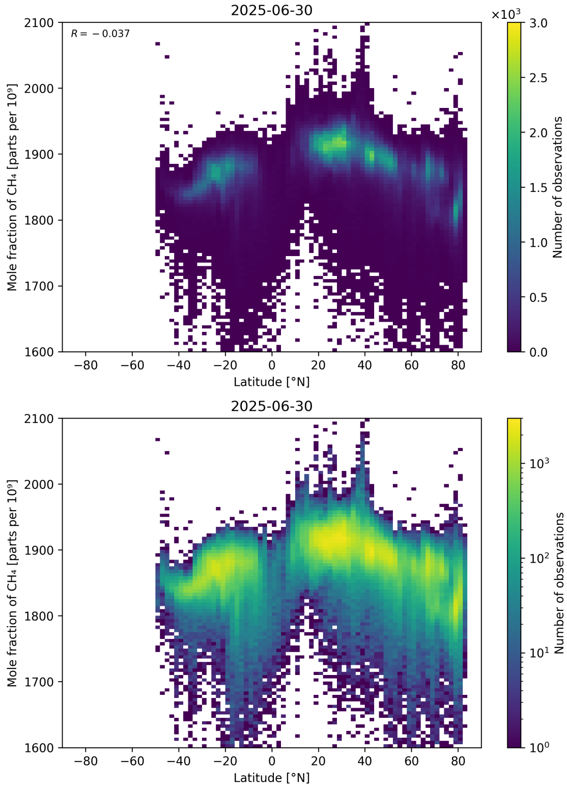
Figure 57: Scatter density plot of “Latitude” against “Mole fraction of \text{CH}_4 ” for 2025-06-29 to 2025-07-01.
