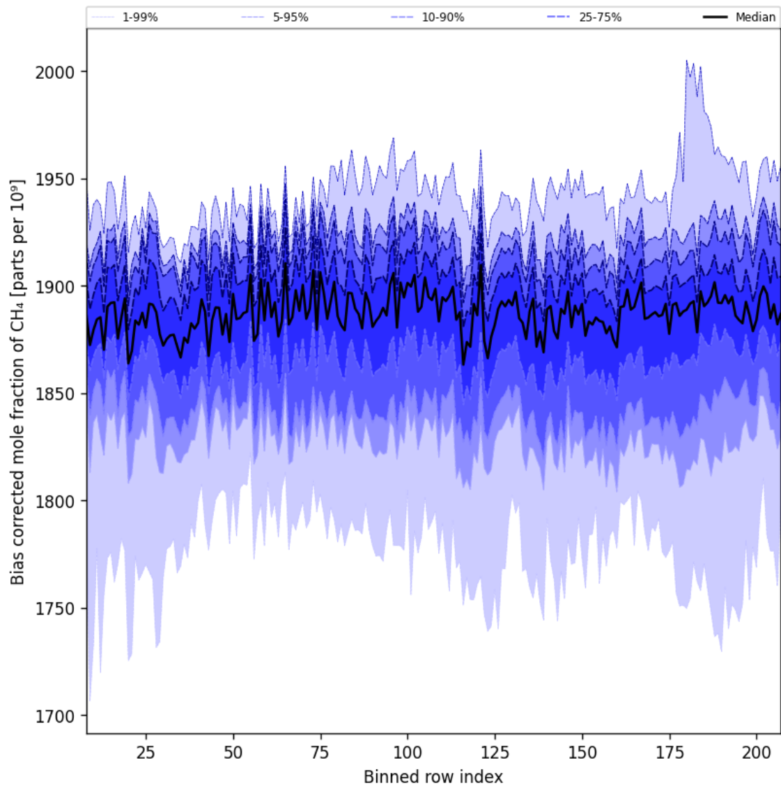
Figure 36: Along track statistics of “Bias corrected mole fraction of CH 4 ” for 2025-06-29 to 2025-07-01
