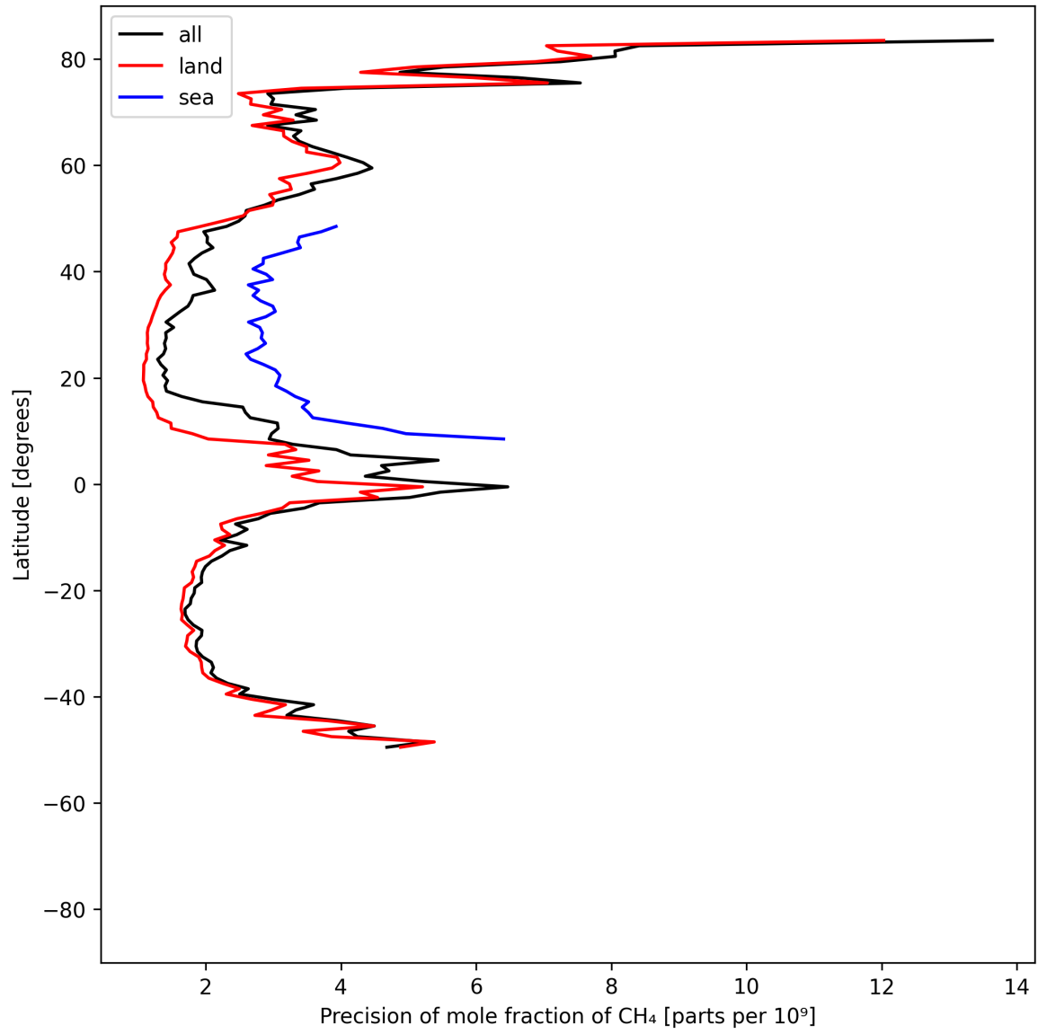
Figure 13: Zonal average of “Precision of mole fraction of CH 4 ” for 2025-06-29 to 2025-07-01.
