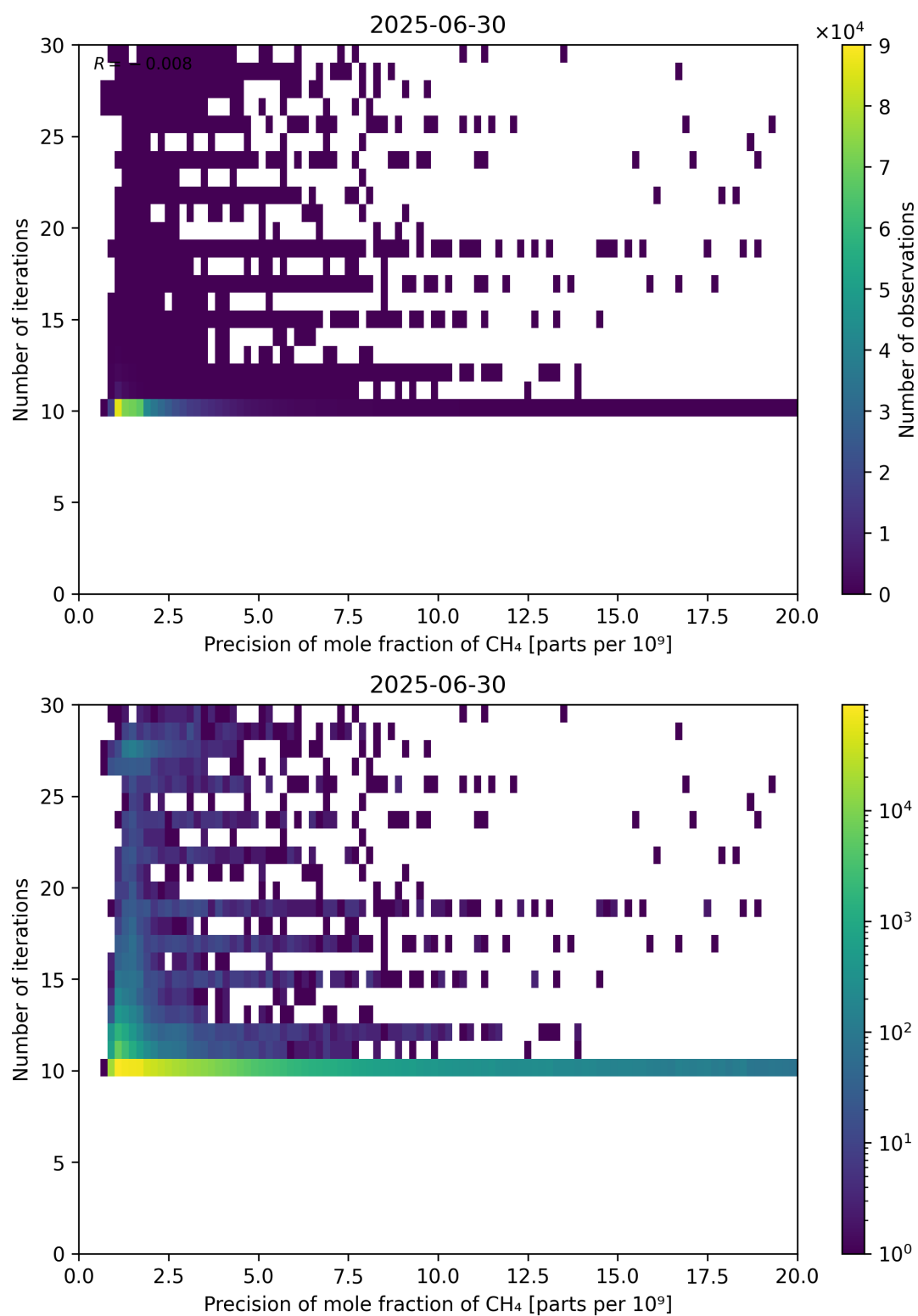
Figure 83: Scatter density plot of “Precision of mole fraction of CH 4 ” against “Number of iterations” for 2025-06-29 to 2025-07-01.
