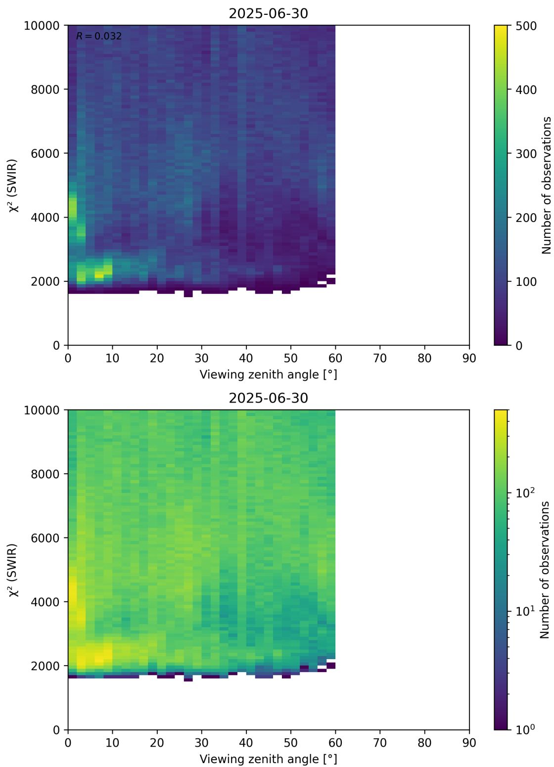
Figure 106: Scatter density plot of “Viewing zenith angle” against “ \chi^2 (SWIR)” for 2025-06-29 to 2025-07-01.
