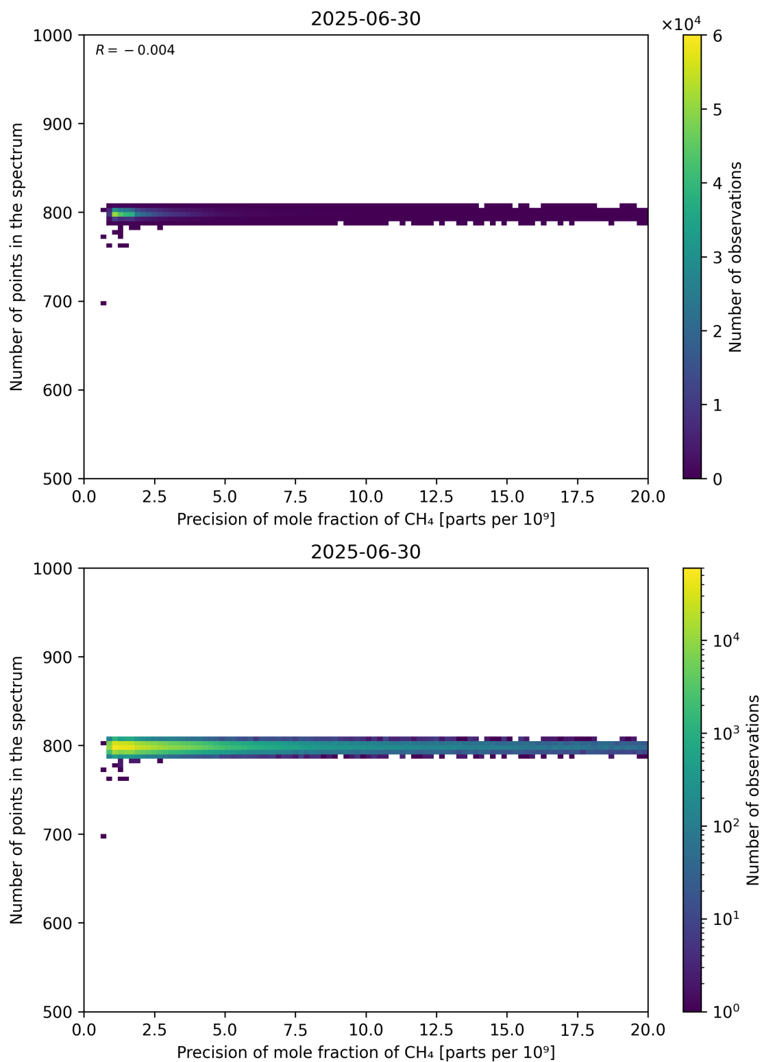
Figure 84: Scatter density plot of “Precision of mole fraction of CH 4 ” against “Number of points in the spectrum” for 2025-06-29 to 2025-07-01.
