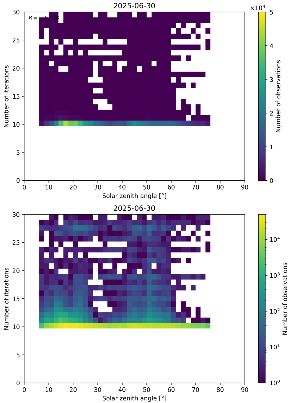
Figure 102: Scatter density plot of “Solar zenith angle” against “Number of iterations” for 2025-06-29 to 2025-07-01.
