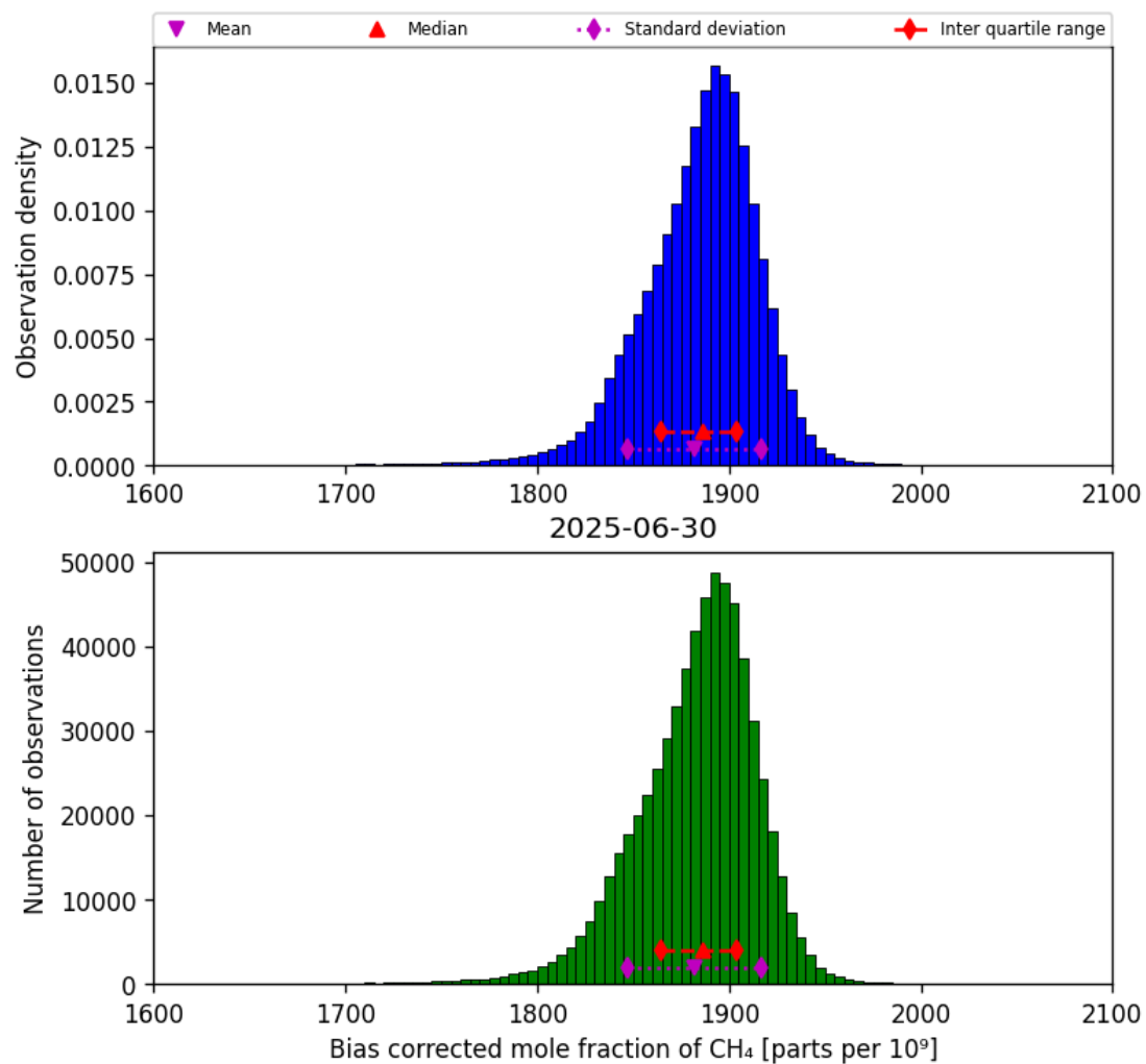
Figure 25: Histogram of “Bias corrected mole fraction of CH 4 ” for 2025-06-29 to 2025-07-01
