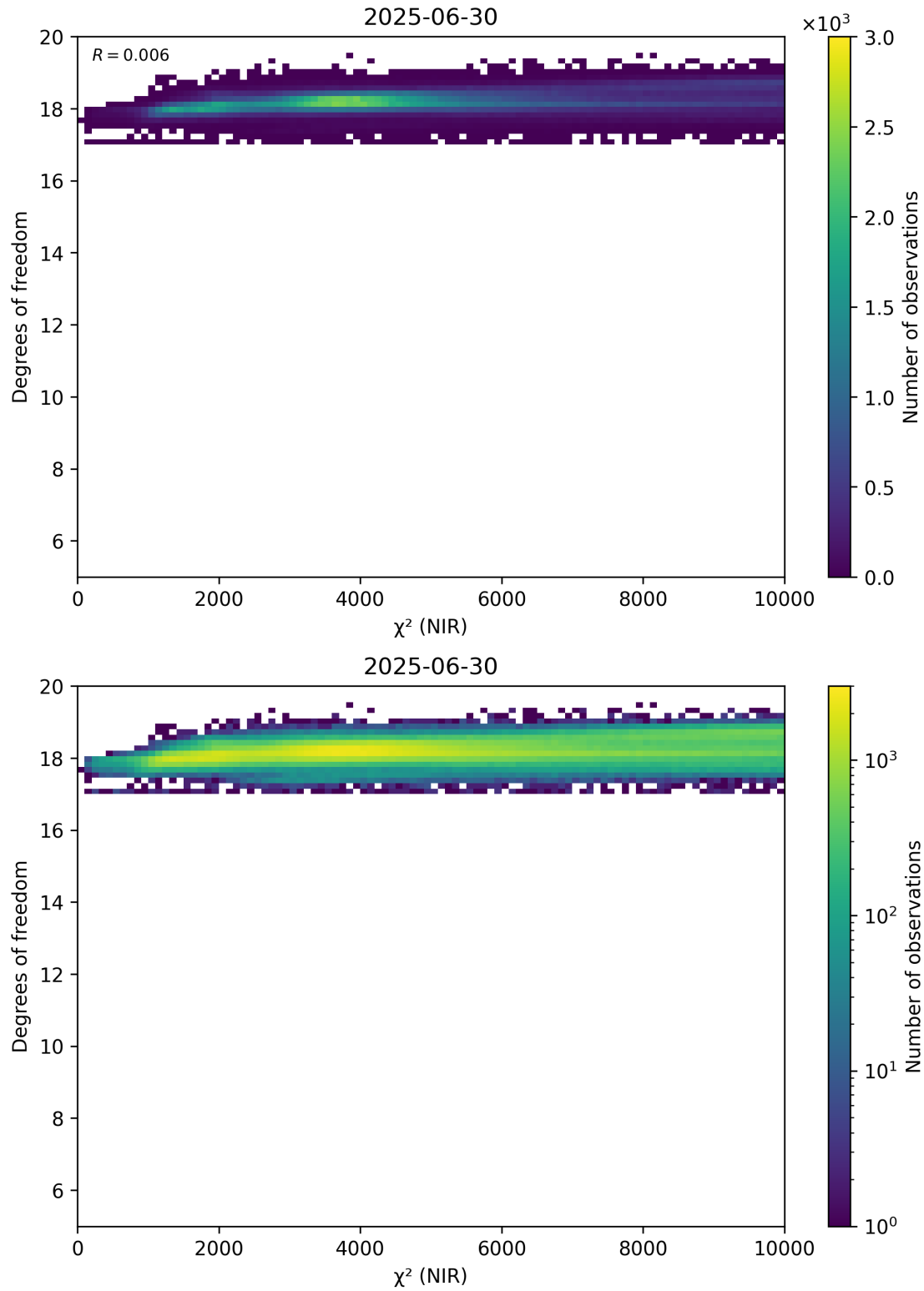
Figure 44: Scatter density plot of “ \chi^2 (NIR)” against “Degrees of freedom” for 2025-06-29 to 2025-07-01.
