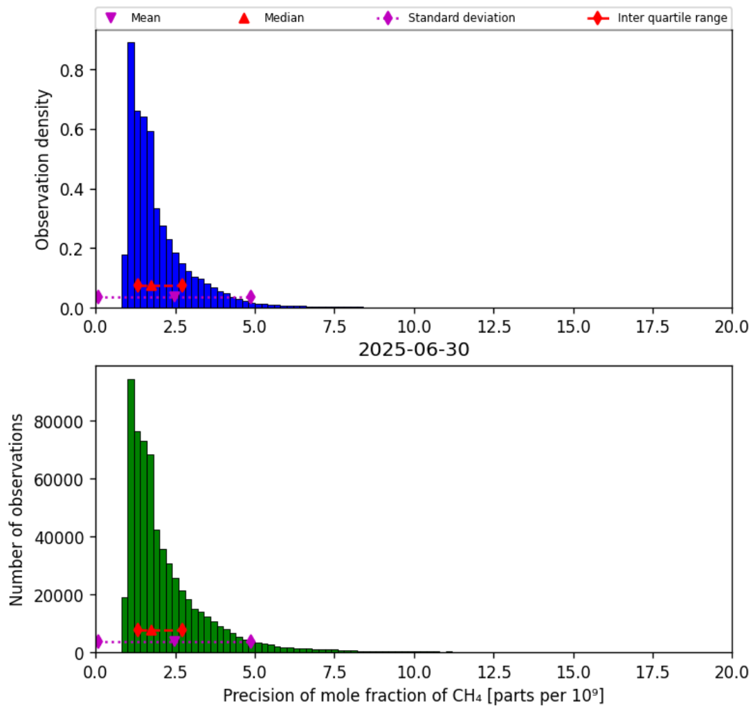
Figure 24: Histogram of “Precision of mole fraction of CH 4 ” for 2025-06-29 to 2025-07-01
