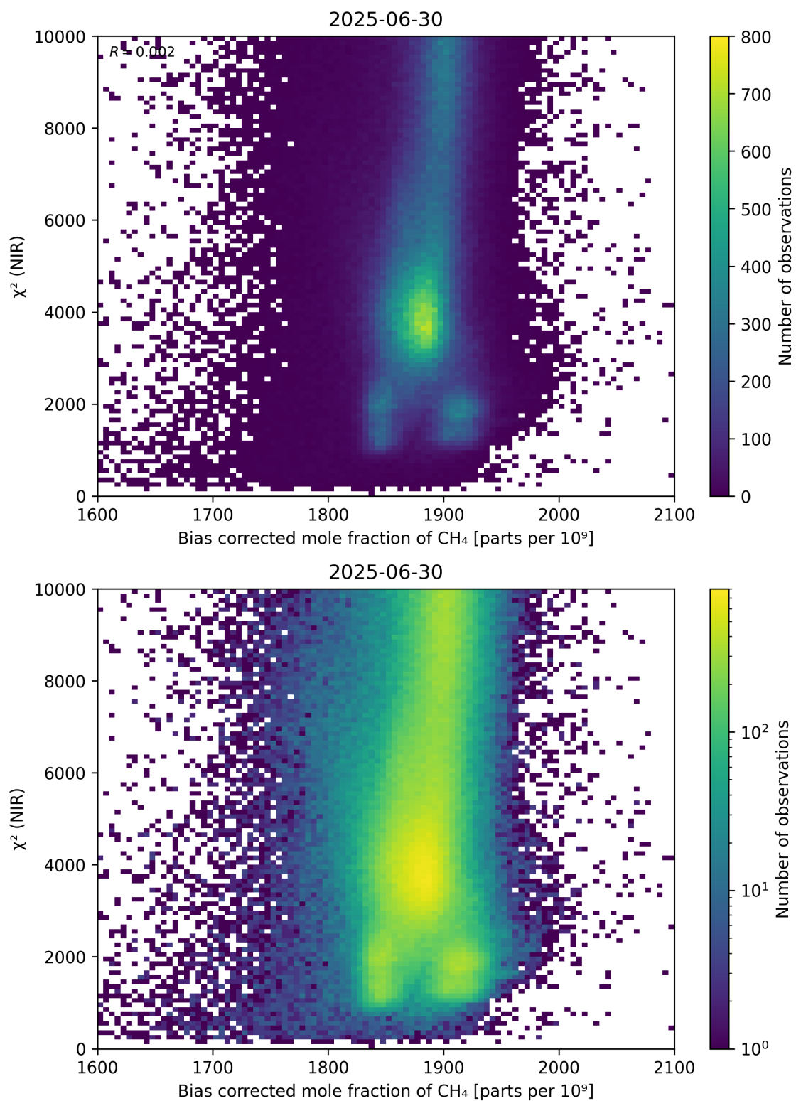
Figure 63: Scatter density plot of “Bias corrected mole fraction of CH 4 ” against “ \chi^2 (NIR)” for 2025-06-29 to 2025-07-01.
