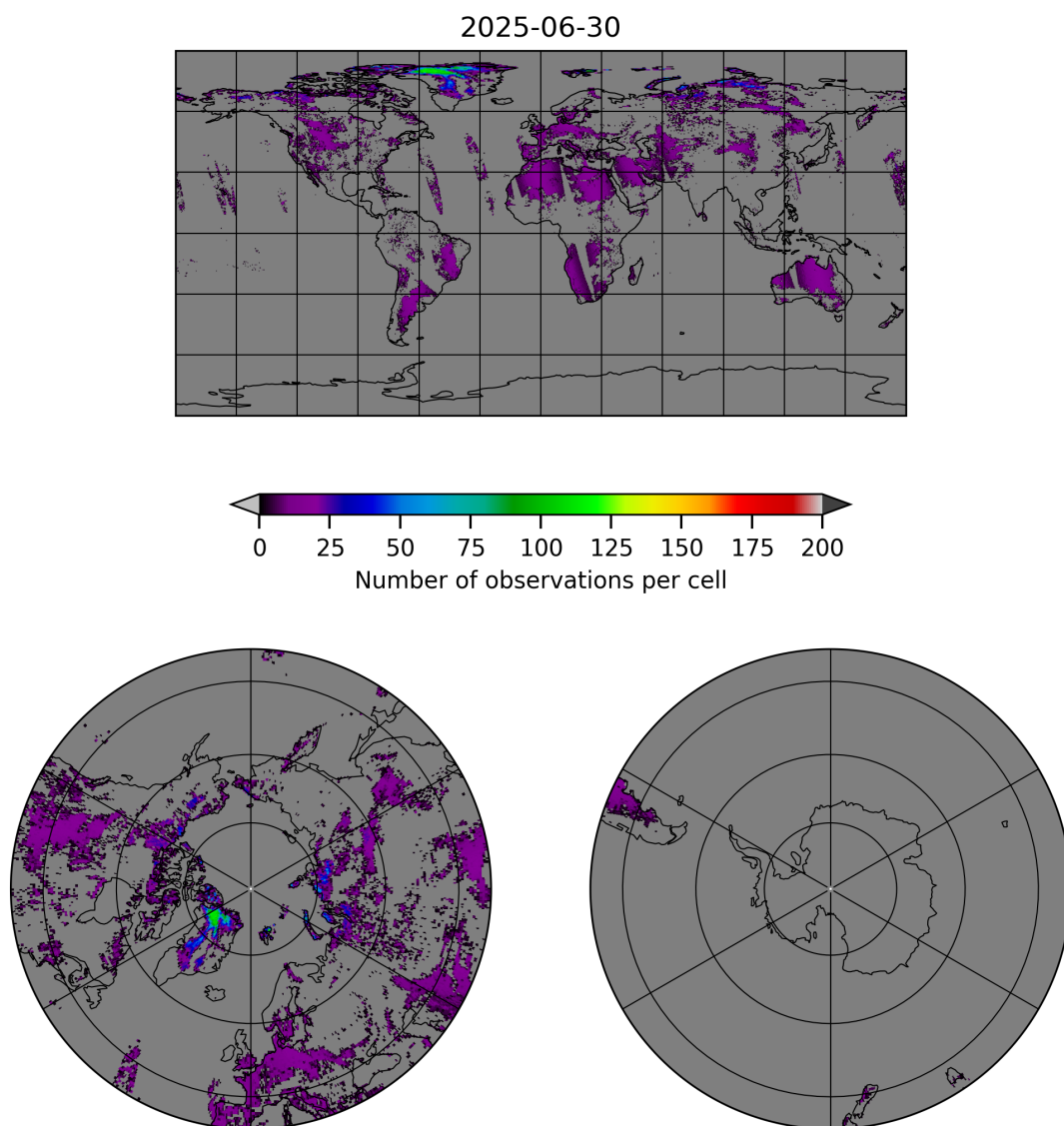
Figure 10: Map of the number of observations for 2025-06-29 to 2025-07-01
