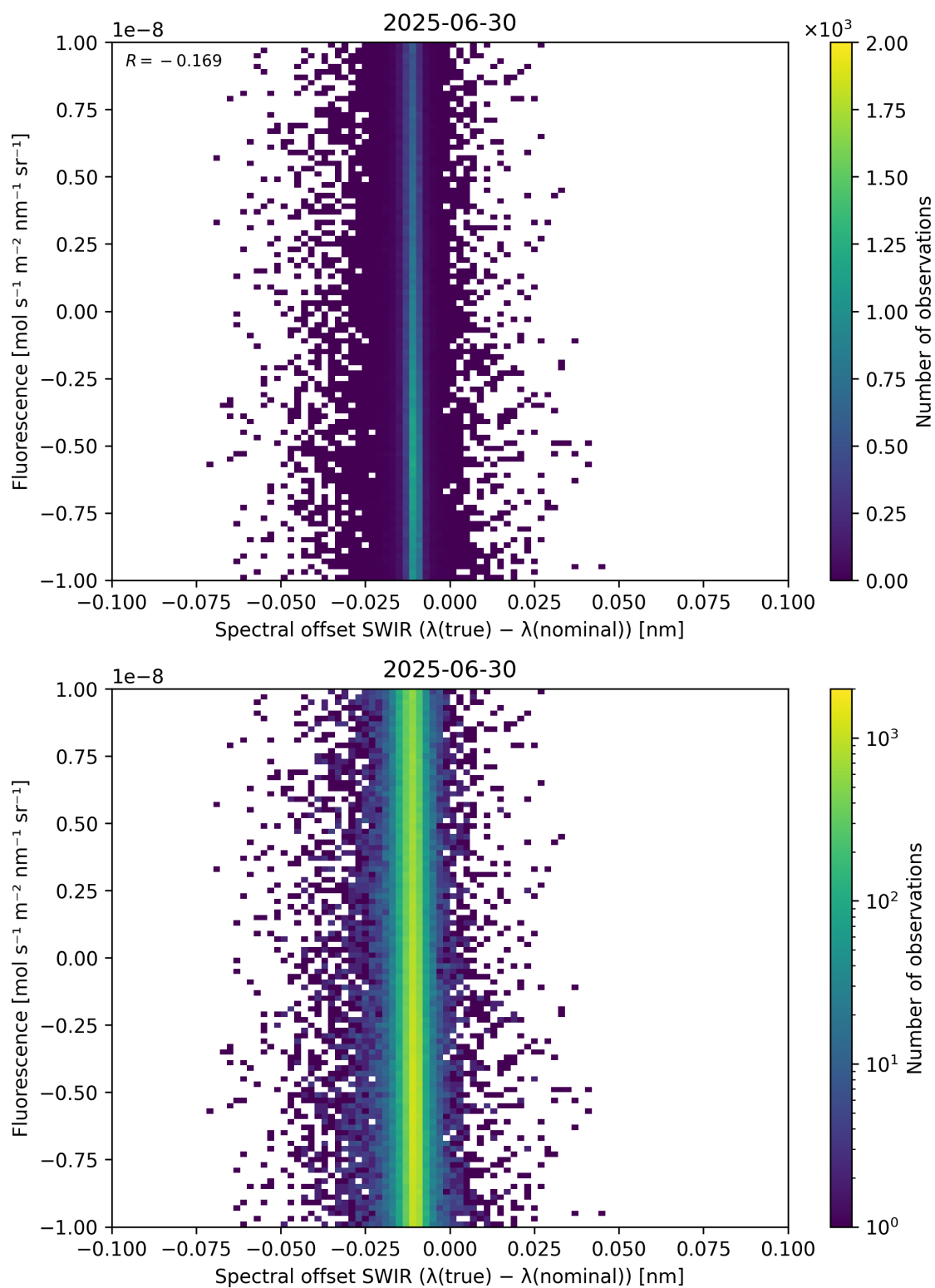
Figure 120: Scatter density plot of “Spectral offset SWIR ( \lambda_{\text{true}} - \lambda_{\text{nominal}} )” against “Fluorescence” for 2025-06-29 to 2025-07-01.
