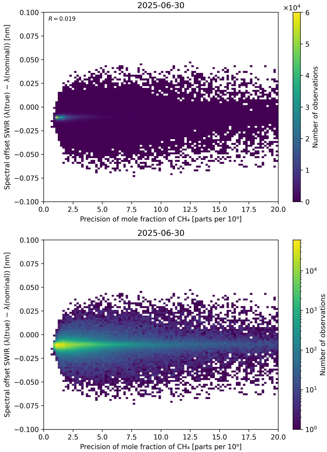
Figure 85: Scatter density plot of “Precision of mole fraction of CH 4 ” against “Spectral offset SWIR ( \lambda_{\text{true}} - \lambda_{\text{nominal}} )” for 2025-06-29 to 2025-07-01.
