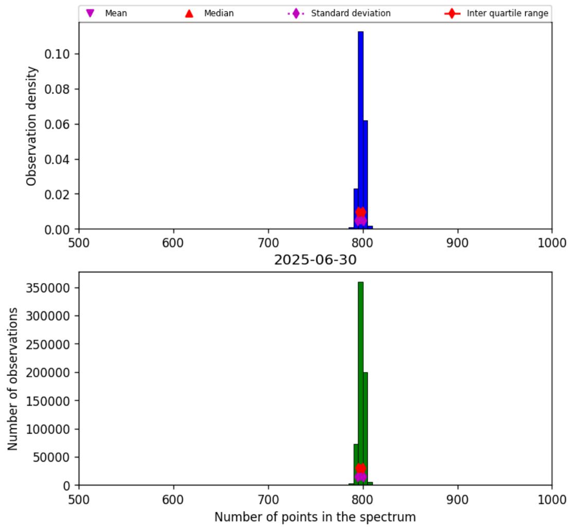
Figure 26: Histogram of “Number of points in the spectrum” for 2025-06-29 to 2025-07-01
