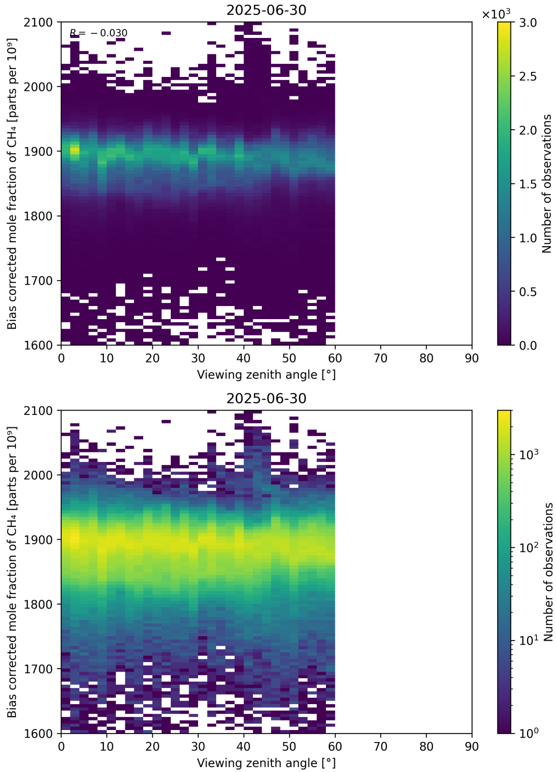
Figure 111: Scatter density plot of “Viewing zenith angle” against “Bias corrected mole fraction of CH 4 ” for 2025-06-29 to 2025-07-01.
