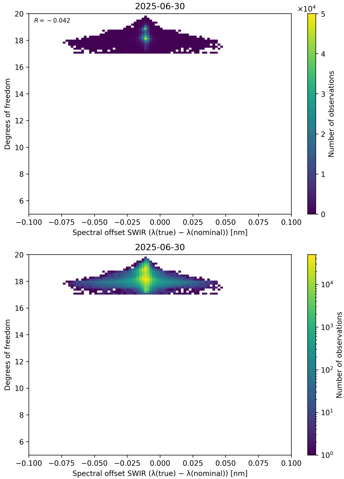
Figure 119: Scatter density plot of “Spectral offset SWIR ( \lambda_{\text{true}} - \lambda_{\text{nominal}} )” against “Degrees of freedom” for 2025-06-29 to 2025-07-01.
