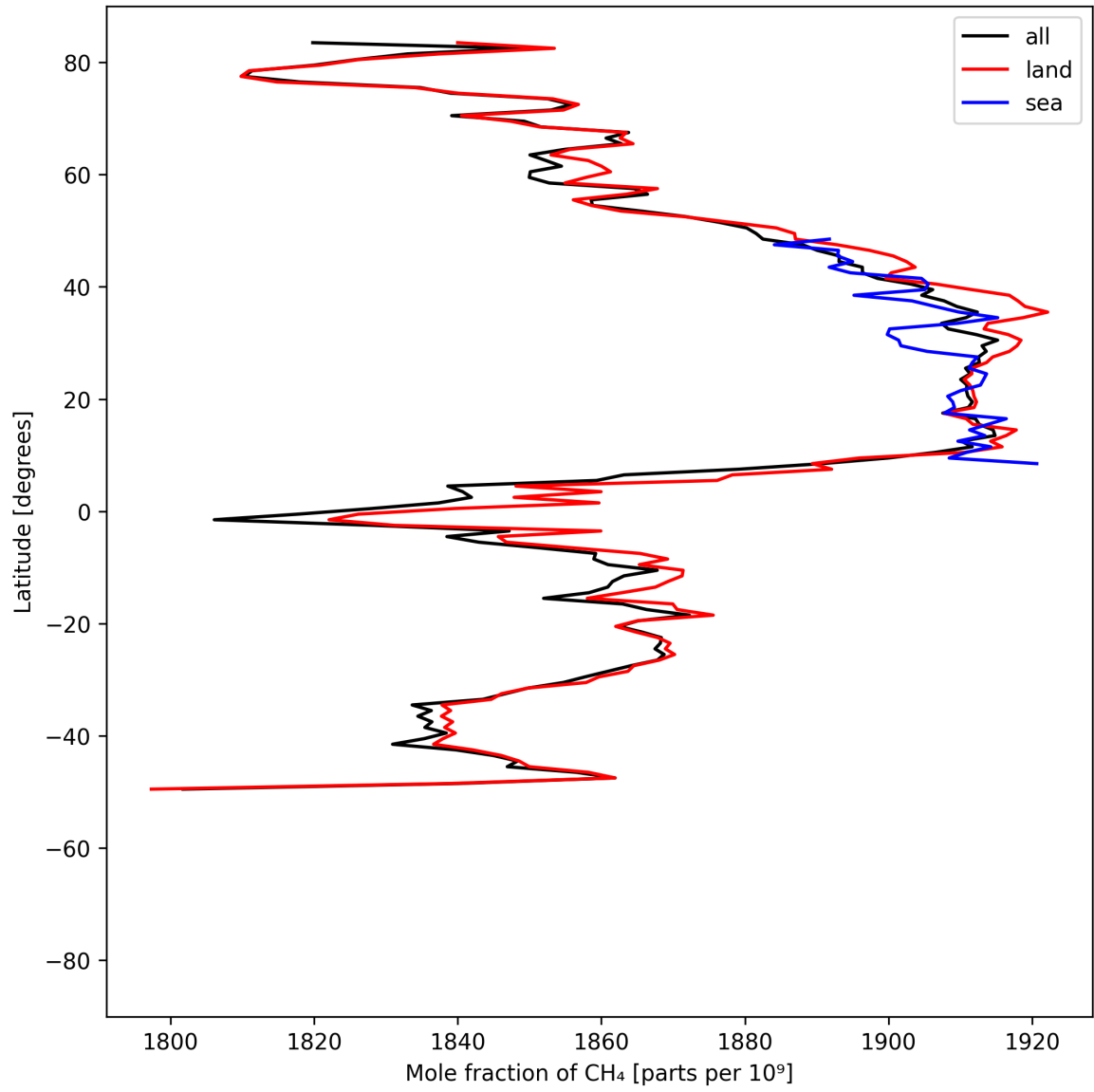
Figure 12: Zonal average of “Mole fraction of \text{CH}_4 ” for 2025-06-29 to 2025-07-01.
