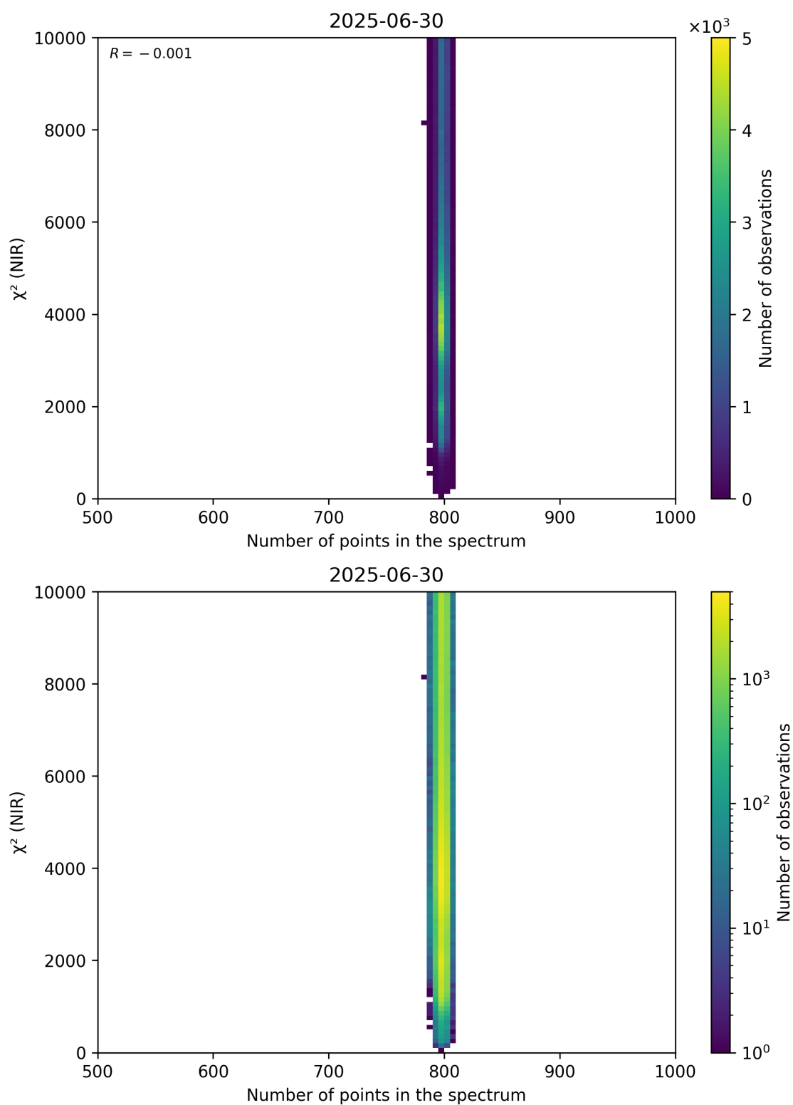
Figure 88: Scatter density plot of “Number of points in the spectrum” against “ \chi^2 (NIR)” for 2025-06-29 to 2025-07-01.
