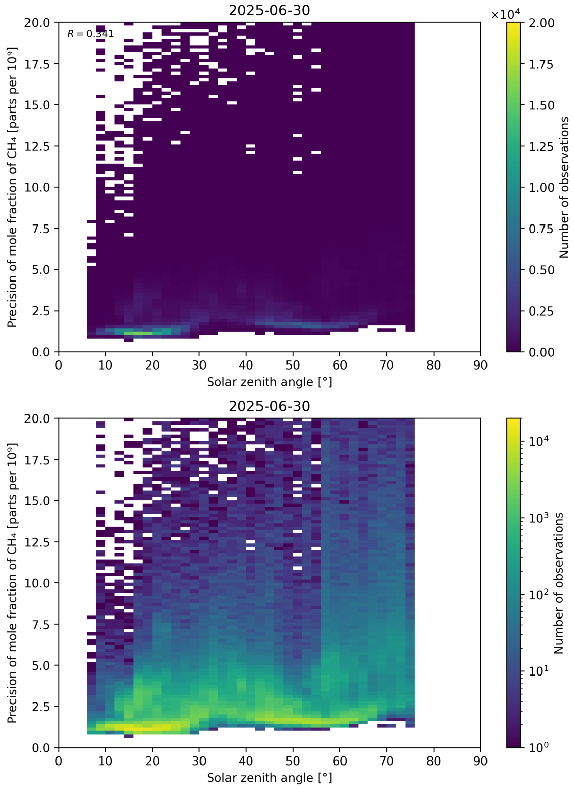
Figure 101: Scatter density plot of “Solar zenith angle” against “Precision of mole fraction of CH 4 ” for 2025-06-29 to 2025-07-01.
