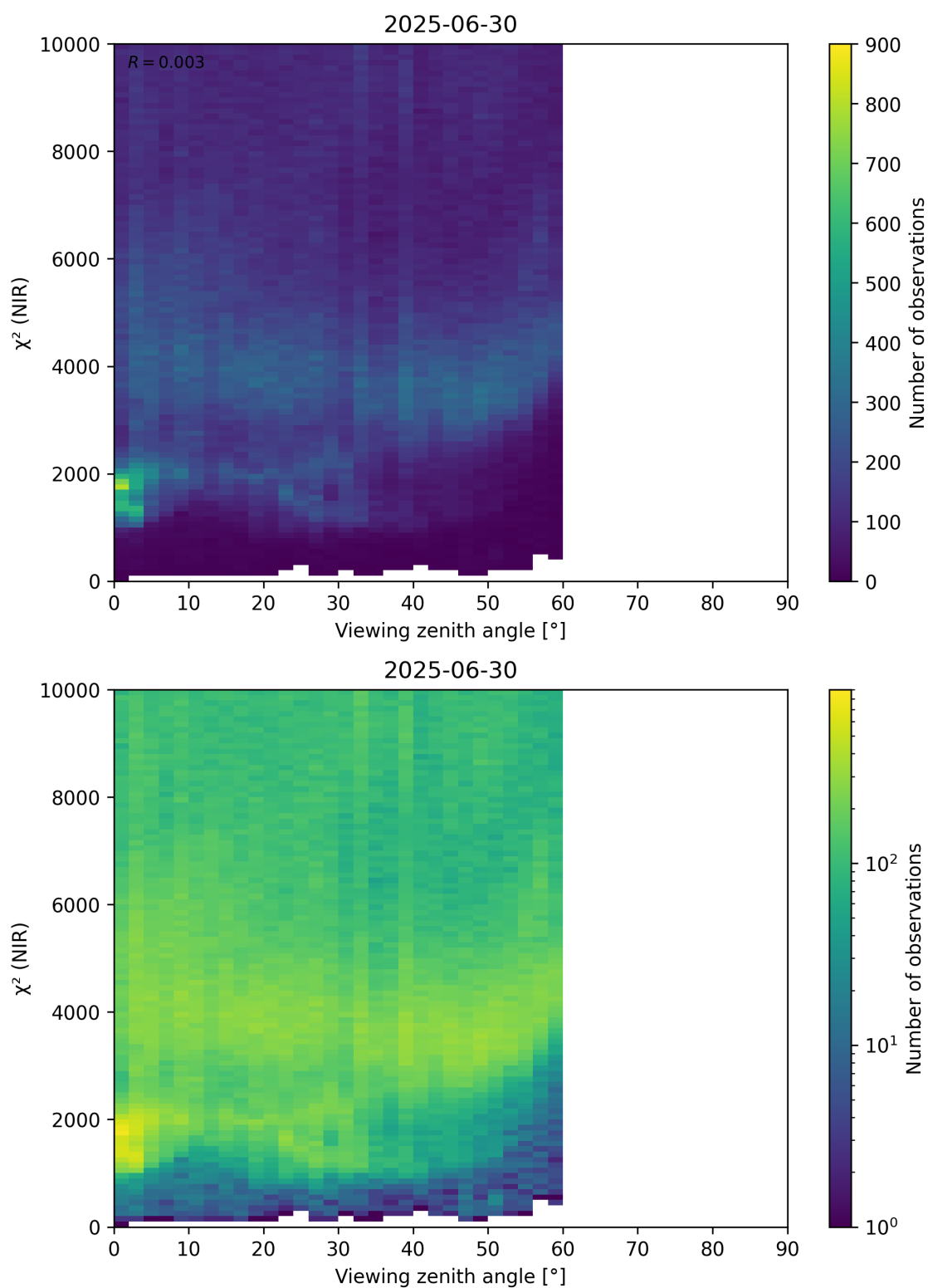
Figure 105: Scatter density plot of “Viewing zenith angle” against “ \chi^2 (NIR)” for 2025-06-29 to 2025-07-01.
