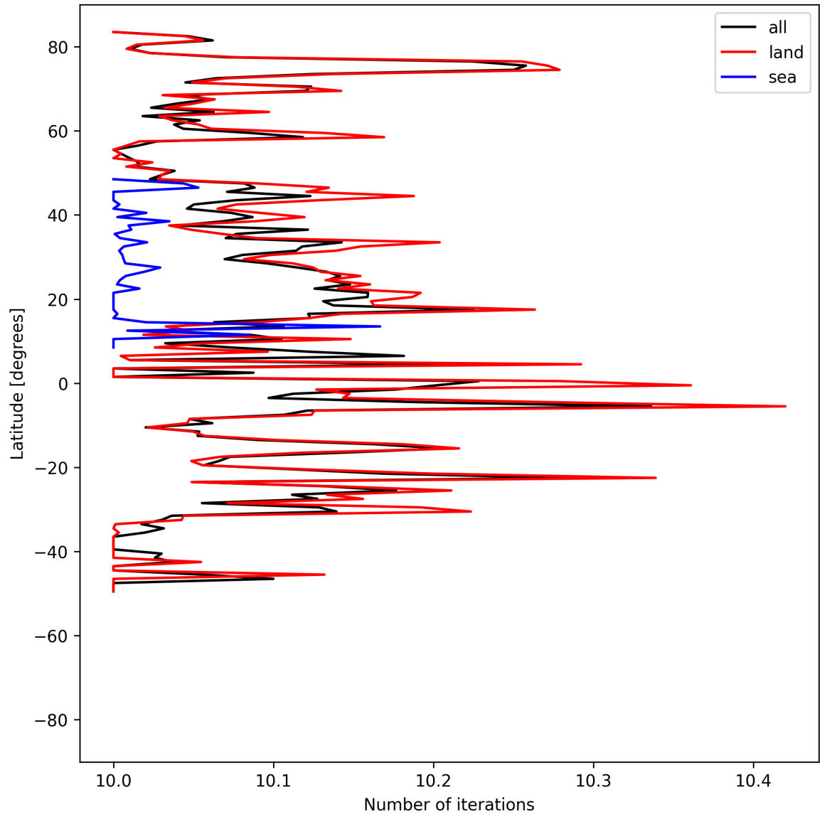
Figure 20: Zonal average of “Number of iterations” for 2025-06-29 to 2025-07-01.
