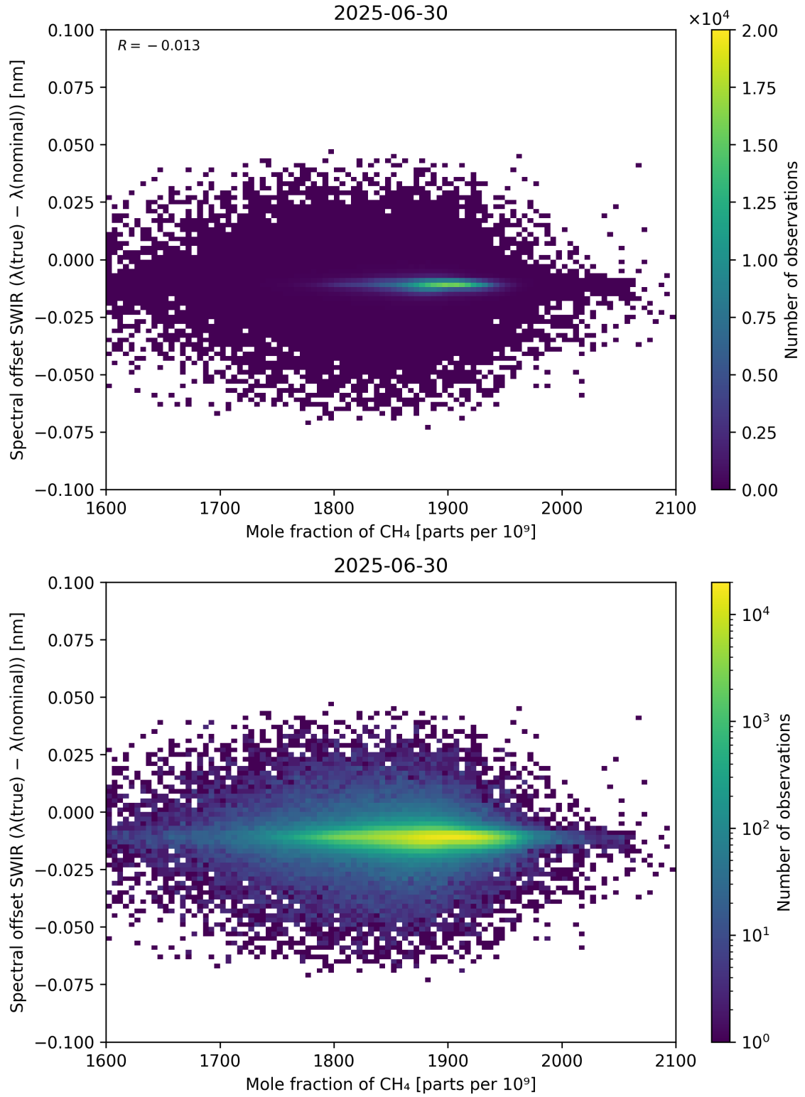
Figure 86: Scatter density plot of “Mole fraction of CH 4 ” against “Spectral offset SWIR ( \lambda_{\text{true}} - \lambda_{\text{nominal}} )” for 2025-06-29 to 2025-07-01.
