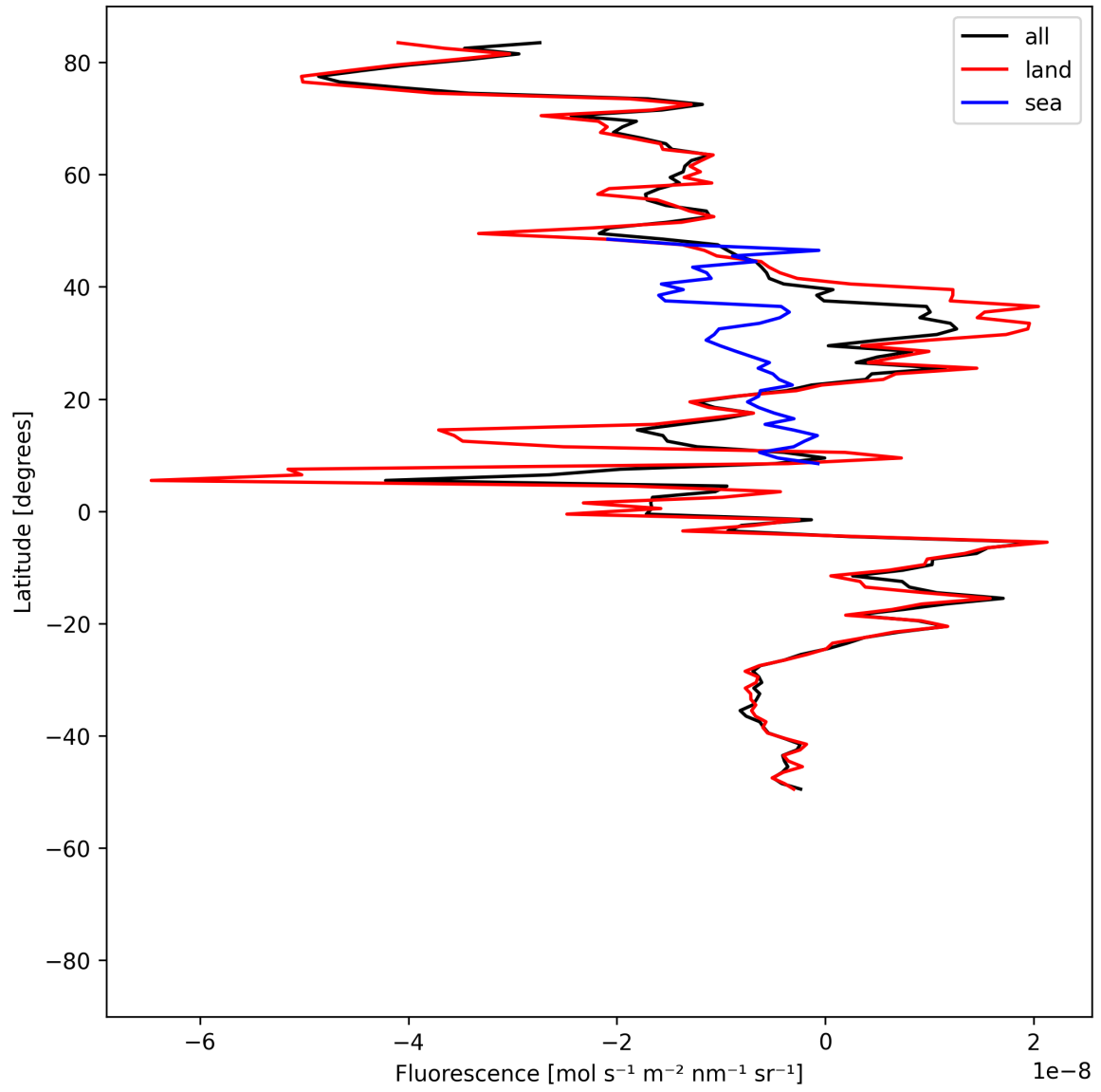
Figure 21: Zonal average of “Fluorescence” for 2025-06-29 to 2025-07-01.
