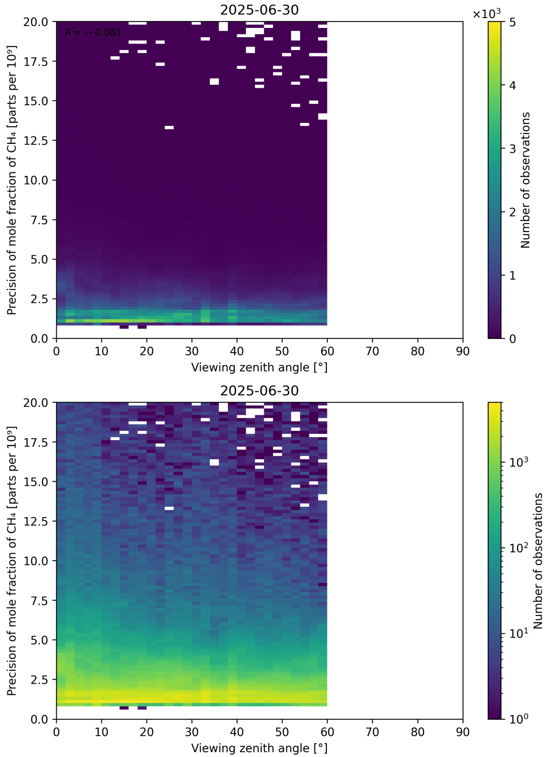
Figure 112: Scatter density plot of “Viewing zenith angle” against “Precision of mole fraction of CH 4 ” for 2025-06-29 to 2025-07-01.
