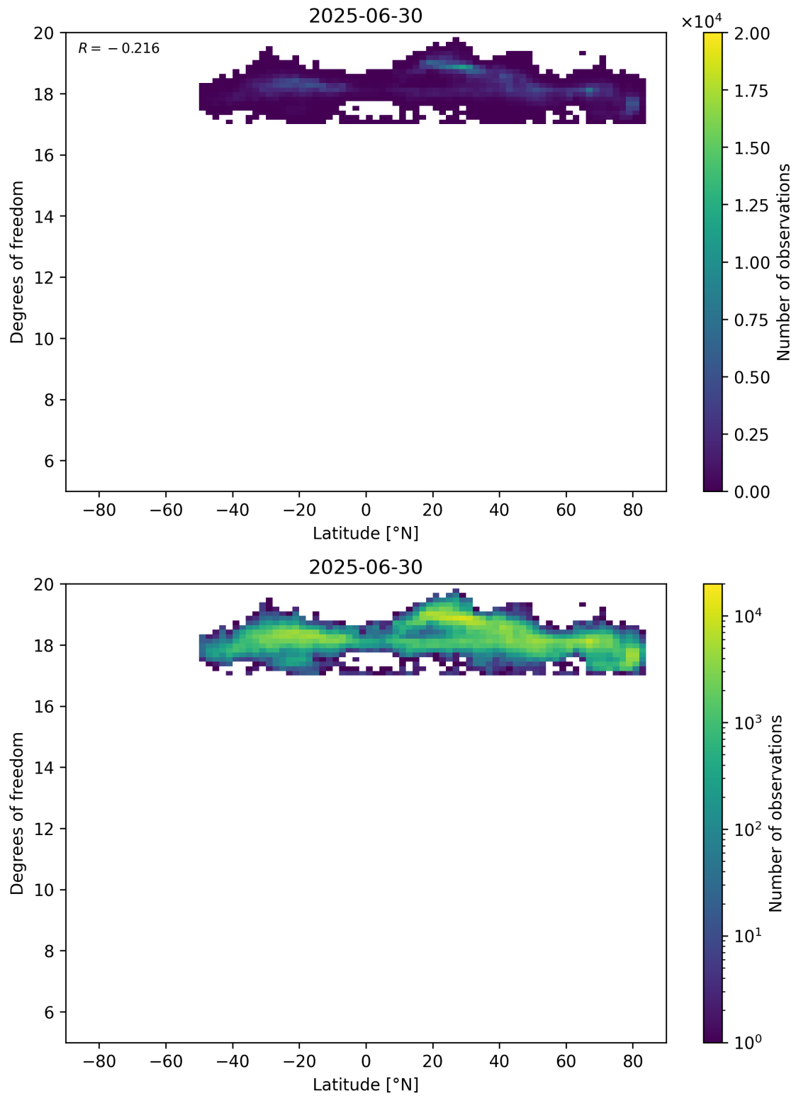
Figure 55: Scatter density plot of “Latitude” against “Degrees of freedom” for 2025-06-29 to 2025-07-01.
