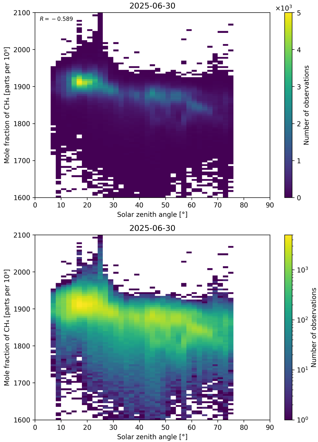
Figure 99: Scatter density plot of “Solar zenith angle” against “Mole fraction of CH 4 ” for 2025-06-29 to 2025-07-01.
