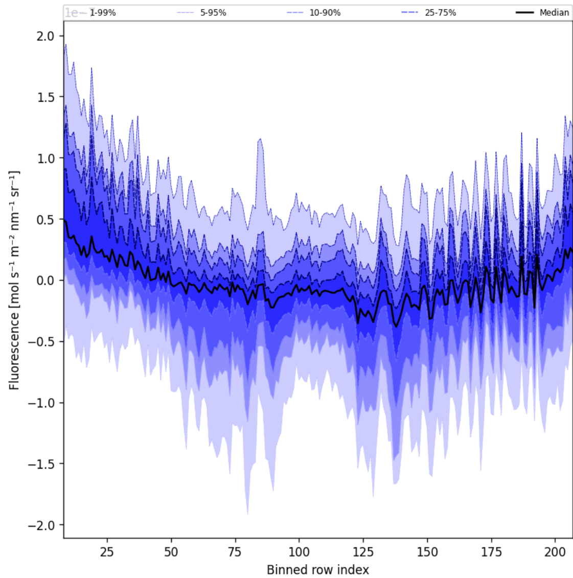
Figure 43: Along track statistics of “Fluorescence” for 2025-06-29 to 2025-07-01
