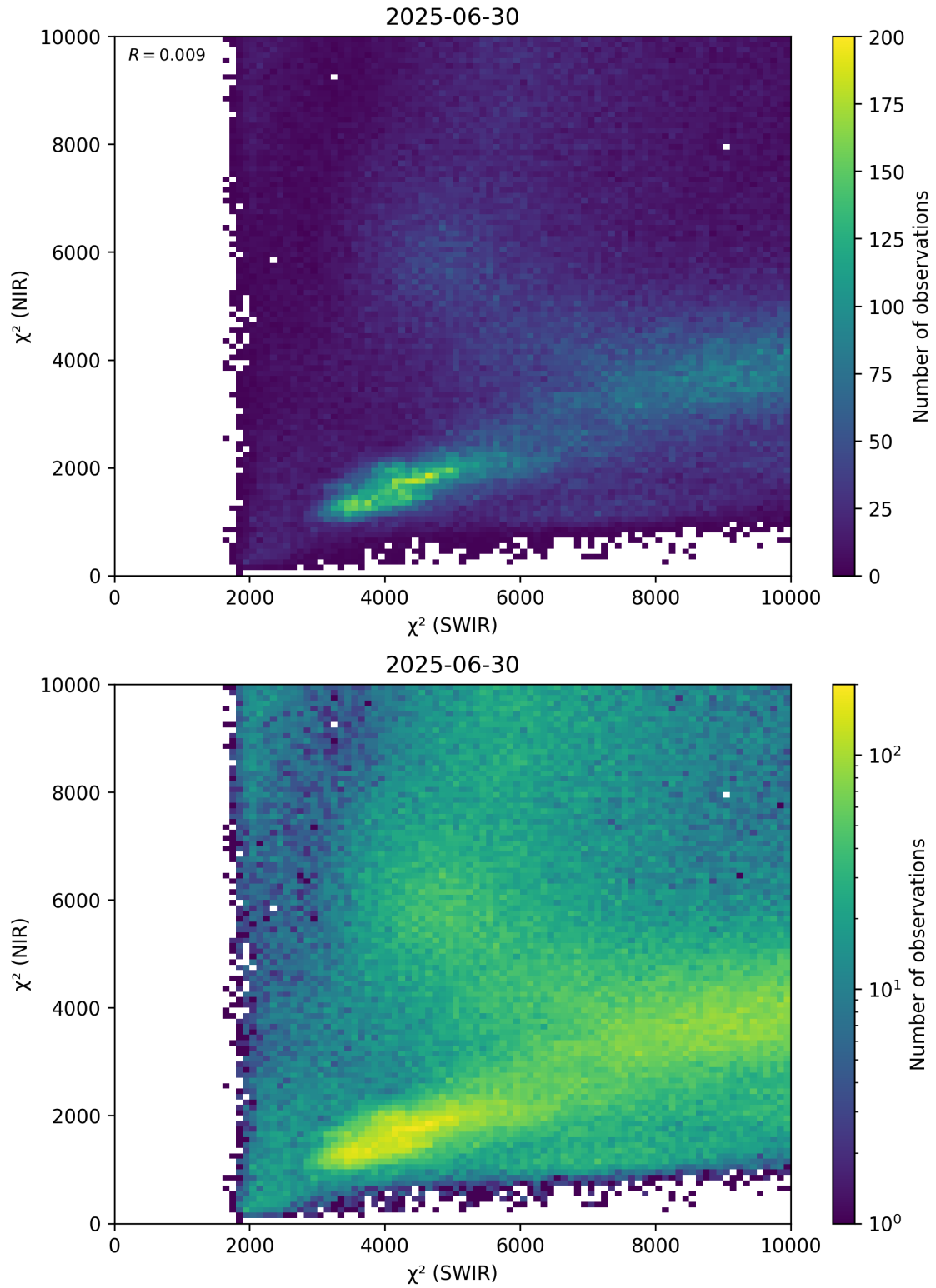
Figure 47: Scatter density plot of “ \chi^2 (SWIR)” against “ \chi^2 (NIR)” for 2025-06-29 to 2025-07-01.
