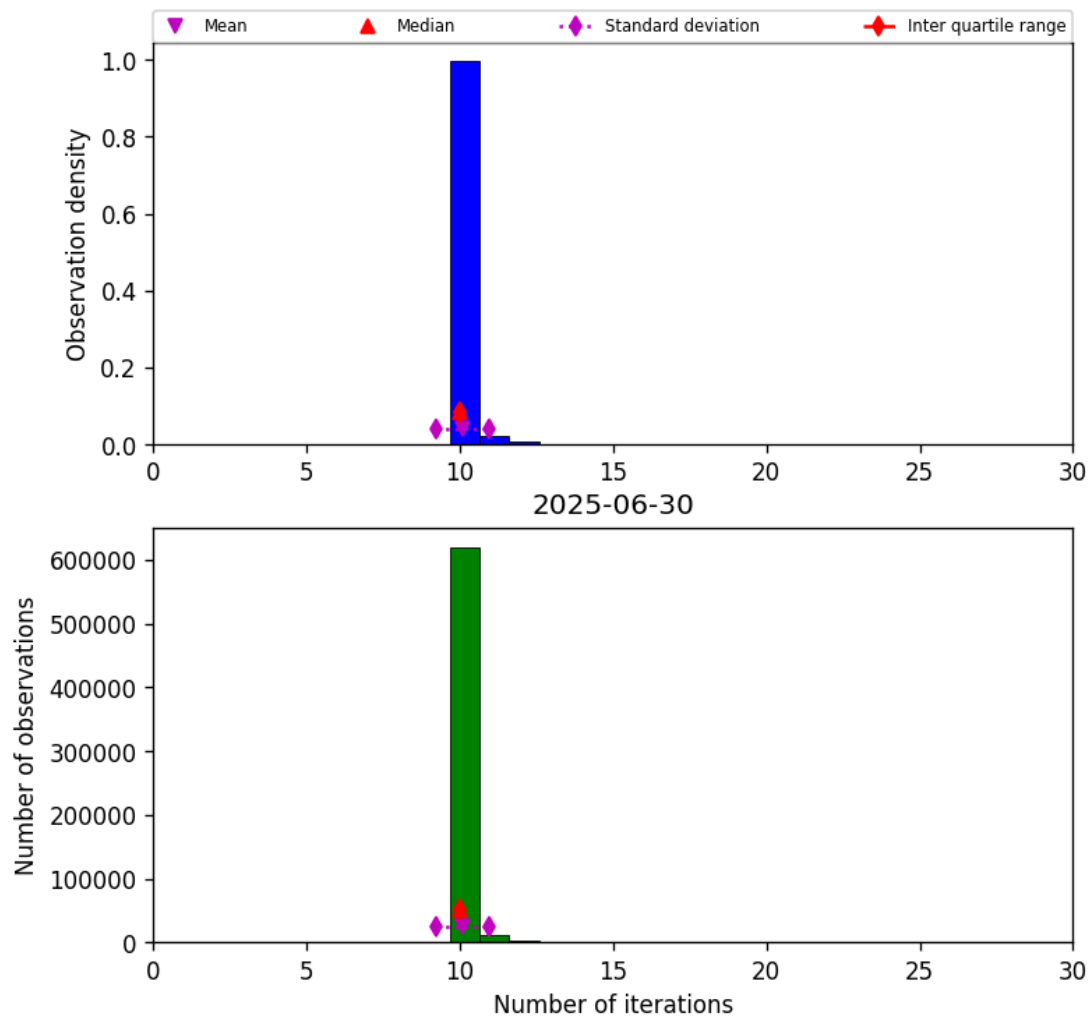
Figure 31: Histogram of “Number of iterations” for 2025-06-29 to 2025-07-01
