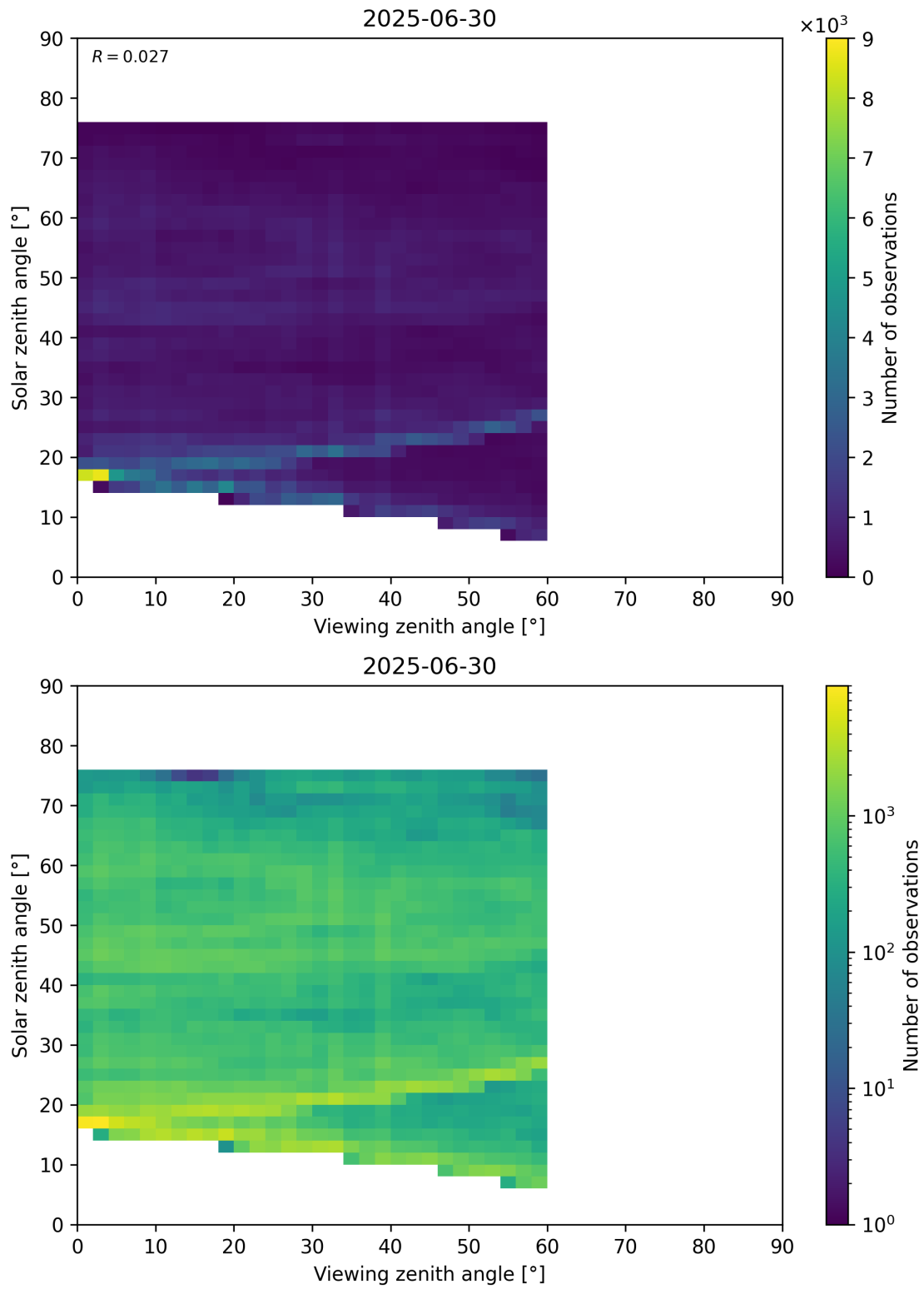
Figure 115: Scatter density plot of “Viewing zenith angle” against “Solar zenith angle” for 2025-06-29 to 2025-07-01.
