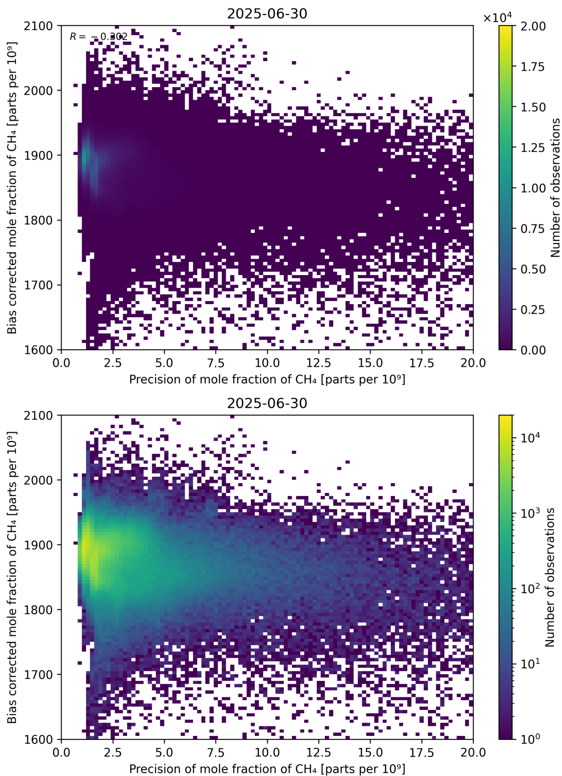
Figure 82: Scatter density plot of “Precision of mole fraction of CH 4 ” against “Bias corrected mole fraction of CH 4 ” for 2025-06-29 to 2025-07-01.
