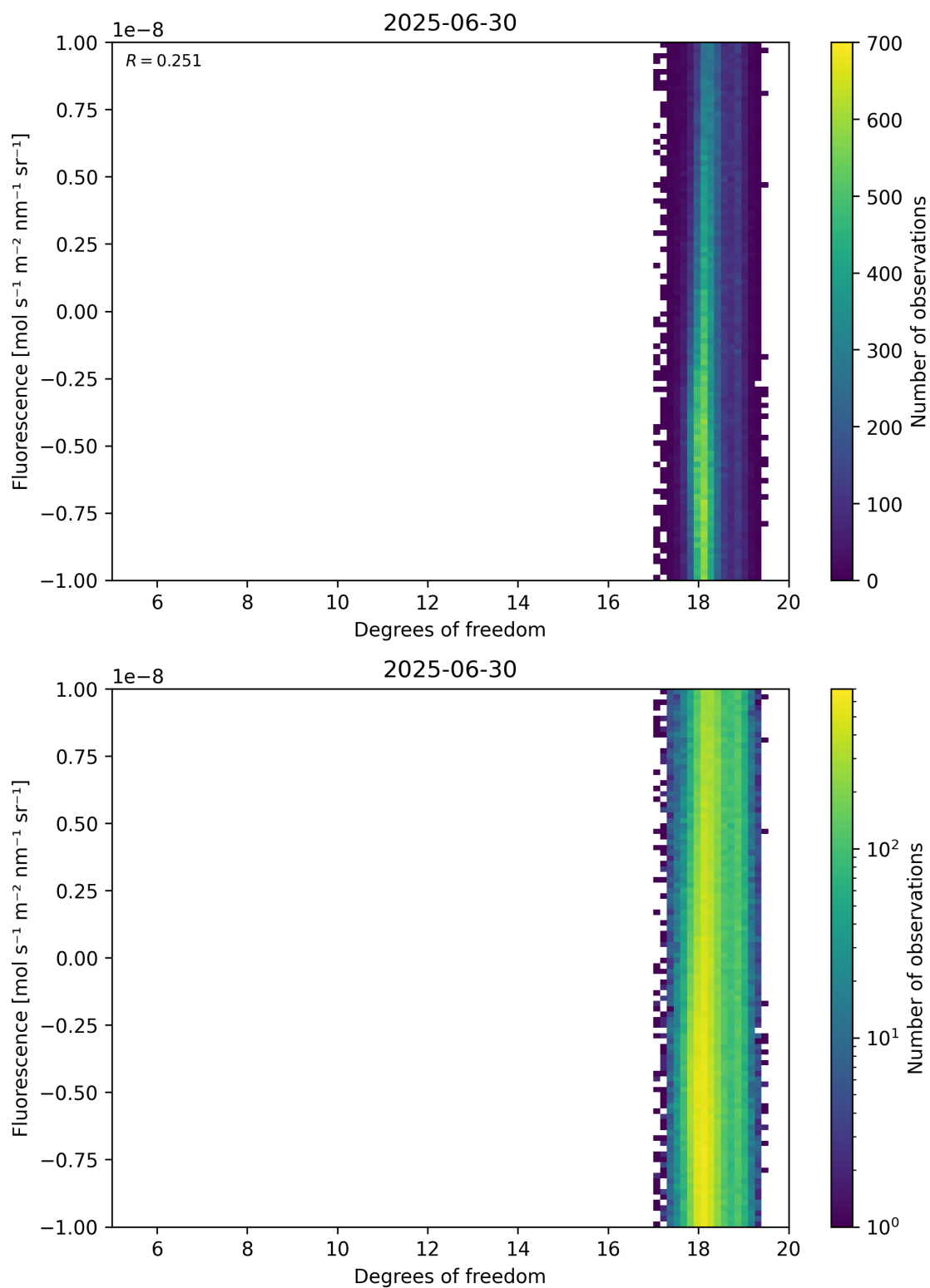
Figure 51: Scatter density plot of “Degrees of freedom” against “Fluorescence” for 2025-06-29 to 2025-07-01.
