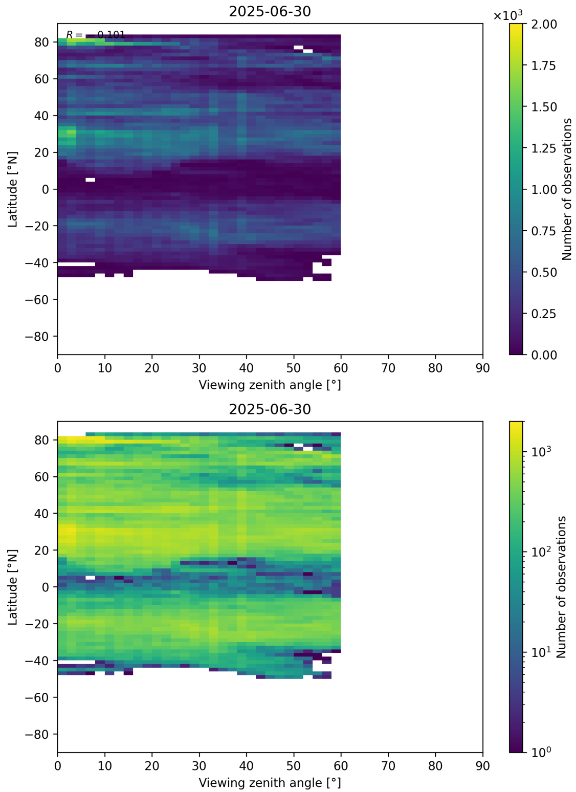
Figure 109: Scatter density plot of “Viewing zenith angle” against “Latitude” for 2025-06-29 to 2025-07-01.
