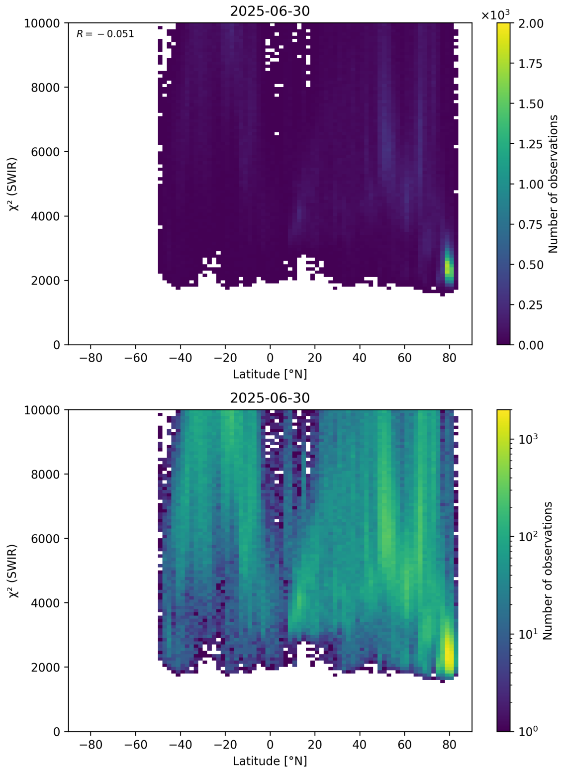
Figure 54: Scatter density plot of “Latitude” against “ \chi^2 (SWIR)” for 2025-06-29 to 2025-07-01.
