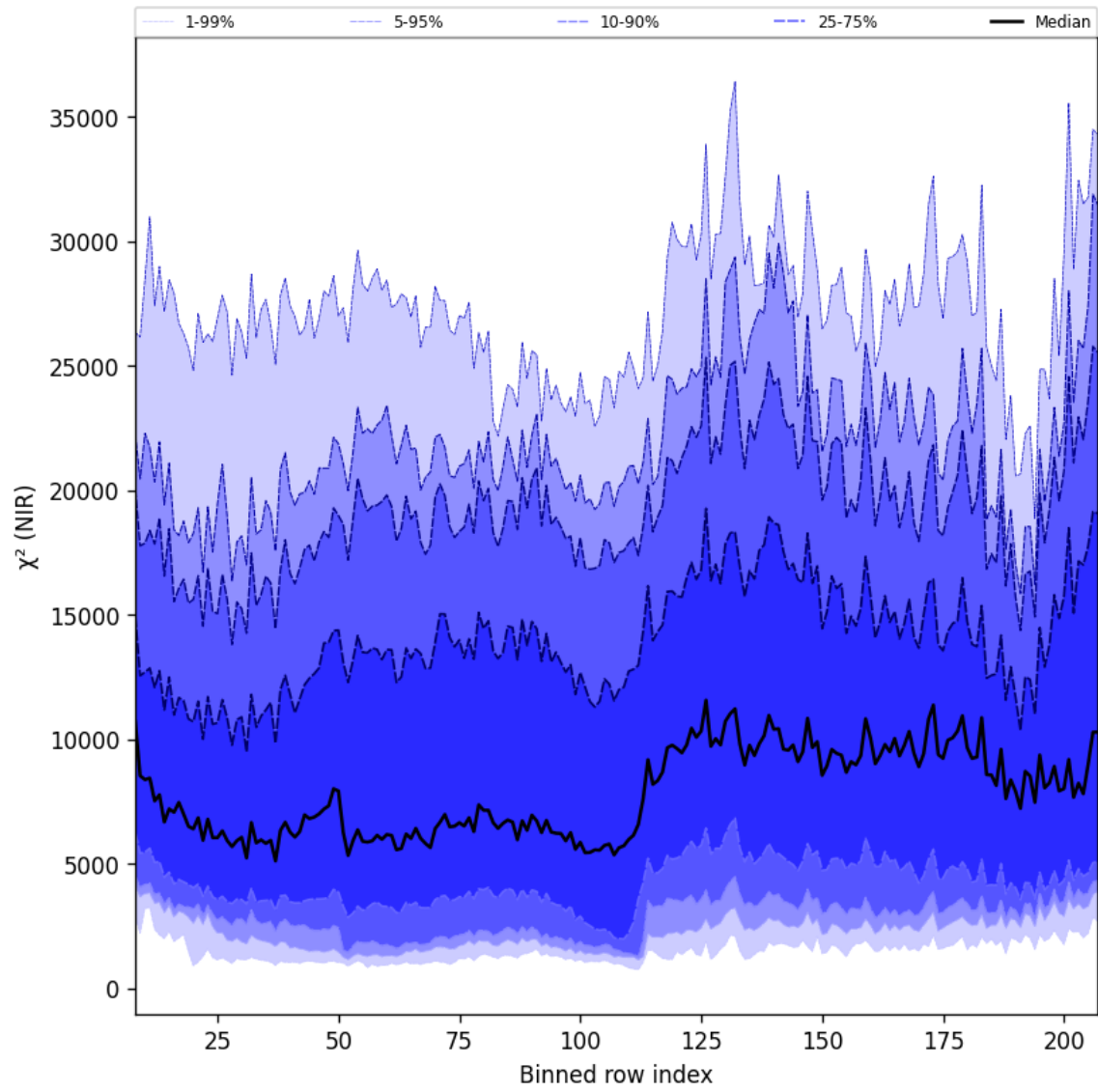
Figure 40: Along track statistics of “ \chi^2 (NIR)” for 2025-06-29 to 2025-07-01
