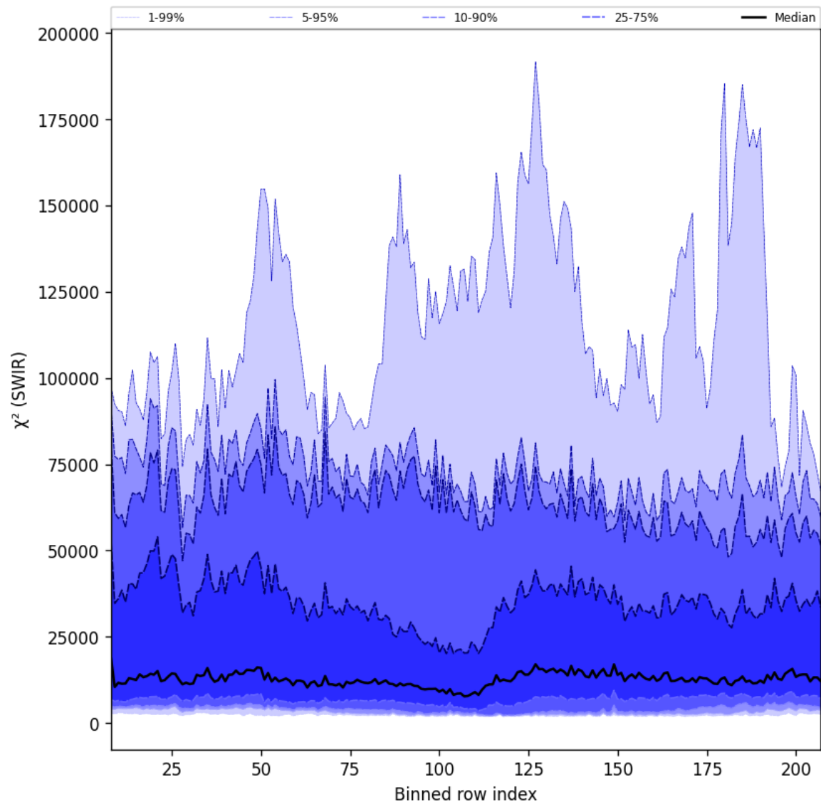
Figure 39: Along track statistics of “ \chi^2 (SWIR)” for 2025-06-29 to 2025-07-01
