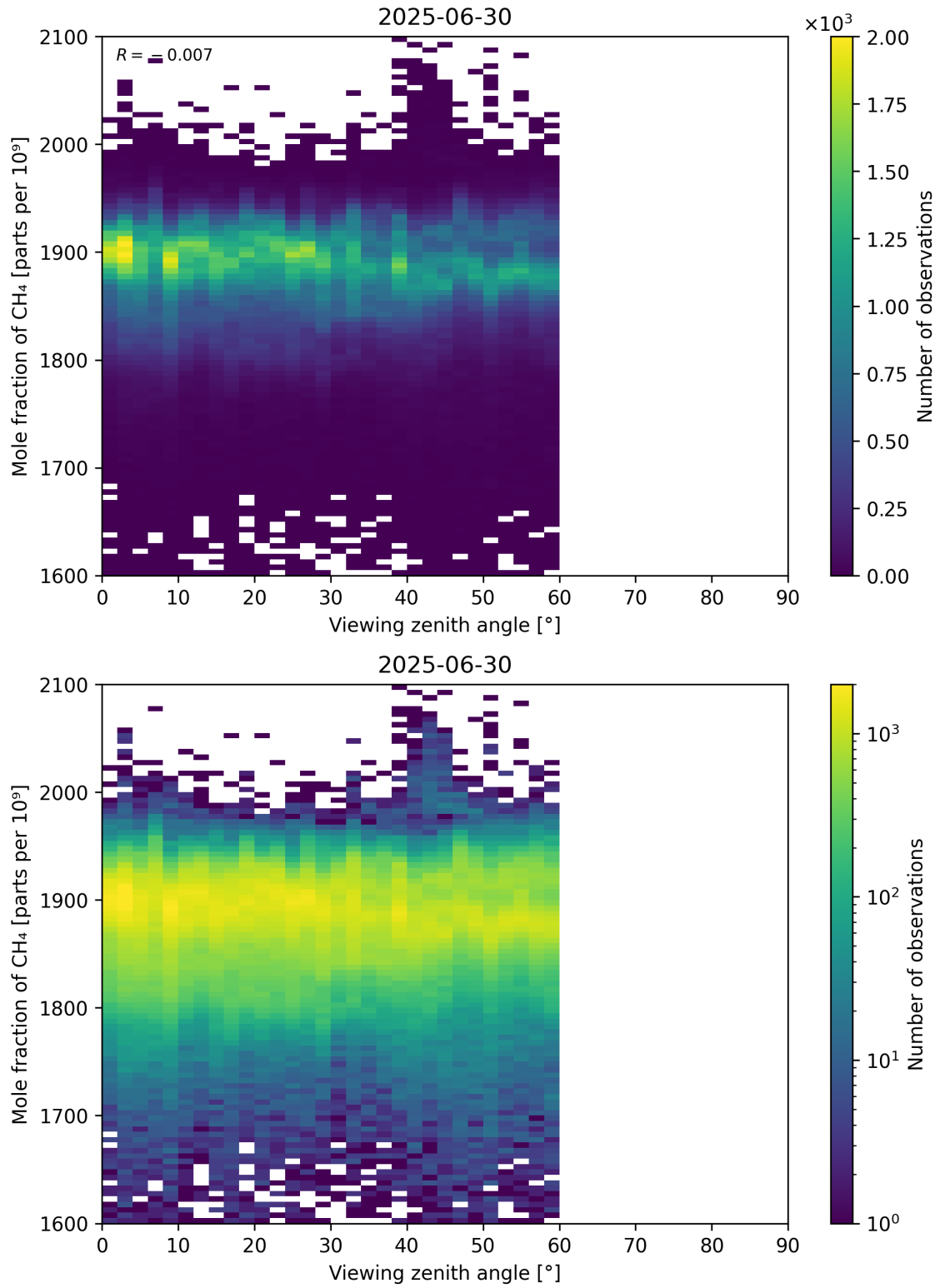
Figure 110: Scatter density plot of “Viewing zenith angle” against “Mole fraction of CH 4 ” for 2025-06-29 to 2025-07-01.
