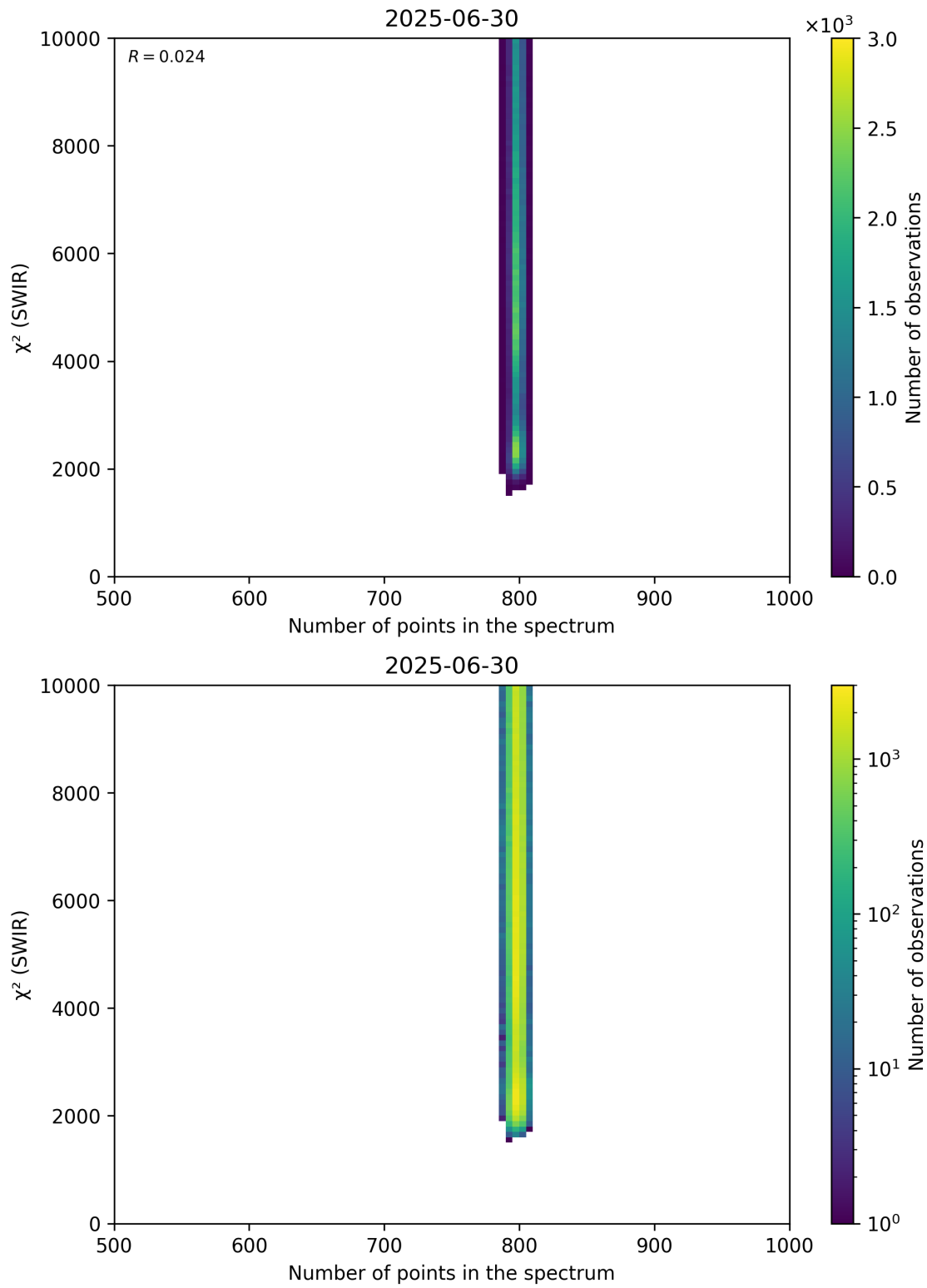
Figure 89: Scatter density plot of “Number of points in the spectrum” against “ \chi^2 (SWIR)” for 2025-06-29 to 2025-07-01.
