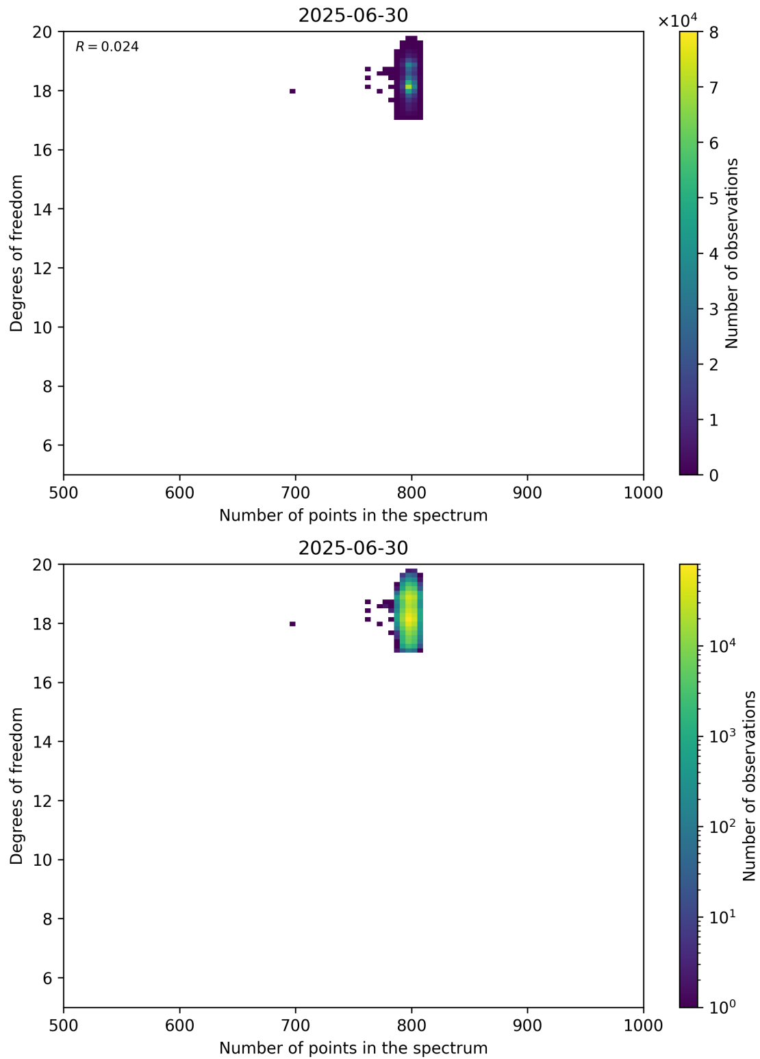
Figure 90: Scatter density plot of “Number of points in the spectrum” against “Degrees of freedom” for 2025-06-29 to 2025-07-01.
