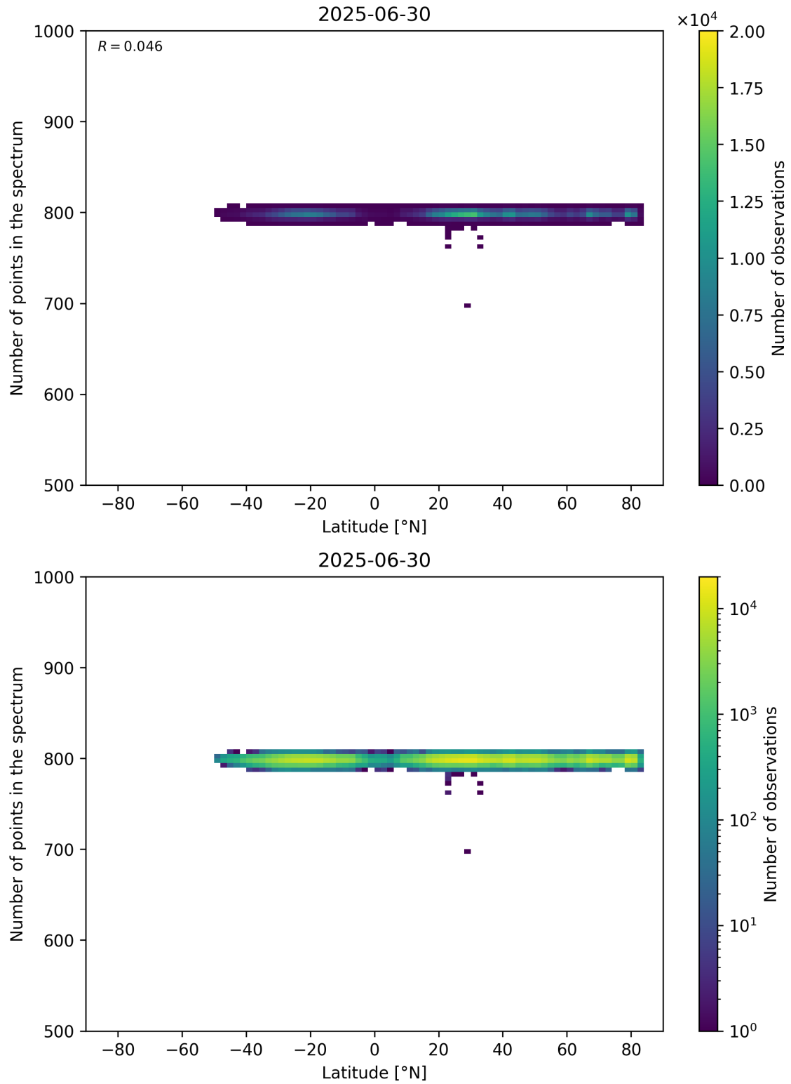
Figure 61: Scatter density plot of “Latitude” against “Number of points in the spectrum” for 2025-06-29 to 2025-07-01.
