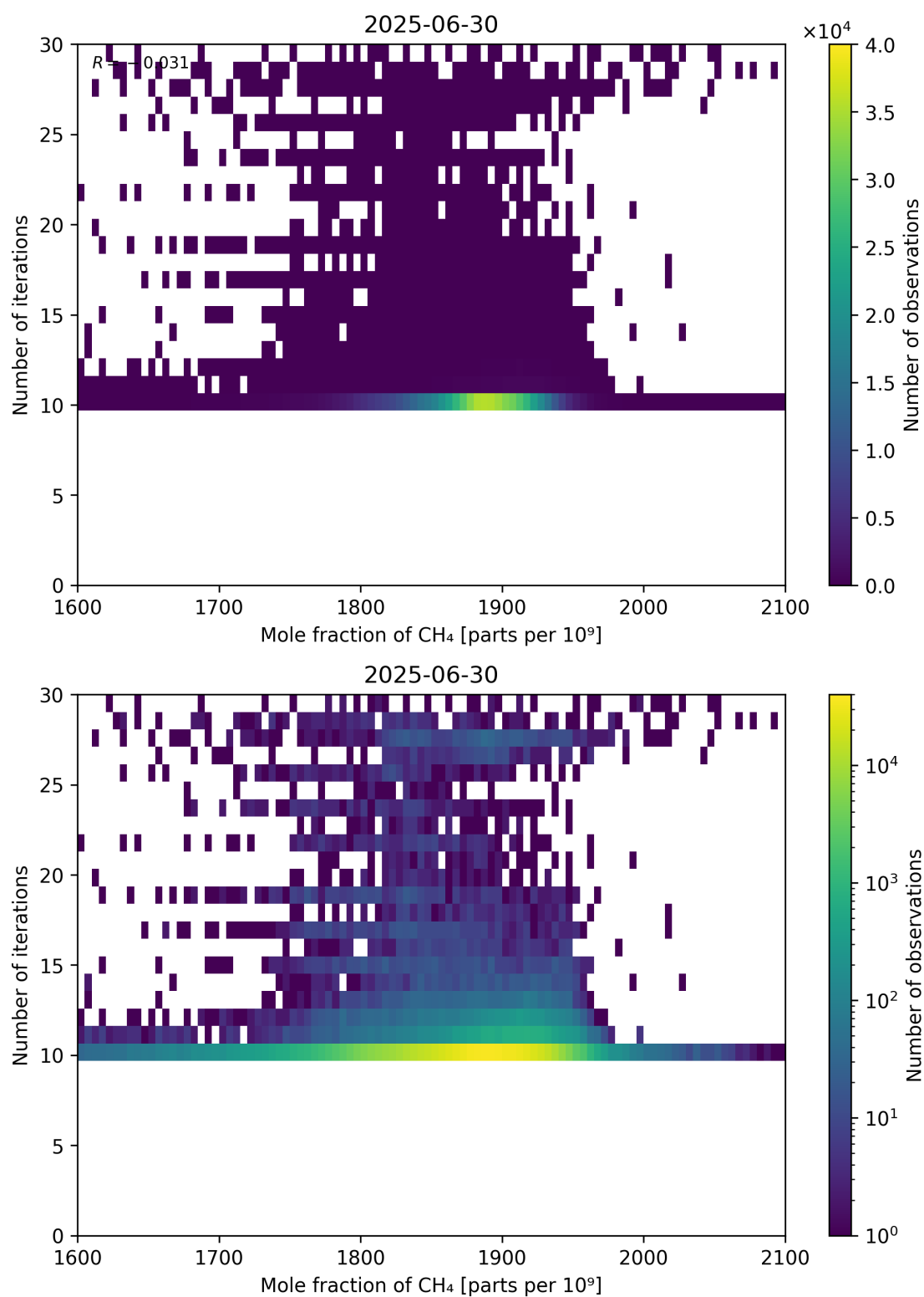
Figure 76: Scatter density plot of “Mole fraction of CH 4 ” against “Number of iterations” for 2025-06-29 to 2025-07-01.
