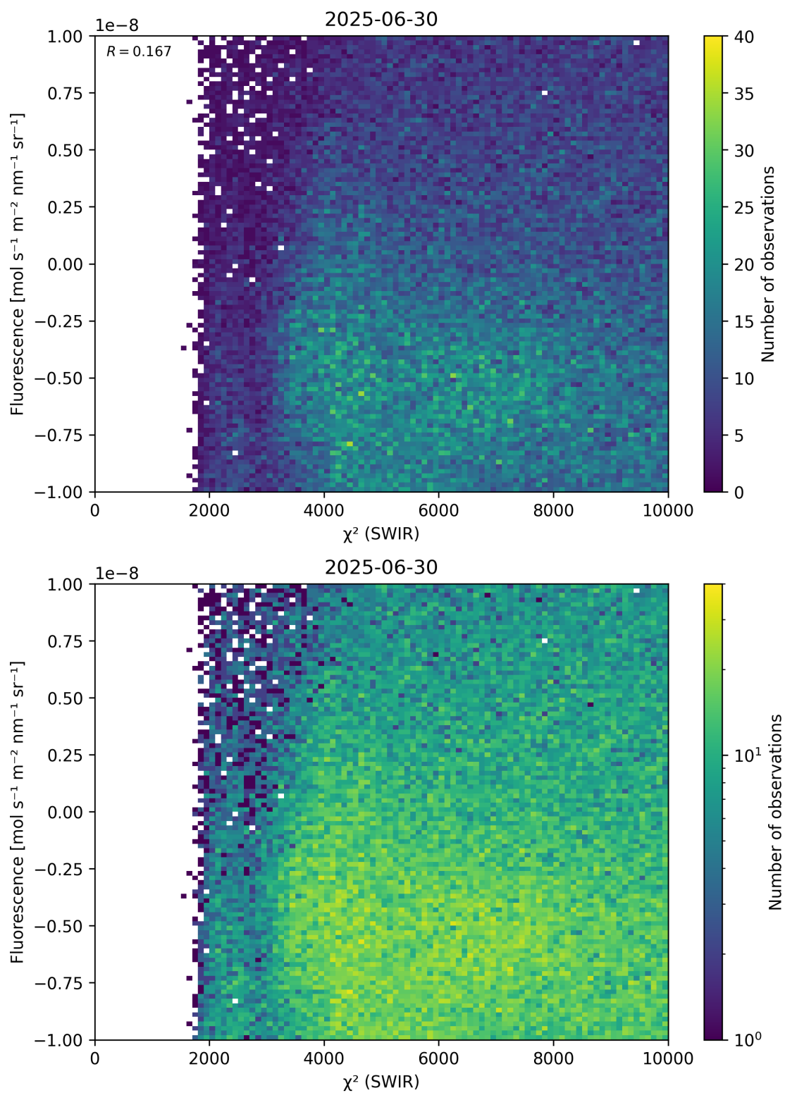
Figure 49: Scatter density plot of “ \chi^2 (SWIR)” against “Fluorescence” for 2025-06-29 to 2025-07-01.
