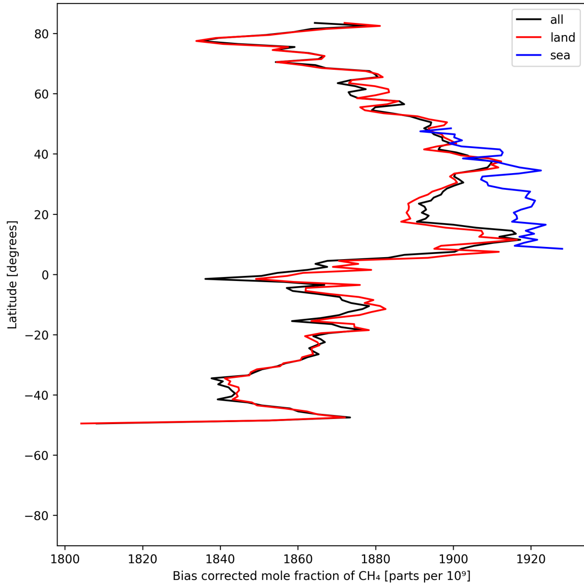
Figure 14: Zonal average of “Bias corrected mole fraction of \text{CH}_4 ” for 2025-06-29 to 2025-07-01.
