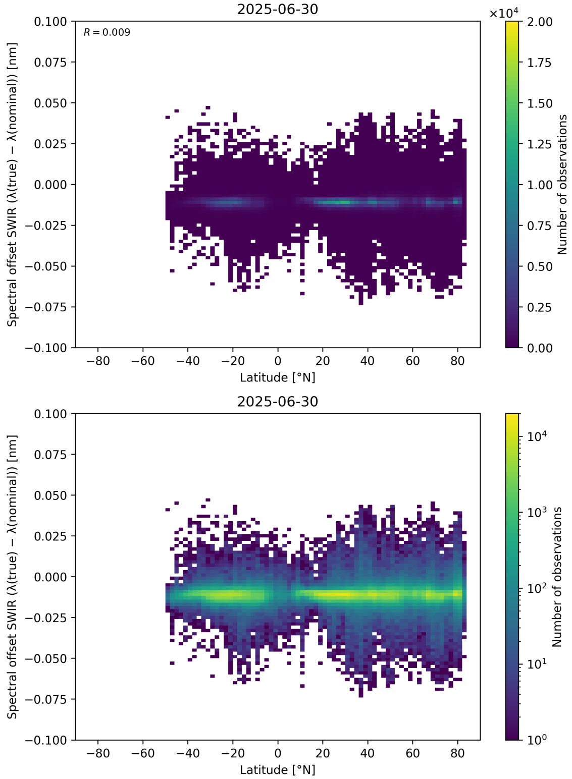
Figure 62: Scatter density plot of “Latitude” against “Spectral offset SWIR ( \lambda_{\text{true}} - \lambda_{\text{nominal}} )” for 2025-06-29 to 2025-07-01.
