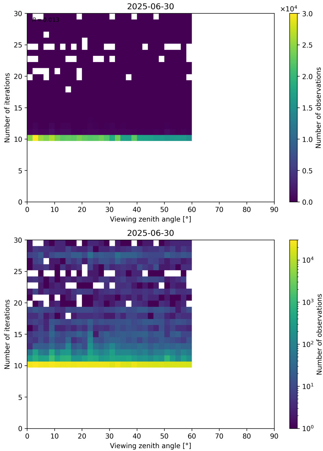
Figure 113: Scatter density plot of “Viewing zenith angle” against “Number of iterations” for 2025-06-29 to 2025-07-01.
