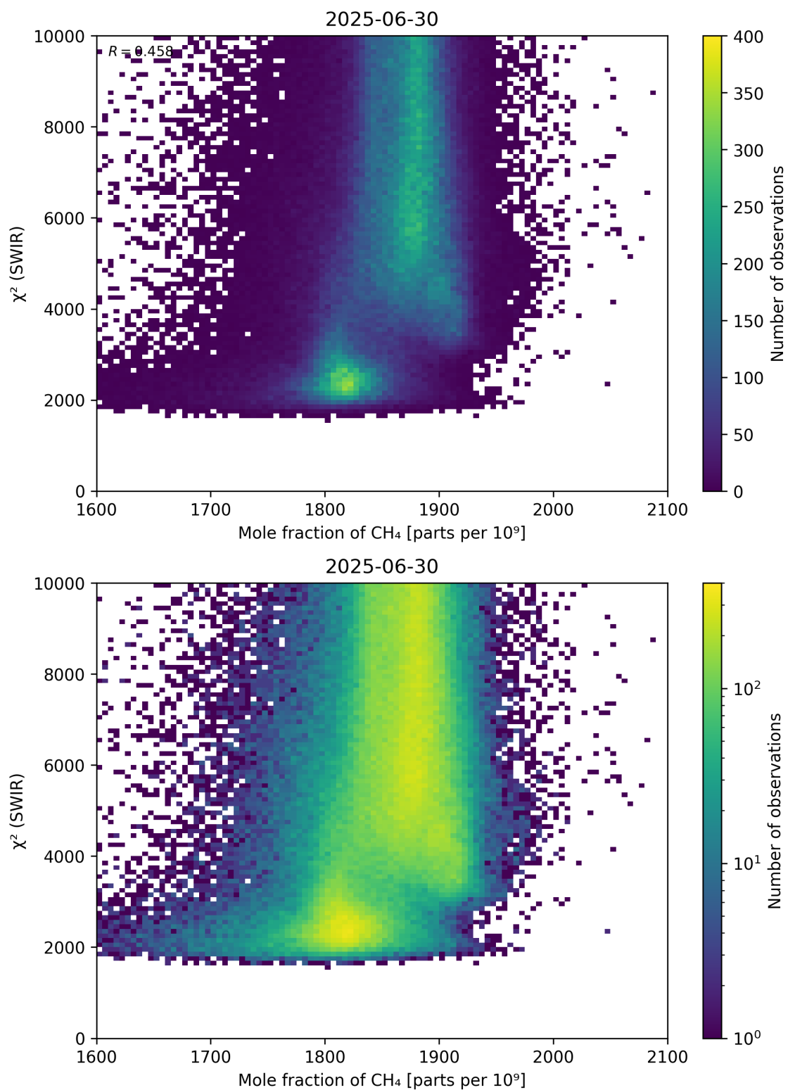
Figure 71: Scatter density plot of “Mole fraction of \text{CH}_4 ” against “ \chi^2 (SWIR)” for 2025-06-29 to 2025-07-01.
