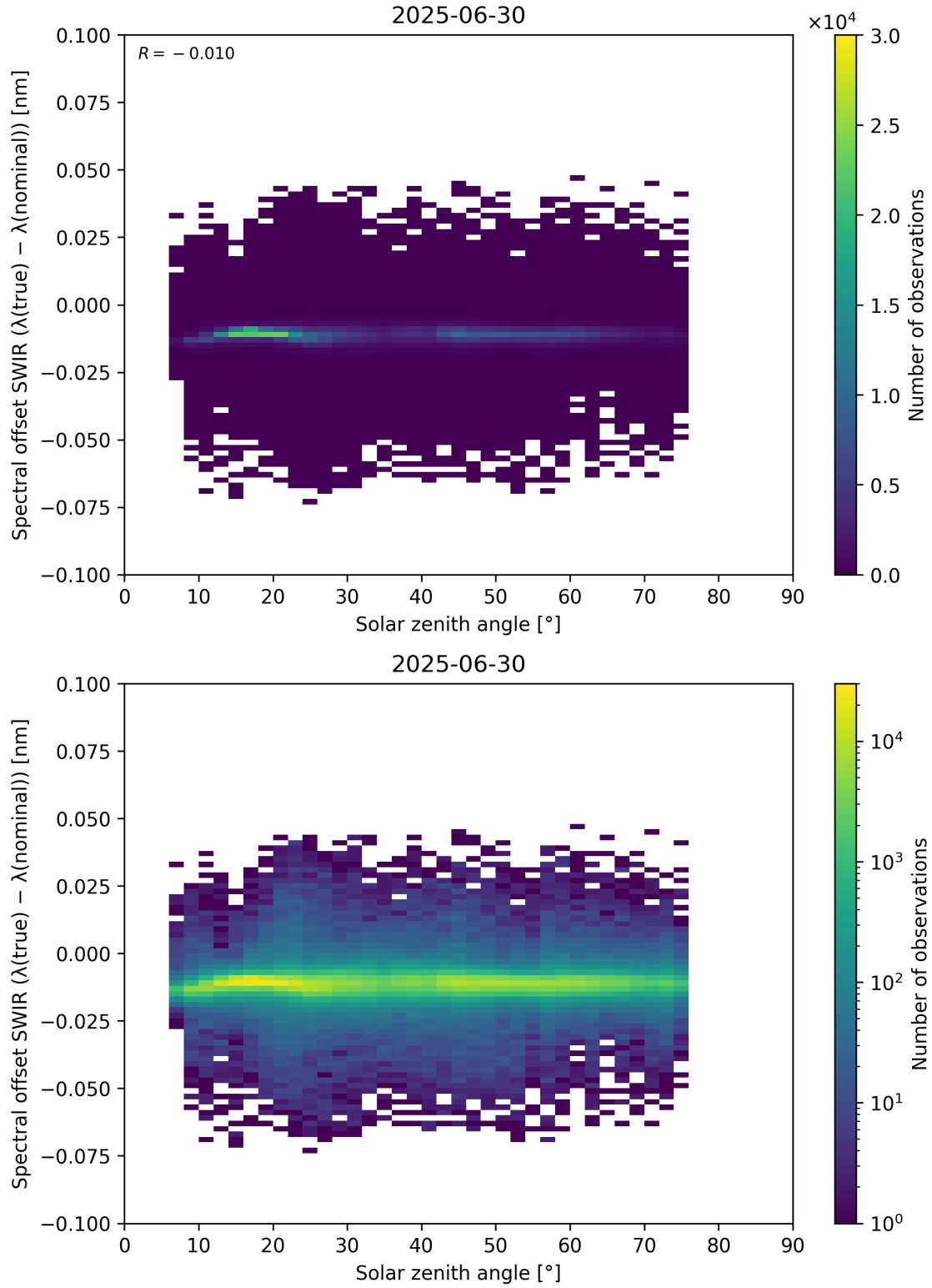
Figure 104: Scatter density plot of “Solar zenith angle” against “Spectral offset SWIR ( \lambda_{\text{true}} - \lambda_{\text{nominal}} )” for 2025-06-29 to 2025-07-01.
