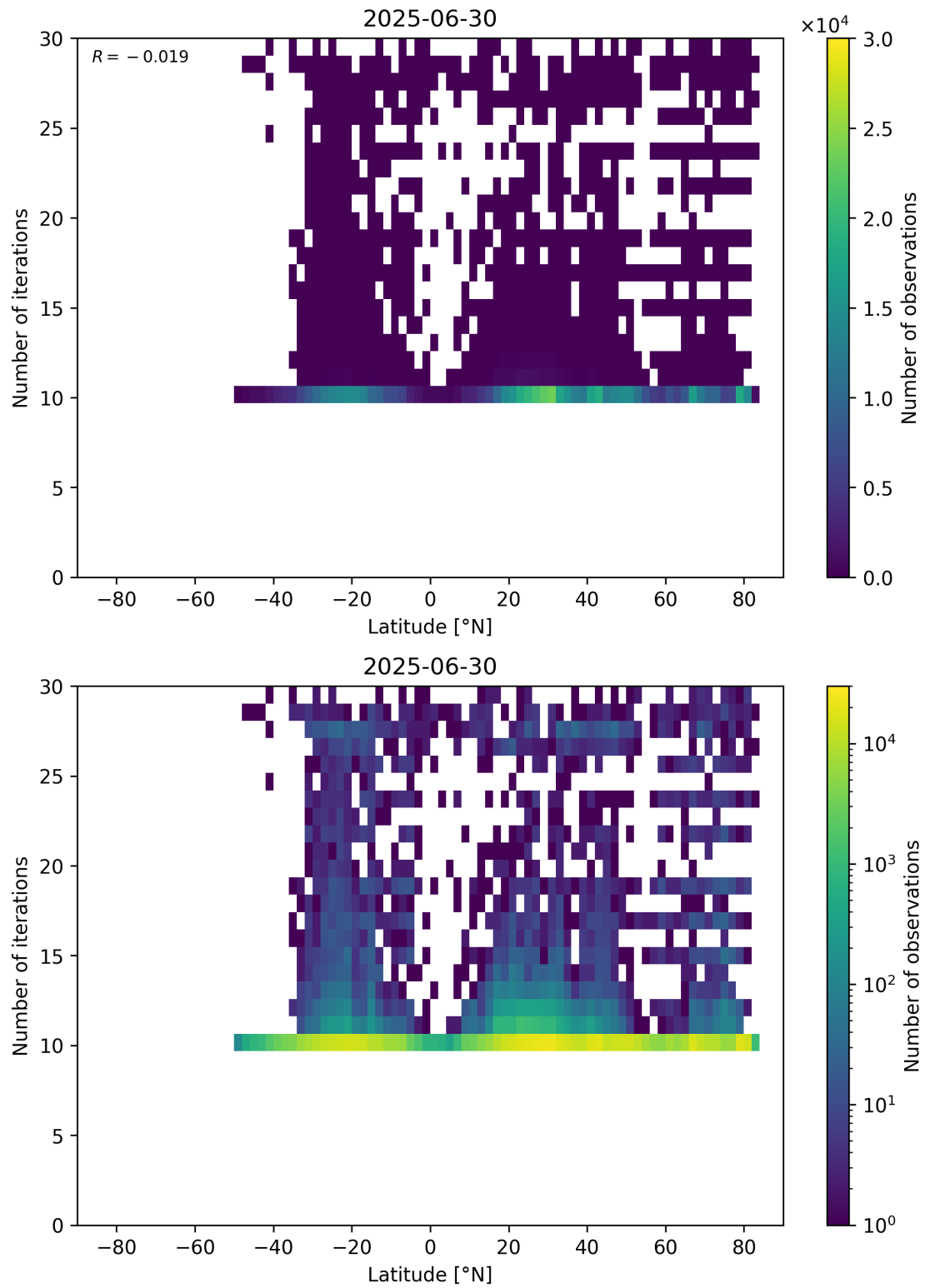
Figure 60: Scatter density plot of “Latitude” against “Number of iterations” for 2025-06-29 to 2025-07-01.
