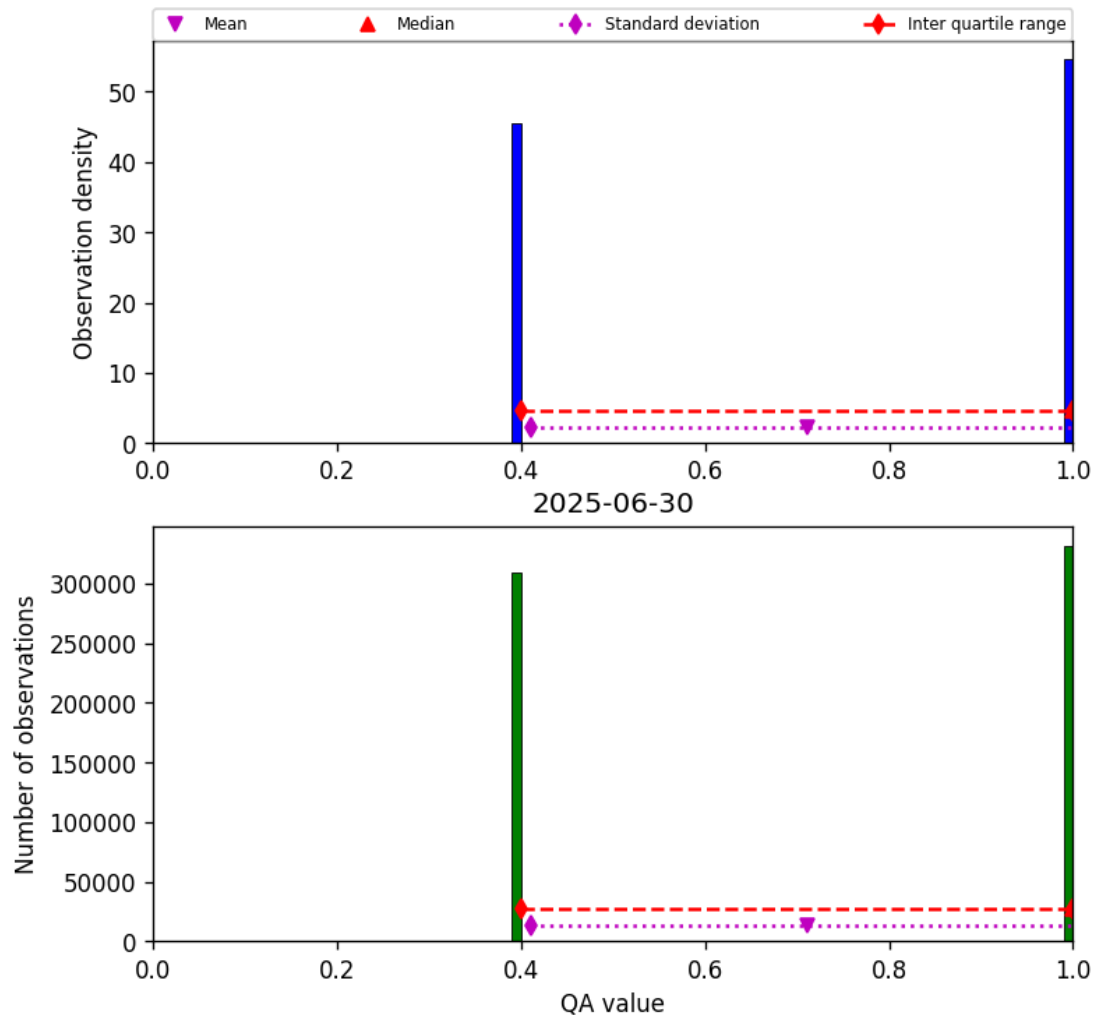
Figure 22: Histogram of “QA value” for 2025-06-29 to 2025-07-01
