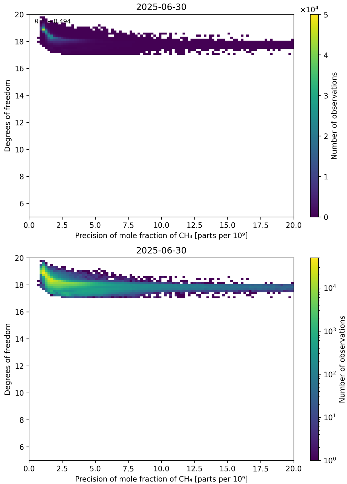
Figure 80: Scatter density plot of “Precision of mole fraction of CH 4 ” against “Degrees of freedom” for 2025-06-29 to 2025-07-01.
