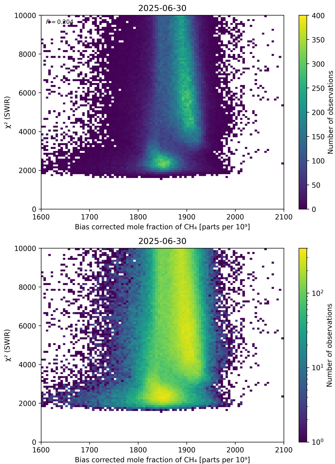
Figure 64: Scatter density plot of “Bias corrected mole fraction of \text{CH}_4 ” against “ \chi^2 (SWIR)” for 2025-06-29 to 2025-07-01.
