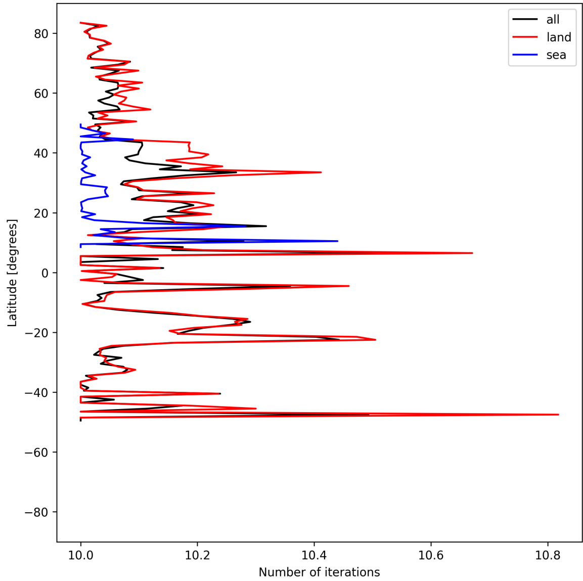
Figure 20: Zonal average of “Number of iterations” for 2025-06-30 to 2025-07-02.
