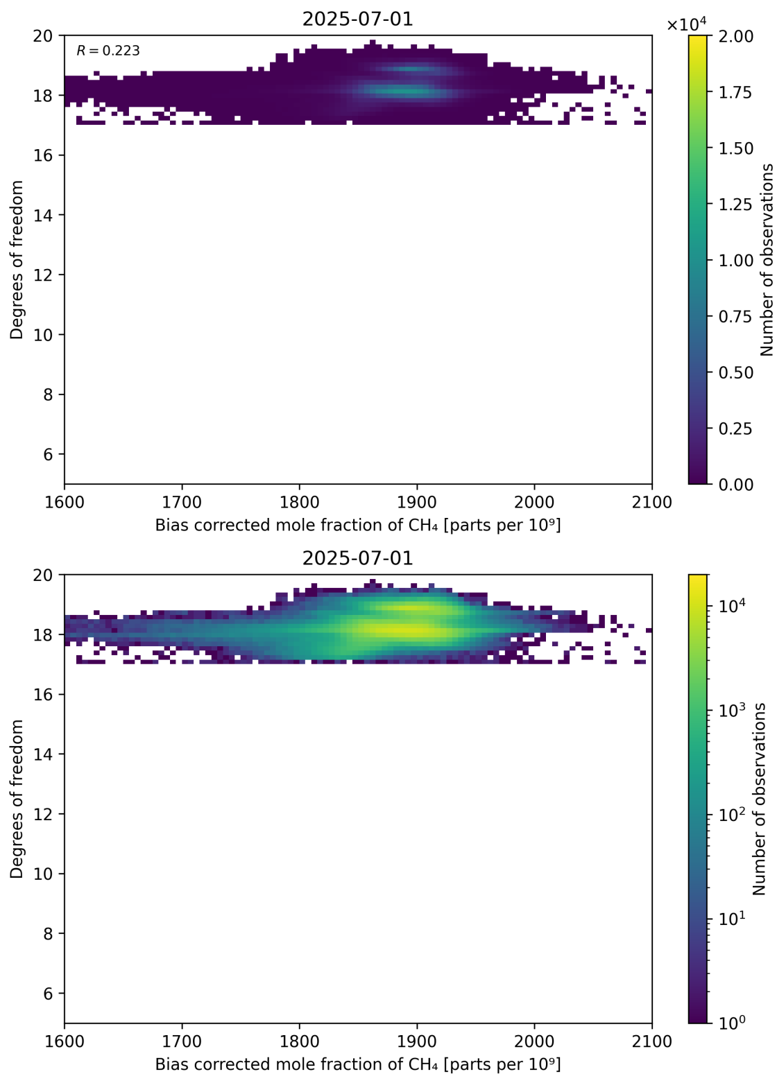
Figure 65: Scatter density plot of “Bias corrected mole fraction of CH 4 ” against “Degrees of freedom” for 2025-06-30 to 2025-07-02.
