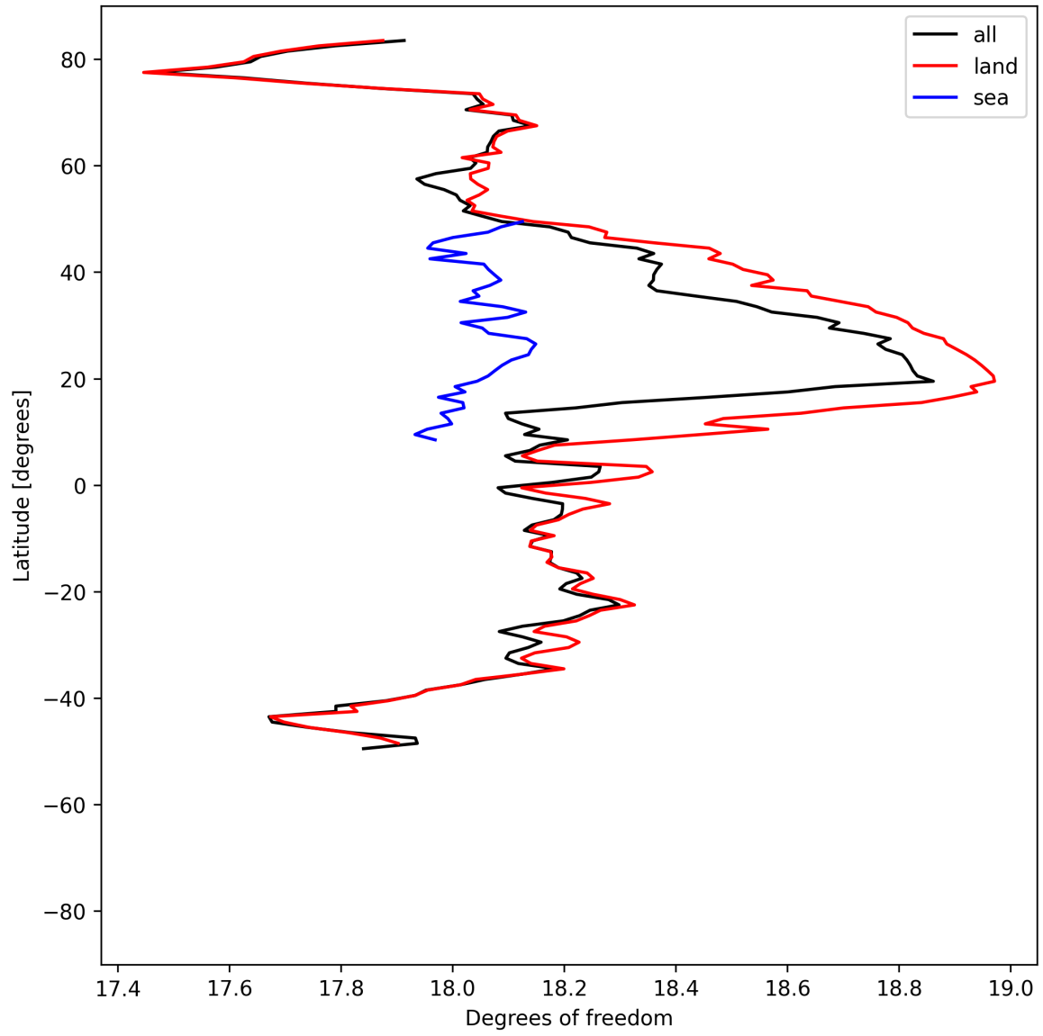
Figure 19: Zonal average of “Degrees of freedom” for 2025-06-30 to 2025-07-02.
