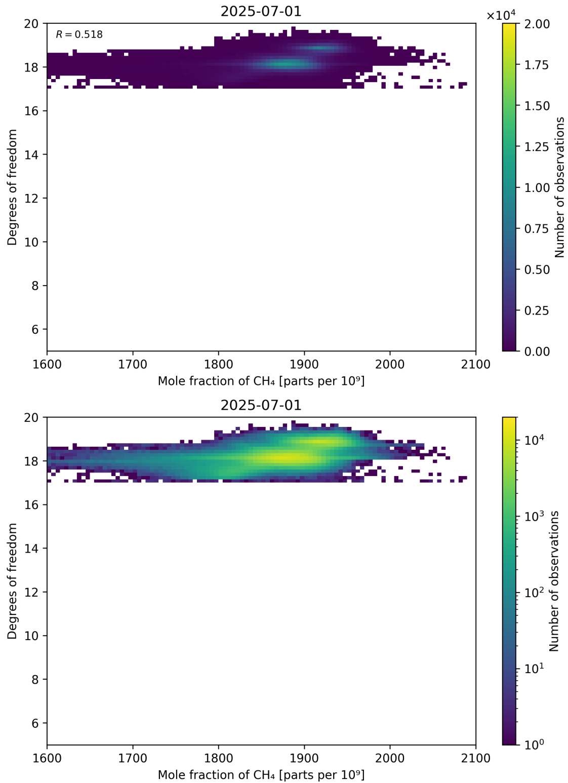
Figure 72: Scatter density plot of “Mole fraction of CH 4 ” against “Degrees of freedom” for 2025-06-30 to 2025-07-02.
