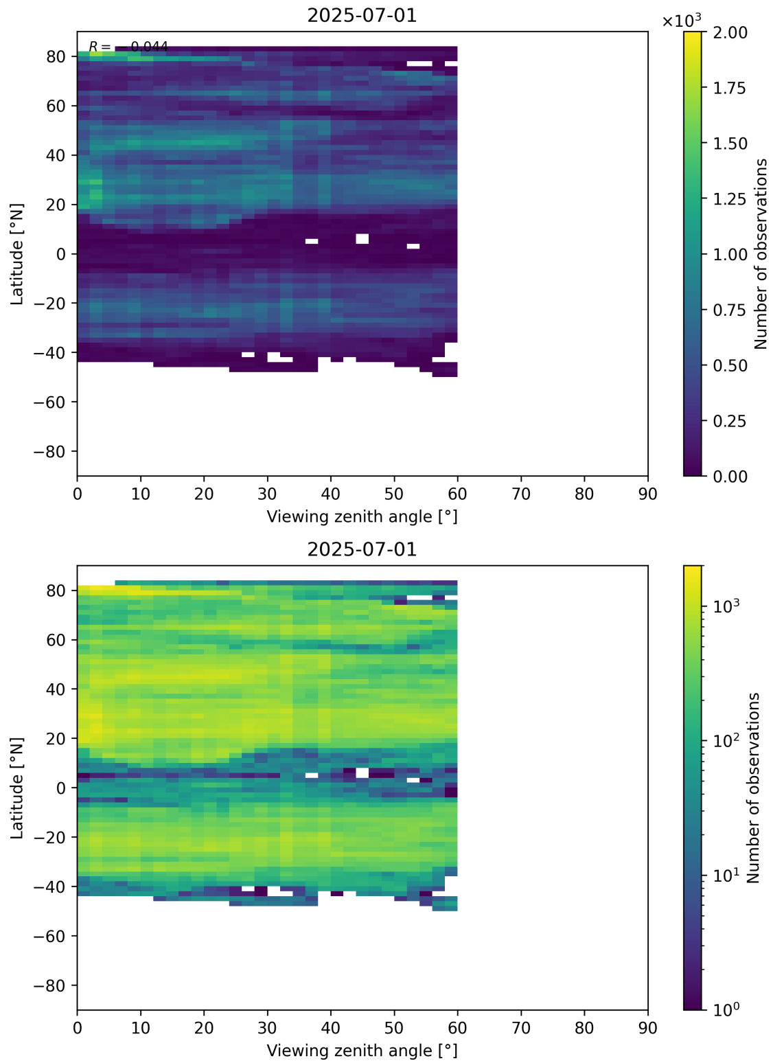
Figure 109: Scatter density plot of “Viewing zenith angle” against “Latitude” for 2025-06-30 to 2025-07-02.
