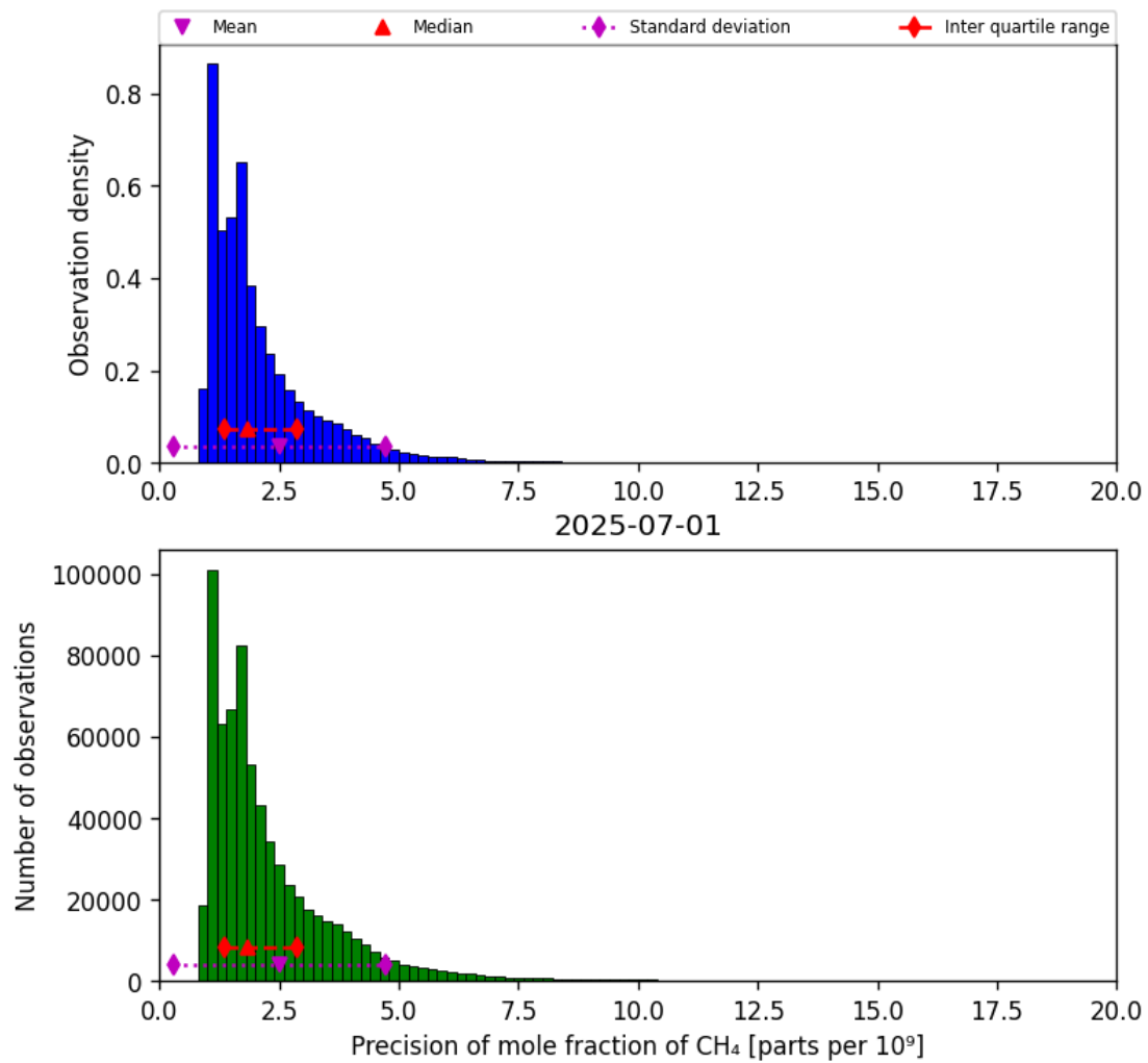
Figure 24: Histogram of “Precision of mole fraction of CH 4 ” for 2025-06-30 to 2025-07-02
