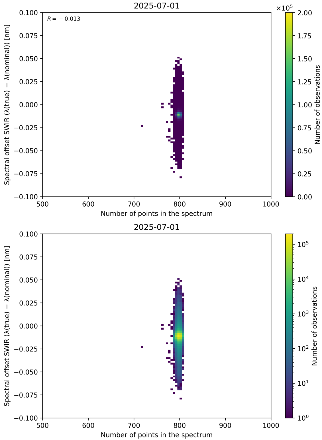
Figure 93: Scatter density plot of “Number of points in the spectrum” against “Spectral offset SWIR ( \lambda_{\text{true}} - \lambda_{\text{nominal}} )” for 2025-06-30 to 2025-07-02.
