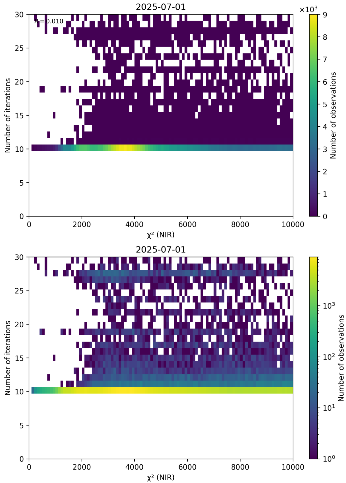
Figure 46: Scatter density plot of “ \chi^2 (NIR)” against “Number of iterations” for 2025-06-30 to 2025-07-02.
