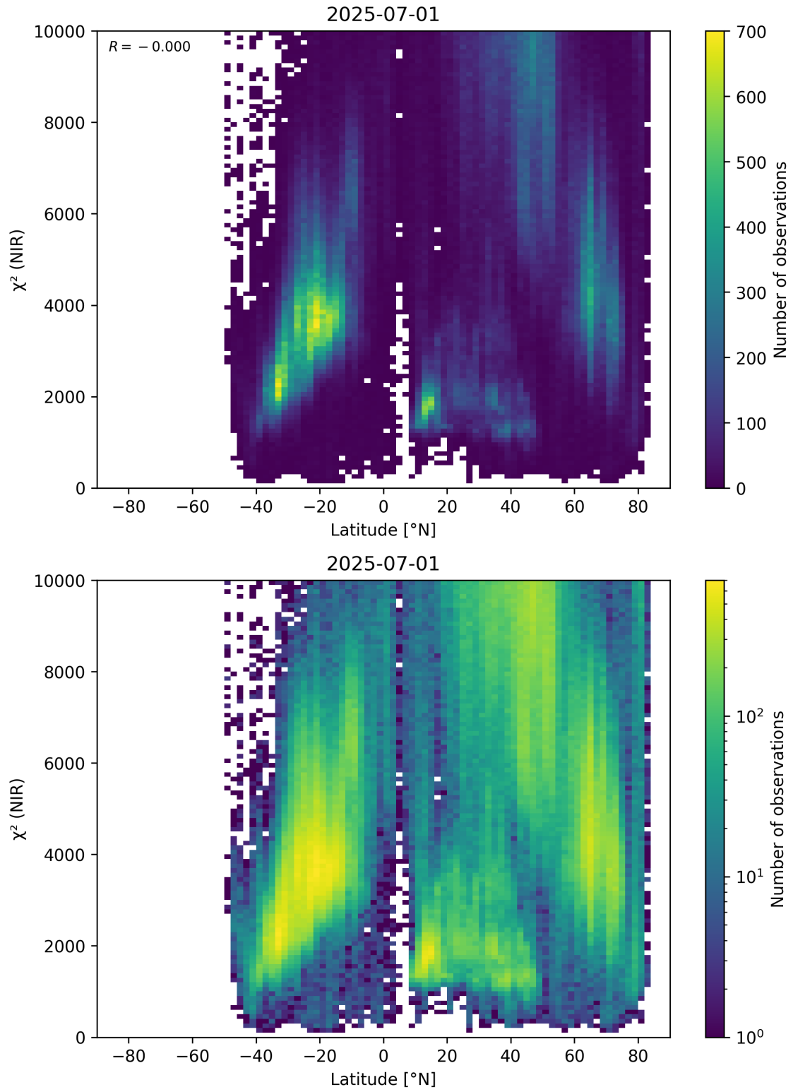
Figure 53: Scatter density plot of “Latitude” against “ \chi^2 (NIR)” for 2025-06-30 to 2025-07-02.
