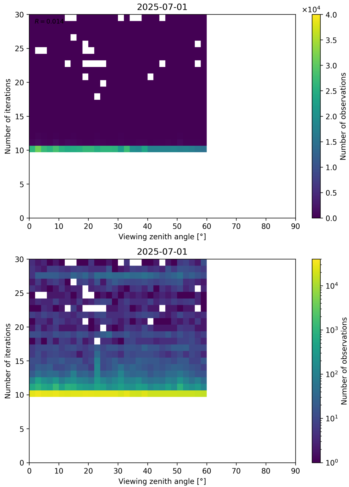
Figure 113: Scatter density plot of “Viewing zenith angle” against “Number of iterations” for 2025-06-30 to 2025-07-02.
