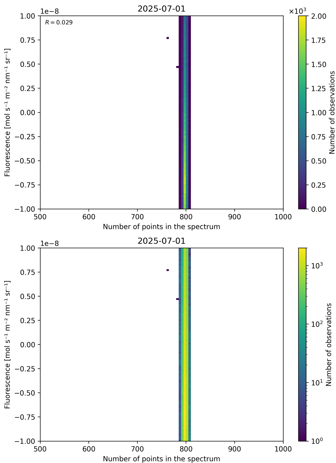
Figure 91: Scatter density plot of “Number of points in the spectrum” against “Fluorescence” for 2025-06-30 to 2025-07-02.
