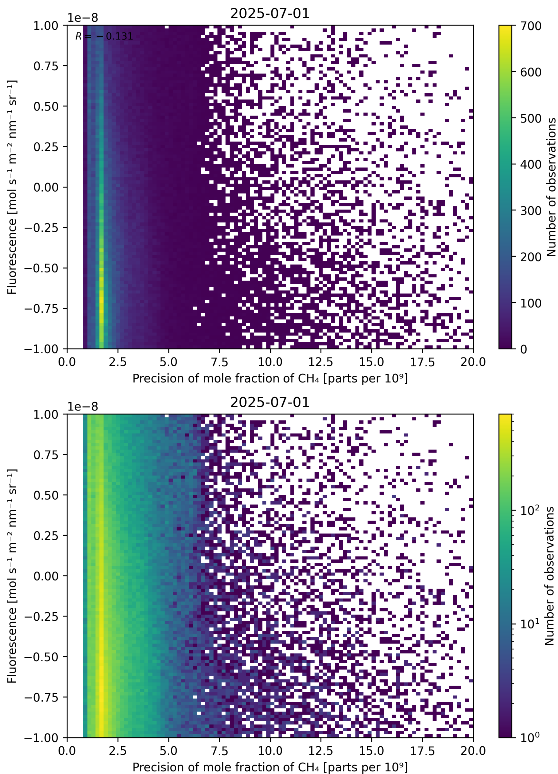
Figure 81: Scatter density plot of “Precision of mole fraction of \text{CH}_4 ” against “Fluorescence” for 2025-06-30 to 2025-07-02.
