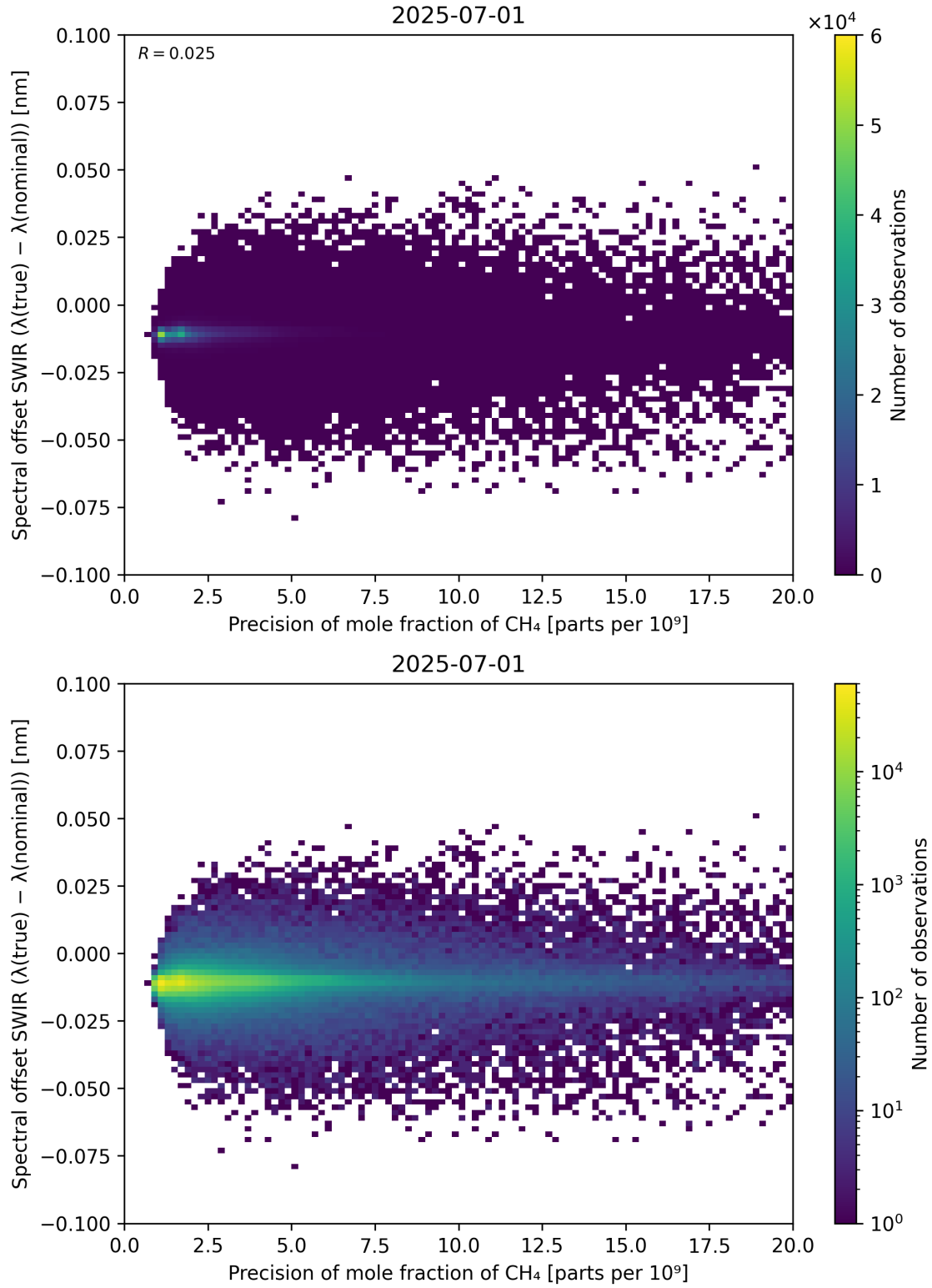
Figure 85: Scatter density plot of “Precision of mole fraction of \text{CH}_4 ” against “Spectral offset SWIR ( \lambda_{\text{true}} - \lambda_{\text{nominal}} )” for 2025-06-30 to 2025-07-02.
