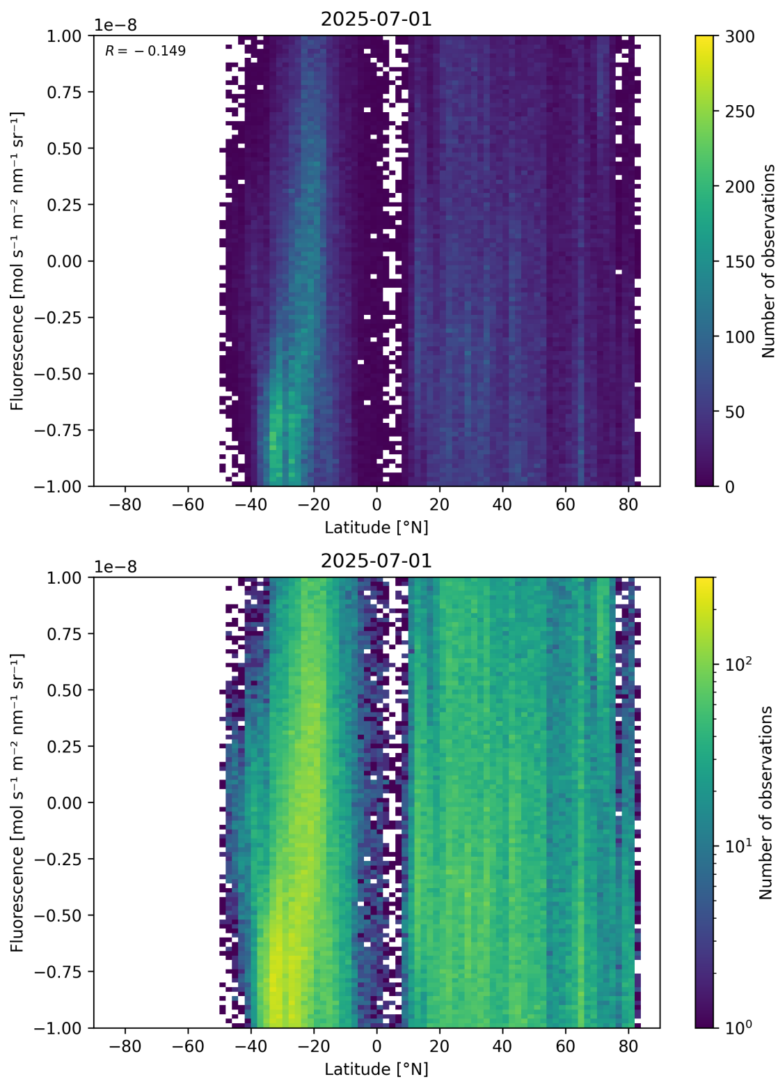
Figure 56: Scatter density plot of “Latitude” against “Fluorescence” for 2025-06-30 to 2025-07-02.
