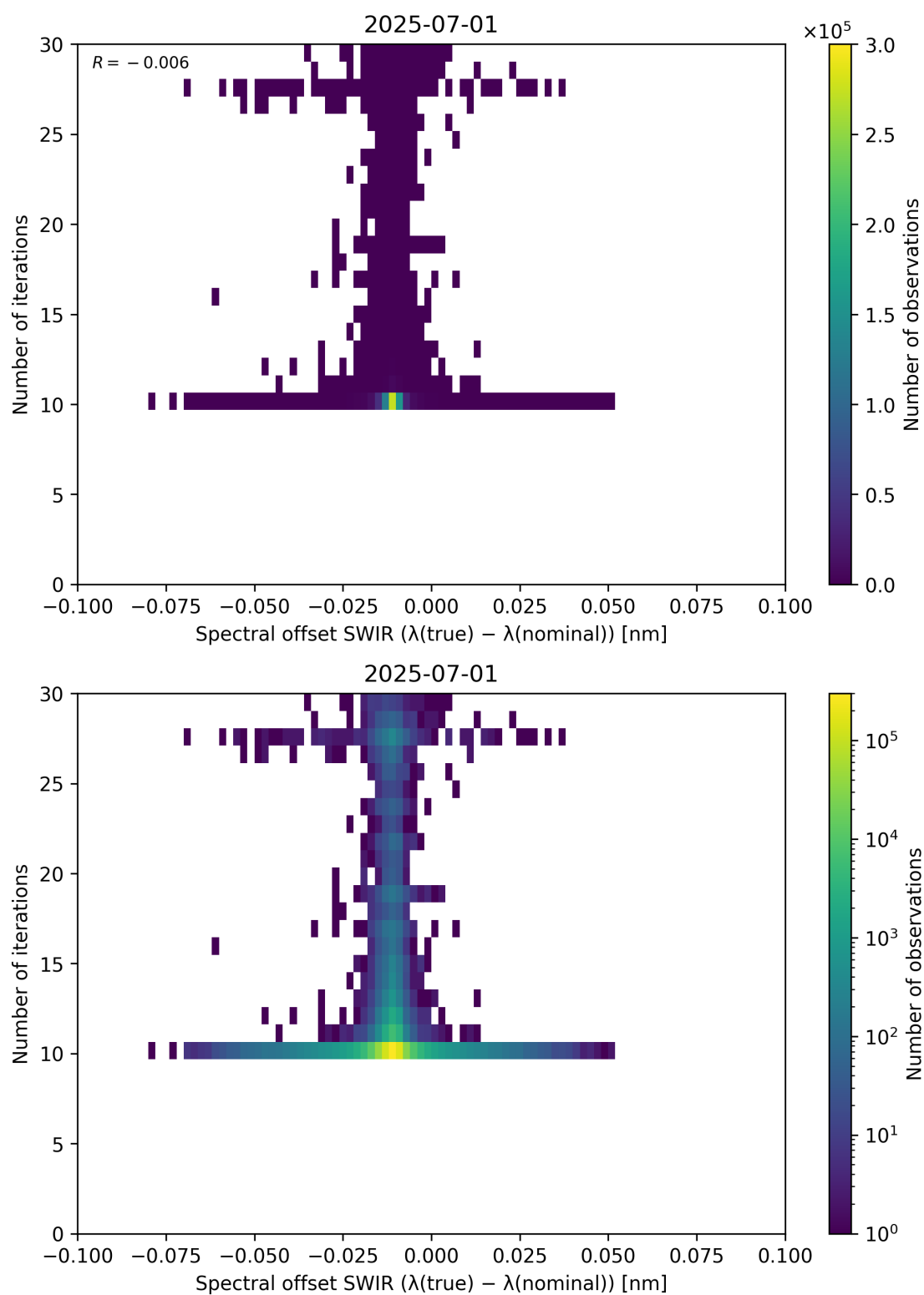
Figure 121: Scatter density plot of “Spectral offset SWIR ( \lambda_{\text{true}} - \lambda_{\text{nominal}} )” against “Number of iterations” for 2025-06-30 to 2025-07-02.
