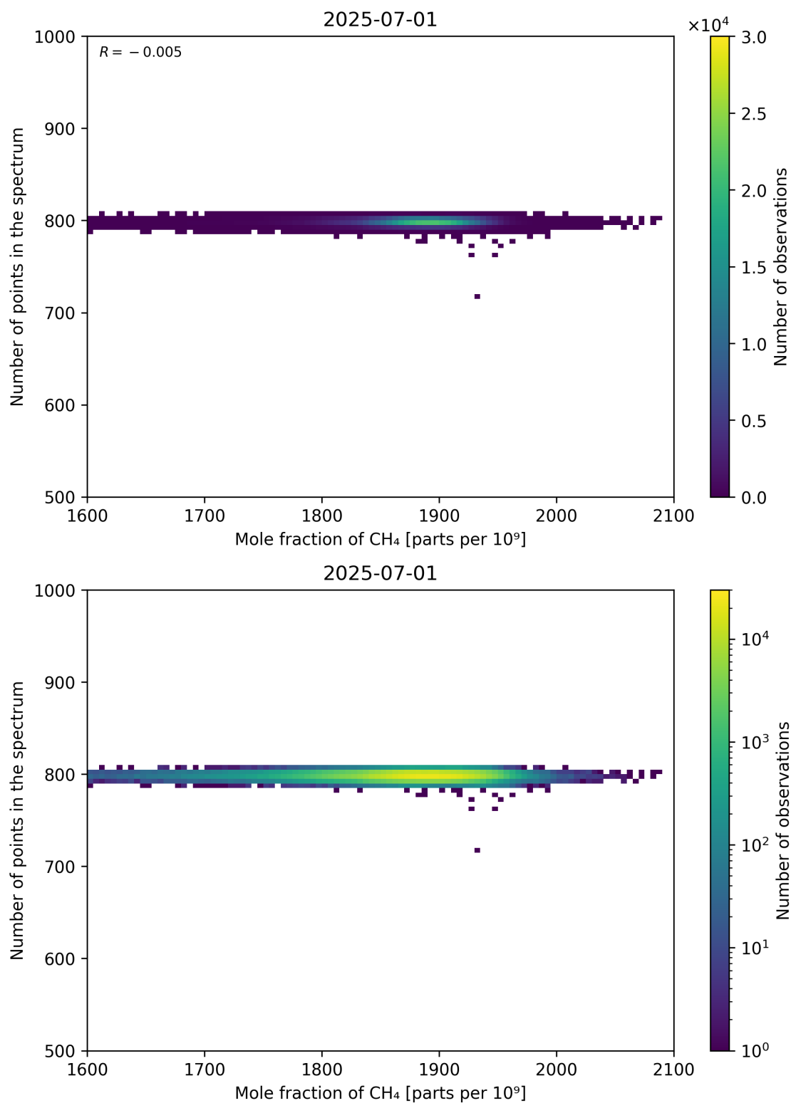
Figure 77: Scatter density plot of “Mole fraction of CH 4 ” against “Number of points in the spectrum” for 2025-06-30 to 2025-07-02.
