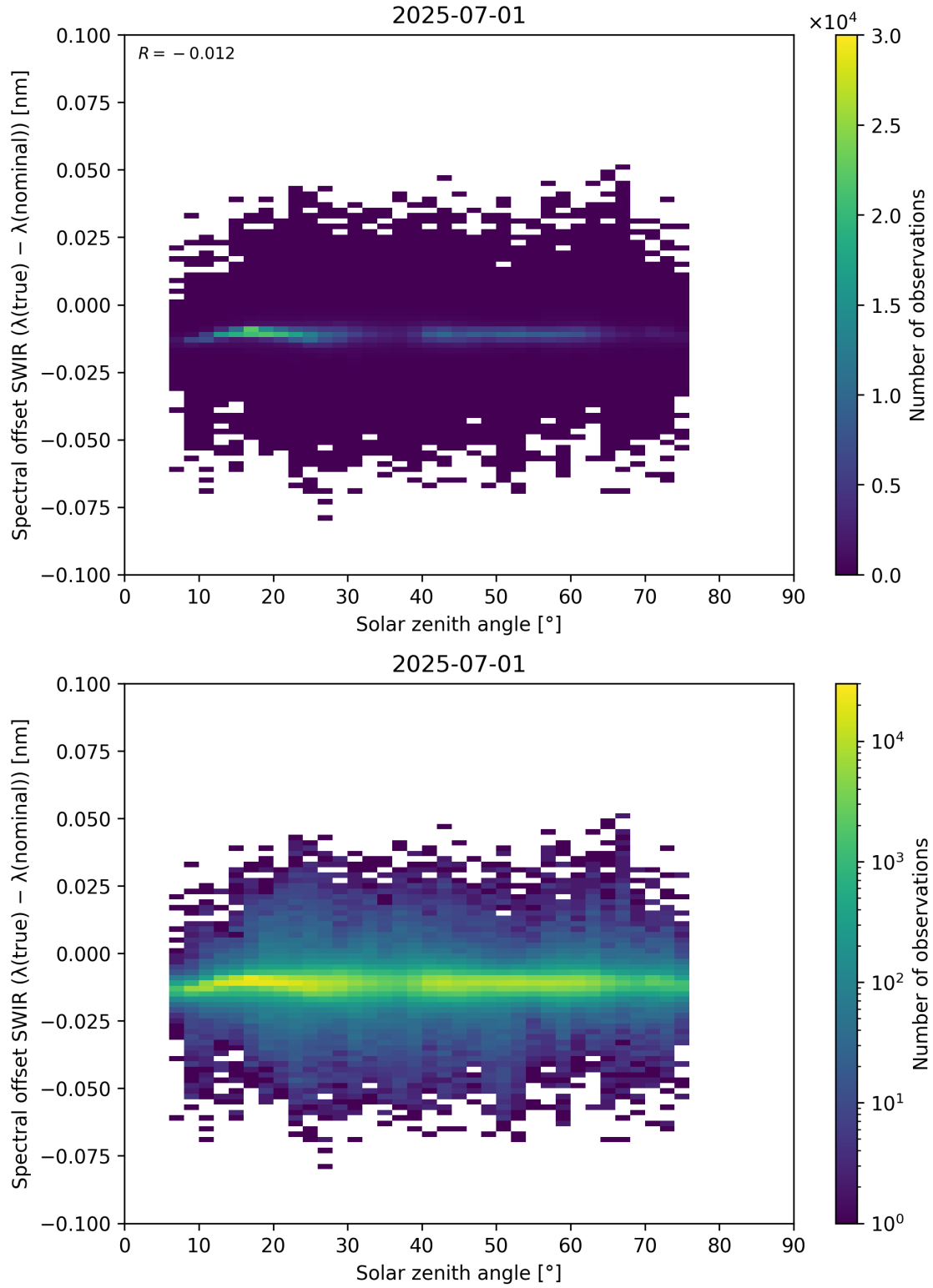
Figure 104: Scatter density plot of “Solar zenith angle” against “Spectral offset SWIR ( \lambda_{\text{true}} - \lambda_{\text{nominal}} )” for 2025-06-30 to 2025-07-02.
