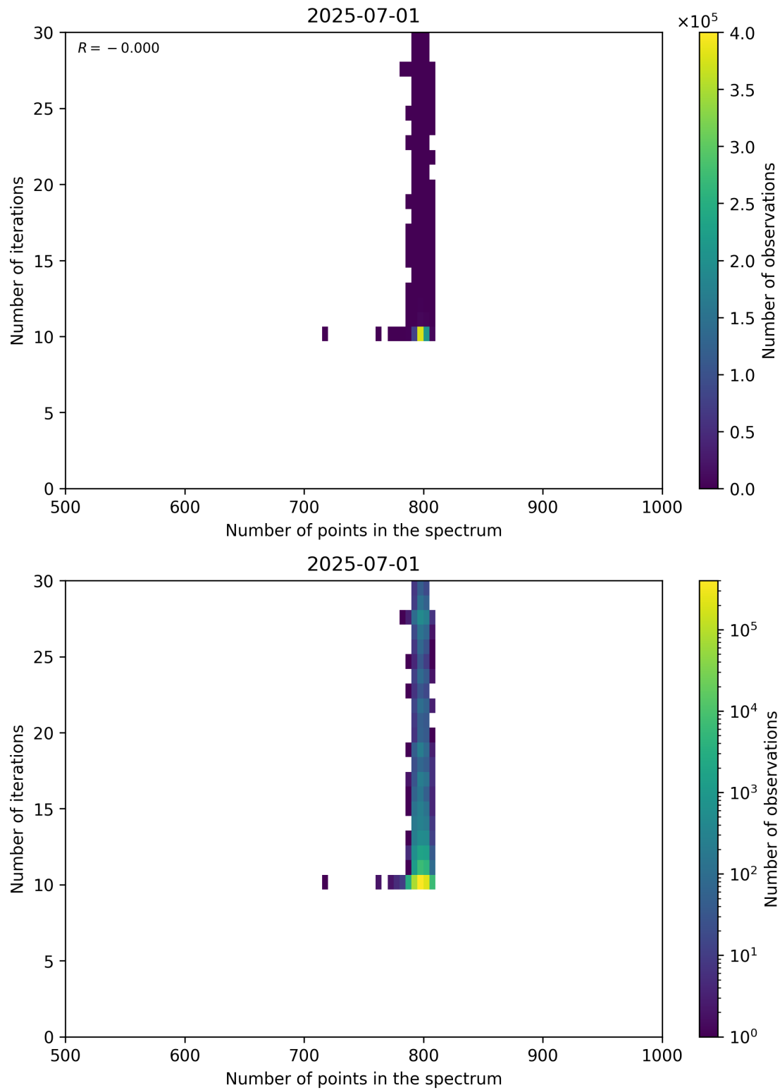
Figure 92: Scatter density plot of “Number of points in the spectrum” against “Number of iterations” for 2025-06-30 to 2025-07-02.
