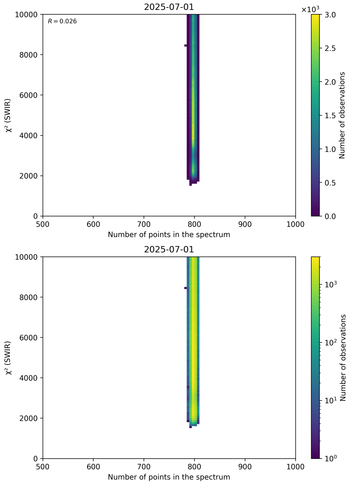
Figure 89: Scatter density plot of “Number of points in the spectrum” against “ \chi^2 (SWIR)” for 2025-06-30 to 2025-07-02.
