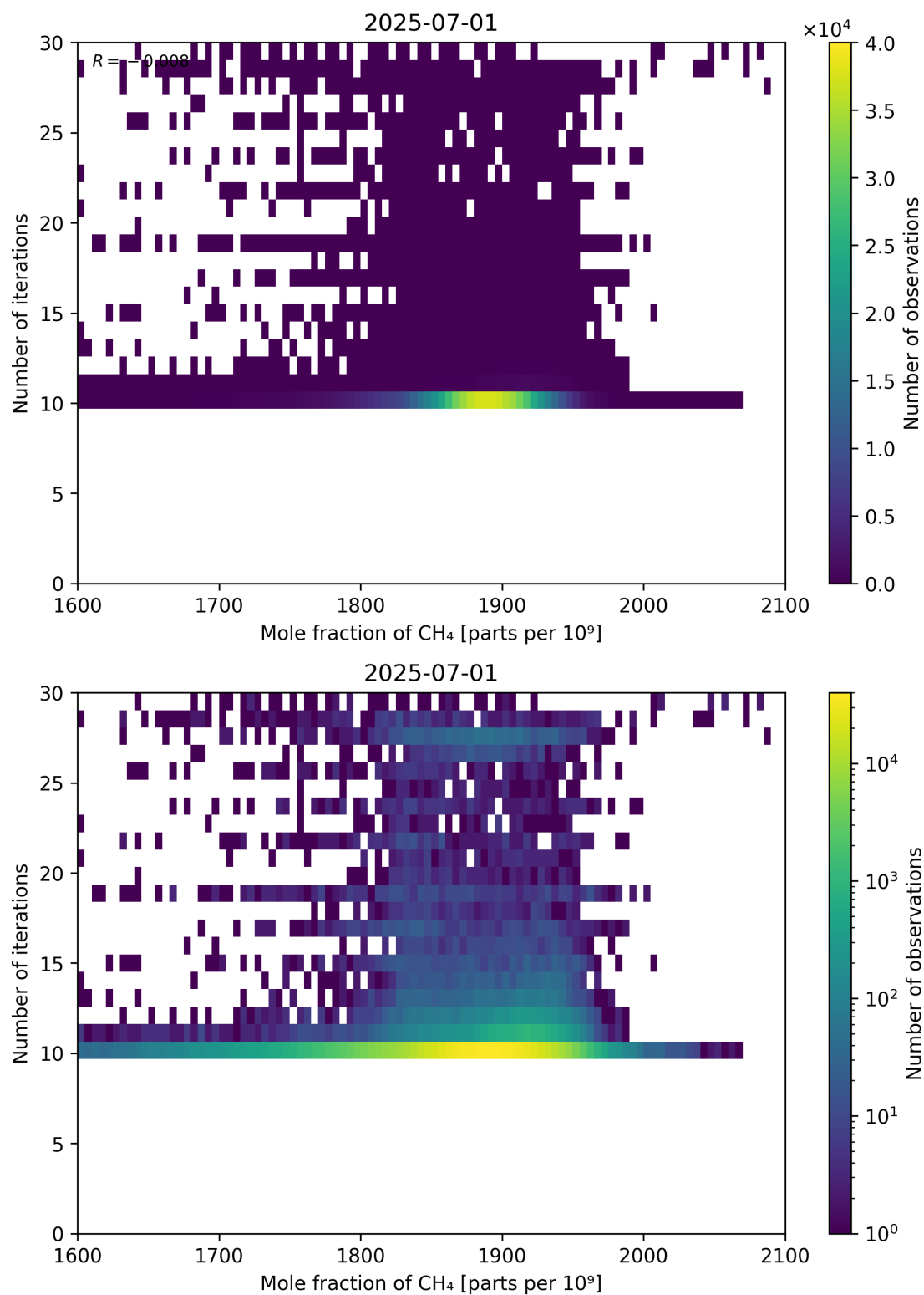
Figure 76: Scatter density plot of “Mole fraction of CH 4 ” against “Number of iterations” for 2025-06-30 to 2025-07-02.
