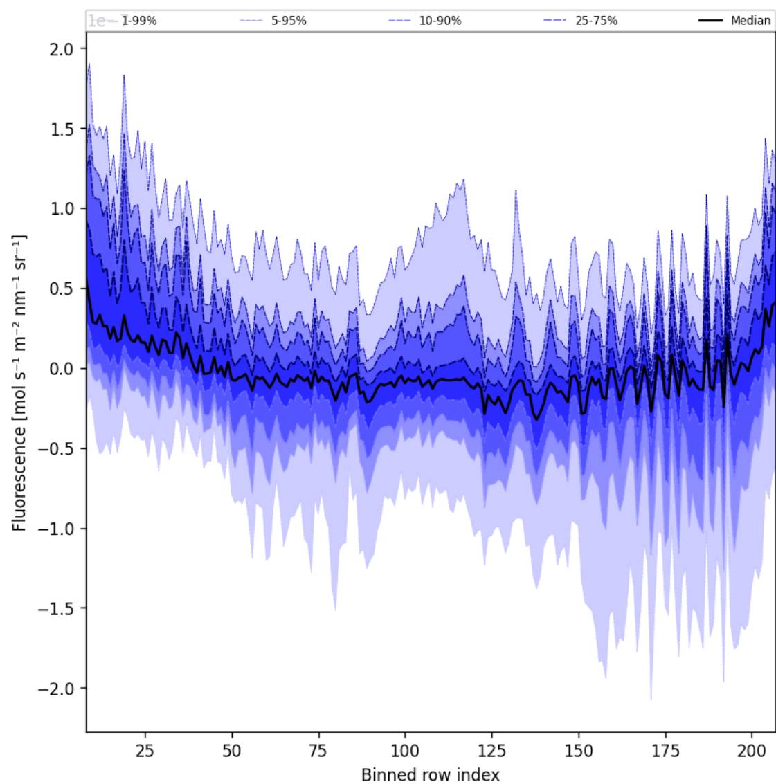
Figure 43: Along track statistics of "Fluorescence" for 2025-06-30 to 2025-07-02
