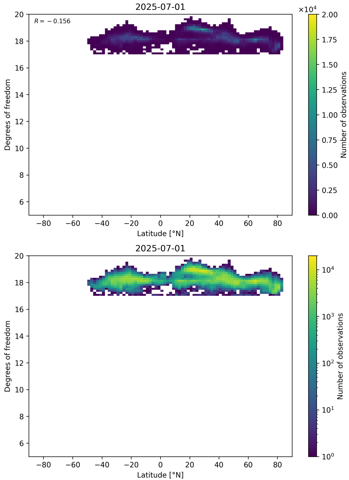
Figure 55: Scatter density plot of “Latitude” against “Degrees of freedom” for 2025-06-30 to 2025-07-02.
