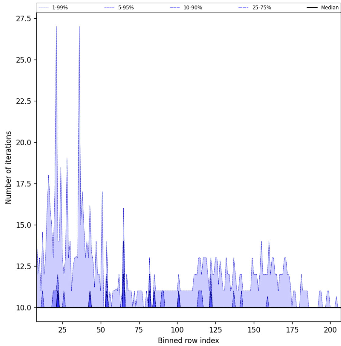
Figure 42: Along track statistics of “Number of iterations” for 2025-06-30 to 2025-07-02
