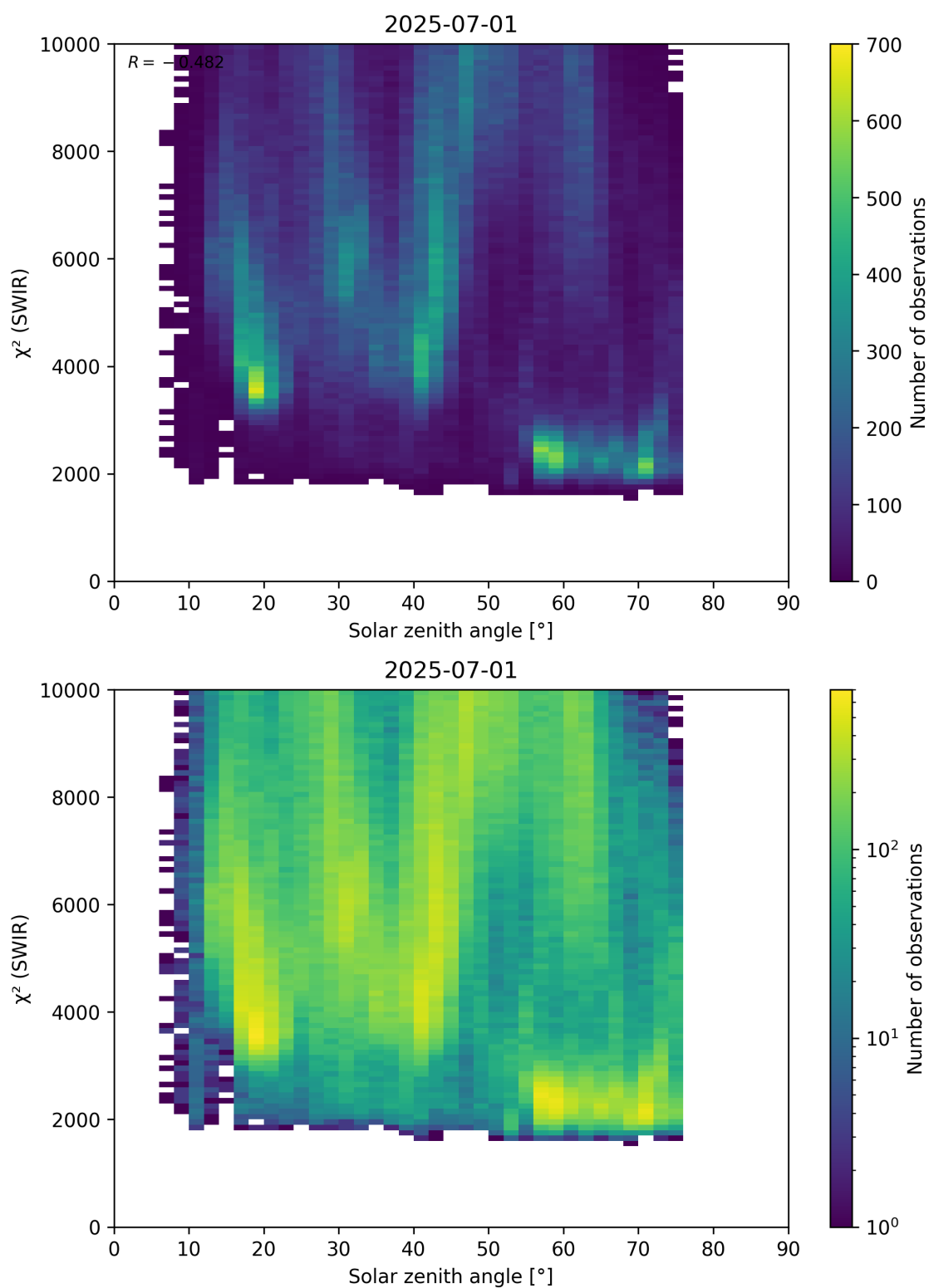
Figure 95: Scatter density plot of “Solar zenith angle” against “ \chi^2 (SWIR)” for 2025-06-30 to 2025-07-02.
