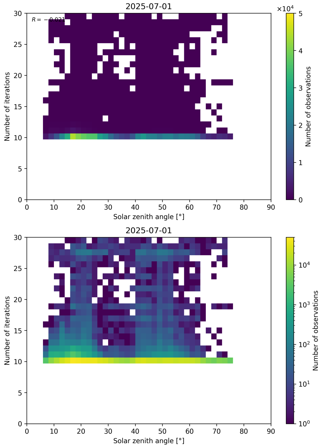
Figure 102: Scatter density plot of “Solar zenith angle” against “Number of iterations” for 2025-06-30 to 2025-07-02.
