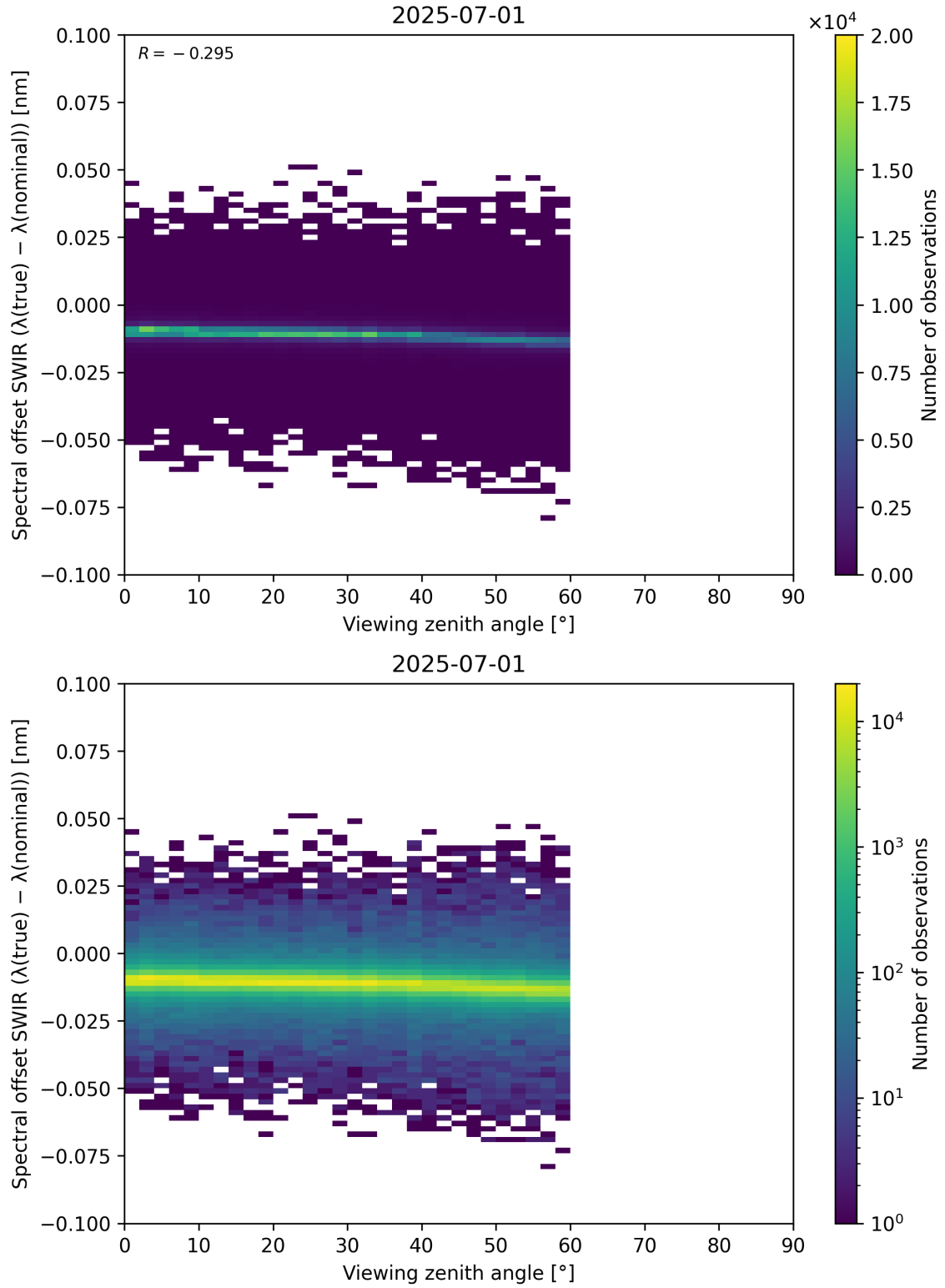
Figure 116: Scatter density plot of “Viewing zenith angle” against “Spectral offset SWIR ( \lambda_{\text{true}} - \lambda_{\text{nominal}} )” for 2025-06-30 to 2025-07-02.
