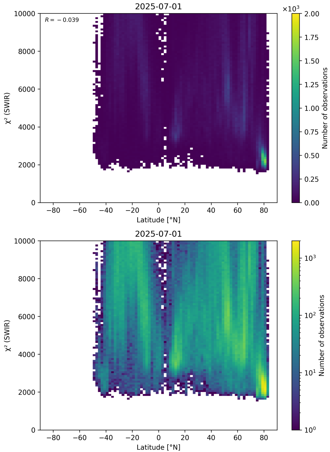
Figure 54: Scatter density plot of “Latitude” against “ \chi^2 (SWIR)” for 2025-06-30 to 2025-07-02.
