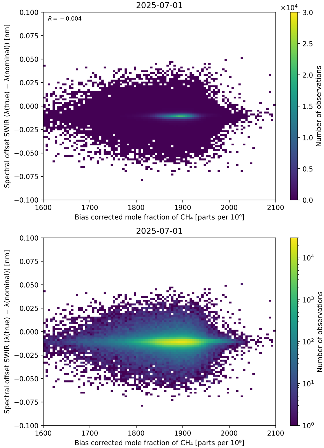
Figure 69: Scatter density plot of “Bias corrected mole fraction of \text{CH}_4 ” against “Spectral offset SWIR ( \lambda_{\text{true}} - \lambda_{\text{nominal}} )” for 2025-06-30 to 2025-07-02.
