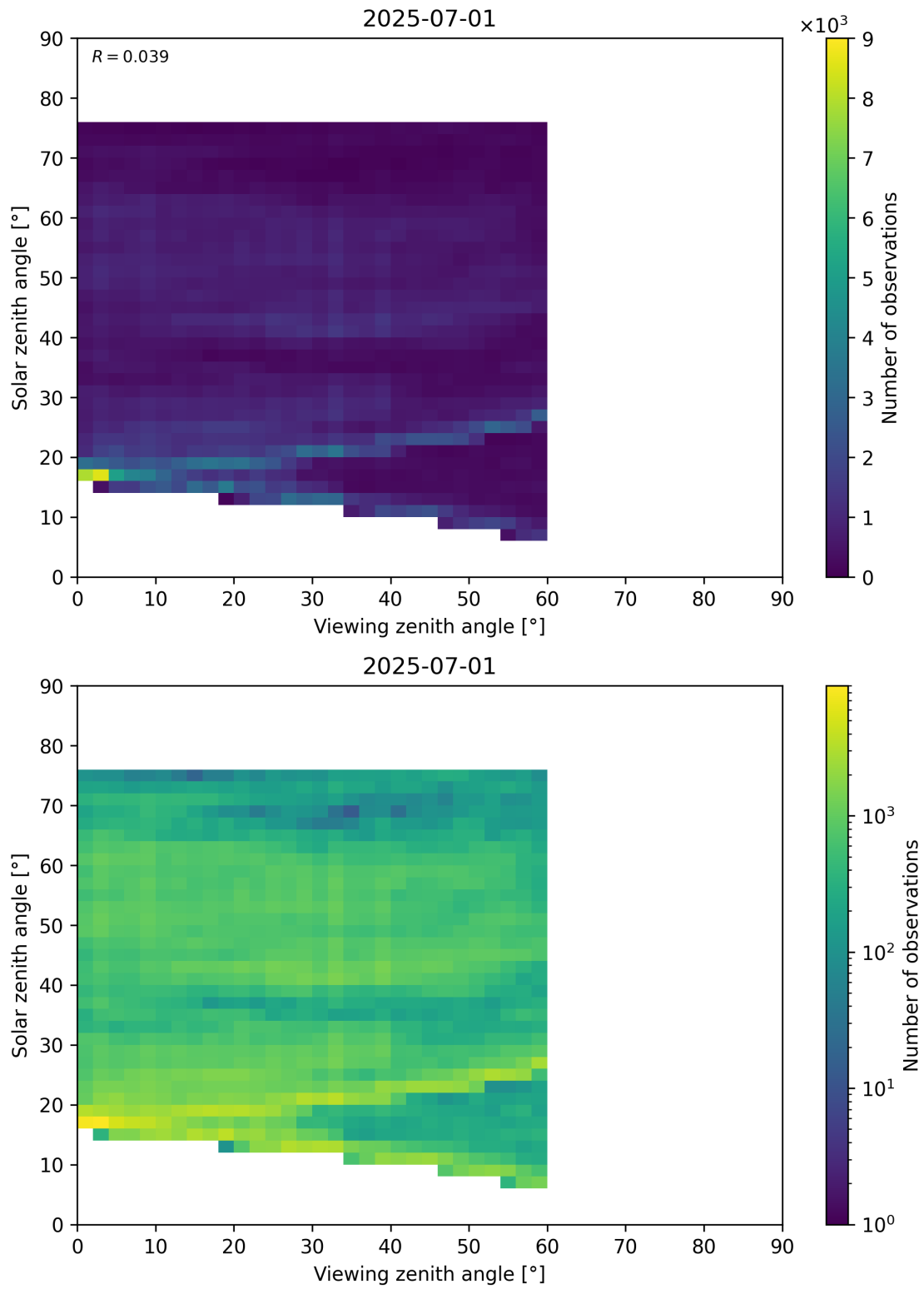
Figure 115: Scatter density plot of “Viewing zenith angle” against “Solar zenith angle” for 2025-06-30 to 2025-07-02.
