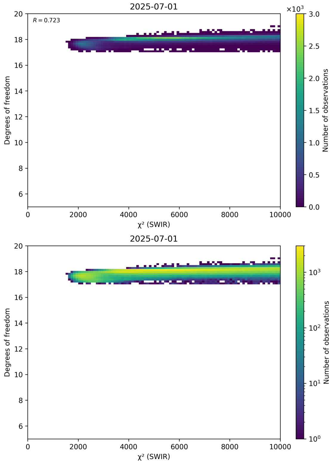
Figure 48: Scatter density plot of “ \chi^2 (SWIR)” against “Degrees of freedom” for 2025-06-30 to 2025-07-02.
