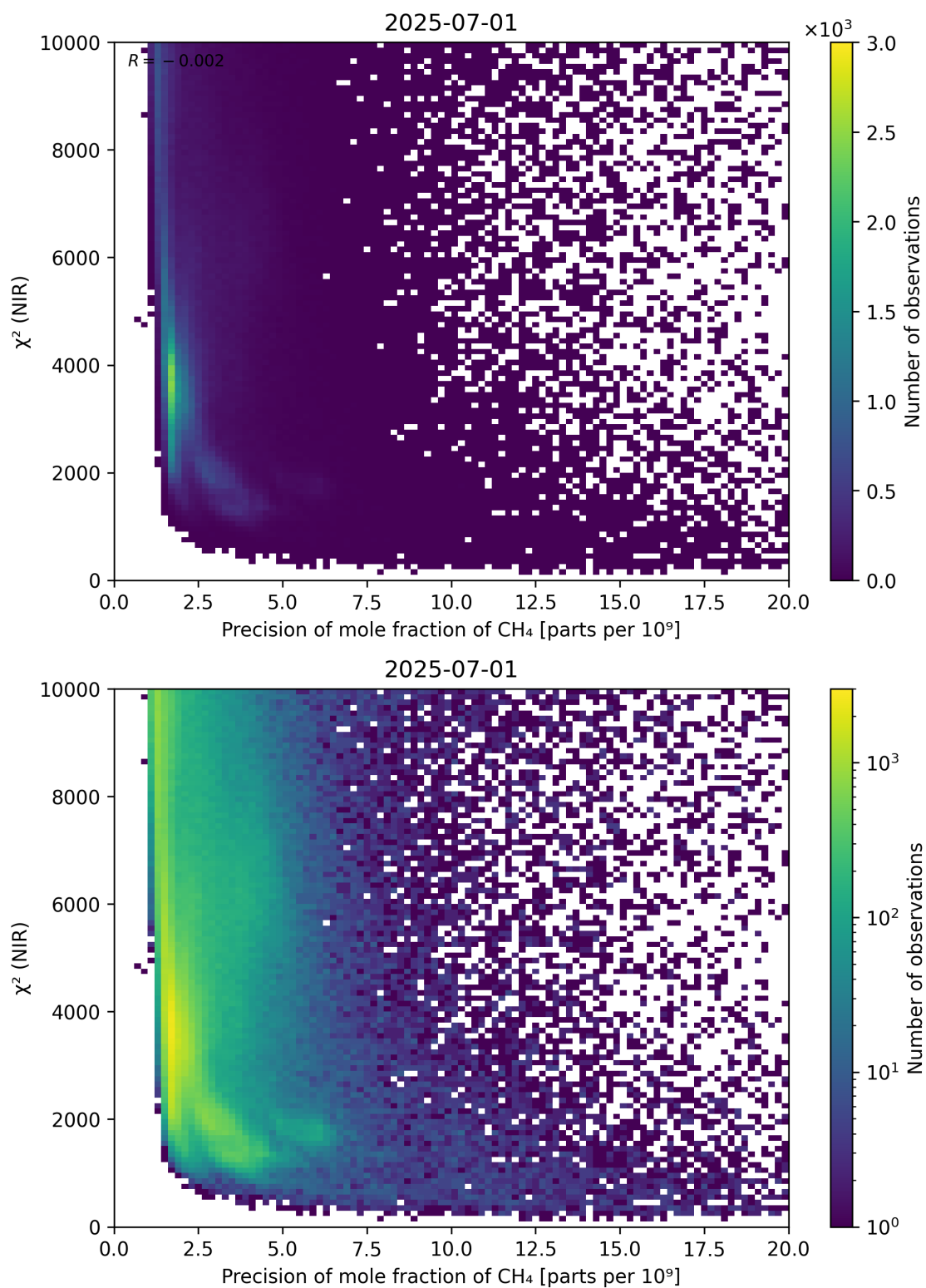
Figure 78: Scatter density plot of “Precision of mole fraction of CH 4 ” against “ \chi^2 (NIR)” for 2025-06-30 to 2025-07-02.
