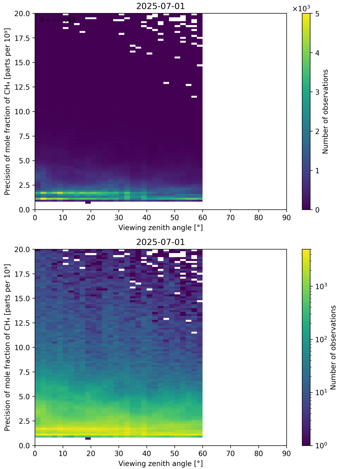
Figure 112: Scatter density plot of “Viewing zenith angle” against “Precision of mole fraction of CH 4 ” for 2025-06-30 to 2025-07-02.
