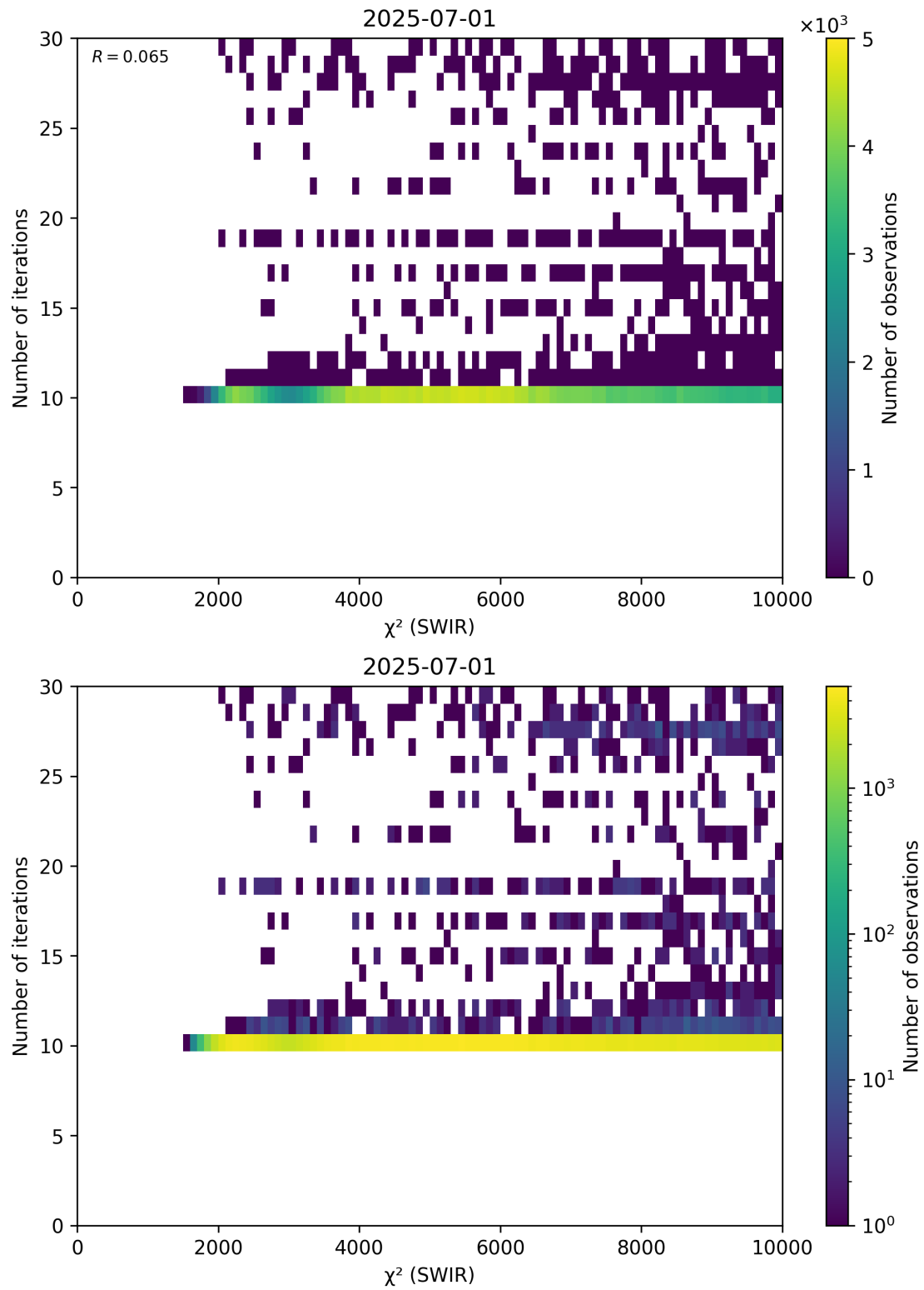
Figure 50: Scatter density plot of “ \chi^2 (SWIR)” against “Number of iterations” for 2025-06-30 to 2025-07-02.
