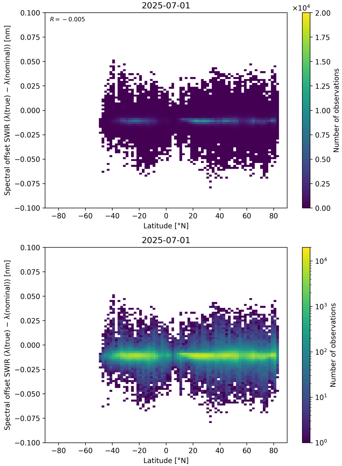
Figure 62: Scatter density plot of “Latitude” against “Spectral offset SWIR ( \lambda_{\text{true}} - \lambda_{\text{nominal}} )” for 2025-06-30 to 2025-07-02.
