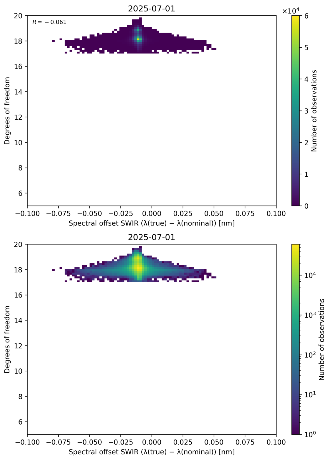
Figure 119: Scatter density plot of “Spectral offset SWIR ( \lambda_{\text{true}} - \lambda_{\text{nominal}} )” against “Degrees of freedom” for 2025-06-30 to 2025-07-02.
