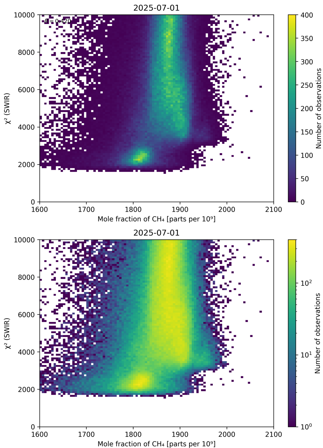
Figure 71: Scatter density plot of “Mole fraction of CH 4 ” against “ \chi^2 (SWIR)” for 2025-06-30 to 2025-07-02.
