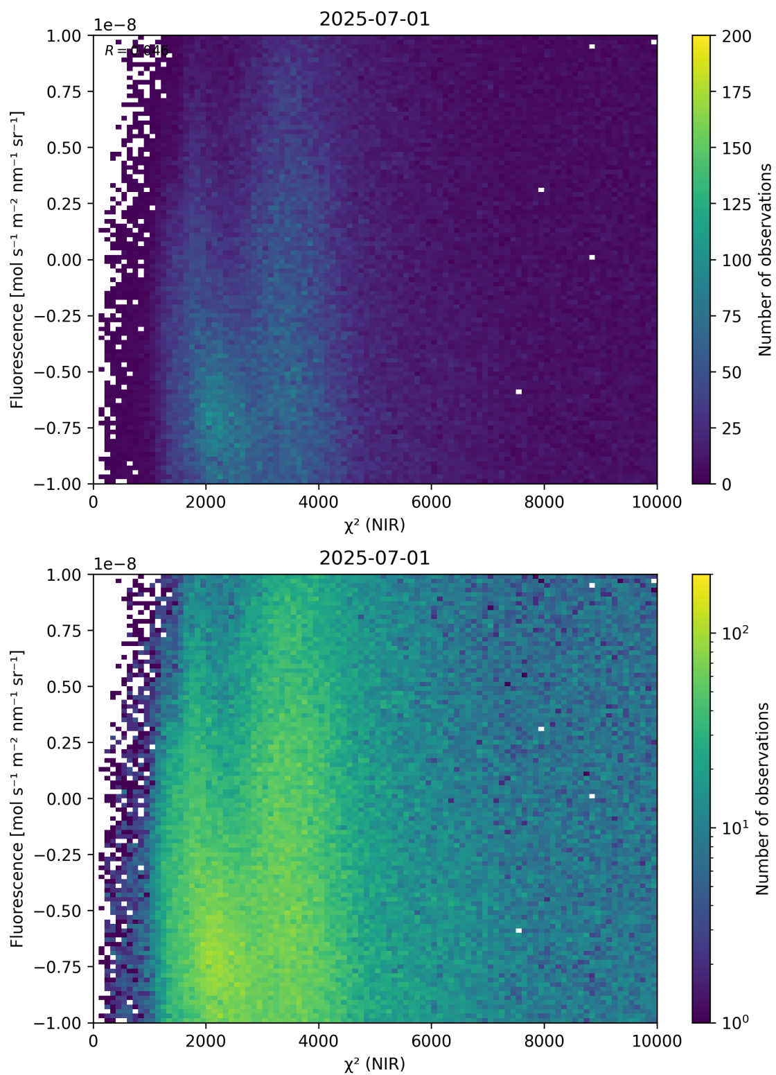
Figure 45: Scatter density plot of “ \chi^2 (NIR)” against “Fluorescence” for 2025-06-30 to 2025-07-02.
