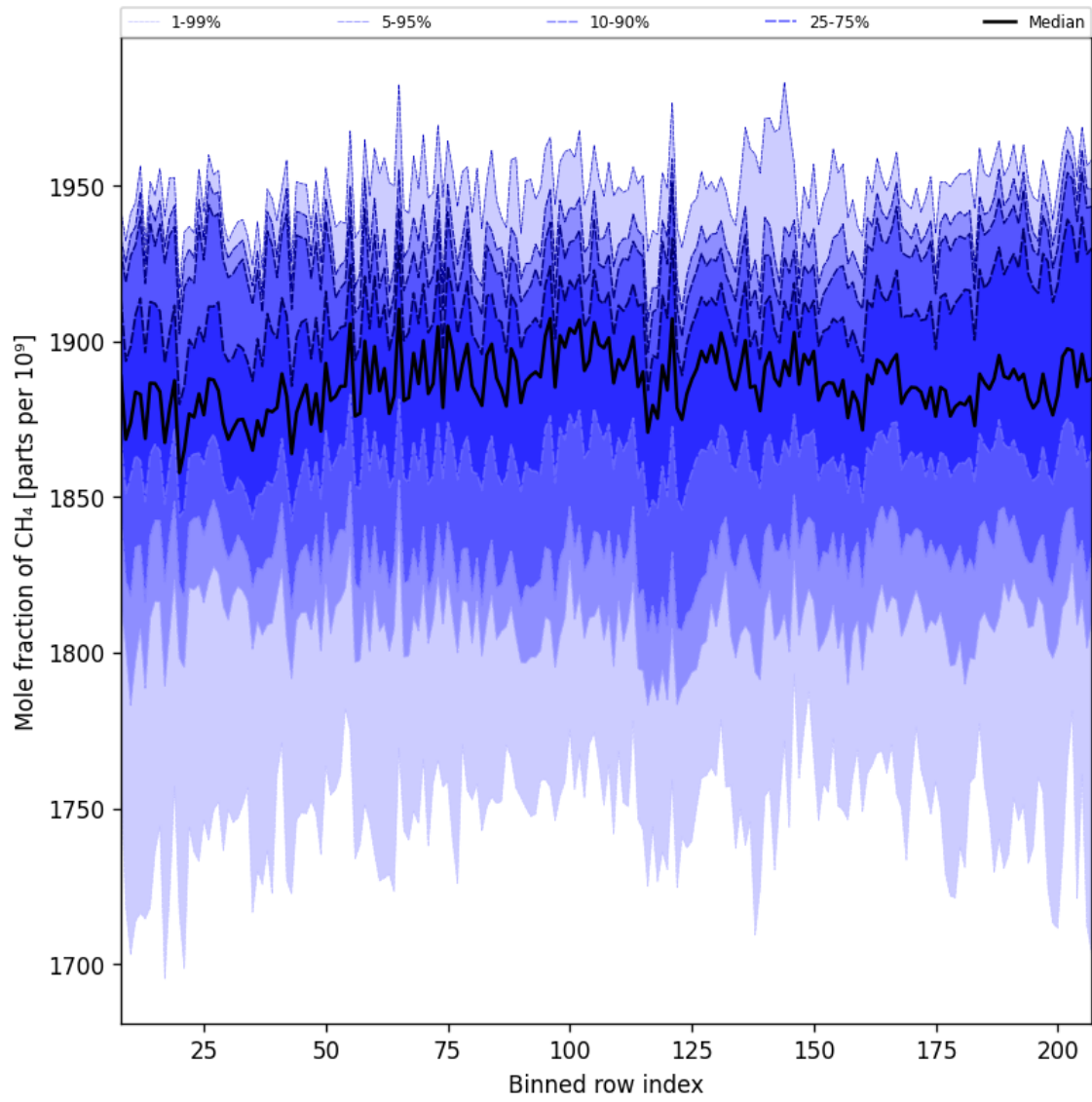
Figure 34: Along track statistics of “Mole fraction of CH 4 ” for 2025-06-30 to 2025-07-02
