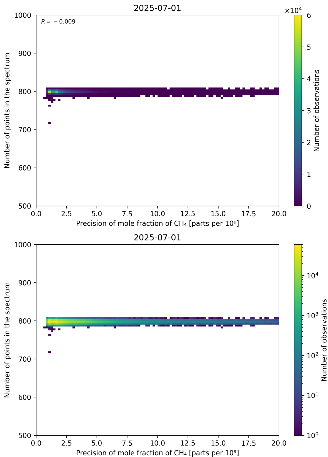
Figure 84: Scatter density plot of “Precision of mole fraction of CH 4 ” against “Number of points in the spectrum” for 2025-06-30 to 2025-07-02.
