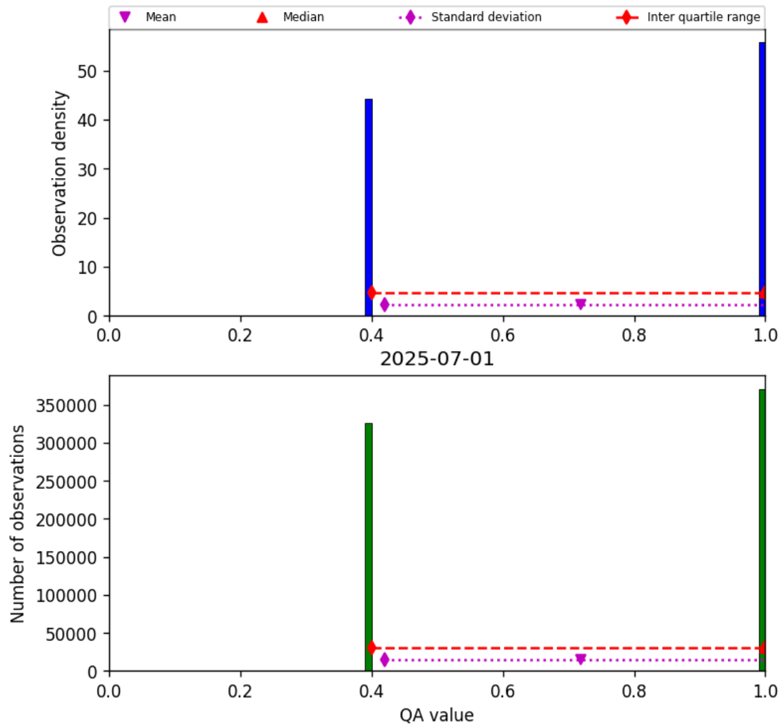
Figure 22: Histogram of “QA value” for 2025-06-30 to 2025-07-02
