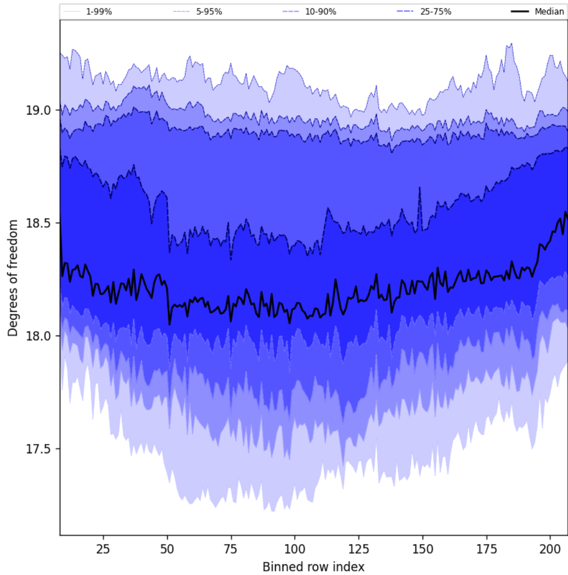
Figure 41: Along track statistics of “Degrees of freedom” for 2025-06-30 to 2025-07-02
