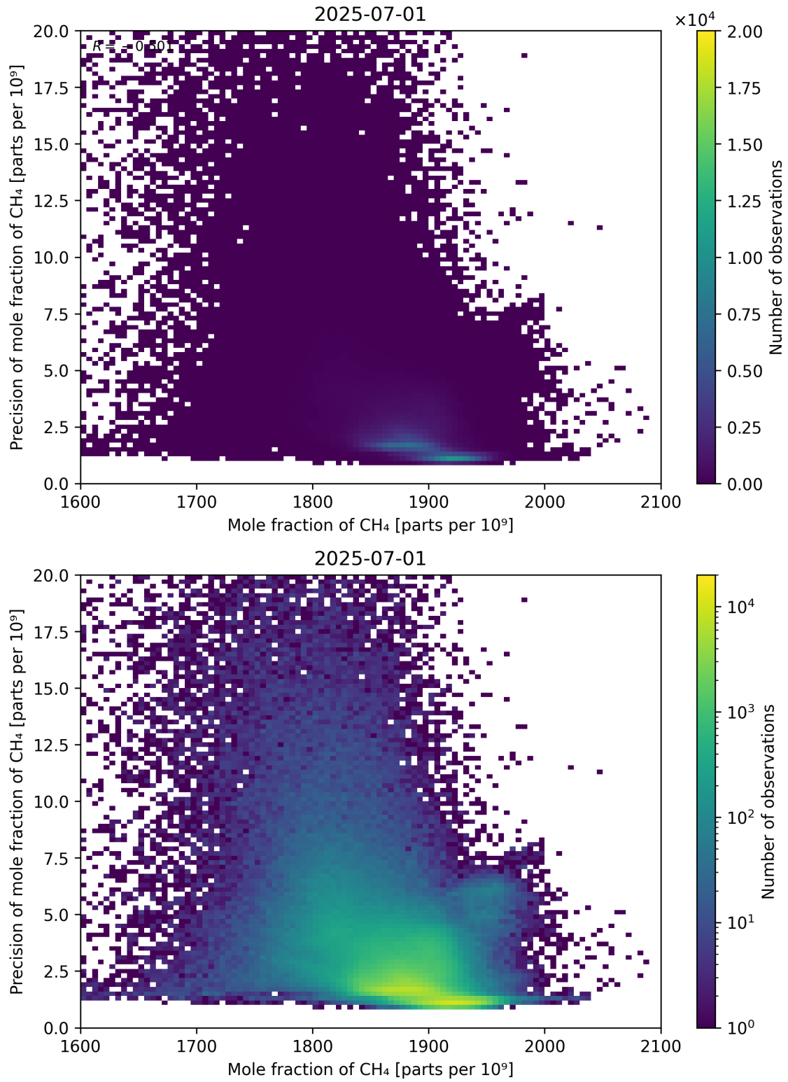
Figure 75: Scatter density plot of “Mole fraction of CH 4 ” against “Precision of mole fraction of CH 4 ” for 2025-06-30 to 2025-07-02.
