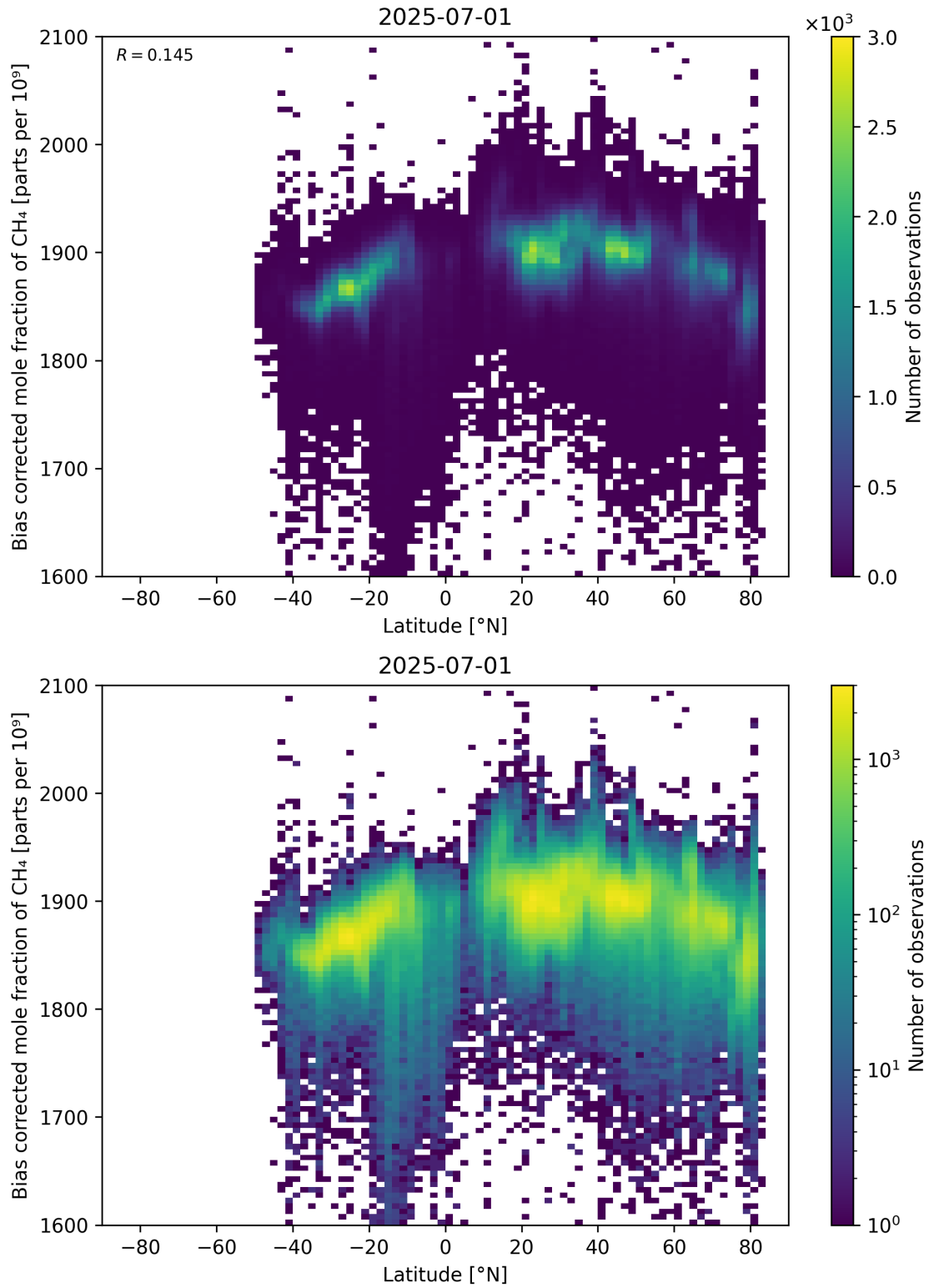
Figure 58: Scatter density plot of “Latitude” against “Bias corrected mole fraction of CH 4 ” for 2025-06-30 to 2025-07-02.
