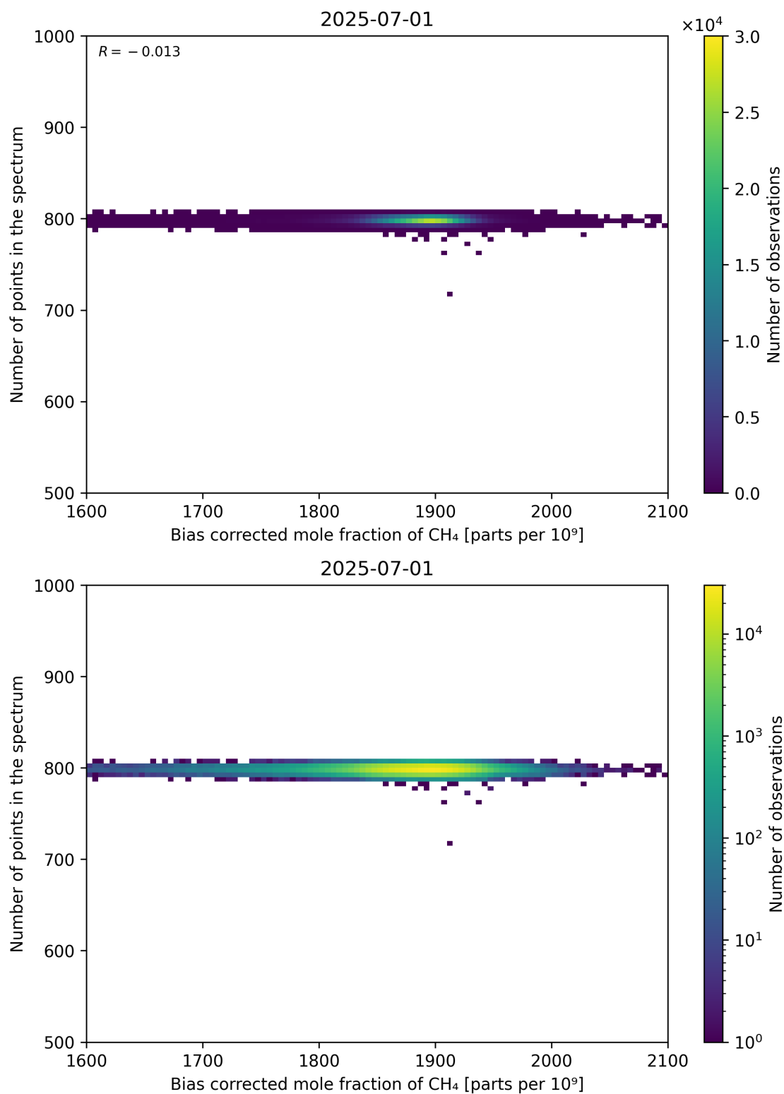
Figure 68: Scatter density plot of “Bias corrected mole fraction of CH 4 ” against “Number of points in the spectrum” for 2025-06-30 to 2025-07-02.
