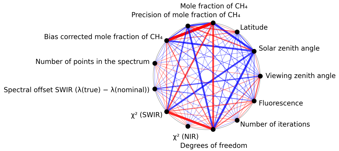
Figure 1: Map of correlation graph for 2025-06-30 to 2025-07-02.
