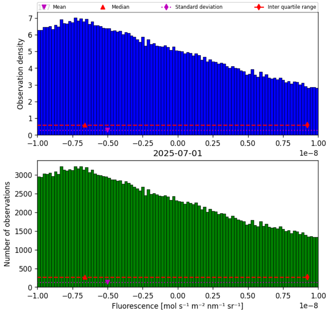
Figure 32: Histogram of “Fluorescence” for 2025-06-30 to 2025-07-02
