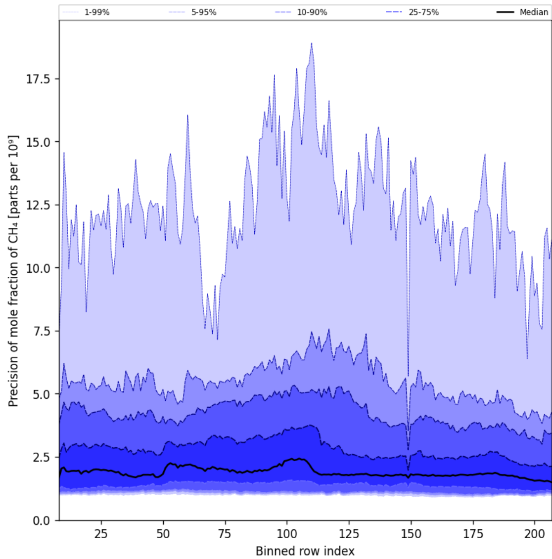
Figure 35: Along track statistics of “Precision of mole fraction of CH 4 ” for 2025-06-30 to 2025-07-02
