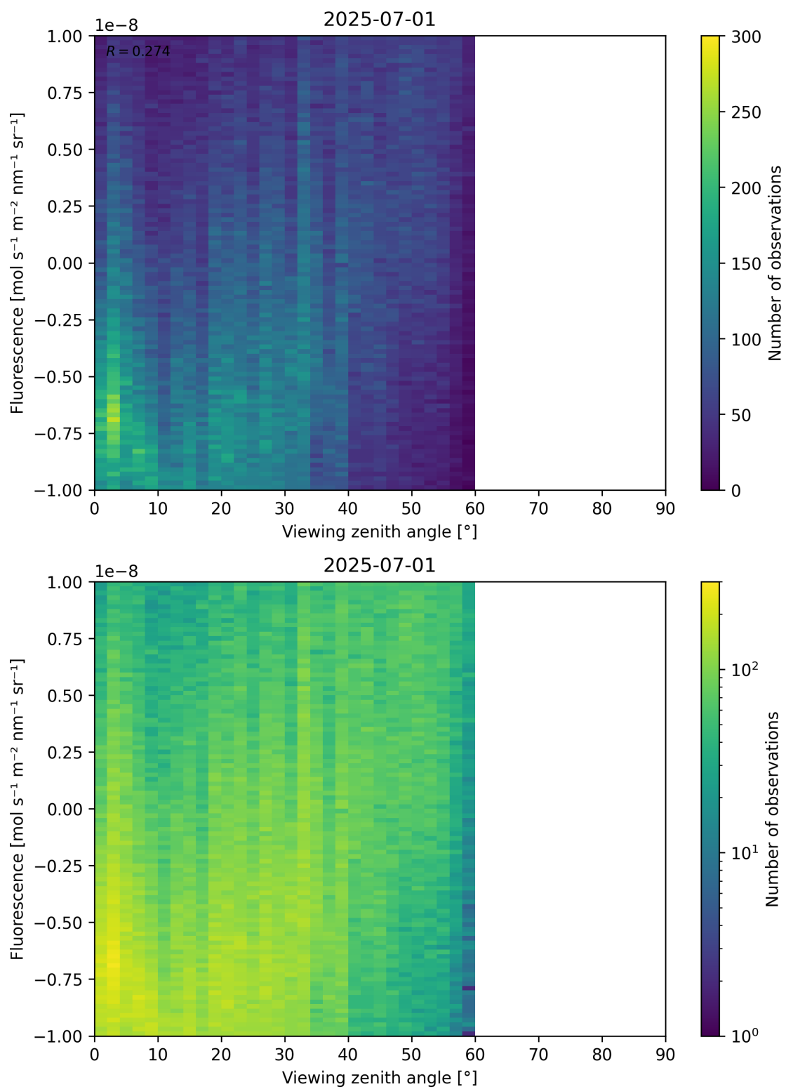
Figure 108: Scatter density plot of “Viewing zenith angle” against “Fluorescence” for 2025-06-30 to 2025-07-02.
