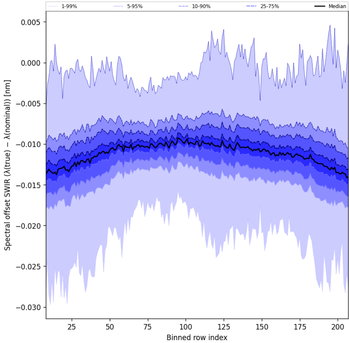
Figure 38: Along track statistics of “Spectral offset SWIR ( \lambda_{\text{true}} - \lambda_{\text{nominal}} )” for 2025-06-30 to 2025-07-02
