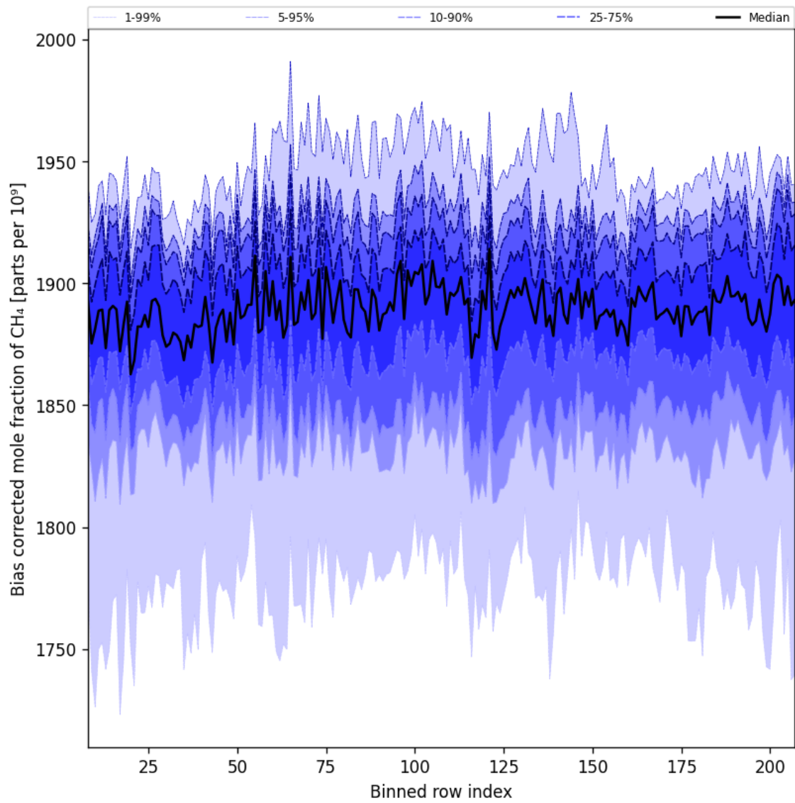
Figure 36: Along track statistics of “Bias corrected mole fraction of CH 4 ” for 2025-06-30 to 2025-07-02
