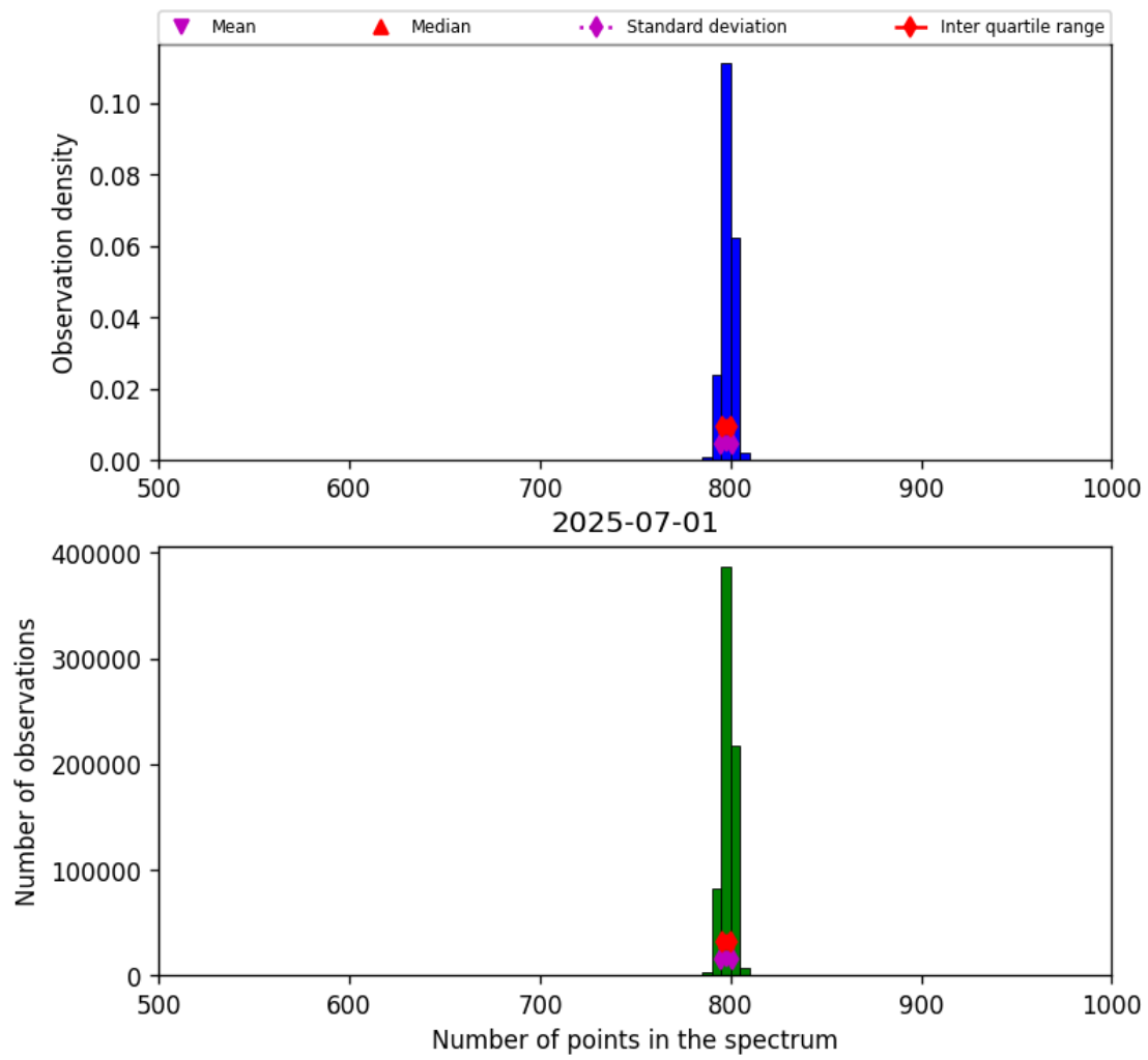
Figure 26: Histogram of “Number of points in the spectrum” for 2025-06-30 to 2025-07-02
