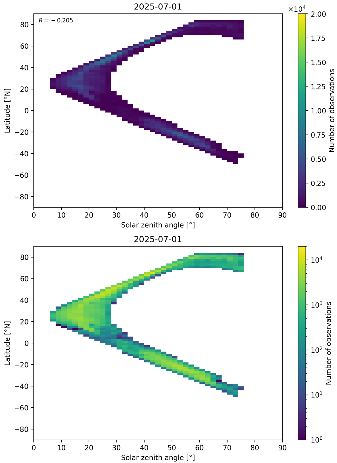
Figure 98: Scatter density plot of “Solar zenith angle” against “Latitude” for 2025-06-30 to 2025-07-02.
