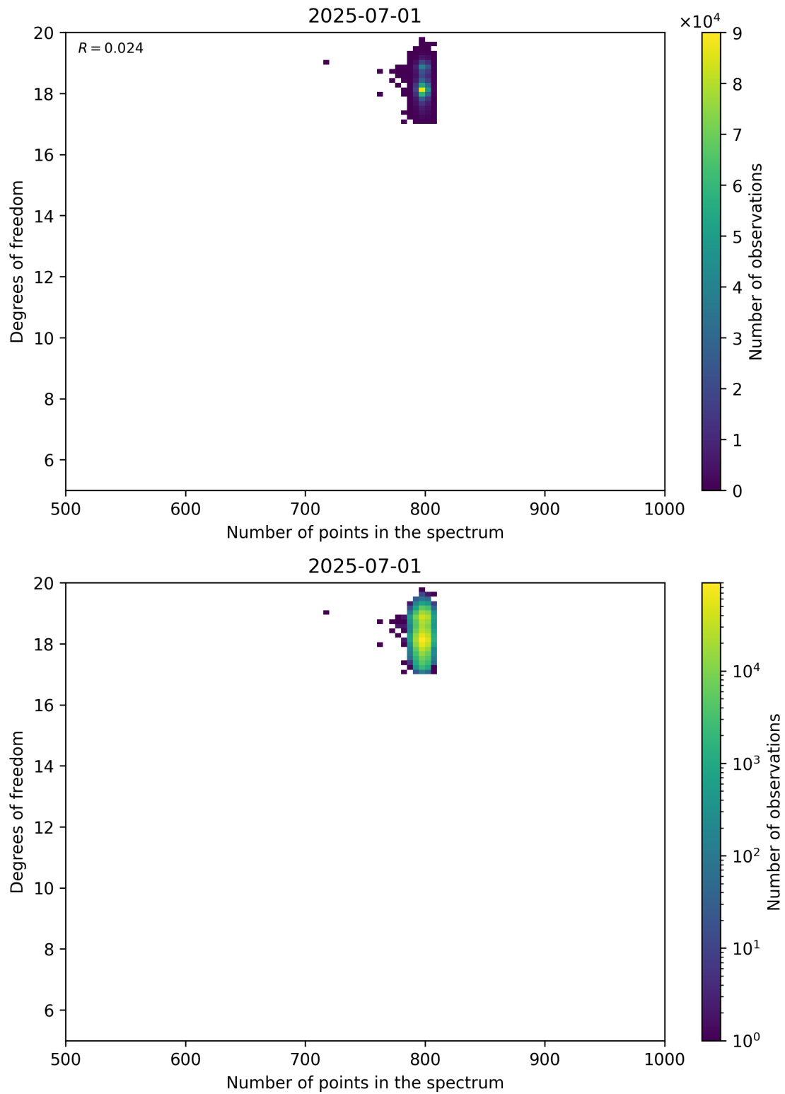
Figure 90: Scatter density plot of “Number of points in the spectrum” against “Degrees of freedom” for 2025-06-30 to 2025-07-02.
