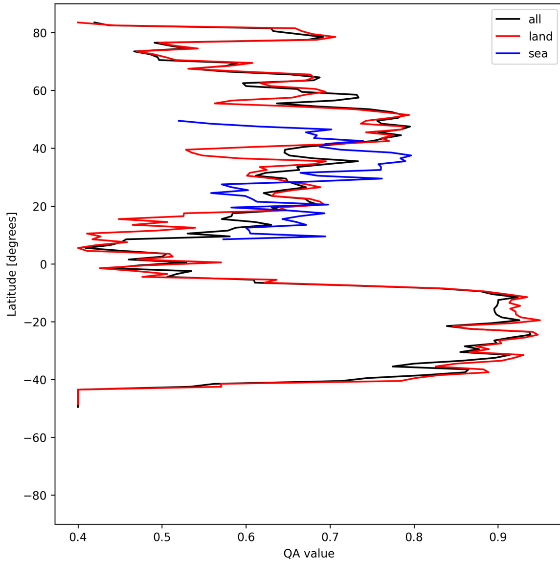
Figure 11: Zonal average of “QA value” for 2025-06-30 to 2025-07-02.
