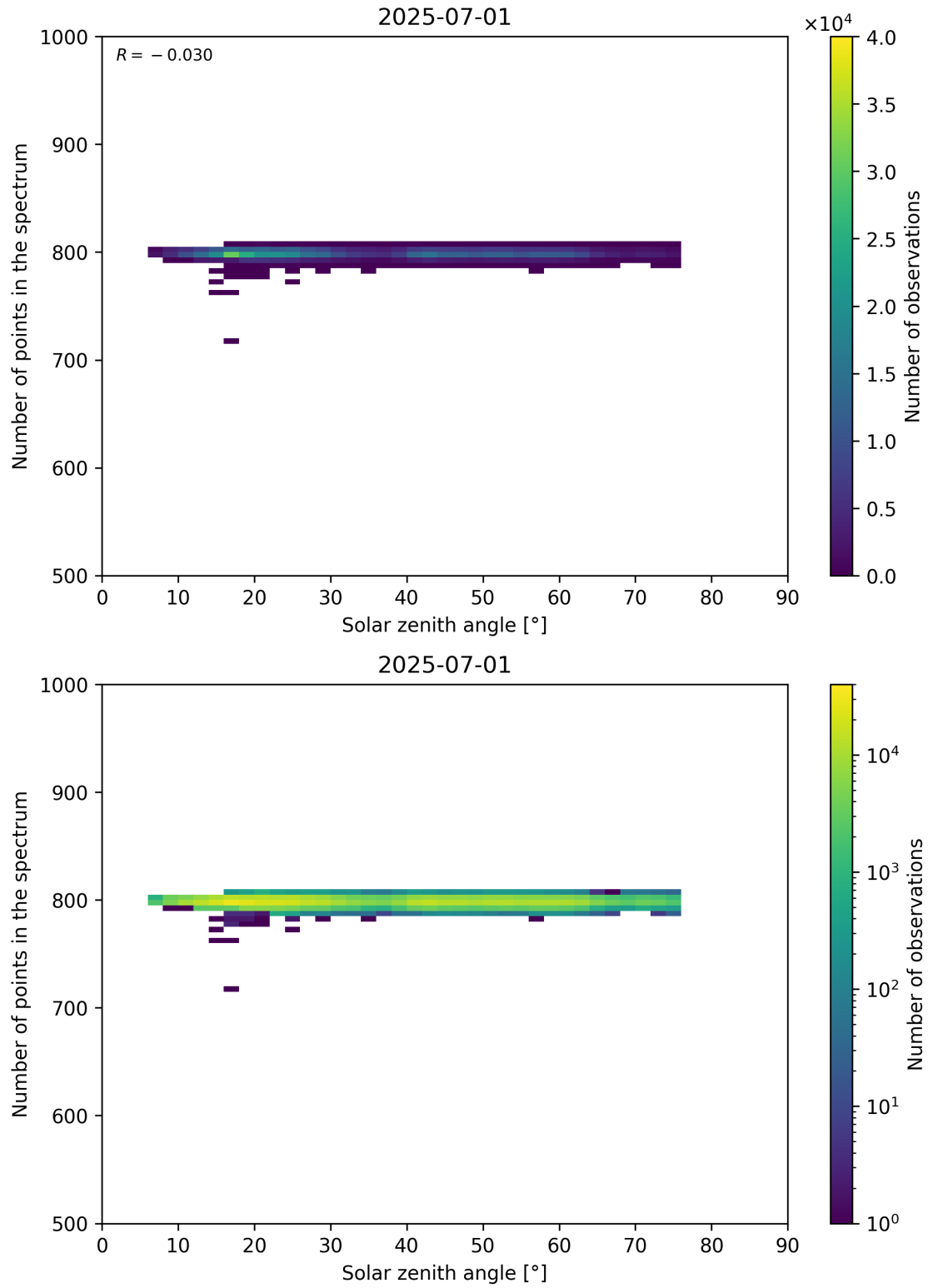
Figure 103: Scatter density plot of “Solar zenith angle” against “Number of points in the spectrum” for 2025-06-30 to 2025-07-02.
