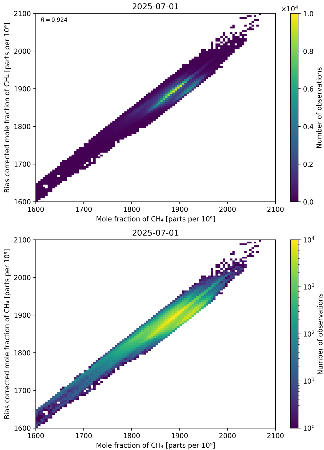
Figure 74: Scatter density plot of “Mole fraction of CH 4 ” against “Bias corrected mole fraction of CH 4 ” for 2025-06-30 to 2025-07-02.
