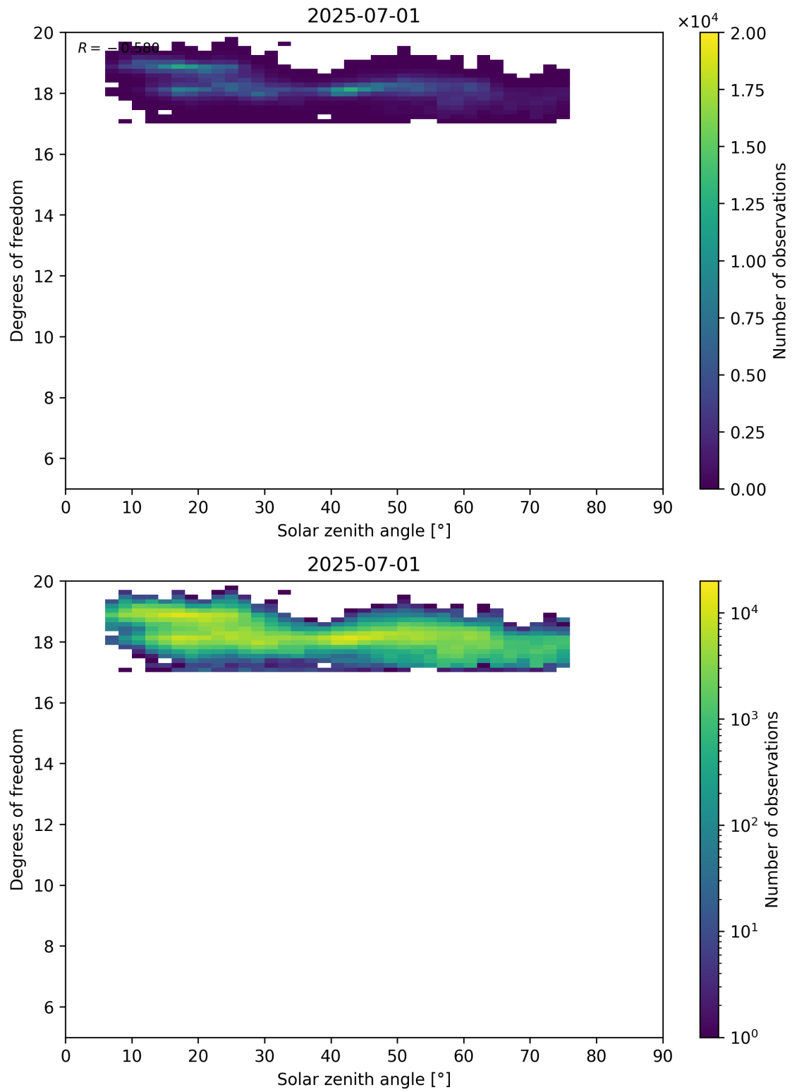
Figure 96: Scatter density plot of “Solar zenith angle” against “Degrees of freedom” for 2025-06-30 to 2025-07-02.
