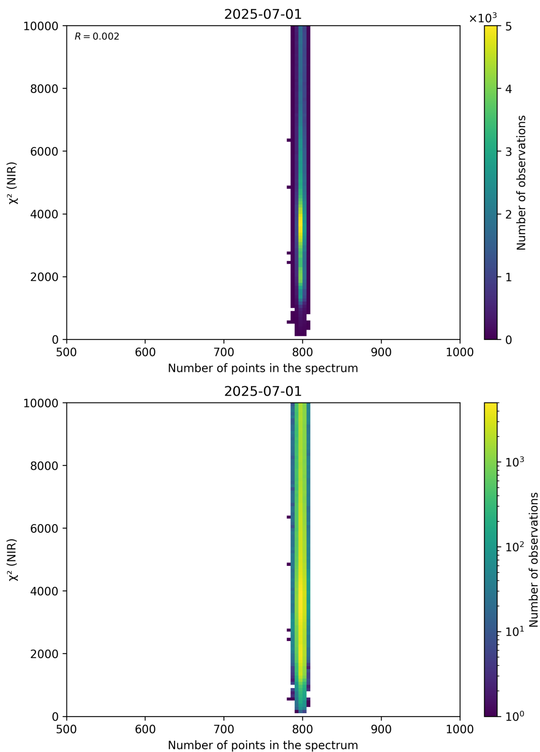
Figure 88: Scatter density plot of “Number of points in the spectrum” against “ \chi^2 (NIR)” for 2025-06-30 to 2025-07-02.
