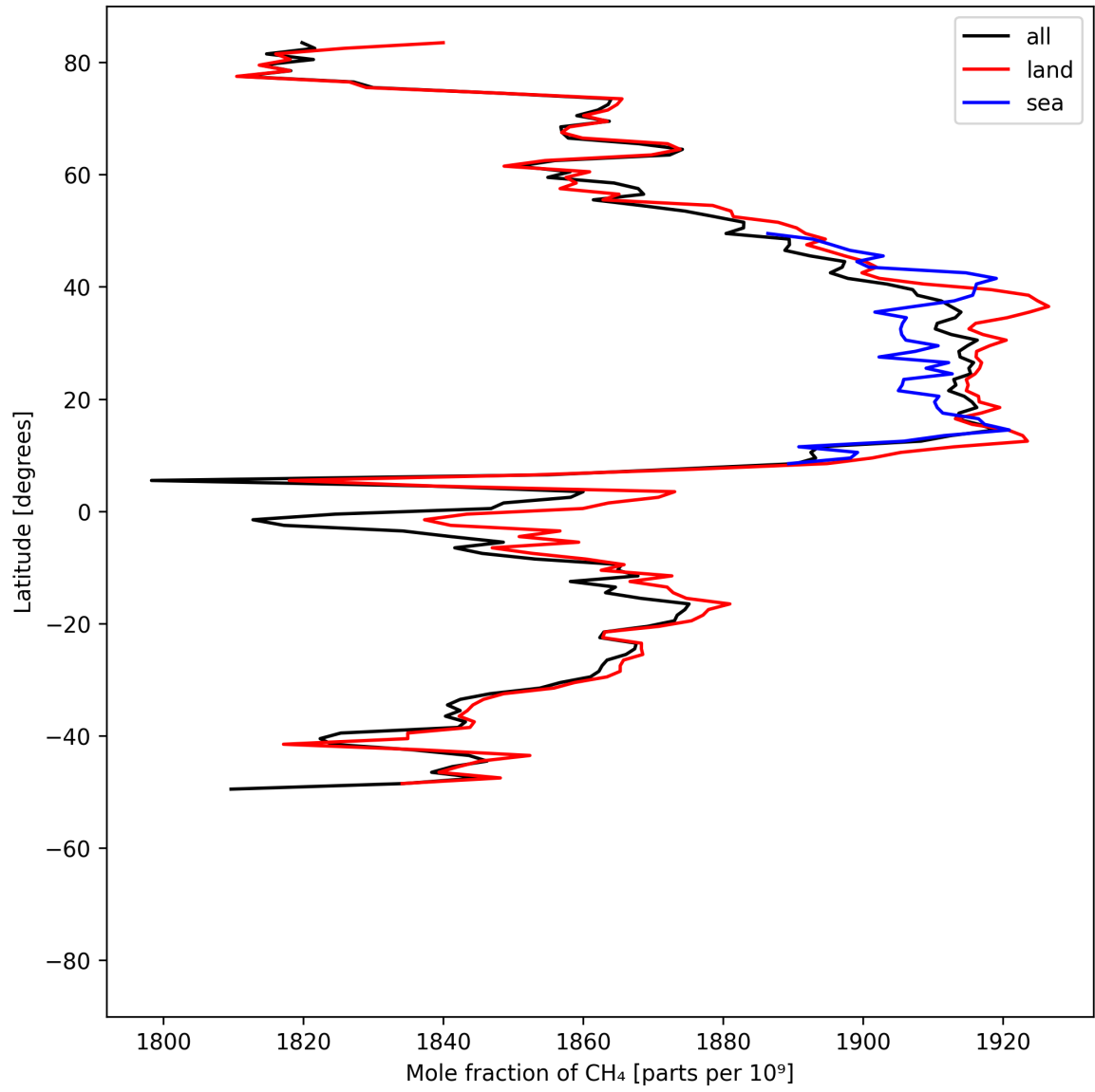
Figure 12: Zonal average of “Mole fraction of CH 4 ” for 2025-06-30 to 2025-07-02.
