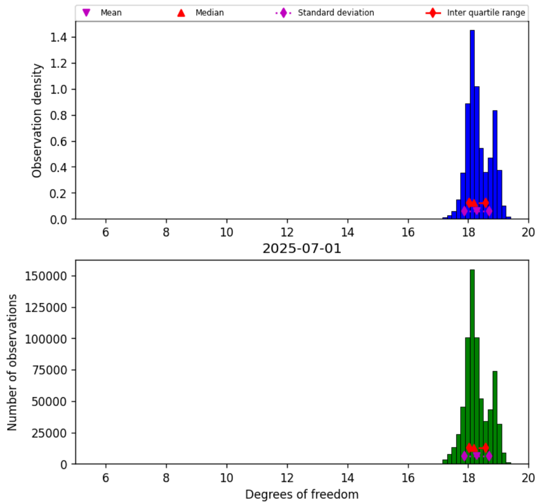
Figure 30: Histogram of “Degrees of freedom” for 2025-06-30 to 2025-07-02
