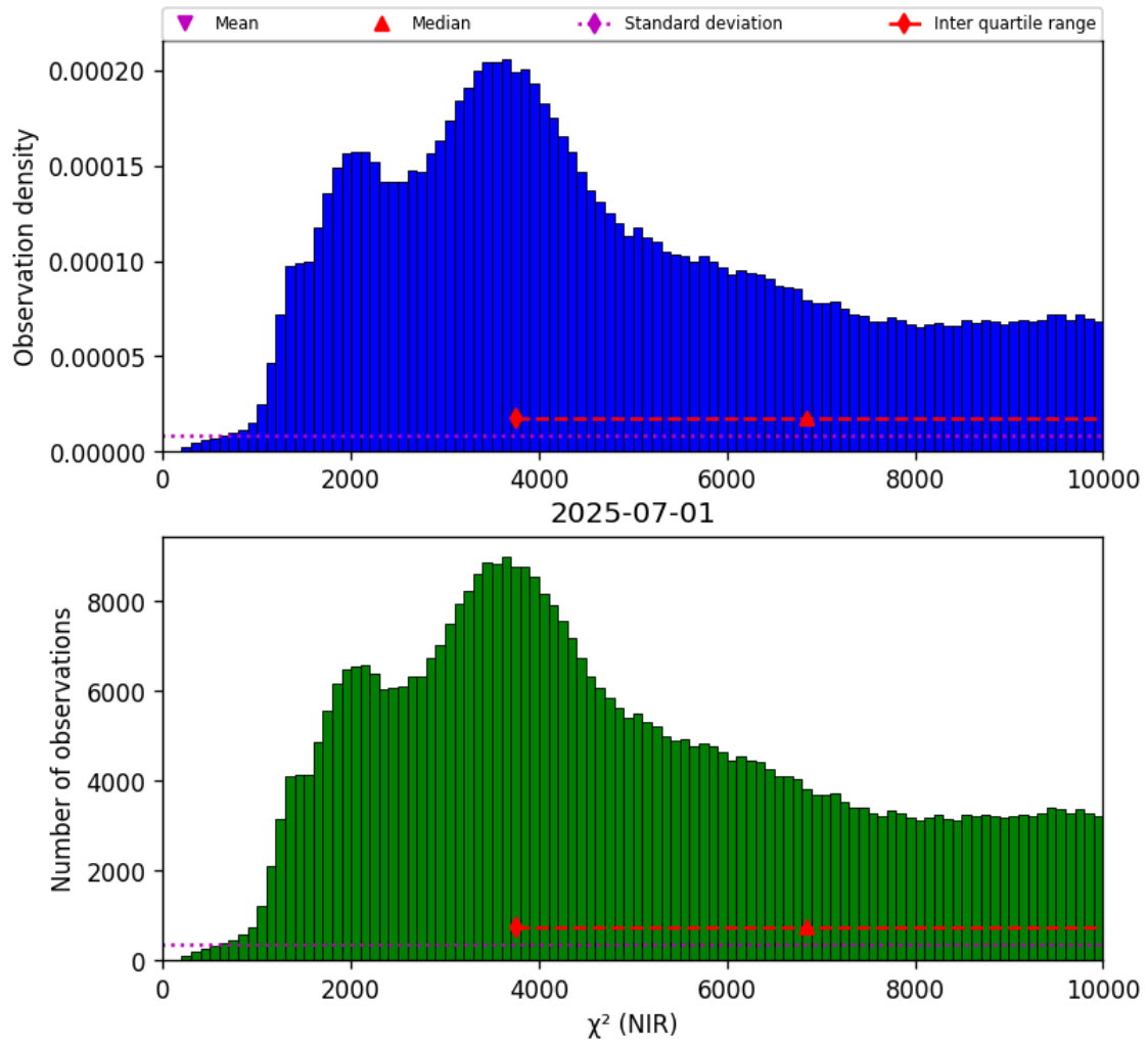
Figure 29: Histogram of “ \chi^2 (NIR)” for 2025-06-30 to 2025-07-02
