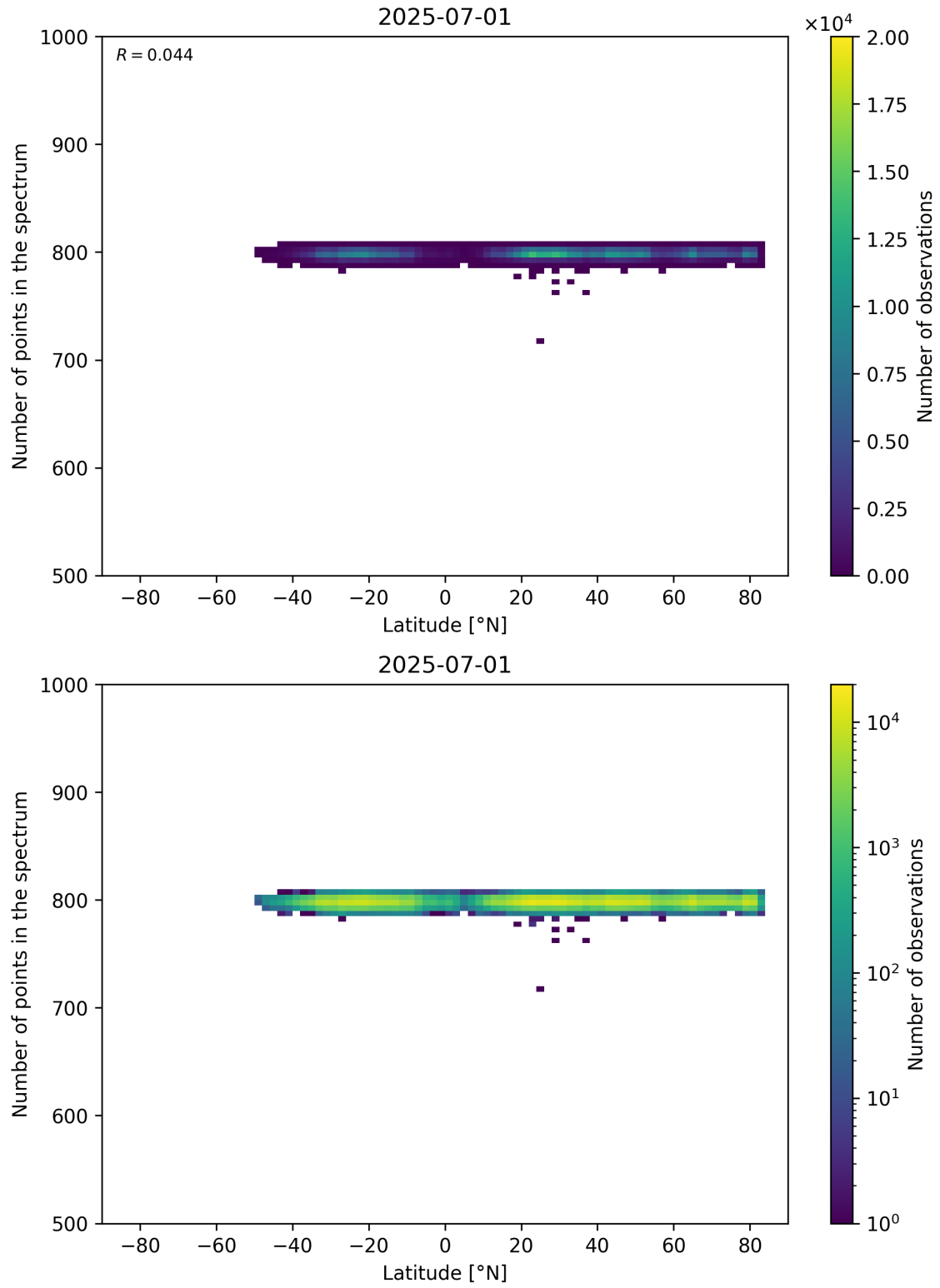
Figure 61: Scatter density plot of “Latitude” against “Number of points in the spectrum” for 2025-06-30 to 2025-07-02.
