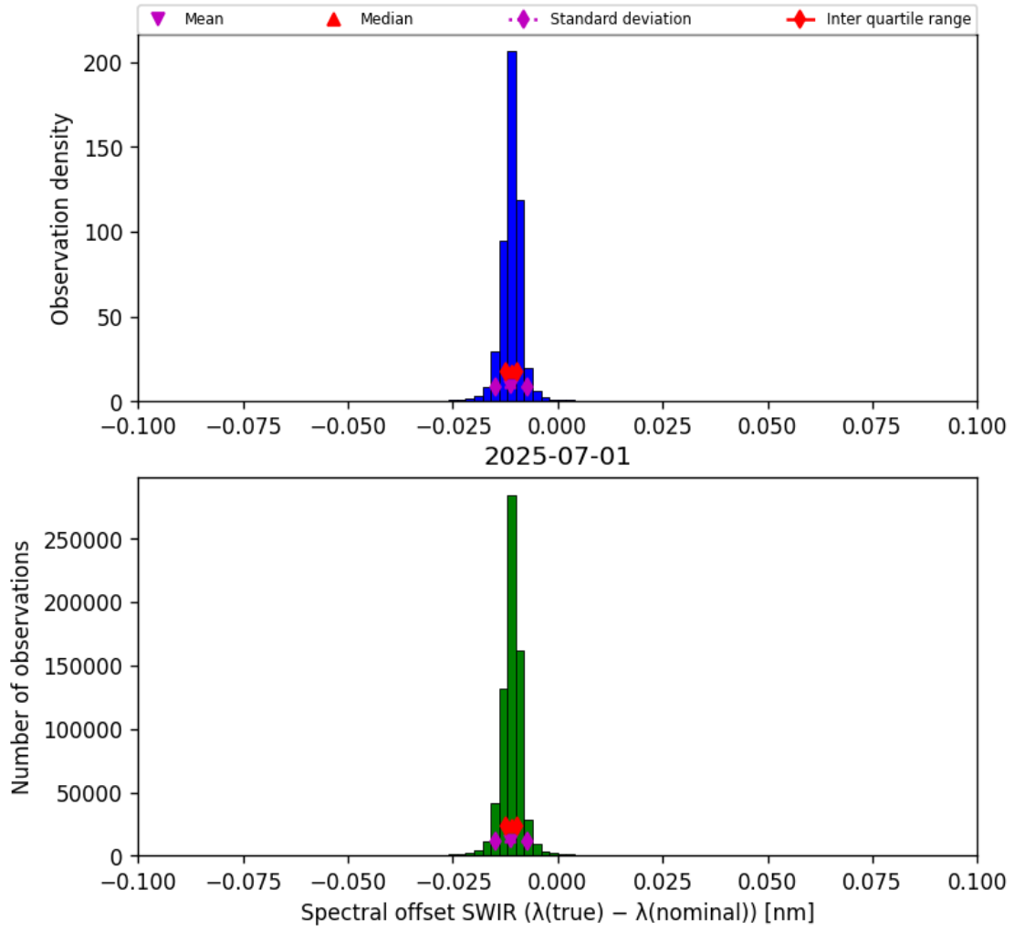
Figure 27: Histogram of “Spectral offset SWIR ( \lambda_{\text{true}} - \lambda_{\text{nominal}} )” for 2025-06-30 to 2025-07-02
