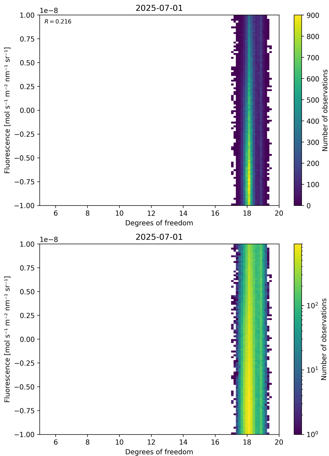
Figure 51: Scatter density plot of “Degrees of freedom” against “Fluorescence” for 2025-06-30 to 2025-07-02.
