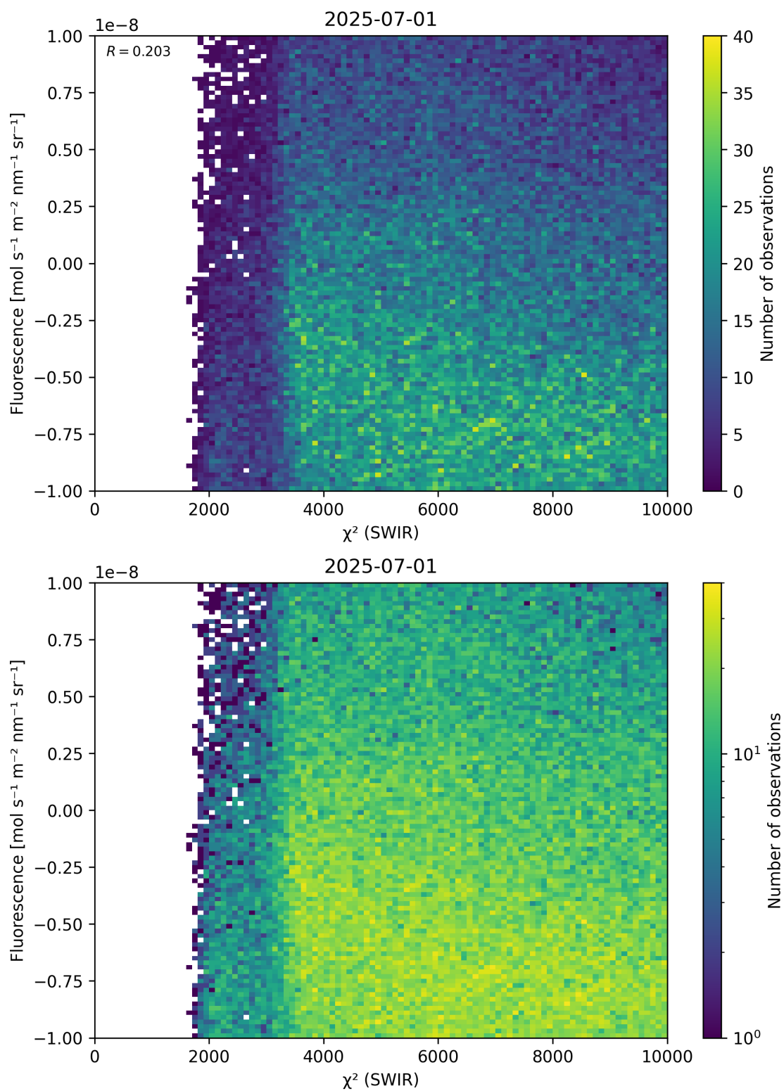
Figure 49: Scatter density plot of “ \chi^2 (SWIR)” against “Fluorescence” for 2025-06-30 to 2025-07-02.
