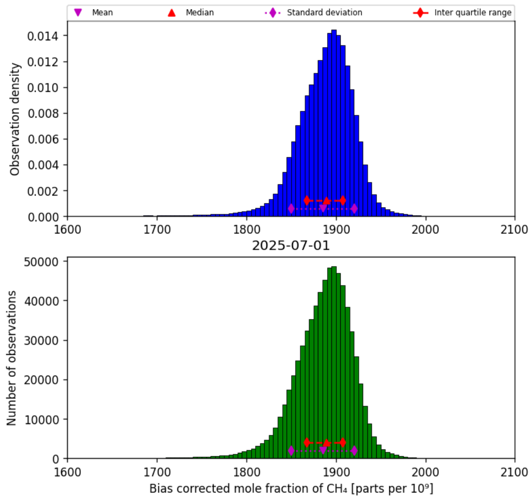
Figure 25: Histogram of “Bias corrected mole fraction of CH 4 ” for 2025-06-30 to 2025-07-02
