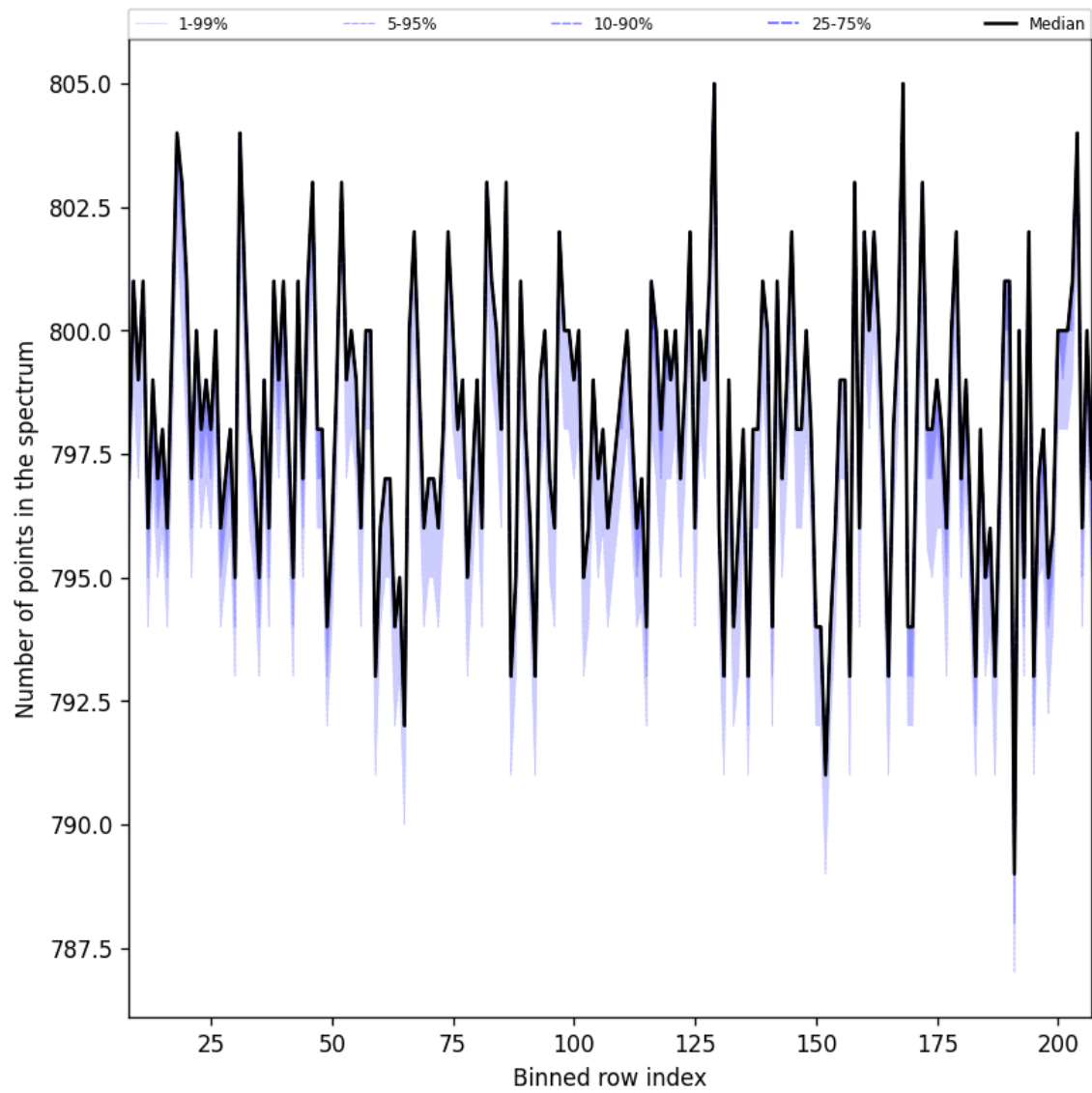
Figure 37: Along track statistics of “Number of points in the spectrum” for 2025-06-30 to 2025-07-02
