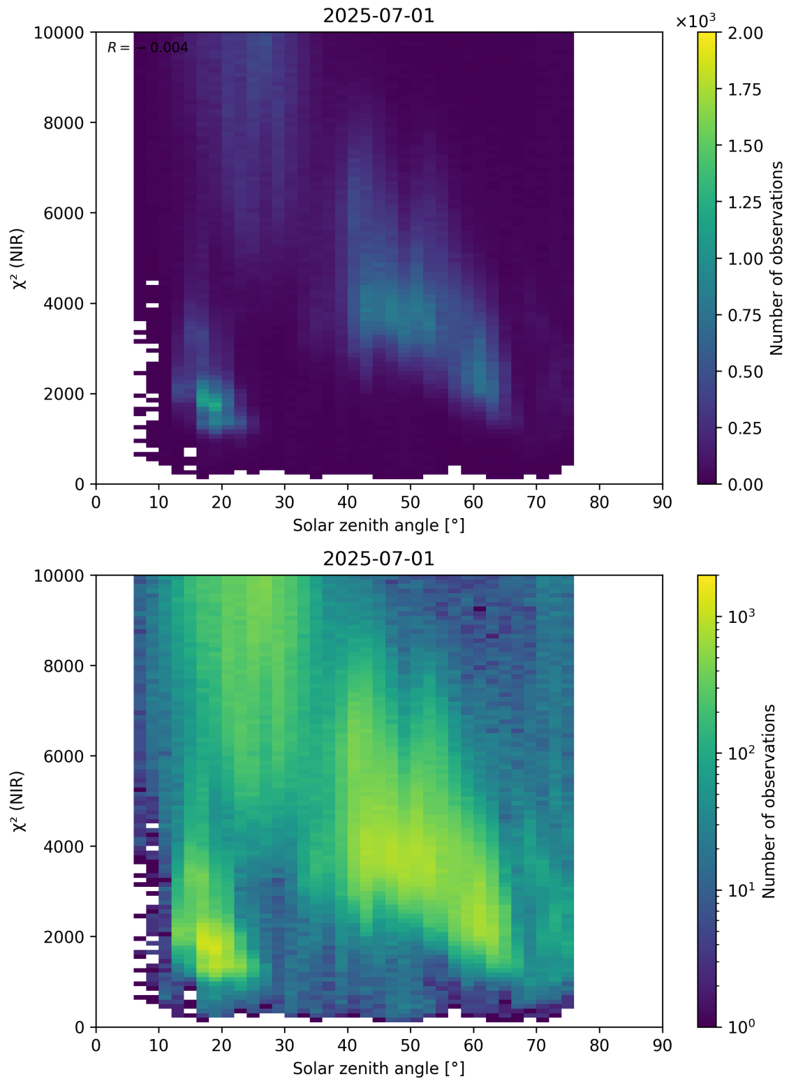
Figure 94: Scatter density plot of “Solar zenith angle” against “ \chi^2 (NIR)” for 2025-06-30 to 2025-07-02.
