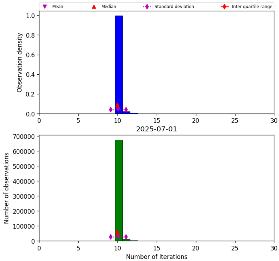
Figure 31: Histogram of “Number of iterations” for 2025-06-30 to 2025-07-02
