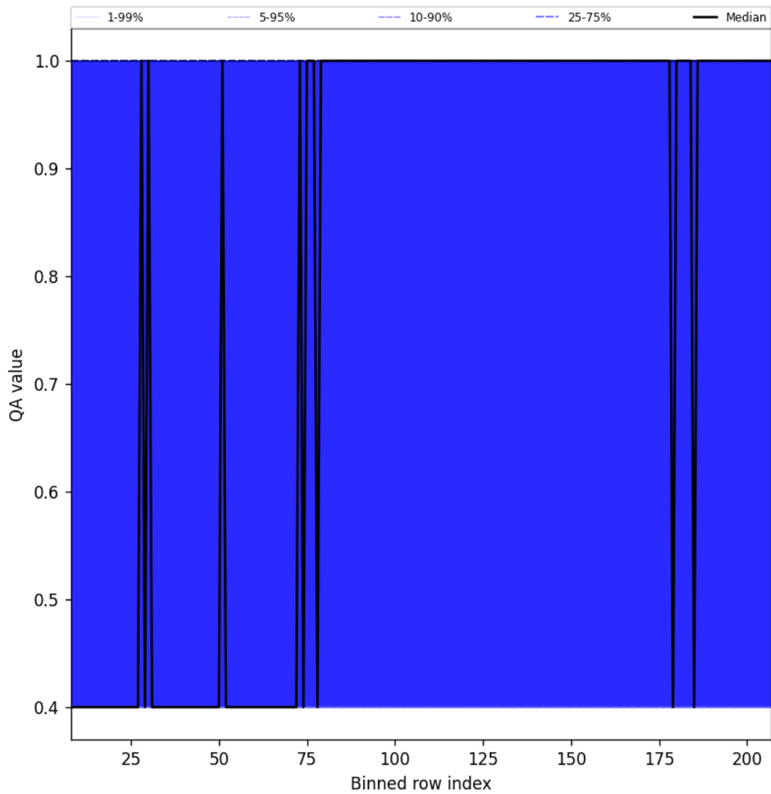
Figure 33: Along track statistics of “QA value” for 2025-06-30 to 2025-07-02
