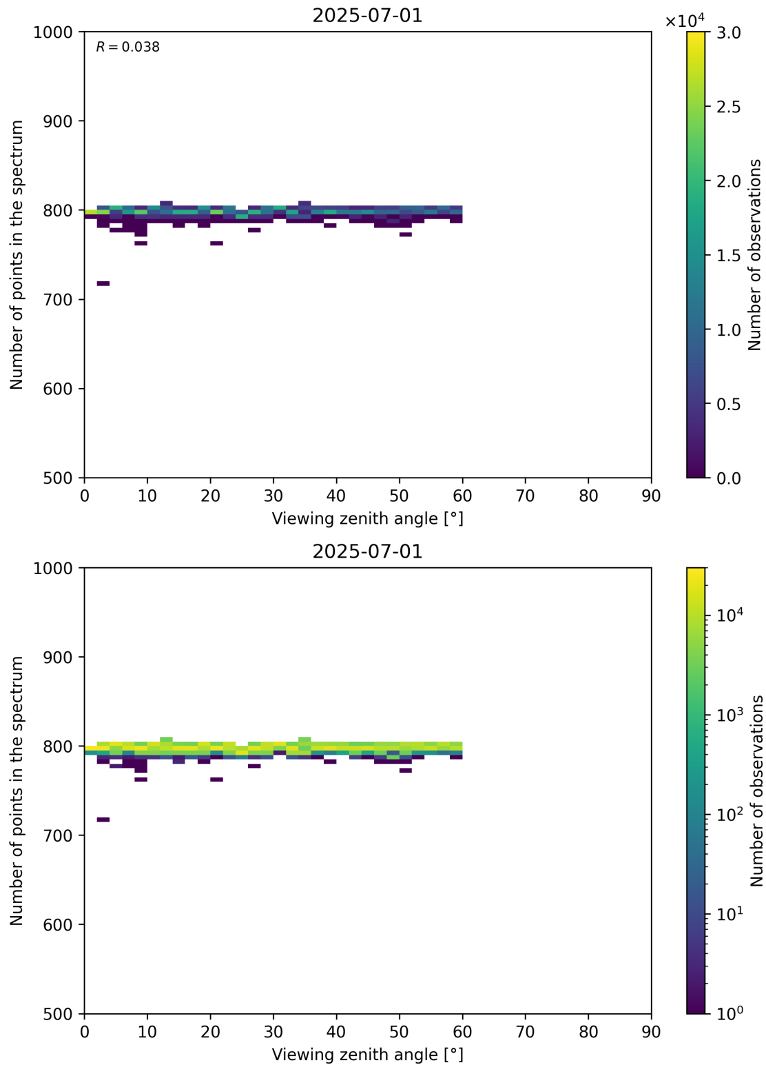
Figure 114: Scatter density plot of “Viewing zenith angle” against “Number of points in the spectrum” for 2025-06-30 to 2025-07-02.
