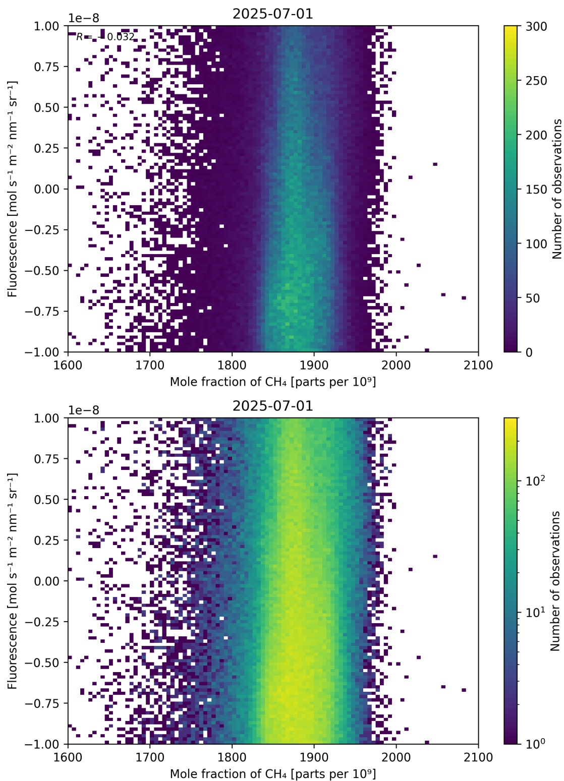
Figure 73: Scatter density plot of “Mole fraction of CH 4 ” against “Fluorescence” for 2025-06-30 to 2025-07-02.
