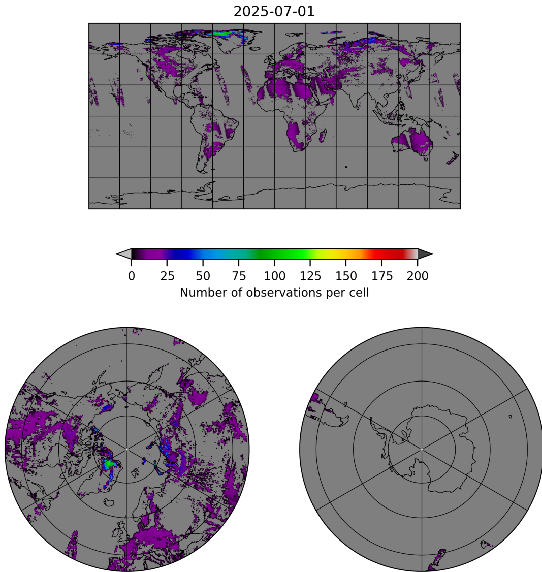
Figure 10: Map of the number of observations for 2025-06-30 to 2025-07-02
