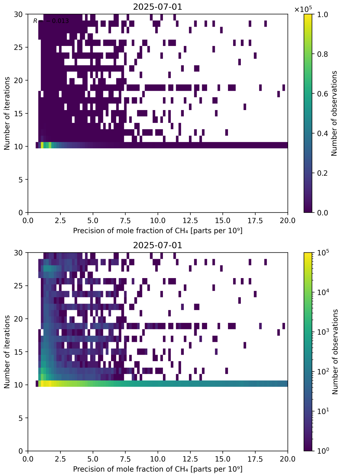
Figure 83: Scatter density plot of “Precision of mole fraction of CH 4 ” against “Number of iterations” for 2025-06-30 to 2025-07-02.
