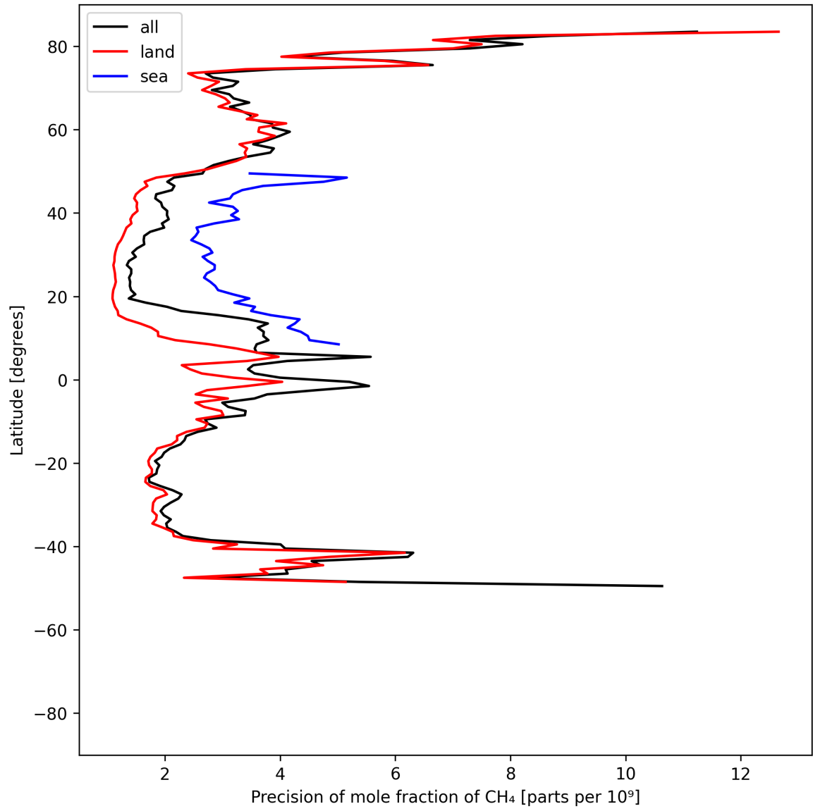
Figure 13: Zonal average of “Precision of mole fraction of CH 4 ” for 2025-06-30 to 2025-07-02.
