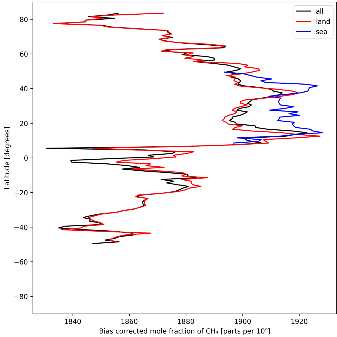
Figure 14: Zonal average of “Bias corrected mole fraction of CH 4 ” for 2025-06-30 to 2025-07-02.
