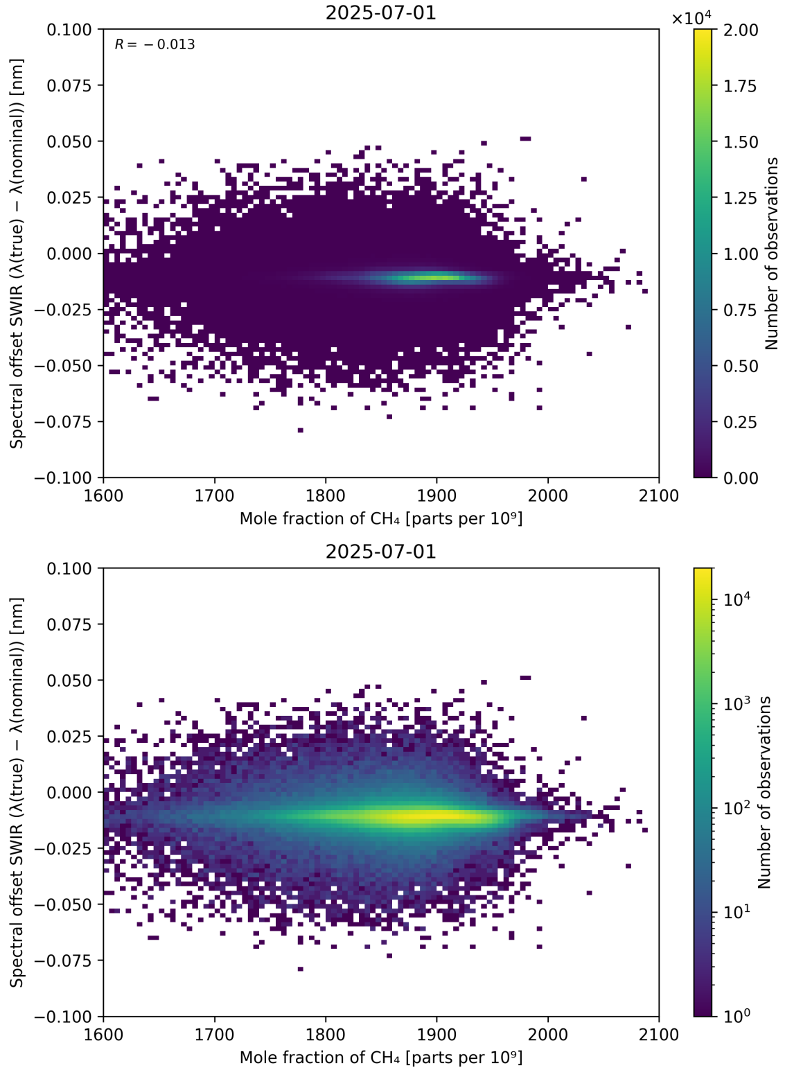
Figure 86: Scatter density plot of “Mole fraction of CH 4 ” against “Spectral offset SWIR ( \lambda_{\text{true}} - \lambda_{\text{nominal}} )” for 2025-06-30 to 2025-07-02.
