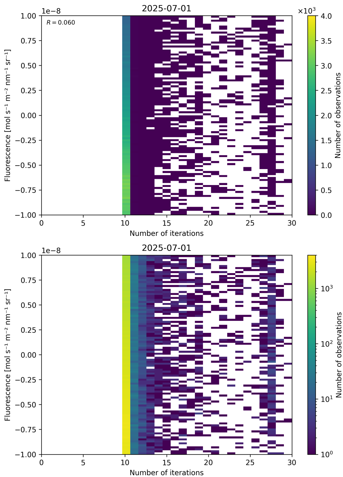
Figure 87: Scatter density plot of “Number of iterations” against “Fluorescence” for 2025-06-30 to 2025-07-02.
