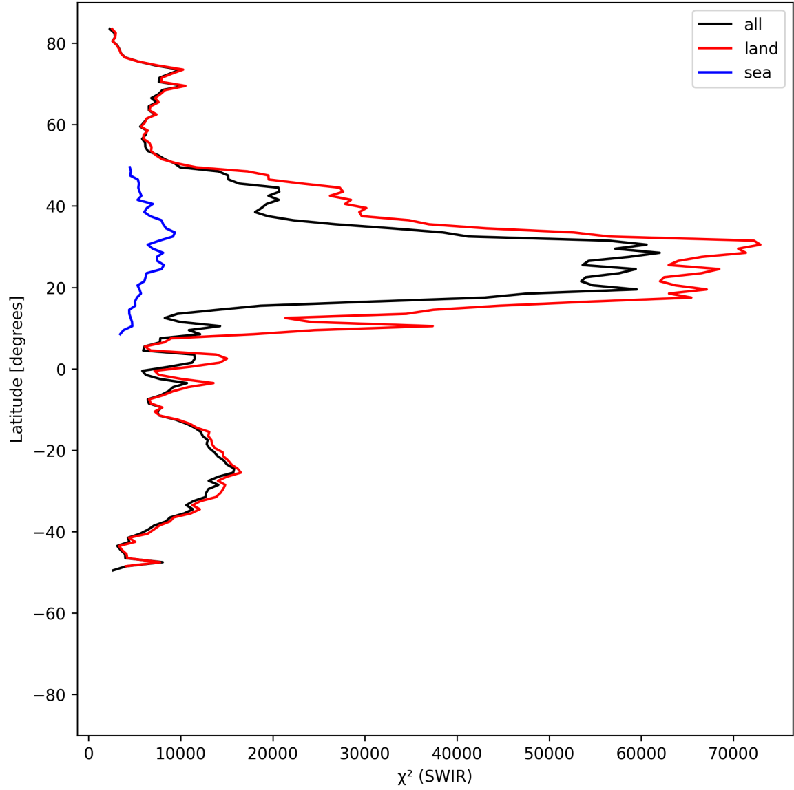
Figure 17: Zonal average of “ \chi^2 (SWIR)” for 2025-06-30 to 2025-07-02.
