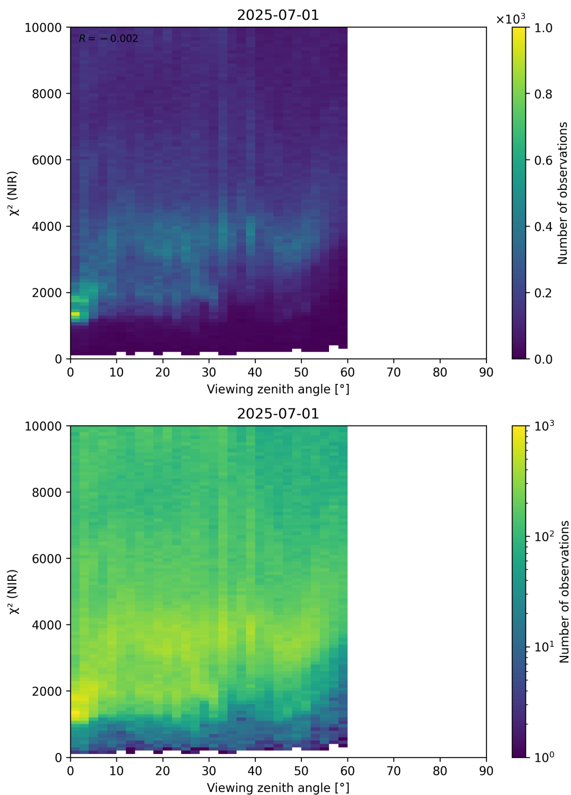
Figure 105: Scatter density plot of “Viewing zenith angle” against “ \chi^2 (NIR)” for 2025-06-30 to 2025-07-02.
