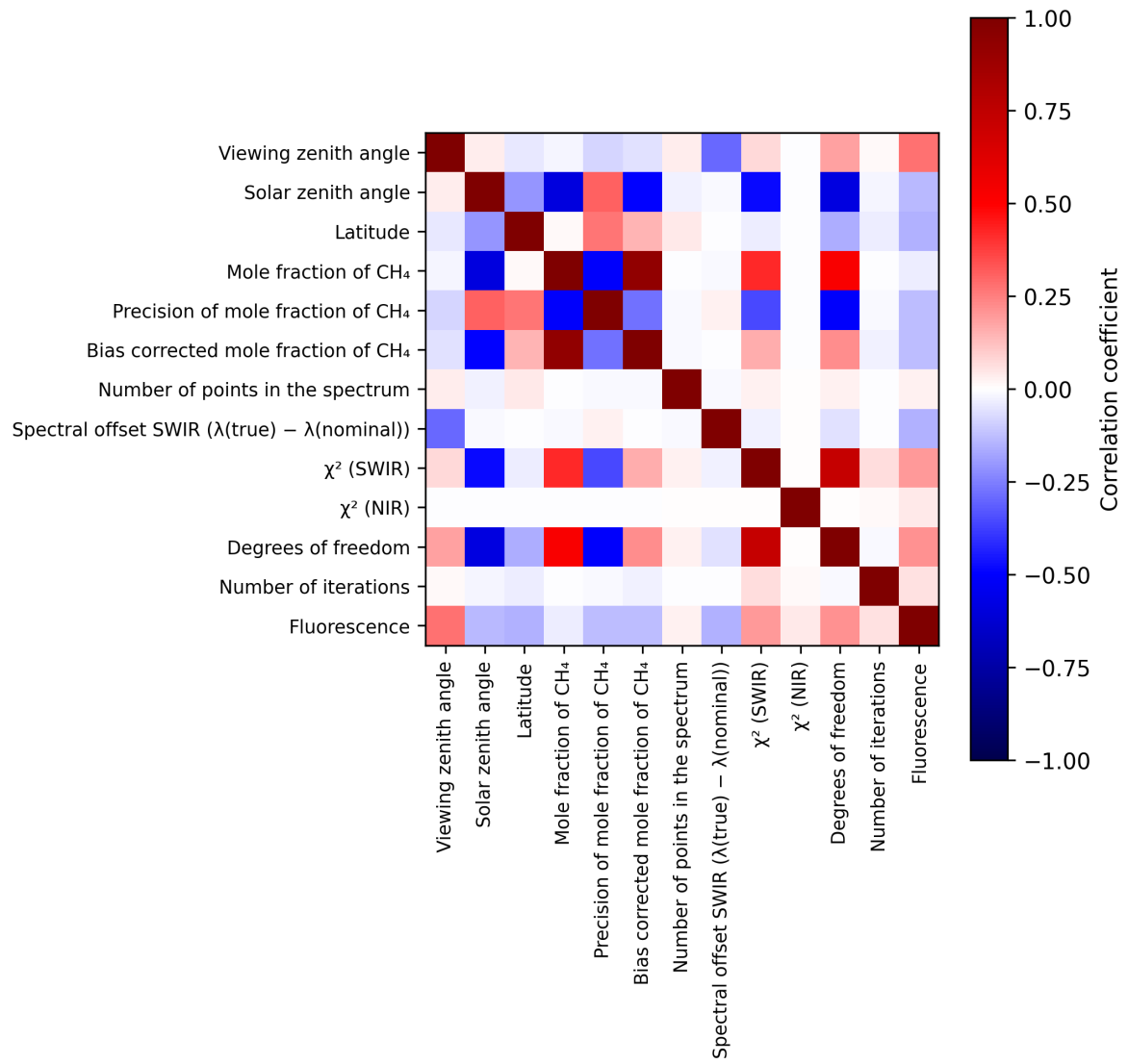
Figure 2: Map of correlation matrix for 2025-06-30 to 2025-07-02.
