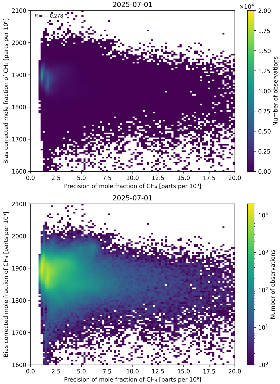
Figure 82: Scatter density plot of “Precision of mole fraction of CH 4 ” against “Bias corrected mole fraction of CH 4 ” for 2025-06-30 to 2025-07-02.
