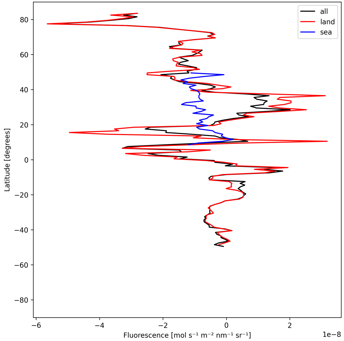
Figure 21: Zonal average of “Fluorescence” for 2025-06-30 to 2025-07-02.
