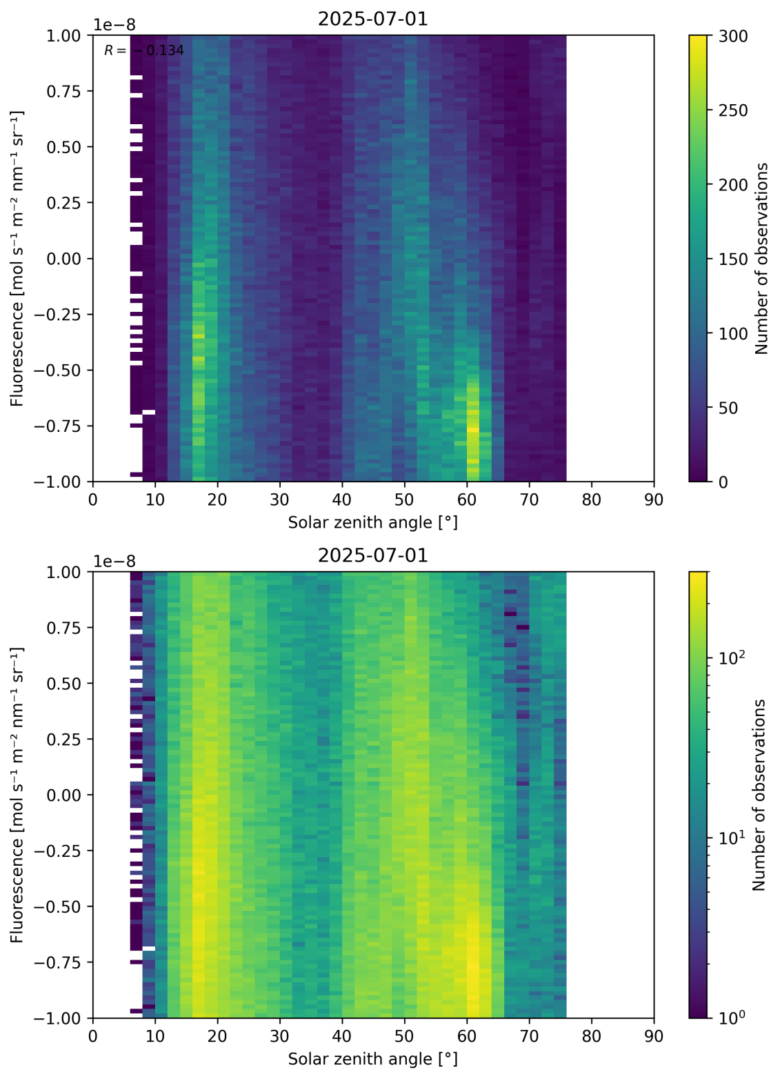
Figure 97: Scatter density plot of “Solar zenith angle” against “Fluorescence” for 2025-06-30 to 2025-07-02.
