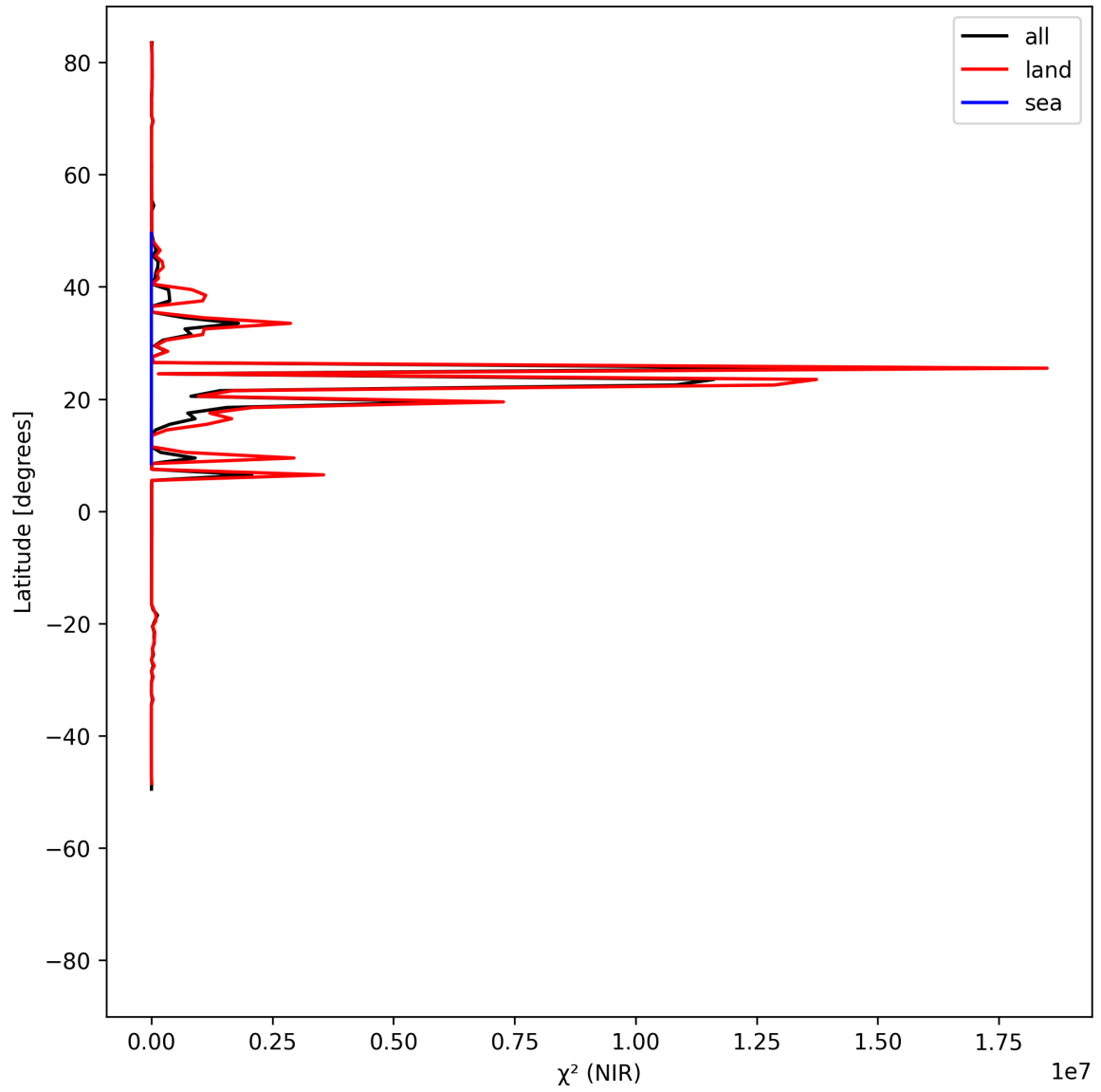
Figure 18: Zonal average of “ \chi^2 (NIR)” for 2025-06-30 to 2025-07-02.
