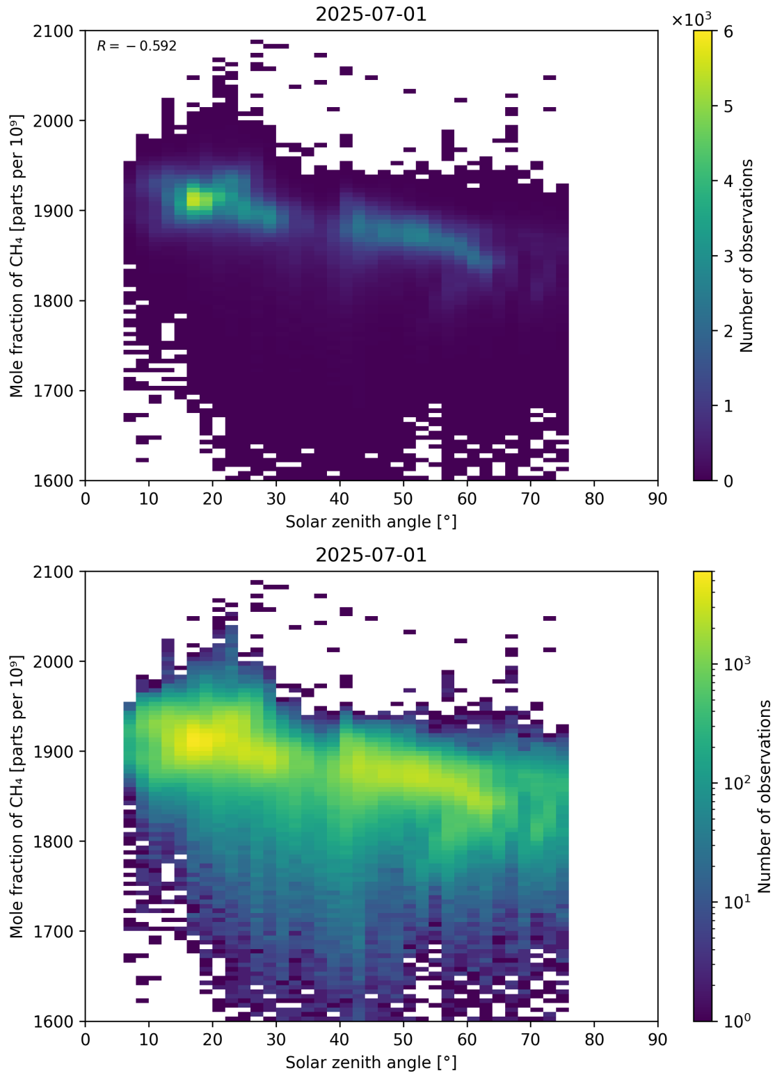
Figure 99: Scatter density plot of “Solar zenith angle” against “Mole fraction of \text{CH}_4 ” for 2025-06-30 to 2025-07-02.
