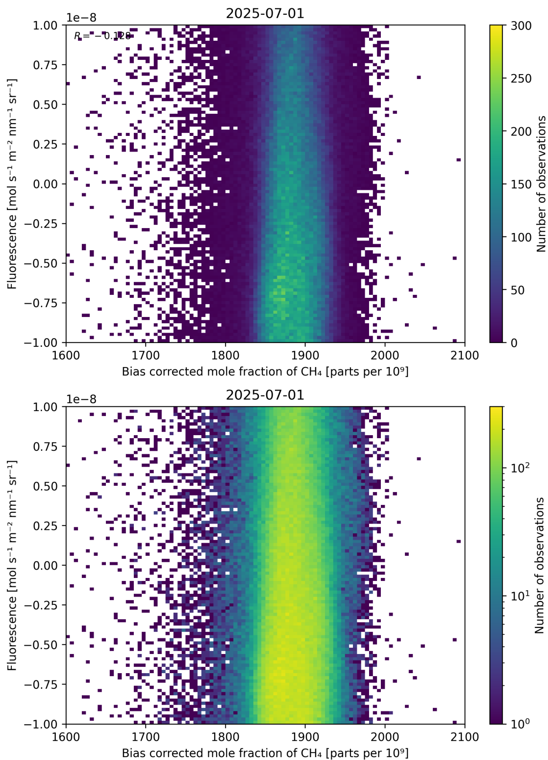
Figure 66: Scatter density plot of “Bias corrected mole fraction of CH 4 ” against “Fluorescence” for 2025-06-30 to 2025-07-02.
