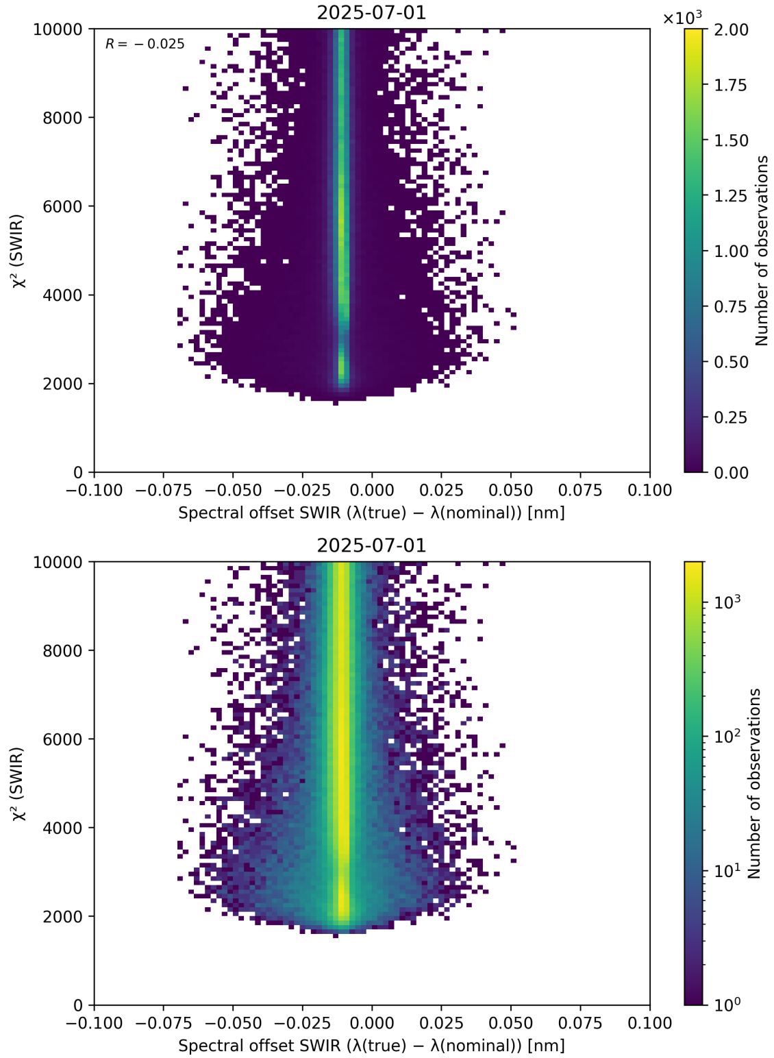
Figure 118: Scatter density plot of “Spectral offset SWIR ( \lambda_{\text{true}} - \lambda_{\text{nominal}} )” against “ \chi^2 (SWIR)” for 2025-06-30 to 2025-07-02.
