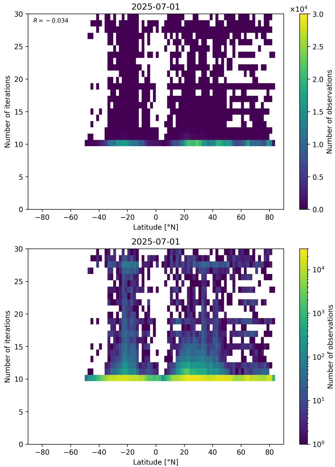
Figure 60: Scatter density plot of “Latitude” against “Number of iterations” for 2025-06-30 to 2025-07-02.
