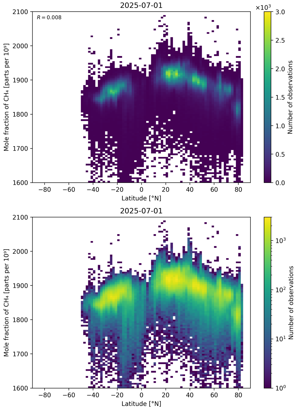
Figure 57: Scatter density plot of “Latitude” against “Mole fraction of CH 4 ” for 2025-06-30 to 2025-07-02.
