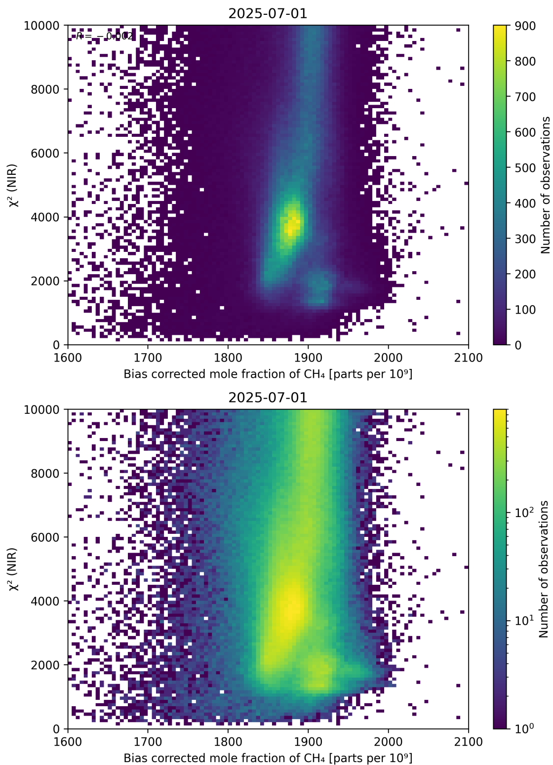
Figure 63: Scatter density plot of “Bias corrected mole fraction of CH 4 ” against “ \chi^2 (NIR)” for 2025-06-30 to 2025-07-02.
