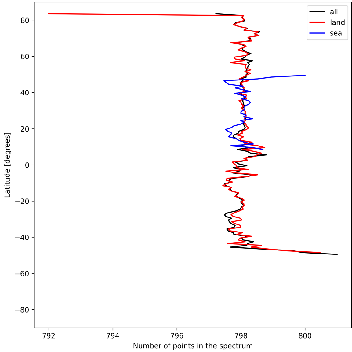
Figure 15: Zonal average of “Number of points in the spectrum” for 2025-06-30 to 2025-07-02.
