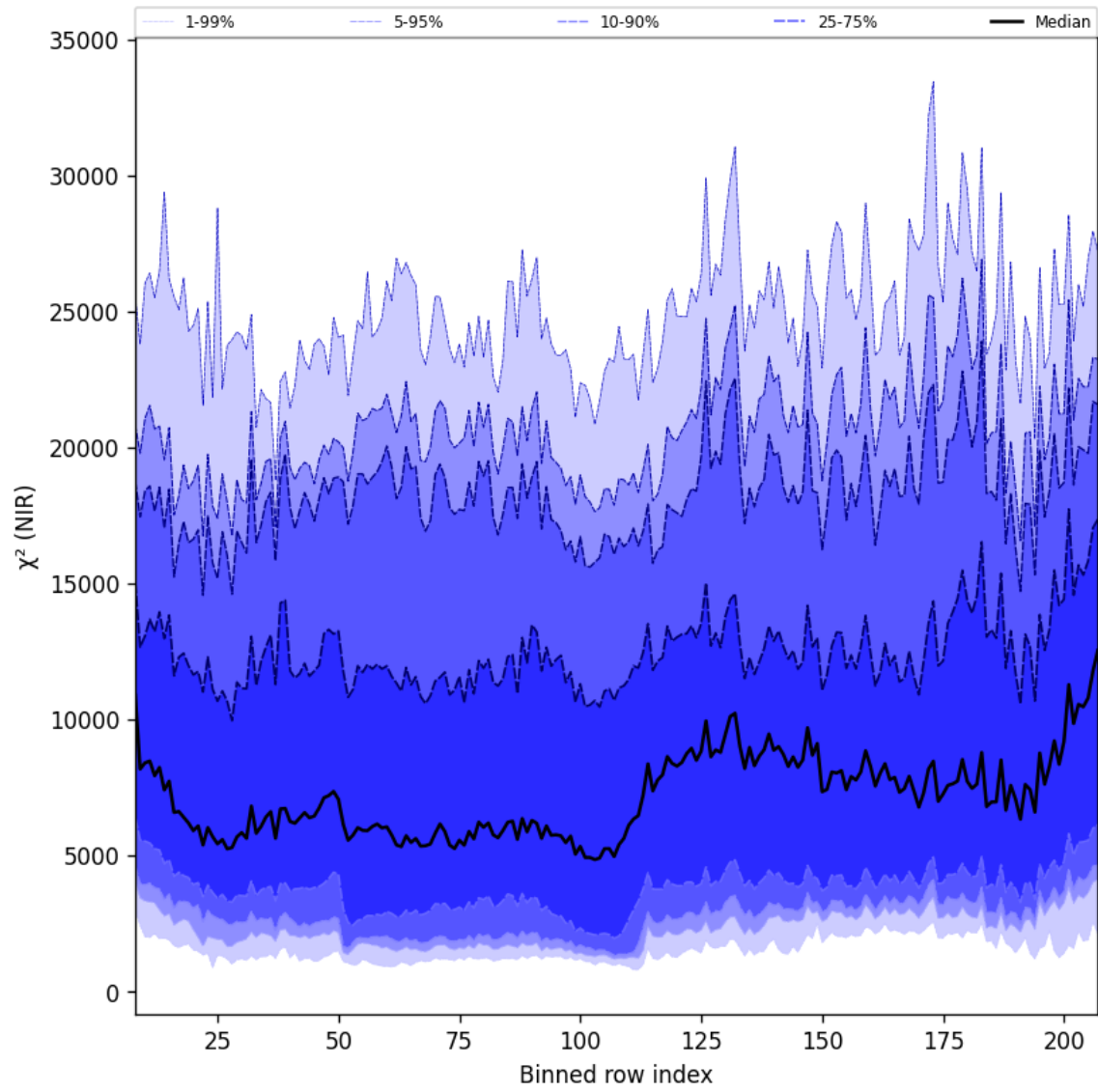
Figure 40: Along track statistics of “ \chi^2 (NIR)” for 2025-06-30 to 2025-07-02
