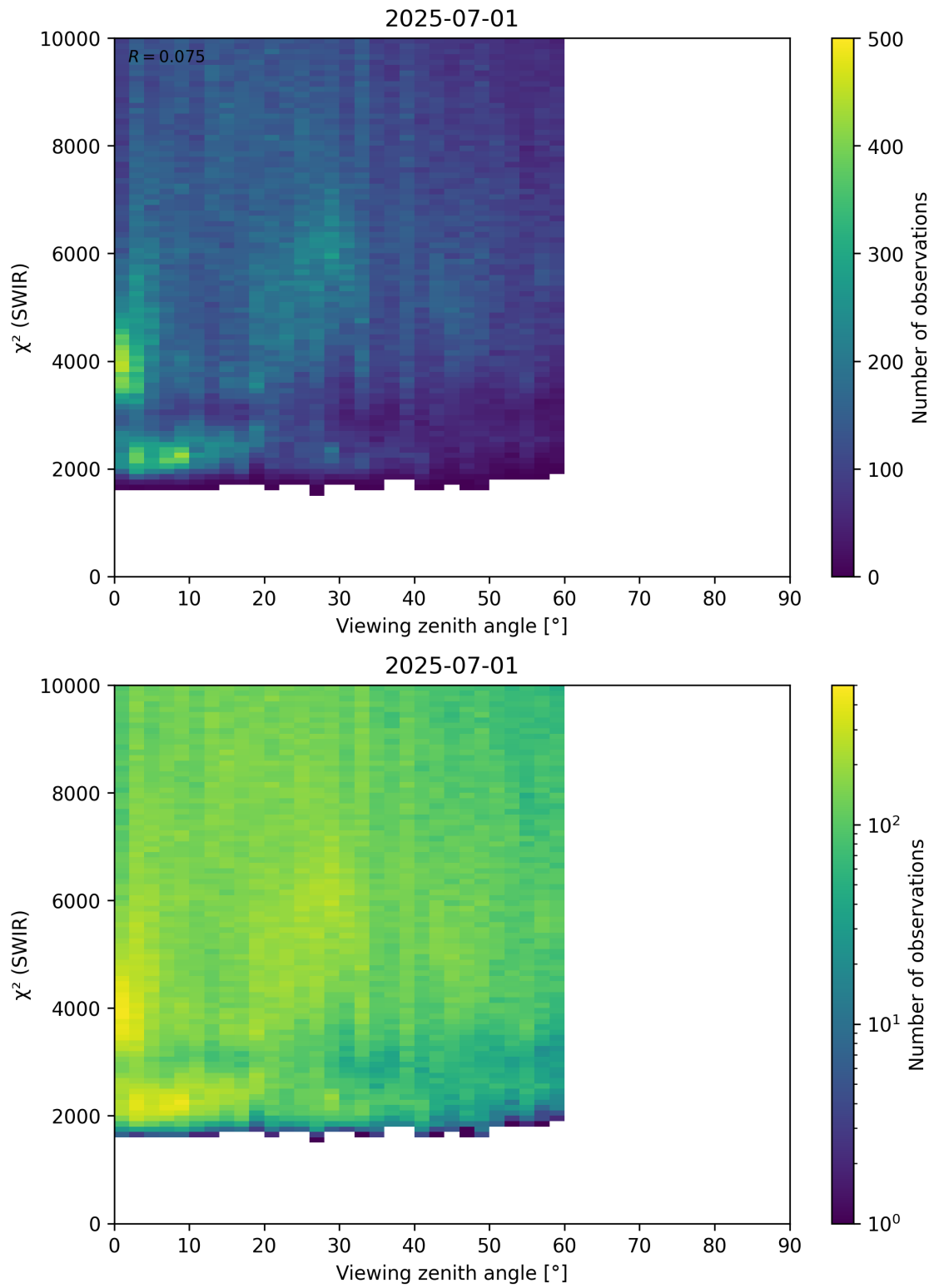
Figure 106: Scatter density plot of “Viewing zenith angle” against “ \chi^2 (SWIR)” for 2025-06-30 to 2025-07-02.
