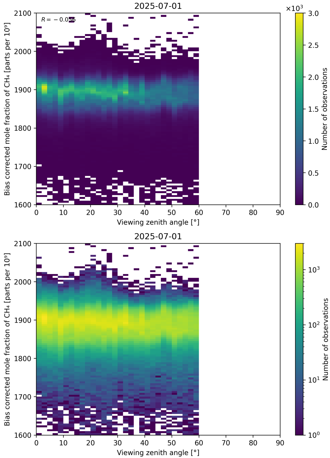
Figure 111: Scatter density plot of “Viewing zenith angle” against “Bias corrected mole fraction of CH 4 ” for 2025-06-30 to 2025-07-02.
