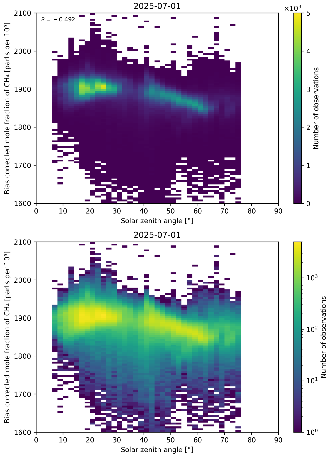
Figure 100: Scatter density plot of “Solar zenith angle” against “Bias corrected mole fraction of CH 4 ” for 2025-06-30 to 2025-07-02.
