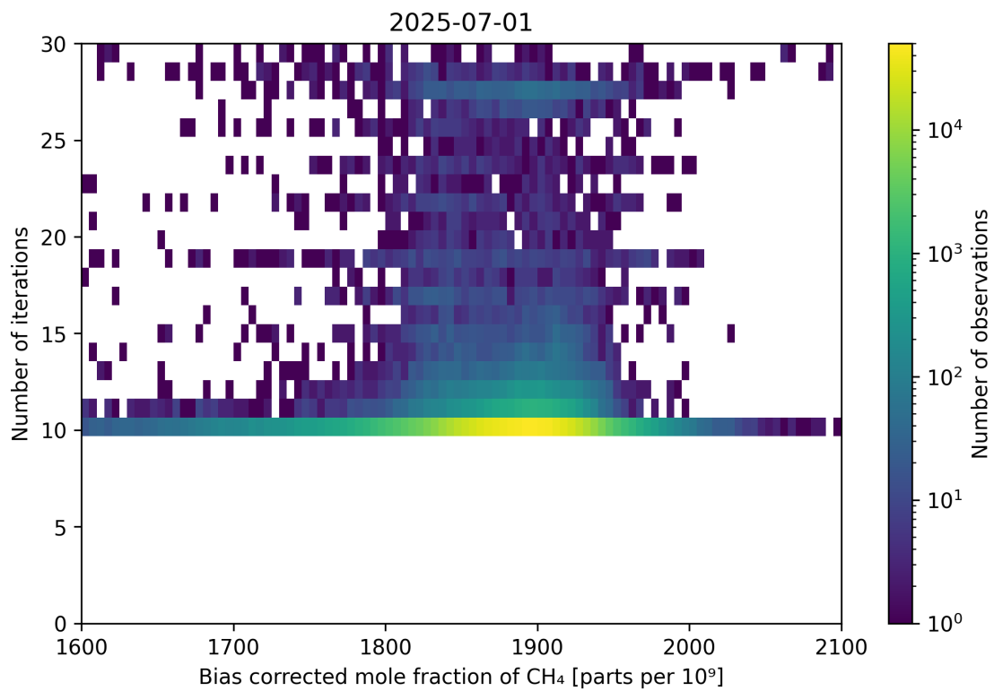
Figure 67: Scatter density plot of “Bias corrected mole fraction of CH 4 ” against “Number of iterations” for 2025-06-30 to 2025-07-02.
