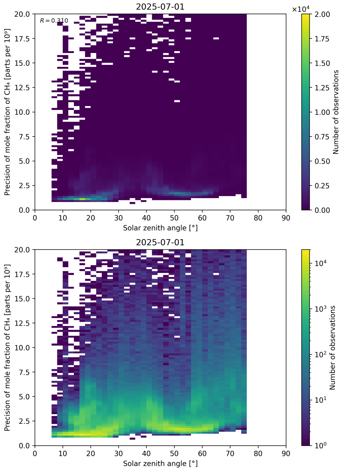
Figure 101: Scatter density plot of “Solar zenith angle” against “Precision of mole fraction of CH 4 ” for 2025-06-30 to 2025-07-02.
