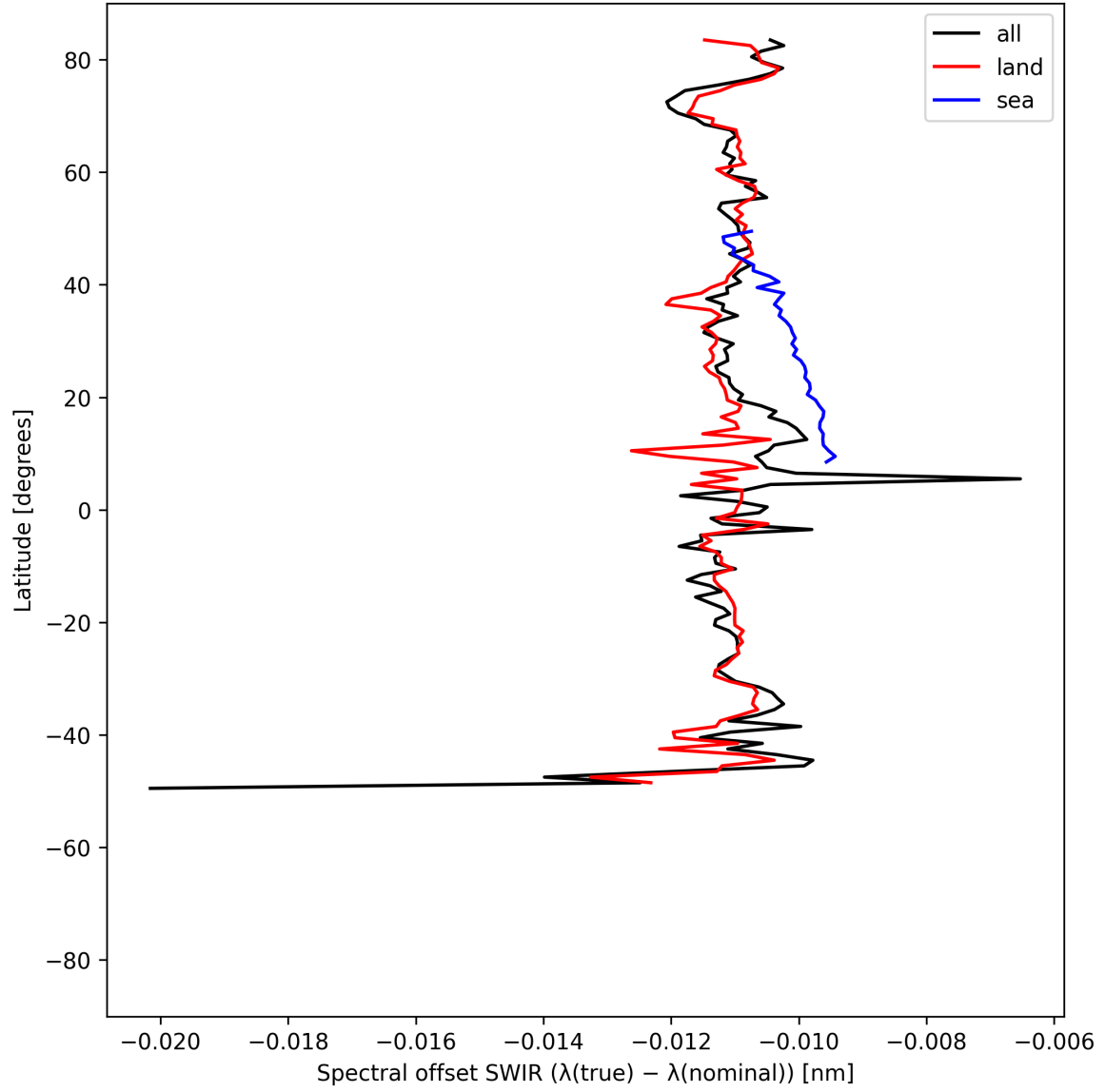
Figure 16: Zonal average of “Spectral offset SWIR ( \lambda_{\text{true}} - \lambda_{\text{nominal}} )” for 2025-06-30 to 2025-07-02.
