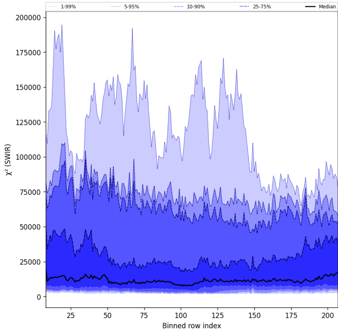
Figure 39: Along track statistics of “ \chi^2 (SWIR)” for 2025-06-30 to 2025-07-02
