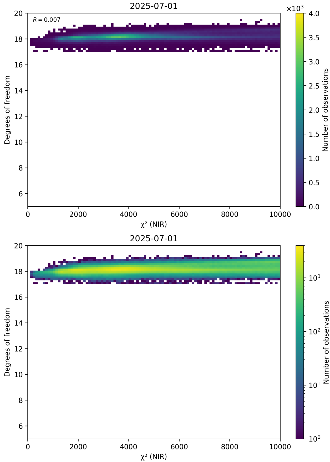
Figure 44: Scatter density plot of “ \chi^2 (NIR)” against “Degrees of freedom” for 2025-06-30 to 2025-07-02.
