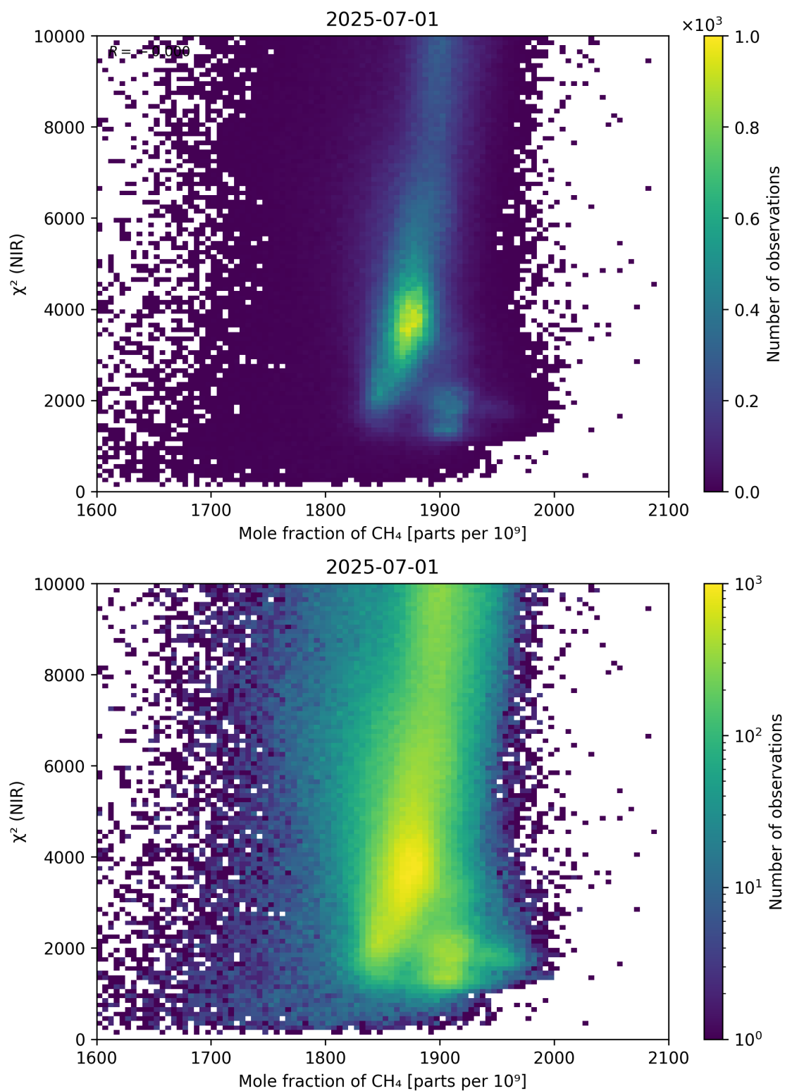
Figure 70: Scatter density plot of “Mole fraction of \text{CH}_4 ” against “ \chi^2 (NIR)” for 2025-06-30 to 2025-07-02.
