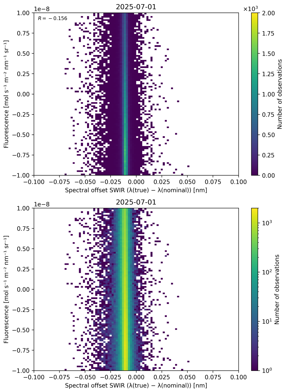
Figure 120: Scatter density plot of “Spectral offset SWIR ( \lambda_{\text{true}} - \lambda_{\text{nominal}} )” against “Fluorescence” for 2025-06-30 to 2025-07-02.
