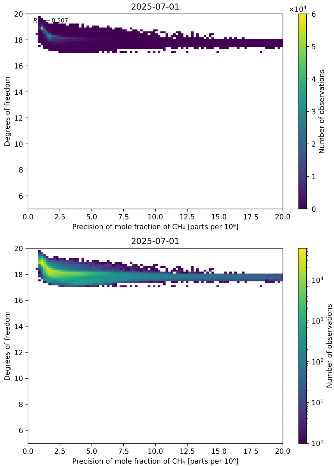
Figure 80: Scatter density plot of “Precision of mole fraction of CH 4 ” against “Degrees of freedom” for 2025-06-30 to 2025-07-02.
