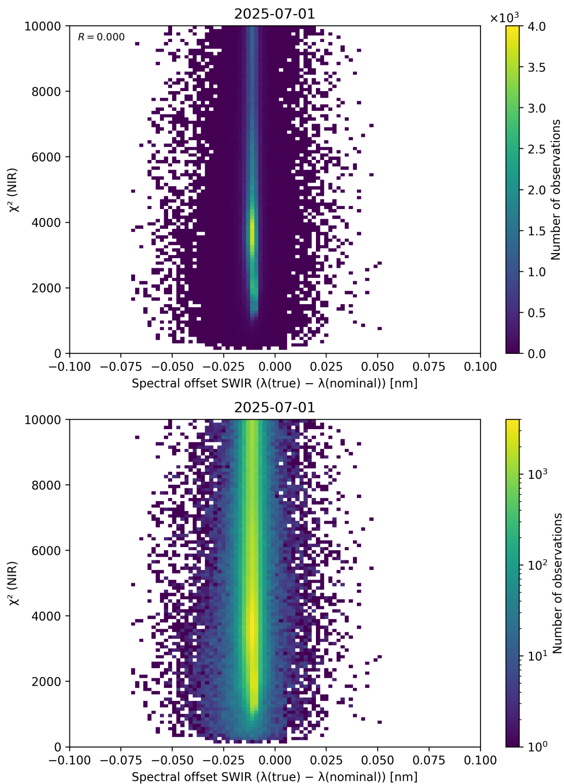
Figure 117: Scatter density plot of “Spectral offset SWIR ( \lambda_{\text{true}} - \lambda_{\text{nominal}} )” against “ \chi^2 (NIR)” for 2025-06-30 to 2025-07-02.
