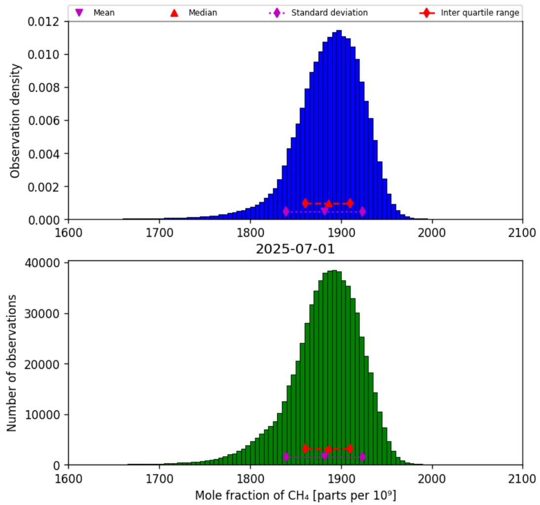
Figure 23: Histogram of “Mole fraction of CH 4 ” for 2025-06-30 to 2025-07-02
