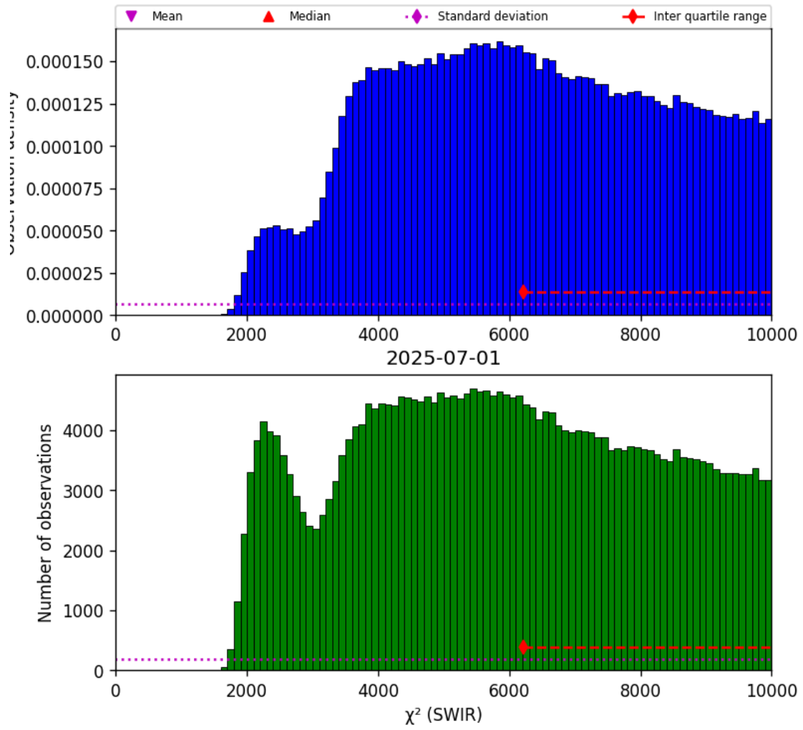
Figure 28: Histogram of “ \chi^2 (SWIR)” for 2025-06-30 to 2025-07-02
