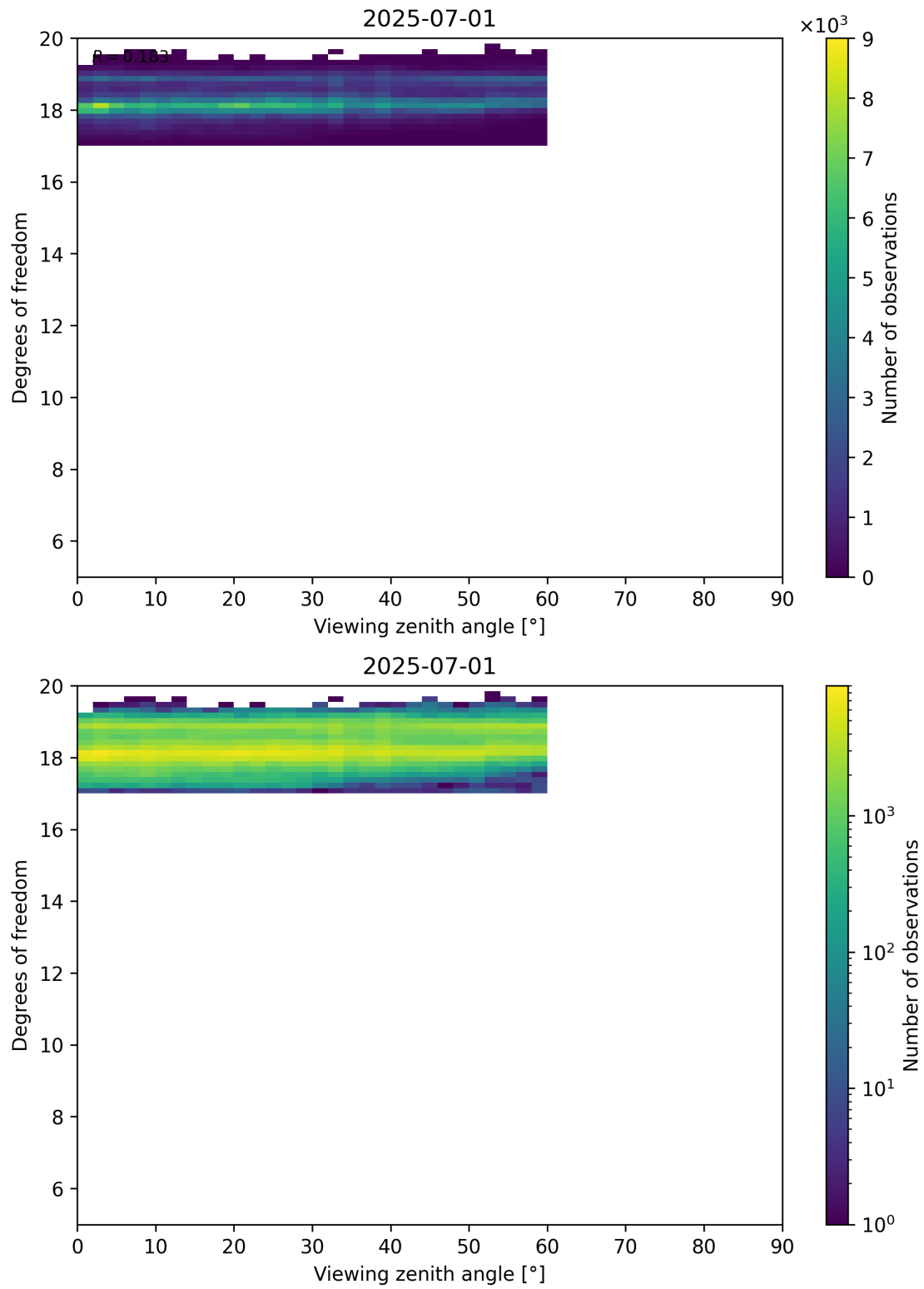
Figure 107: Scatter density plot of “Viewing zenith angle” against “Degrees of freedom” for 2025-06-30 to 2025-07-02.
