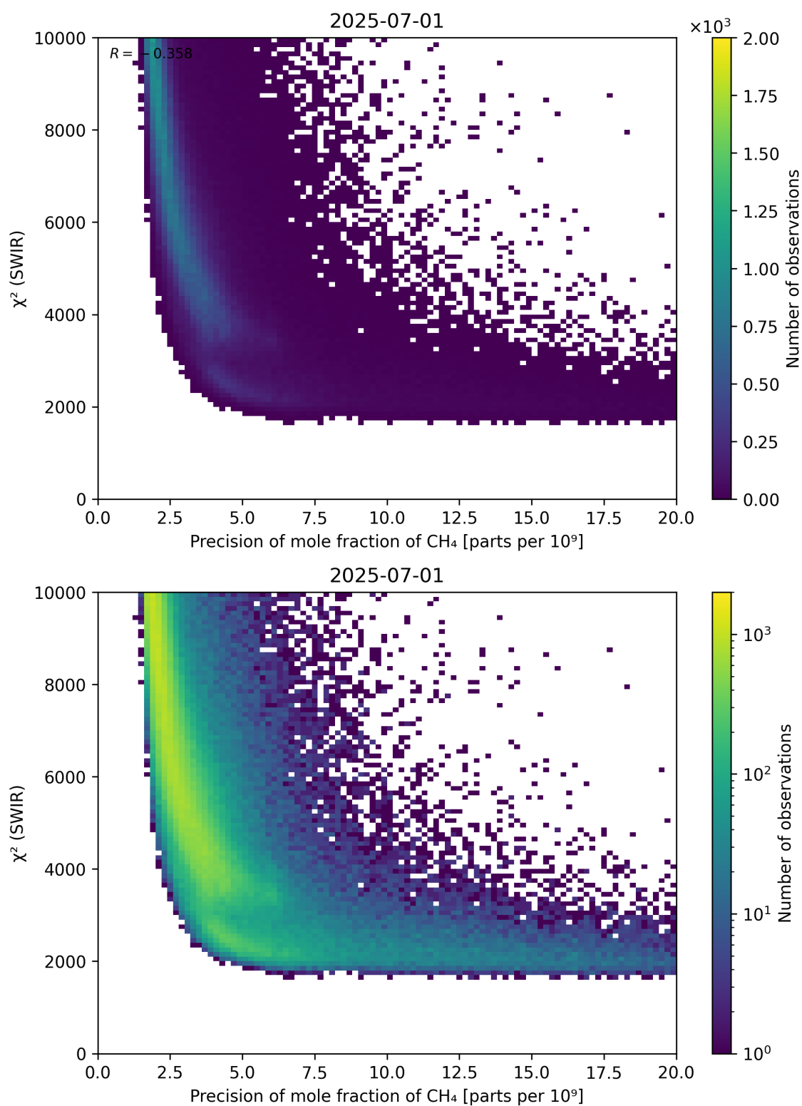
Figure 79: Scatter density plot of “Precision of mole fraction of \text{CH}_4 ” against “ \chi^2 (SWIR)” for 2025-06-30 to 2025-07-02.
