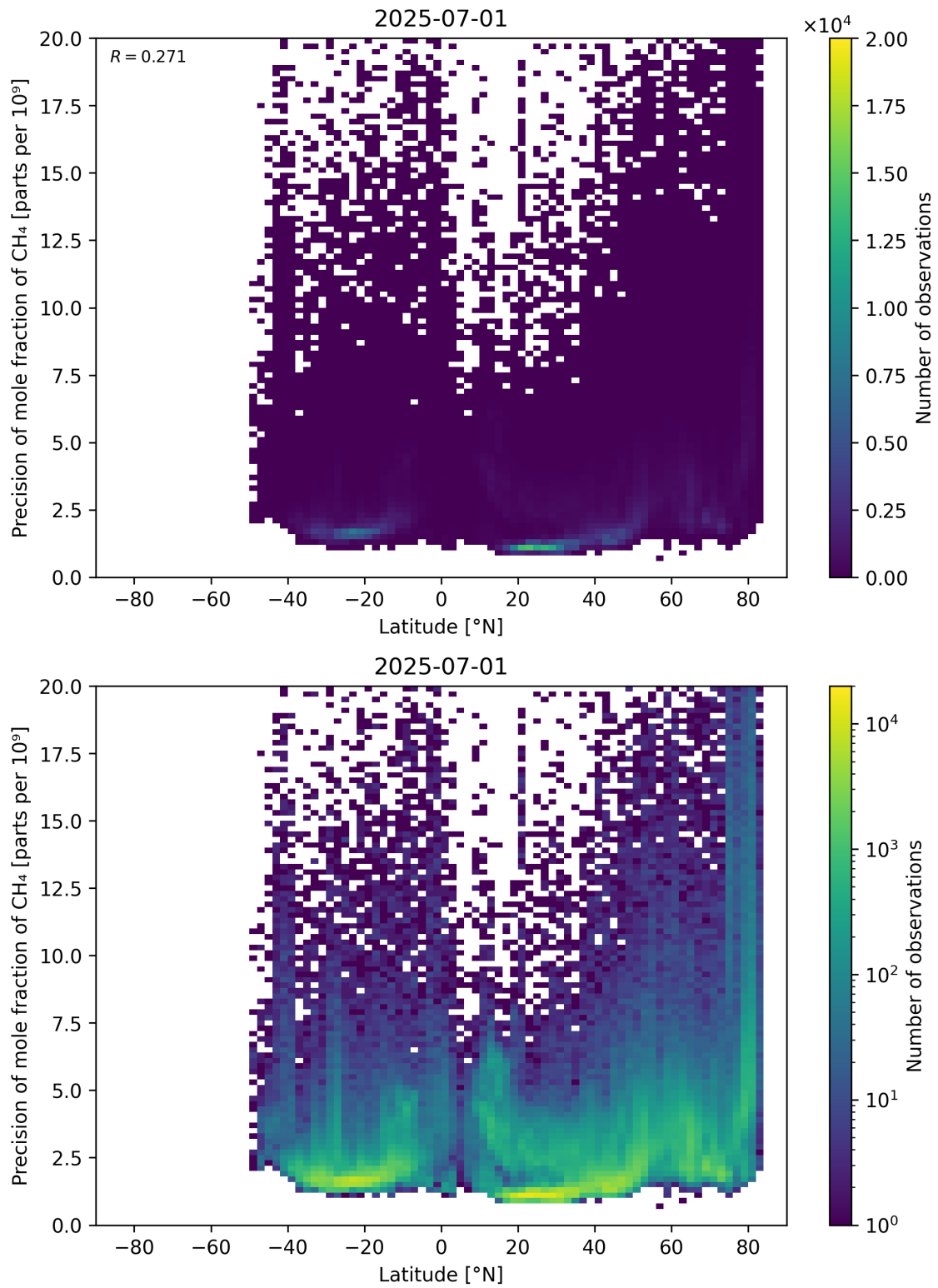
Figure 59: Scatter density plot of “Latitude” against “Precision of mole fraction of \text{CH}_4 ” for 2025-06-30 to 2025-07-02.
