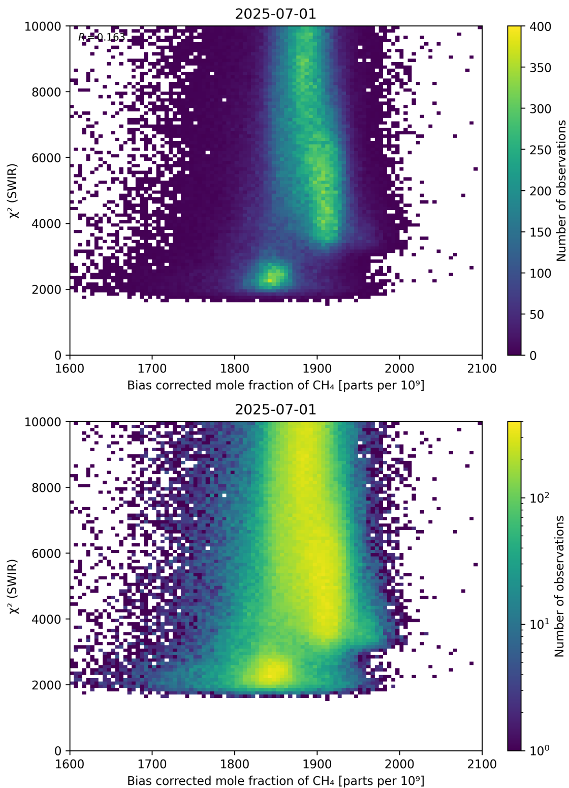
Figure 64: Scatter density plot of “Bias corrected mole fraction of \text{CH}_4 ” against “ \chi^2 (SWIR)” for 2025-06-30 to 2025-07-02.
