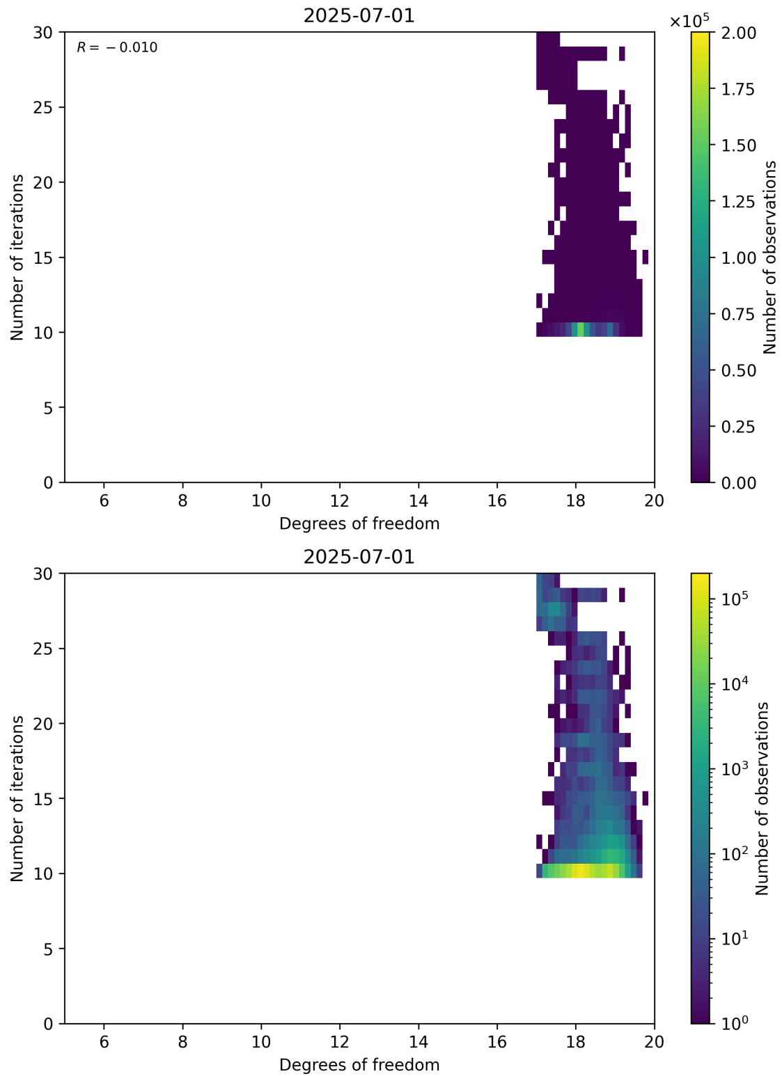
Figure 52: Scatter density plot of “Degrees of freedom” against “Number of iterations” for 2025-06-30 to 2025-07-02.
