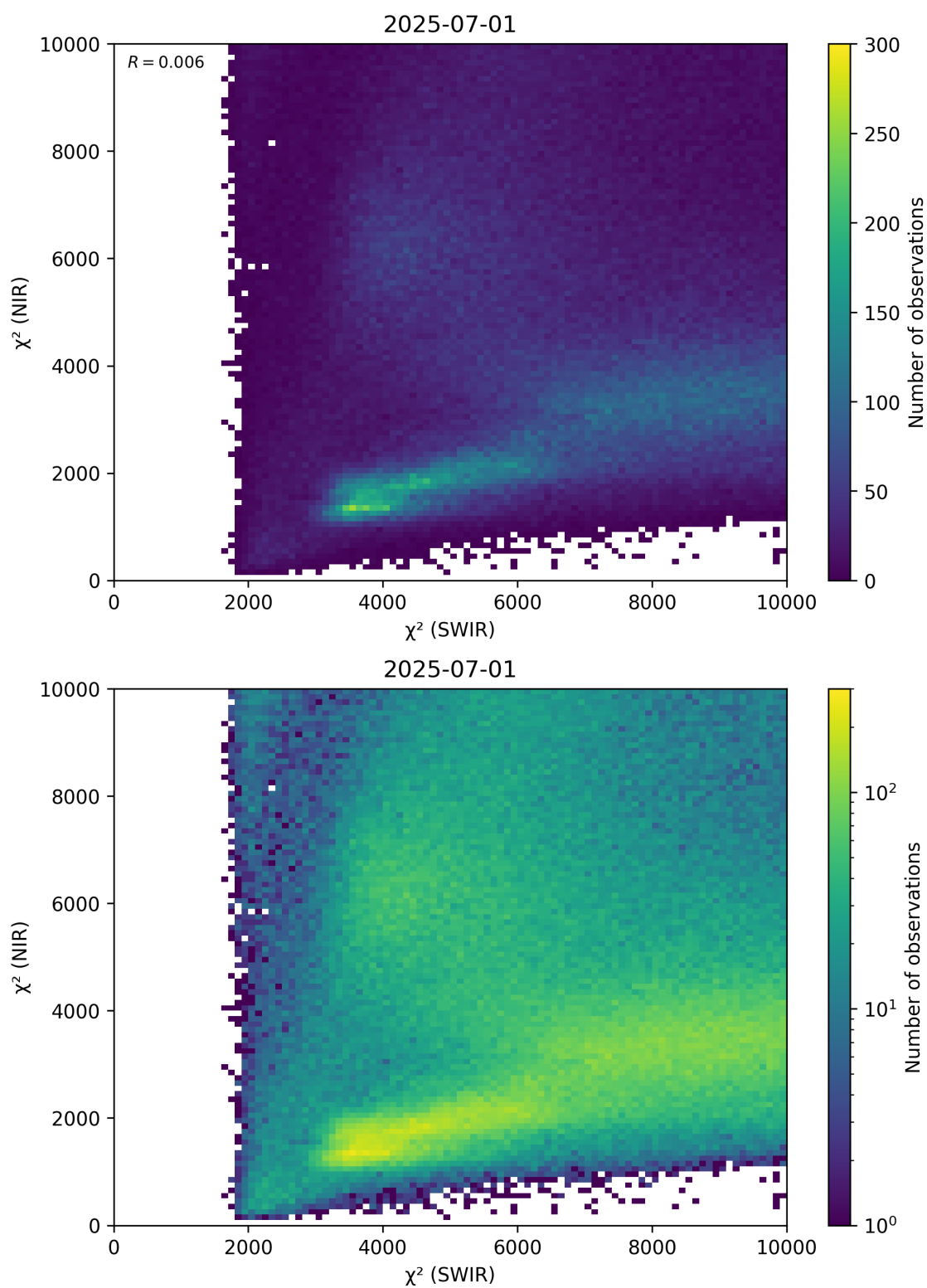
Figure 47: Scatter density plot of “ \chi^2 (SWIR)” against “ \chi^2 (NIR)” for 2025-06-30 to 2025-07-02.
