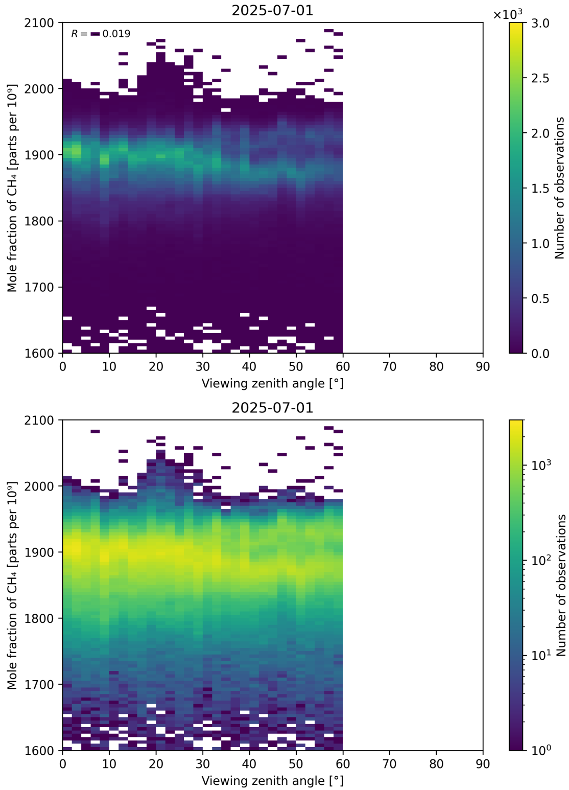
Figure 110: Scatter density plot of “Viewing zenith angle” against “Mole fraction of \text{CH}_4 ” for 2025-06-30 to 2025-07-02.
