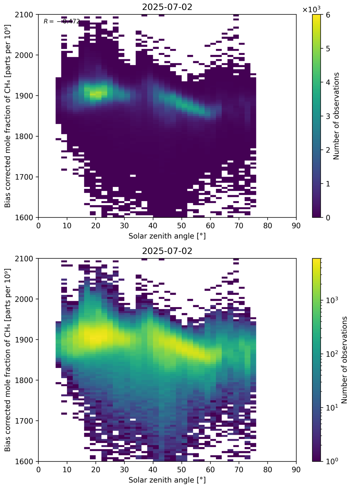
Figure 100: Scatter density plot of “Solar zenith angle” against “Bias corrected mole fraction of CH 4 ” for 2025-07-02 to 2025-07-03.
