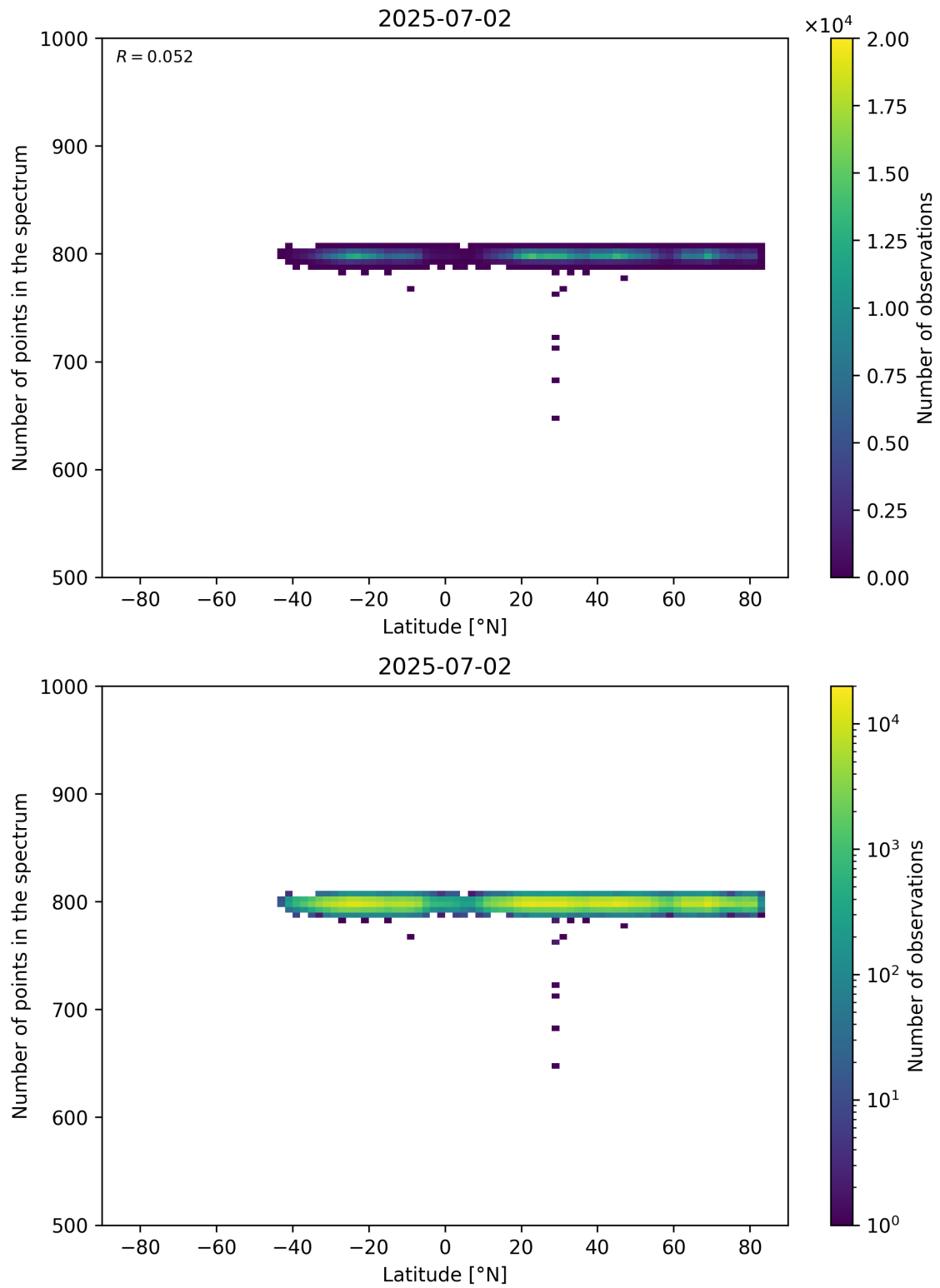
Figure 61: Scatter density plot of “Latitude” against “Number of points in the spectrum” for 2025-07-02 to 2025-07-03.
