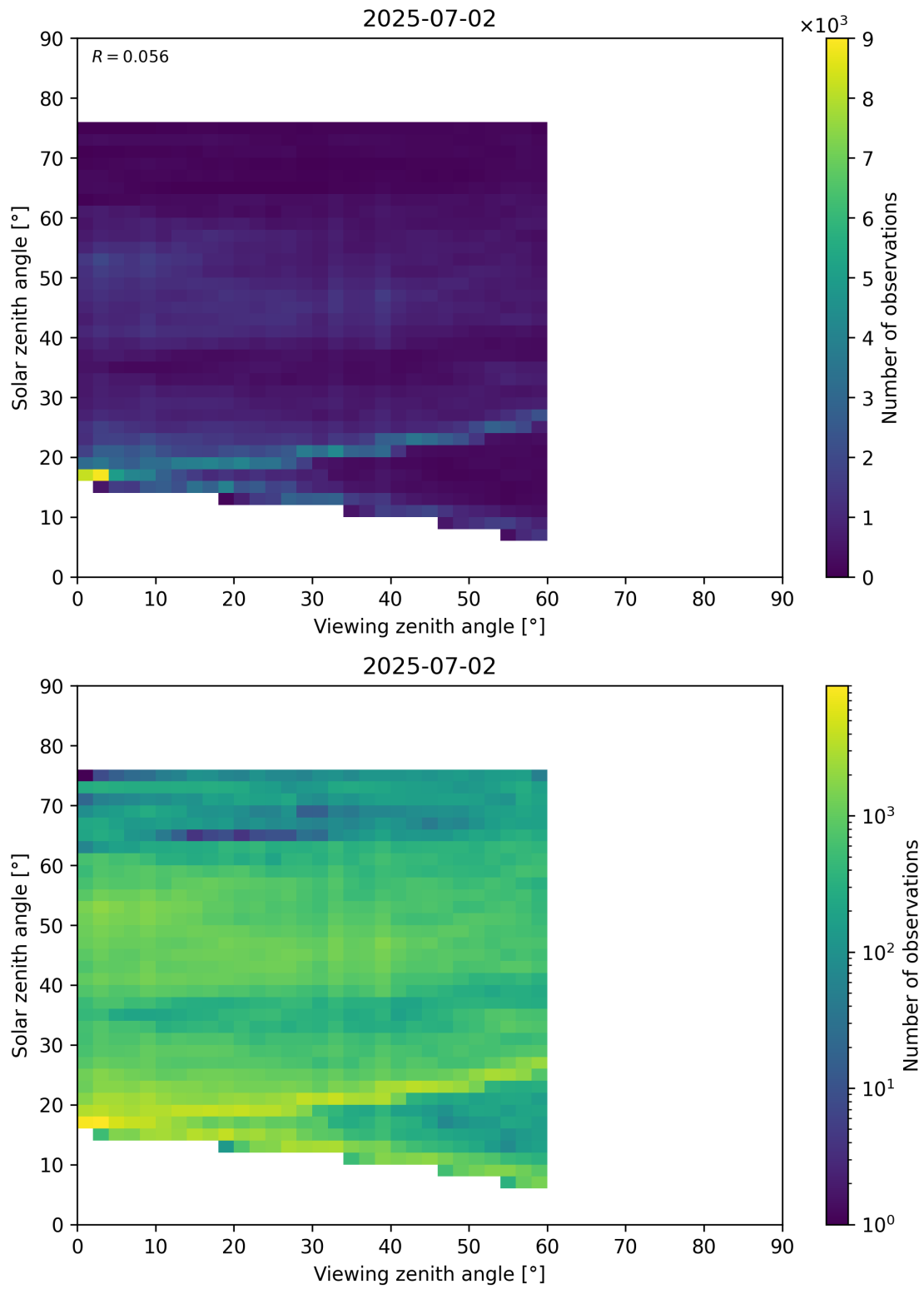
Figure 115: Scatter density plot of “Viewing zenith angle” against “Solar zenith angle” for 2025-07-02 to 2025-07-03.
