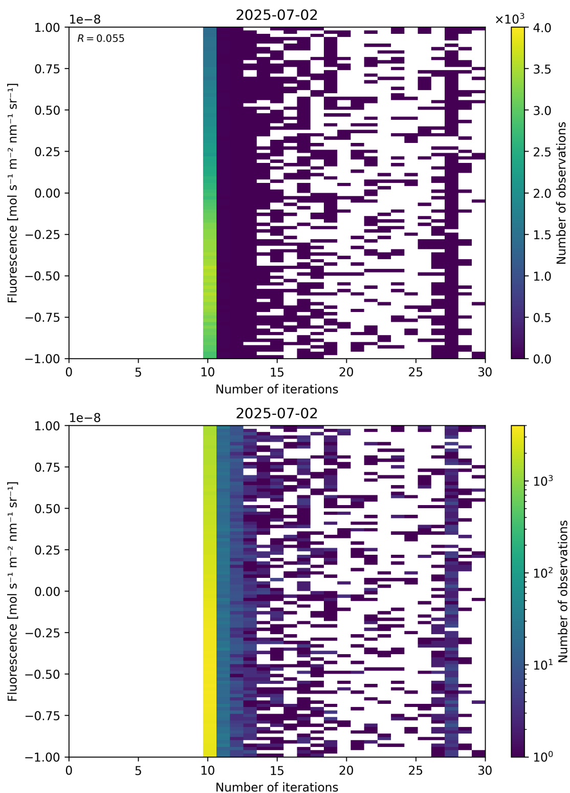
Figure 87: Scatter density plot of “Number of iterations” against “Fluorescence” for 2025-07-02 to 2025-07-03.
