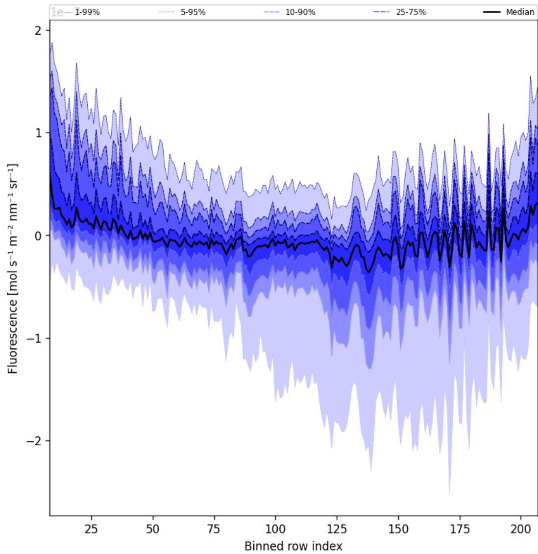
Figure 43: Along track statistics of “Fluorescence” for 2025-07-02 to 2025-07-03
