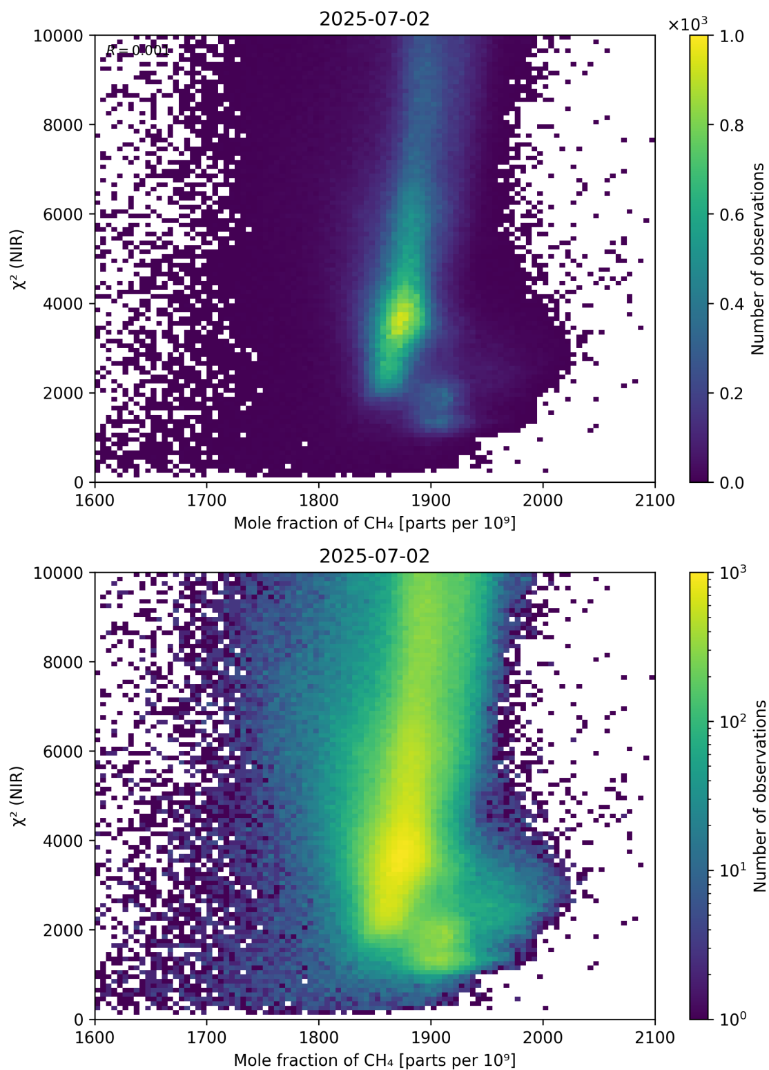
Figure 70: Scatter density plot of “Mole fraction of CH 4 ” against “ \chi^2 (NIR)” for 2025-07-02 to 2025-07-03.
