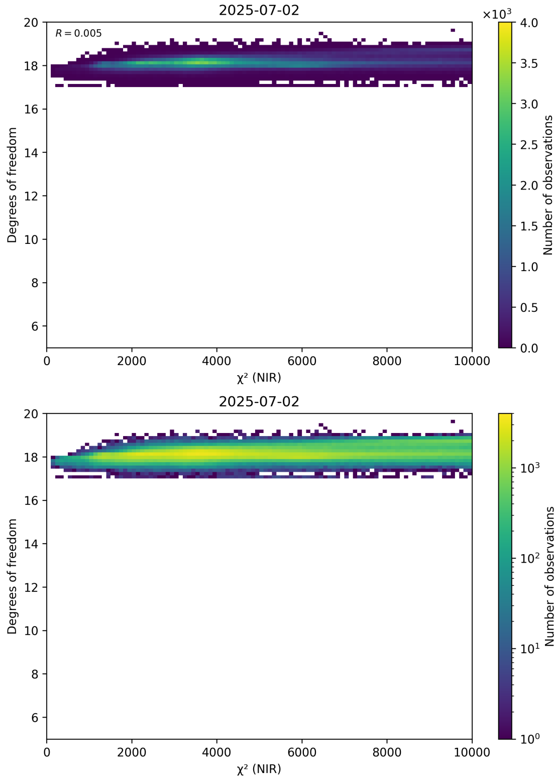
Figure 44: Scatter density plot of “ \chi^2 (NIR)” against “Degrees of freedom” for 2025-07-02 to 2025-07-03.
