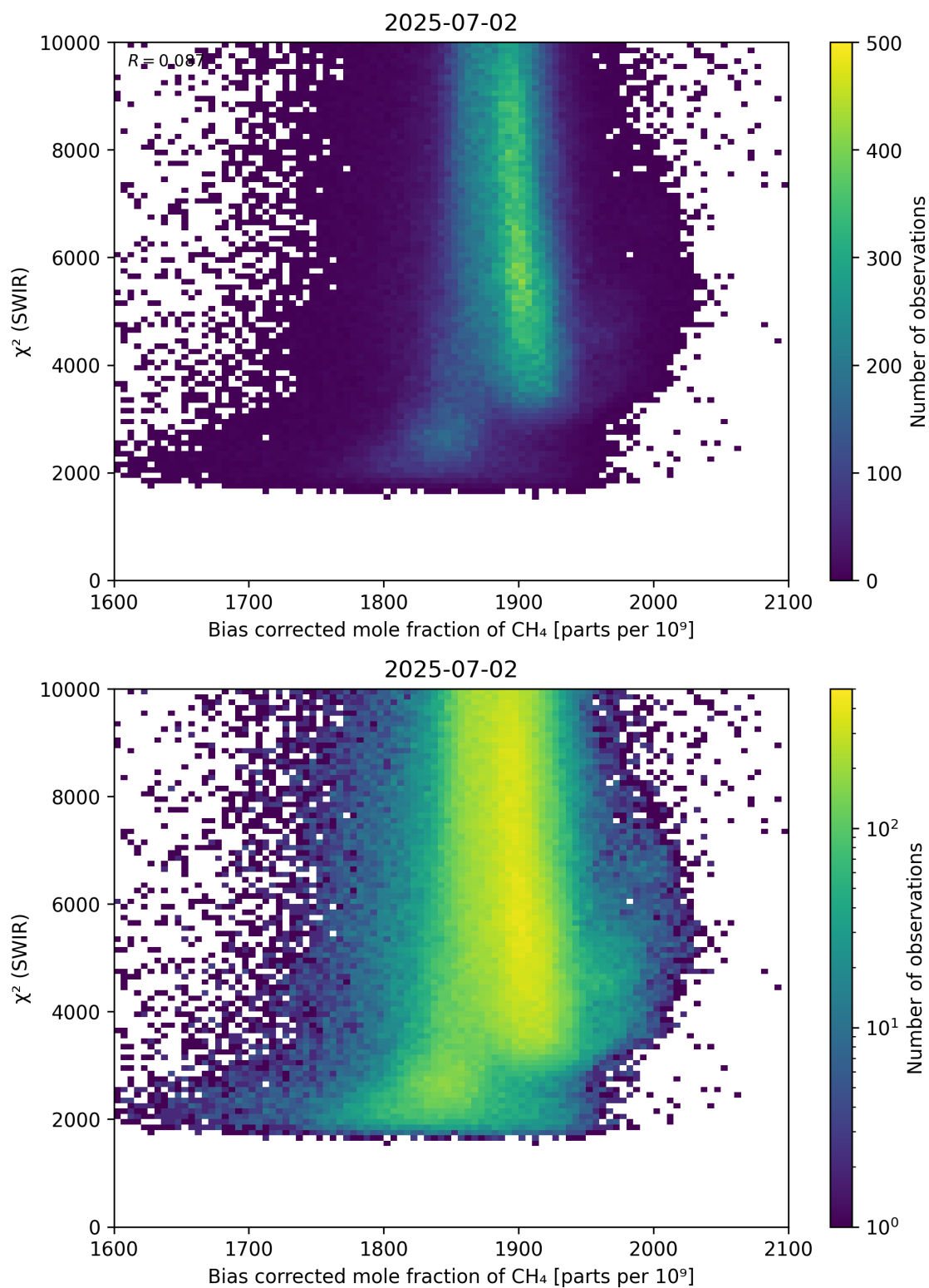
Figure 64: Scatter density plot of “Bias corrected mole fraction of \text{CH}_4 ” against “ \chi^2 (SWIR)” for 2025-07-02 to 2025-07-03.
