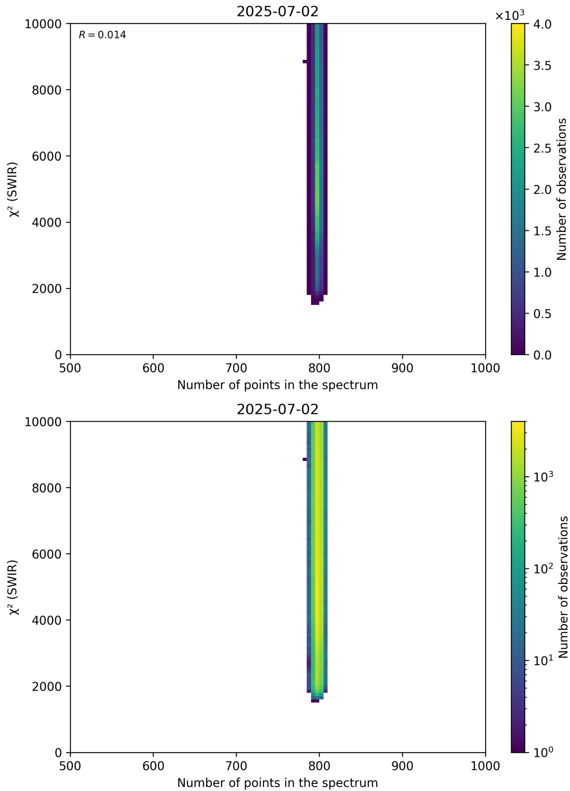
Figure 89: Scatter density plot of “Number of points in the spectrum” against “ \chi^2 (SWIR)” for 2025-07-02 to 2025-07-03.
