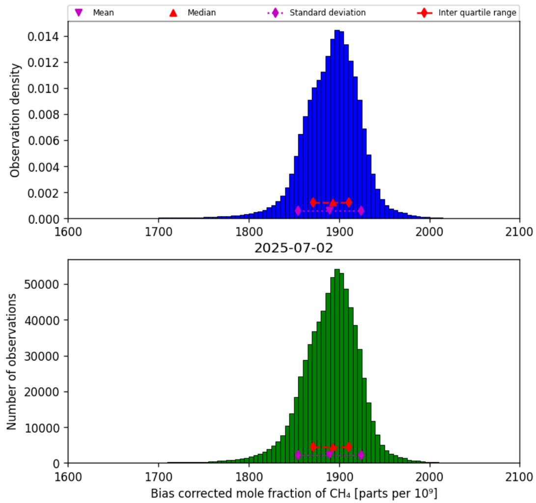
Figure 25: Histogram of “Bias corrected mole fraction of CH 4 ” for 2025-07-02 to 2025-07-03
