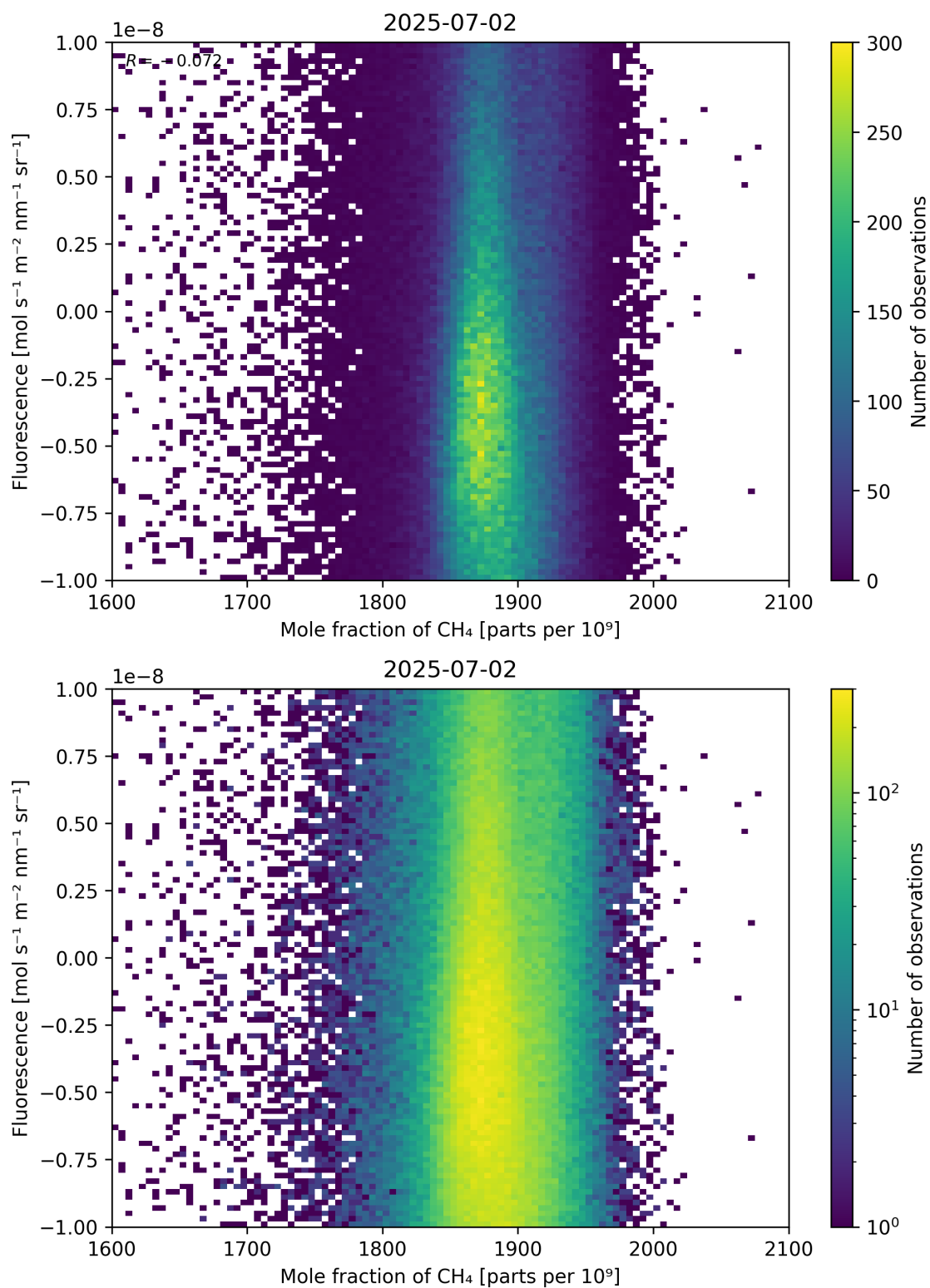
Figure 73: Scatter density plot of “Mole fraction of \text{CH}_4 ” against “Fluorescence” for 2025-07-02 to 2025-07-03.
