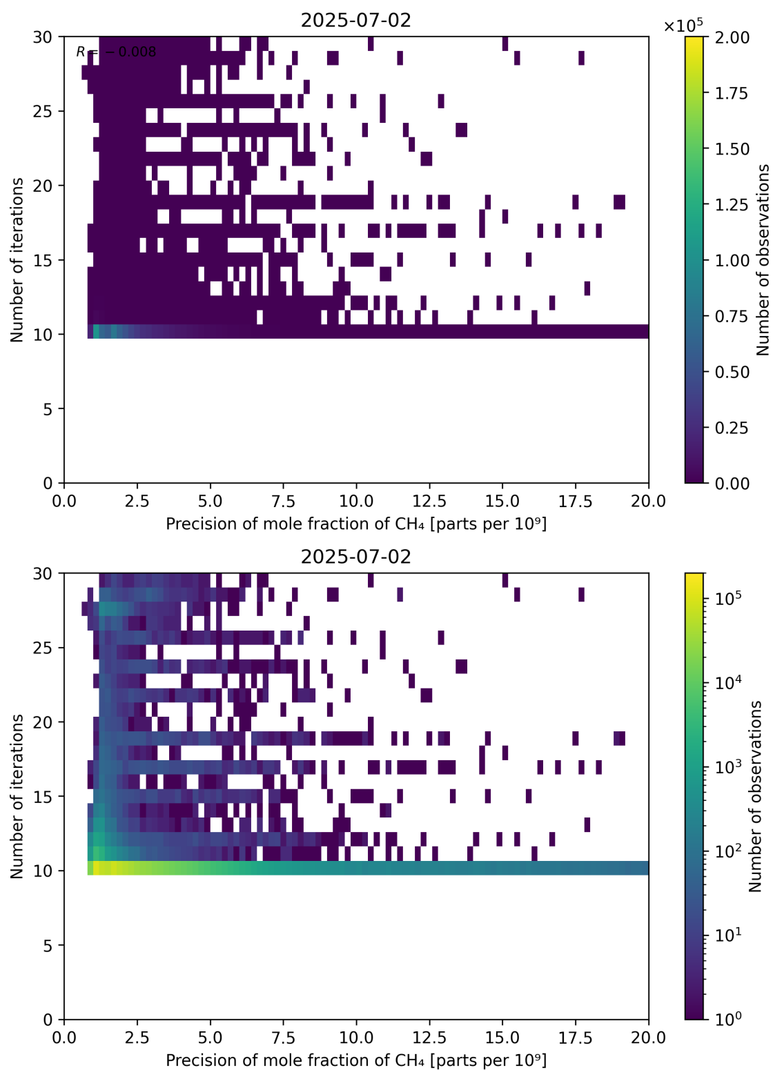
Figure 83: Scatter density plot of “Precision of mole fraction of CH 4 ” against “Number of iterations” for 2025-07-02 to 2025-07-03.
