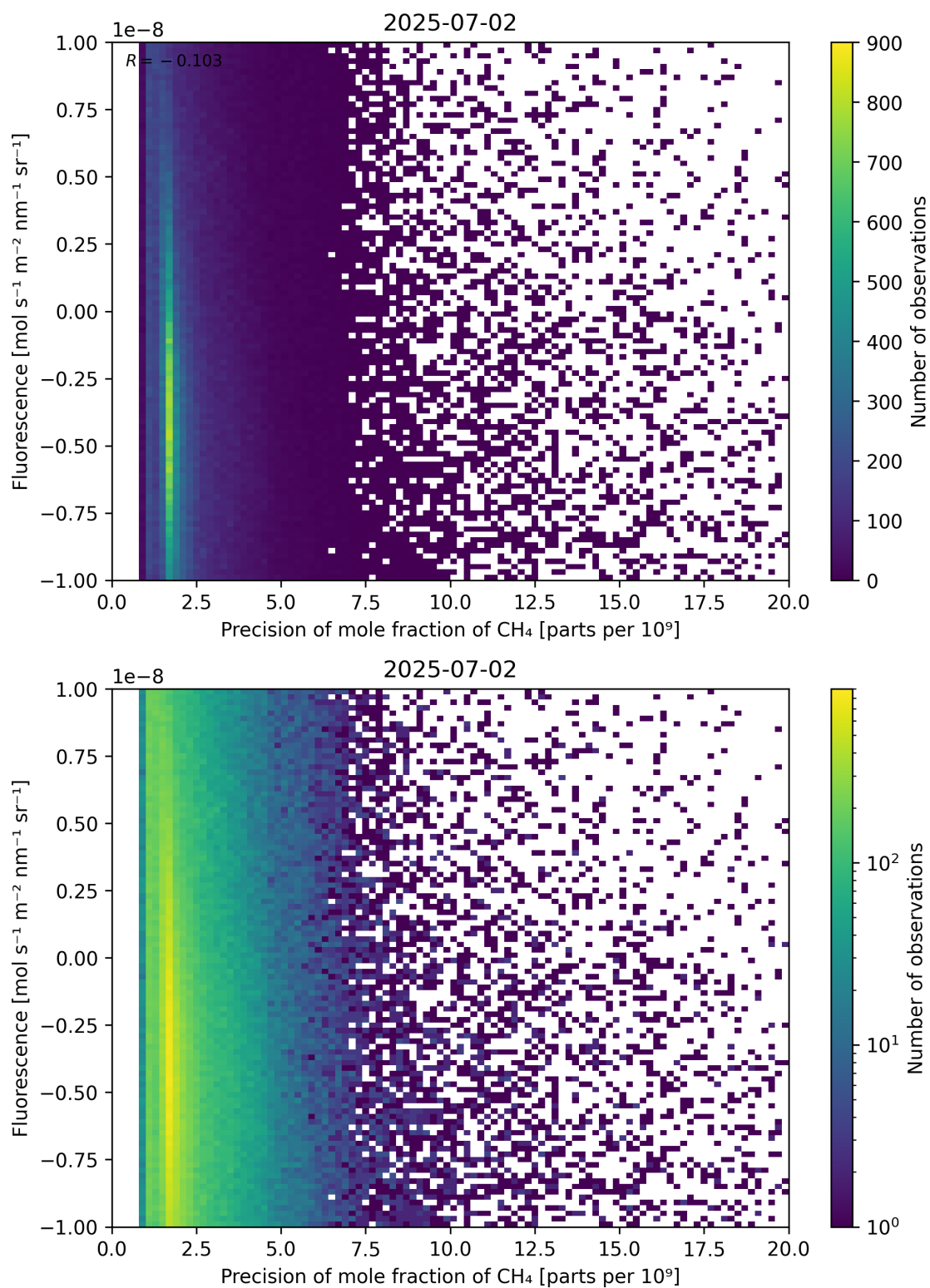
Figure 81: Scatter density plot of “Precision of mole fraction of CH 4 ” against “Fluorescence” for 2025-07-02 to 2025-07-03.
