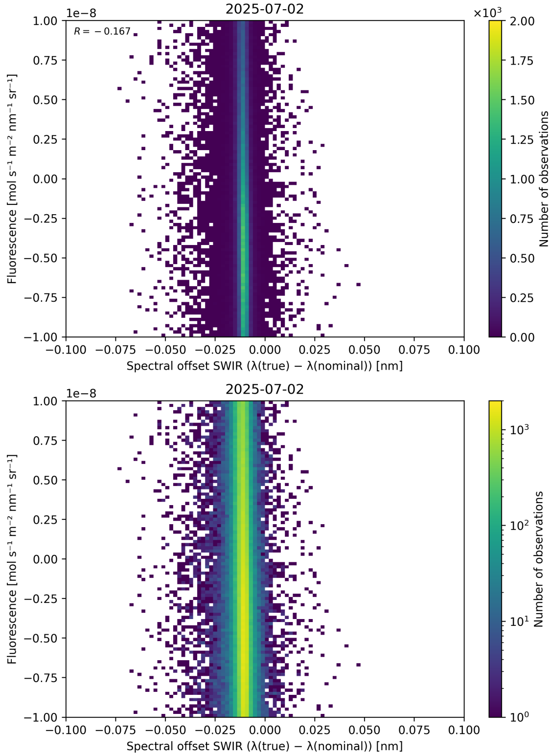
Figure 120: Scatter density plot of “Spectral offset SWIR ( \lambda_{\text{true}} - \lambda_{\text{nominal}} )” against “Fluorescence” for 2025-07-02 to 2025-07-03.
