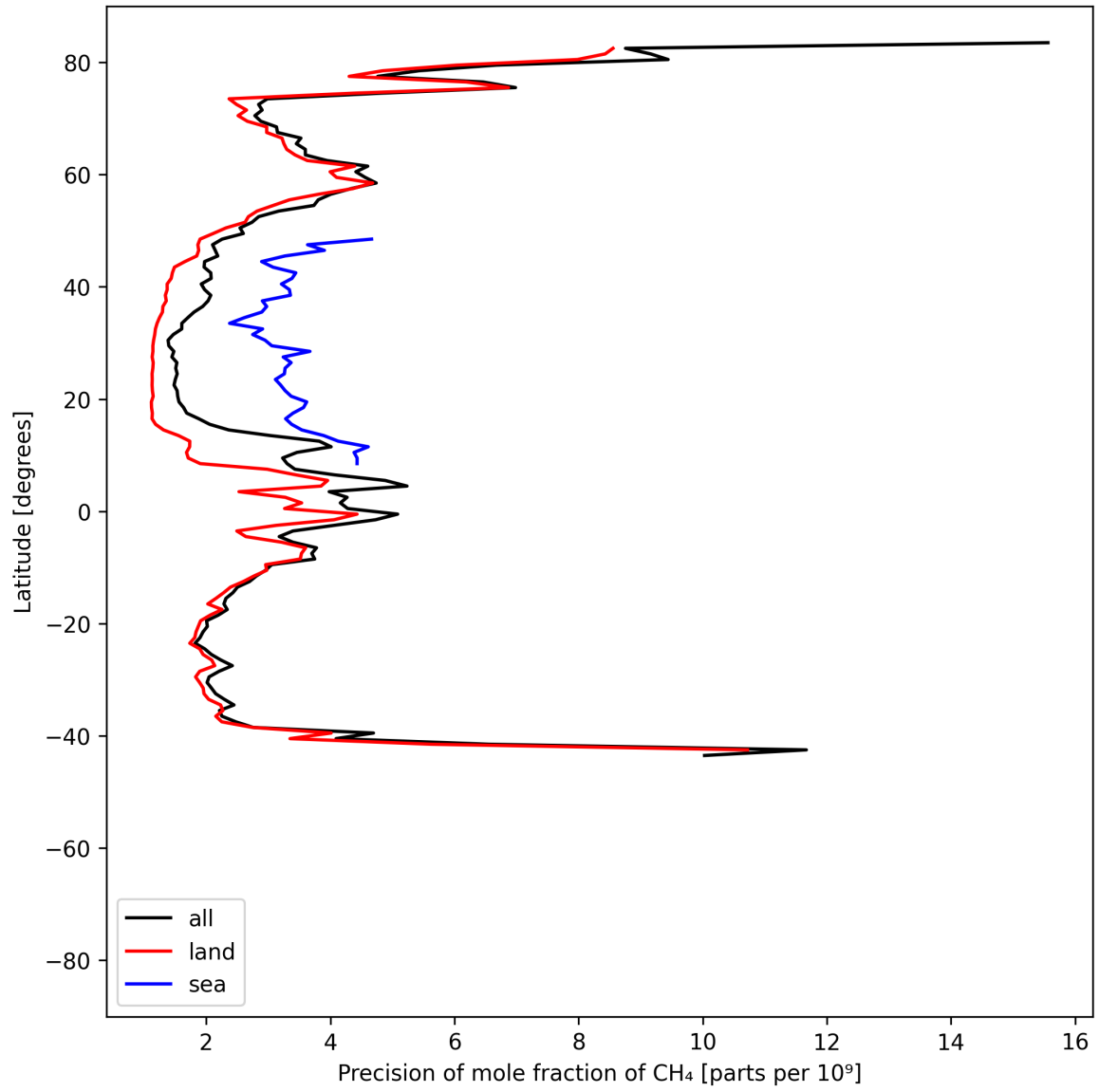
Figure 13: Zonal average of “Precision of mole fraction of \text{CH}_4 ” for 2025-07-02 to 2025-07-03.
