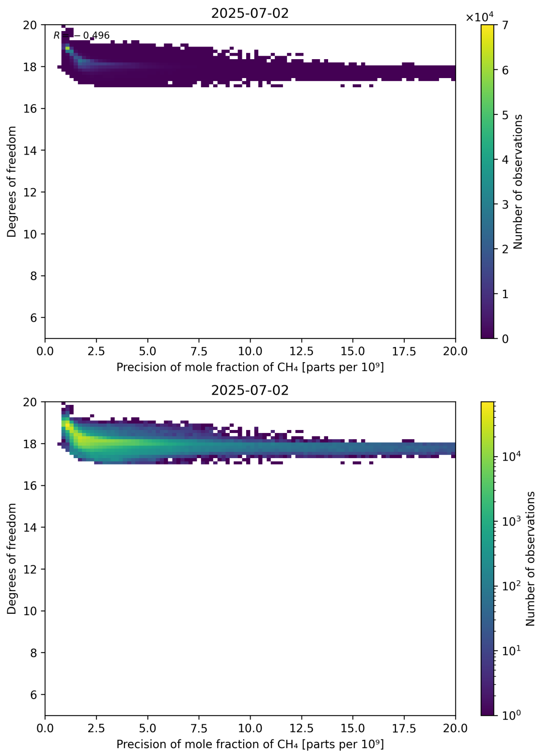
Figure 80: Scatter density plot of “Precision of mole fraction of CH 4 ” against “Degrees of freedom” for 2025-07-02 to 2025-07-03.
