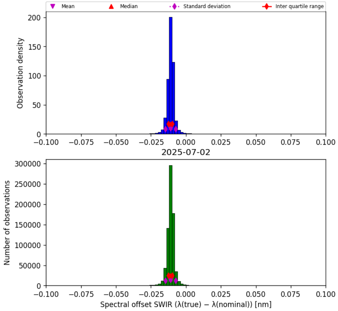
Figure 27: Histogram of “Spectral offset SWIR ( \lambda_{\text{true}} - \lambda_{\text{nominal}} )” for 2025-07-02 to 2025-07-03
