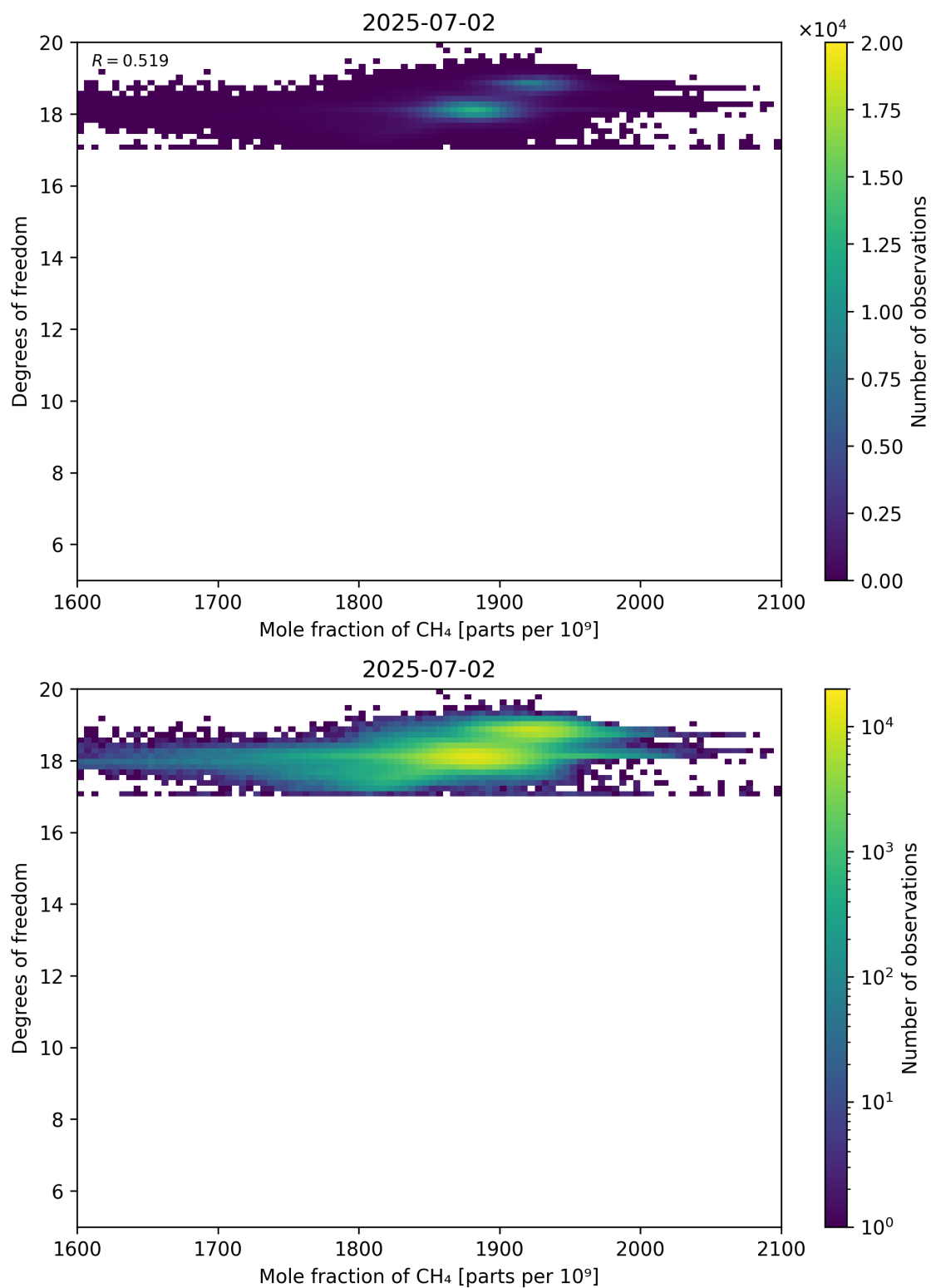
Figure 72: Scatter density plot of “Mole fraction of CH 4 ” against “Degrees of freedom” for 2025-07-02 to 2025-07-03.
