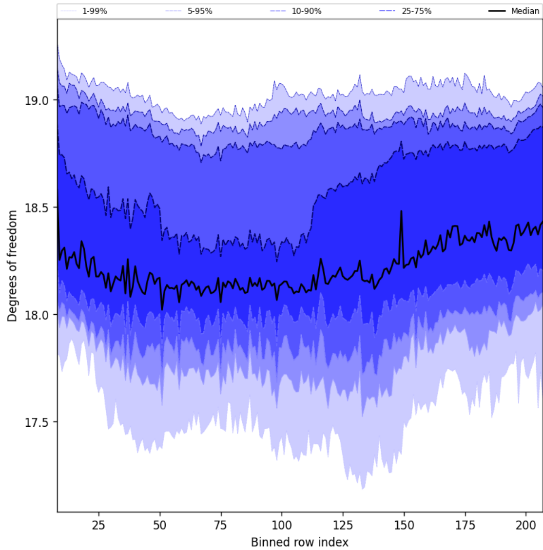
Figure 41: Along track statistics of “Degrees of freedom” for 2025-07-02 to 2025-07-03
