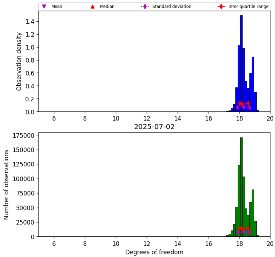
Figure 30: Histogram of “Degrees of freedom” for 2025-07-02 to 2025-07-03
