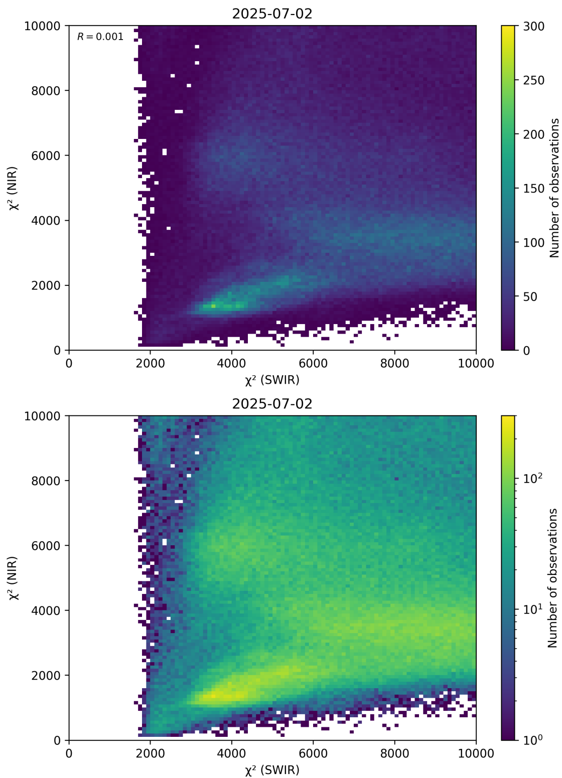
Figure 47: Scatter density plot of “ \chi^2 (SWIR)” against “ \chi^2 (NIR)” for 2025-07-02 to 2025-07-03.
