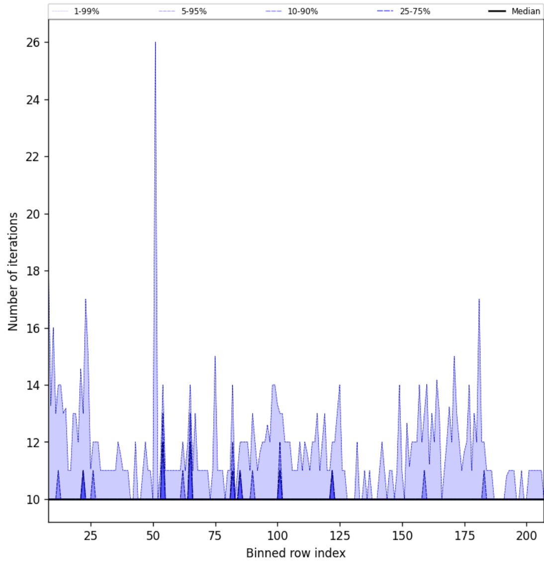
Figure 42: Along track statistics of “Number of iterations” for 2025-07-02 to 2025-07-03
