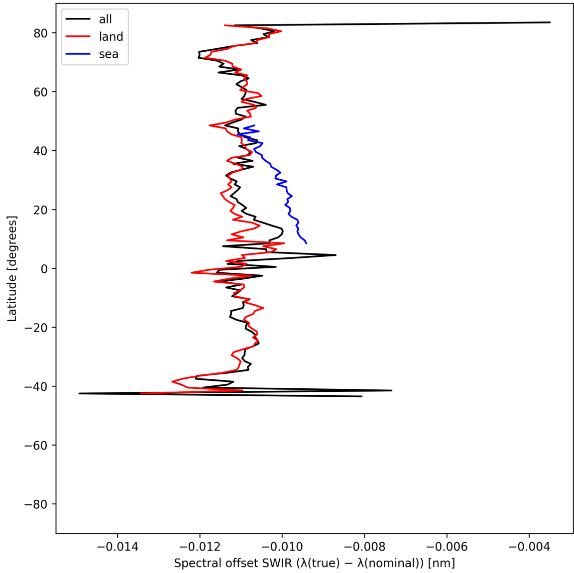
Figure 16: Zonal average of “Spectral offset SWIR ( \lambda_{\text{true}} - \lambda_{\text{nominal}} )” for 2025-07-02 to 2025-07-03.
