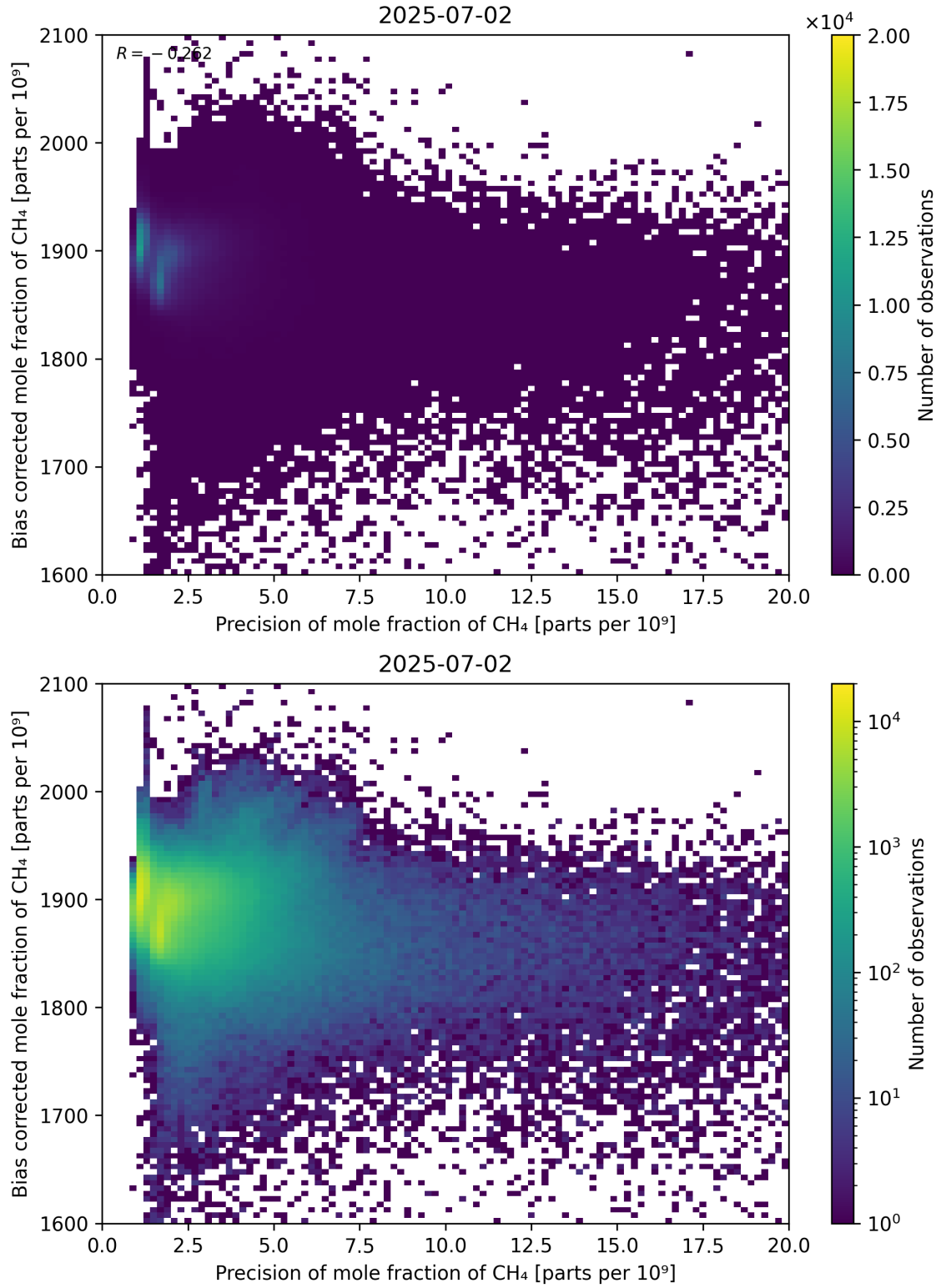
Figure 82: Scatter density plot of “Precision of mole fraction of CH 4 ” against “Bias corrected mole fraction of CH 4 ” for 2025-07-02 to 2025-07-03.
