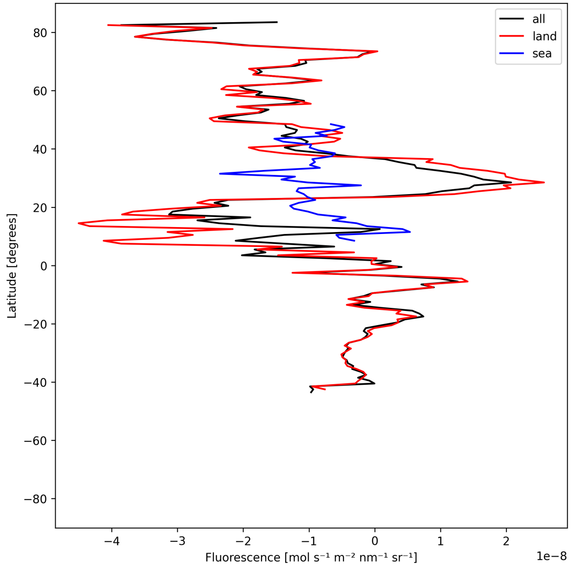
Figure 21: Zonal average of “Fluorescence” for 2025-07-02 to 2025-07-03.
