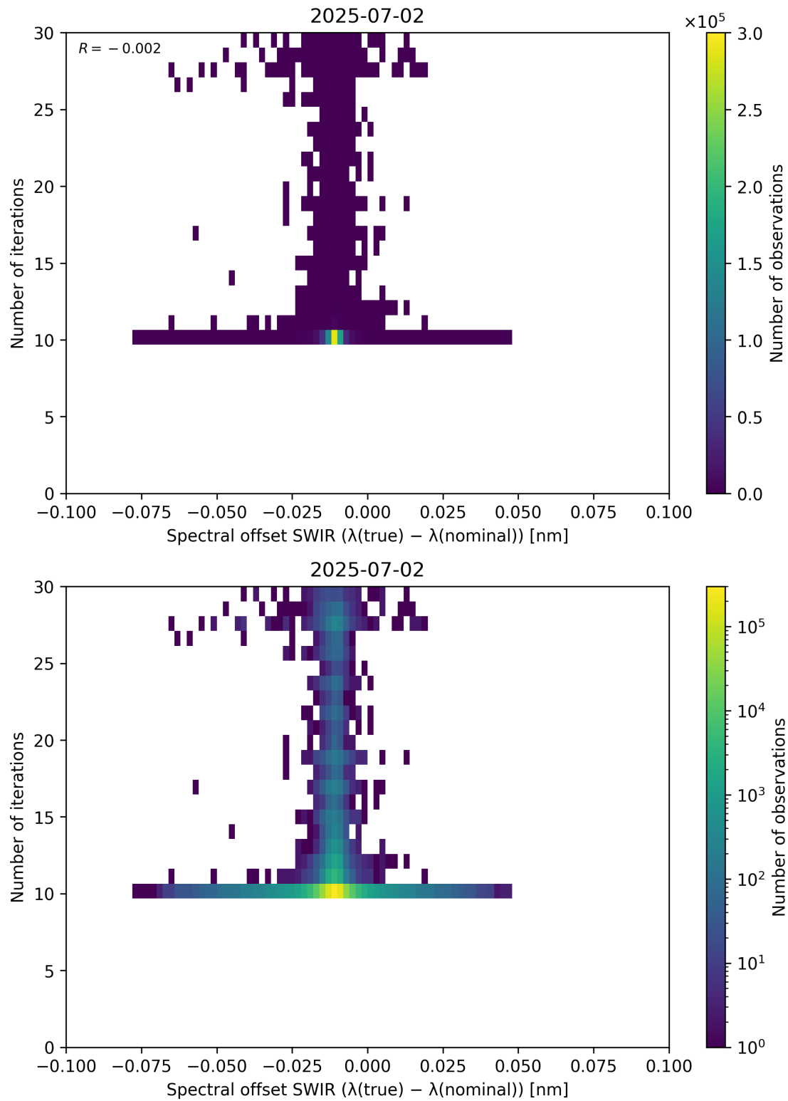
Figure 121: Scatter density plot of “Spectral offset SWIR ( \lambda_{\text{true}} - \lambda_{\text{nominal}} )” against “Number of iterations” for 2025-07-02 to 2025-07-03.
