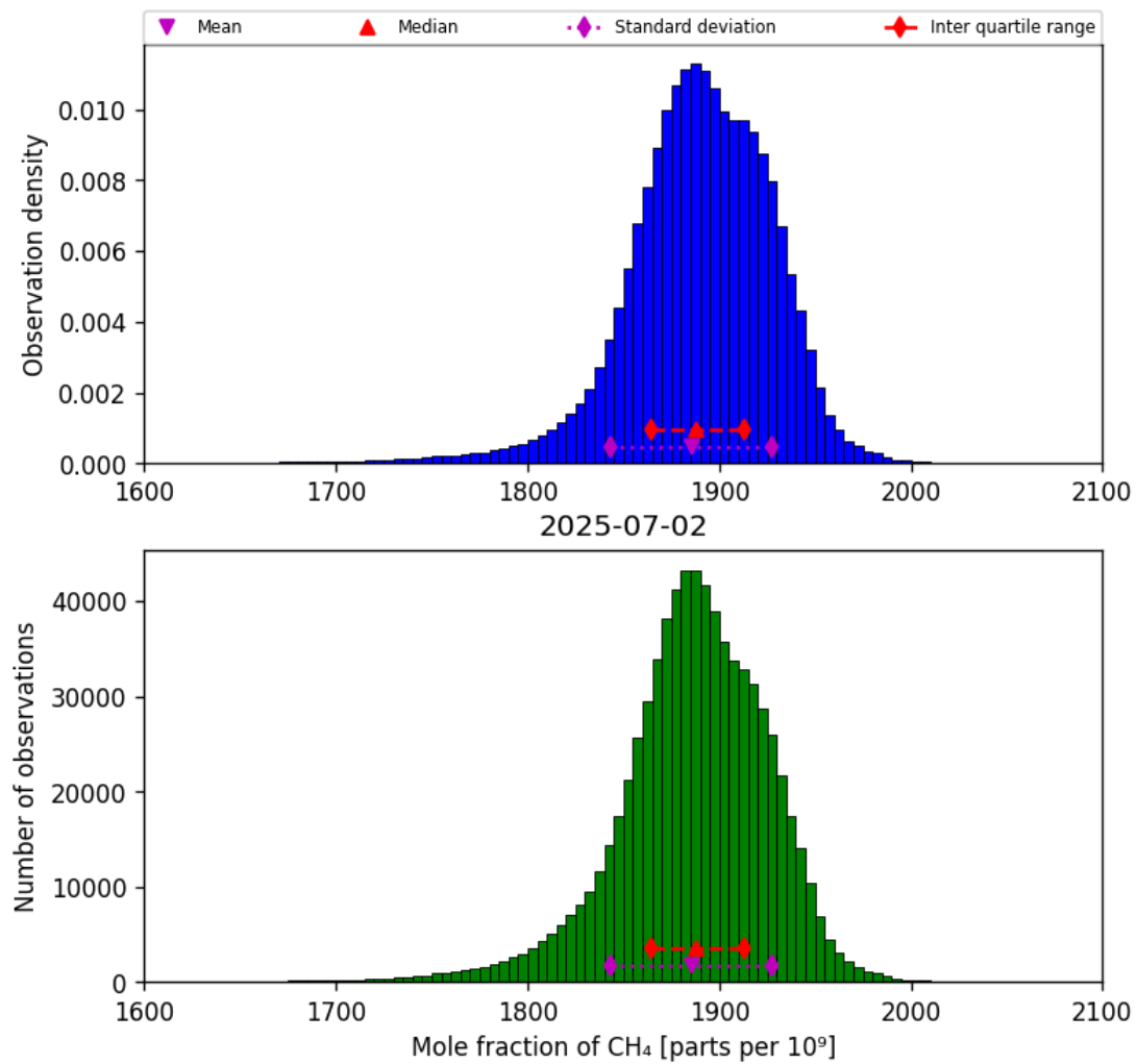
Figure 23: Histogram of “Mole fraction of CH 4 ” for 2025-07-02 to 2025-07-03
