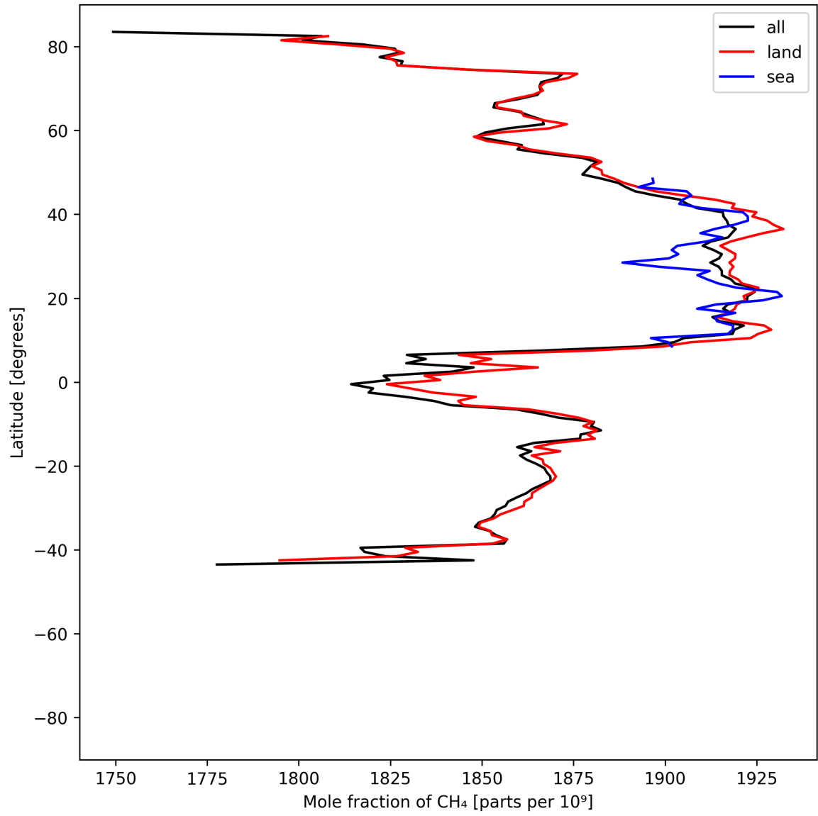
Figure 12: Zonal average of “Mole fraction of \text{CH}_4 ” for 2025-07-02 to 2025-07-03.
