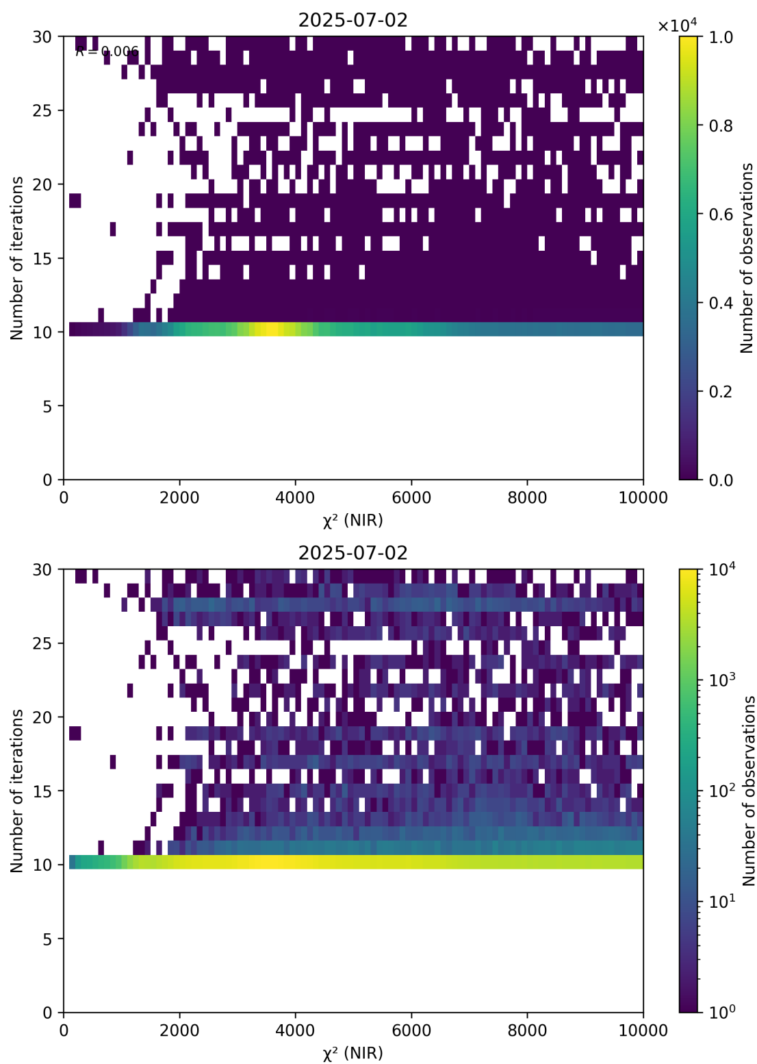
Figure 46: Scatter density plot of “ \chi^2 (NIR)” against “Number of iterations” for 2025-07-02 to 2025-07-03.
