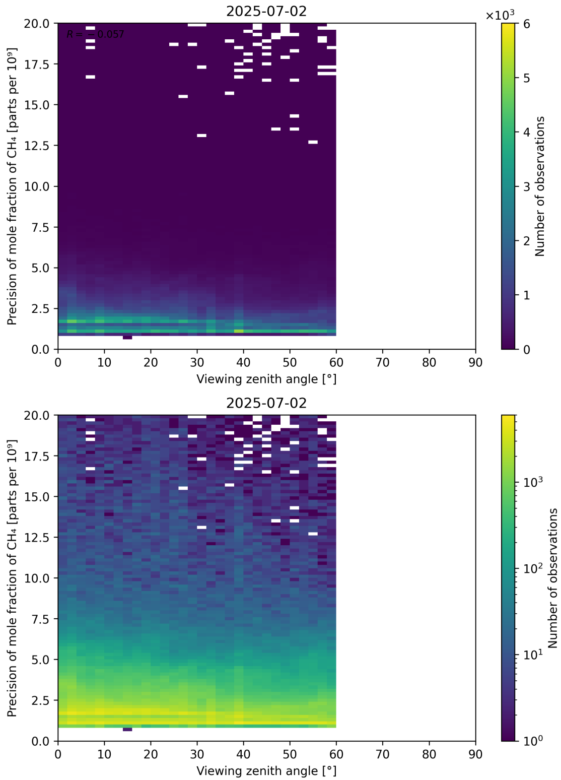
Figure 112: Scatter density plot of “Viewing zenith angle” against “Precision of mole fraction of CH 4 ” for 2025-07-02 to 2025-07-03.
