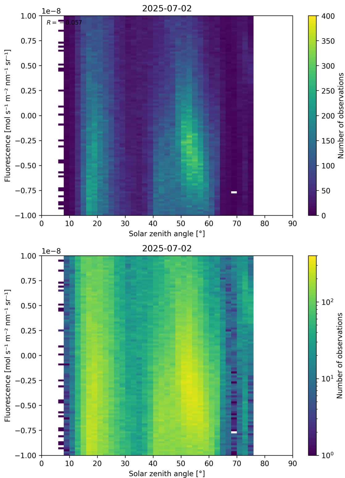
Figure 97: Scatter density plot of “Solar zenith angle” against “Fluorescence” for 2025-07-02 to 2025-07-03.
