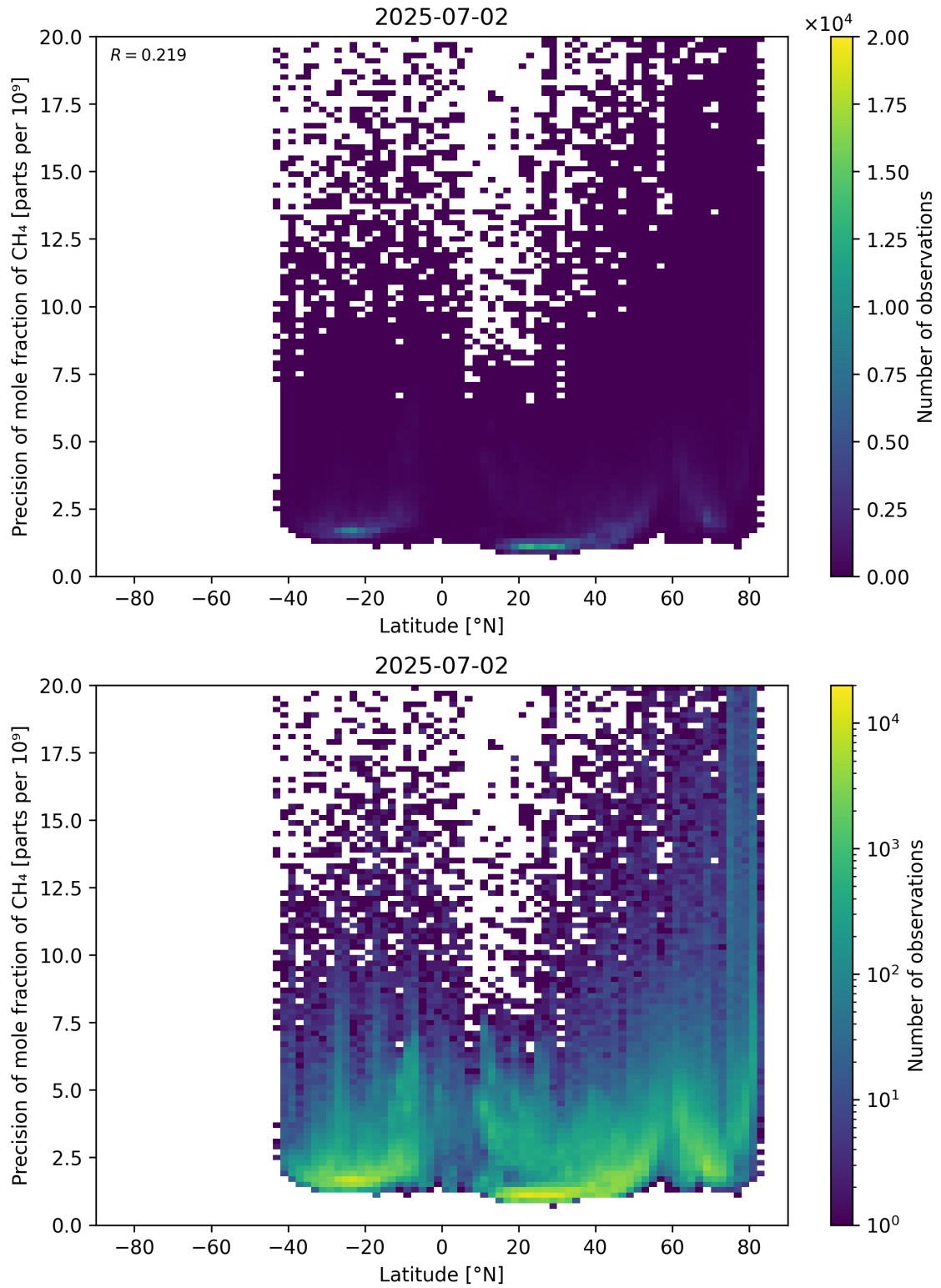
Figure 59: Scatter density plot of “Latitude” against “Precision of mole fraction of \text{CH}_4 ” for 2025-07-02 to 2025-07-03.
