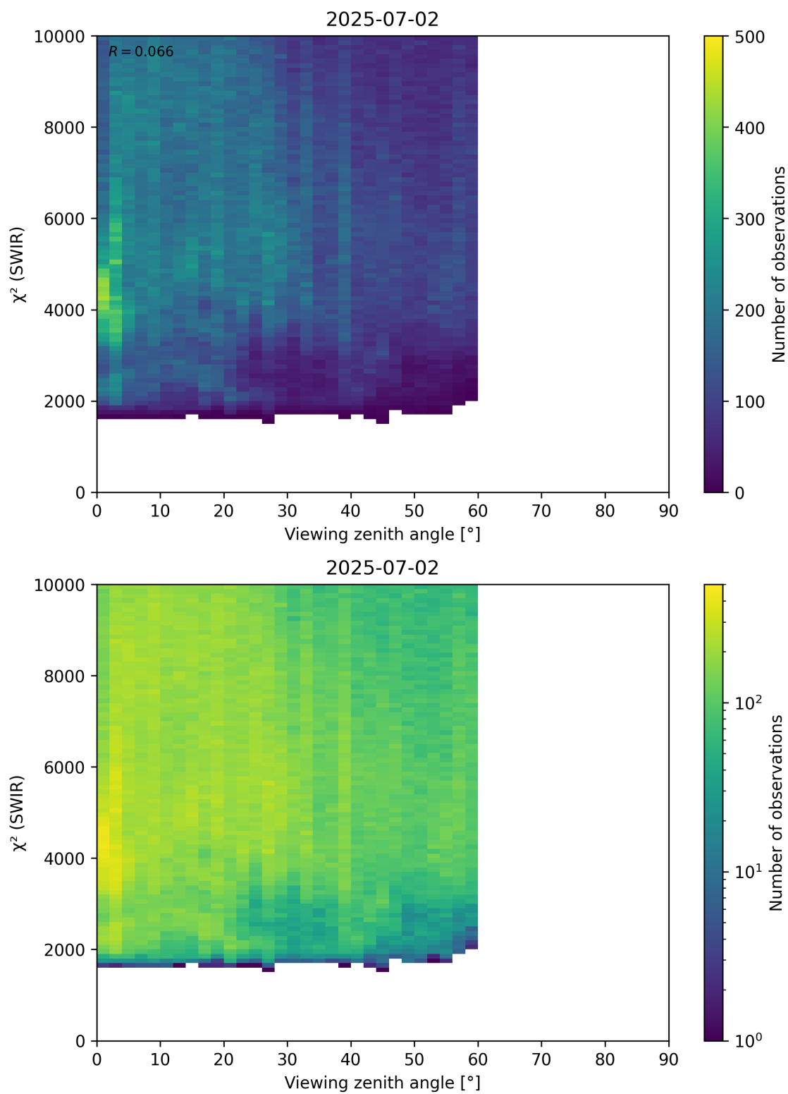
Figure 106: Scatter density plot of “Viewing zenith angle” against “ \chi^2 (SWIR)” for 2025-07-02 to 2025-07-03.
