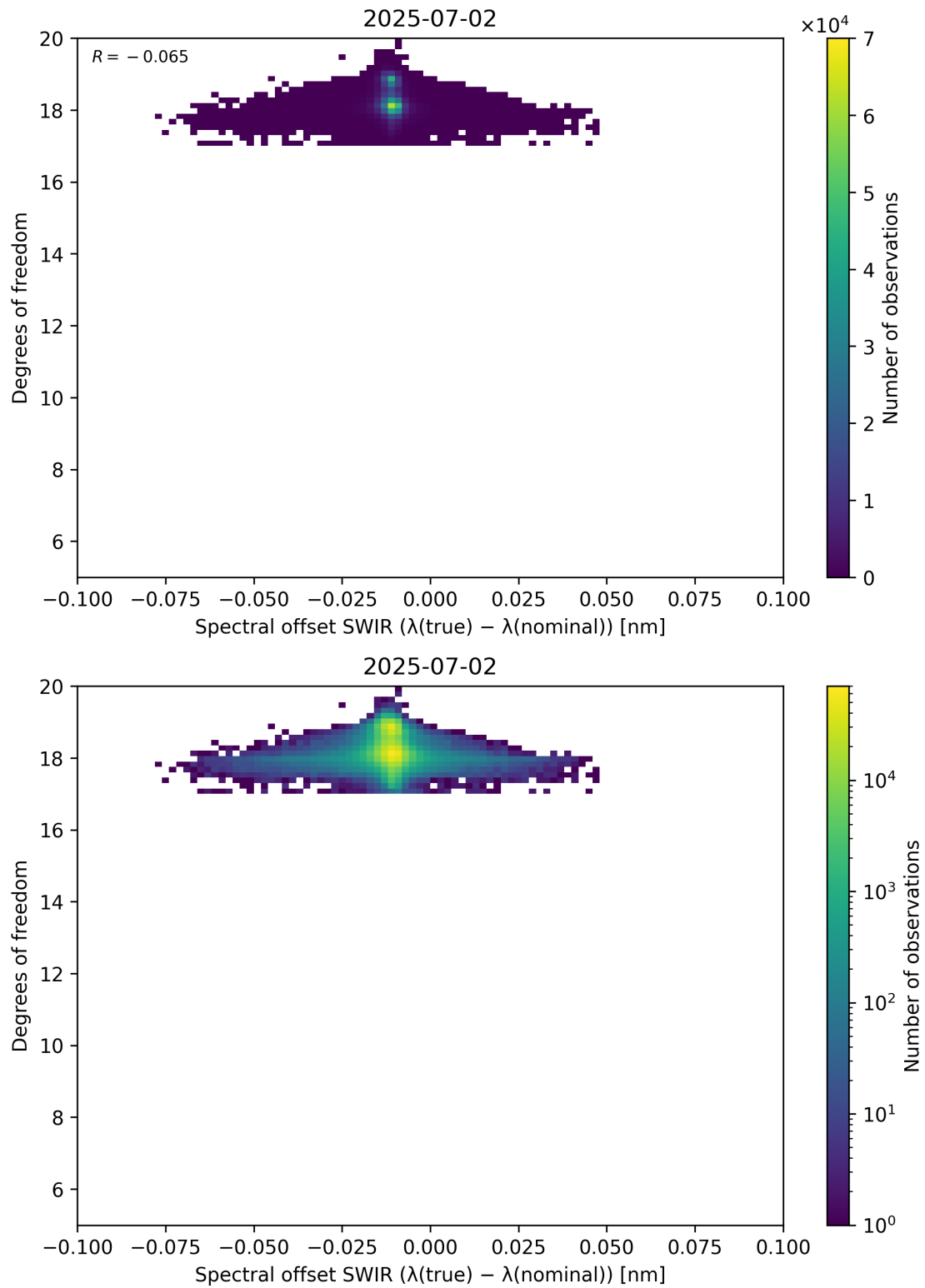
Figure 119: Scatter density plot of “Spectral offset SWIR ( \lambda_{\text{true}} - \lambda_{\text{nominal}} )” against “Degrees of freedom” for 2025-07-02 to 2025-07-03.
