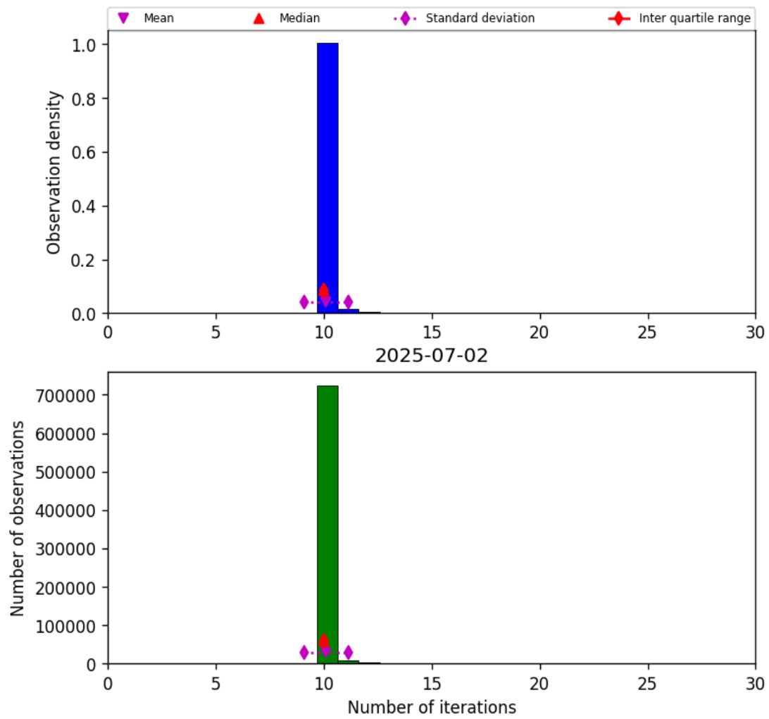
Figure 31: Histogram of “Number of iterations” for 2025-07-02 to 2025-07-03
