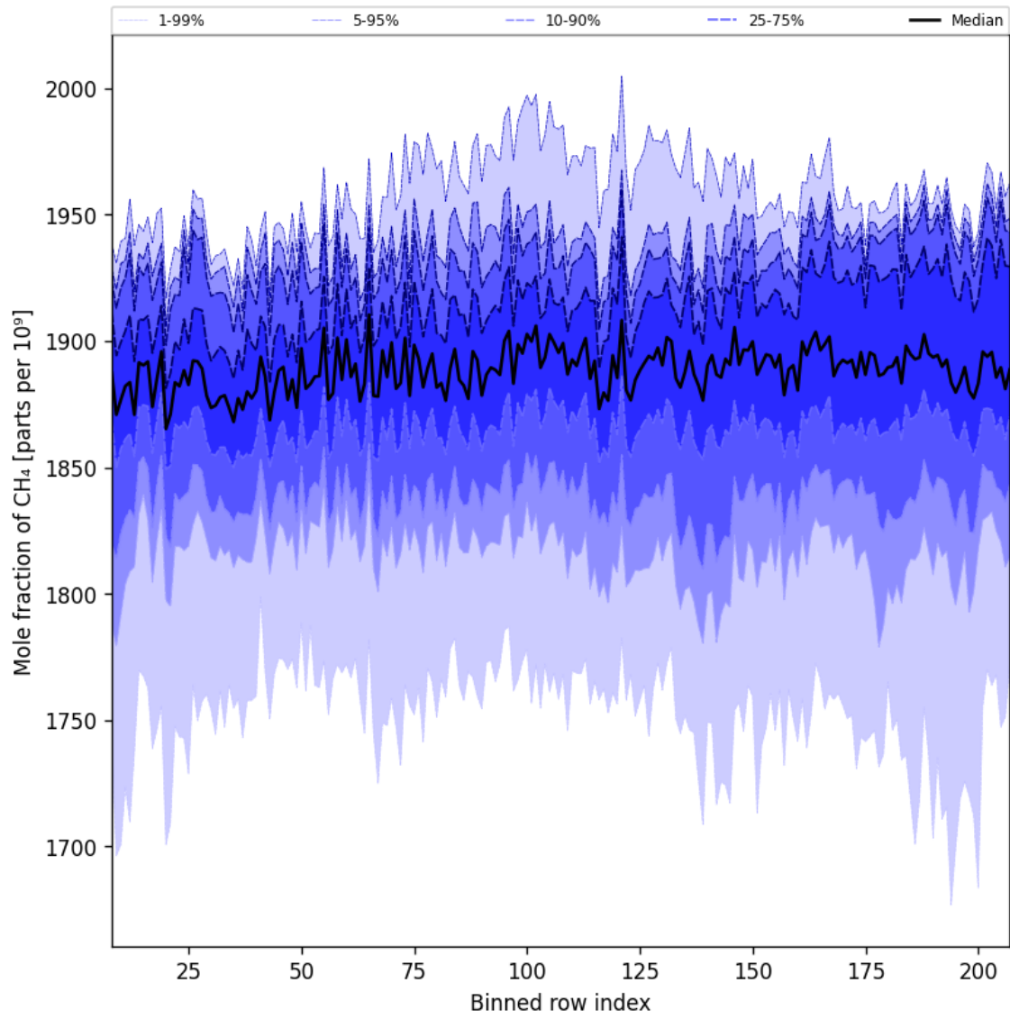
Figure 34: Along track statistics of “Mole fraction of CH 4 ” for 2025-07-02 to 2025-07-03
