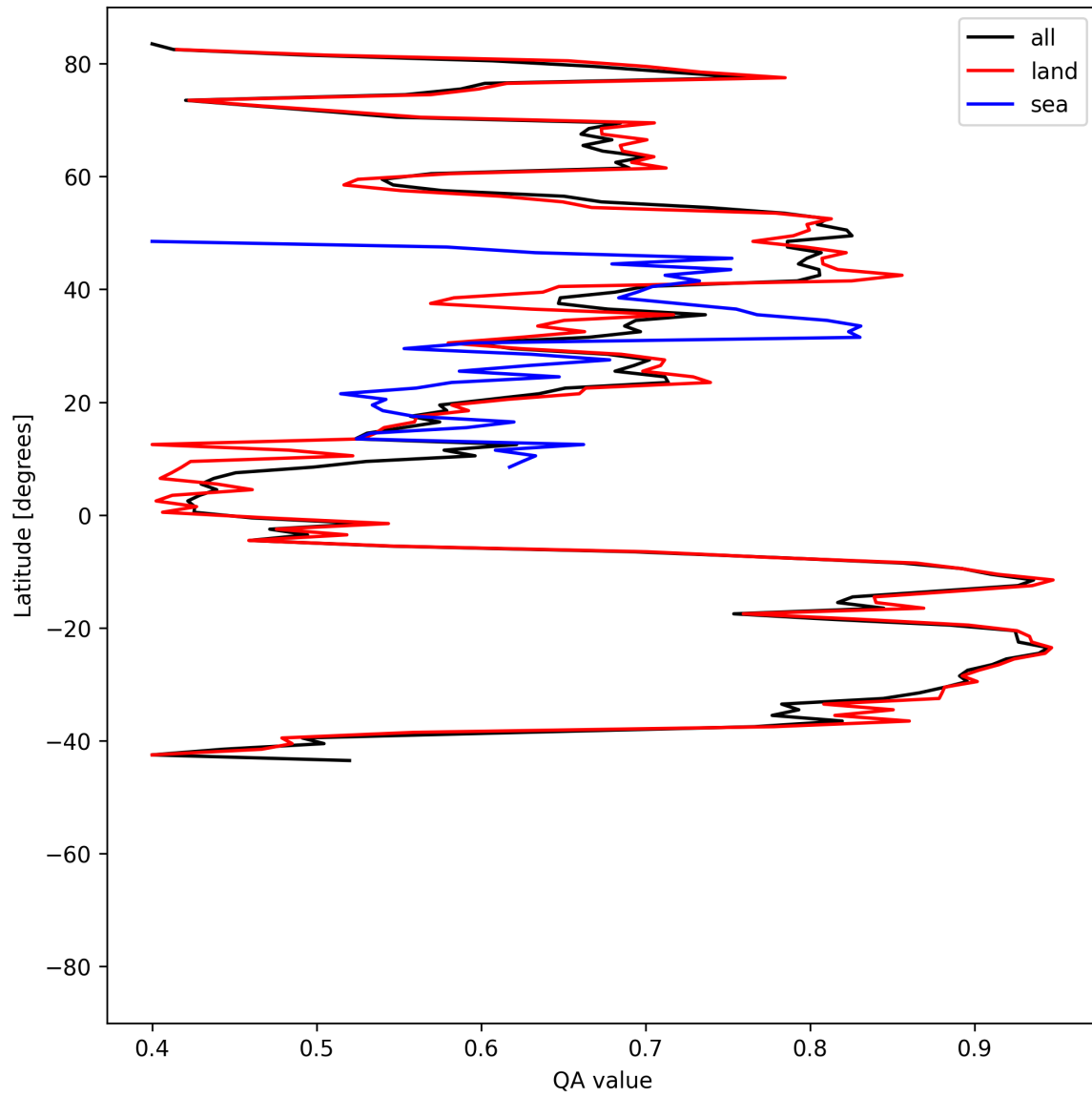
Figure 11: Zonal average of “QA value” for 2025-07-02 to 2025-07-03.
