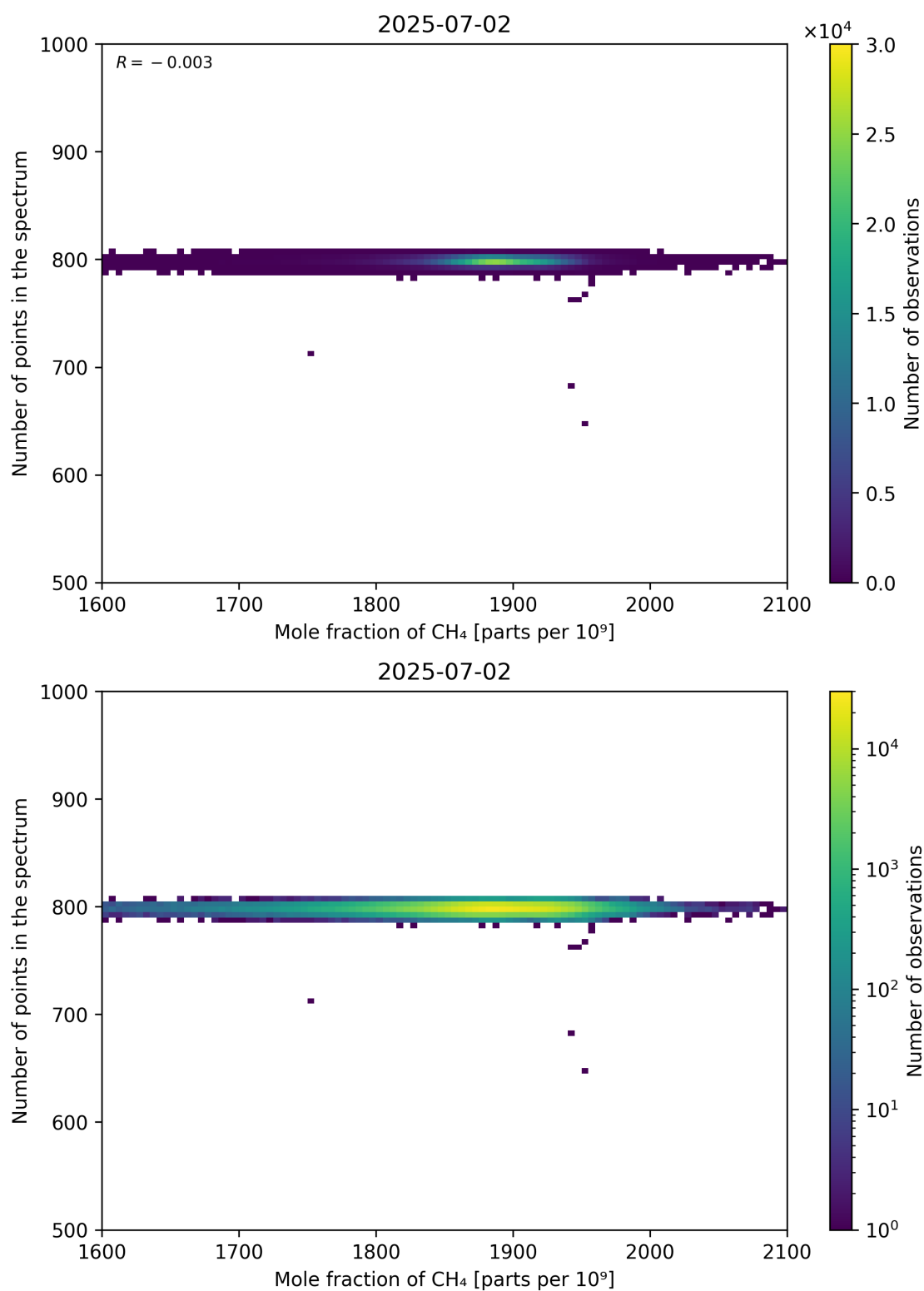
Figure 77: Scatter density plot of “Mole fraction of CH 4 ” against “Number of points in the spectrum” for 2025-07-02 to 2025-07-03.
