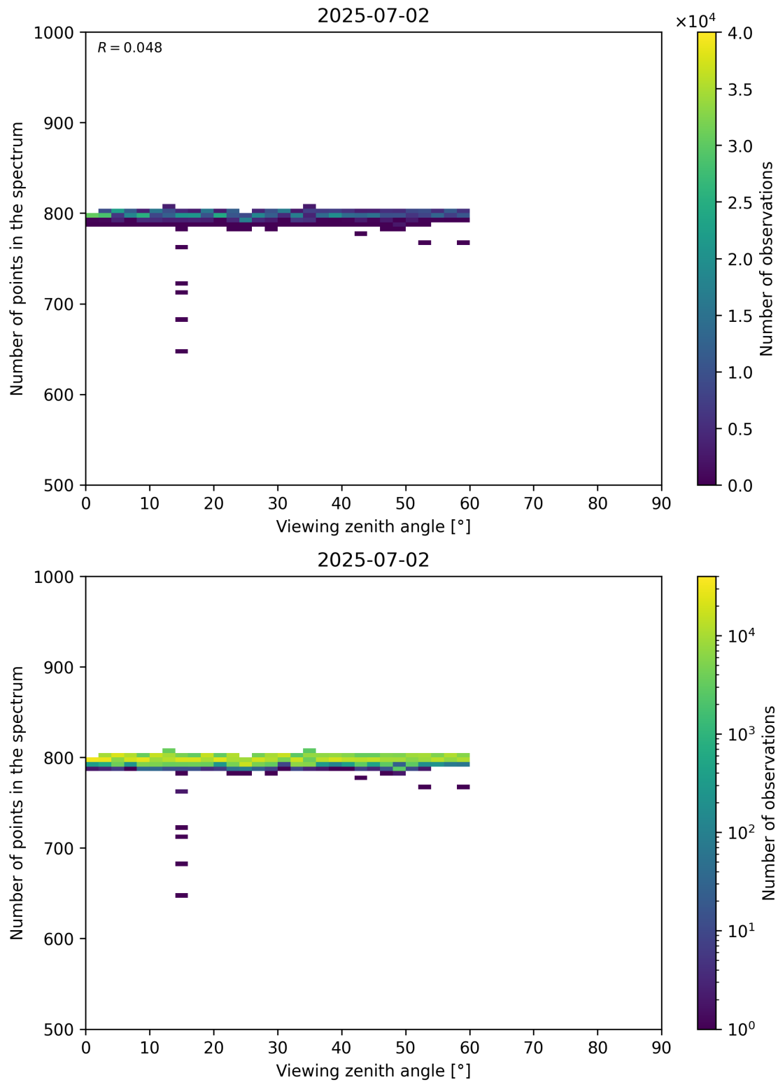
Figure 114: Scatter density plot of “Viewing zenith angle” against “Number of points in the spectrum” for 2025-07-02 to 2025-07-03.
