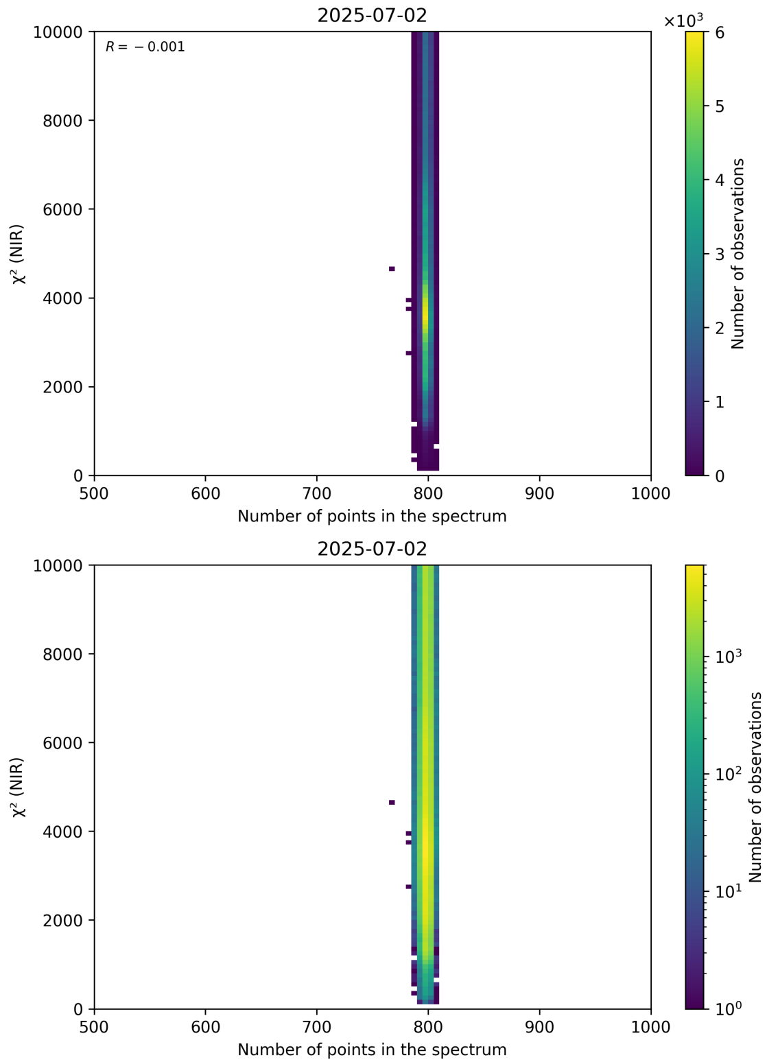
Figure 88: Scatter density plot of “Number of points in the spectrum” against “ \chi^2 (NIR)” for 2025-07-02 to 2025-07-03.
