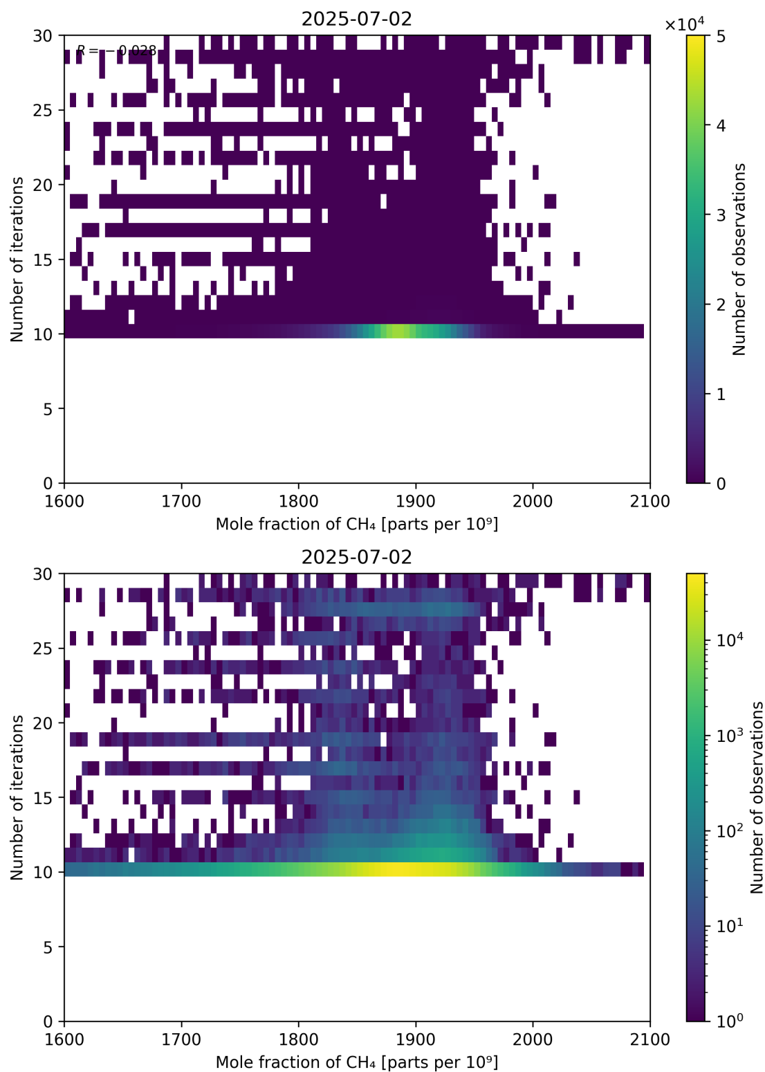
Figure 76: Scatter density plot of “Mole fraction of CH 4 ” against “Number of iterations” for 2025-07-02 to 2025-07-03.
