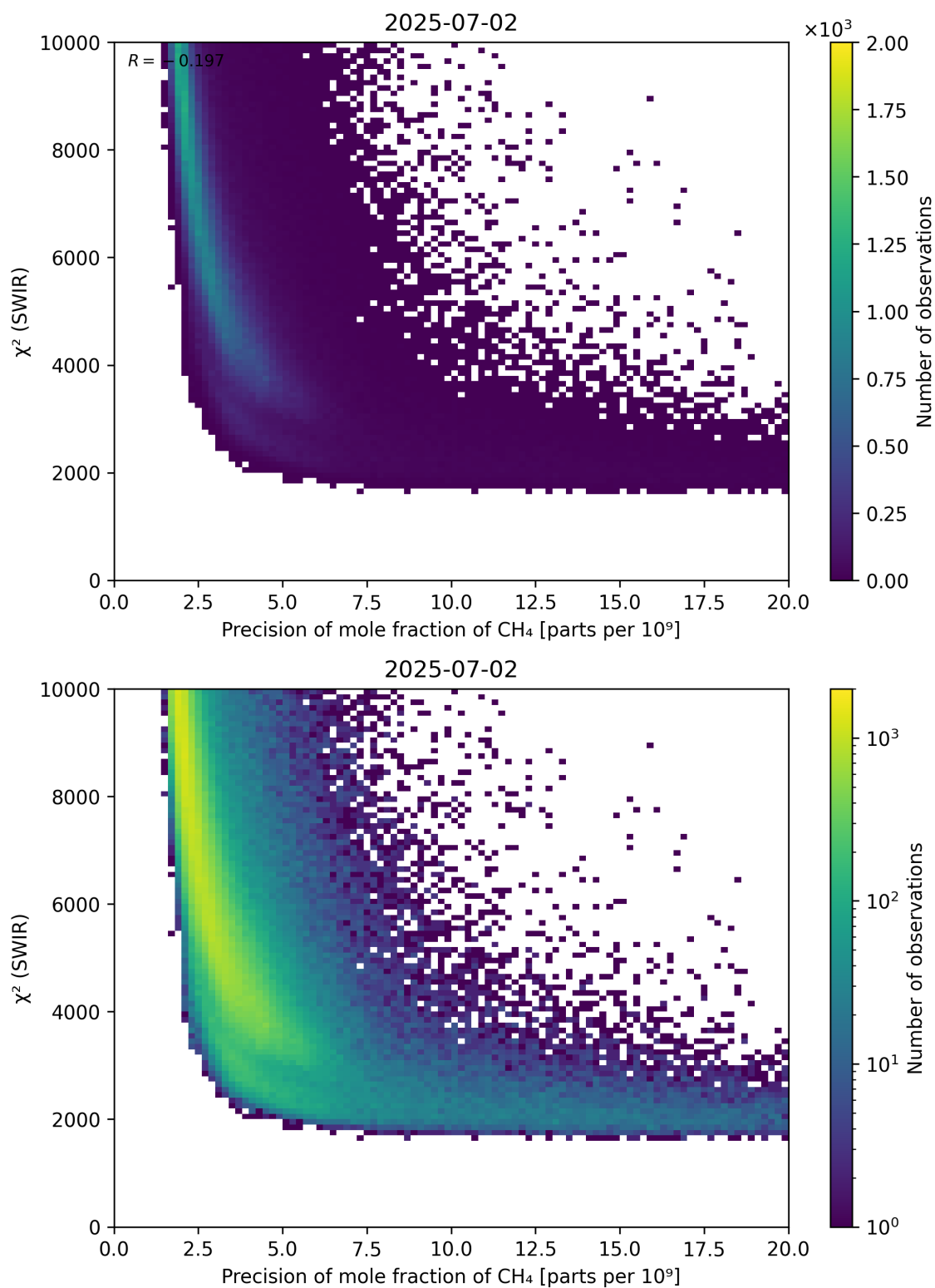
Figure 79: Scatter density plot of “Precision of mole fraction of CH 4 ” against “ \chi^2 (SWIR)” for 2025-07-02 to 2025-07-03.
