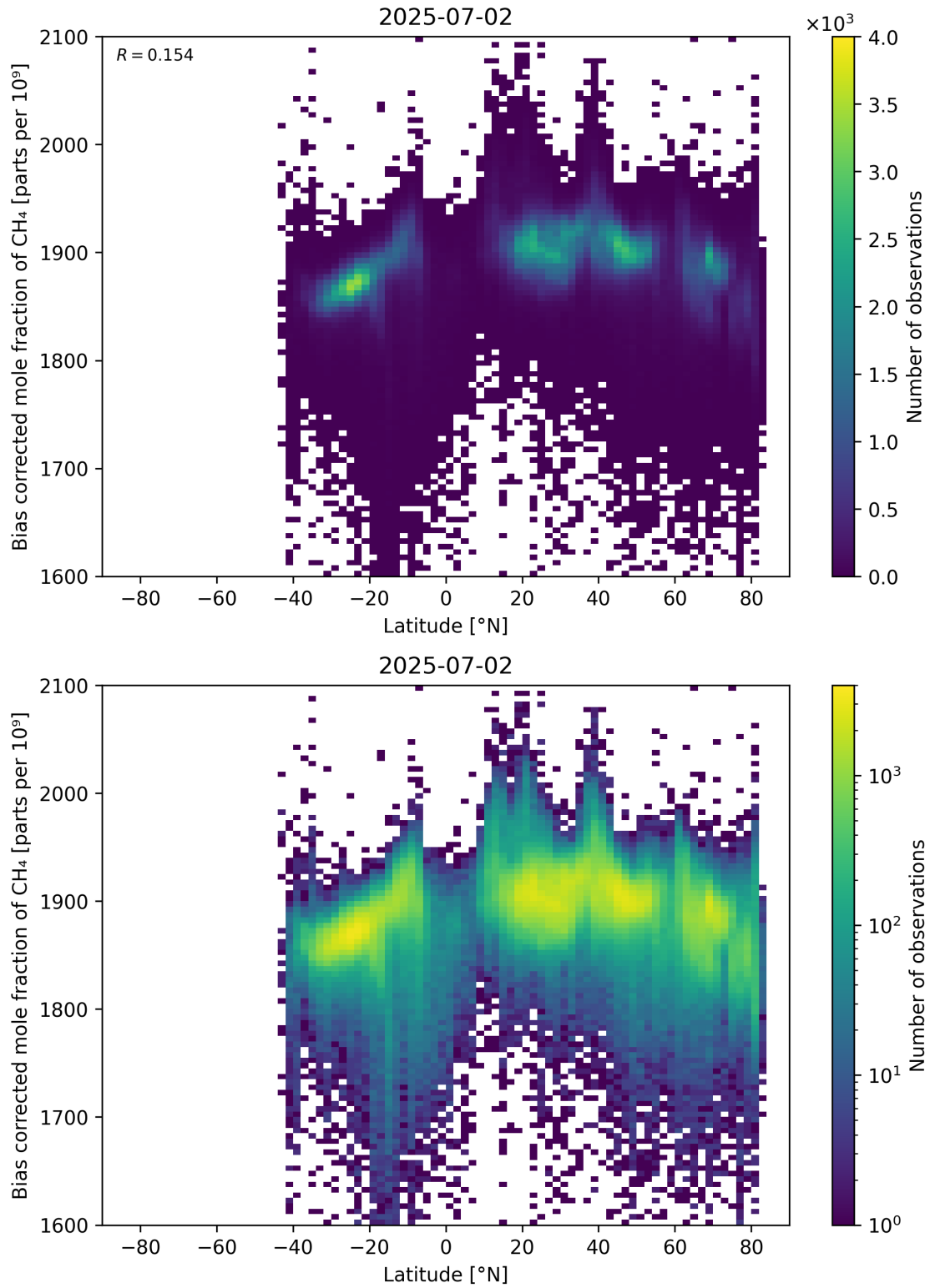
Figure 58: Scatter density plot of “Latitude” against “Bias corrected mole fraction of CH 4 ” for 2025-07-02 to 2025-07-03.
