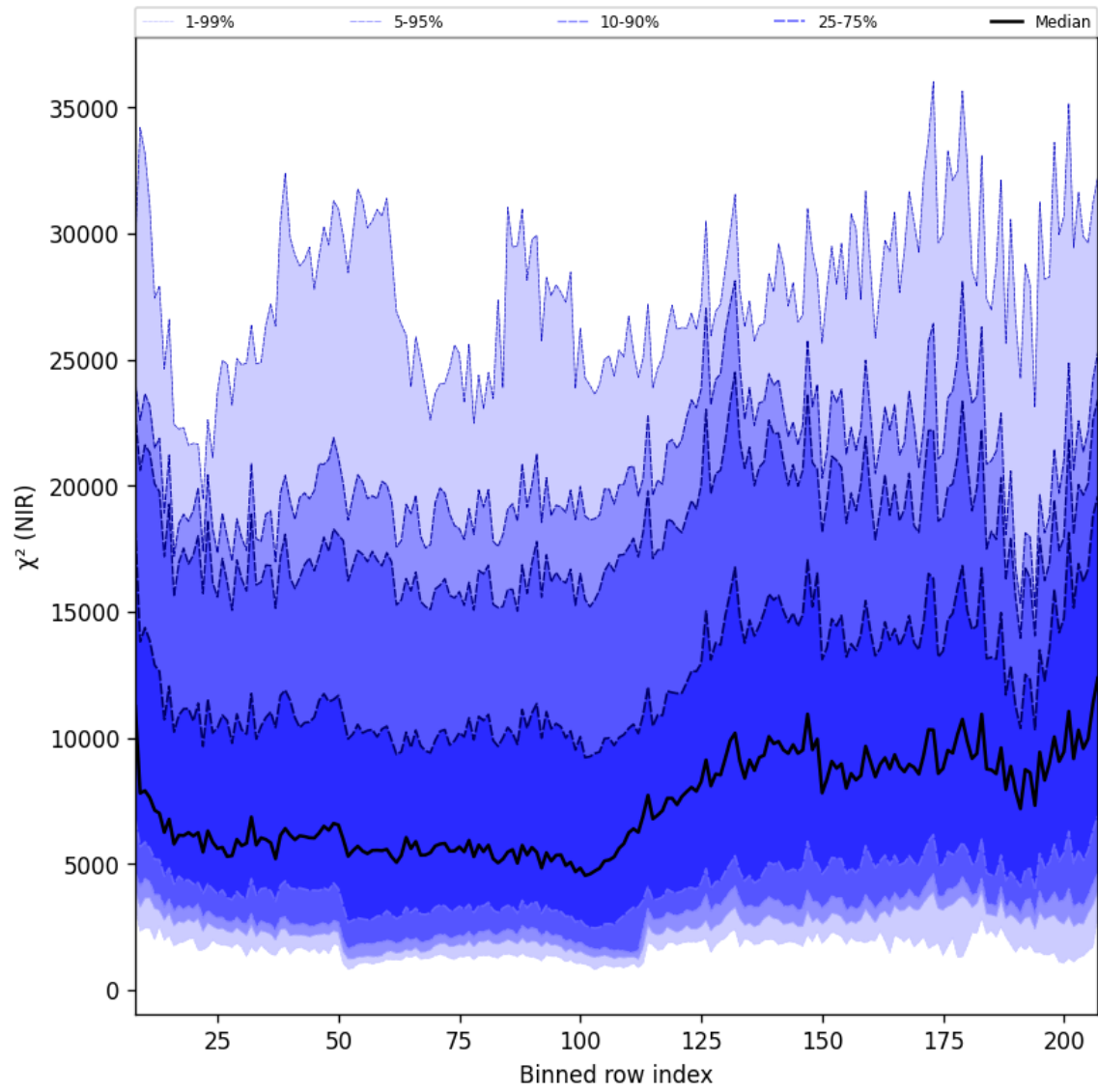
Figure 40: Along track statistics of “ \chi^2 (NIR)” for 2025-07-02 to 2025-07-03
