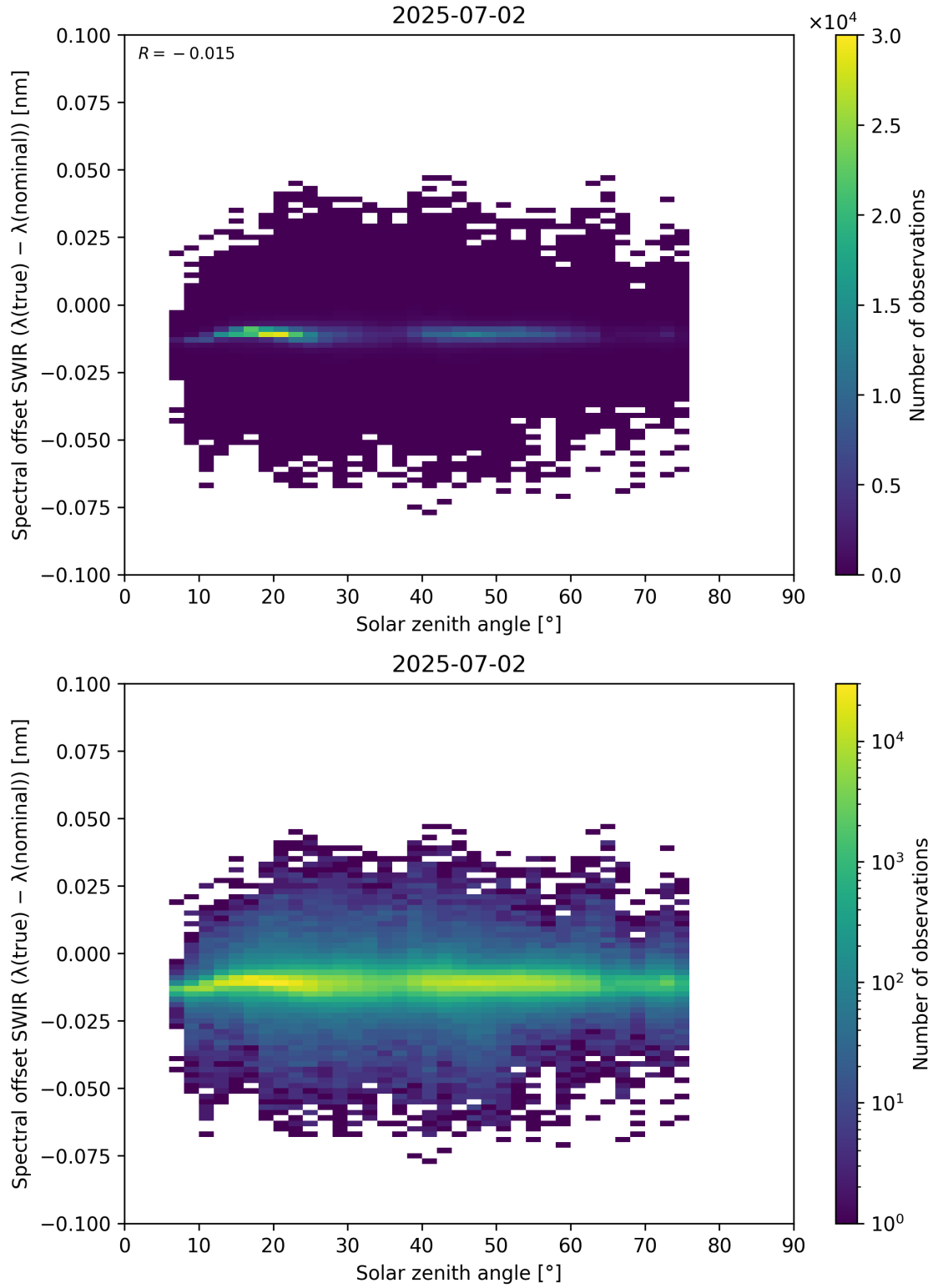
Figure 104: Scatter density plot of “Solar zenith angle” against “Spectral offset SWIR ( \lambda_{\text{true}} - \lambda_{\text{nominal}} )” for 2025-07-02 to 2025-07-03.
