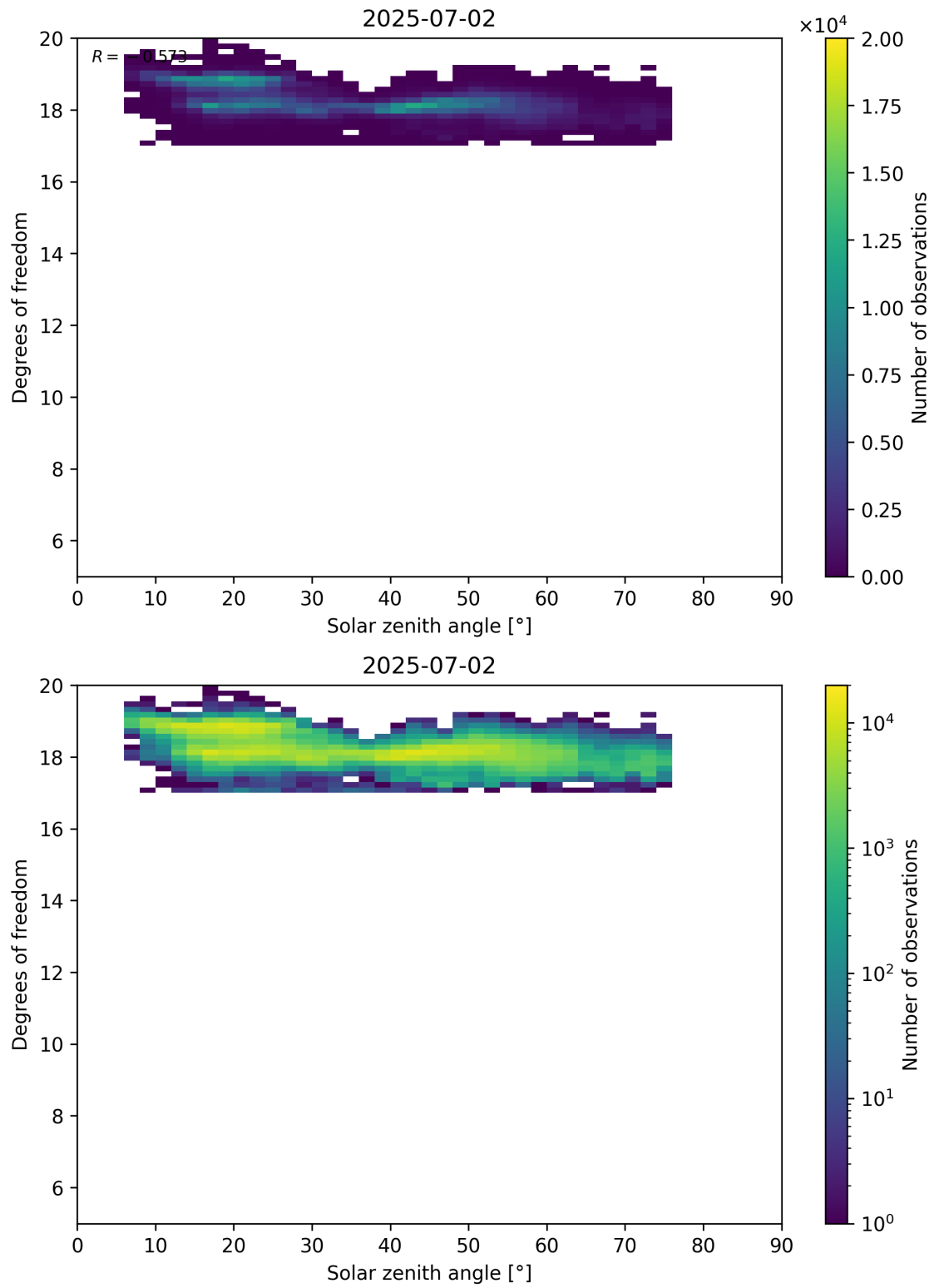
Figure 96: Scatter density plot of “Solar zenith angle” against “Degrees of freedom” for 2025-07-02 to 2025-07-03.
