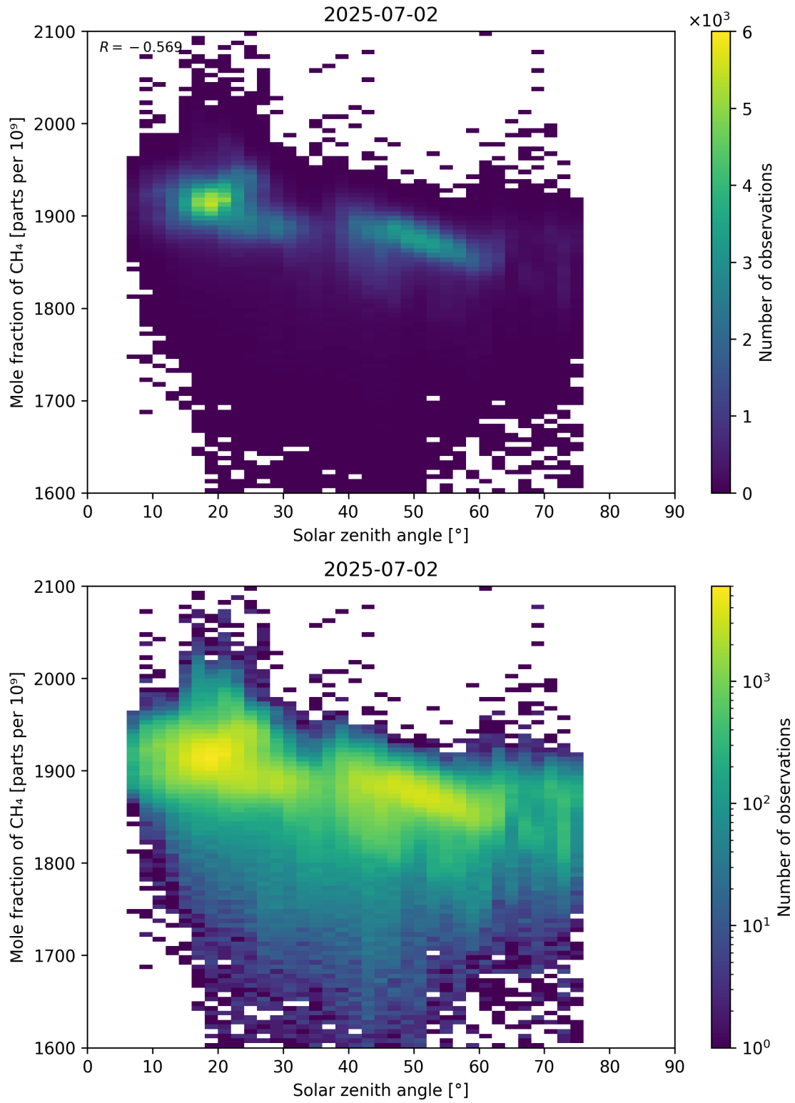
Figure 99: Scatter density plot of “Solar zenith angle” against “Mole fraction of CH 4 ” for 2025-07-02 to 2025-07-03.
