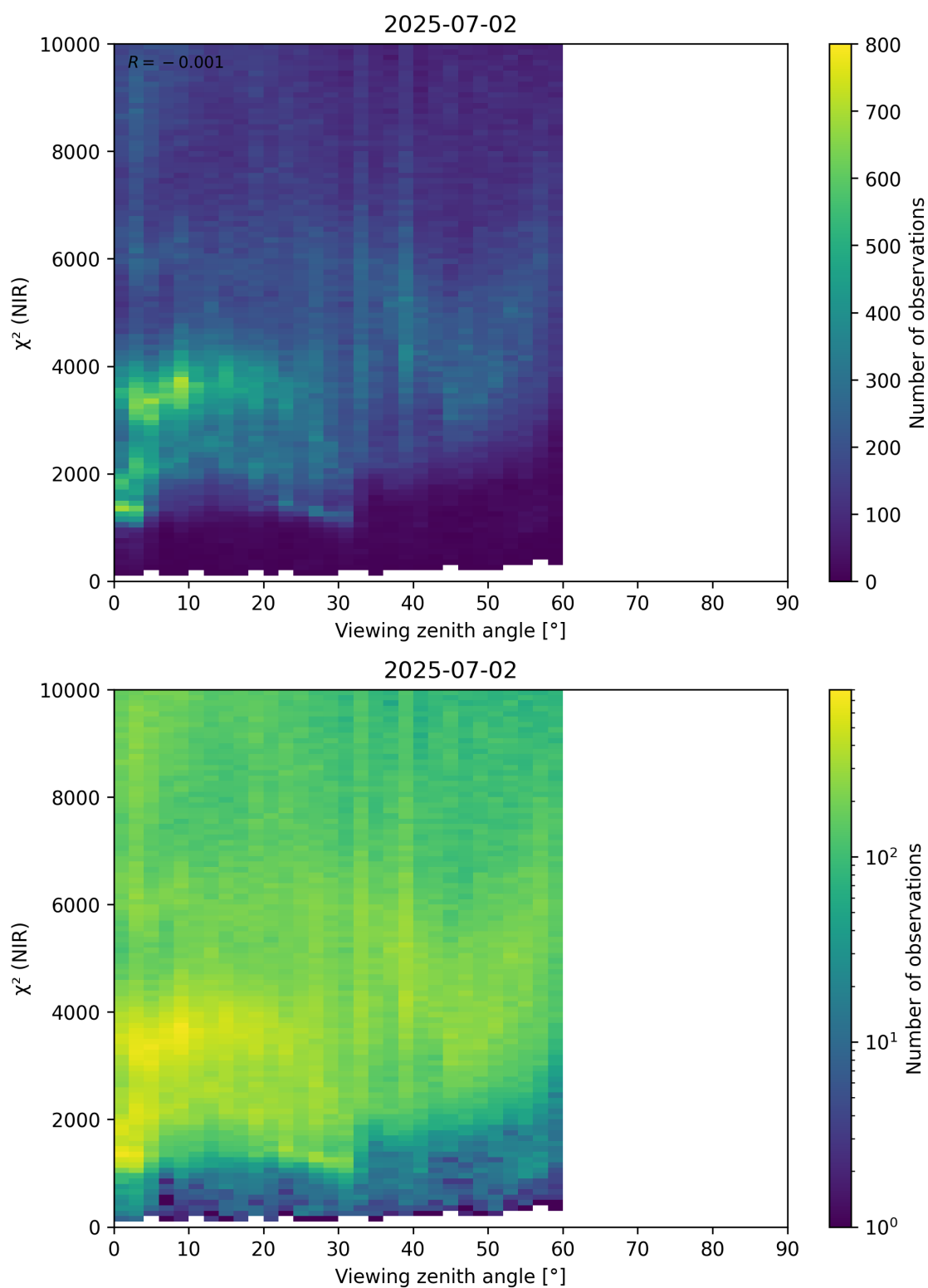
Figure 105: Scatter density plot of “Viewing zenith angle” against “ \chi^2 (NIR)” for 2025-07-02 to 2025-07-03.
