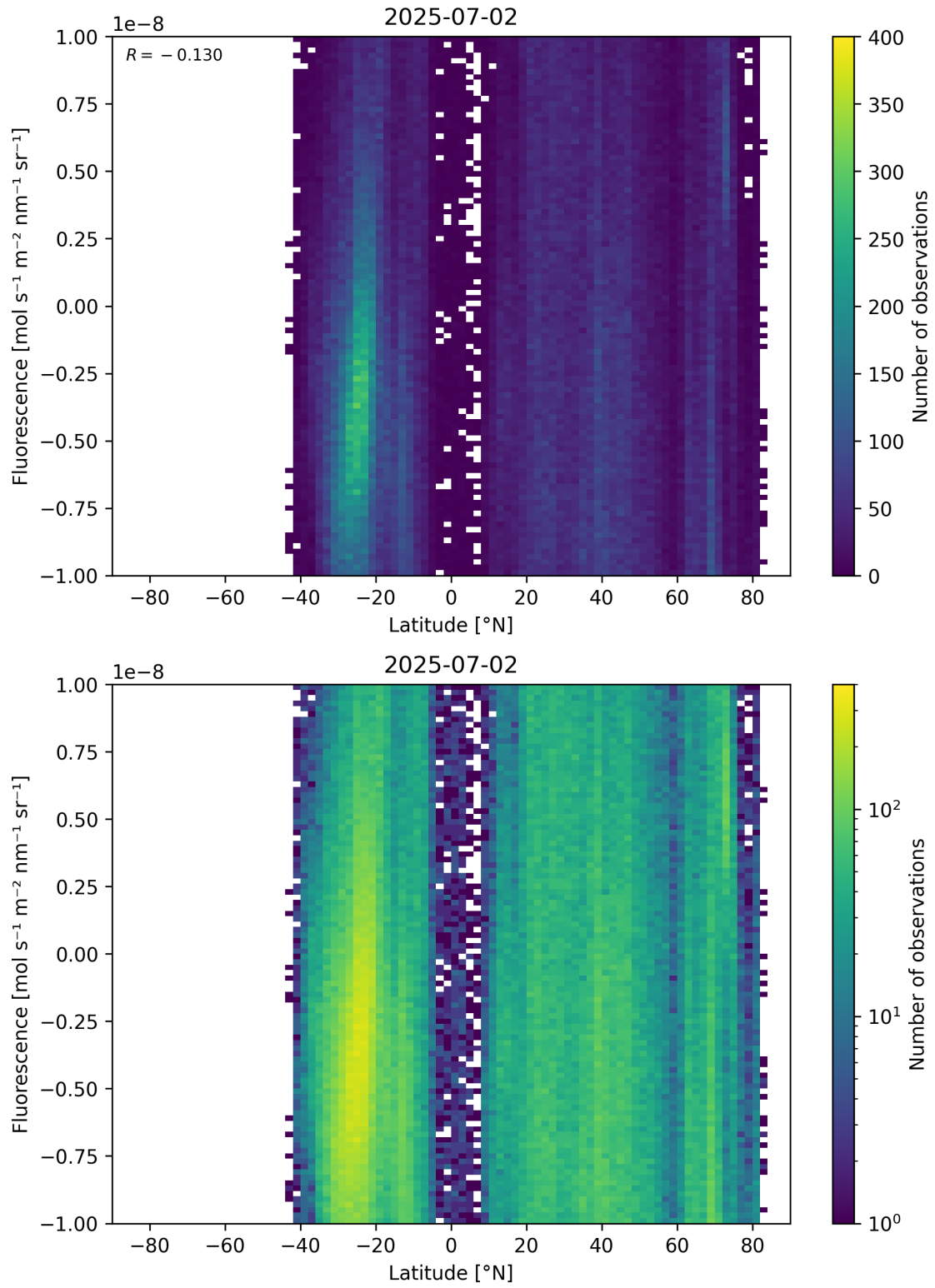
Figure 56: Scatter density plot of “Latitude” against “Fluorescence” for 2025-07-02 to 2025-07-03.
