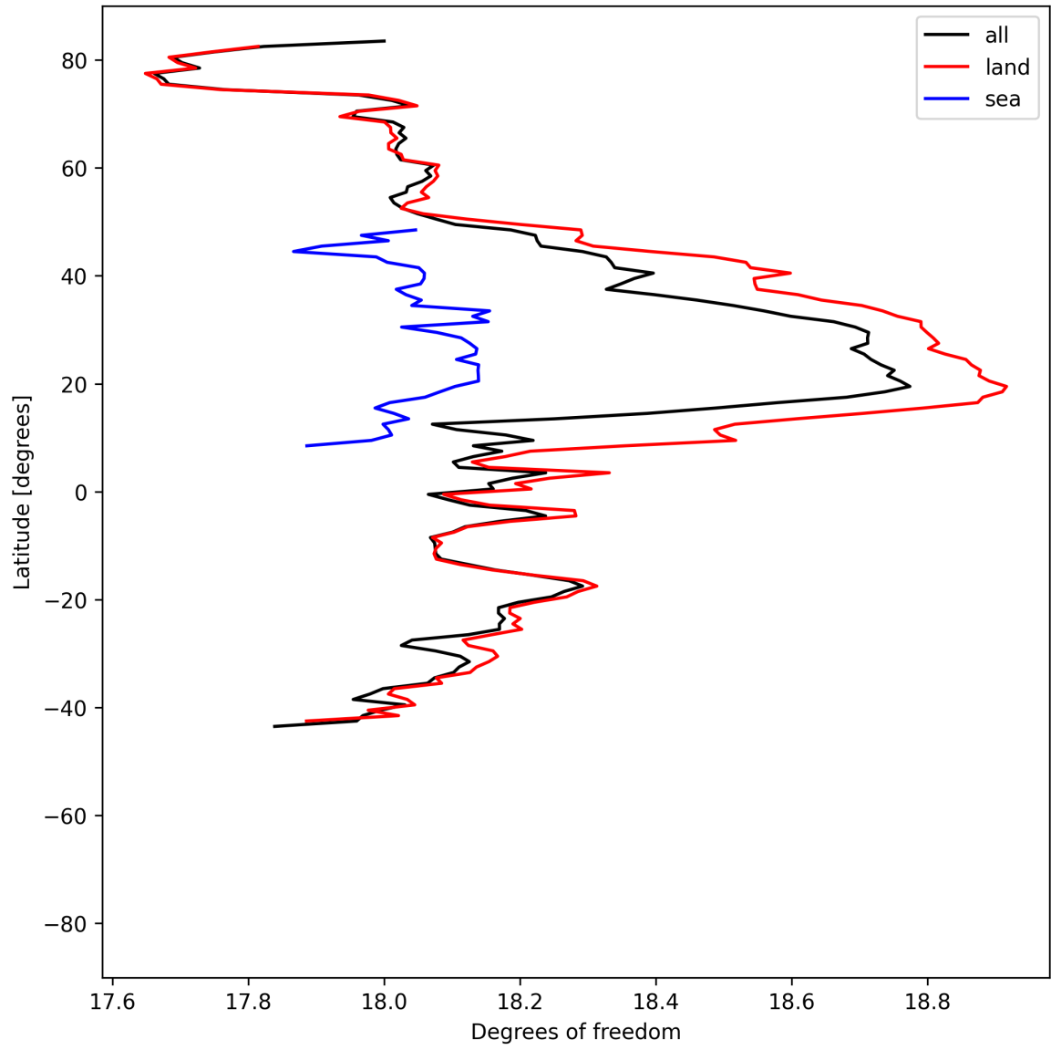
Figure 19: Zonal average of “Degrees of freedom” for 2025-07-02 to 2025-07-03.
