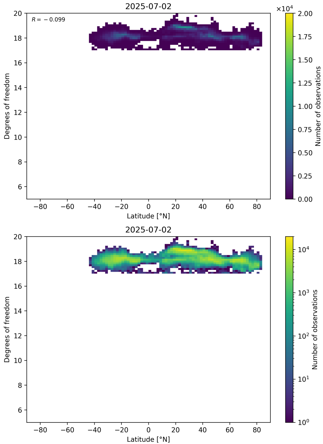
Figure 55: Scatter density plot of “Latitude” against “Degrees of freedom” for 2025-07-02 to 2025-07-03.
