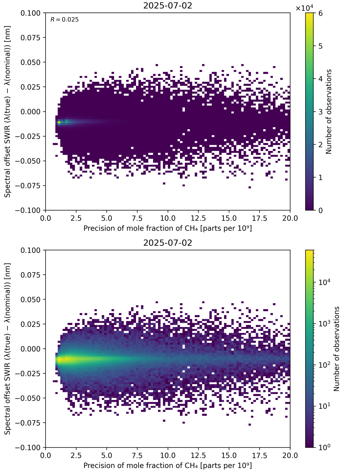
Figure 85: Scatter density plot of “Precision of mole fraction of \text{CH}_4 ” against “Spectral offset SWIR ( \lambda_{\text{true}} - \lambda_{\text{nominal}} )” for 2025-07-02 to 2025-07-03.
