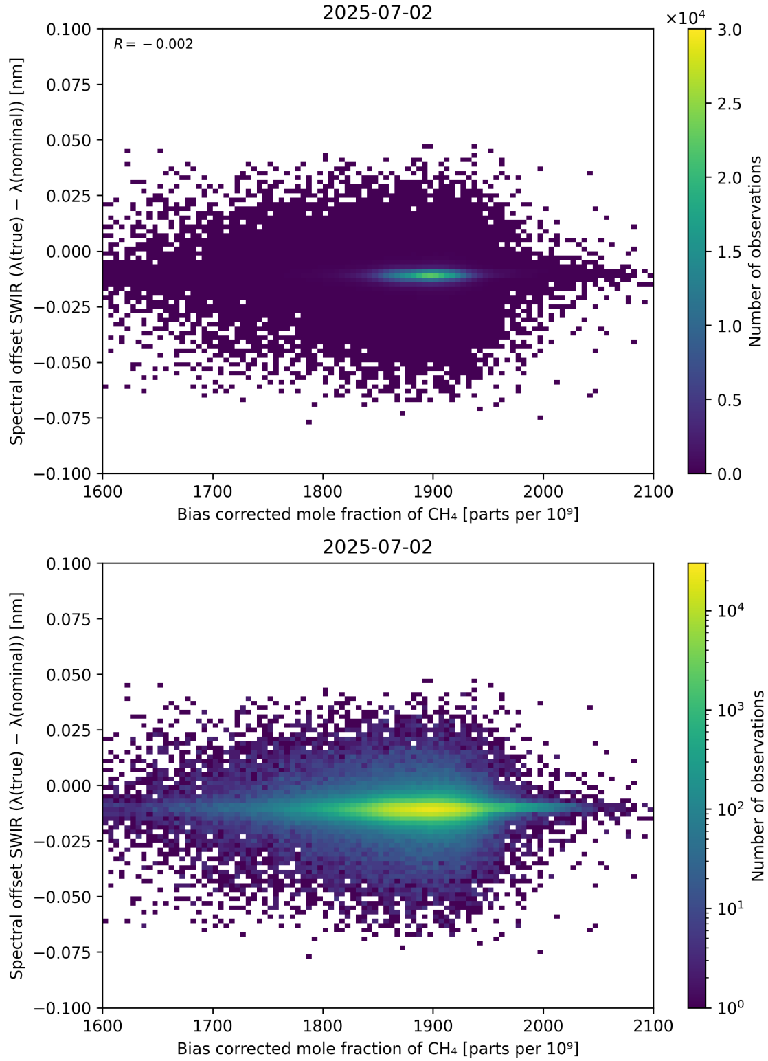
Figure 69: Scatter density plot of “Bias corrected mole fraction of CH 4 ” against “Spectral offset SWIR ( \lambda_{\text{true}} - \lambda_{\text{nominal}} )” for 2025-07-02 to 2025-07-03.
