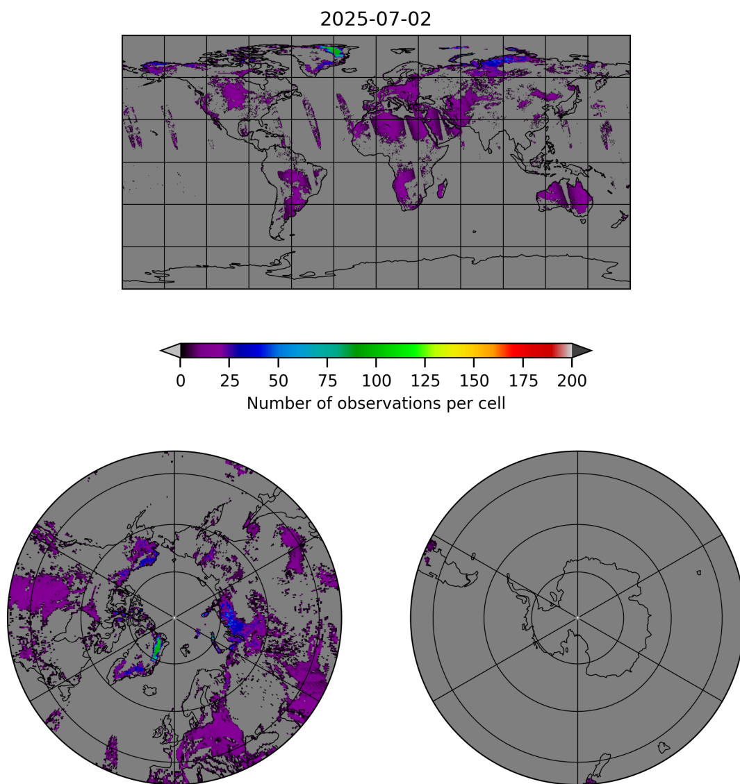
Figure 10: Map of the number of observations for 2025-07-02 to 2025-07-03
