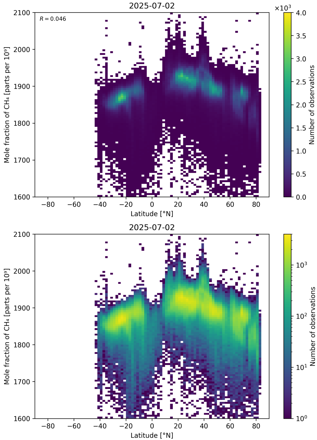
Figure 57: Scatter density plot of “Latitude” against “Mole fraction of CH 4 ” for 2025-07-02 to 2025-07-03.
