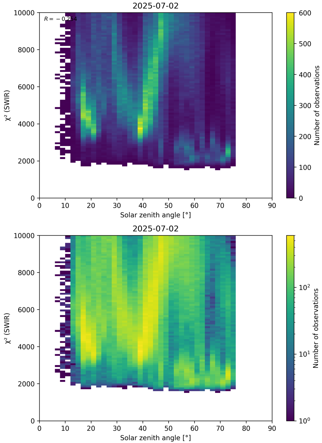
Figure 95: Scatter density plot of “Solar zenith angle” against “ \chi^2 (SWIR)” for 2025-07-02 to 2025-07-03.
