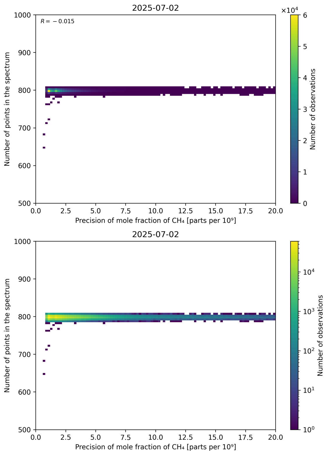
Figure 84: Scatter density plot of “Precision of mole fraction of CH 4 ” against “Number of points in the spectrum” for 2025-07-02 to 2025-07-03.
