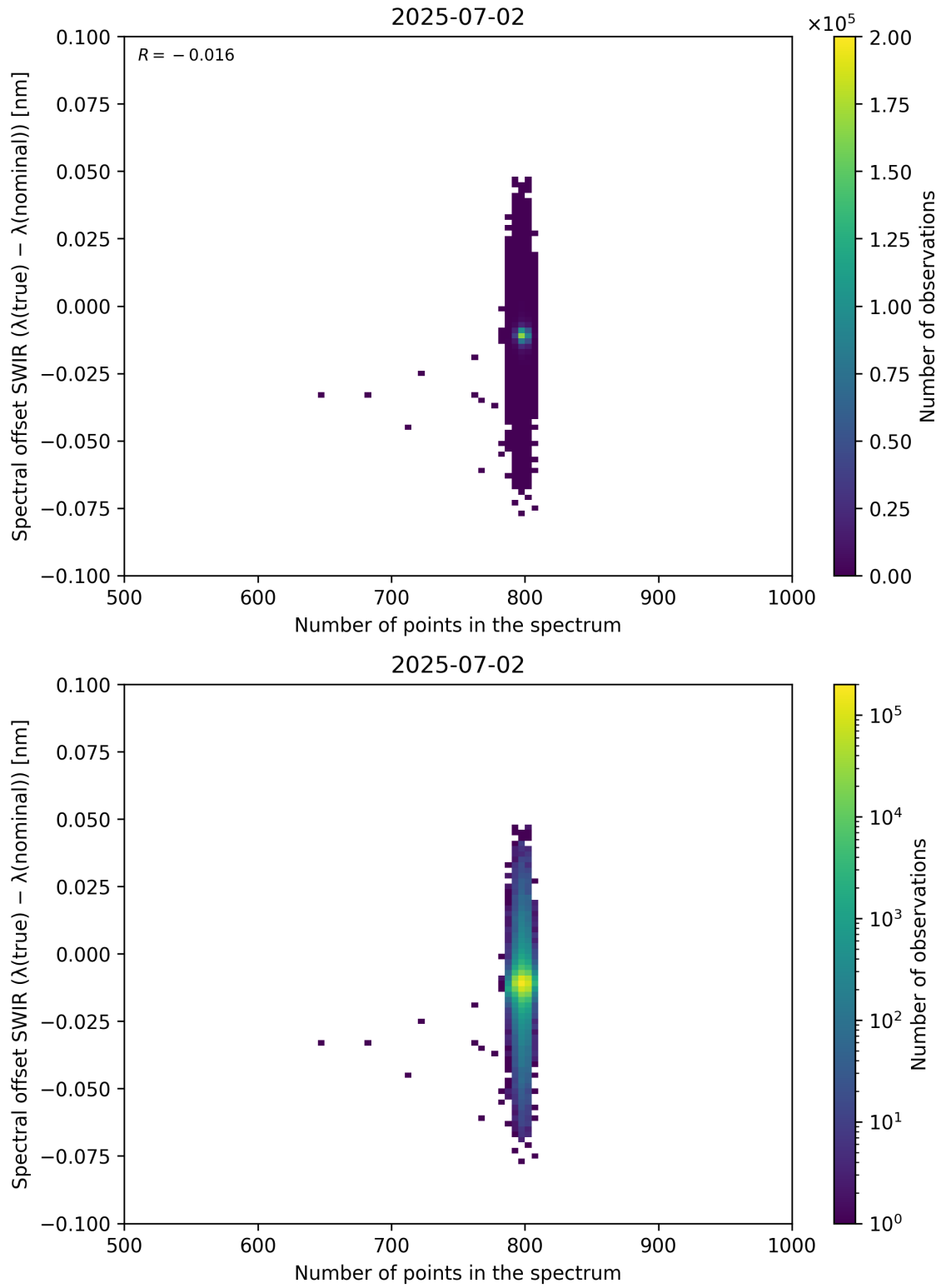
Figure 93: Scatter density plot of “Number of points in the spectrum” against “Spectral offset SWIR ( \lambda_{\text{true}} - \lambda_{\text{nominal}} )” for 2025-07-02 to 2025-07-03.
