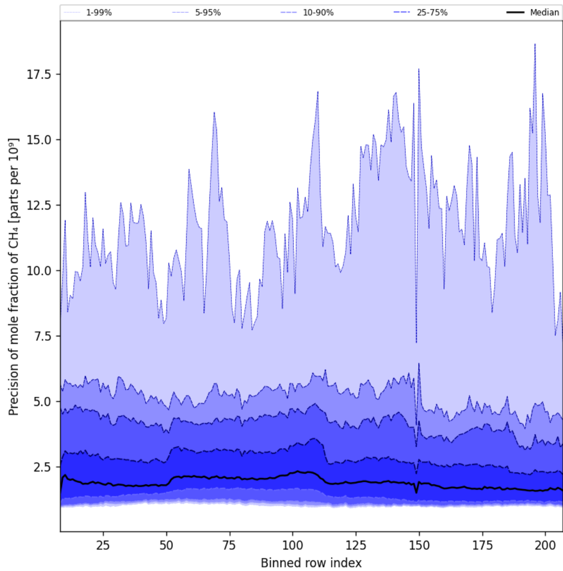
Figure 35: Along track statistics of “Precision of mole fraction of CH 4 ” for 2025-07-02 to 2025-07-03
