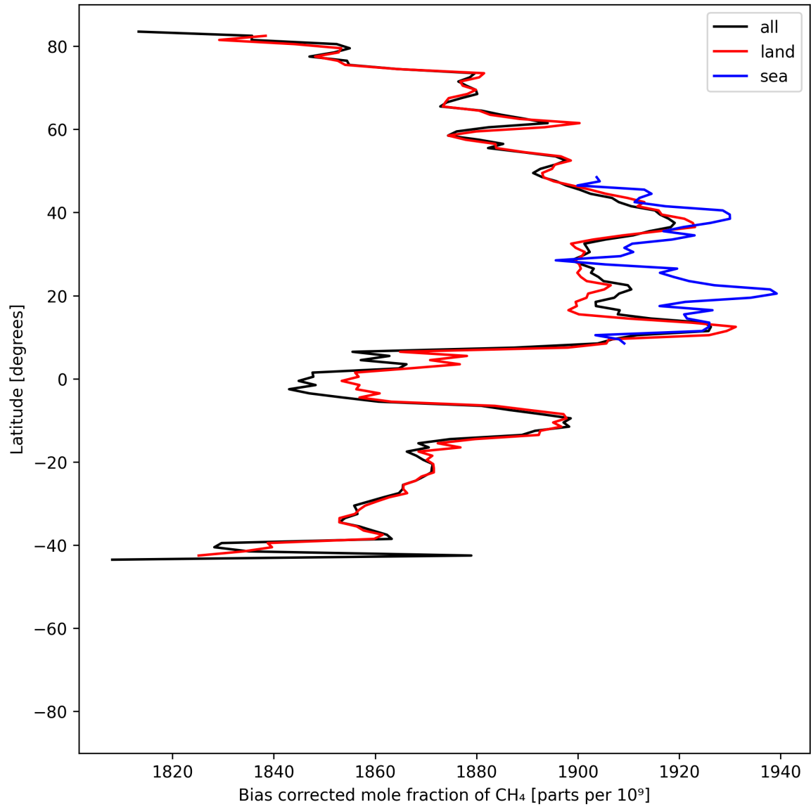
Figure 14: Zonal average of “Bias corrected mole fraction of CH 4 ” for 2025-07-02 to 2025-07-03.
