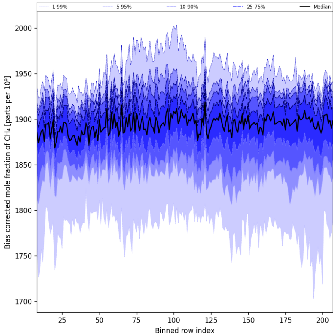
Figure 36: Along track statistics of “Bias corrected mole fraction of CH 4 ” for 2025-07-02 to 2025-07-03
