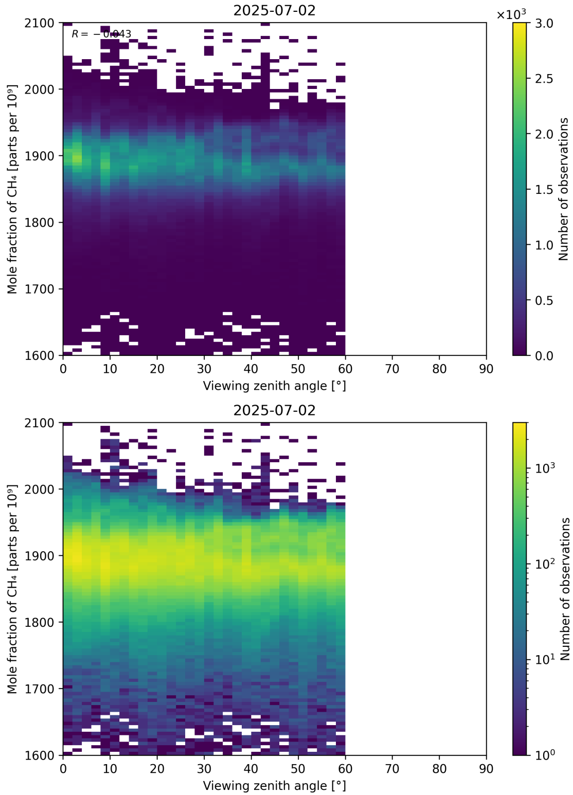
Figure 110: Scatter density plot of “Viewing zenith angle” against “Mole fraction of CH 4 ” for 2025-07-02 to 2025-07-03.
