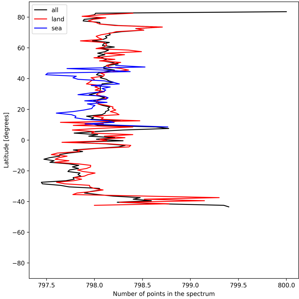
Figure 15: Zonal average of “Number of points in the spectrum” for 2025-07-02 to 2025-07-03.
