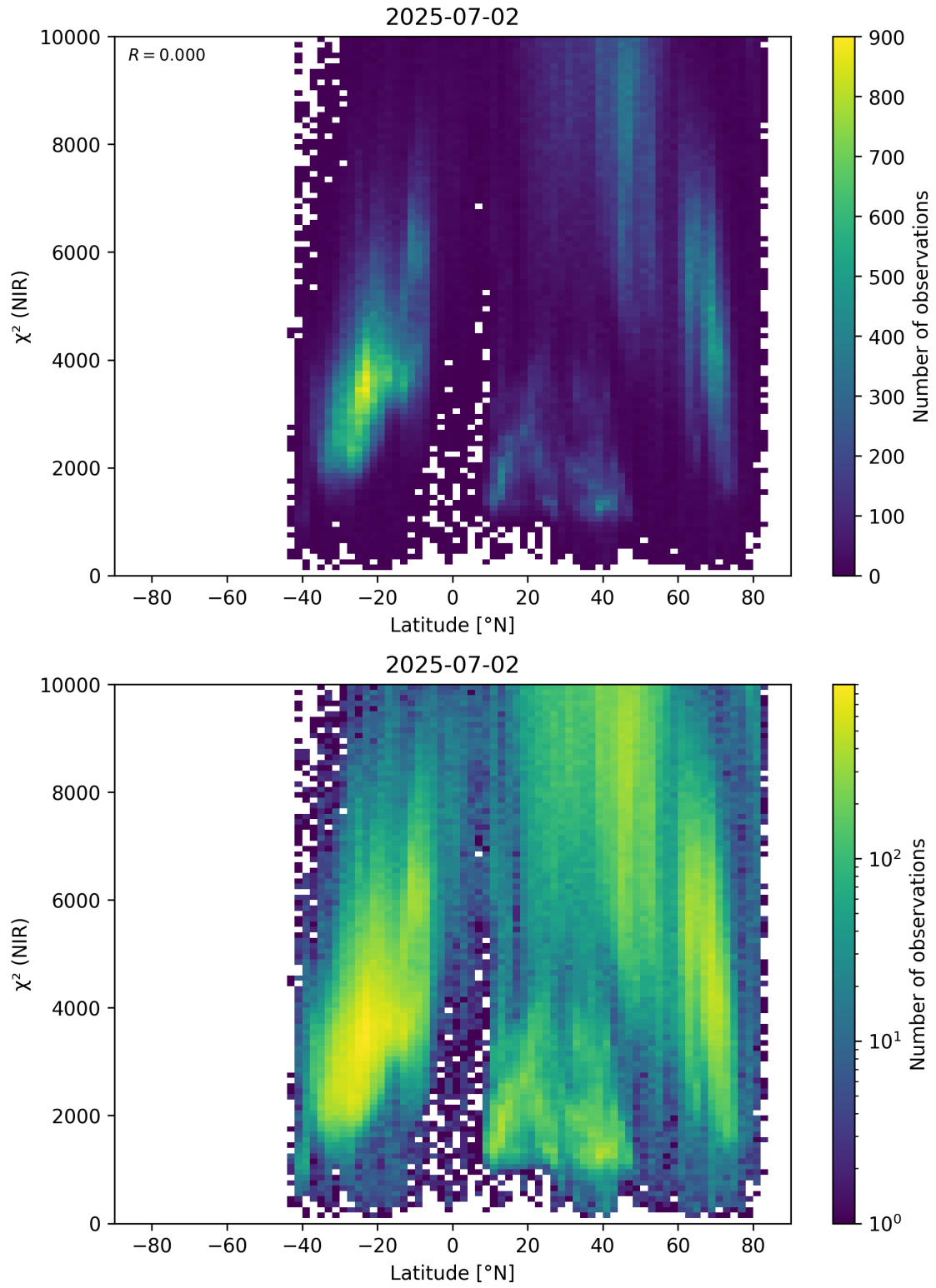
Figure 53: Scatter density plot of “Latitude” against “ \chi^2 (NIR)” for 2025-07-02 to 2025-07-03.
