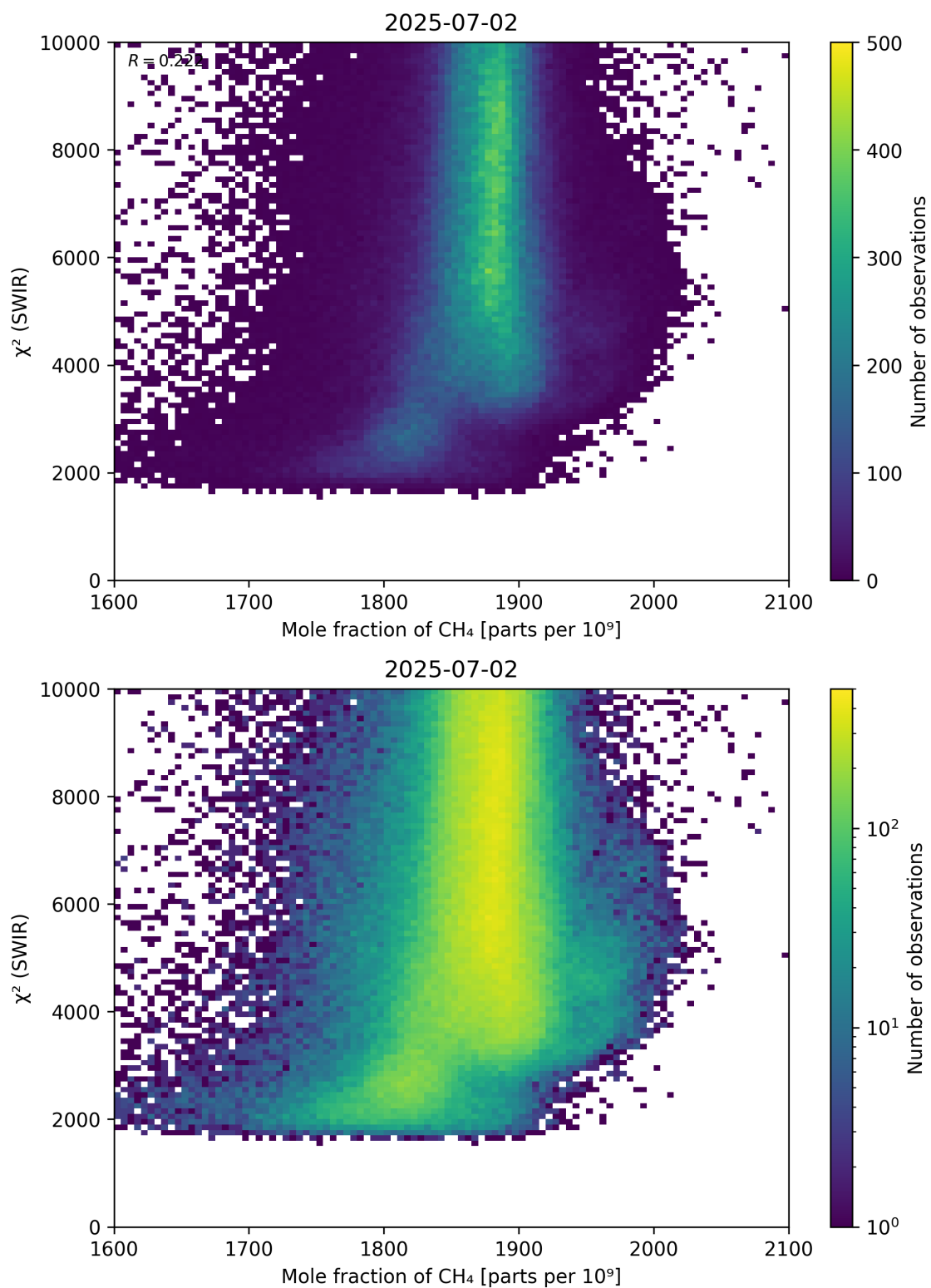
Figure 71: Scatter density plot of “Mole fraction of CH 4 ” against “ \chi^2 (SWIR)” for 2025-07-02 to 2025-07-03.
