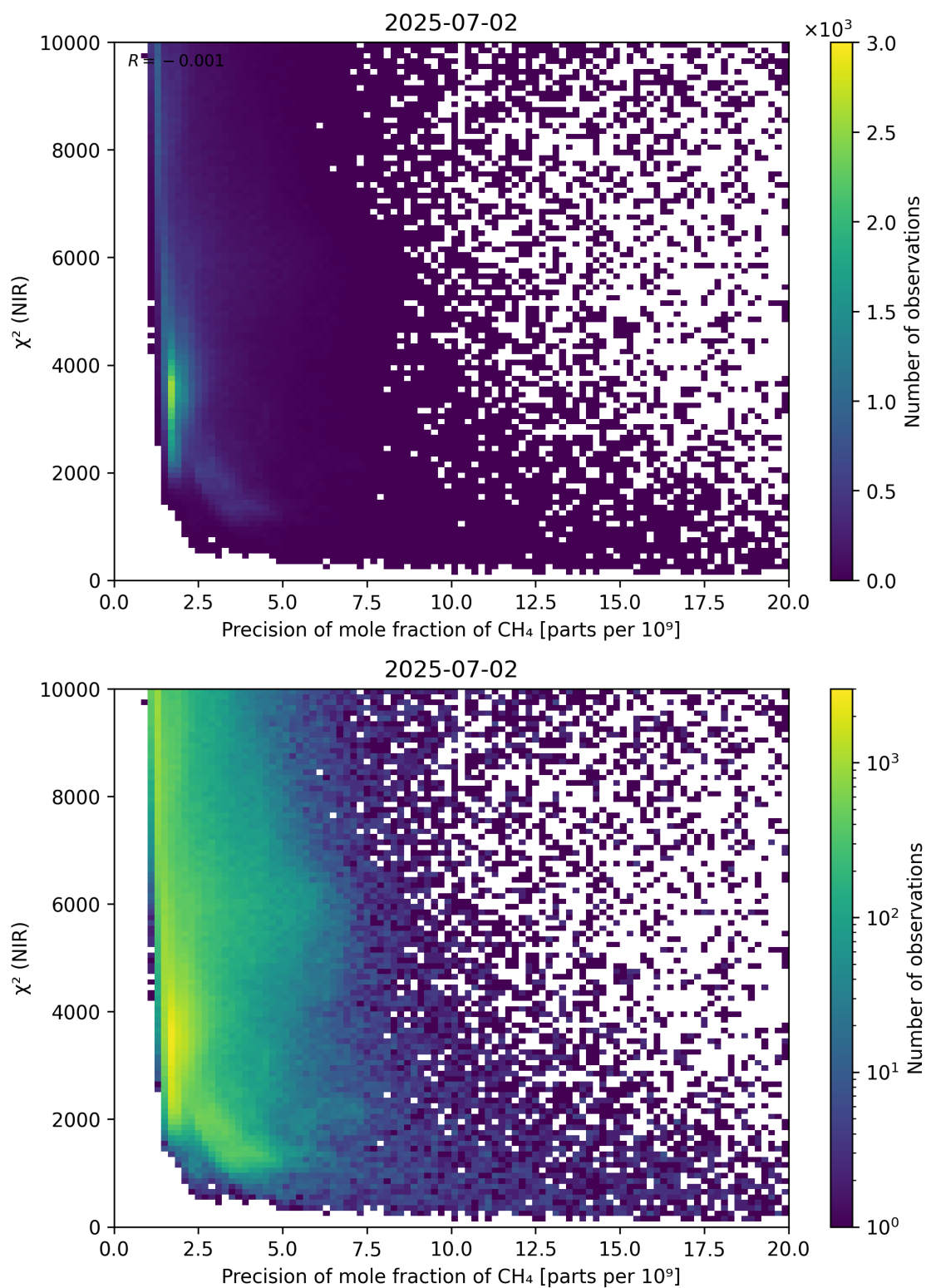
Figure 78: Scatter density plot of “Precision of mole fraction of CH 4 ” against “ \chi^2 (NIR)” for 2025-07-02 to 2025-07-03.
