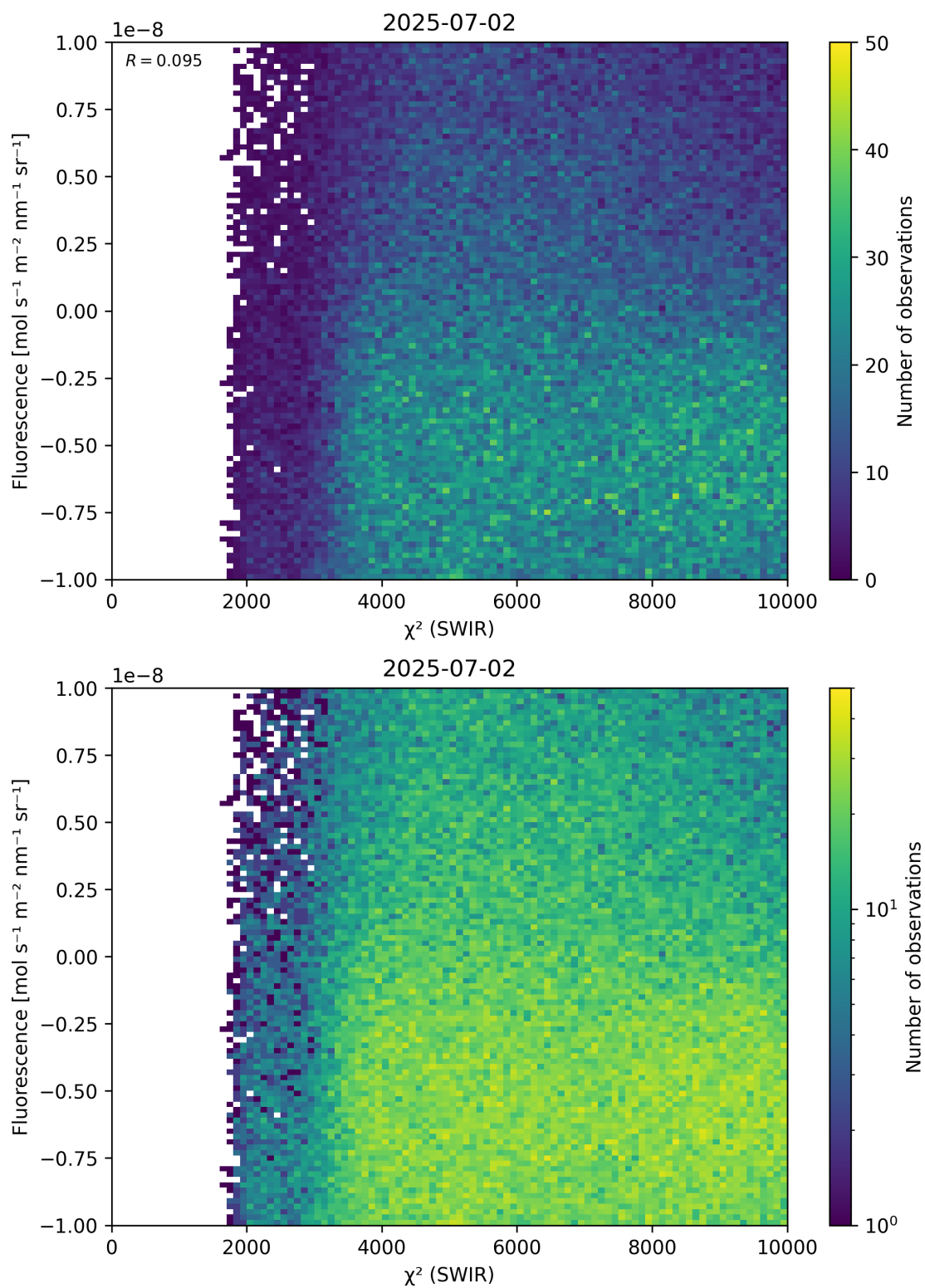
Figure 49: Scatter density plot of “ \chi^2 (SWIR)” against “Fluorescence” for 2025-07-02 to 2025-07-03.
