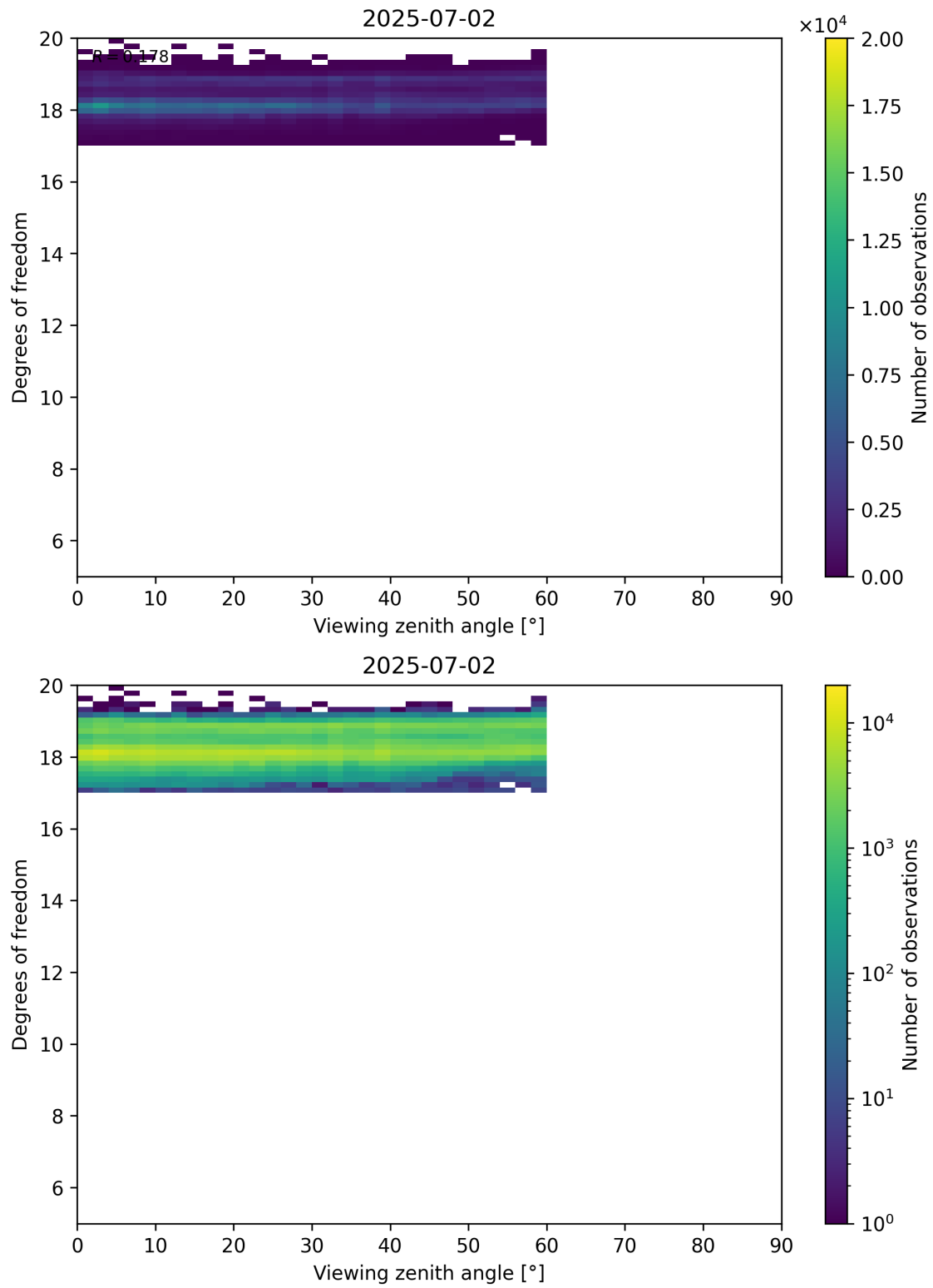
Figure 107: Scatter density plot of “Viewing zenith angle” against “Degrees of freedom” for 2025-07-02 to 2025-07-03.
