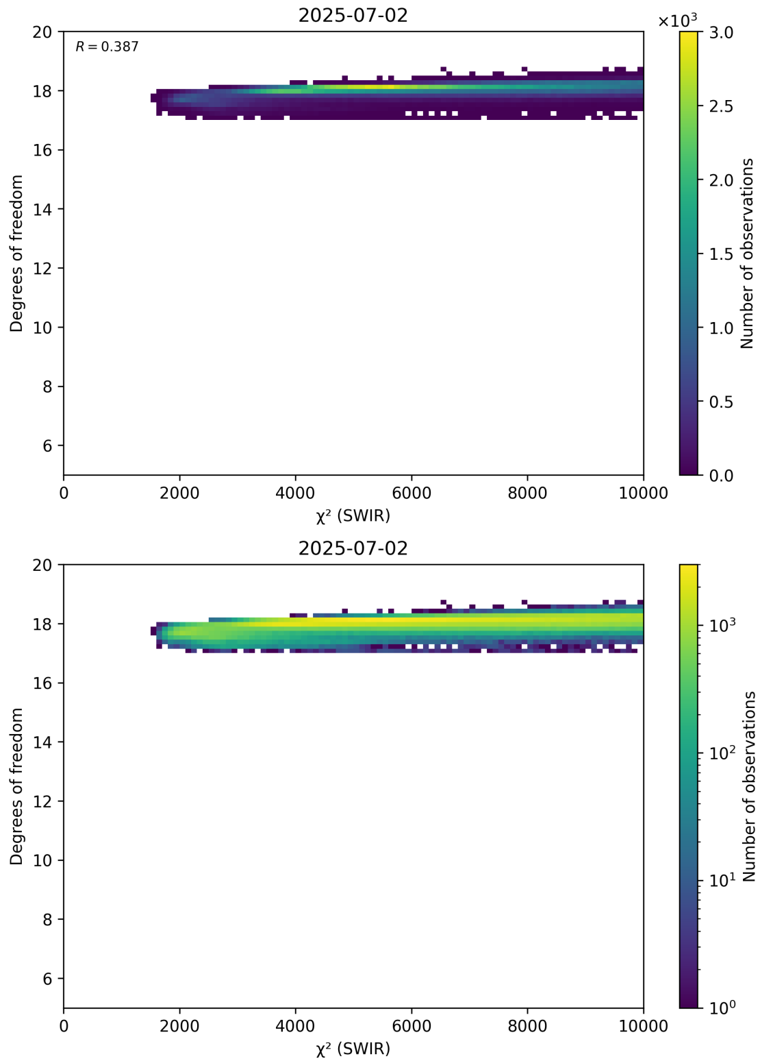
Figure 48: Scatter density plot of “ \chi^2 (SWIR)” against “Degrees of freedom” for 2025-07-02 to 2025-07-03.
