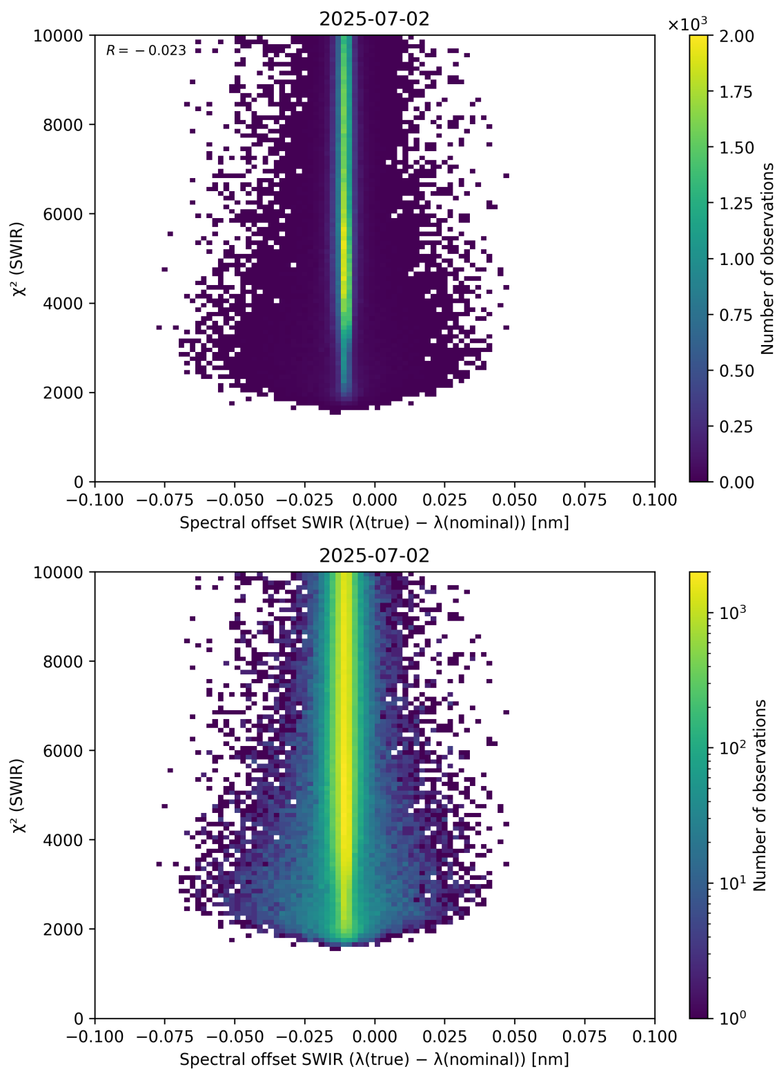
Figure 118: Scatter density plot of “Spectral offset SWIR ( \lambda_{\text{true}} - \lambda_{\text{nominal}} )” against “ \chi^2 (SWIR)” for 2025-07-02 to 2025-07-03.
