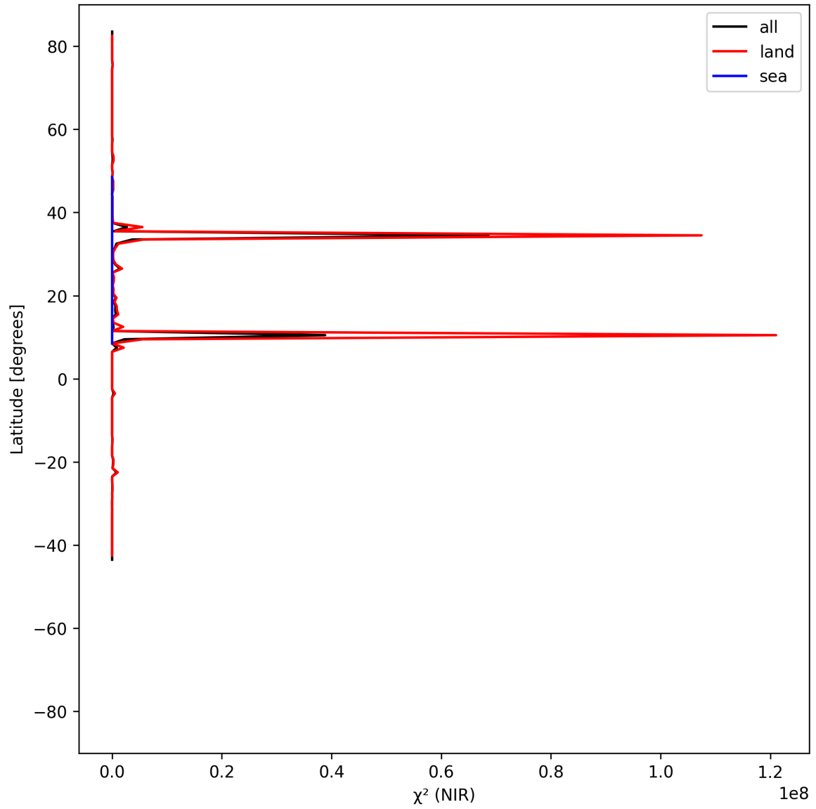
Figure 18: Zonal average of “ \chi^2 (NIR)” for 2025-07-02 to 2025-07-03.
