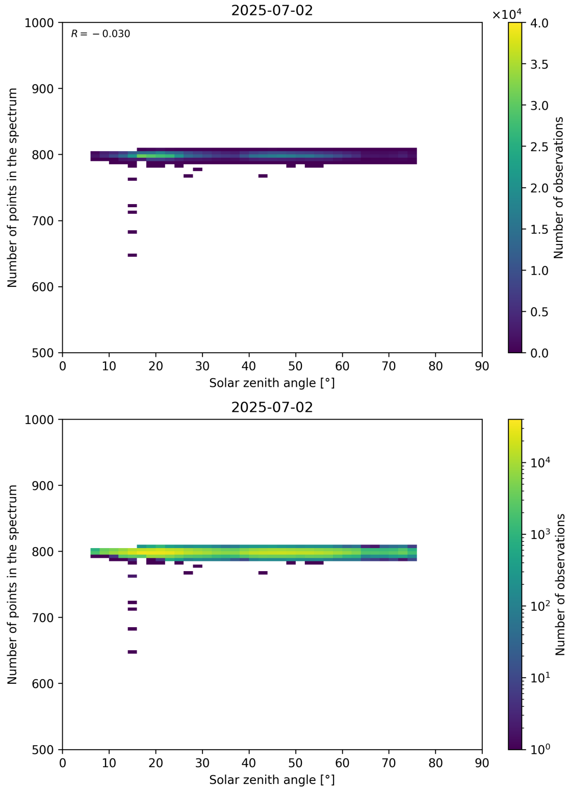
Figure 103: Scatter density plot of “Solar zenith angle” against “Number of points in the spectrum” for 2025-07-02 to 2025-07-03.
