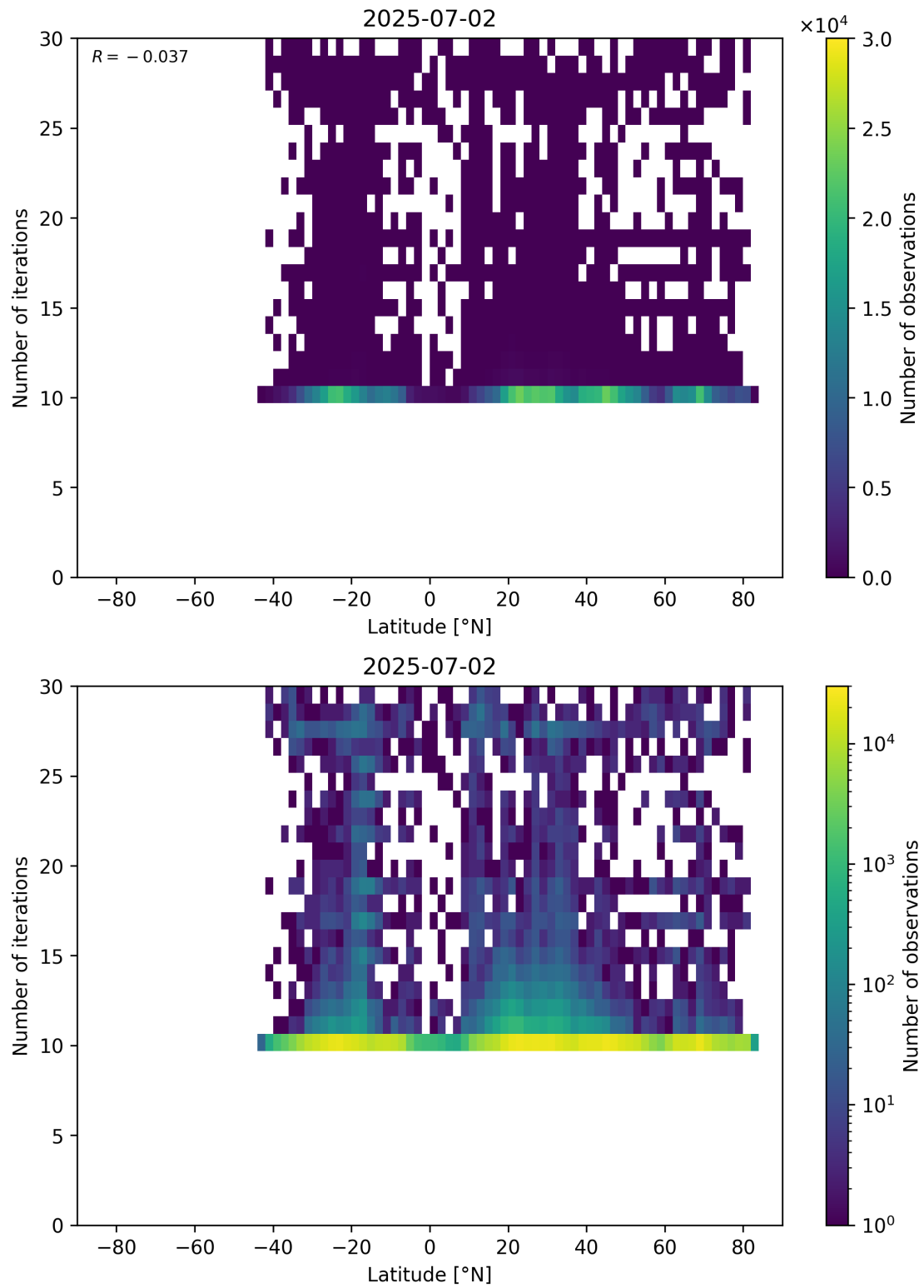
Figure 60: Scatter density plot of “Latitude” against “Number of iterations” for 2025-07-02 to 2025-07-03.
