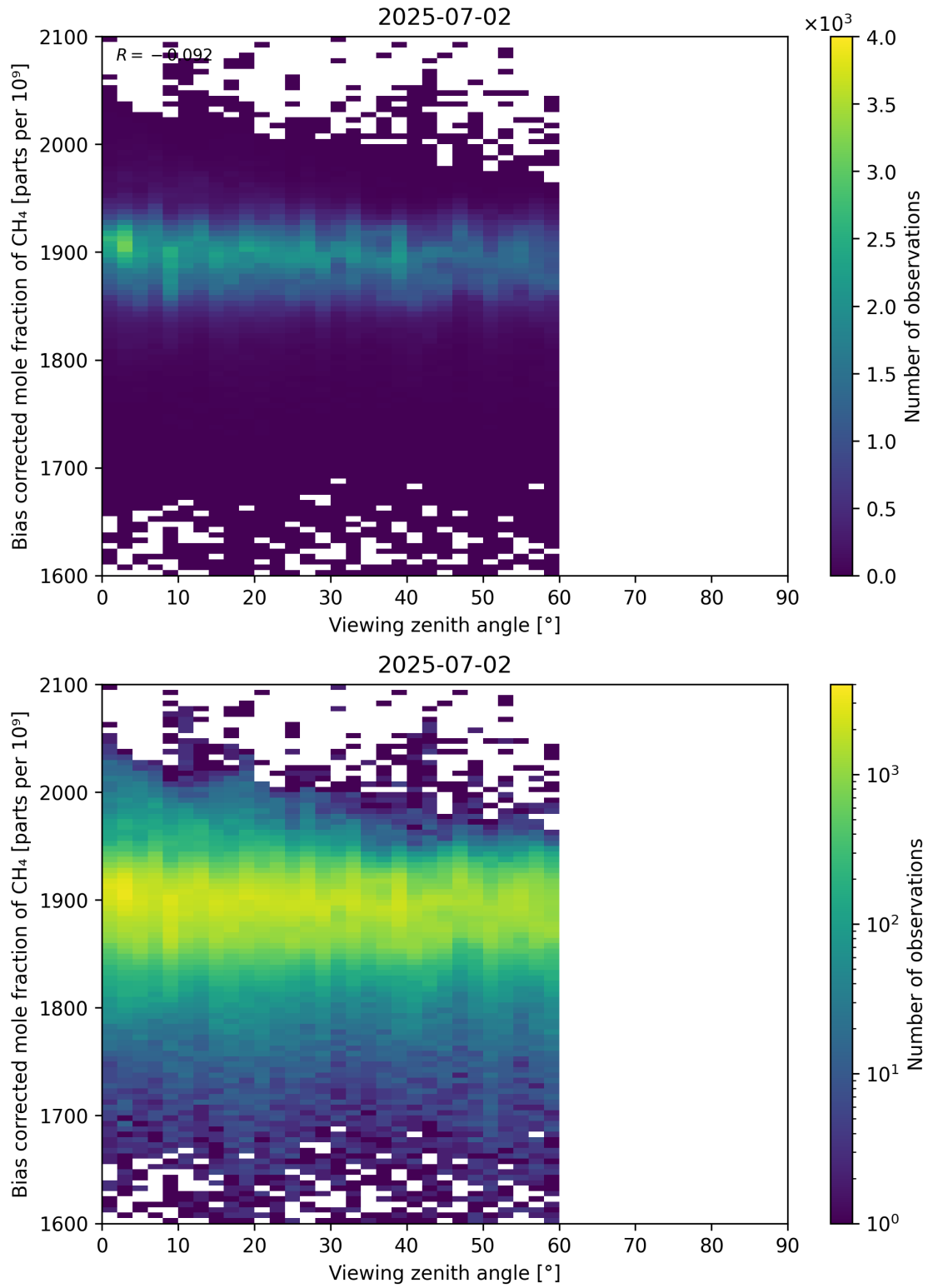
Figure 111: Scatter density plot of “Viewing zenith angle” against “Bias corrected mole fraction of CH 4 ” for 2025-07-02 to 2025-07-03.
