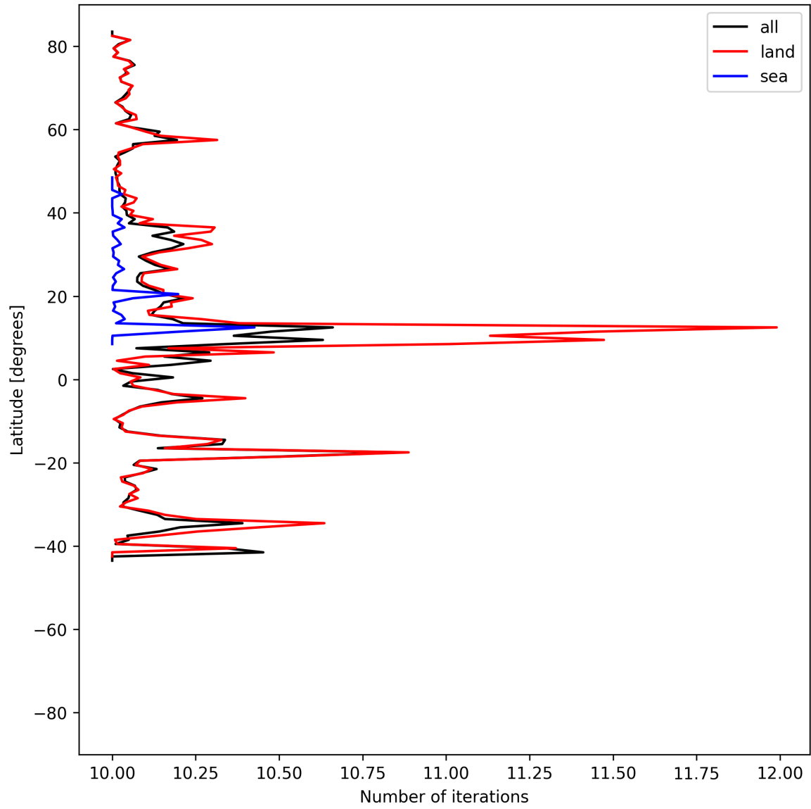
Figure 20: Zonal average of “Number of iterations” for 2025-07-02 to 2025-07-03.
