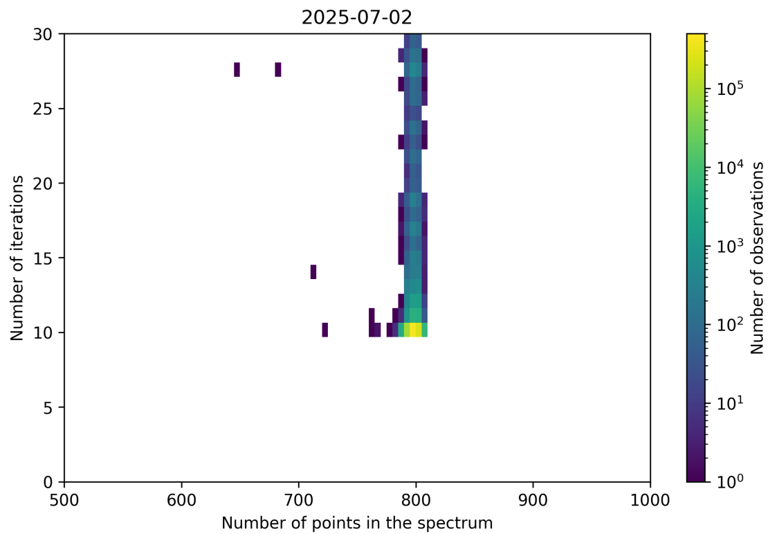
Figure 92: Scatter density plot of “Number of points in the spectrum” against “Number of iterations” for 2025-07-02 to 2025-07-03.
