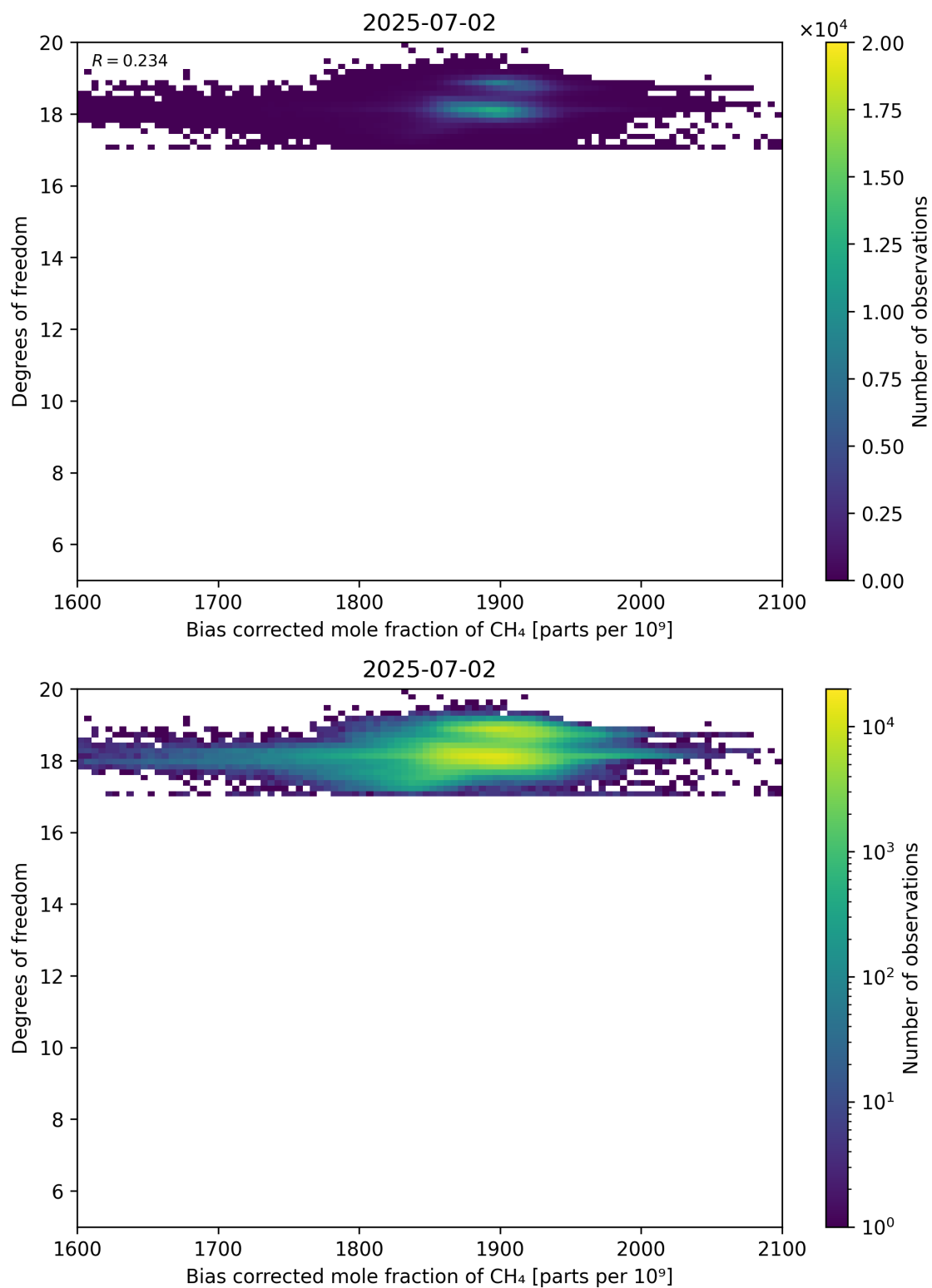
Figure 65: Scatter density plot of “Bias corrected mole fraction of CH 4 ” against “Degrees of freedom” for 2025-07-02 to 2025-07-03.
