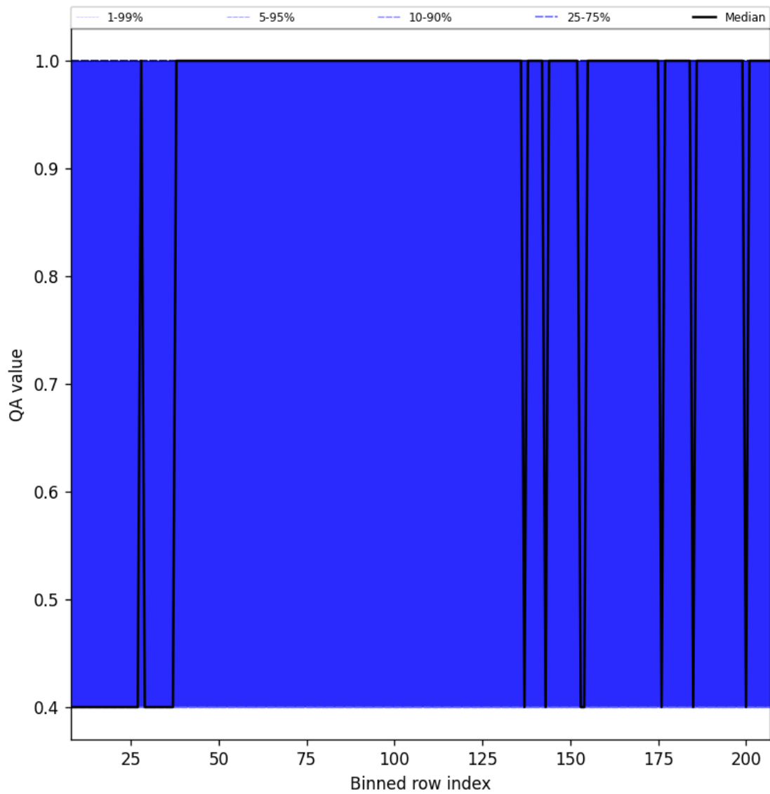
Figure 33: Along track statistics of “QA value” for 2025-07-02 to 2025-07-03
