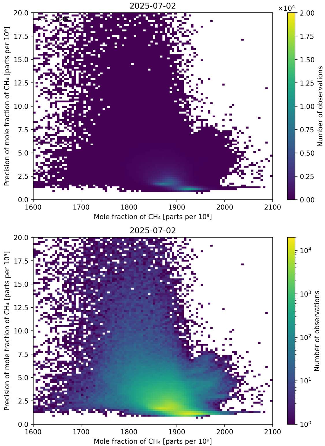
Figure 75: Scatter density plot of “Mole fraction of CH 4 ” against “Precision of mole fraction of CH 4 ” for 2025-07-02 to 2025-07-03.
