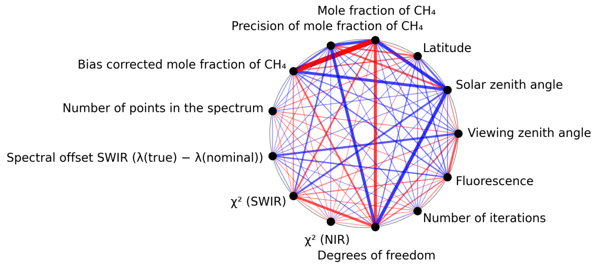
Figure 1: Map of correlation graph for 2025-07-02 to 2025-07-03.
