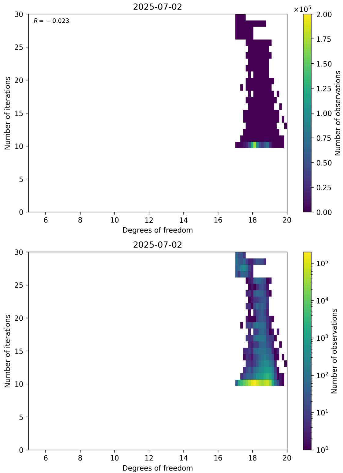
Figure 52: Scatter density plot of “Degrees of freedom” against “Number of iterations” for 2025-07-02 to 2025-07-03.
