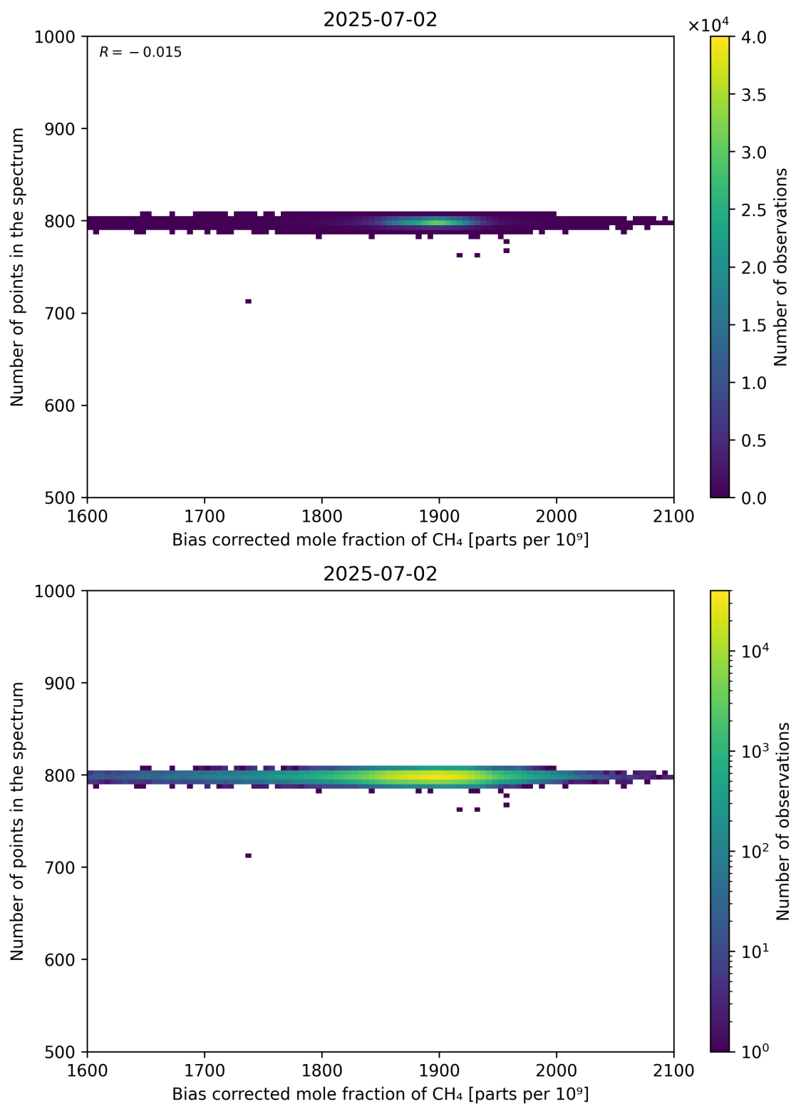
Figure 68: Scatter density plot of “Bias corrected mole fraction of CH 4 ” against “Number of points in the spectrum” for 2025-07-02 to 2025-07-03.
