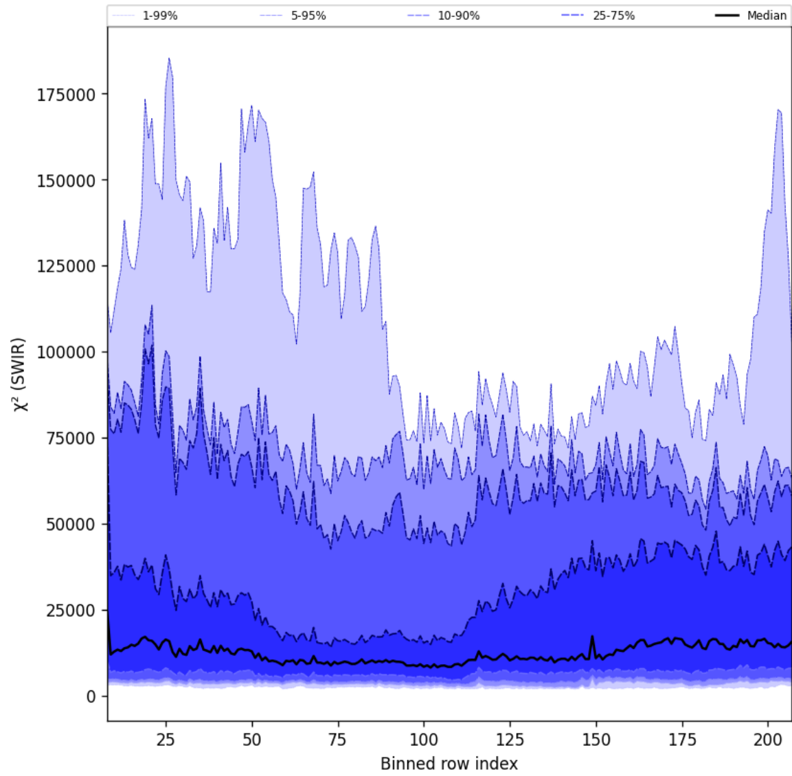
Figure 39: Along track statistics of “ \chi^2 (SWIR)” for 2025-07-02 to 2025-07-03
