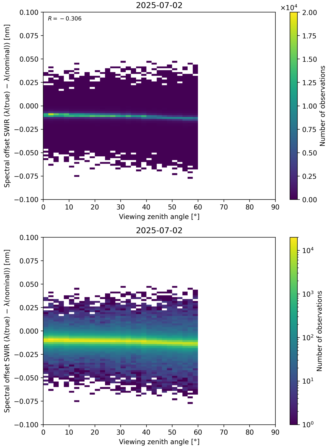
Figure 116: Scatter density plot of “Viewing zenith angle” against “Spectral offset SWIR ( \lambda_{\text{true}} - \lambda_{\text{nominal}} )” for 2025-07-02 to 2025-07-03.
