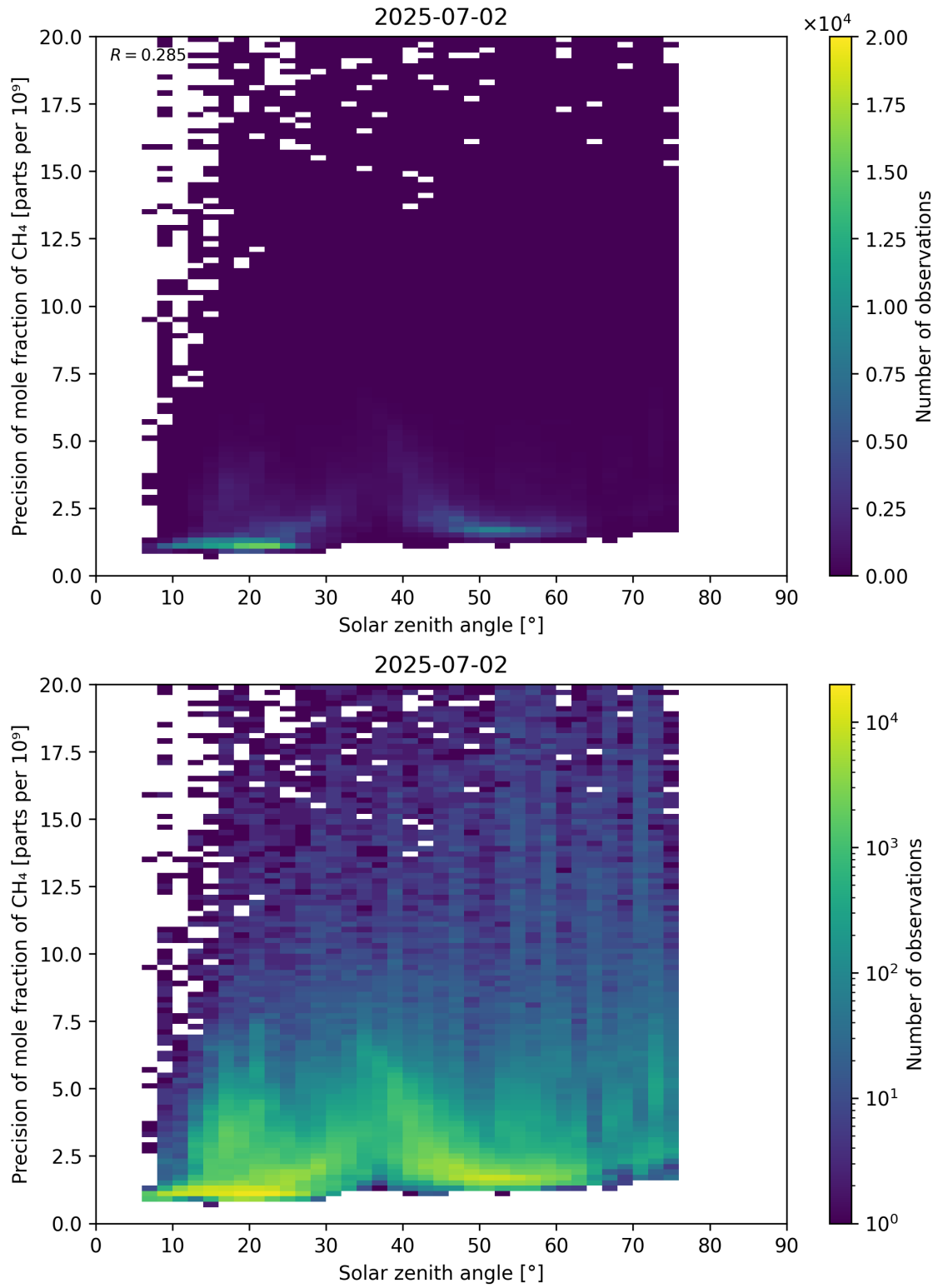
Figure 101: Scatter density plot of “Solar zenith angle” against “Precision of mole fraction of CH 4 ” for 2025-07-02 to 2025-07-03.
