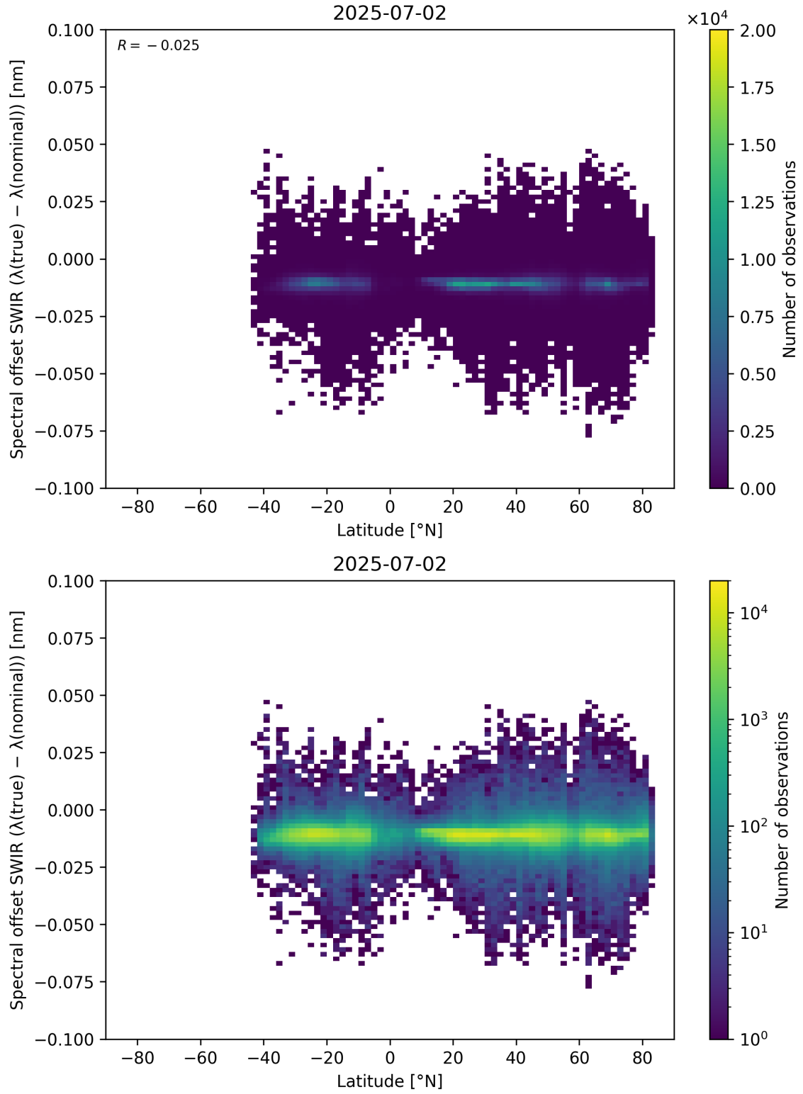
Figure 62: Scatter density plot of “Latitude” against “Spectral offset SWIR ( \lambda_{\text{true}} - \lambda_{\text{nominal}} )” for 2025-07-02 to 2025-07-03.
