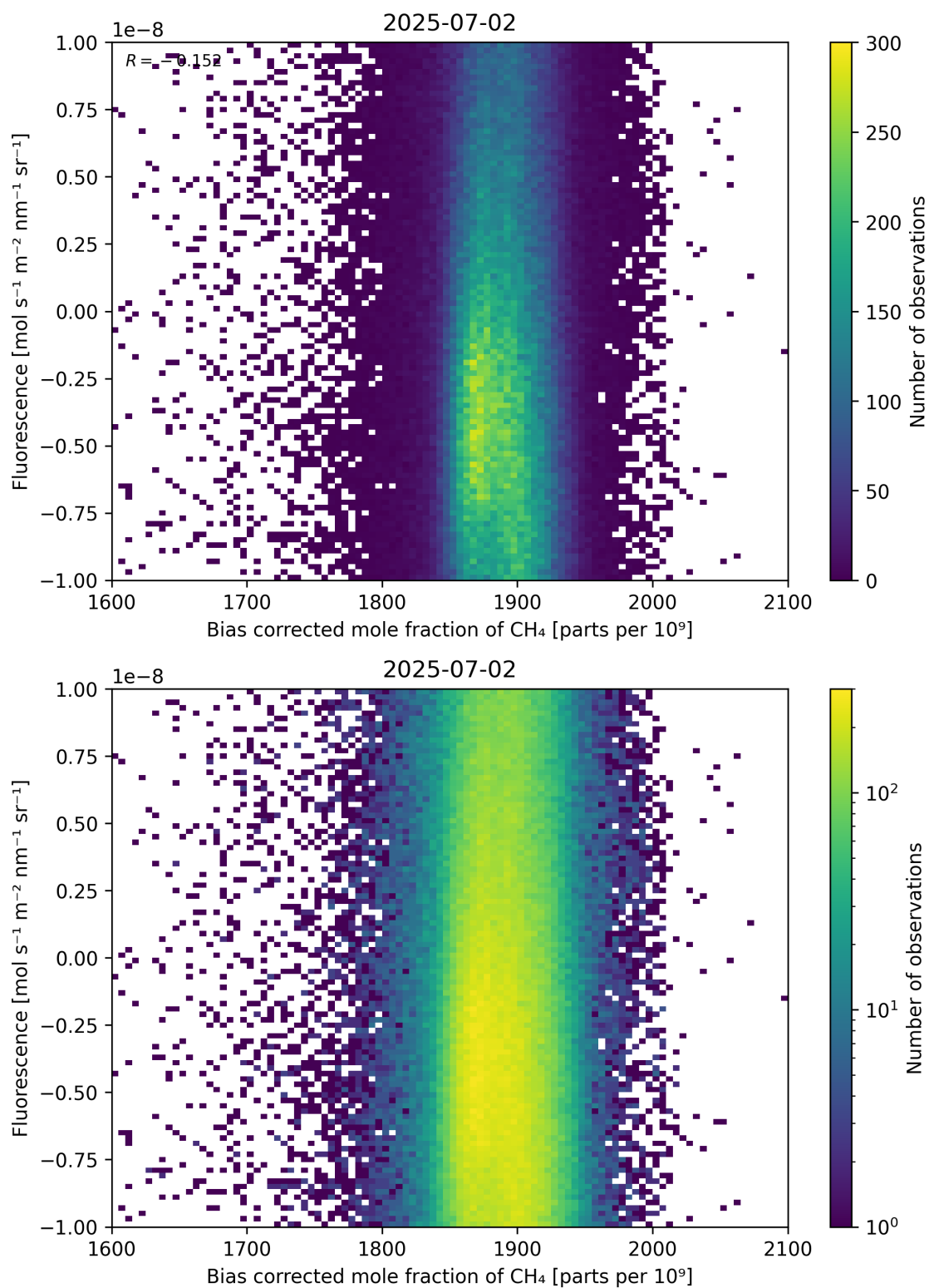
Figure 66: Scatter density plot of “Bias corrected mole fraction of \text{CH}_4 ” against “Fluorescence” for 2025-07-02 to 2025-07-03.
