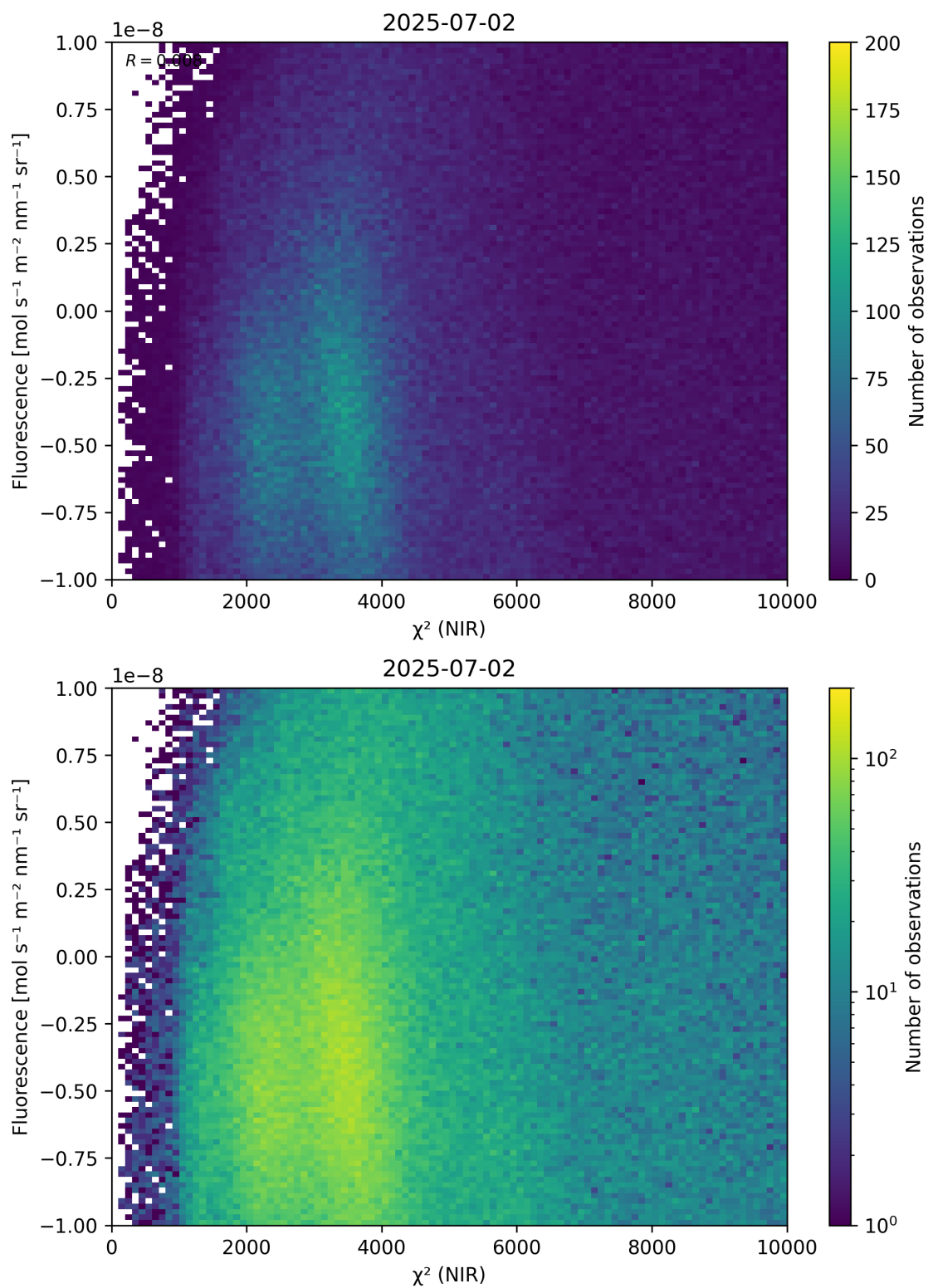
Figure 45: Scatter density plot of “ \chi^2 (NIR)” against “Fluorescence” for 2025-07-02 to 2025-07-03.
