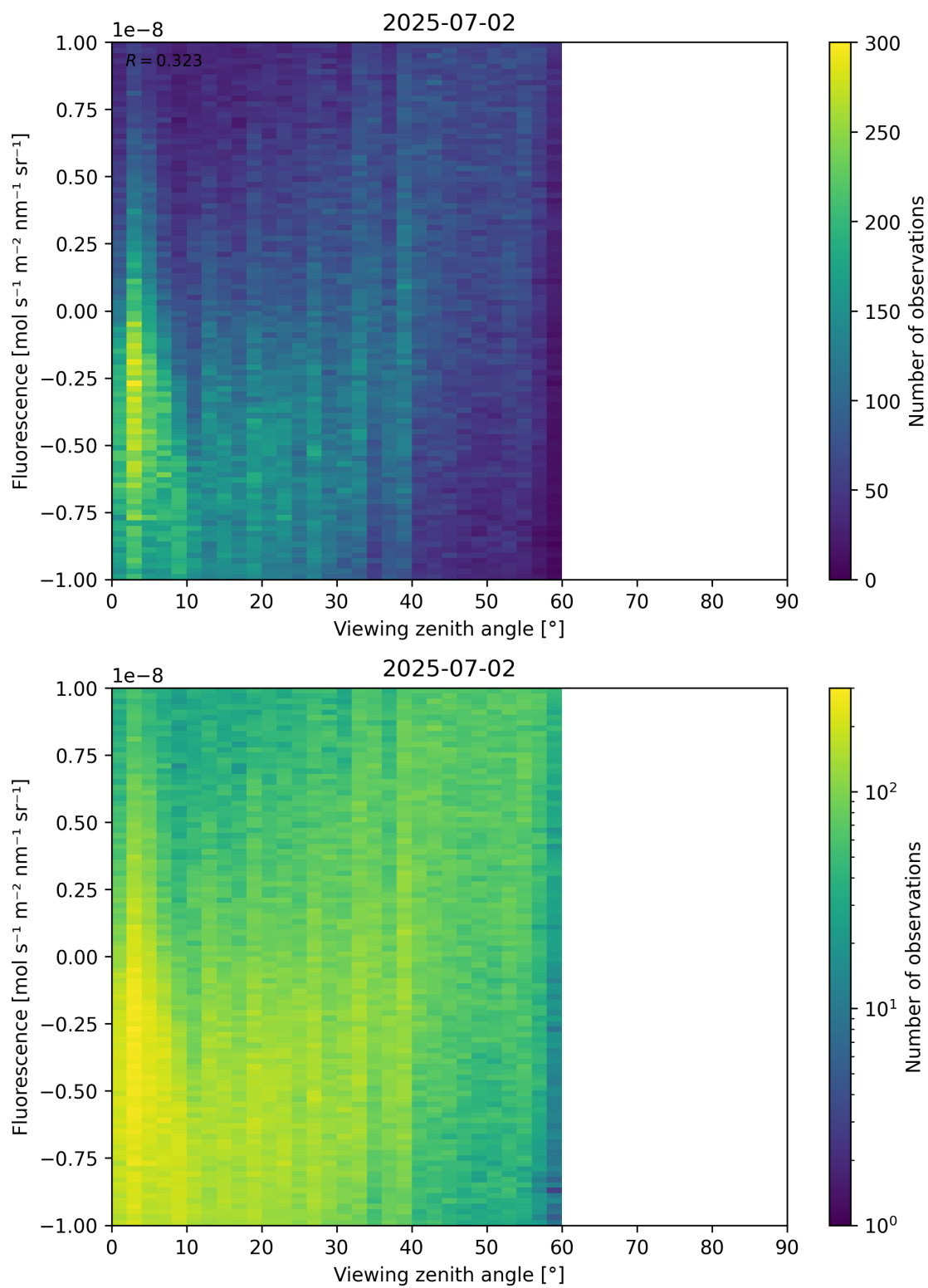
Figure 108: Scatter density plot of “Viewing zenith angle” against “Fluorescence” for 2025-07-02 to 2025-07-03.
