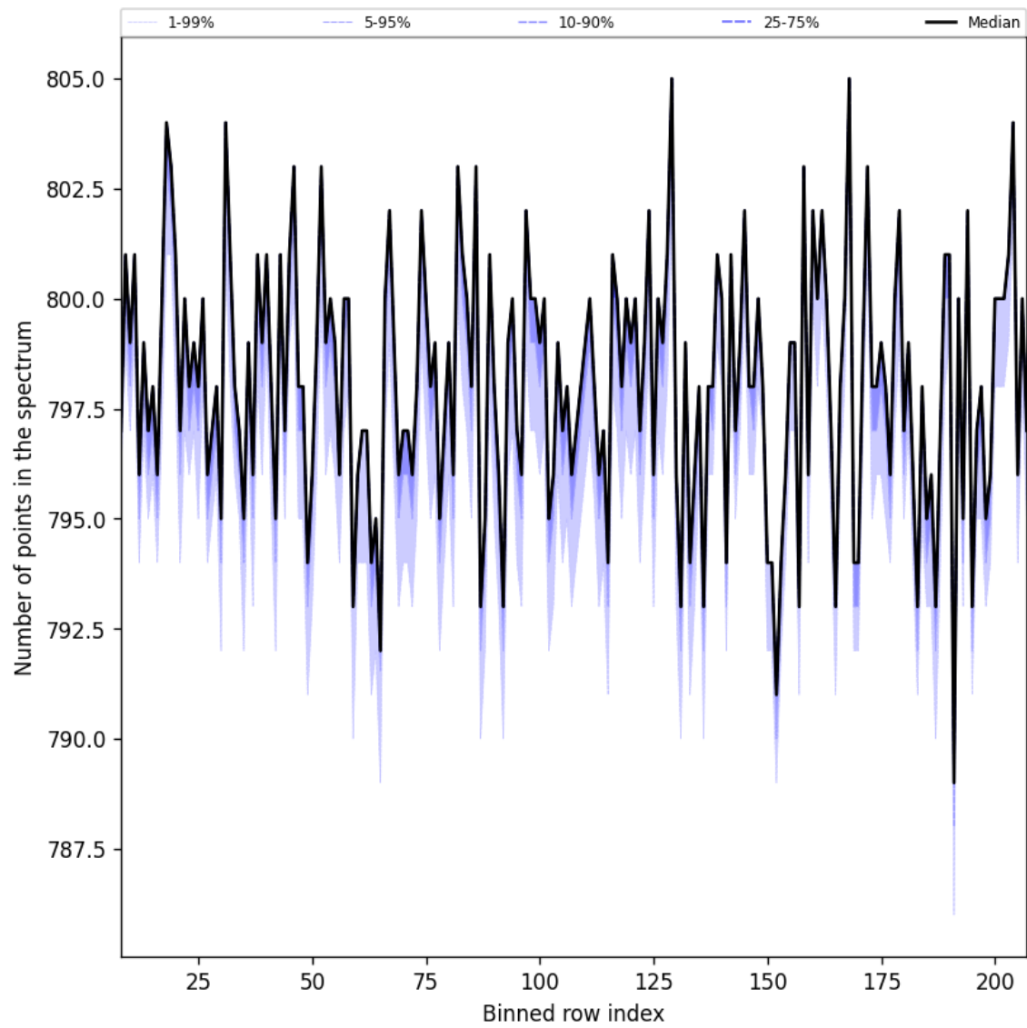
Figure 37: Along track statistics of “Number of points in the spectrum” for 2025-07-02 to 2025-07-03
