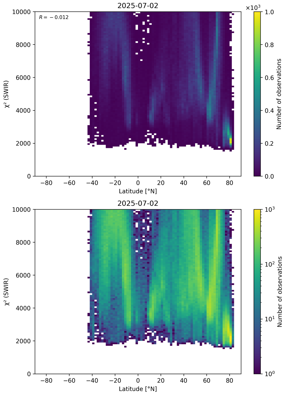
Figure 54: Scatter density plot of “Latitude” against “ \chi^2 (SWIR)” for 2025-07-02 to 2025-07-03.
