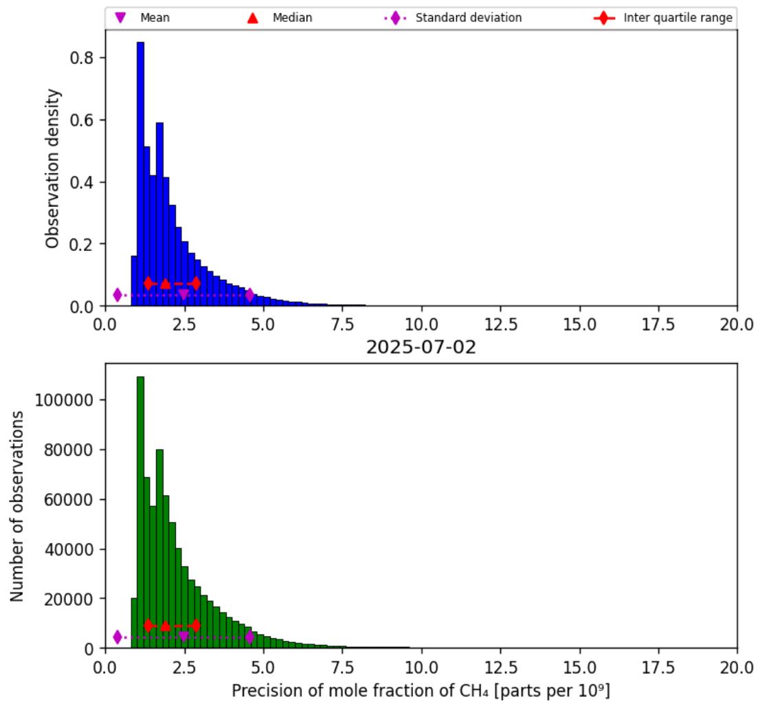
Figure 24: Histogram of “Precision of mole fraction of CH 4 ” for 2025-07-02 to 2025-07-03
