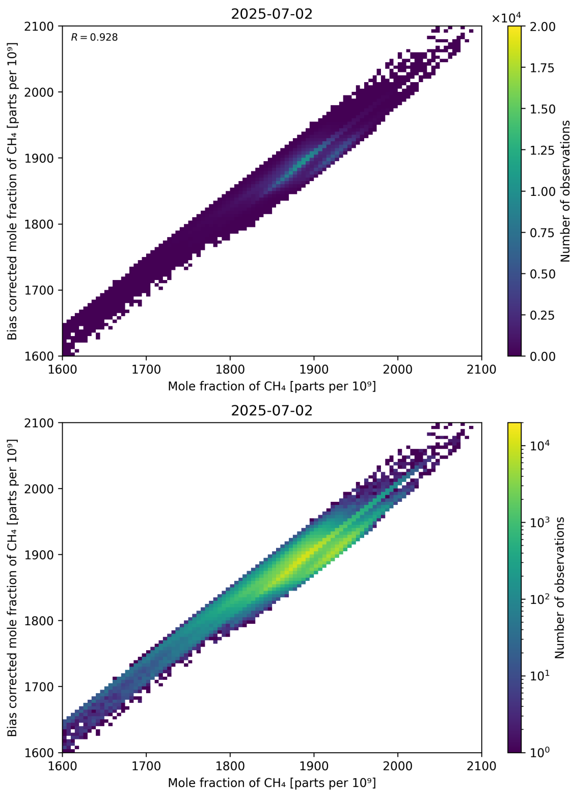
Figure 74: Scatter density plot of “Mole fraction of CH 4 ” against “Bias corrected mole fraction of CH 4 ” for 2025-07-02 to 2025-07-03.
