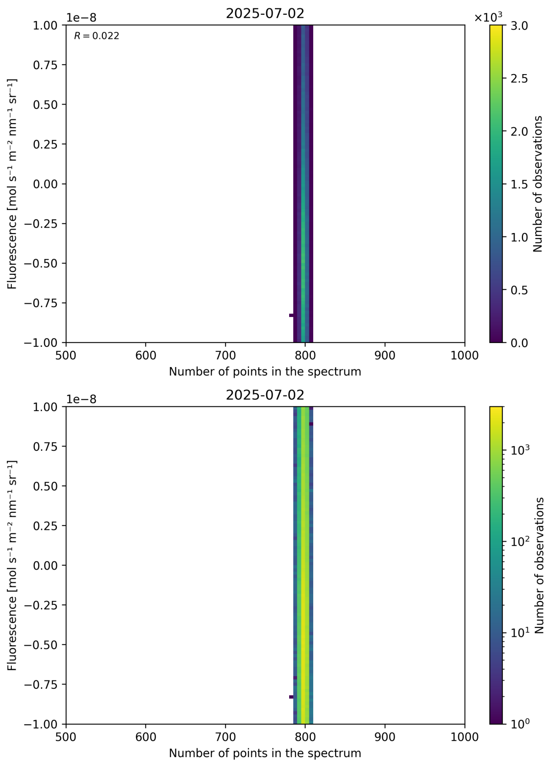
Figure 91: Scatter density plot of “Number of points in the spectrum” against “Fluorescence” for 2025-07-02 to 2025-07-03.
