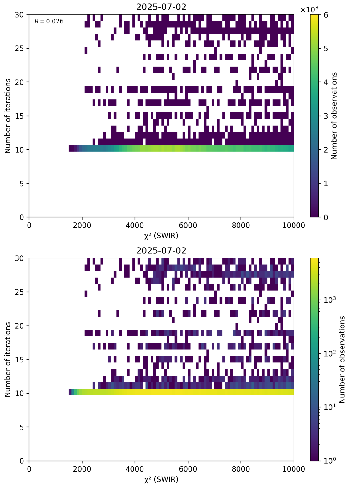
Figure 50: Scatter density plot of " \chi^2 (SWIR)" against "Number of iterations" for 2025-07-02 to 2025-07-03.
