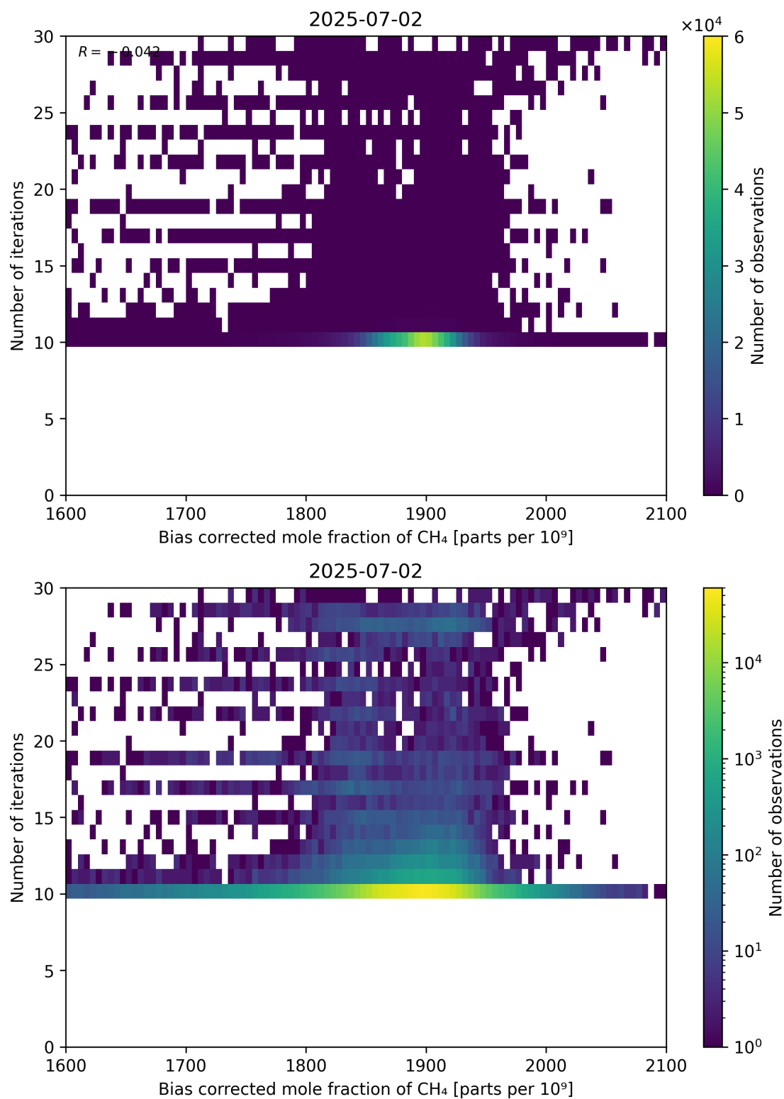
Figure 67: Scatter density plot of “Bias corrected mole fraction of CH 4 ” against “Number of iterations” for 2025-07-02 to 2025-07-03.
