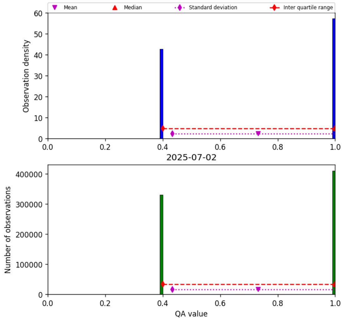
Figure 22: Histogram of “QA value” for 2025-07-02 to 2025-07-03
