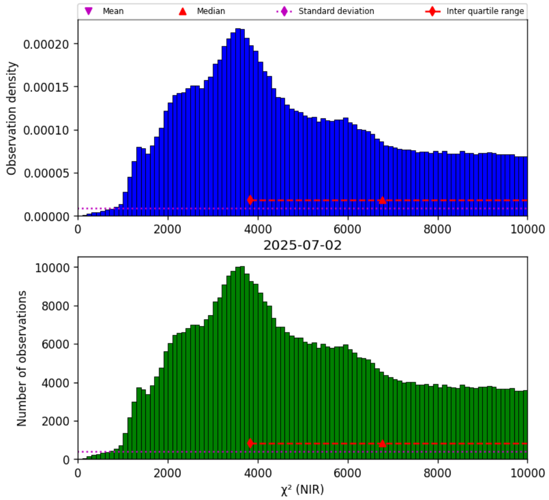
Figure 29: Histogram of " \chi^2 (NIR)" for 2025-07-02 to 2025-07-03
