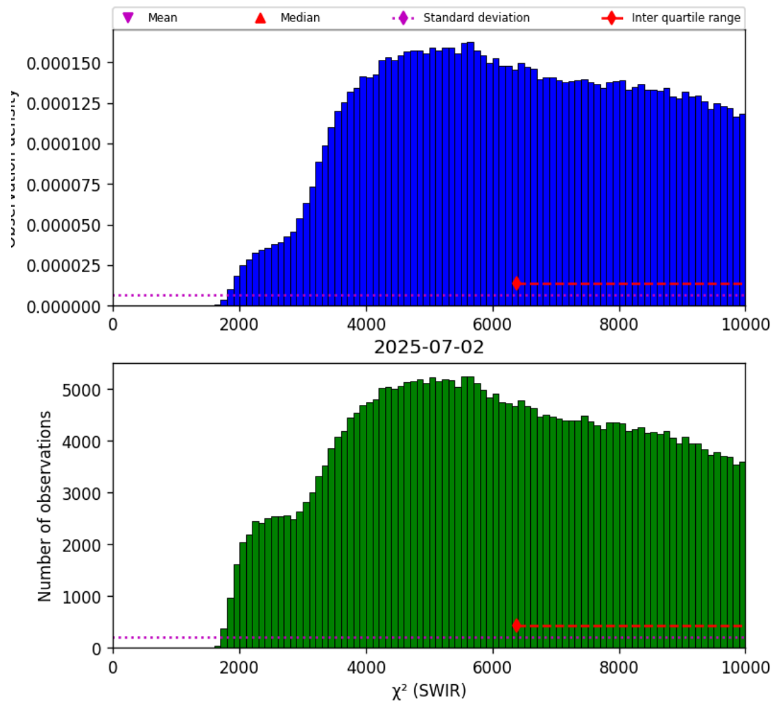
Figure 28: Histogram of “ \chi^2 (SWIR)” for 2025-07-02 to 2025-07-03
