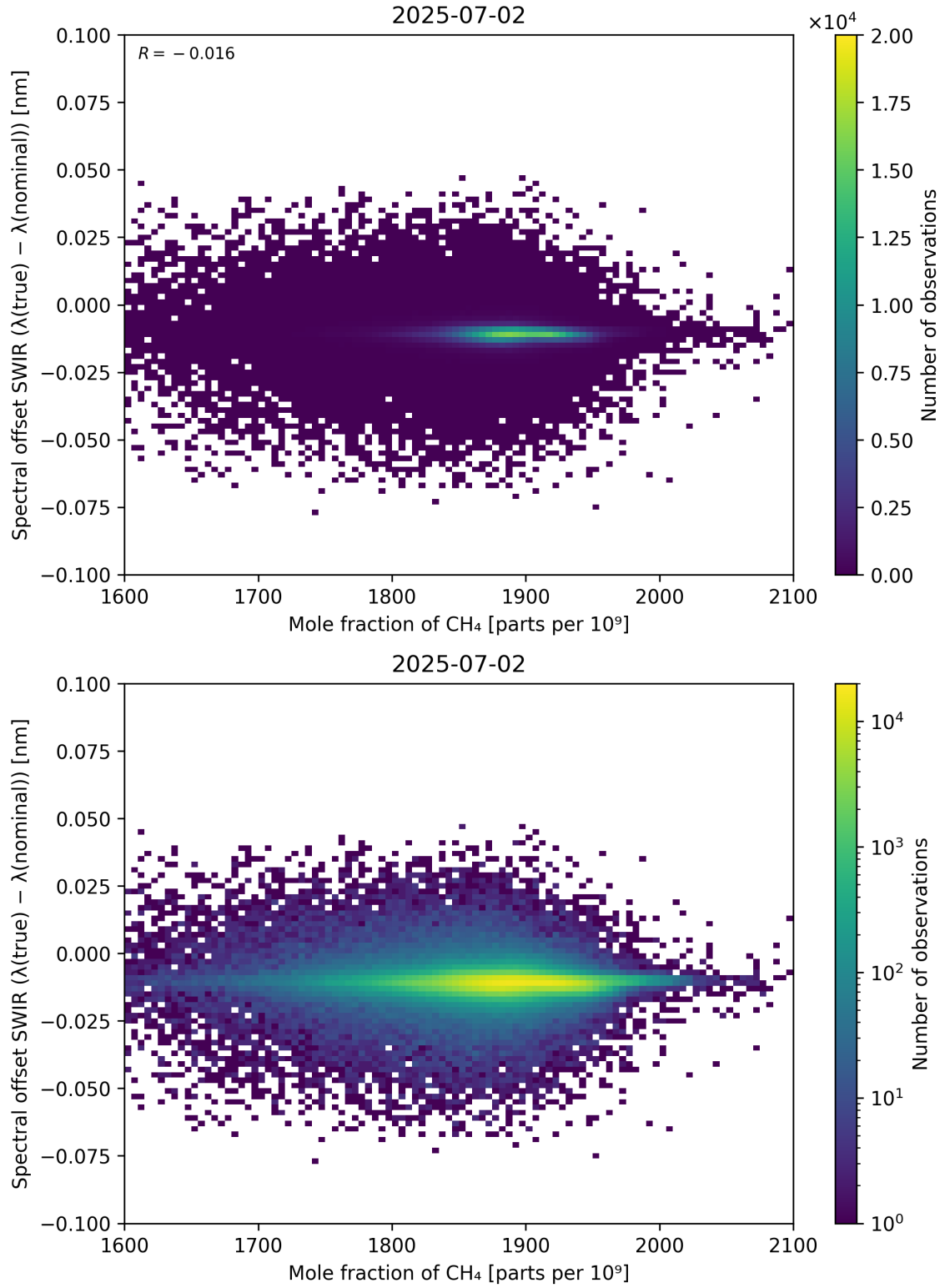
Figure 86: Scatter density plot of “Mole fraction of CH 4 ” against “Spectral offset SWIR ( \lambda_{\text{true}} - \lambda_{\text{nominal}} )” for 2025-07-02 to 2025-07-03.
