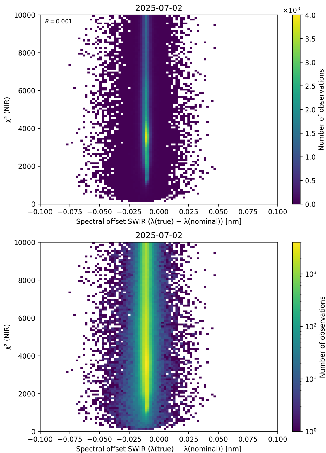
Figure 117: Scatter density plot of “Spectral offset SWIR ( \lambda_{\text{true}} - \lambda_{\text{nominal}} )” against “ \chi^2 (NIR)” for 2025-07-02 to 2025-07-03.
