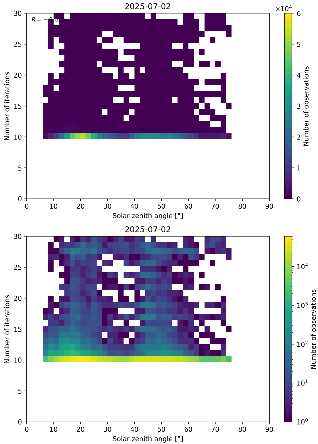
Figure 102: Scatter density plot of “Solar zenith angle” against “Number of iterations” for 2025-07-02 to 2025-07-03.
