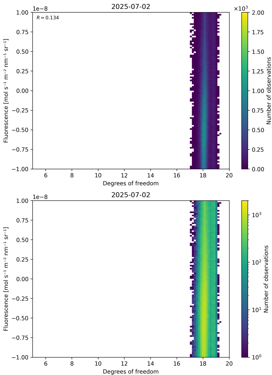
Figure 51: Scatter density plot of “Degrees of freedom” against “Fluorescence” for 2025-07-02 to 2025-07-03.
