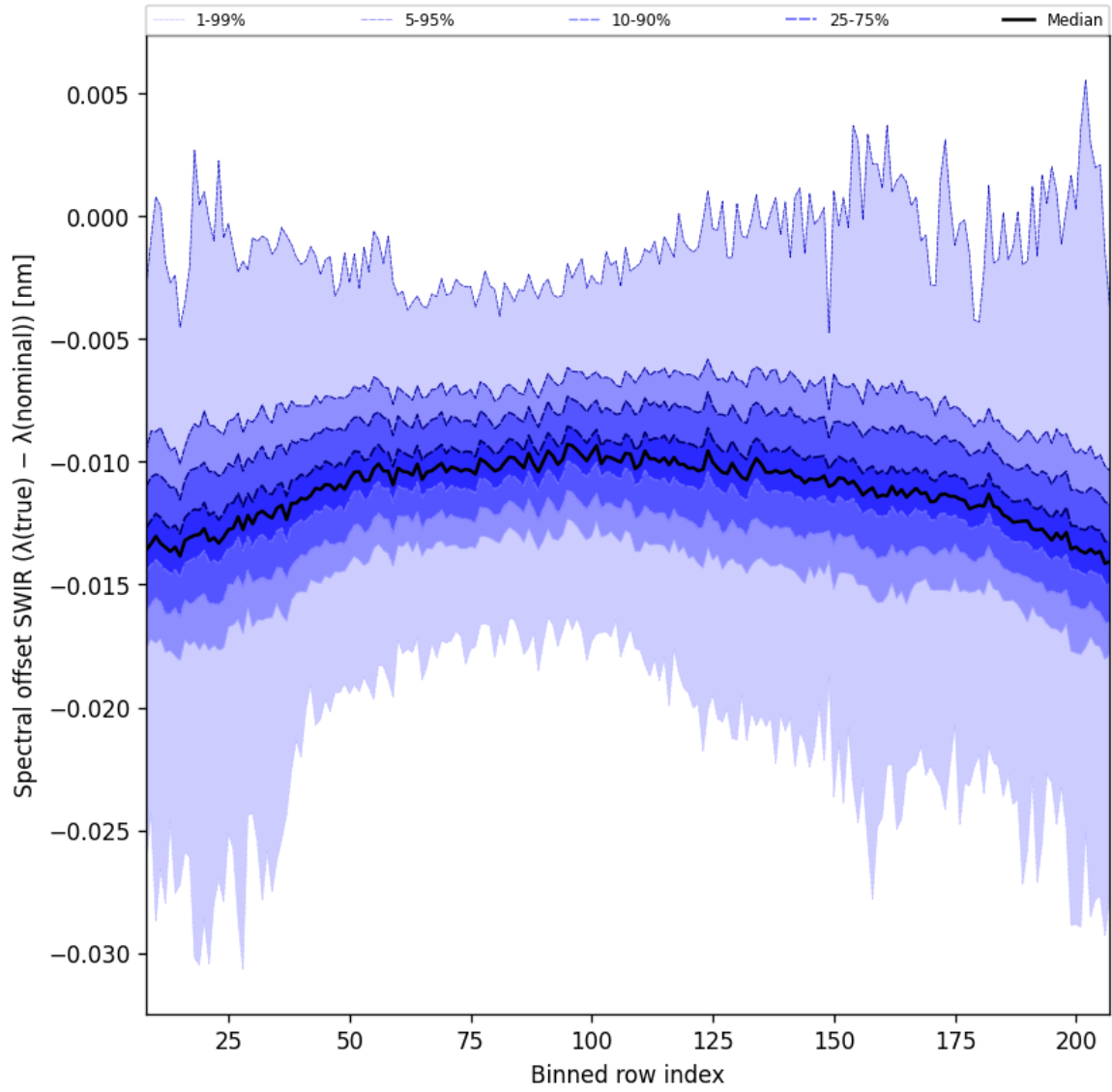
Figure 38: Along track statistics of “Spectral offset SWIR ( \lambda_{\text{true}} - \lambda_{\text{nominal}} )” for 2025-07-02 to 2025-07-03
