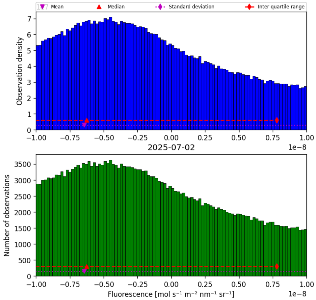
Figure 32: Histogram of “Fluorescence” for 2025-07-02 to 2025-07-03
