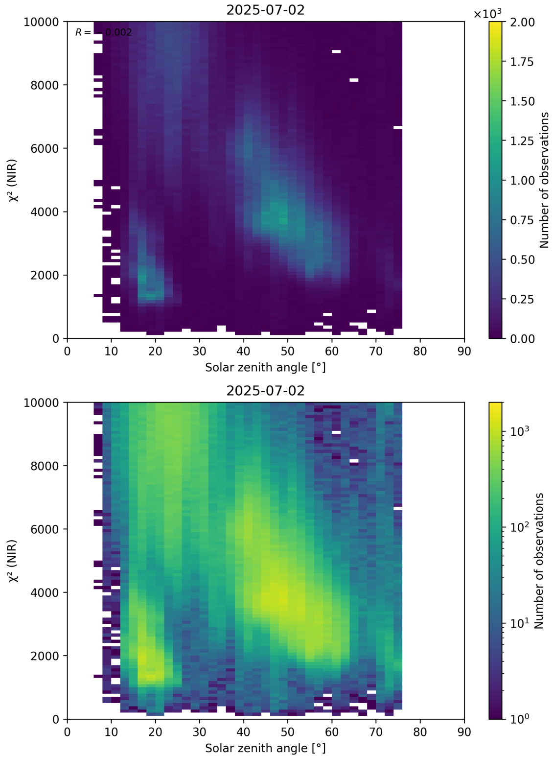
Figure 94: Scatter density plot of “Solar zenith angle” against “ \chi^2 (NIR)” for 2025-07-02 to 2025-07-03.
