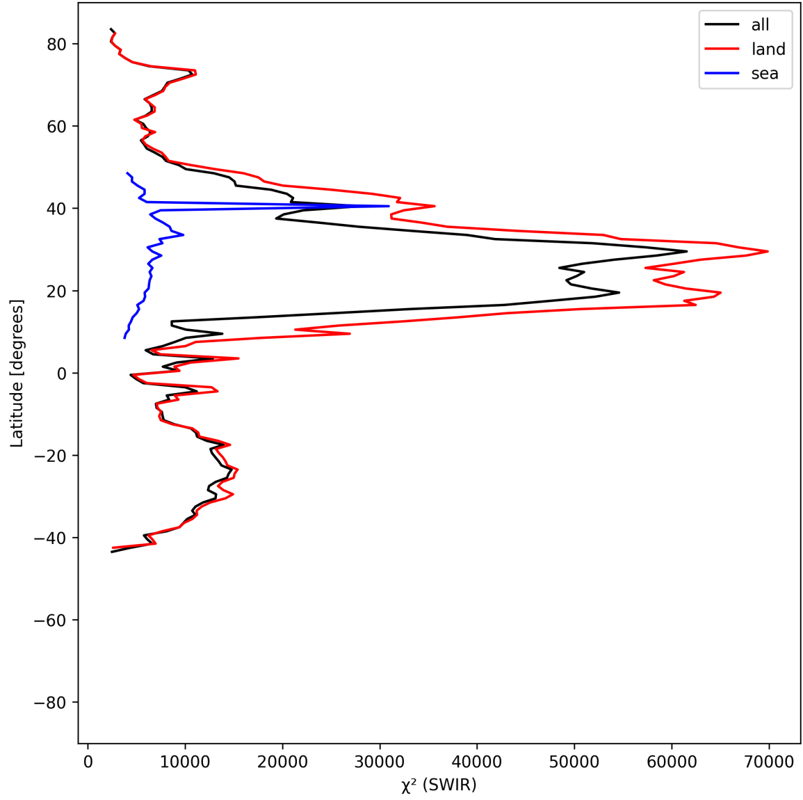
Figure 17: Zonal average of “ \chi^2 (SWIR)” for 2025-07-02 to 2025-07-03.
