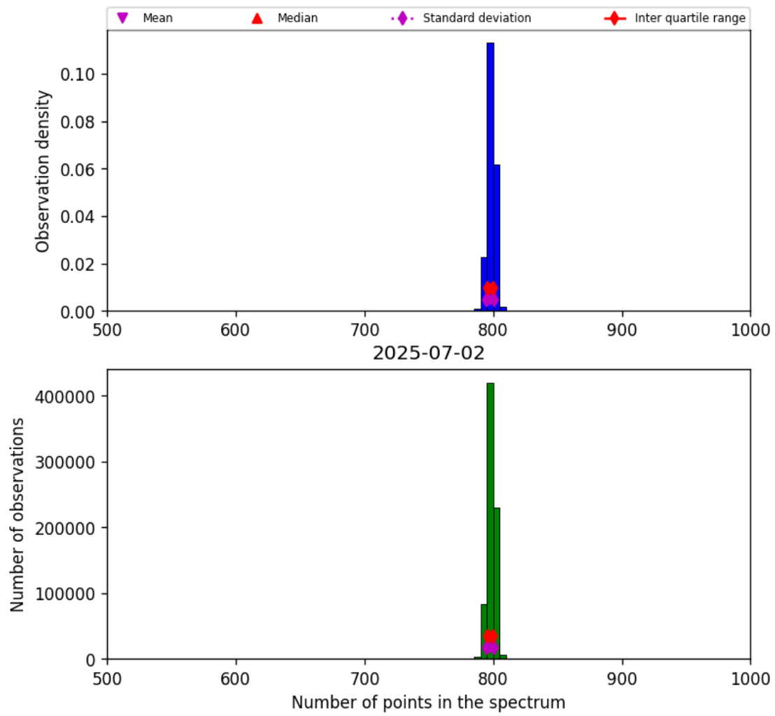
Figure 26: Histogram of “Number of points in the spectrum” for 2025-07-02 to 2025-07-03
