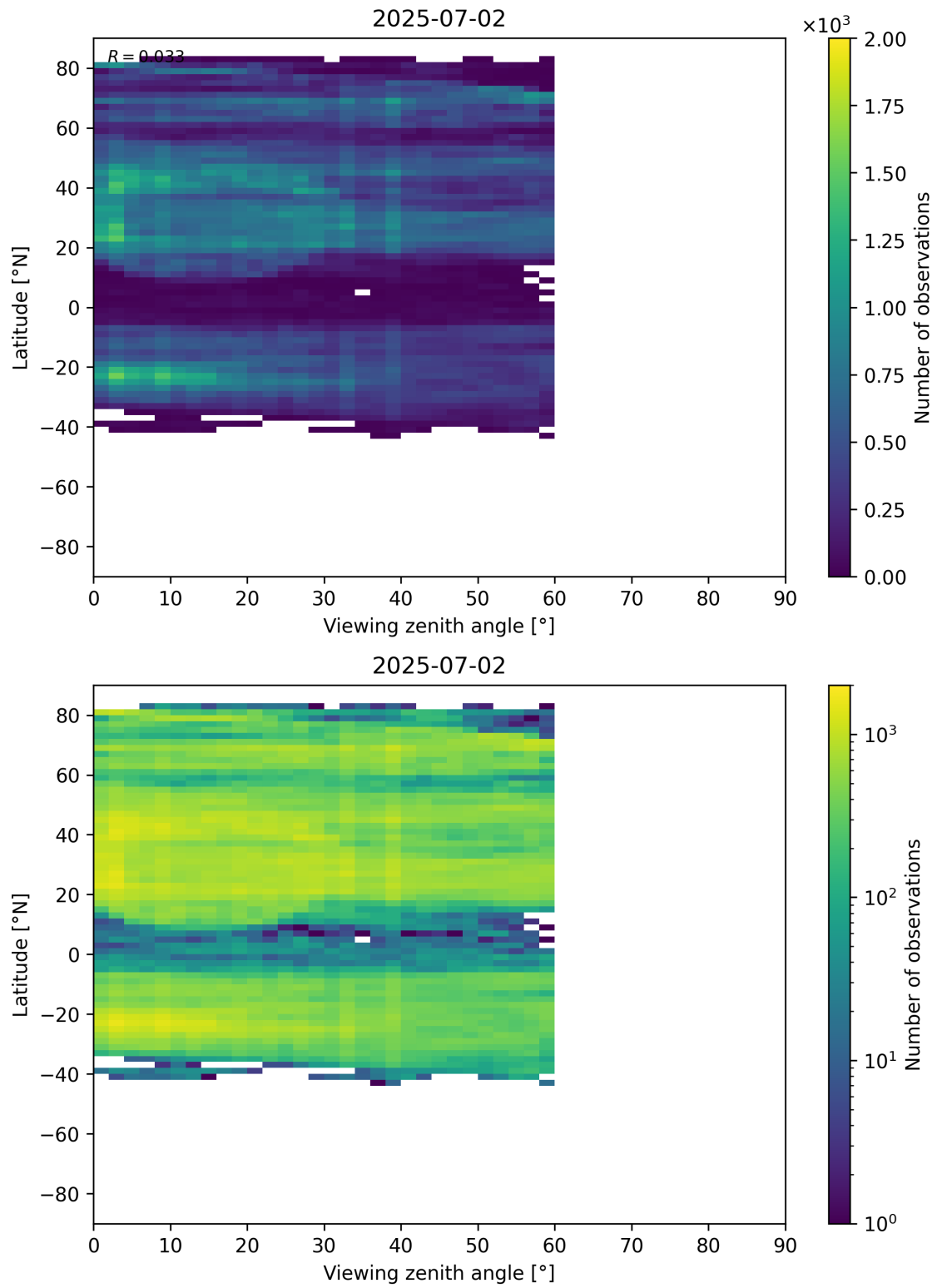
Figure 109: Scatter density plot of “Viewing zenith angle” against “Latitude” for 2025-07-02 to 2025-07-03.
