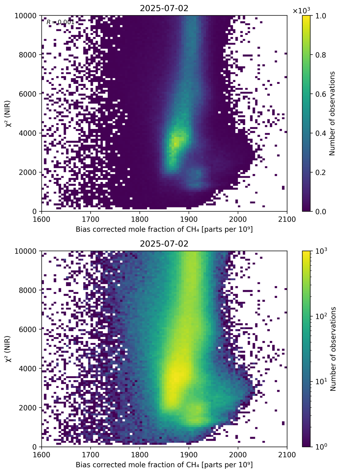
Figure 63: Scatter density plot of “Bias corrected mole fraction of \text{CH}_4 ” against “ \chi^2 (NIR)” for 2025-07-02 to 2025-07-03.
