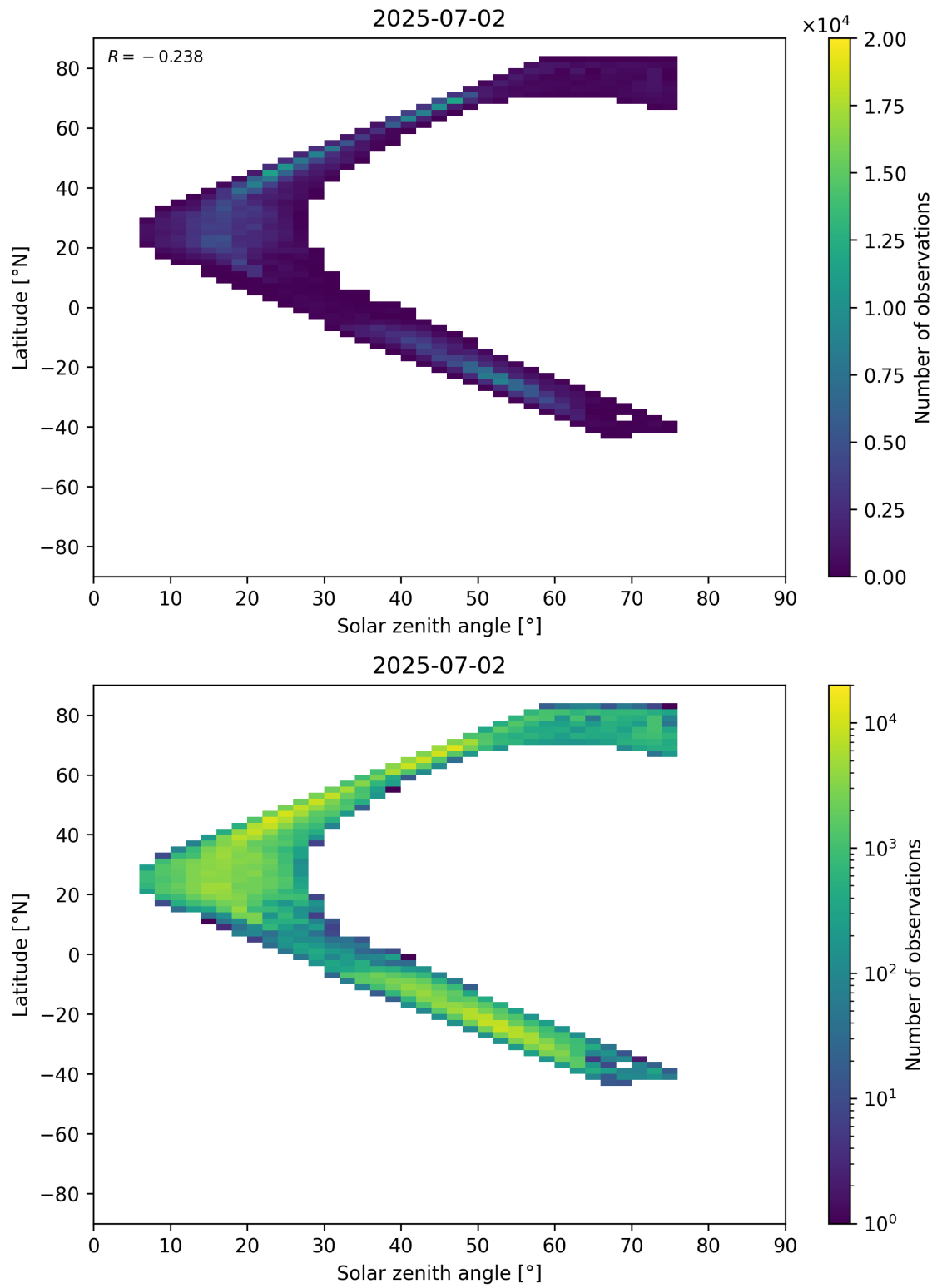
Figure 98: Scatter density plot of “Solar zenith angle” against “Latitude” for 2025-07-02 to 2025-07-03.
