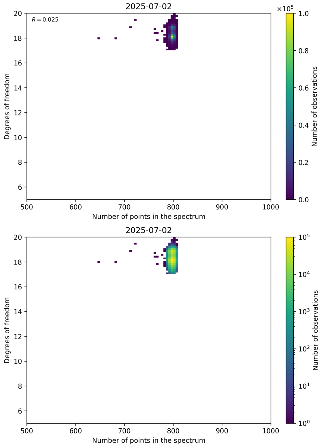
Figure 90: Scatter density plot of “Number of points in the spectrum” against “Degrees of freedom” for 2025-07-02 to 2025-07-03.
