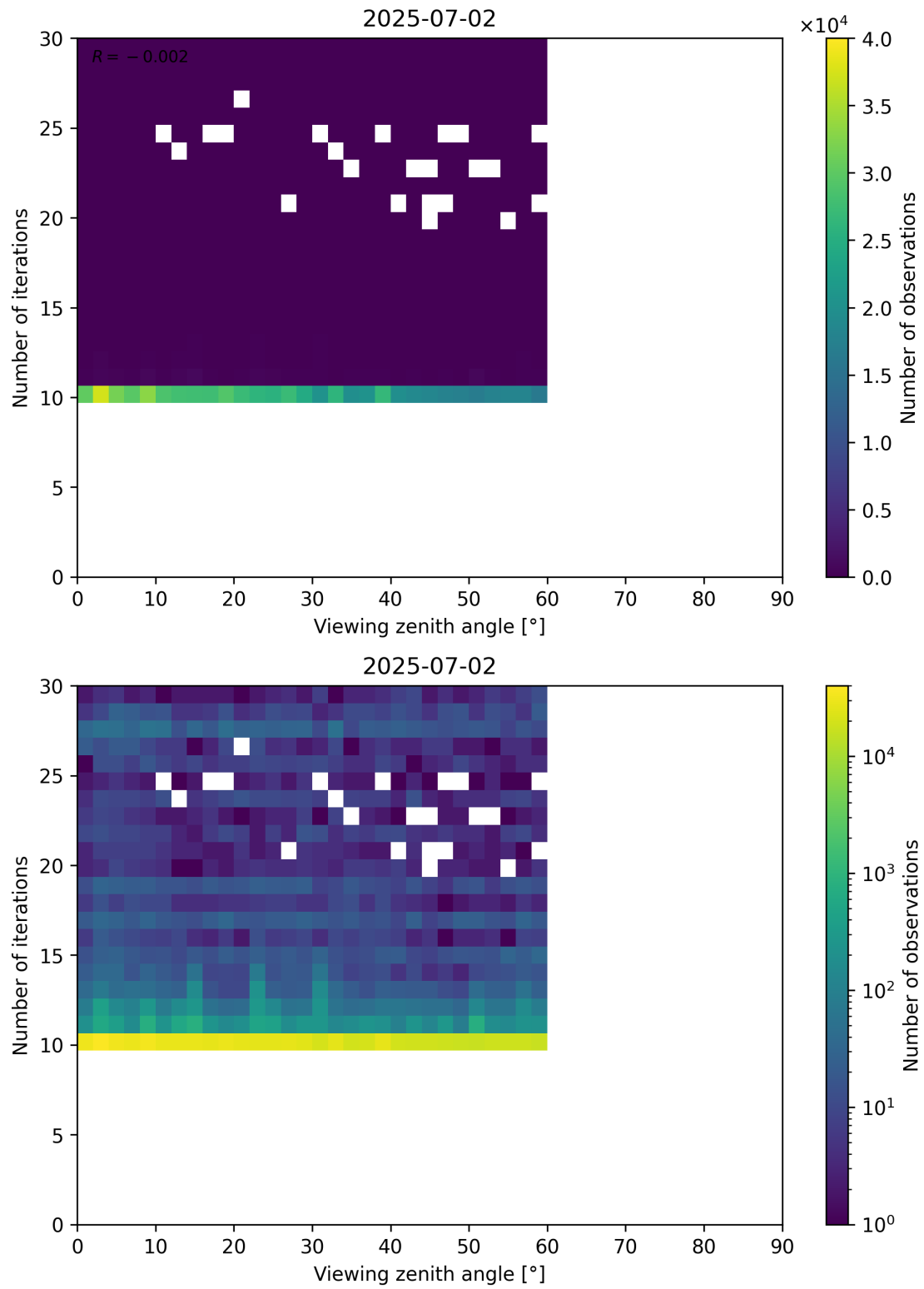
Figure 113: Scatter density plot of “Viewing zenith angle” against “Number of iterations” for 2025-07-02 to 2025-07-03.
