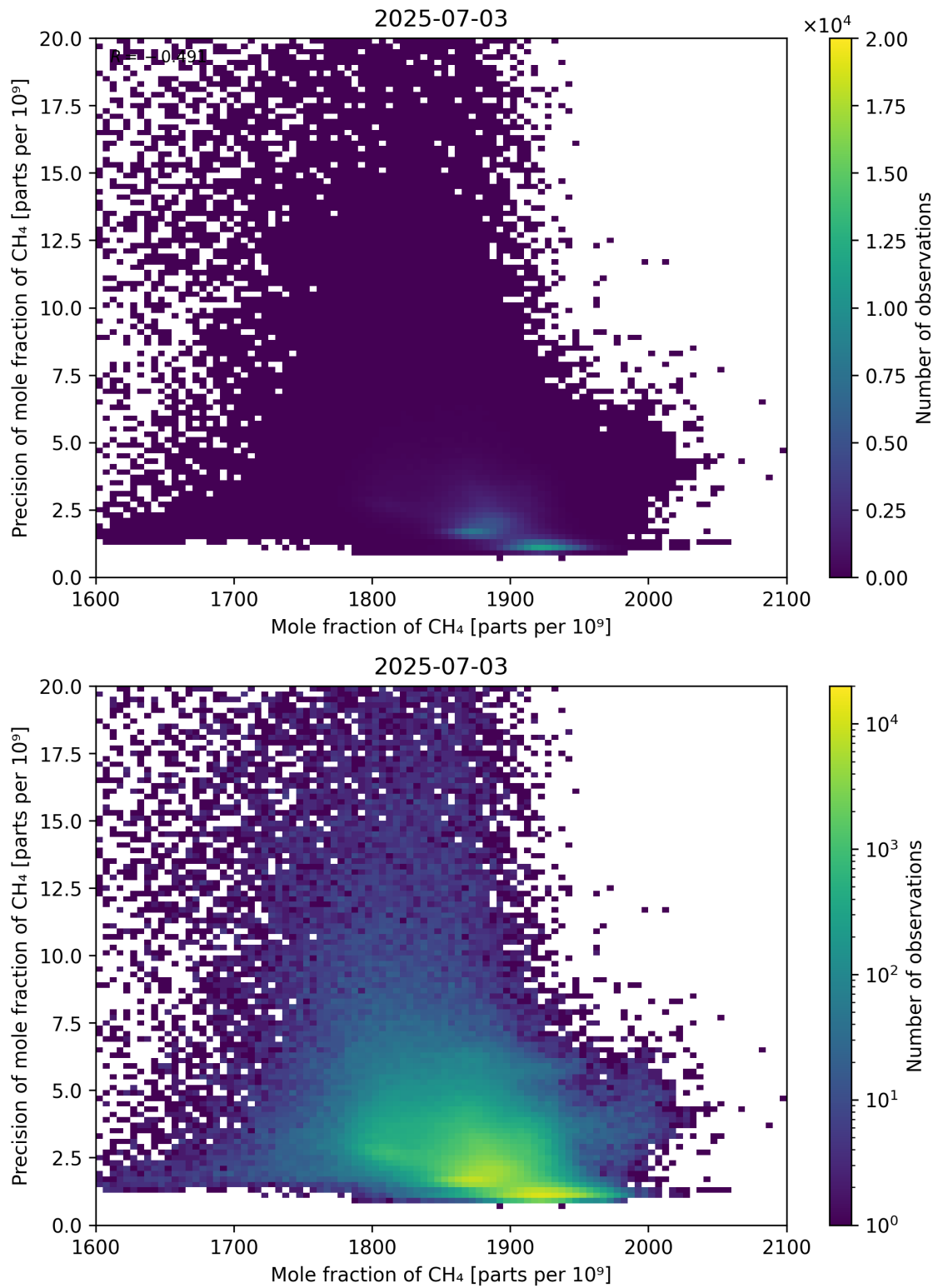
Figure 75: Scatter density plot of “Mole fraction of CH 4 ” against “Precision of mole fraction of CH 4 ” for 2025-07-03 to 2025-07-04.
