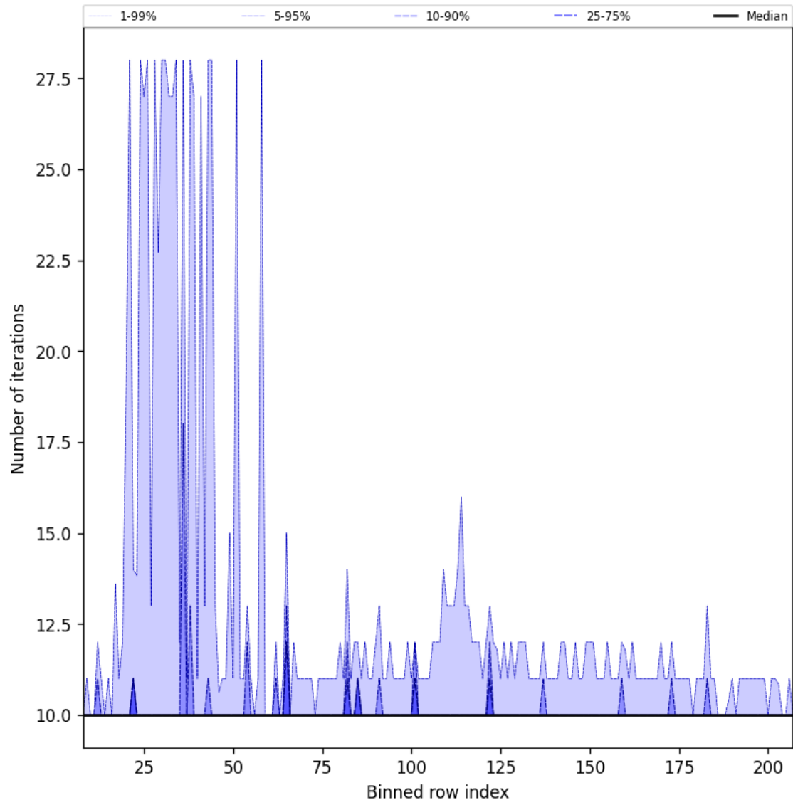
Figure 42: Along track statistics of “Number of iterations” for 2025-07-03 to 2025-07-04
