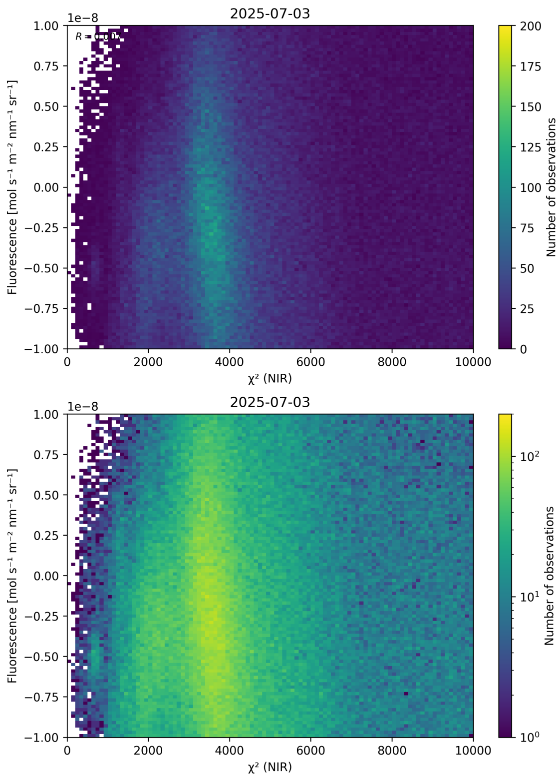
Figure 45: Scatter density plot of “ \chi^2 (NIR)” against “Fluorescence” for 2025-07-03 to 2025-07-04.
