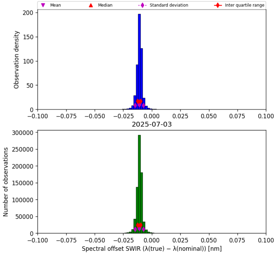
Figure 27: Histogram of “Spectral offset SWIR ( \lambda_{\text{true}} - \lambda_{\text{nominal}} )” for 2025-07-03 to 2025-07-04
