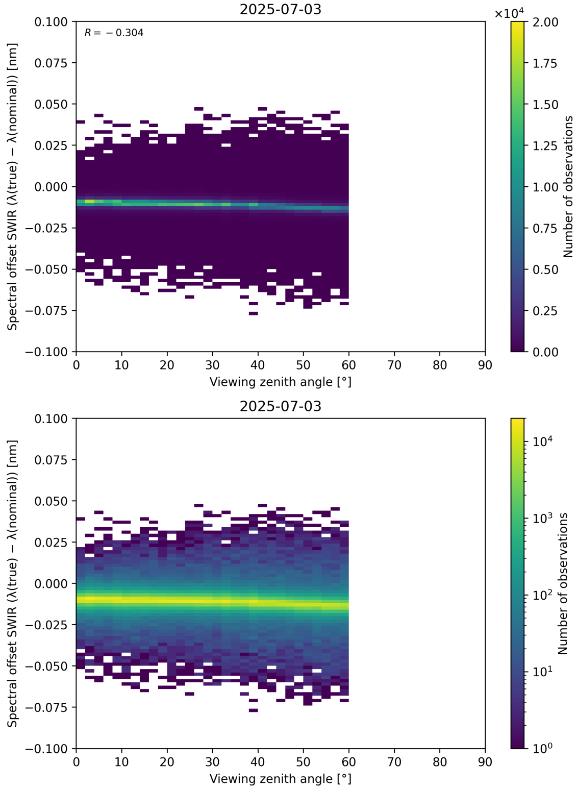
Figure 116: Scatter density plot of “Viewing zenith angle” against “Spectral offset SWIR ( \lambda_{\text{true}} - \lambda_{\text{nominal}} )” for 2025-07-03 to 2025-07-04.
