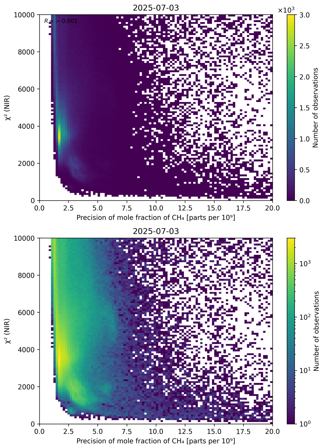
Figure 78: Scatter density plot of “Precision of mole fraction of CH 4 ” against “ \chi^2 (NIR)” for 2025-07-03 to 2025-07-04.
