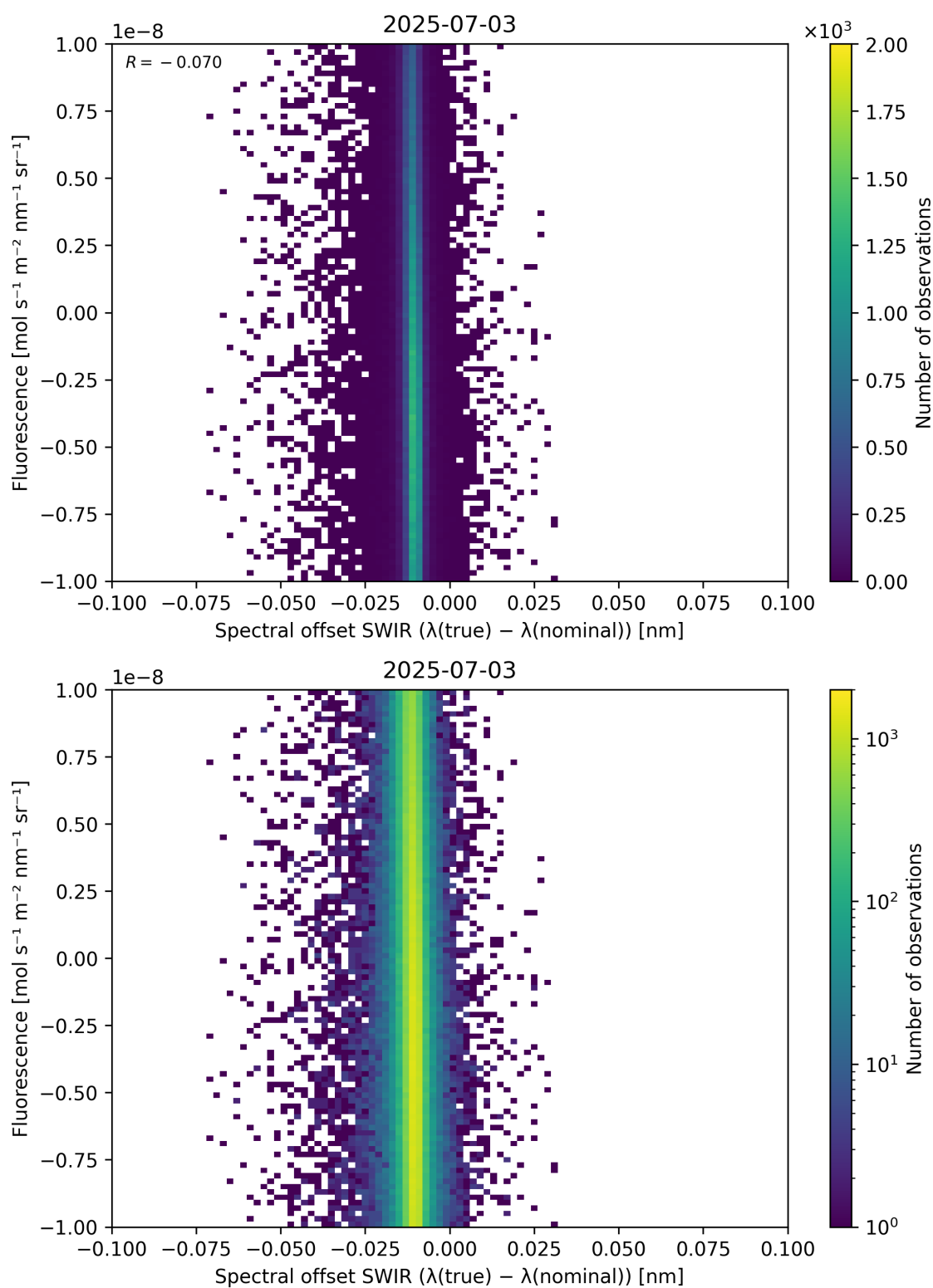
Figure 120: Scatter density plot of “Spectral offset SWIR ( \lambda_{\text{true}} - \lambda_{\text{nominal}} )” against “Fluorescence” for 2025-07-03 to 2025-07-04.
