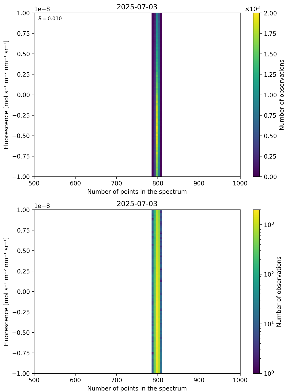
Figure 91: Scatter density plot of “Number of points in the spectrum” against “Fluorescence” for 2025-07-03 to 2025-07-04.
