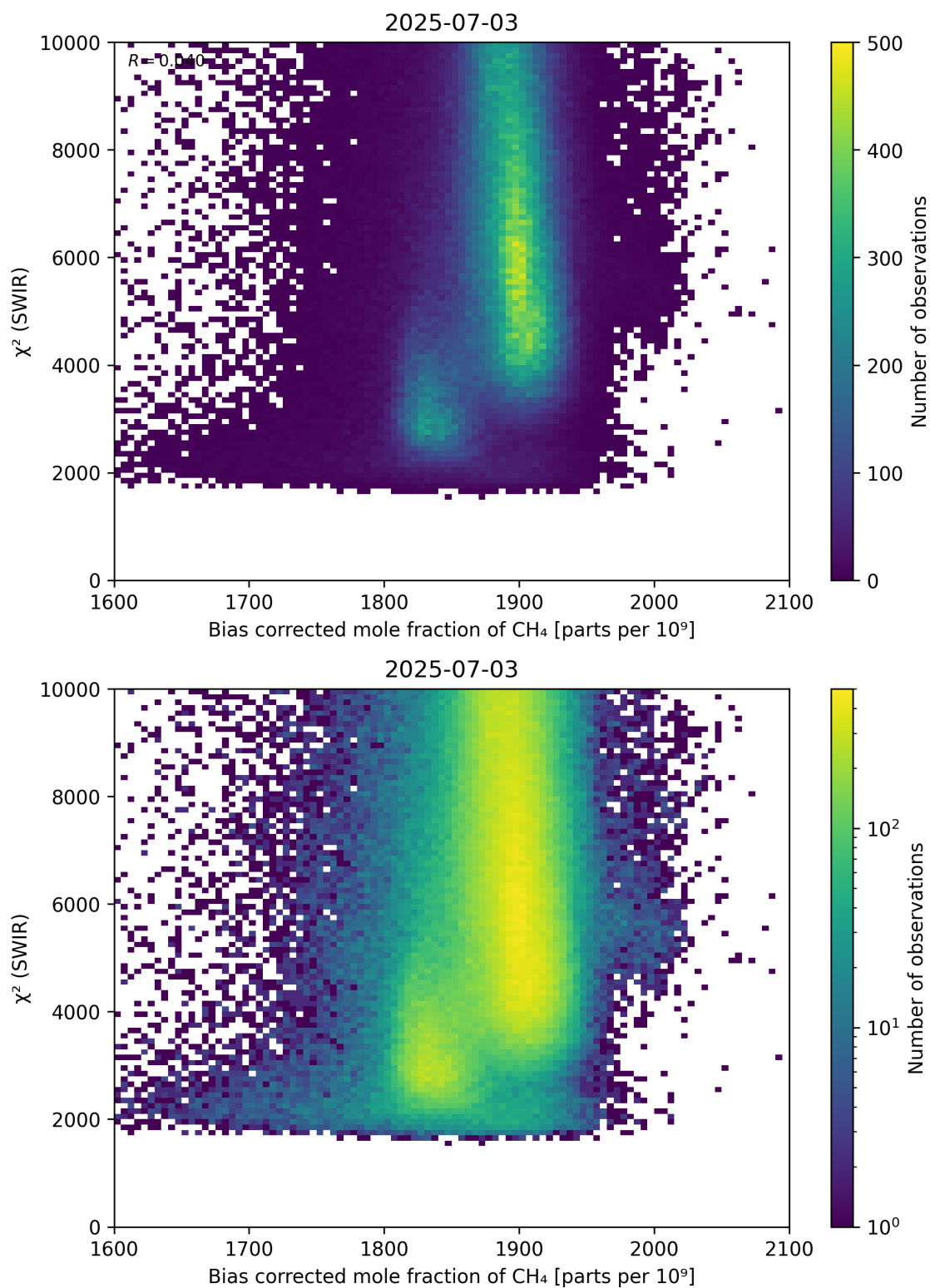
Figure 64: Scatter density plot of “Bias corrected mole fraction of \text{CH}_4 ” against “ \chi^2 (SWIR)” for 2025-07-03 to 2025-07-04.
