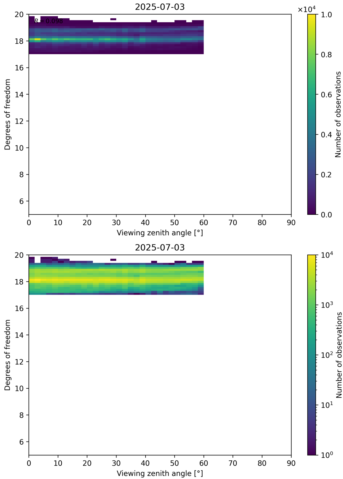
Figure 107: Scatter density plot of “Viewing zenith angle” against “Degrees of freedom” for 2025-07-03 to 2025-07-04.
