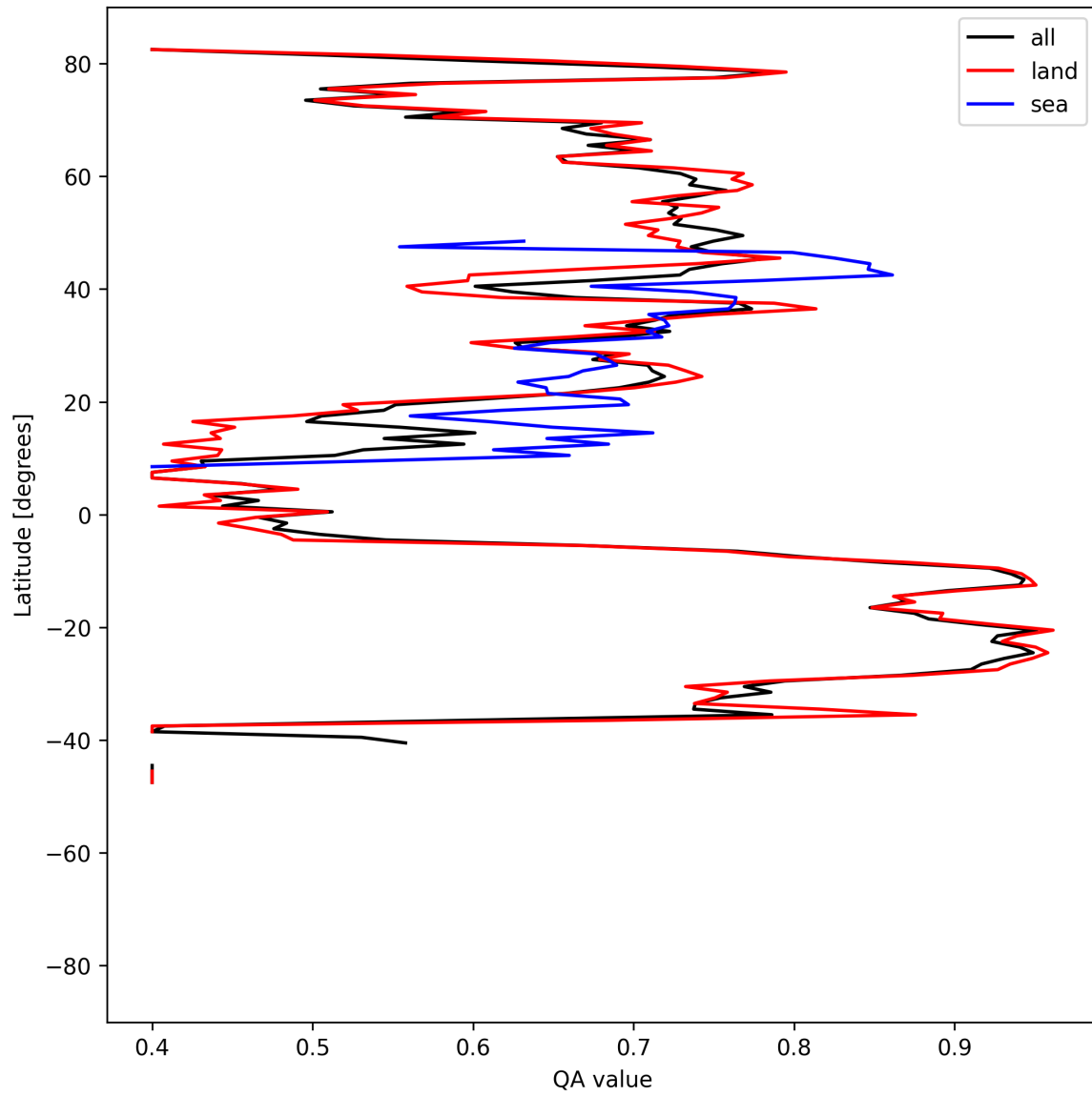
Figure 11: Zonal average of “QA value” for 2025-07-03 to 2025-07-04.
