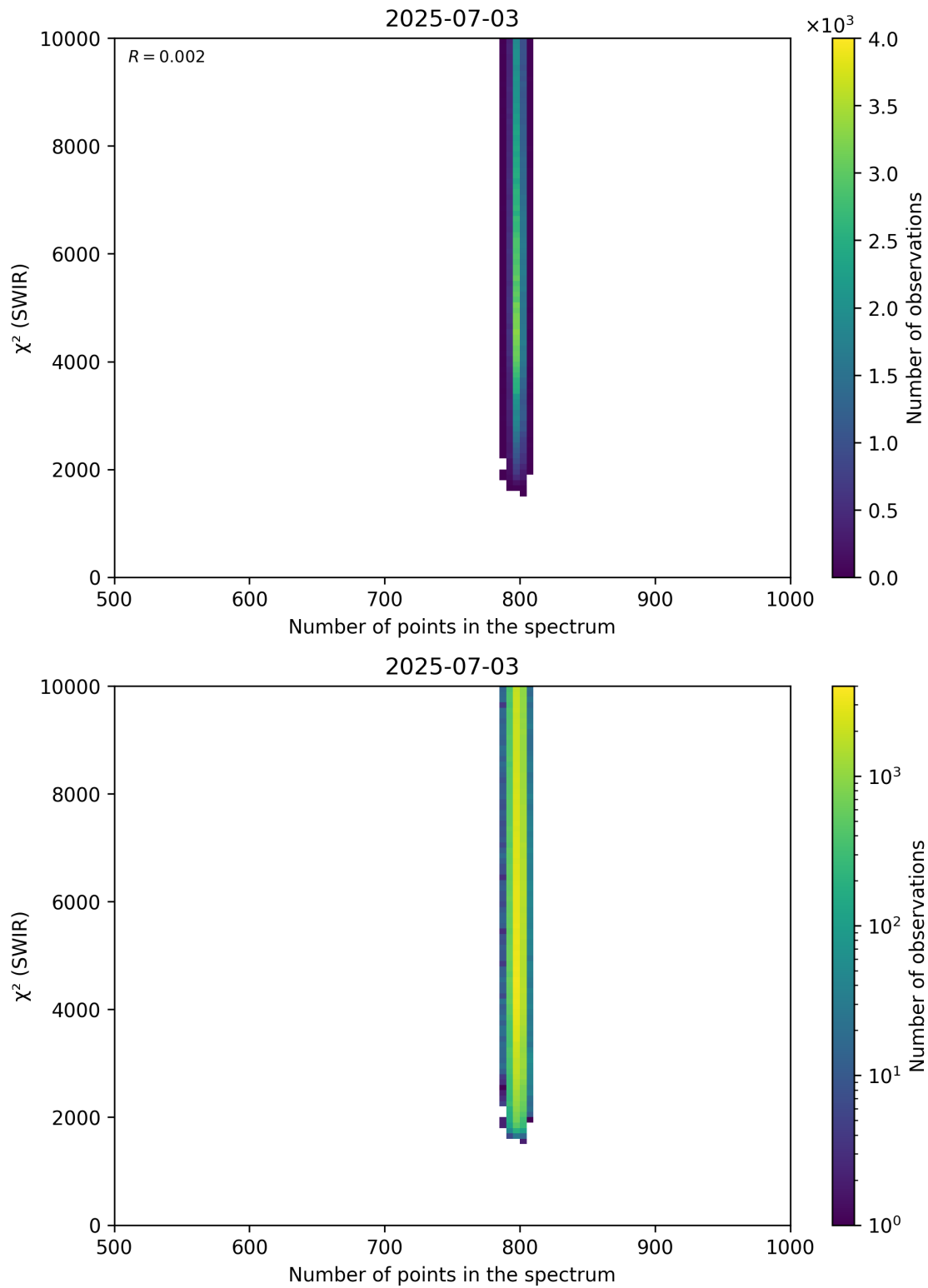
Figure 89: Scatter density plot of “Number of points in the spectrum” against “ \chi^2 (SWIR)” for 2025-07-03 to 2025-07-04.
