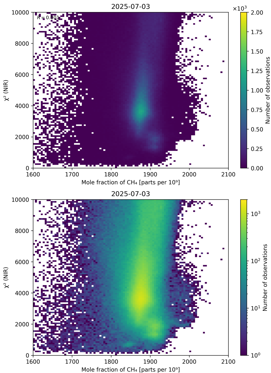
Figure 70: Scatter density plot of “Mole fraction of CH 4 ” against “ \chi^2 (NIR)” for 2025-07-03 to 2025-07-04.
