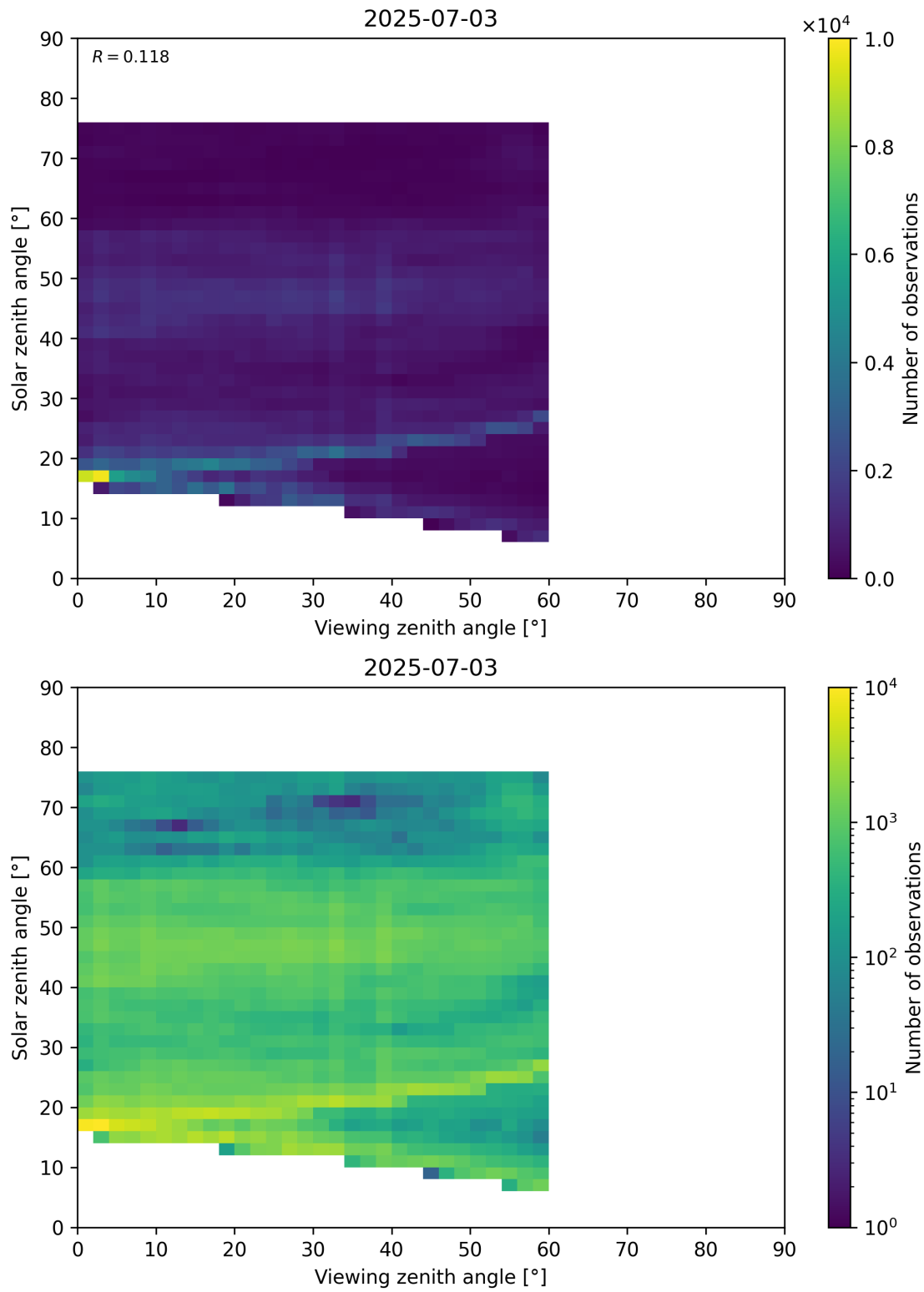
Figure 115: Scatter density plot of “Viewing zenith angle” against “Solar zenith angle” for 2025-07-03 to 2025-07-04.
