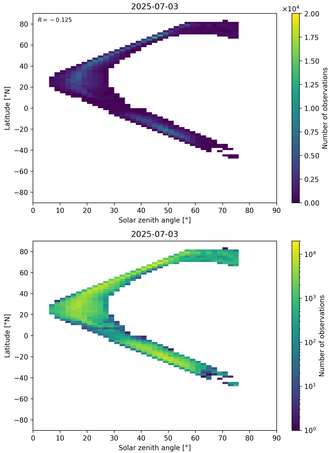
Figure 98: Scatter density plot of “Solar zenith angle” against “Latitude” for 2025-07-03 to 2025-07-04.
