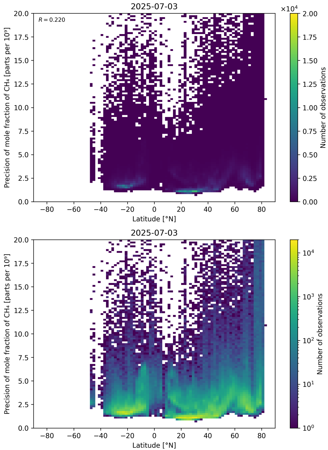
Figure 59: Scatter density plot of “Latitude” against “Precision of mole fraction of \text{CH}_4 ” for 2025-07-03 to 2025-07-04.
