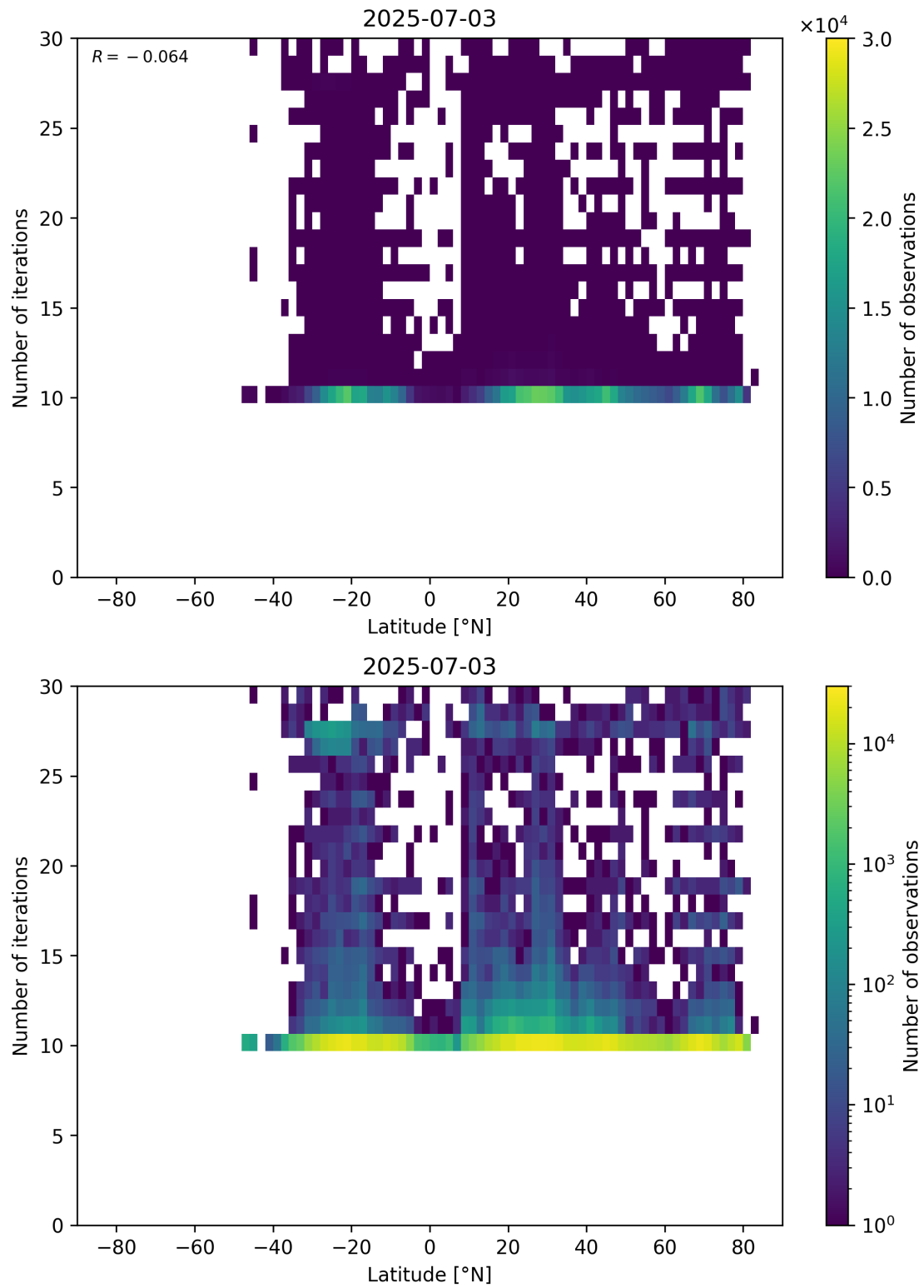
Figure 60: Scatter density plot of “Latitude” against “Number of iterations” for 2025-07-03 to 2025-07-04.
