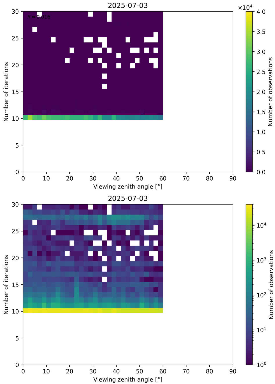
Figure 113: Scatter density plot of “Viewing zenith angle” against “Number of iterations” for 2025-07-03 to 2025-07-04.
