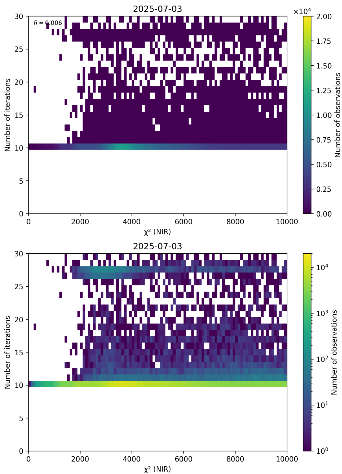
Figure 46: Scatter density plot of “ \chi^2 (NIR)” against “Number of iterations” for 2025-07-03 to 2025-07-04.
