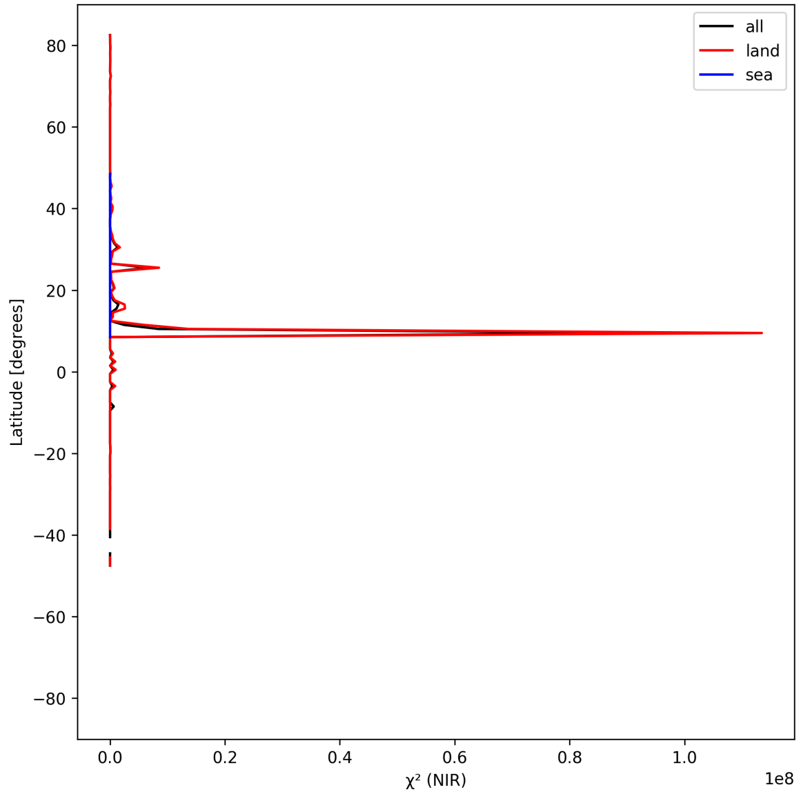
Figure 18: Zonal average of “ \chi^2 (NIR)” for 2025-07-03 to 2025-07-04.
