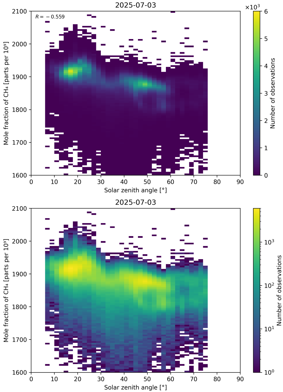
Figure 99: Scatter density plot of “Solar zenith angle” against “Mole fraction of CH 4 ” for 2025-07-03 to 2025-07-04.
