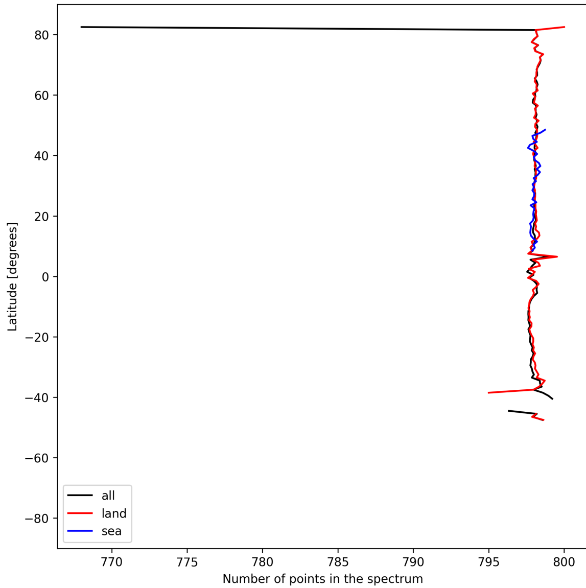
Figure 15: Zonal average of “Number of points in the spectrum” for 2025-07-03 to 2025-07-04.
