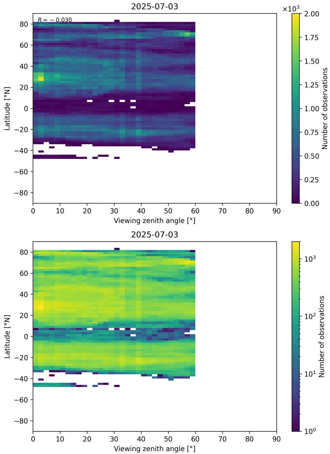
Figure 109: Scatter density plot of “Viewing zenith angle” against “Latitude” for 2025-07-03 to 2025-07-04.
