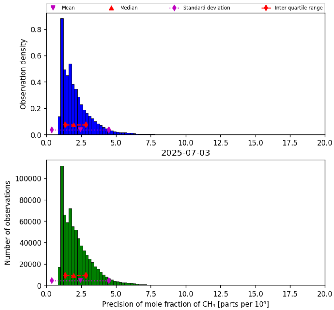
Figure 24: Histogram of “Precision of mole fraction of CH 4 ” for 2025-07-03 to 2025-07-04
