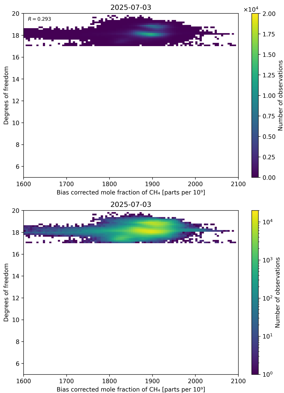
Figure 65: Scatter density plot of “Bias corrected mole fraction of CH 4 ” against “Degrees of freedom” for 2025-07-03 to 2025-07-04.
