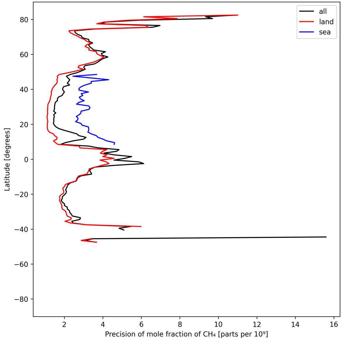
Figure 13: Zonal average of “Precision of mole fraction of CH 4 ” for 2025-07-03 to 2025-07-04.
