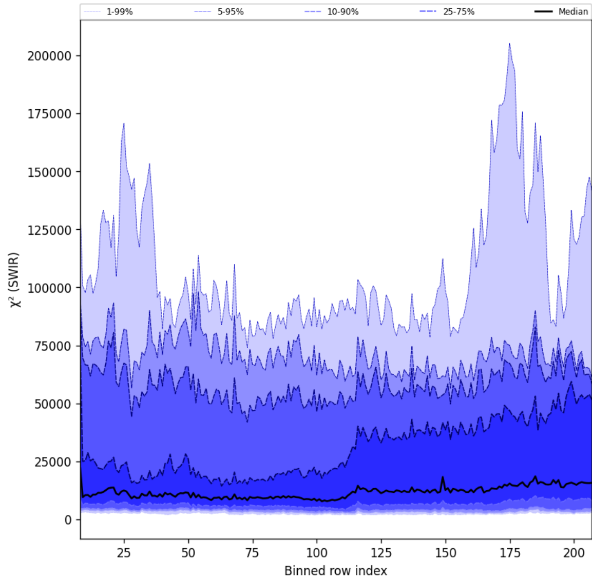
Figure 39: Along track statistics of “ \chi^2 (SWIR)” for 2025-07-03 to 2025-07-04
