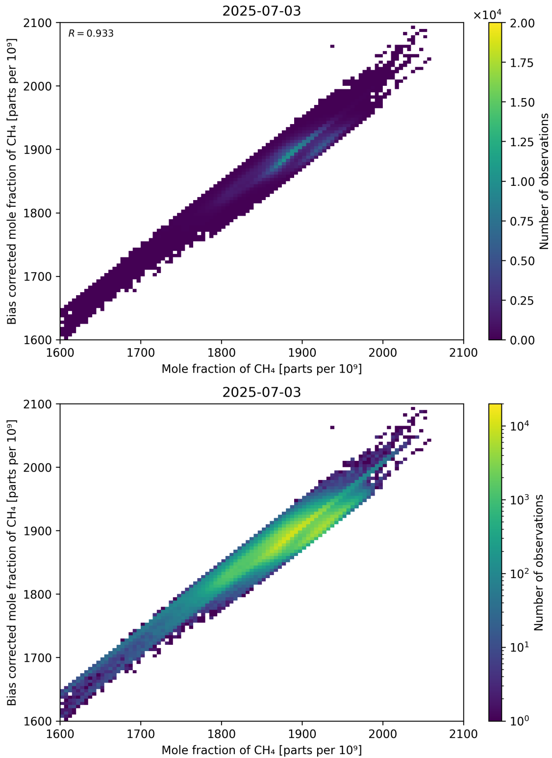
Figure 74: Scatter density plot of “Mole fraction of CH 4 ” against “Bias corrected mole fraction of CH 4 ” for 2025-07-03 to 2025-07-04.
