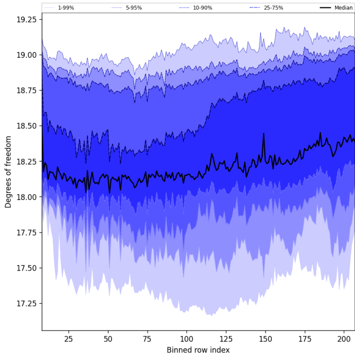
Figure 41: Along track statistics of “Degrees of freedom” for 2025-07-03 to 2025-07-04
