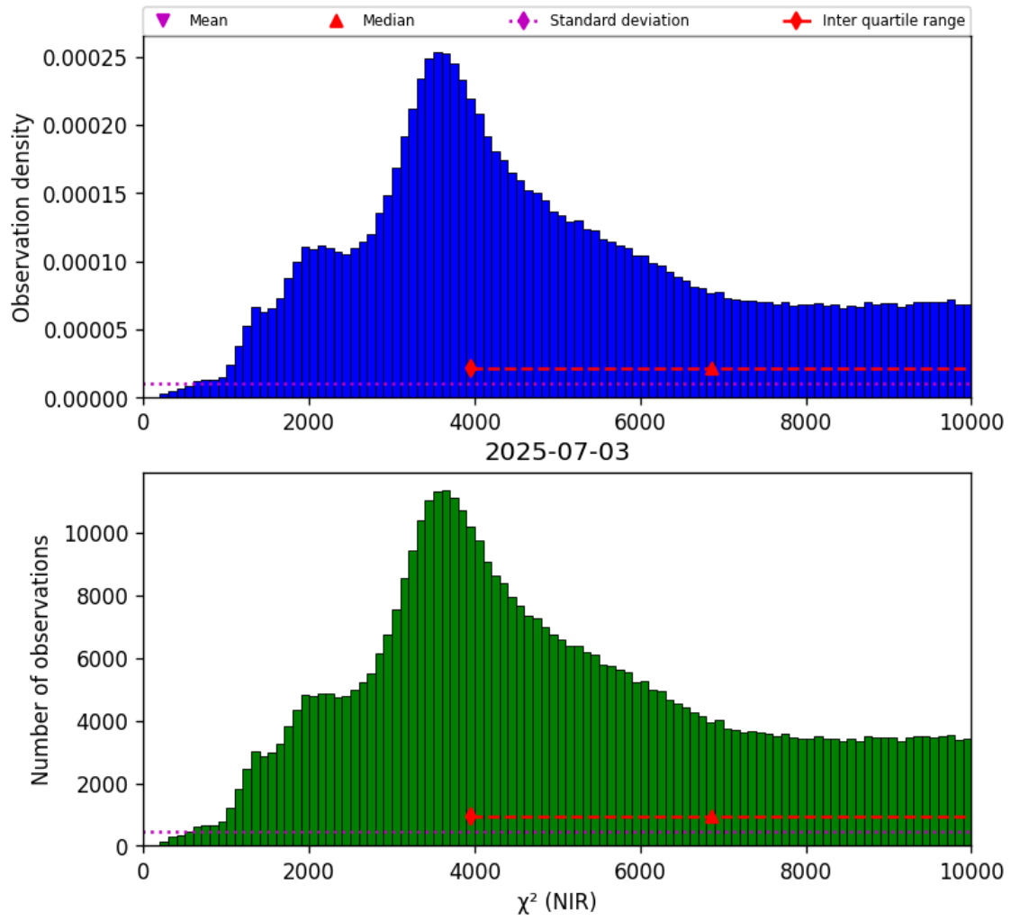
Figure 29: Histogram of “ \chi^2 (NIR)” for 2025-07-03 to 2025-07-04
