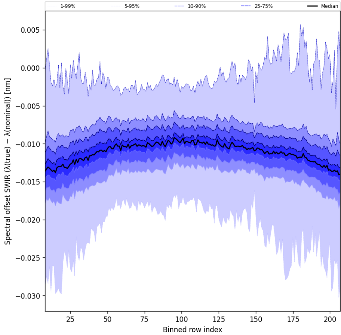
Figure 38: Along track statistics of “Spectral offset SWIR ( \lambda_{\text{true}} - \lambda_{\text{nominal}} )” for 2025-07-03 to 2025-07-04
