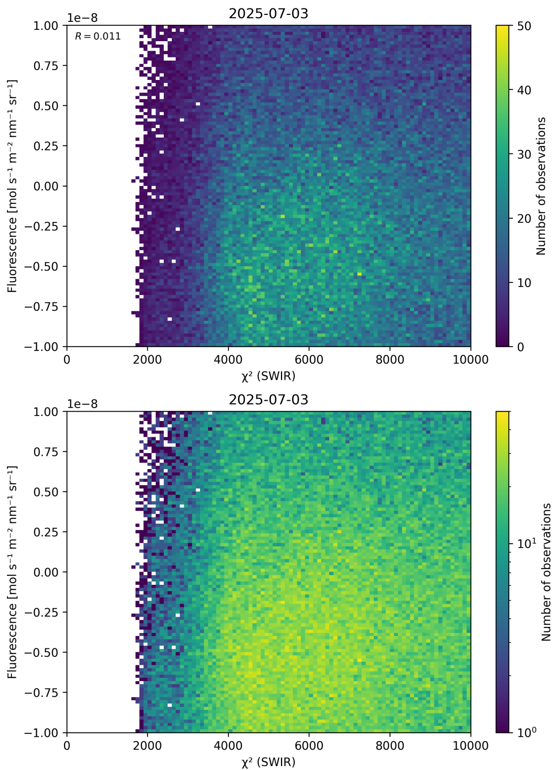
Figure 49: Scatter density plot of “ \chi^2 (SWIR)” against “Fluorescence” for 2025-07-03 to 2025-07-04.
