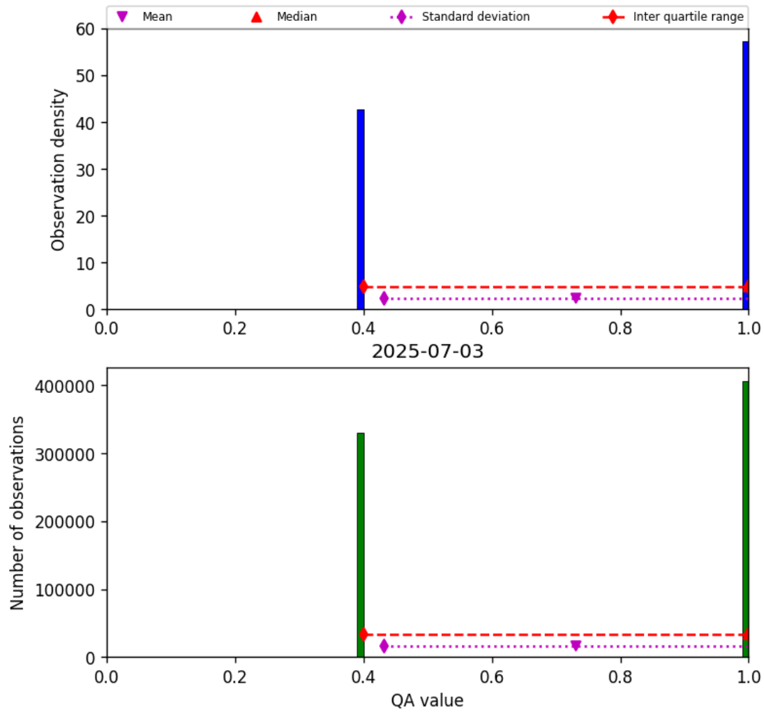
Figure 22: Histogram of “QA value” for 2025-07-03 to 2025-07-04
