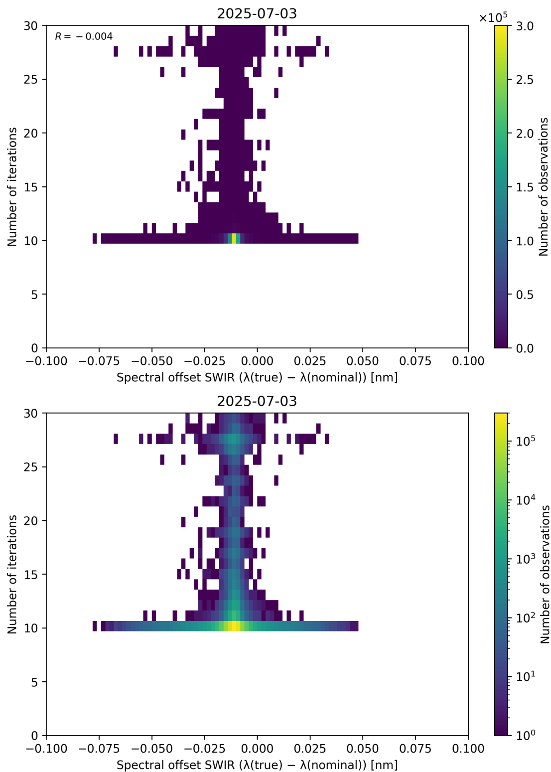
Figure 121: Scatter density plot of “Spectral offset SWIR ( \lambda_{\text{true}} - \lambda_{\text{nominal}} )” against “Number of iterations” for 2025-07-03 to 2025-07-04.
