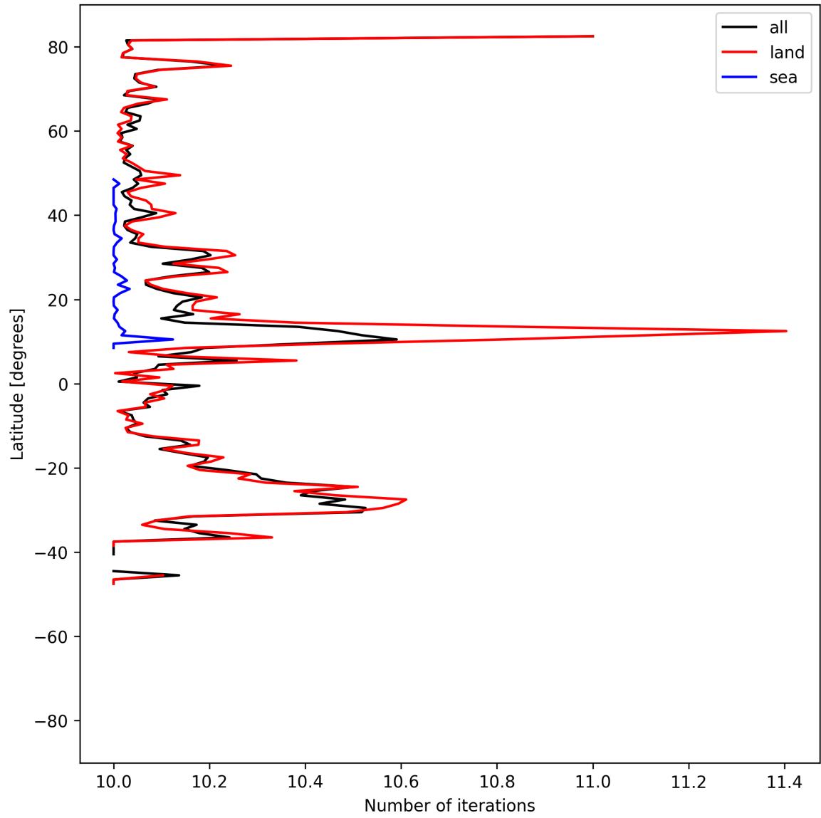
Figure 20: Zonal average of “Number of iterations” for 2025-07-03 to 2025-07-04.
