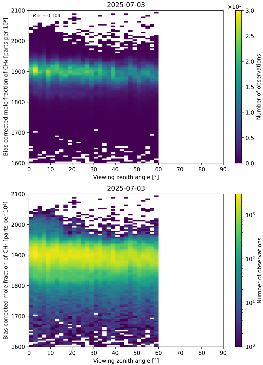
Figure 111: Scatter density plot of “Viewing zenith angle” against “Bias corrected mole fraction of CH 4 ” for 2025-07-03 to 2025-07-04.
