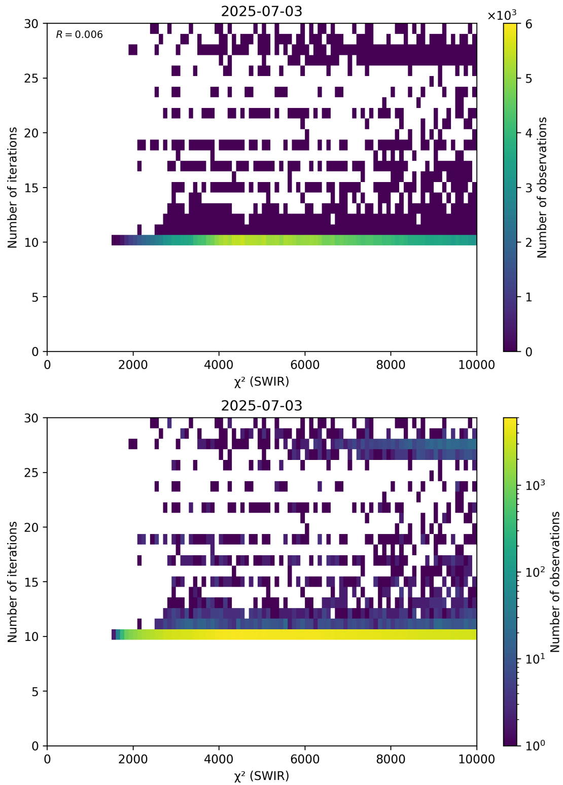
Figure 50: Scatter density plot of “ \chi^2 (SWIR)” against “Number of iterations” for 2025-07-03 to 2025-07-04.
