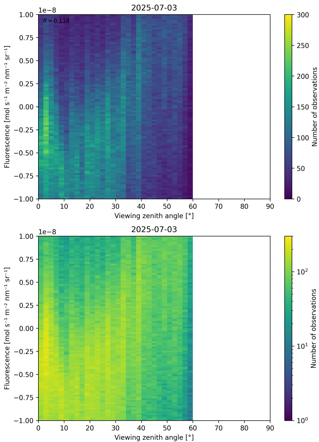
Figure 108: Scatter density plot of “Viewing zenith angle” against “Fluorescence” for 2025-07-03 to 2025-07-04.
