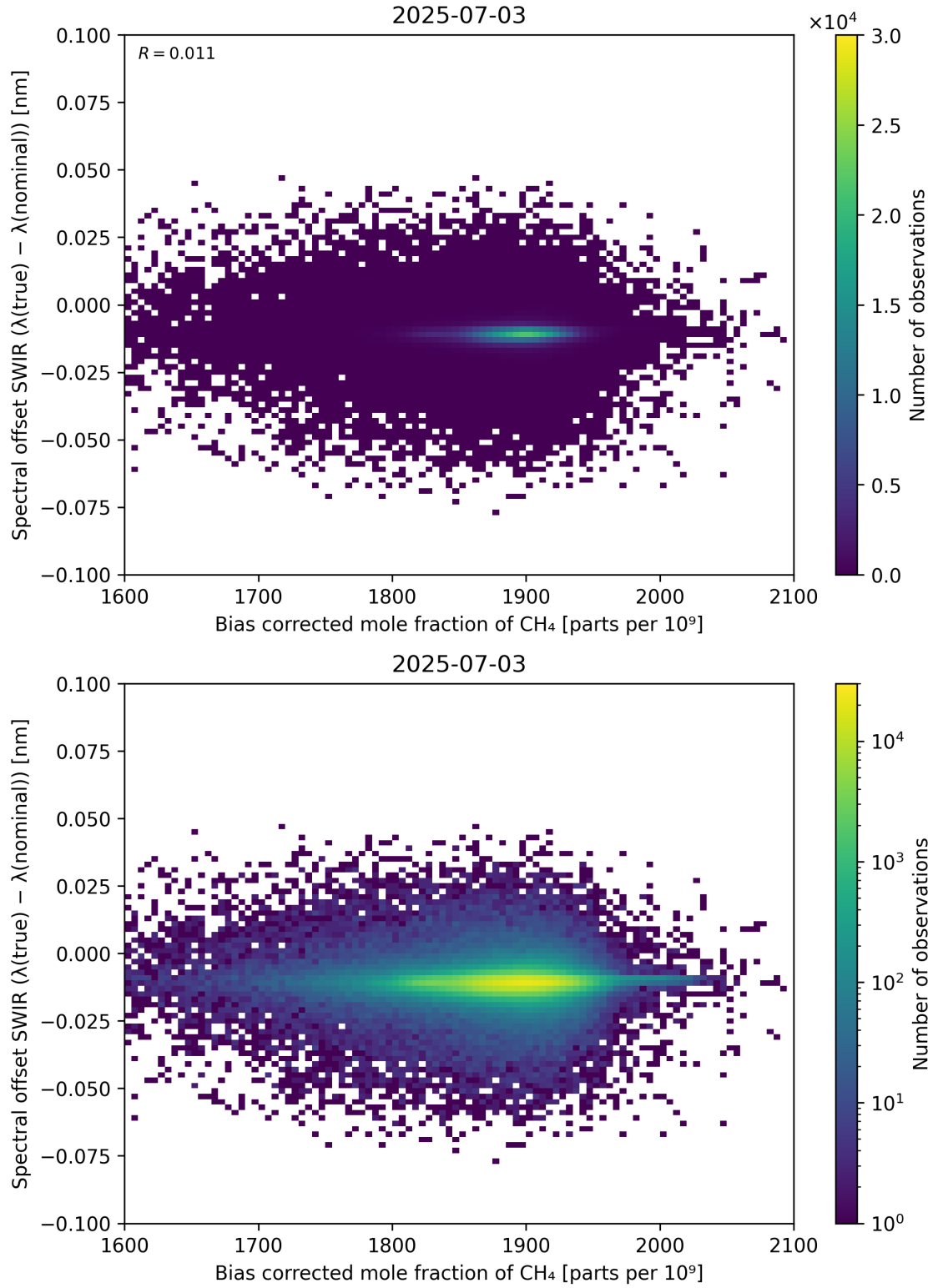
Figure 69: Scatter density plot of “Bias corrected mole fraction of CH 4 ” against “Spectral offset SWIR ( \lambda_{\text{true}} - \lambda_{\text{nominal}} )” for 2025-07-03 to 2025-07-04.
