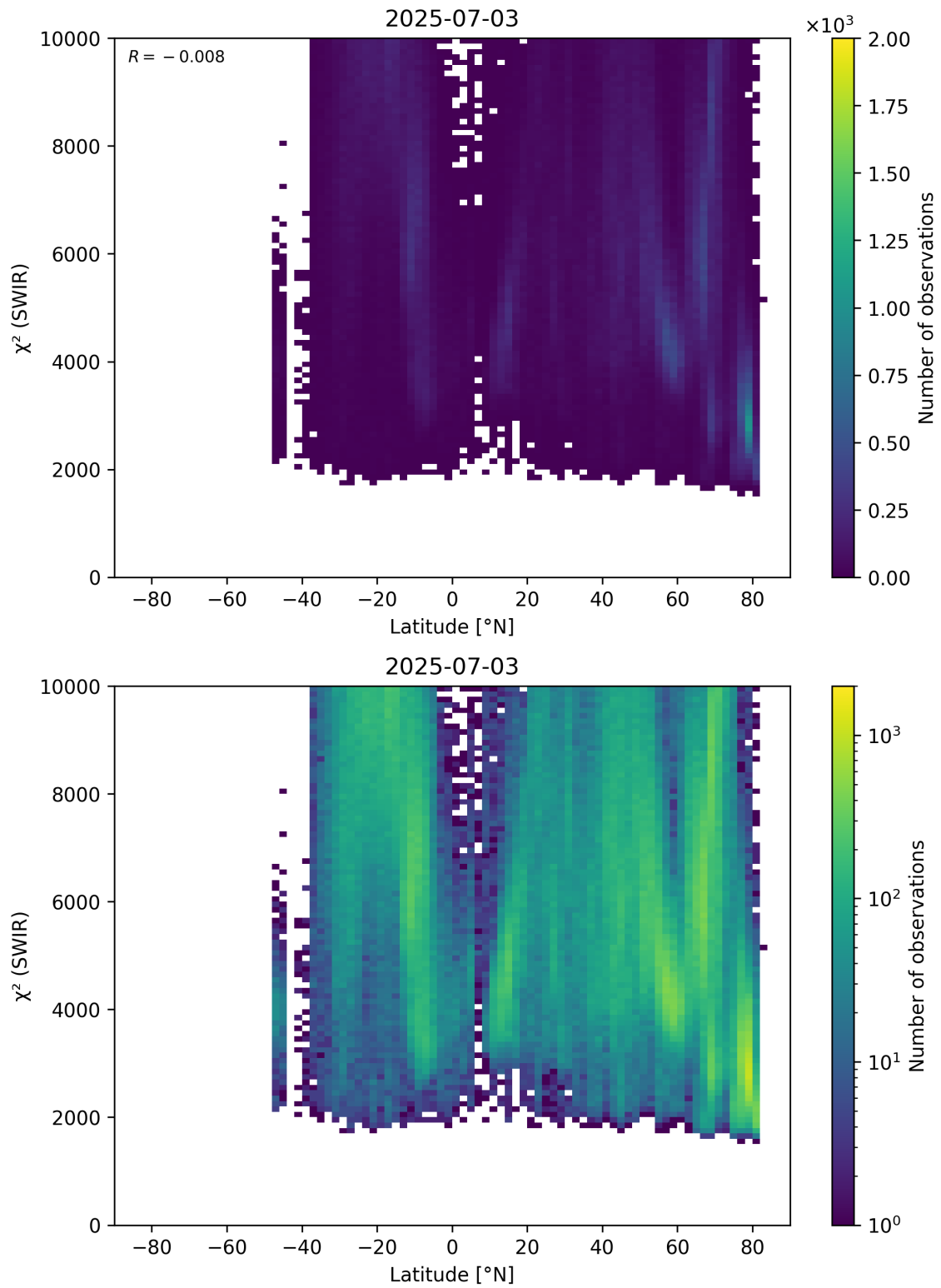
Figure 54: Scatter density plot of “Latitude” against “ \chi^2 (SWIR)” for 2025-07-03 to 2025-07-04.
