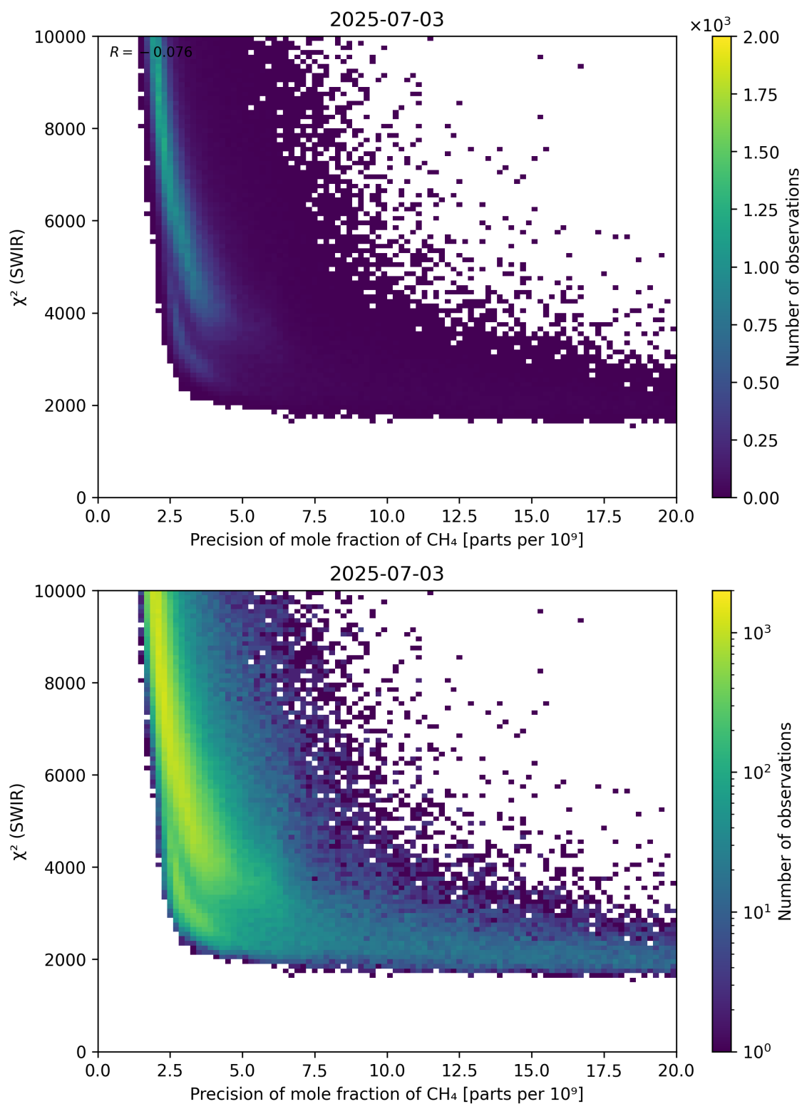
Figure 79: Scatter density plot of “Precision of mole fraction of \text{CH}_4 ” against “ \chi^2 (SWIR)” for 2025-07-03 to 2025-07-04.
