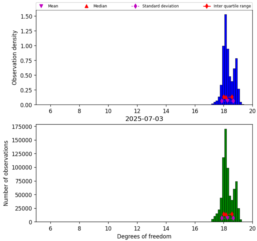
Figure 30: Histogram of “Degrees of freedom” for 2025-07-03 to 2025-07-04
