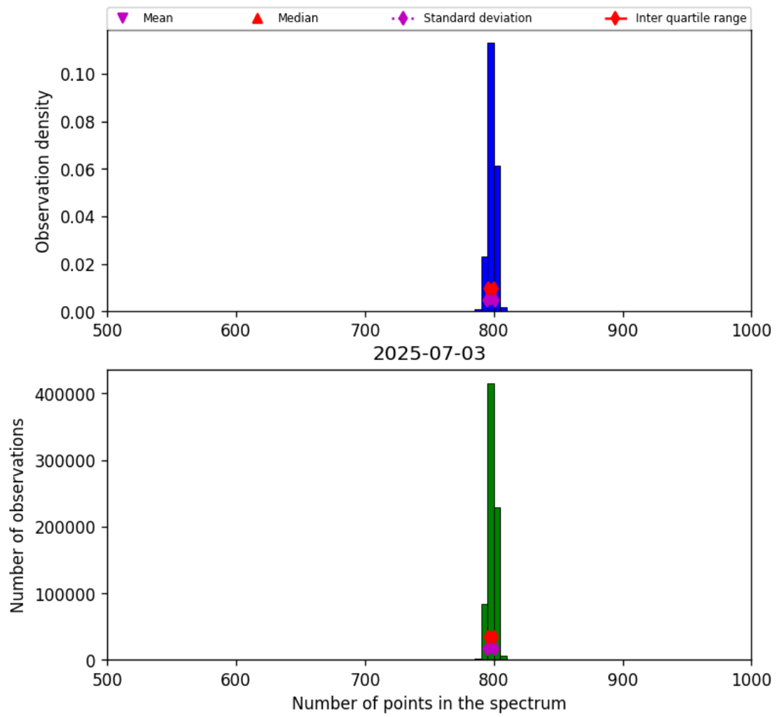
Figure 26: Histogram of “Number of points in the spectrum” for 2025-07-03 to 2025-07-04
