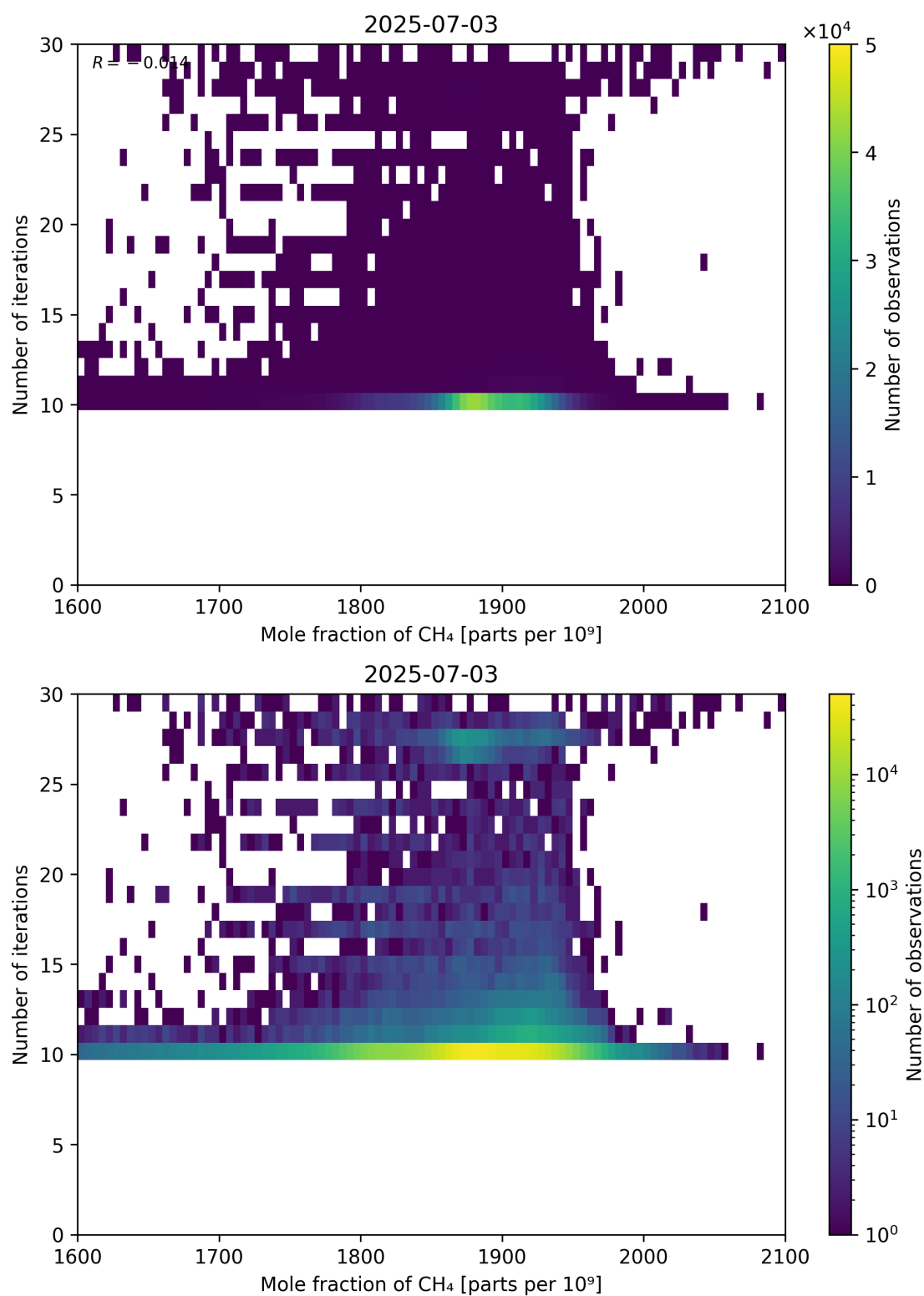
Figure 76: Scatter density plot of “Mole fraction of CH 4 ” against “Number of iterations” for 2025-07-03 to 2025-07-04.
