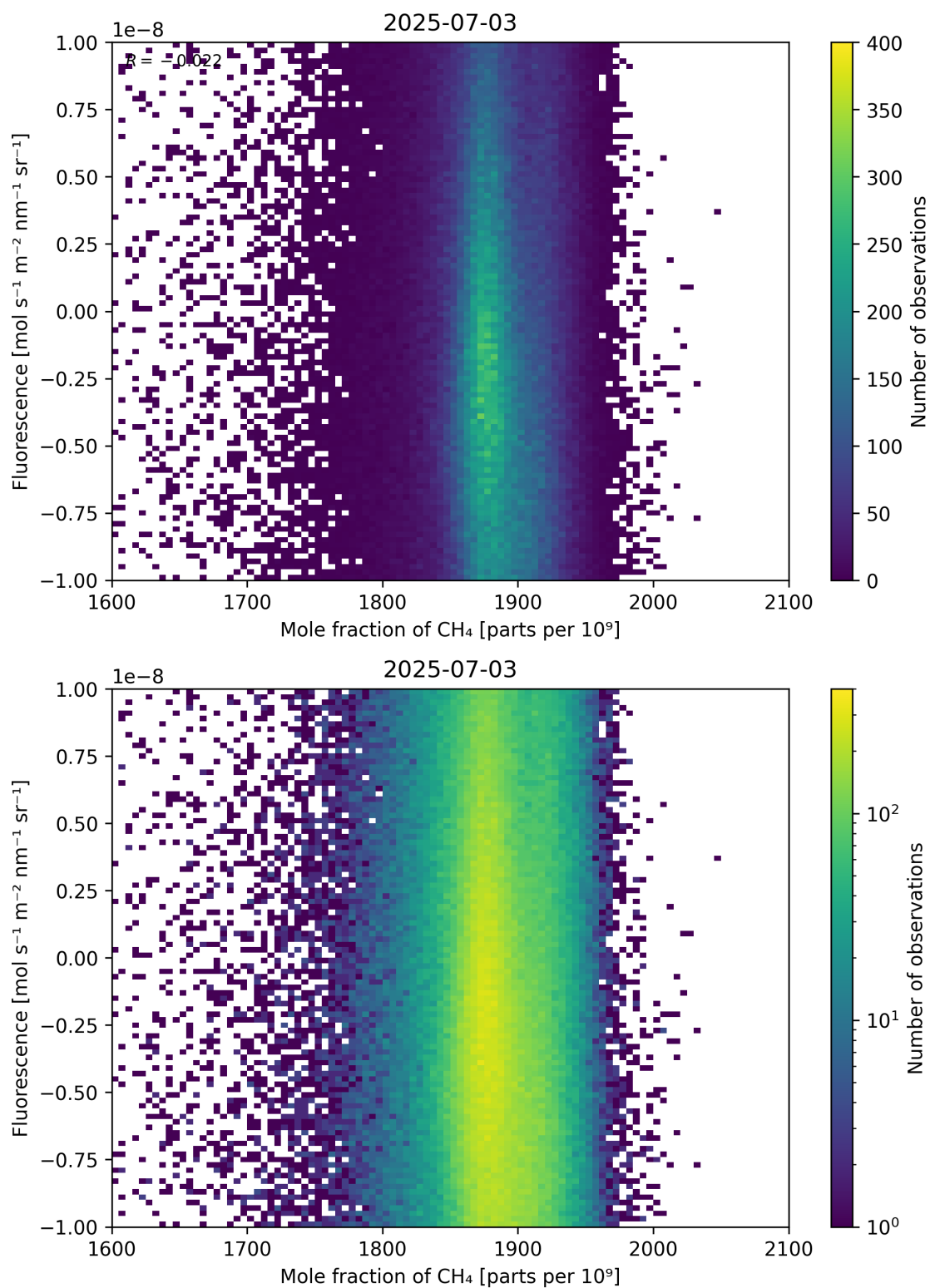
Figure 73: Scatter density plot of “Mole fraction of \text{CH}_4 ” against “Fluorescence” for 2025-07-03 to 2025-07-04.
