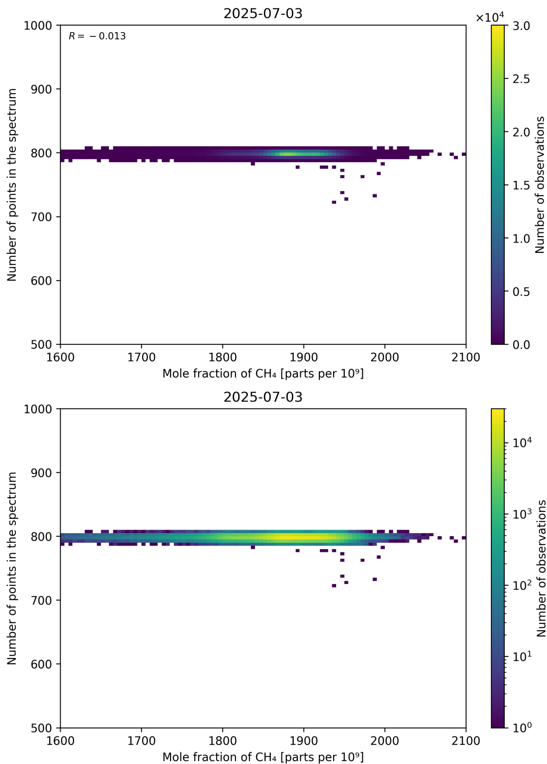
Figure 77: Scatter density plot of “Mole fraction of CH 4 ” against “Number of points in the spectrum” for 2025-07-03 to 2025-07-04.
