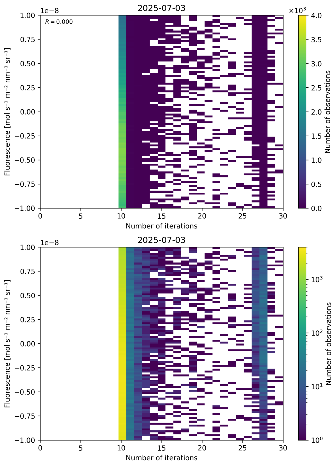
Figure 87: Scatter density plot of “Number of iterations” against “Fluorescence” for 2025-07-03 to 2025-07-04.
