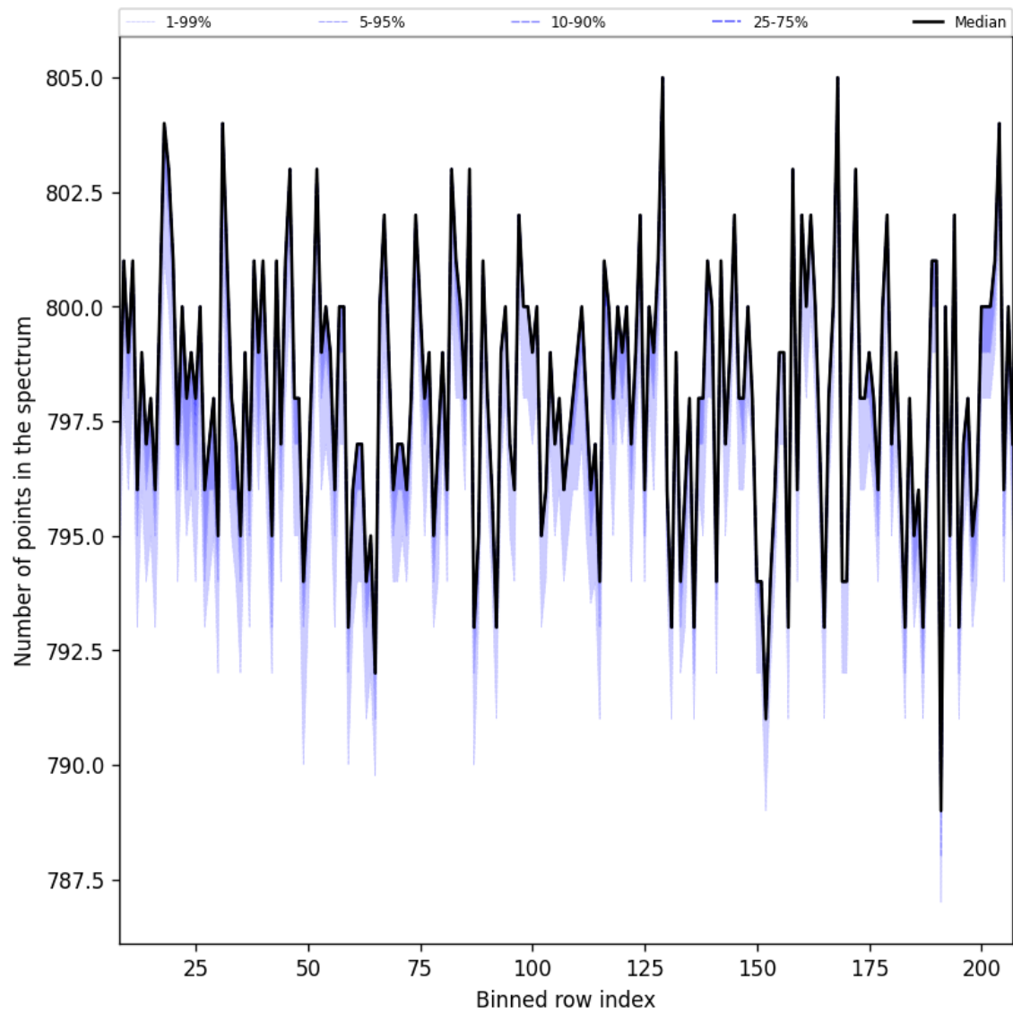
Figure 37: Along track statistics of “Number of points in the spectrum” for 2025-07-03 to 2025-07-04
