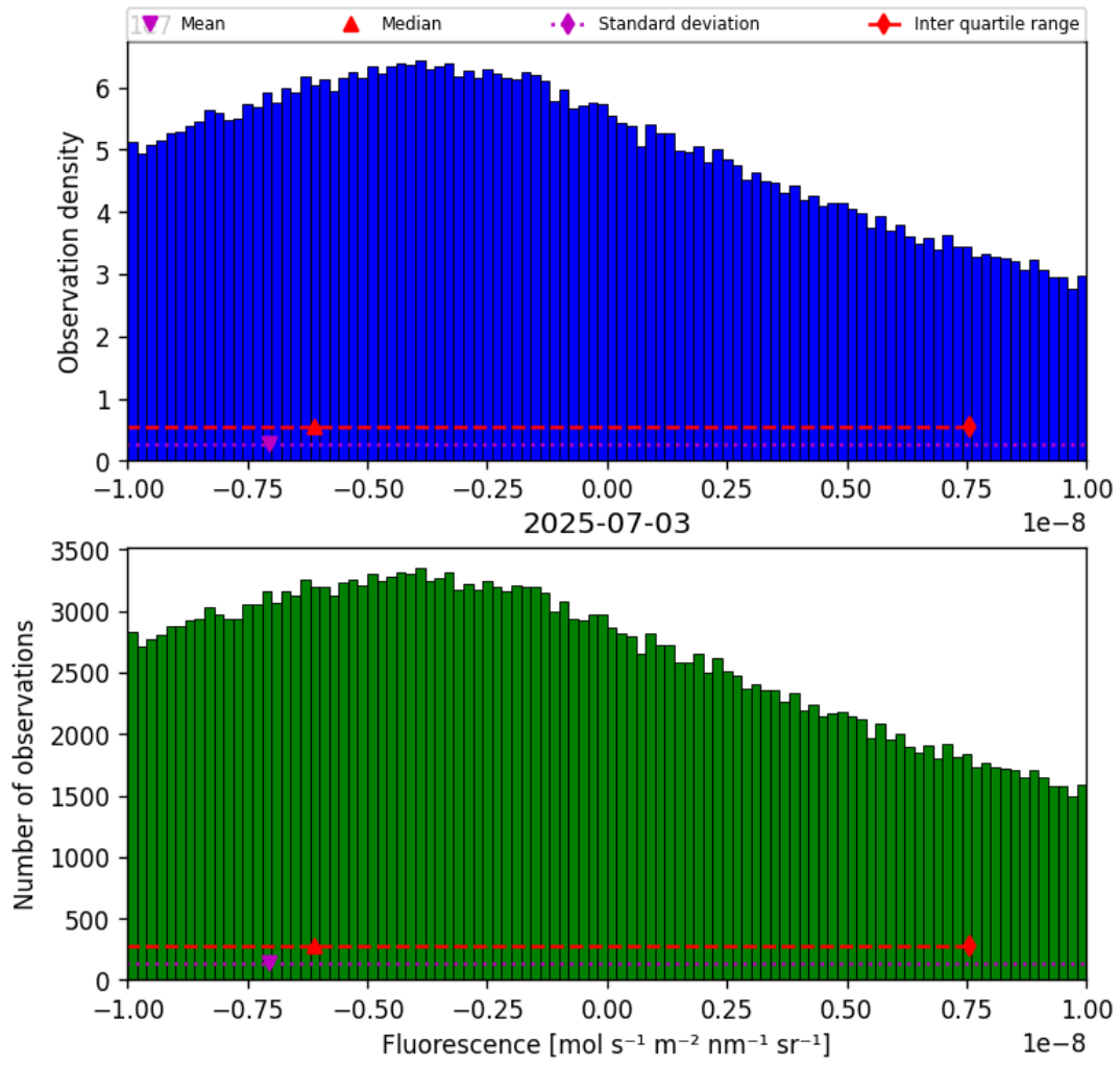
Figure 32: Histogram of “Fluorescence” for 2025-07-03 to 2025-07-04
