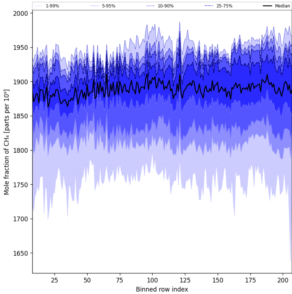
Figure 34: Along track statistics of “Mole fraction of CH 4 ” for 2025-07-03 to 2025-07-04
