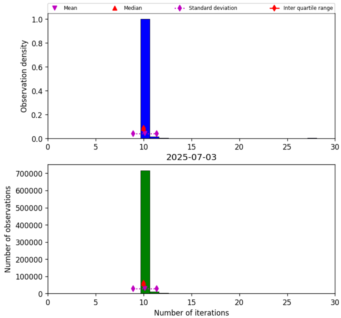
Figure 31: Histogram of “Number of iterations” for 2025-07-03 to 2025-07-04
