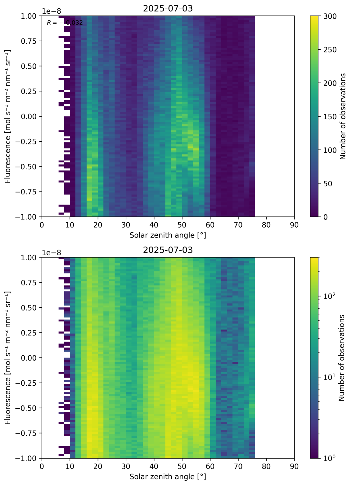
Figure 97: Scatter density plot of “Solar zenith angle” against “Fluorescence” for 2025-07-03 to 2025-07-04.
