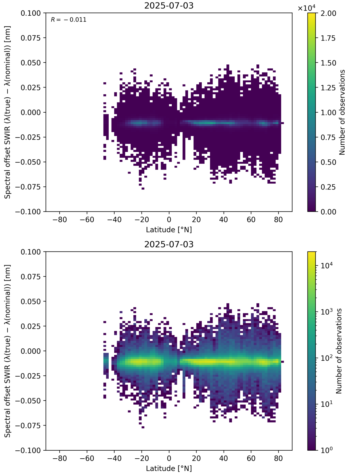
Figure 62: Scatter density plot of “Latitude” against “Spectral offset SWIR ( \lambda_{\text{true}} - \lambda_{\text{nominal}} )” for 2025-07-03 to 2025-07-04.
