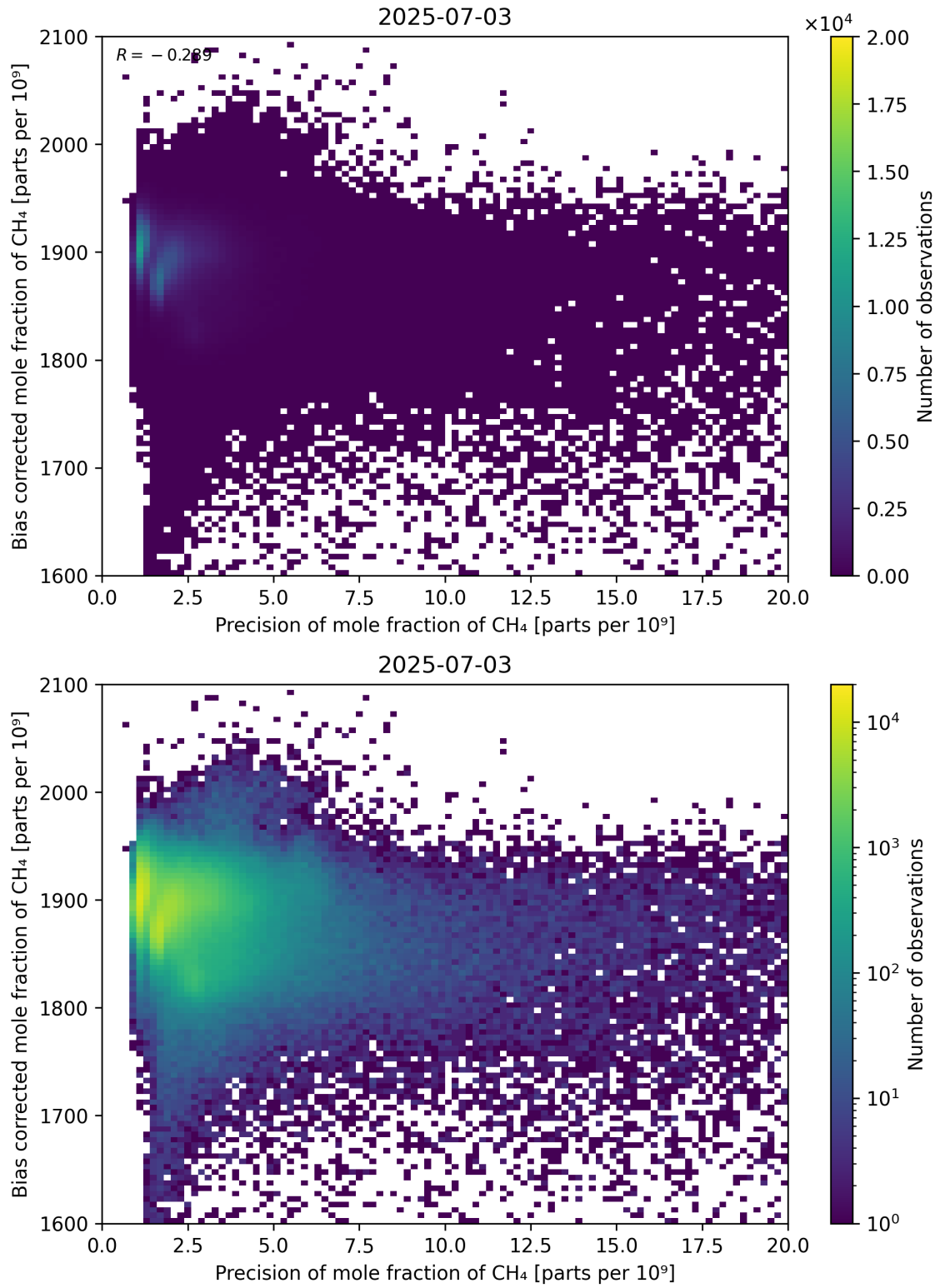
Figure 82: Scatter density plot of “Precision of mole fraction of CH 4 ” against “Bias corrected mole fraction of CH 4 ” for 2025-07-03 to 2025-07-04.
