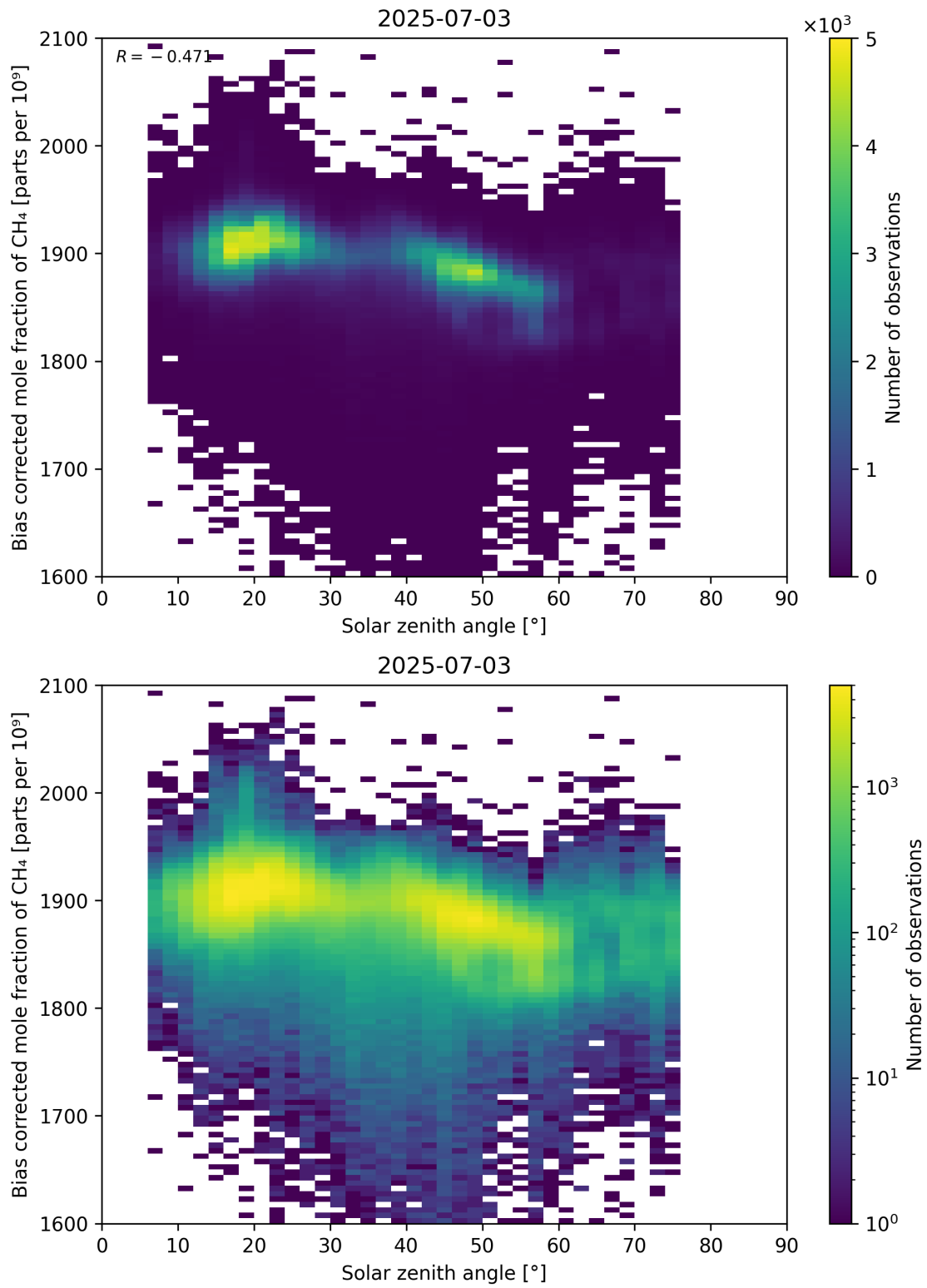
Figure 100: Scatter density plot of “Solar zenith angle” against “Bias corrected mole fraction of CH 4 ” for 2025-07-03 to 2025-07-04.
