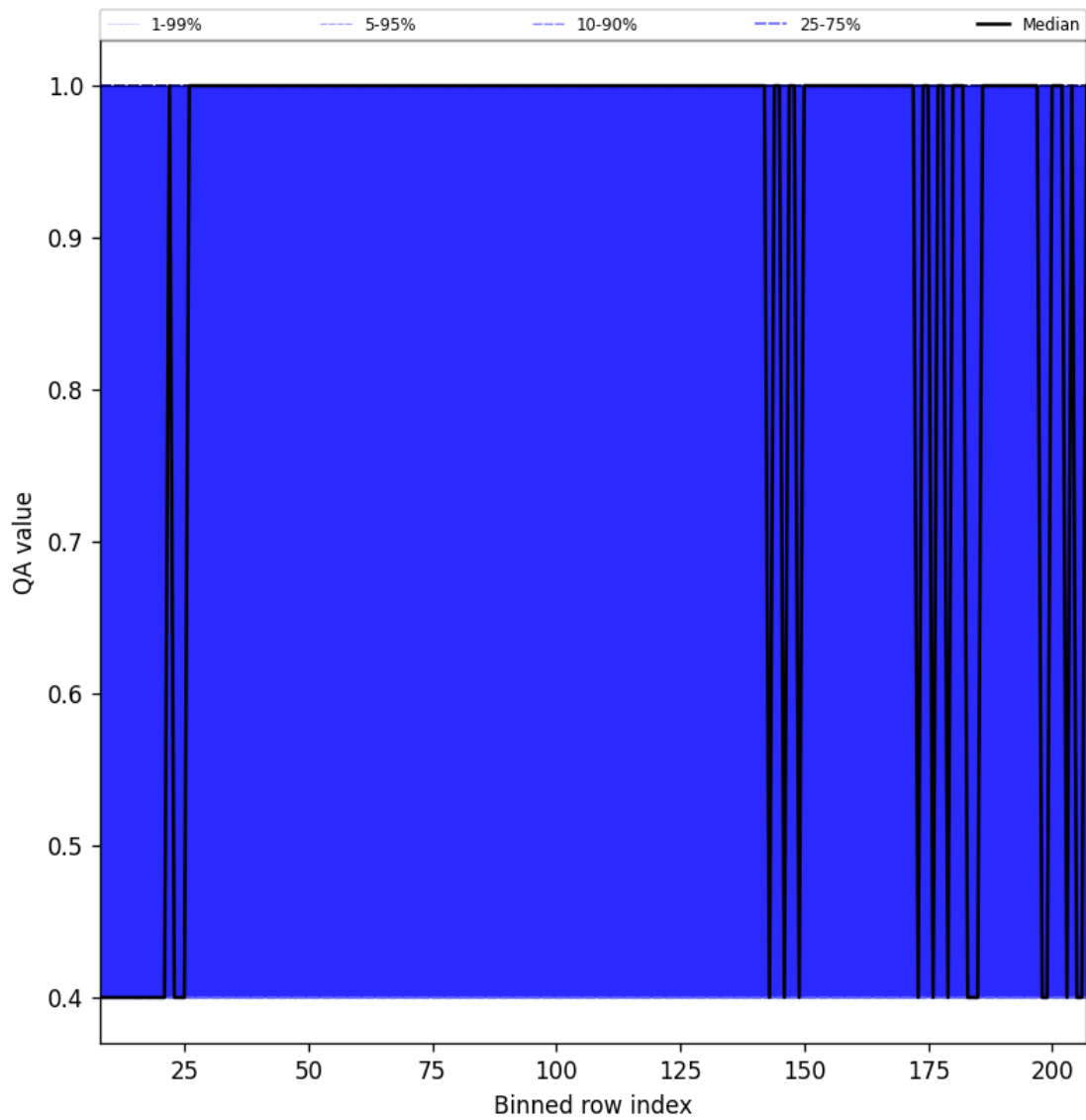
Figure 33: Along track statistics of “QA value” for 2025-07-03 to 2025-07-04
