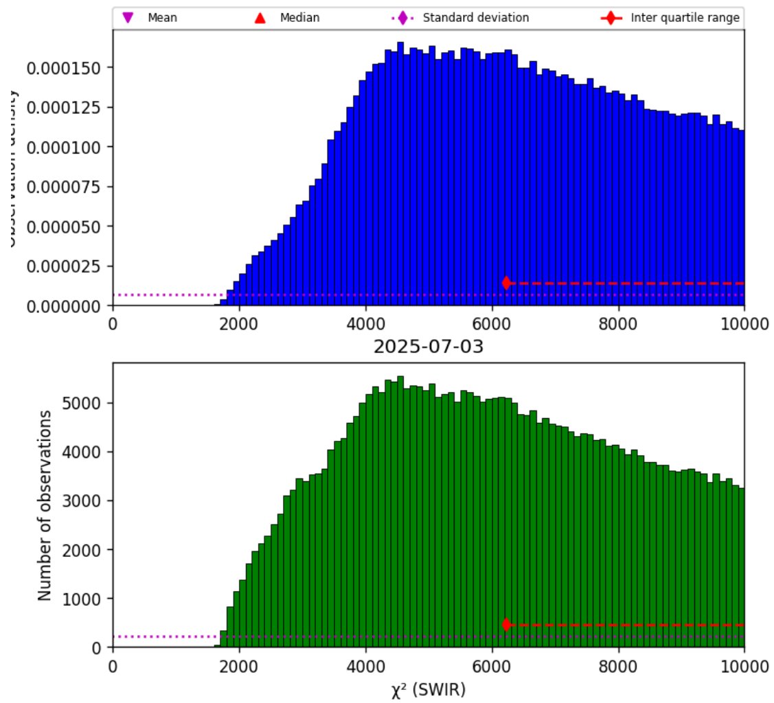
Figure 28: Histogram of “ \chi^2 (SWIR)” for 2025-07-03 to 2025-07-04
