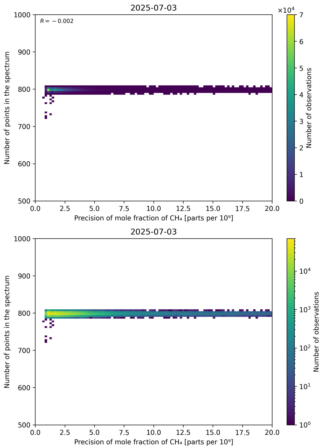
Figure 84: Scatter density plot of “Precision of mole fraction of CH 4 ” against “Number of points in the spectrum” for 2025-07-03 to 2025-07-04.
