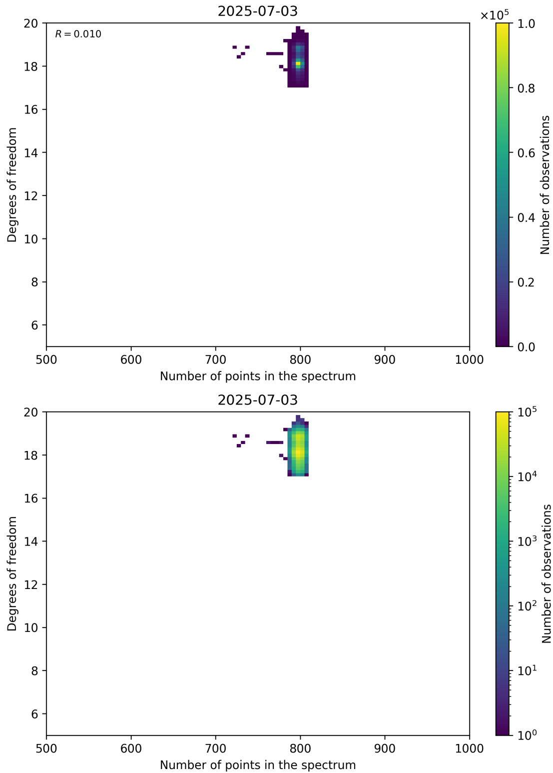
Figure 90: Scatter density plot of “Number of points in the spectrum” against “Degrees of freedom” for 2025-07-03 to 2025-07-04.
