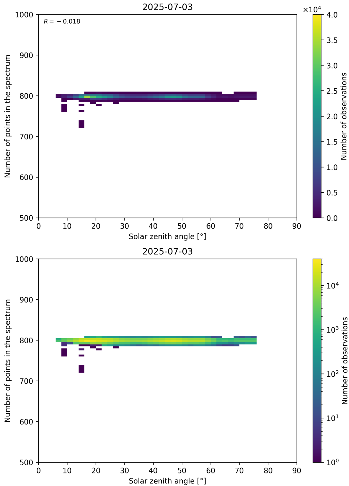
Figure 103: Scatter density plot of “Solar zenith angle” against “Number of points in the spectrum” for 2025-07-03 to 2025-07-04.
