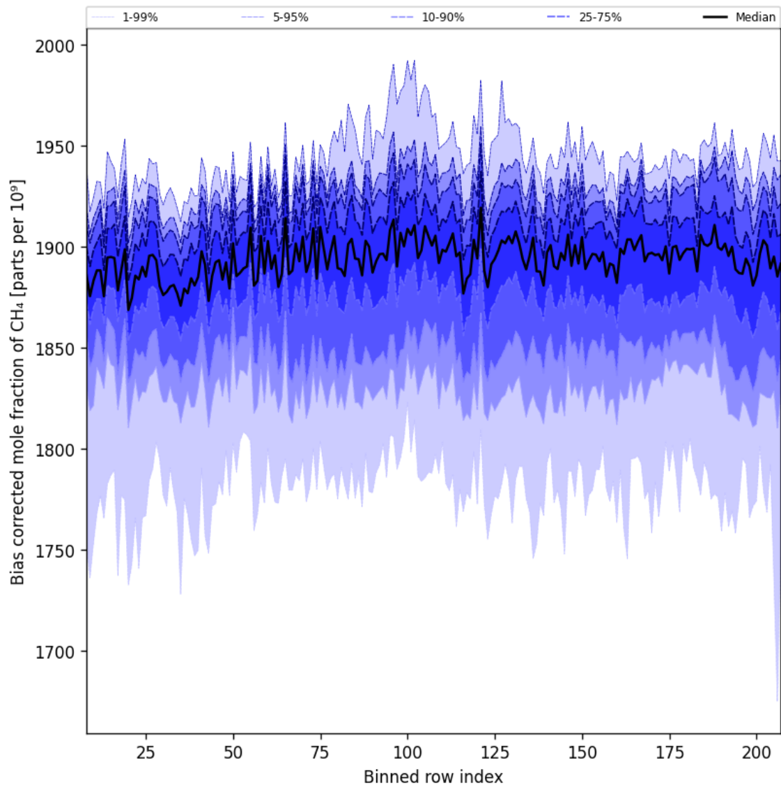
Figure 36: Along track statistics of “Bias corrected mole fraction of CH 4 ” for 2025-07-03 to 2025-07-04
