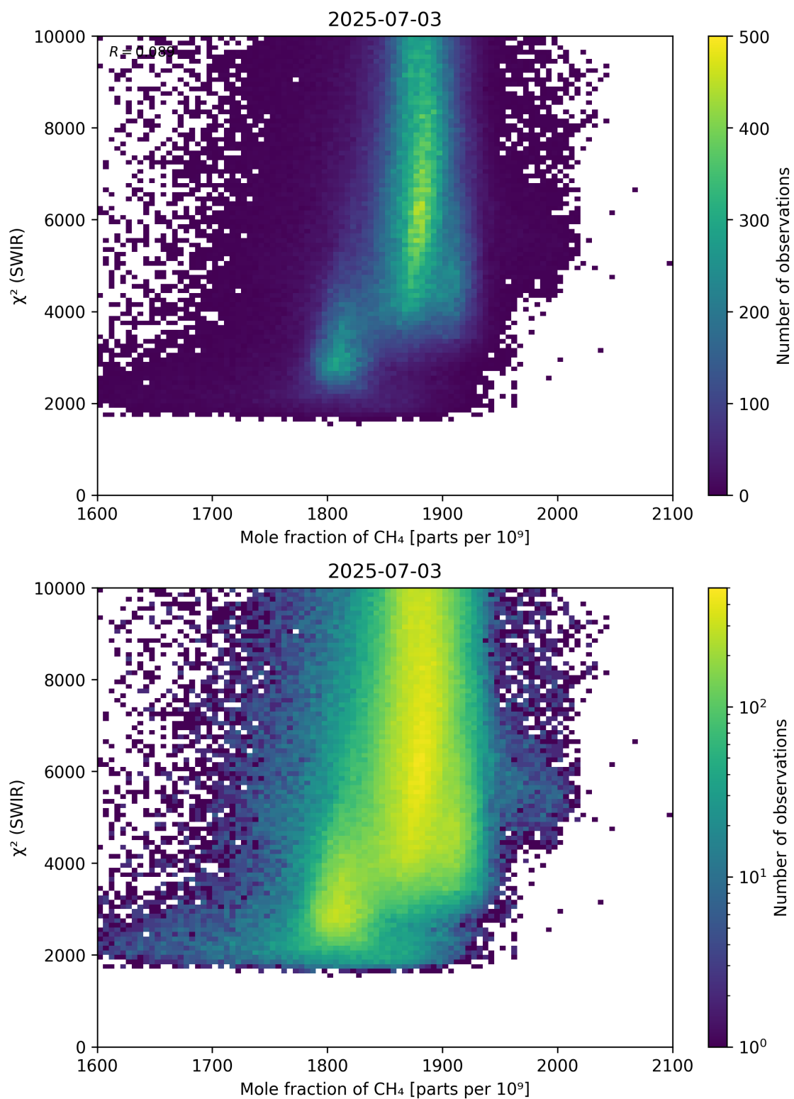
Figure 71: Scatter density plot of “Mole fraction of \text{CH}_4 ” against “ \chi^2 (SWIR)” for 2025-07-03 to 2025-07-04.
