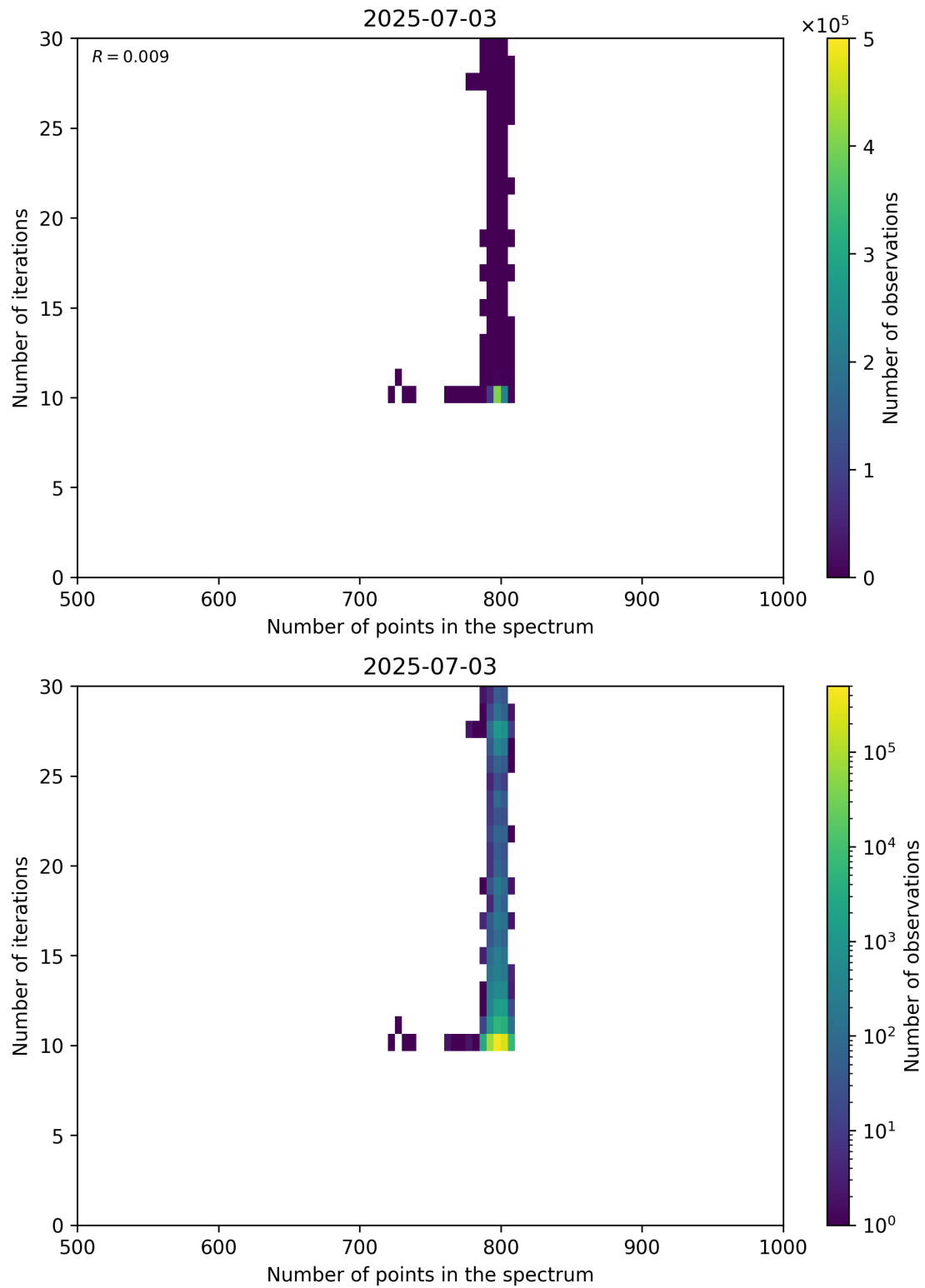
Figure 92: Scatter density plot of “Number of points in the spectrum” against “Number of iterations” for 2025-07-03 to 2025-07-04.
