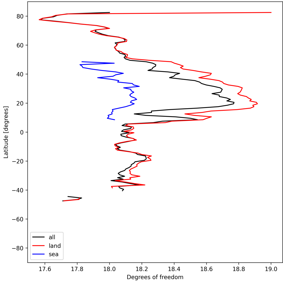
Figure 19: Zonal average of “Degrees of freedom” for 2025-07-03 to 2025-07-04.
