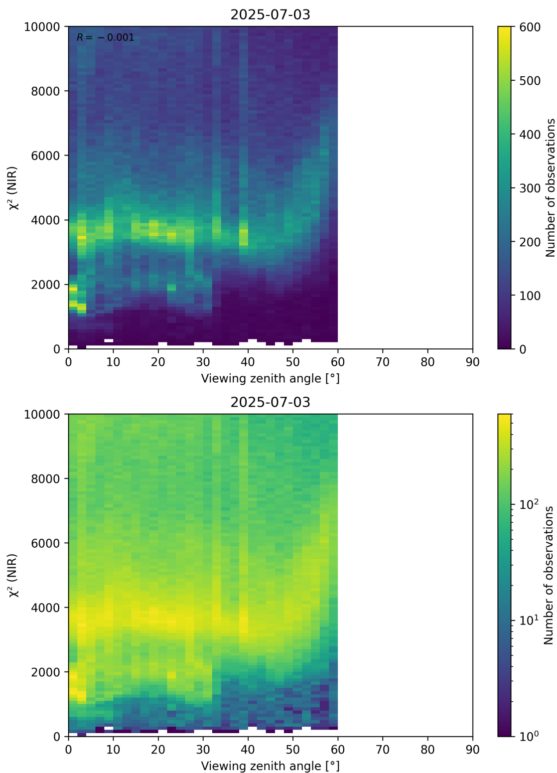
Figure 105: Scatter density plot of “Viewing zenith angle” against “ \chi^2 (NIR)” for 2025-07-03 to 2025-07-04.
