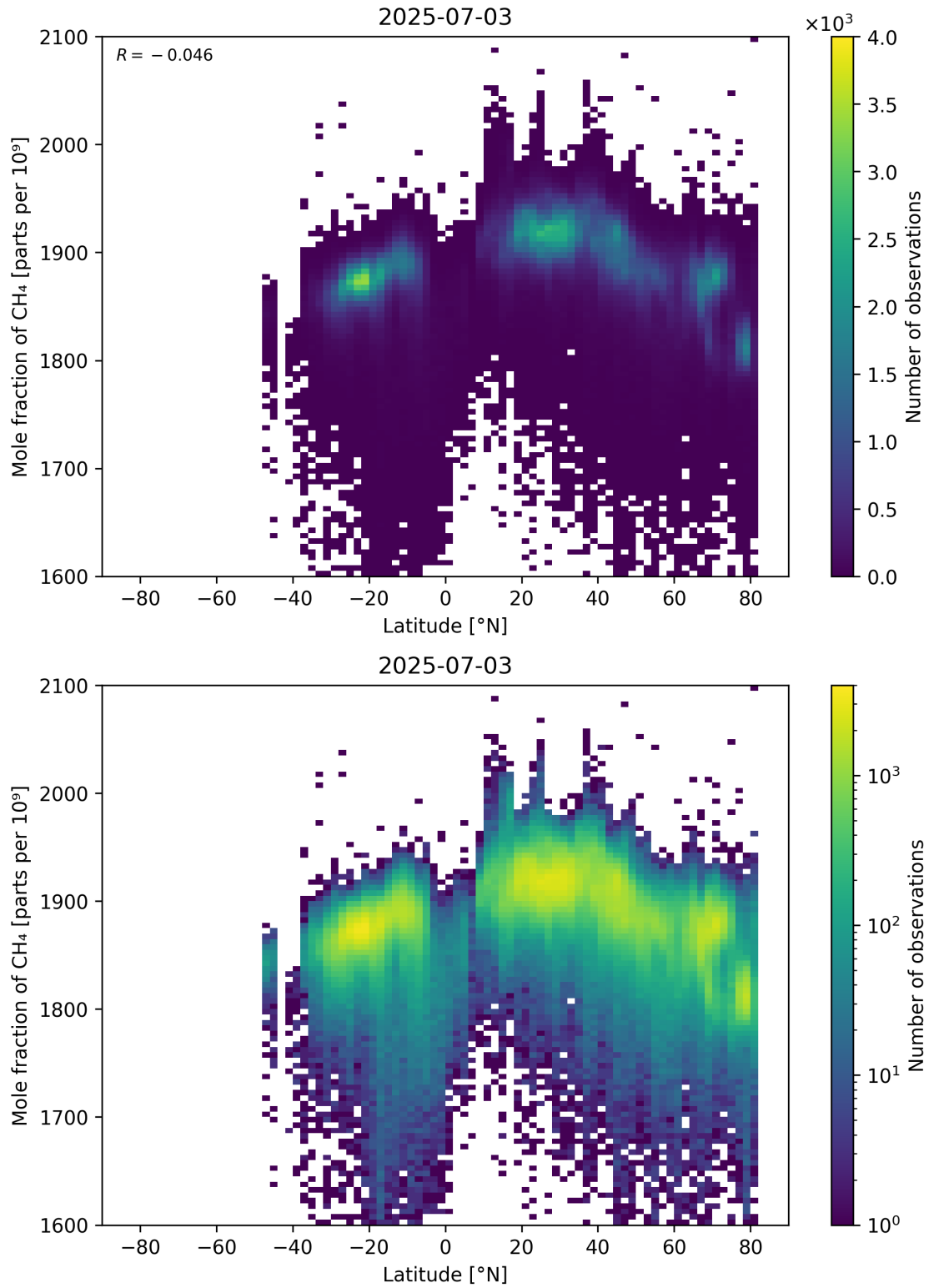
Figure 57: Scatter density plot of “Latitude” against “Mole fraction of CH 4 ” for 2025-07-03 to 2025-07-04.
