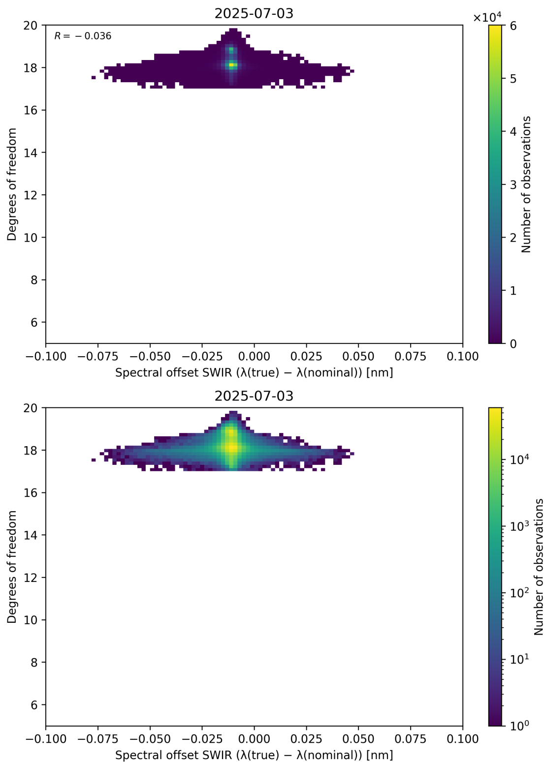
Figure 119: Scatter density plot of “Spectral offset SWIR ( \lambda_{\text{true}} - \lambda_{\text{nominal}} )” against “Degrees of freedom” for 2025-07-03 to 2025-07-04.
