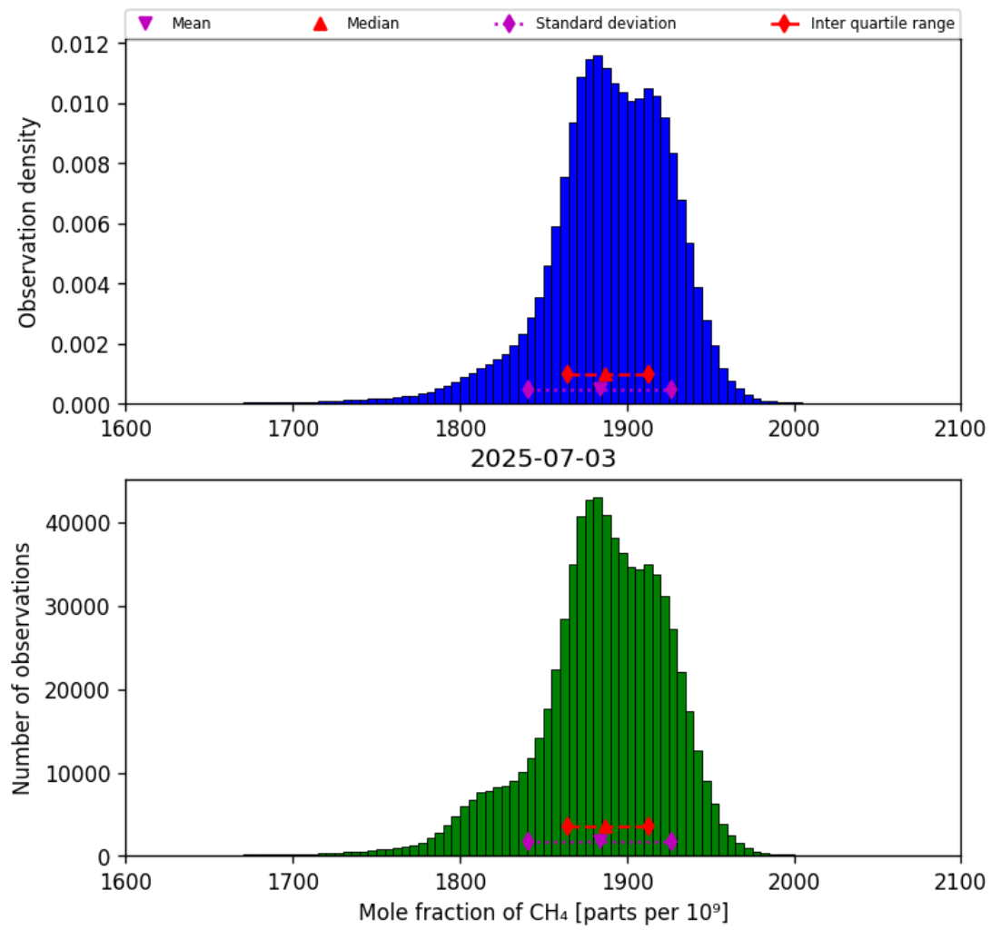
Figure 23: Histogram of “Mole fraction of CH 4 ” for 2025-07-03 to 2025-07-04
