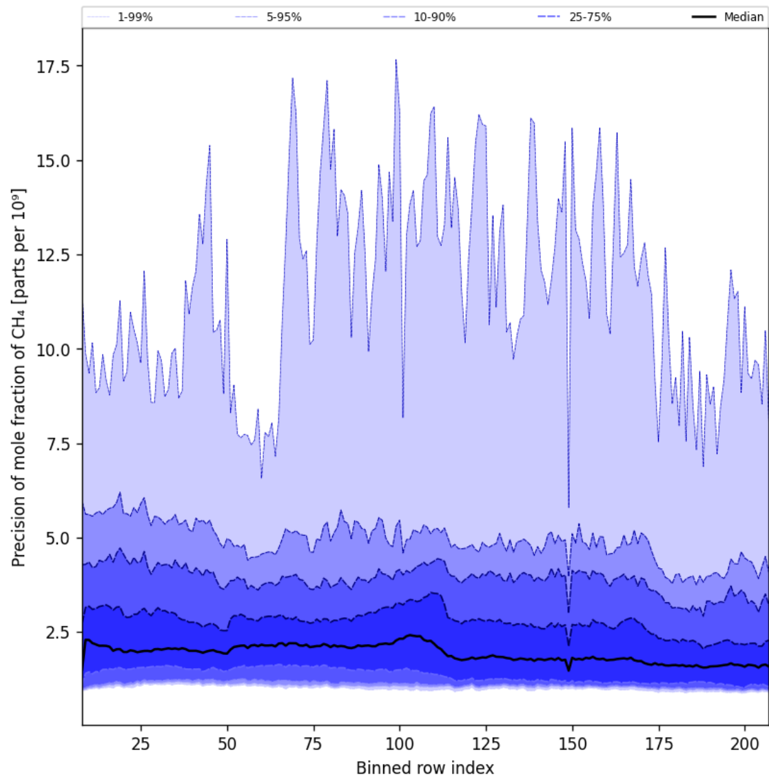
Figure 35: Along track statistics of “Precision of mole fraction of CH 4 ” for 2025-07-03 to 2025-07-04
