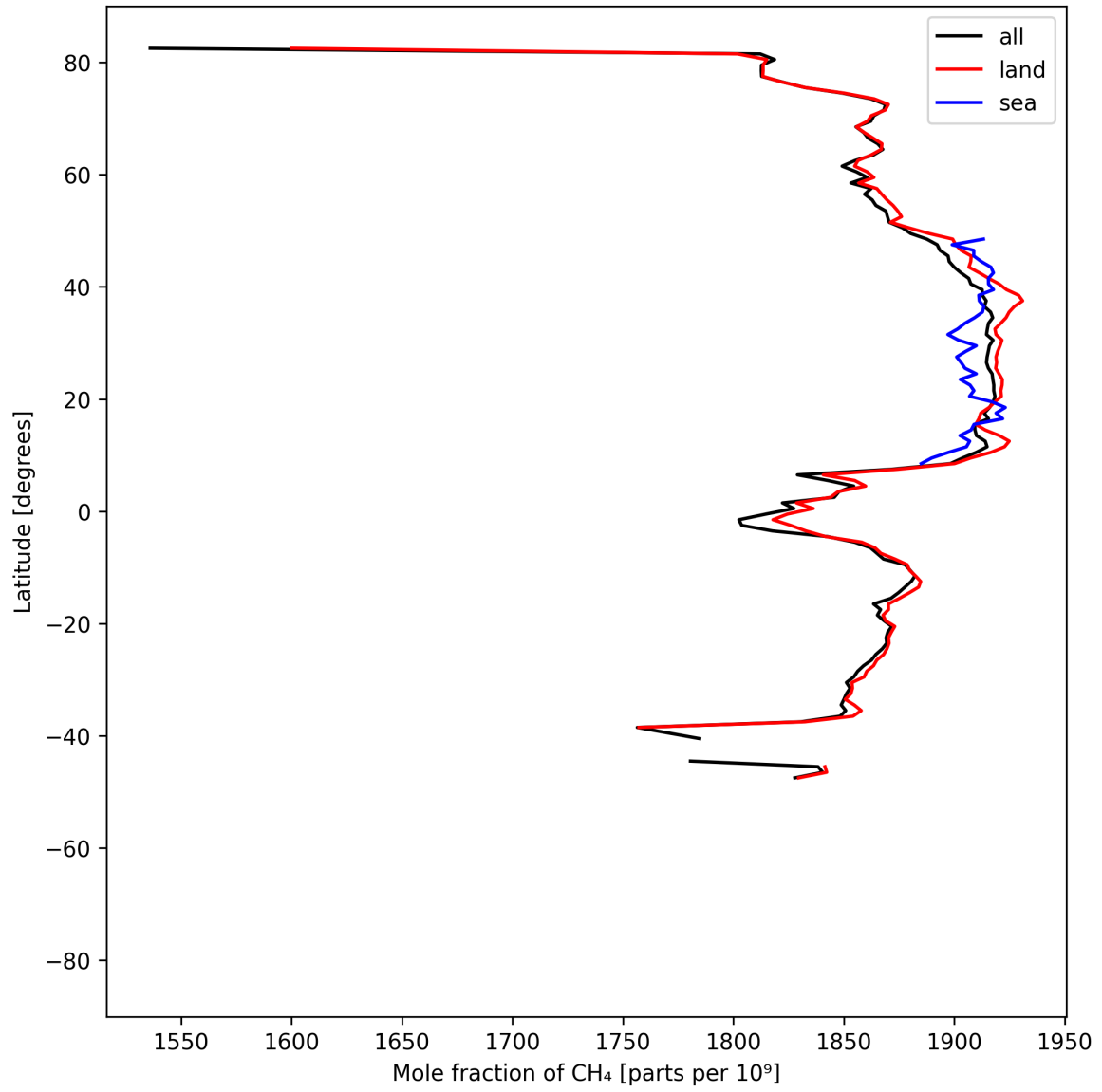
Figure 12: Zonal average of “Mole fraction of \text{CH}_4 ” for 2025-07-03 to 2025-07-04.
