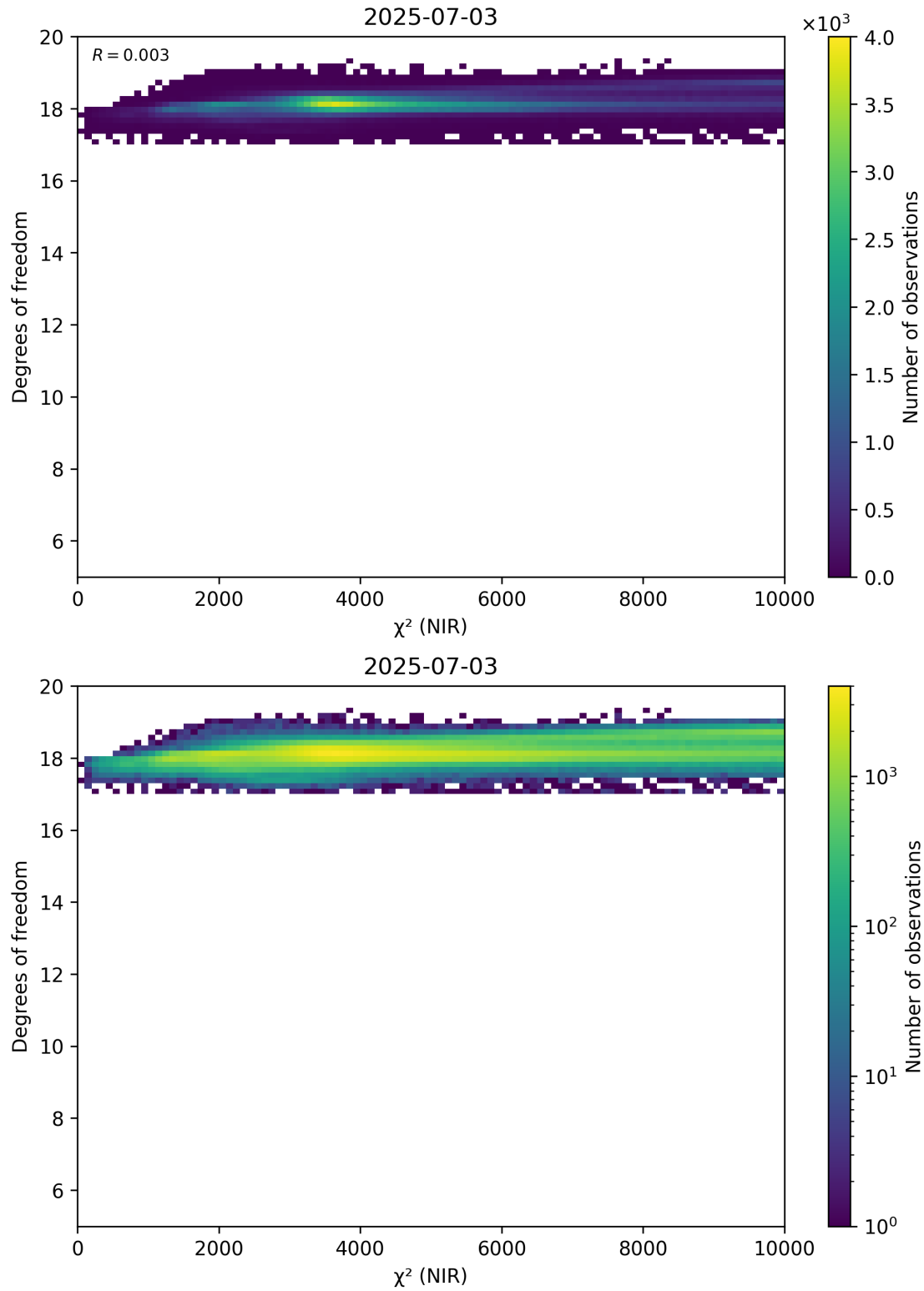
Figure 44: Scatter density plot of “ \chi^2 (NIR)” against “Degrees of freedom” for 2025-07-03 to 2025-07-04.
