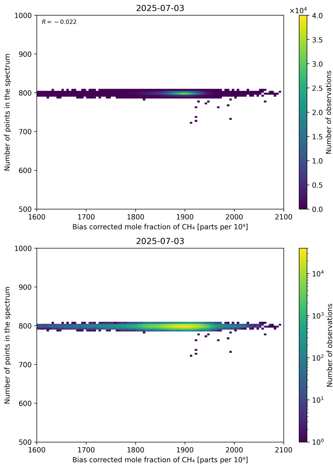
Figure 68: Scatter density plot of “Bias corrected mole fraction of CH 4 ” against “Number of points in the spectrum” for 2025-07-03 to 2025-07-04.
