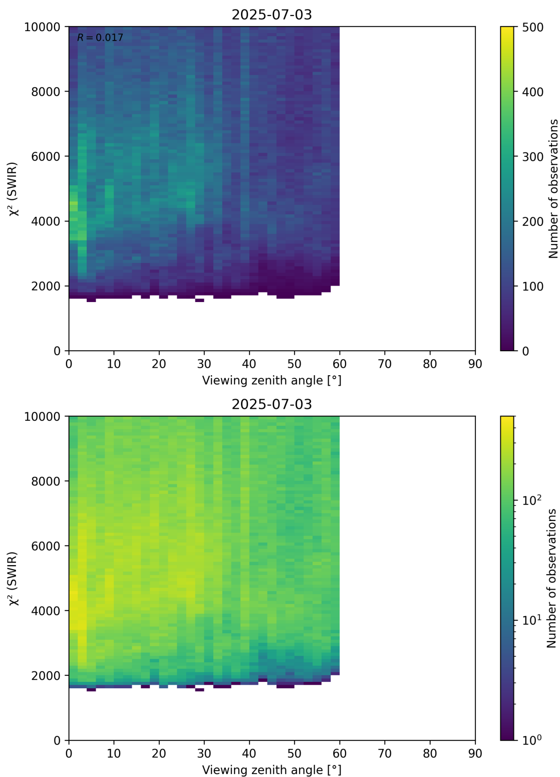
Figure 106: Scatter density plot of “Viewing zenith angle” against “ \chi^2 (SWIR)” for 2025-07-03 to 2025-07-04.
