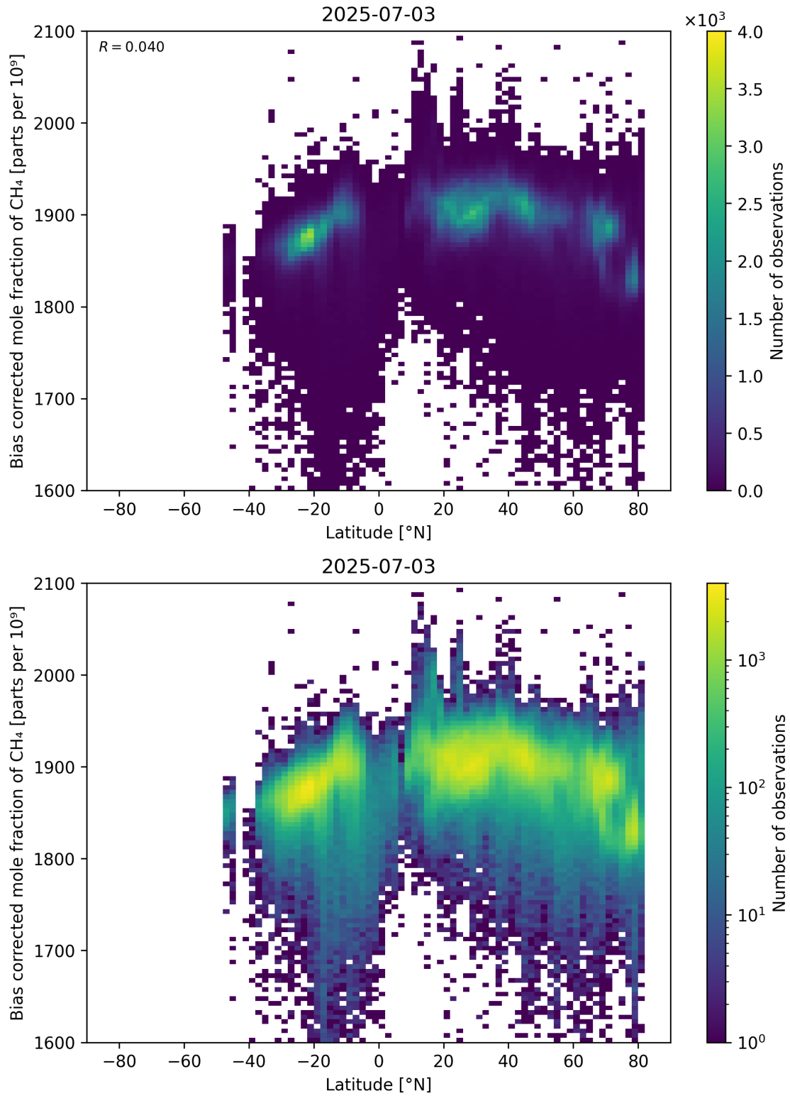
Figure 58: Scatter density plot of “Latitude” against “Bias corrected mole fraction of \text{CH}_4 ” for 2025-07-03 to 2025-07-04.
