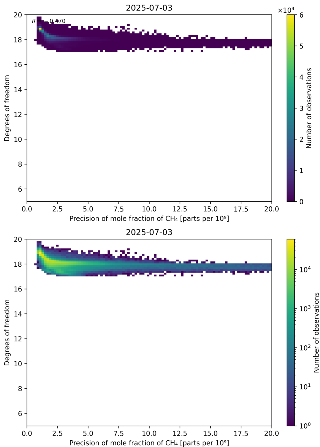
Figure 80: Scatter density plot of “Precision of mole fraction of CH 4 ” against “Degrees of freedom” for 2025-07-03 to 2025-07-04.
