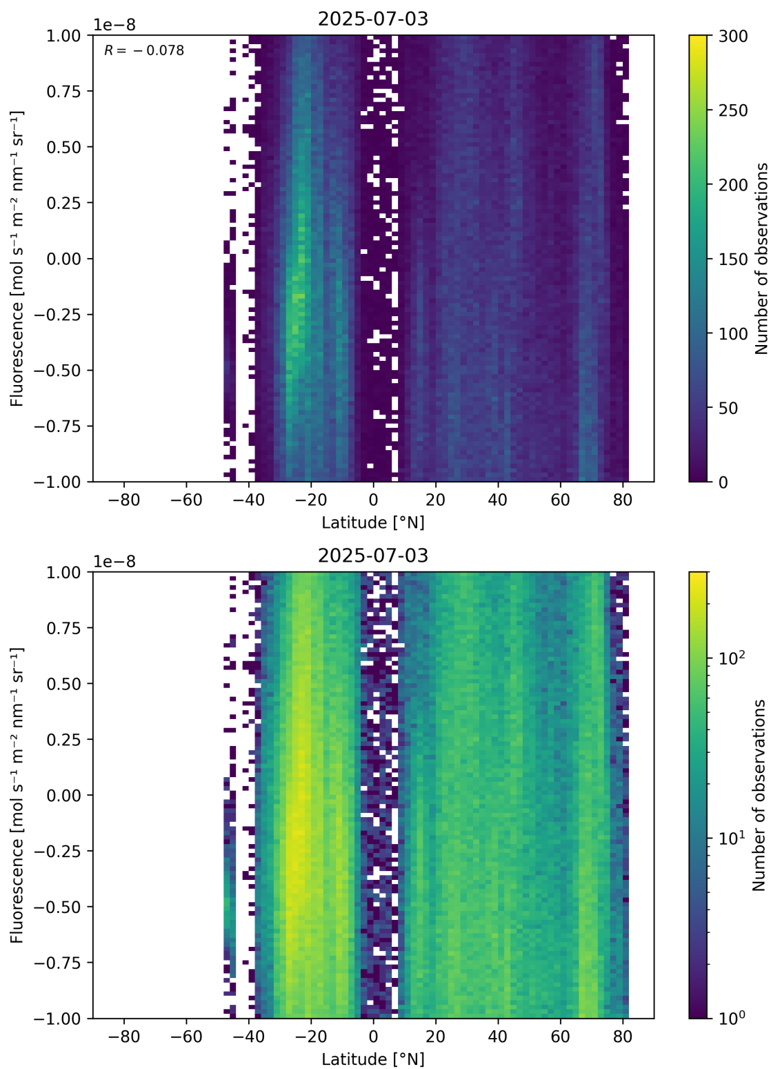
Figure 56: Scatter density plot of “Latitude” against “Fluorescence” for 2025-07-03 to 2025-07-04.
