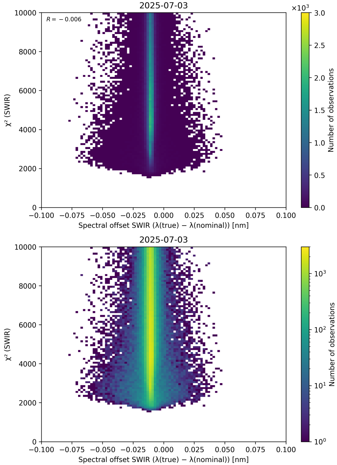
Figure 118: Scatter density plot of “Spectral offset SWIR ( \lambda_{\text{true}} - \lambda_{\text{nominal}} )” against “ \chi^2 (SWIR)” for 2025-07-03 to 2025-07-04.
