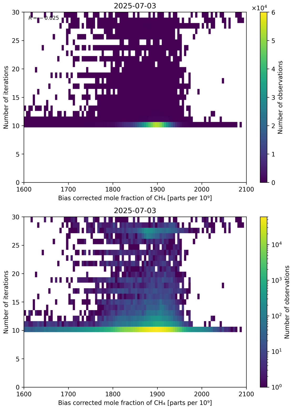
Figure 67: Scatter density plot of “Bias corrected mole fraction of CH 4 ” against “Number of iterations” for 2025-07-03 to 2025-07-04.
