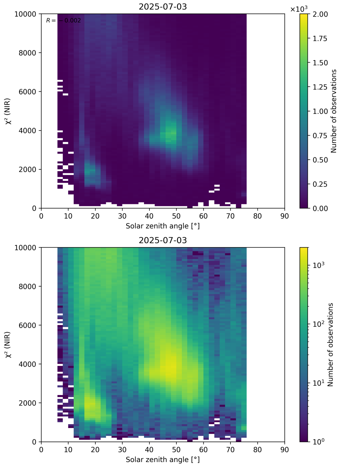
Figure 94: Scatter density plot of “Solar zenith angle” against “ \chi^2 (NIR)” for 2025-07-03 to 2025-07-04.
