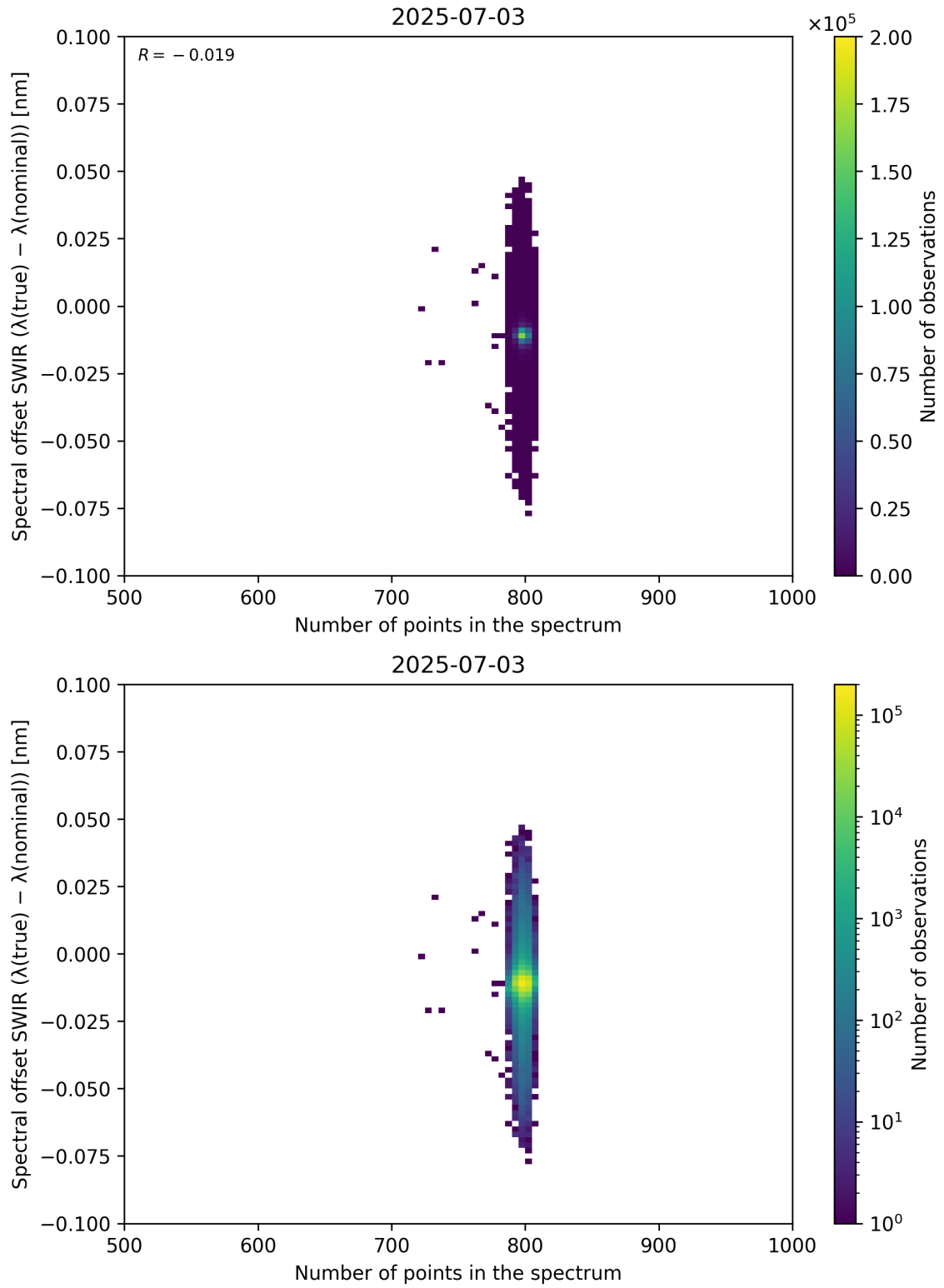
Figure 93: Scatter density plot of “Number of points in the spectrum” against “Spectral offset SWIR ( \lambda_{\text{true}} - \lambda_{\text{nominal}} )” for 2025-07-03 to 2025-07-04.
