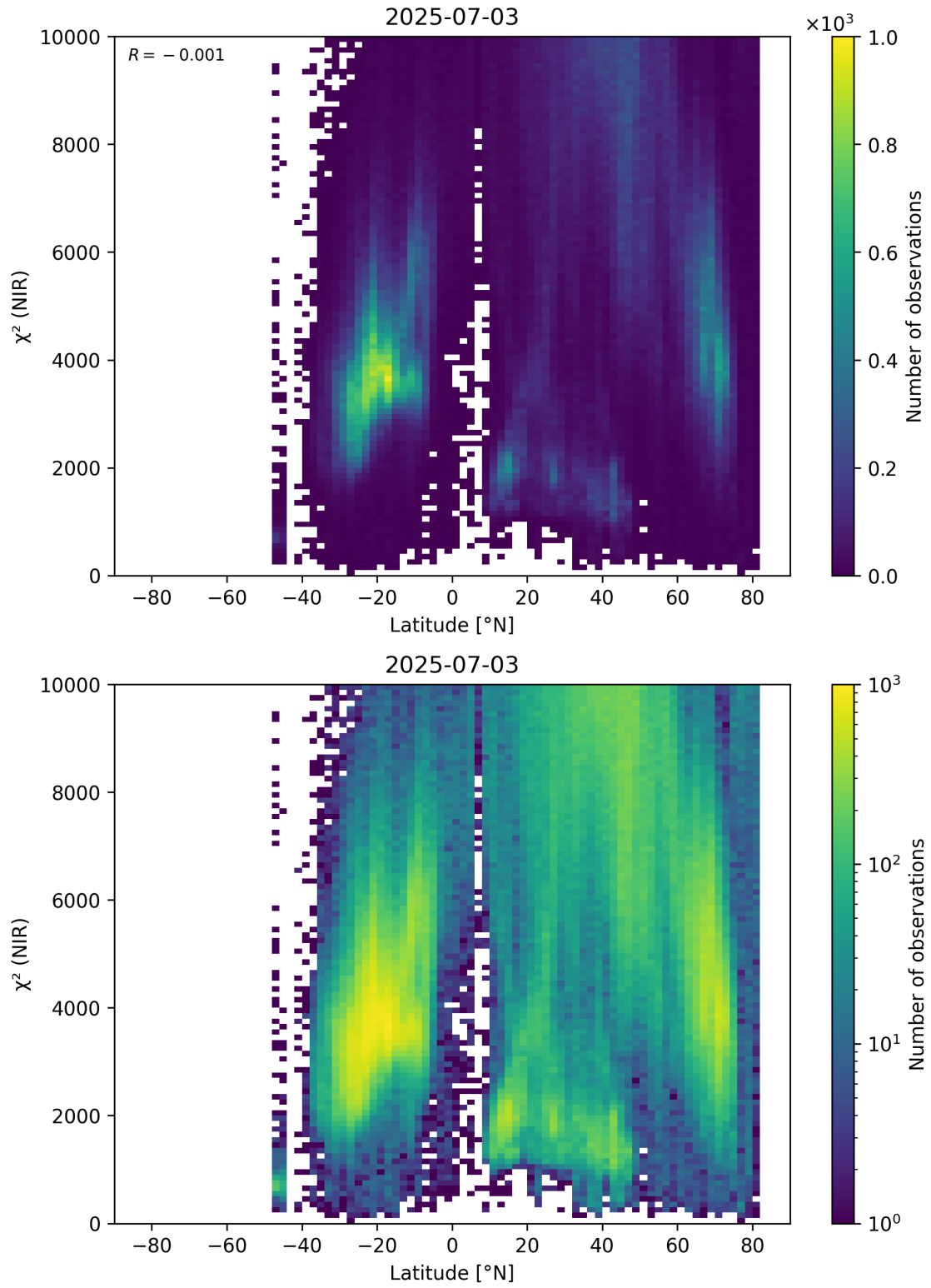
Figure 53: Scatter density plot of “Latitude” against “ \chi^2 (NIR)” for 2025-07-03 to 2025-07-04.
