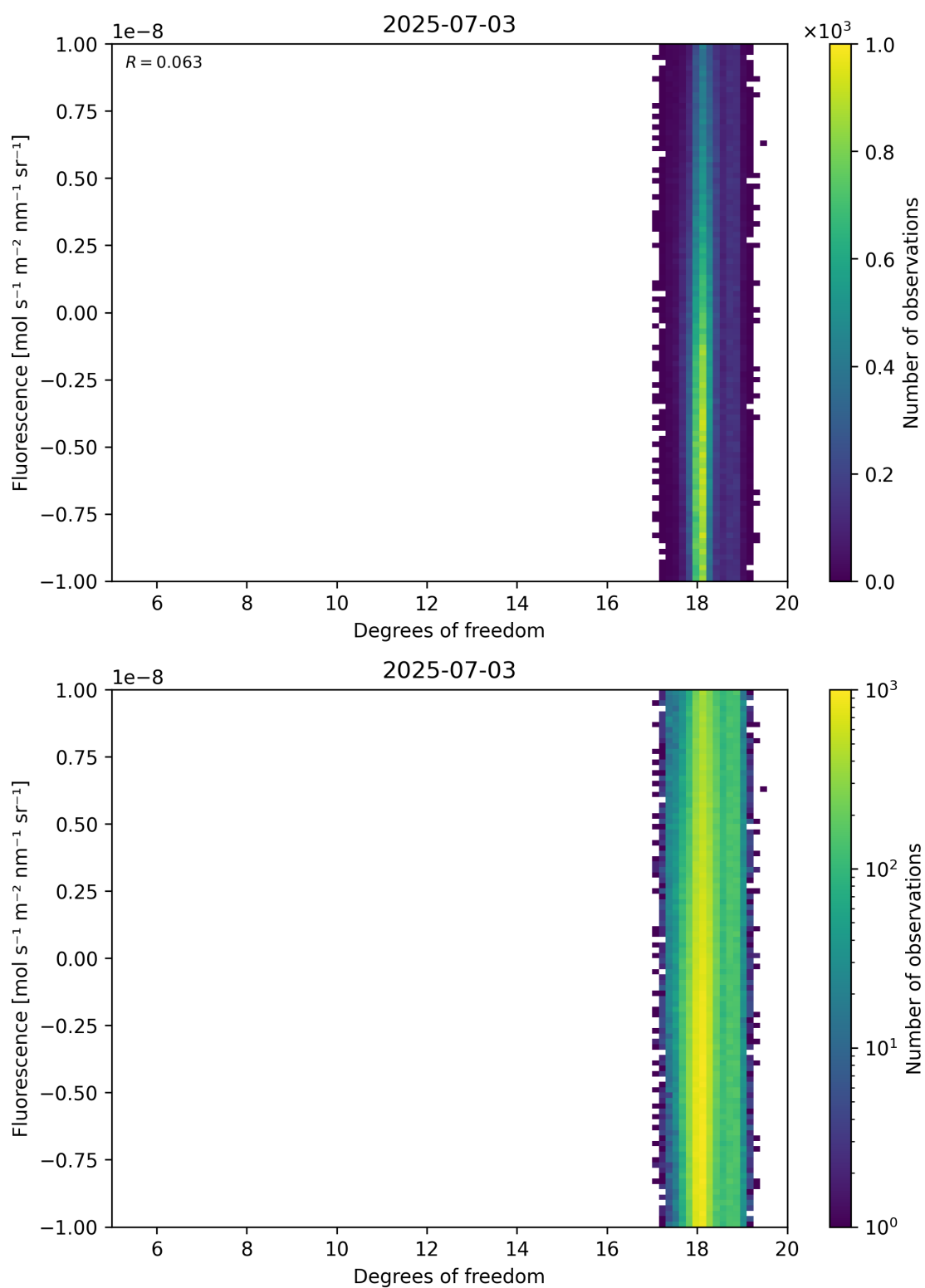
Figure 51: Scatter density plot of “Degrees of freedom” against “Fluorescence” for 2025-07-03 to 2025-07-04.
