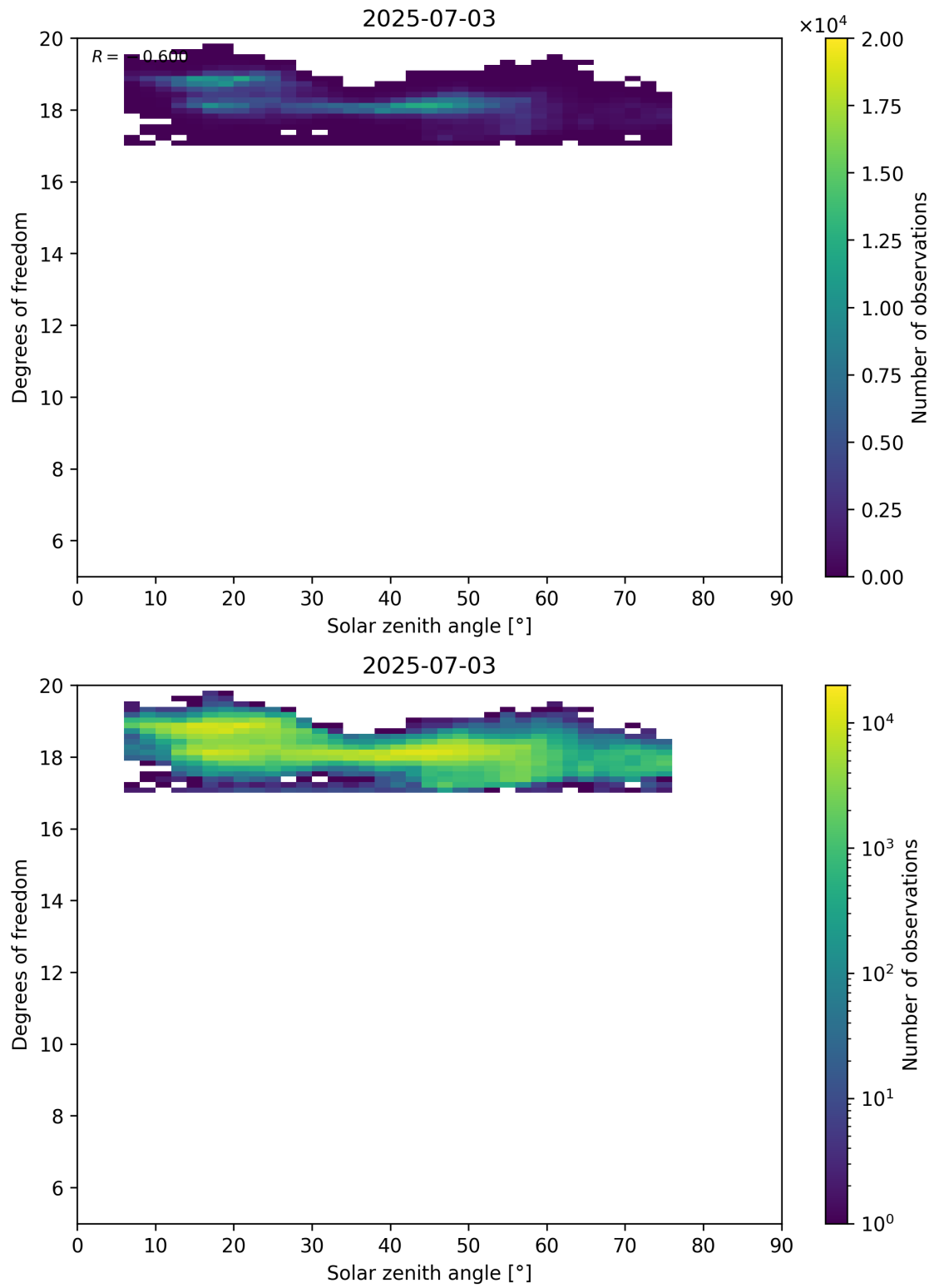
Figure 96: Scatter density plot of “Solar zenith angle” against “Degrees of freedom” for 2025-07-03 to 2025-07-04.
