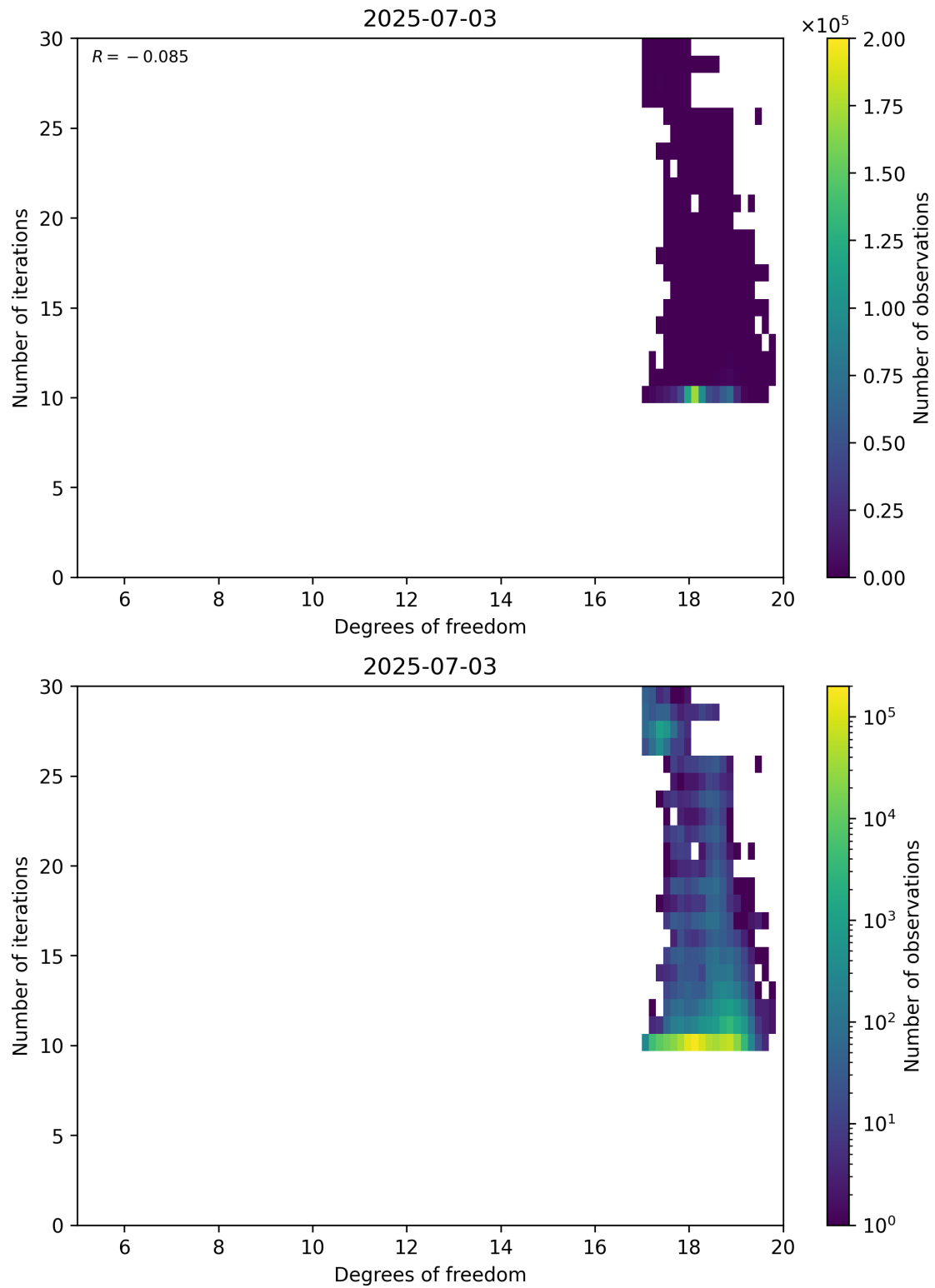
Figure 52: Scatter density plot of “Degrees of freedom” against “Number of iterations” for 2025-07-03 to 2025-07-04.
