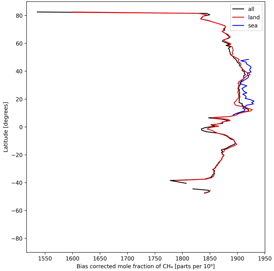
Figure 14: Zonal average of “Bias corrected mole fraction of \text{CH}_4 ” for 2025-07-03 to 2025-07-04.
