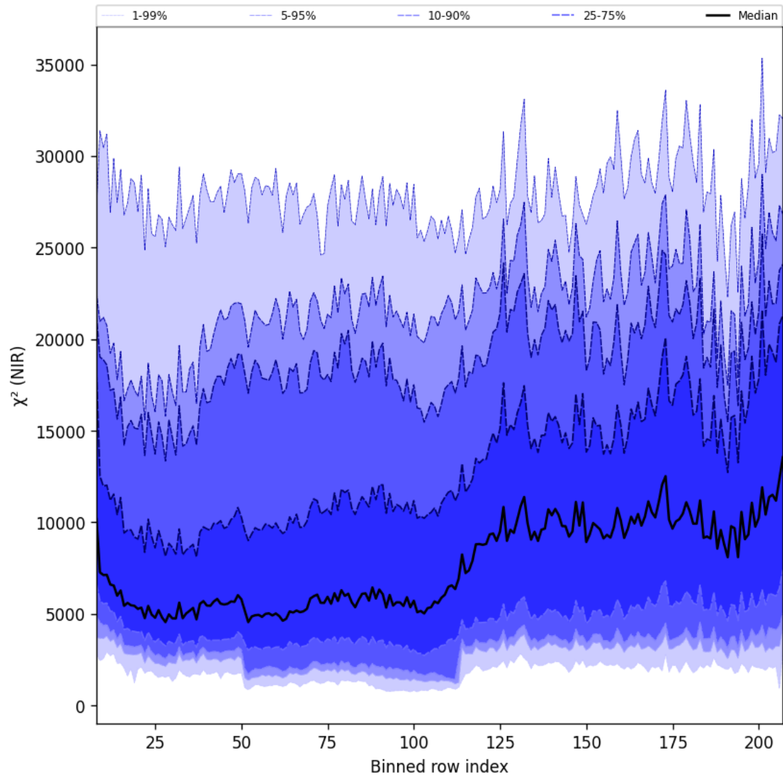
Figure 40: Along track statistics of “ \chi^2 (NIR)” for 2025-07-03 to 2025-07-04
