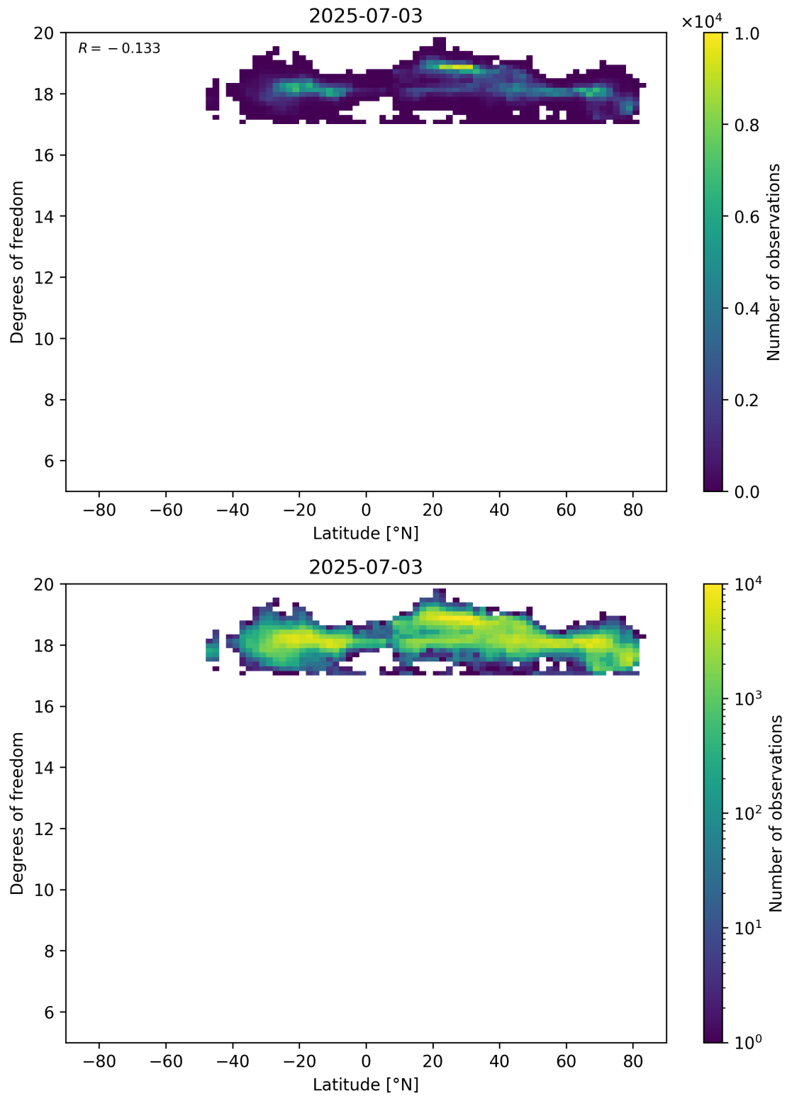
Figure 55: Scatter density plot of “Latitude” against “Degrees of freedom” for 2025-07-03 to 2025-07-04.
