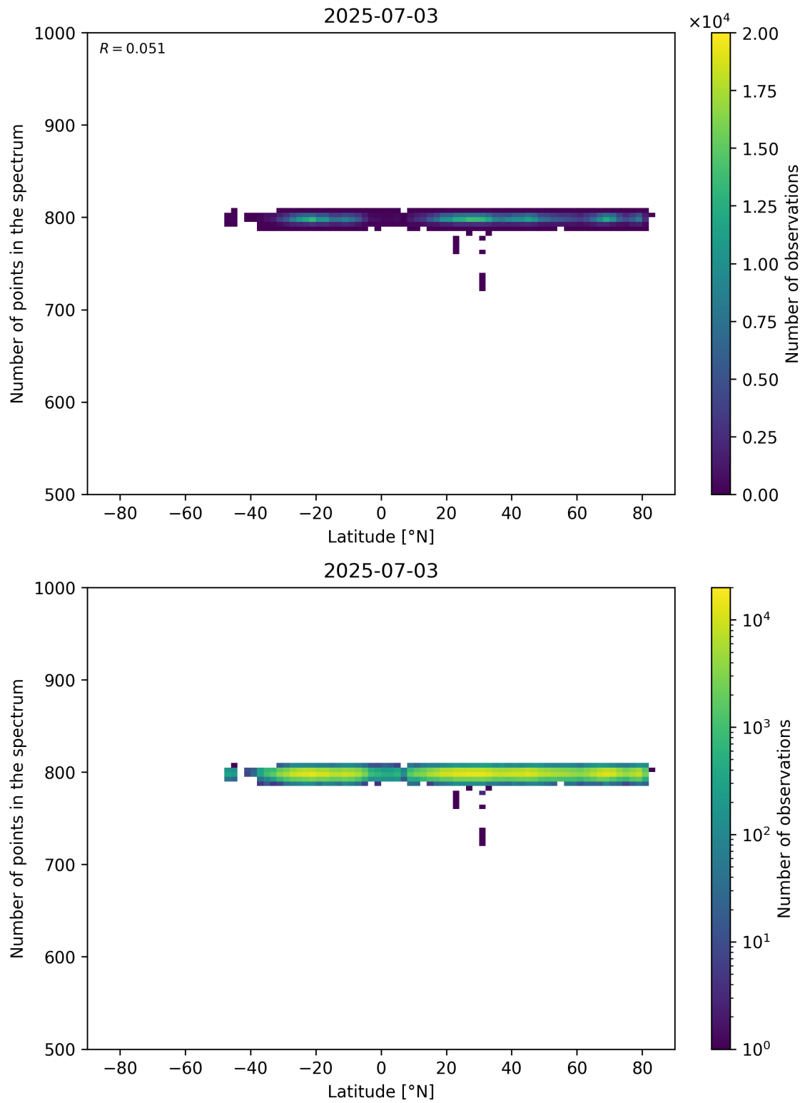
Figure 61: Scatter density plot of “Latitude” against “Number of points in the spectrum” for 2025-07-03 to 2025-07-04.
