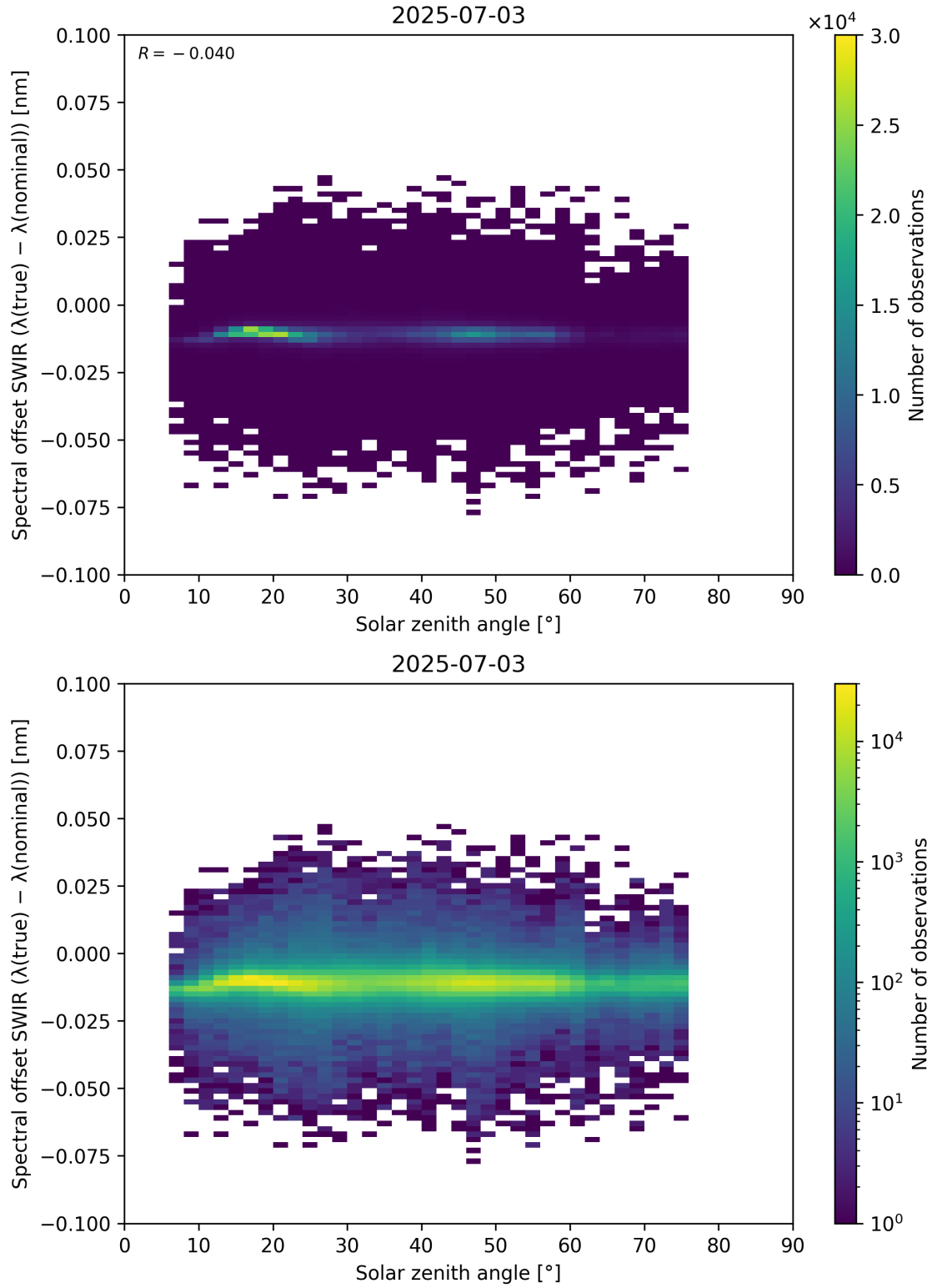
Figure 104: Scatter density plot of “Solar zenith angle” against “Spectral offset SWIR ( \lambda_{\text{true}} - \lambda_{\text{nominal}} )” for 2025-07-03 to 2025-07-04.
