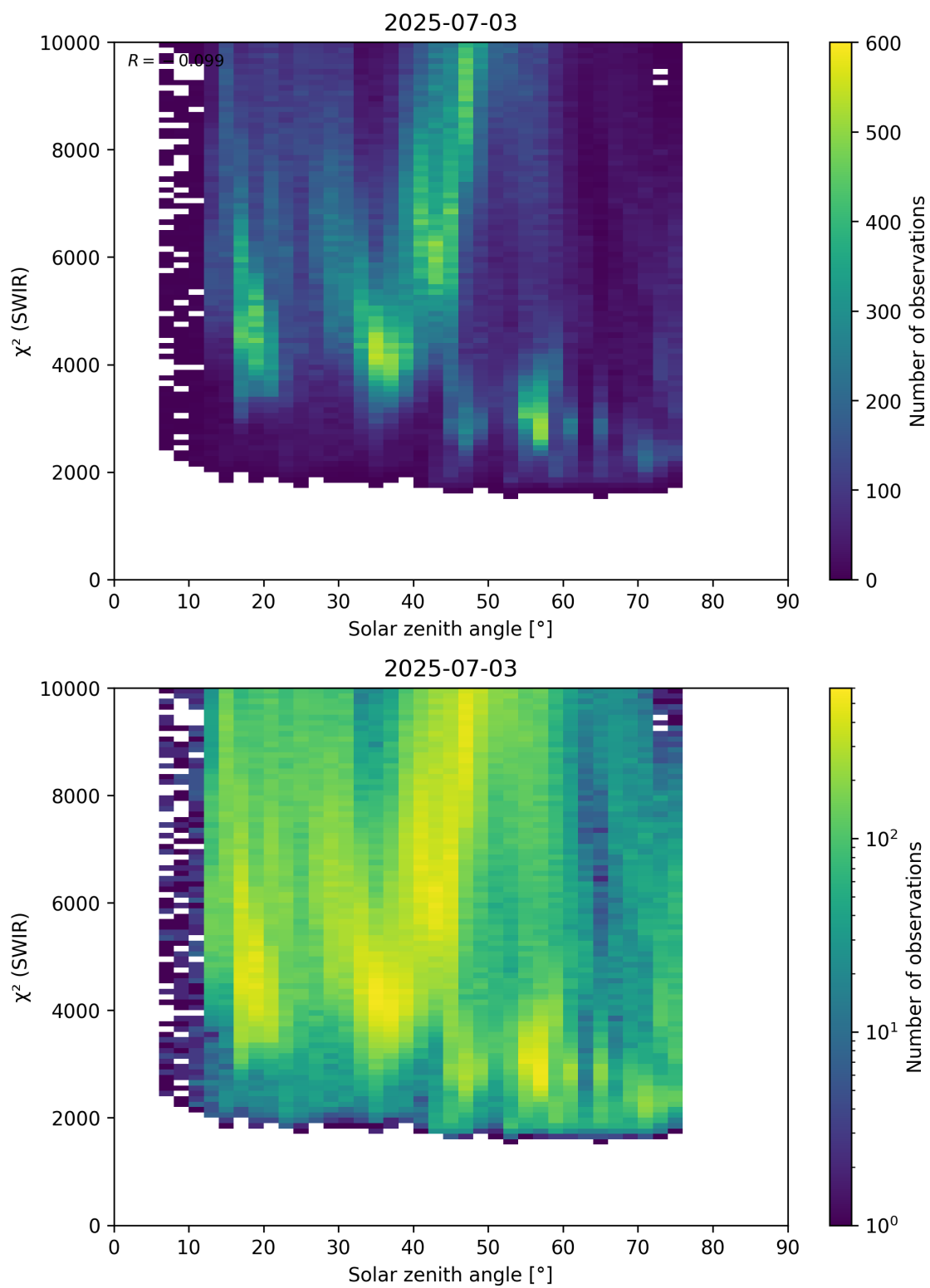
Figure 95: Scatter density plot of “Solar zenith angle” against “ \chi^2 (SWIR)” for 2025-07-03 to 2025-07-04.
