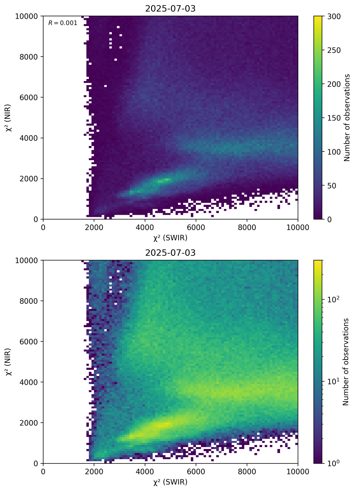
Figure 47: Scatter density plot of “ \chi^2 (SWIR)” against “ \chi^2 (NIR)” for 2025-07-03 to 2025-07-04.
