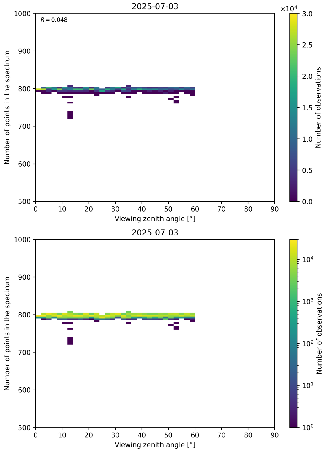
Figure 114: Scatter density plot of “Viewing zenith angle” against “Number of points in the spectrum” for 2025-07-03 to 2025-07-04.
