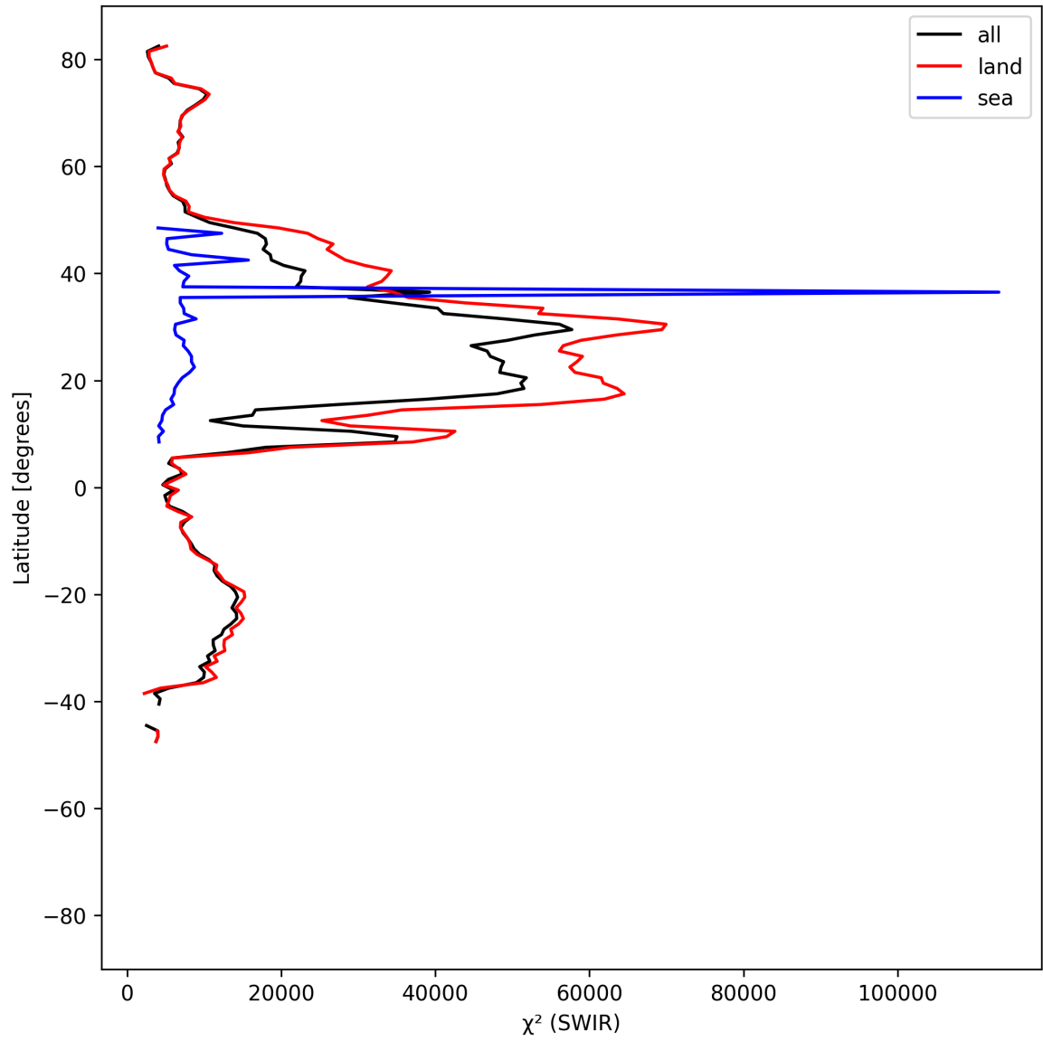
Figure 17: Zonal average of “ \chi^2 (SWIR)” for 2025-07-03 to 2025-07-04.
