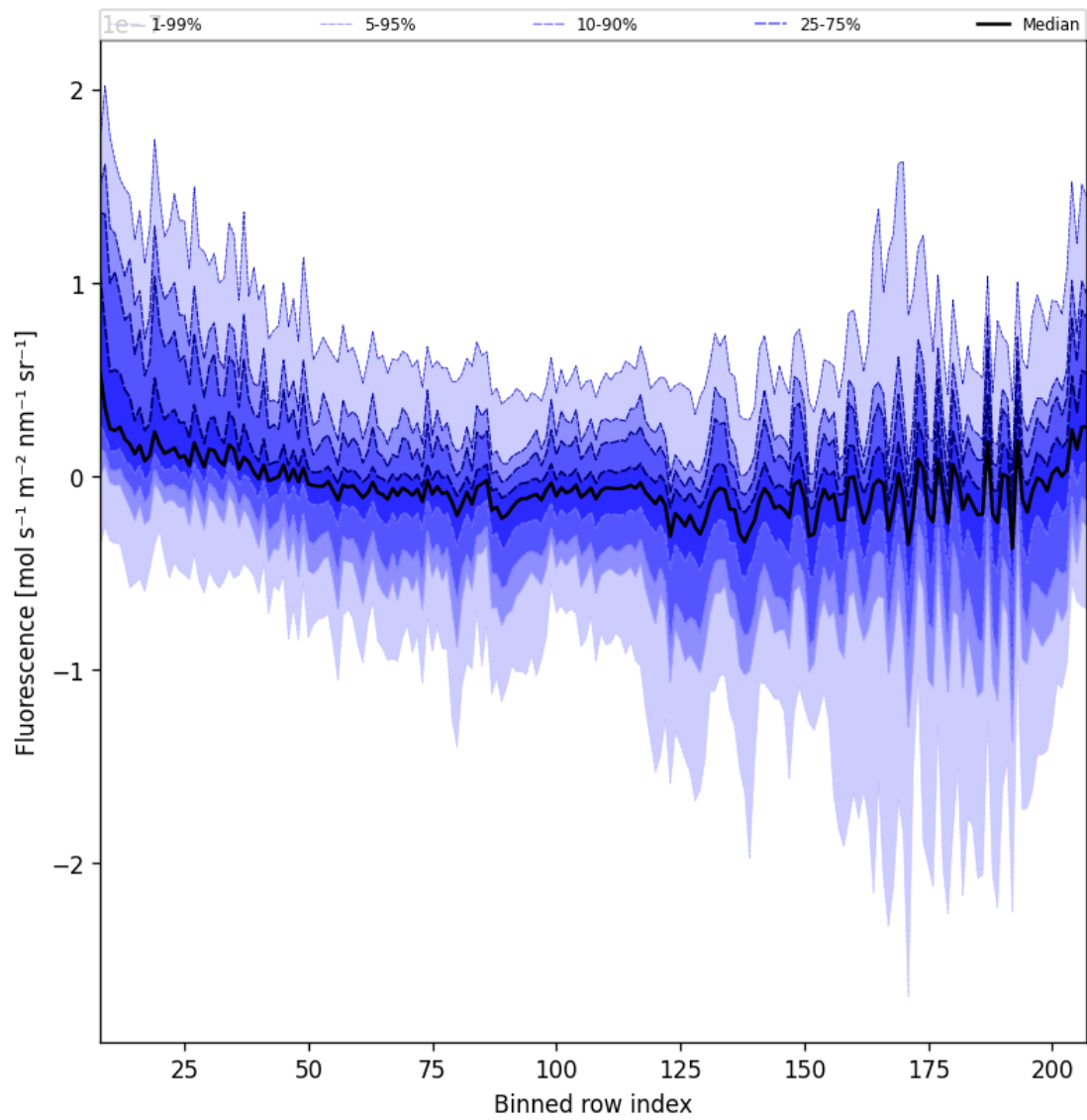
Figure 43: Along track statistics of “Fluorescence” for 2025-07-03 to 2025-07-04
