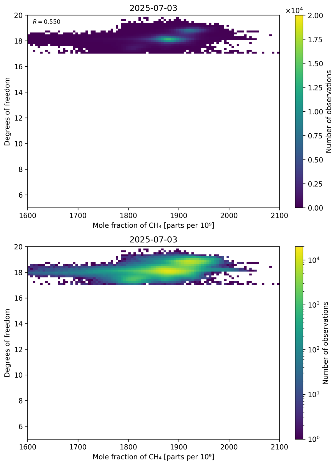
Figure 72: Scatter density plot of “Mole fraction of CH 4 ” against “Degrees of freedom” for 2025-07-03 to 2025-07-04.
