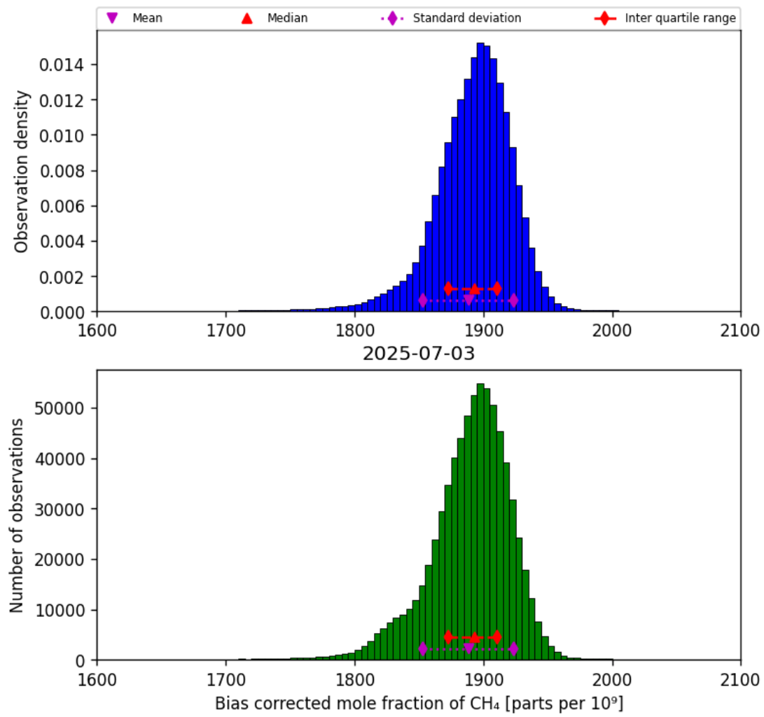
Figure 25: Histogram of “Bias corrected mole fraction of CH 4 ” for 2025-07-03 to 2025-07-04
