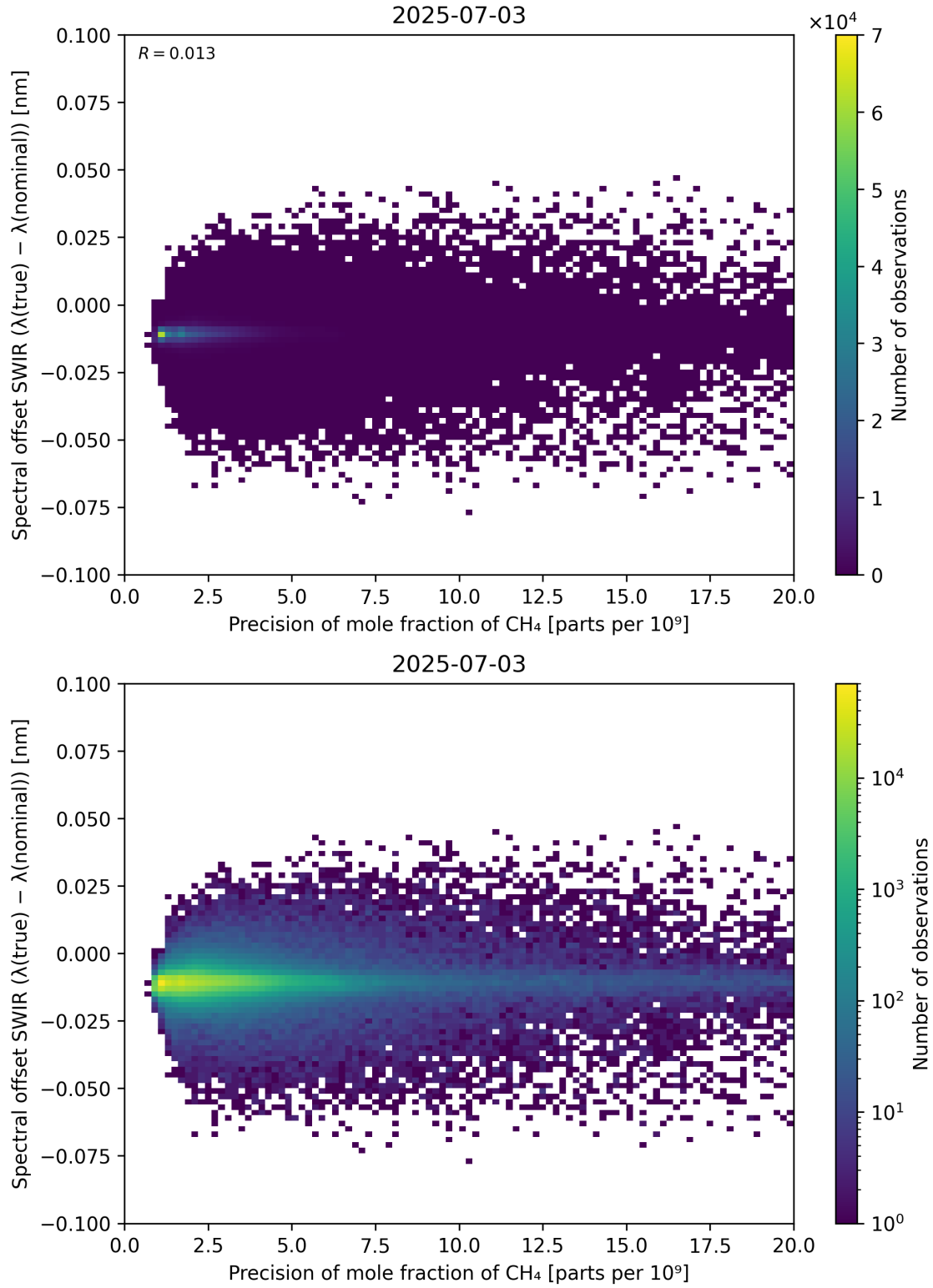
Figure 85: Scatter density plot of “Precision of mole fraction of CH 4 ” against “Spectral offset SWIR ( \lambda_{\text{true}} - \lambda_{\text{nominal}} )” for 2025-07-03 to 2025-07-04.
