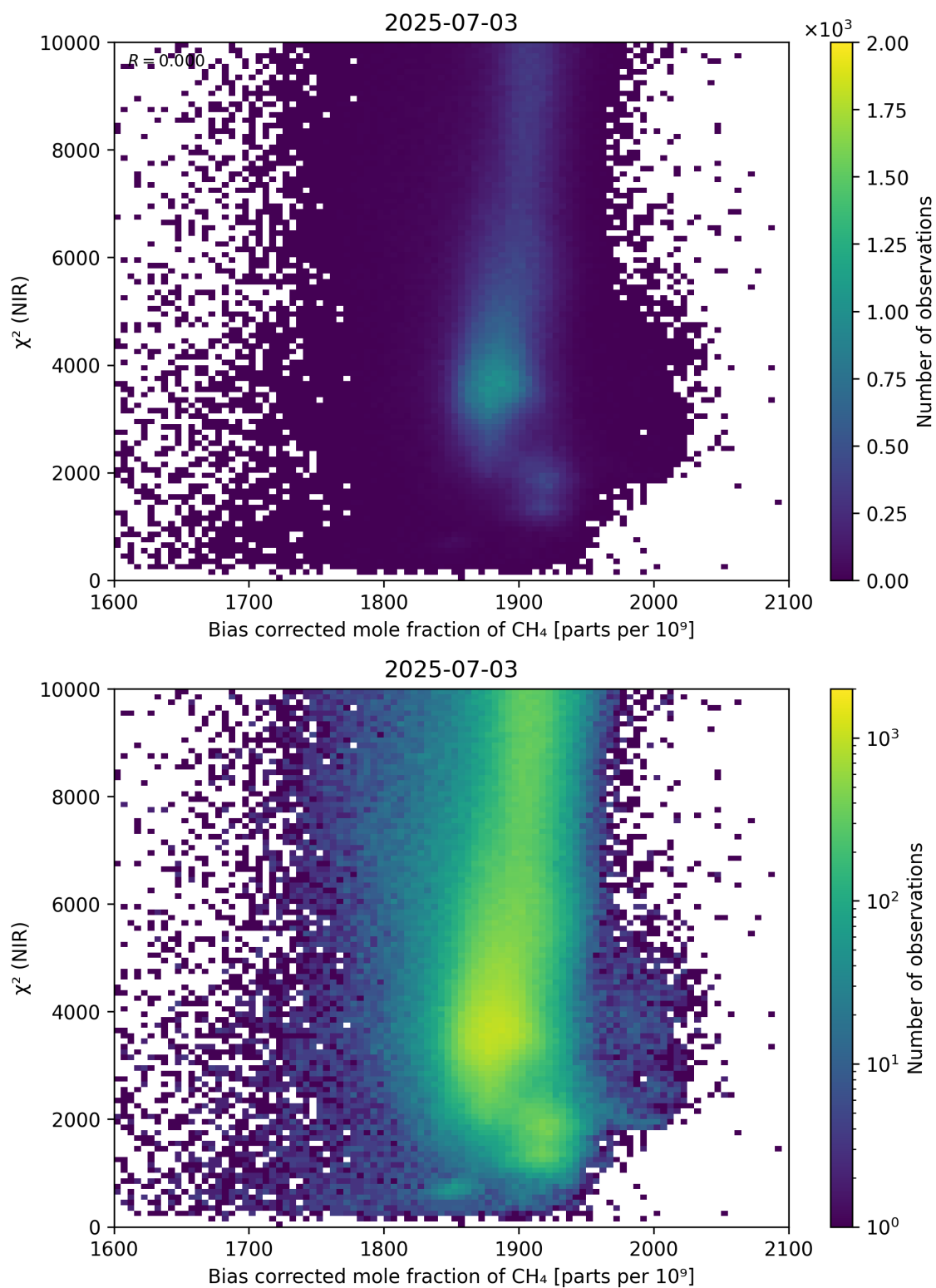
Figure 63: Scatter density plot of “Bias corrected mole fraction of \text{CH}_4 ” against “ \chi^2 (NIR)” for 2025-07-03 to 2025-07-04.
