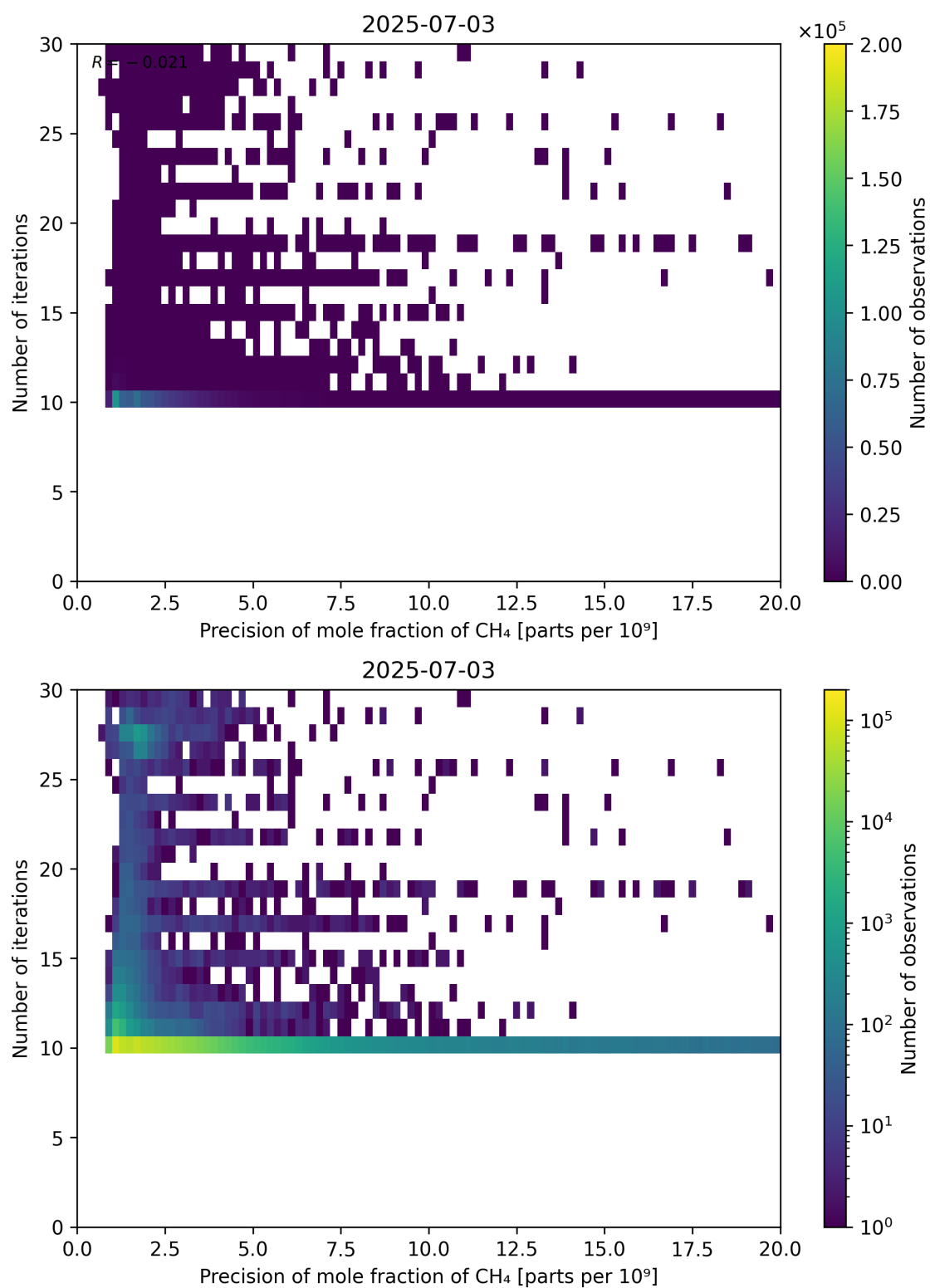
Figure 83: Scatter density plot of “Precision of mole fraction of CH 4 ” against “Number of iterations” for 2025-07-03 to 2025-07-04.
