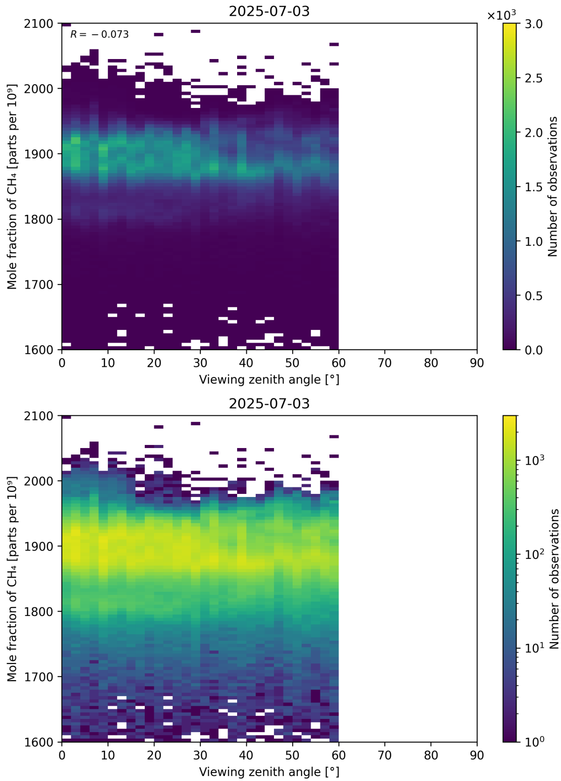
Figure 110: Scatter density plot of “Viewing zenith angle” against “Mole fraction of CH 4 ” for 2025-07-03 to 2025-07-04.
