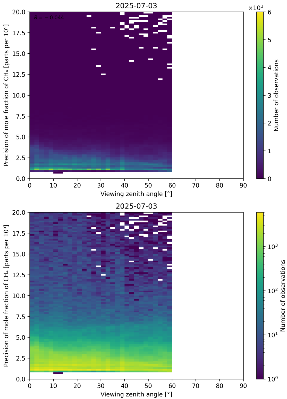
Figure 112: Scatter density plot of “Viewing zenith angle” against “Precision of mole fraction of CH 4 ” for 2025-07-03 to 2025-07-04.
