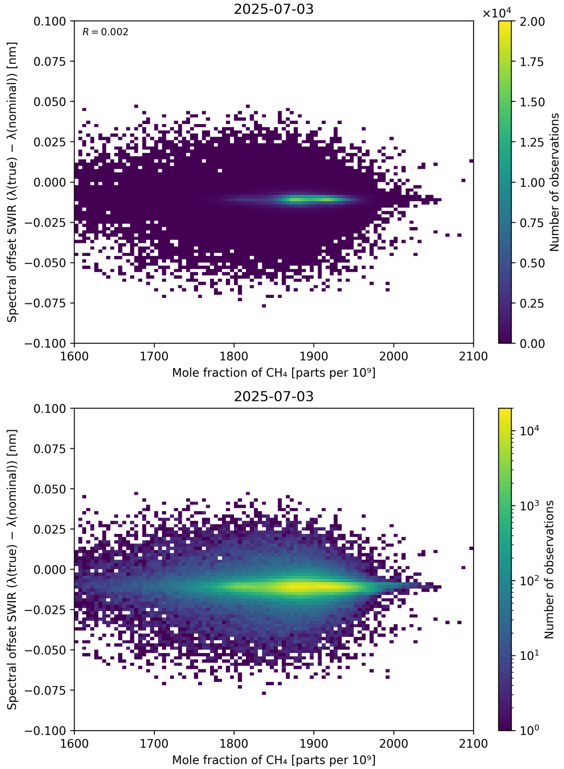
Figure 86: Scatter density plot of “Mole fraction of CH 4 ” against “Spectral offset SWIR ( \lambda_{\text{true}} - \lambda_{\text{nominal}} )” for 2025-07-03 to 2025-07-04.
