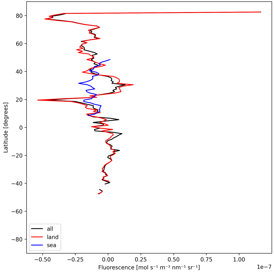
Figure 21: Zonal average of “Fluorescence” for 2025-07-03 to 2025-07-04.
