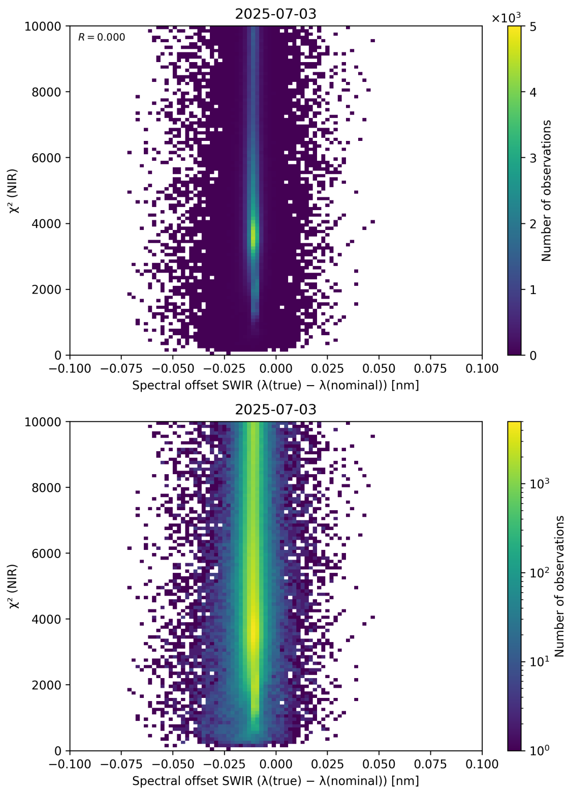
Figure 117: Scatter density plot of “Spectral offset SWIR ( \lambda_{\text{true}} - \lambda_{\text{nominal}} )” against “ \chi^2 (NIR)” for 2025-07-03 to 2025-07-04.
