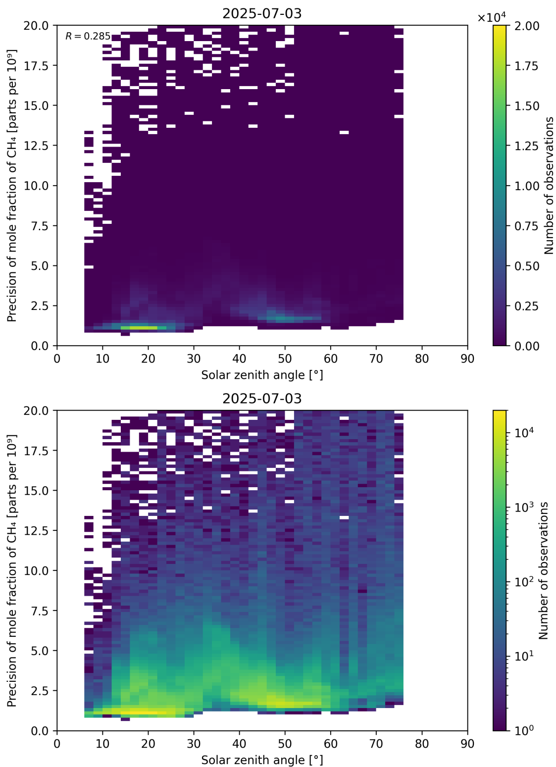
Figure 101: Scatter density plot of “Solar zenith angle” against “Precision of mole fraction of CH 4 ” for 2025-07-03 to 2025-07-04.
