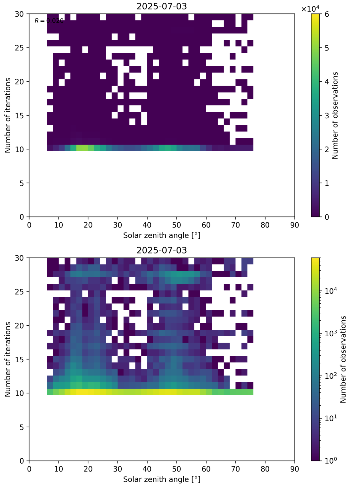
Figure 102: Scatter density plot of “Solar zenith angle” against “Number of iterations” for 2025-07-03 to 2025-07-04.
