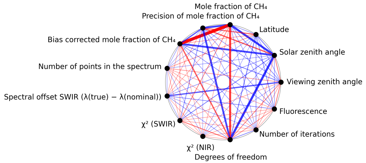
Figure 1: Map of correlation graph for 2025-07-03 to 2025-07-04.
