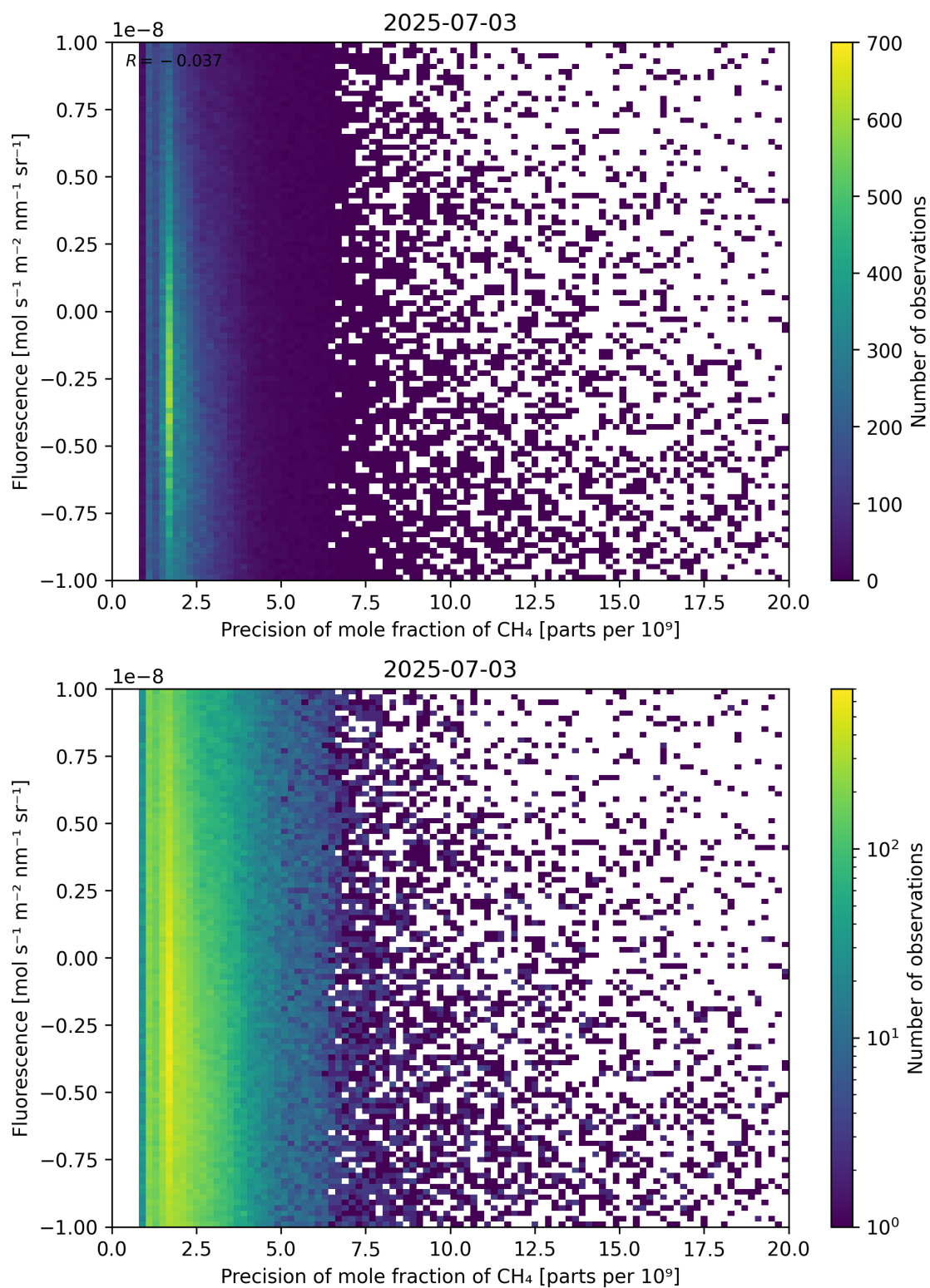
Figure 81: Scatter density plot of “Precision of mole fraction of CH 4 ” against “Fluorescence” for 2025-07-03 to 2025-07-04.
