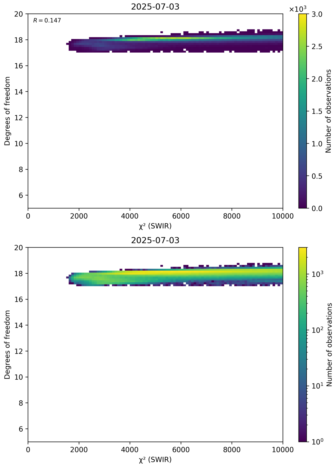
Figure 48: Scatter density plot of “ \chi^2 (SWIR)” against “Degrees of freedom” for 2025-07-03 to 2025-07-04.
