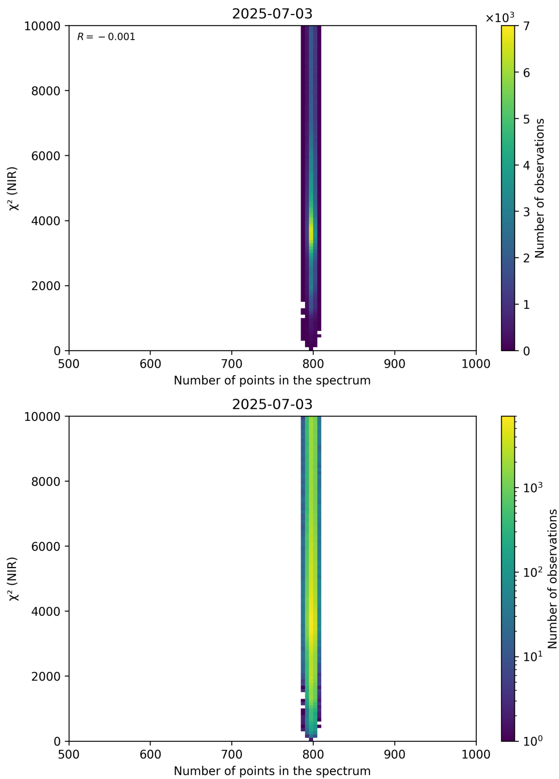
Figure 88: Scatter density plot of “Number of points in the spectrum” against “ \chi^2 (NIR)” for 2025-07-03 to 2025-07-04.
