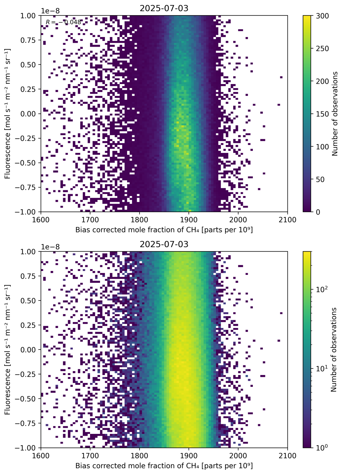
Figure 66: Scatter density plot of “Bias corrected mole fraction of \text{CH}_4 ” against “Fluorescence” for 2025-07-03 to 2025-07-04.
