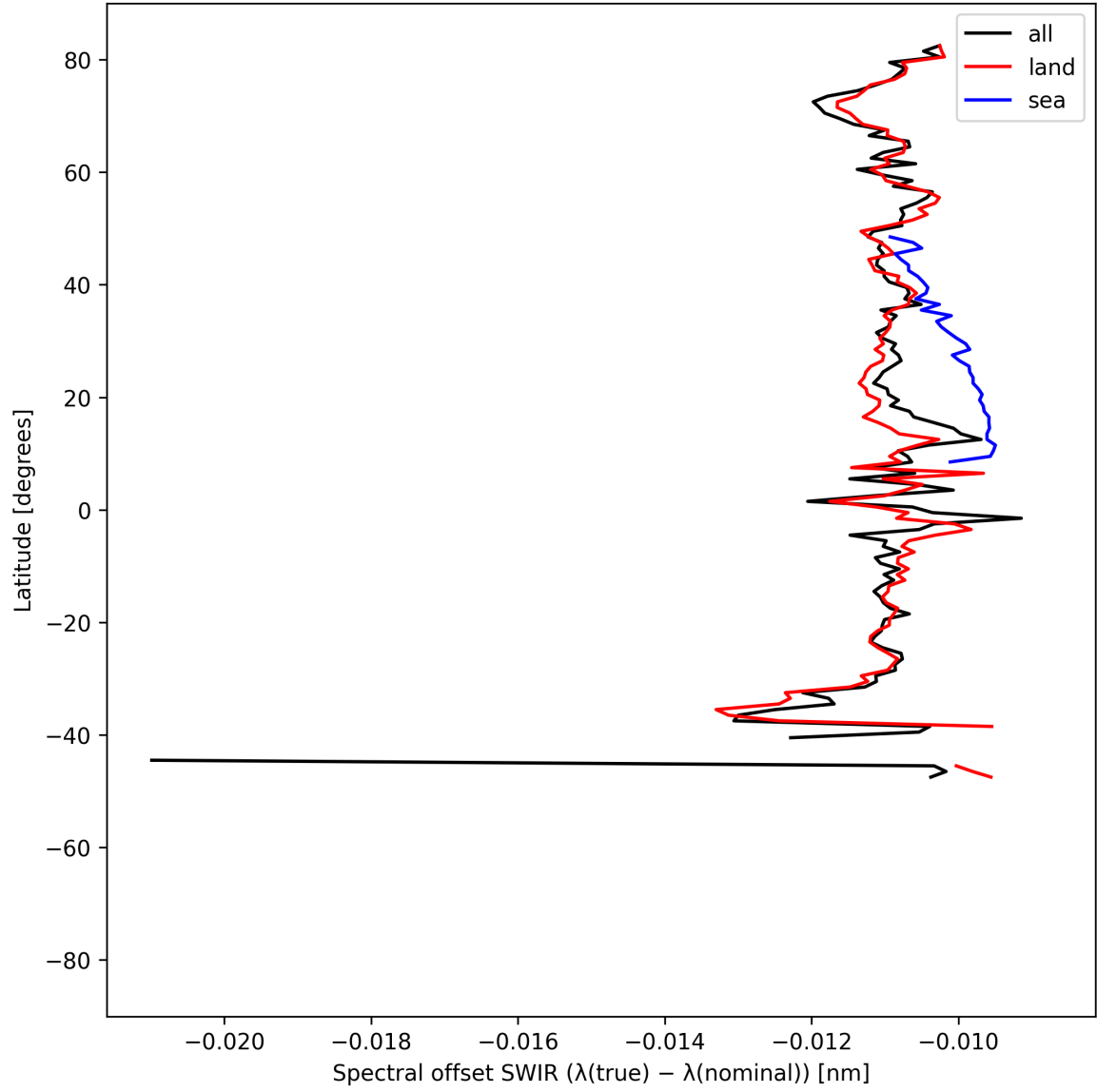
Figure 16: Zonal average of “Spectral offset SWIR ( \lambda_{\text{true}} - \lambda_{\text{nominal}} )” for 2025-07-03 to 2025-07-04.
