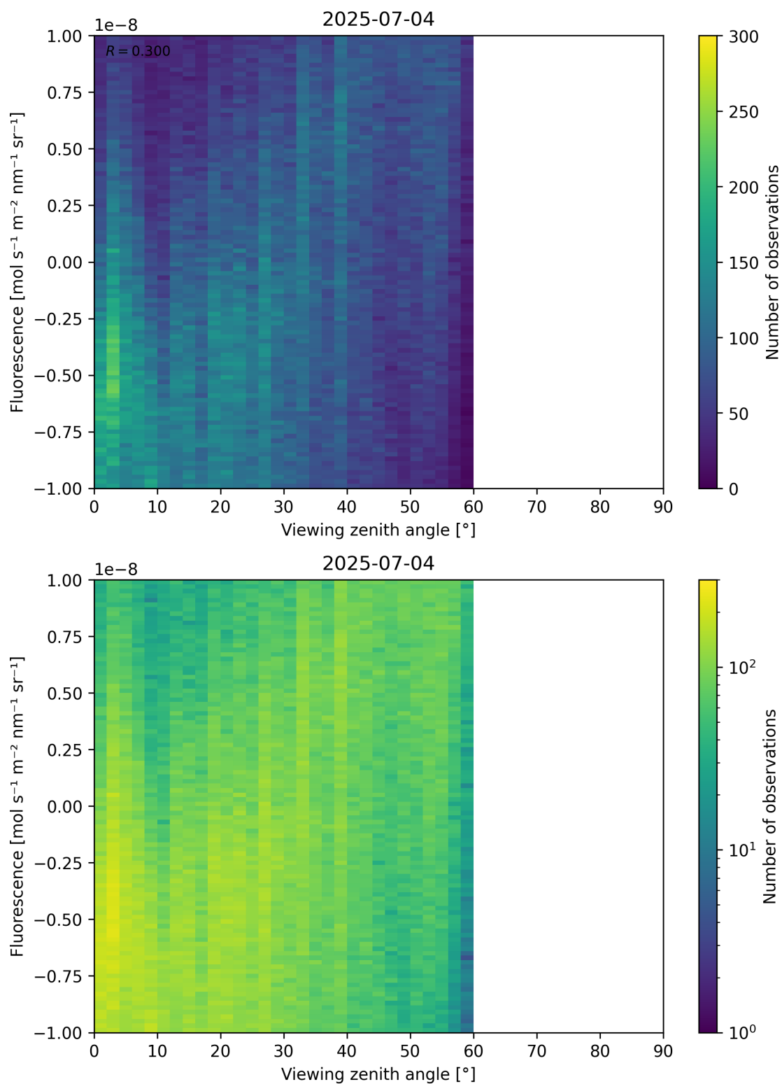
Figure 108: Scatter density plot of “Viewing zenith angle” against “Fluorescence” for 2025-07-03 to 2025-07-05.
