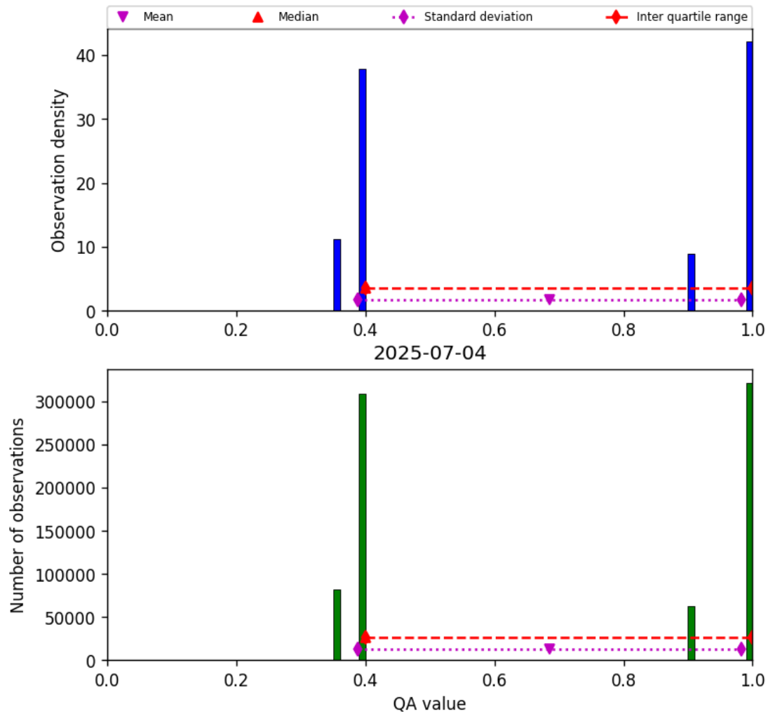
Figure 22: Histogram of “QA value” for 2025-07-03 to 2025-07-05
