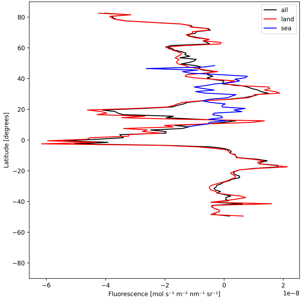
Figure 21: Zonal average of “Fluorescence” for 2025-07-03 to 2025-07-05.
