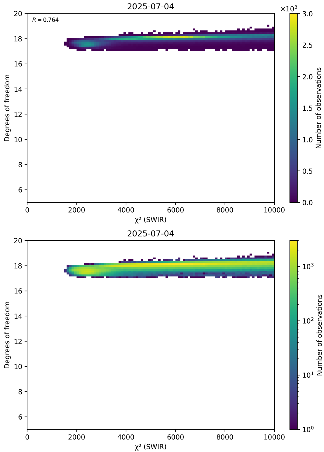
Figure 48: Scatter density plot of “ \chi^2 (SWIR)” against “Degrees of freedom” for 2025-07-03 to 2025-07-05.
