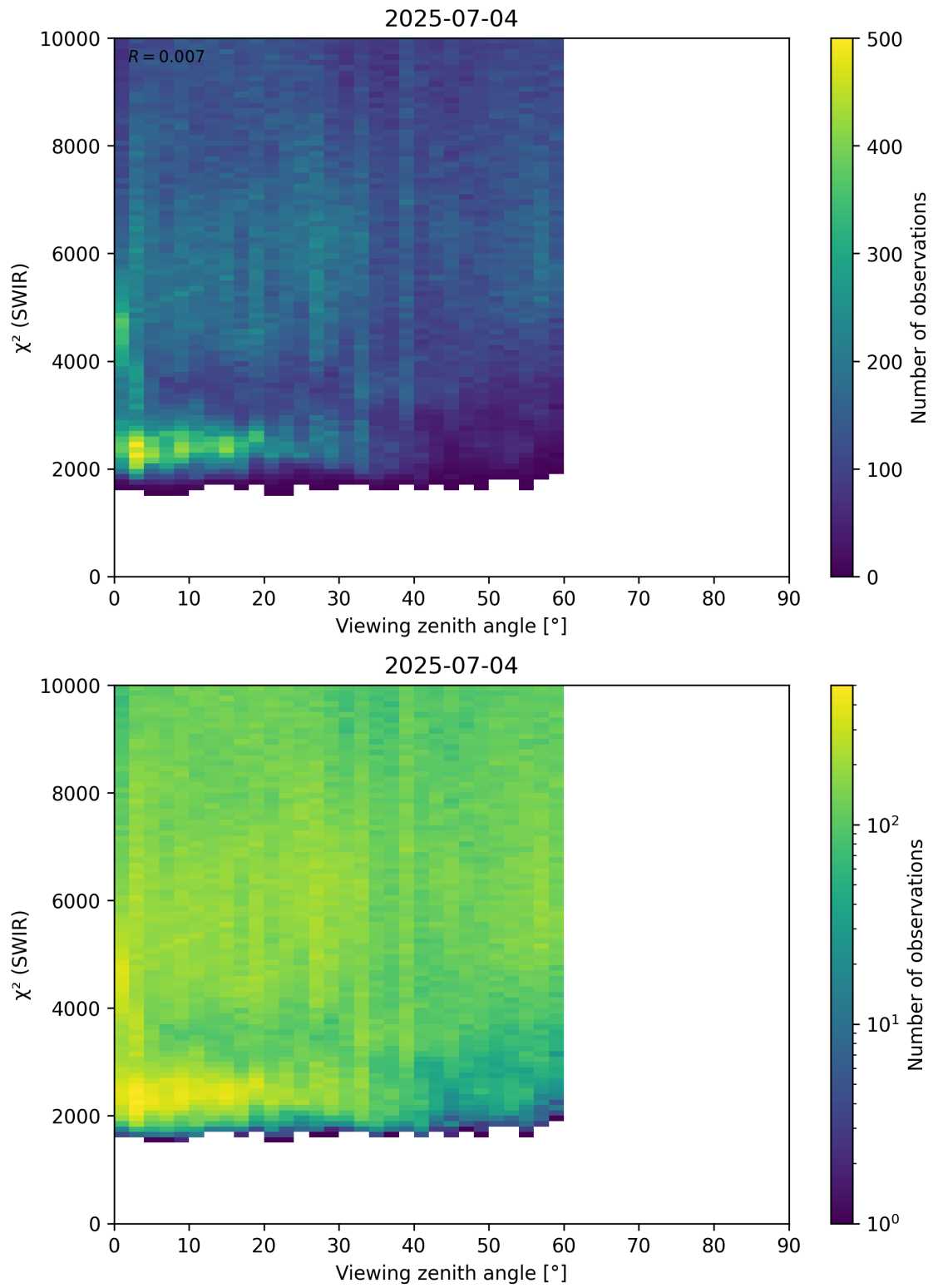
Figure 106: Scatter density plot of “Viewing zenith angle” against “ \chi^2 (SWIR)” for 2025-07-03 to 2025-07-05.
