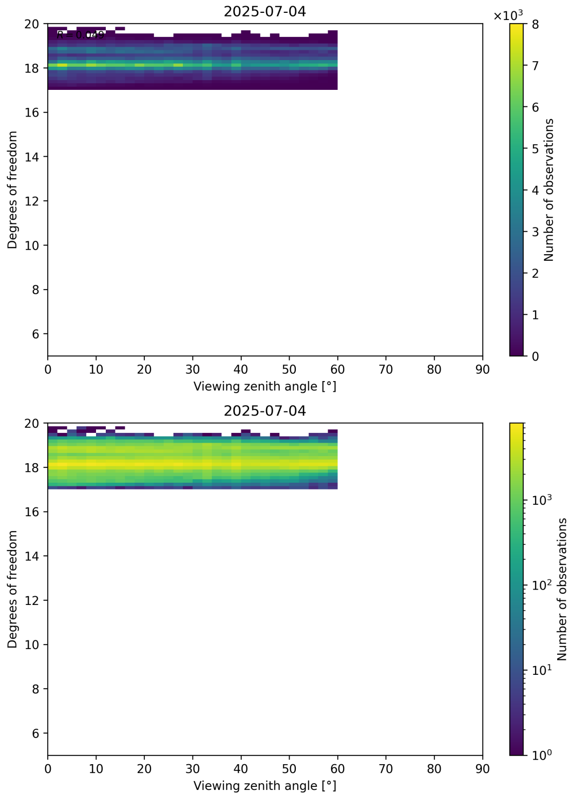
Figure 107: Scatter density plot of “Viewing zenith angle” against “Degrees of freedom” for 2025-07-03 to 2025-07-05.
