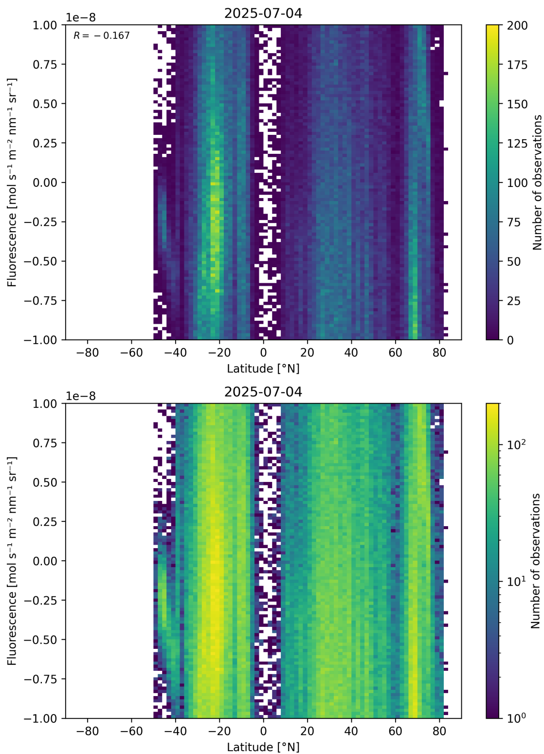
Figure 56: Scatter density plot of “Latitude” against “Fluorescence” for 2025-07-03 to 2025-07-05.
