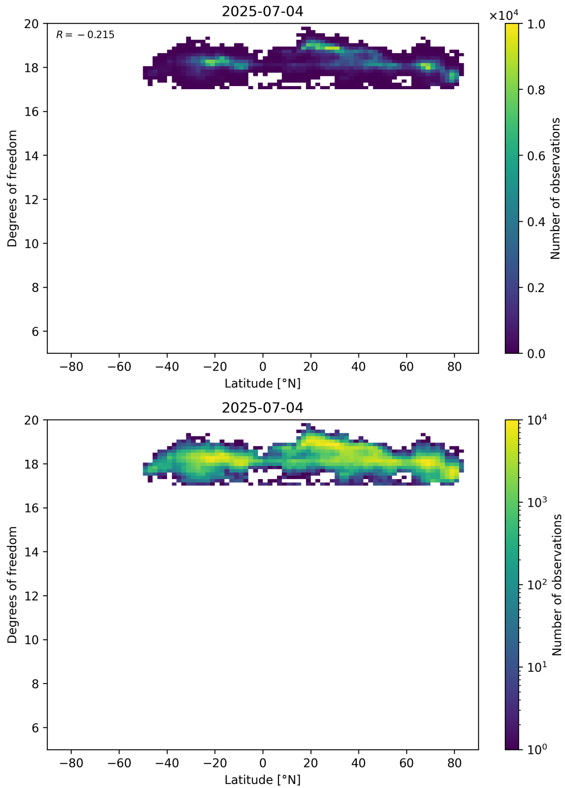
Figure 55: Scatter density plot of “Latitude” against “Degrees of freedom” for 2025-07-03 to 2025-07-05.
