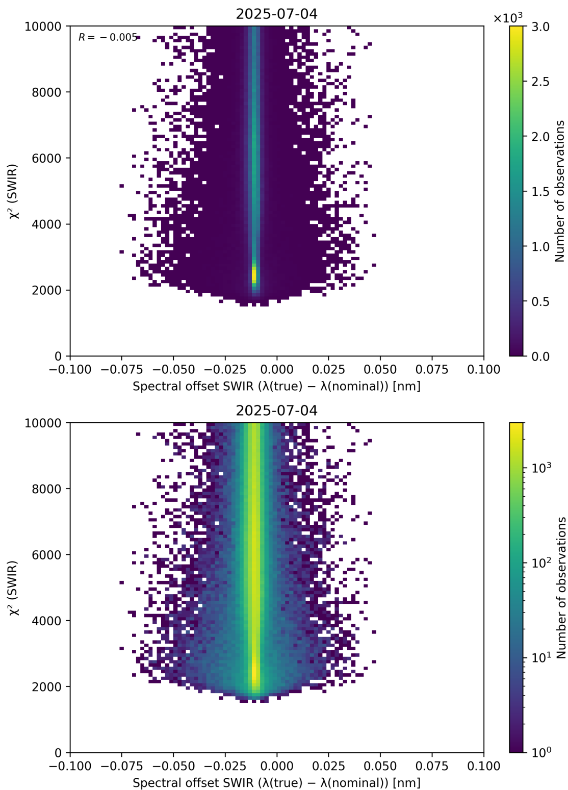
Figure 118: Scatter density plot of “Spectral offset SWIR ( \lambda_{\text{true}} - \lambda_{\text{nominal}} )” against “ \chi^2 (SWIR)” for 2025-07-03 to 2025-07-05.
