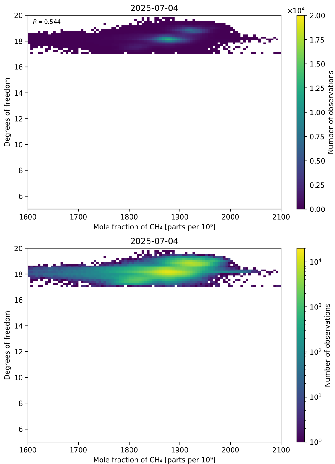
Figure 72: Scatter density plot of “Mole fraction of CH 4 ” against “Degrees of freedom” for 2025-07-03 to 2025-07-05.
