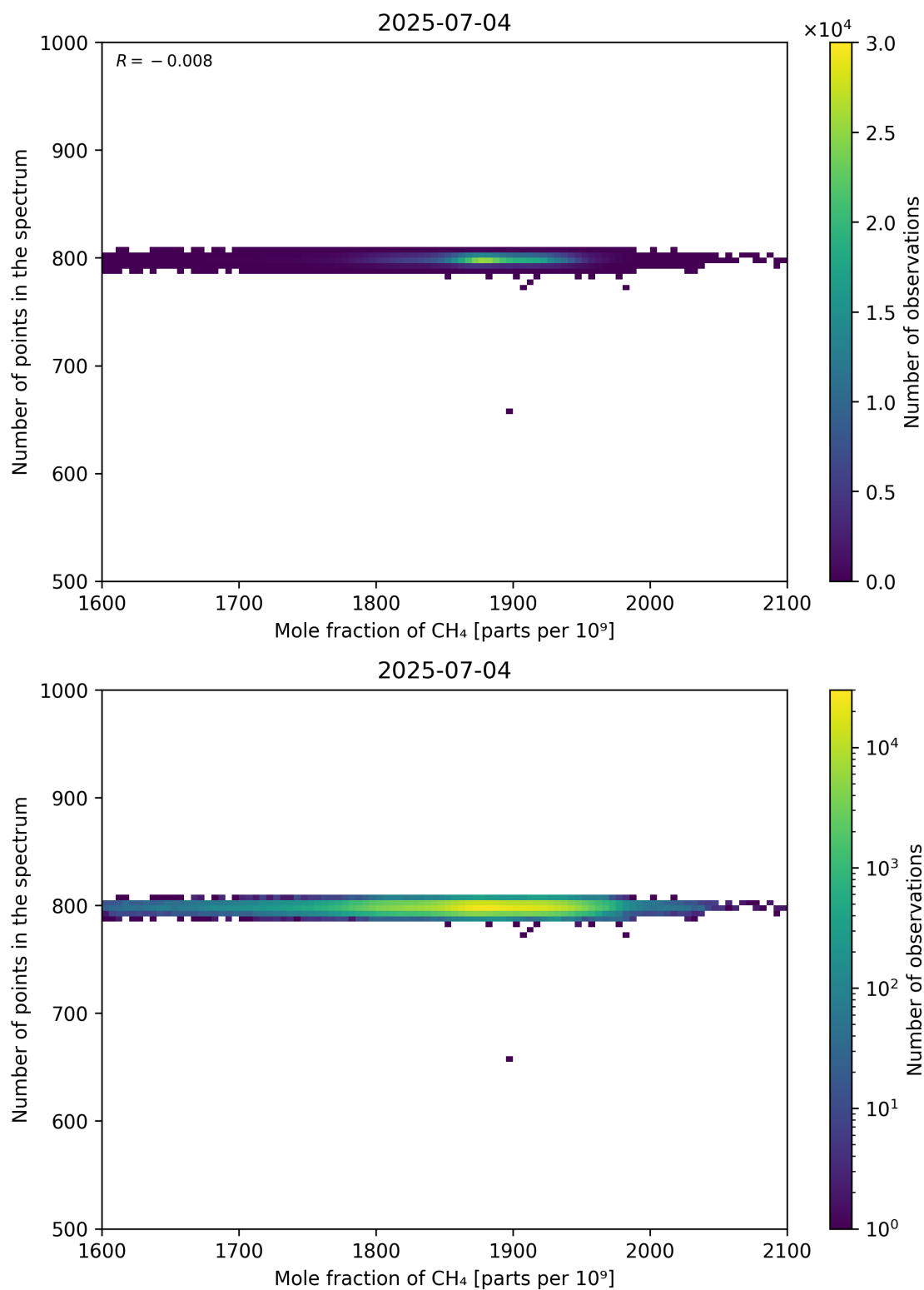
Figure 77: Scatter density plot of “Mole fraction of CH 4 ” against “Number of points in the spectrum” for 2025-07-03 to 2025-07-05.
