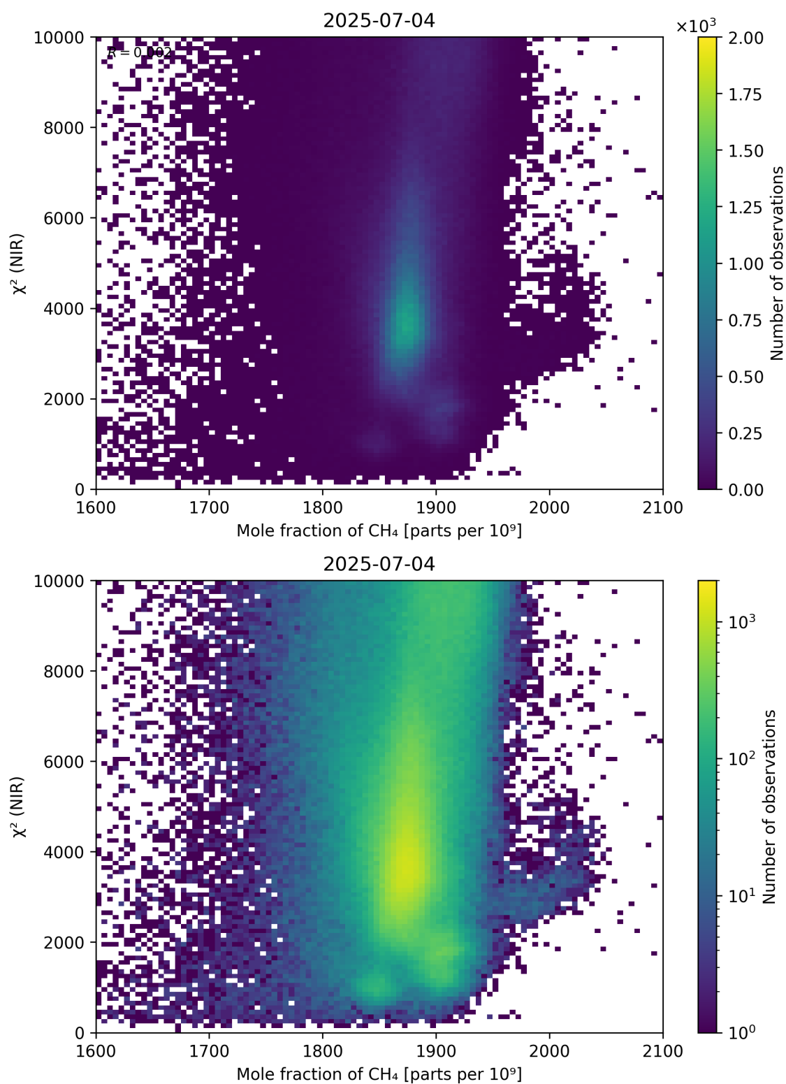
Figure 70: Scatter density plot of “Mole fraction of CH 4 ” against “ \chi^2 (NIR)” for 2025-07-03 to 2025-07-05.
