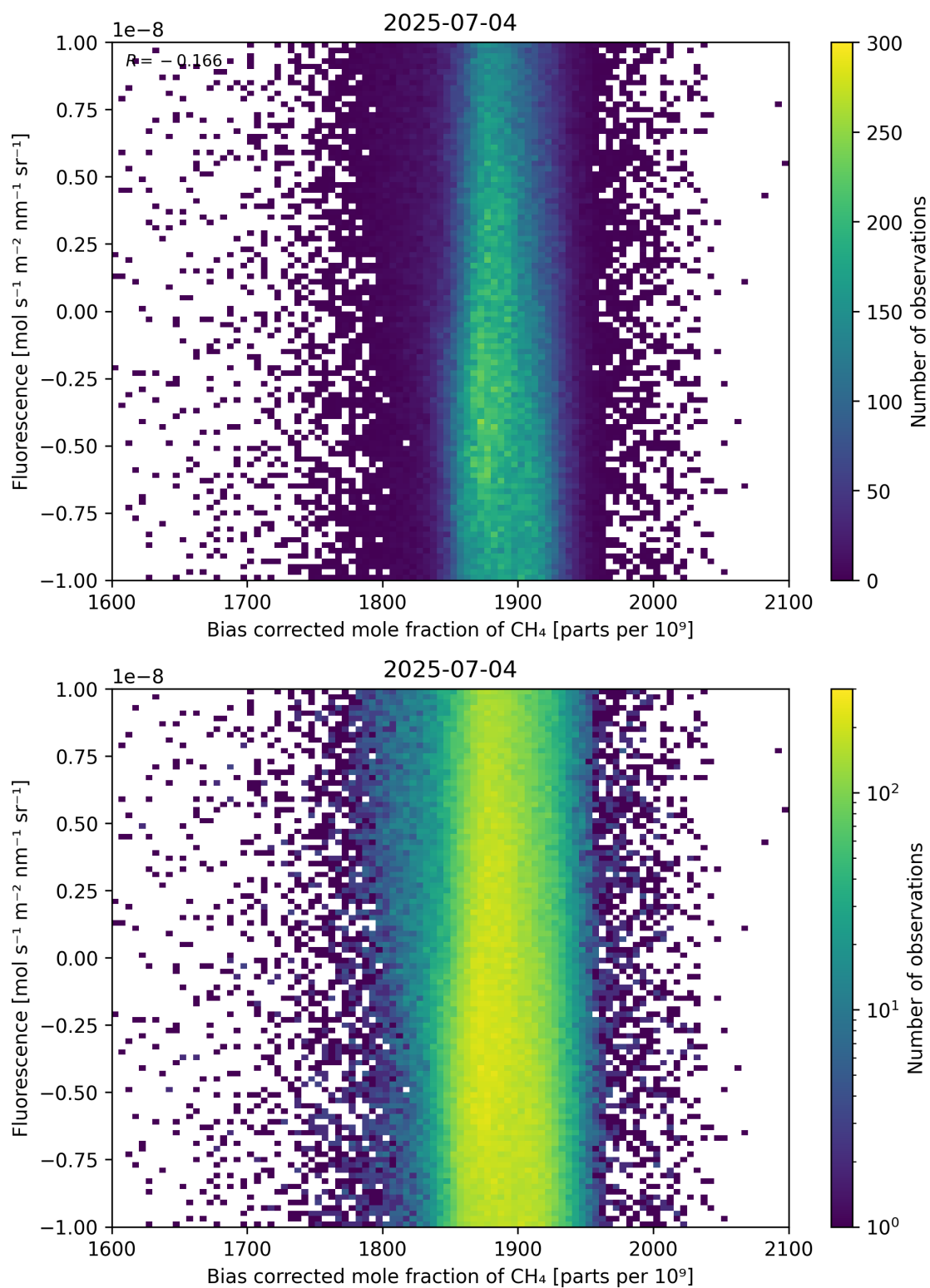
Figure 66: Scatter density plot of “Bias corrected mole fraction of \text{CH}_4 ” against “Fluorescence” for 2025-07-03 to 2025-07-05.
