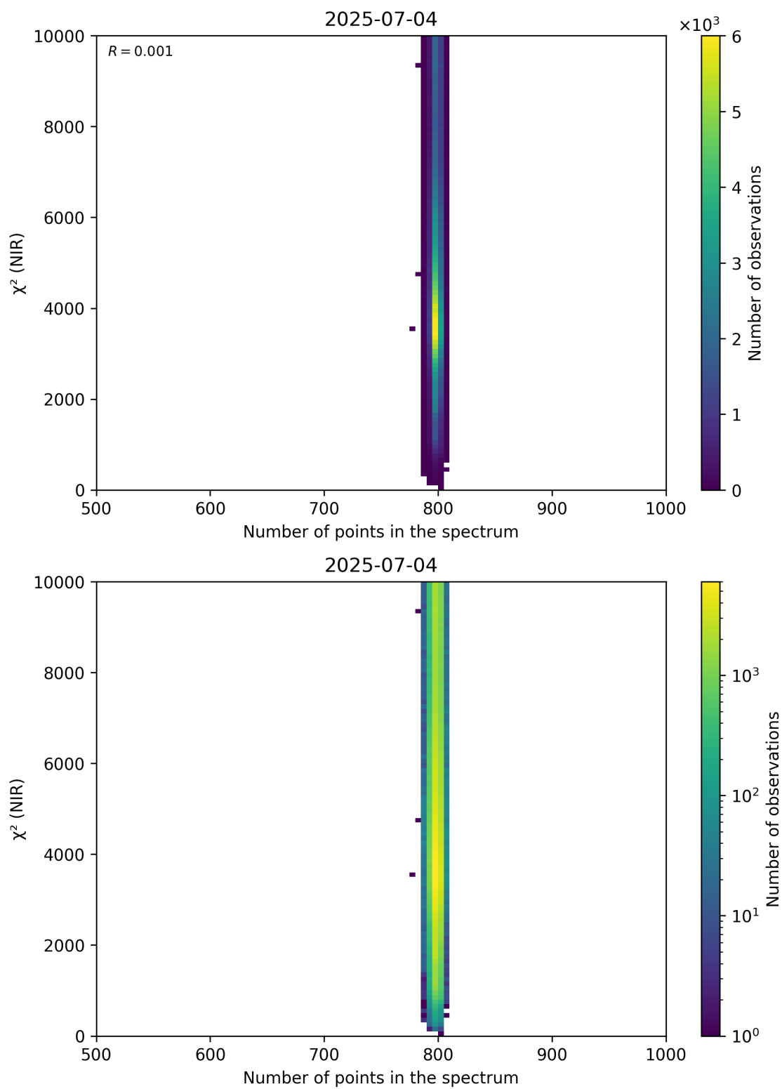
Figure 88: Scatter density plot of “Number of points in the spectrum” against “ \chi^2 (NIR)” for 2025-07-03 to 2025-07-05.
