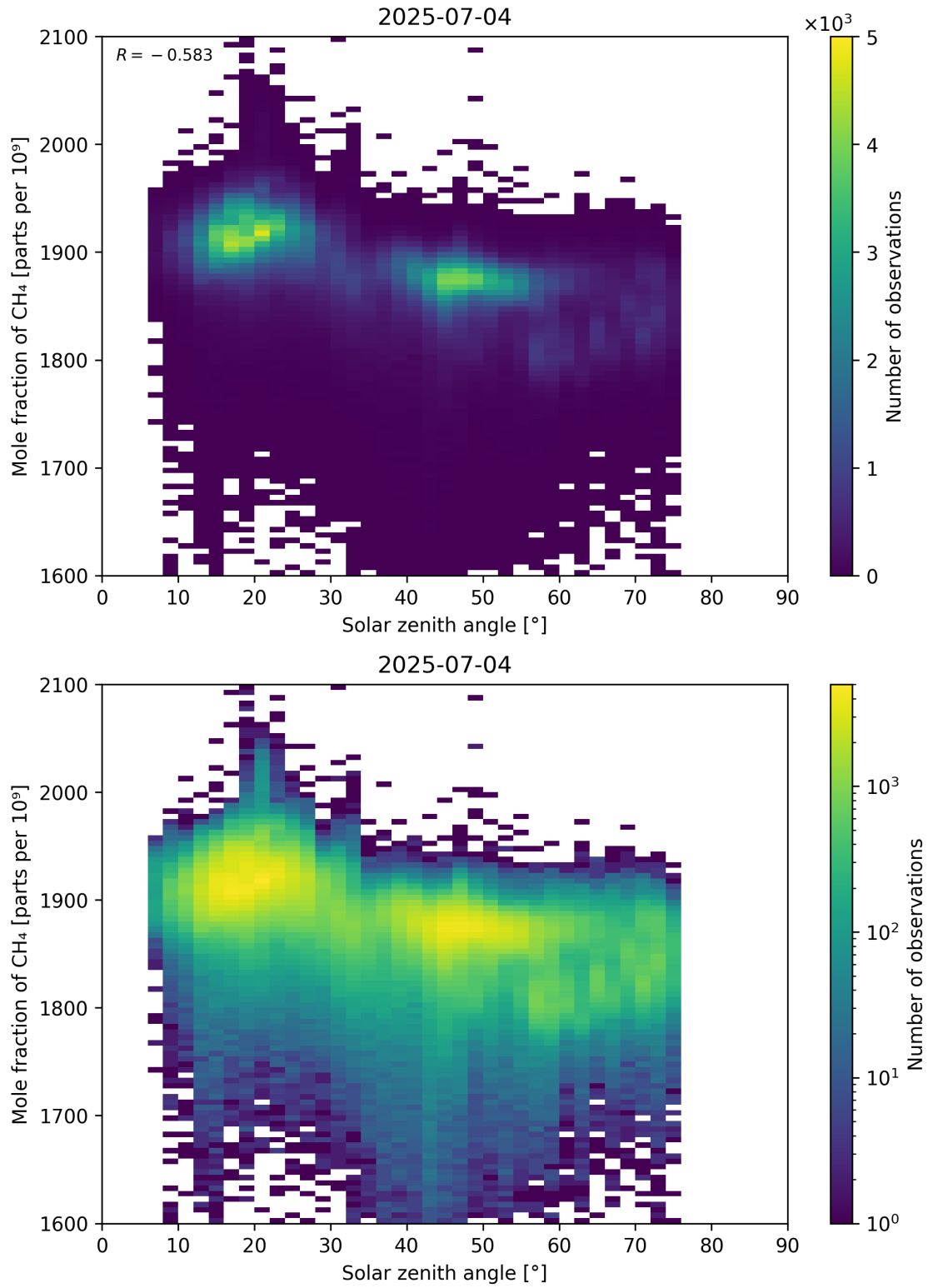
Figure 99: Scatter density plot of “Solar zenith angle” against “Mole fraction of CH 4 ” for 2025-07-03 to 2025-07-05.
