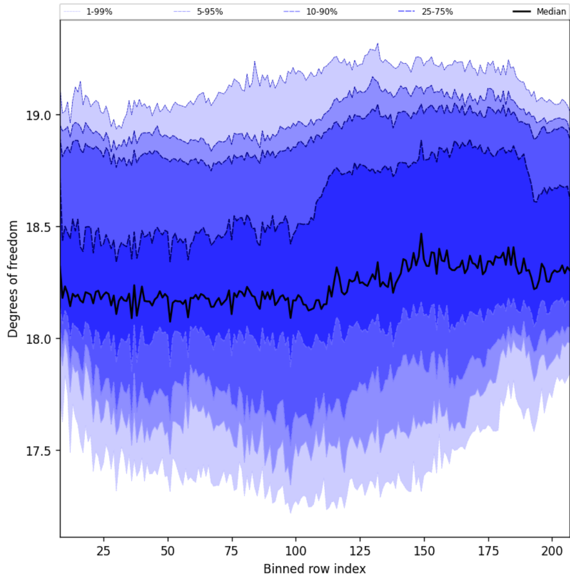
Figure 41: Along track statistics of “Degrees of freedom” for 2025-07-03 to 2025-07-05
