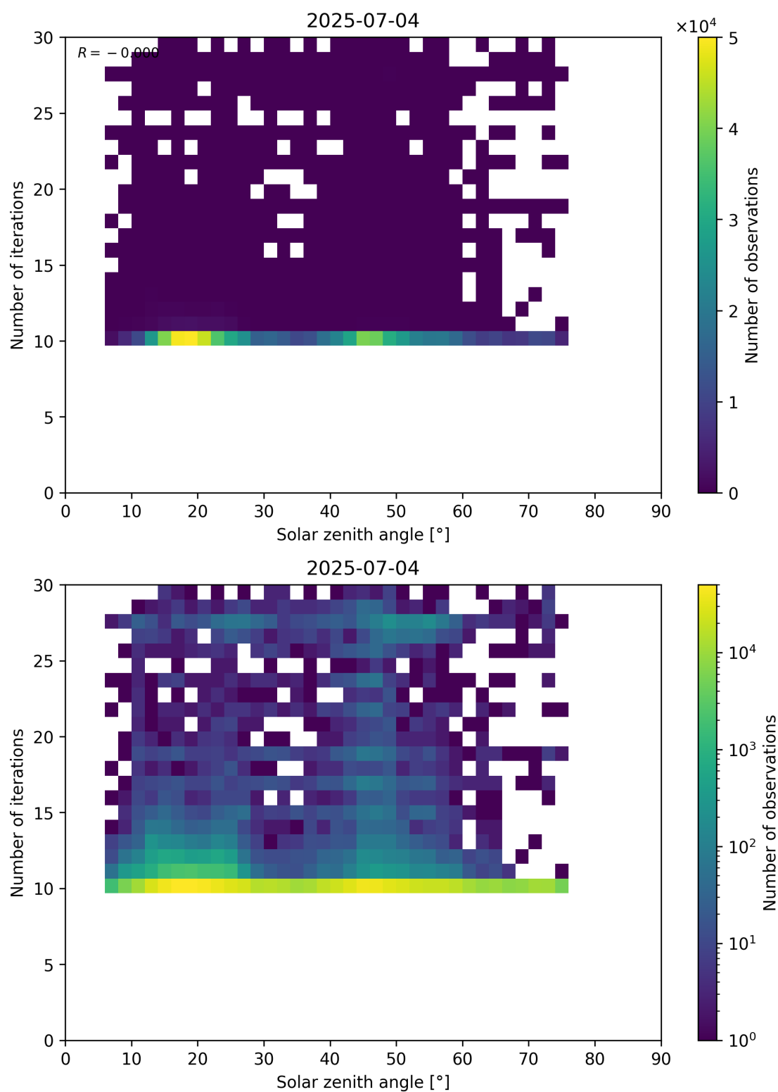
Figure 102: Scatter density plot of “Solar zenith angle” against “Number of iterations” for 2025-07-03 to 2025-07-05.
