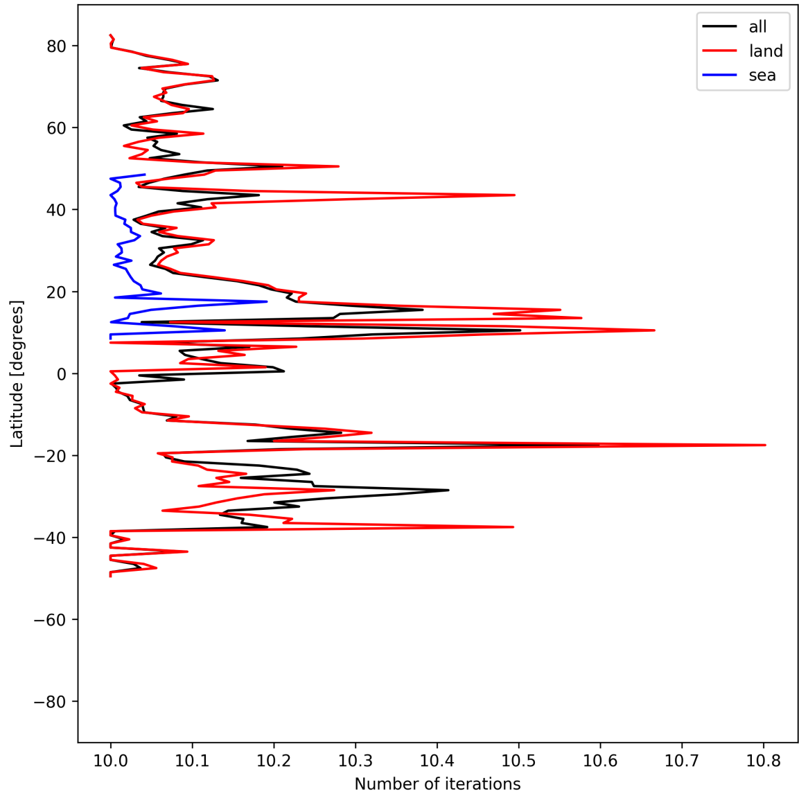
Figure 20: Zonal average of “Number of iterations” for 2025-07-03 to 2025-07-05.
