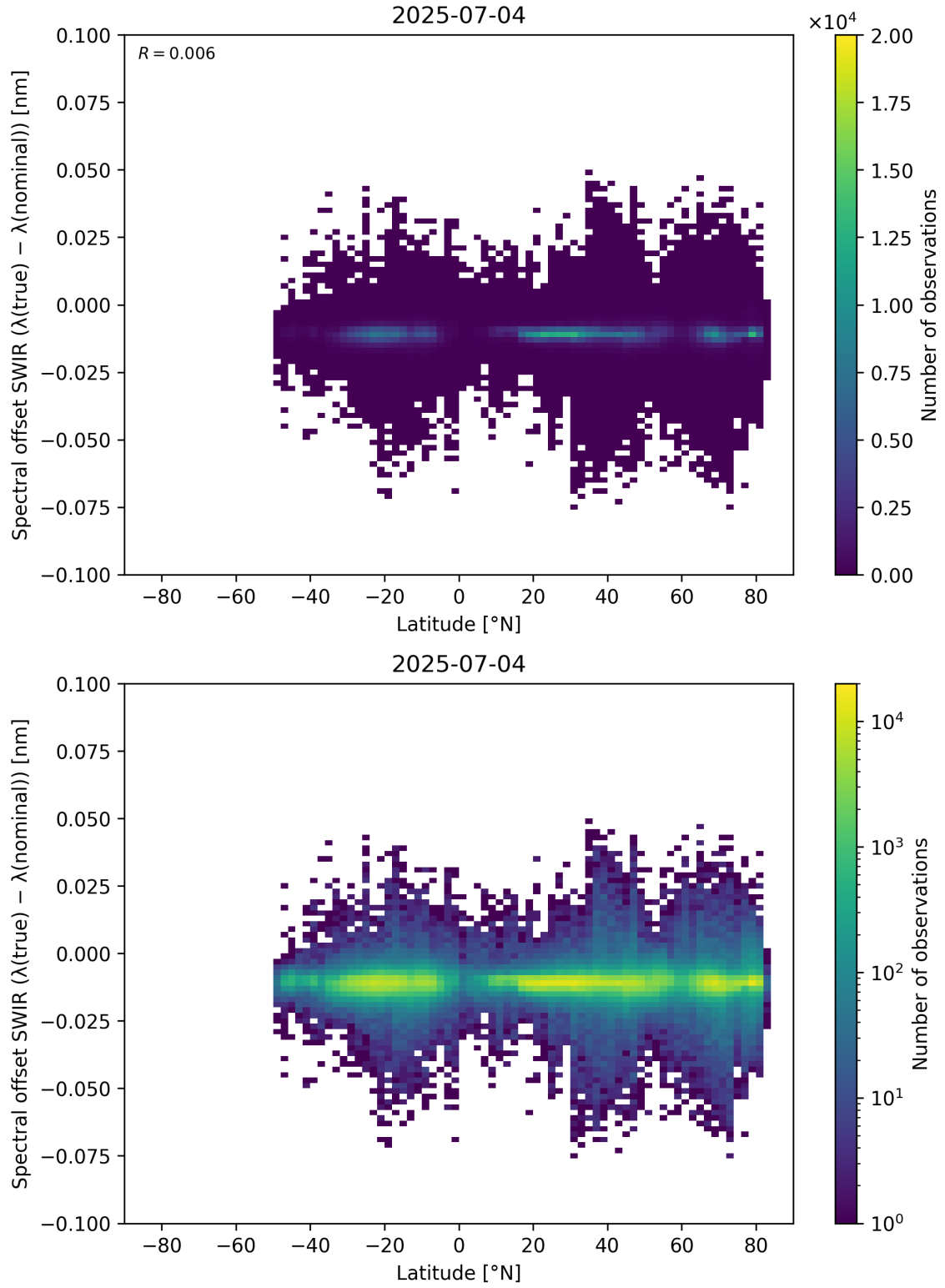
Figure 62: Scatter density plot of “Latitude” against “Spectral offset SWIR ( \lambda_{\text{true}} - \lambda_{\text{nominal}} )” for 2025-07-03 to 2025-07-05.
