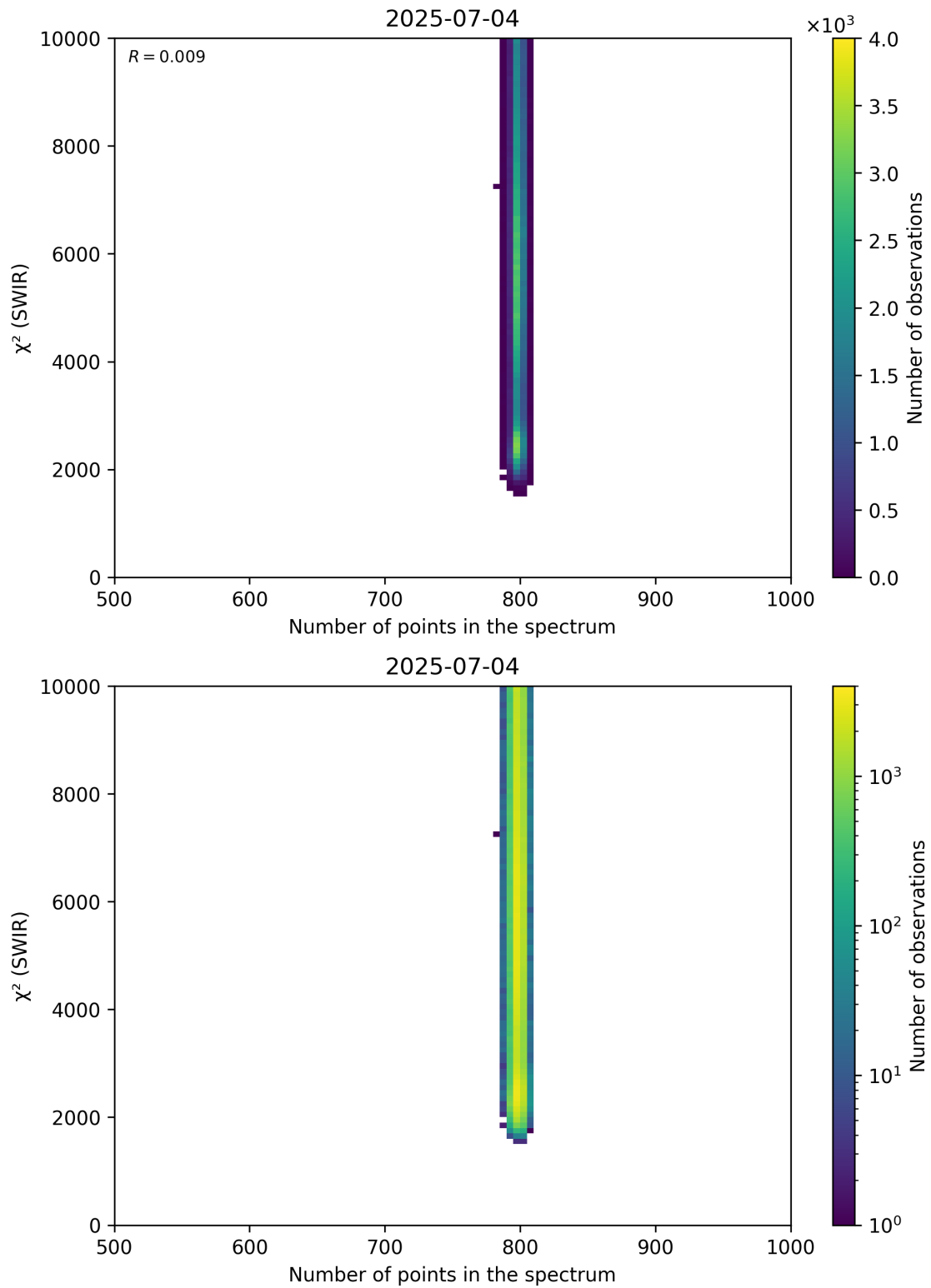
Figure 89: Scatter density plot of “Number of points in the spectrum” against “ \chi^2 (SWIR)” for 2025-07-03 to 2025-07-05.
