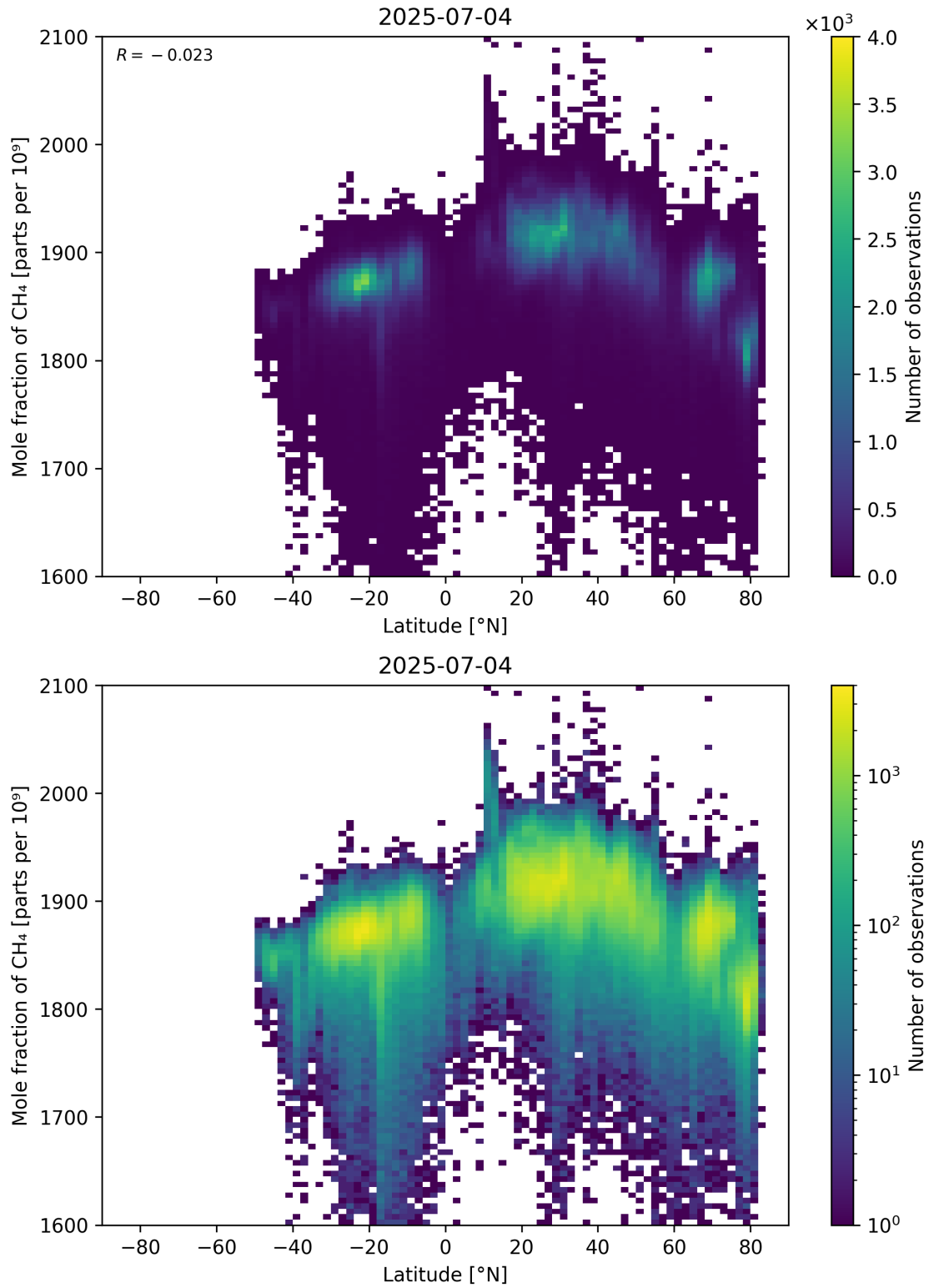
Figure 57: Scatter density plot of “Latitude” against “Mole fraction of \text{CH}_4 ” for 2025-07-03 to 2025-07-05.
