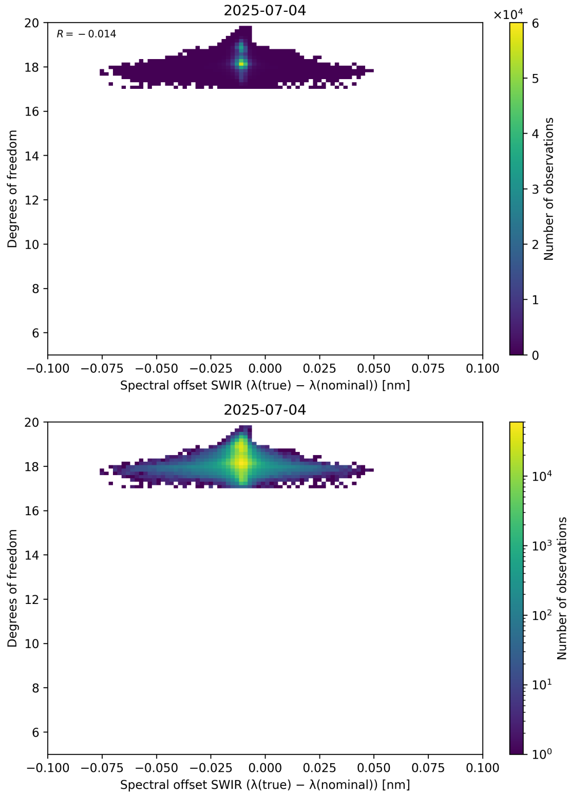
Figure 119: Scatter density plot of “Spectral offset SWIR ( \lambda_{\text{true}} - \lambda_{\text{nominal}} )” against “Degrees of freedom” for 2025-07-03 to 2025-07-05.
