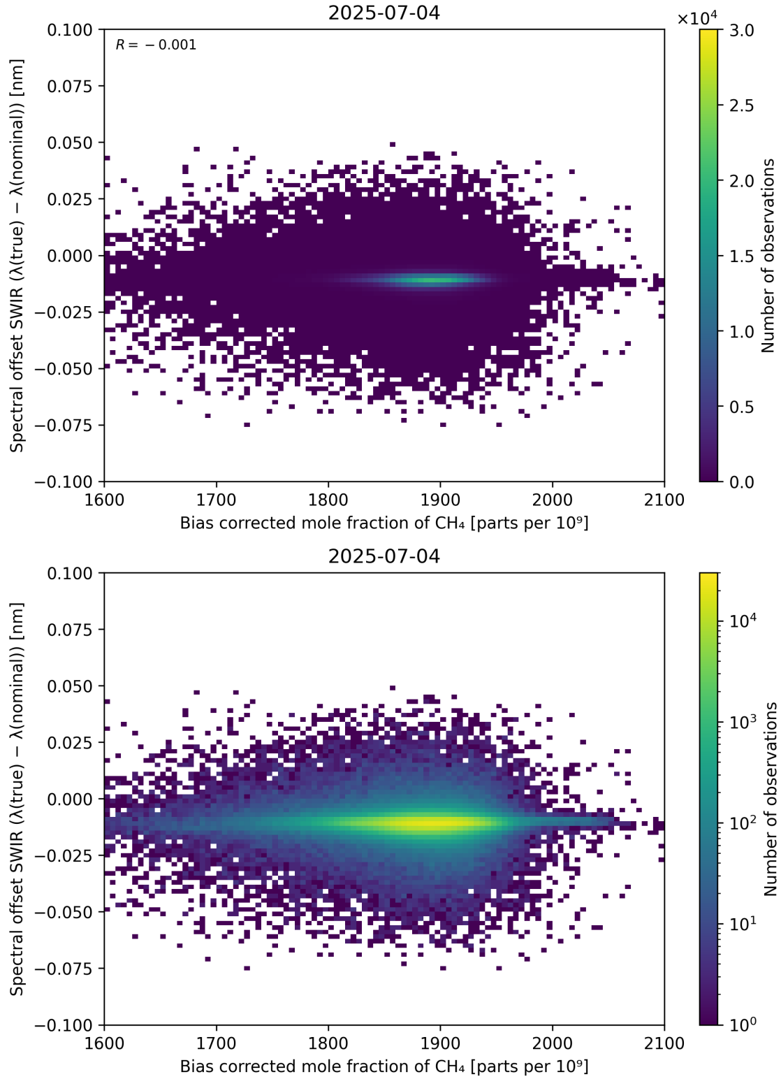
Figure 69: Scatter density plot of “Bias corrected mole fraction of \text{CH}_4 ” against “Spectral offset SWIR ( \lambda_{\text{true}} - \lambda_{\text{nominal}} )” for 2025-07-03 to 2025-07-05.
