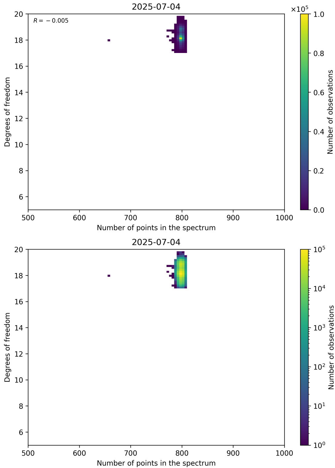
Figure 90: Scatter density plot of “Number of points in the spectrum” against “Degrees of freedom” for 2025-07-03 to 2025-07-05.
