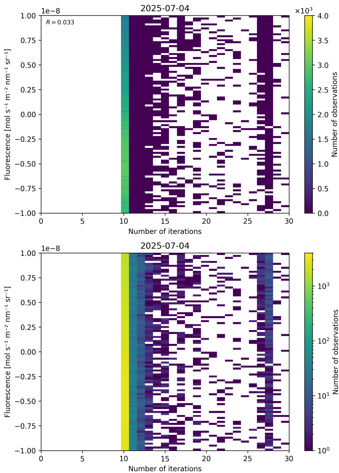
Figure 87: Scatter density plot of “Number of iterations” against “Fluorescence” for 2025-07-03 to 2025-07-05.
