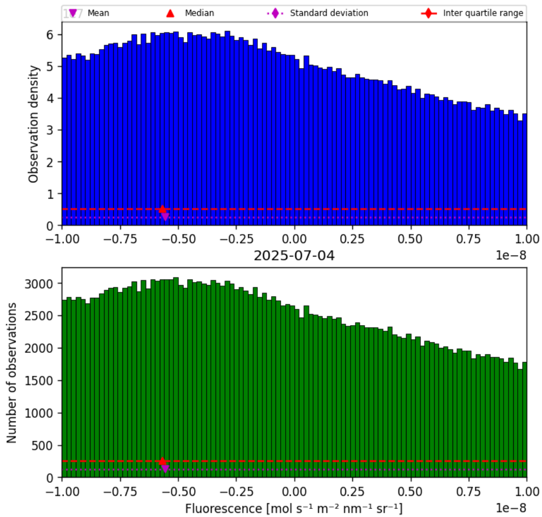
Figure 32: Histogram of “Fluorescence” for 2025-07-03 to 2025-07-05
