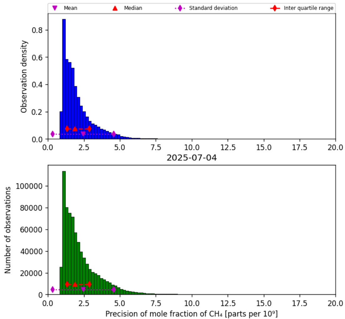
Figure 24: Histogram of “Precision of mole fraction of CH 4 ” for 2025-07-03 to 2025-07-05
