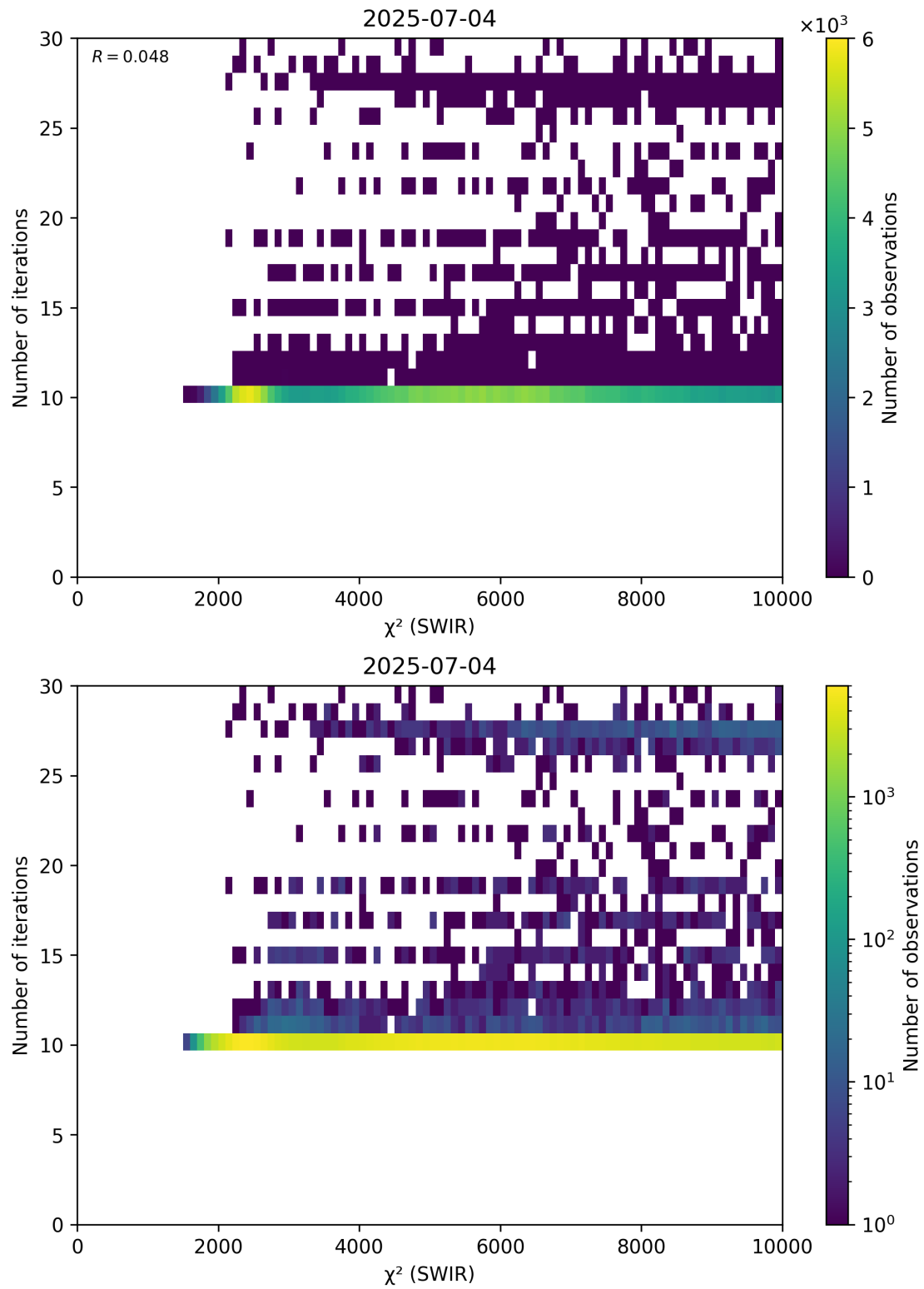
Figure 50: Scatter density plot of “ \chi^2 (SWIR)” against “Number of iterations” for 2025-07-03 to 2025-07-05.
