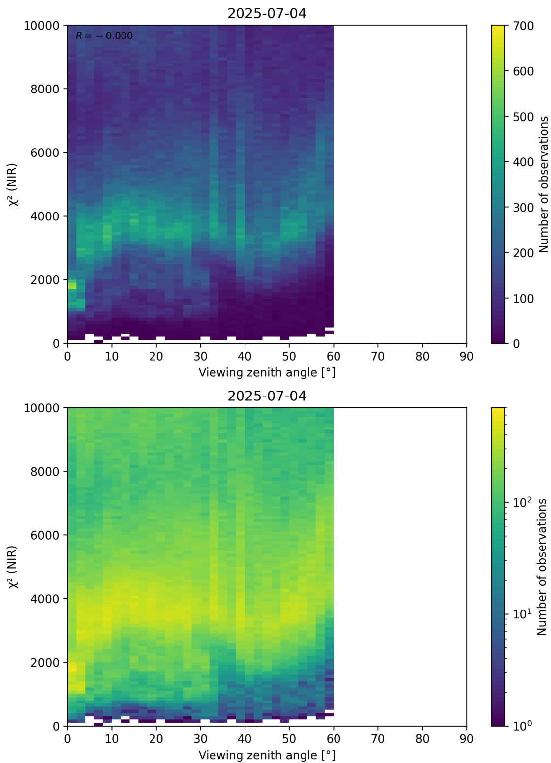
Figure 105: Scatter density plot of “Viewing zenith angle” against “ \chi^2 (NIR)” for 2025-07-03 to 2025-07-05.
