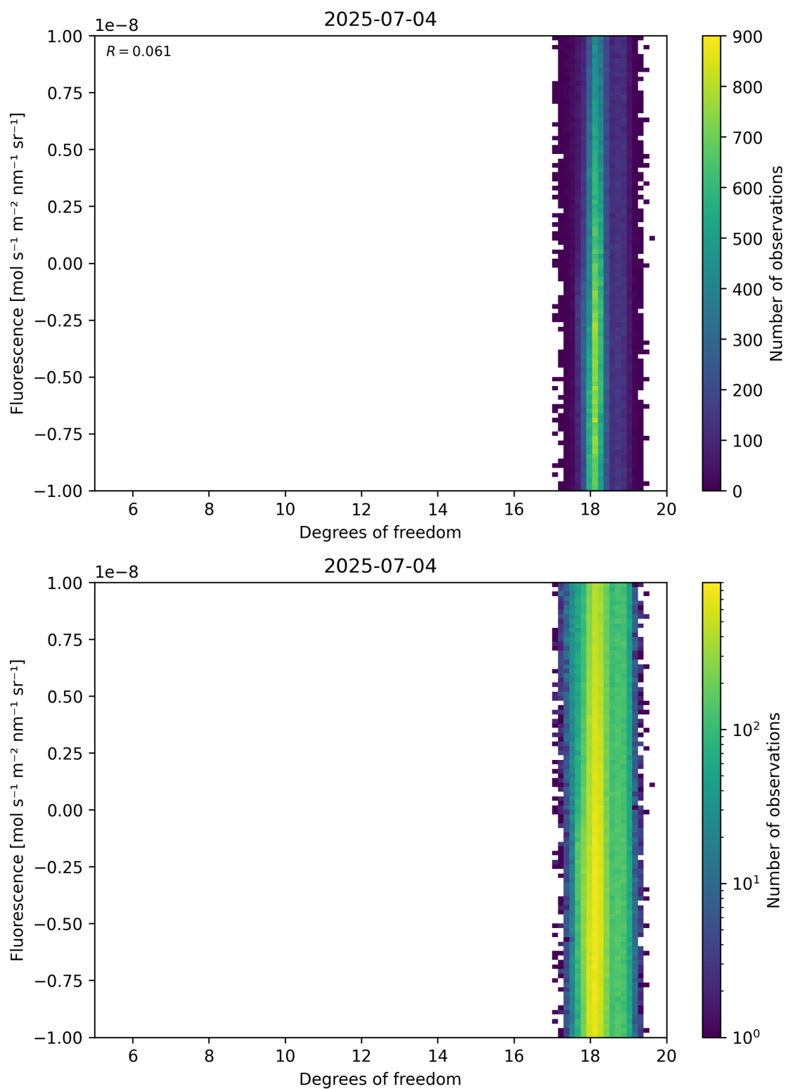
Figure 51: Scatter density plot of “Degrees of freedom” against “Fluorescence” for 2025-07-03 to 2025-07-05.
