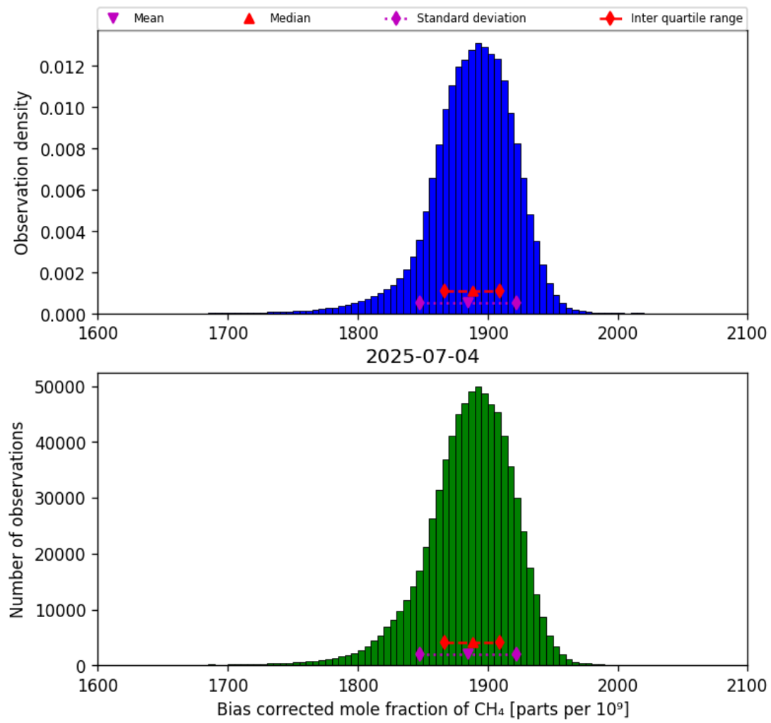
Figure 25: Histogram of “Bias corrected mole fraction of CH 4 ” for 2025-07-03 to 2025-07-05
