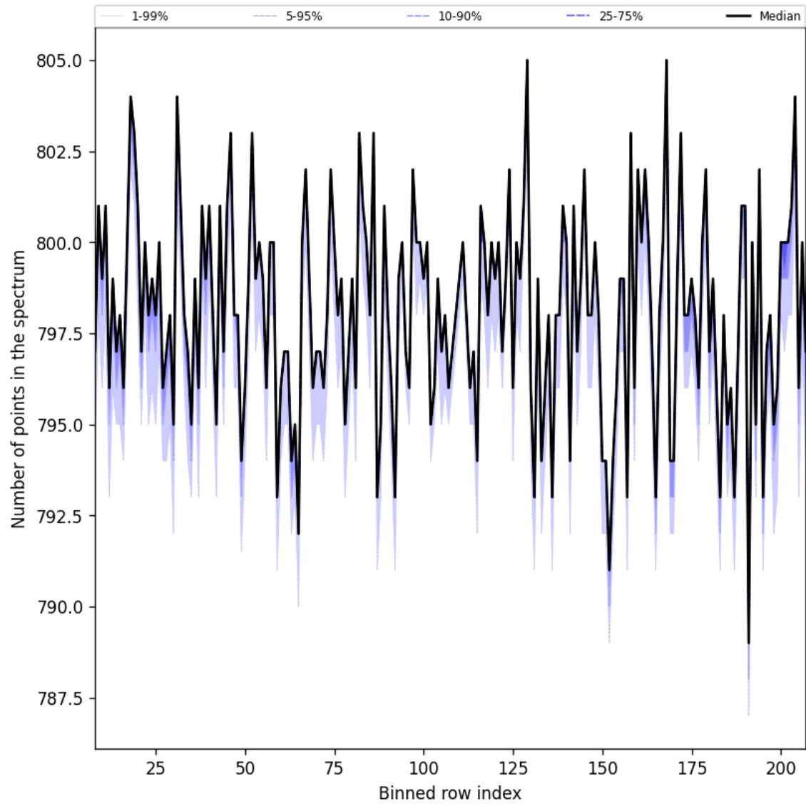
Figure 37: Along track statistics of “Number of points in the spectrum” for 2025-07-03 to 2025-07-05
