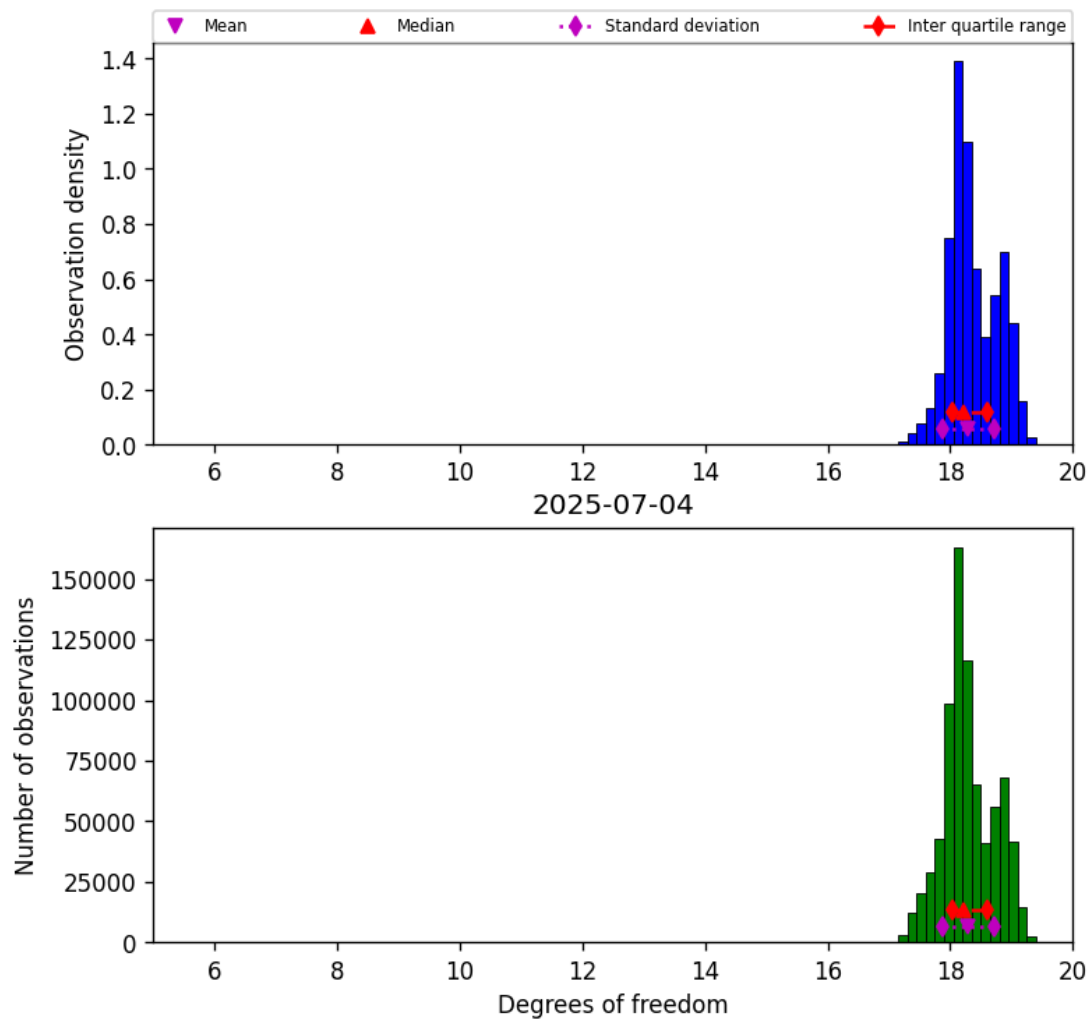
Figure 30: Histogram of “Degrees of freedom” for 2025-07-03 to 2025-07-05
