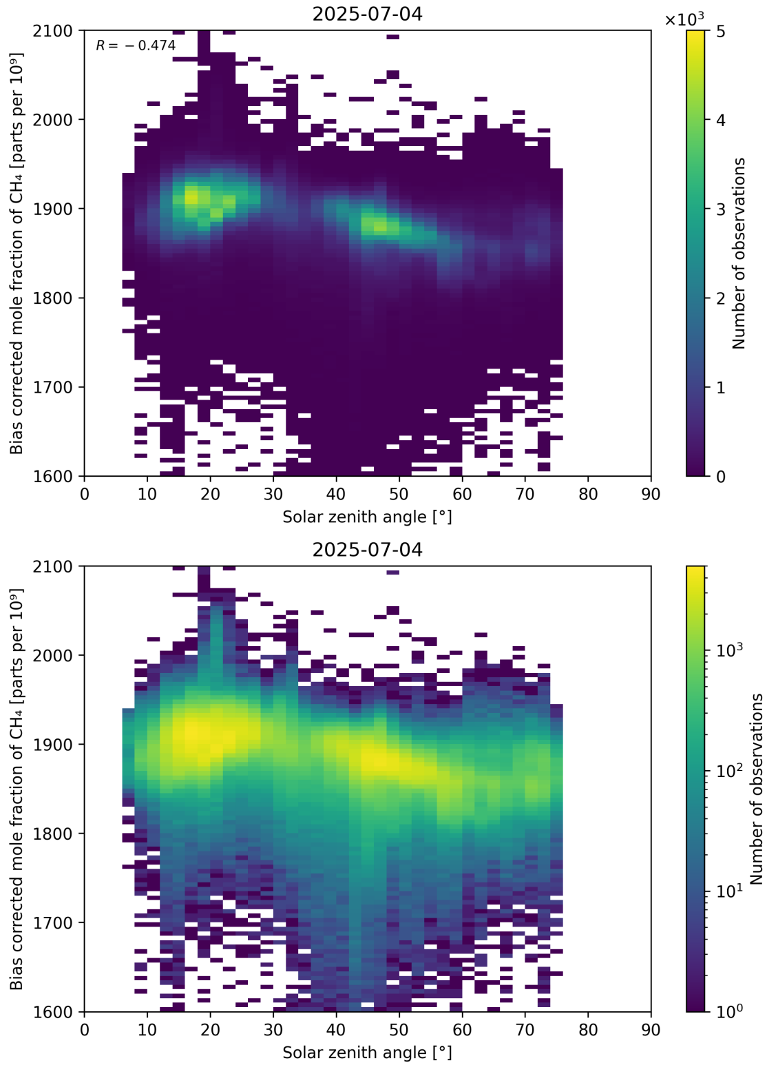
Figure 100: Scatter density plot of “Solar zenith angle” against “Bias corrected mole fraction of CH 4 ” for 2025-07-03 to 2025-07-05.
