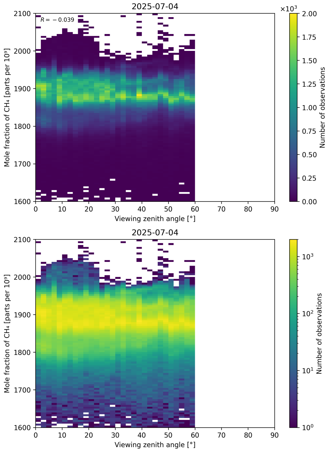
Figure 110: Scatter density plot of “Viewing zenith angle” against “Mole fraction of CH 4 ” for 2025-07-03 to 2025-07-05.
