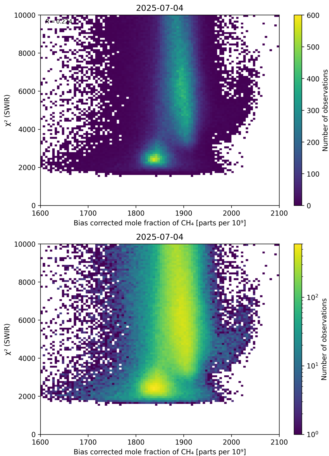
Figure 64: Scatter density plot of “Bias corrected mole fraction of \text{CH}_4 ” against “ \chi^2 (SWIR)” for 2025-07-03 to 2025-07-05.
