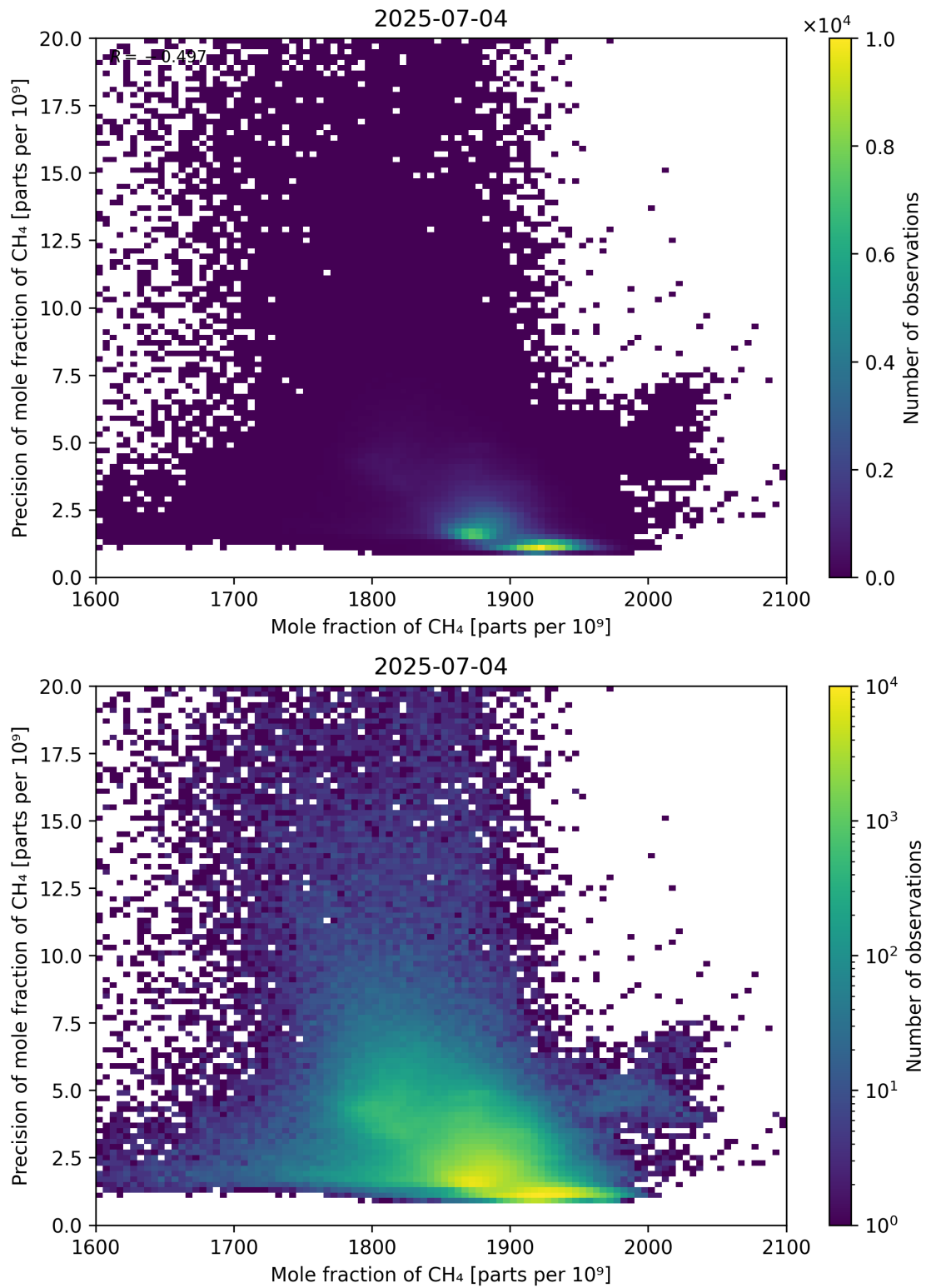
Figure 75: Scatter density plot of “Mole fraction of CH 4 ” against “Precision of mole fraction of CH 4 ” for 2025-07-03 to 2025-07-05.
