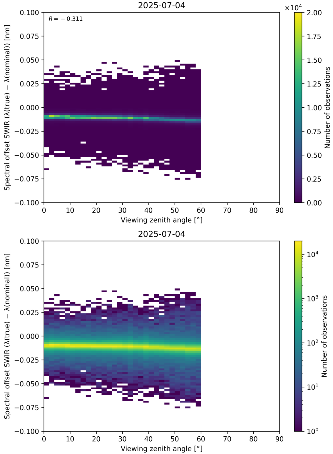
Figure 116: Scatter density plot of “Viewing zenith angle” against “Spectral offset SWIR ( \lambda_{\text{true}} - \lambda_{\text{nominal}} )” for 2025-07-03 to 2025-07-05.
