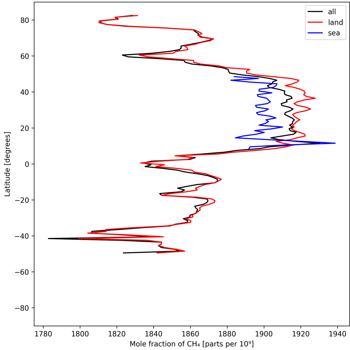
Figure 12: Zonal average of “Mole fraction of \text{CH}_4 ” for 2025-07-03 to 2025-07-05.
