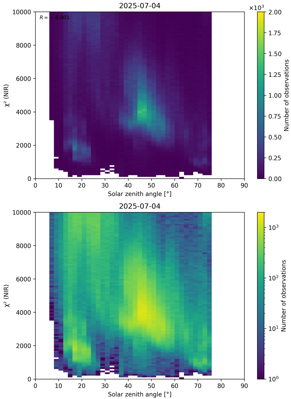
Figure 94: Scatter density plot of “Solar zenith angle” against “ \chi^2 (NIR)” for 2025-07-03 to 2025-07-05.
