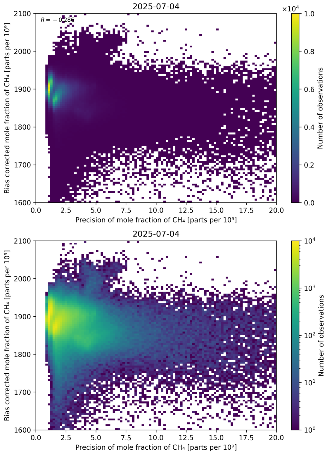
Figure 82: Scatter density plot of “Precision of mole fraction of CH 4 ” against “Bias corrected mole fraction of CH 4 ” for 2025-07-03 to 2025-07-05.
