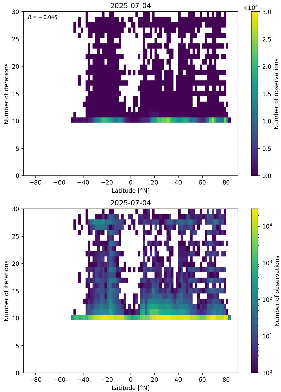
Figure 60: Scatter density plot of “Latitude” against “Number of iterations” for 2025-07-03 to 2025-07-05.
