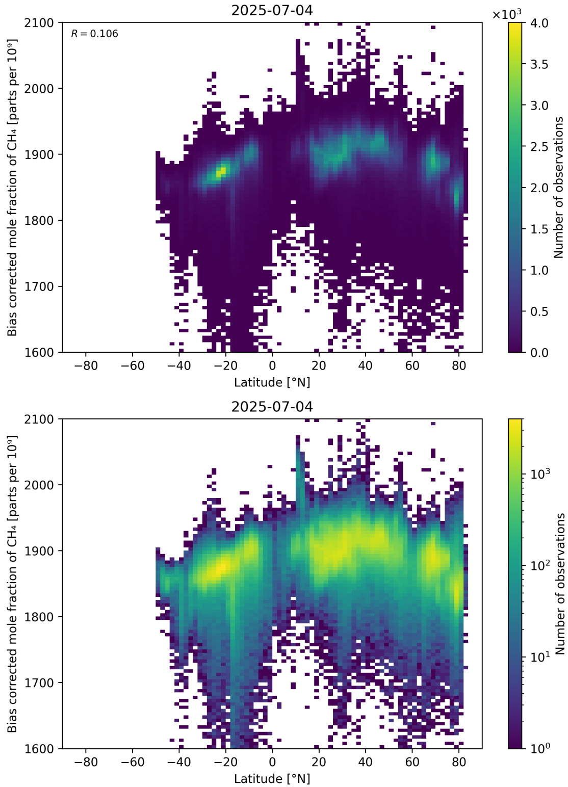
Figure 58: Scatter density plot of “Latitude” against “Bias corrected mole fraction of \text{CH}_4 ” for 2025-07-03 to 2025-07-05.
