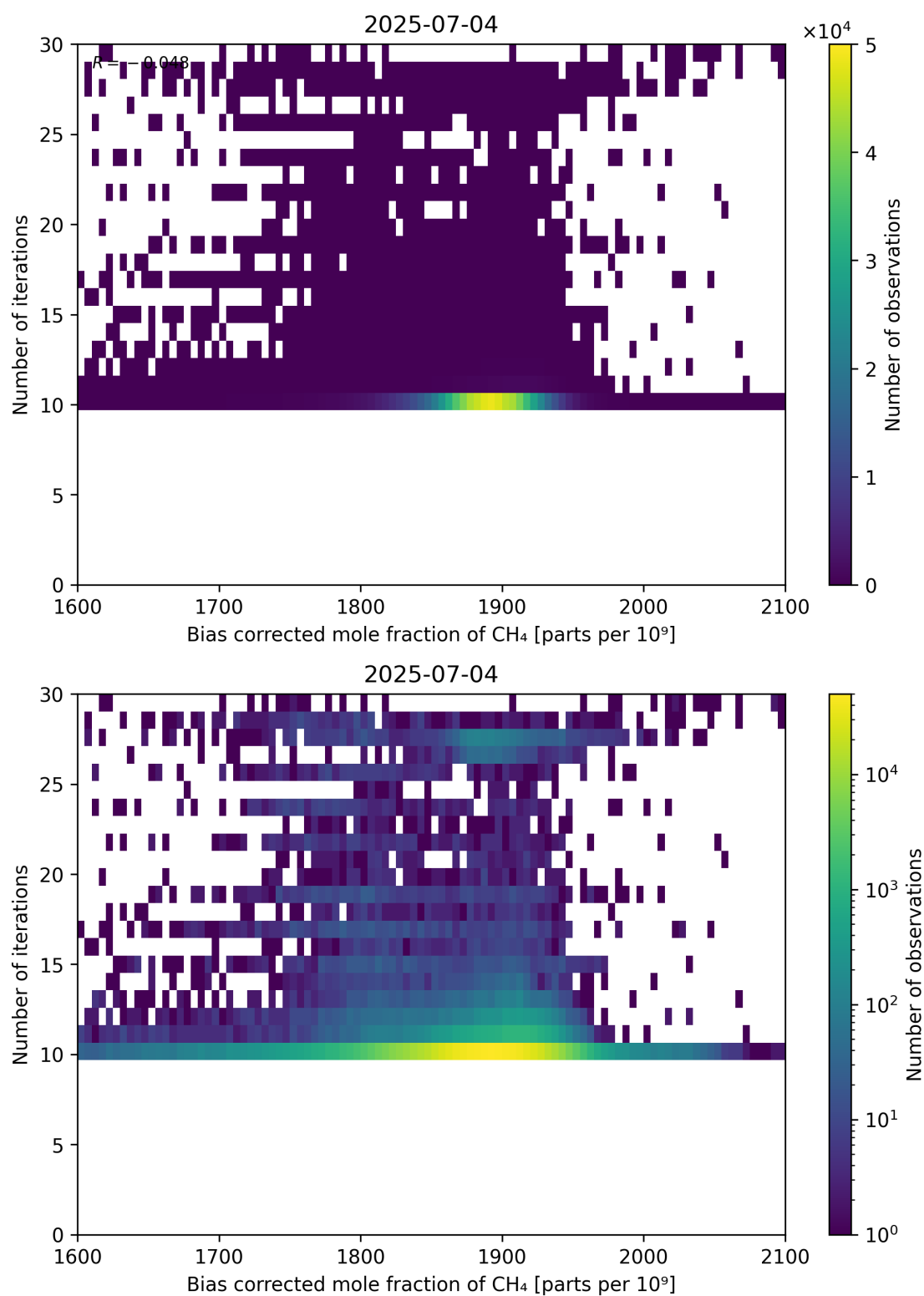
Figure 67: Scatter density plot of “Bias corrected mole fraction of CH 4 ” against “Number of iterations” for 2025-07-03 to 2025-07-05.
