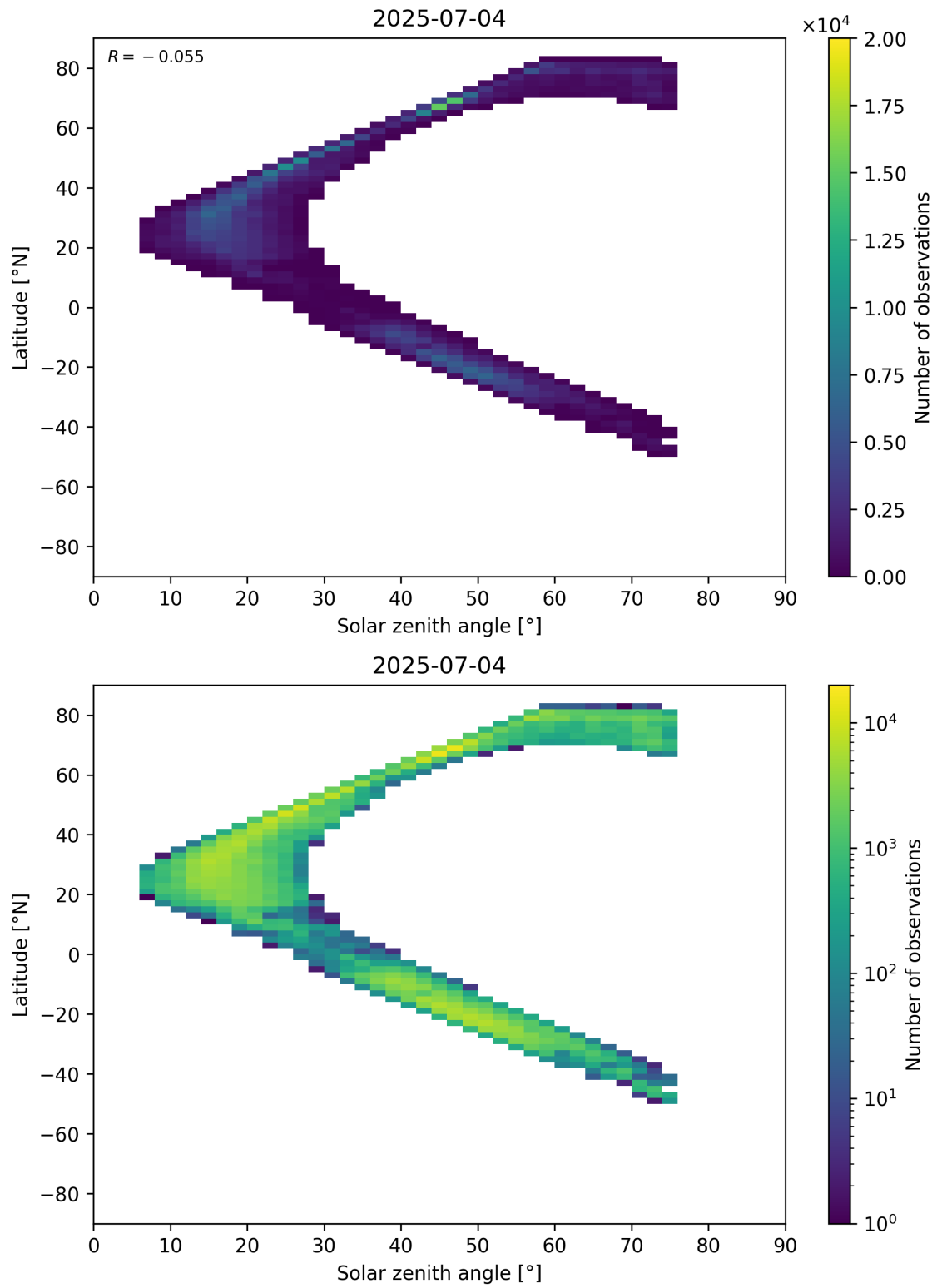
Figure 98: Scatter density plot of “Solar zenith angle” against “Latitude” for 2025-07-03 to 2025-07-05.
