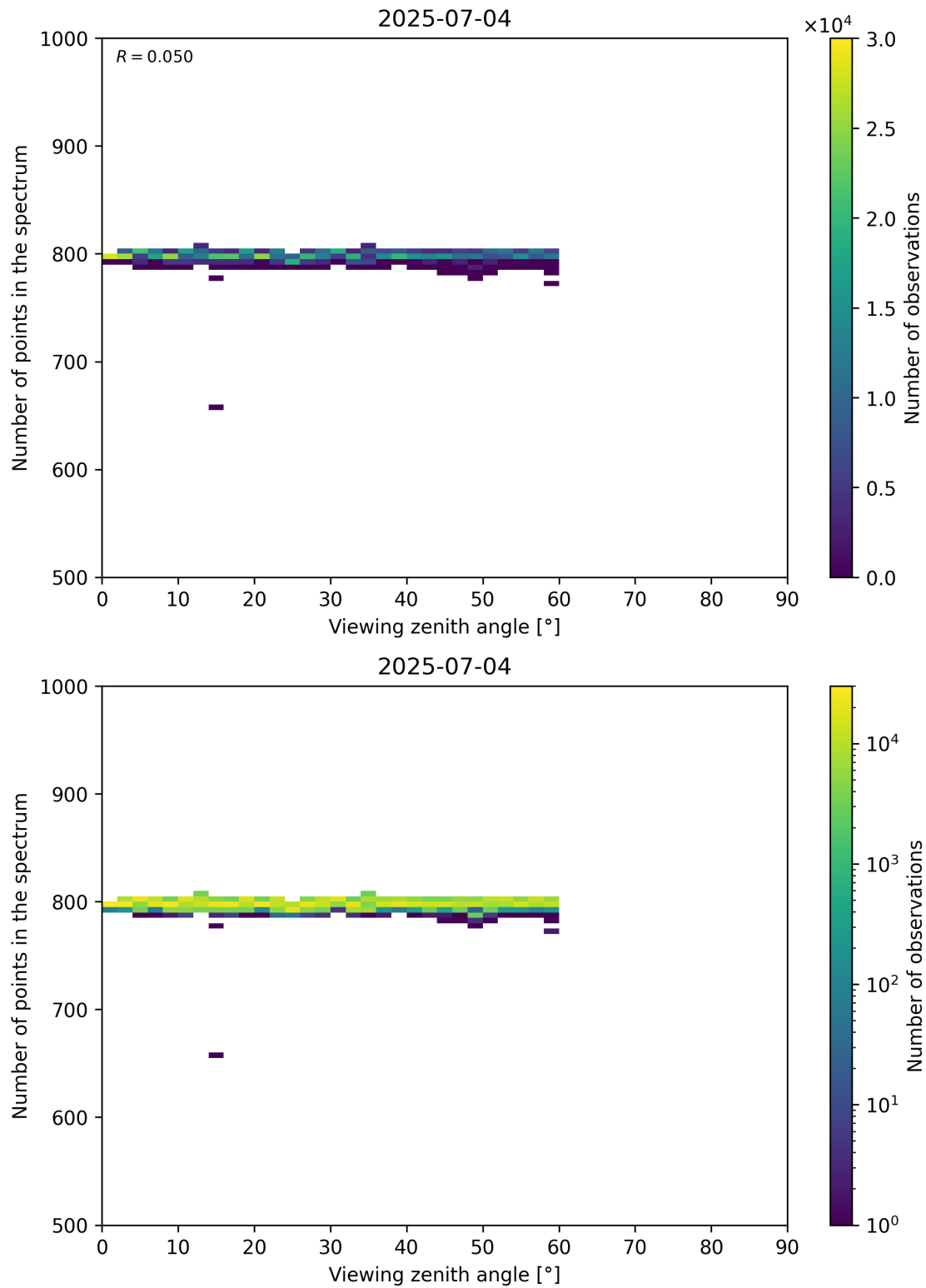
Figure 114: Scatter density plot of “Viewing zenith angle” against “Number of points in the spectrum” for 2025-07-03 to 2025-07-05.
