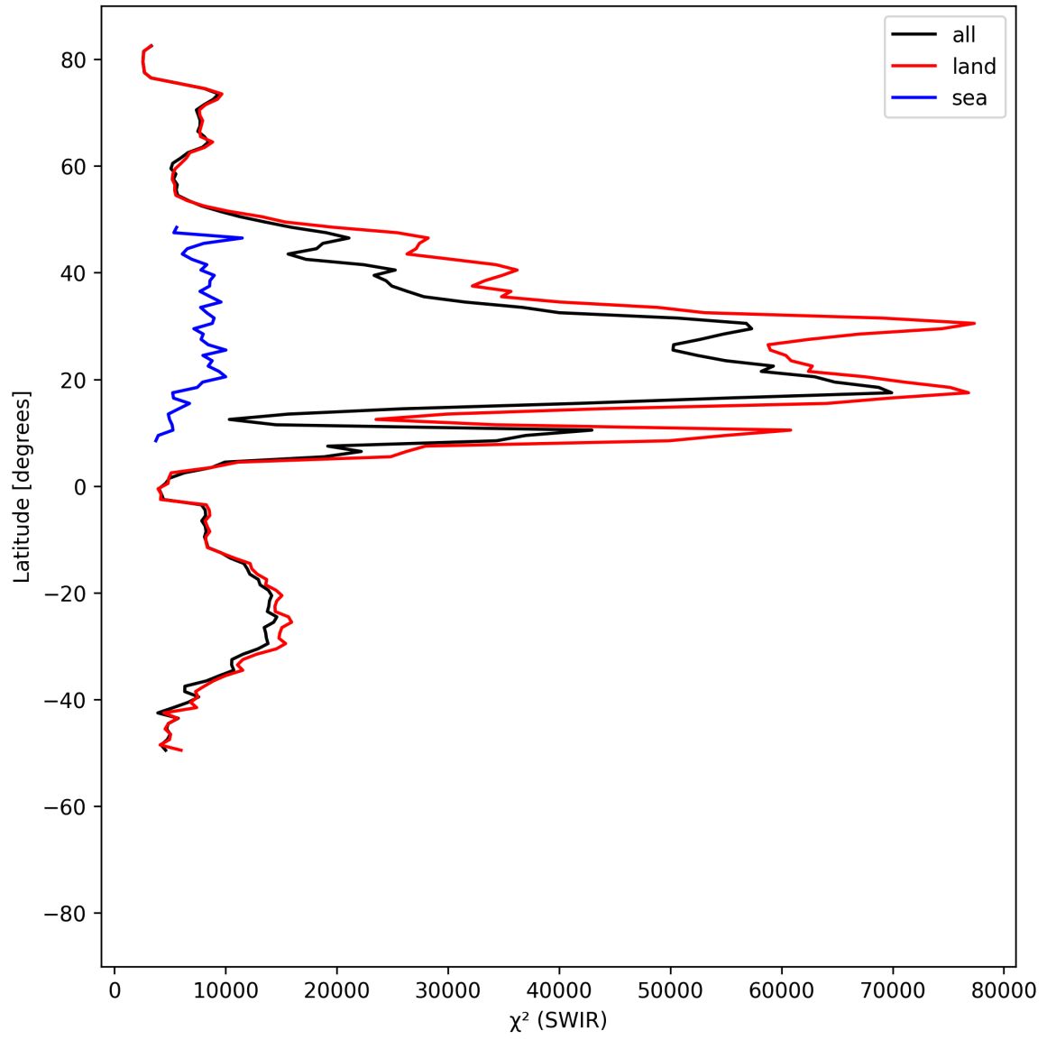
Figure 17: Zonal average of “ \chi^2 (SWIR)” for 2025-07-03 to 2025-07-05.
