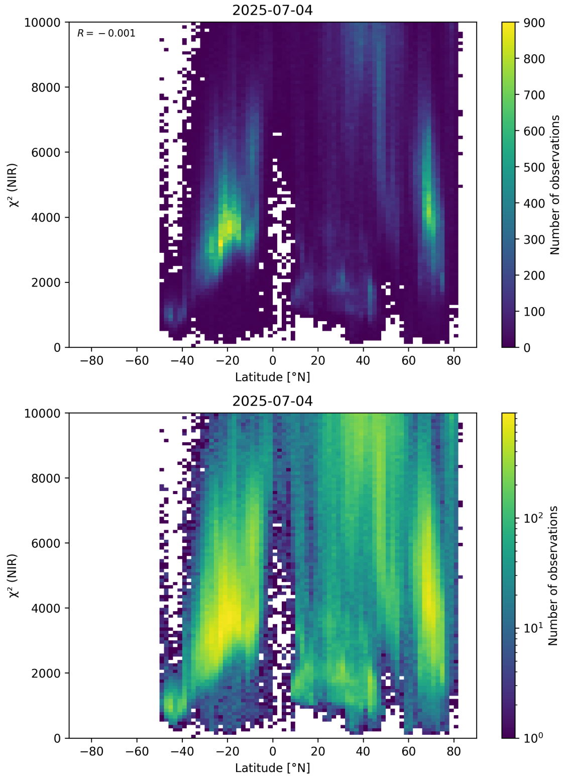
Figure 53: Scatter density plot of “Latitude” against “ \chi^2 (NIR)” for 2025-07-03 to 2025-07-05.
