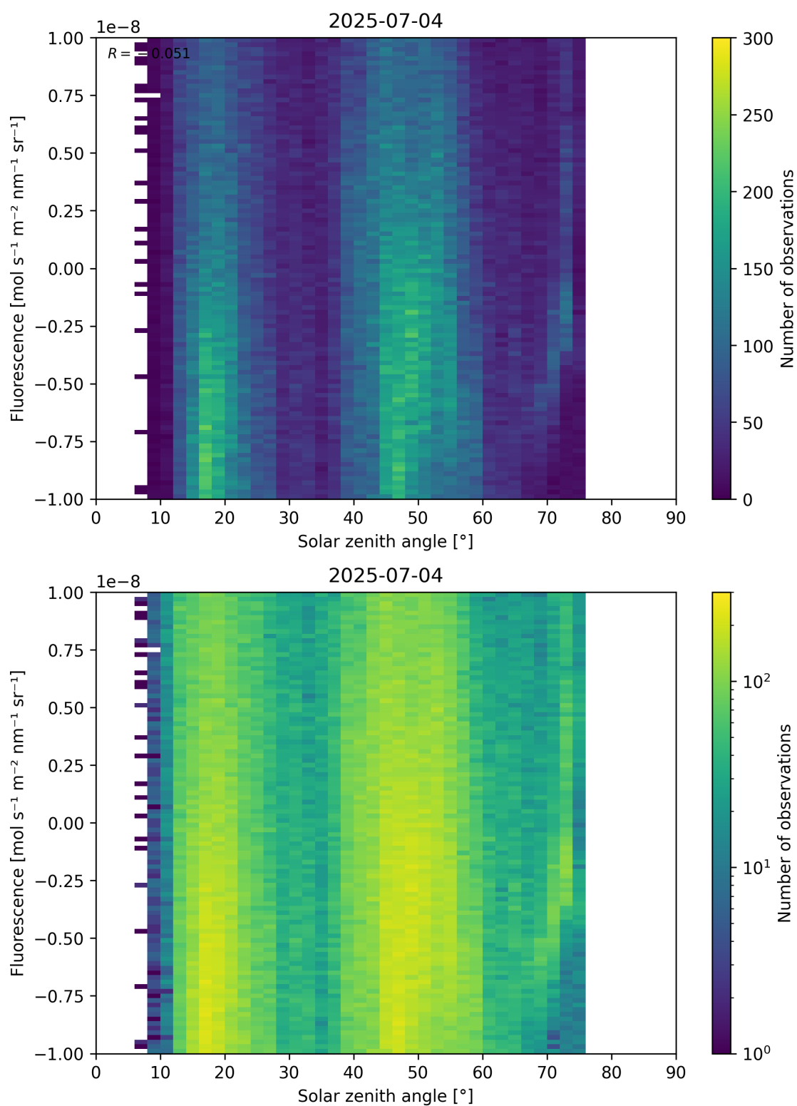
Figure 97: Scatter density plot of “Solar zenith angle” against “Fluorescence” for 2025-07-03 to 2025-07-05.
