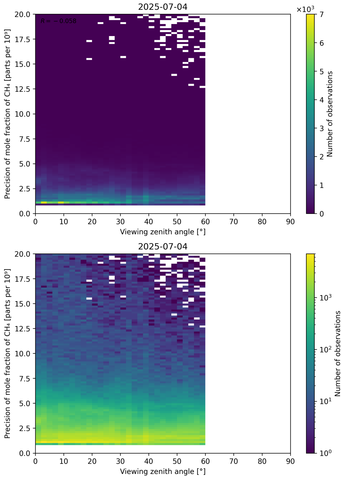
Figure 112: Scatter density plot of “Viewing zenith angle” against “Precision of mole fraction of CH 4 ” for 2025-07-03 to 2025-07-05.
