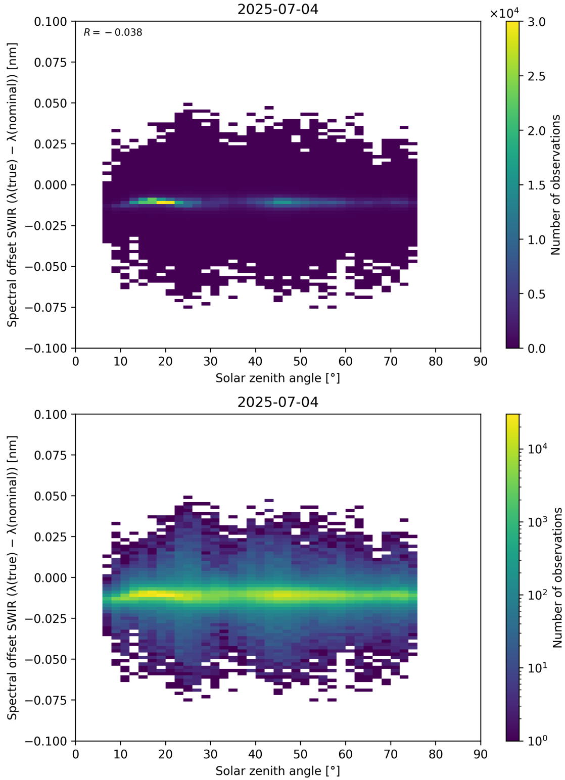
Figure 104: Scatter density plot of “Solar zenith angle” against “Spectral offset SWIR ( \lambda_{\text{true}} - \lambda_{\text{nominal}} )” for 2025-07-03 to 2025-07-05.
