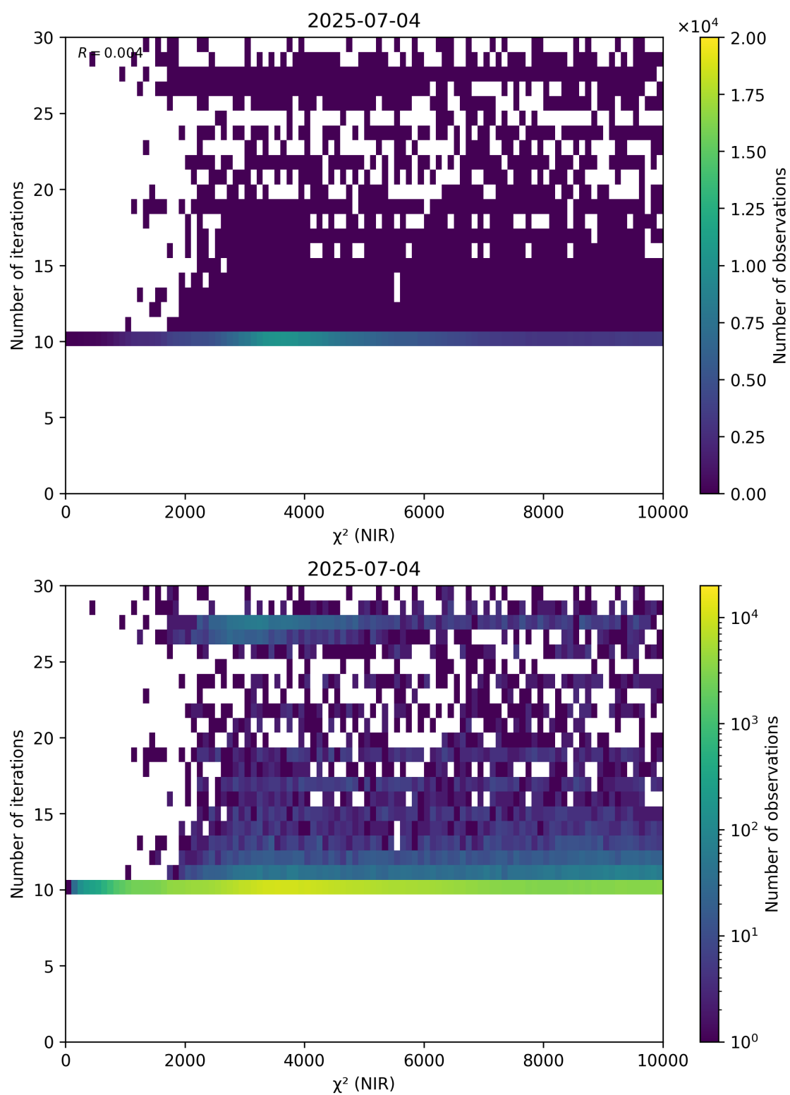
Figure 46: Scatter density plot of “ \chi^2 (NIR)” against “Number of iterations” for 2025-07-03 to 2025-07-05.
