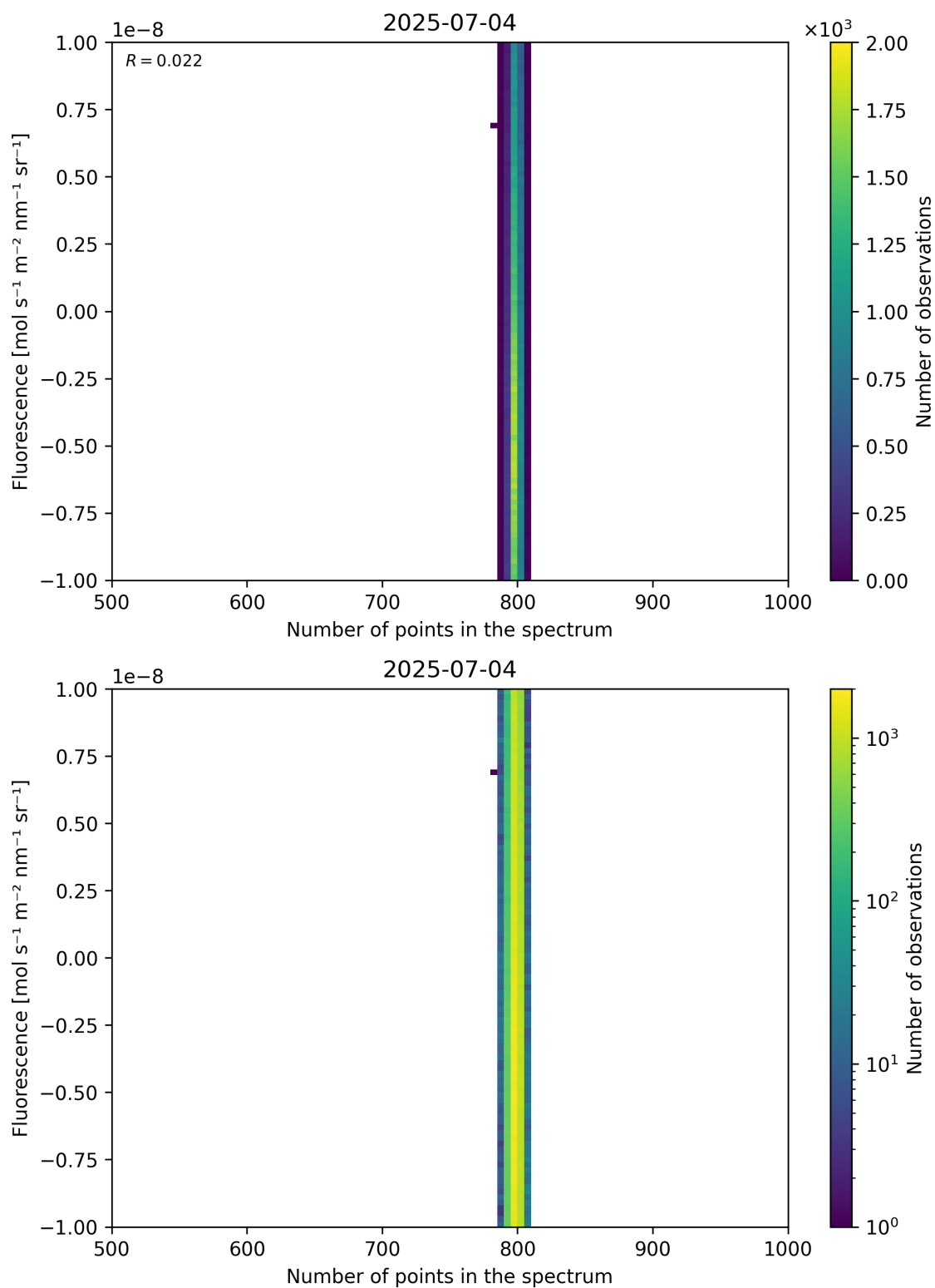
Figure 91: Scatter density plot of “Number of points in the spectrum” against “Fluorescence” for 2025-07-03 to 2025-07-05.
