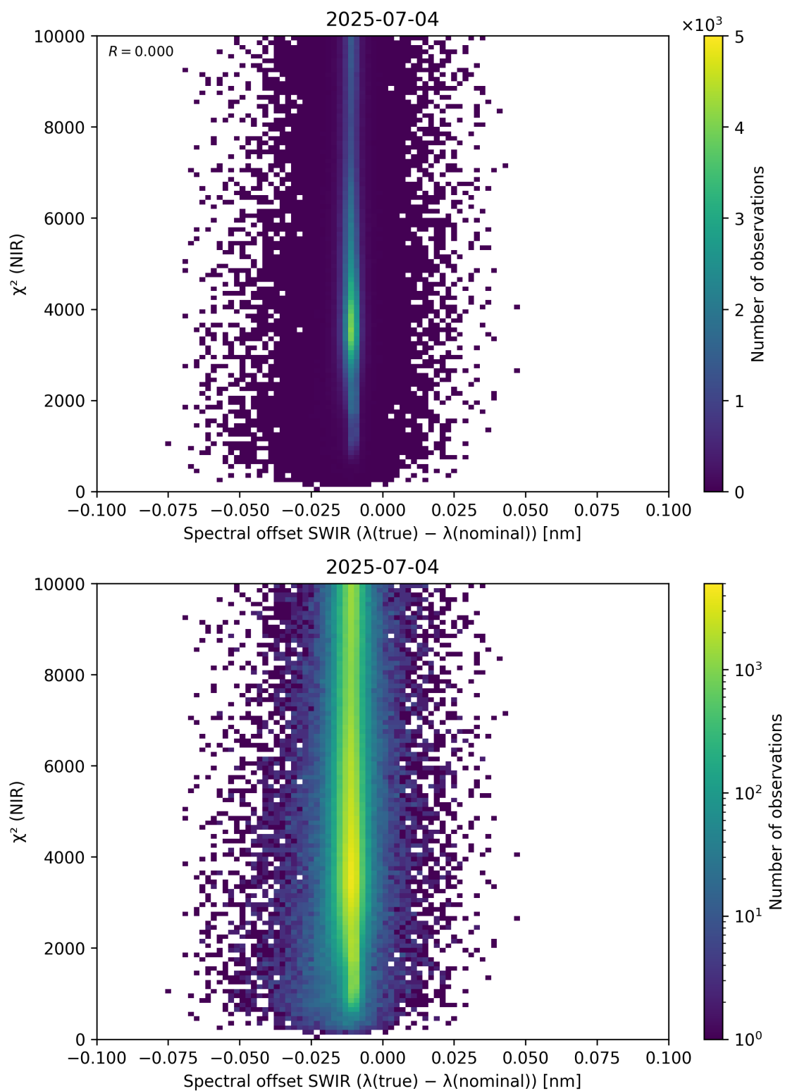
Figure 117: Scatter density plot of “Spectral offset SWIR ( \lambda_{\text{true}} - \lambda_{\text{nominal}} )” against “ \chi^2 (NIR)” for 2025-07-03 to 2025-07-05.
