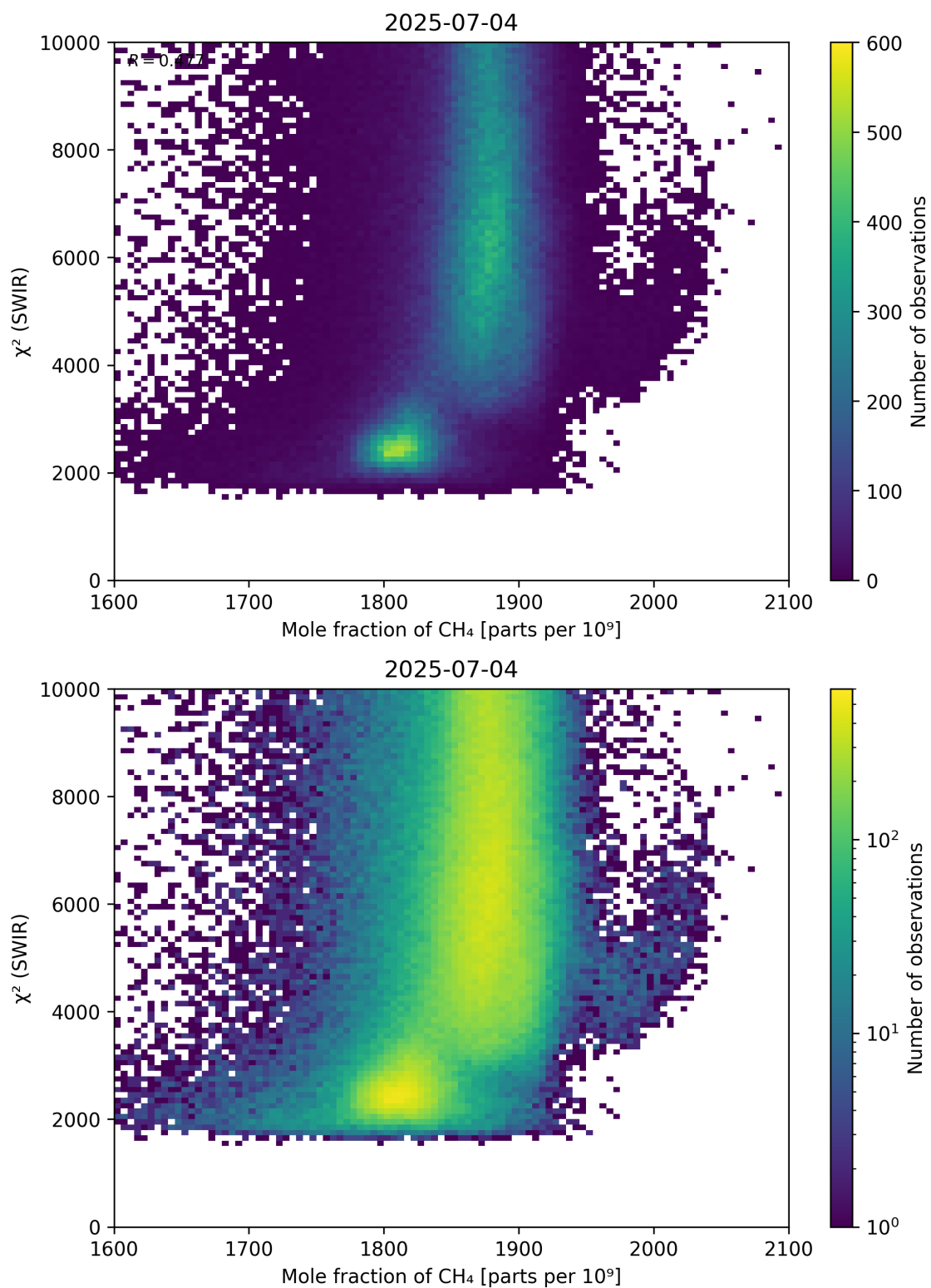
Figure 71: Scatter density plot of “Mole fraction of CH 4 ” against “ \chi^2 (SWIR)” for 2025-07-03 to 2025-07-05.
