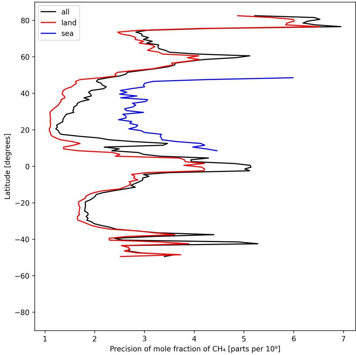
Figure 13: Zonal average of “Precision of mole fraction of CH 4 ” for 2025-07-03 to 2025-07-05.
