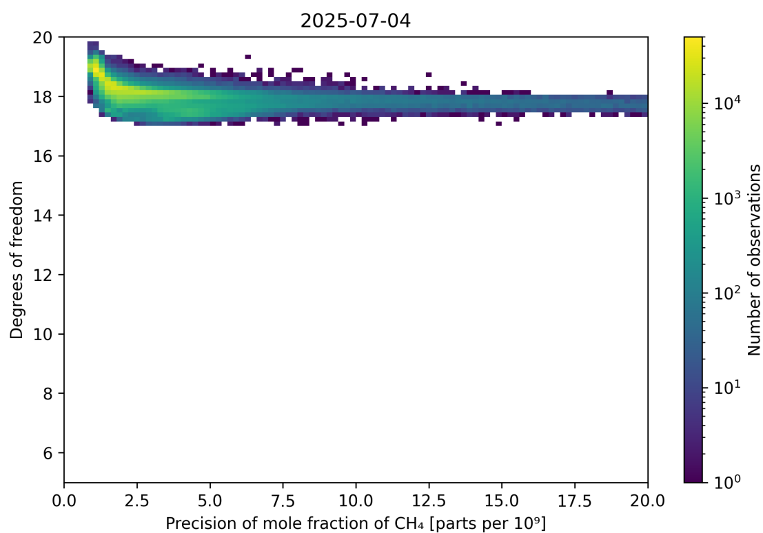
Figure 80: Scatter density plot of “Precision of mole fraction of CH 4 ” against “Degrees of freedom” for 2025-07-03 to 2025-07-05.
