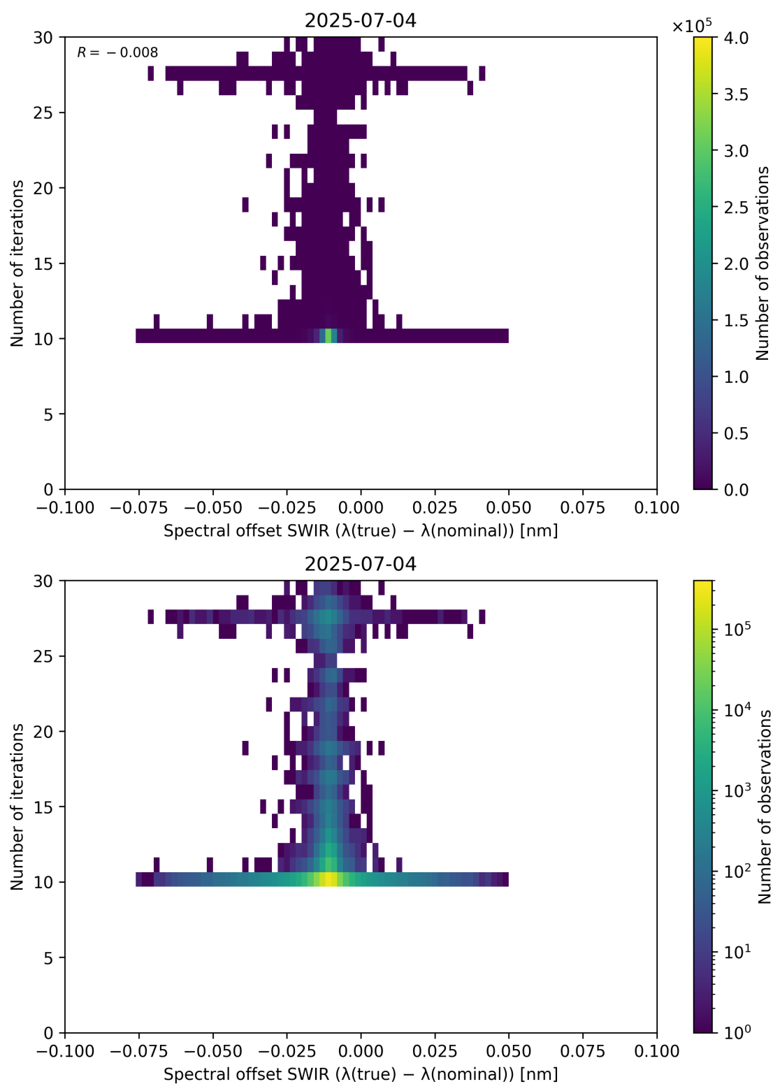
Figure 121: Scatter density plot of “Spectral offset SWIR ( \lambda_{\text{true}} - \lambda_{\text{nominal}} )” against “Number of iterations” for 2025-07-03 to 2025-07-05.
