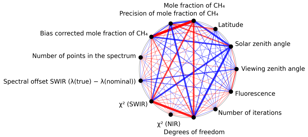
Figure 1: Map of correlation graph for 2025-07-03 to 2025-07-05.
