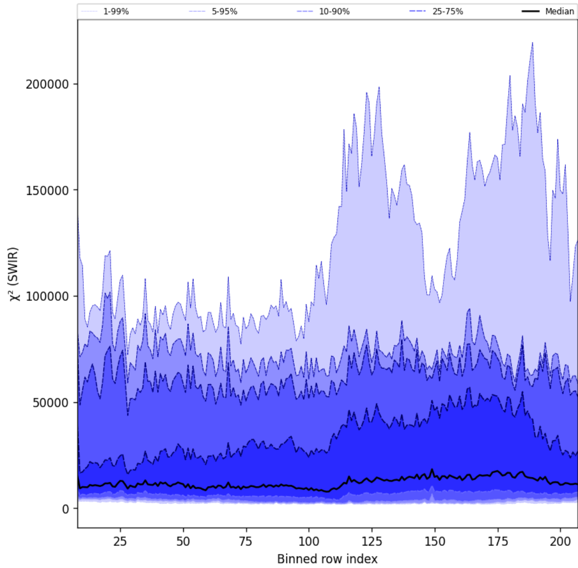
Figure 39: Along track statistics of “ \chi^2 (SWIR)” for 2025-07-03 to 2025-07-05
