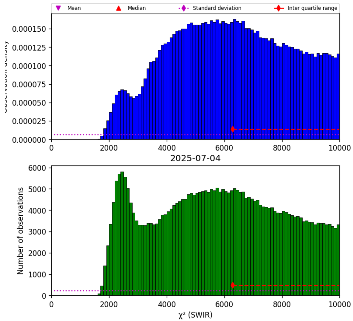
Figure 28: Histogram of “ \chi^2 (SWIR)” for 2025-07-03 to 2025-07-05
