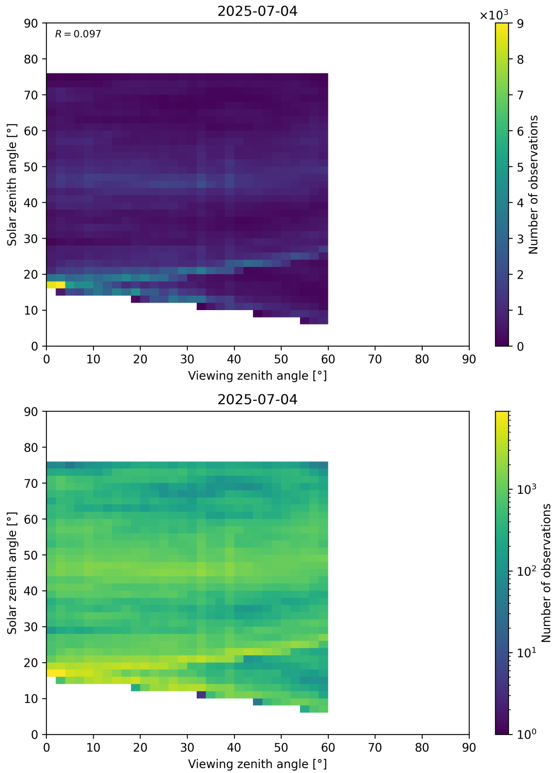
Figure 115: Scatter density plot of “Viewing zenith angle” against “Solar zenith angle” for 2025-07-03 to 2025-07-05.
