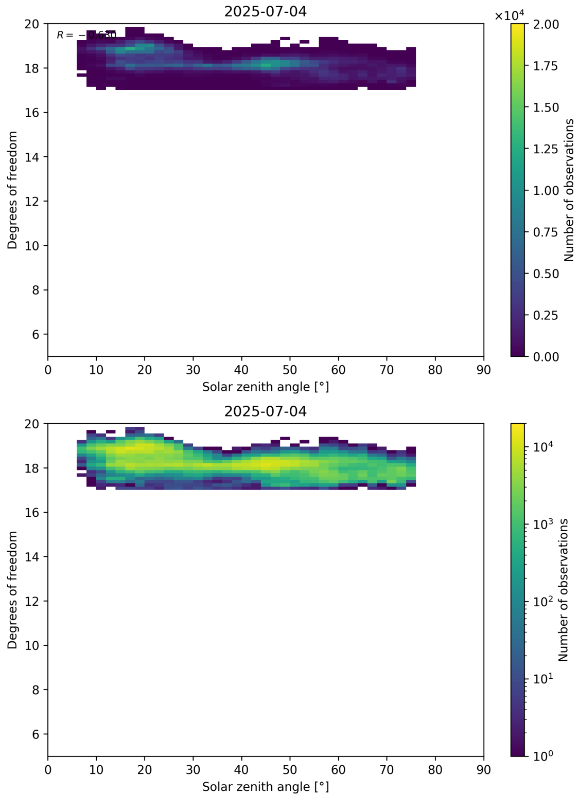
Figure 96: Scatter density plot of “Solar zenith angle” against “Degrees of freedom” for 2025-07-03 to 2025-07-05.
