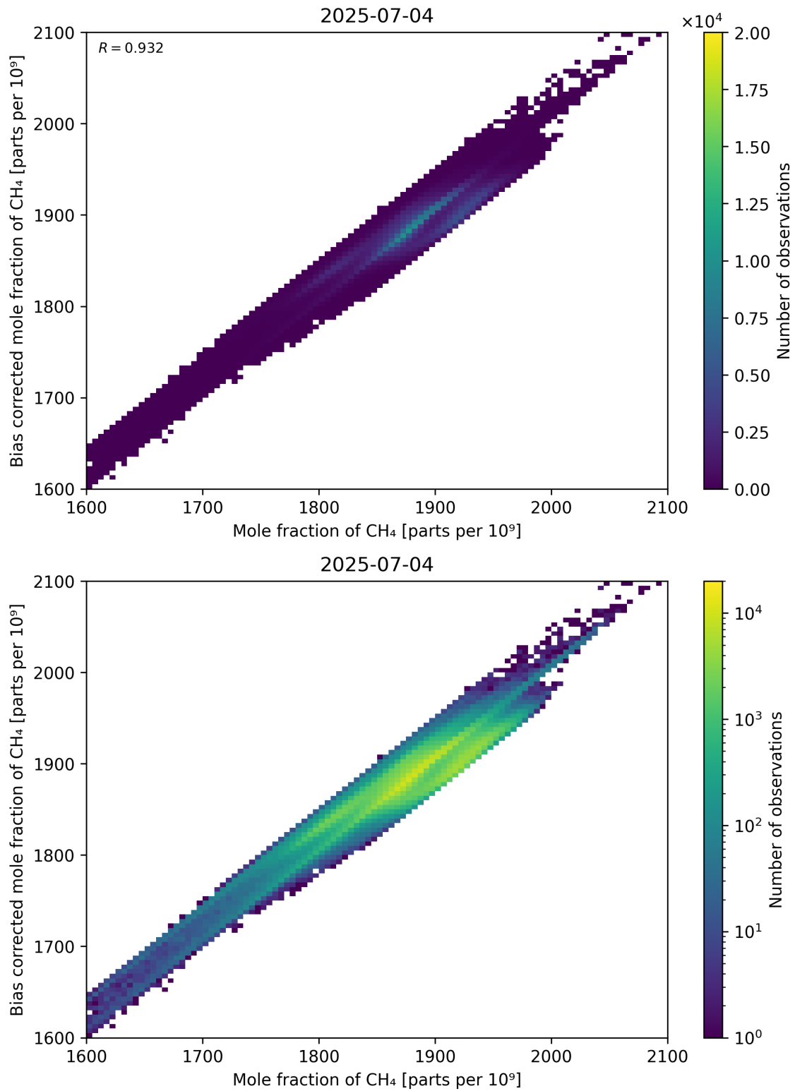
Figure 74: Scatter density plot of “Mole fraction of CH 4 ” against “Bias corrected mole fraction of CH 4 ” for 2025-07-03 to 2025-07-05.
