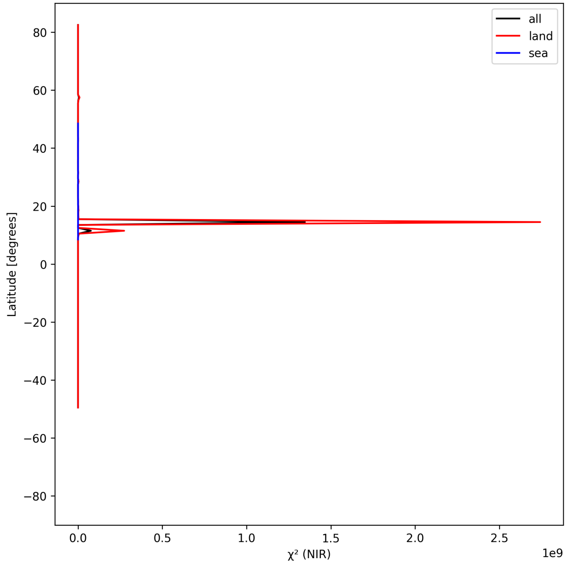
Figure 18: Zonal average of “ \chi^2 (NIR)” for 2025-07-03 to 2025-07-05.
