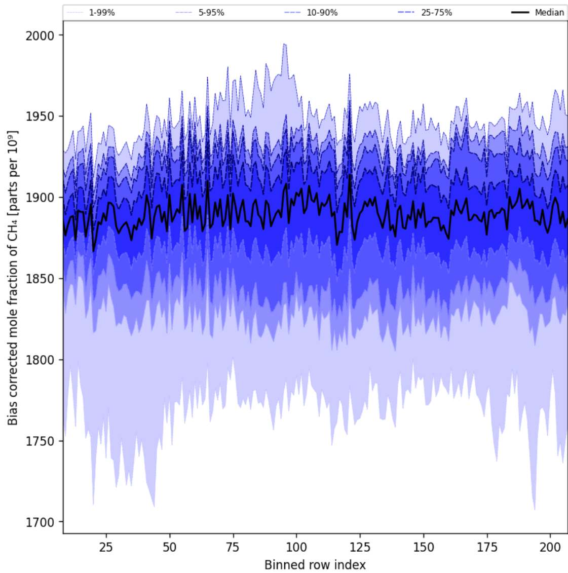
Figure 36: Along track statistics of “Bias corrected mole fraction of CH 4 ” for 2025-07-03 to 2025-07-05
