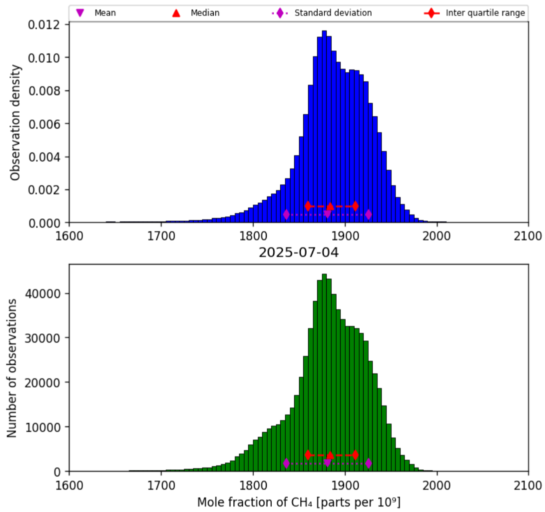
Figure 23: Histogram of “Mole fraction of CH 4 ” for 2025-07-03 to 2025-07-05
