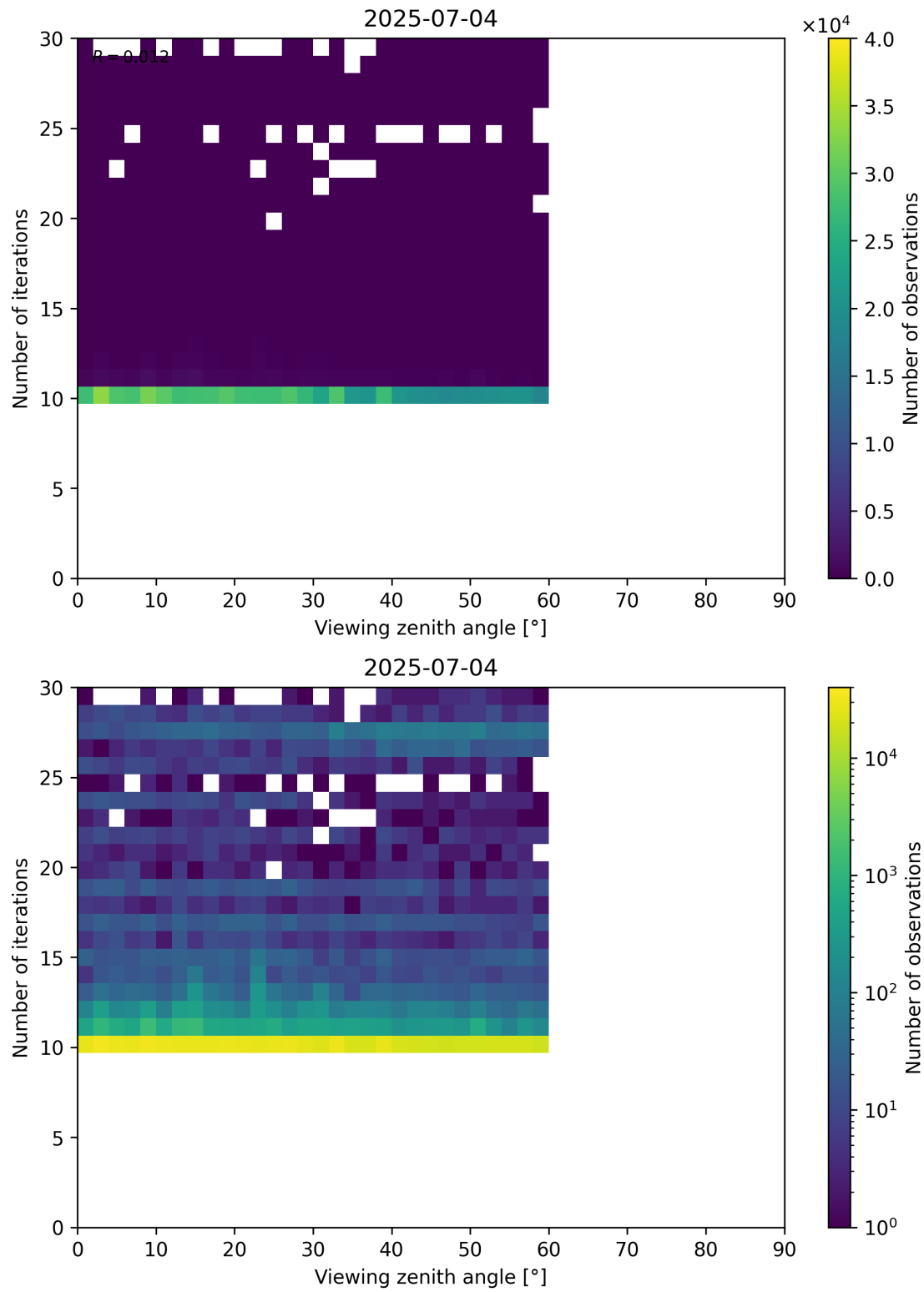
Figure 113: Scatter density plot of “Viewing zenith angle” against “Number of iterations” for 2025-07-03 to 2025-07-05.
