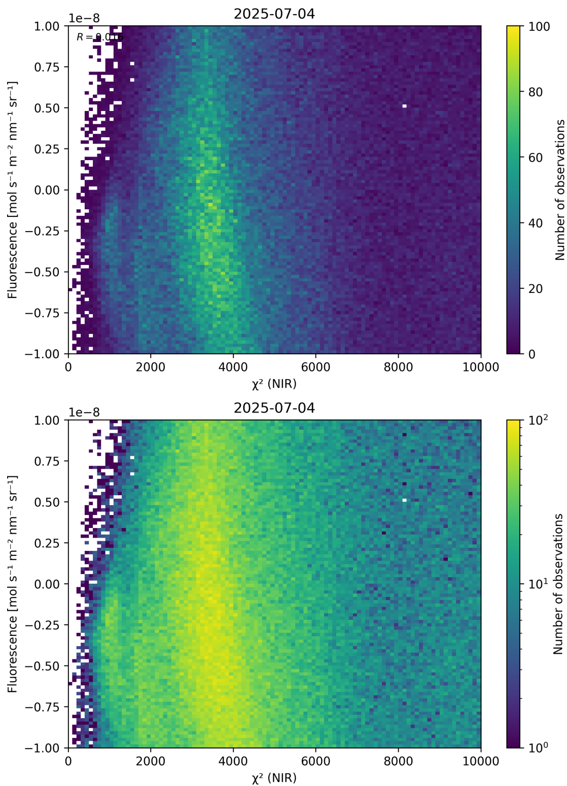
Figure 45: Scatter density plot of “ \chi^2 (NIR)” against “Fluorescence” for 2025-07-03 to 2025-07-05.
