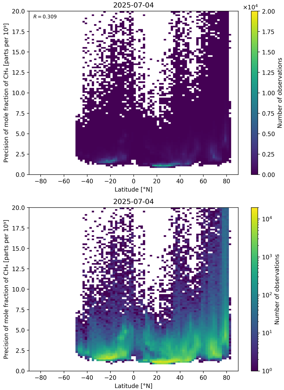
Figure 59: Scatter density plot of “Latitude” against “Precision of mole fraction of \text{CH}_4 ” for 2025-07-03 to 2025-07-05.
