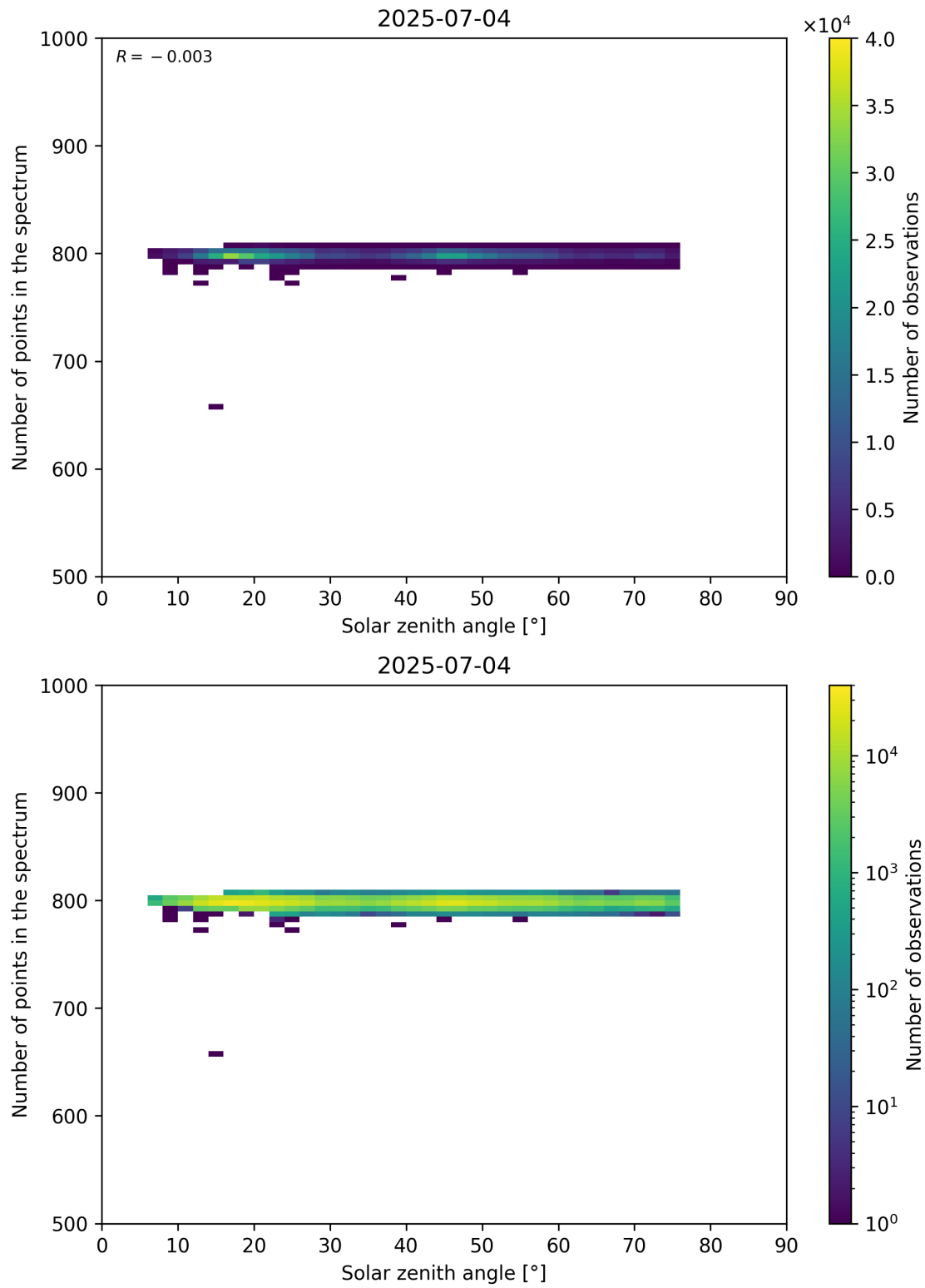
Figure 103: Scatter density plot of “Solar zenith angle” against “Number of points in the spectrum” for 2025-07-03 to 2025-07-05.
