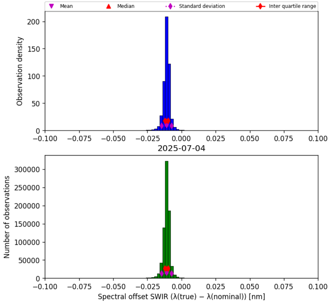
Figure 27: Histogram of “Spectral offset SWIR ( \lambda_{\text{true}} - \lambda_{\text{nominal}} )” for 2025-07-03 to 2025-07-05
