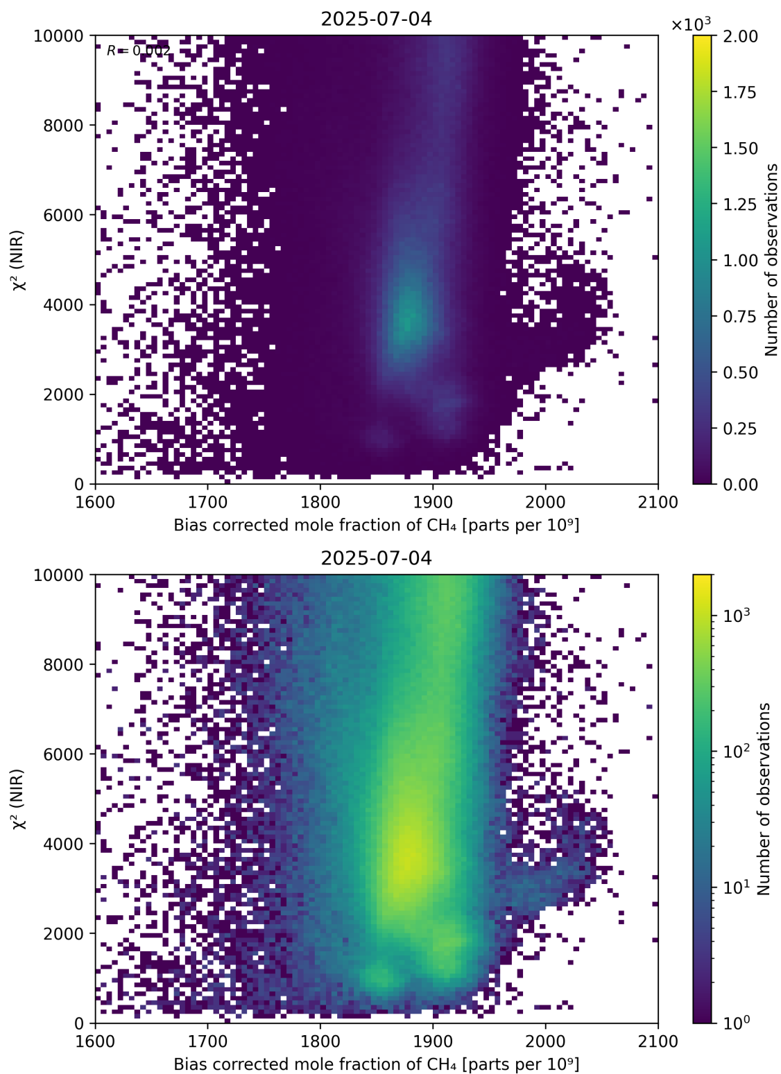
Figure 63: Scatter density plot of “Bias corrected mole fraction of CH 4 ” against “ \chi^2 (NIR)” for 2025-07-03 to 2025-07-05.
