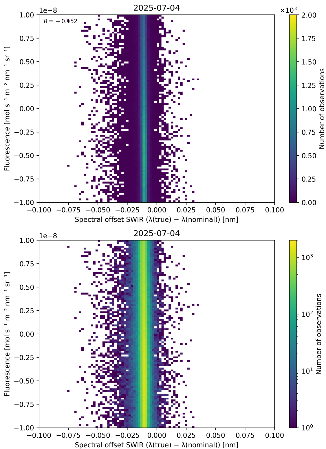
Figure 120: Scatter density plot of “Spectral offset SWIR ( \lambda_{\text{true}} - \lambda_{\text{nominal}} )” against “Fluorescence” for 2025-07-03 to 2025-07-05.
