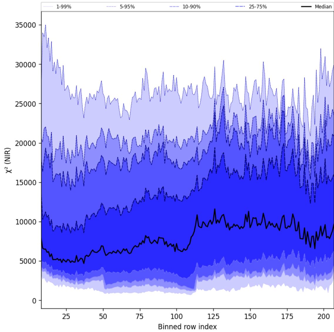
Figure 40: Along track statistics of “ \chi^2 (NIR)” for 2025-07-03 to 2025-07-05
