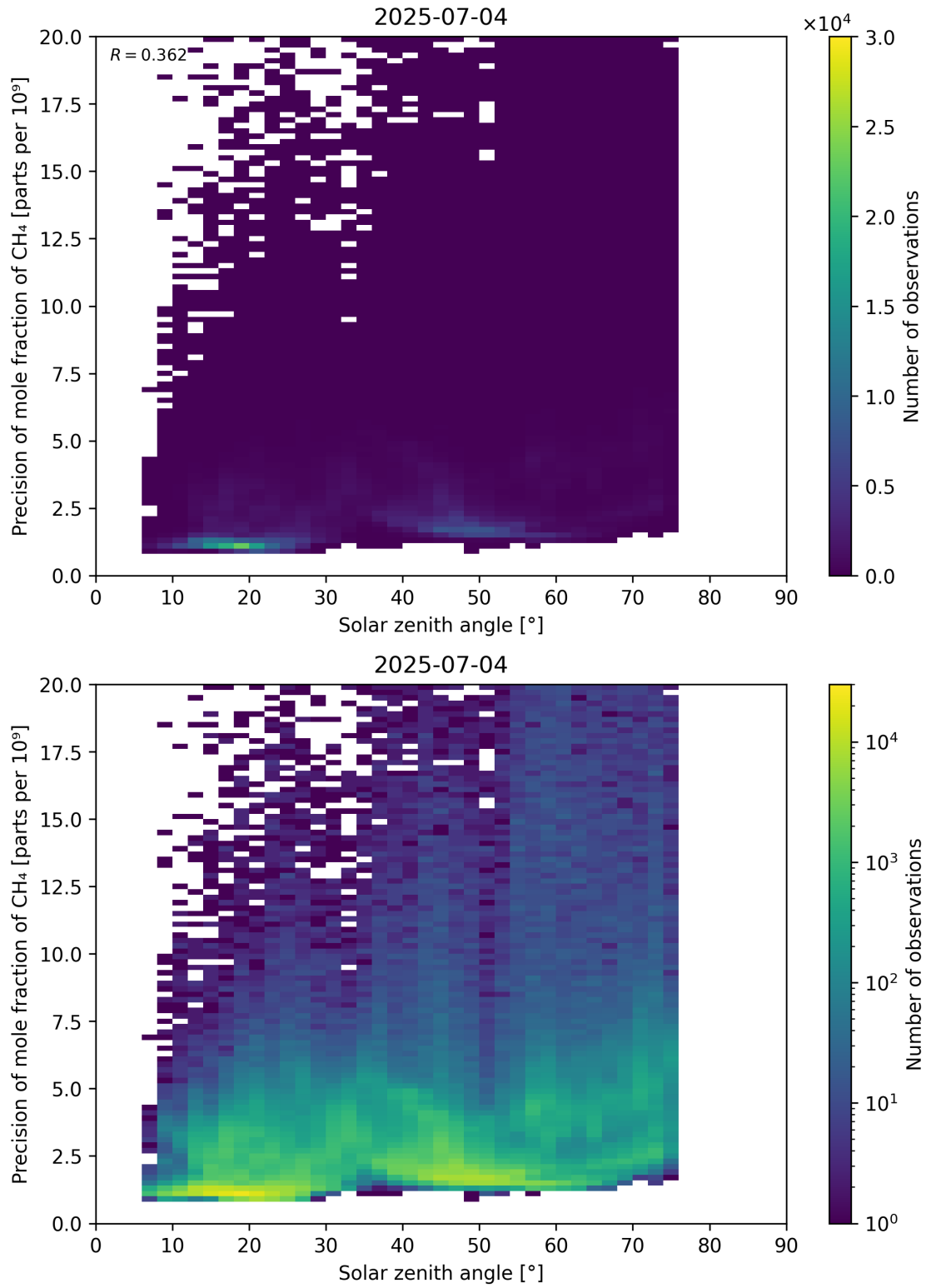
Figure 101: Scatter density plot of “Solar zenith angle” against “Precision of mole fraction of CH 4 ” for 2025-07-03 to 2025-07-05.
