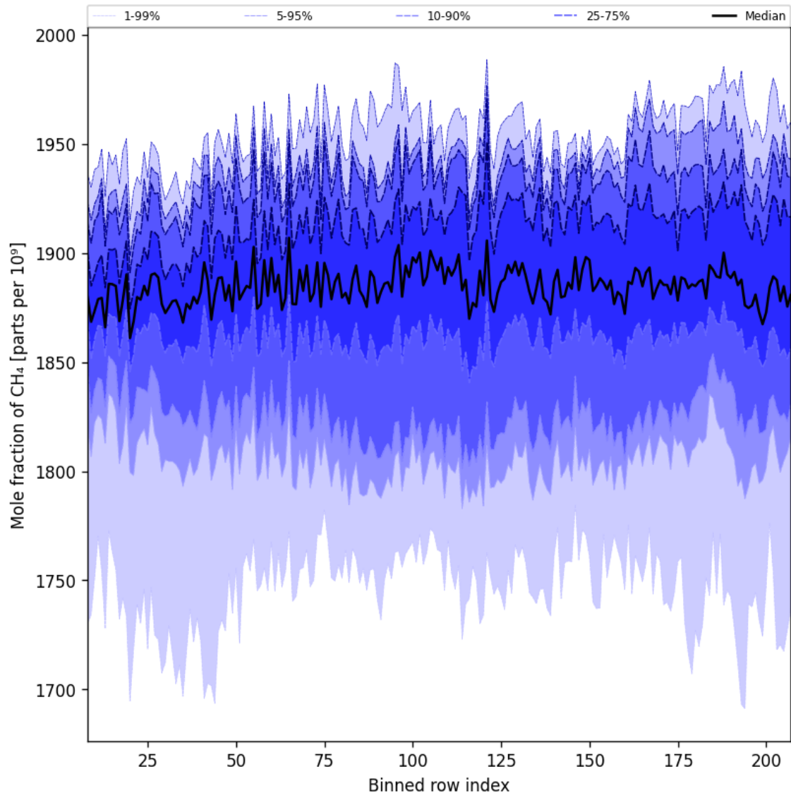
Figure 34: Along track statistics of “Mole fraction of CH 4 ” for 2025-07-03 to 2025-07-05
