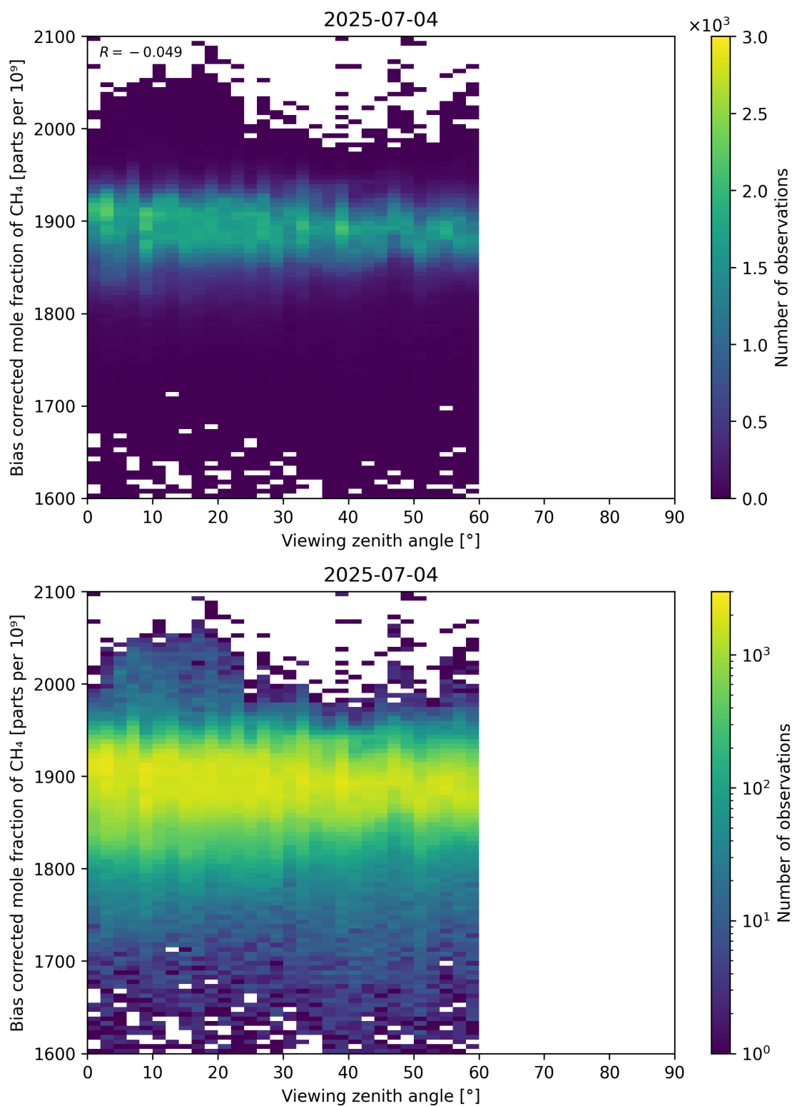
Figure 111: Scatter density plot of “Viewing zenith angle” against “Bias corrected mole fraction of CH 4 ” for 2025-07-03 to 2025-07-05.
