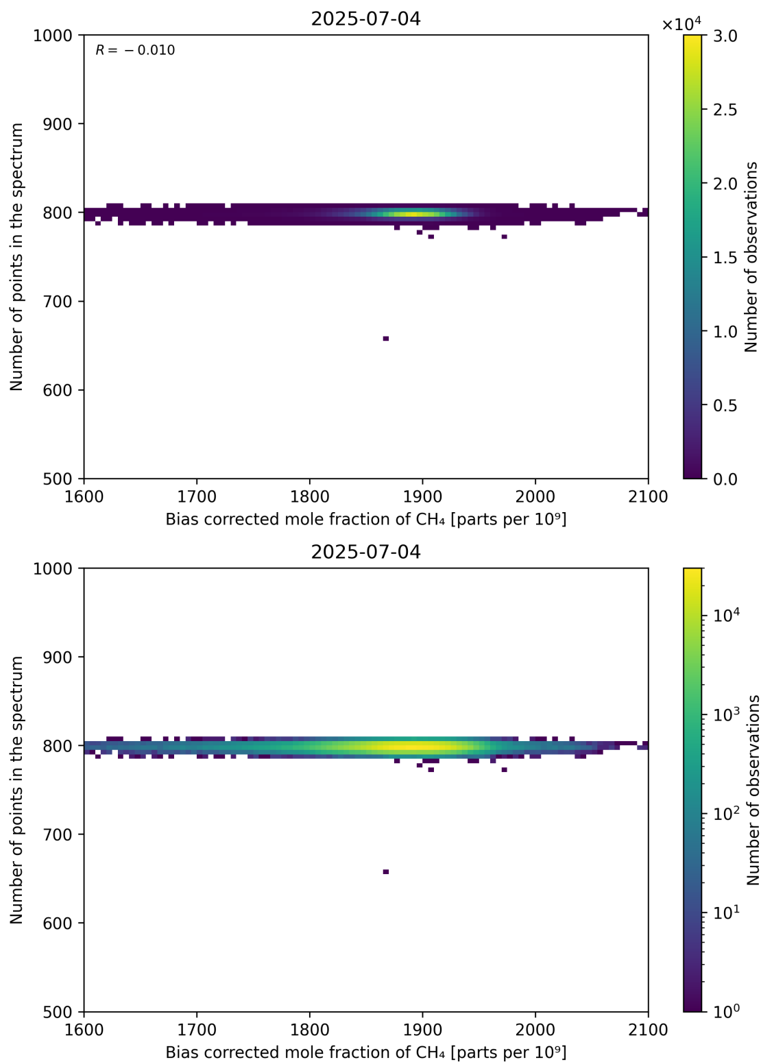
Figure 68: Scatter density plot of “Bias corrected mole fraction of CH 4 ” against “Number of points in the spectrum” for 2025-07-03 to 2025-07-05.
