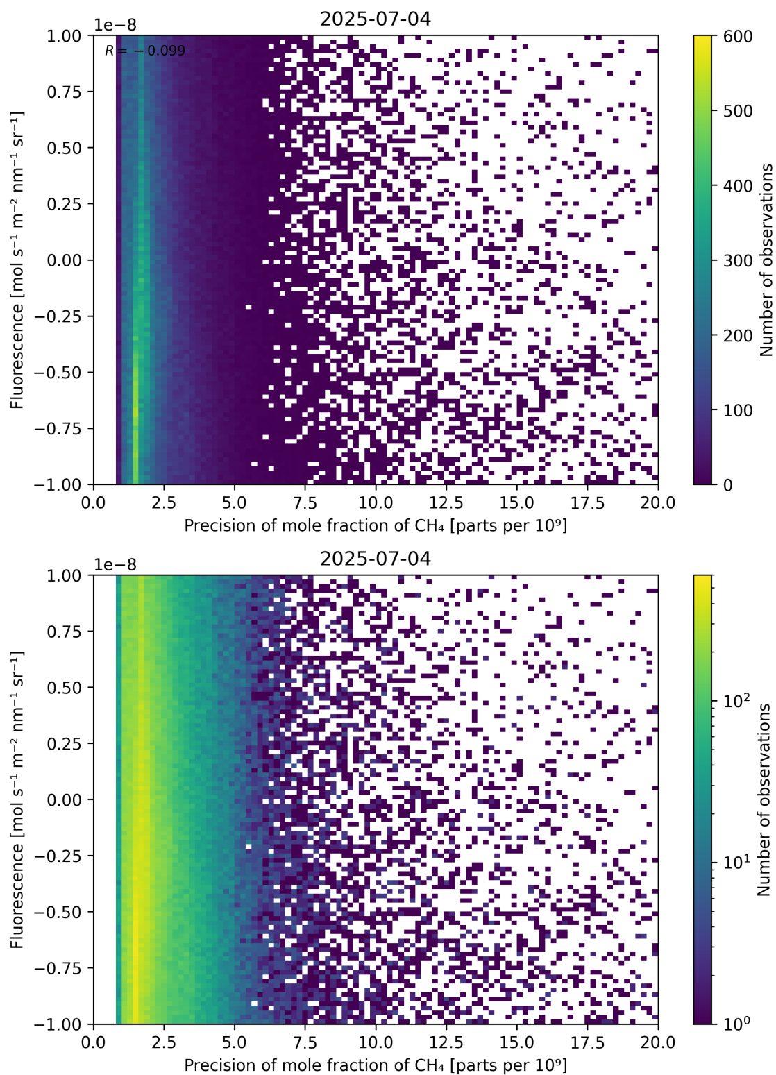
Figure 81: Scatter density plot of “Precision of mole fraction of \text{CH}_4 ” against “Fluorescence” for 2025-07-03 to 2025-07-05.
