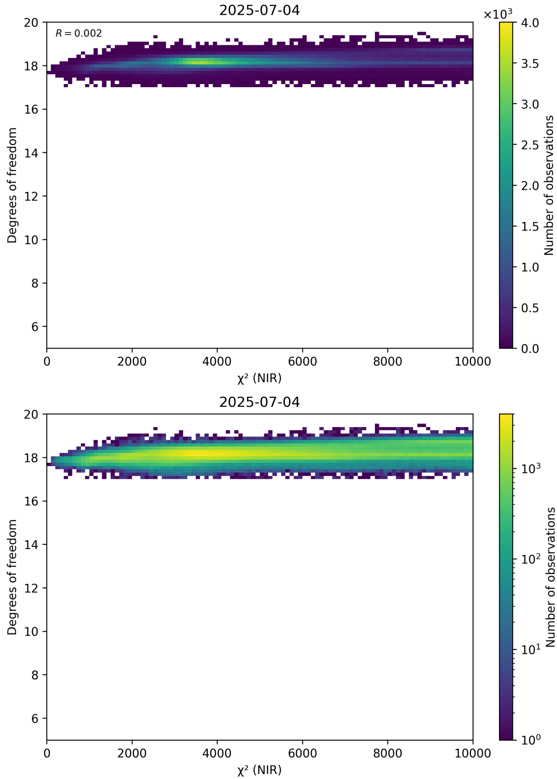
Figure 44: Scatter density plot of “ \chi^2 (NIR)” against “Degrees of freedom” for 2025-07-03 to 2025-07-05.
