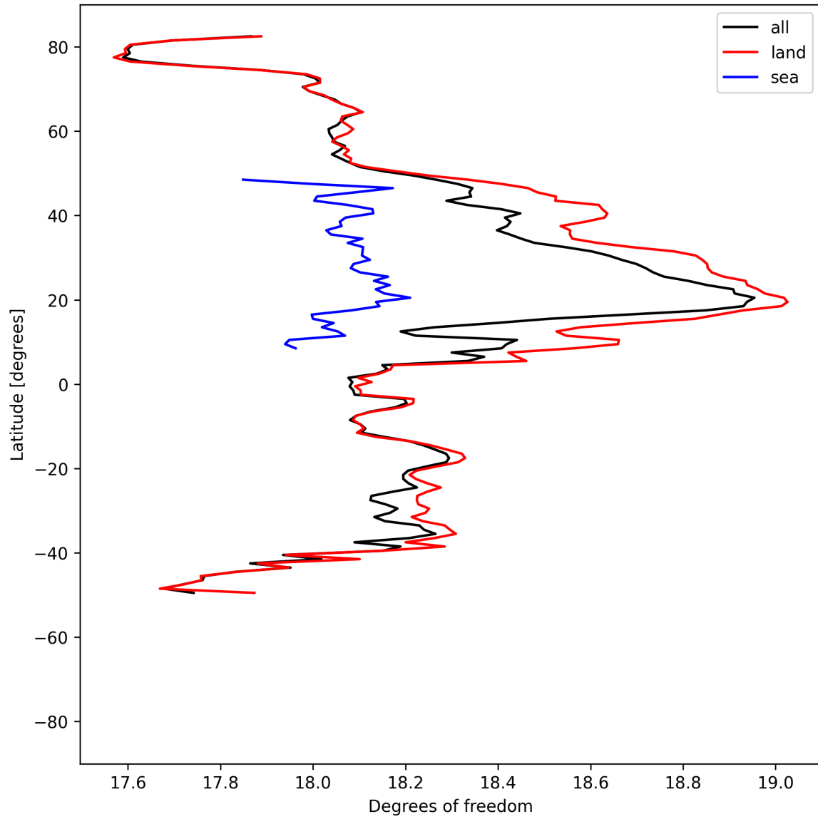
Figure 19: Zonal average of “Degrees of freedom” for 2025-07-03 to 2025-07-05.
