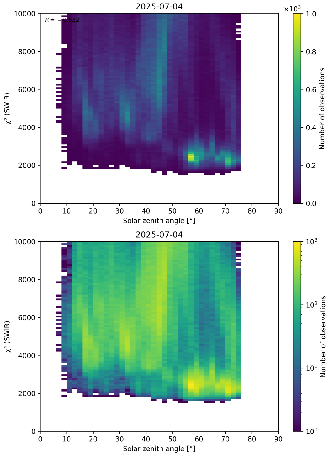
Figure 95: Scatter density plot of “Solar zenith angle” against “ \chi^2 (SWIR)” for 2025-07-03 to 2025-07-05.
