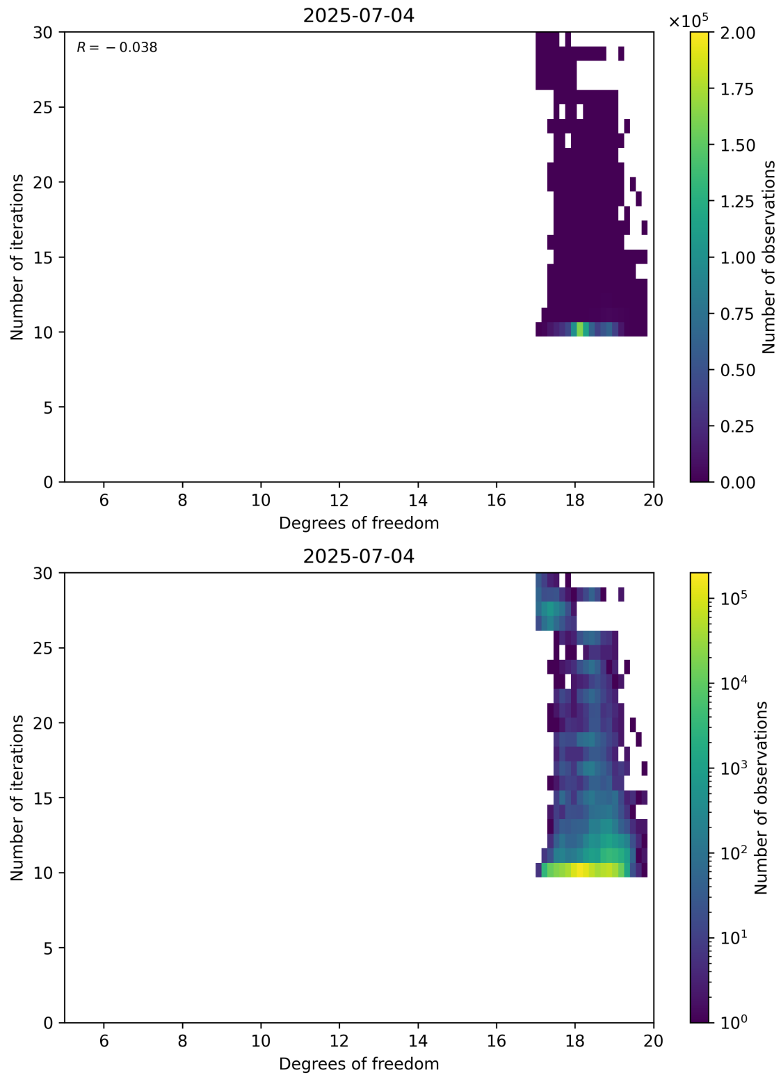
Figure 52: Scatter density plot of “Degrees of freedom” against “Number of iterations” for 2025-07-03 to 2025-07-05.
