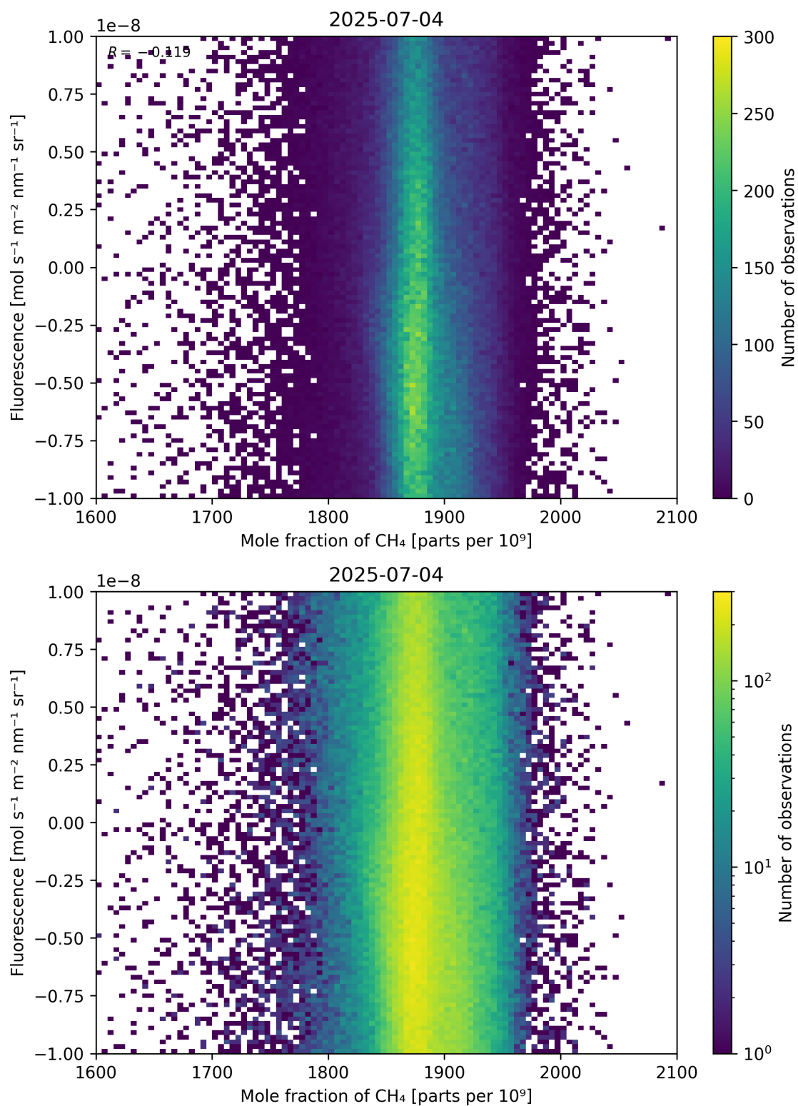
Figure 73: Scatter density plot of “Mole fraction of \text{CH}_4 ” against “Fluorescence” for 2025-07-03 to 2025-07-05.
