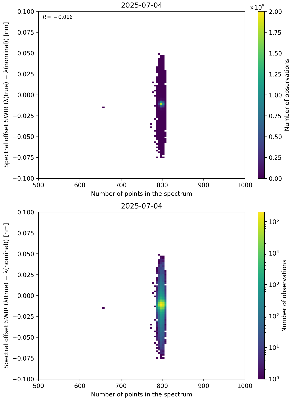
Figure 93: Scatter density plot of “Number of points in the spectrum” against “Spectral offset SWIR ( \lambda_{\text{true}} - \lambda_{\text{nominal}} )” for 2025-07-03 to 2025-07-05.
