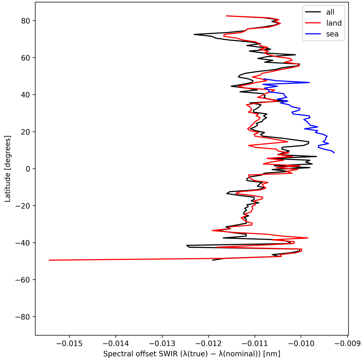
Figure 16: Zonal average of “Spectral offset SWIR ( \lambda_{\text{true}} - \lambda_{\text{nominal}} )” for 2025-07-03 to 2025-07-05.
