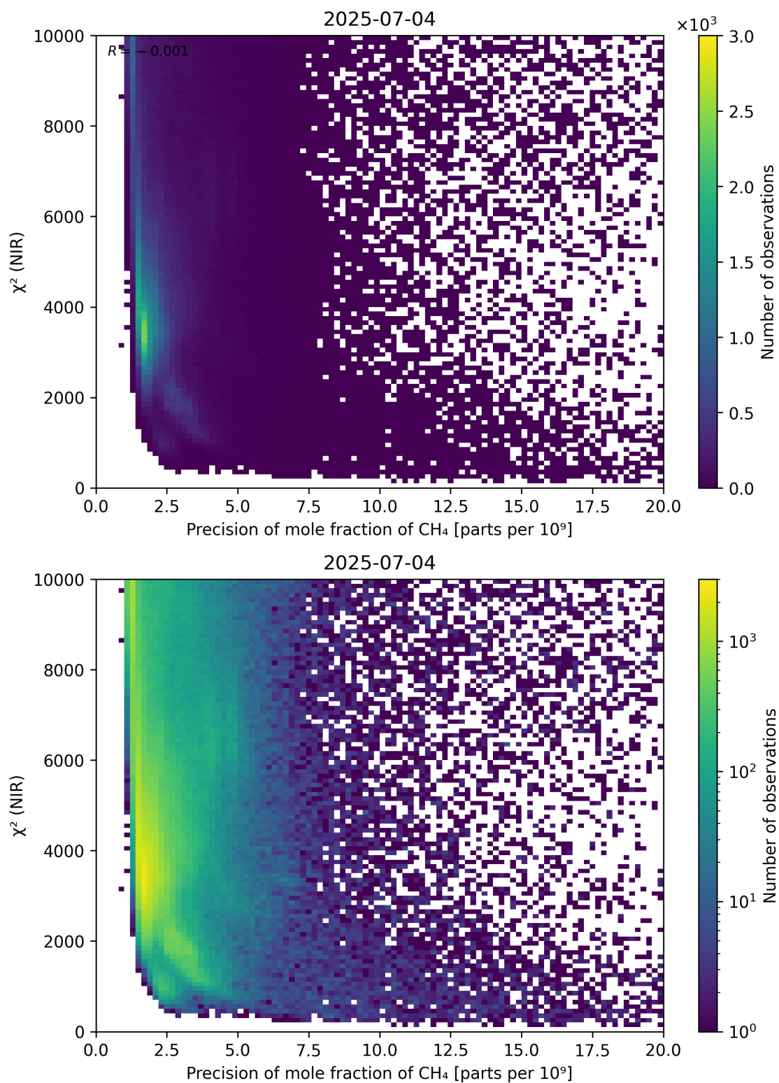
Figure 78: Scatter density plot of “Precision of mole fraction of \text{CH}_4 ” against “ \chi^2 (NIR)” for 2025-07-03 to 2025-07-05.
