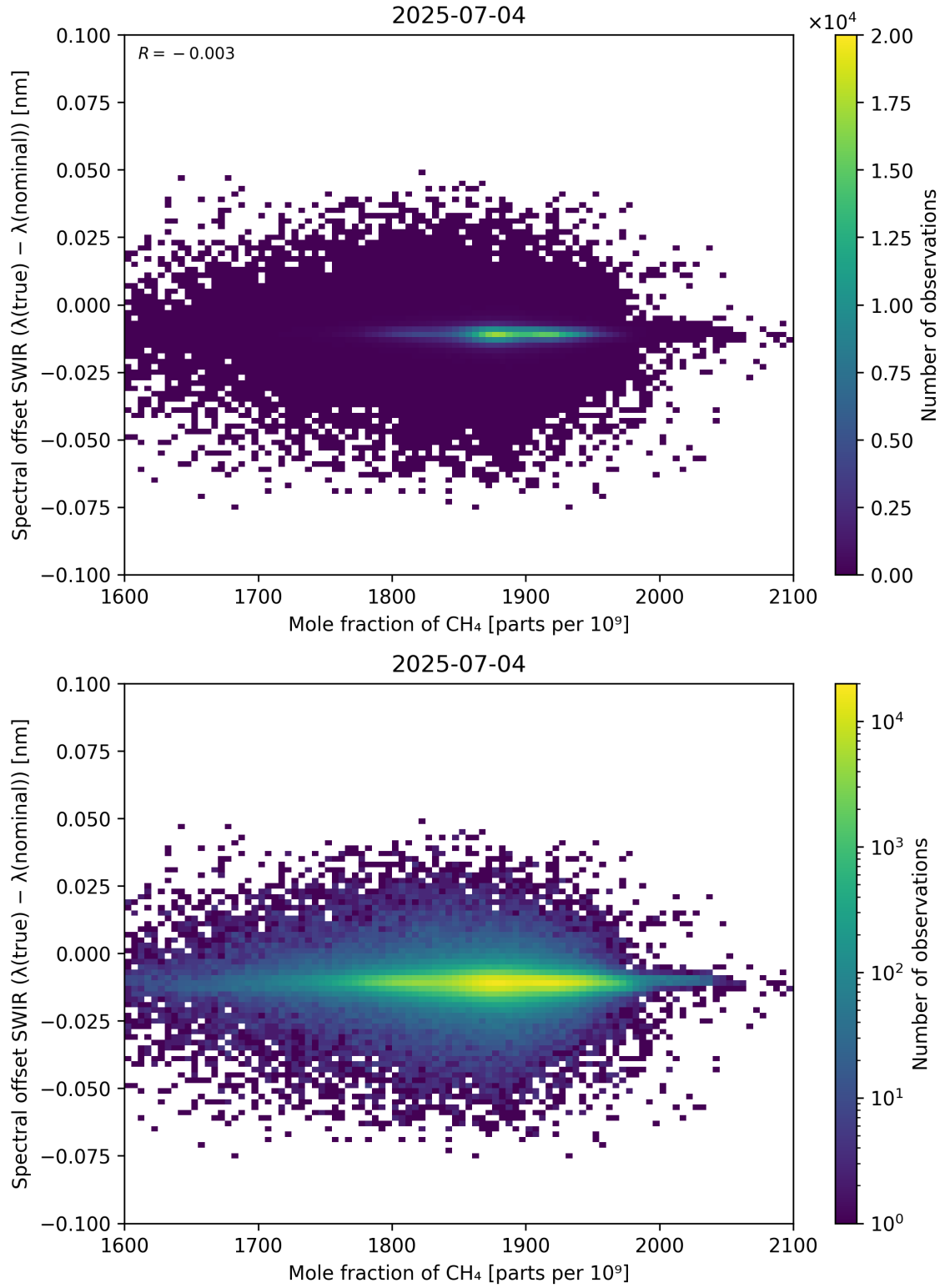
Figure 86: Scatter density plot of “Mole fraction of CH 4 ” against “Spectral offset SWIR ( \lambda_{\text{true}} - \lambda_{\text{nominal}} )” for 2025-07-03 to 2025-07-05.
