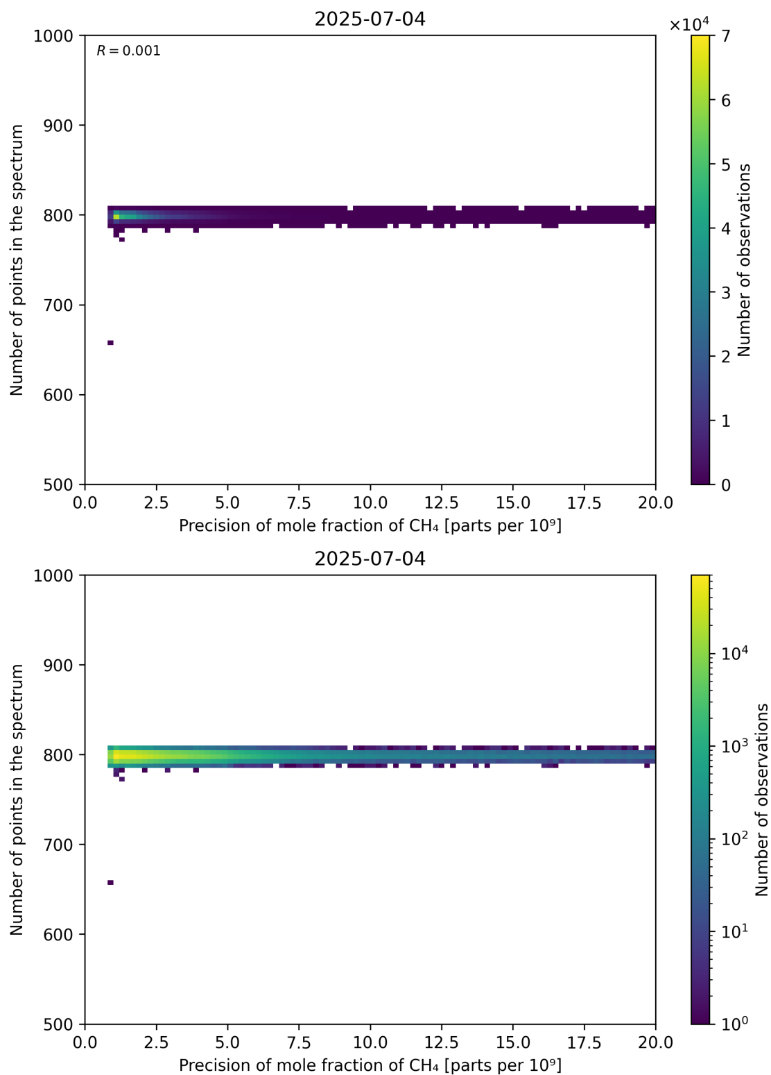
Figure 84: Scatter density plot of “Precision of mole fraction of CH 4 ” against “Number of points in the spectrum” for 2025-07-03 to 2025-07-05.
