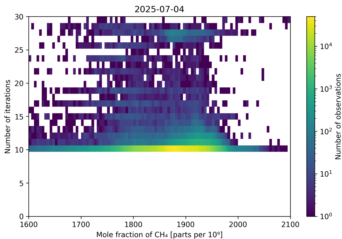
Figure 76: Scatter density plot of “Mole fraction of CH 4 ” against “Number of iterations” for 2025-07-03 to 2025-07-05.
