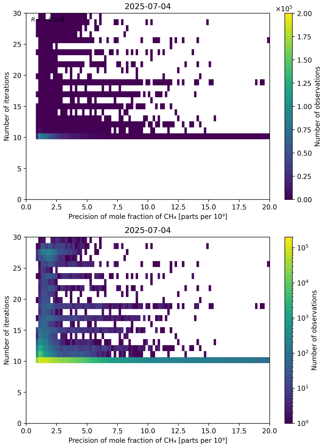
Figure 83: Scatter density plot of “Precision of mole fraction of CH 4 ” against “Number of iterations” for 2025-07-03 to 2025-07-05.
