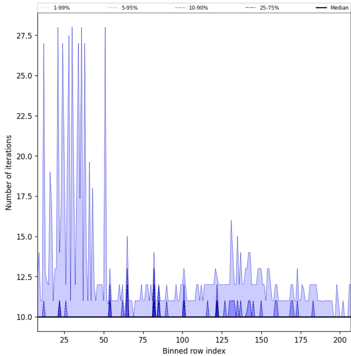
Figure 42: Along track statistics of “Number of iterations” for 2025-07-03 to 2025-07-05
