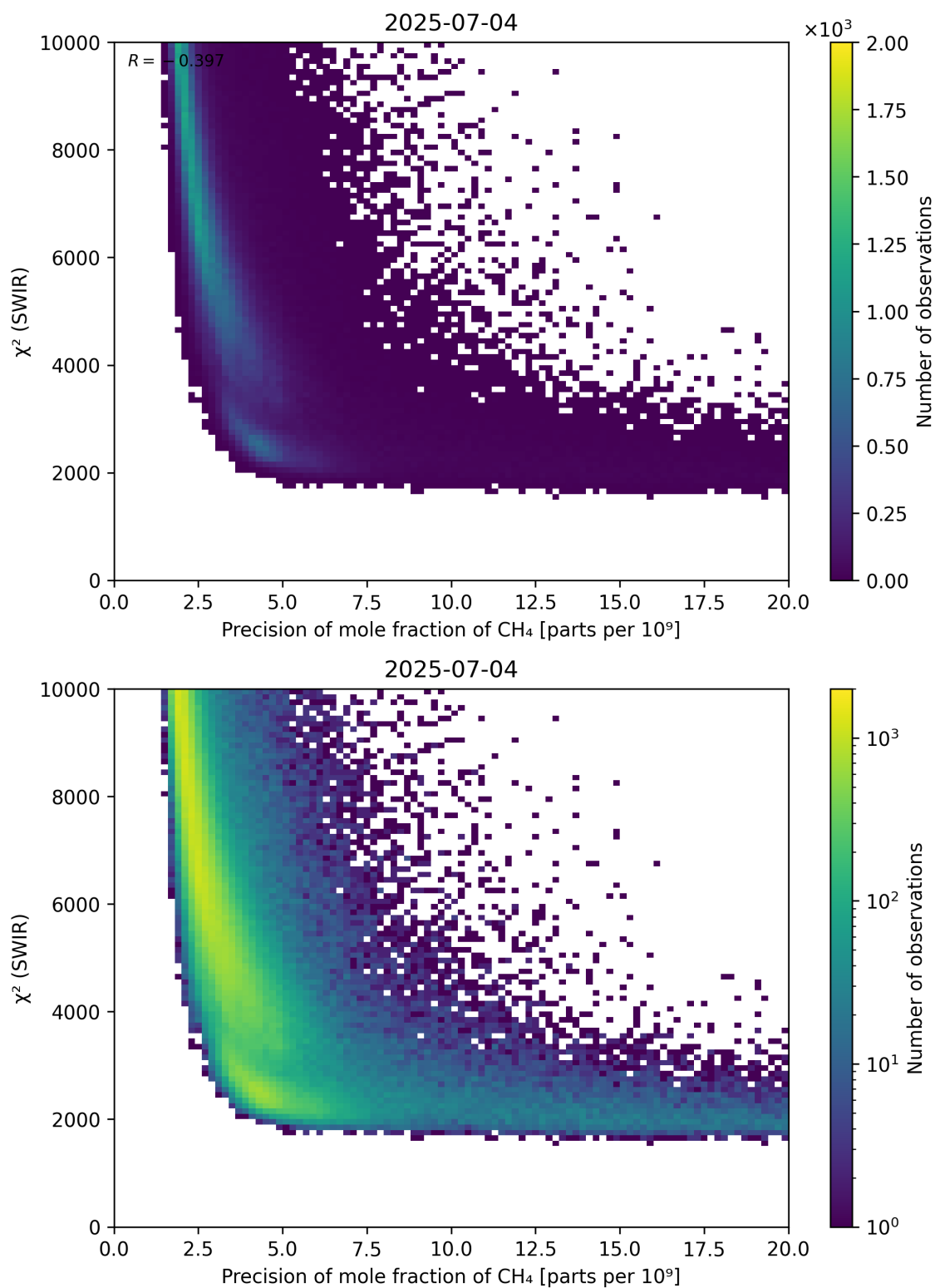
Figure 79: Scatter density plot of “Precision of mole fraction of \text{CH}_4 ” against “ \chi^2 (SWIR)” for 2025-07-03 to 2025-07-05.
