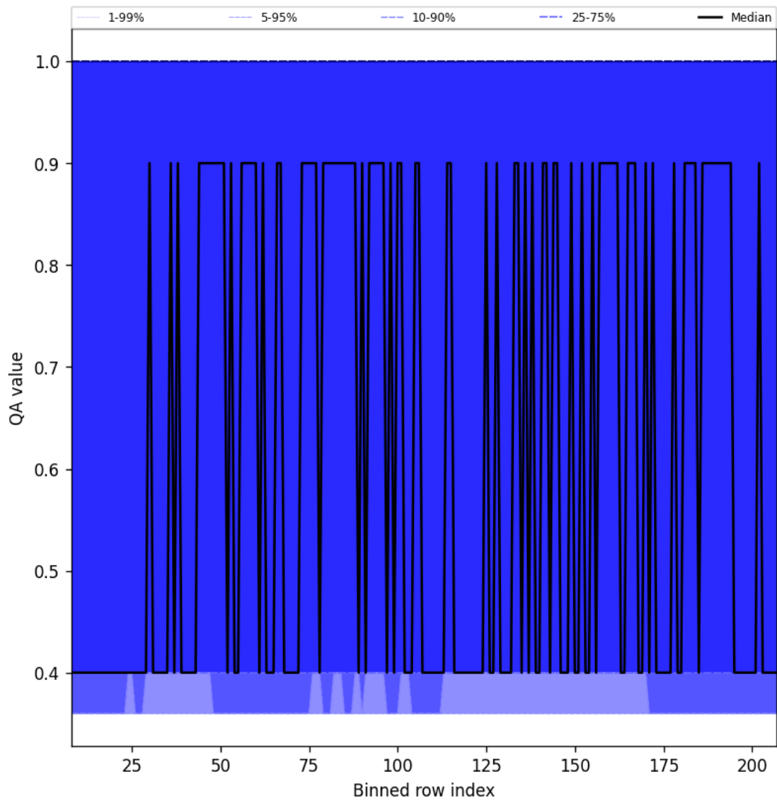
Figure 33: Along track statistics of “QA value” for 2025-07-03 to 2025-07-05
