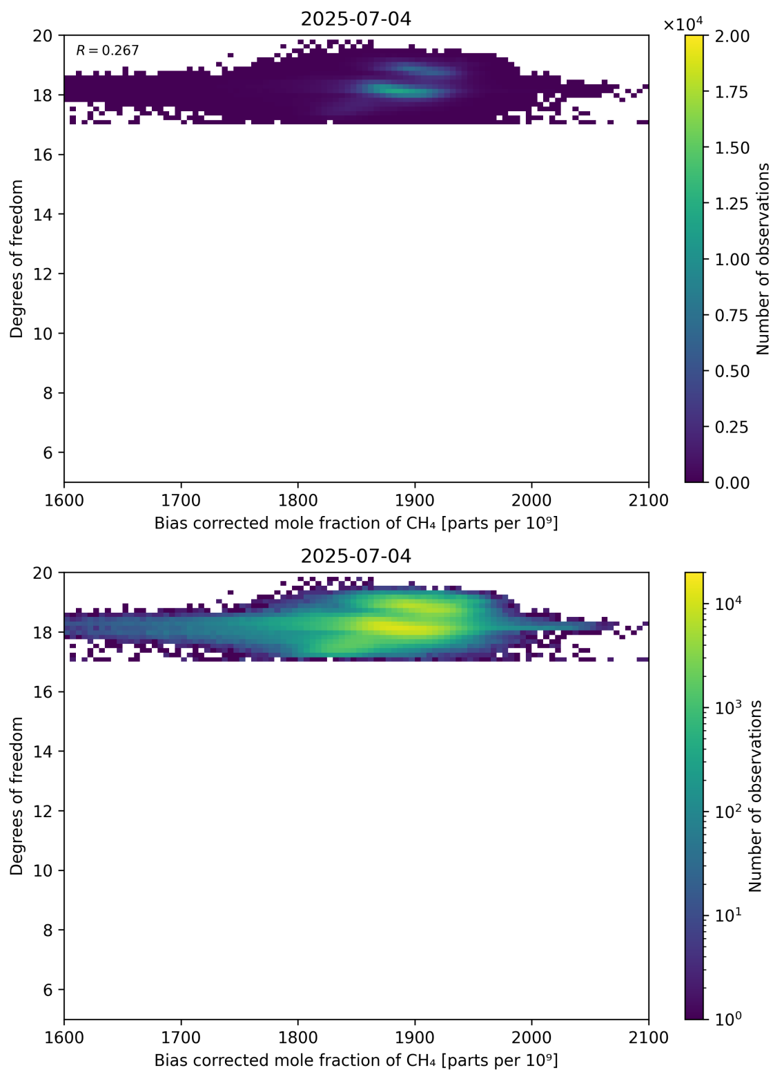
Figure 65: Scatter density plot of “Bias corrected mole fraction of CH 4 ” against “Degrees of freedom” for 2025-07-03 to 2025-07-05.
