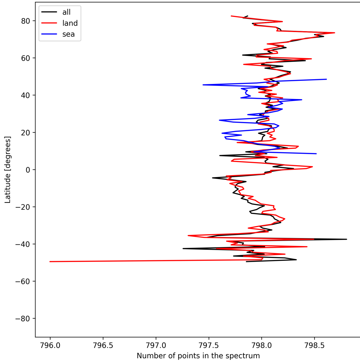
Figure 15: Zonal average of “Number of points in the spectrum” for 2025-07-03 to 2025-07-05.
