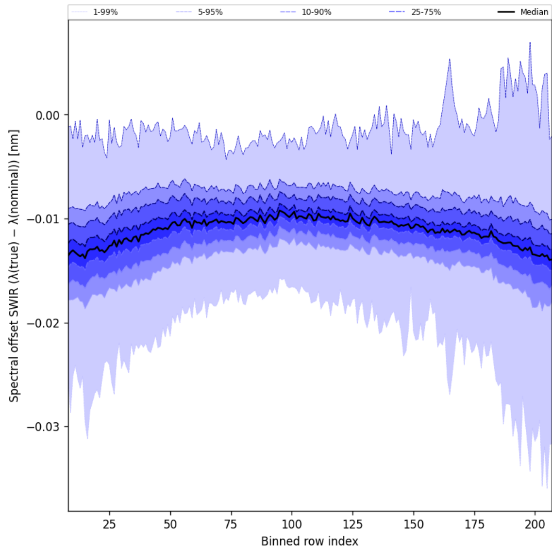
Figure 38: Along track statistics of “Spectral offset SWIR ( \lambda_{\text{true}} - \lambda_{\text{nominal}} )” for 2025-07-03 to 2025-07-05
