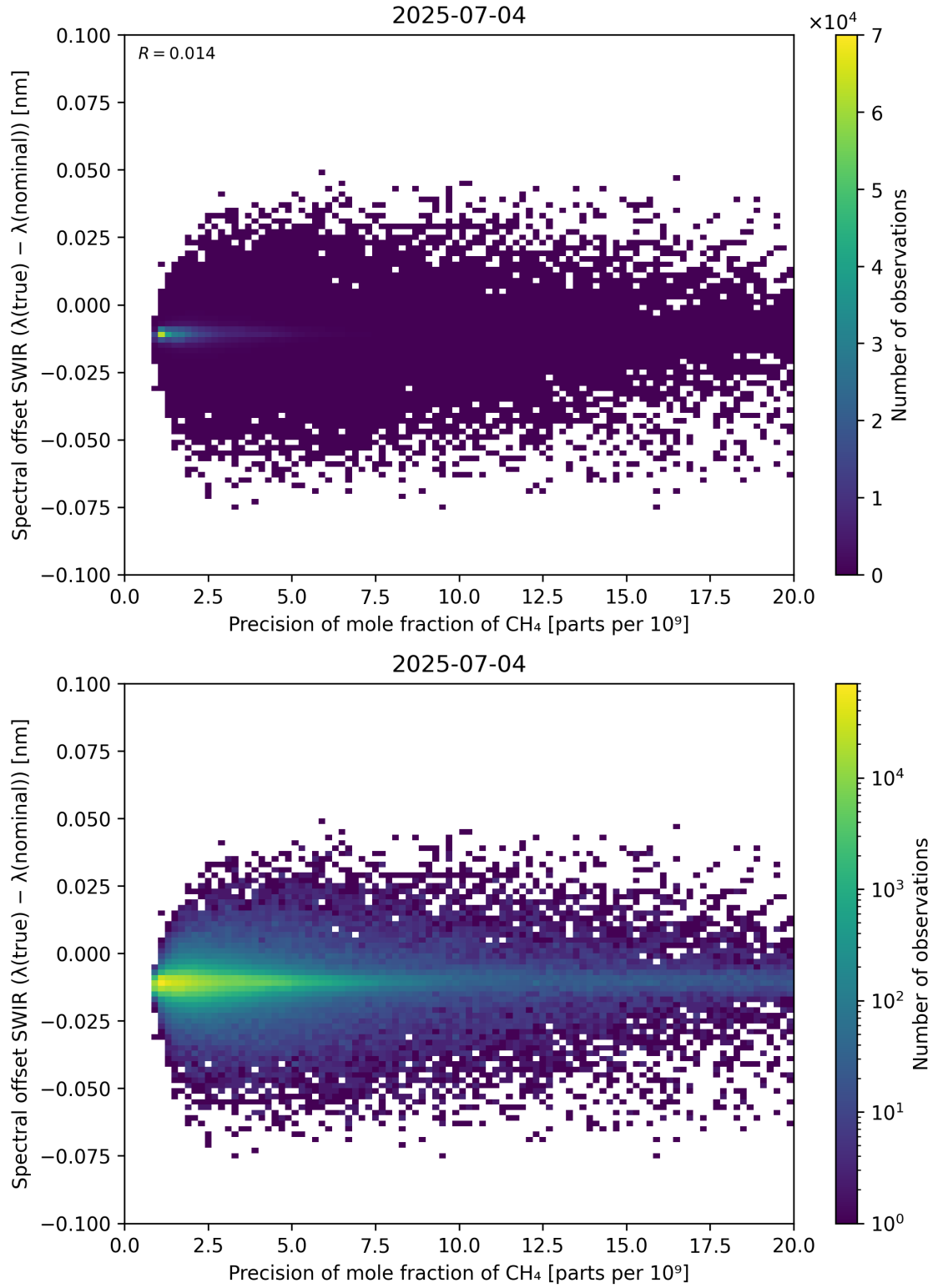
Figure 85: Scatter density plot of “Precision of mole fraction of CH 4 ” against “Spectral offset SWIR ( \lambda_{\text{true}} - \lambda_{\text{nominal}} )” for 2025-07-03 to 2025-07-05.
