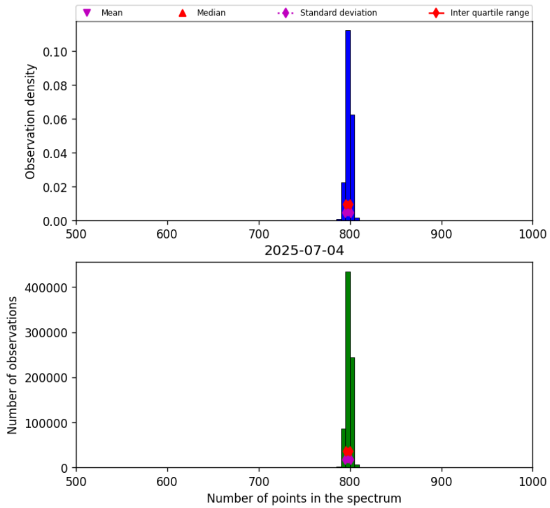
Figure 26: Histogram of “Number of points in the spectrum” for 2025-07-03 to 2025-07-05
