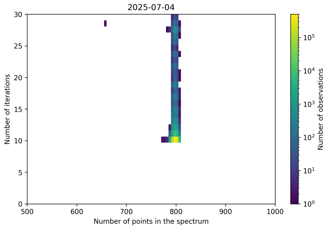
Figure 92: Scatter density plot of “Number of points in the spectrum” against “Number of iterations” for 2025-07-03 to 2025-07-05.
