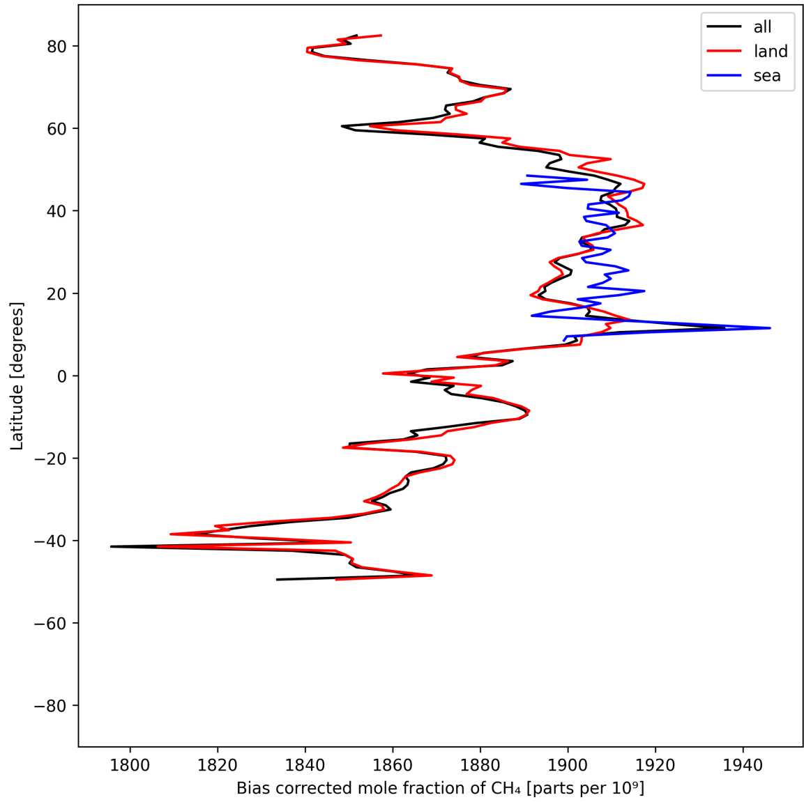
Figure 14: Zonal average of “Bias corrected mole fraction of \text{CH}_4 ” for 2025-07-03 to 2025-07-05.
