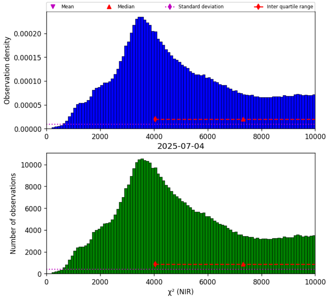
Figure 29: Histogram of " \chi^2 (NIR)" for 2025-07-03 to 2025-07-05
