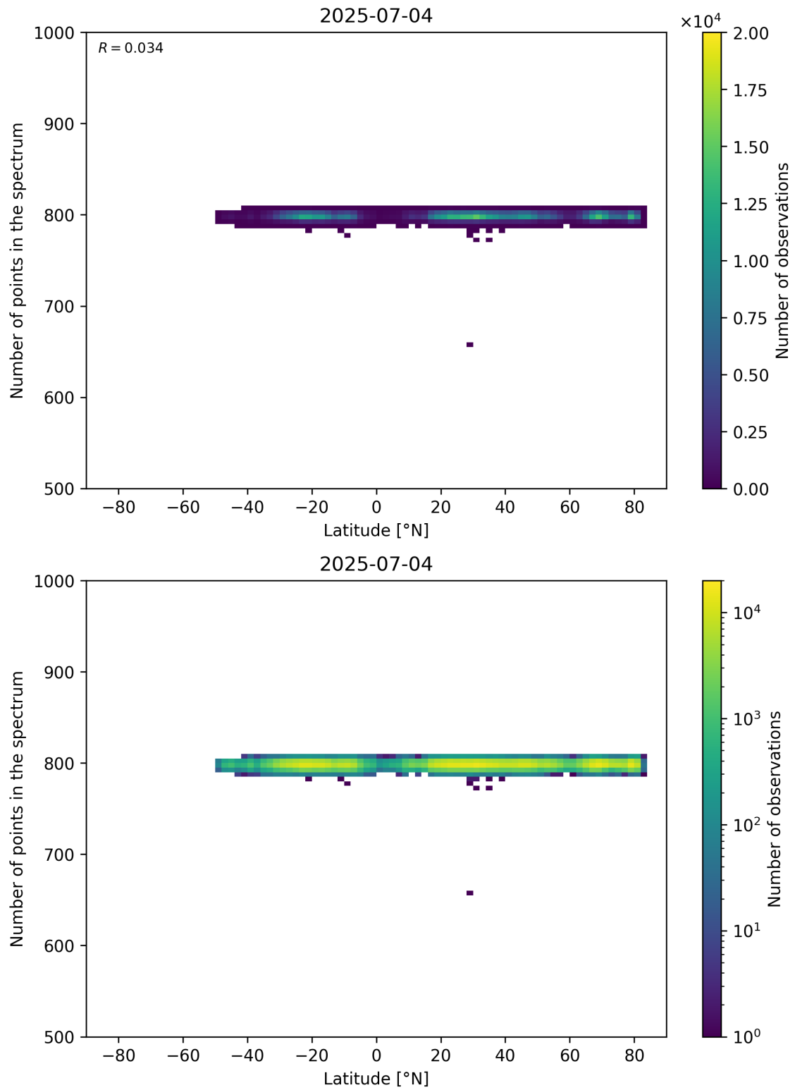
Figure 61: Scatter density plot of “Latitude” against “Number of points in the spectrum” for 2025-07-03 to 2025-07-05.
