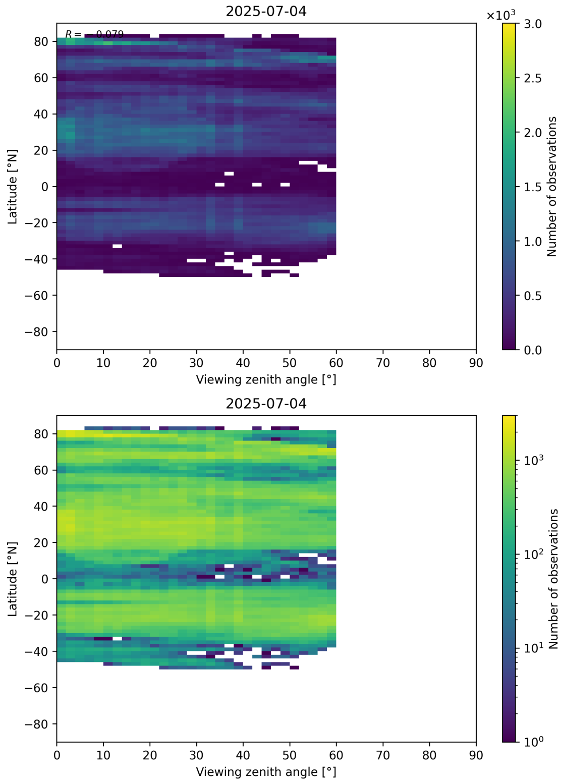
Figure 109: Scatter density plot of “Viewing zenith angle” against “Latitude” for 2025-07-03 to 2025-07-05.
