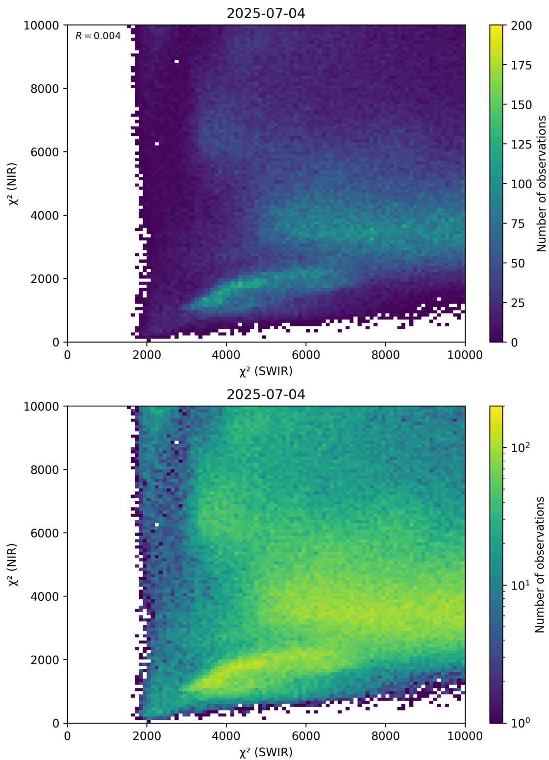
Figure 47: Scatter density plot of “ \chi^2 (SWIR)” against “ \chi^2 (NIR)” for 2025-07-03 to 2025-07-05.
