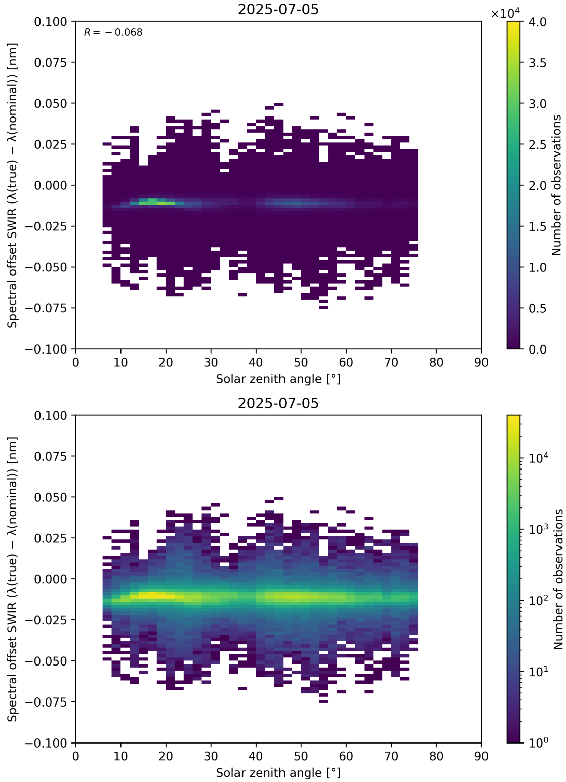
Figure 104: Scatter density plot of “Solar zenith angle” against “Spectral offset SWIR ( \lambda_{\text{true}} - \lambda_{\text{nominal}} )” for 2025-07-04 to 2025-07-06.
