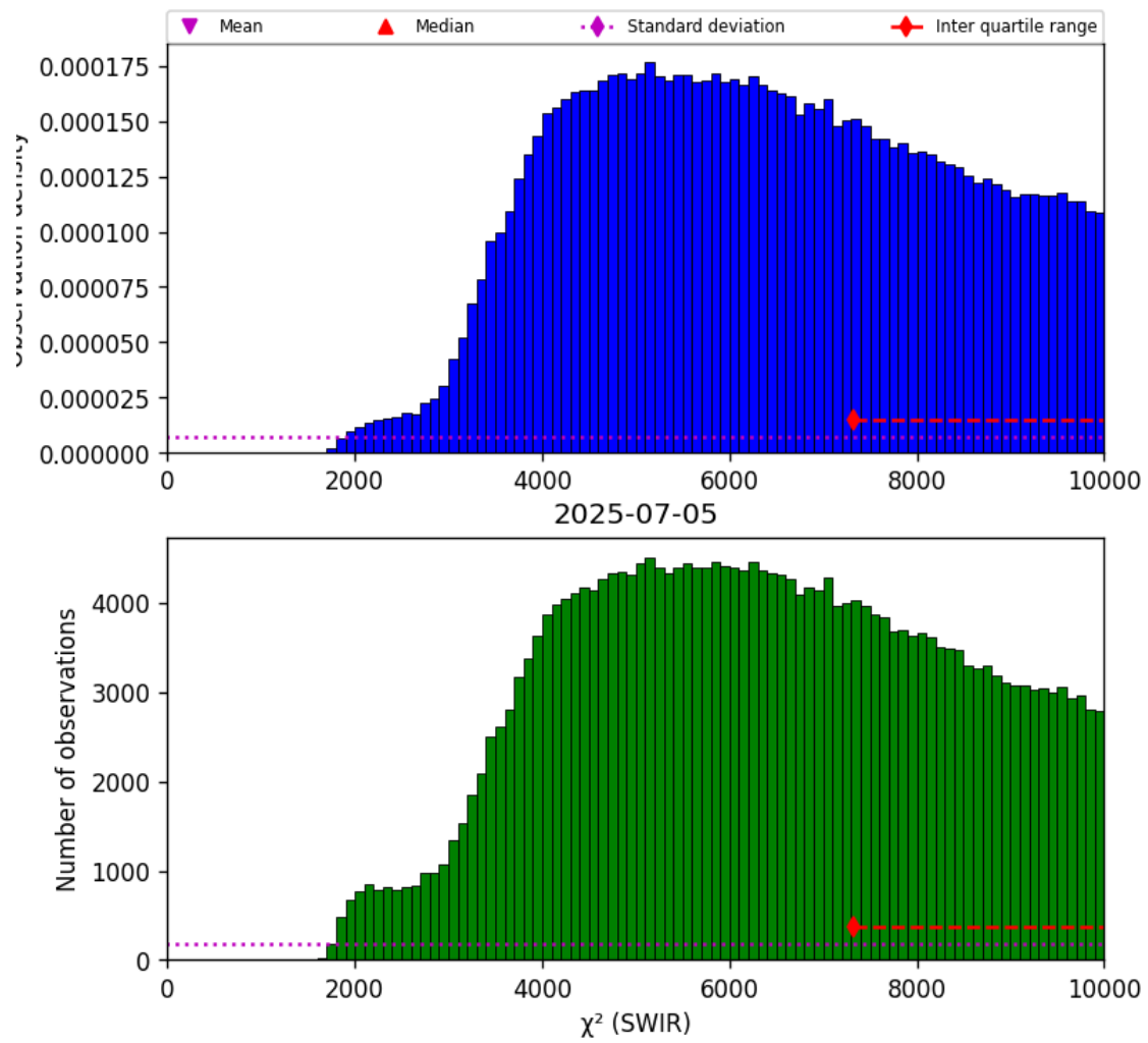
Figure 28: Histogram of “ \chi^2 (SWIR)” for 2025-07-04 to 2025-07-06
