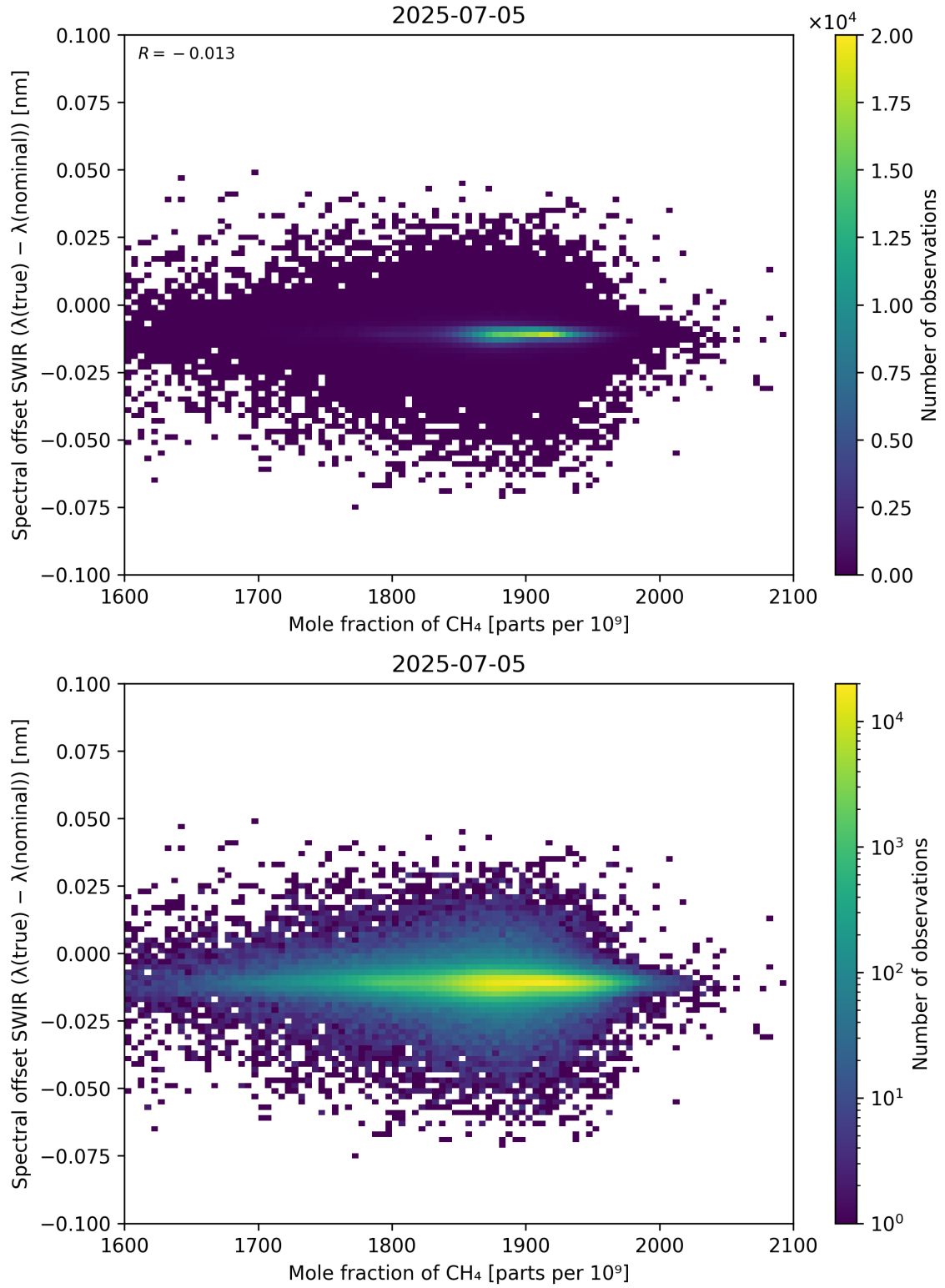
Figure 86: Scatter density plot of “Mole fraction of CH 4 ” against “Spectral offset SWIR ( \lambda_{\text{true}} - \lambda_{\text{nominal}} )” for 2025-07-04 to 2025-07-06.
