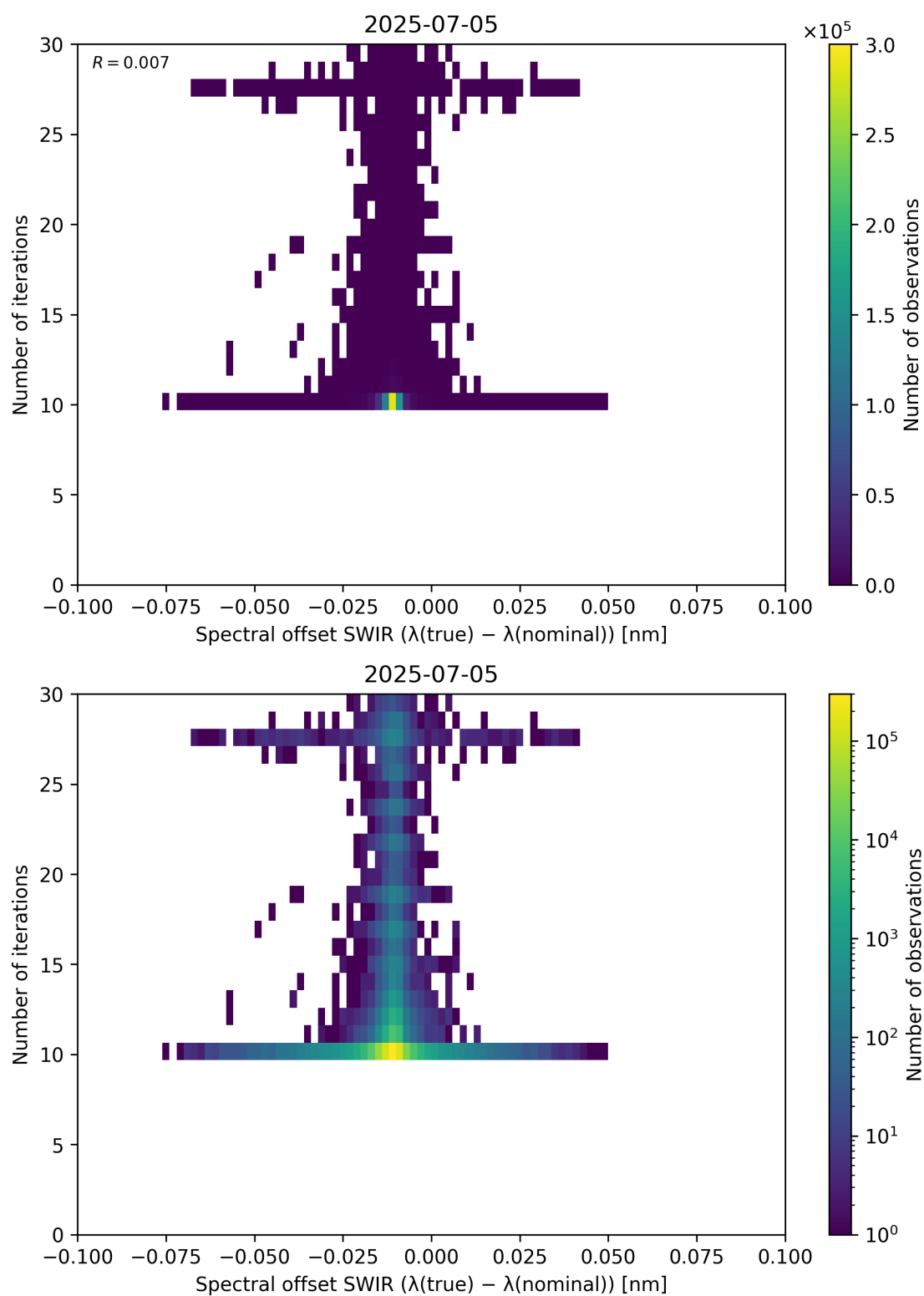
Figure 121: Scatter density plot of “Spectral offset SWIR ( \lambda_{\text{true}} - \lambda_{\text{nominal}} )” against “Number of iterations” for 2025-07-04 to 2025-07-06.
