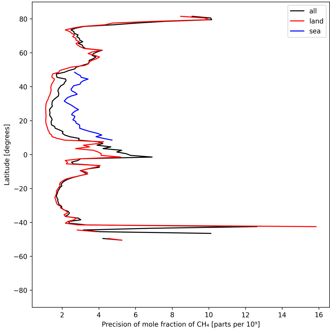
Figure 13: Zonal average of “Precision of mole fraction of CH 4 ” for 2025-07-04 to 2025-07-06.
