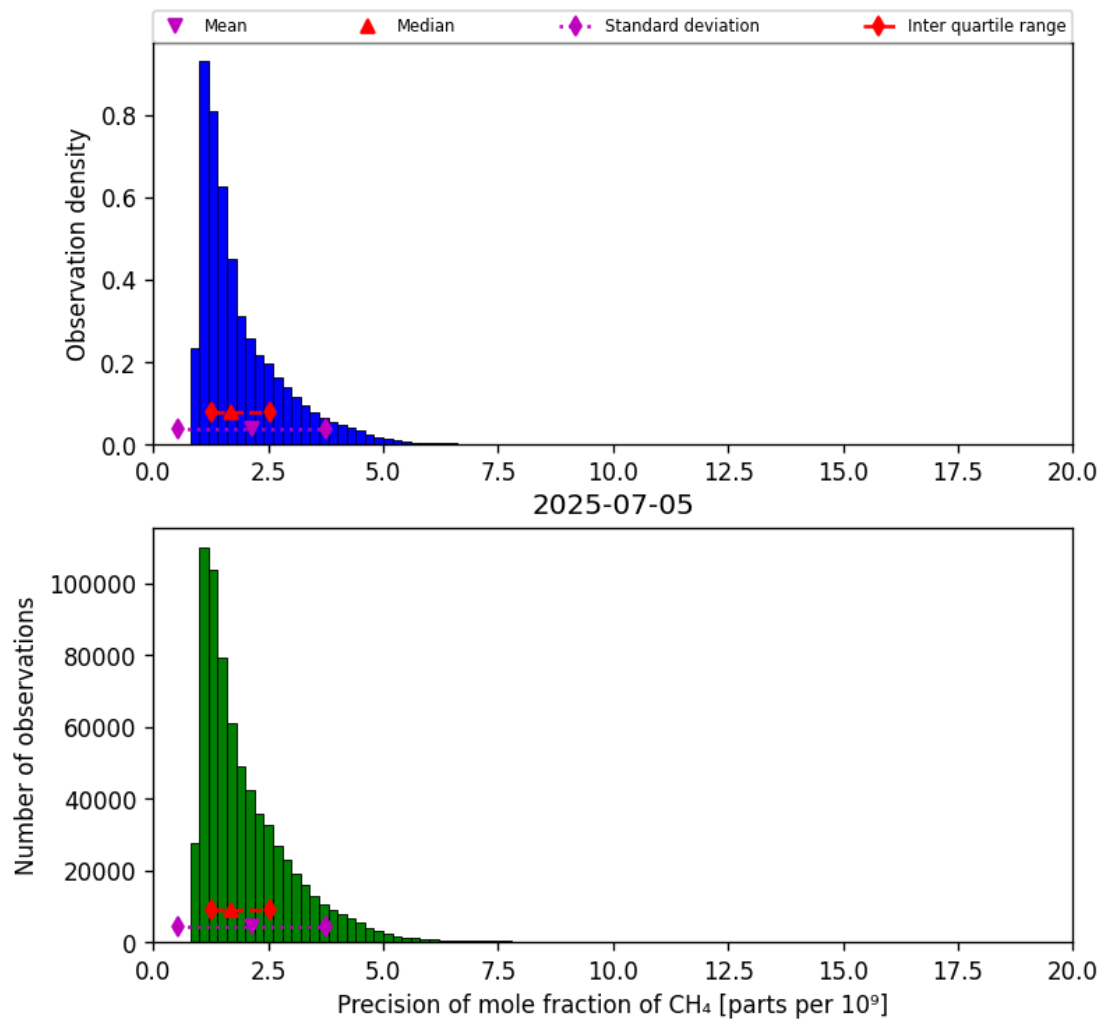
Figure 24: Histogram of “Precision of mole fraction of CH 4 ” for 2025-07-04 to 2025-07-06
