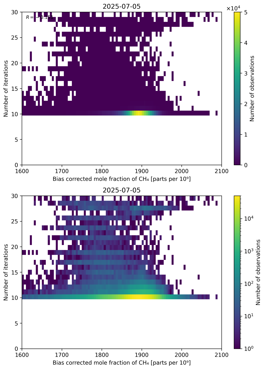
Figure 67: Scatter density plot of “Bias corrected mole fraction of CH 4 ” against “Number of iterations” for 2025-07-04 to 2025-07-06.
