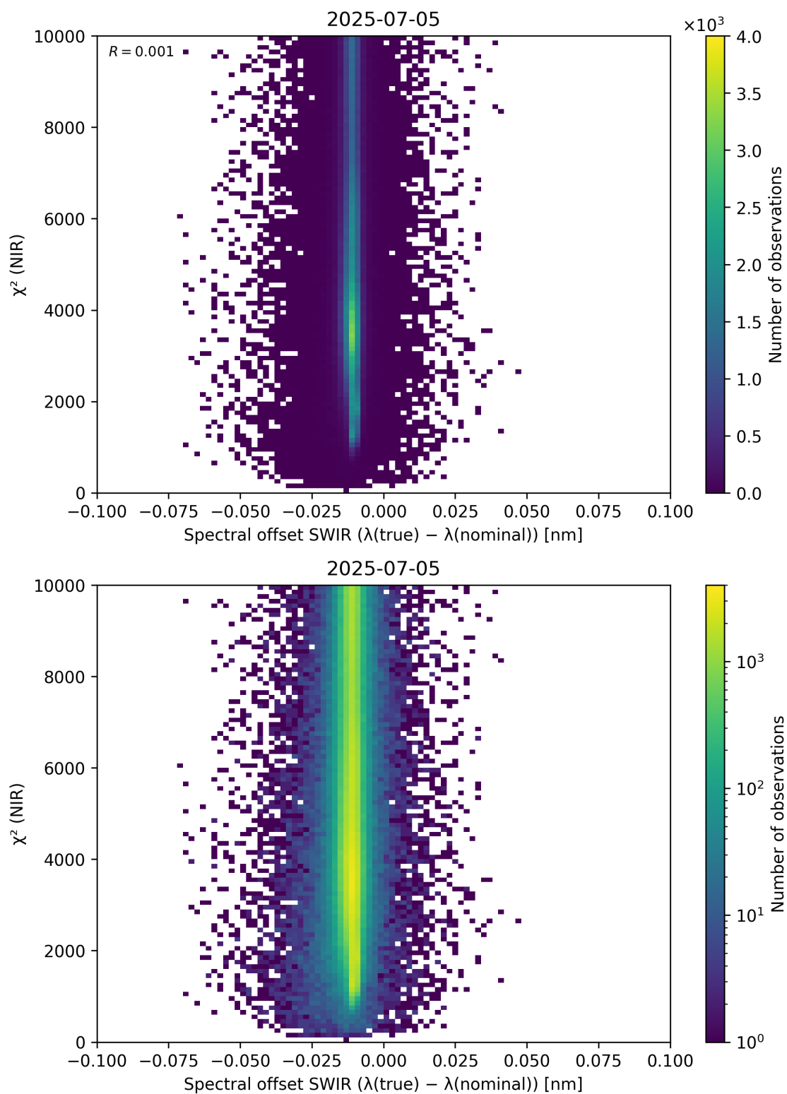
Figure 117: Scatter density plot of “Spectral offset SWIR ( \lambda_{\text{true}} - \lambda_{\text{nominal}} )” against “ \chi^2 (NIR)” for 2025-07-04 to 2025-07-06.
