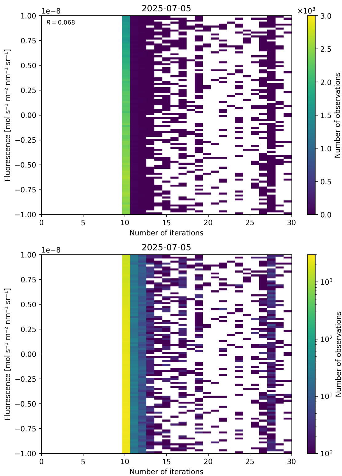
Figure 87: Scatter density plot of “Number of iterations” against “Fluorescence” for 2025-07-04 to 2025-07-06.
