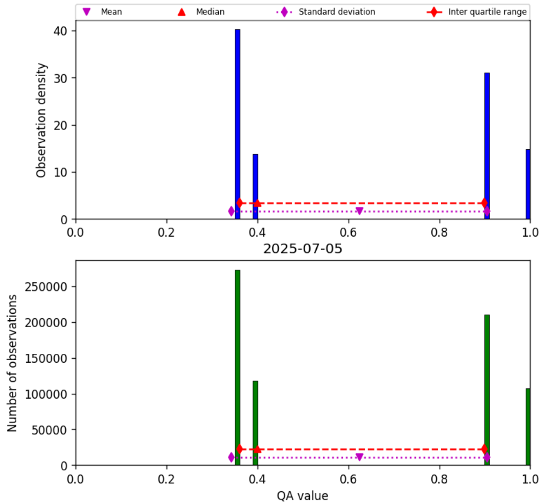
Figure 22: Histogram of “QA value” for 2025-07-04 to 2025-07-06
