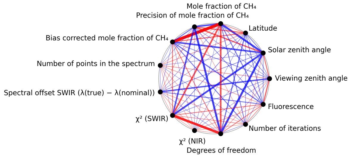
Figure 1: Map of correlation graph for 2025-07-04 to 2025-07-06.
