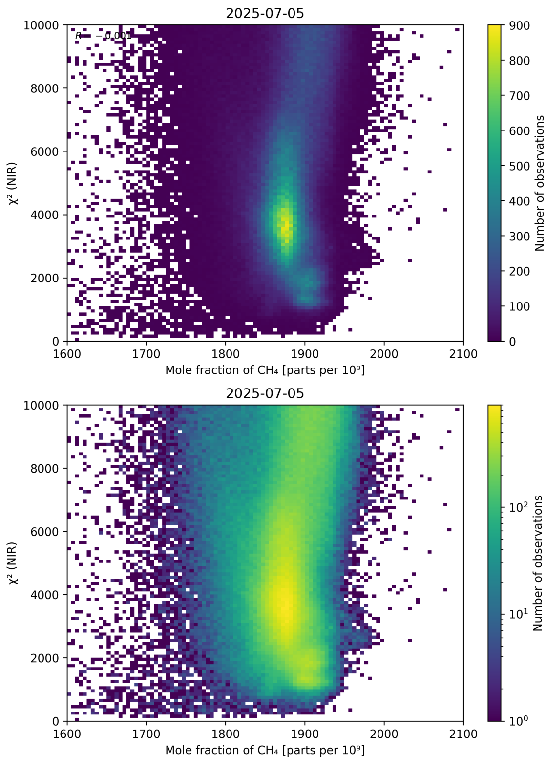
Figure 70: Scatter density plot of “Mole fraction of \text{CH}_4 ” against “ \chi^2 (NIR)” for 2025-07-04 to 2025-07-06.
