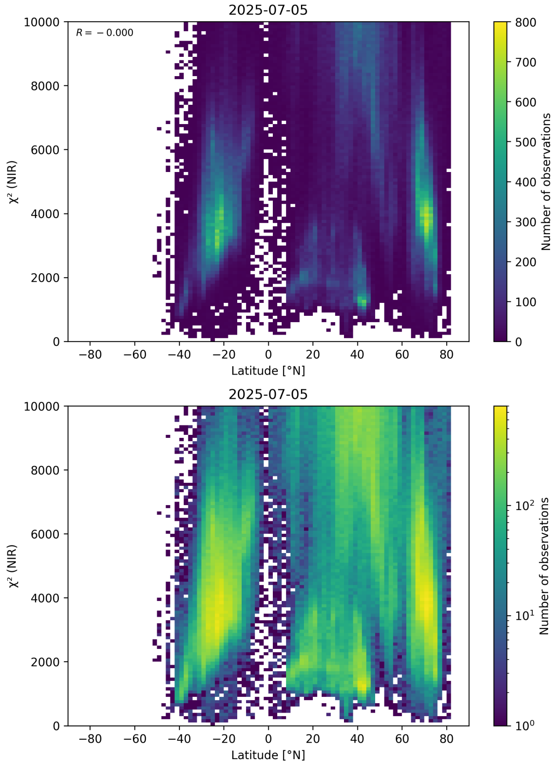
Figure 53: Scatter density plot of “Latitude” against “ \chi^2 (NIR)” for 2025-07-04 to 2025-07-06.
