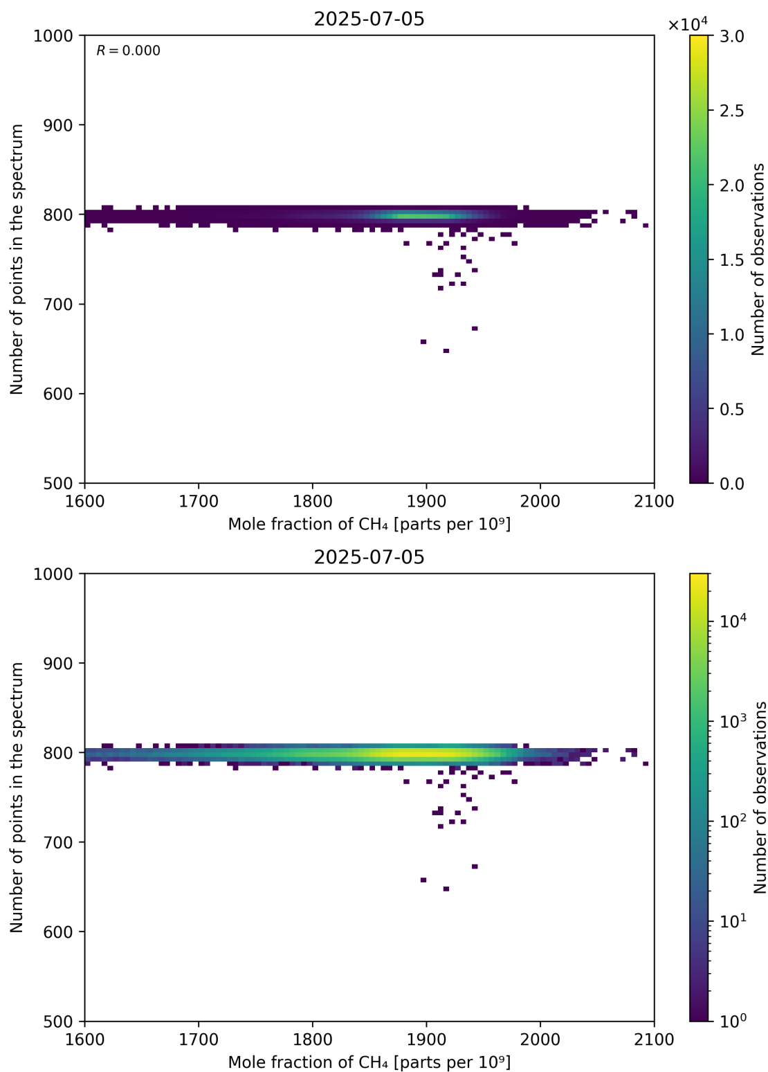
Figure 77: Scatter density plot of “Mole fraction of CH 4 ” against “Number of points in the spectrum” for 2025-07-04 to 2025-07-06.
