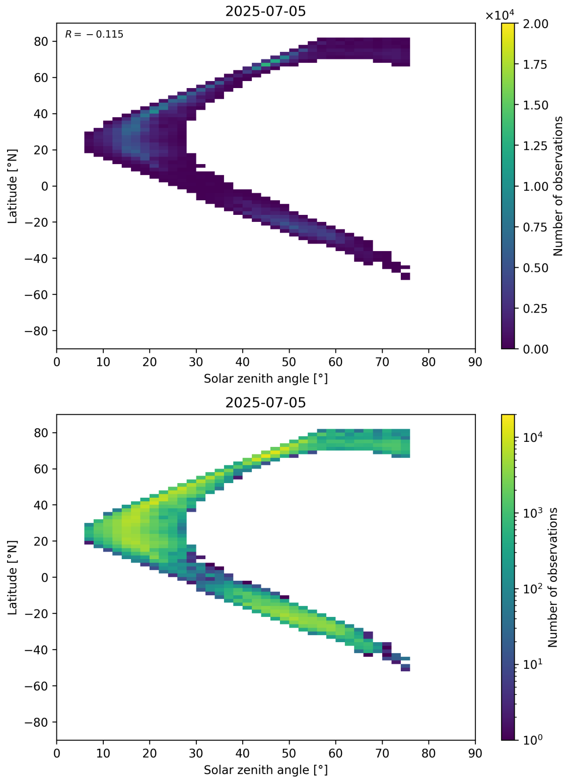
Figure 98: Scatter density plot of “Solar zenith angle” against “Latitude” for 2025-07-04 to 2025-07-06.
