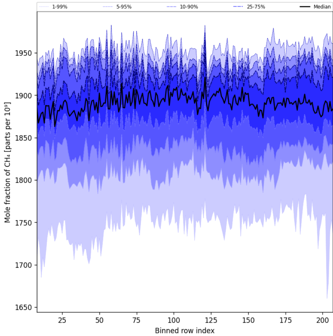
Figure 34: Along track statistics of “Mole fraction of CH 4 ” for 2025-07-04 to 2025-07-06
