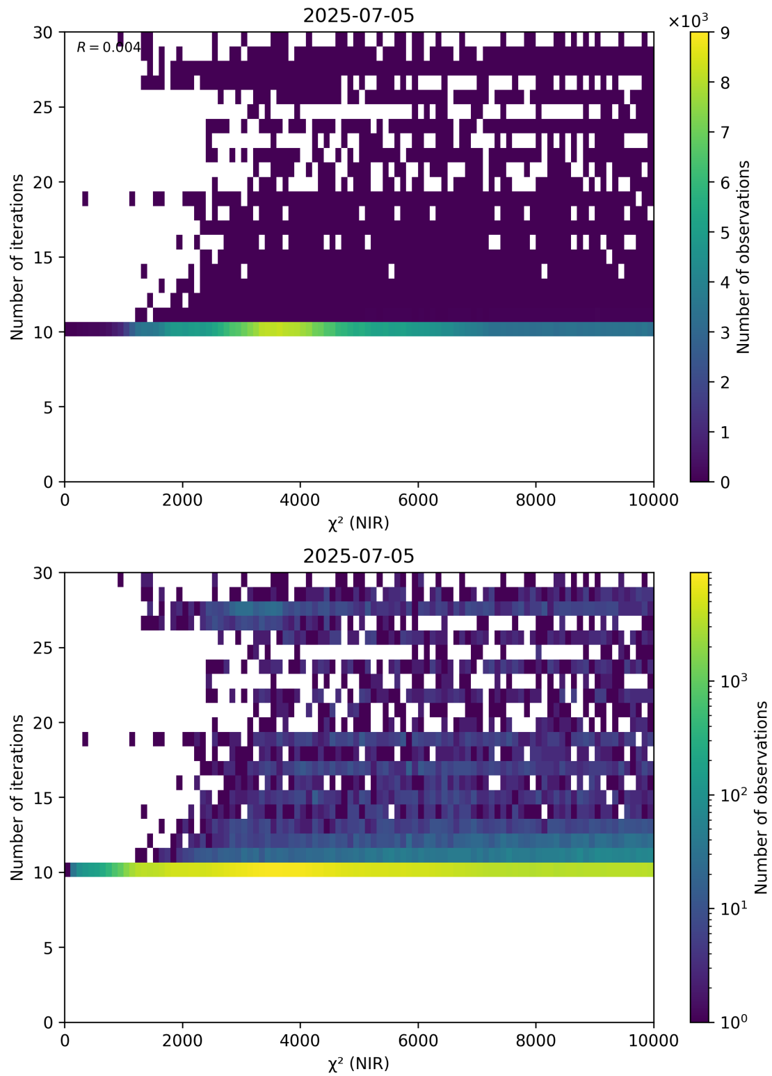
Figure 46: Scatter density plot of “ \chi^2 (NIR)” against “Number of iterations” for 2025-07-04 to 2025-07-06.
