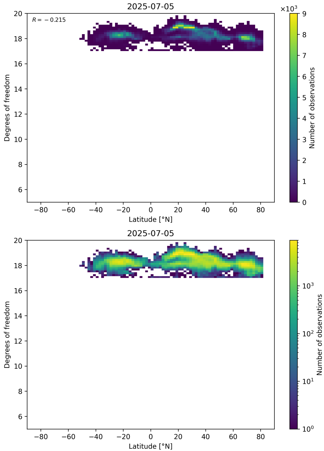
Figure 55: Scatter density plot of “Latitude” against “Degrees of freedom” for 2025-07-04 to 2025-07-06.
