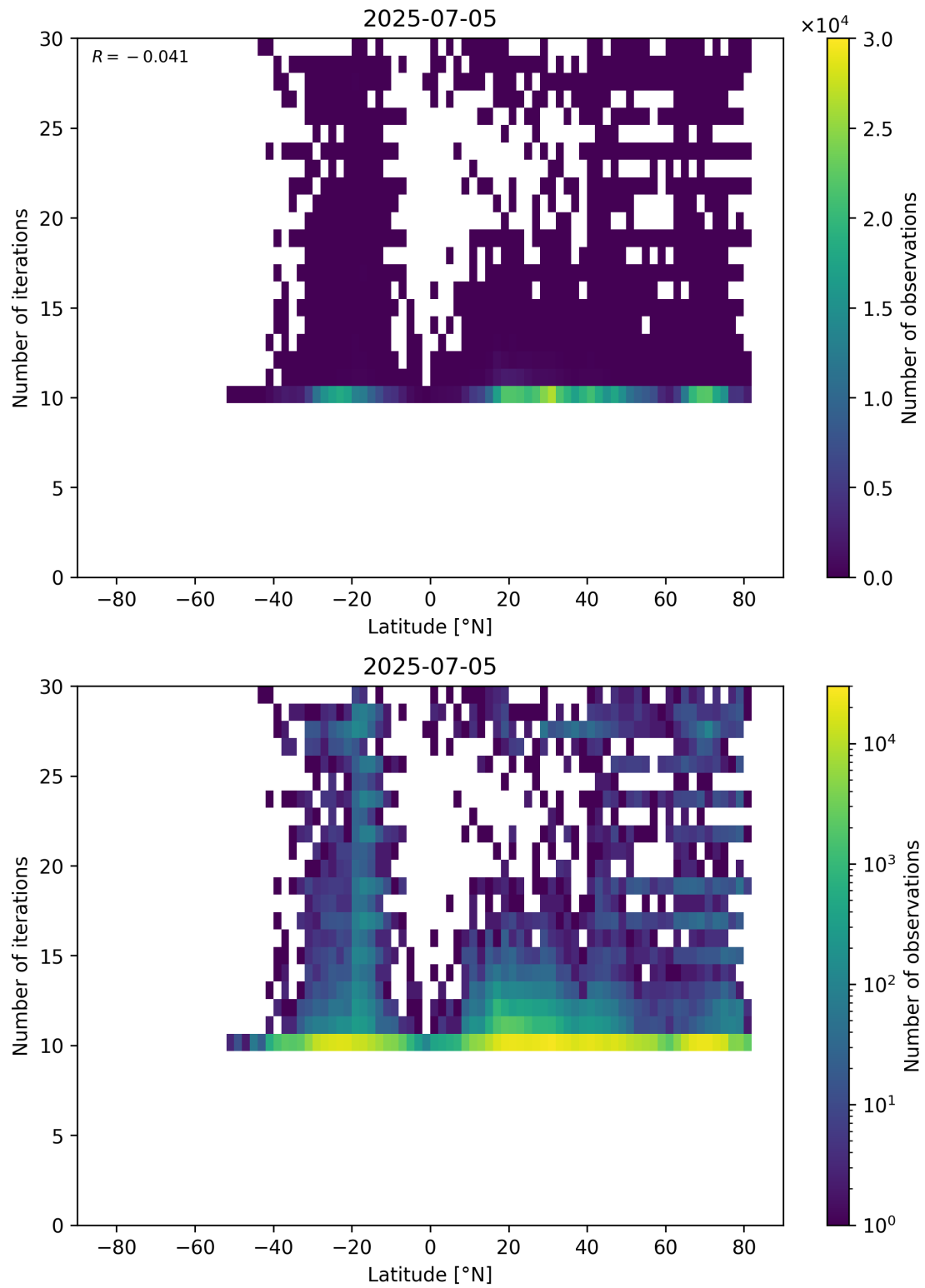
Figure 60: Scatter density plot of “Latitude” against “Number of iterations” for 2025-07-04 to 2025-07-06.
