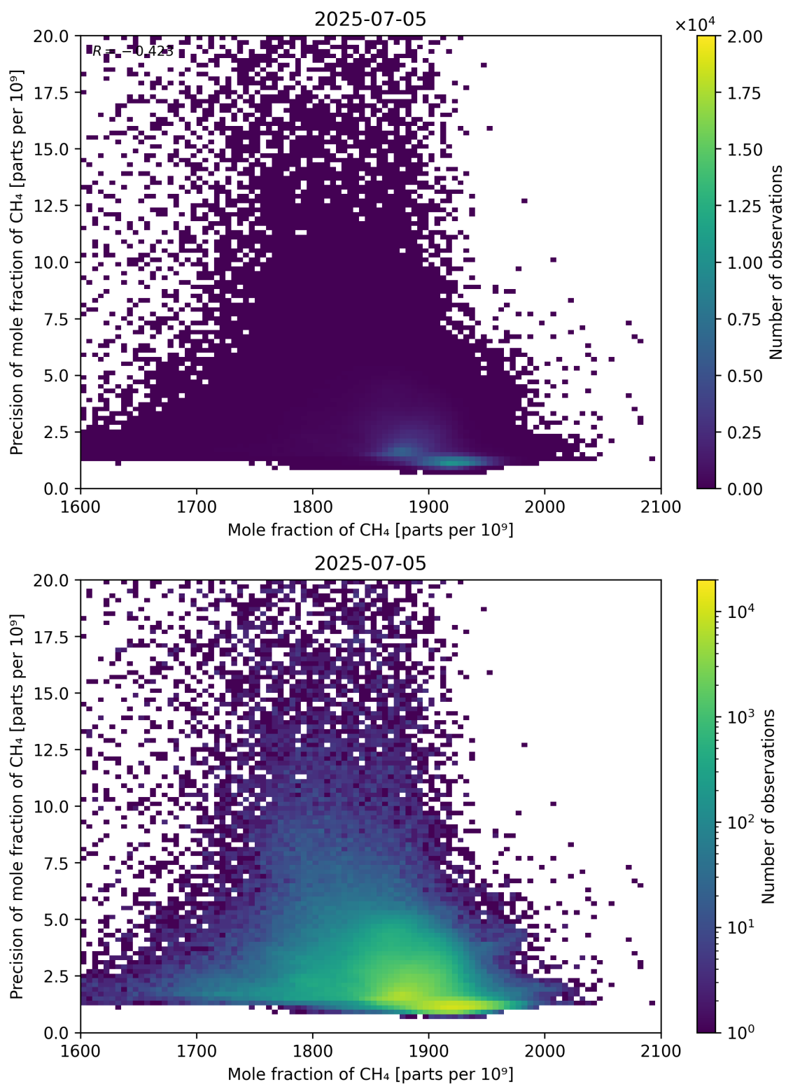
Figure 75: Scatter density plot of “Mole fraction of CH 4 ” against “Precision of mole fraction of CH 4 ” for 2025-07-04 to 2025-07-06.
