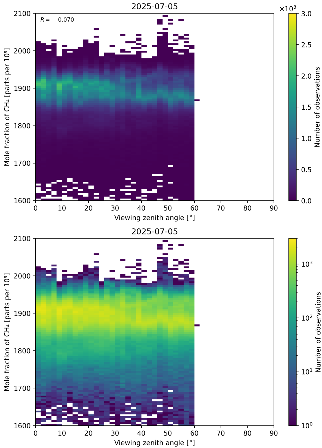
Figure 110: Scatter density plot of “Viewing zenith angle” against “Mole fraction of CH 4 ” for 2025-07-04 to 2025-07-06.
