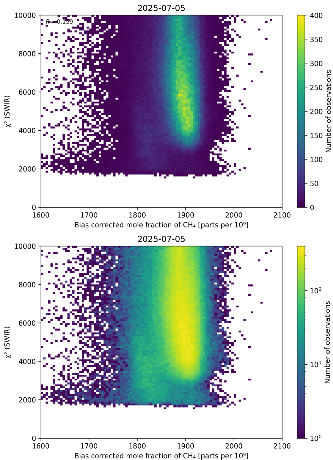
Figure 64: Scatter density plot of “Bias corrected mole fraction of \text{CH}_4 ” against “ \chi^2 (SWIR)” for 2025-07-04 to 2025-07-06.
