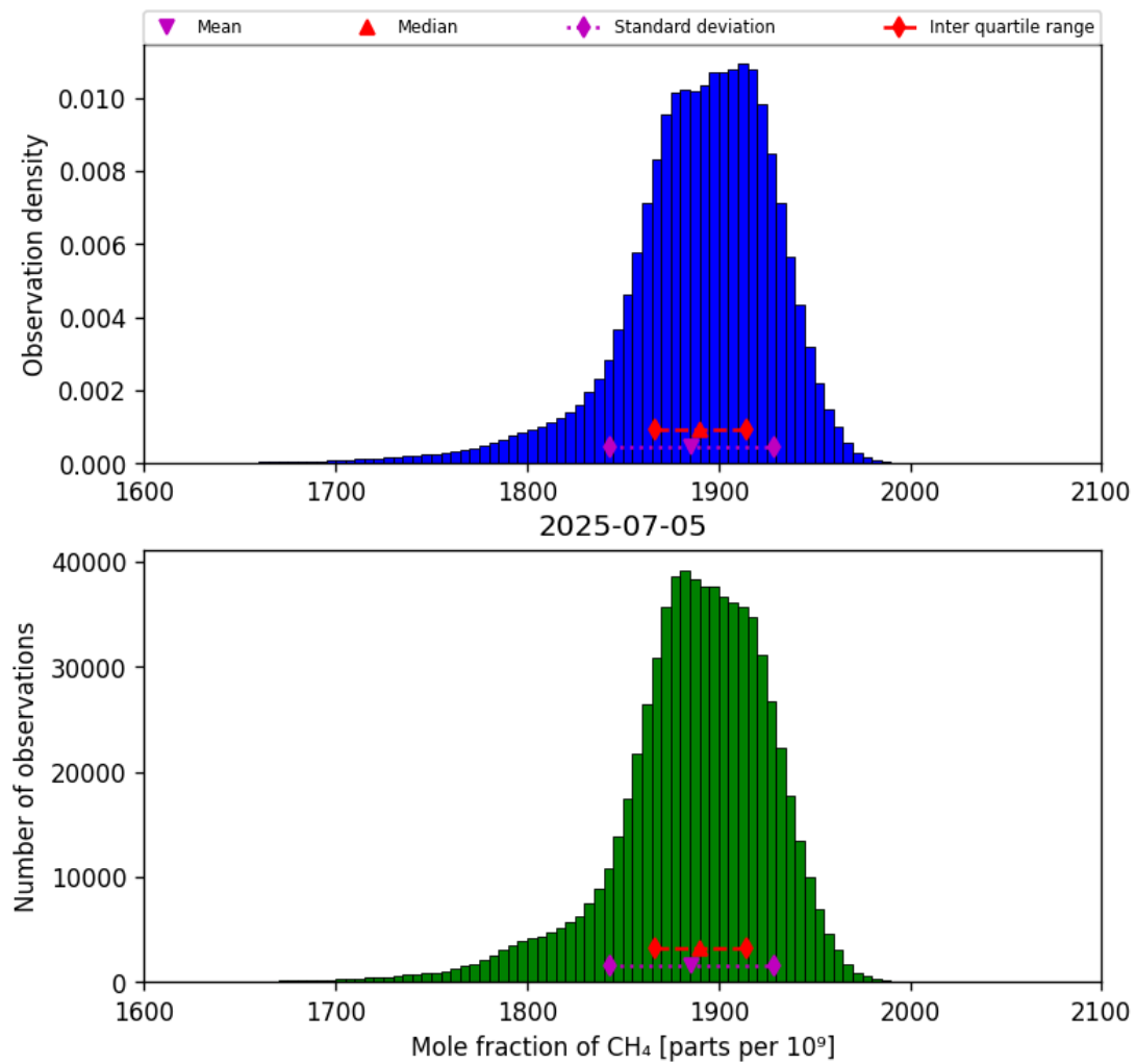
Figure 23: Histogram of “Mole fraction of CH 4 ” for 2025-07-04 to 2025-07-06
