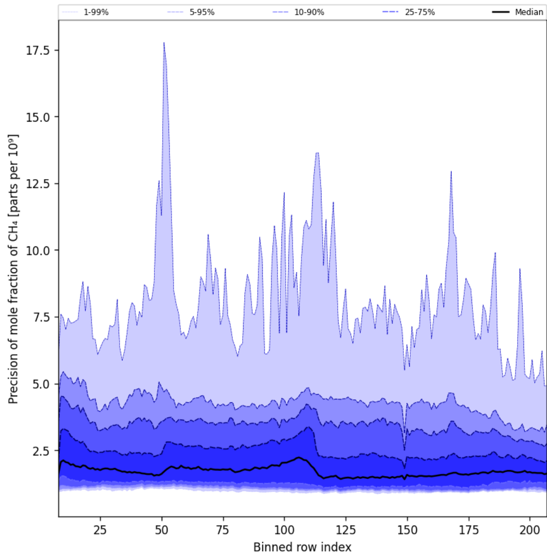
Figure 35: Along track statistics of “Precision of mole fraction of CH 4 ” for 2025-07-04 to 2025-07-06
