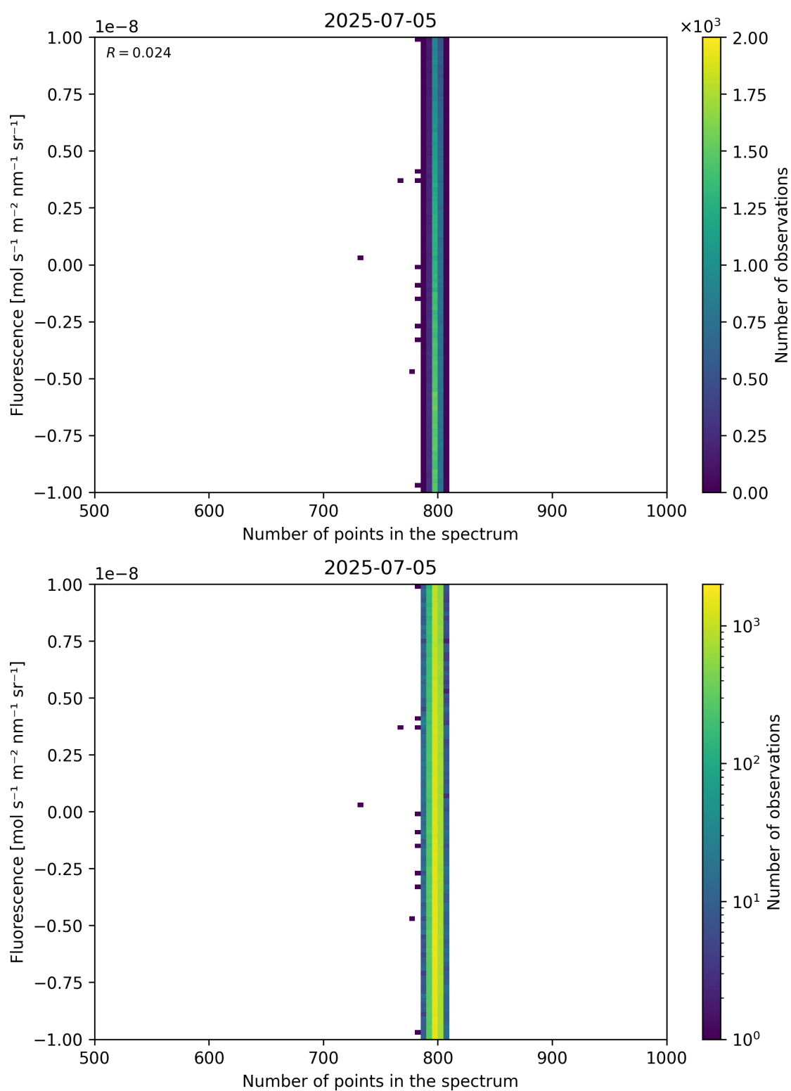
Figure 91: Scatter density plot of “Number of points in the spectrum” against “Fluorescence” for 2025-07-04 to 2025-07-06.
