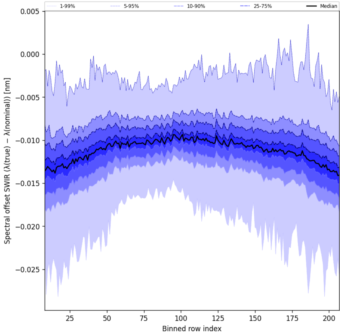
Figure 38: Along track statistics of “Spectral offset SWIR ( \lambda_{\text{true}} - \lambda_{\text{nominal}} )” for 2025-07-04 to 2025-07-06
