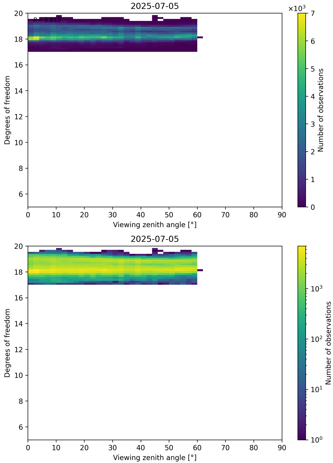
Figure 107: Scatter density plot of “Viewing zenith angle” against “Degrees of freedom” for 2025-07-04 to 2025-07-06.
