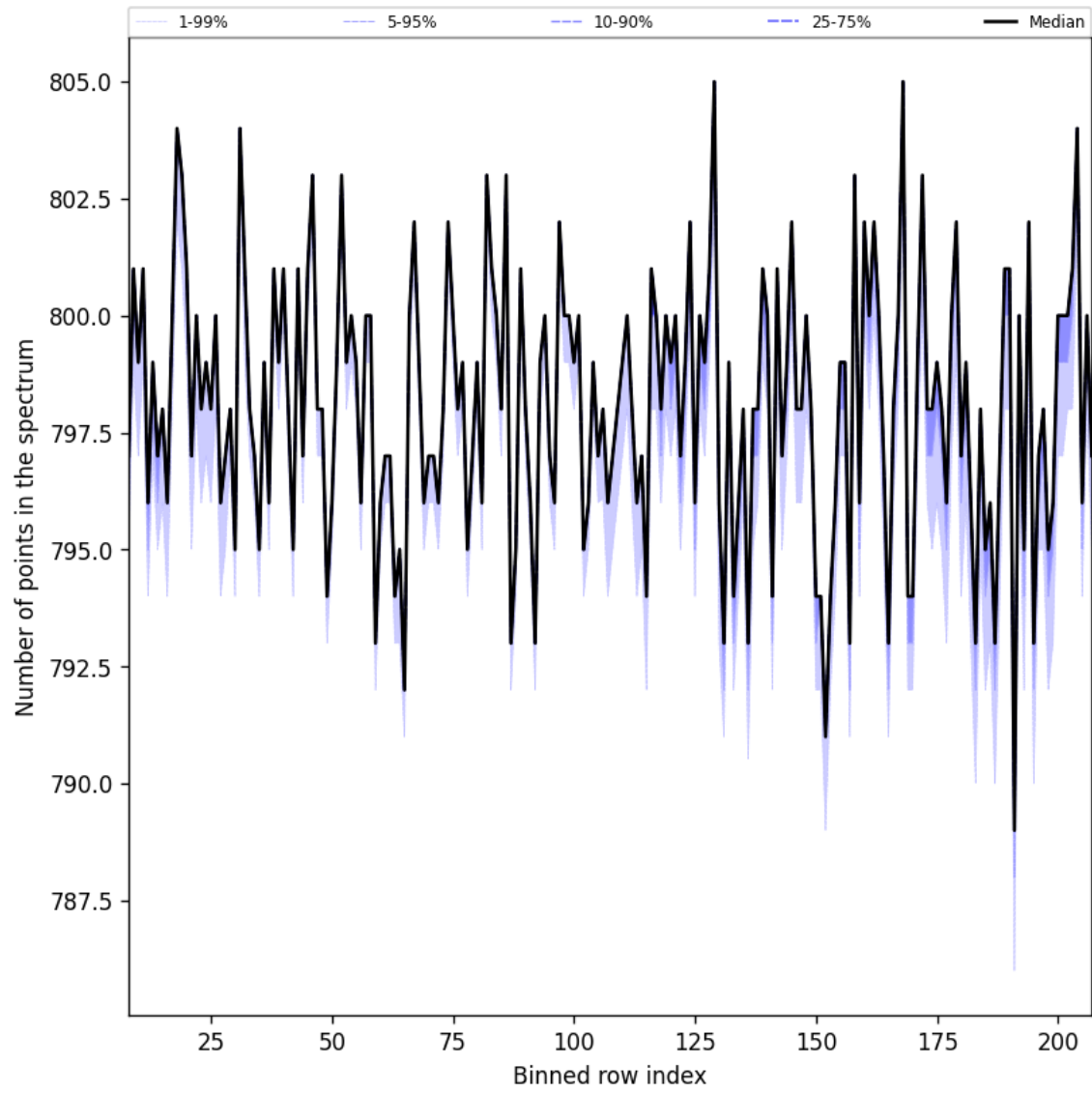
Figure 37: Along track statistics of “Number of points in the spectrum” for 2025-07-04 to 2025-07-06
