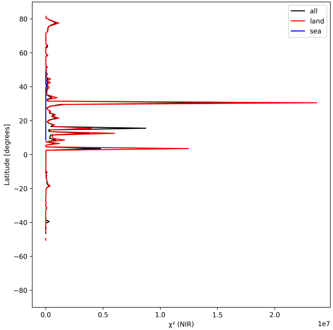
Figure 18: Zonal average of “ \chi^2 (NIR)” for 2025-07-04 to 2025-07-06.
