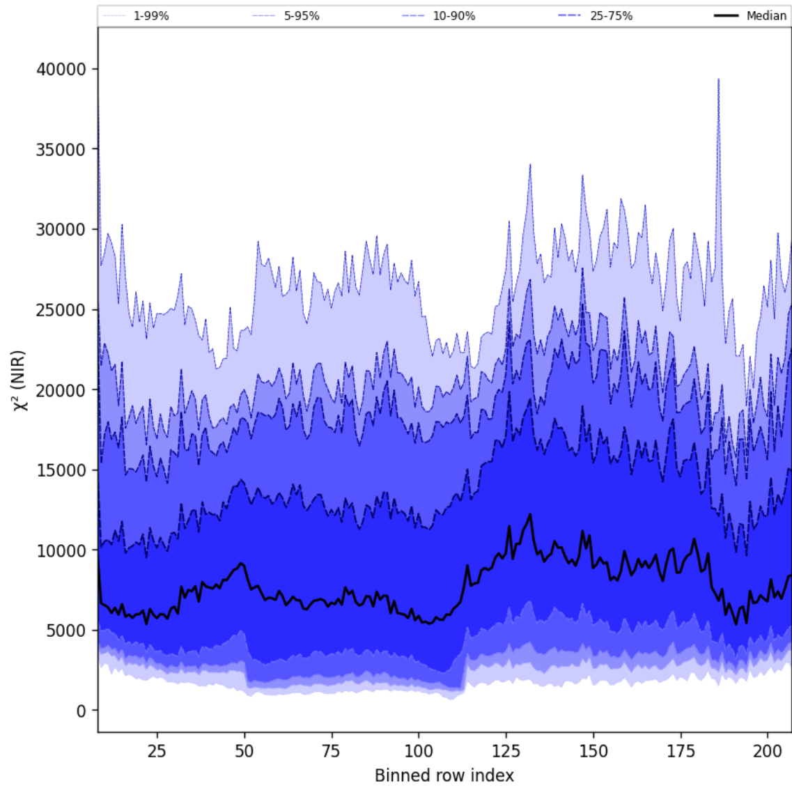
Figure 40: Along track statistics of " \chi^2 (NIR)" for 2025-07-04 to 2025-07-06
