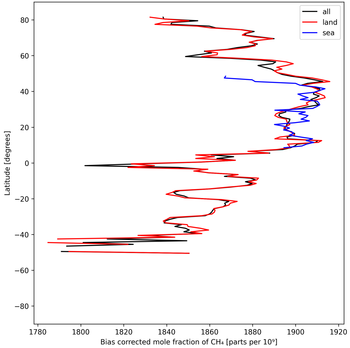
Figure 14: Zonal average of “Bias corrected mole fraction of CH 4 ” for 2025-07-04 to 2025-07-06.
