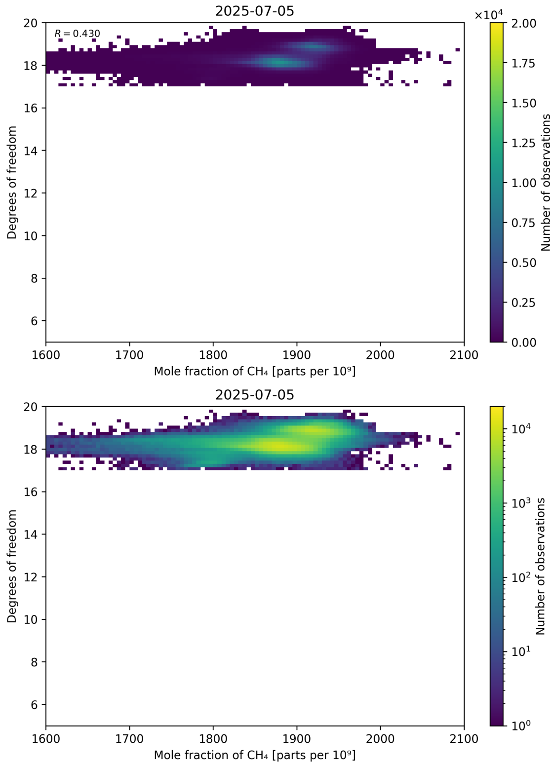
Figure 72: Scatter density plot of “Mole fraction of CH 4 ” against “Degrees of freedom” for 2025-07-04 to 2025-07-06.
