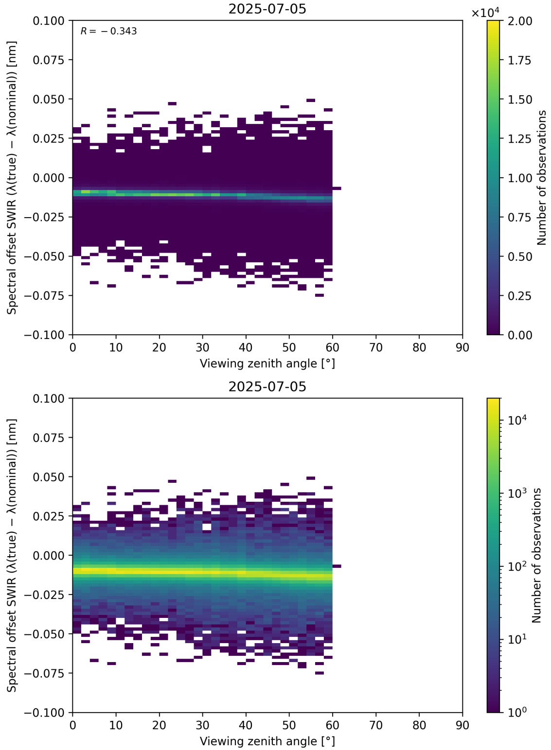
Figure 116: Scatter density plot of “Viewing zenith angle” against “Spectral offset SWIR ( \lambda_{\text{true}} - \lambda_{\text{nominal}} )” for 2025-07-04 to 2025-07-06.
