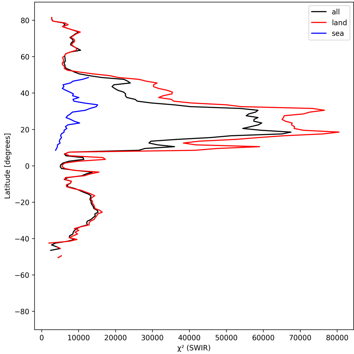
Figure 17: Zonal average of “ \chi^2 (SWIR)” for 2025-07-04 to 2025-07-06.
