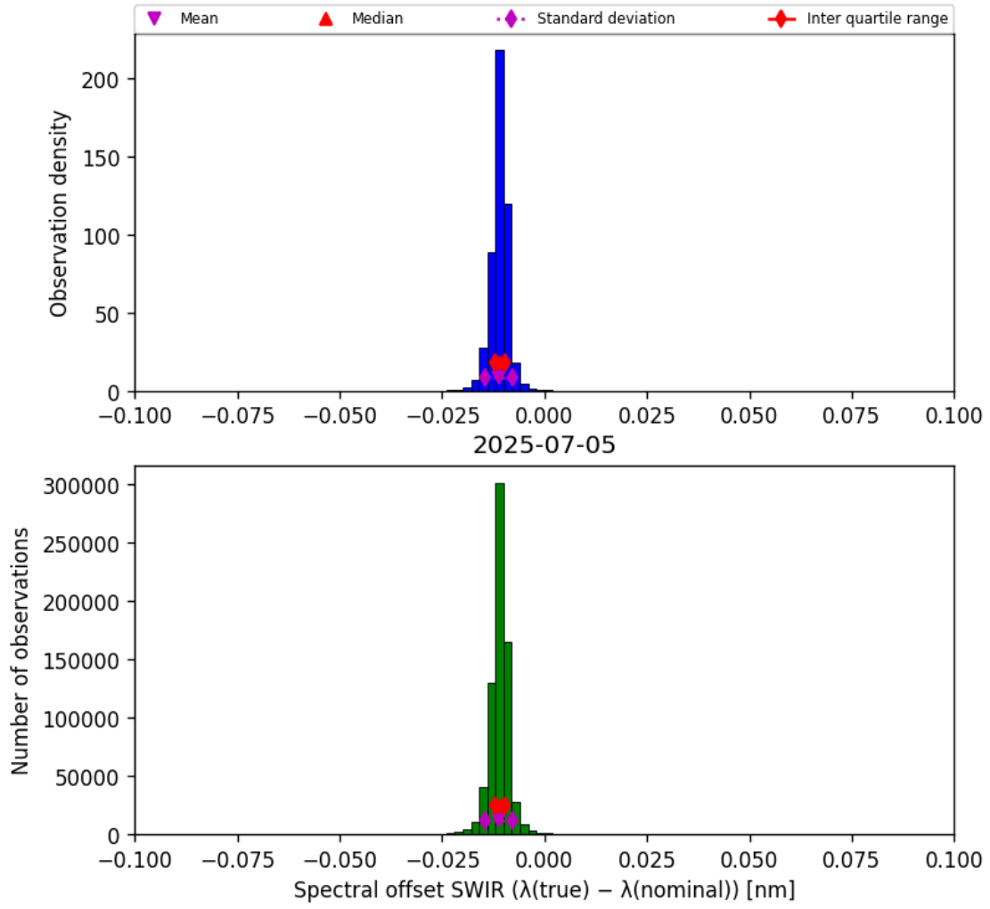
Figure 27: Histogram of “Spectral offset SWIR ( \lambda_{\text{true}} - \lambda_{\text{nominal}} )” for 2025-07-04 to 2025-07-06
