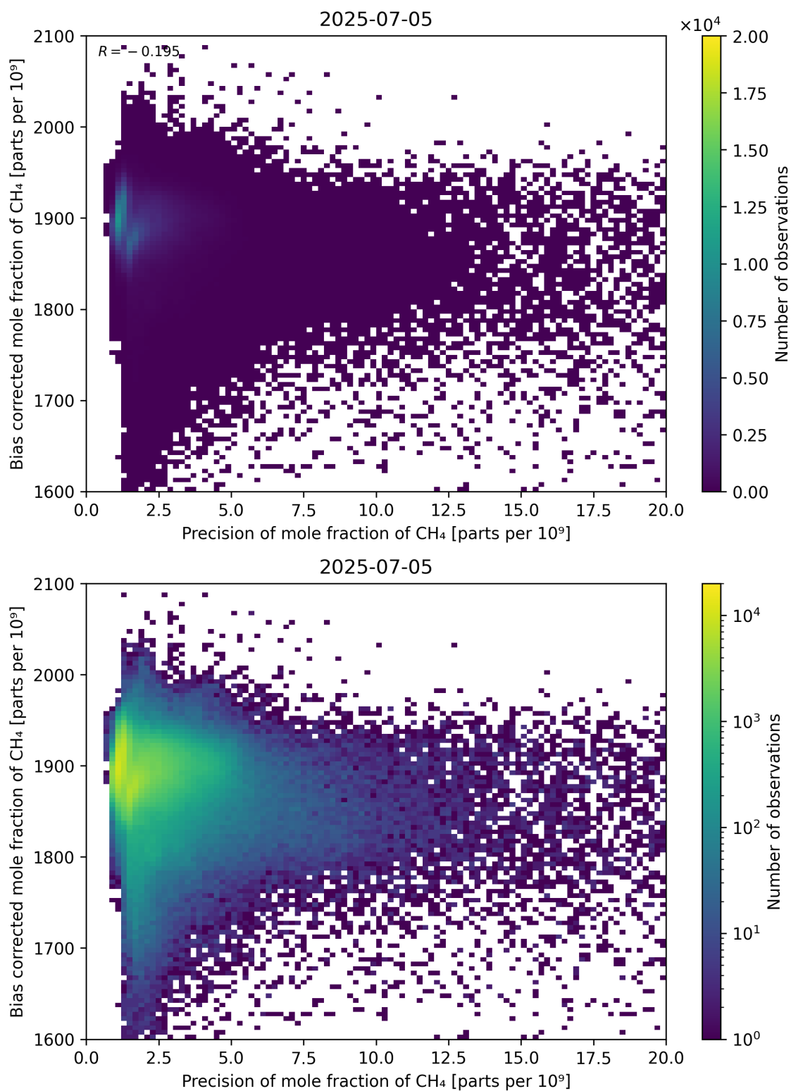
Figure 82: Scatter density plot of “Precision of mole fraction of CH 4 ” against “Bias corrected mole fraction of CH 4 ” for 2025-07-04 to 2025-07-06.
