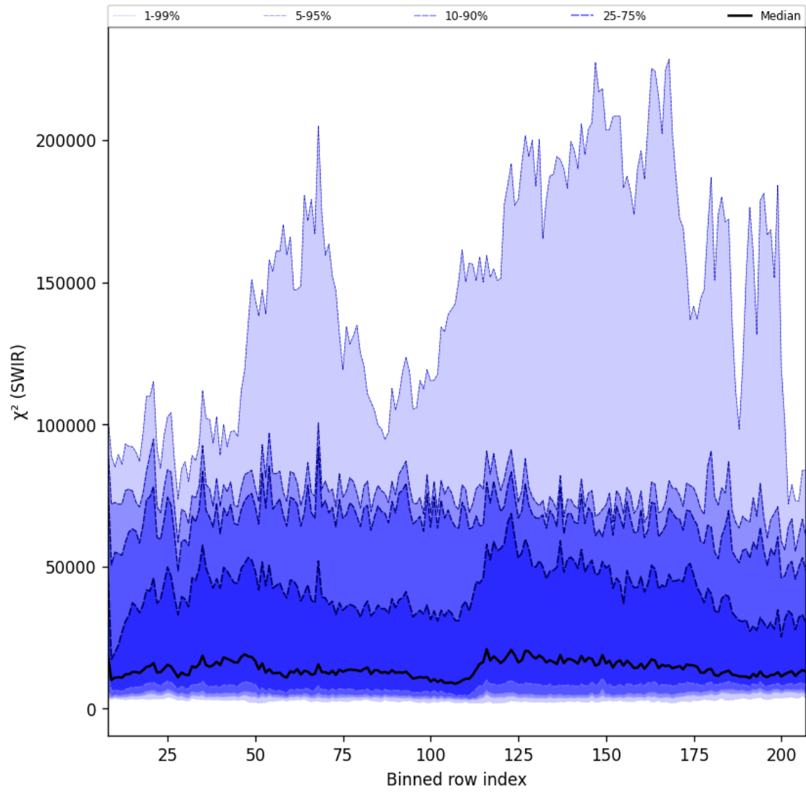
Figure 39: Along track statistics of “ \chi^2 (SWIR)” for 2025-07-04 to 2025-07-06
