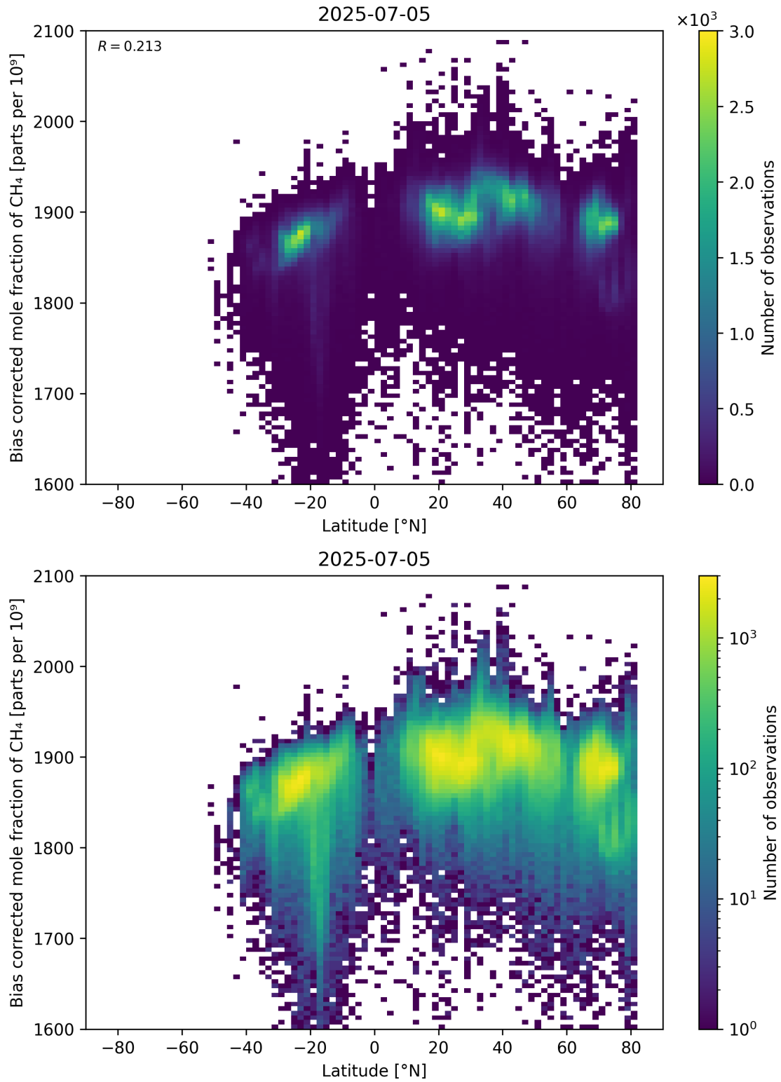
Figure 58: Scatter density plot of “Latitude” against “Bias corrected mole fraction of \text{CH}_4 ” for 2025-07-04 to 2025-07-06.
