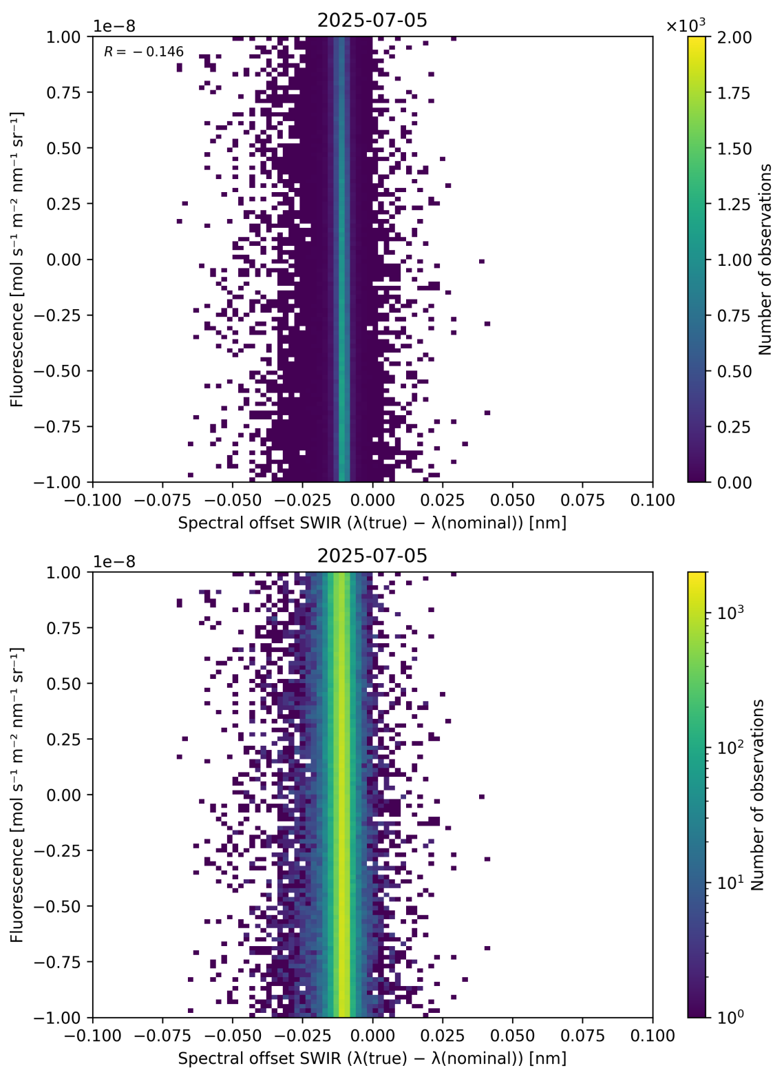
Figure 120: Scatter density plot of “Spectral offset SWIR ( \lambda_{\text{true}} - \lambda_{\text{nominal}} )” against “Fluorescence” for 2025-07-04 to 2025-07-06.
