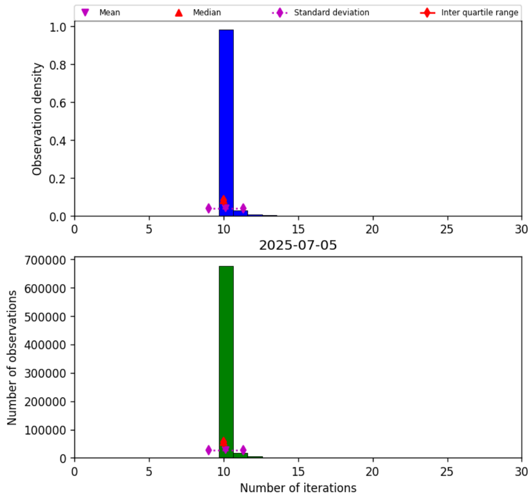
Figure 31: Histogram of “Number of iterations” for 2025-07-04 to 2025-07-06
