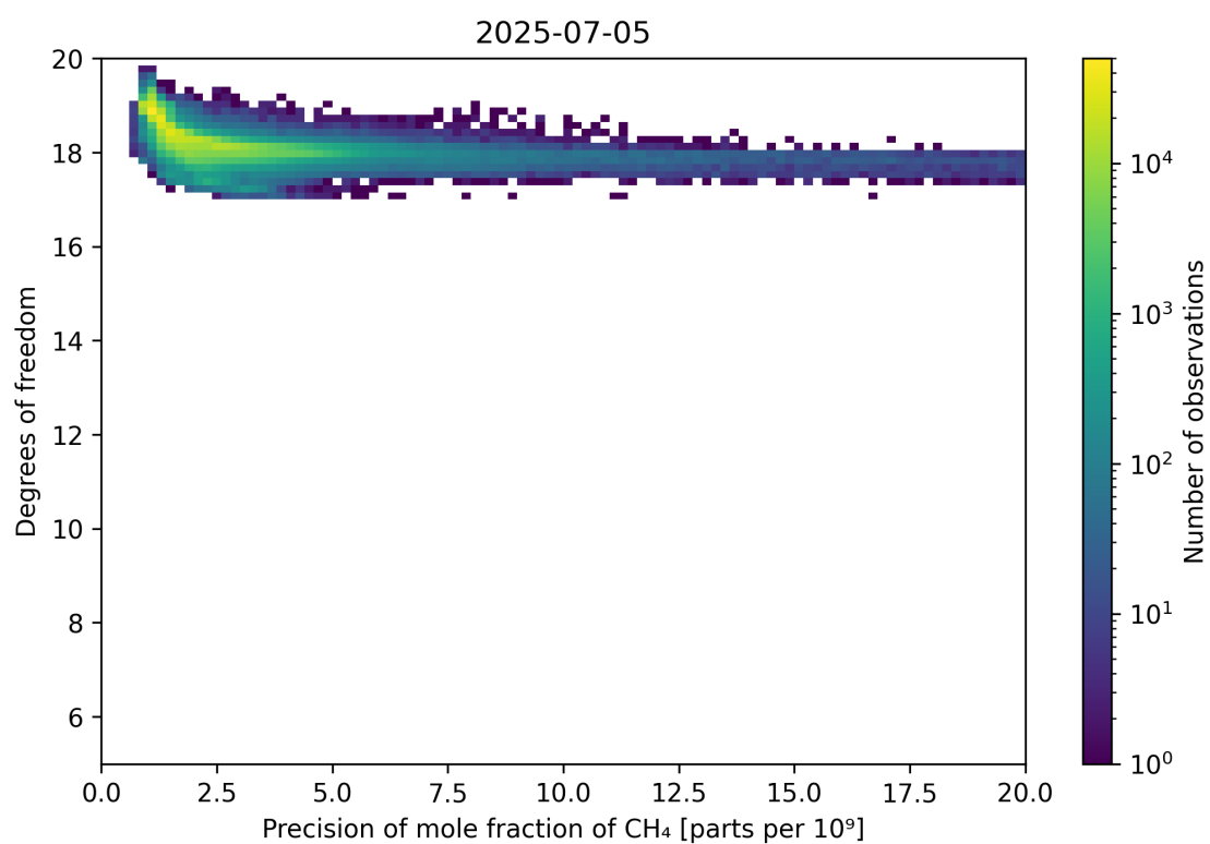
Figure 80: Scatter density plot of “Precision of mole fraction of CH 4 ” against “Degrees of freedom” for 2025-07-04 to 2025-07-06.
