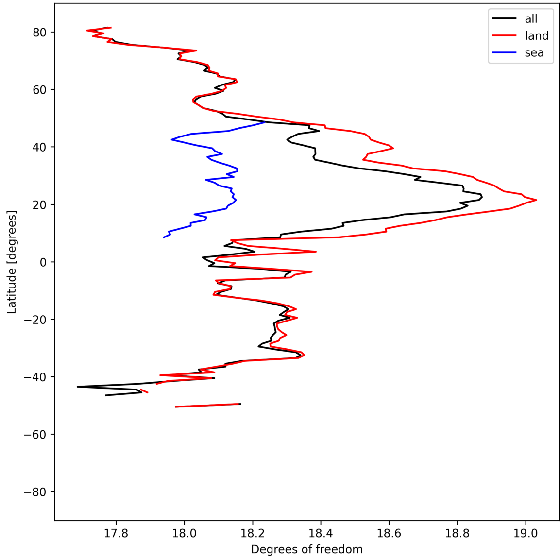
Figure 19: Zonal average of “Degrees of freedom” for 2025-07-04 to 2025-07-06.
