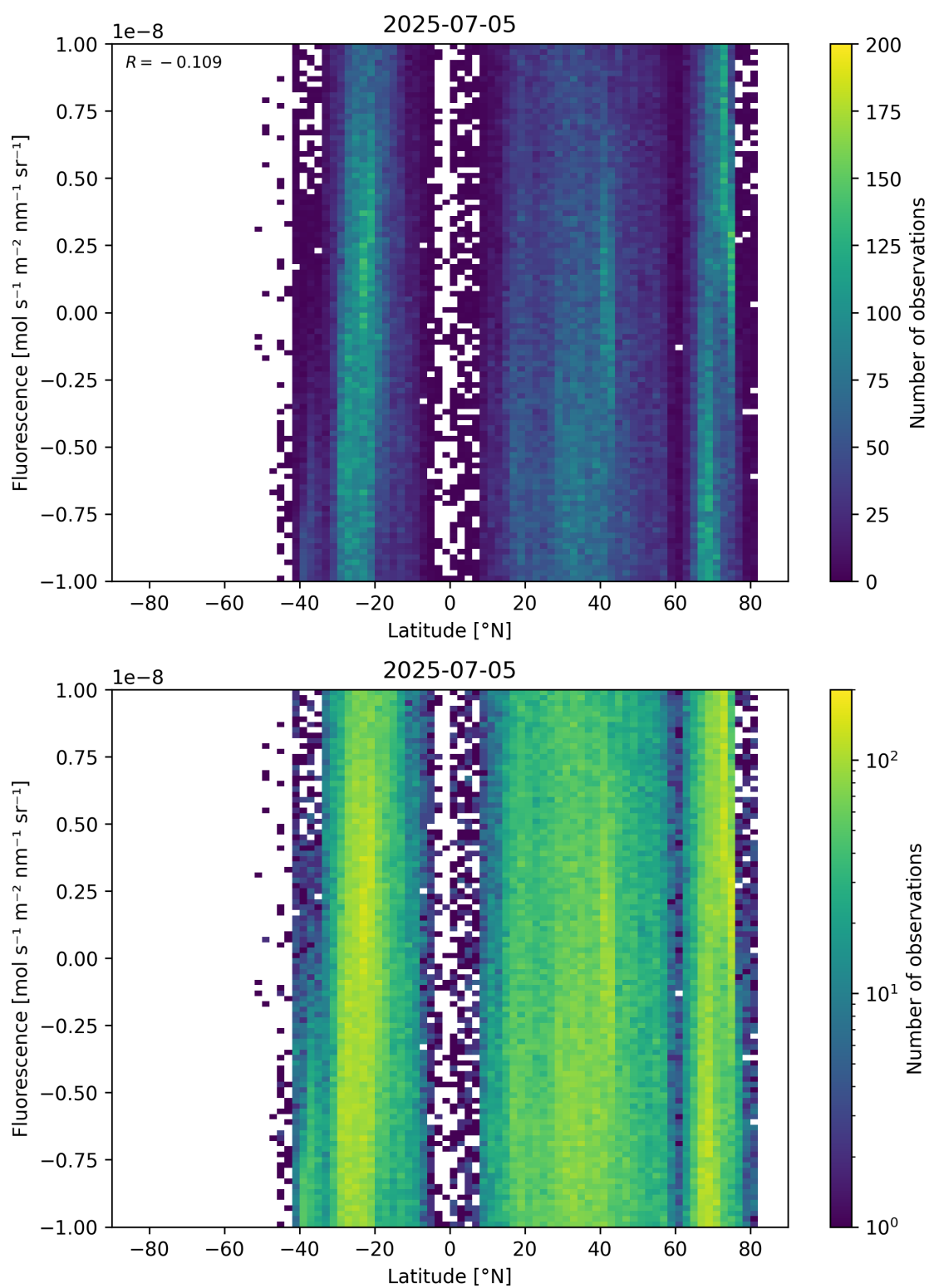
Figure 56: Scatter density plot of “Latitude” against “Fluorescence” for 2025-07-04 to 2025-07-06.
