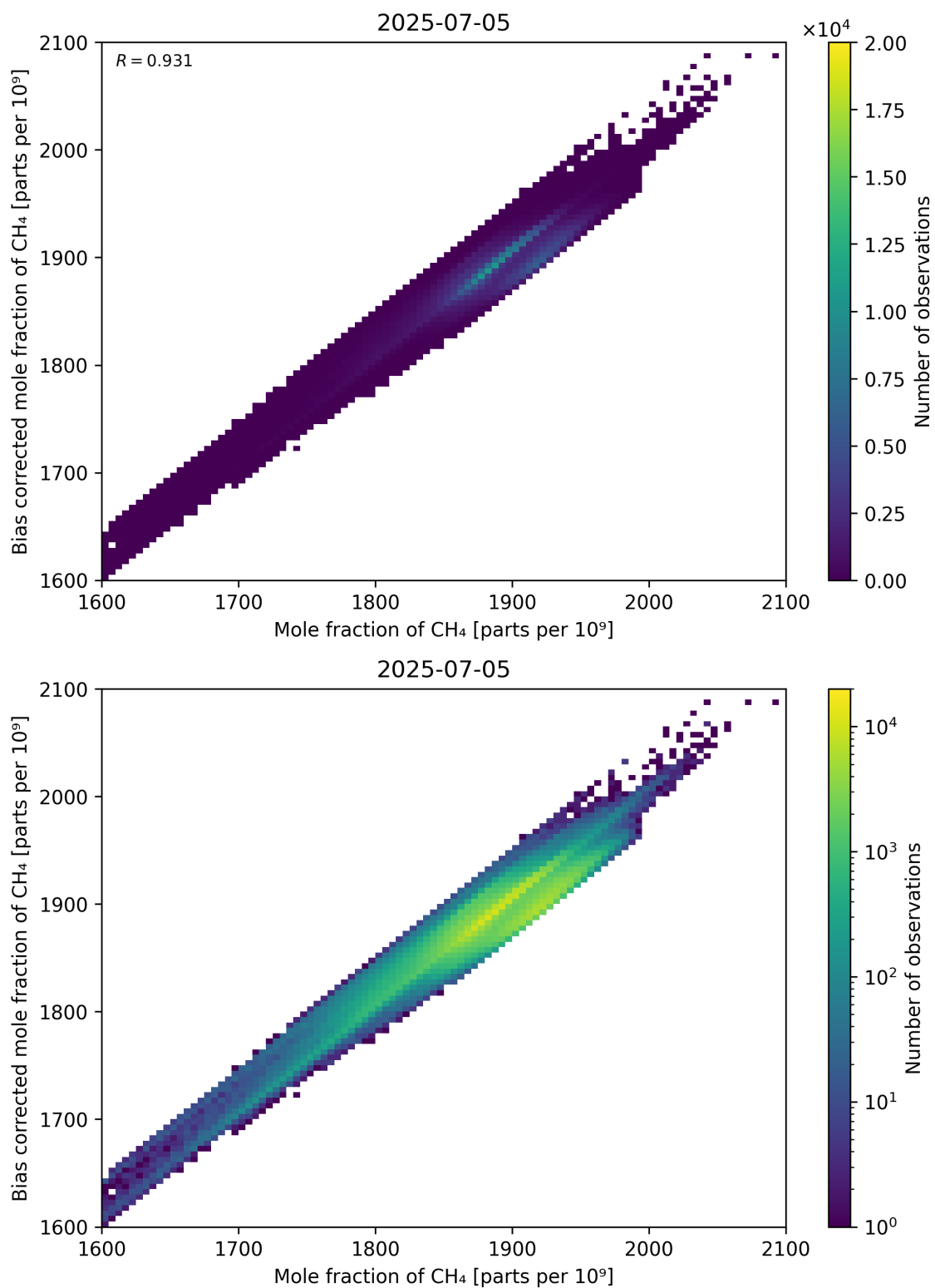
Figure 74: Scatter density plot of “Mole fraction of CH 4 ” against “Bias corrected mole fraction of CH 4 ” for 2025-07-04 to 2025-07-06.
