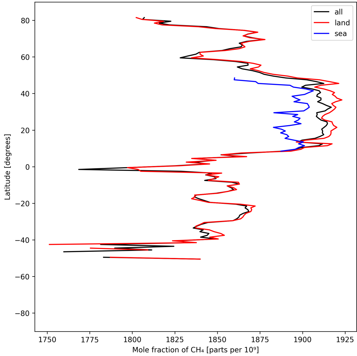
Figure 12: Zonal average of “Mole fraction of CH 4 ” for 2025-07-04 to 2025-07-06.
