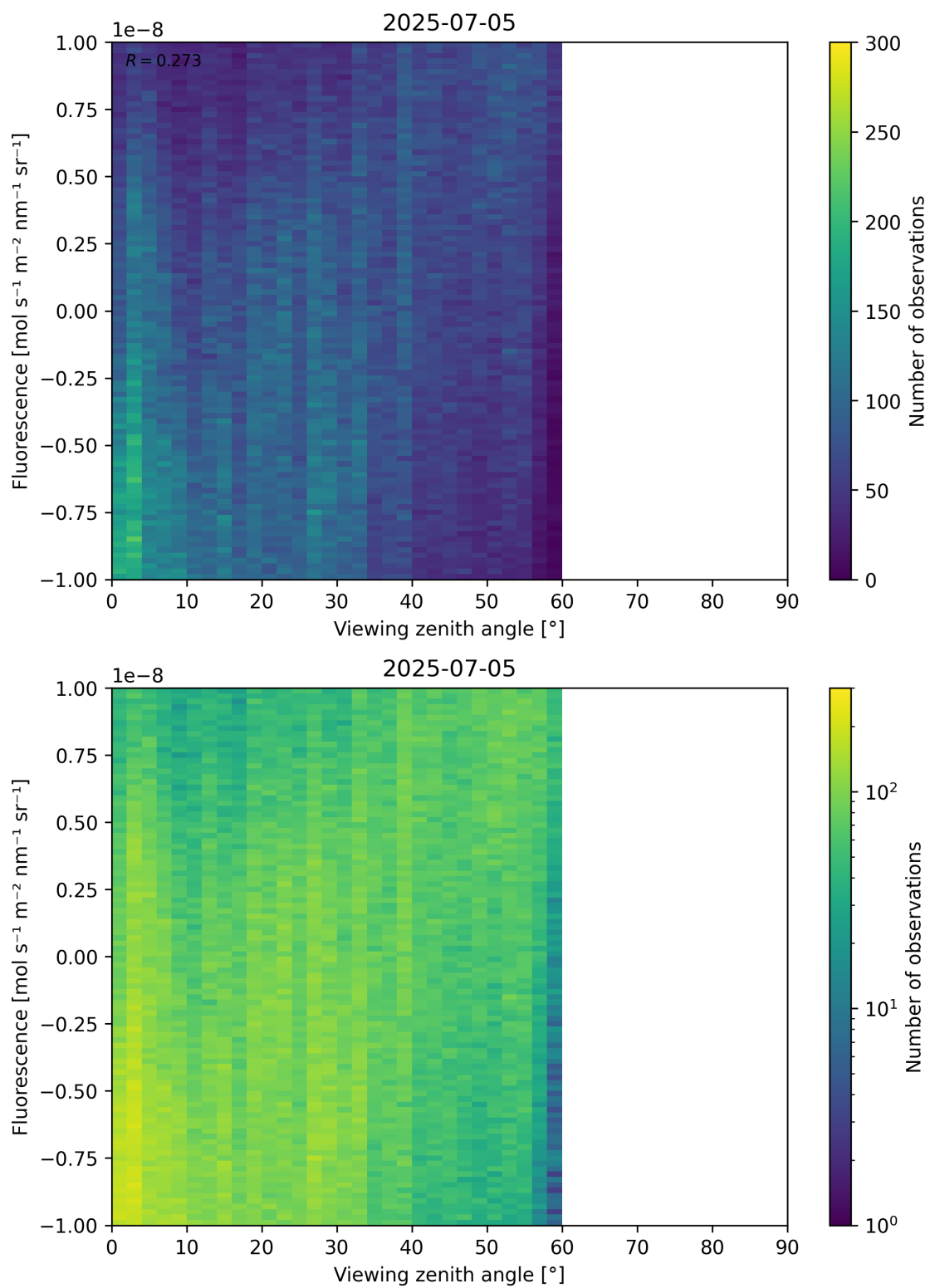
Figure 108: Scatter density plot of “Viewing zenith angle” against “Fluorescence” for 2025-07-04 to 2025-07-06.
