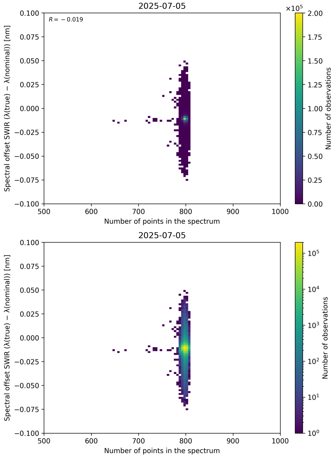
Figure 93: Scatter density plot of “Number of points in the spectrum” against “Spectral offset SWIR ( \lambda_{\text{true}} - \lambda_{\text{nominal}} )” for 2025-07-04 to 2025-07-06.
