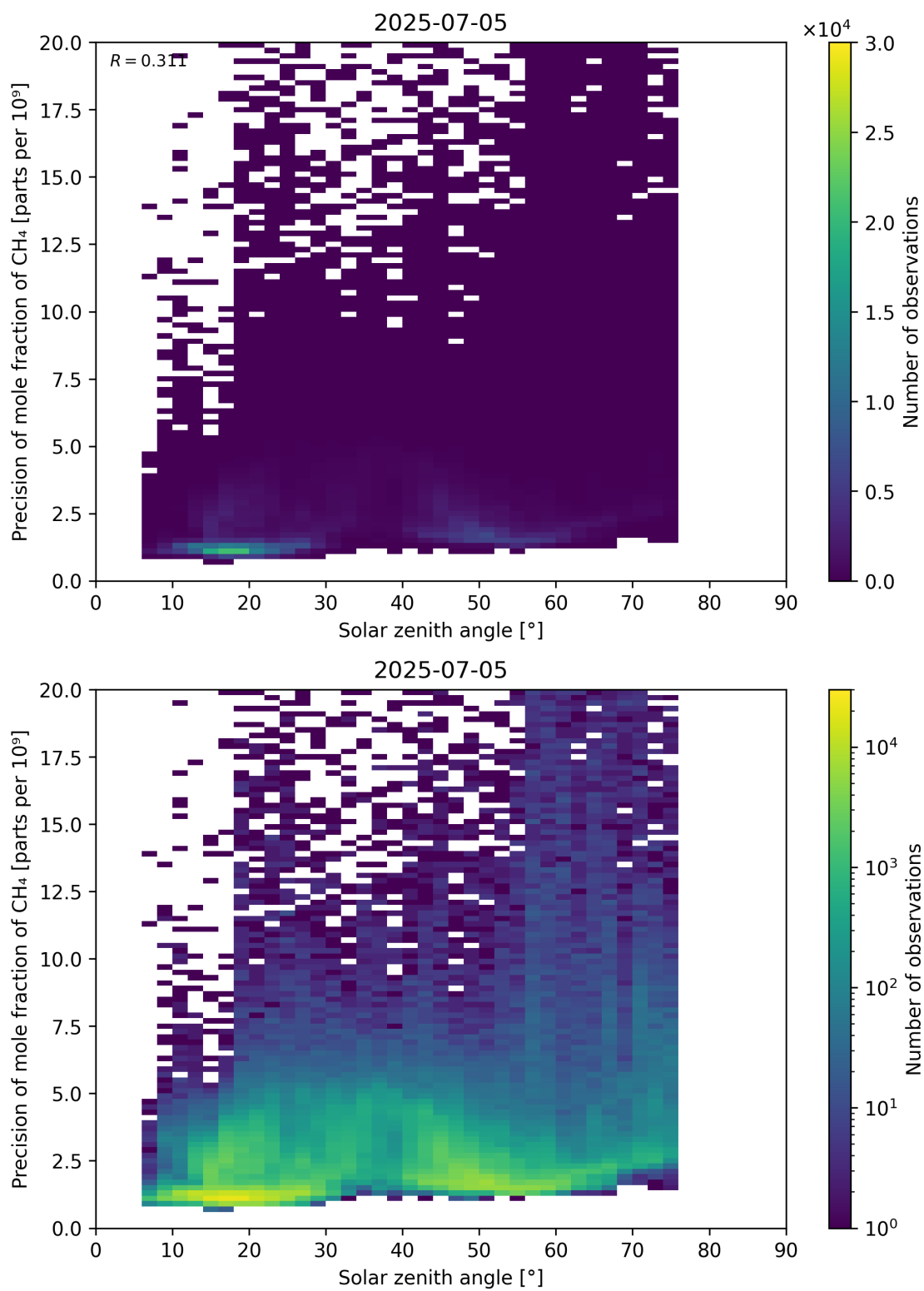
Figure 101: Scatter density plot of “Solar zenith angle” against “Precision of mole fraction of CH 4 ” for 2025-07-04 to 2025-07-06.
