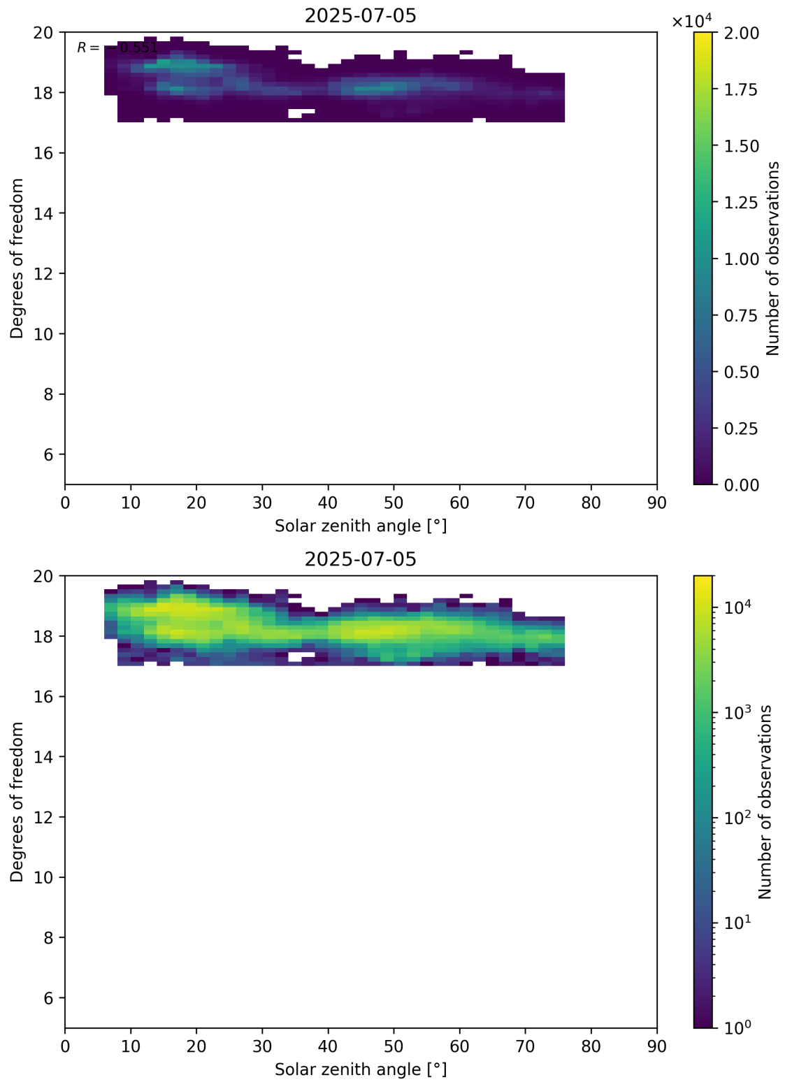
Figure 96: Scatter density plot of “Solar zenith angle” against “Degrees of freedom” for 2025-07-04 to 2025-07-06.
