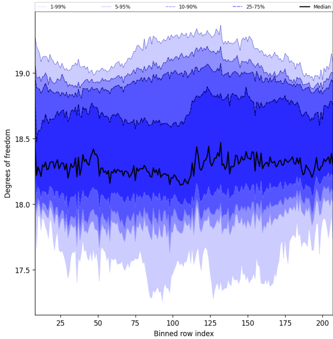
Figure 41: Along track statistics of “Degrees of freedom” for 2025-07-04 to 2025-07-06
