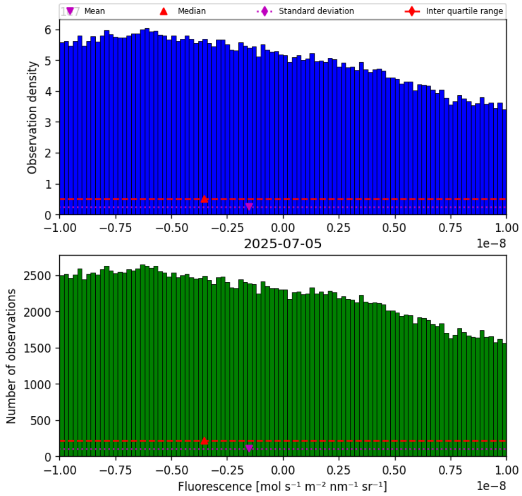
Figure 32: Histogram of “Fluorescence” for 2025-07-04 to 2025-07-06
