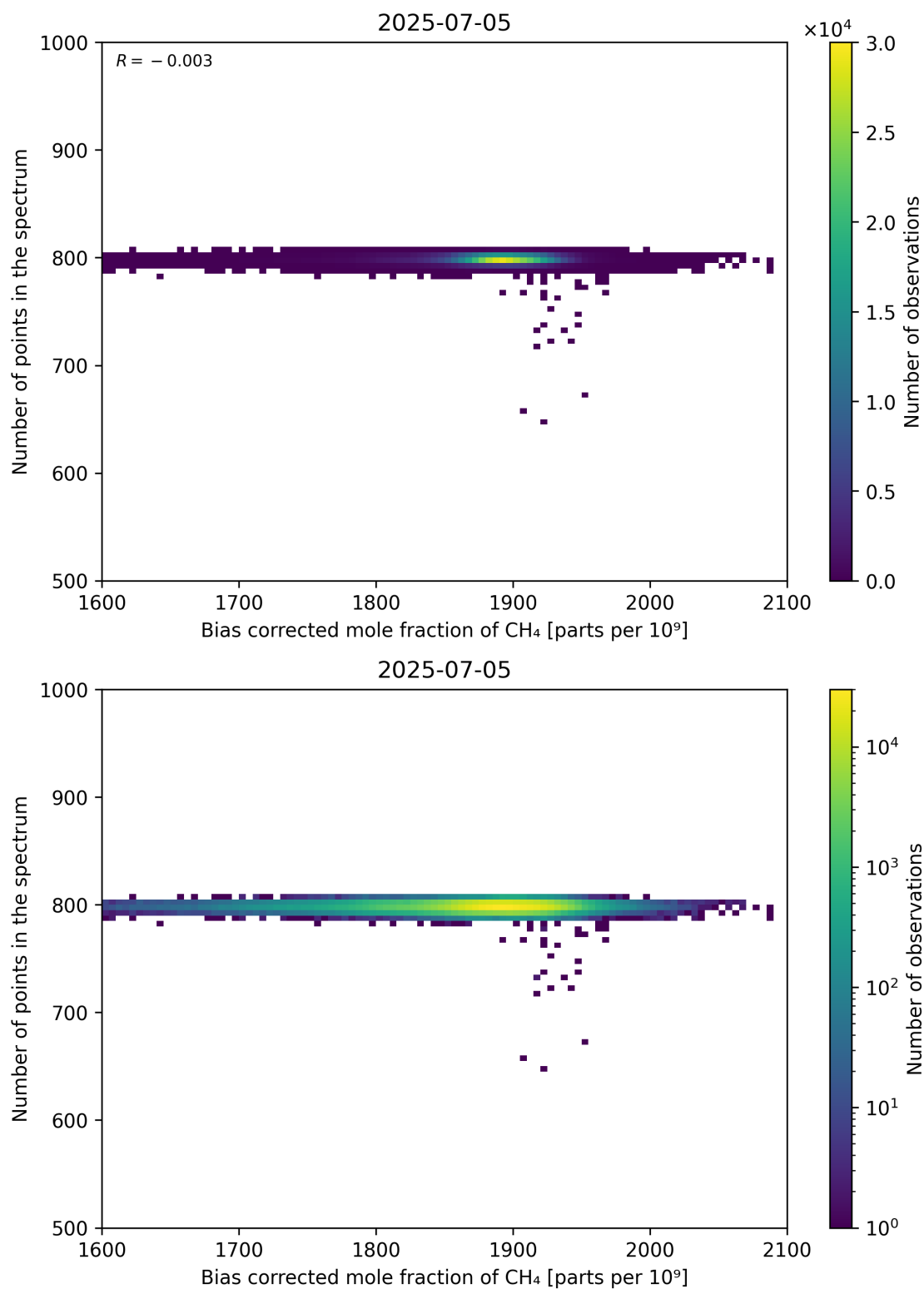
Figure 68: Scatter density plot of “Bias corrected mole fraction of CH 4 ” against “Number of points in the spectrum” for 2025-07-04 to 2025-07-06.
