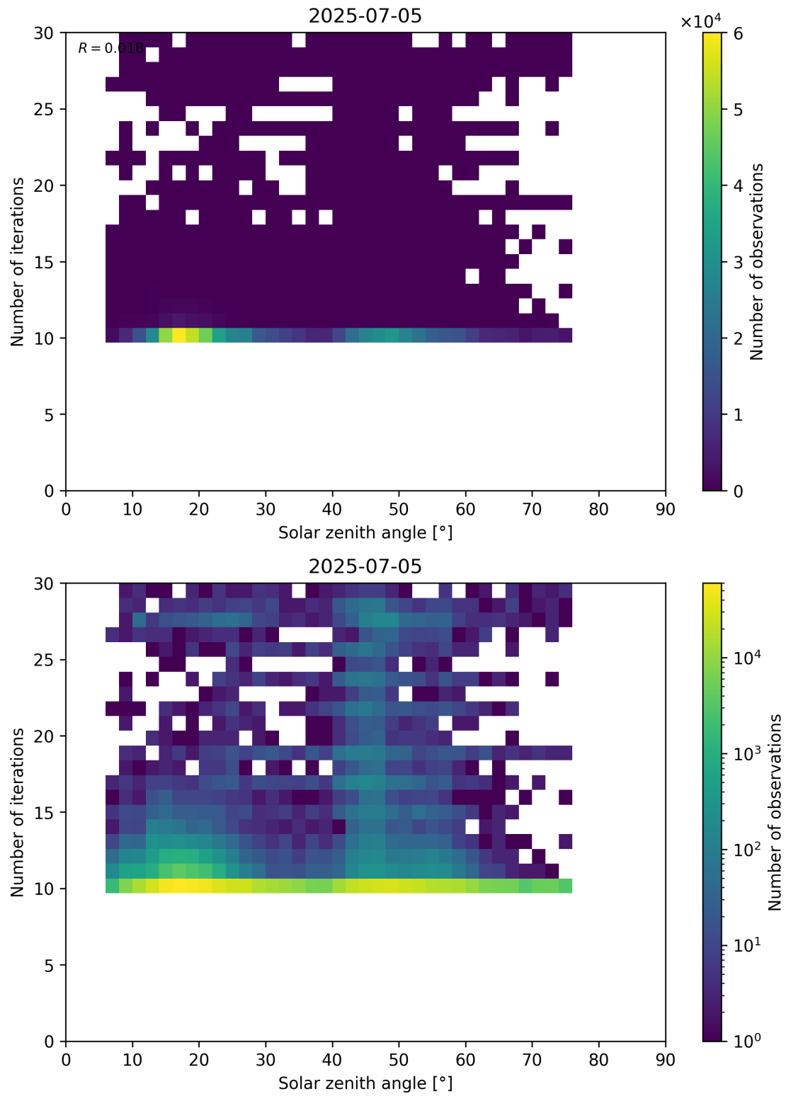
Figure 102: Scatter density plot of “Solar zenith angle” against “Number of iterations” for 2025-07-04 to 2025-07-06.
