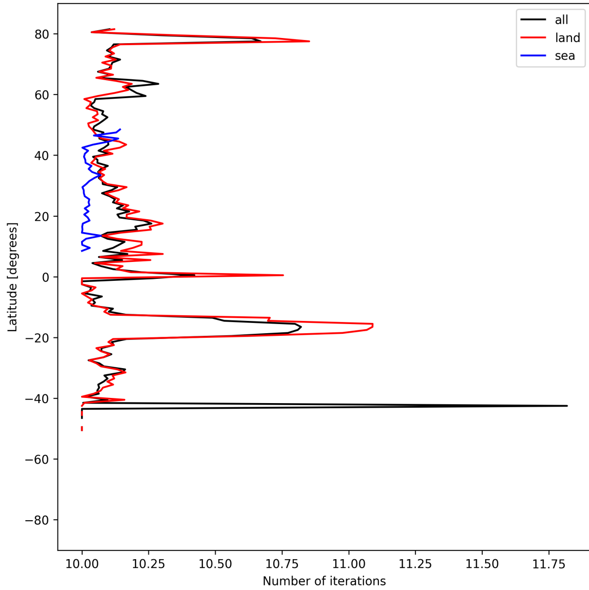
Figure 20: Zonal average of “Number of iterations” for 2025-07-04 to 2025-07-06.
