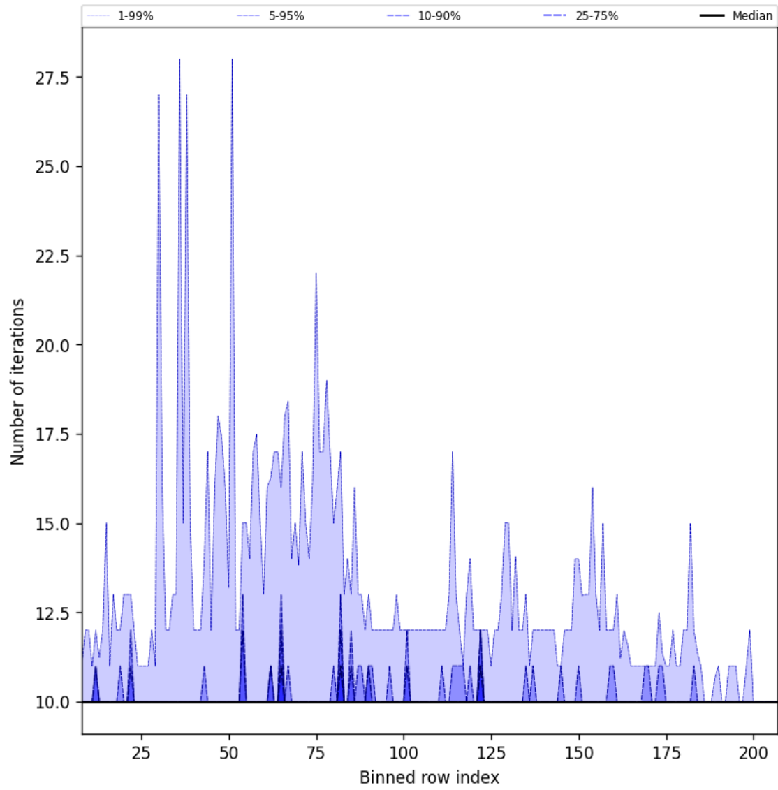
Figure 42: Along track statistics of “Number of iterations” for 2025-07-04 to 2025-07-06
