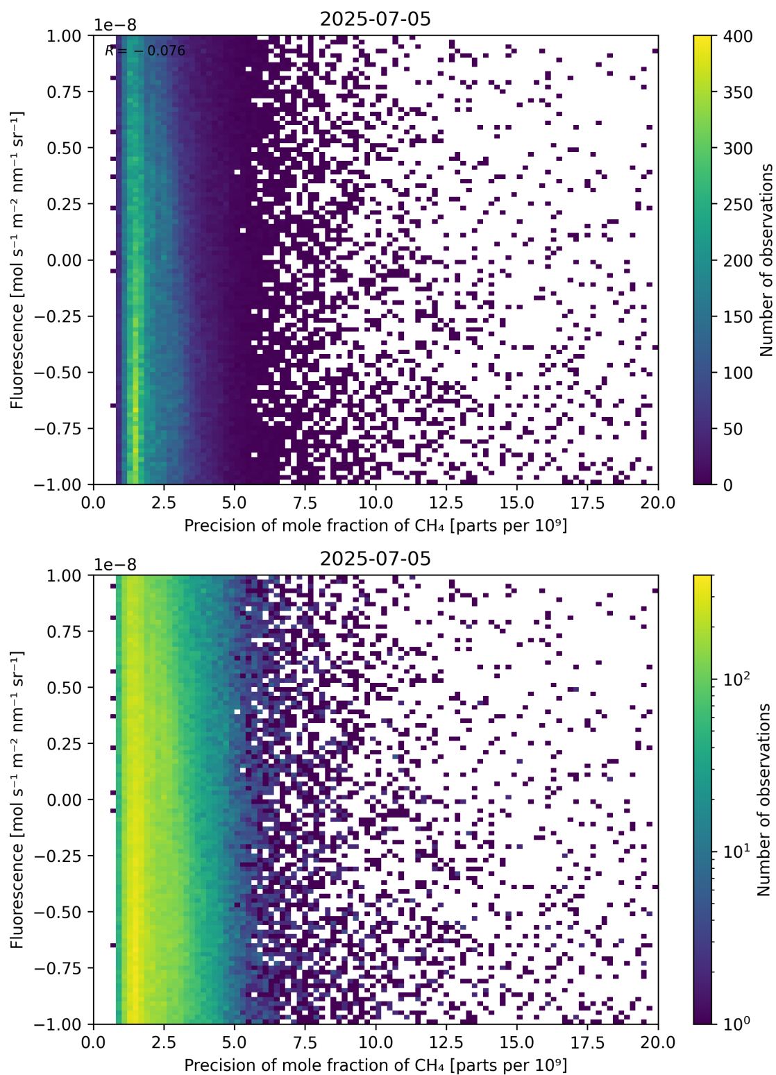
Figure 81: Scatter density plot of “Precision of mole fraction of \text{CH}_4 ” against “Fluorescence” for 2025-07-04 to 2025-07-06.
