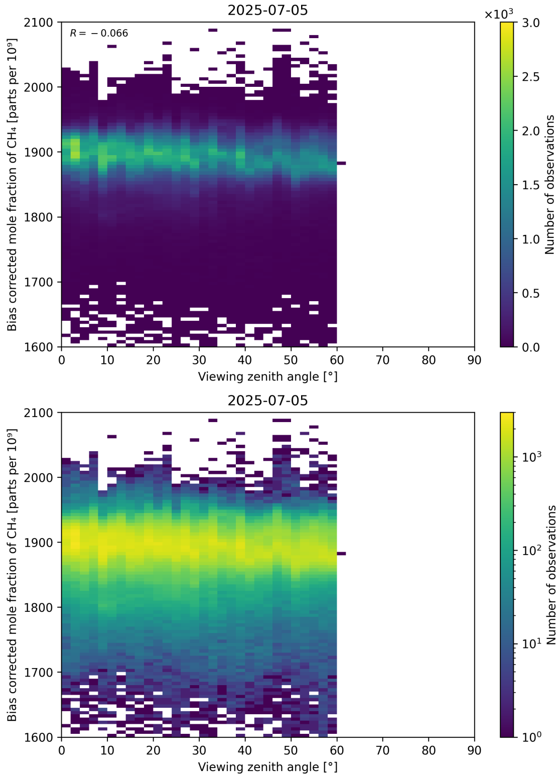
Figure 111: Scatter density plot of “Viewing zenith angle” against “Bias corrected mole fraction of CH 4 ” for 2025-07-04 to 2025-07-06.
