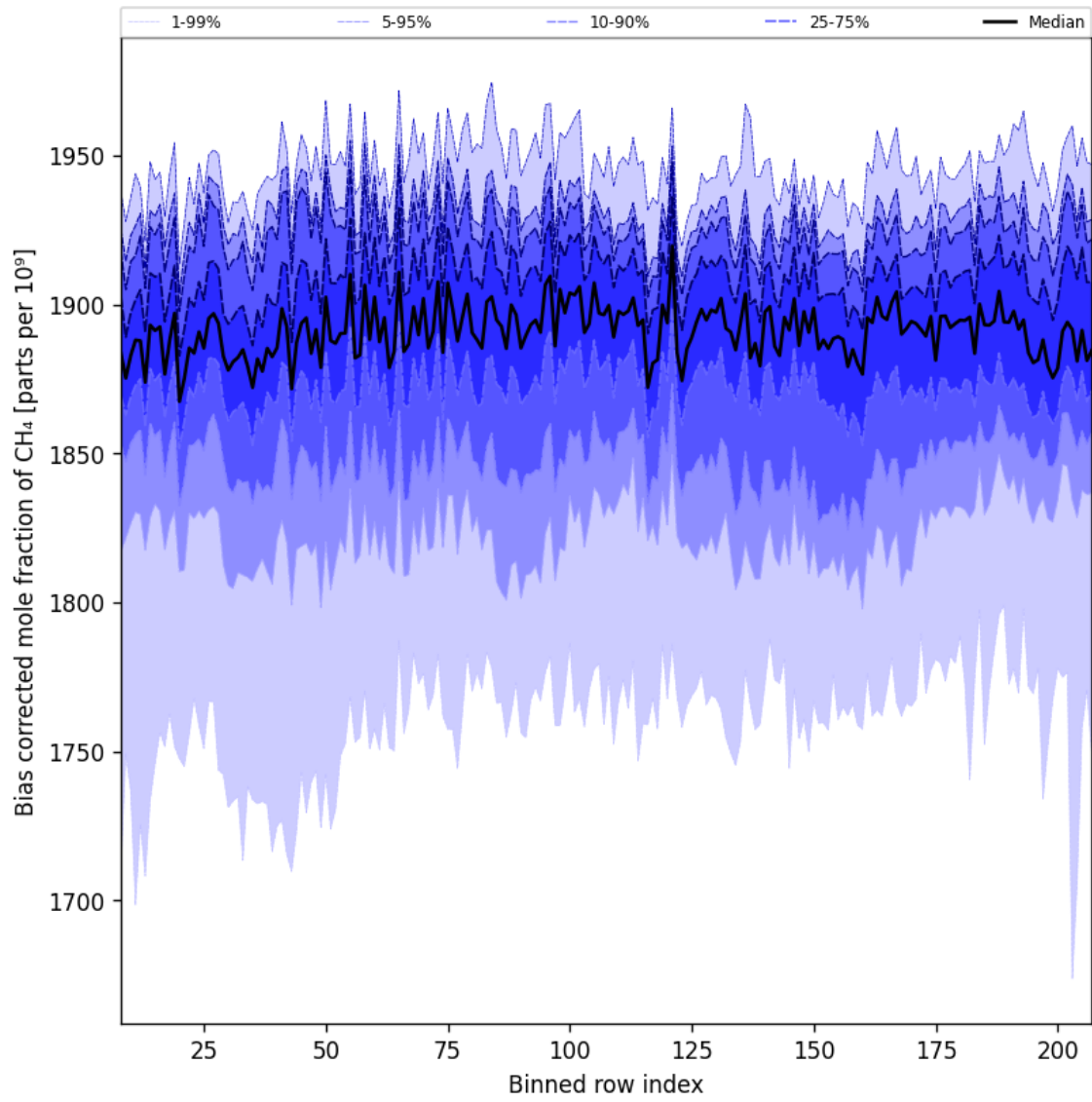
Figure 36: Along track statistics of “Bias corrected mole fraction of CH 4 ” for 2025-07-04 to 2025-07-06
