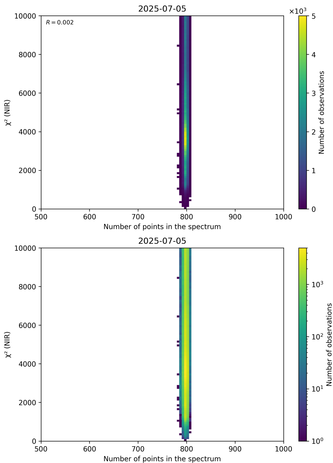
Figure 88: Scatter density plot of “Number of points in the spectrum” against “ \chi^2 (NIR)” for 2025-07-04 to 2025-07-06.
