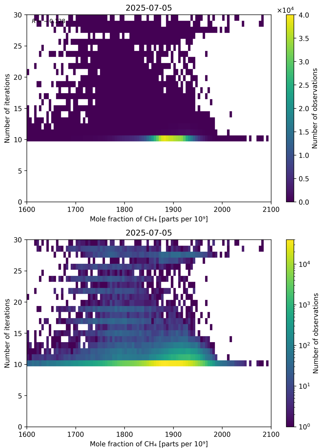
Figure 76: Scatter density plot of “Mole fraction of CH 4 ” against “Number of iterations” for 2025-07-04 to 2025-07-06.
