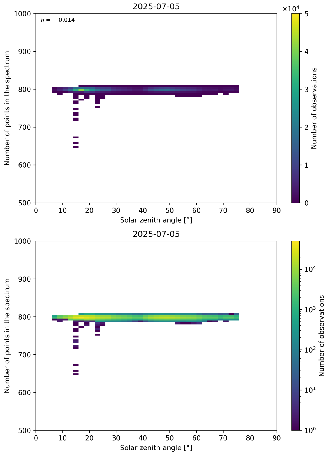
Figure 103: Scatter density plot of “Solar zenith angle” against “Number of points in the spectrum” for 2025-07-04 to 2025-07-06.
