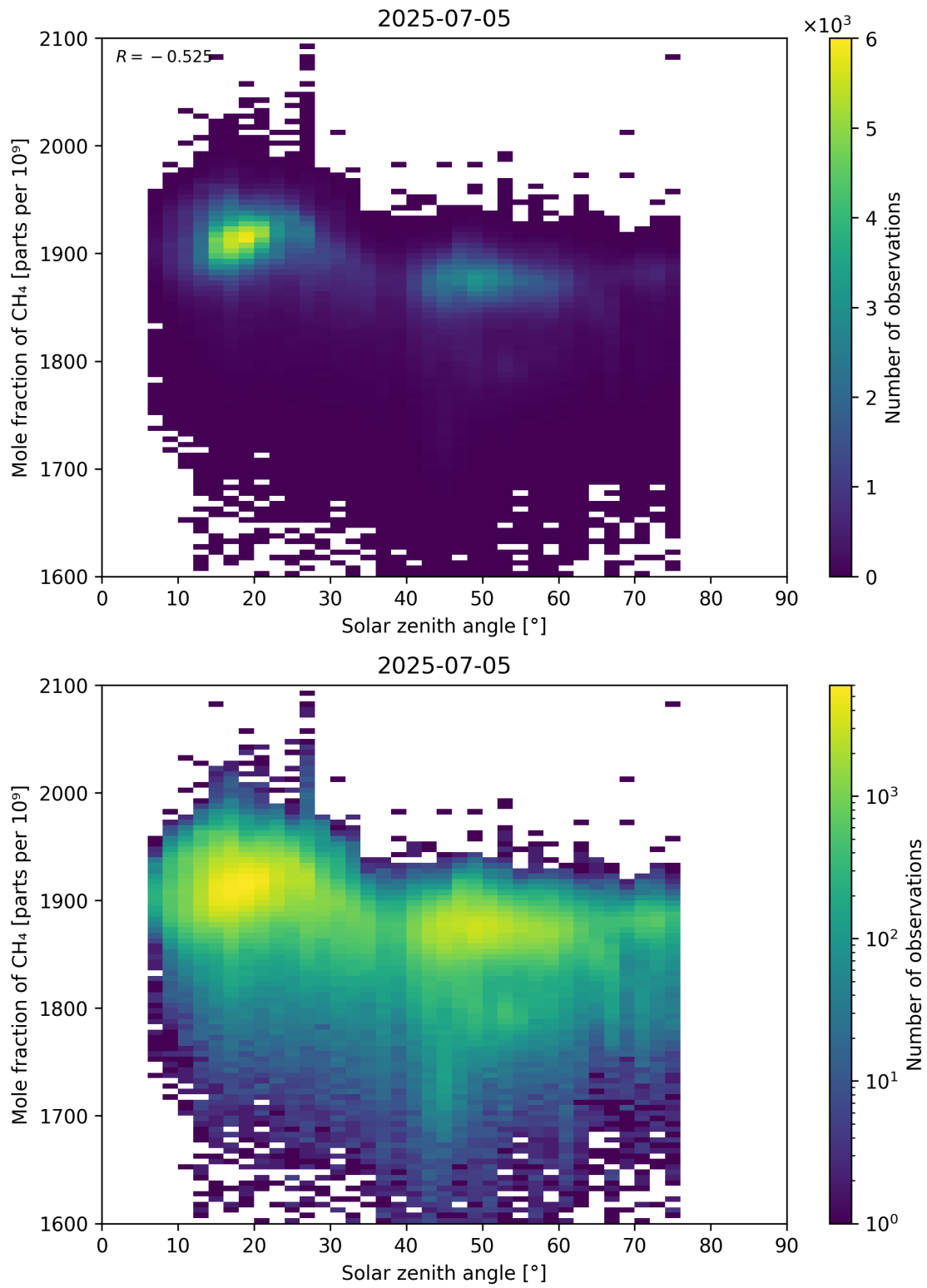
Figure 99: Scatter density plot of “Solar zenith angle” against “Mole fraction of \text{CH}_4 ” for 2025-07-04 to 2025-07-06.
