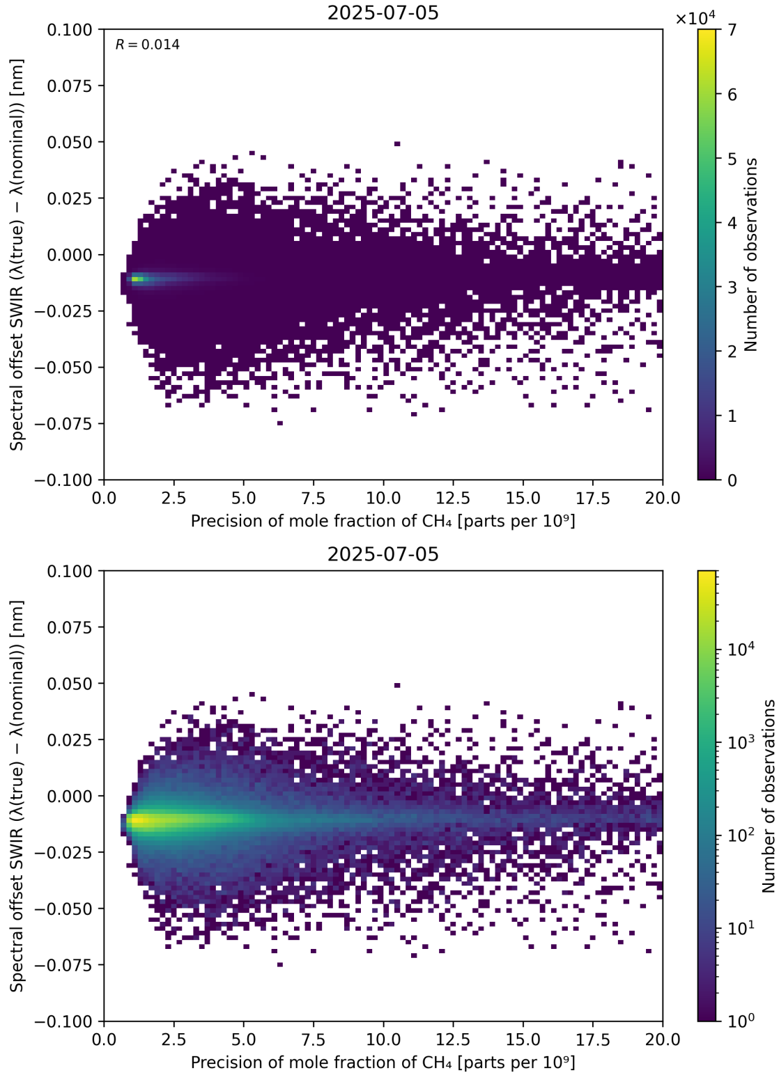
Figure 85: Scatter density plot of “Precision of mole fraction of CH 4 ” against “Spectral offset SWIR ( \lambda_{\text{true}} - \lambda_{\text{nominal}} )” for 2025-07-04 to 2025-07-06.
