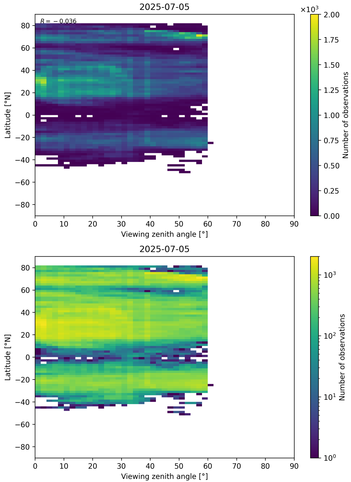
Figure 109: Scatter density plot of “Viewing zenith angle” against “Latitude” for 2025-07-04 to 2025-07-06.
