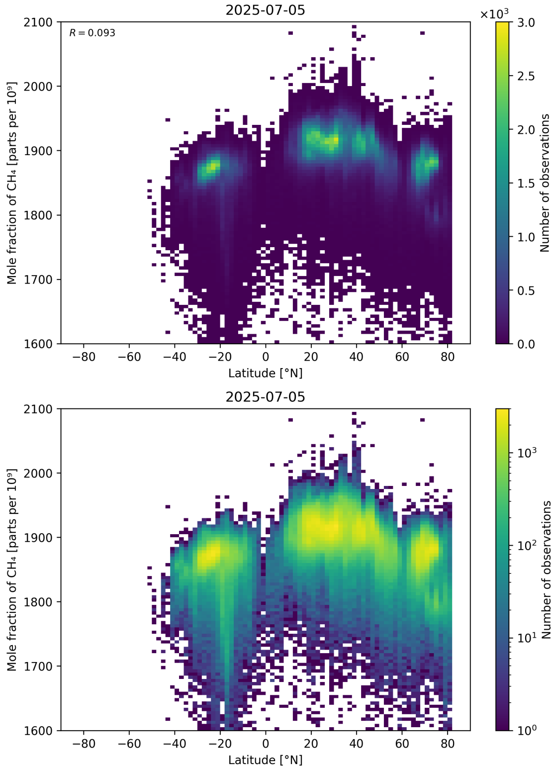
Figure 57: Scatter density plot of “Latitude” against “Mole fraction of \text{CH}_4 ” for 2025-07-04 to 2025-07-06.
