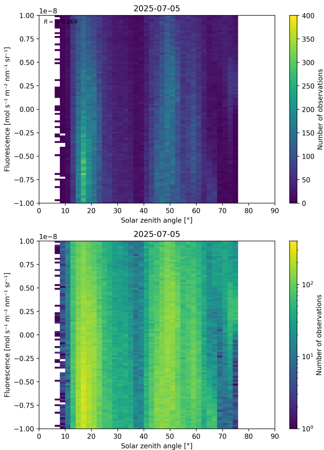
Figure 97: Scatter density plot of “Solar zenith angle” against “Fluorescence” for 2025-07-04 to 2025-07-06.
