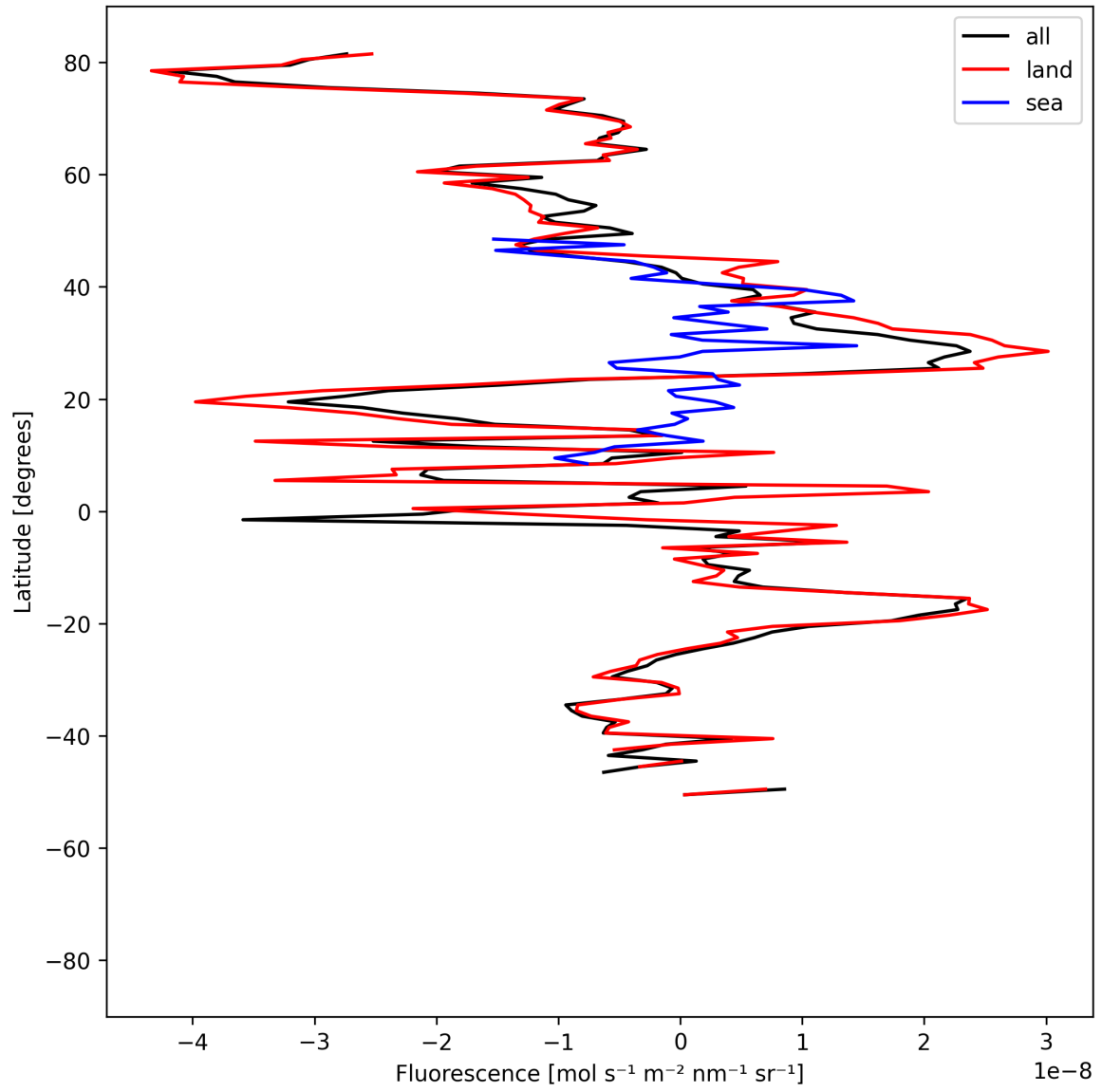
Figure 21: Zonal average of “Fluorescence” for 2025-07-04 to 2025-07-06.
