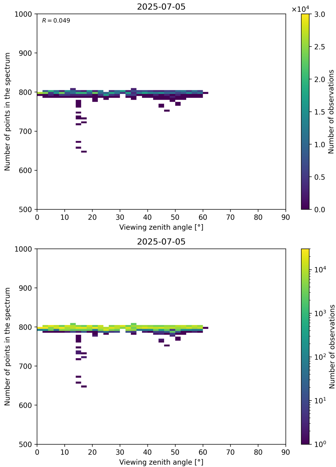
Figure 114: Scatter density plot of “Viewing zenith angle” against “Number of points in the spectrum” for 2025-07-04 to 2025-07-06.
