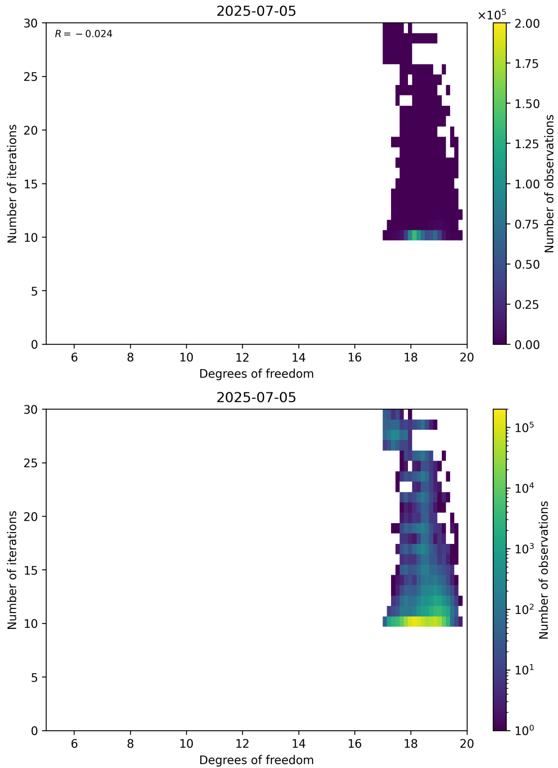
Figure 52: Scatter density plot of “Degrees of freedom” against “Number of iterations” for 2025-07-04 to 2025-07-06.
