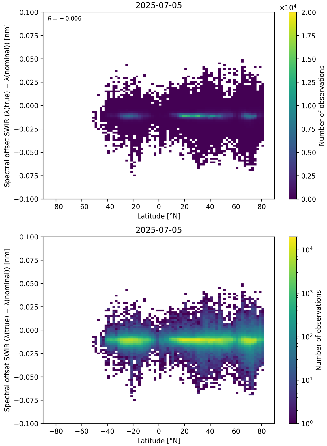
Figure 62: Scatter density plot of “Latitude” against “Spectral offset SWIR ( \lambda_{\text{true}} - \lambda_{\text{nominal}} )” for 2025-07-04 to 2025-07-06.
