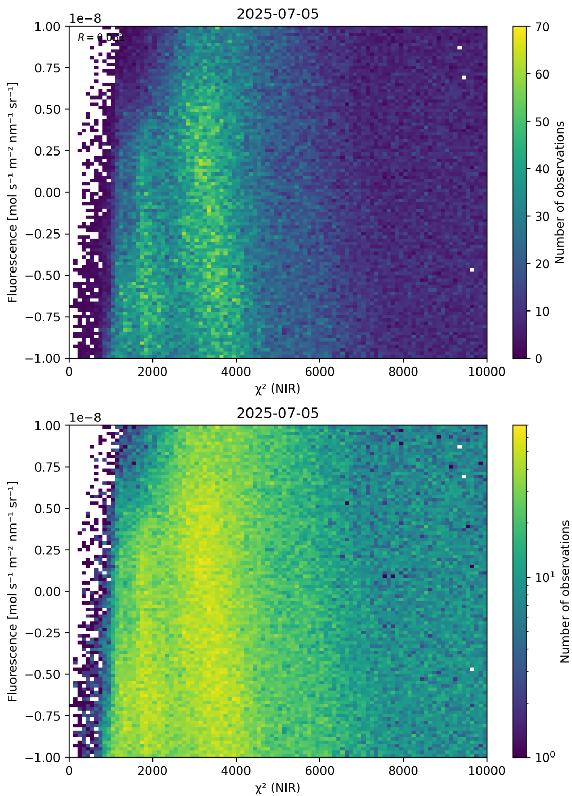
Figure 45: Scatter density plot of “ \chi^2 (NIR)” against “Fluorescence” for 2025-07-04 to 2025-07-06.
