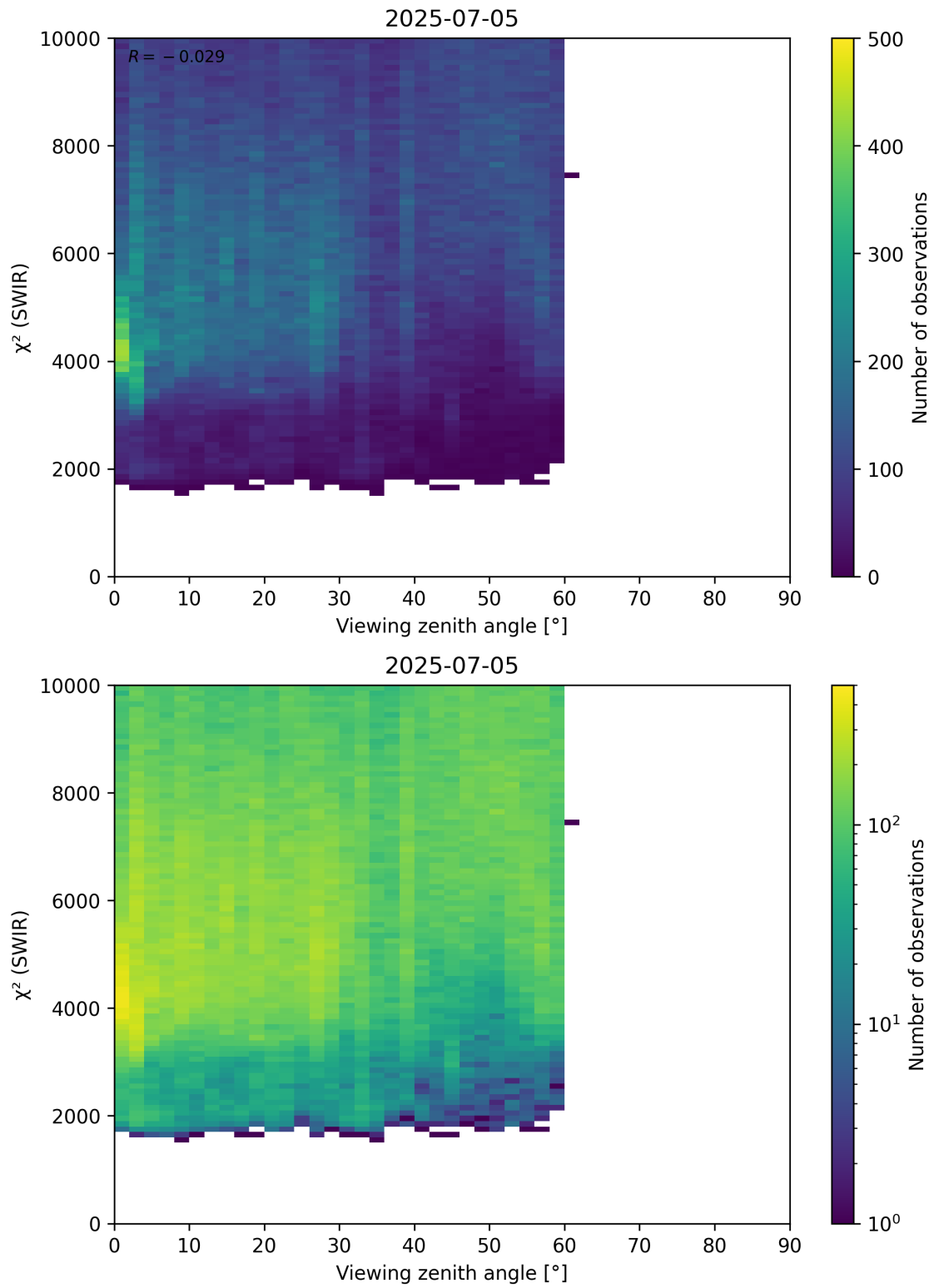
Figure 106: Scatter density plot of “Viewing zenith angle” against “ \chi^2 (SWIR)” for 2025-07-04 to 2025-07-06.
