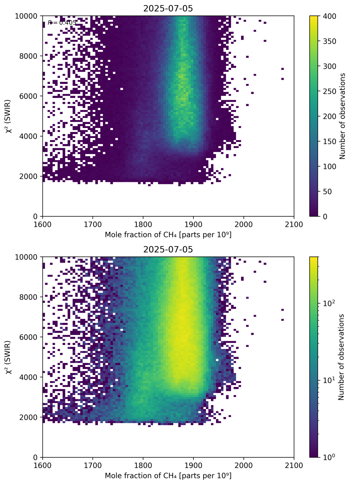
Figure 71: Scatter density plot of “Mole fraction of CH 4 ” against “ \chi^2 (SWIR)” for 2025-07-04 to 2025-07-06.
