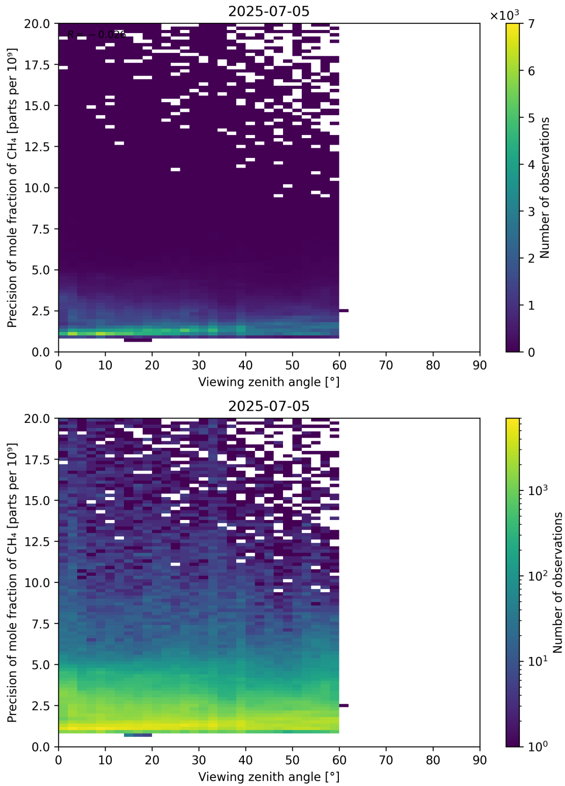
Figure 112: Scatter density plot of “Viewing zenith angle” against “Precision of mole fraction of CH 4 ” for 2025-07-04 to 2025-07-06.
