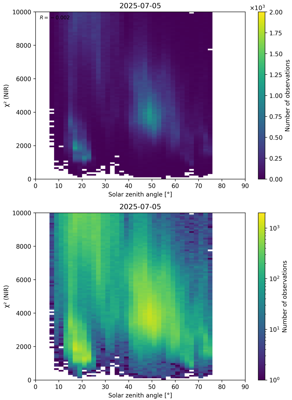
Figure 94: Scatter density plot of “Solar zenith angle” against “ \chi^2 (NIR)” for 2025-07-04 to 2025-07-06.
