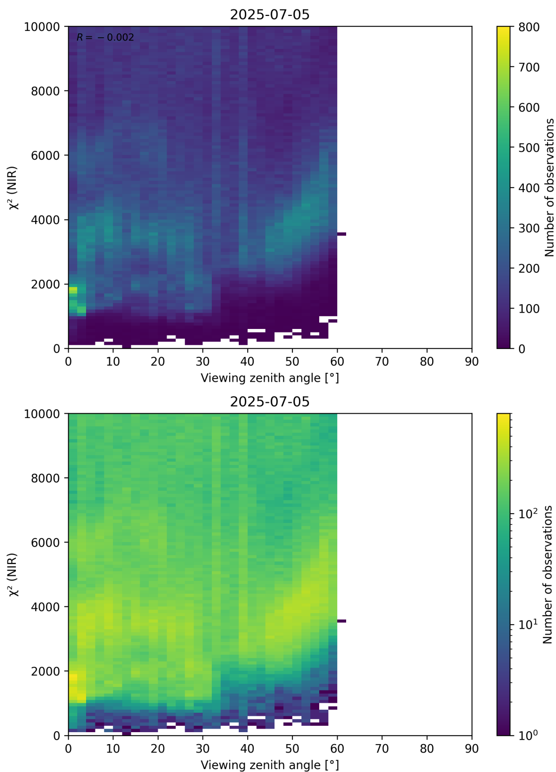
Figure 105: Scatter density plot of “Viewing zenith angle” against “ \chi^2 (NIR)” for 2025-07-04 to 2025-07-06.
