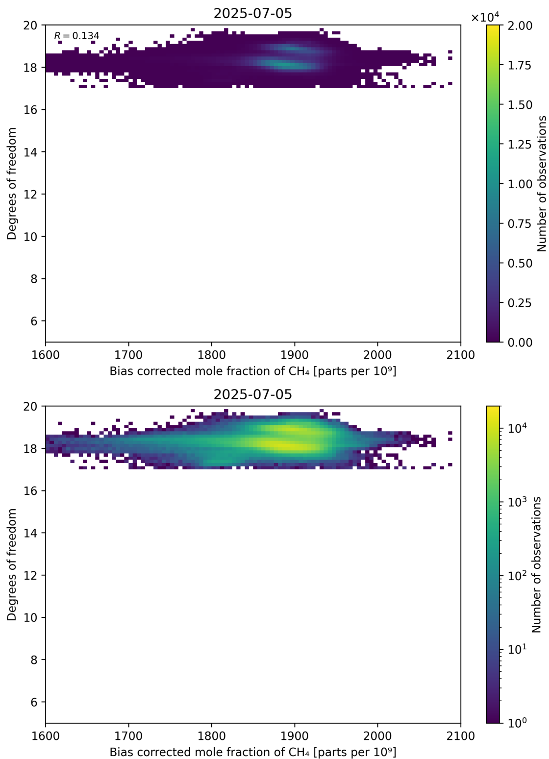
Figure 65: Scatter density plot of “Bias corrected mole fraction of CH 4 ” against “Degrees of freedom” for 2025-07-04 to 2025-07-06.
