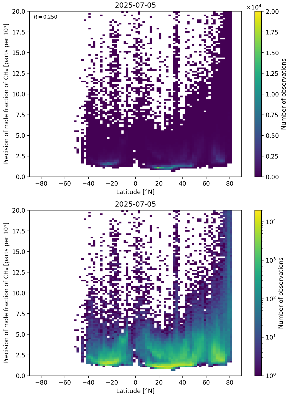
Figure 59: Scatter density plot of “Latitude” against “Precision of mole fraction of \text{CH}_4 ” for 2025-07-04 to 2025-07-06.
