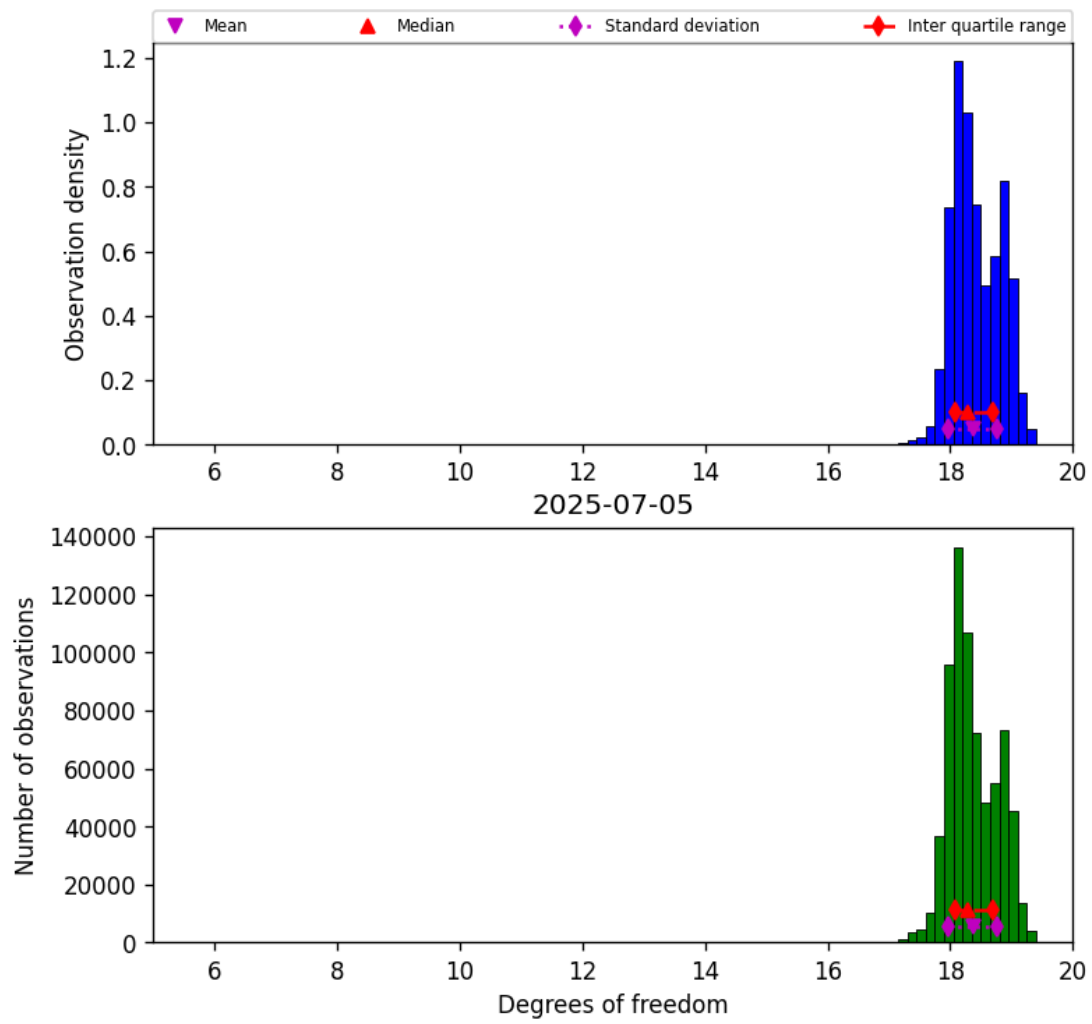
Figure 30: Histogram of “Degrees of freedom” for 2025-07-04 to 2025-07-06
