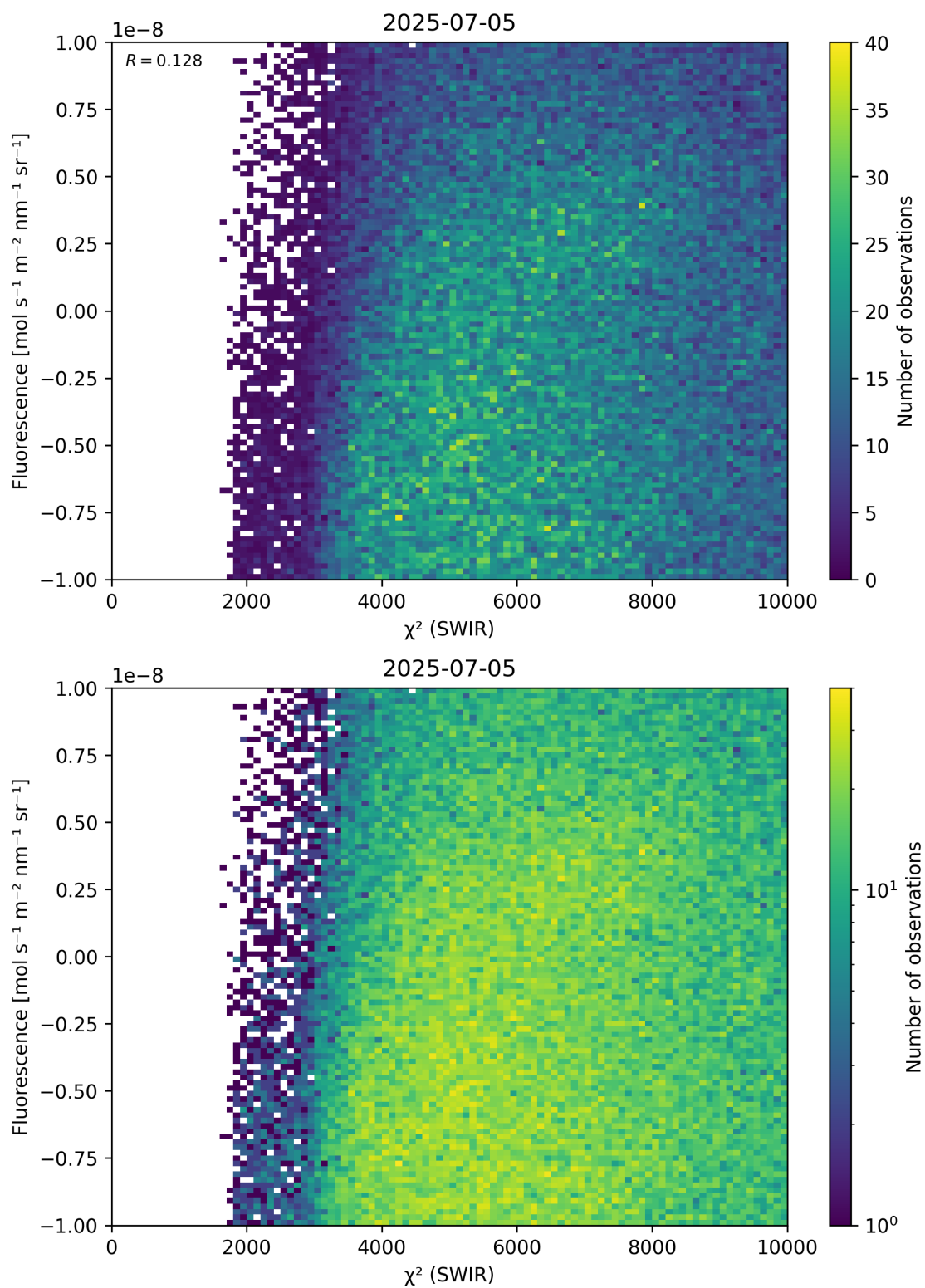
Figure 49: Scatter density plot of “ \chi^2 (SWIR)” against “Fluorescence” for 2025-07-04 to 2025-07-06.
