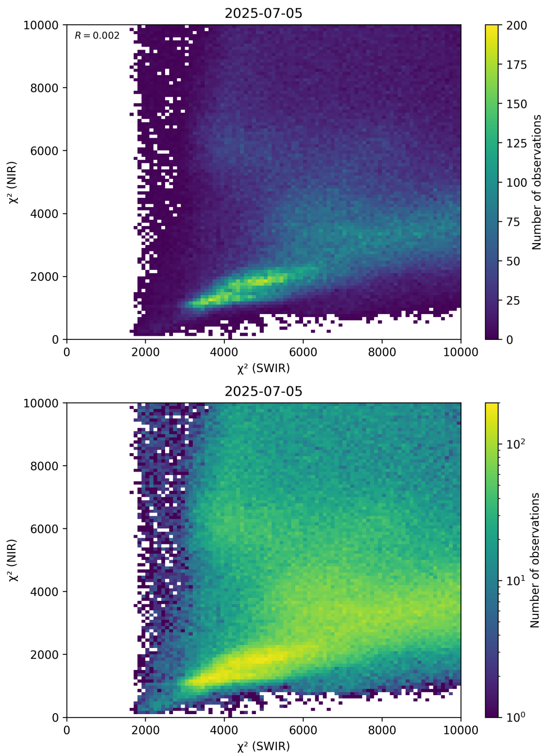
Figure 47: Scatter density plot of “ \chi^2 (SWIR)” against “ \chi^2 (NIR)” for 2025-07-04 to 2025-07-06.
