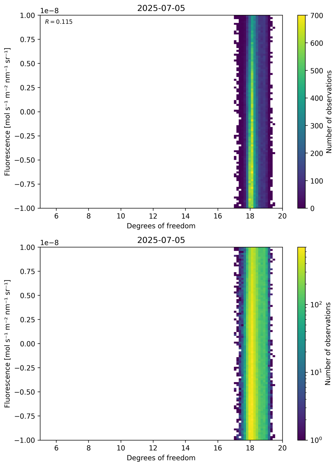
Figure 51: Scatter density plot of “Degrees of freedom” against “Fluorescence” for 2025-07-04 to 2025-07-06.
