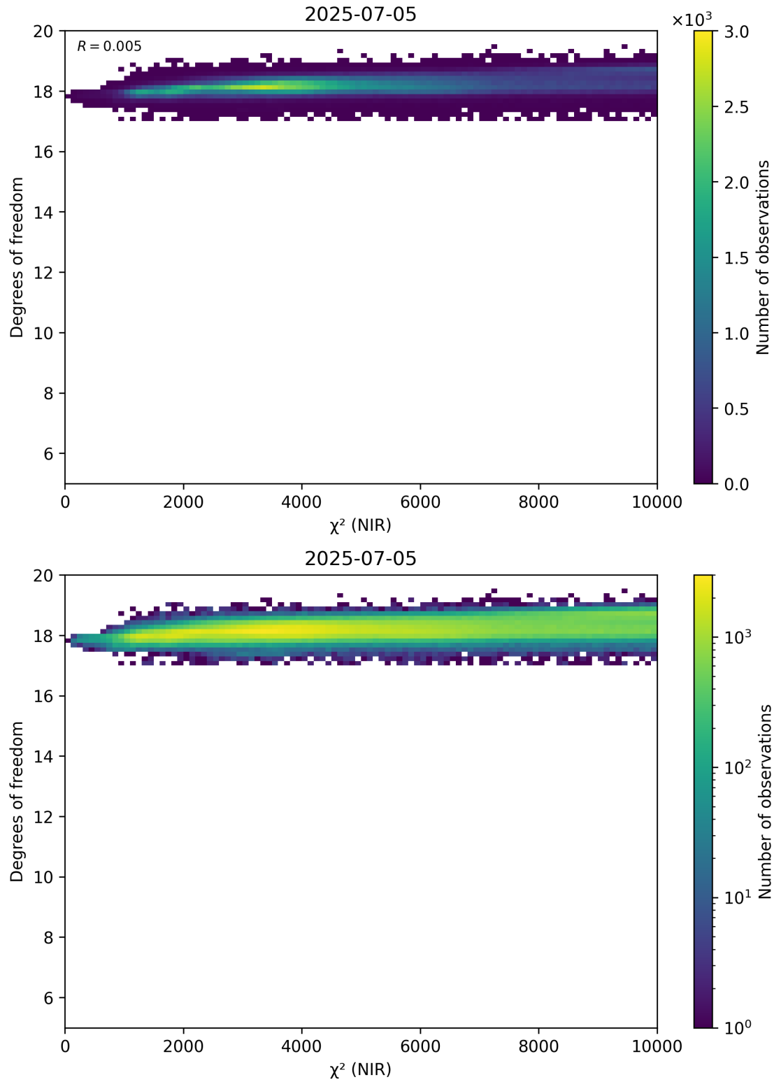
Figure 44: Scatter density plot of “ \chi^2 (NIR)” against “Degrees of freedom” for 2025-07-04 to 2025-07-06.
