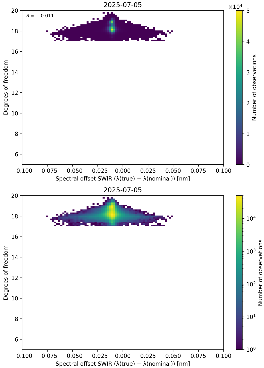
Figure 119: Scatter density plot of “Spectral offset SWIR ( \lambda_{\text{true}} - \lambda_{\text{nominal}} )” against “Degrees of freedom” for 2025-07-04 to 2025-07-06.
