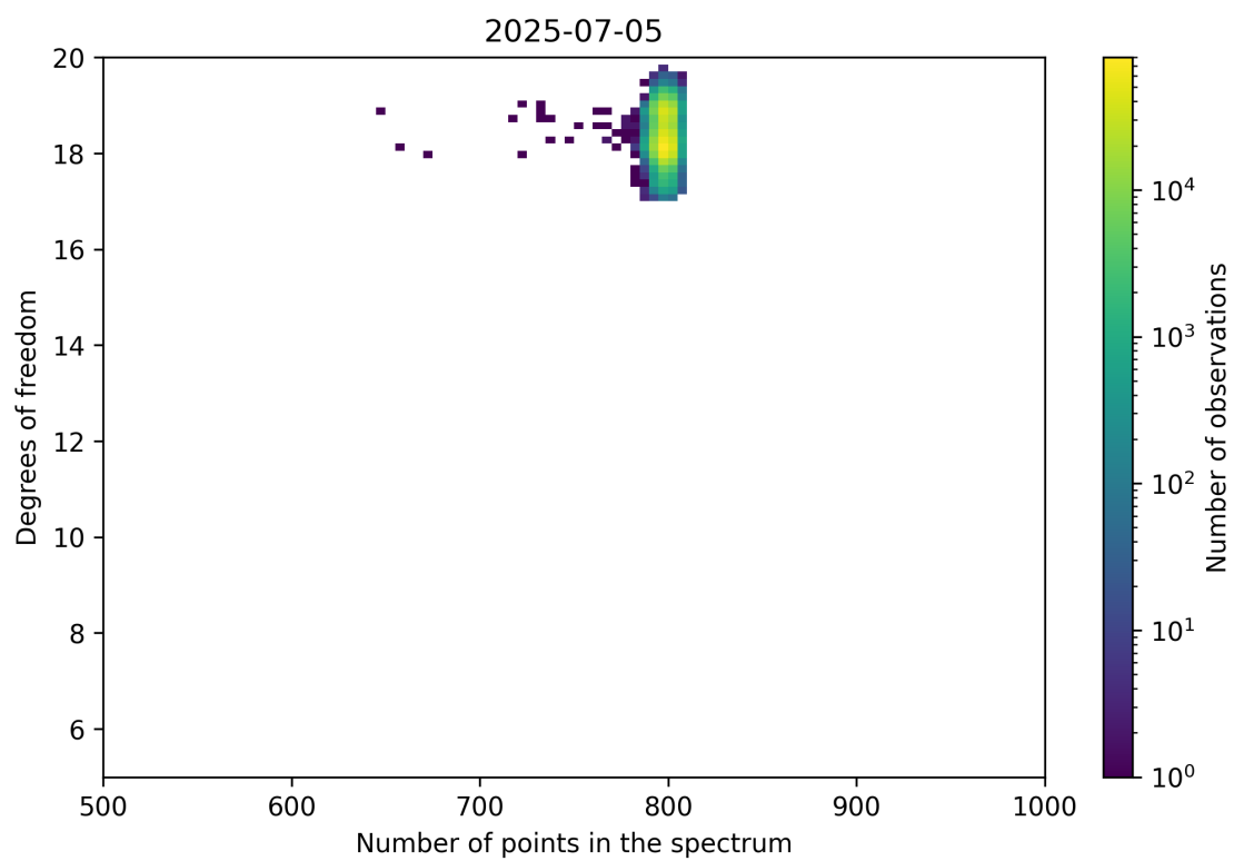
Figure 90: Scatter density plot of “Number of points in the spectrum” against “Degrees of freedom” for 2025-07-04 to 2025-07-06.
