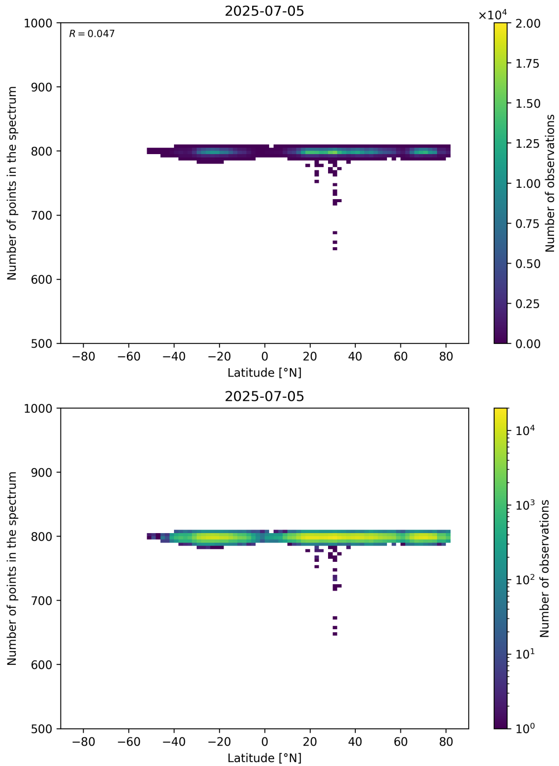
Figure 61: Scatter density plot of “Latitude” against “Number of points in the spectrum” for 2025-07-04 to 2025-07-06.
