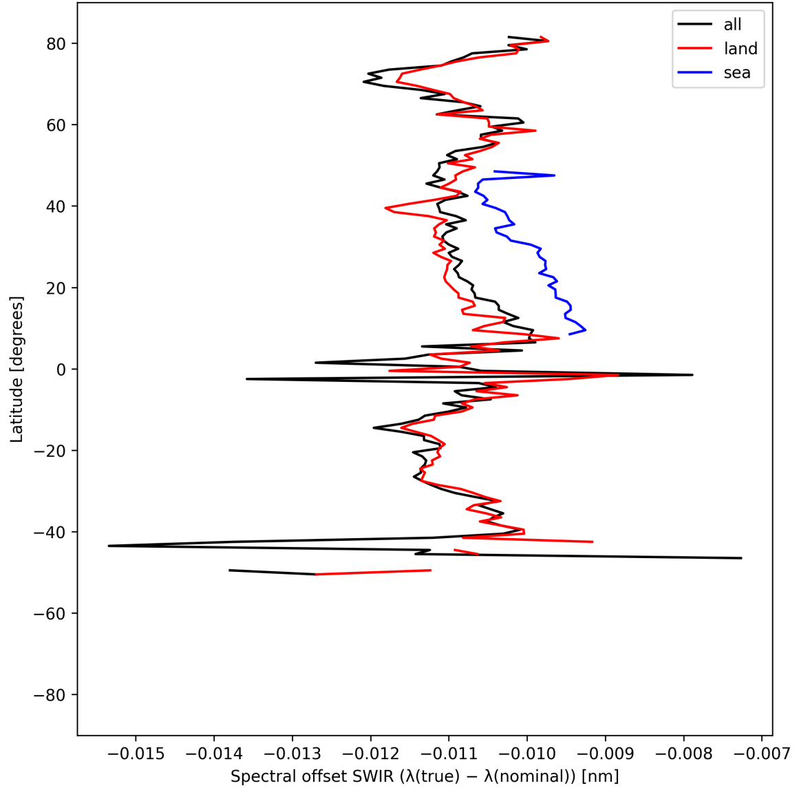
Figure 16: Zonal average of “Spectral offset SWIR ( \lambda_{\text{true}} - \lambda_{\text{nominal}} )” for 2025-07-04 to 2025-07-06.
