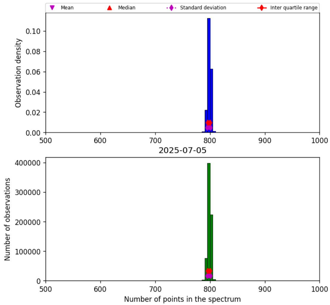
Figure 26: Histogram of “Number of points in the spectrum” for 2025-07-04 to 2025-07-06
