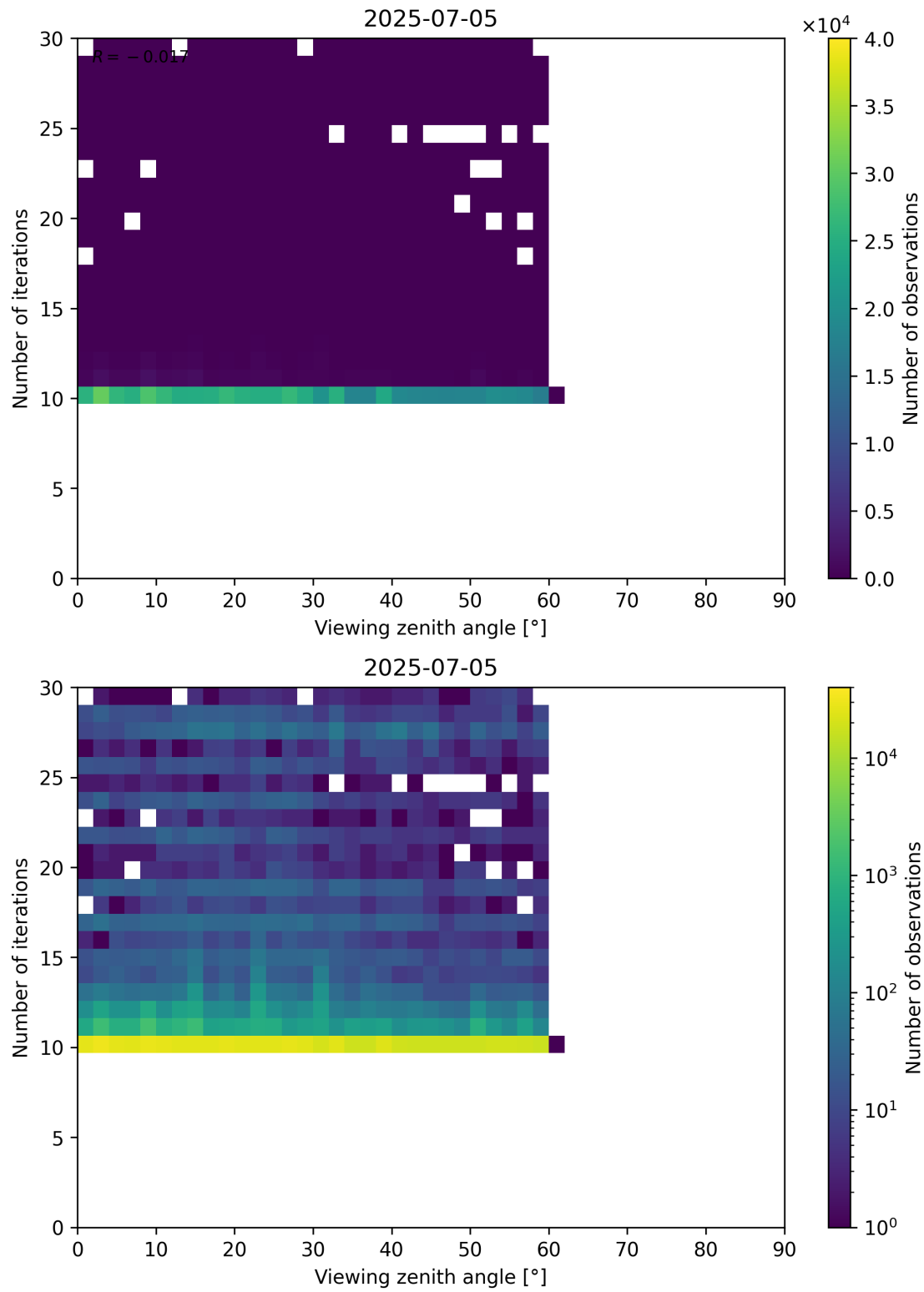
Figure 113: Scatter density plot of “Viewing zenith angle” against “Number of iterations” for 2025-07-04 to 2025-07-06.
