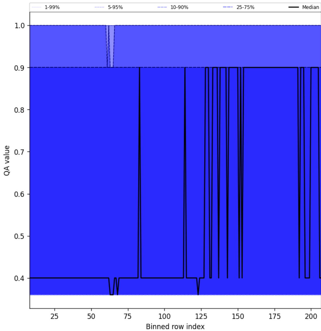
Figure 33: Along track statistics of “QA value” for 2025-07-04 to 2025-07-06
