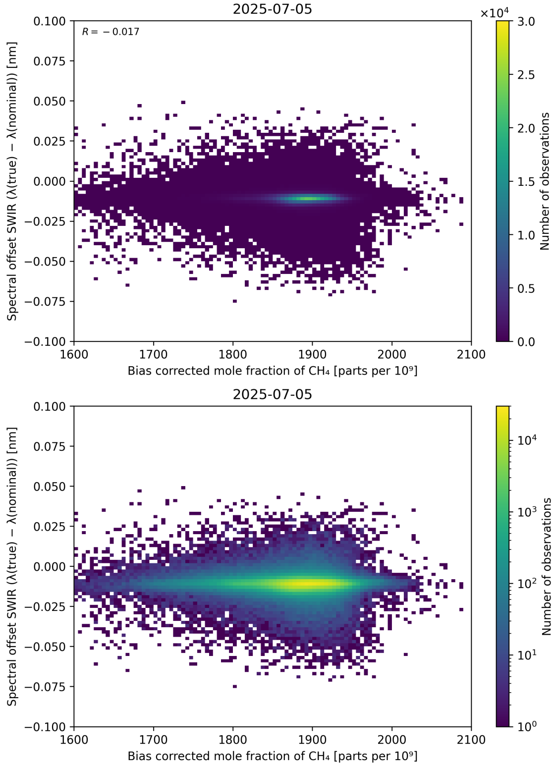
Figure 69: Scatter density plot of “Bias corrected mole fraction of CH 4 ” against “Spectral offset SWIR ( \lambda_{\text{true}} - \lambda_{\text{nominal}} )” for 2025-07-04 to 2025-07-06.
