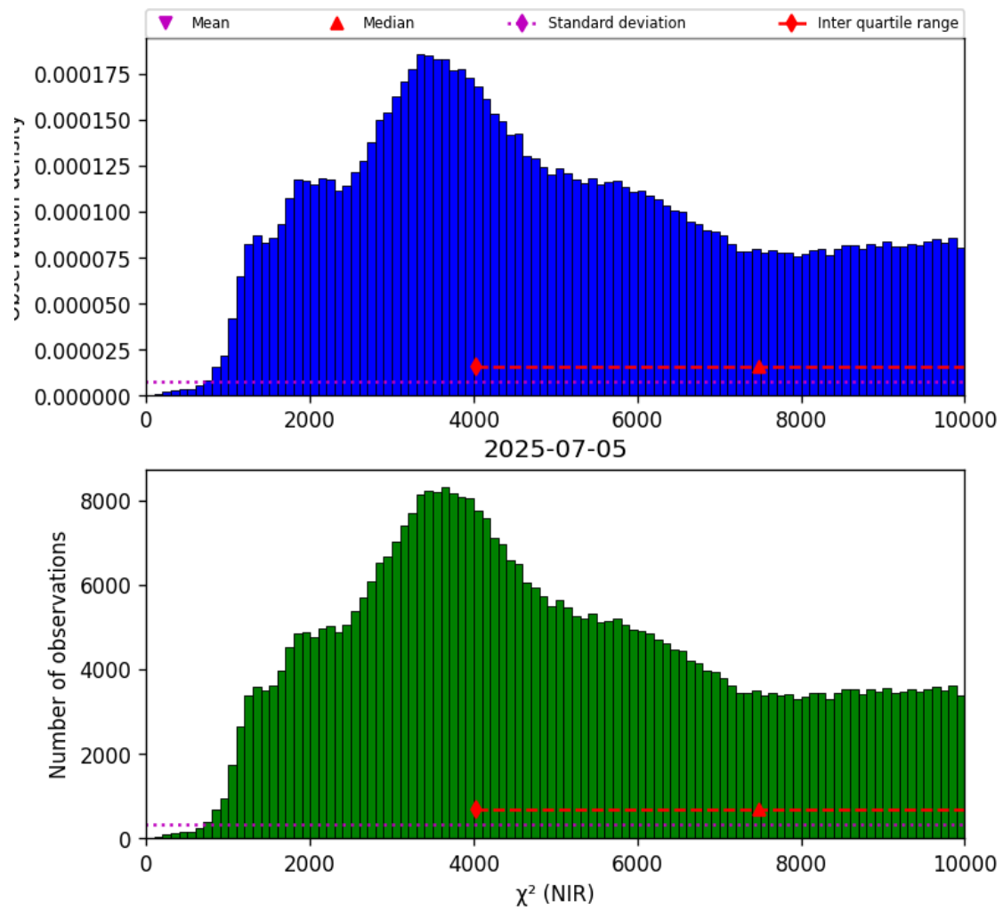
Figure 29: Histogram of “ \chi^2 (NIR)” for 2025-07-04 to 2025-07-06
