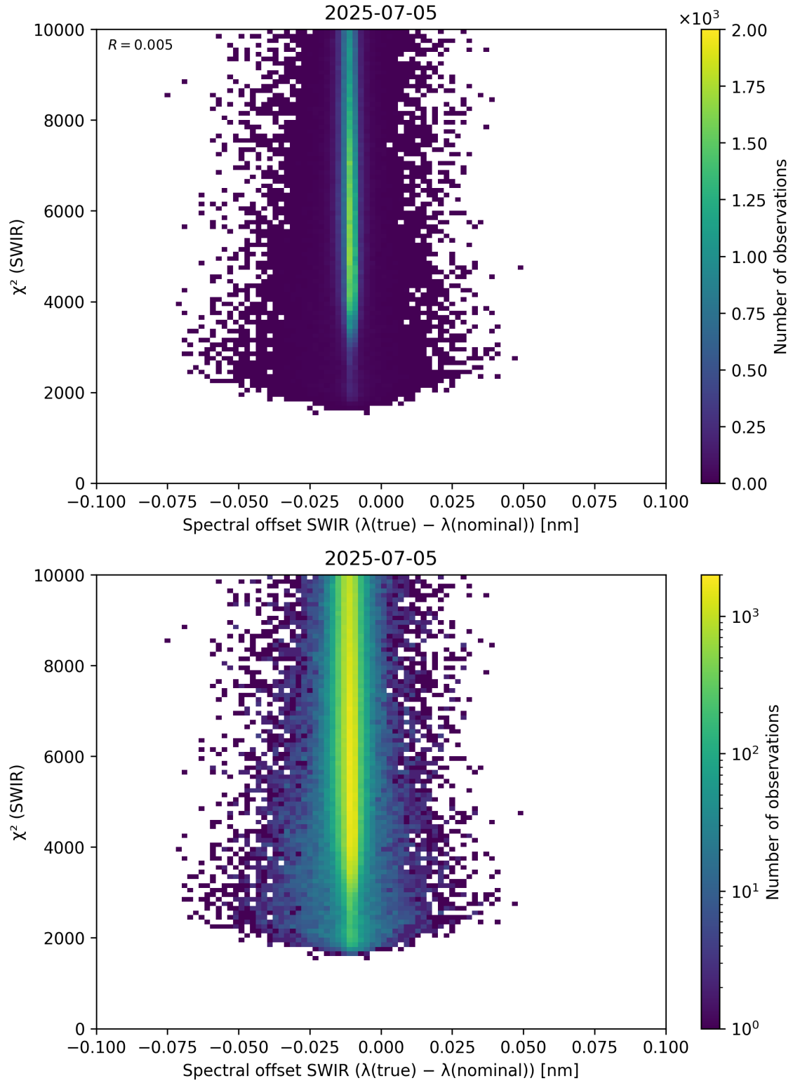
Figure 118: Scatter density plot of “Spectral offset SWIR ( \lambda_{\text{true}} - \lambda_{\text{nominal}} )” against “ \chi^2 (SWIR)” for 2025-07-04 to 2025-07-06.
