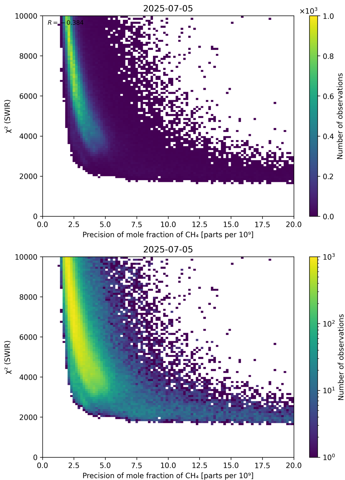
Figure 79: Scatter density plot of “Precision of mole fraction of CH 4 ” against “ \chi^2 (SWIR)” for 2025-07-04 to 2025-07-06.
