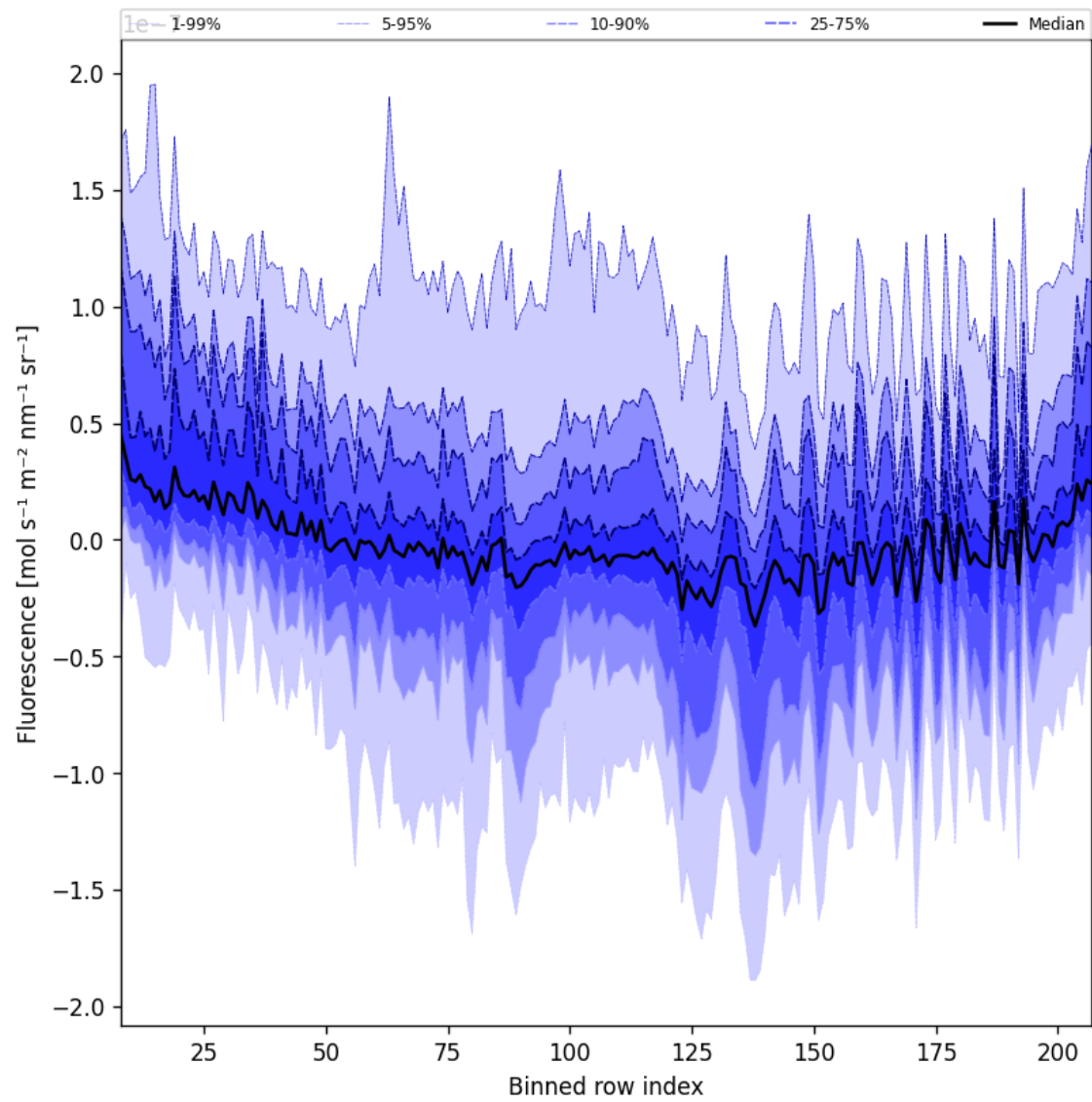
Figure 43: Along track statistics of “Fluorescence” for 2025-07-04 to 2025-07-06
