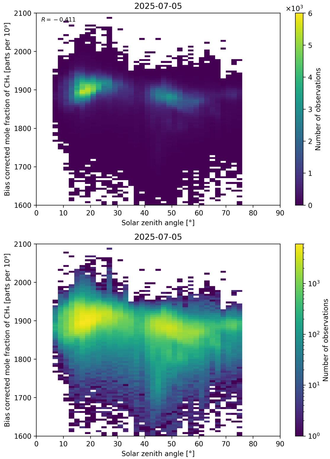
Figure 100: Scatter density plot of “Solar zenith angle” against “Bias corrected mole fraction of CH 4 ” for 2025-07-04 to 2025-07-06.
