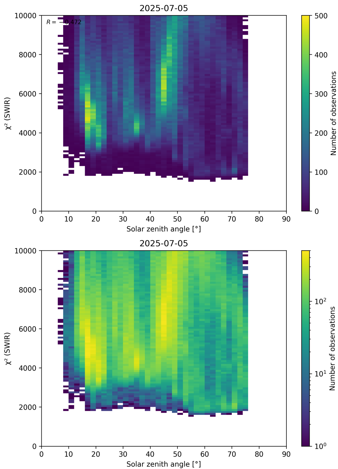
Figure 95: Scatter density plot of “Solar zenith angle” against “ \chi^2 (SWIR)” for 2025-07-04 to 2025-07-06.
