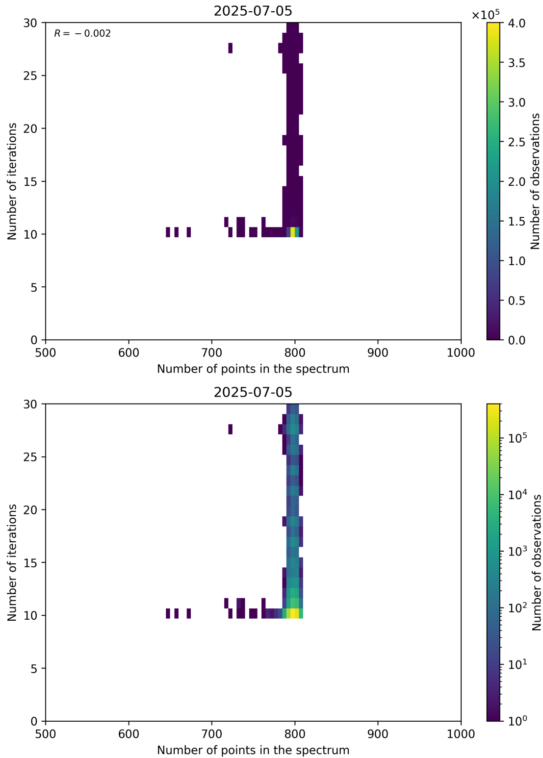
Figure 92: Scatter density plot of “Number of points in the spectrum” against “Number of iterations” for 2025-07-04 to 2025-07-06.
