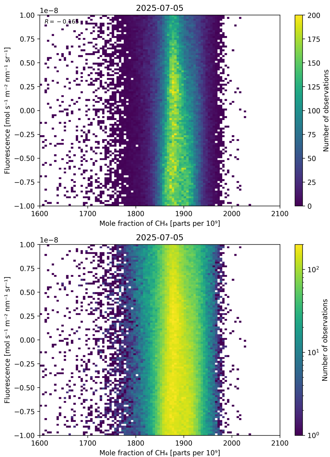
Figure 73: Scatter density plot of “Mole fraction of \text{CH}_4 ” against “Fluorescence” for 2025-07-04 to 2025-07-06.
