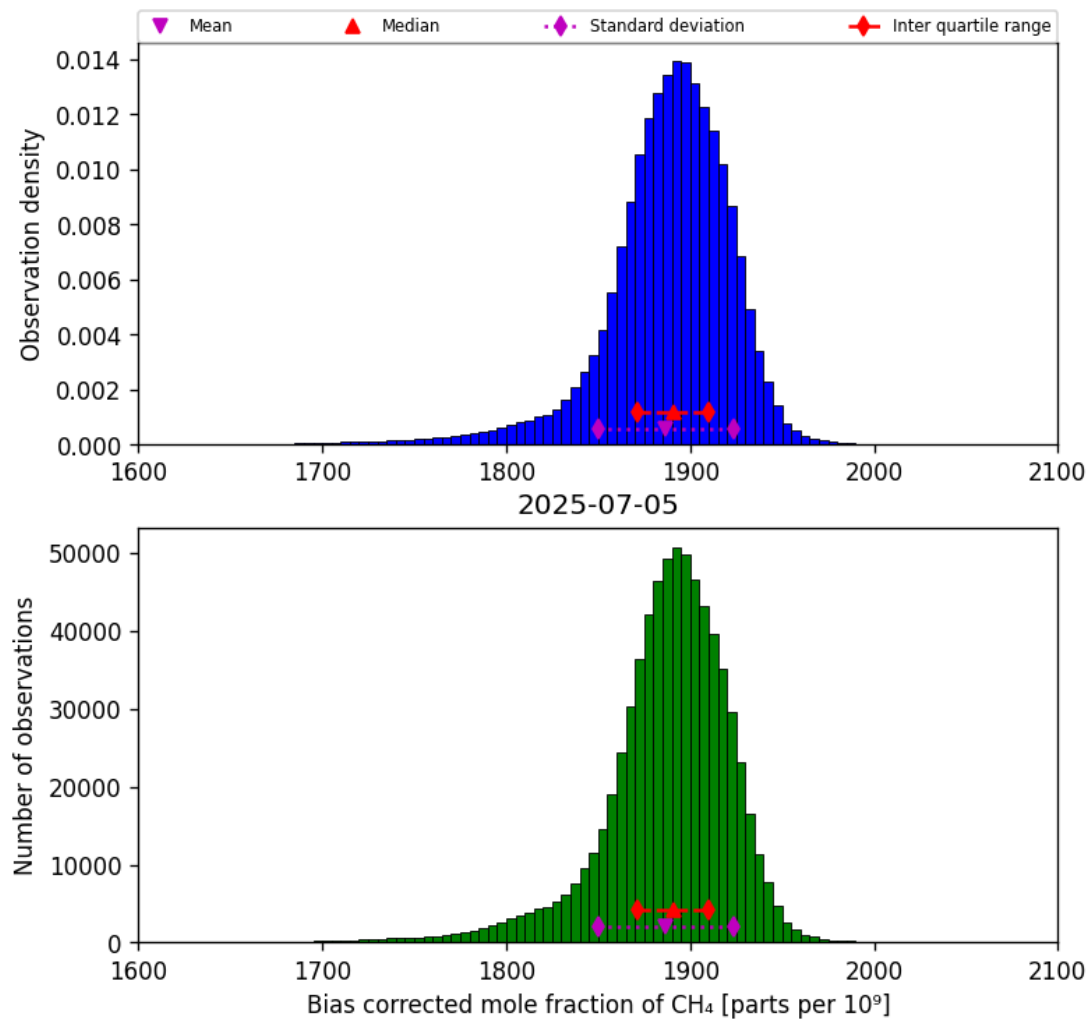
Figure 25: Histogram of “Bias corrected mole fraction of CH 4 ” for 2025-07-04 to 2025-07-06
