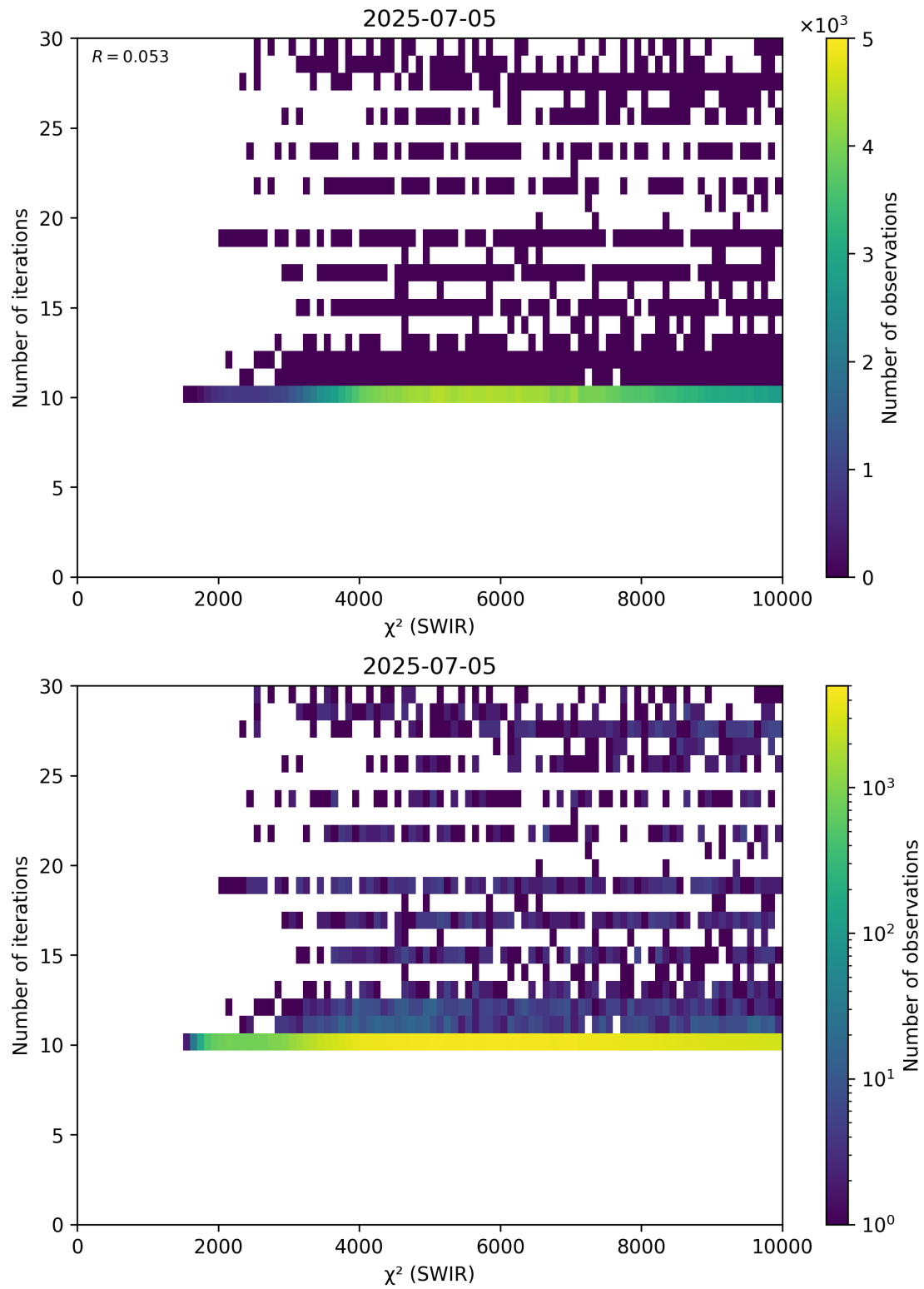
Figure 50: Scatter density plot of “ \chi^2 (SWIR)” against “Number of iterations” for 2025-07-04 to 2025-07-06.
