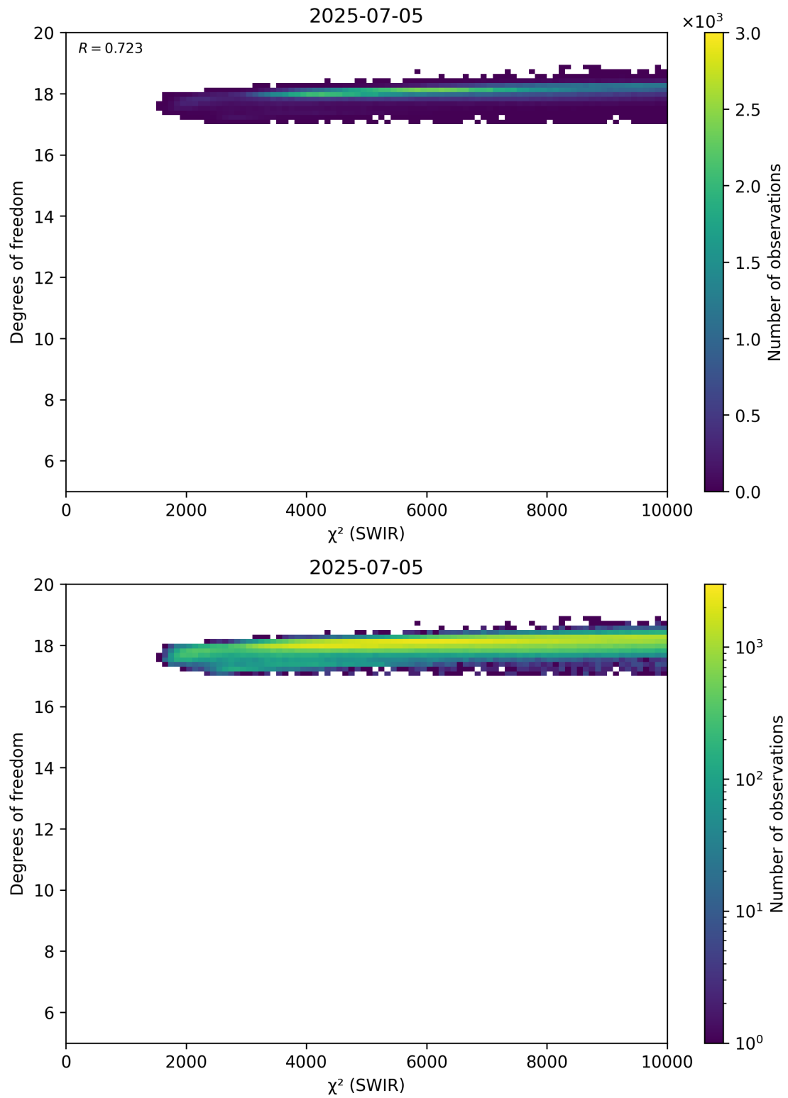
Figure 48: Scatter density plot of “ \chi^2 (SWIR)” against “Degrees of freedom” for 2025-07-04 to 2025-07-06.
