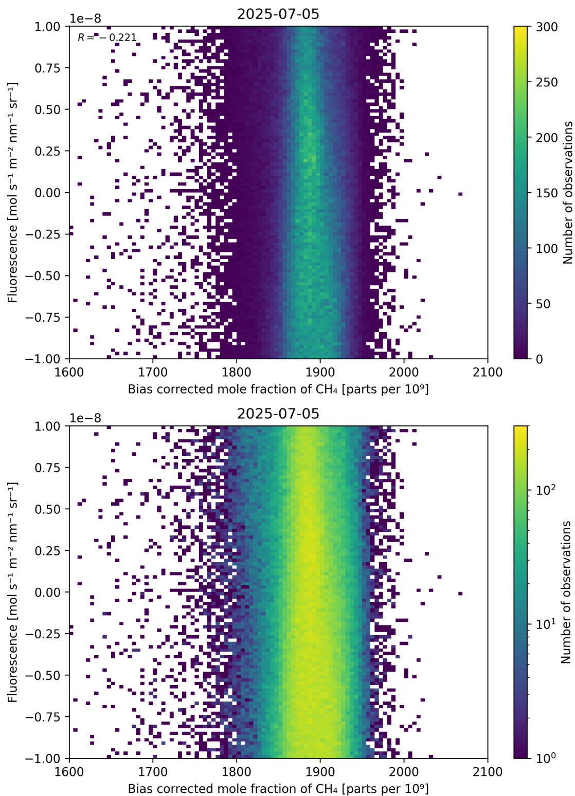
Figure 66: Scatter density plot of “Bias corrected mole fraction of \text{CH}_4 ” against “Fluorescence” for 2025-07-04 to 2025-07-06.
