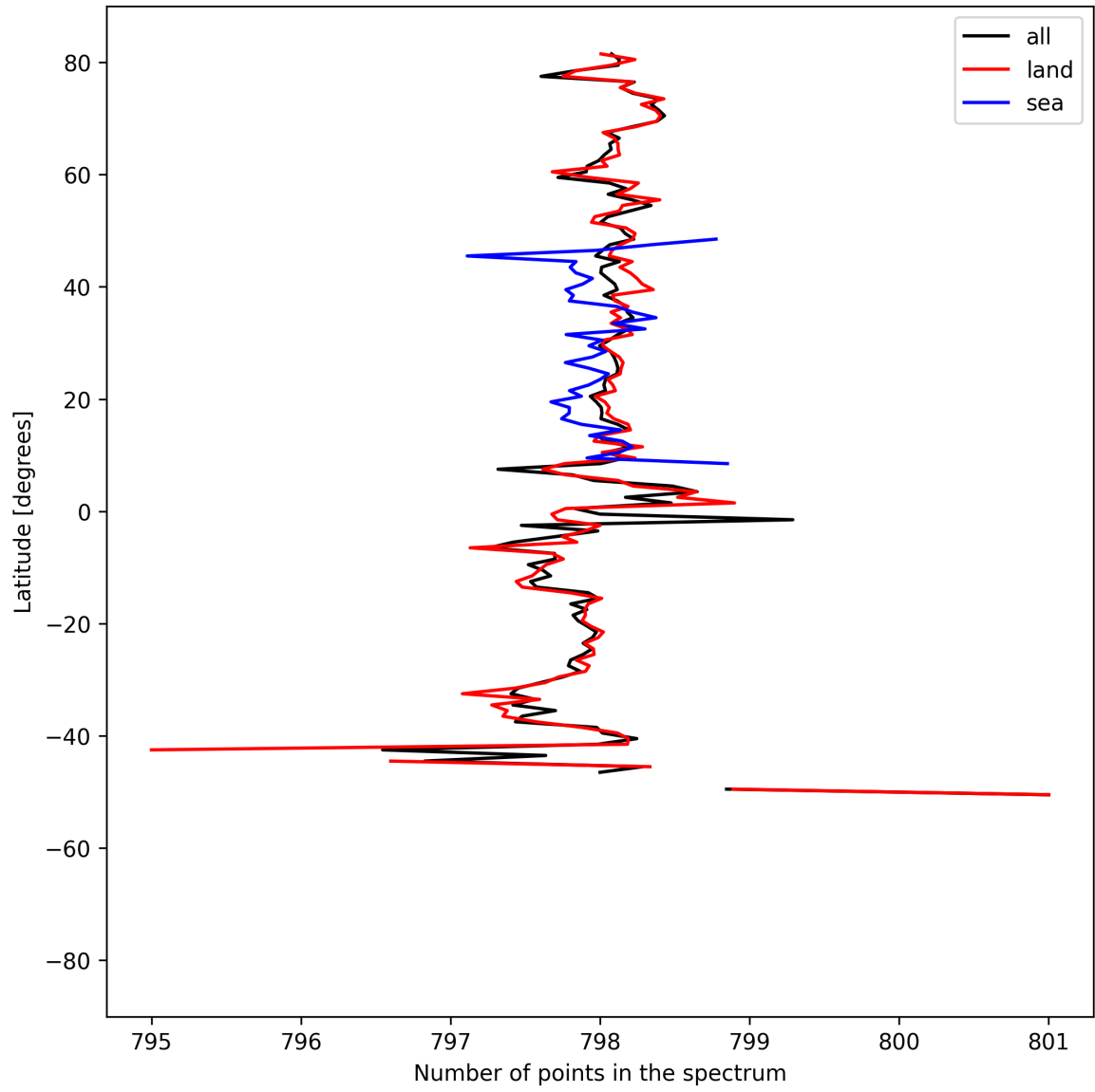
Figure 15: Zonal average of “Number of points in the spectrum” for 2025-07-04 to 2025-07-06.
