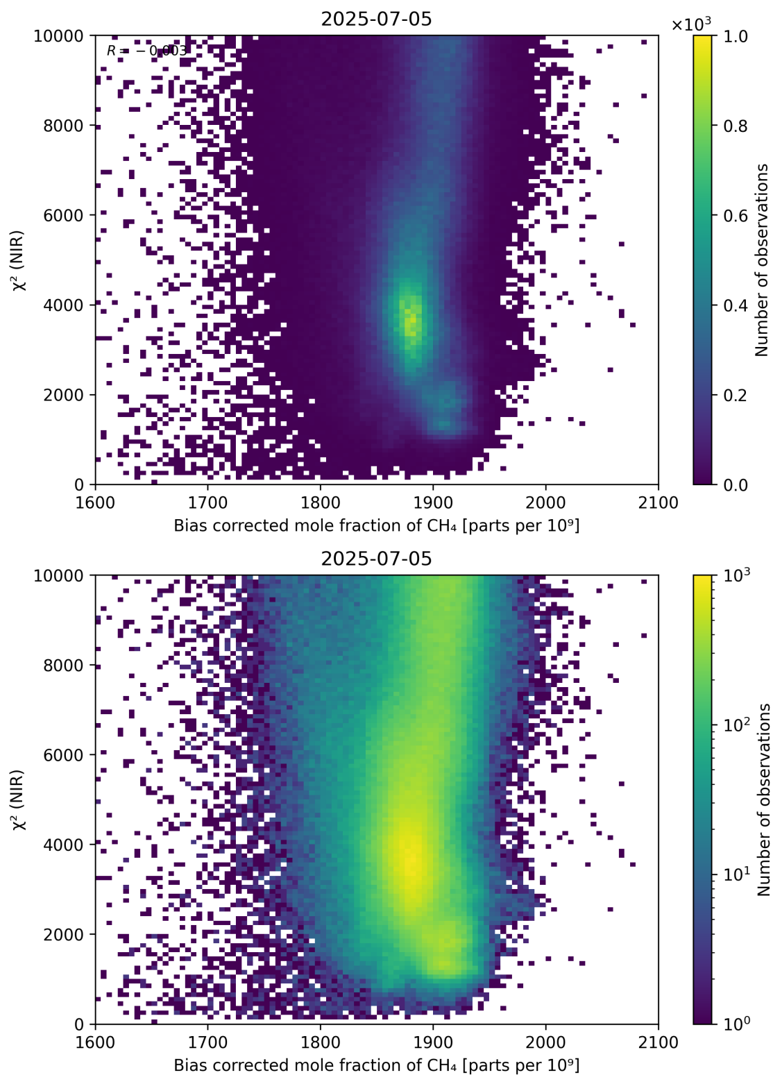
Figure 63: Scatter density plot of “Bias corrected mole fraction of CH 4 ” against “ \chi^2 (NIR)” for 2025-07-04 to 2025-07-06.
