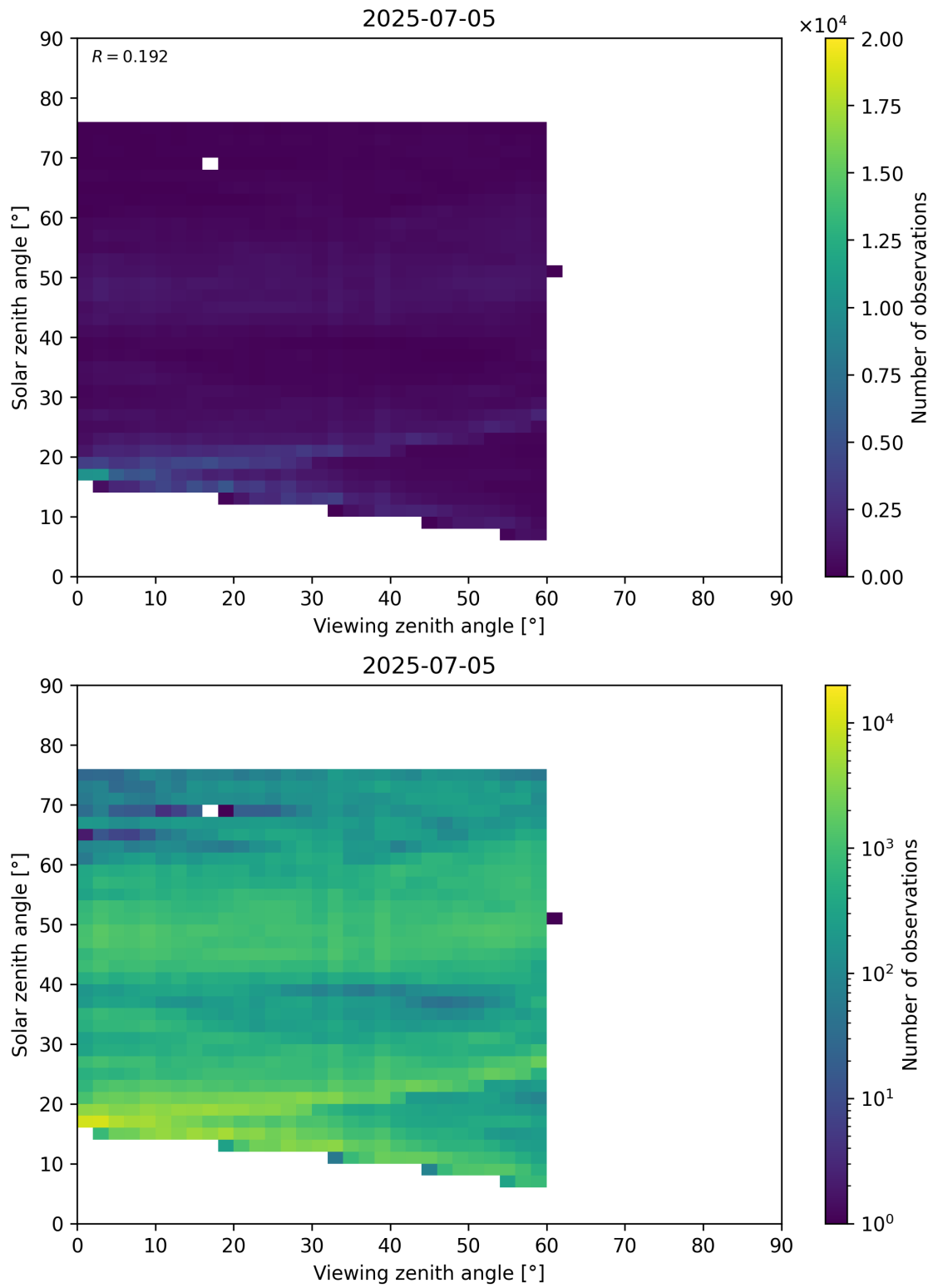
Figure 115: Scatter density plot of “Viewing zenith angle” against “Solar zenith angle” for 2025-07-04 to 2025-07-06.
