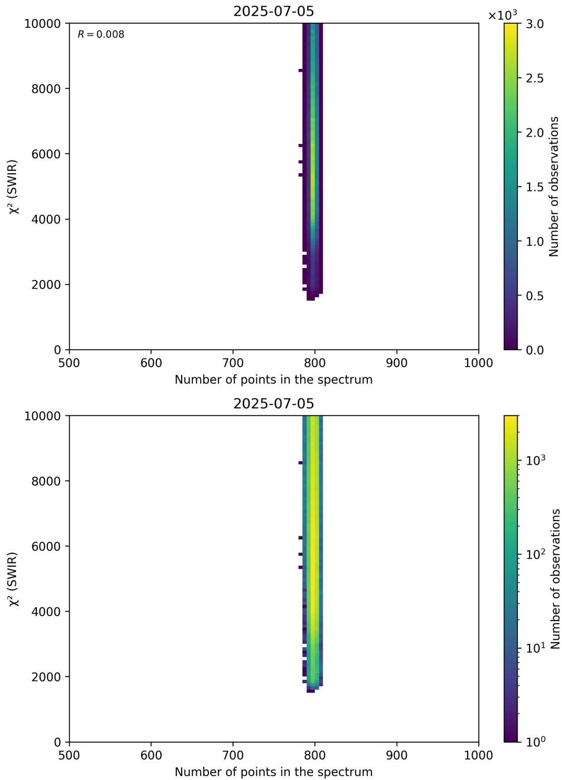
Figure 89: Scatter density plot of “Number of points in the spectrum” against “ \chi^2 (SWIR)” for 2025-07-04 to 2025-07-06.
