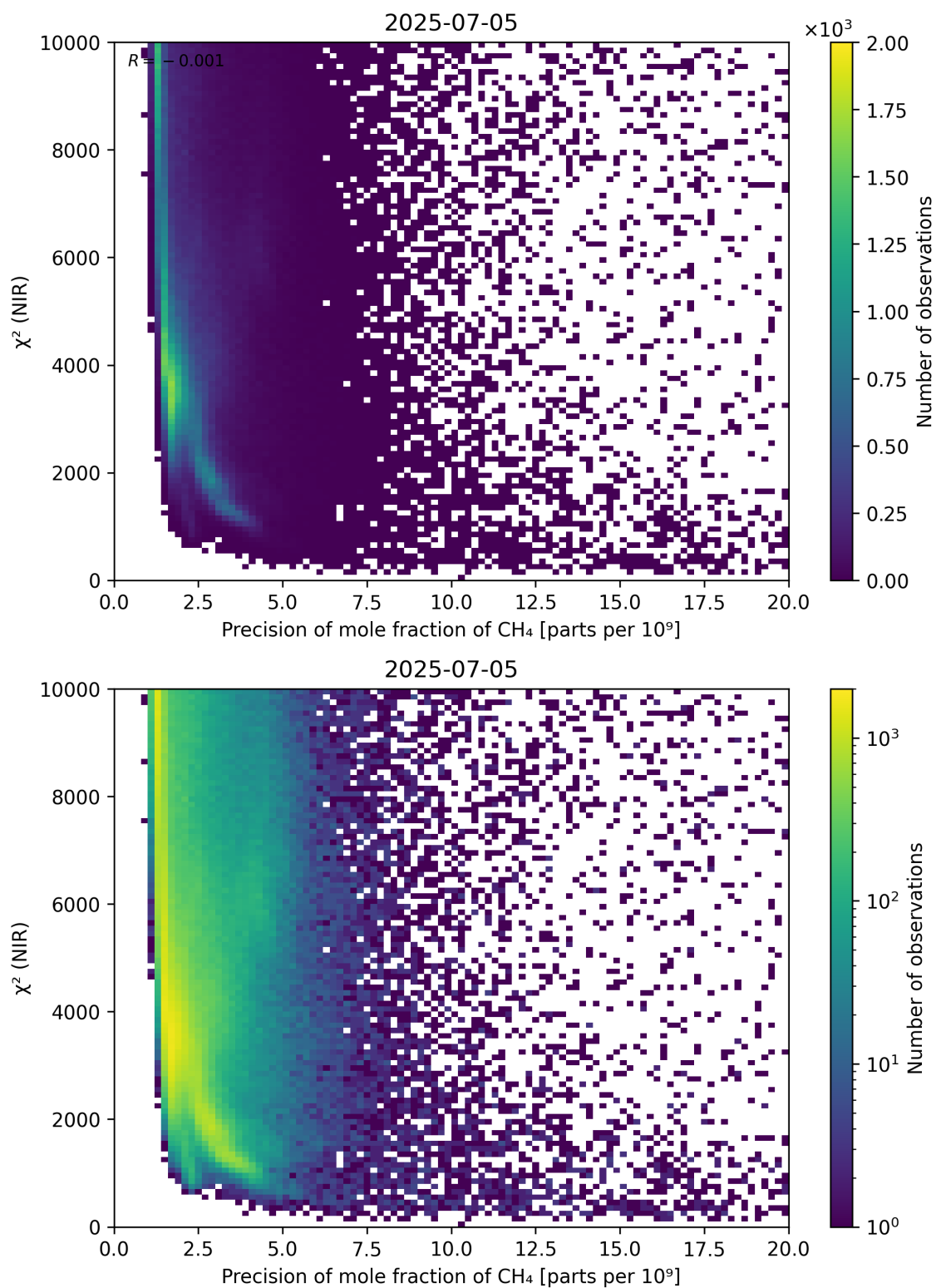
Figure 78: Scatter density plot of “Precision of mole fraction of \text{CH}_4 ” against “ \chi^2 (NIR)” for 2025-07-04 to 2025-07-06.
