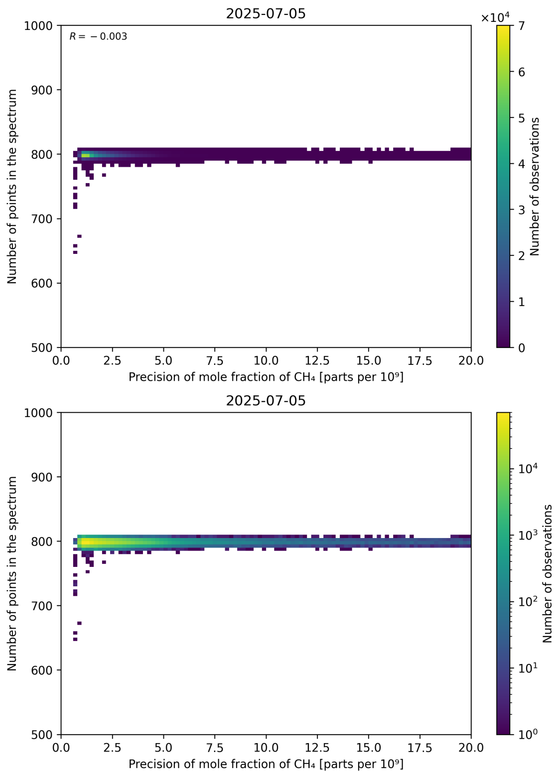
Figure 84: Scatter density plot of “Precision of mole fraction of CH 4 ” against “Number of points in the spectrum” for 2025-07-04 to 2025-07-06.
