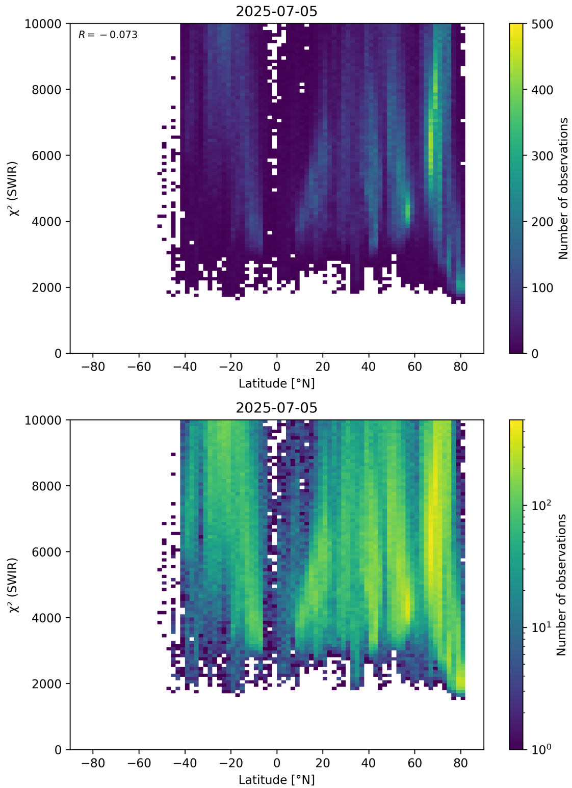
Figure 54: Scatter density plot of “Latitude” against “ \chi^2 (SWIR)” for 2025-07-04 to 2025-07-06.
