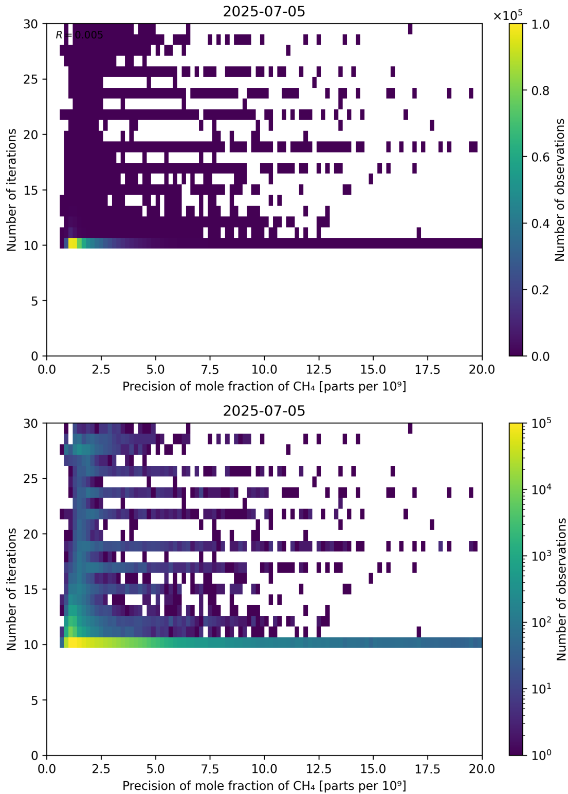
Figure 83: Scatter density plot of “Precision of mole fraction of CH 4 ” against “Number of iterations” for 2025-07-04 to 2025-07-06.
