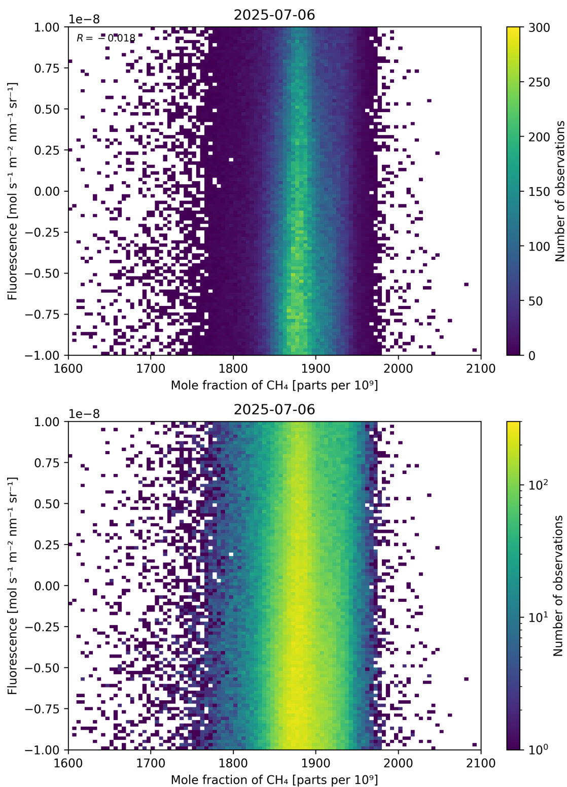
Figure 73: Scatter density plot of “Mole fraction of \text{CH}_4 ” against “Fluorescence” for 2025-07-05 to 2025-07-07.
