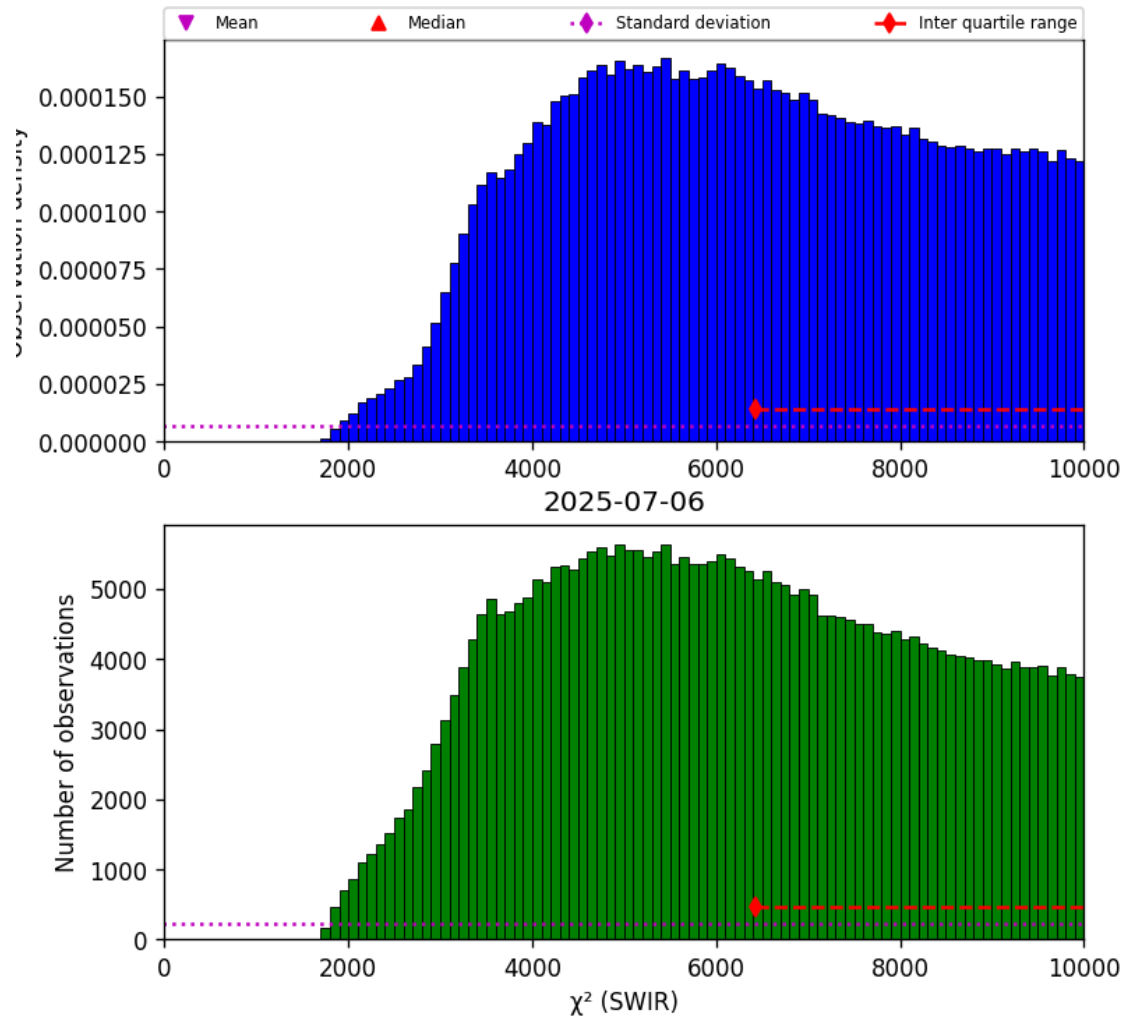
Figure 28: Histogram of “ \chi^2 (SWIR)” for 2025-07-05 to 2025-07-07
