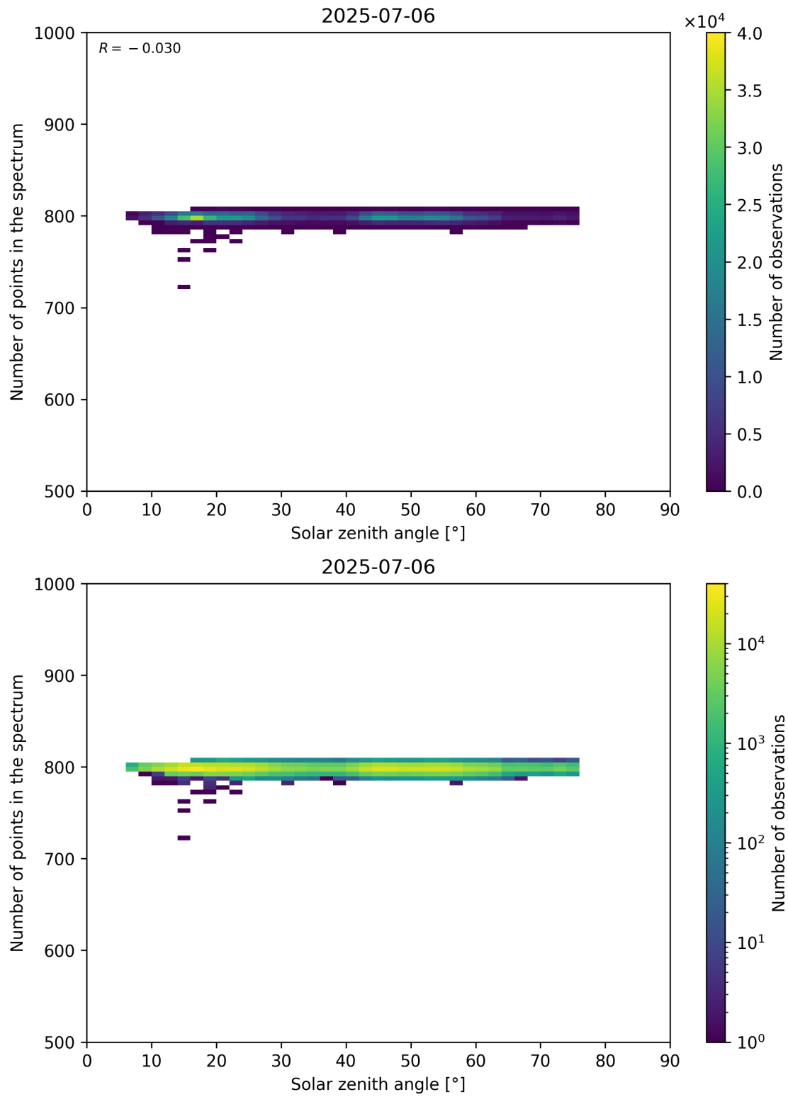
Figure 103: Scatter density plot of “Solar zenith angle” against “Number of points in the spectrum” for 2025-07-05 to 2025-07-07.
