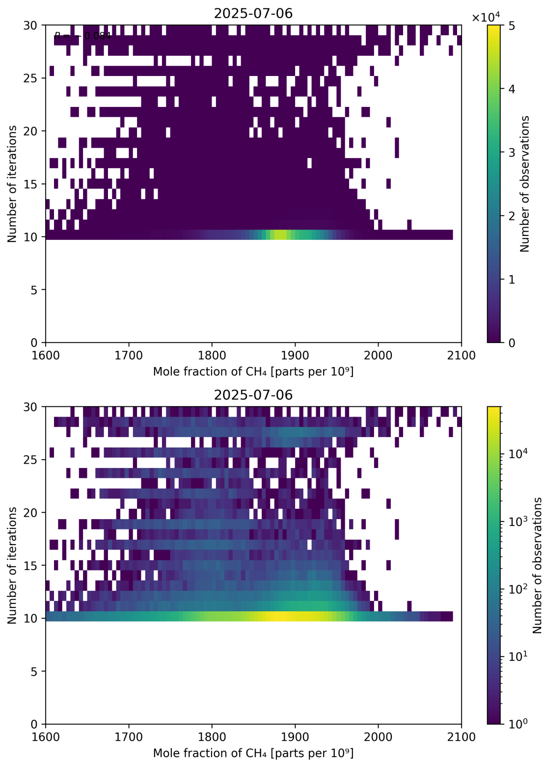
Figure 76: Scatter density plot of “Mole fraction of CH 4 ” against “Number of iterations” for 2025-07-05 to 2025-07-07.
