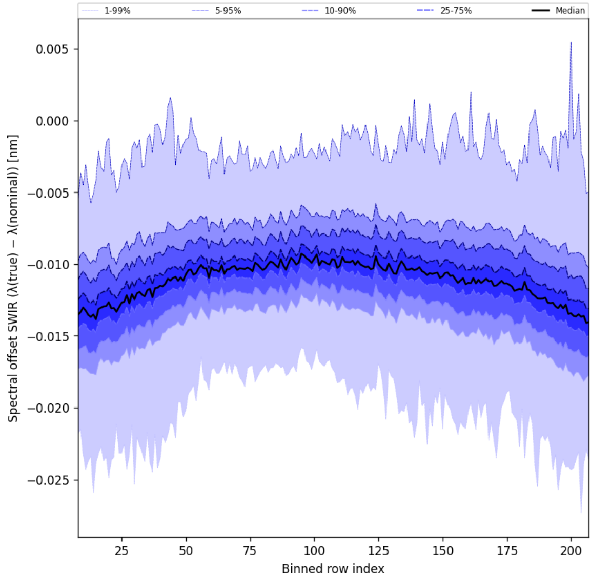
Figure 38: Along track statistics of “Spectral offset SWIR ( \lambda_{\text{true}} - \lambda_{\text{nominal}} )” for 2025-07-05 to 2025-07-07
