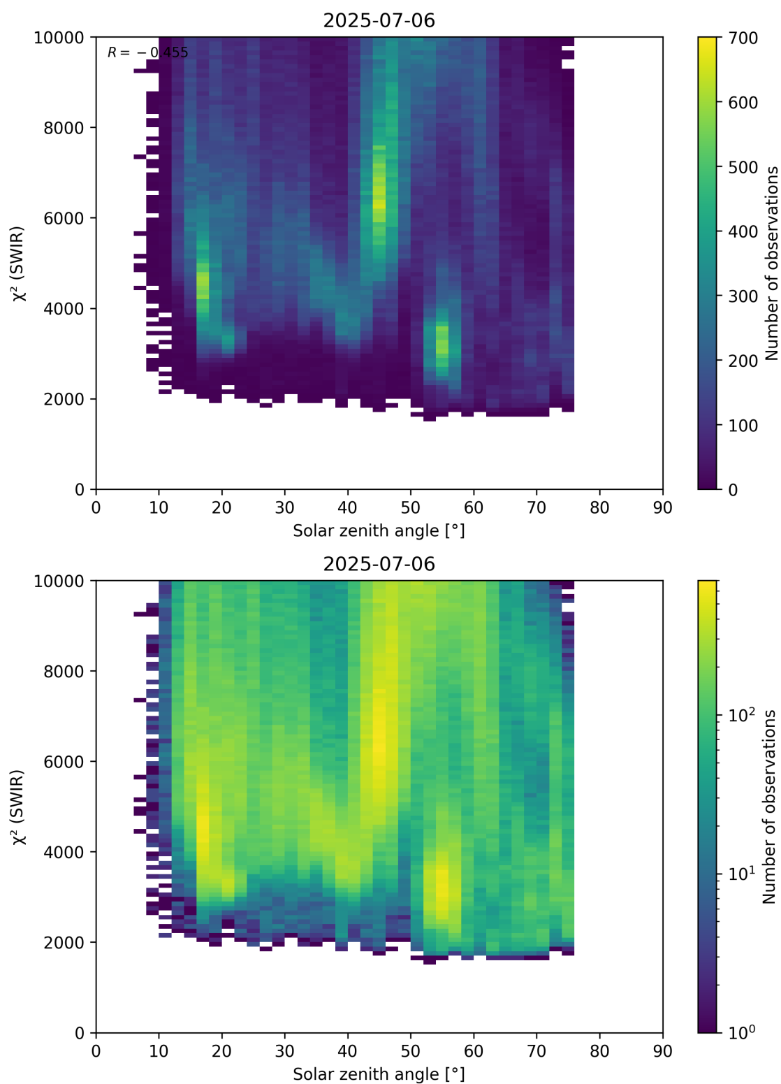
Figure 95: Scatter density plot of “Solar zenith angle” against “ \chi^2 (SWIR)” for 2025-07-05 to 2025-07-07.
