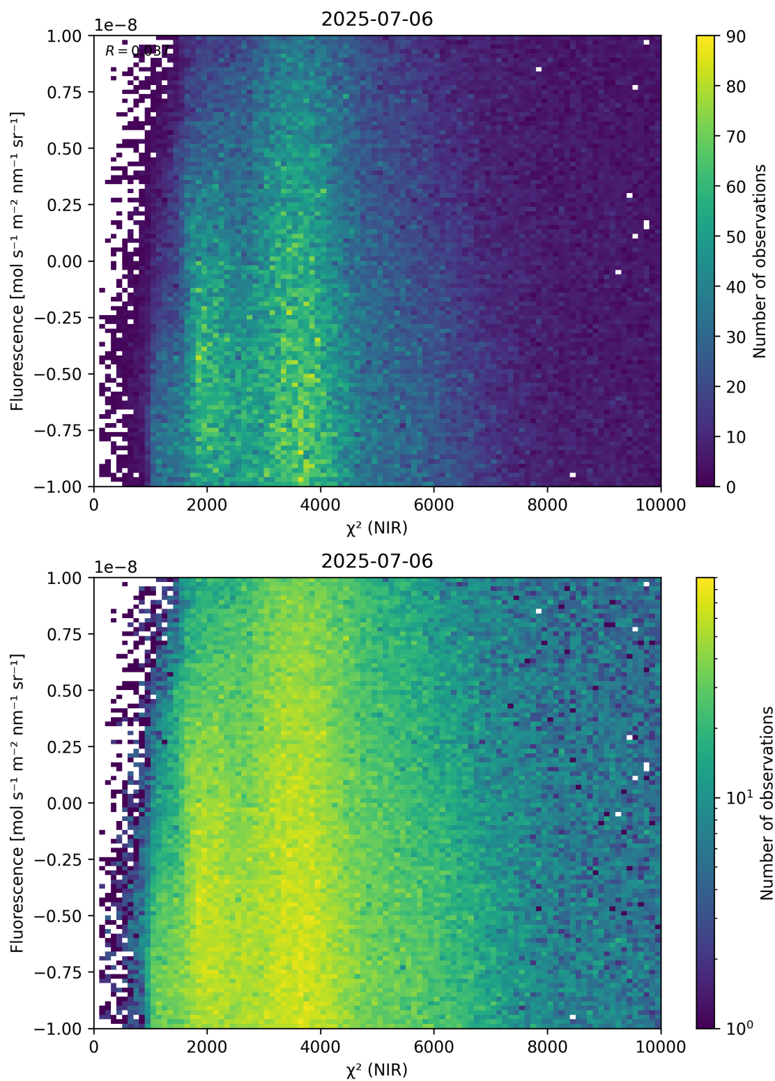
Figure 45: Scatter density plot of “ \chi^2 (NIR)” against “Fluorescence” for 2025-07-05 to 2025-07-07.
