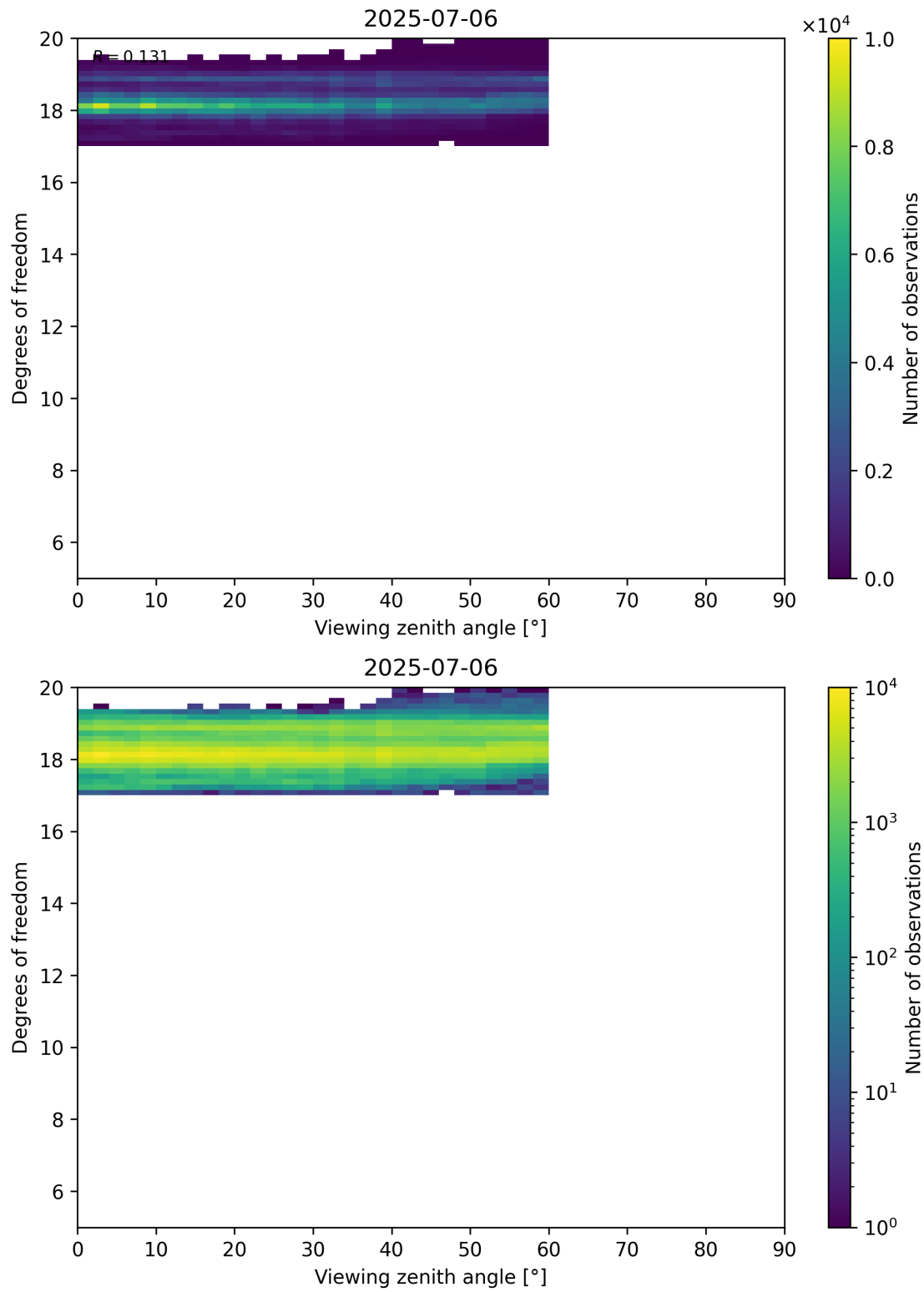
Figure 107: Scatter density plot of “Viewing zenith angle” against “Degrees of freedom” for 2025-07-05 to 2025-07-07.
