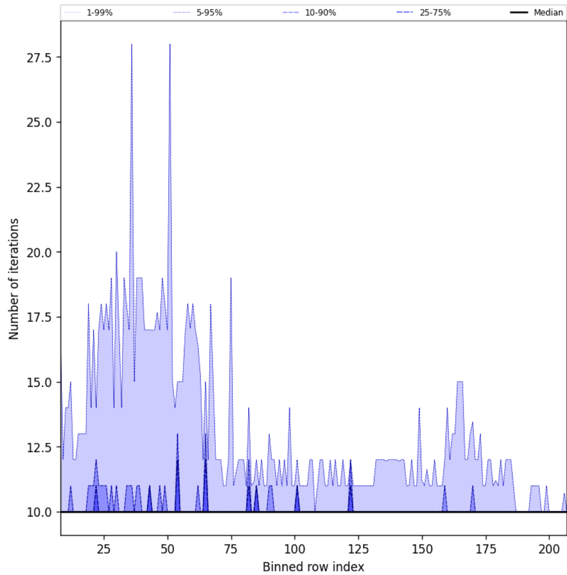
Figure 42: Along track statistics of “Number of iterations” for 2025-07-05 to 2025-07-07
