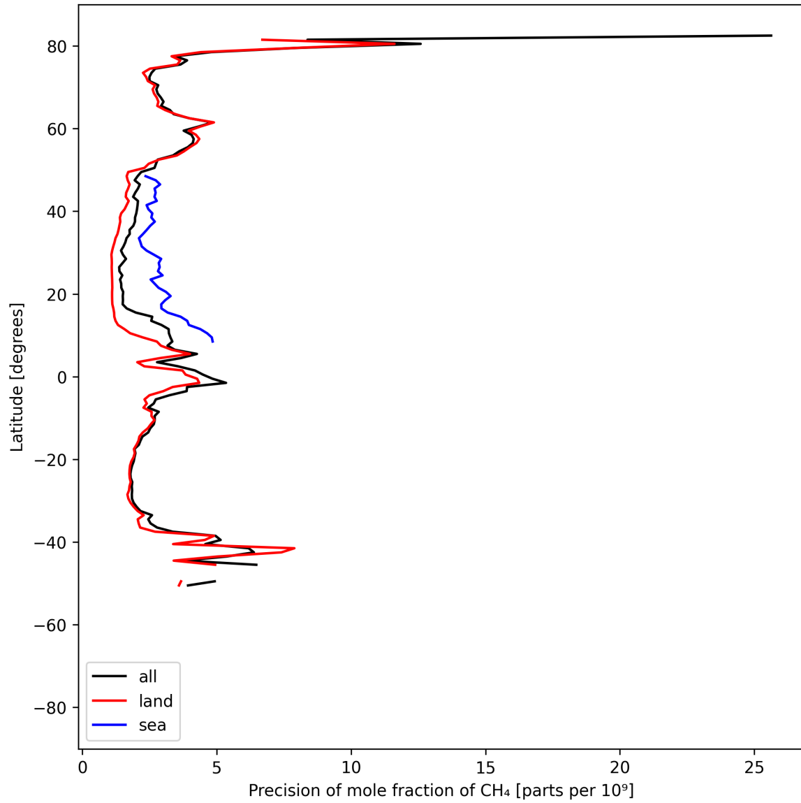
Figure 13: Zonal average of “Precision of mole fraction of CH 4 ” for 2025-07-05 to 2025-07-07.
