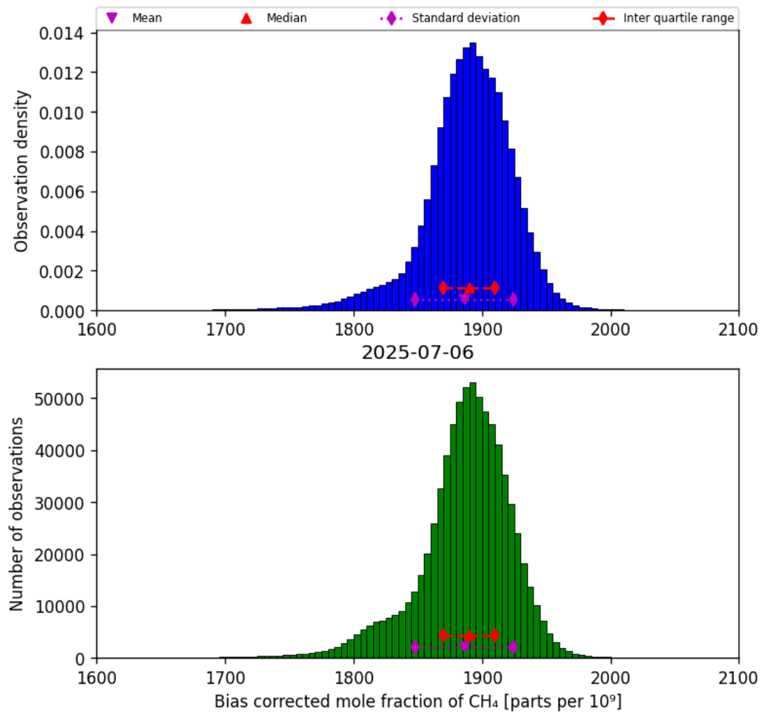
Figure 25: Histogram of “Bias corrected mole fraction of CH 4 ” for 2025-07-05 to 2025-07-07
