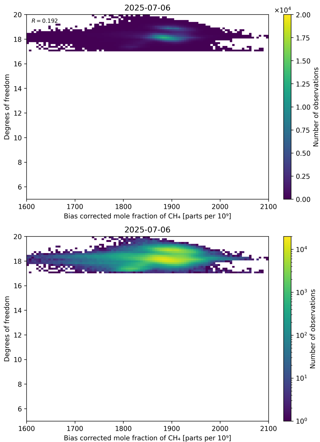
Figure 65: Scatter density plot of “Bias corrected mole fraction of CH 4 ” against “Degrees of freedom” for 2025-07-05 to 2025-07-07.
