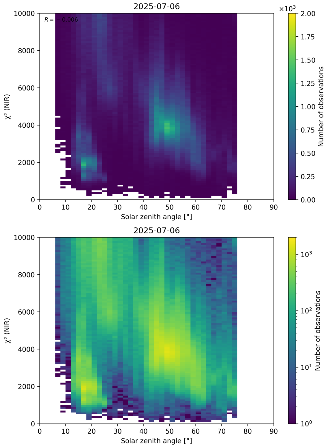
Figure 94: Scatter density plot of “Solar zenith angle” against “ \chi^2 (NIR)” for 2025-07-05 to 2025-07-07.
