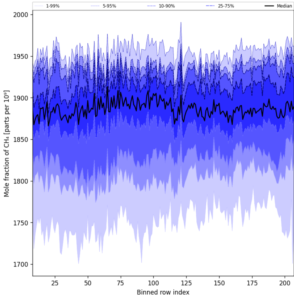
Figure 34: Along track statistics of “Mole fraction of CH 4 ” for 2025-07-05 to 2025-07-07
