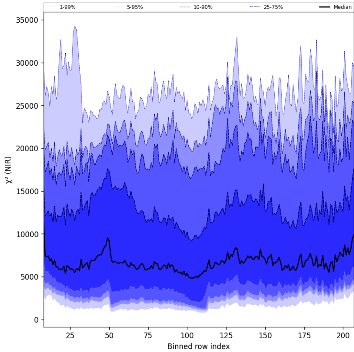
Figure 40: Along track statistics of “ \chi^2 (NIR)” for 2025-07-05 to 2025-07-07
