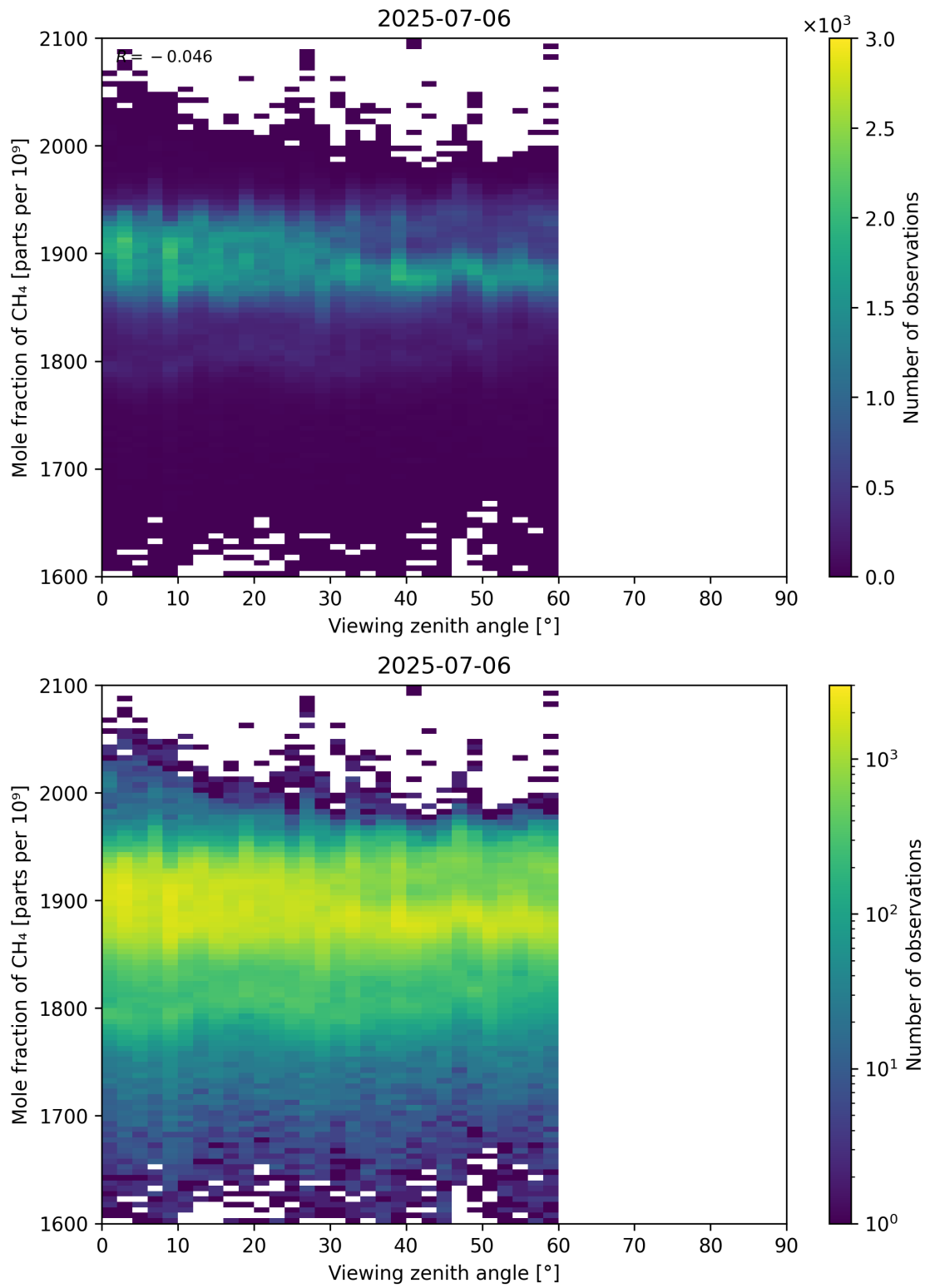
Figure 110: Scatter density plot of “Viewing zenith angle” against “Mole fraction of CH 4 ” for 2025-07-05 to 2025-07-07.
