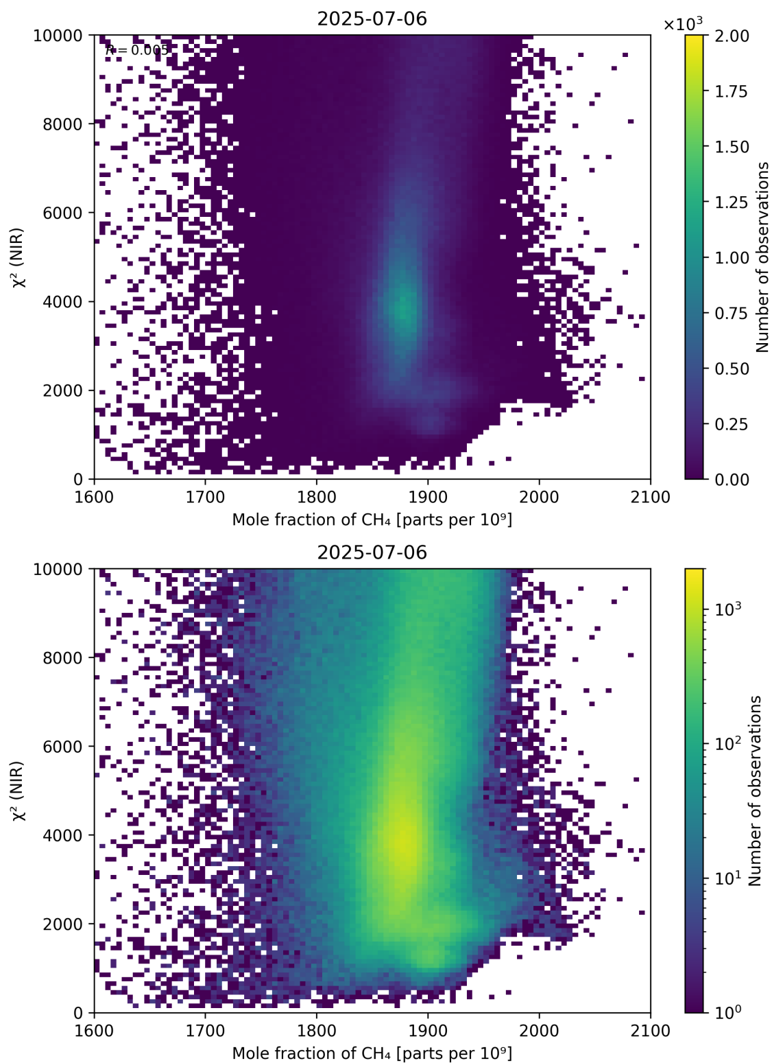
Figure 70: Scatter density plot of “Mole fraction of CH 4 ” against “ \chi^2 (NIR)” for 2025-07-05 to 2025-07-07.
