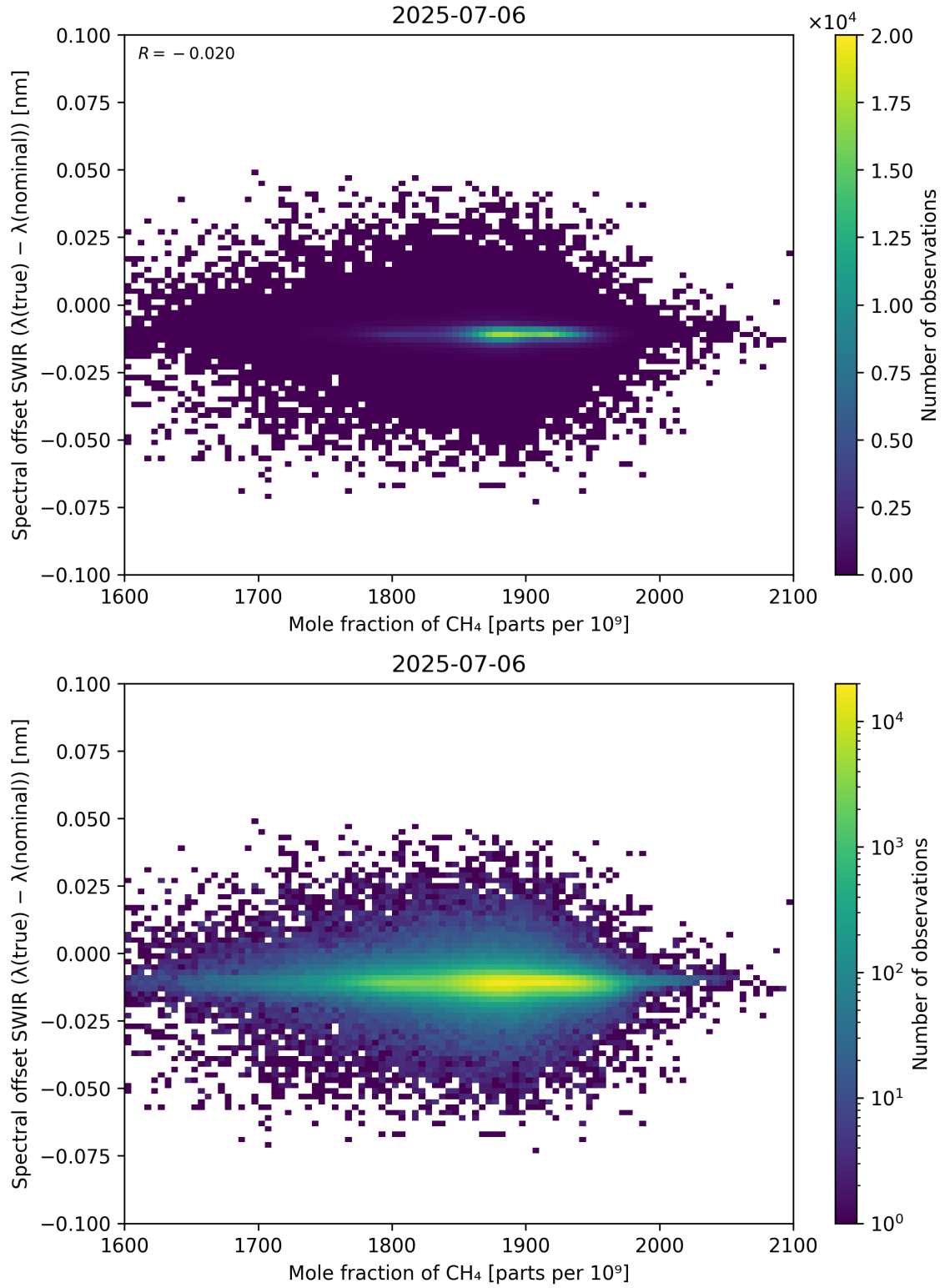
Figure 86: Scatter density plot of “Mole fraction of CH 4 ” against “Spectral offset SWIR ( \lambda_{\text{true}} - \lambda_{\text{nominal}} )” for 2025-07-05 to 2025-07-07.
