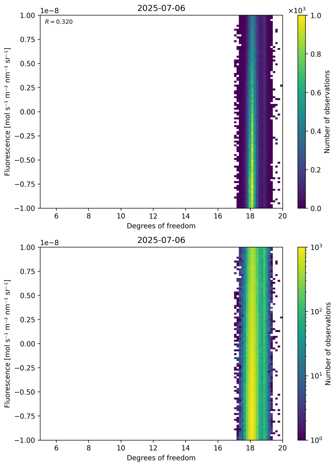
Figure 51: Scatter density plot of “Degrees of freedom” against “Fluorescence” for 2025-07-05 to 2025-07-07.
