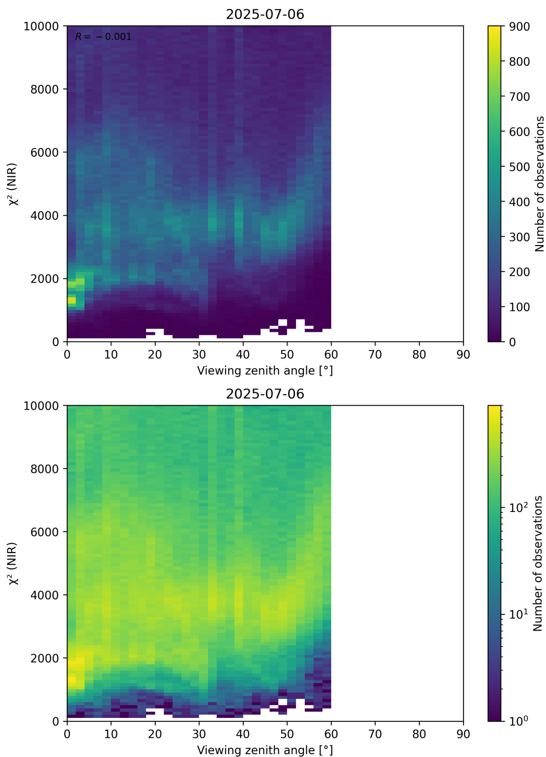
Figure 105: Scatter density plot of “Viewing zenith angle” against “ \chi^2 (NIR)” for 2025-07-05 to 2025-07-07.
