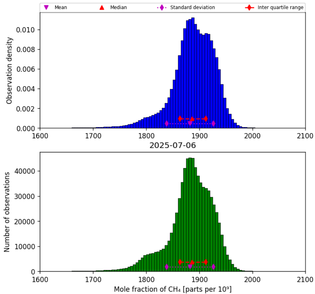
Figure 23: Histogram of “Mole fraction of CH 4 ” for 2025-07-05 to 2025-07-07
