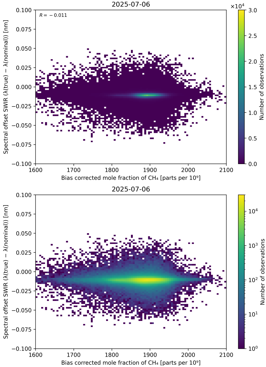
Figure 69: Scatter density plot of “Bias corrected mole fraction of \text{CH}_4 ” against “Spectral offset SWIR ( \lambda_{\text{true}} - \lambda_{\text{nominal}} )” for 2025-07-05 to 2025-07-07.
