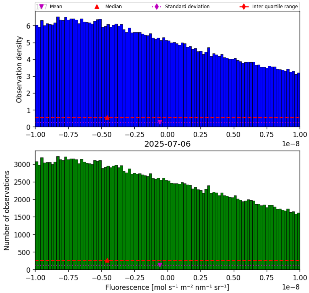
Figure 32: Histogram of “Fluorescence” for 2025-07-05 to 2025-07-07
