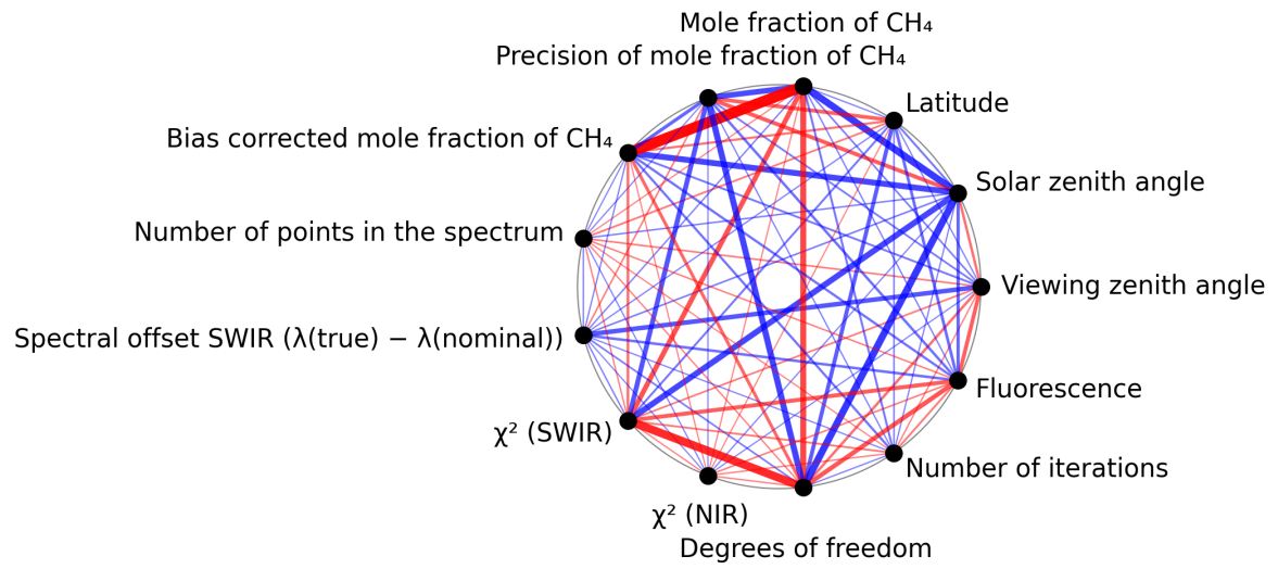
Figure 1: Map of correlation graph for 2025-07-05 to 2025-07-07.
