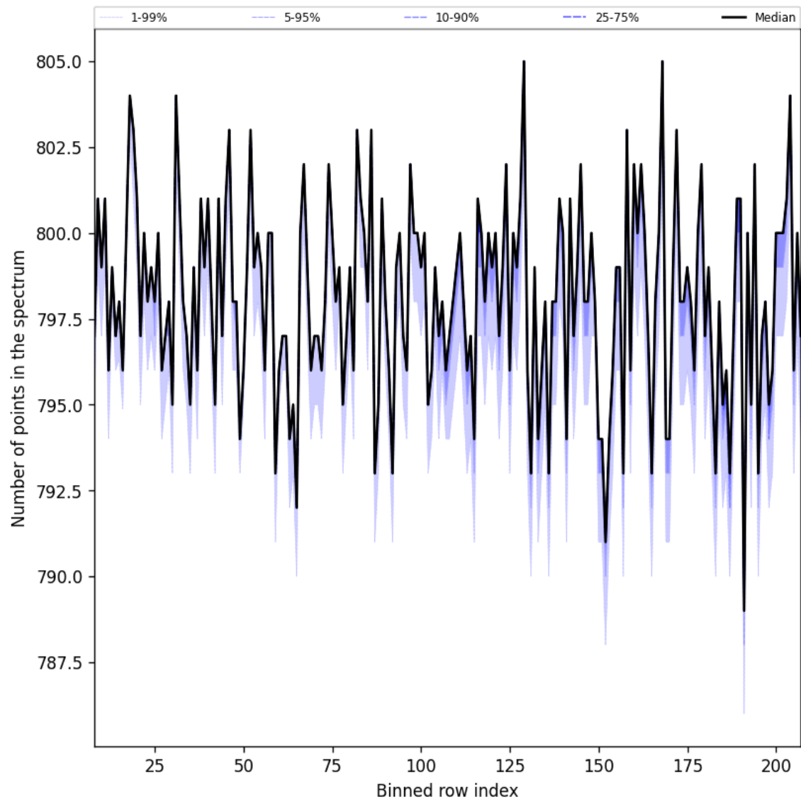
Figure 37: Along track statistics of “Number of points in the spectrum” for 2025-07-05 to 2025-07-07
