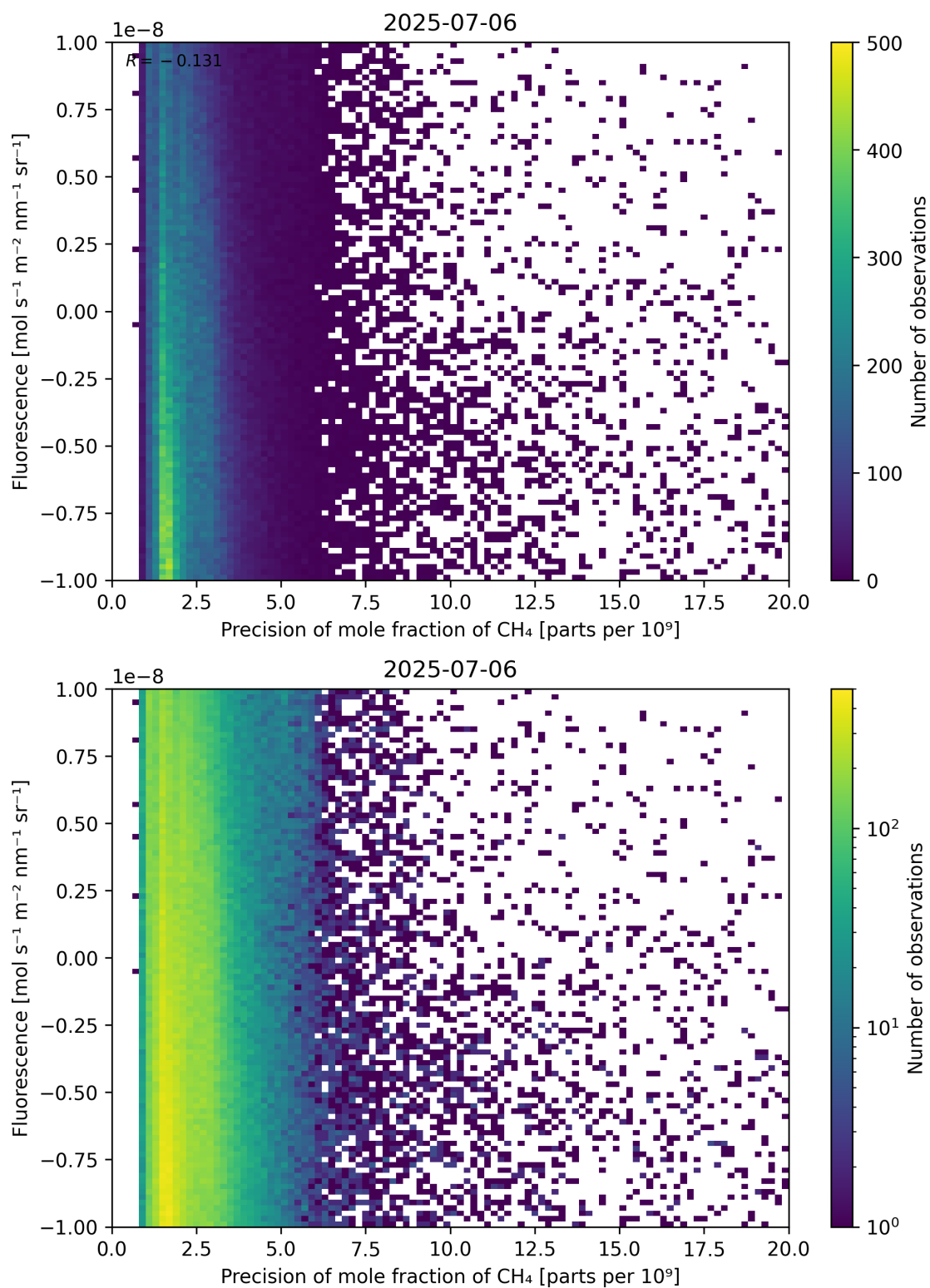
Figure 81: Scatter density plot of “Precision of mole fraction of \text{CH}_4 ” against “Fluorescence” for 2025-07-05 to 2025-07-07.
