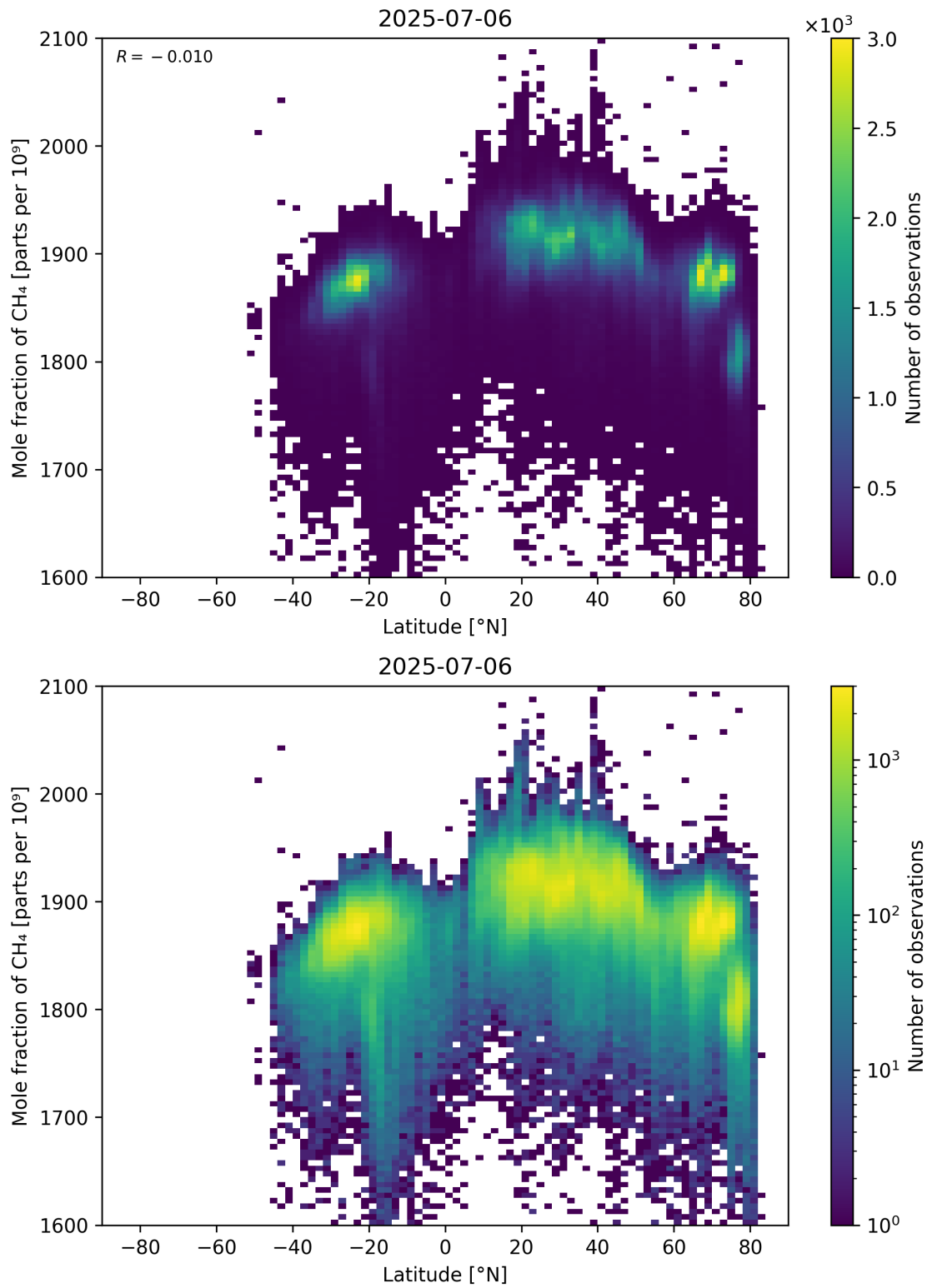
Figure 57: Scatter density plot of “Latitude” against “Mole fraction of CH 4 ” for 2025-07-05 to 2025-07-07.
