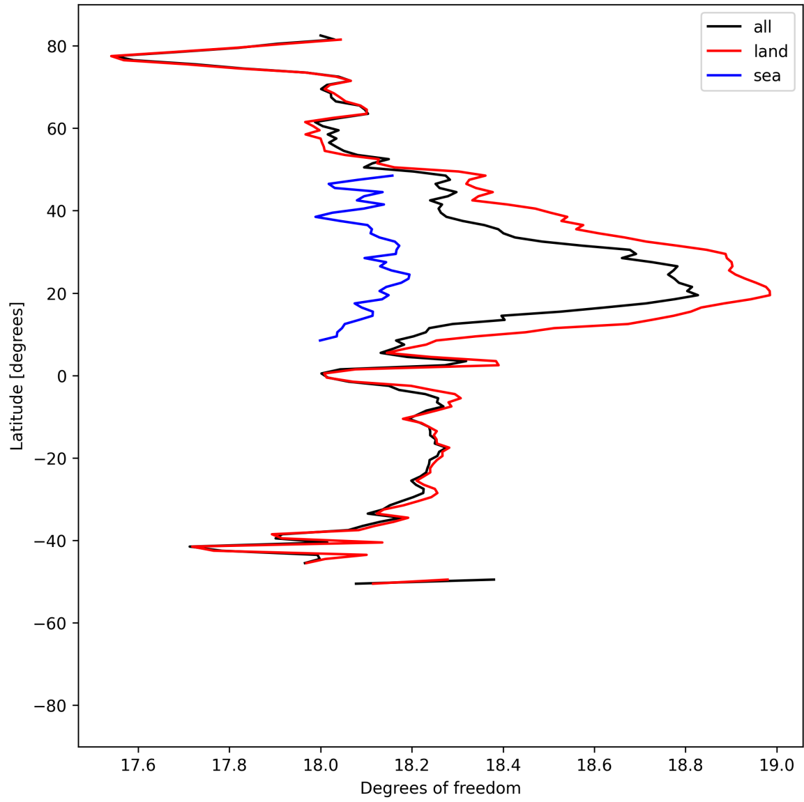
Figure 19: Zonal average of “Degrees of freedom” for 2025-07-05 to 2025-07-07.
