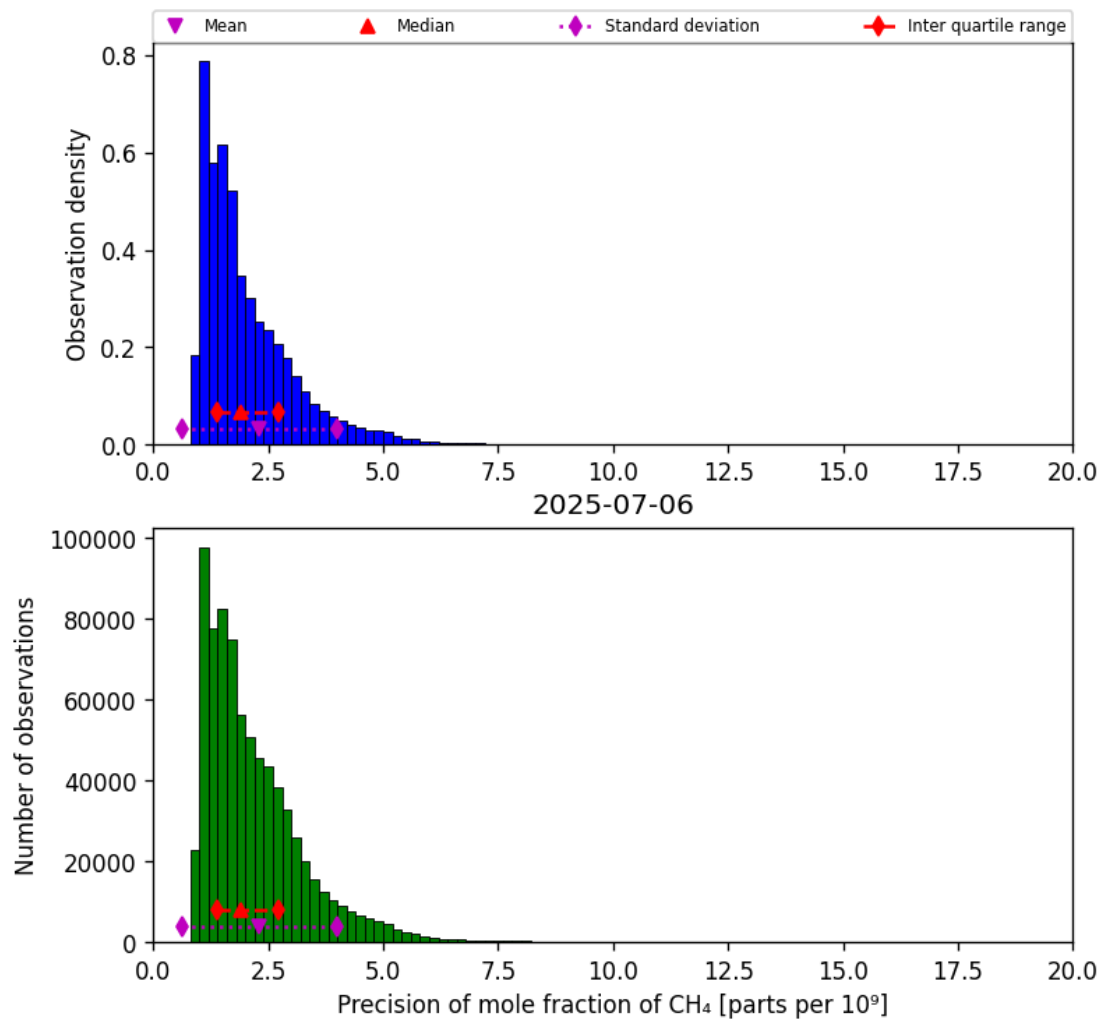
Figure 24: Histogram of “Precision of mole fraction of CH 4 ” for 2025-07-05 to 2025-07-07
