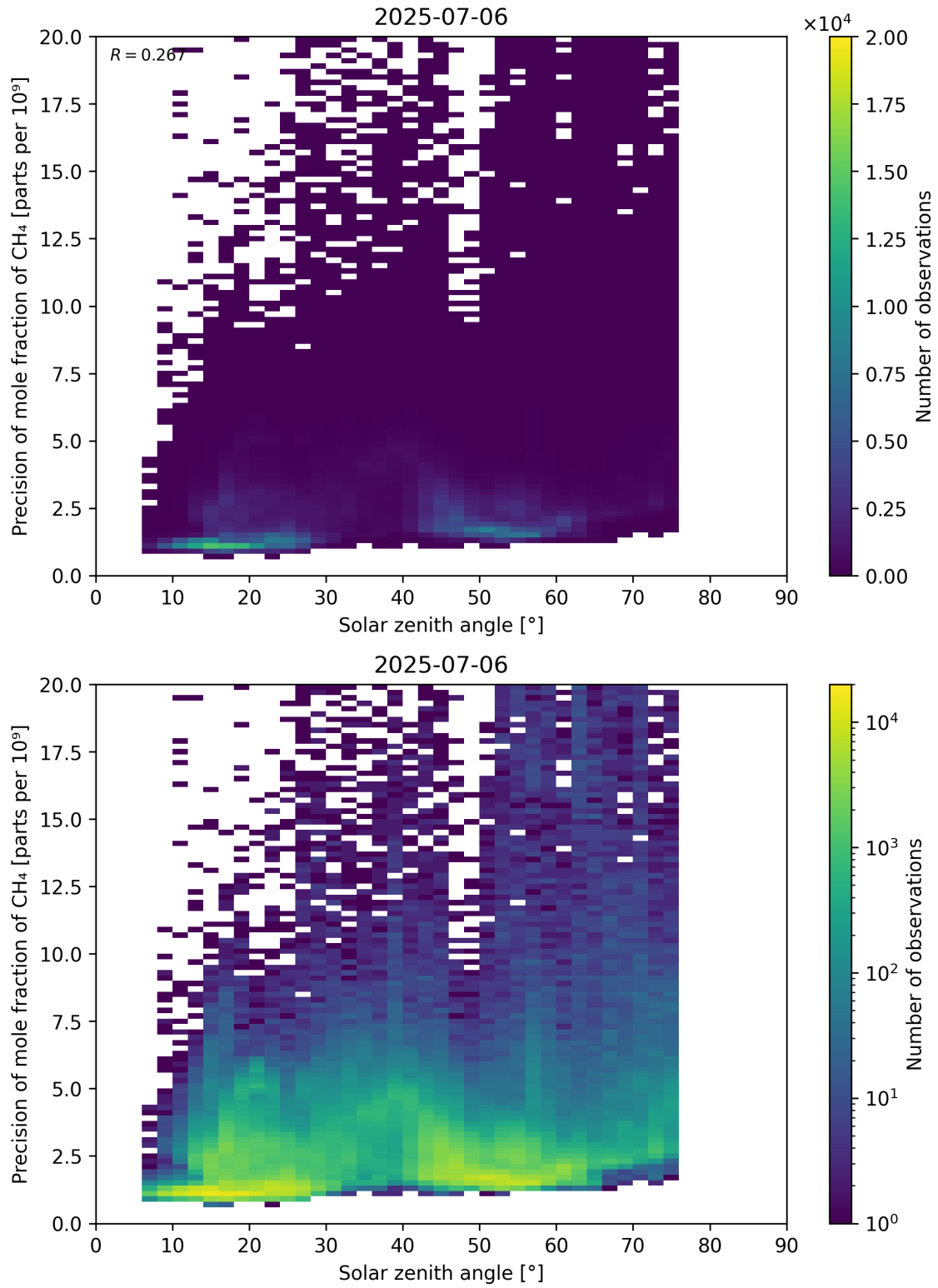
Figure 101: Scatter density plot of “Solar zenith angle” against “Precision of mole fraction of CH 4 ” for 2025-07-05 to 2025-07-07.
