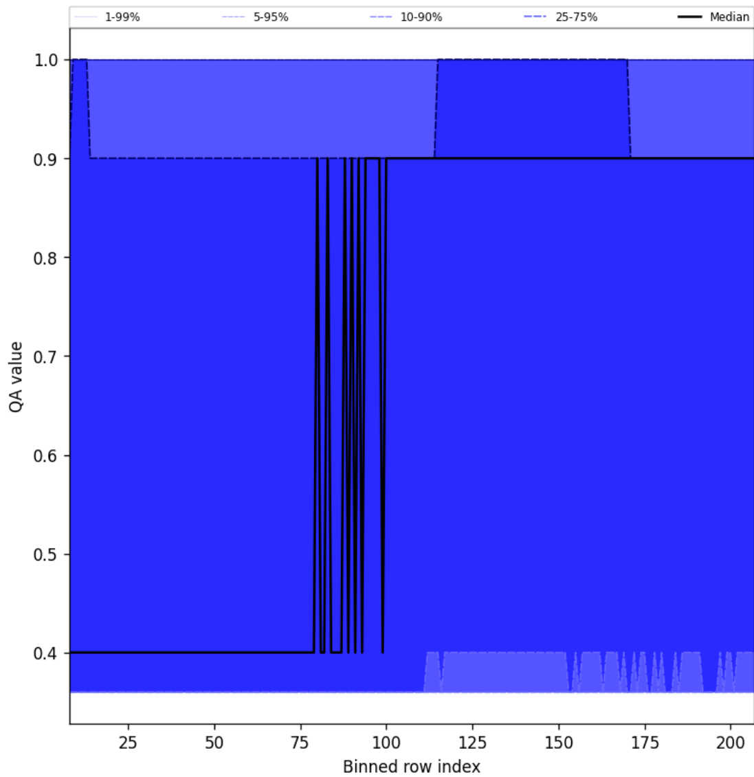
Figure 33: Along track statistics of “QA value” for 2025-07-05 to 2025-07-07
