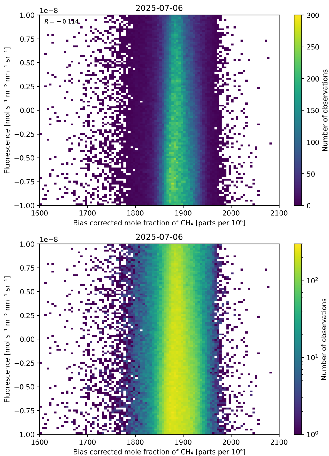
Figure 66: Scatter density plot of “Bias corrected mole fraction of \text{CH}_4 ” against “Fluorescence” for 2025-07-05 to 2025-07-07.
