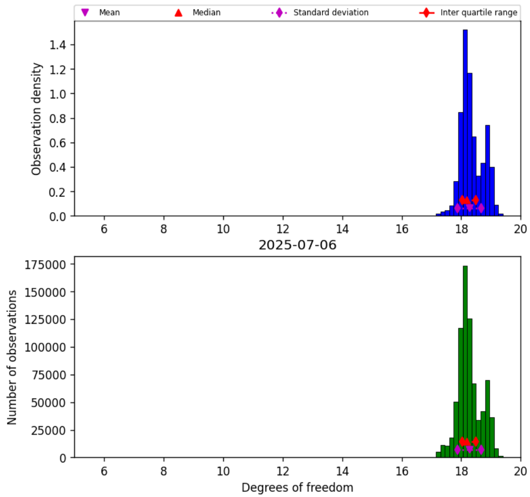
Figure 30: Histogram of “Degrees of freedom” for 2025-07-05 to 2025-07-07
