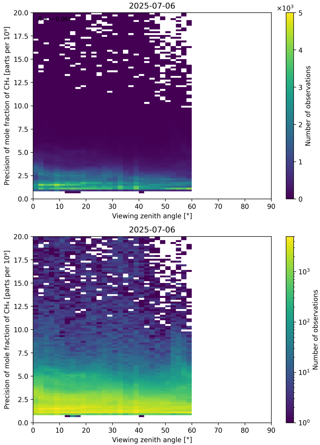
Figure 112: Scatter density plot of “Viewing zenith angle” against “Precision of mole fraction of CH 4 ” for 2025-07-05 to 2025-07-07.
