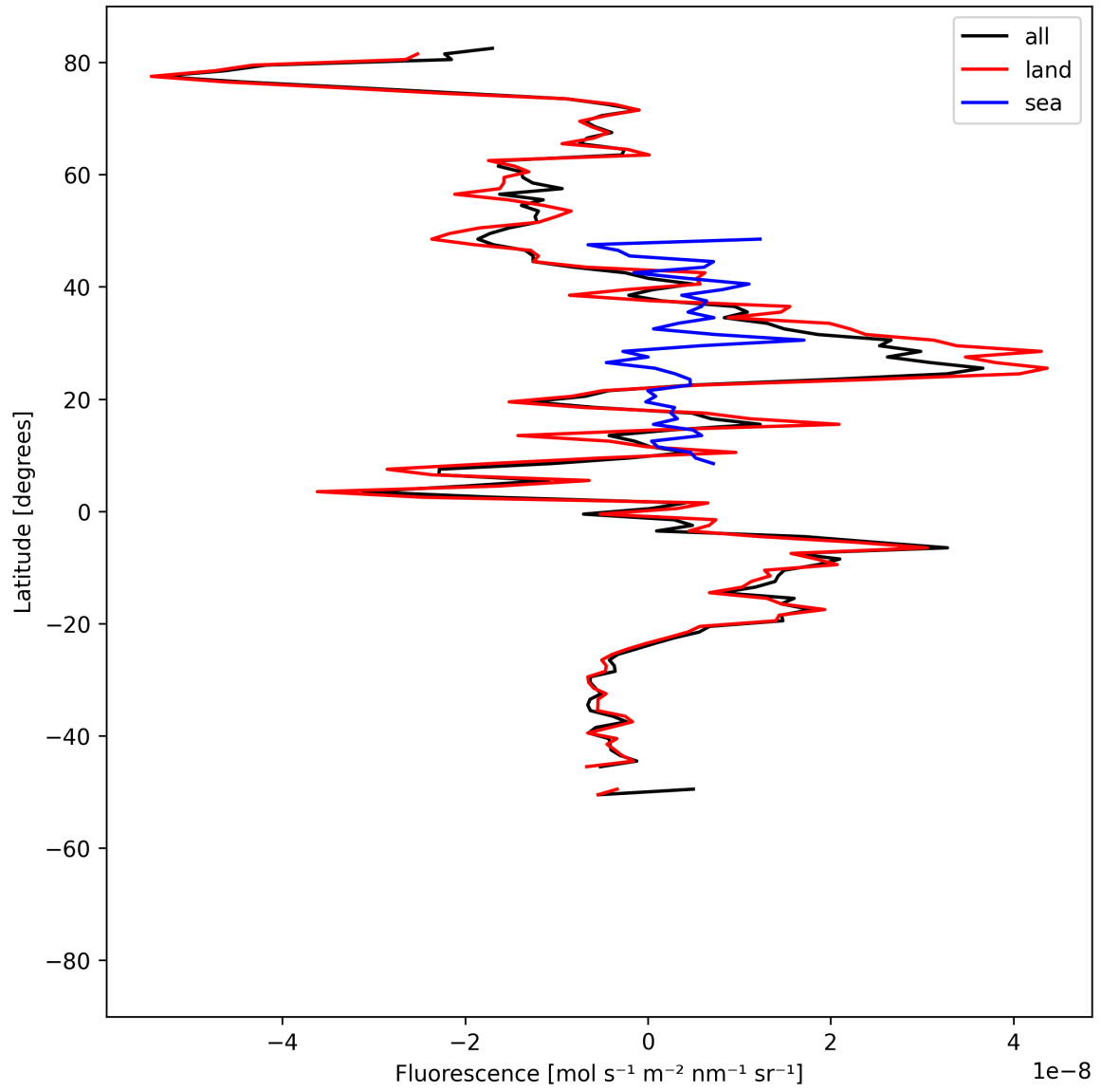
Figure 21: Zonal average of “Fluorescence” for 2025-07-05 to 2025-07-07.
