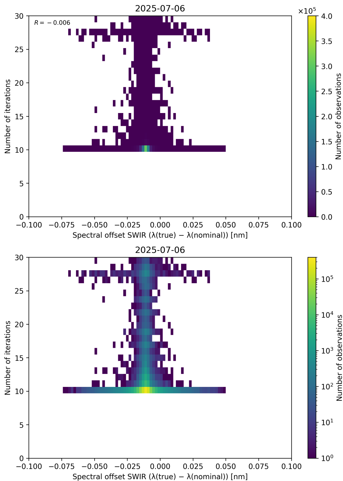
Figure 121: Scatter density plot of “Spectral offset SWIR ( \lambda_{\text{true}} - \lambda_{\text{nominal}} )” against “Number of iterations” for 2025-07-05 to 2025-07-07.
