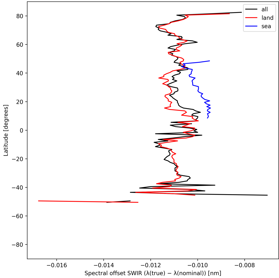
Figure 16: Zonal average of “Spectral offset SWIR ( \lambda_{\text{true}} - \lambda_{\text{nominal}} )” for 2025-07-05 to 2025-07-07.
