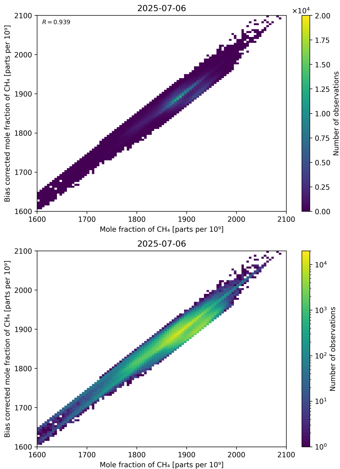
Figure 74: Scatter density plot of “Mole fraction of CH 4 ” against “Bias corrected mole fraction of CH 4 ” for 2025-07-05 to 2025-07-07.
