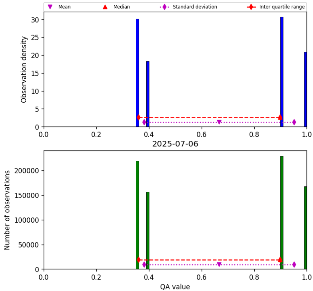
Figure 22: Histogram of “QA value” for 2025-07-05 to 2025-07-07
