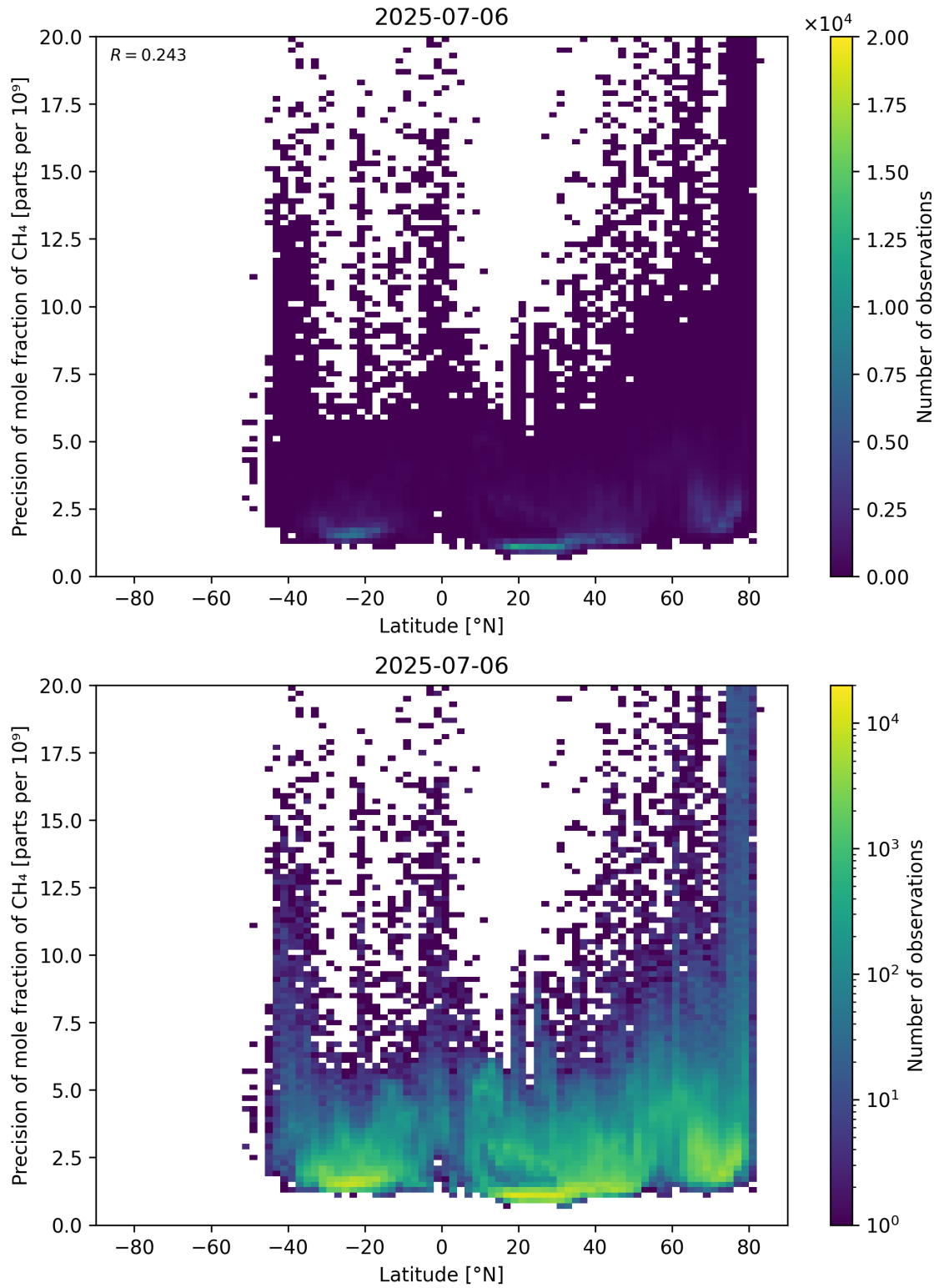
Figure 59: Scatter density plot of “Latitude” against “Precision of mole fraction of \text{CH}_4 ” for 2025-07-05 to 2025-07-07.
