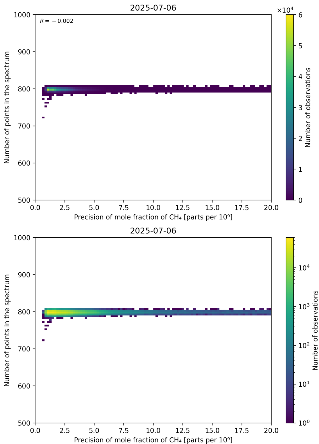
Figure 84: Scatter density plot of “Precision of mole fraction of CH 4 ” against “Number of points in the spectrum” for 2025-07-05 to 2025-07-07.
