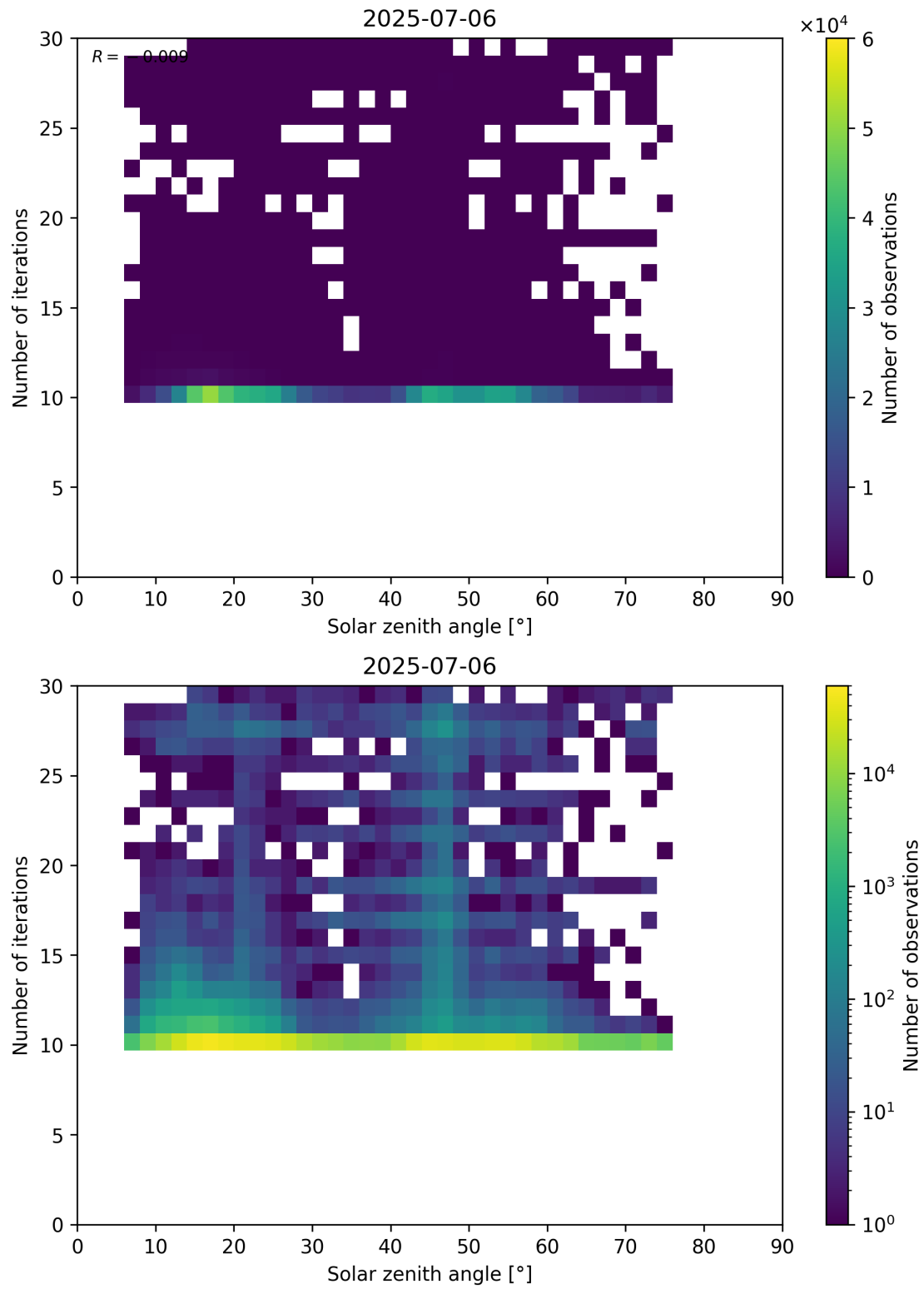
Figure 102: Scatter density plot of “Solar zenith angle” against “Number of iterations” for 2025-07-05 to 2025-07-07.
