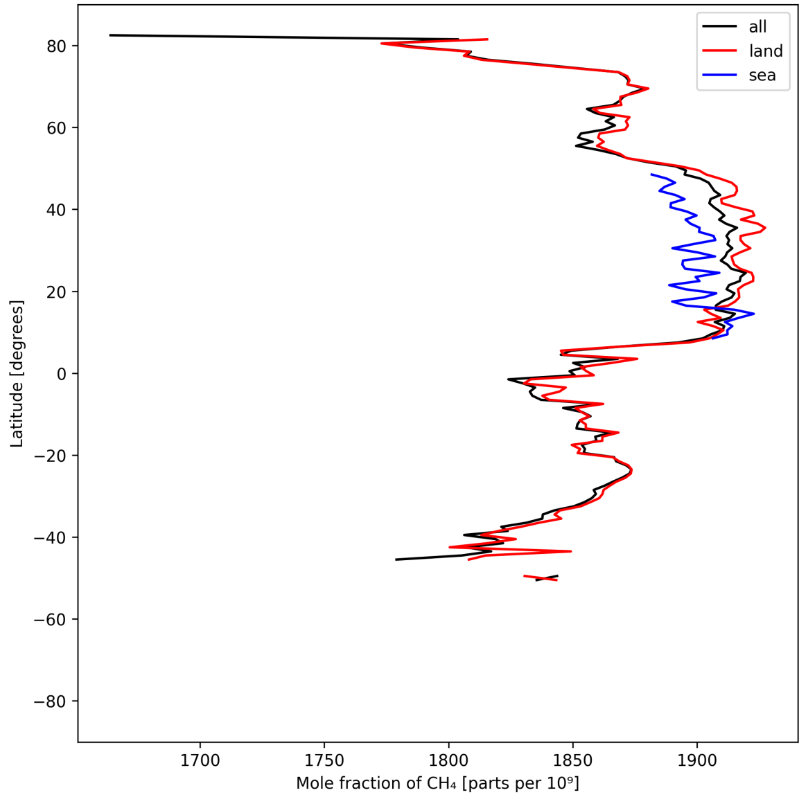
Figure 12: Zonal average of “Mole fraction of \text{CH}_4 ” for 2025-07-05 to 2025-07-07.
