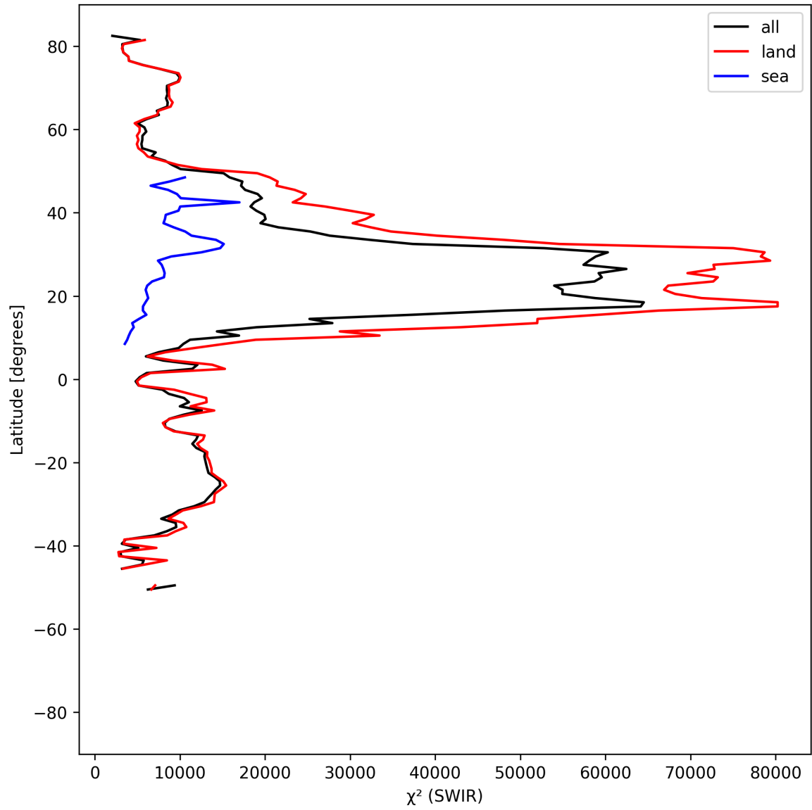
Figure 17: Zonal average of “ \chi^2 (SWIR)” for 2025-07-05 to 2025-07-07.
