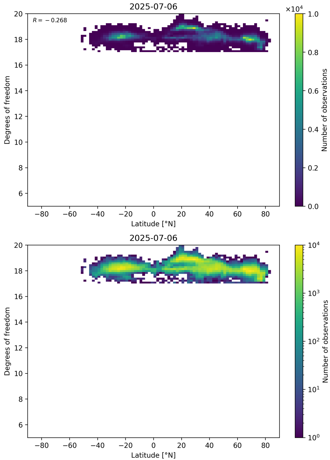
Figure 55: Scatter density plot of “Latitude” against “Degrees of freedom” for 2025-07-05 to 2025-07-07.
