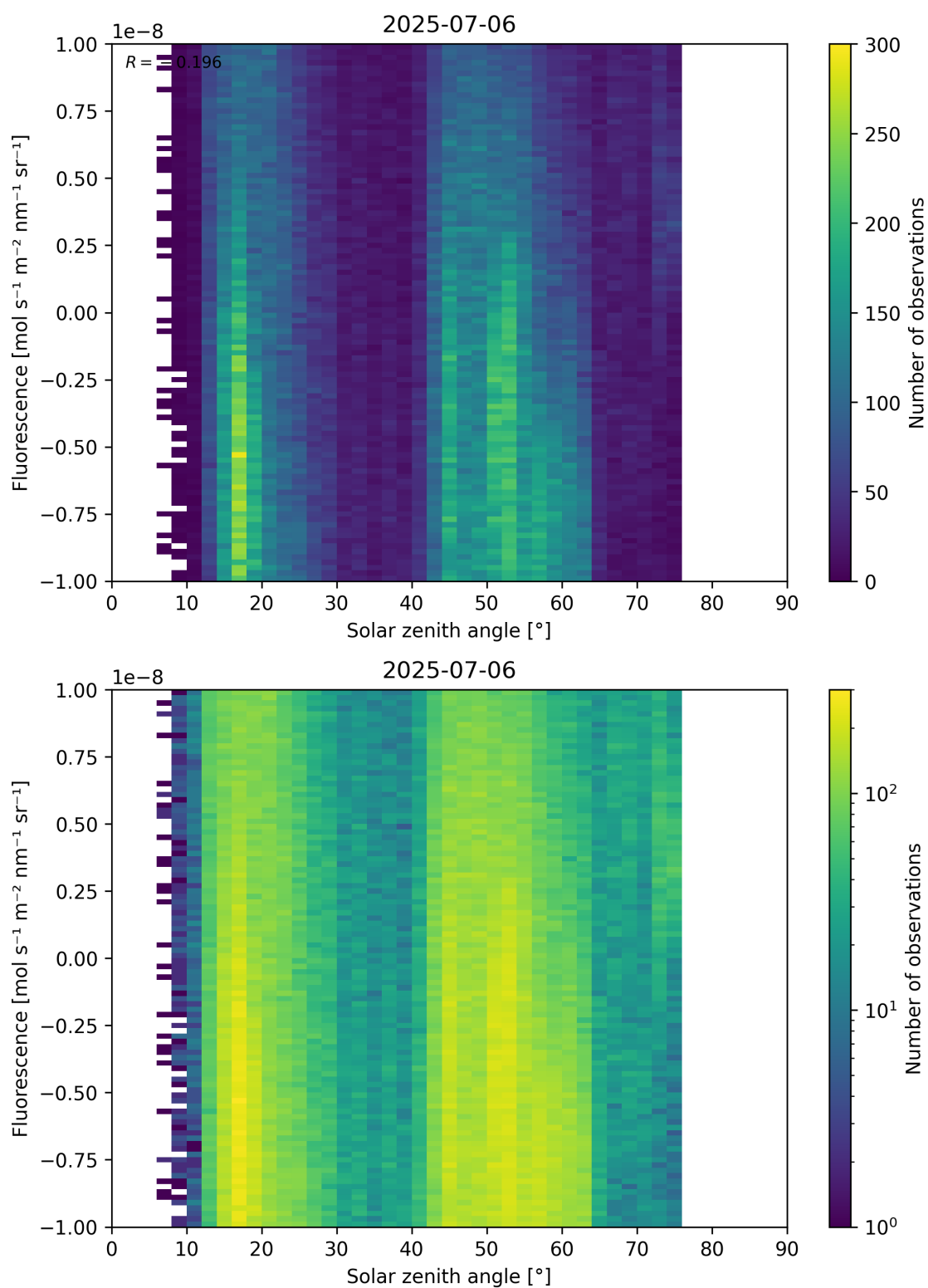
Figure 97: Scatter density plot of “Solar zenith angle” against “Fluorescence” for 2025-07-05 to 2025-07-07.
