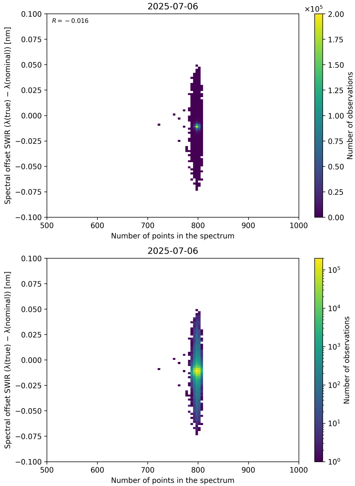
Figure 93: Scatter density plot of “Number of points in the spectrum” against “Spectral offset SWIR ( \lambda_{\text{true}} - \lambda_{\text{nominal}} )” for 2025-07-05 to 2025-07-07.
