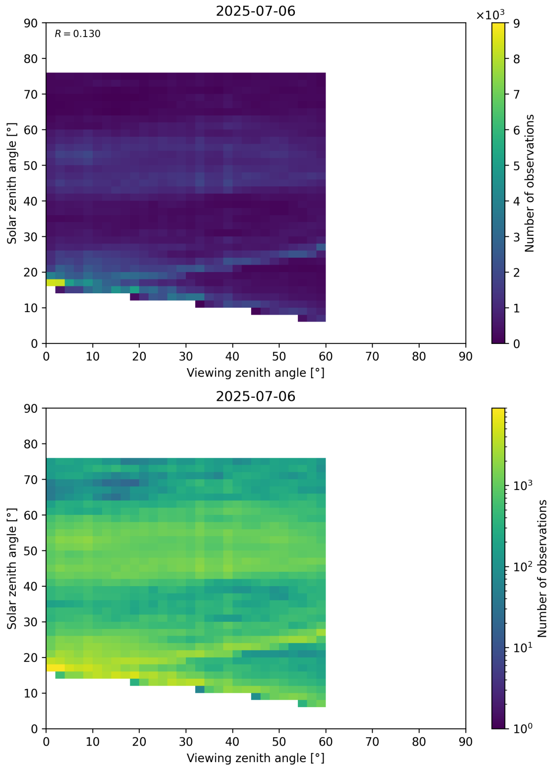
Figure 115: Scatter density plot of “Viewing zenith angle” against “Solar zenith angle” for 2025-07-05 to 2025-07-07.
