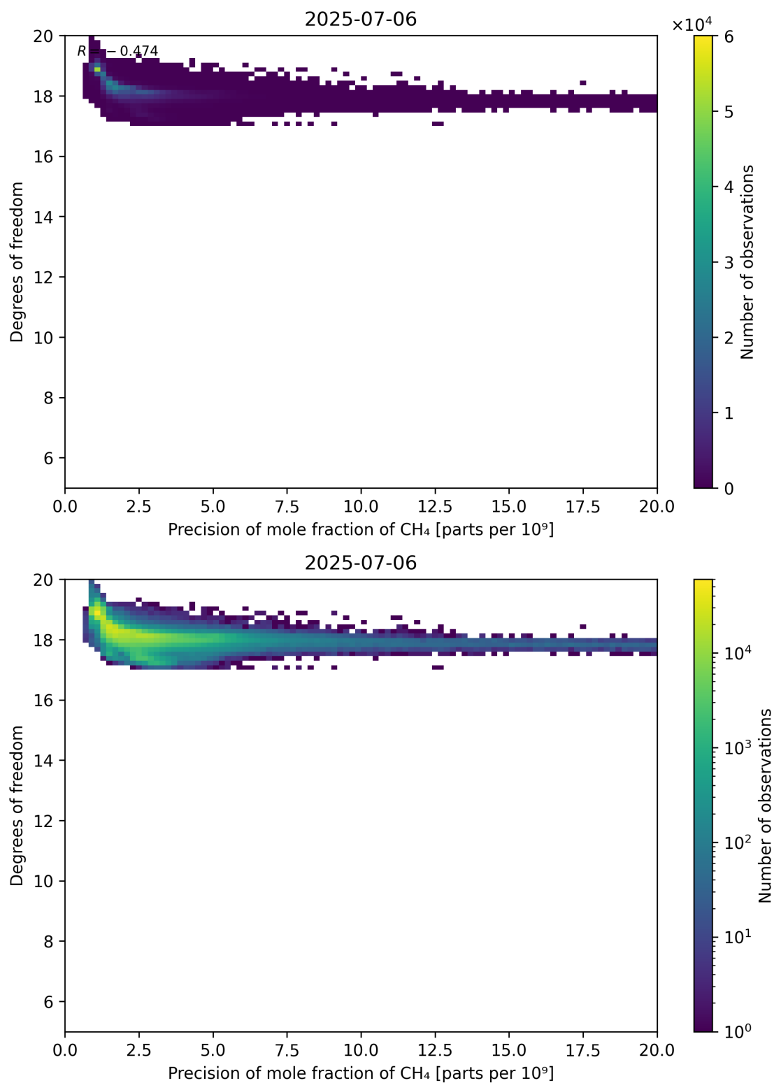
Figure 80: Scatter density plot of “Precision of mole fraction of CH 4 ” against “Degrees of freedom” for 2025-07-05 to 2025-07-07.
