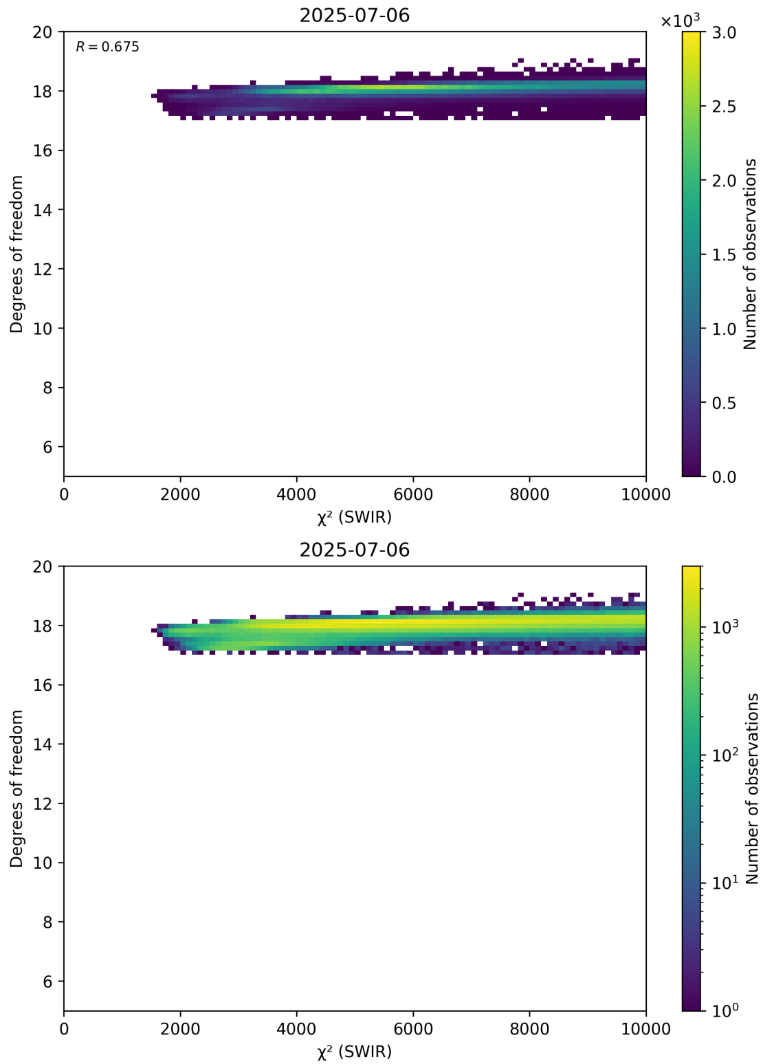
Figure 48: Scatter density plot of “ \chi^2 (SWIR)” against “Degrees of freedom” for 2025-07-05 to 2025-07-07.
