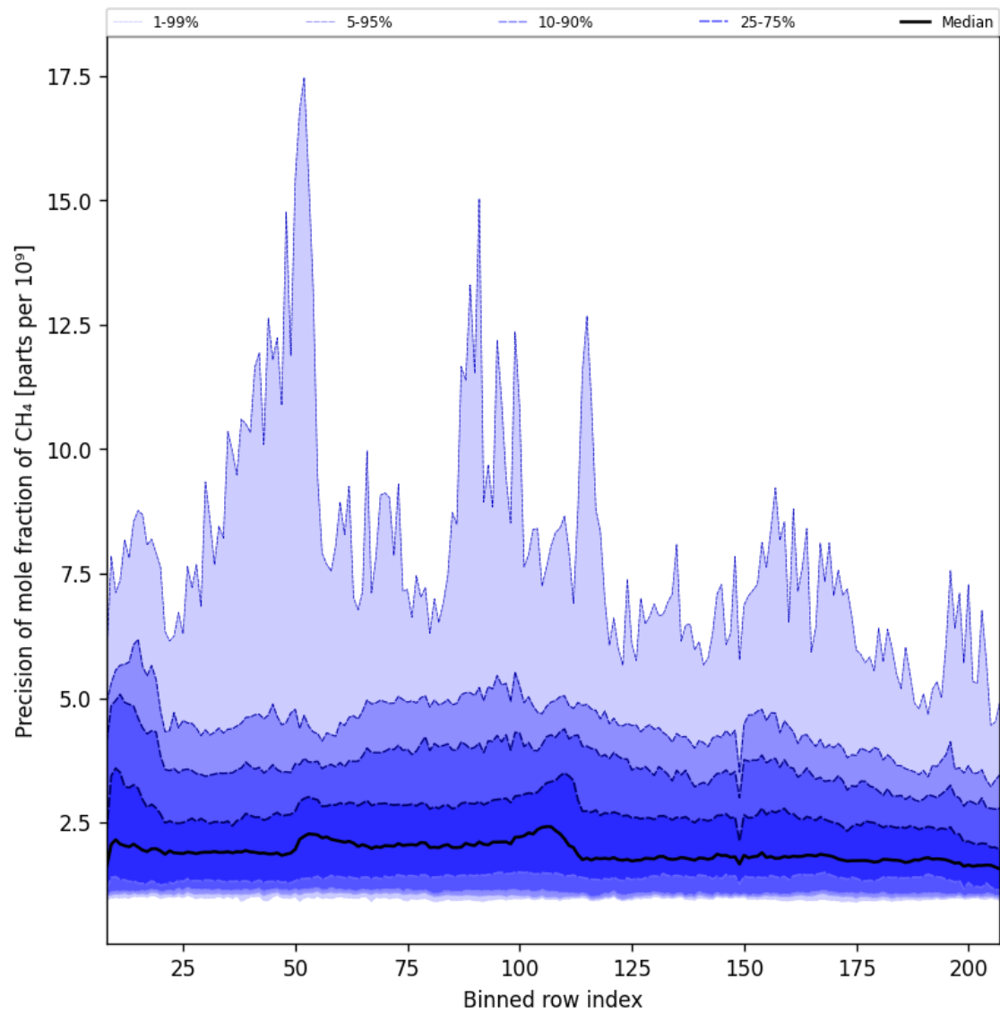
Figure 35: Along track statistics of “Precision of mole fraction of CH 4 ” for 2025-07-05 to 2025-07-07
