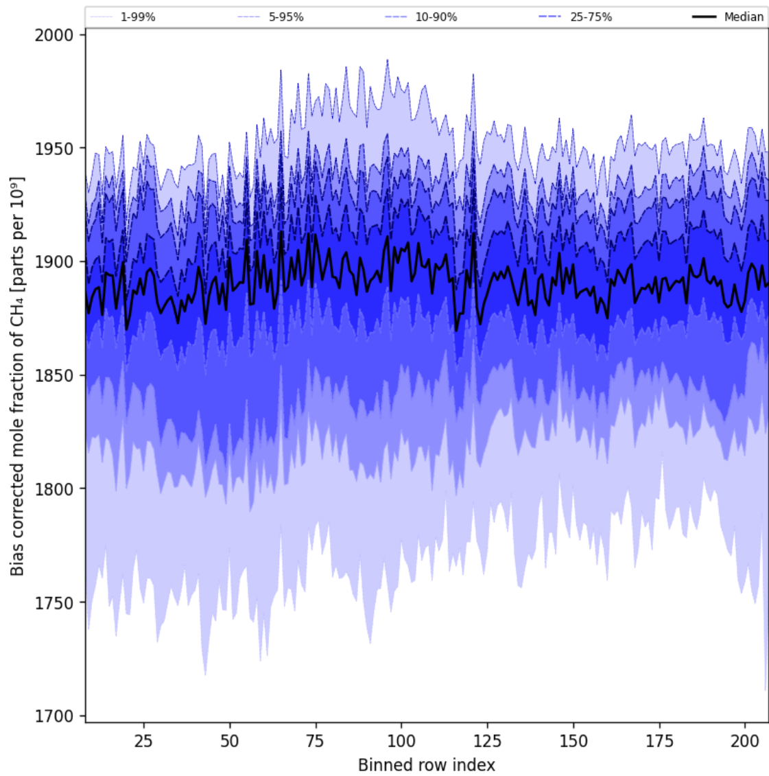
Figure 36: Along track statistics of “Bias corrected mole fraction of CH 4 ” for 2025-07-05 to 2025-07-07
