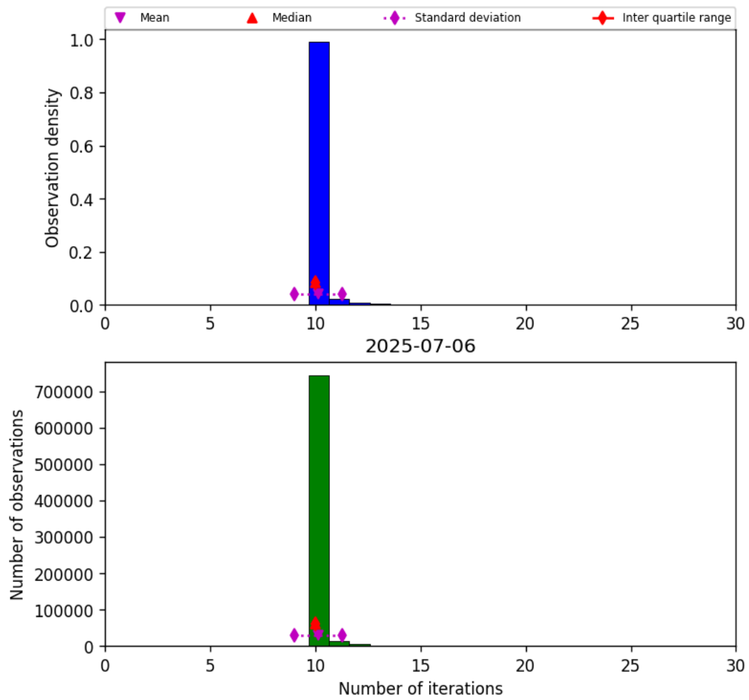
Figure 31: Histogram of “Number of iterations” for 2025-07-05 to 2025-07-07
