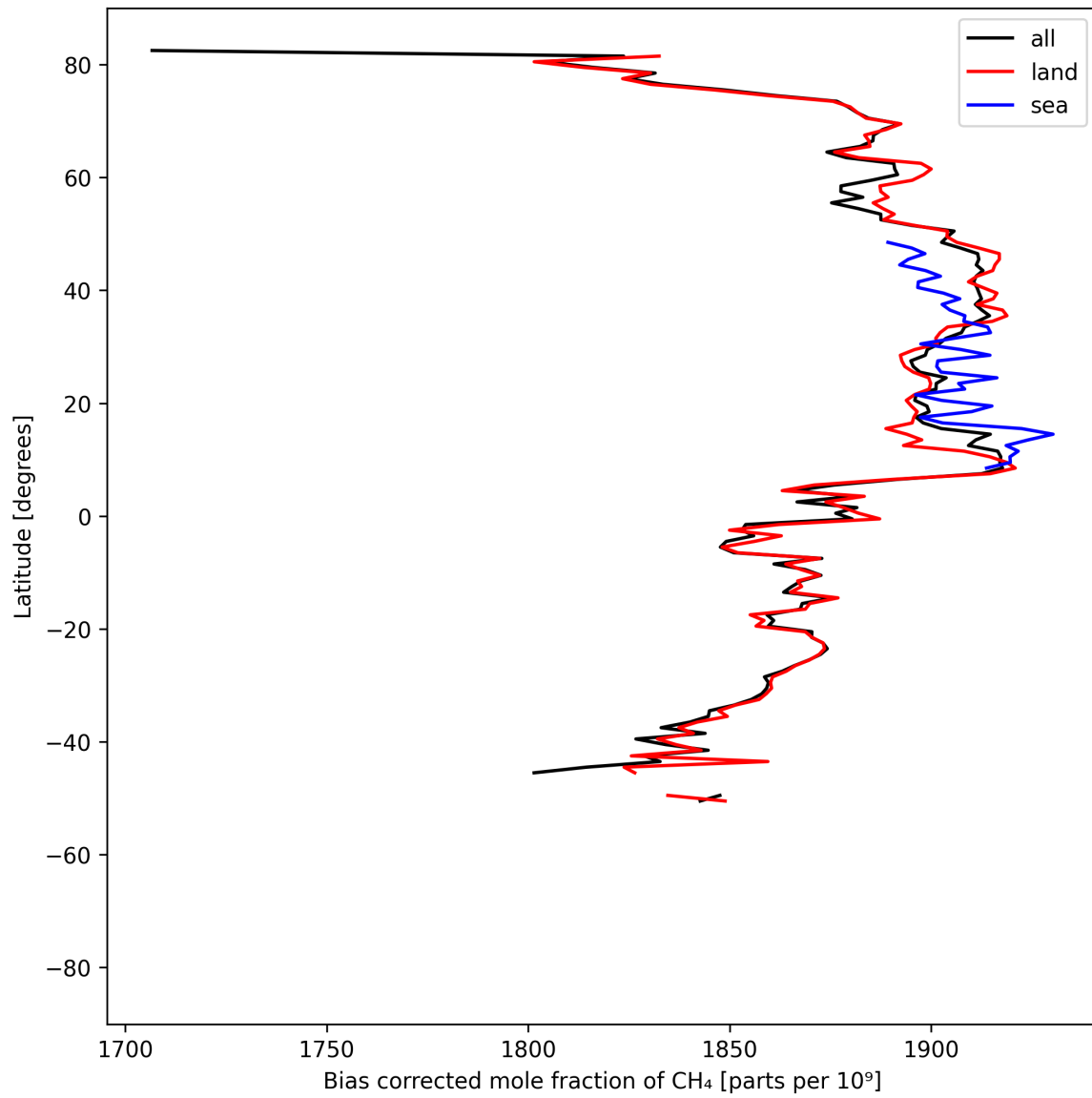
Figure 14: Zonal average of “Bias corrected mole fraction of \text{CH}_4 ” for 2025-07-05 to 2025-07-07.
