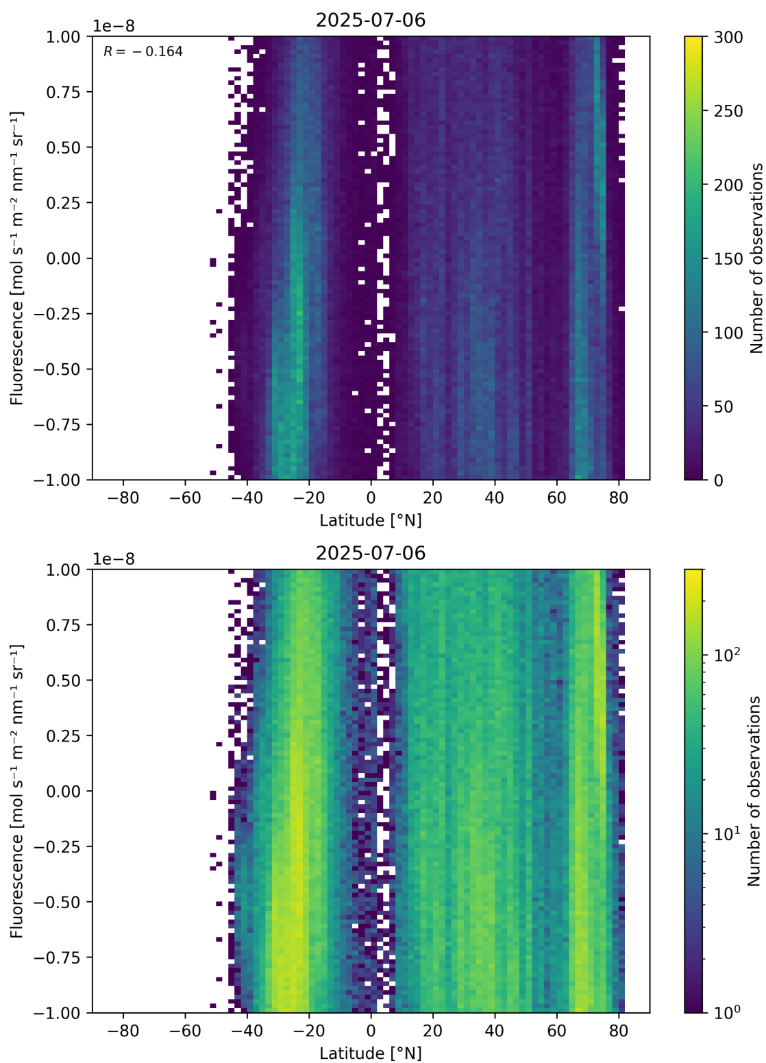
Figure 56: Scatter density plot of “Latitude” against “Fluorescence” for 2025-07-05 to 2025-07-07.
