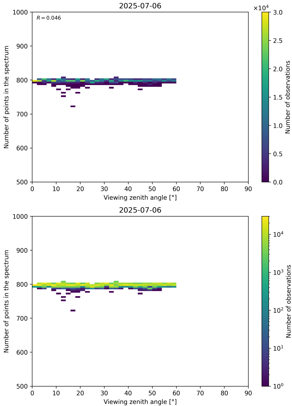
Figure 114: Scatter density plot of “Viewing zenith angle” against “Number of points in the spectrum” for 2025-07-05 to 2025-07-07.
