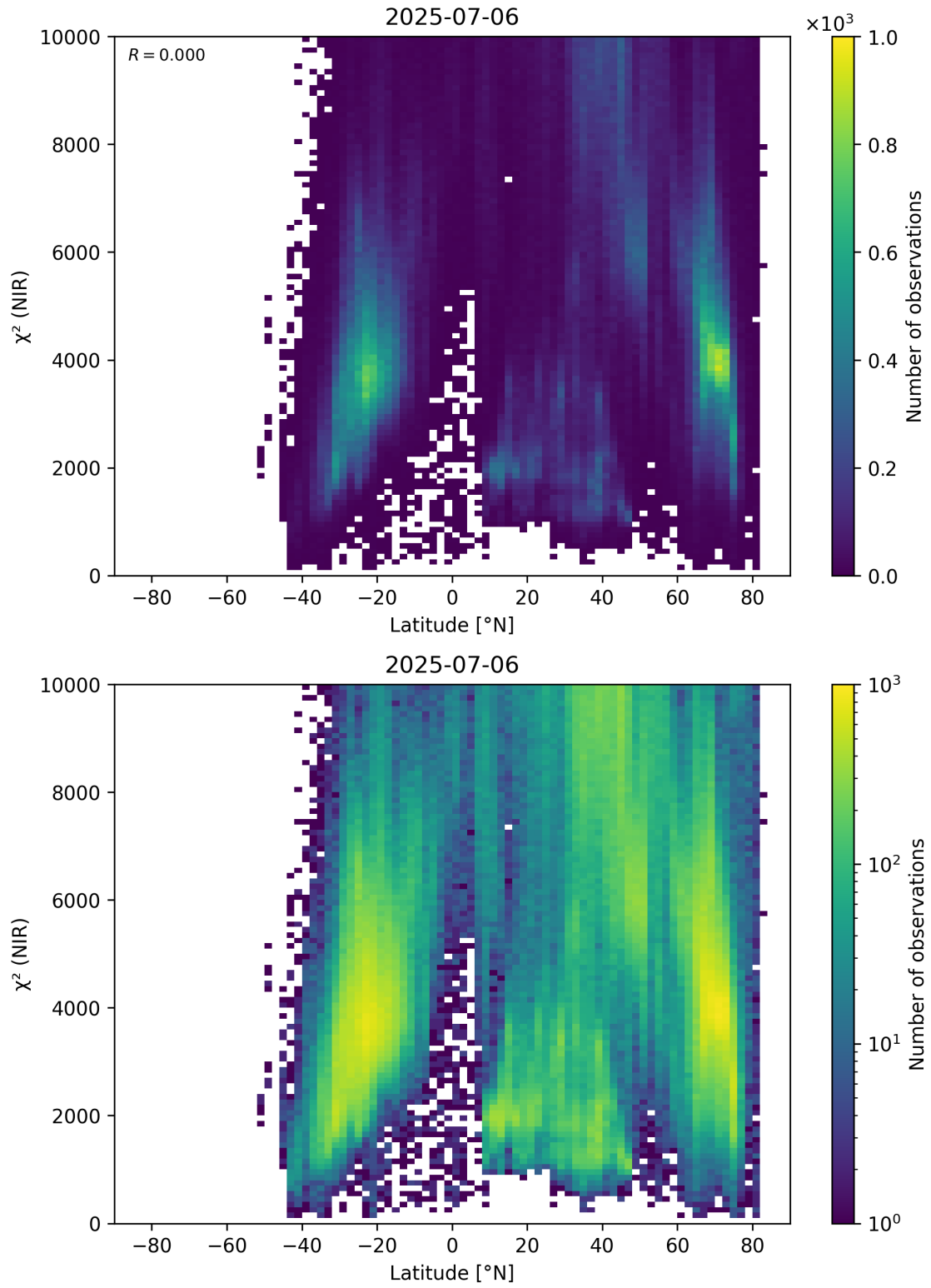
Figure 53: Scatter density plot of “Latitude” against “ \chi^2 (NIR)” for 2025-07-05 to 2025-07-07.
