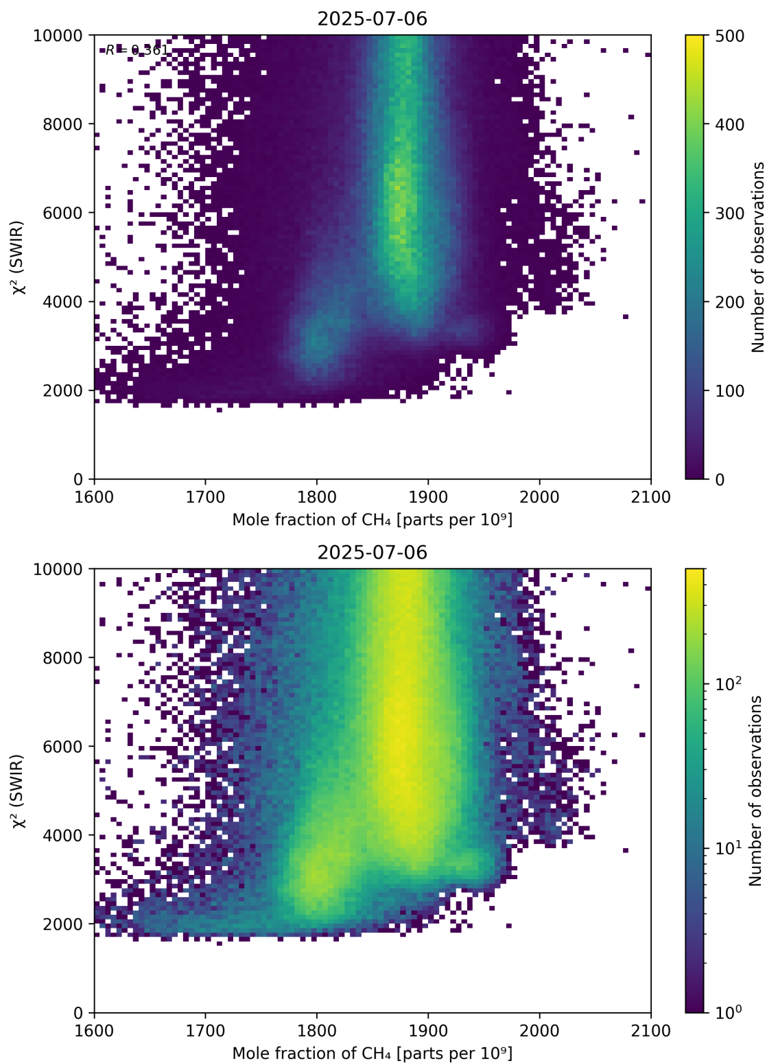
Figure 71: Scatter density plot of “Mole fraction of CH 4 ” against “ \chi^2 (SWIR)” for 2025-07-05 to 2025-07-07.
