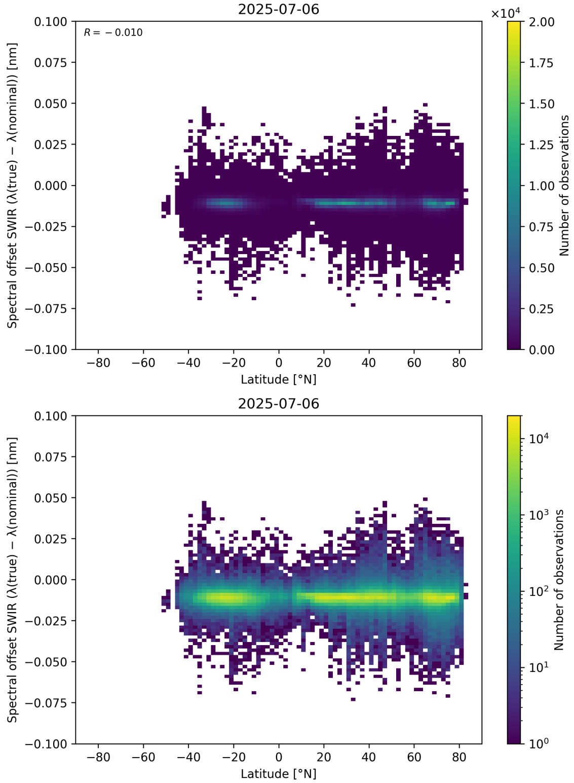
Figure 62: Scatter density plot of “Latitude” against “Spectral offset SWIR ( \lambda_{\text{true}} - \lambda_{\text{nominal}} )” for 2025-07-05 to 2025-07-07.
