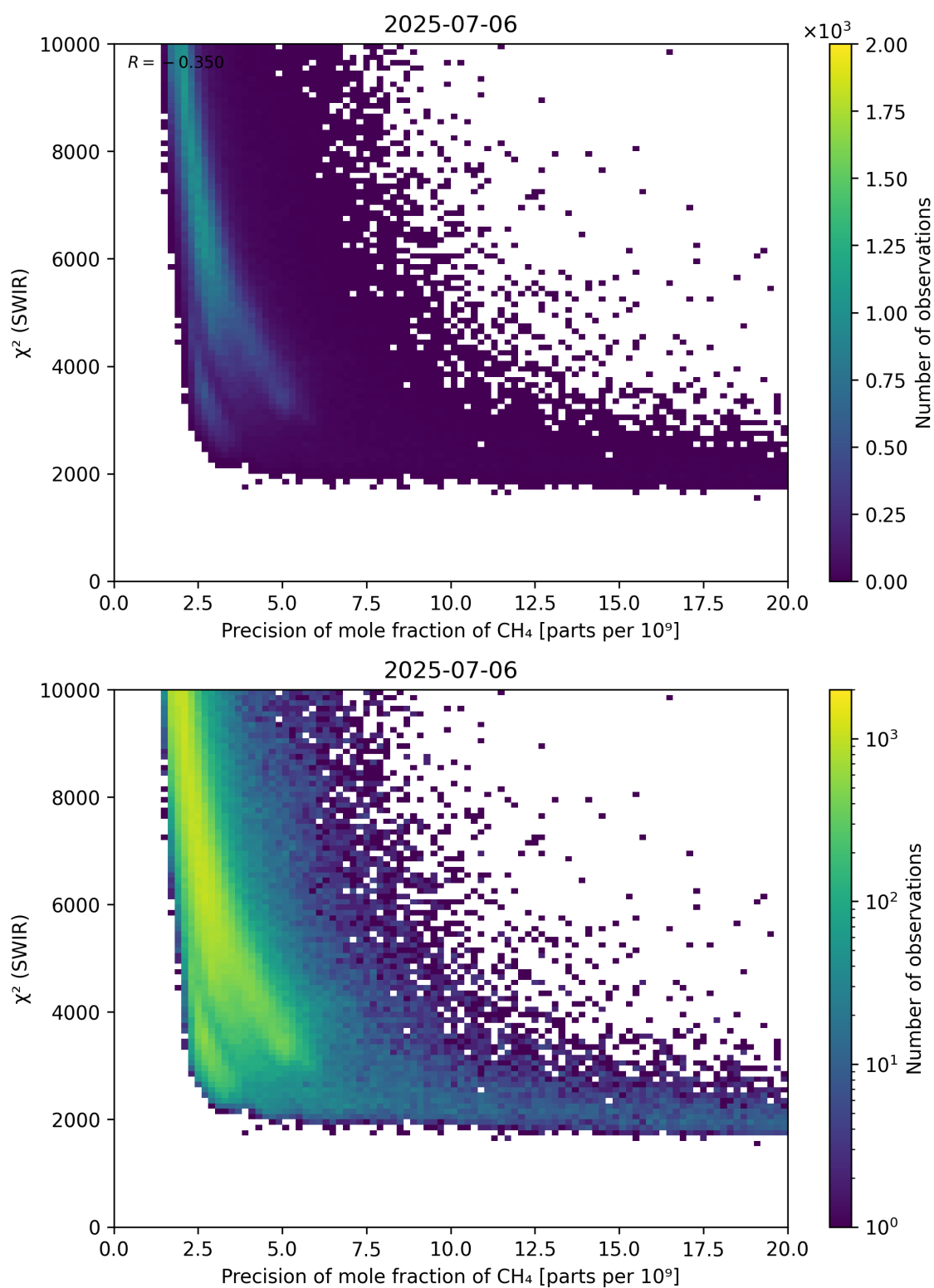
Figure 79: Scatter density plot of “Precision of mole fraction of CH 4 ” against “ \chi^2 (SWIR)” for 2025-07-05 to 2025-07-07.
