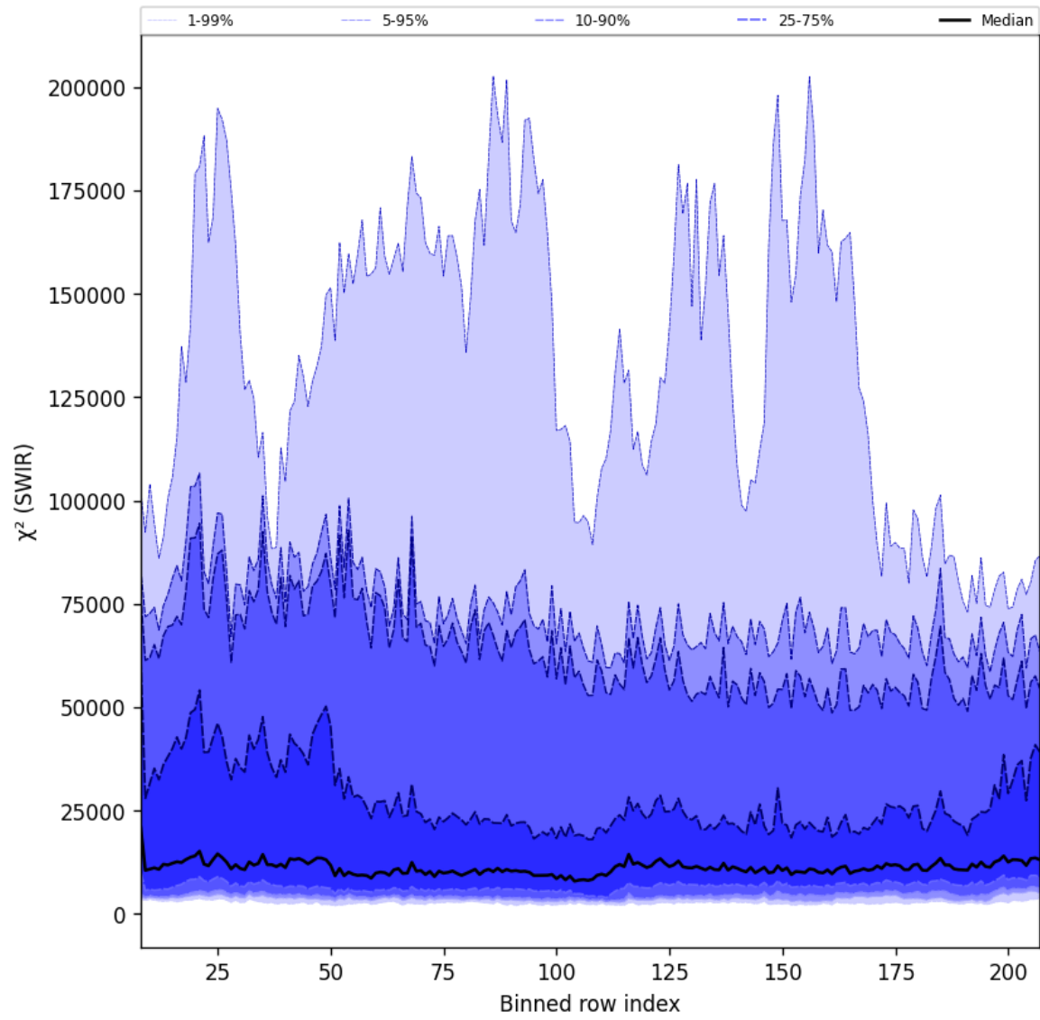
Figure 39: Along track statistics of “ \chi^2 (SWIR)” for 2025-07-05 to 2025-07-07
