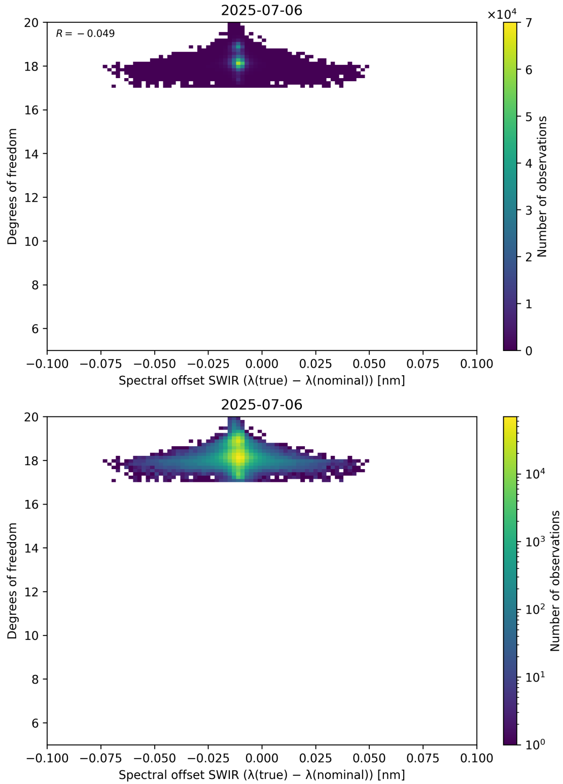
Figure 119: Scatter density plot of “Spectral offset SWIR ( \lambda_{\text{true}} - \lambda_{\text{nominal}} )” against “Degrees of freedom” for 2025-07-05 to 2025-07-07.
