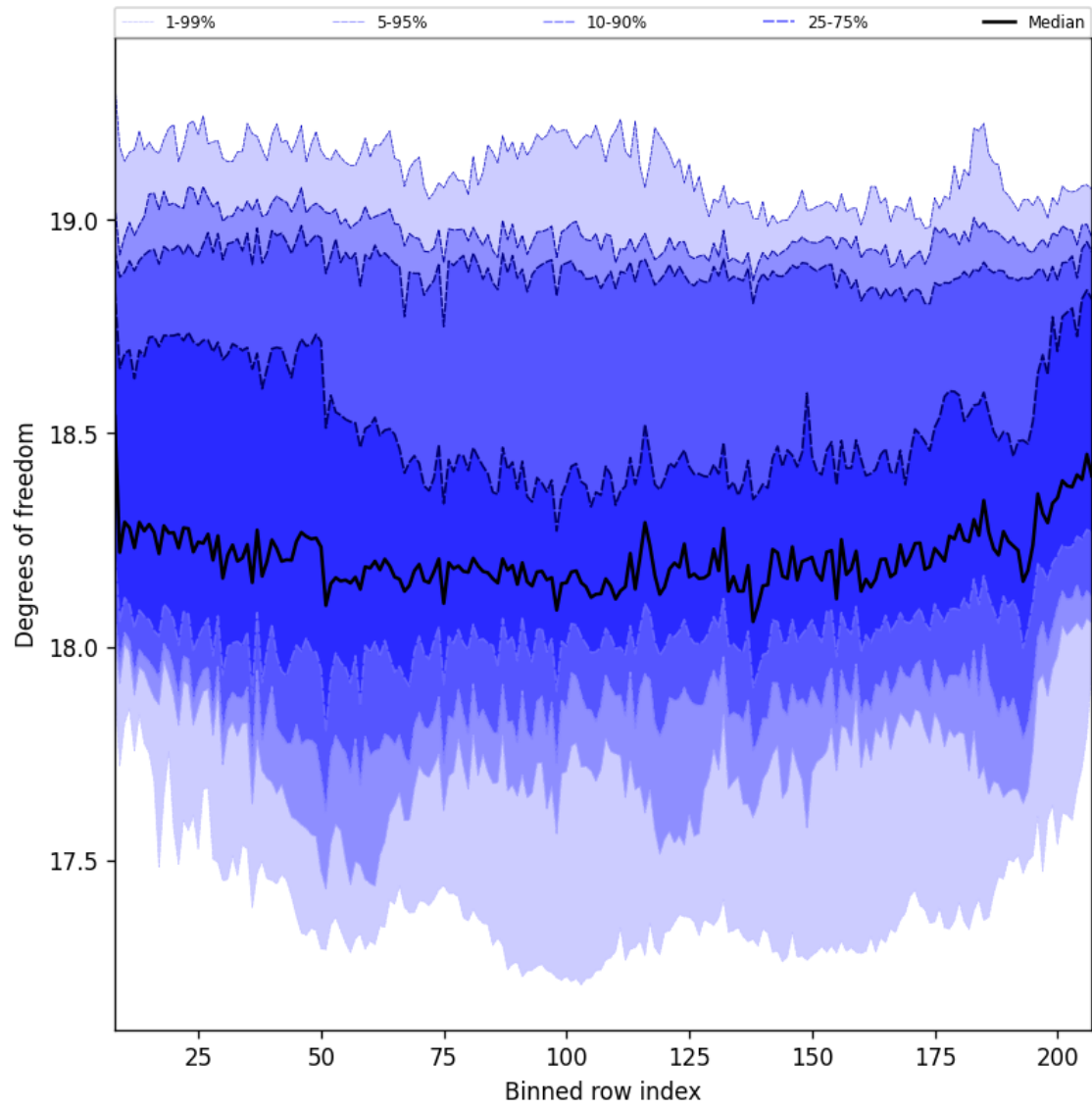
Figure 41: Along track statistics of “Degrees of freedom” for 2025-07-05 to 2025-07-07
