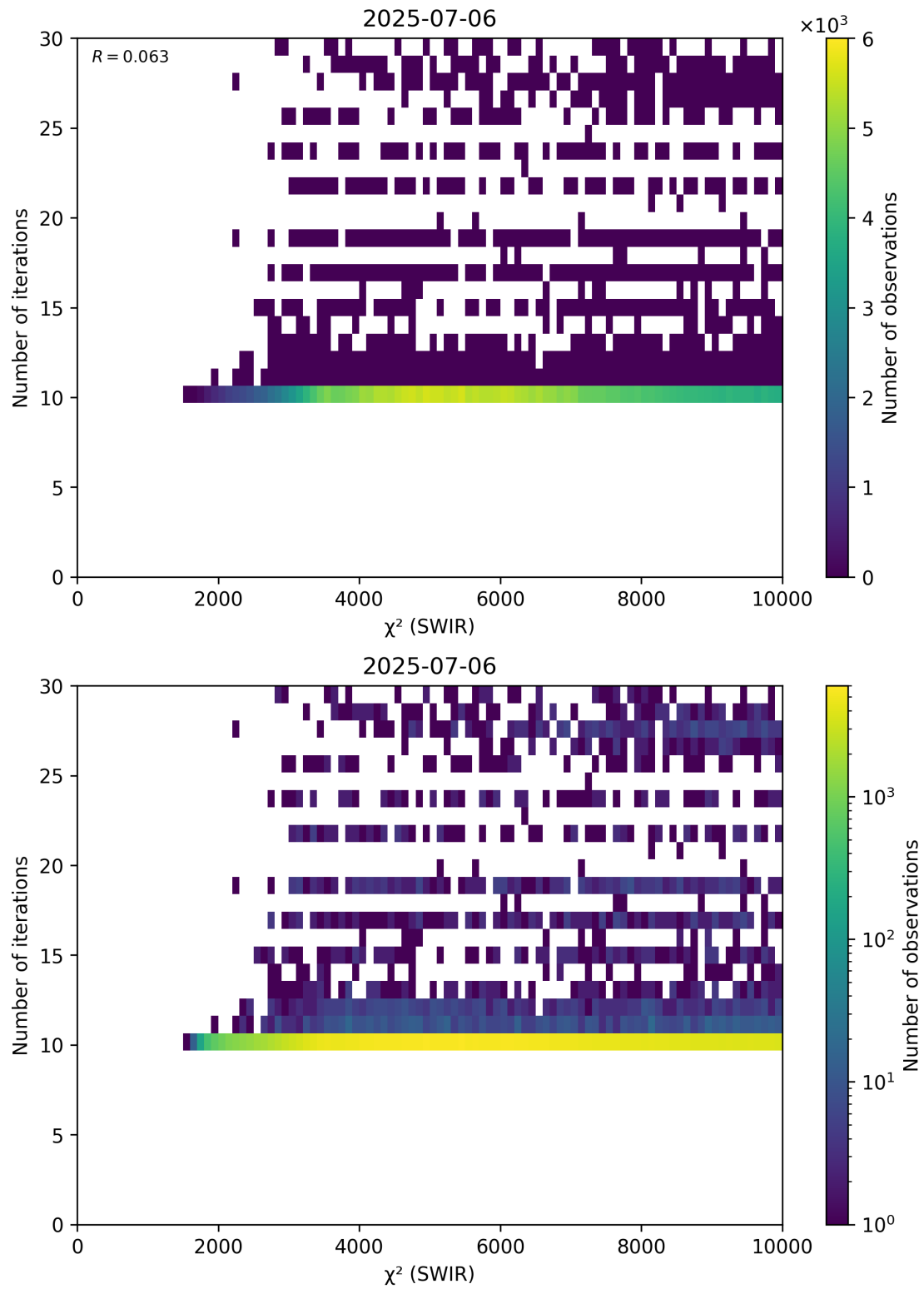
Figure 50: Scatter density plot of “ \chi^2 (SWIR)” against “Number of iterations” for 2025-07-05 to 2025-07-07.
