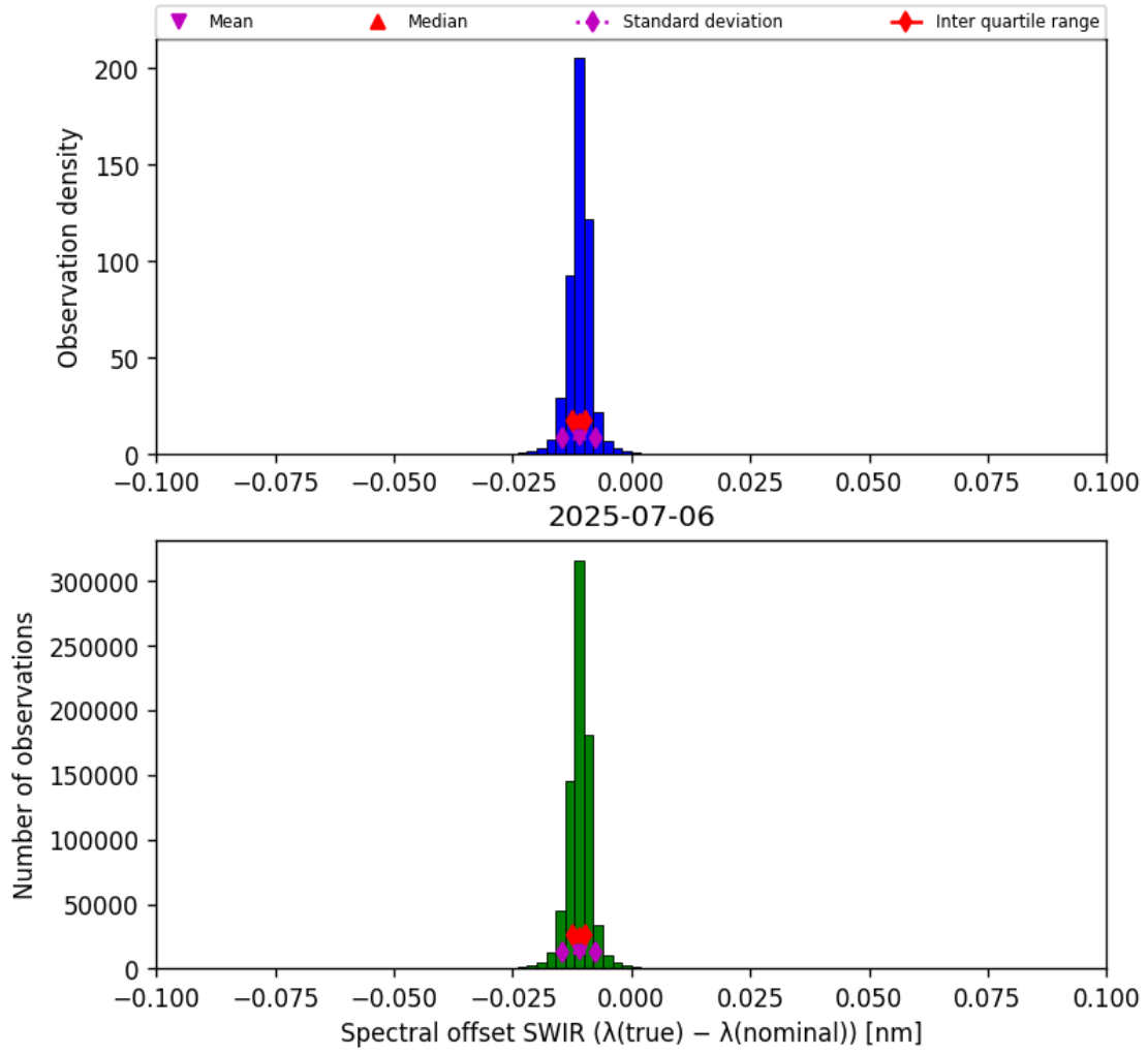
Figure 27: Histogram of “Spectral offset SWIR ( \lambda_{\text{true}} - \lambda_{\text{nominal}} )” for 2025-07-05 to 2025-07-07
