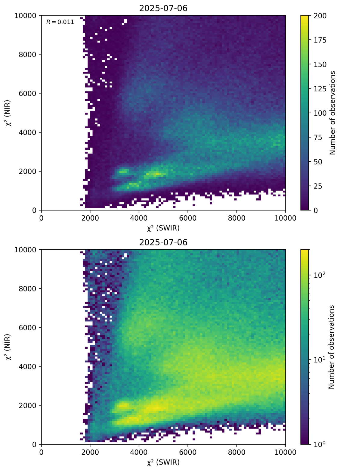
Figure 47: Scatter density plot of “ \chi^2 (SWIR)” against “ \chi^2 (NIR)” for 2025-07-05 to 2025-07-07.
