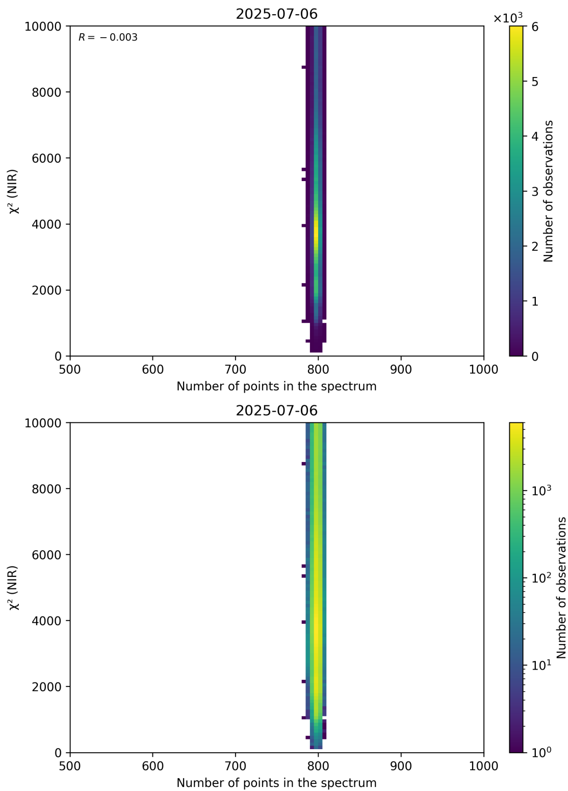
Figure 88: Scatter density plot of “Number of points in the spectrum” against “ \chi^2 (NIR)” for 2025-07-05 to 2025-07-07.
