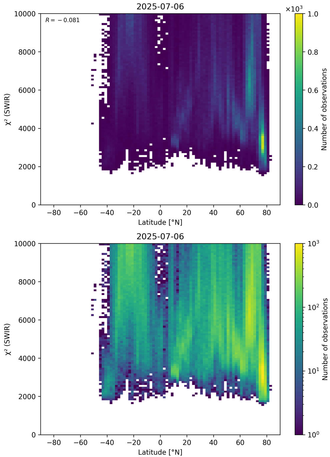
Figure 54: Scatter density plot of “Latitude” against “ \chi^2 (SWIR)” for 2025-07-05 to 2025-07-07.
