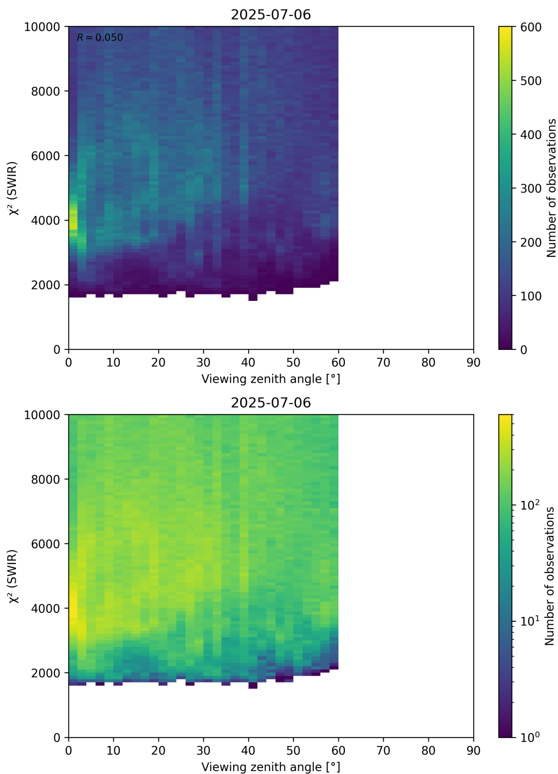
Figure 106: Scatter density plot of “Viewing zenith angle” against “ \chi^2 (SWIR)” for 2025-07-05 to 2025-07-07.
