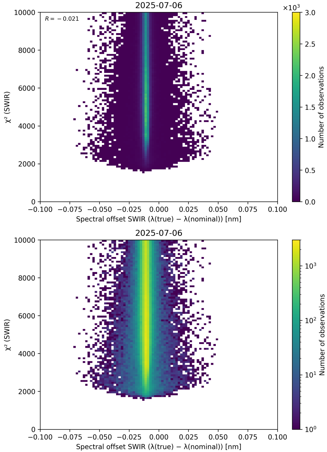
Figure 118: Scatter density plot of “Spectral offset SWIR ( \lambda_{\text{true}} - \lambda_{\text{nominal}} )” against “ \chi^2 (SWIR)” for 2025-07-05 to 2025-07-07.
