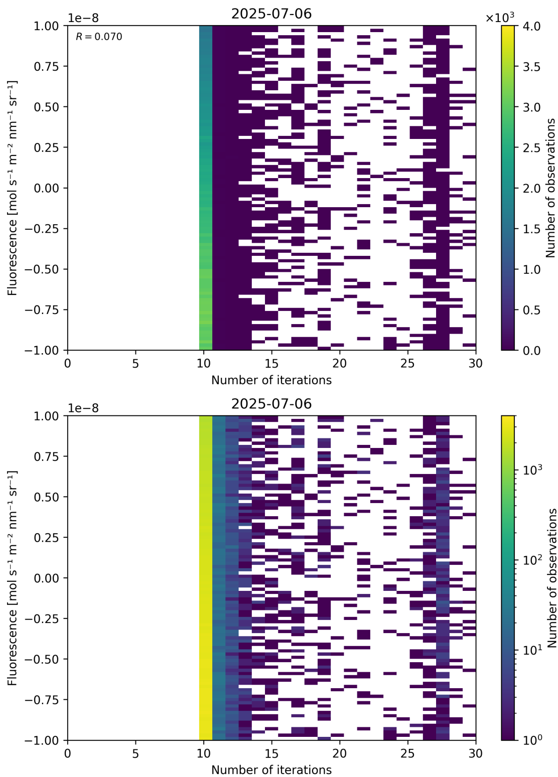
Figure 87: Scatter density plot of “Number of iterations” against “Fluorescence” for 2025-07-05 to 2025-07-07.
