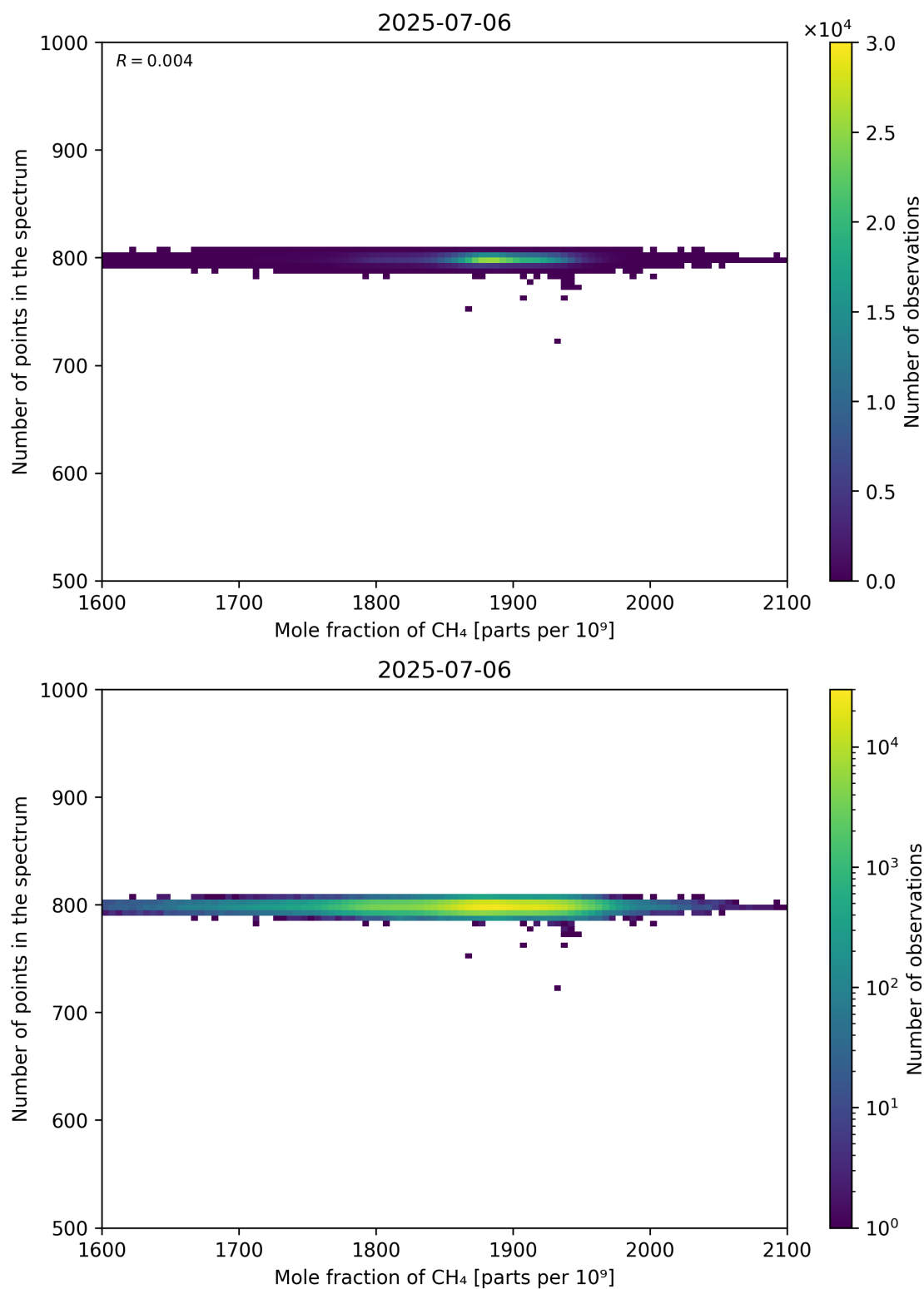
Figure 77: Scatter density plot of “Mole fraction of CH 4 ” against “Number of points in the spectrum” for 2025-07-05 to 2025-07-07.
