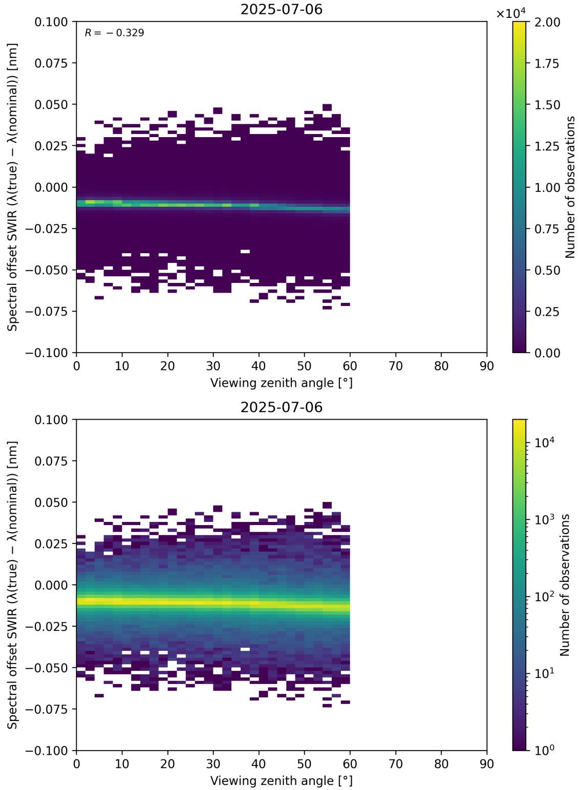
Figure 116: Scatter density plot of “Viewing zenith angle” against “Spectral offset SWIR ( \lambda_{\text{true}} - \lambda_{\text{nominal}} )” for 2025-07-05 to 2025-07-07.
