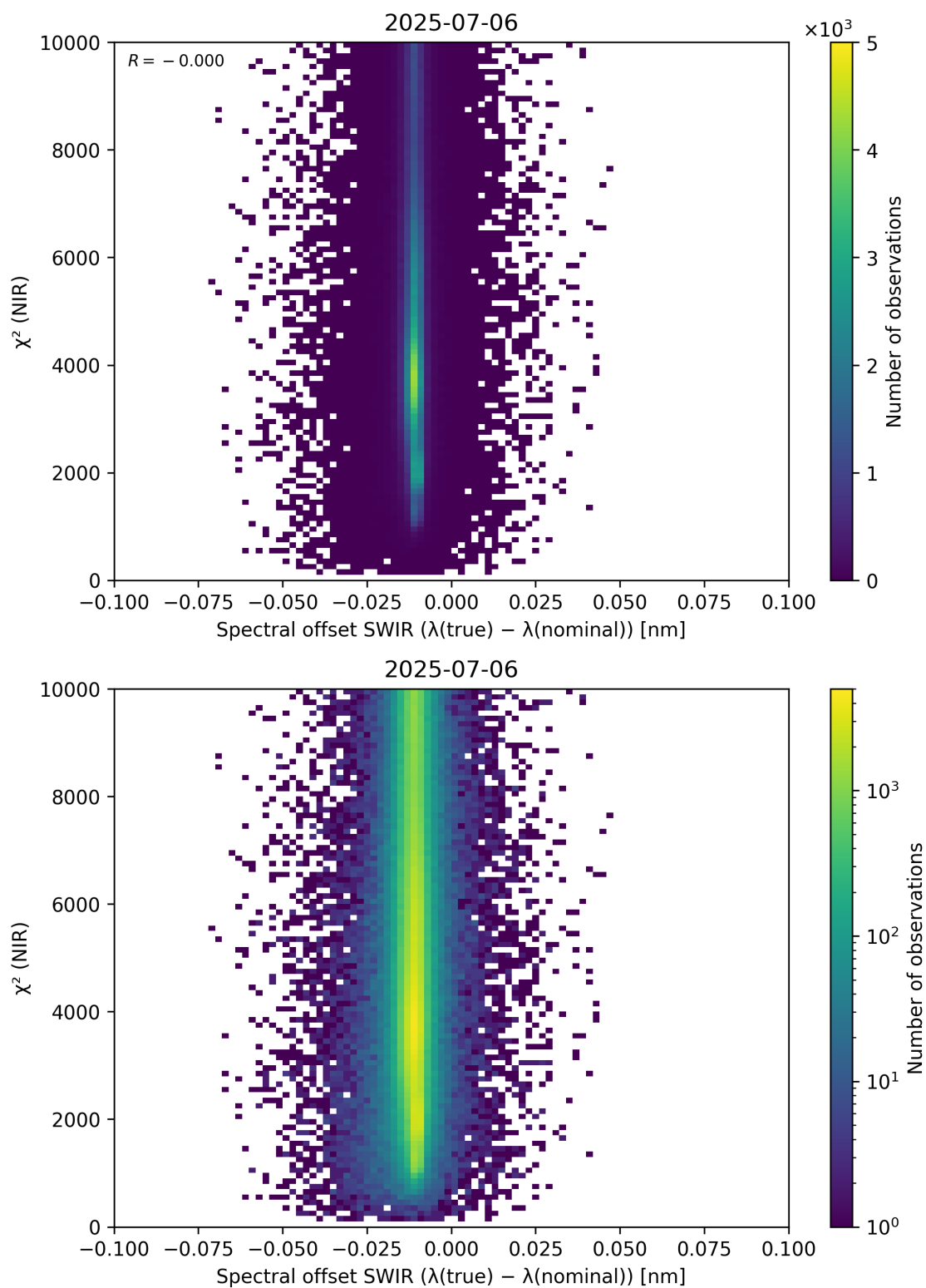
Figure 117: Scatter density plot of “Spectral offset SWIR ( \lambda_{\text{true}} - \lambda_{\text{nominal}} )” against “ \chi^2 (NIR)” for 2025-07-05 to 2025-07-07.
