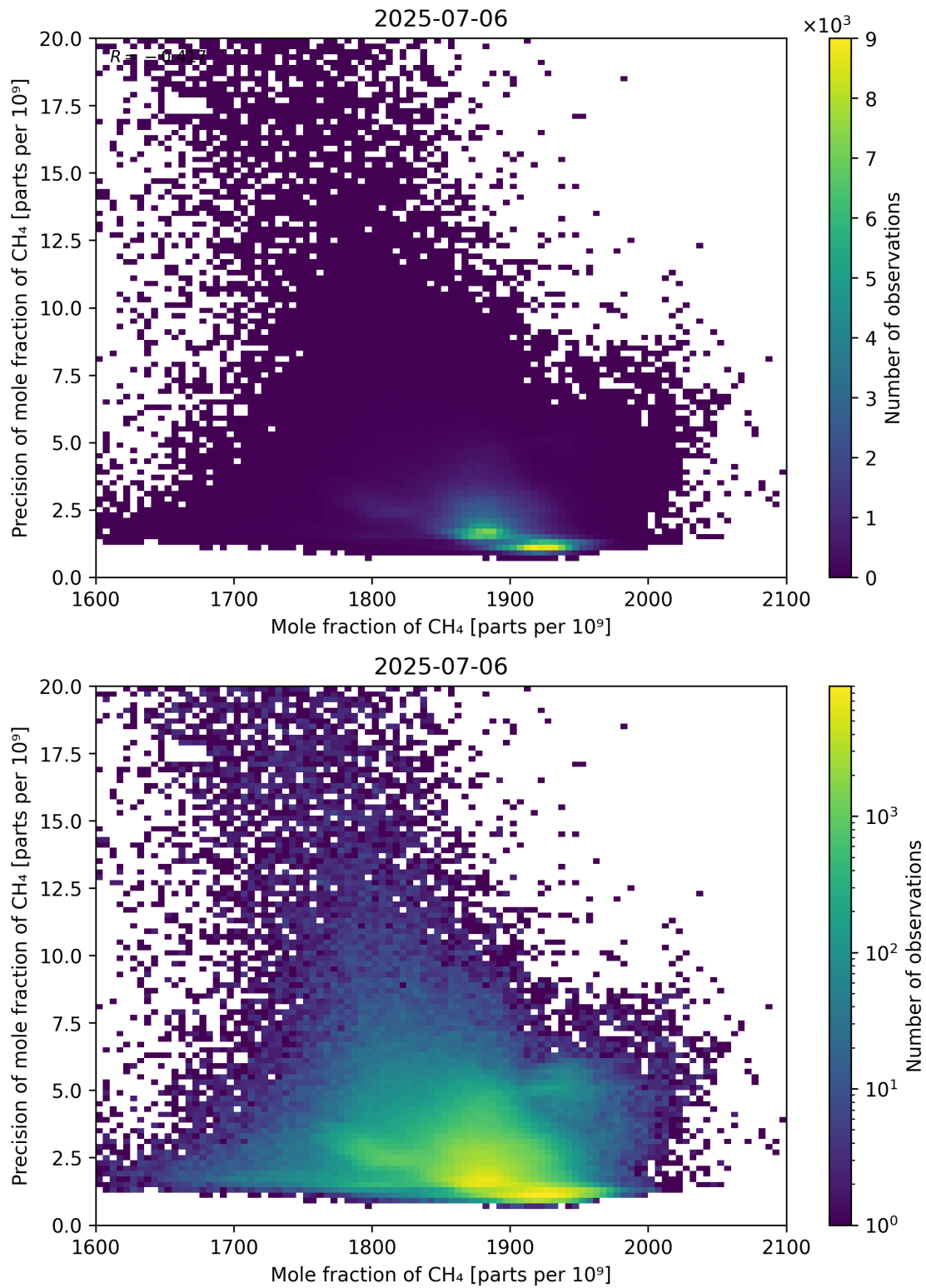
Figure 75: Scatter density plot of “Mole fraction of CH 4 ” against “Precision of mole fraction of CH 4 ” for 2025-07-05 to 2025-07-07.
