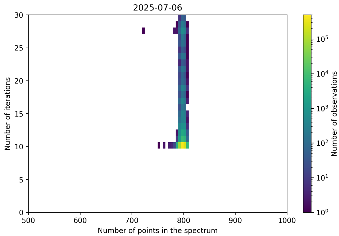
Figure 92: Scatter density plot of “Number of points in the spectrum” against “Number of iterations” for 2025-07-05 to 2025-07-07.
