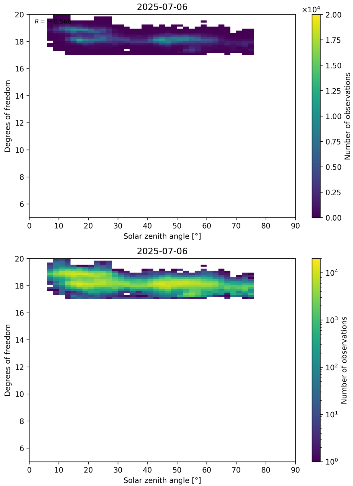
Figure 96: Scatter density plot of “Solar zenith angle” against “Degrees of freedom” for 2025-07-05 to 2025-07-07.
