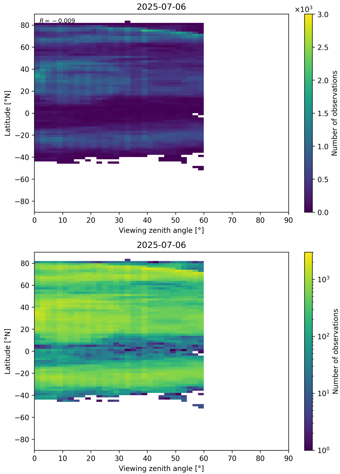
Figure 109: Scatter density plot of “Viewing zenith angle” against “Latitude” for 2025-07-05 to 2025-07-07.
