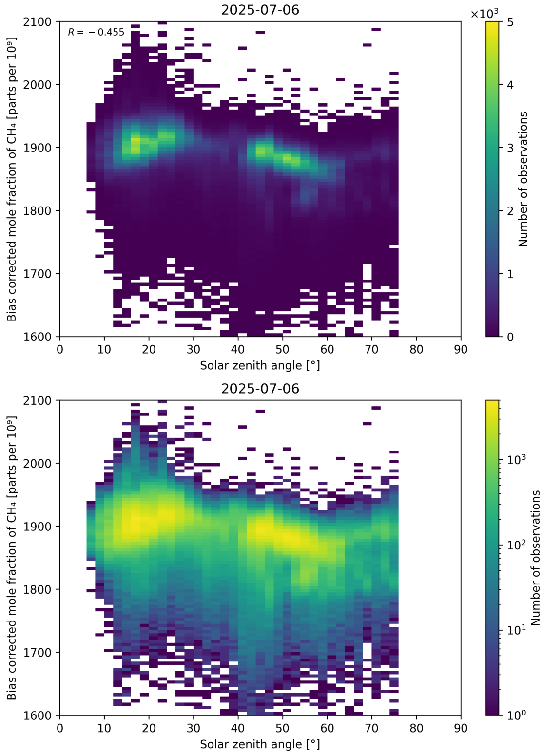
Figure 100: Scatter density plot of “Solar zenith angle” against “Bias corrected mole fraction of \text{CH}_4 ” for 2025-07-05 to 2025-07-07.
