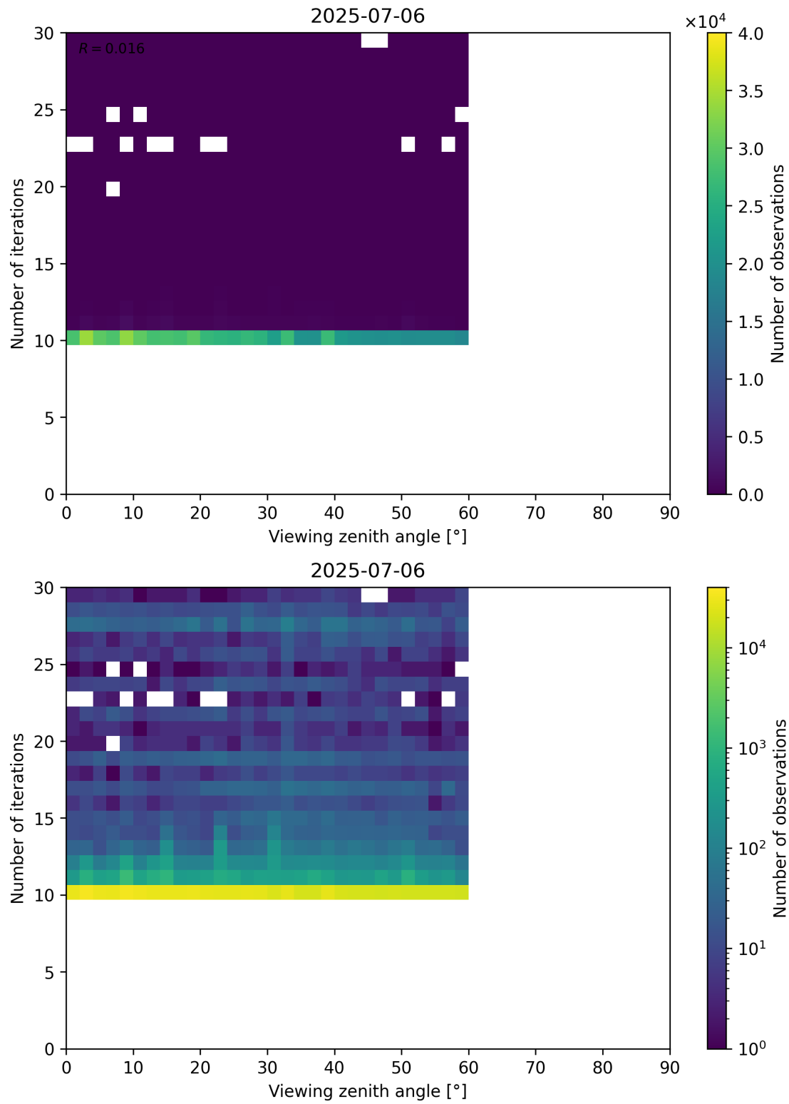
Figure 113: Scatter density plot of “Viewing zenith angle” against “Number of iterations” for 2025-07-05 to 2025-07-07.
