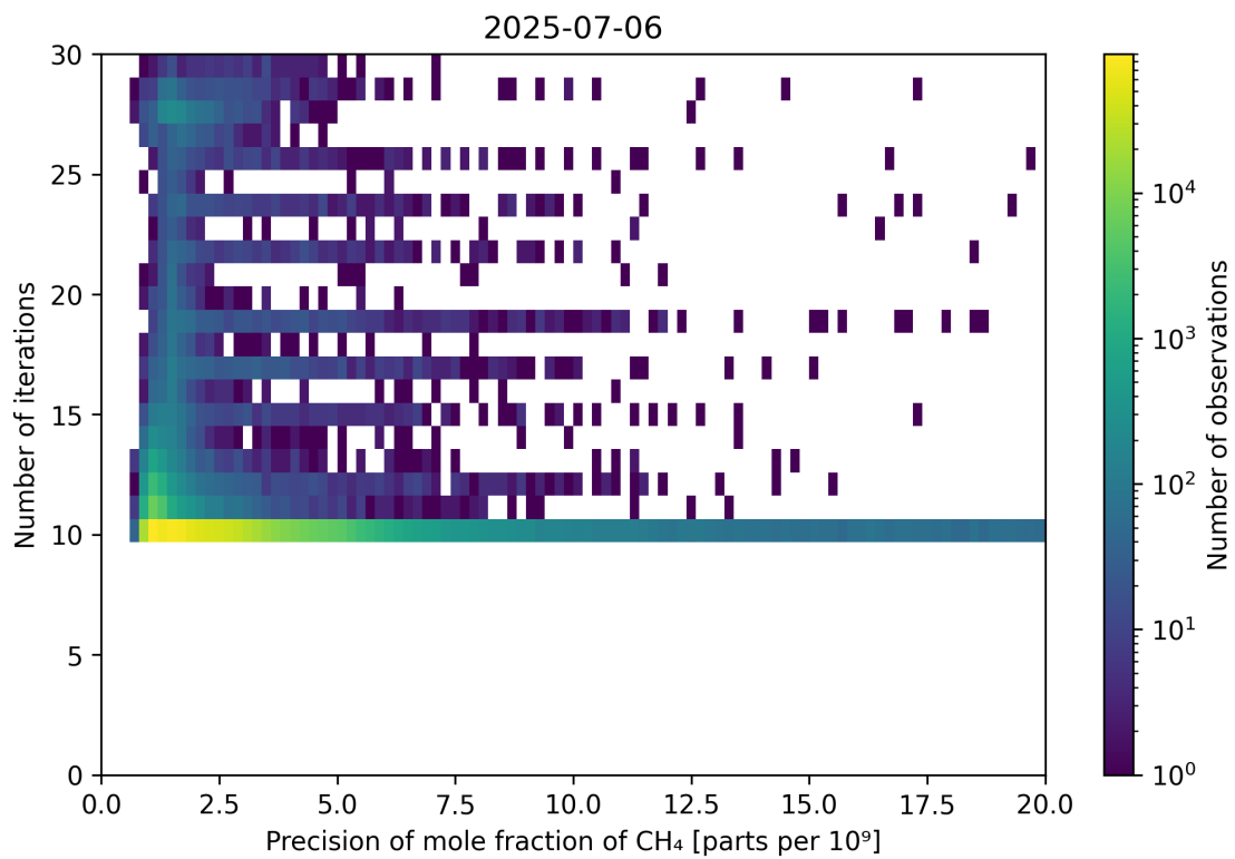
Figure 83: Scatter density plot of “Precision of mole fraction of CH 4 ” against “Number of iterations” for 2025-07-05 to 2025-07-07.
