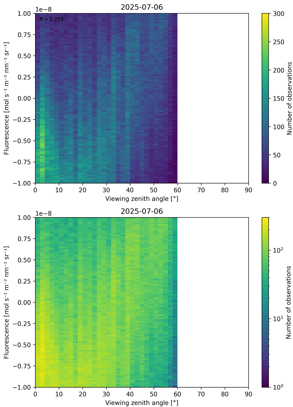
Figure 108: Scatter density plot of “Viewing zenith angle” against “Fluorescence” for 2025-07-05 to 2025-07-07.
