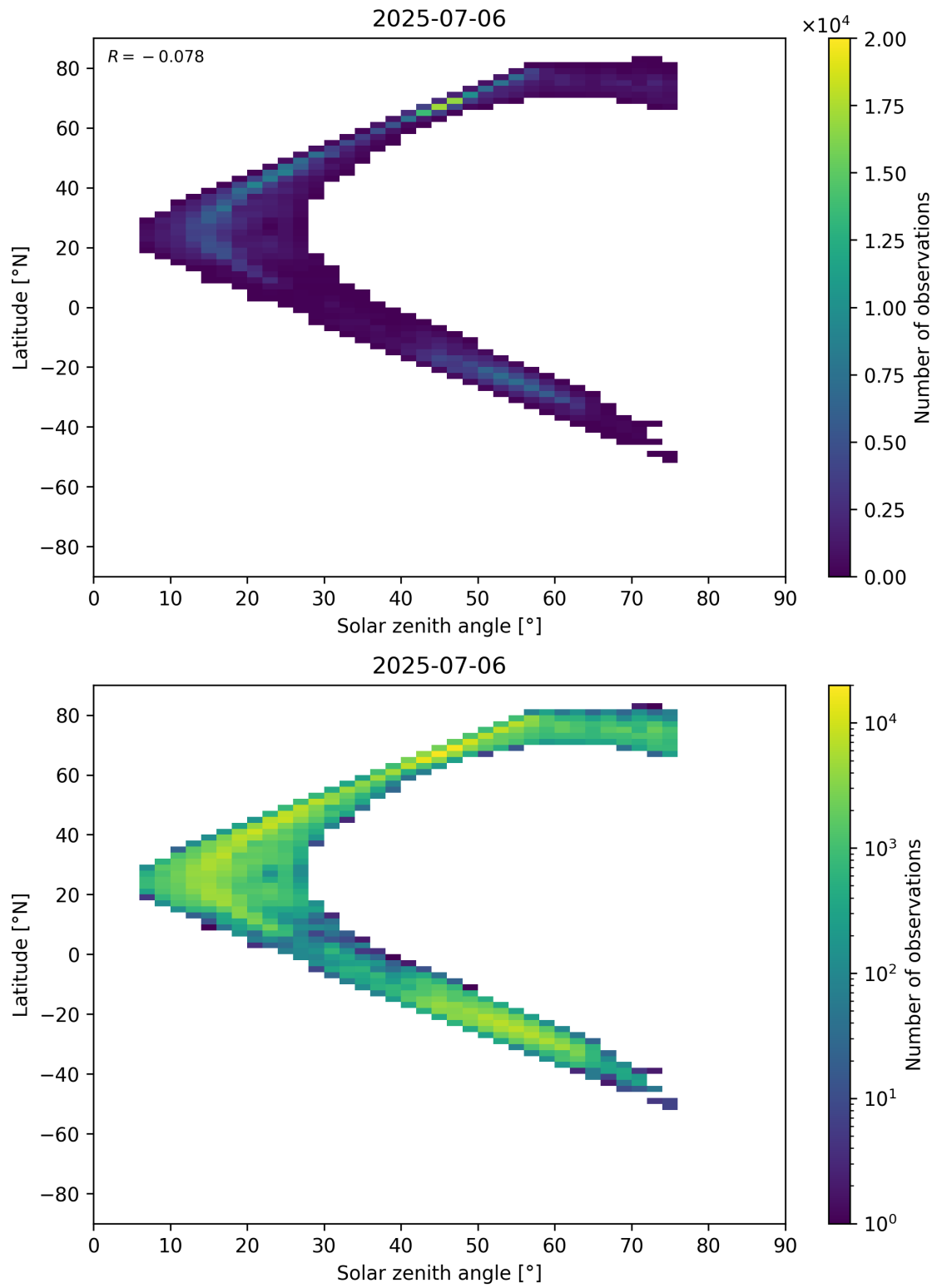
Figure 98: Scatter density plot of “Solar zenith angle” against “Latitude” for 2025-07-05 to 2025-07-07.
