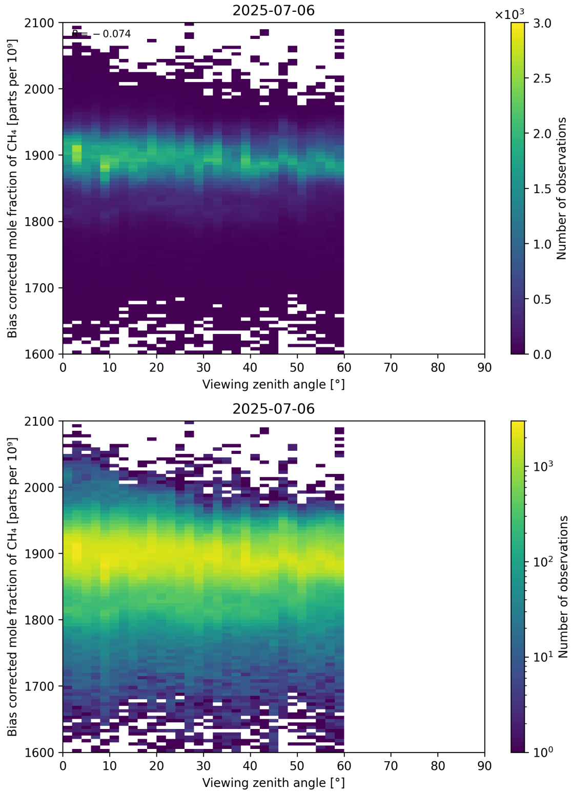
Figure 111: Scatter density plot of “Viewing zenith angle” against “Bias corrected mole fraction of CH 4 ” for 2025-07-05 to 2025-07-07.
