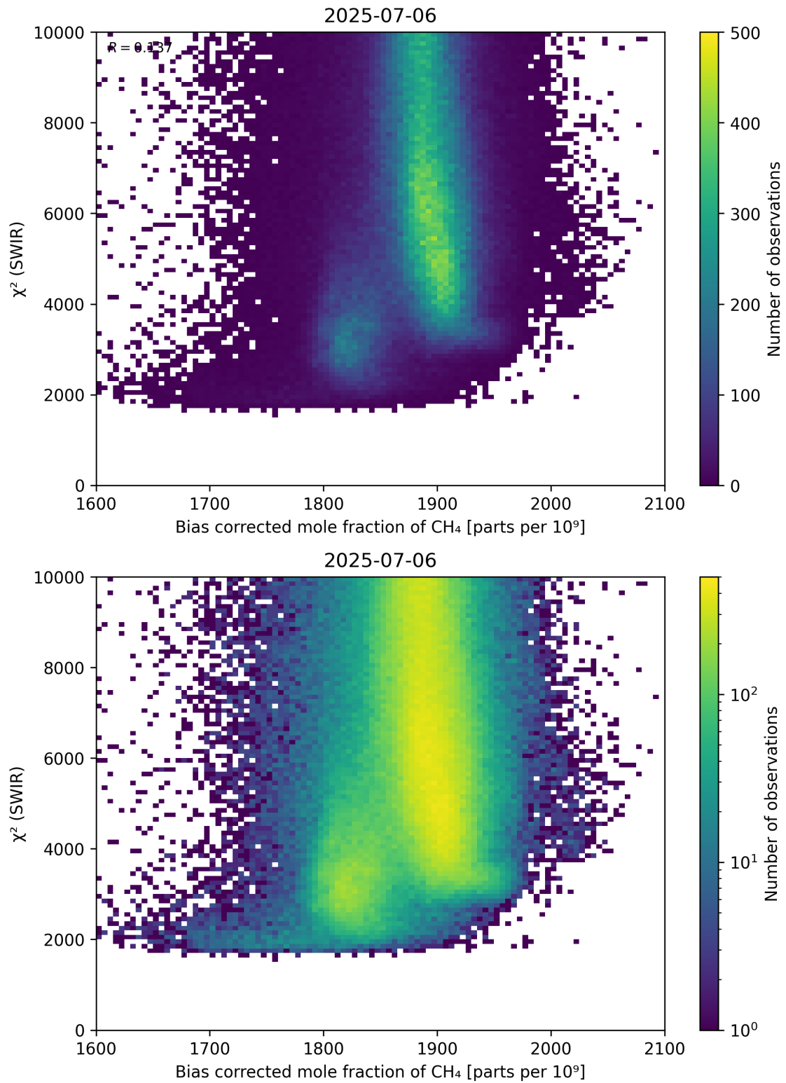
Figure 64: Scatter density plot of “Bias corrected mole fraction of \text{CH}_4 ” against “ \chi^2 (SWIR)” for 2025-07-05 to 2025-07-07.
