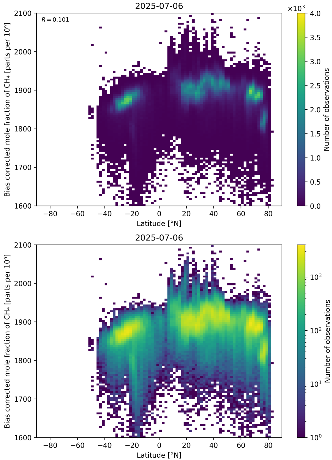
Figure 58: Scatter density plot of “Latitude” against “Bias corrected mole fraction of CH 4 ” for 2025-07-05 to 2025-07-07.
