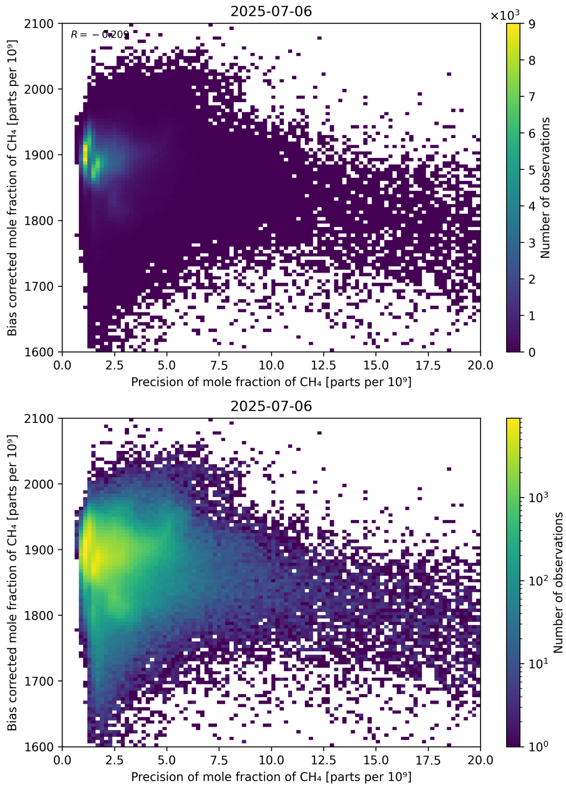
Figure 82: Scatter density plot of “Precision of mole fraction of CH 4 ” against “Bias corrected mole fraction of CH 4 ” for 2025-07-05 to 2025-07-07.
