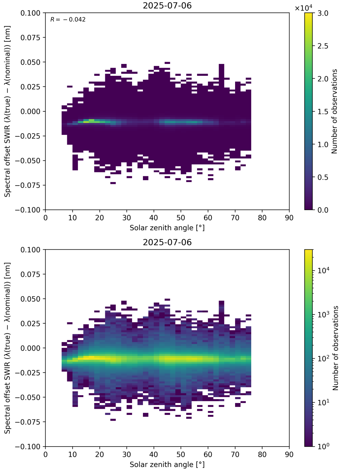
Figure 104: Scatter density plot of “Solar zenith angle” against “Spectral offset SWIR ( \lambda_{\text{true}} - \lambda_{\text{nominal}} )” for 2025-07-05 to 2025-07-07.
