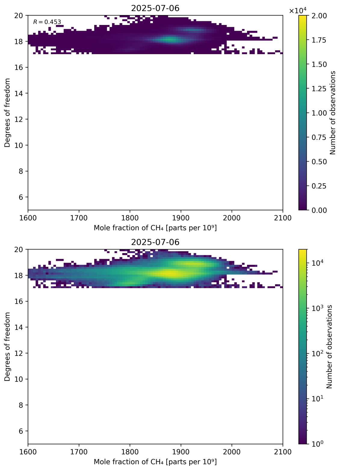
Figure 72: Scatter density plot of “Mole fraction of CH 4 ” against “Degrees of freedom” for 2025-07-05 to 2025-07-07.
