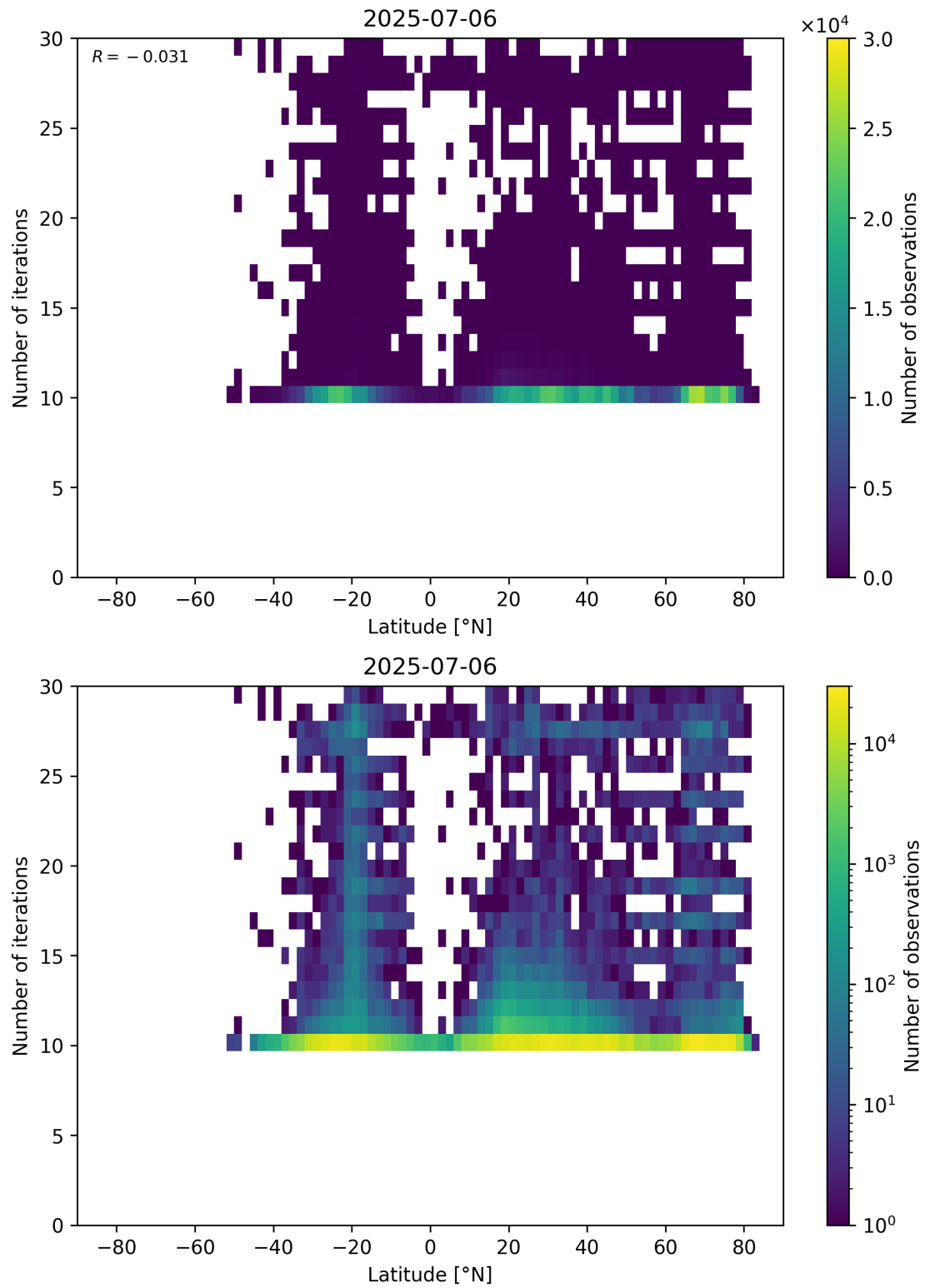
Figure 60: Scatter density plot of “Latitude” against “Number of iterations” for 2025-07-05 to 2025-07-07.
