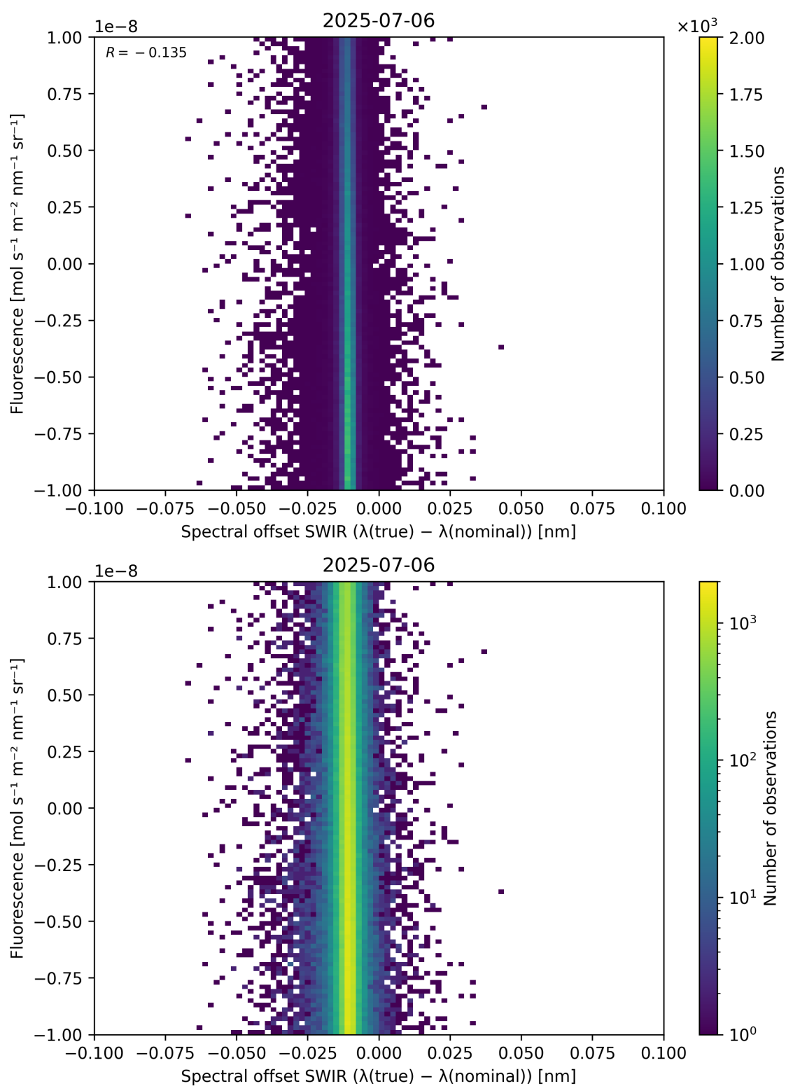
Figure 120: Scatter density plot of “Spectral offset SWIR ( \lambda_{\text{true}} - \lambda_{\text{nominal}} )” against “Fluorescence” for 2025-07-05 to 2025-07-07.
