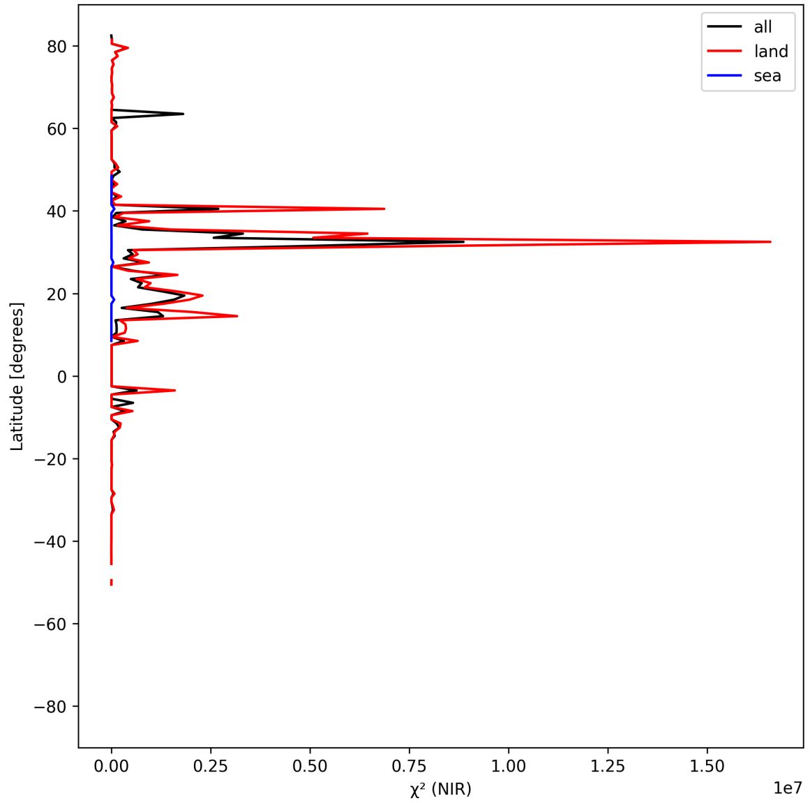
Figure 18: Zonal average of “ \chi^2 (NIR)” for 2025-07-05 to 2025-07-07.
