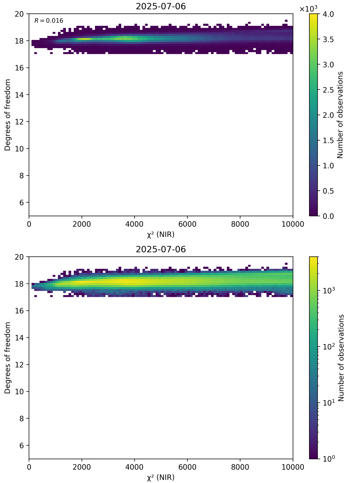
Figure 44: Scatter density plot of “ \chi^2 (NIR)” against “Degrees of freedom” for 2025-07-05 to 2025-07-07.
