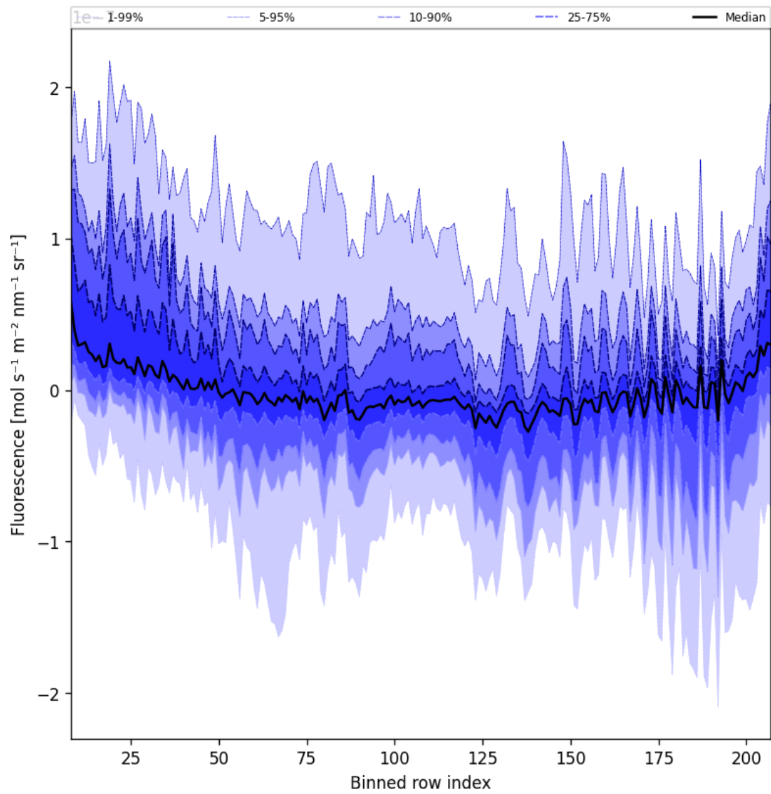
Figure 43: Along track statistics of “Fluorescence” for 2025-07-05 to 2025-07-07
