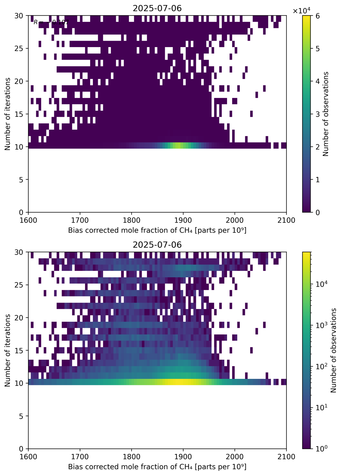
Figure 67: Scatter density plot of “Bias corrected mole fraction of CH 4 ” against “Number of iterations” for 2025-07-05 to 2025-07-07.
