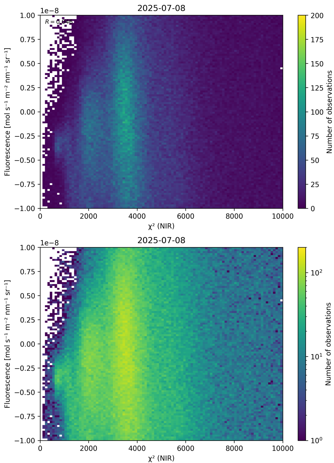
Figure 45: Scatter density plot of “ \chi^2 (NIR)” against “Fluorescence” for 2025-07-08 to 2025-07-09.
