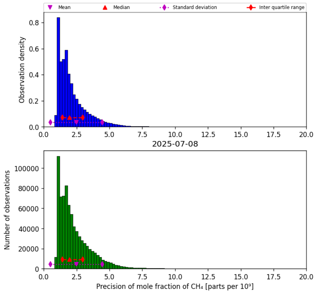
Figure 24: Histogram of “Precision of mole fraction of CH 4 ” for 2025-07-08 to 2025-07-09
