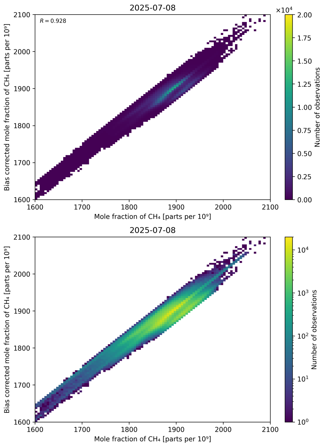
Figure 74: Scatter density plot of “Mole fraction of CH 4 ” against “Bias corrected mole fraction of CH 4 ” for 2025-07-08 to 2025-07-09.
