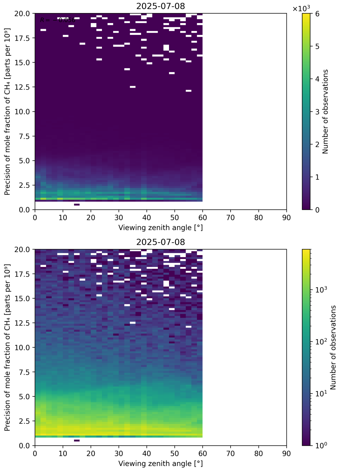
Figure 112: Scatter density plot of “Viewing zenith angle” against “Precision of mole fraction of CH 4 ” for 2025-07-08 to 2025-07-09.
