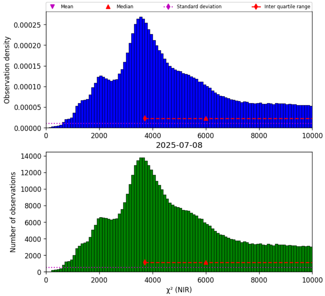
Figure 29: Histogram of " \chi^2 (NIR)" for 2025-07-08 to 2025-07-09
