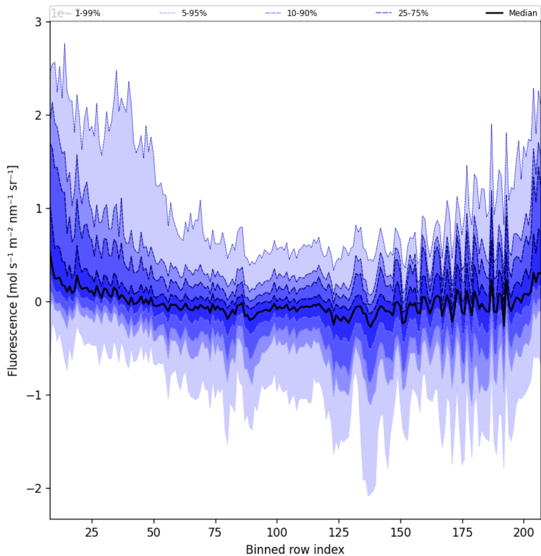
Figure 43: Along track statistics of “Fluorescence” for 2025-07-08 to 2025-07-09
