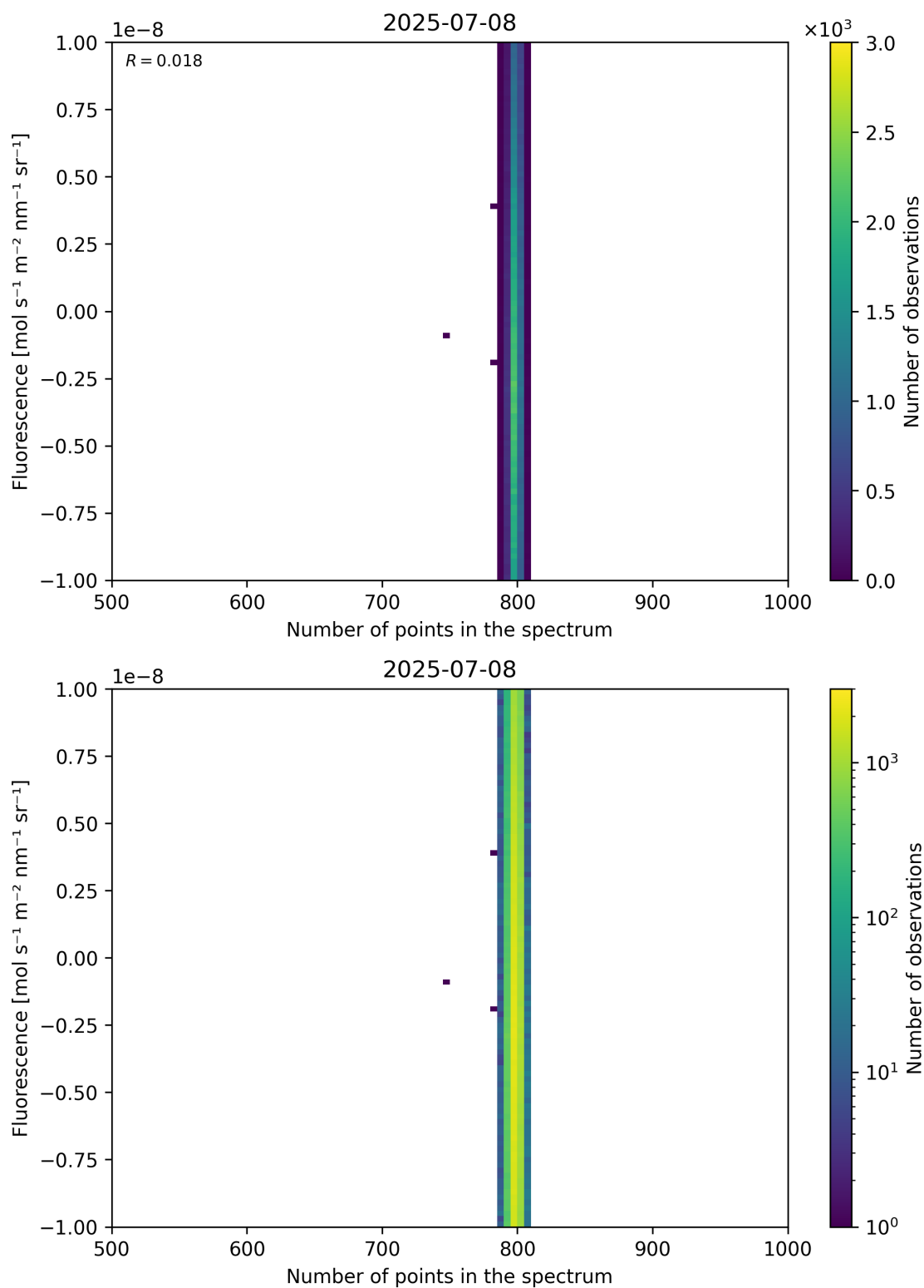
Figure 91: Scatter density plot of “Number of points in the spectrum” against “Fluorescence” for 2025-07-08 to 2025-07-09.
