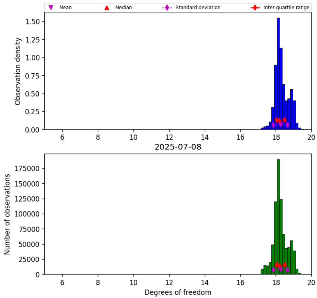
Figure 30: Histogram of “Degrees of freedom” for 2025-07-08 to 2025-07-09
