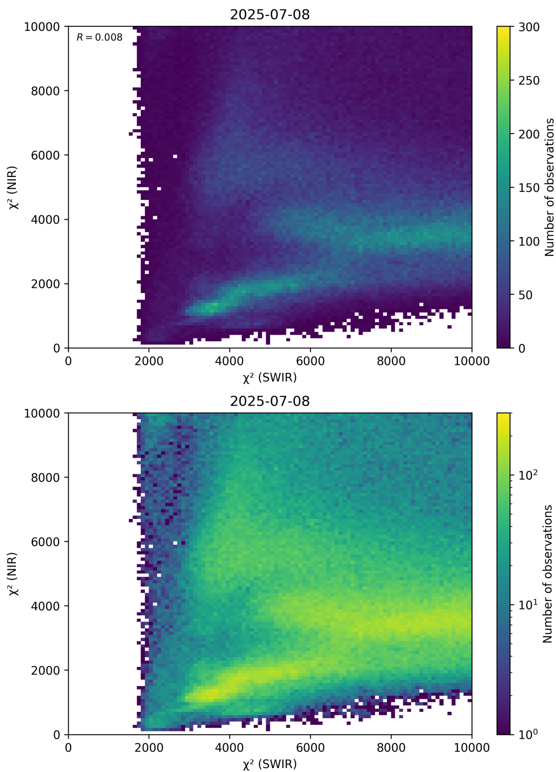
Figure 47: Scatter density plot of “ \chi^2 (SWIR)” against “ \chi^2 (NIR)” for 2025-07-08 to 2025-07-09.
