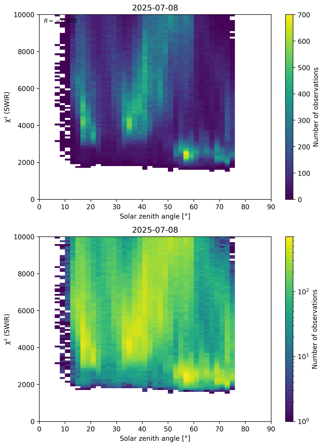
Figure 95: Scatter density plot of “Solar zenith angle” against “ \chi^2 (SWIR)” for 2025-07-08 to 2025-07-09.
