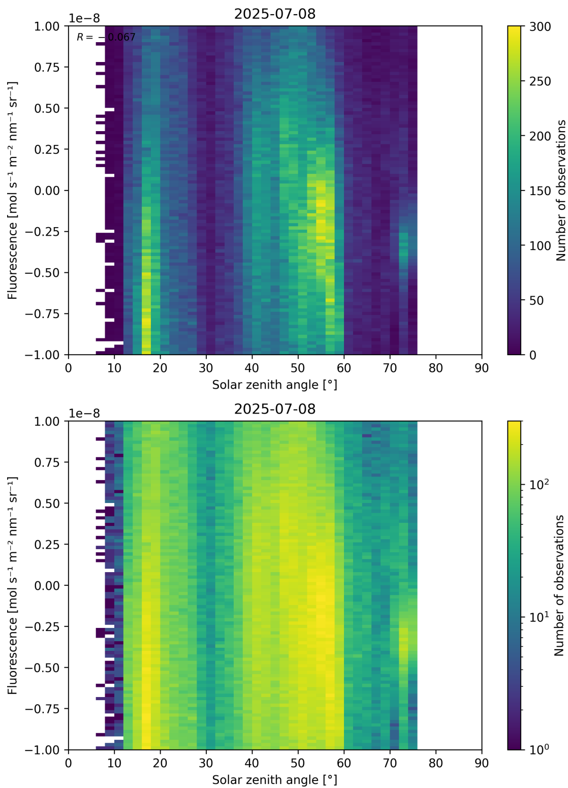
Figure 97: Scatter density plot of “Solar zenith angle” against “Fluorescence” for 2025-07-08 to 2025-07-09.
