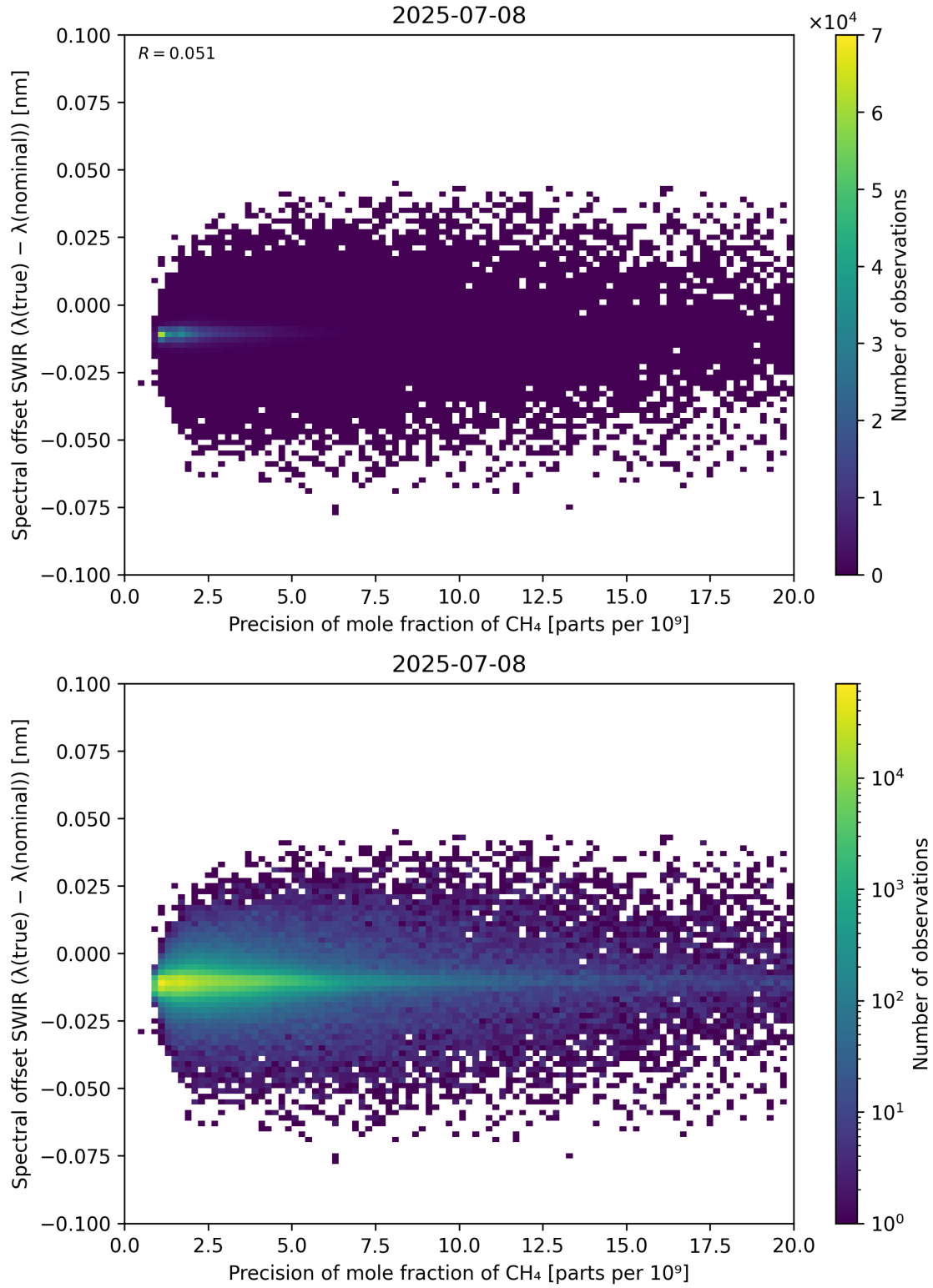
Figure 85: Scatter density plot of “Precision of mole fraction of CH 4 ” against “Spectral offset SWIR ( \lambda_{\text{true}} - \lambda_{\text{nominal}} )” for 2025-07-08 to 2025-07-09.
