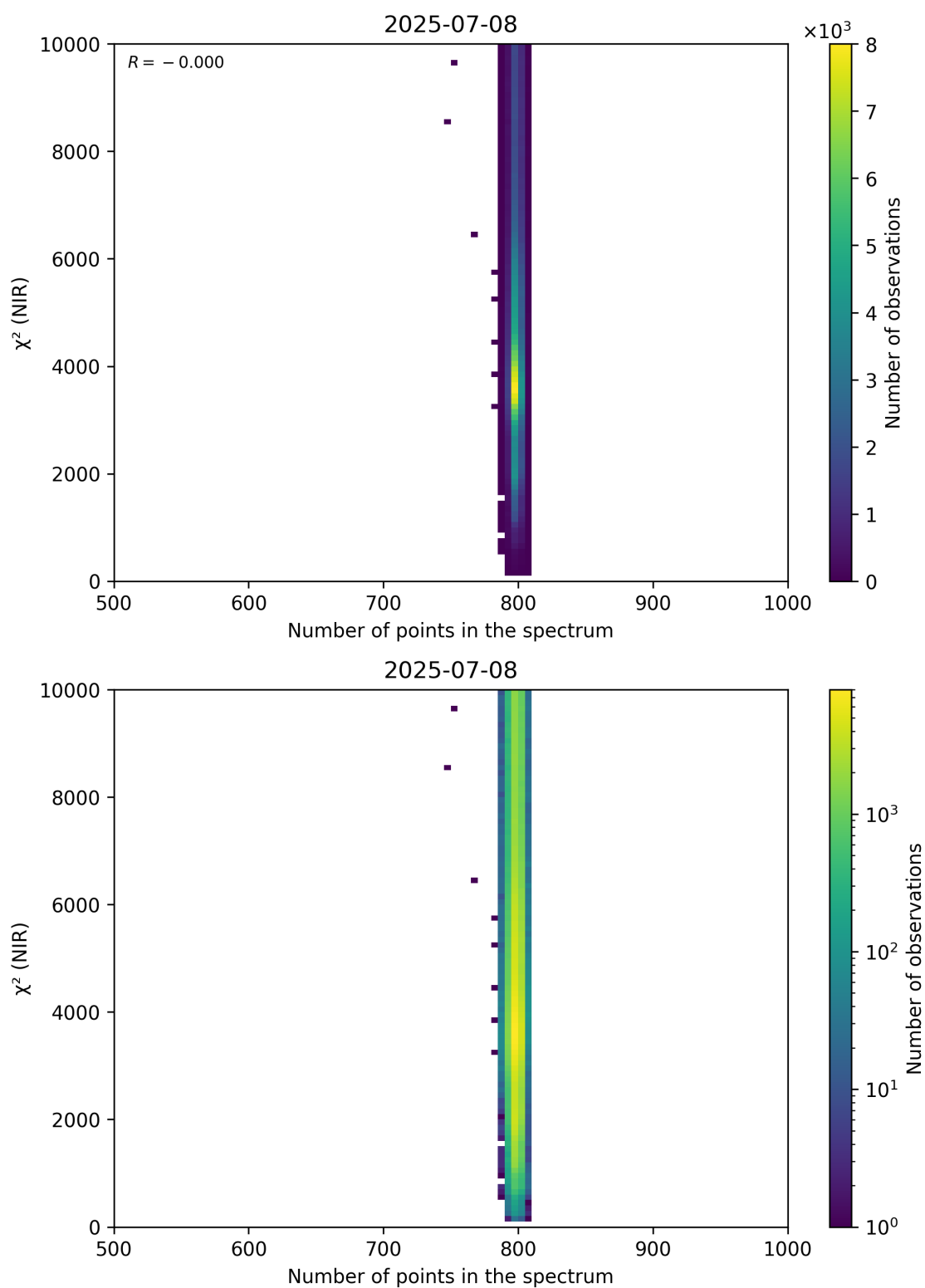
Figure 88: Scatter density plot of “Number of points in the spectrum” against “ \chi^2 (NIR)” for 2025-07-08 to 2025-07-09.
