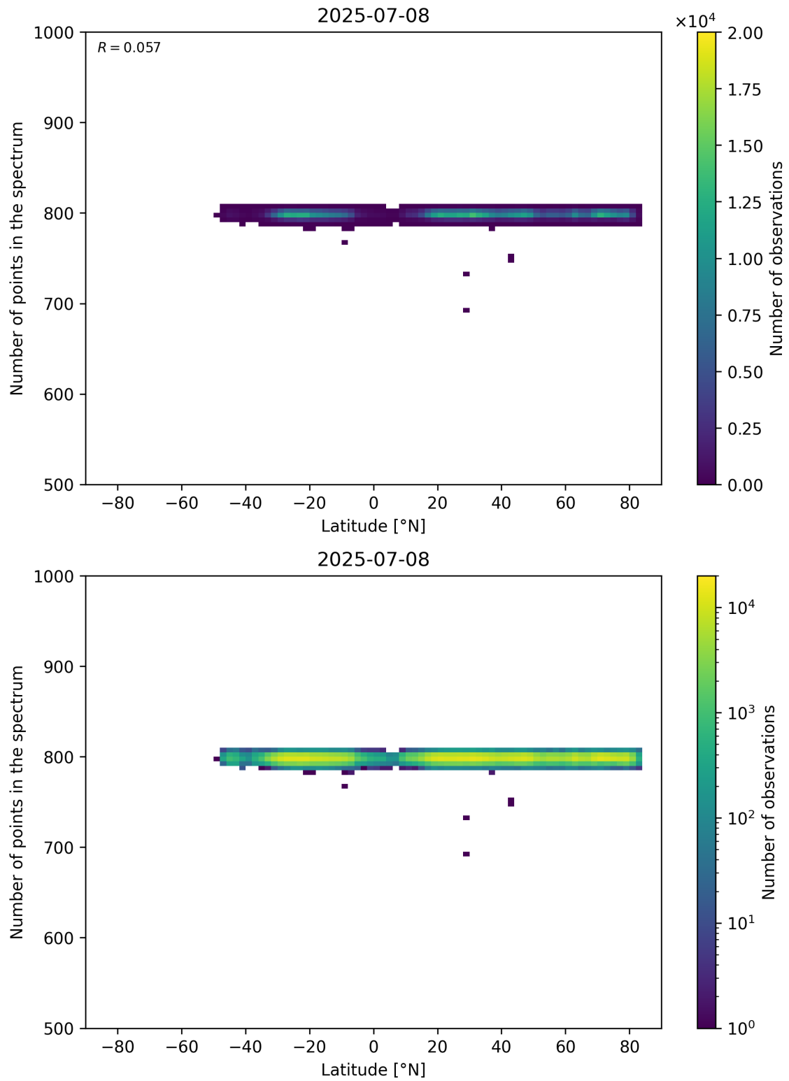
Figure 61: Scatter density plot of “Latitude” against “Number of points in the spectrum” for 2025-07-08 to 2025-07-09.
