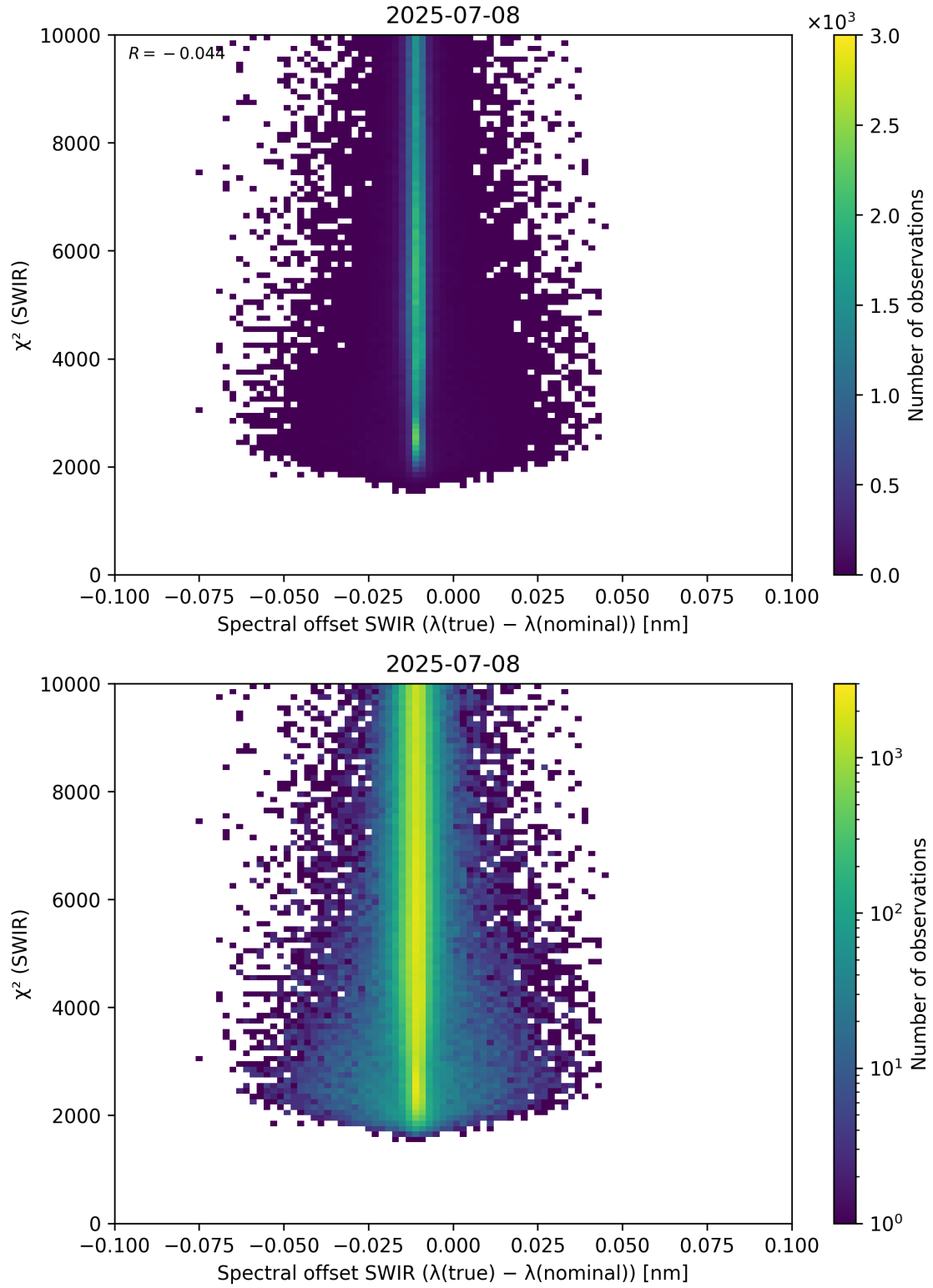
Figure 118: Scatter density plot of “Spectral offset SWIR ( \lambda_{\text{true}} - \lambda_{\text{nominal}} )” against “ \chi^2 (SWIR)” for 2025-07-08 to 2025-07-09.
