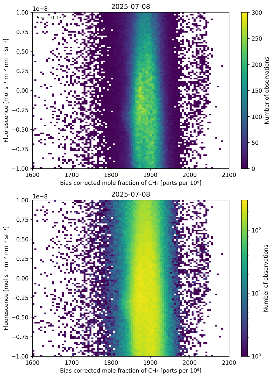
Figure 66: Scatter density plot of “Bias corrected mole fraction of \text{CH}_4 ” against “Fluorescence” for 2025-07-08 to 2025-07-09.
