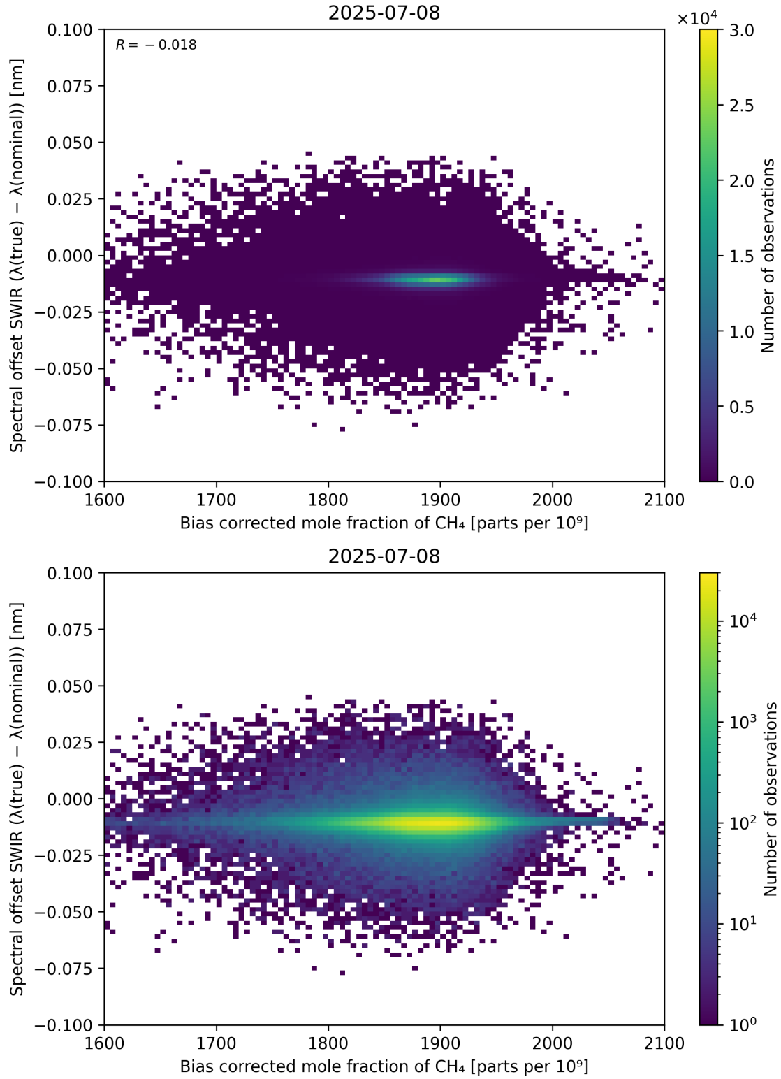
Figure 69: Scatter density plot of “Bias corrected mole fraction of CH 4 ” against “Spectral offset SWIR ( \lambda_{\text{true}} - \lambda_{\text{nominal}} )” for 2025-07-08 to 2025-07-09.
