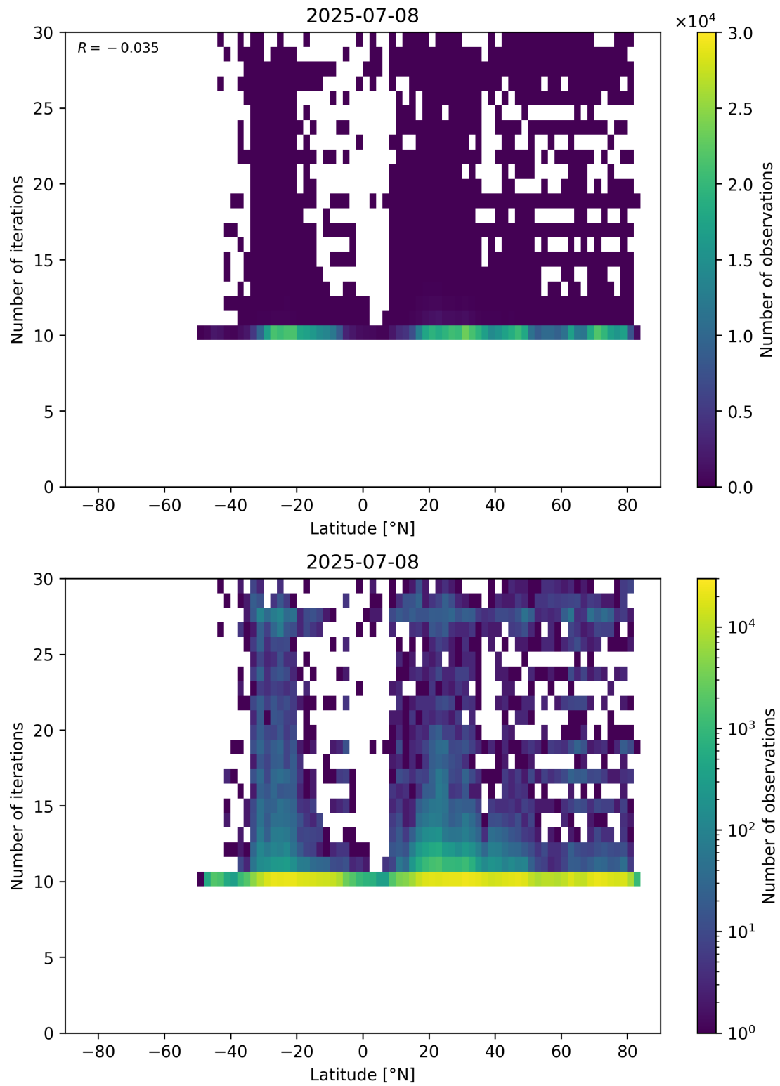
Figure 60: Scatter density plot of “Latitude” against “Number of iterations” for 2025-07-08 to 2025-07-09.
