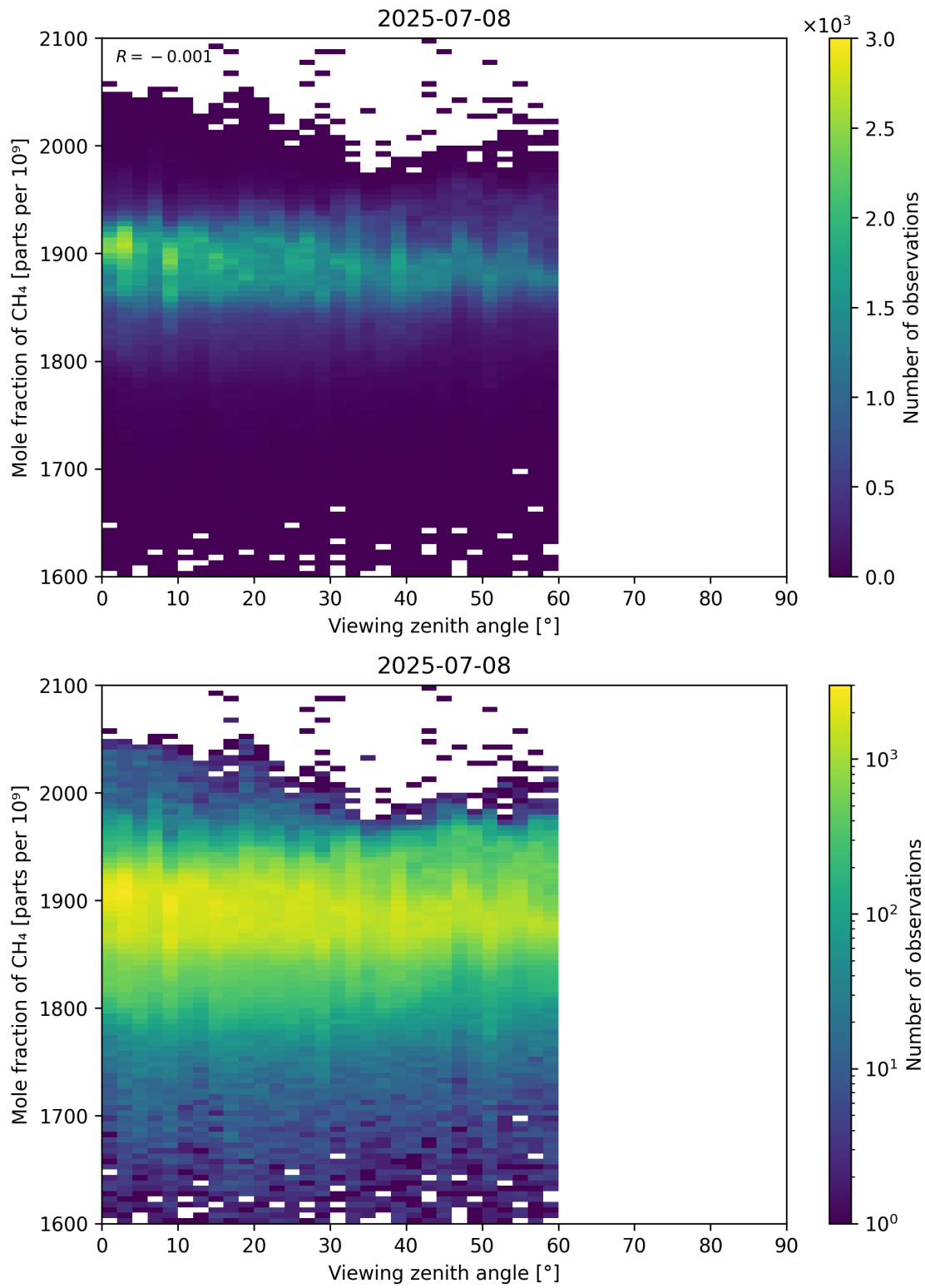
Figure 110: Scatter density plot of “Viewing zenith angle” against “Mole fraction of CH 4 ” for 2025-07-08 to 2025-07-09.
