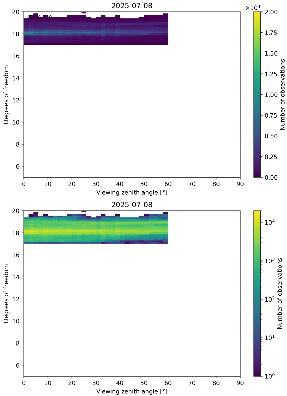
Figure 107: Scatter density plot of “Viewing zenith angle” against “Degrees of freedom” for 2025-07-08 to 2025-07-09.
