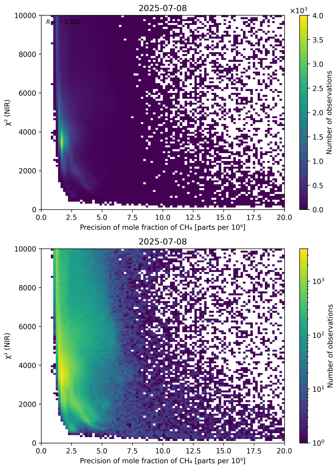
Figure 78: Scatter density plot of “Precision of mole fraction of \text{CH}_4 ” against “ \chi^2 (NIR)” for 2025-07-08 to 2025-07-09.
