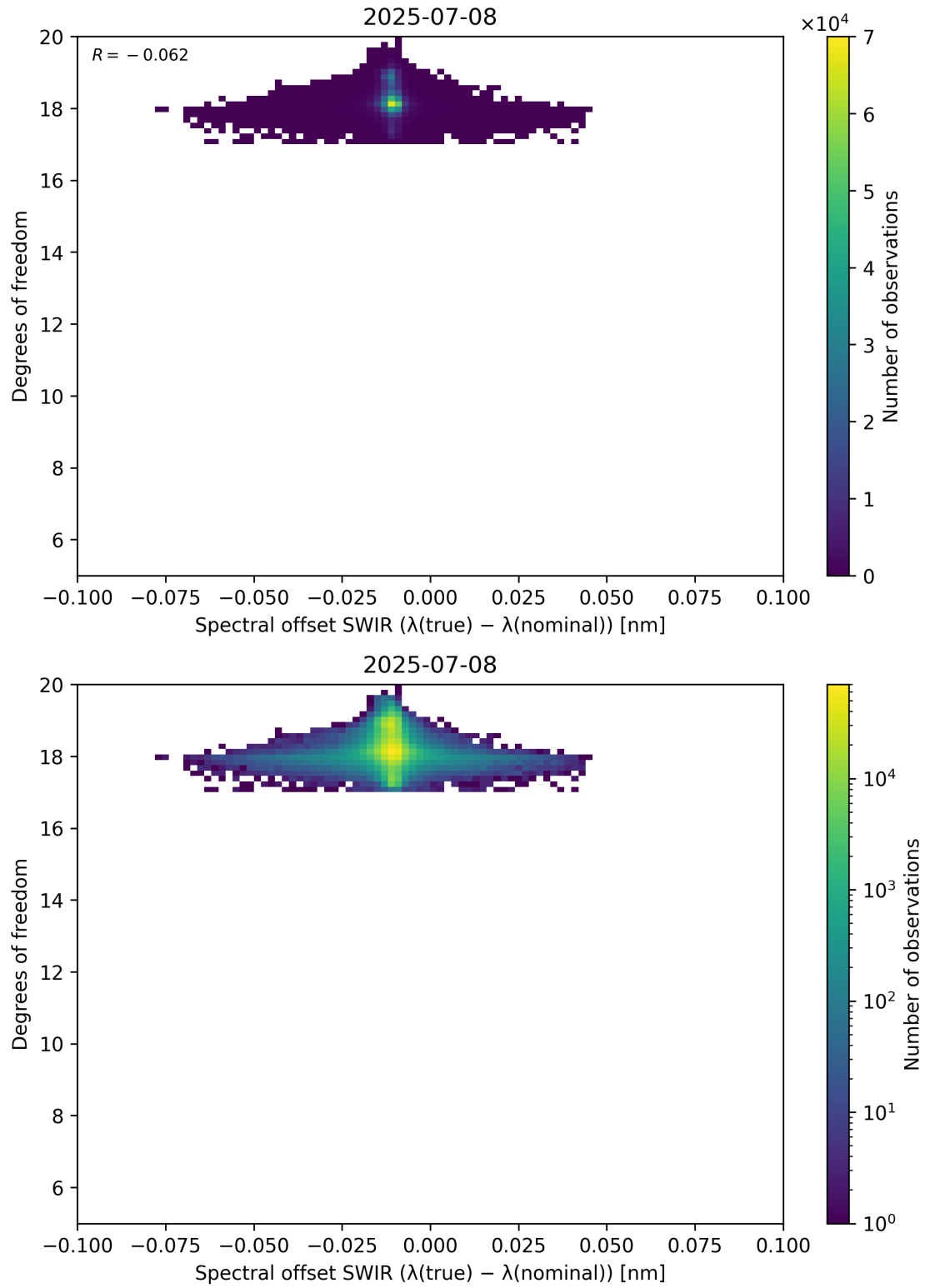
Figure 119: Scatter density plot of “Spectral offset SWIR ( \lambda_{\text{true}} - \lambda_{\text{nominal}} )” against “Degrees of freedom” for 2025-07-08 to 2025-07-09.
