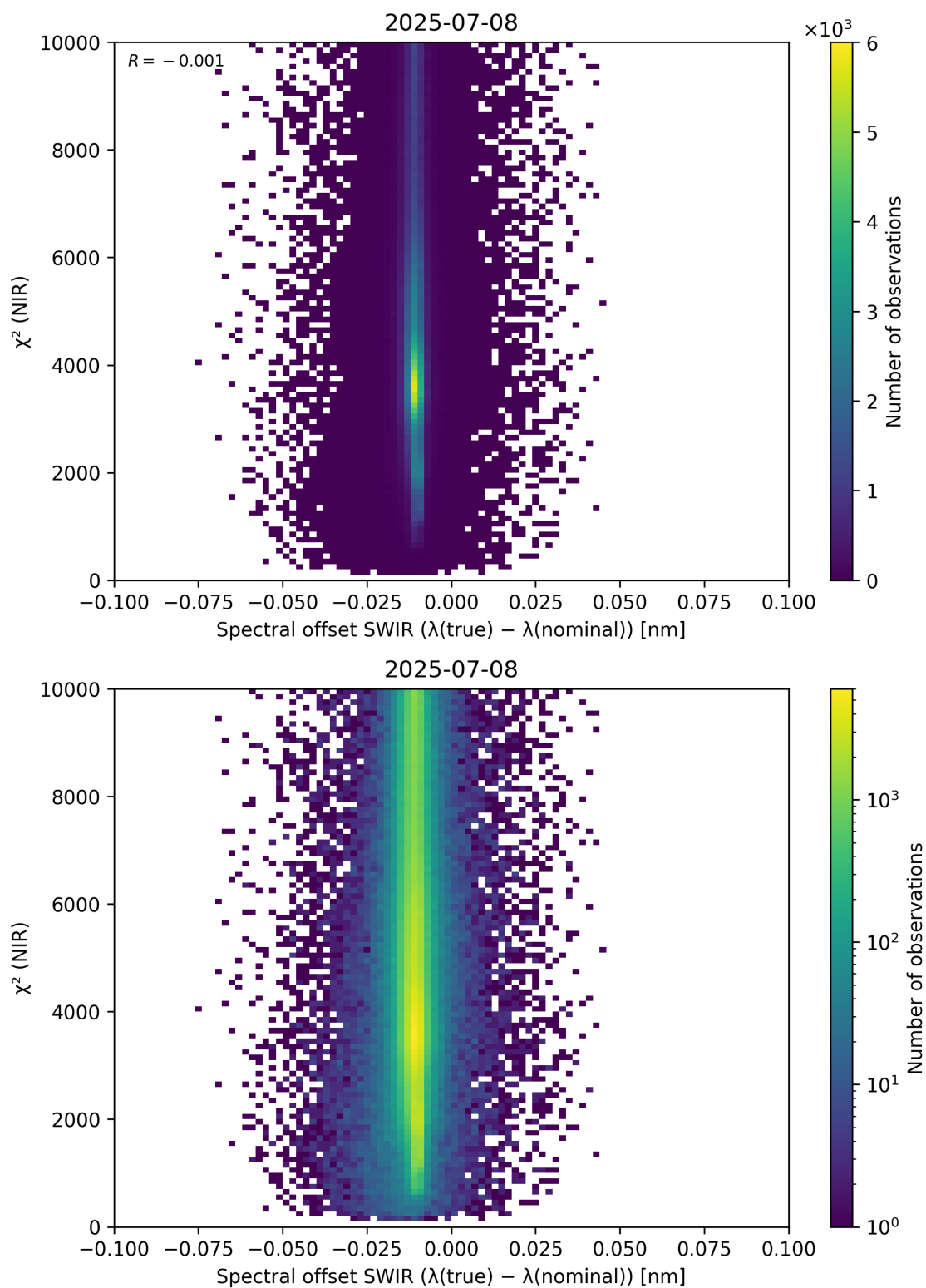
Figure 117: Scatter density plot of “Spectral offset SWIR ( \lambda_{\text{true}} - \lambda_{\text{nominal}} )” against “ \chi^2 (NIR)” for 2025-07-08 to 2025-07-09.
