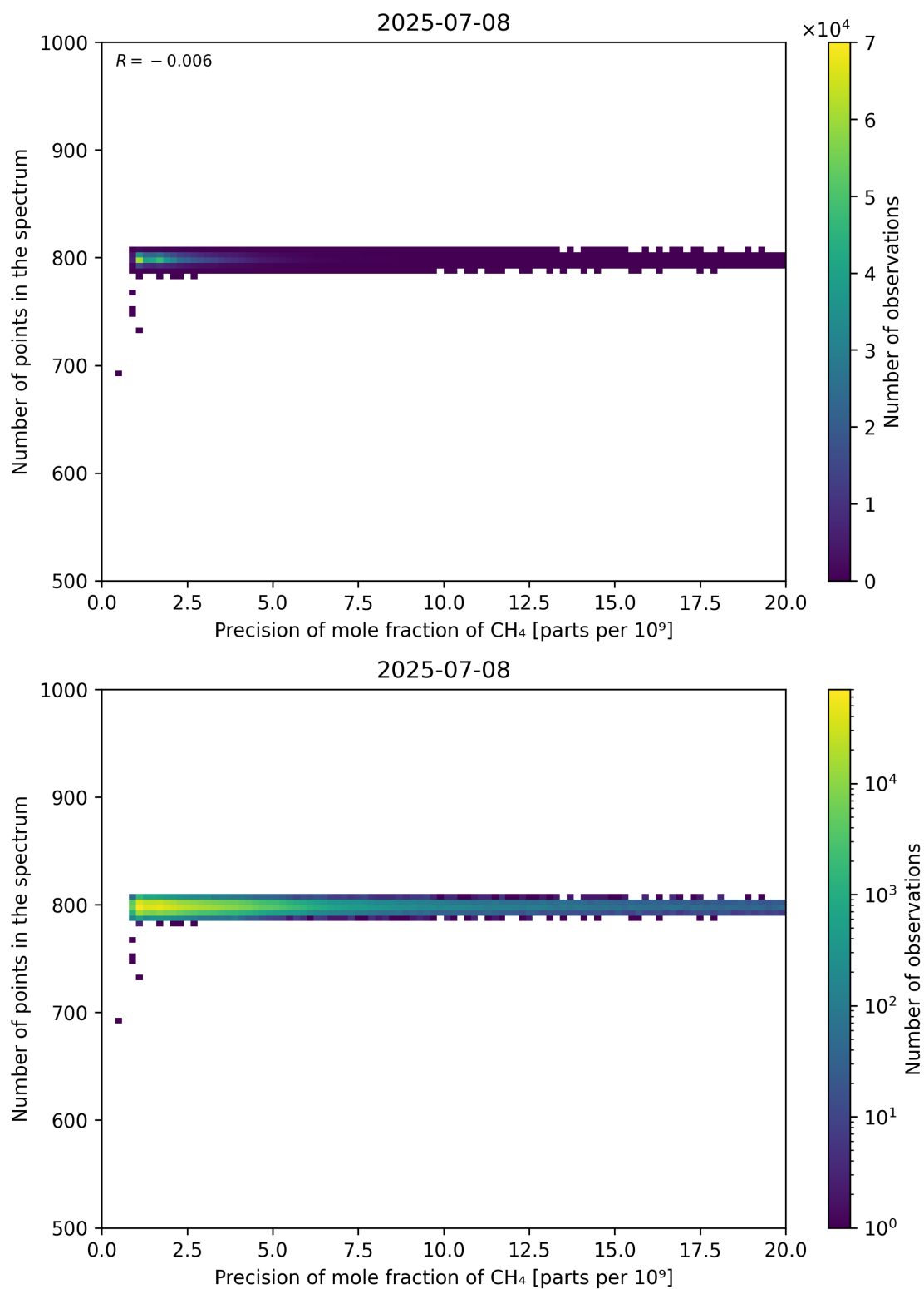
Figure 84: Scatter density plot of “Precision of mole fraction of CH 4 ” against “Number of points in the spectrum” for 2025-07-08 to 2025-07-09.
