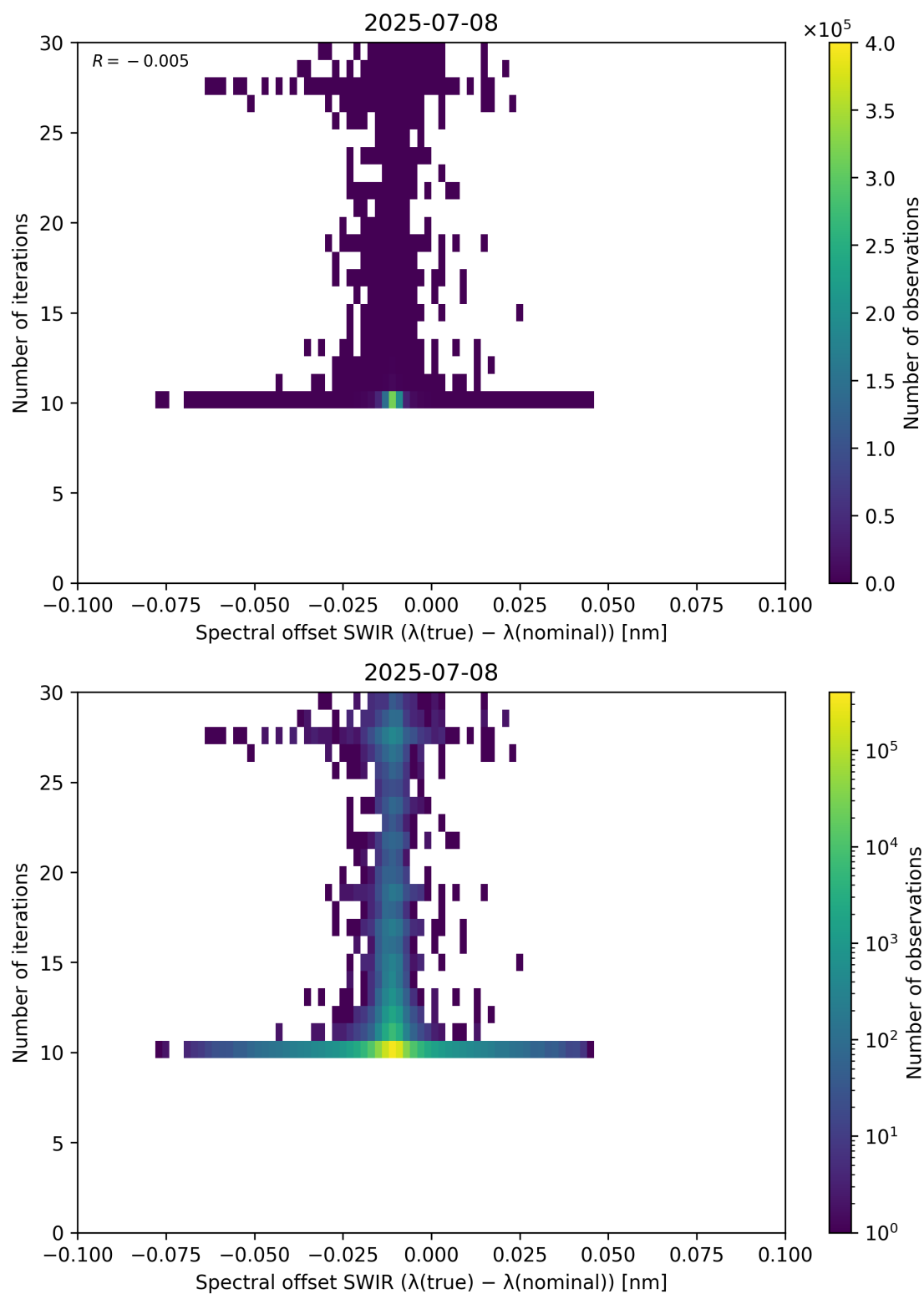
Figure 121: Scatter density plot of “Spectral offset SWIR ( \lambda_{\text{true}} - \lambda_{\text{nominal}} )” against “Number of iterations” for 2025-07-08 to 2025-07-09.
