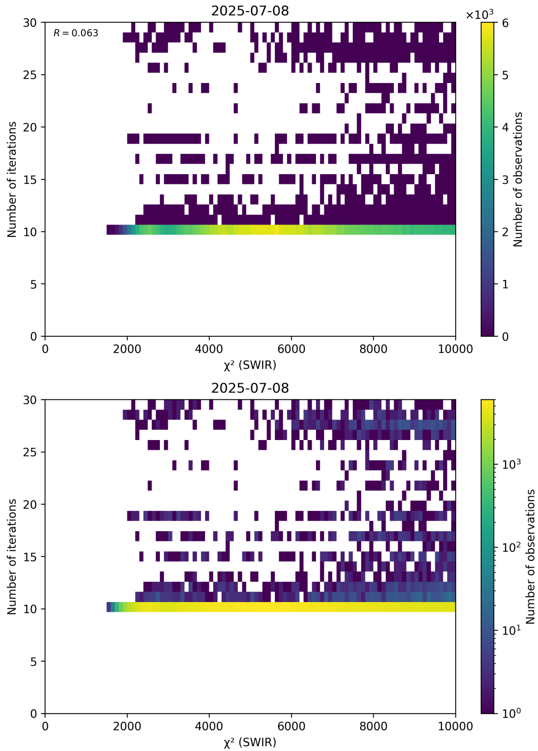
Figure 50: Scatter density plot of “ \chi^2 (SWIR)” against “Number of iterations” for 2025-07-08 to 2025-07-09.
