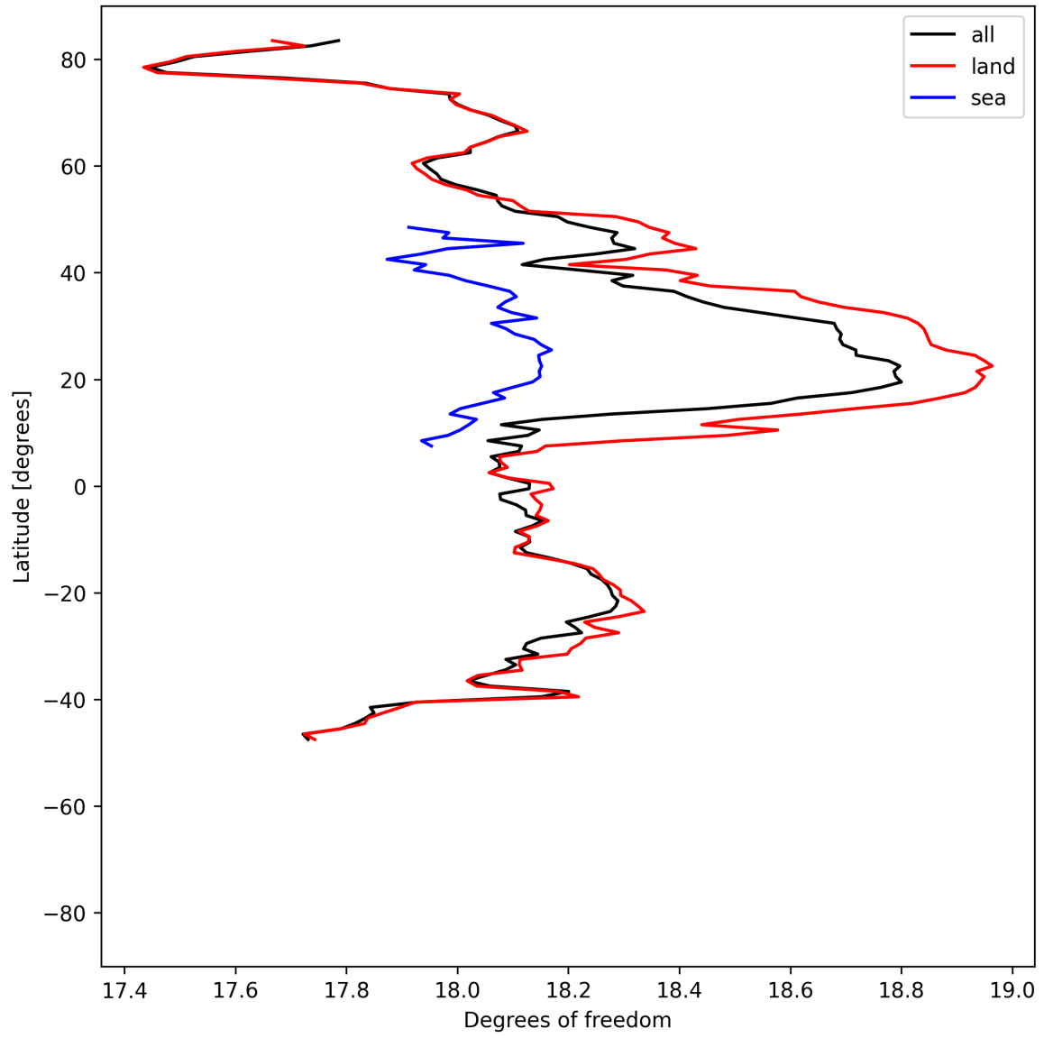
Figure 19: Zonal average of “Degrees of freedom” for 2025-07-08 to 2025-07-09.
