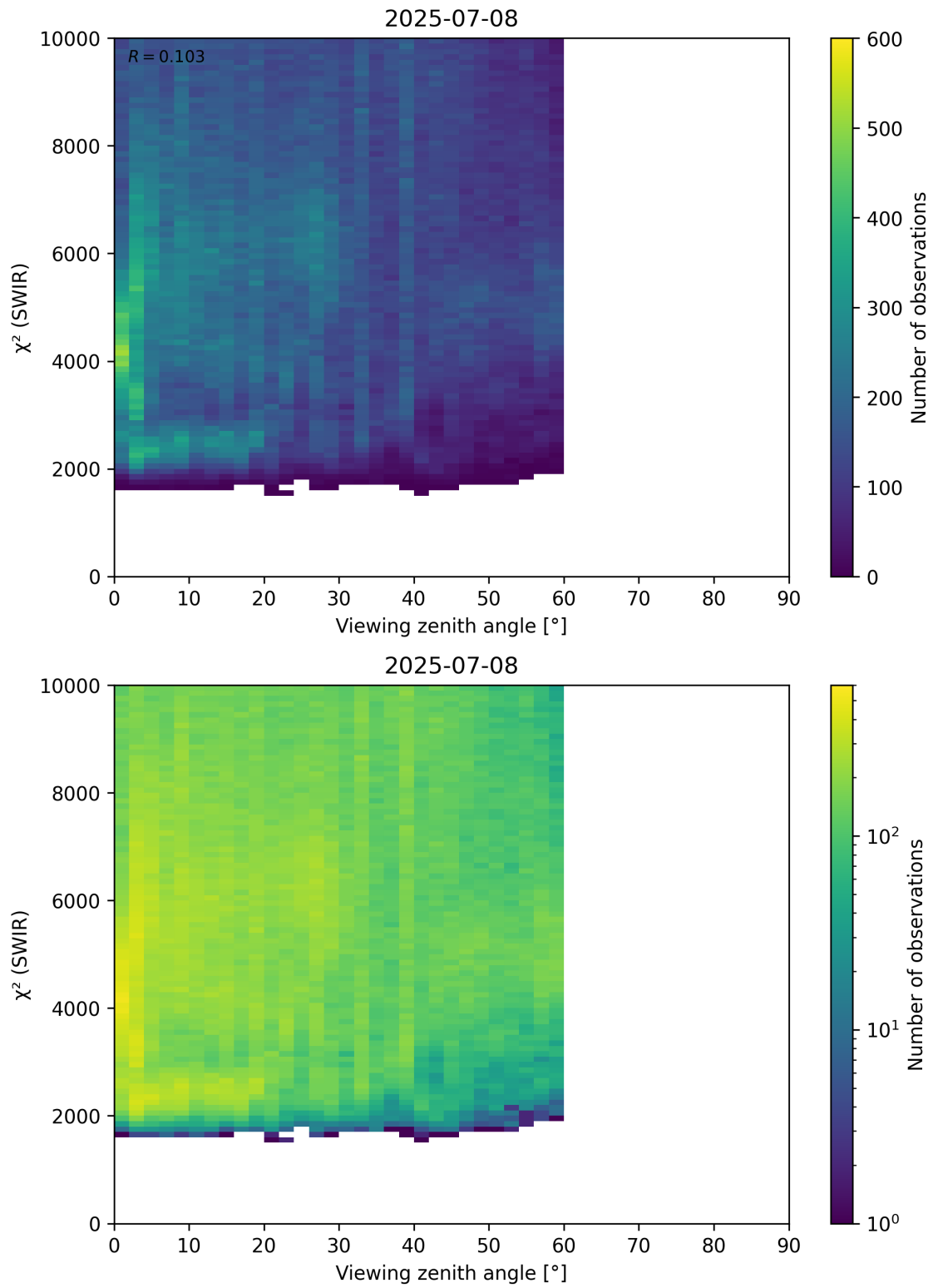
Figure 106: Scatter density plot of “Viewing zenith angle” against “ \chi^2 (SWIR)” for 2025-07-08 to 2025-07-09.
