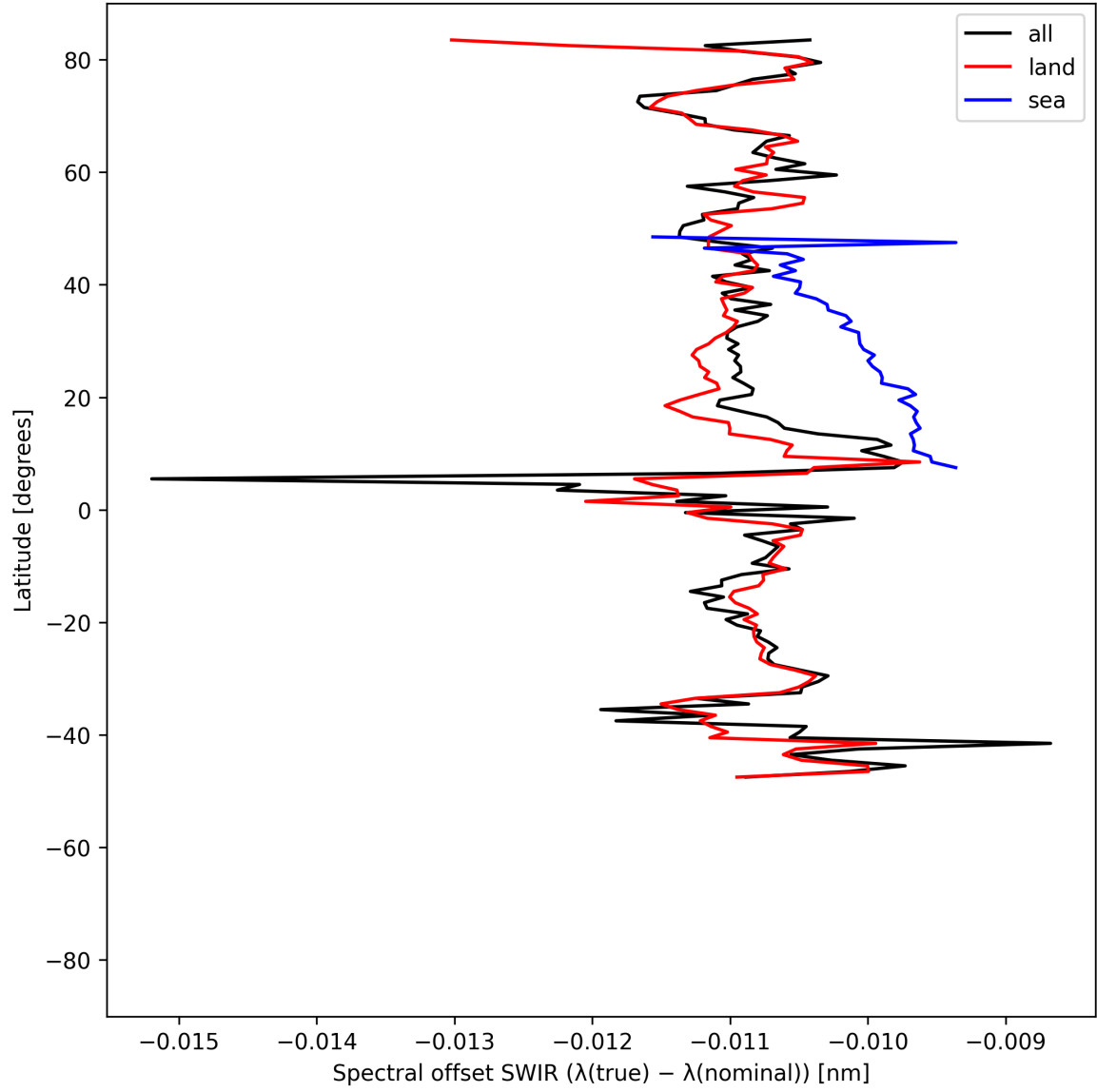
Figure 16: Zonal average of “Spectral offset SWIR ( \lambda_{\text{true}} - \lambda_{\text{nominal}} )” for 2025-07-08 to 2025-07-09.
