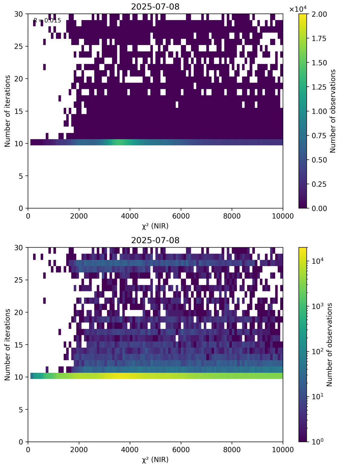
Figure 46: Scatter density plot of " \chi^2 (NIR)" against "Number of iterations" for 2025-07-08 to 2025-07-09.
