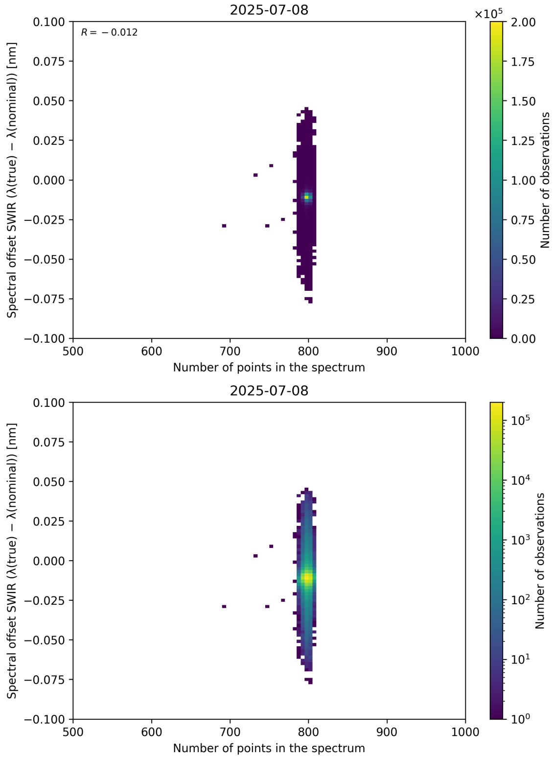
Figure 93: Scatter density plot of “Number of points in the spectrum” against “Spectral offset SWIR ( \lambda_{\text{true}} - \lambda_{\text{nominal}} )” for 2025-07-08 to 2025-07-09.
