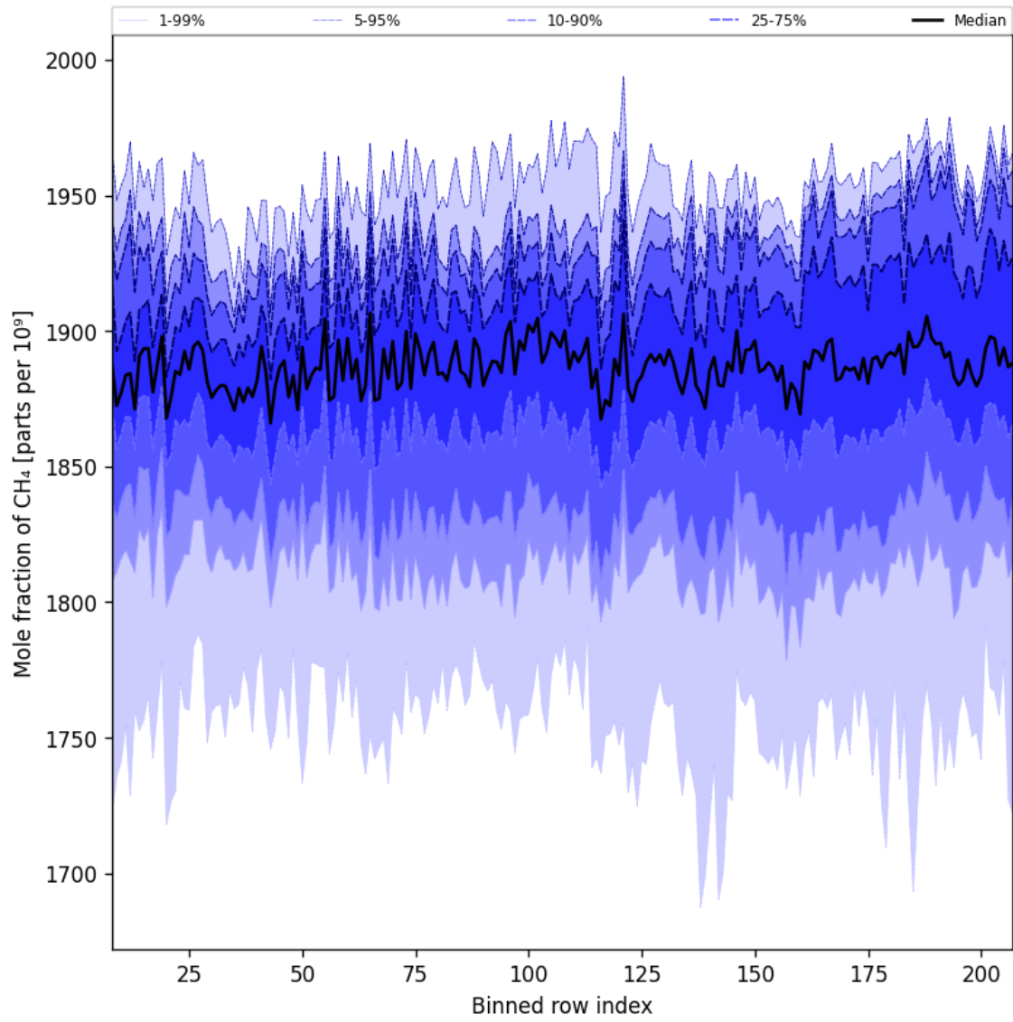
Figure 34: Along track statistics of “Mole fraction of CH 4 ” for 2025-07-08 to 2025-07-09
