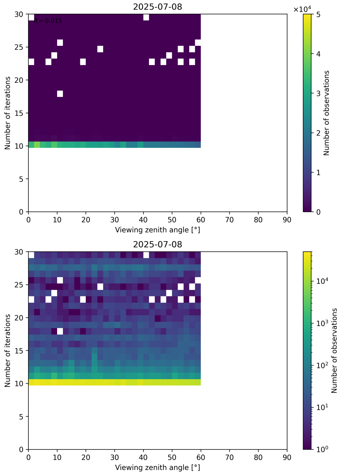
Figure 113: Scatter density plot of “Viewing zenith angle” against “Number of iterations” for 2025-07-08 to 2025-07-09.
