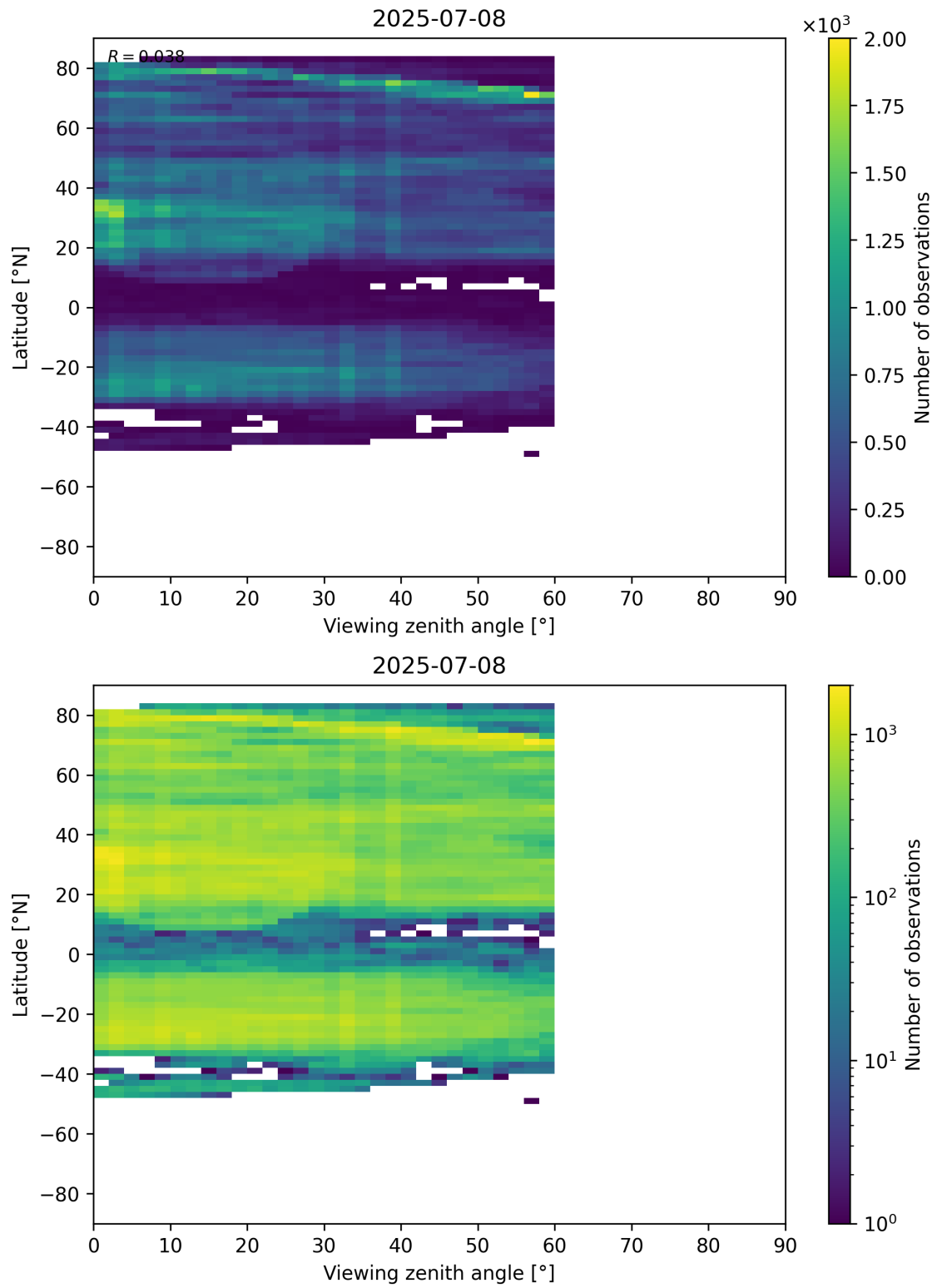
Figure 109: Scatter density plot of “Viewing zenith angle” against “Latitude” for 2025-07-08 to 2025-07-09.
