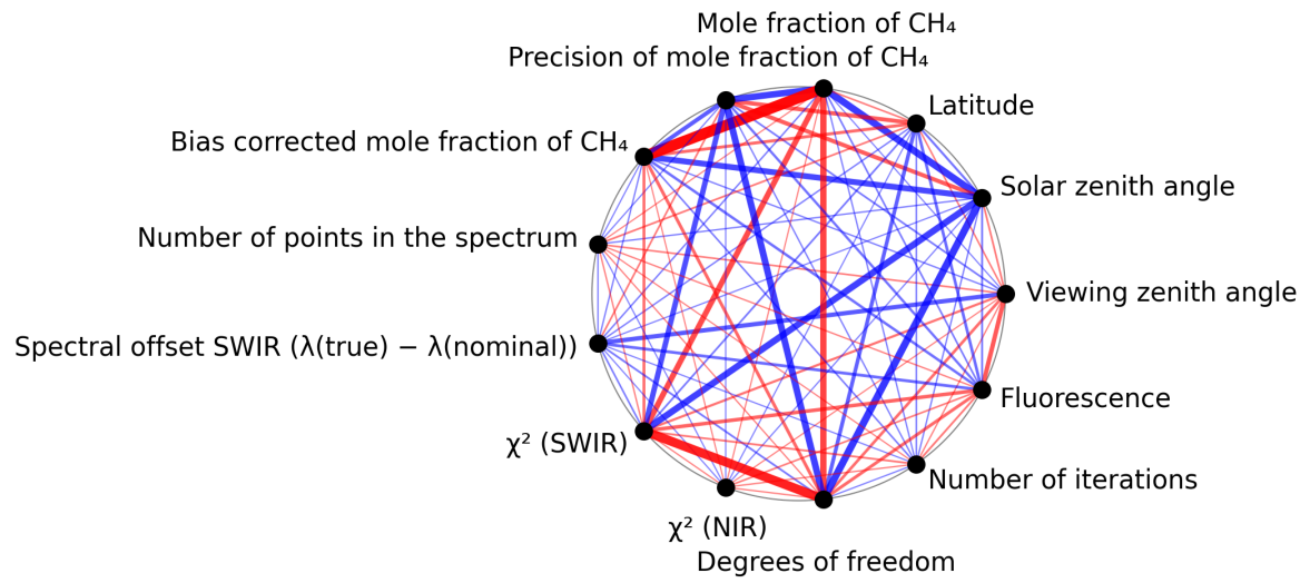
Figure 1: Map of correlation graph for 2025-07-08 to 2025-07-09.
