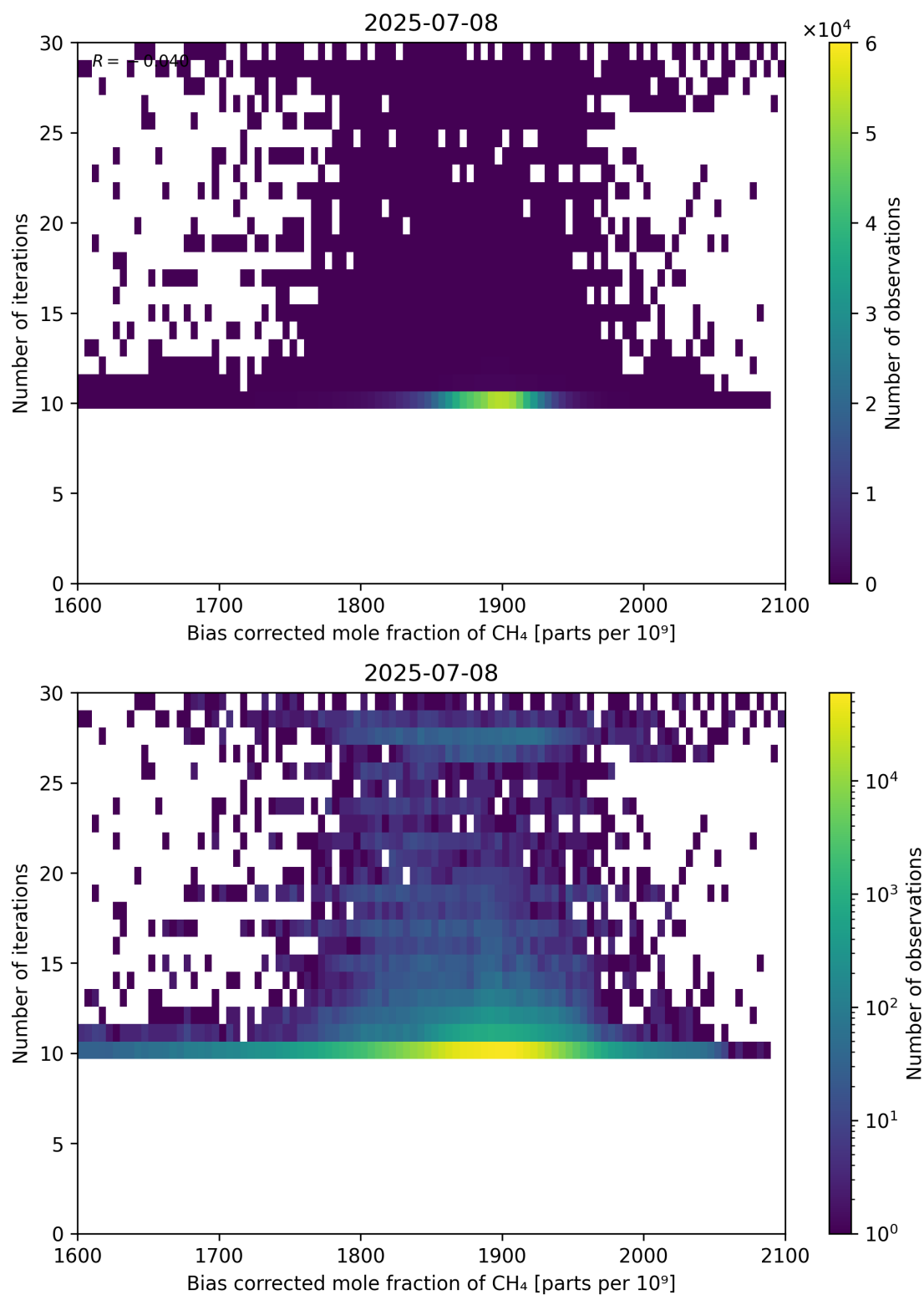
Figure 67: Scatter density plot of “Bias corrected mole fraction of CH 4 ” against “Number of iterations” for 2025-07-08 to 2025-07-09.
