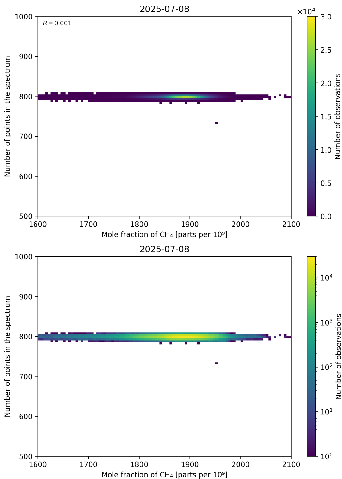
Figure 77: Scatter density plot of “Mole fraction of CH 4 ” against “Number of points in the spectrum” for 2025-07-08 to 2025-07-09.
