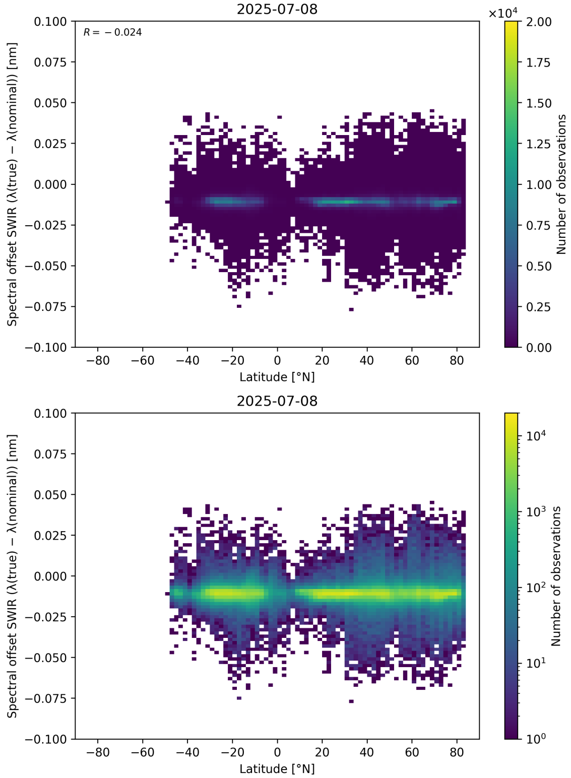
Figure 62: Scatter density plot of “Latitude” against “Spectral offset SWIR ( \lambda_{\text{true}} - \lambda_{\text{nominal}} )” for 2025-07-08 to 2025-07-09.
