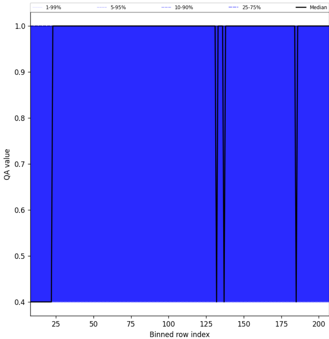
Figure 33: Along track statistics of “QA value” for 2025-07-08 to 2025-07-09
