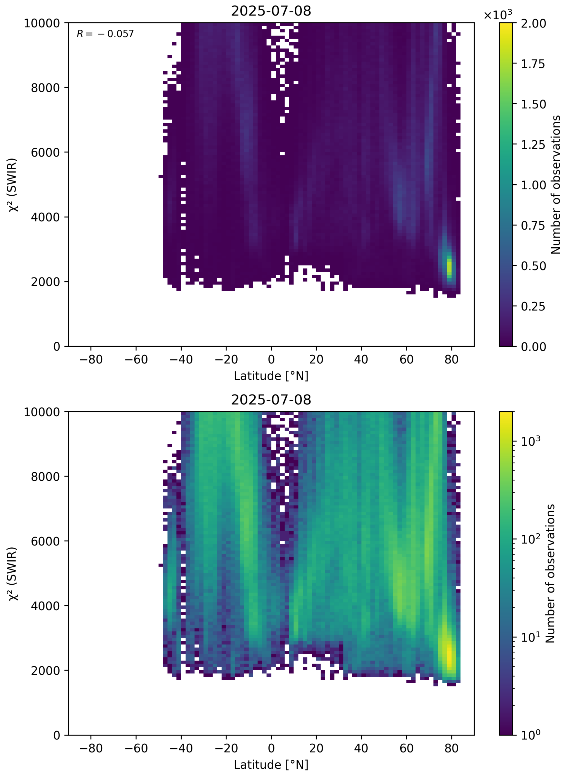
Figure 54: Scatter density plot of “Latitude” against “ \chi^2 (SWIR)” for 2025-07-08 to 2025-07-09.
