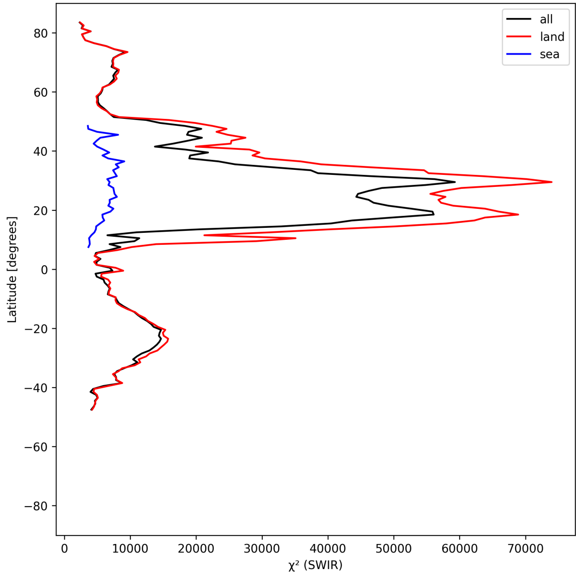
Figure 17: Zonal average of “ \chi^2 (SWIR)” for 2025-07-08 to 2025-07-09.
