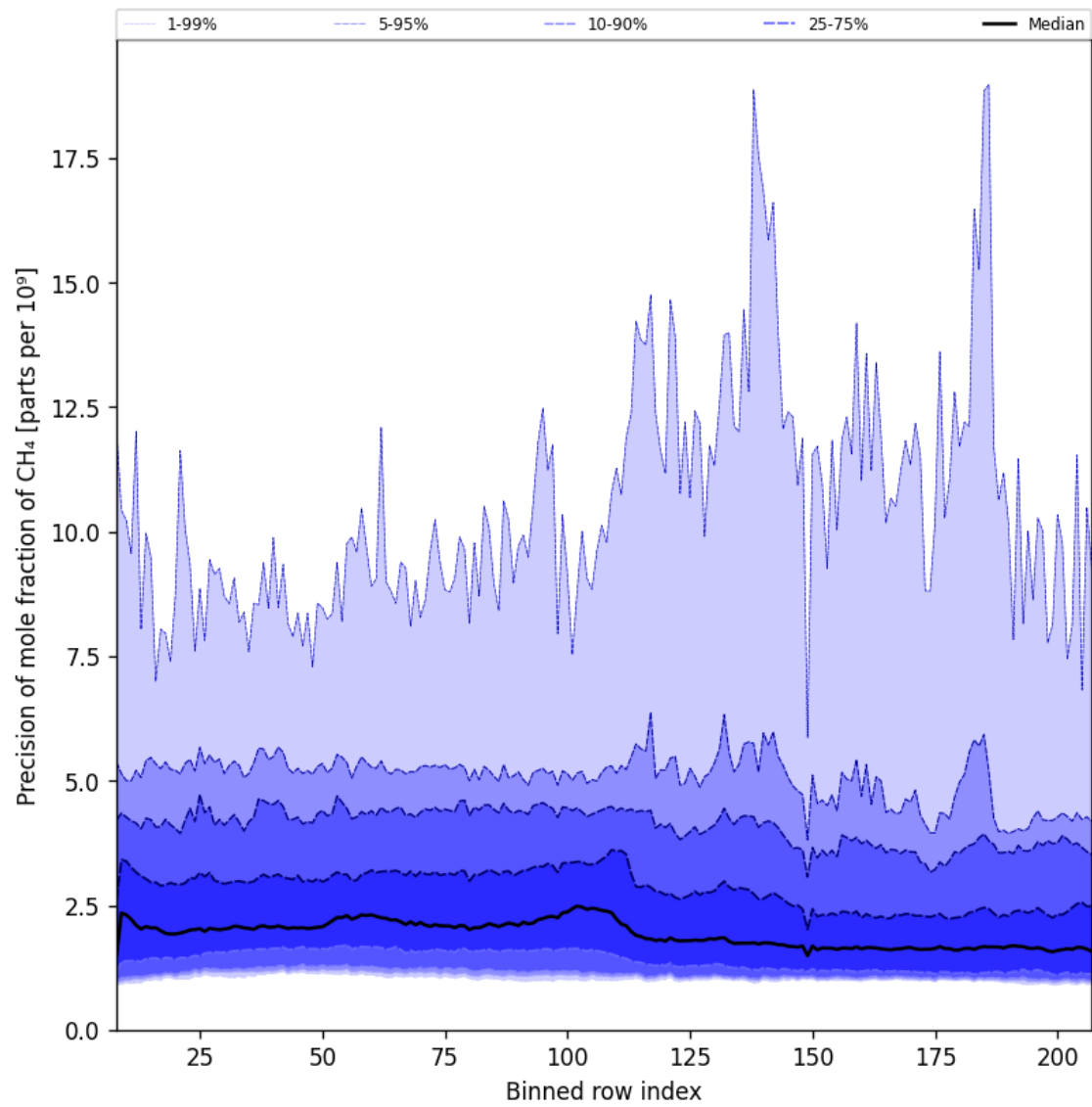
Figure 35: Along track statistics of “Precision of mole fraction of CH 4 ” for 2025-07-08 to 2025-07-09
