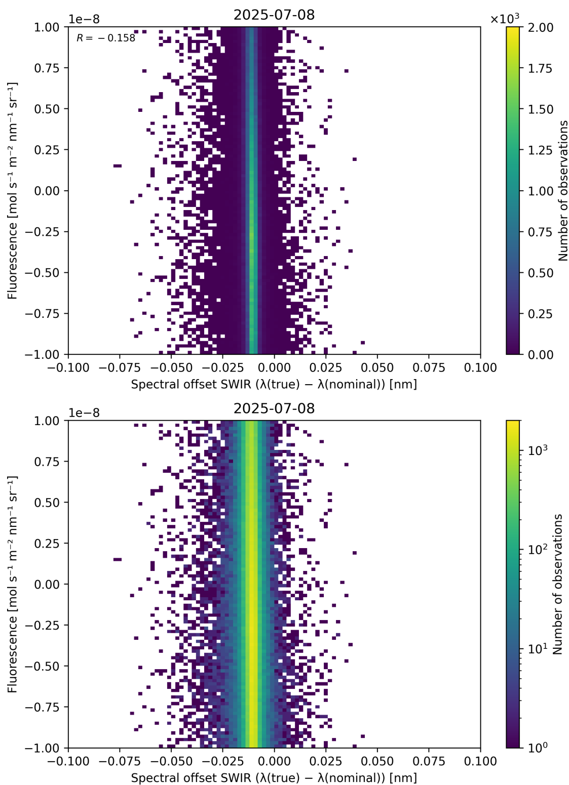
Figure 120: Scatter density plot of “Spectral offset SWIR ( \lambda_{\text{true}} - \lambda_{\text{nominal}} )” against “Fluorescence” for 2025-07-08 to 2025-07-09.
