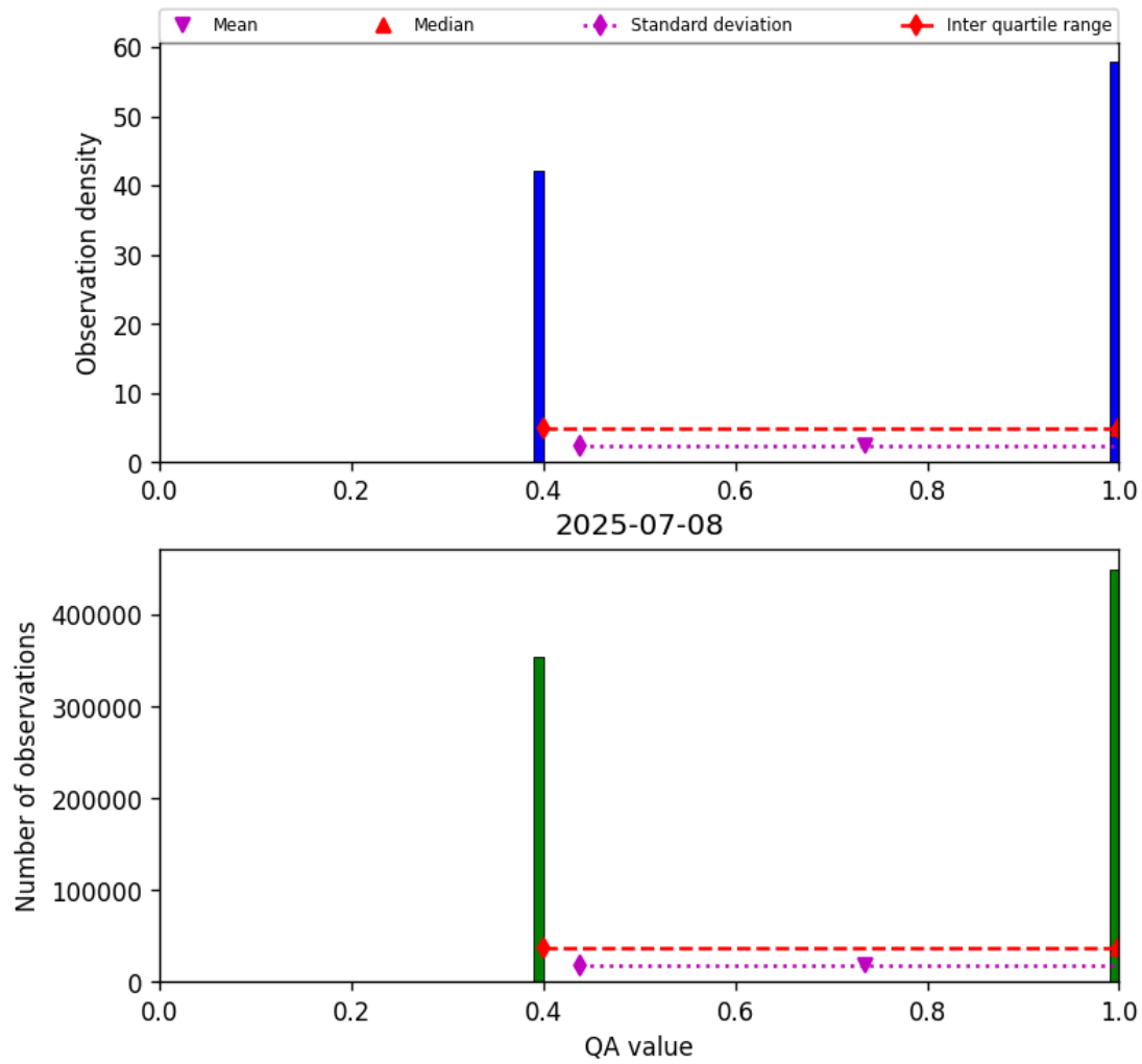
Figure 22: Histogram of “QA value” for 2025-07-08 to 2025-07-09
