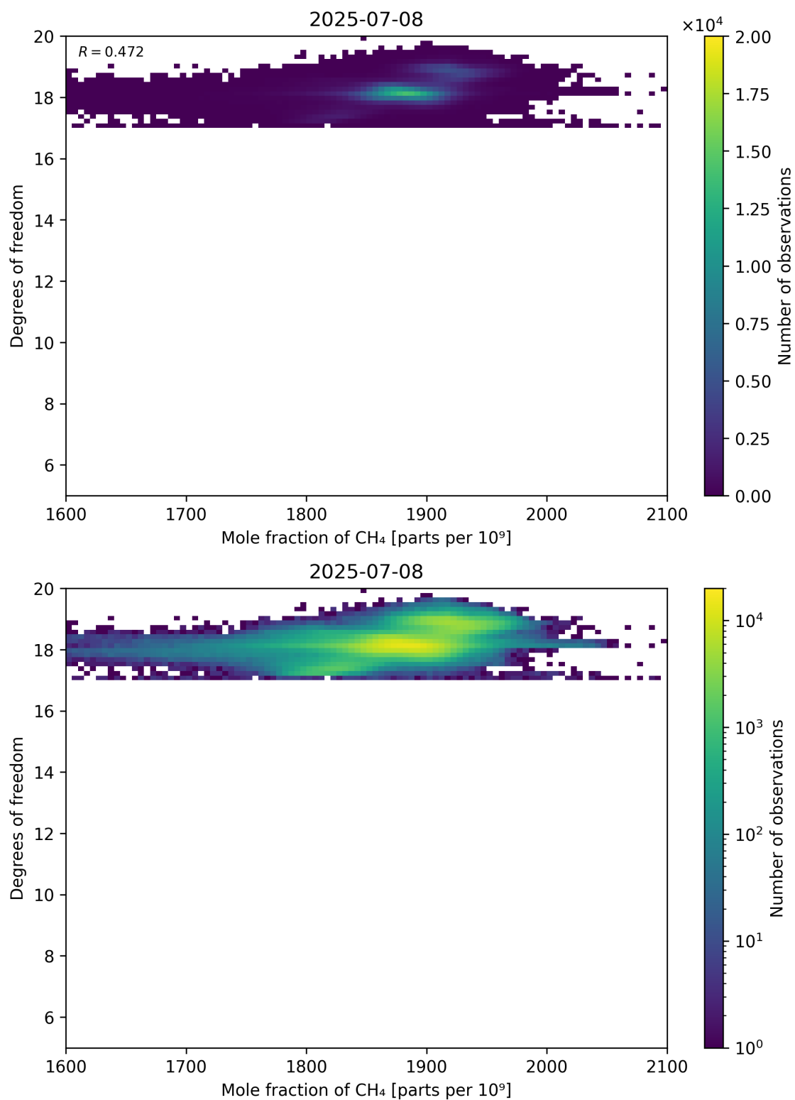
Figure 72: Scatter density plot of “Mole fraction of CH 4 ” against “Degrees of freedom” for 2025-07-08 to 2025-07-09.
