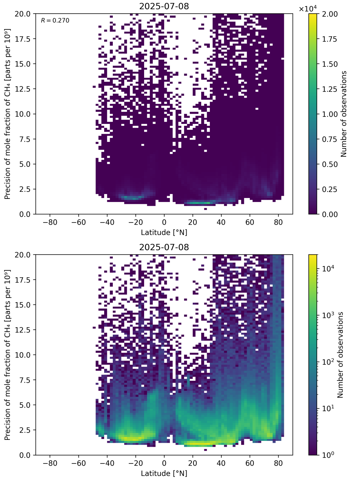
Figure 59: Scatter density plot of “Latitude” against “Precision of mole fraction of \text{CH}_4 ” for 2025-07-08 to 2025-07-09.
