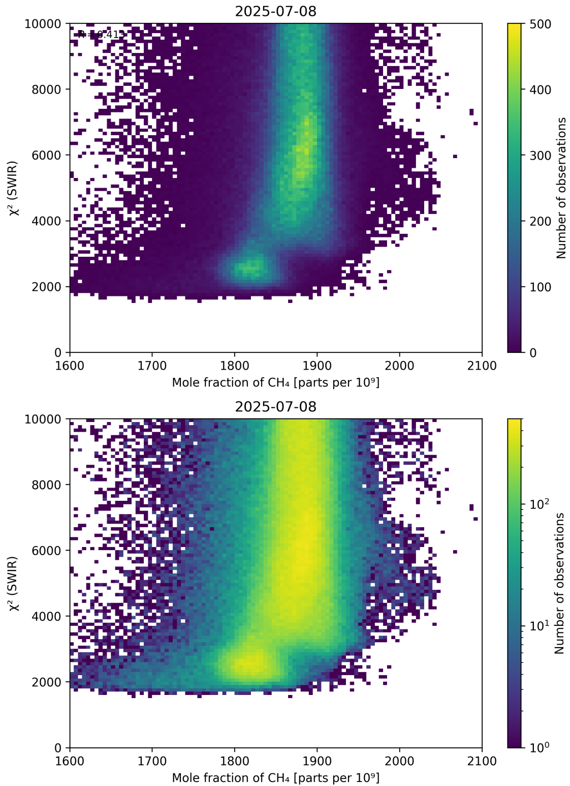
Figure 71: Scatter density plot of “Mole fraction of CH 4 ” against “ \chi^2 (SWIR)” for 2025-07-08 to 2025-07-09.
