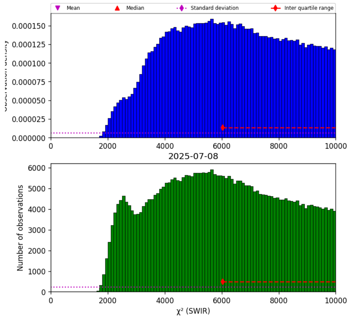
Figure 28: Histogram of “ \chi^2 (SWIR)” for 2025-07-08 to 2025-07-09
