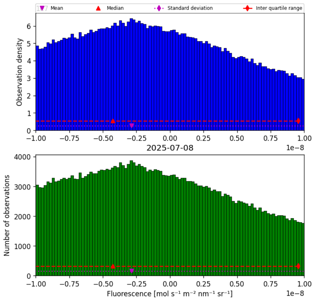
Figure 32: Histogram of “Fluorescence” for 2025-07-08 to 2025-07-09
