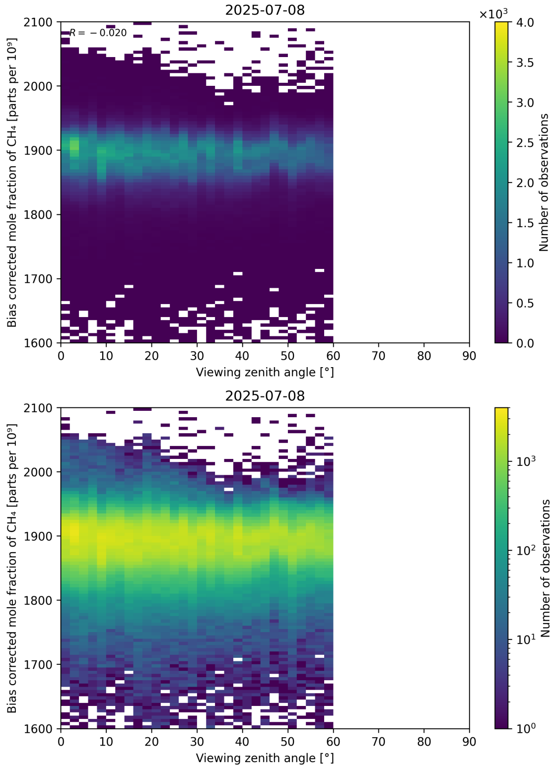
Figure 111: Scatter density plot of “Viewing zenith angle” against “Bias corrected mole fraction of CH 4 ” for 2025-07-08 to 2025-07-09.
