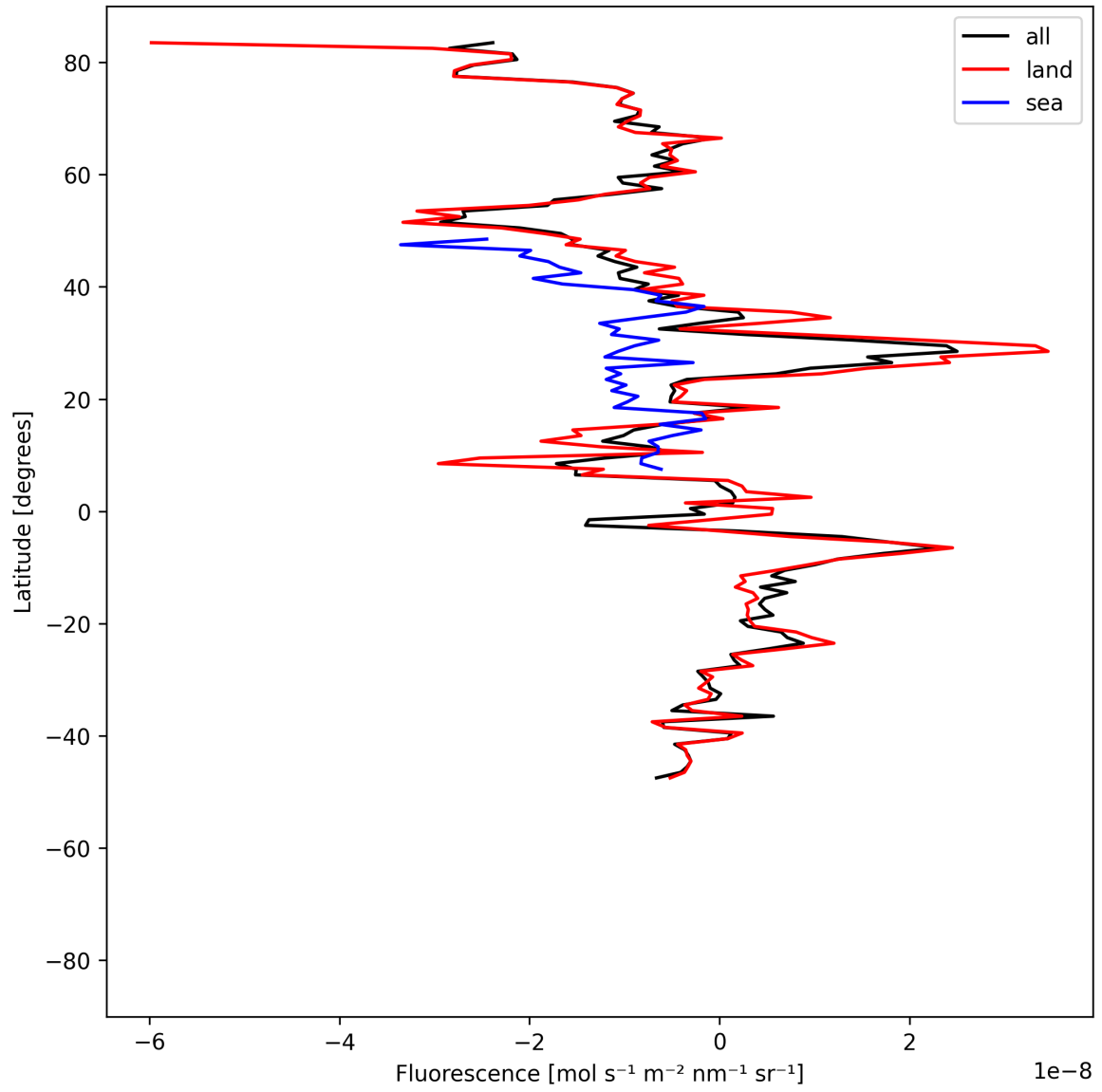
Figure 21: Zonal average of “Fluorescence” for 2025-07-08 to 2025-07-09.
