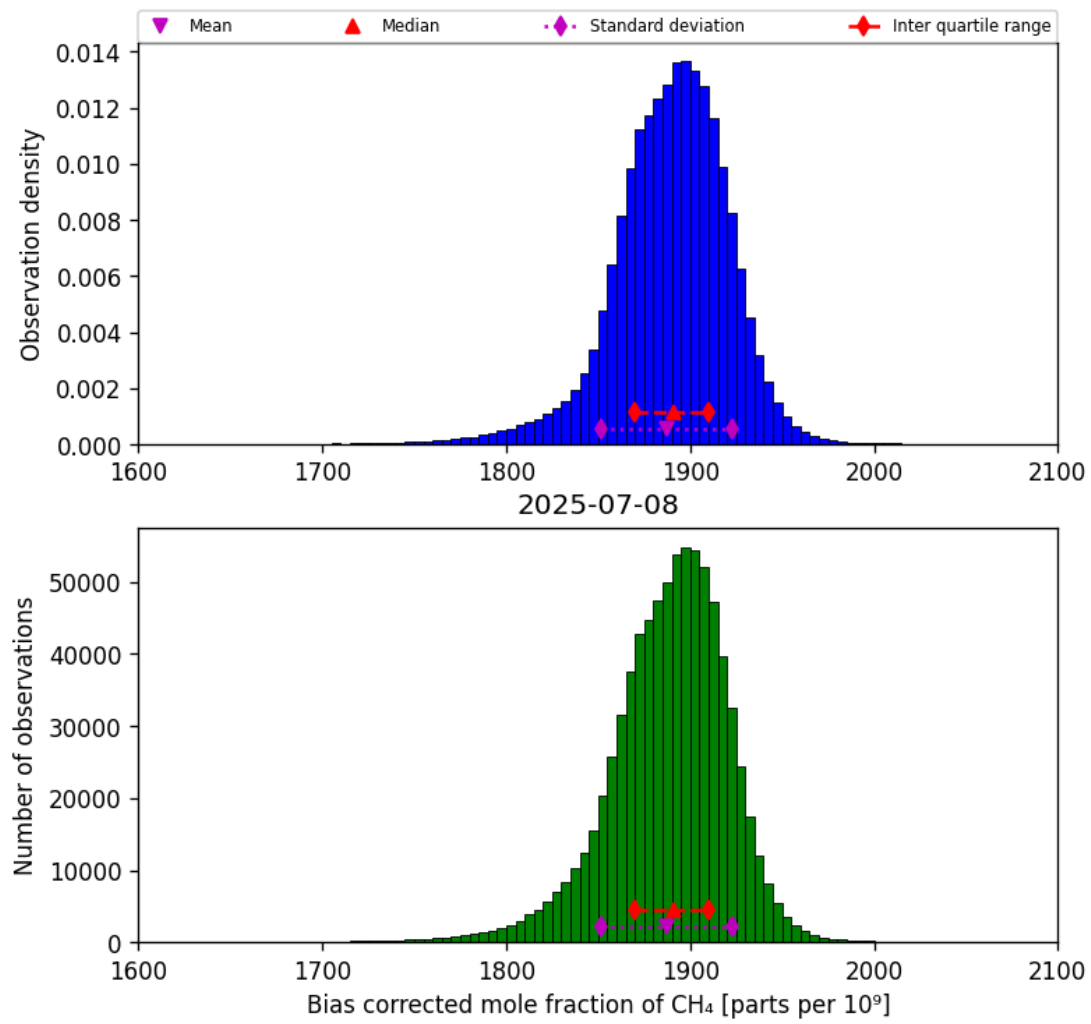
Figure 25: Histogram of “Bias corrected mole fraction of CH 4 ” for 2025-07-08 to 2025-07-09
