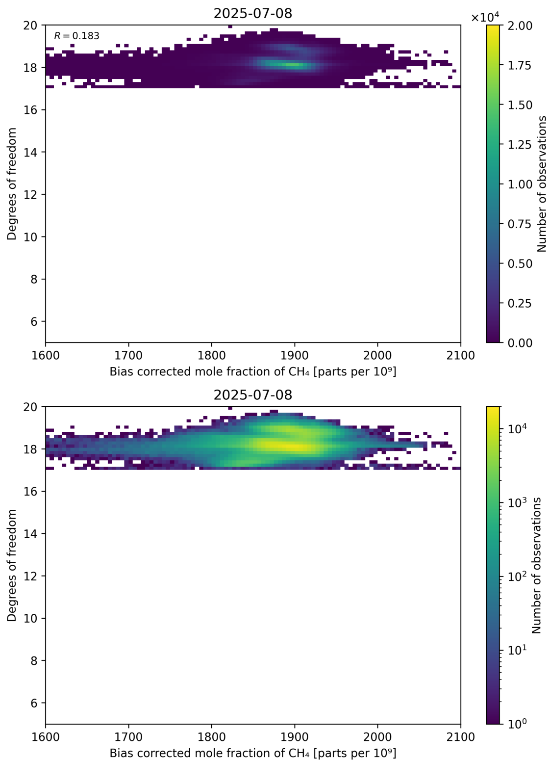
Figure 65: Scatter density plot of “Bias corrected mole fraction of \text{CH}_4 ” against “Degrees of freedom” for 2025-07-08 to 2025-07-09.
