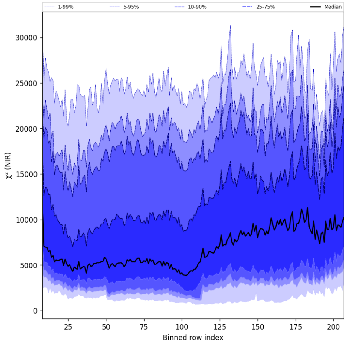
Figure 40: Along track statistics of “ \chi^2 (NIR)” for 2025-07-08 to 2025-07-09
