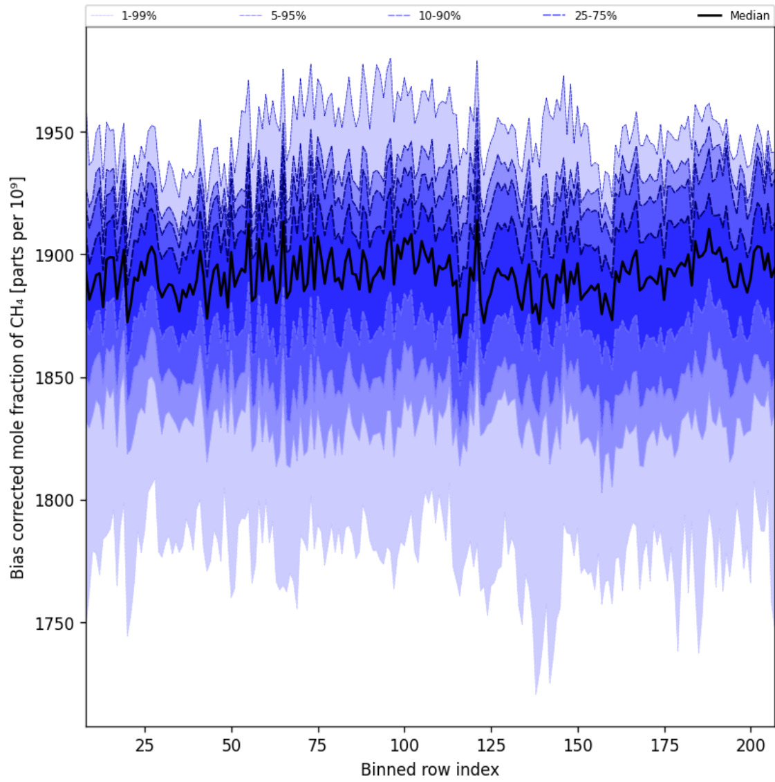
Figure 36: Along track statistics of “Bias corrected mole fraction of CH 4 ” for 2025-07-08 to 2025-07-09
