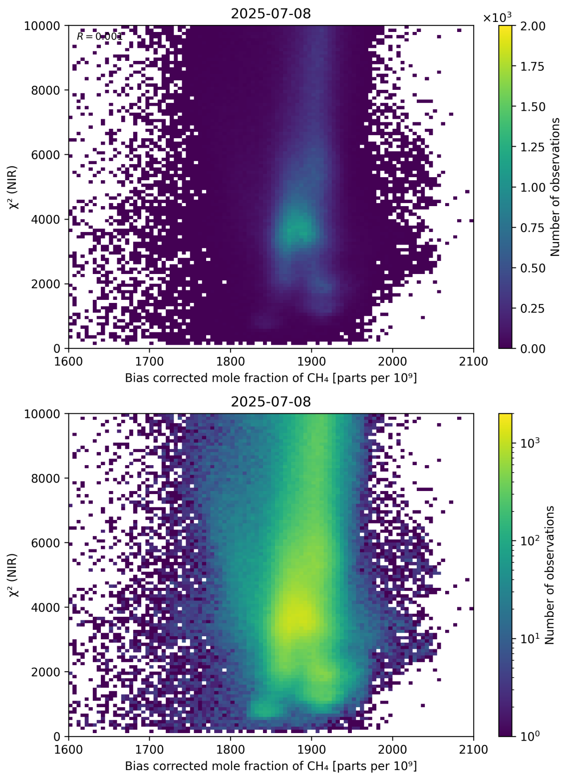
Figure 63: Scatter density plot of “Bias corrected mole fraction of CH 4 ” against “ \chi^2 (NIR)” for 2025-07-08 to 2025-07-09.
