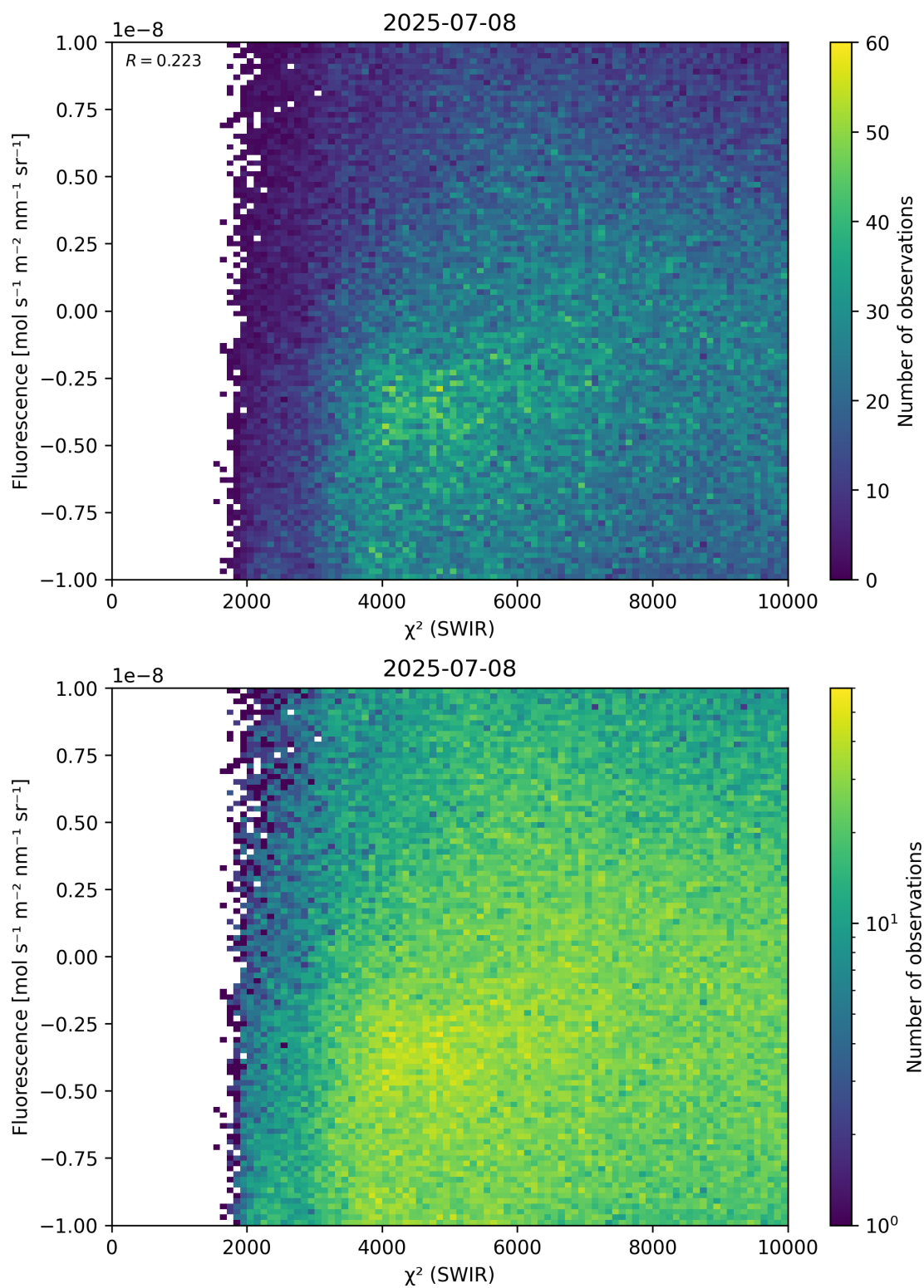
Figure 49: Scatter density plot of “ \chi^2 (SWIR)” against “Fluorescence” for 2025-07-08 to 2025-07-09.
