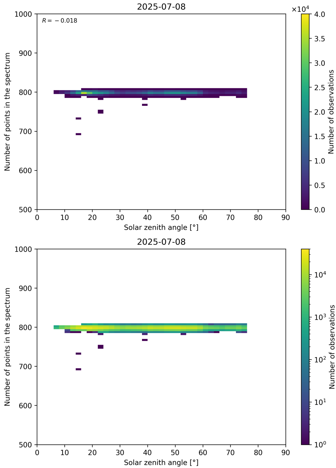
Figure 103: Scatter density plot of “Solar zenith angle” against “Number of points in the spectrum” for 2025-07-08 to 2025-07-09.
