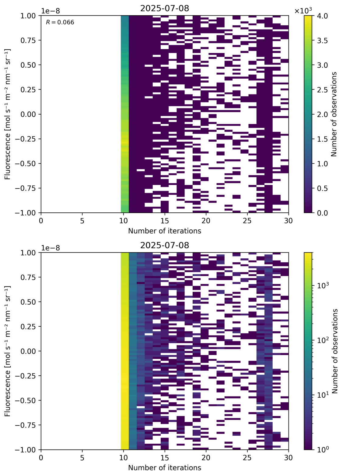
Figure 87: Scatter density plot of “Number of iterations” against “Fluorescence” for 2025-07-08 to 2025-07-09.
