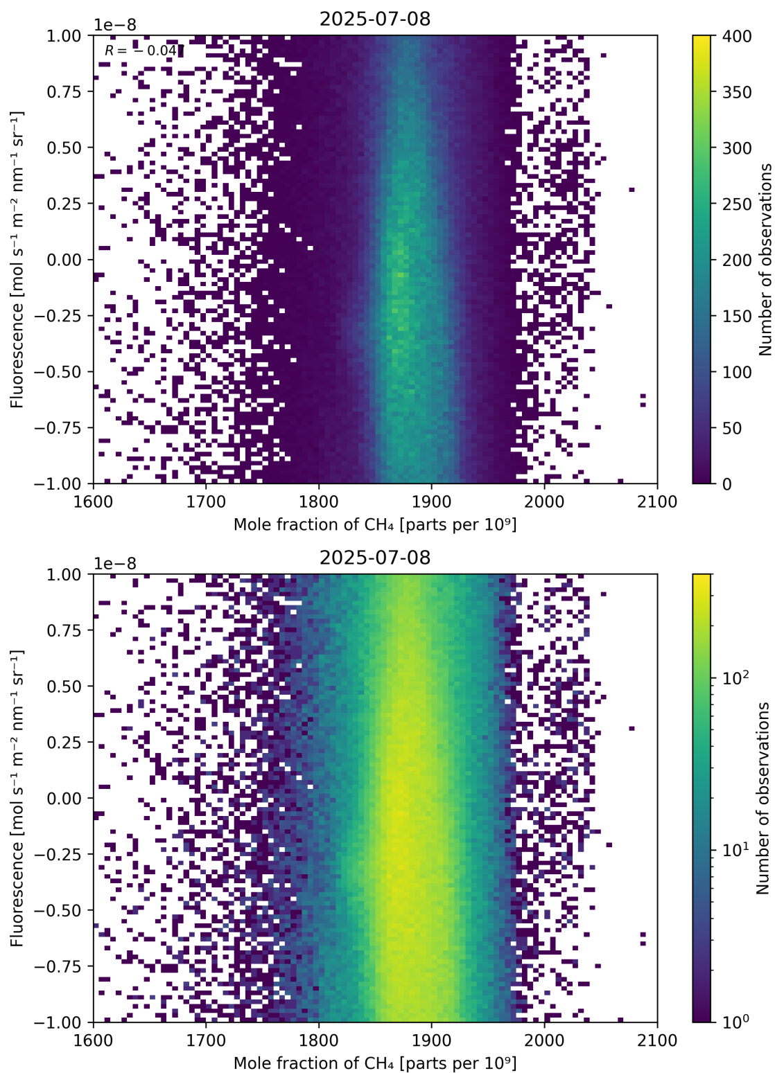
Figure 73: Scatter density plot of “Mole fraction of \text{CH}_4 ” against “Fluorescence” for 2025-07-08 to 2025-07-09.
