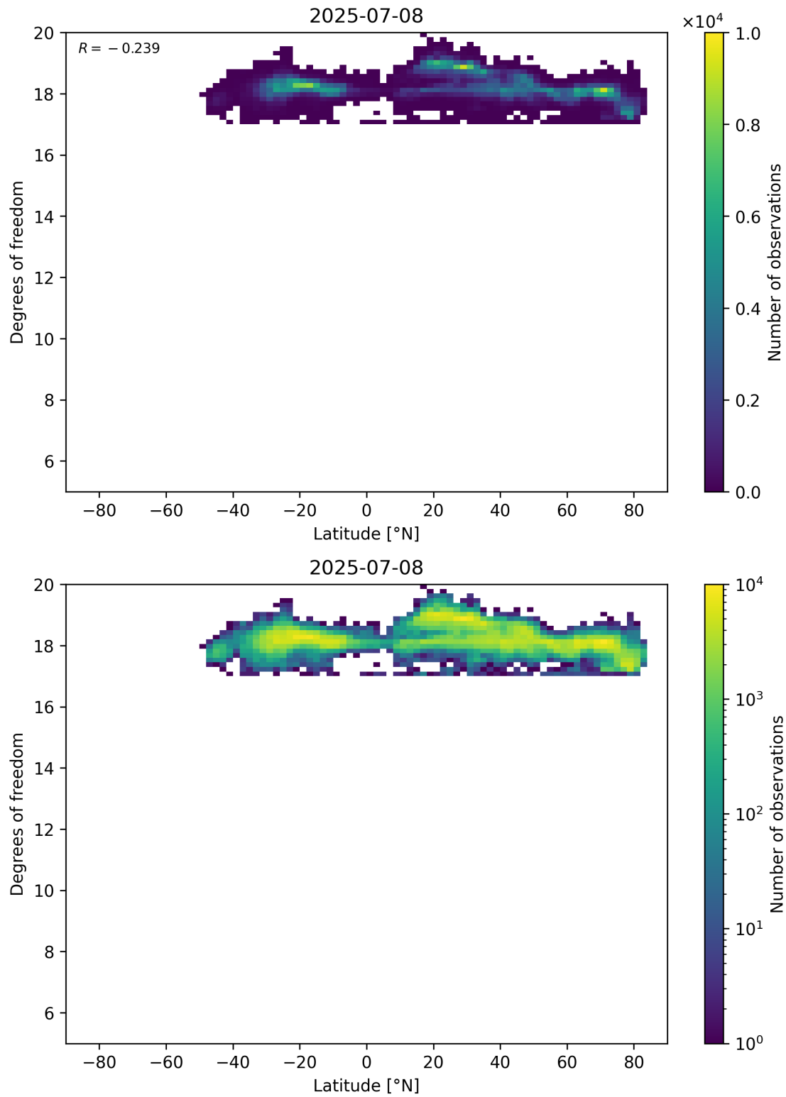
Figure 55: Scatter density plot of “Latitude” against “Degrees of freedom” for 2025-07-08 to 2025-07-09.
