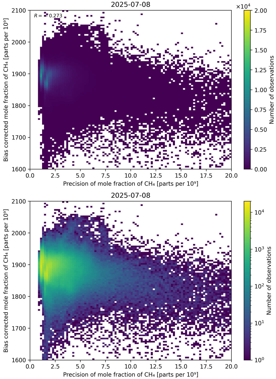
Figure 82: Scatter density plot of “Precision of mole fraction of CH 4 ” against “Bias corrected mole fraction of CH 4 ” for 2025-07-08 to 2025-07-09.
