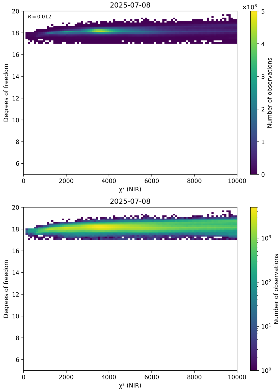
Figure 44: Scatter density plot of “ \chi^2 (NIR)” against “Degrees of freedom” for 2025-07-08 to 2025-07-09.
