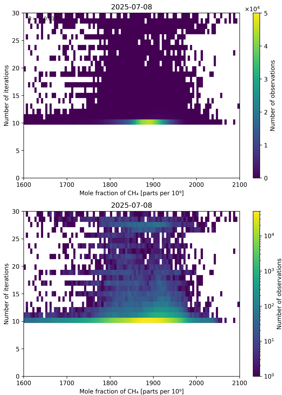
Figure 76: Scatter density plot of “Mole fraction of CH 4 ” against “Number of iterations” for 2025-07-08 to 2025-07-09.
