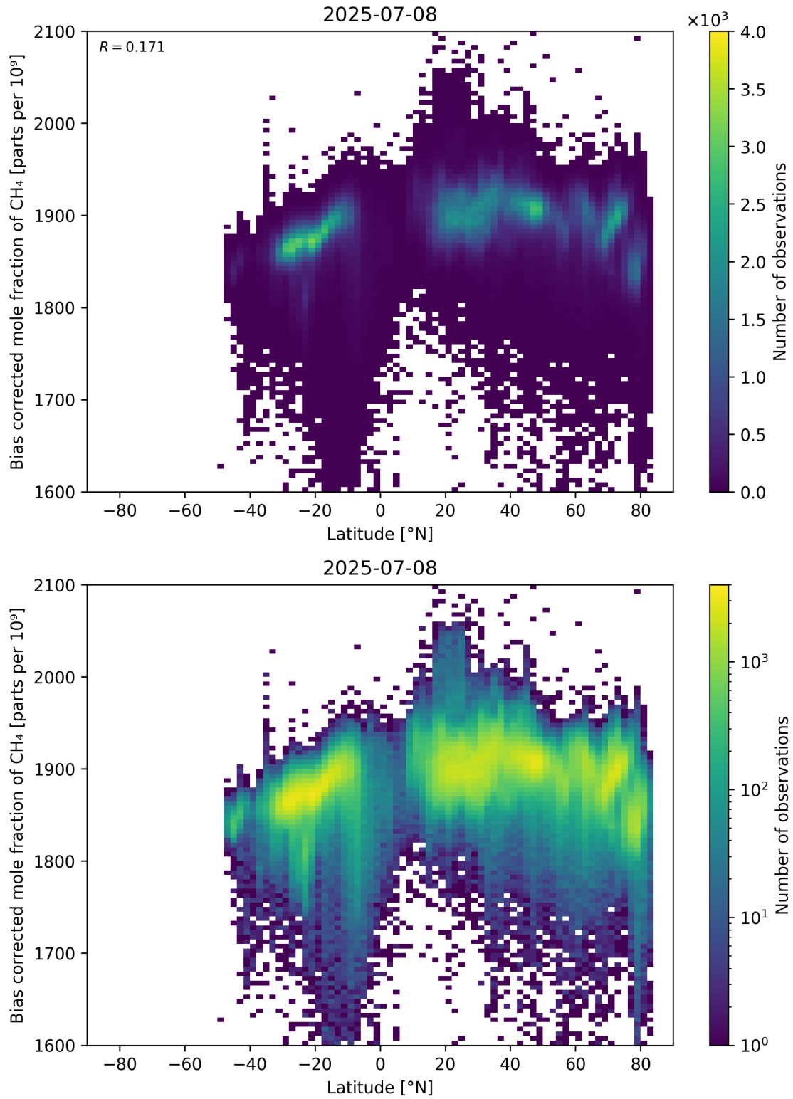
Figure 58: Scatter density plot of “Latitude” against “Bias corrected mole fraction of CH 4 ” for 2025-07-08 to 2025-07-09.
