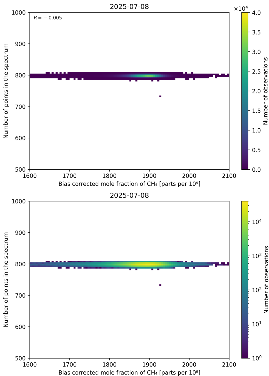
Figure 68: Scatter density plot of “Bias corrected mole fraction of CH 4 ” against “Number of points in the spectrum” for 2025-07-08 to 2025-07-09.
