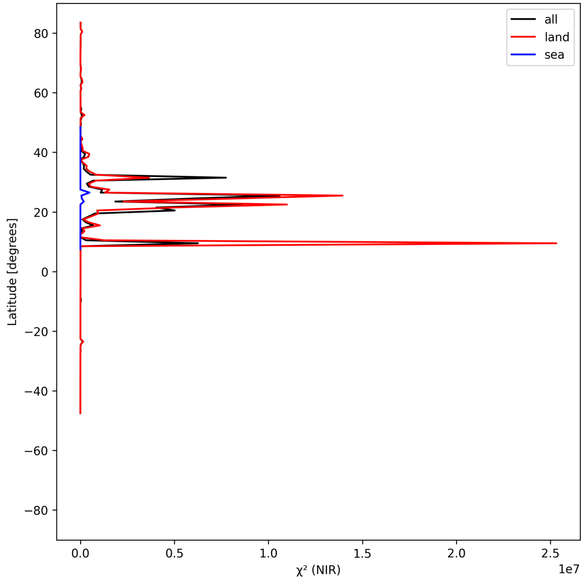
Figure 18: Zonal average of “ \chi^2 (NIR)” for 2025-07-08 to 2025-07-09.
