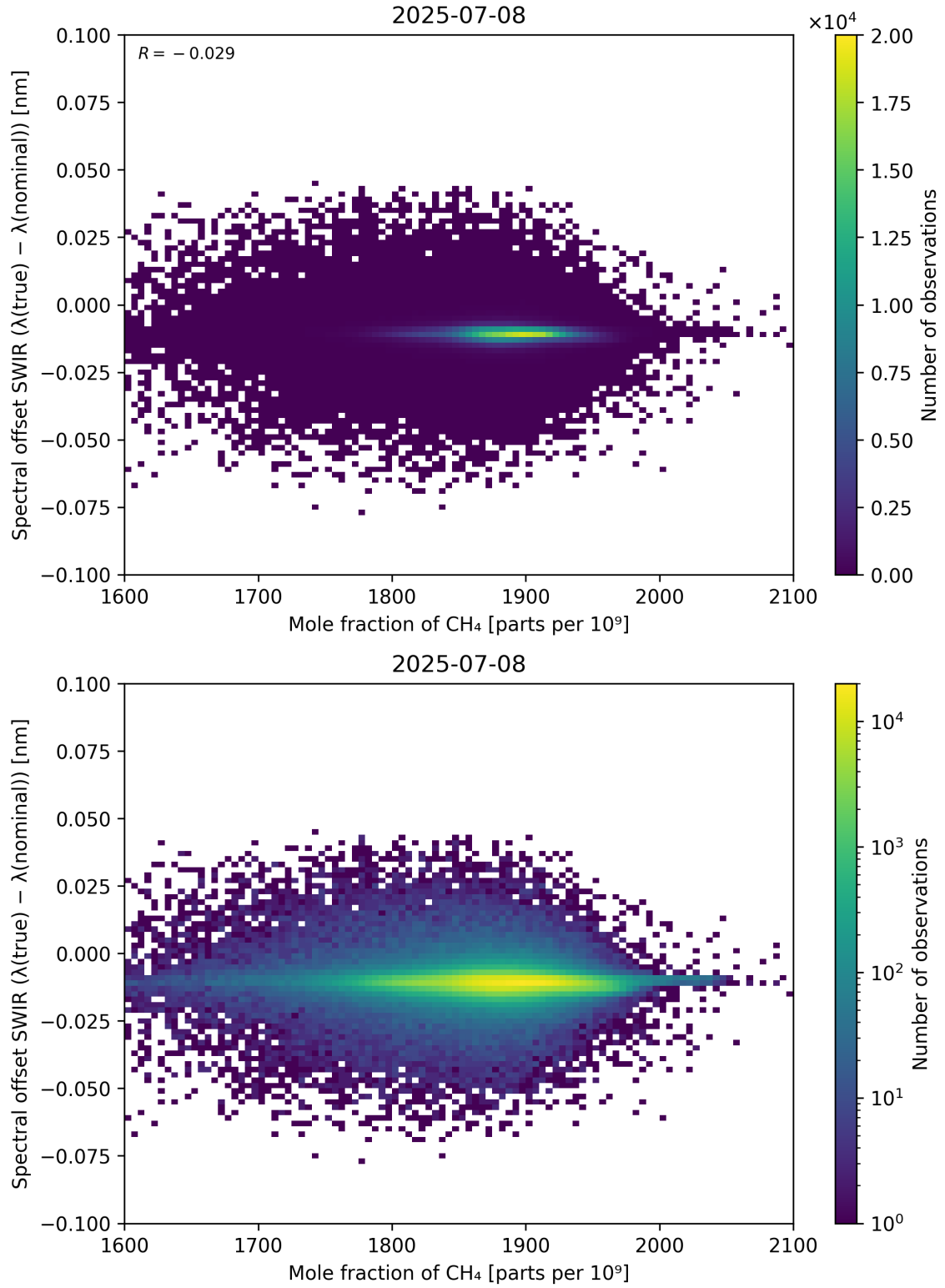
Figure 86: Scatter density plot of “Mole fraction of CH 4 ” against “Spectral offset SWIR ( \lambda_{\text{true}} - \lambda_{\text{nominal}} )” for 2025-07-08 to 2025-07-09.
