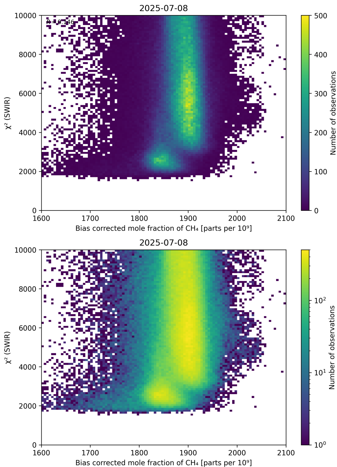
Figure 64: Scatter density plot of “Bias corrected mole fraction of CH 4 ” against “ \chi^2 (SWIR)” for 2025-07-08 to 2025-07-09.
