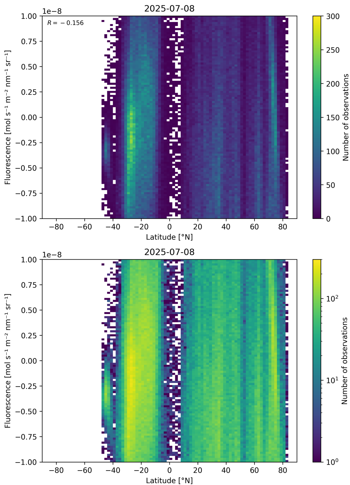
Figure 56: Scatter density plot of “Latitude” against “Fluorescence” for 2025-07-08 to 2025-07-09.
