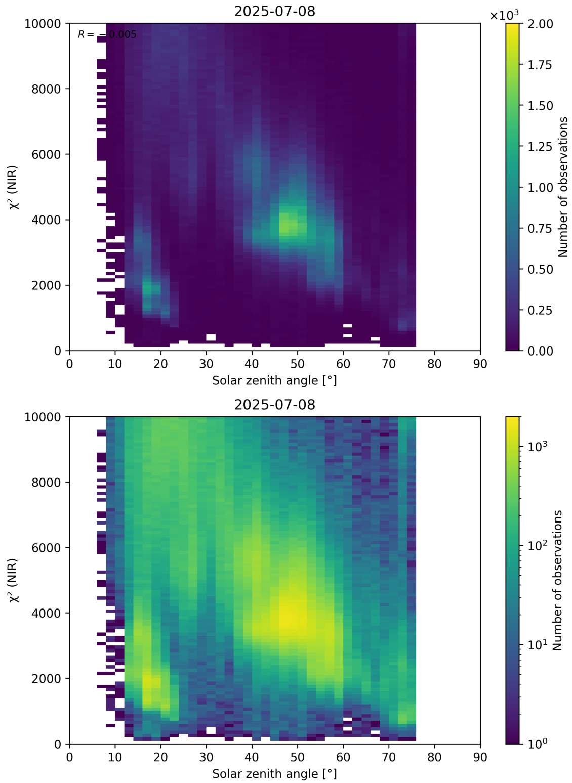
Figure 94: Scatter density plot of “Solar zenith angle” against “ \chi^2 (NIR)” for 2025-07-08 to 2025-07-09.
