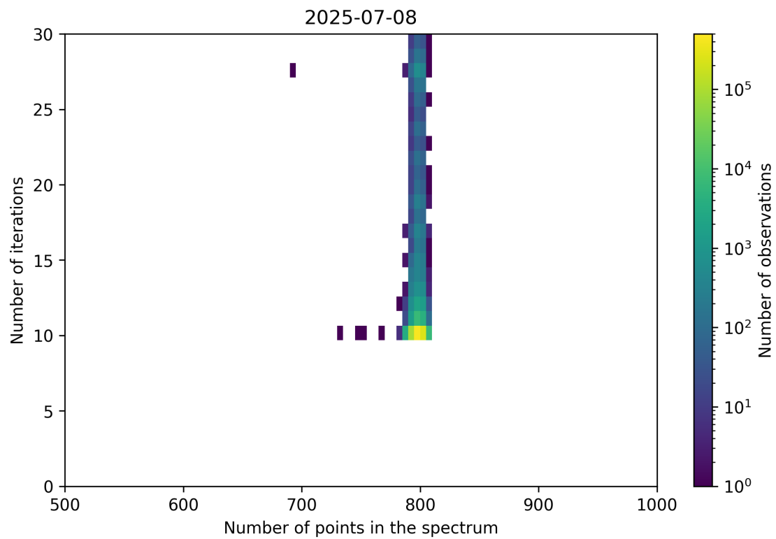
Figure 92: Scatter density plot of “Number of points in the spectrum” against “Number of iterations” for 2025-07-08 to 2025-07-09.
