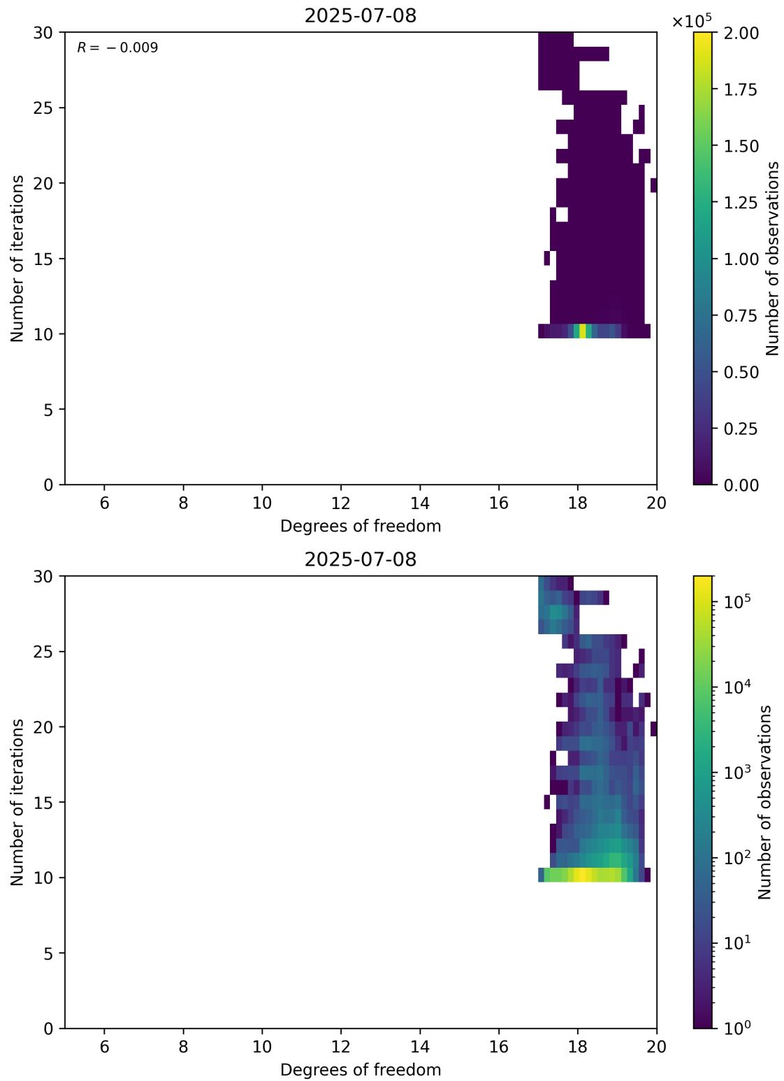
Figure 52: Scatter density plot of “Degrees of freedom” against “Number of iterations” for 2025-07-08 to 2025-07-09.
