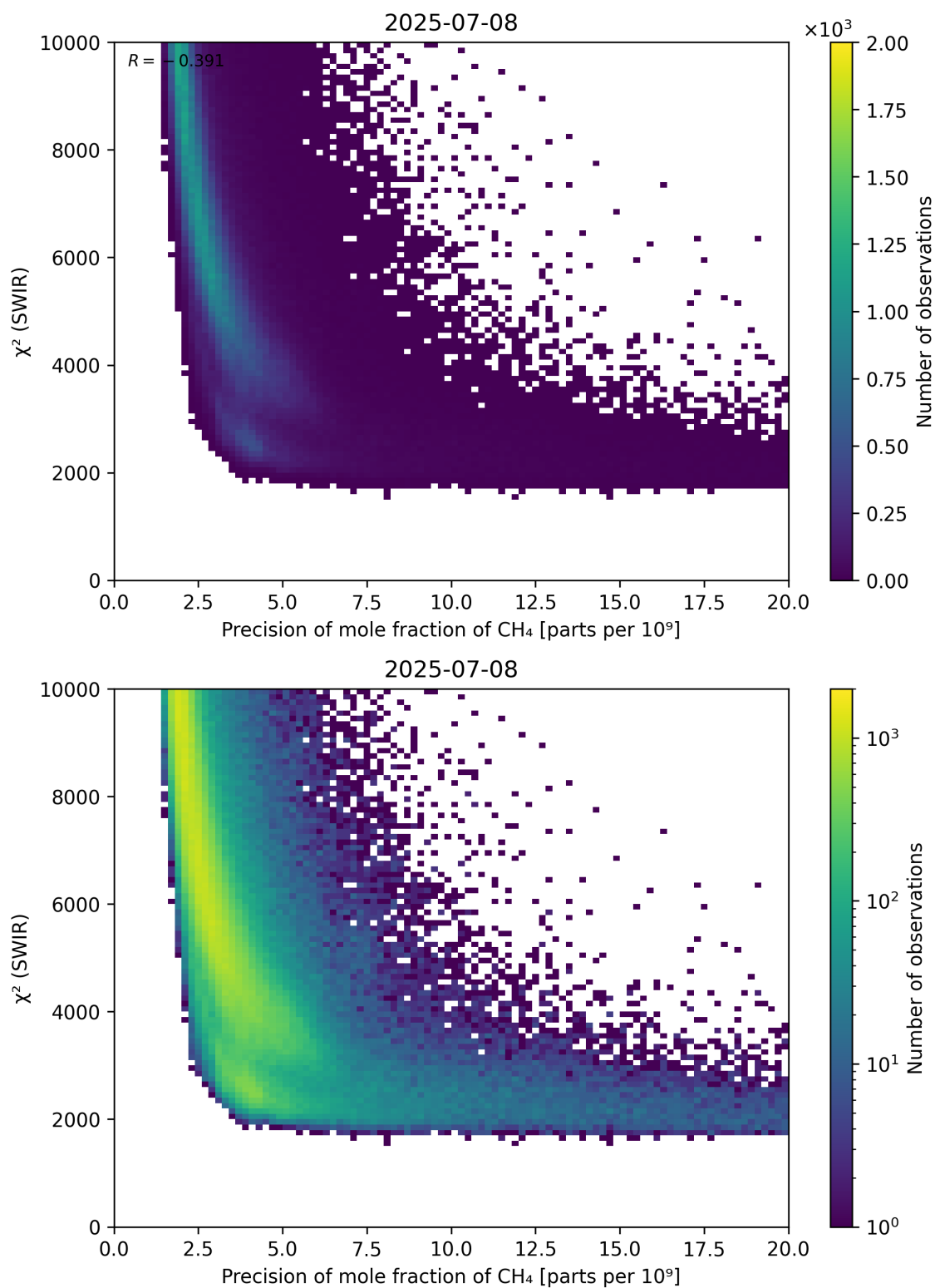
Figure 79: Scatter density plot of “Precision of mole fraction of \text{CH}_4 ” against “ \chi^2 (SWIR)” for 2025-07-08 to 2025-07-09.
