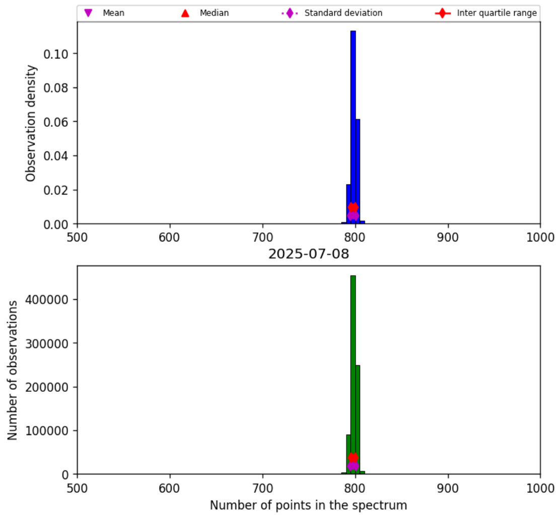
Figure 26: Histogram of “Number of points in the spectrum” for 2025-07-08 to 2025-07-09
