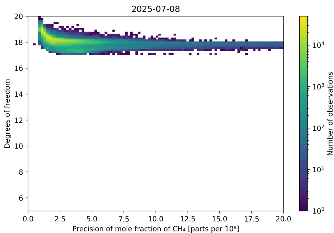
Figure 80: Scatter density plot of “Precision of mole fraction of CH 4 ” against “Degrees of freedom” for 2025-07-08 to 2025-07-09.
