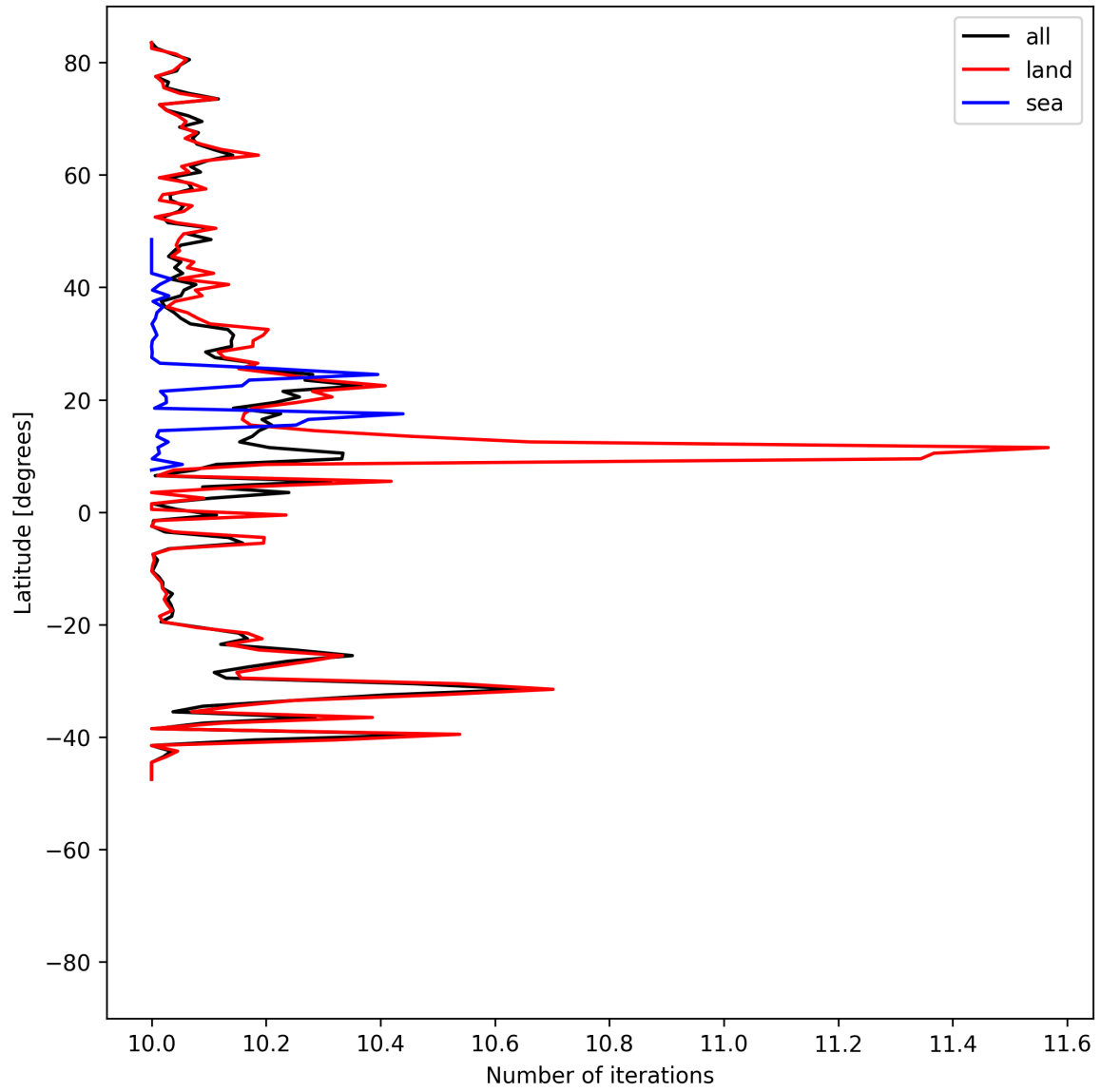
Figure 20: Zonal average of “Number of iterations” for 2025-07-08 to 2025-07-09.
