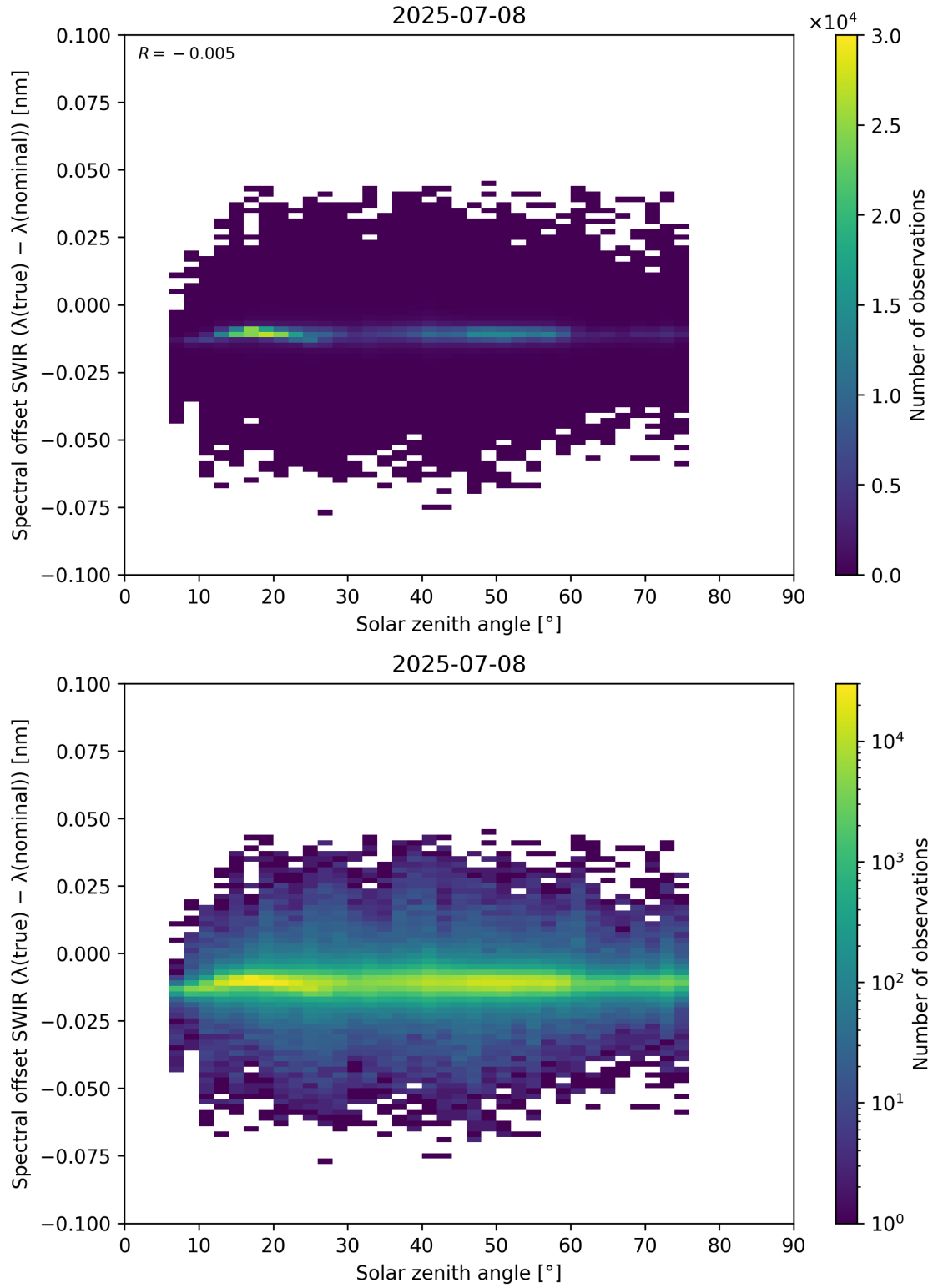
Figure 104: Scatter density plot of “Solar zenith angle” against “Spectral offset SWIR ( \lambda_{\text{true}} - \lambda_{\text{nominal}} )” for 2025-07-08 to 2025-07-09.
