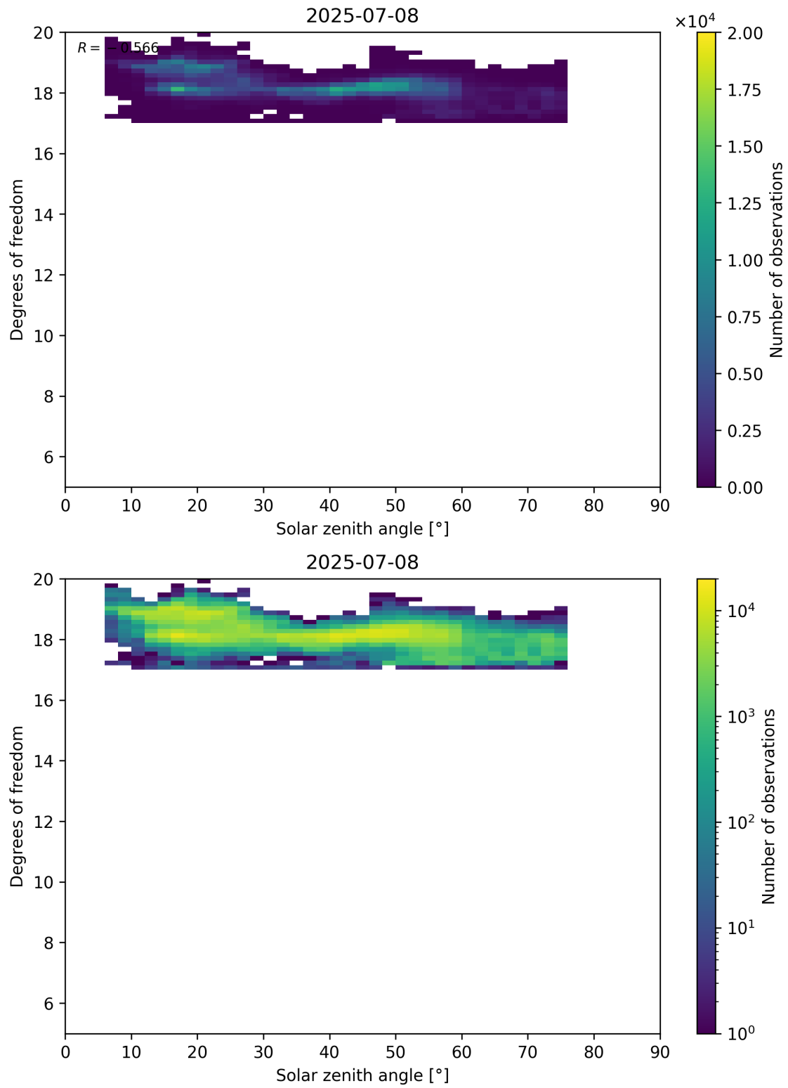
Figure 96: Scatter density plot of “Solar zenith angle” against “Degrees of freedom” for 2025-07-08 to 2025-07-09.
