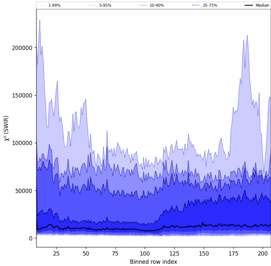
Figure 39: Along track statistics of “ \chi^2 (SWIR)” for 2025-07-08 to 2025-07-09
