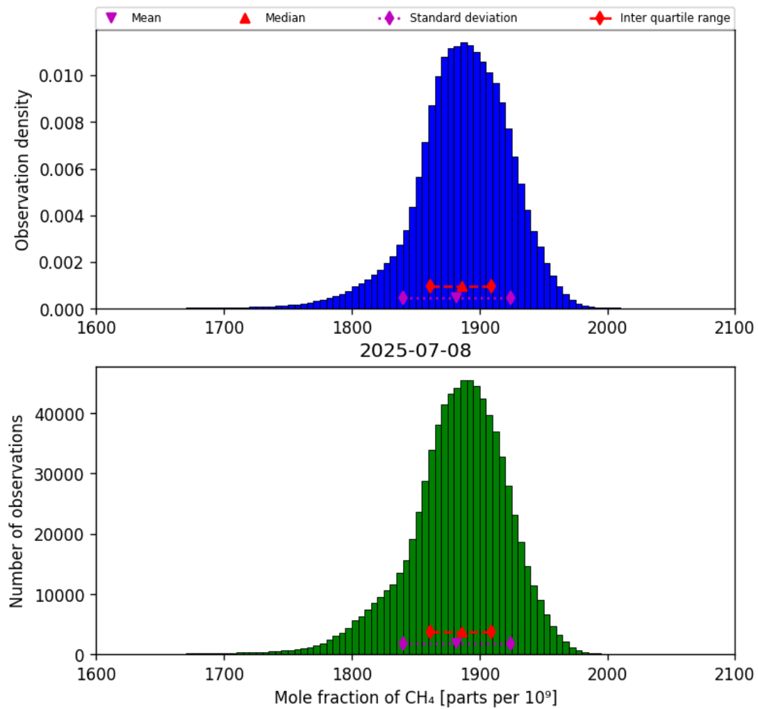
Figure 23: Histogram of “Mole fraction of CH 4 ” for 2025-07-08 to 2025-07-09
