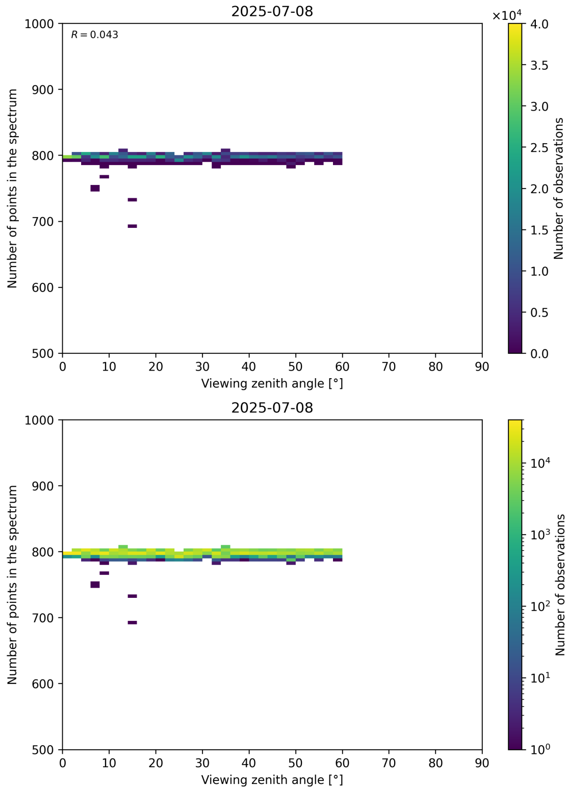
Figure 114: Scatter density plot of “Viewing zenith angle” against “Number of points in the spectrum” for 2025-07-08 to 2025-07-09.
