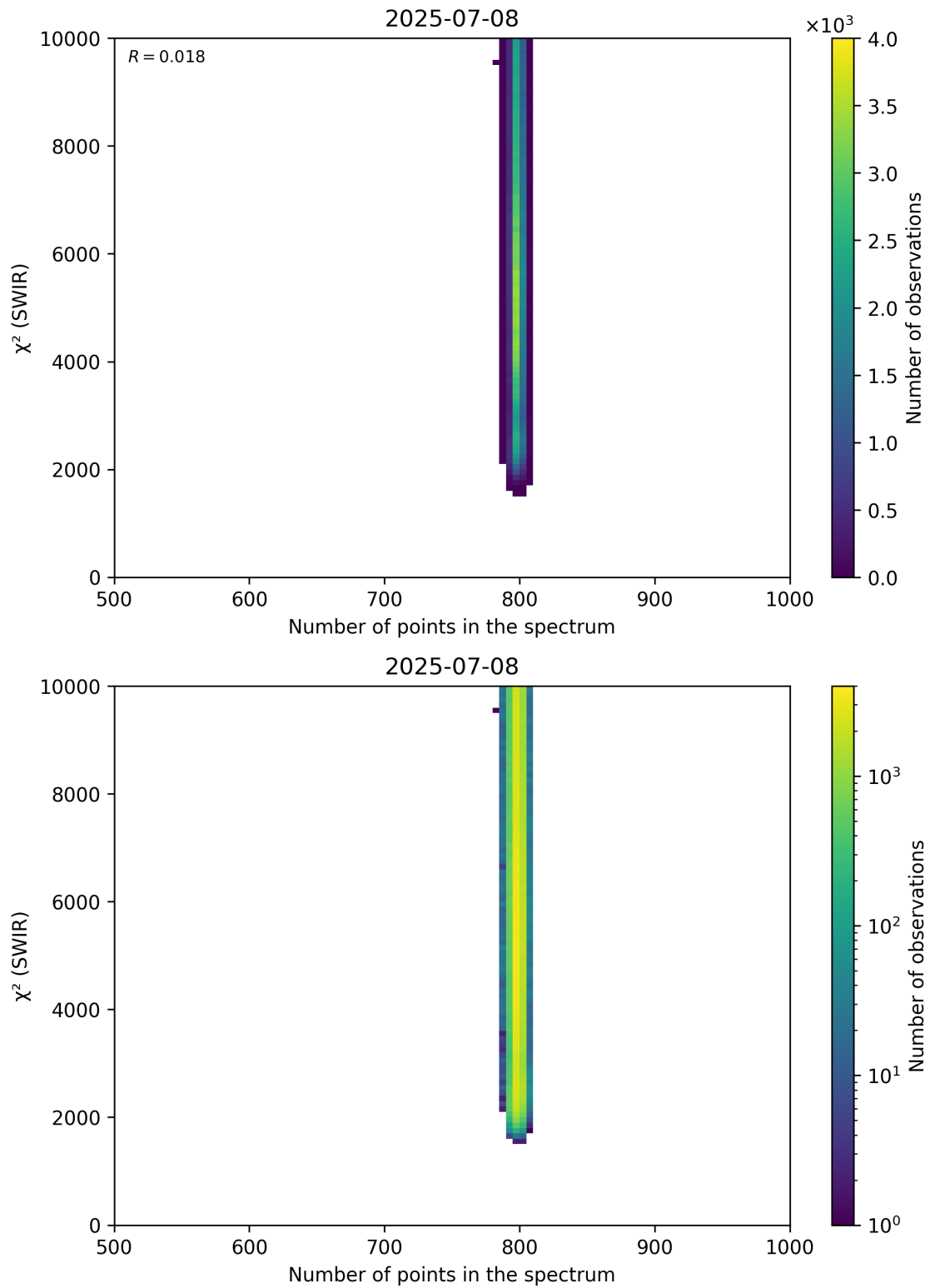
Figure 89: Scatter density plot of “Number of points in the spectrum” against “ \chi^2 (SWIR)” for 2025-07-08 to 2025-07-09.
