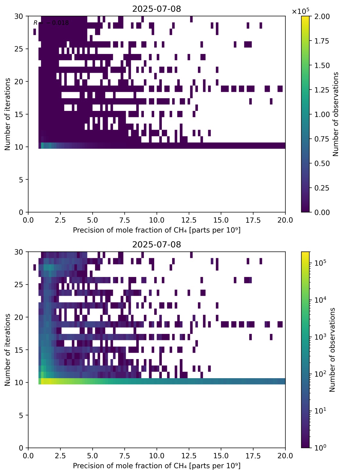
Figure 83: Scatter density plot of “Precision of mole fraction of CH 4 ” against “Number of iterations” for 2025-07-08 to 2025-07-09.
