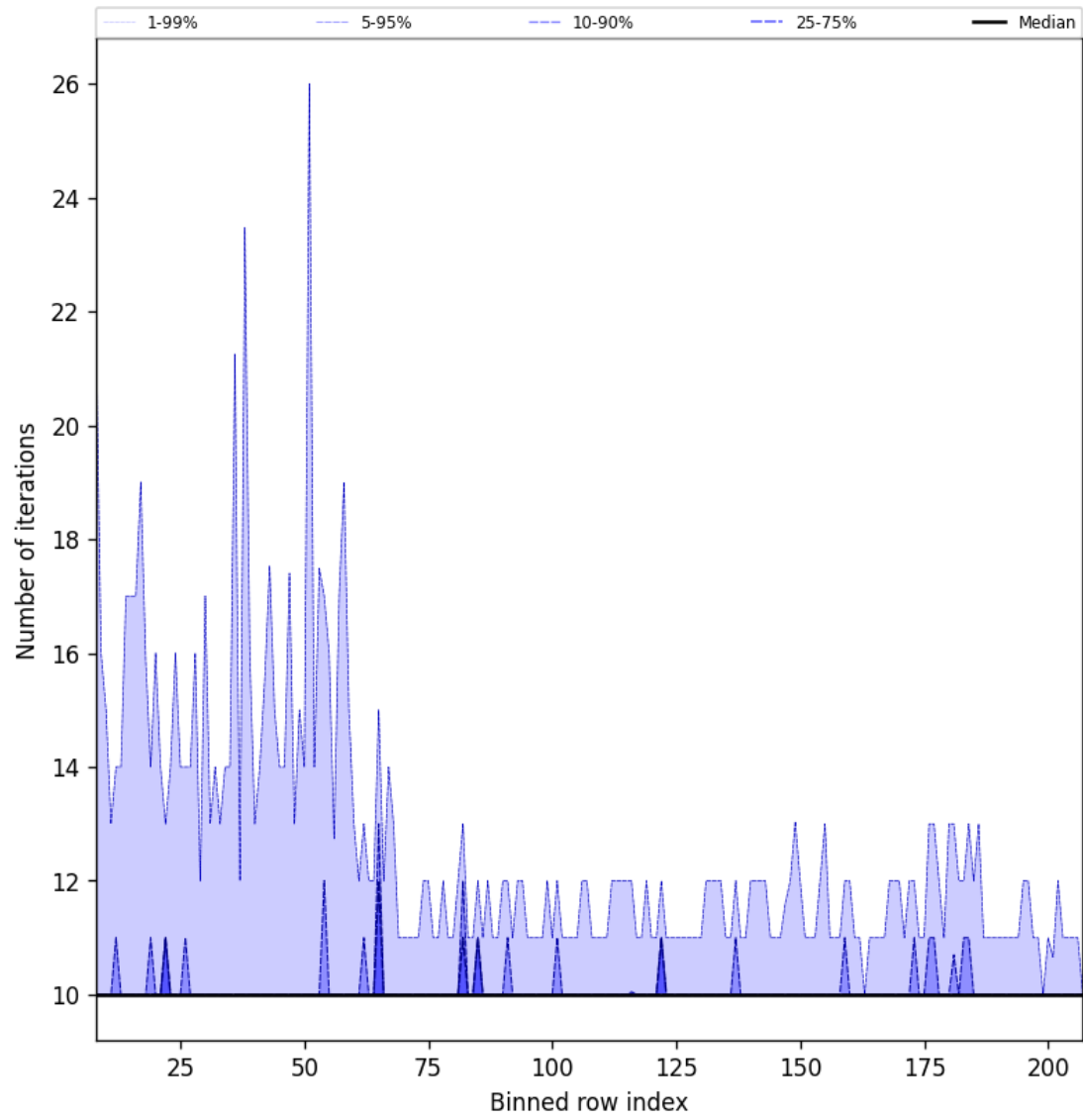
Figure 42: Along track statistics of “Number of iterations” for 2025-07-08 to 2025-07-09
