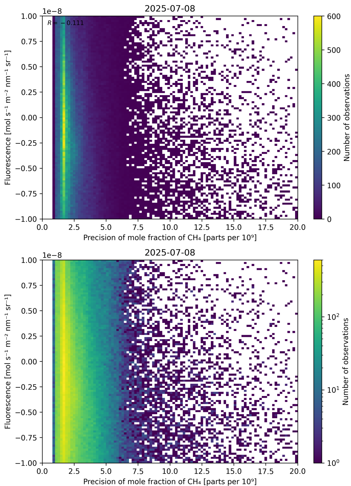
Figure 81: Scatter density plot of “Precision of mole fraction of CH 4 ” against “Fluorescence” for 2025-07-08 to 2025-07-09.
