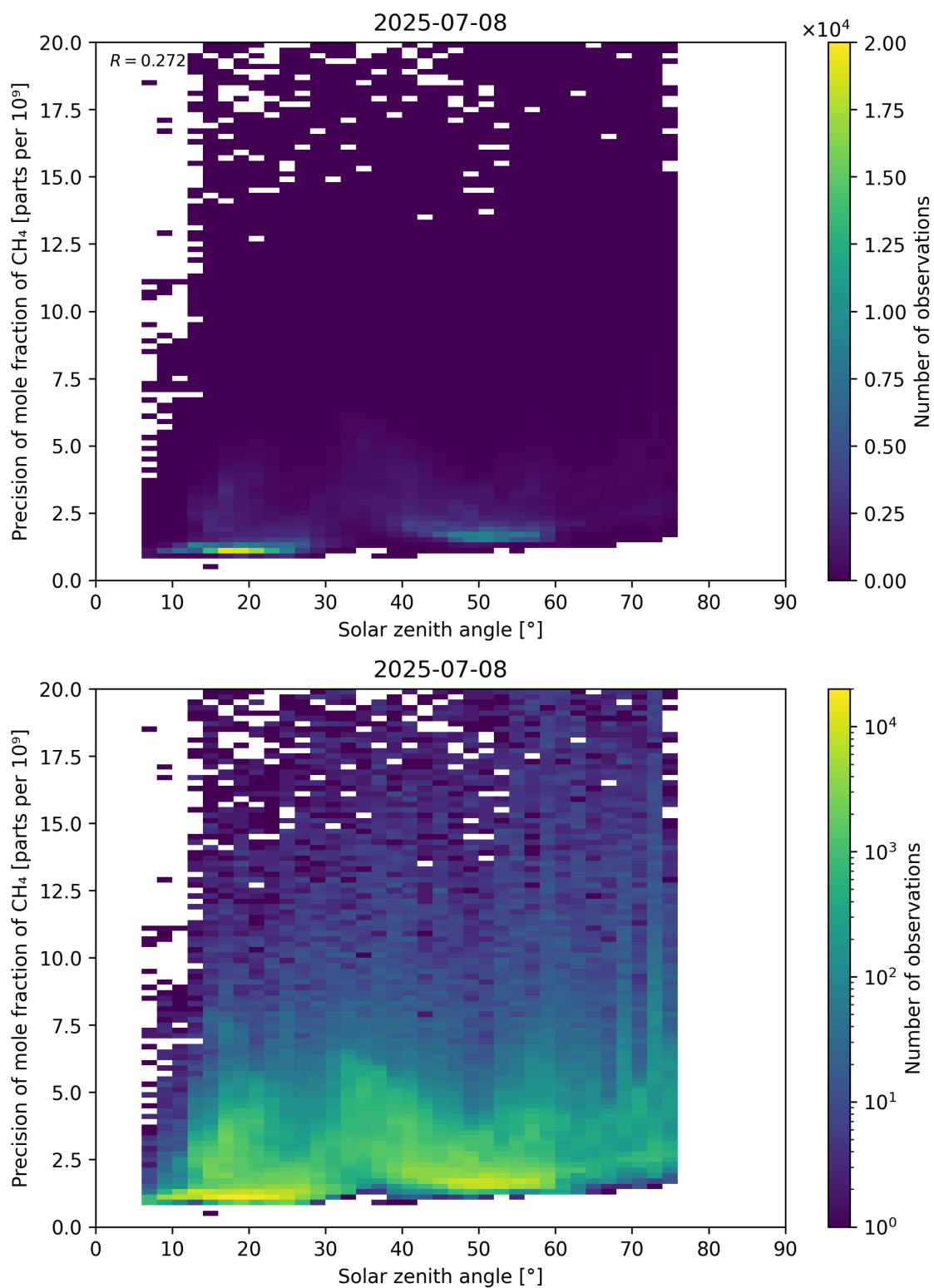
Figure 101: Scatter density plot of “Solar zenith angle” against “Precision of mole fraction of CH 4 ” for 2025-07-08 to 2025-07-09.
