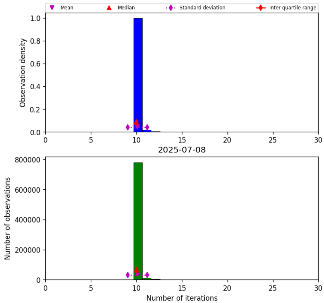
Figure 31: Histogram of “Number of iterations” for 2025-07-08 to 2025-07-09
