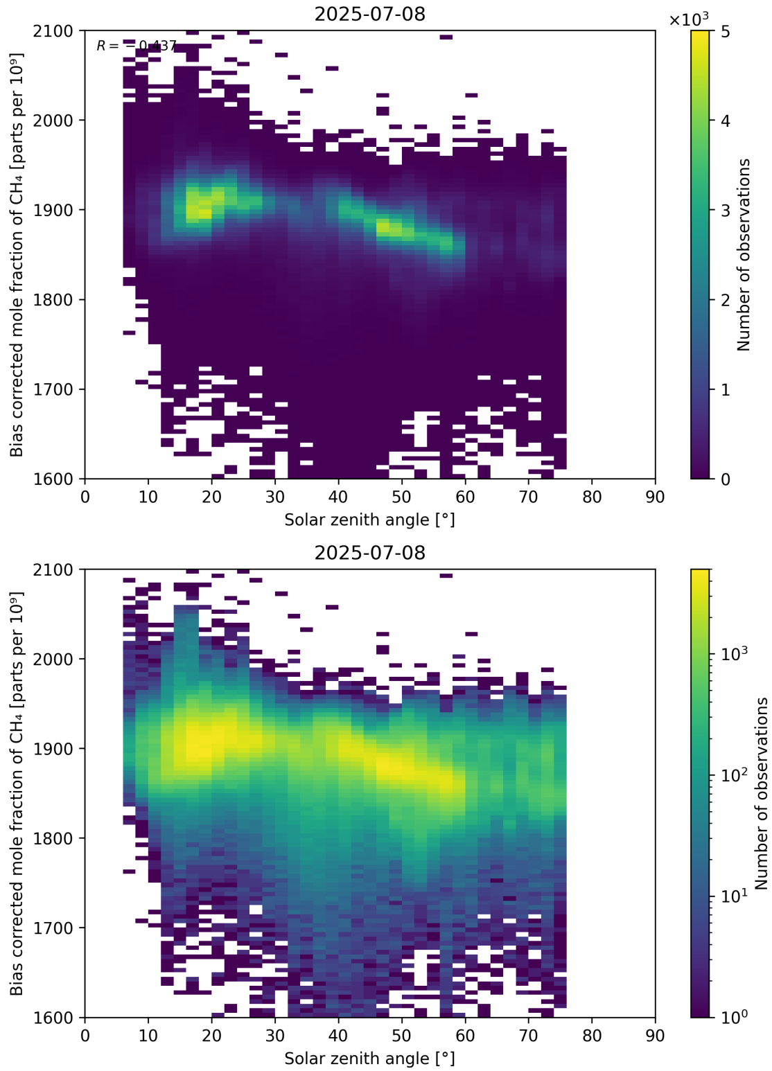
Figure 100: Scatter density plot of “Solar zenith angle” against “Bias corrected mole fraction of CH 4 ” for 2025-07-08 to 2025-07-09.
