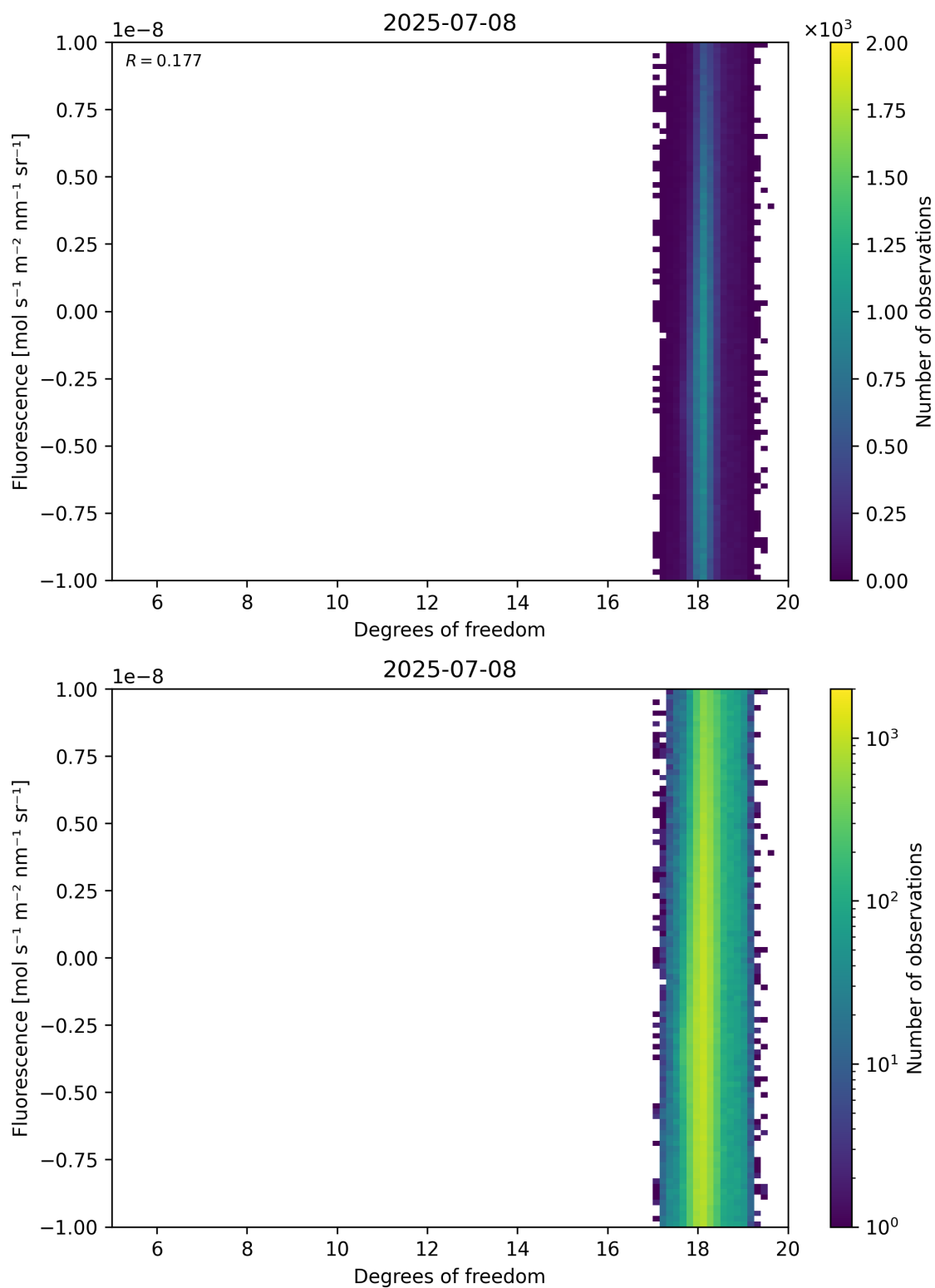
Figure 51: Scatter density plot of “Degrees of freedom” against “Fluorescence” for 2025-07-08 to 2025-07-09.
