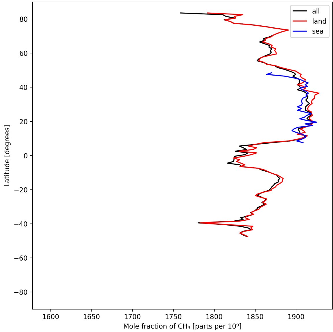
Figure 12: Zonal average of “Mole fraction of \text{CH}_4 ” for 2025-07-08 to 2025-07-09.
