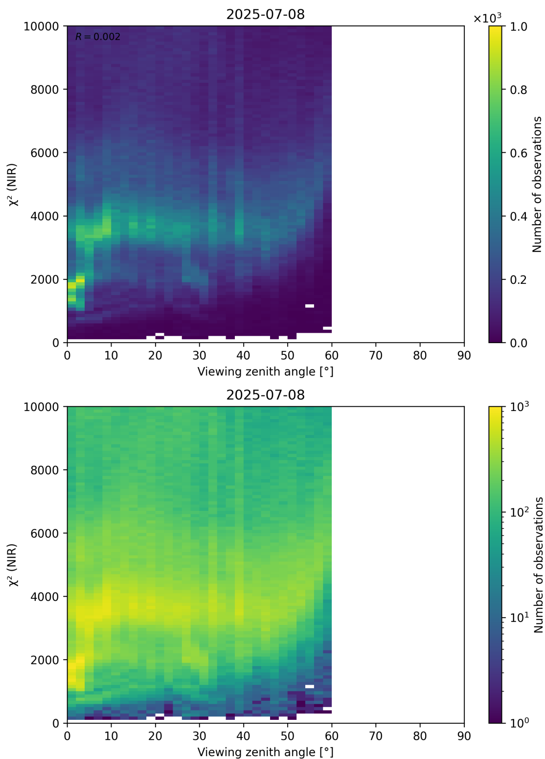
Figure 105: Scatter density plot of “Viewing zenith angle” against “ \chi^2 (NIR)” for 2025-07-08 to 2025-07-09.
