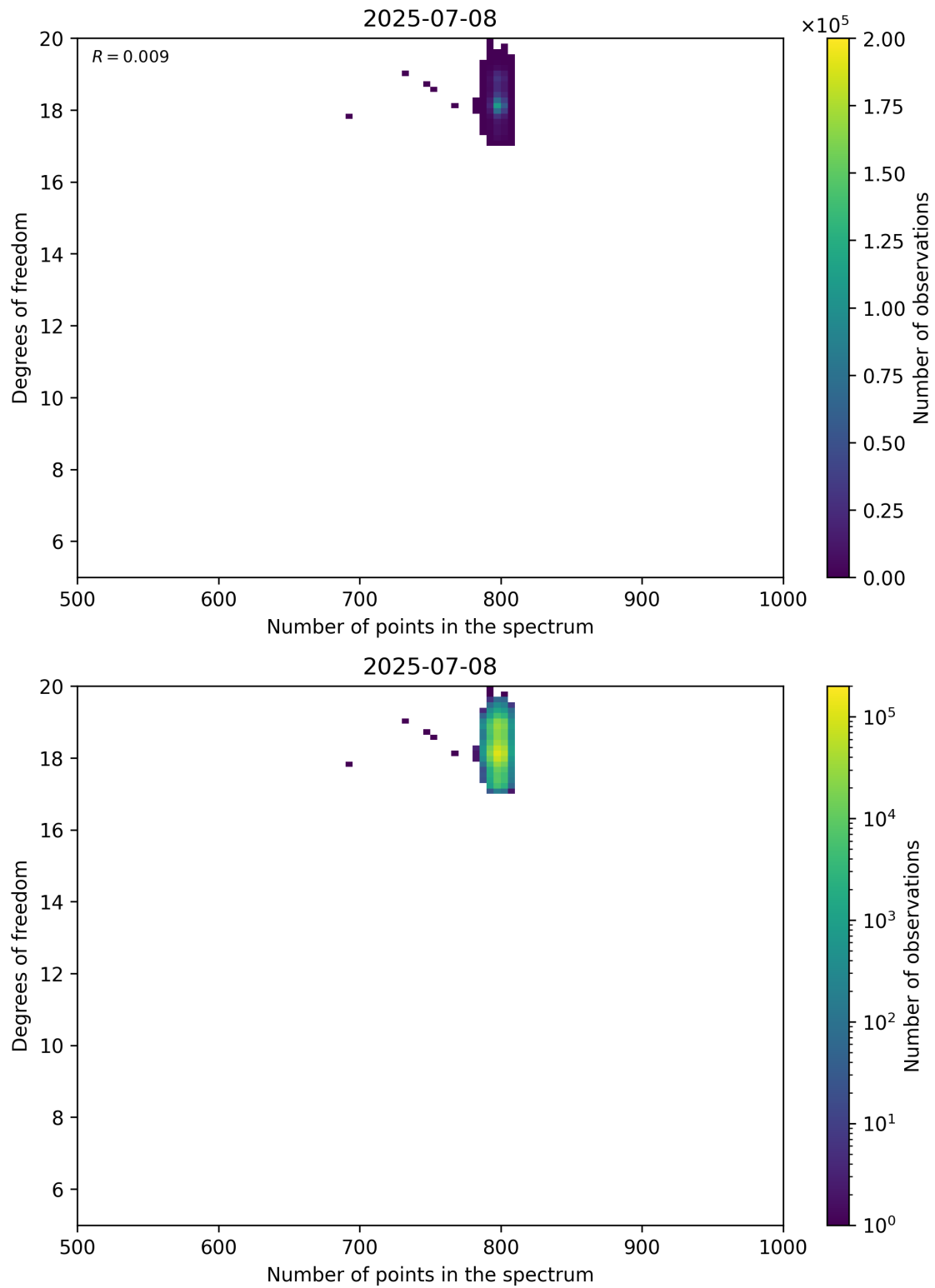
Figure 90: Scatter density plot of “Number of points in the spectrum” against “Degrees of freedom” for 2025-07-08 to 2025-07-09.
