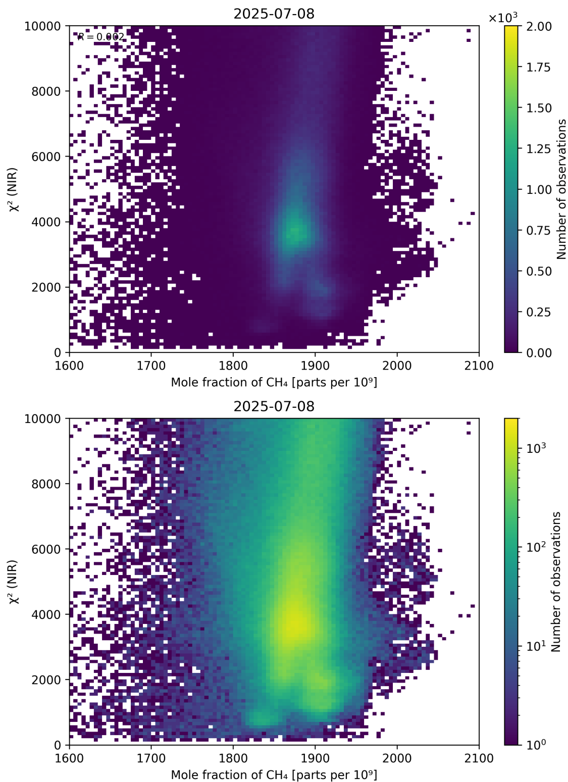
Figure 70: Scatter density plot of “Mole fraction of \text{CH}_4 ” against “ \chi^2 (NIR)” for 2025-07-08 to 2025-07-09.
