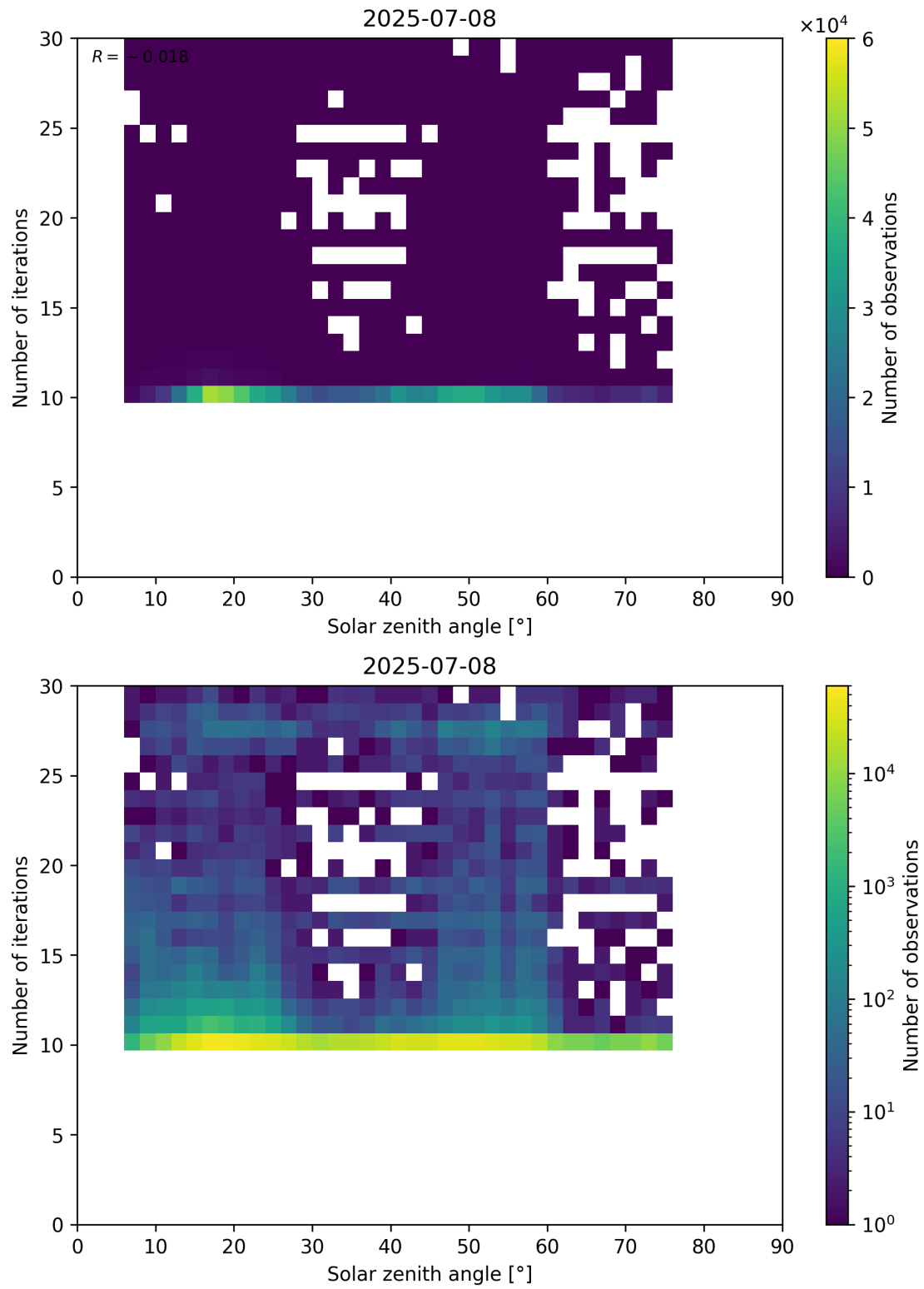
Figure 102: Scatter density plot of “Solar zenith angle” against “Number of iterations” for 2025-07-08 to 2025-07-09.
