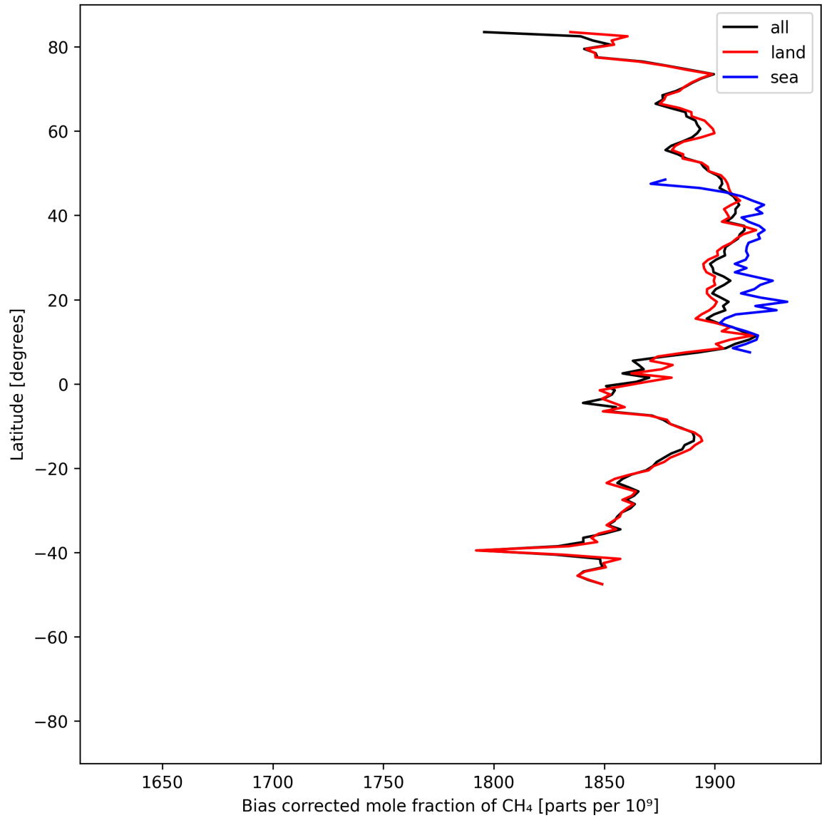
Figure 14: Zonal average of “Bias corrected mole fraction of \text{CH}_4 ” for 2025-07-08 to 2025-07-09.
