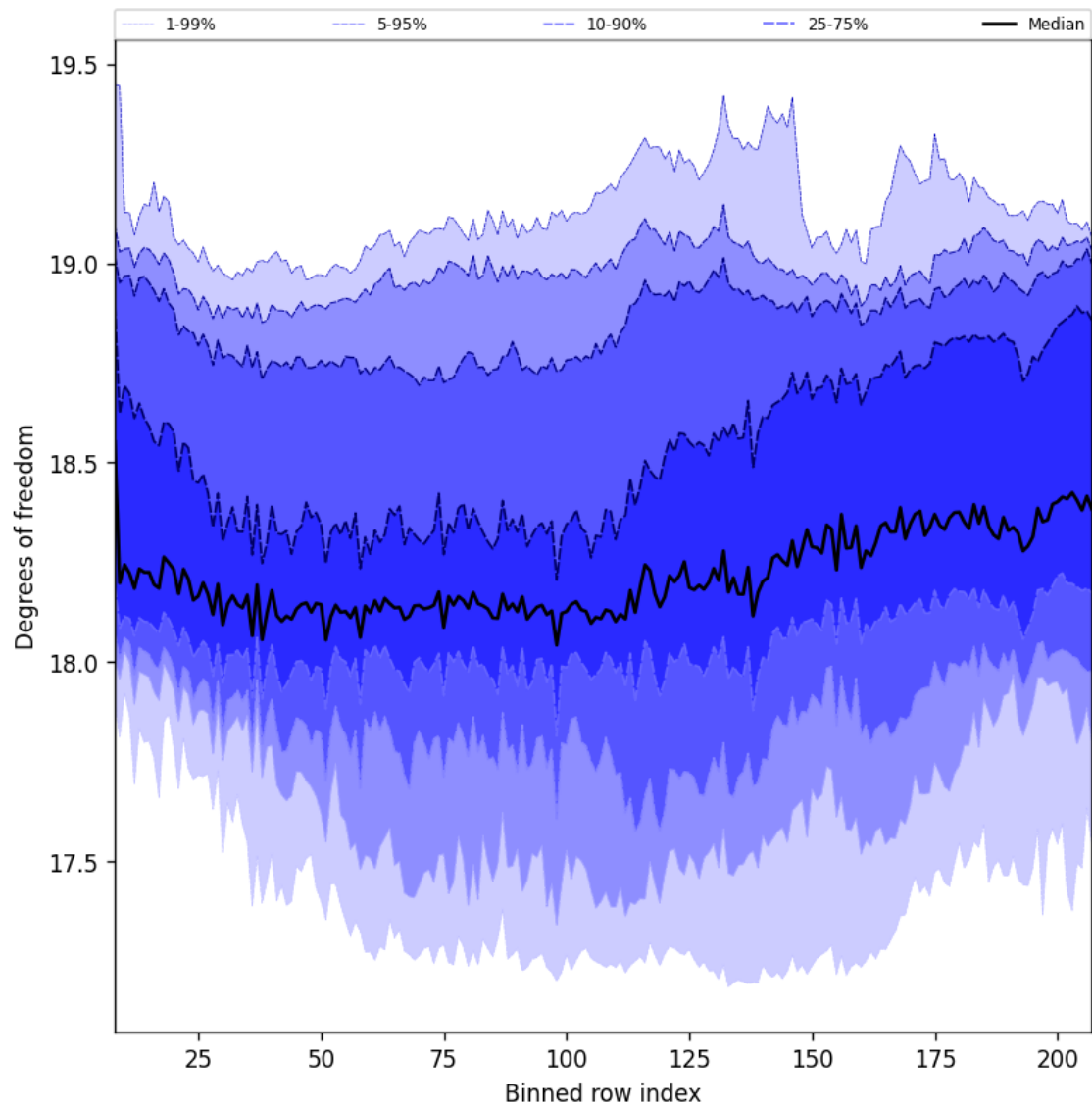
Figure 41: Along track statistics of “Degrees of freedom” for 2025-07-08 to 2025-07-09
