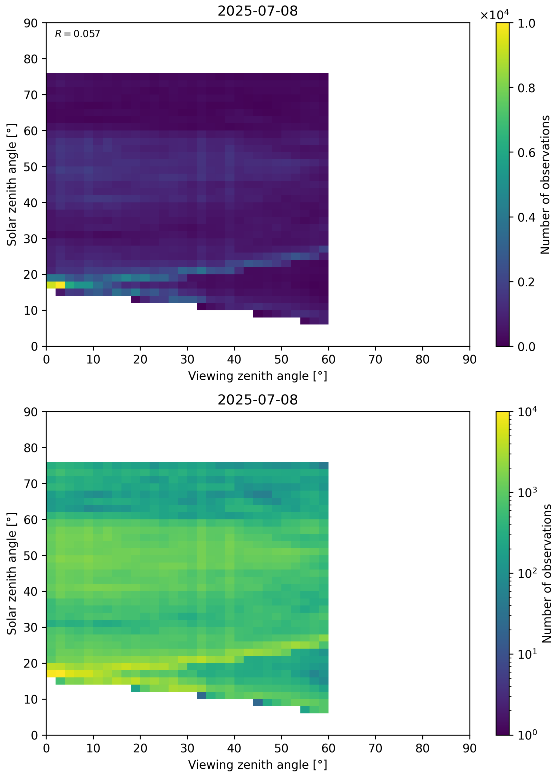
Figure 115: Scatter density plot of “Viewing zenith angle” against “Solar zenith angle” for 2025-07-08 to 2025-07-09.
