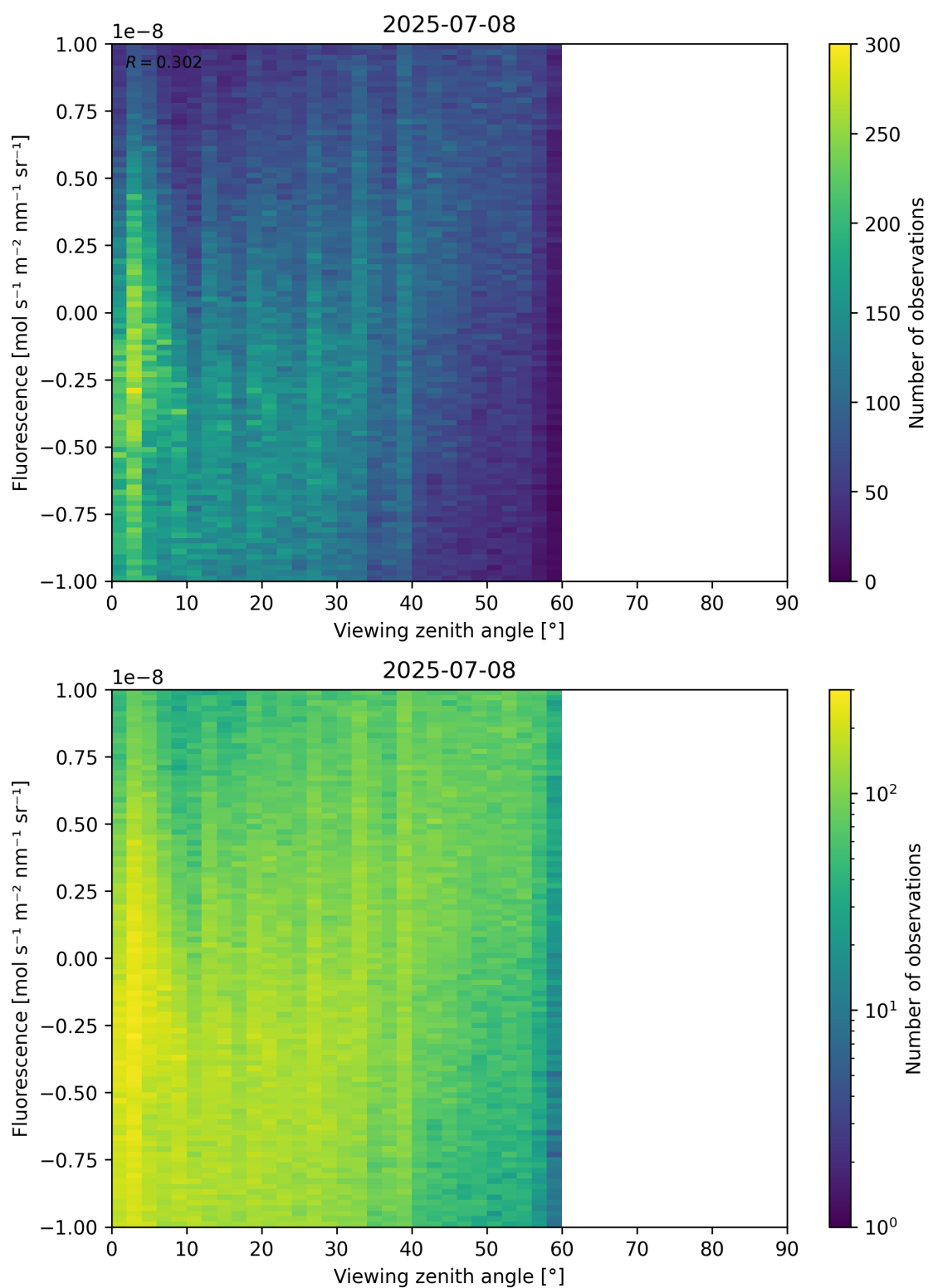
Figure 108: Scatter density plot of “Viewing zenith angle” against “Fluorescence” for 2025-07-08 to 2025-07-09.
