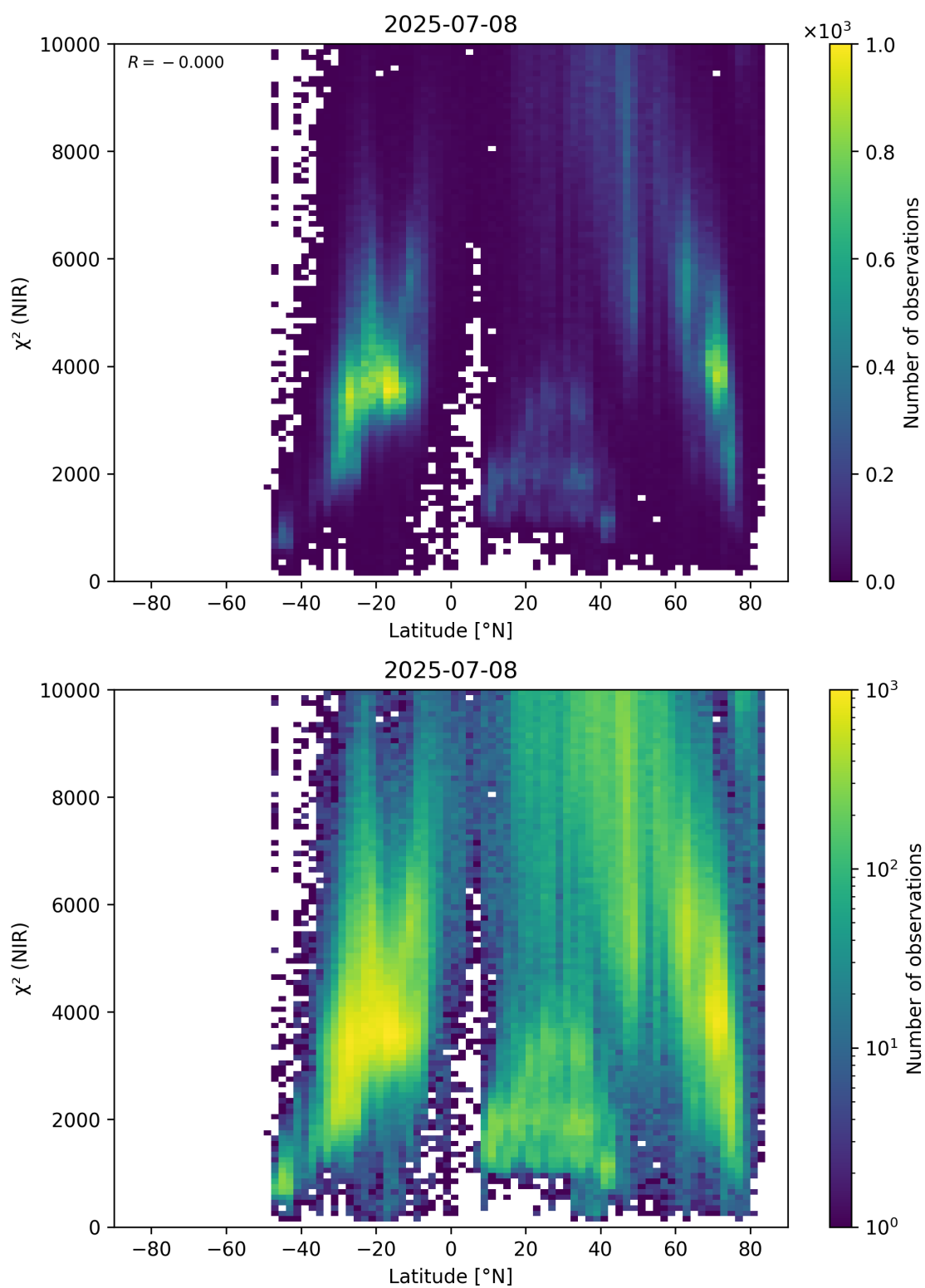
Figure 53: Scatter density plot of “Latitude” against “ \chi^2 (NIR)” for 2025-07-08 to 2025-07-09.
