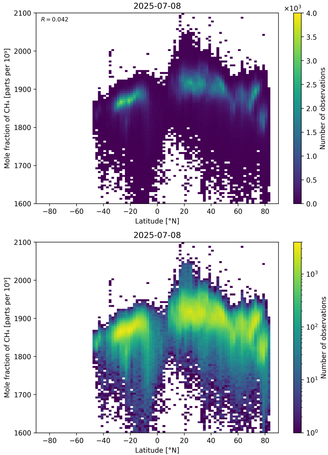
Figure 57: Scatter density plot of “Latitude” against “Mole fraction of CH 4 ” for 2025-07-08 to 2025-07-09.
