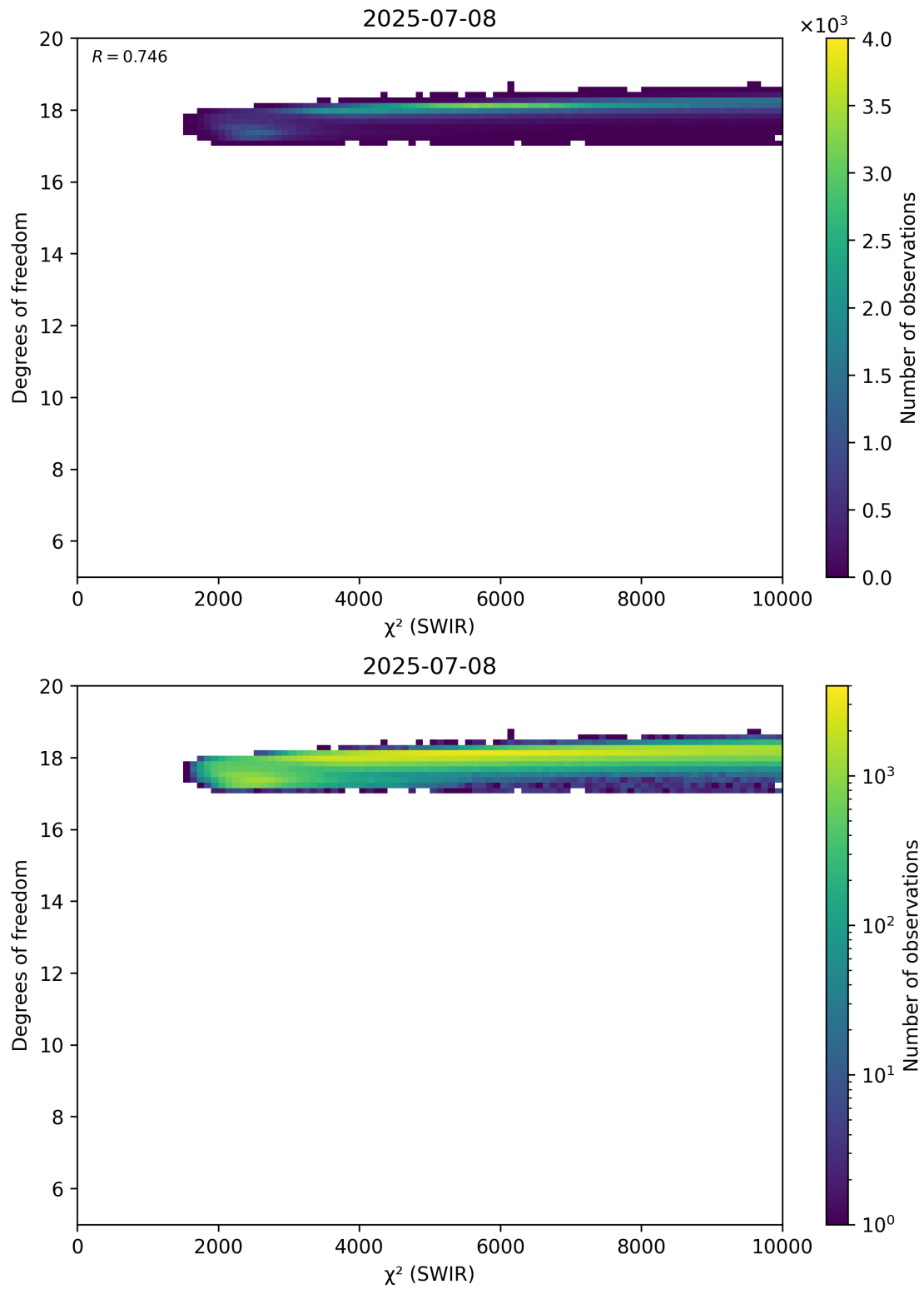
Figure 48: Scatter density plot of “ \chi^2 (SWIR)” against “Degrees of freedom” for 2025-07-08 to 2025-07-09.
