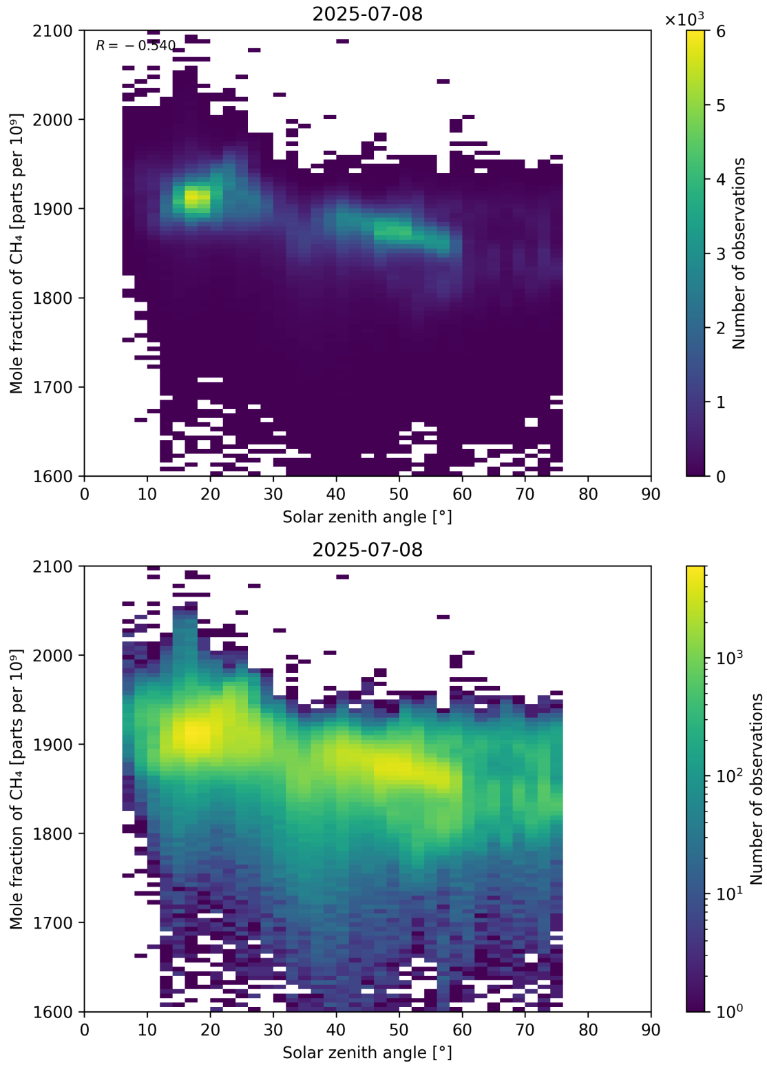
Figure 99: Scatter density plot of “Solar zenith angle” against “Mole fraction of CH 4 ” for 2025-07-08 to 2025-07-09.
