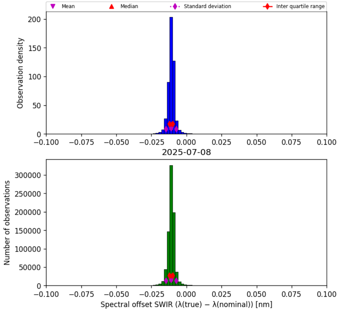
Figure 27: Histogram of “Spectral offset SWIR ( \lambda_{\text{true}} - \lambda_{\text{nominal}} )” for 2025-07-08 to 2025-07-09
