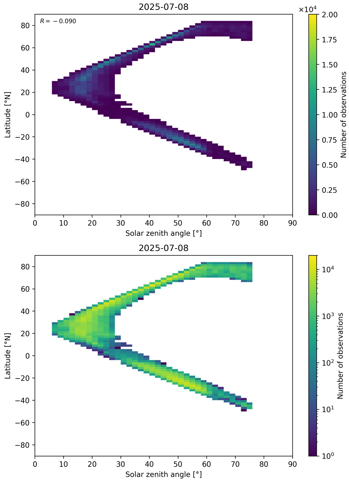
Figure 98: Scatter density plot of “Solar zenith angle” against “Latitude” for 2025-07-08 to 2025-07-09.
