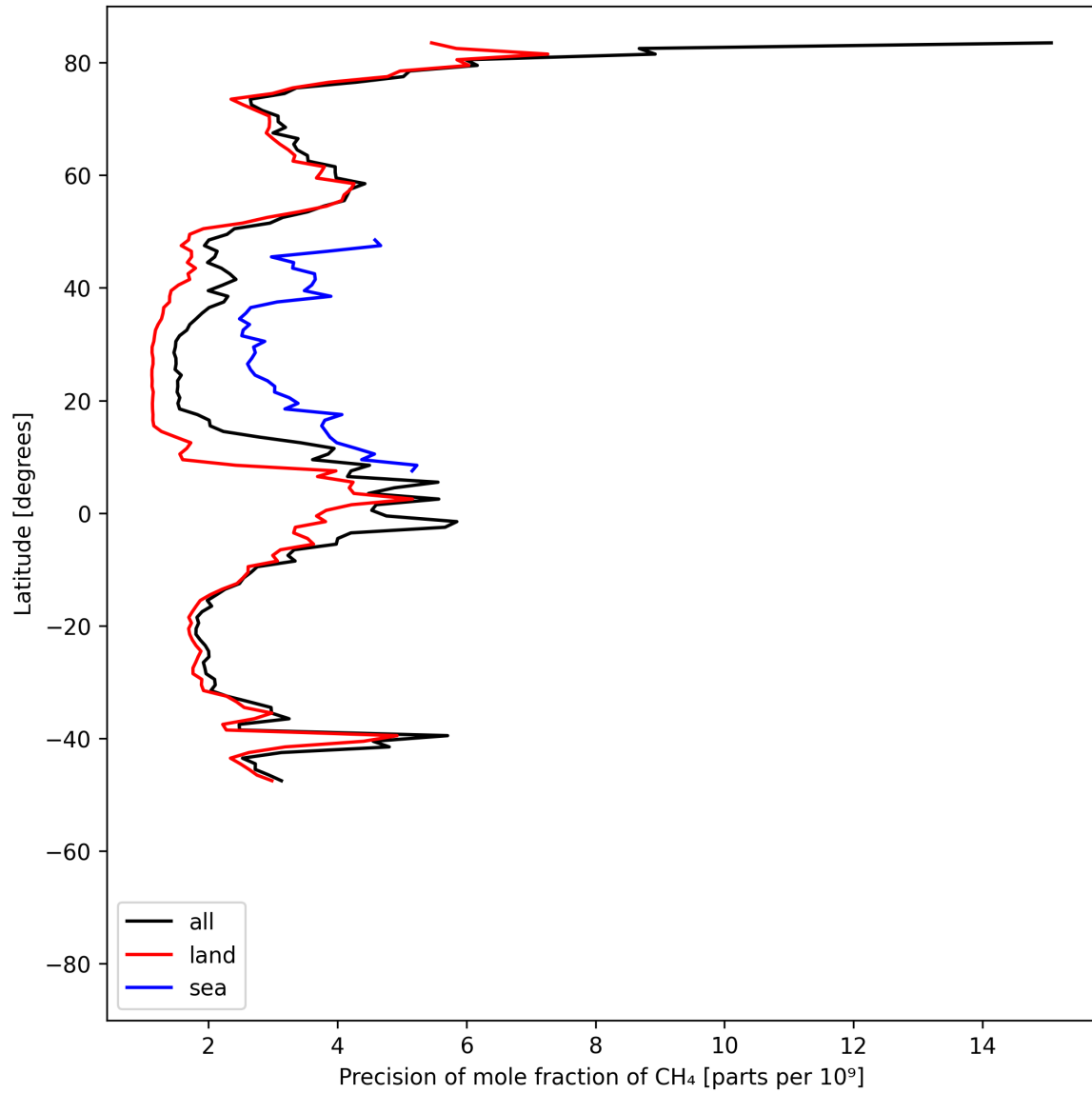
Figure 13: Zonal average of “Precision of mole fraction of CH 4 ” for 2025-07-08 to 2025-07-09.
