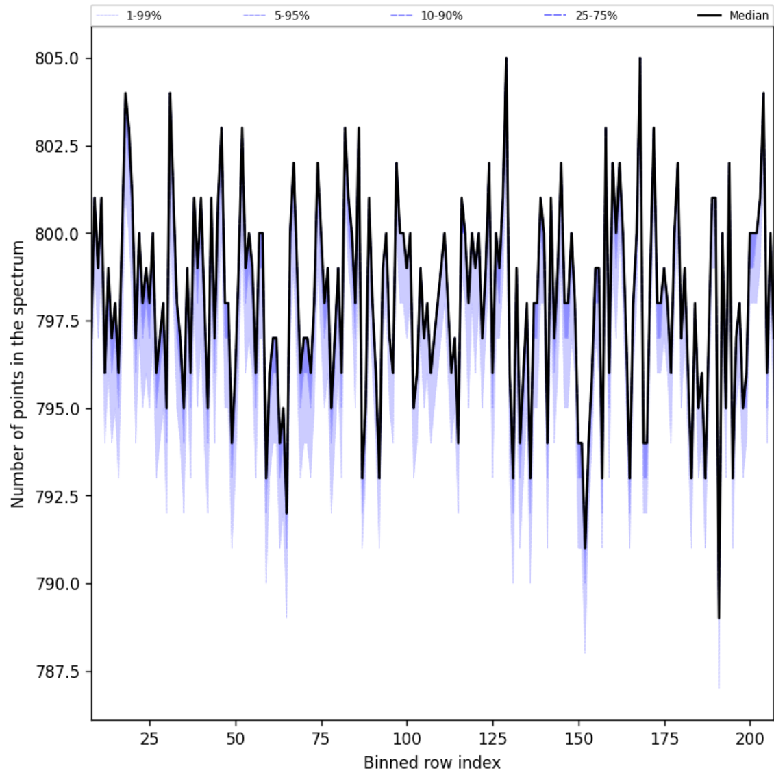
Figure 37: Along track statistics of “Number of points in the spectrum” for 2025-07-08 to 2025-07-09
