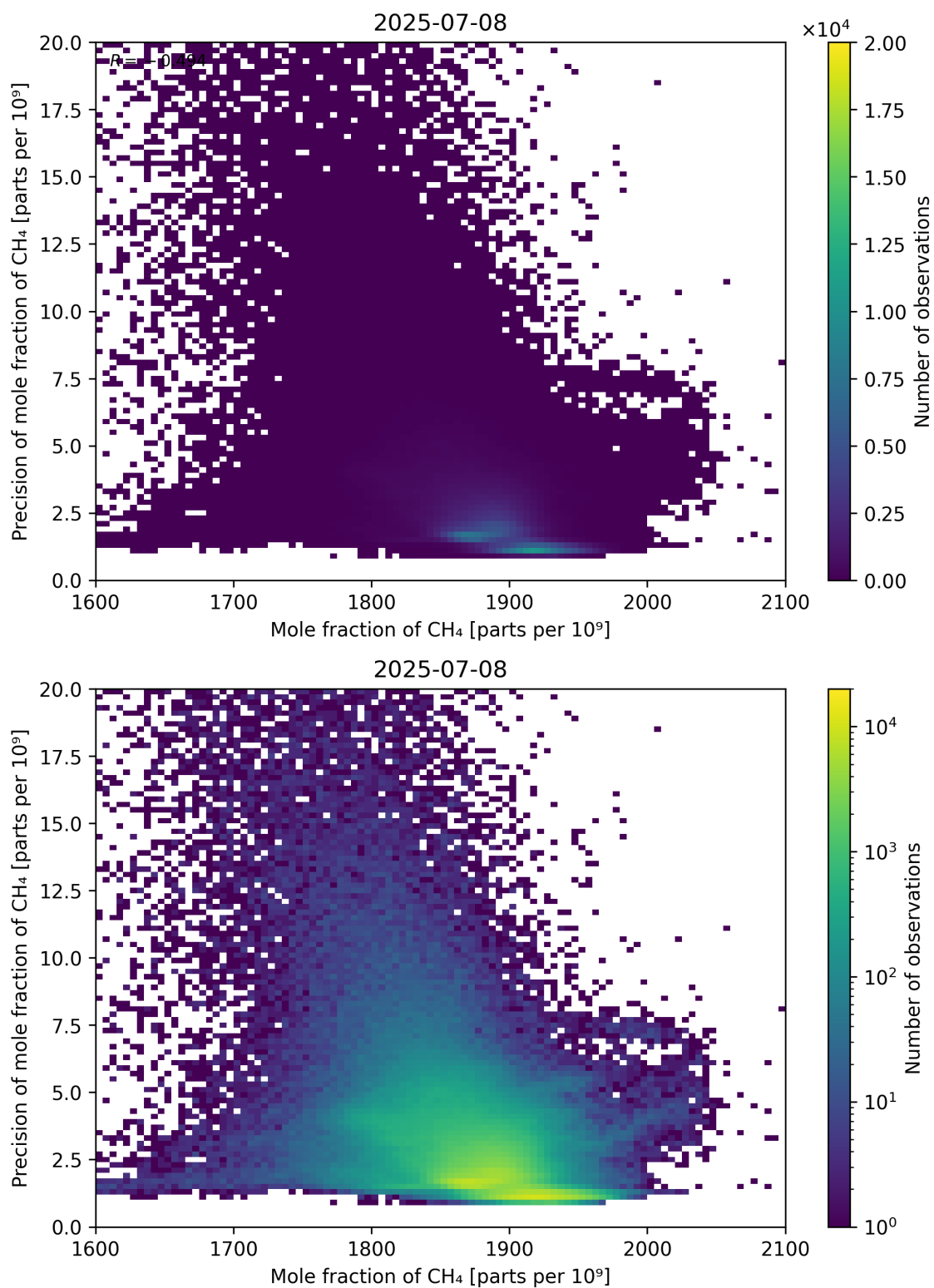
Figure 75: Scatter density plot of “Mole fraction of CH 4 ” against “Precision of mole fraction of CH 4 ” for 2025-07-08 to 2025-07-09.
