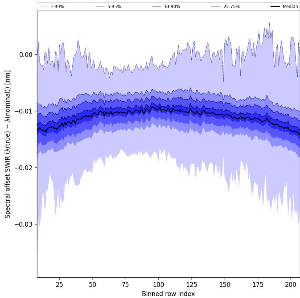
Figure 38: Along track statistics of “Spectral offset SWIR ( \lambda_{\text{true}} - \lambda_{\text{nominal}} )” for 2025-07-08 to 2025-07-09
