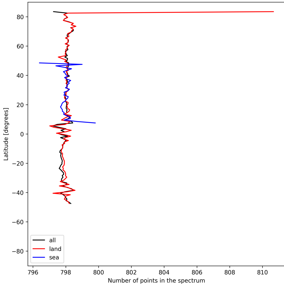
Figure 15: Zonal average of “Number of points in the spectrum” for 2025-07-08 to 2025-07-09.
