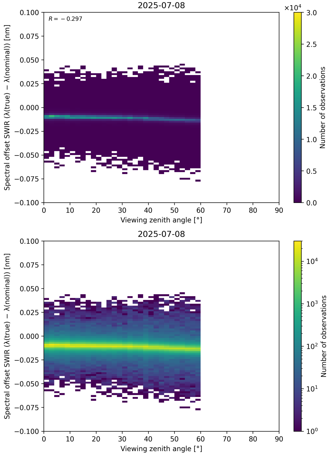
Figure 116: Scatter density plot of “Viewing zenith angle” against “Spectral offset SWIR ( \lambda_{\text{true}} - \lambda_{\text{nominal}} )” for 2025-07-08 to 2025-07-09.
