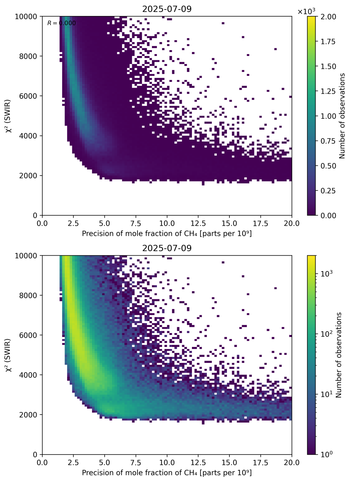
Figure 79: Scatter density plot of “Precision of mole fraction of CH 4 ” against “ \chi^2 (SWIR)” for 2025-07-08 to 2025-07-10.
