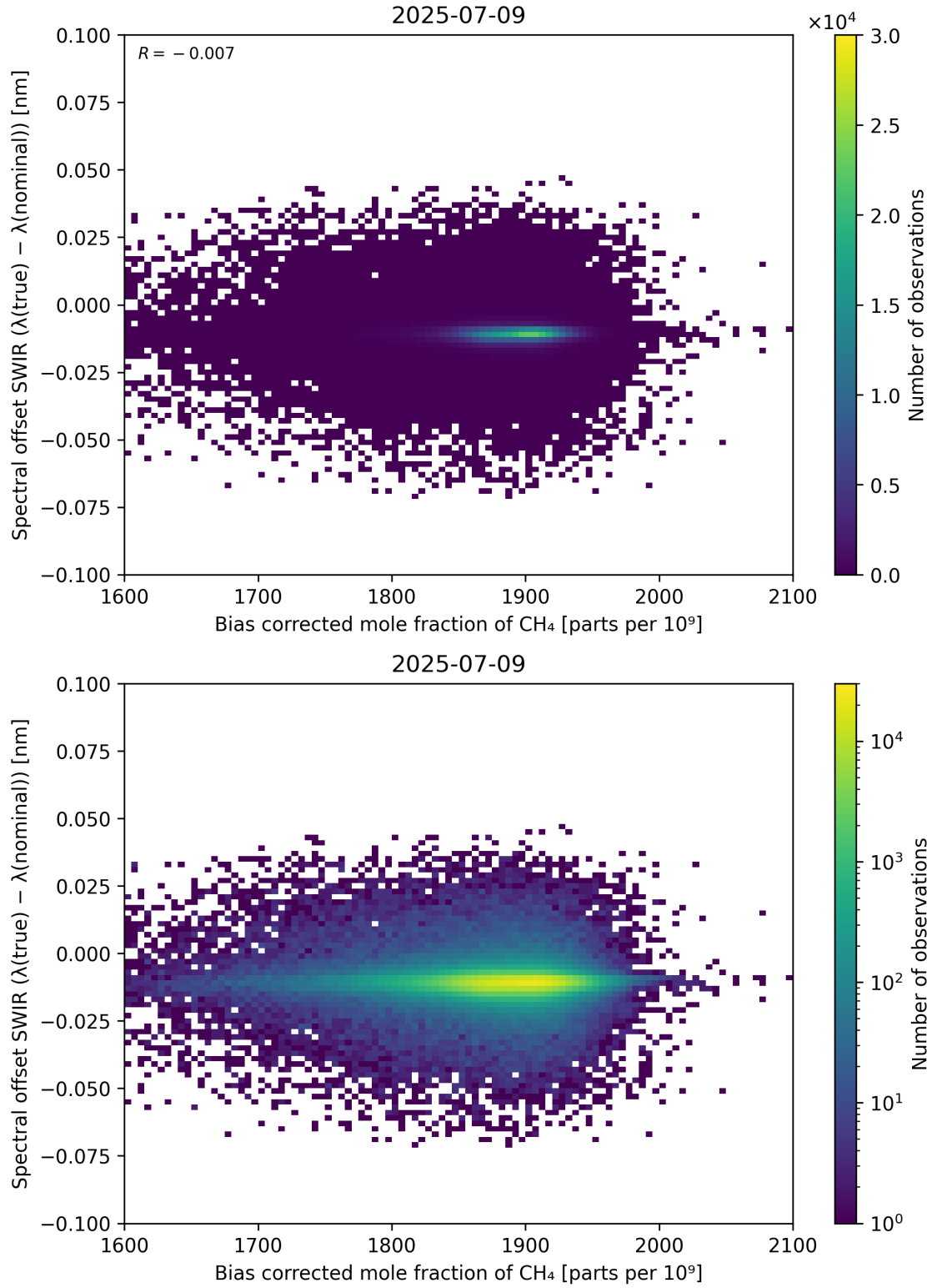
Figure 69: Scatter density plot of “Bias corrected mole fraction of CH 4 ” against “Spectral offset SWIR ( \lambda_{\text{true}} - \lambda_{\text{nominal}} )” for 2025-07-08 to 2025-07-10.
