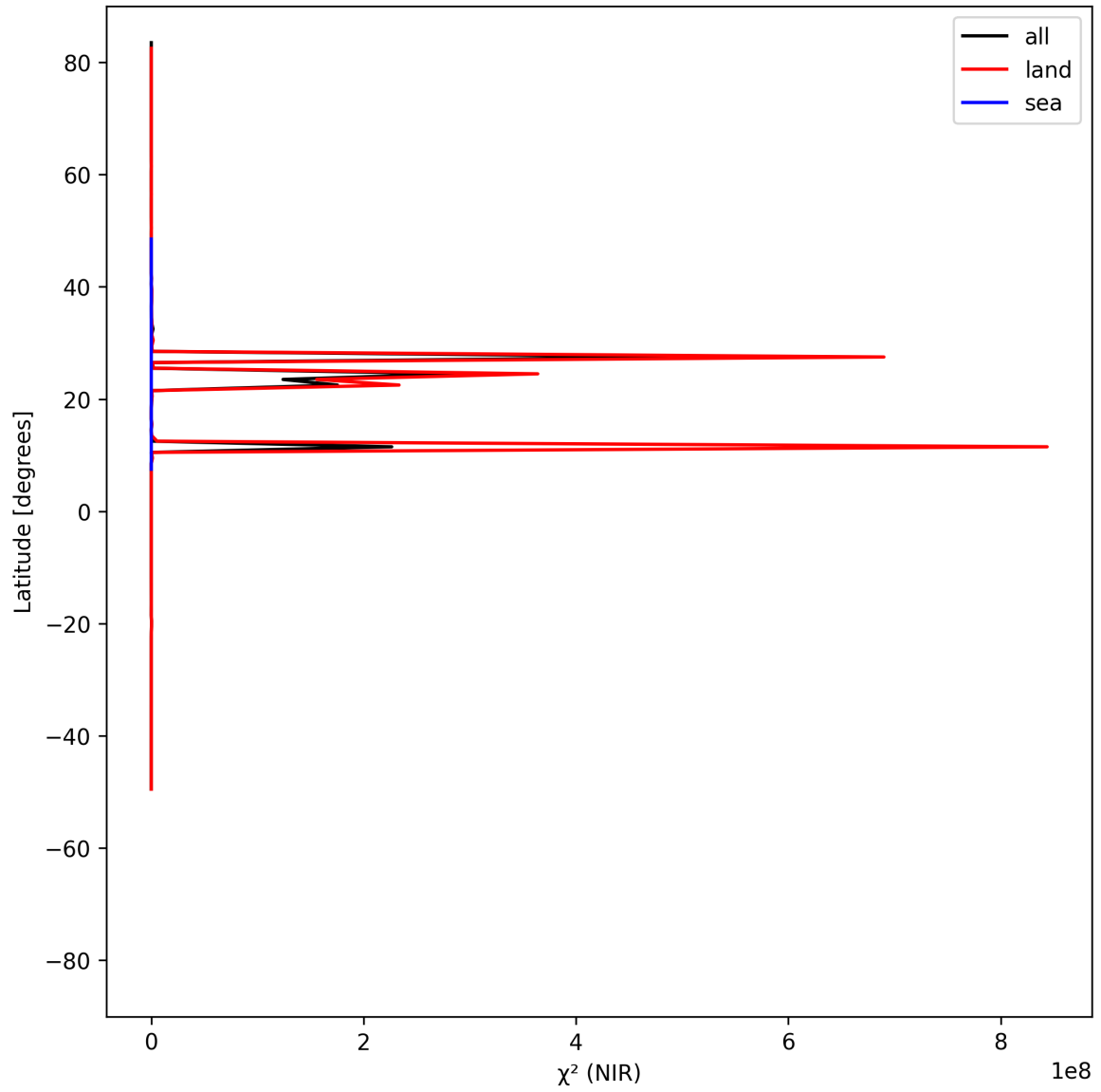
Figure 18: Zonal average of “ \chi^2 (NIR)” for 2025-07-08 to 2025-07-10.
