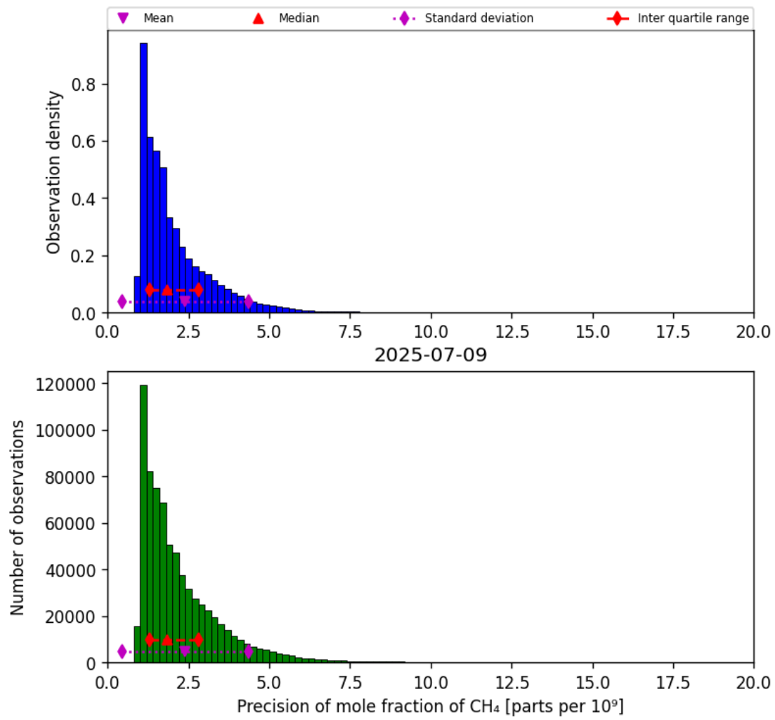
Figure 24: Histogram of “Precision of mole fraction of CH 4 ” for 2025-07-08 to 2025-07-10
