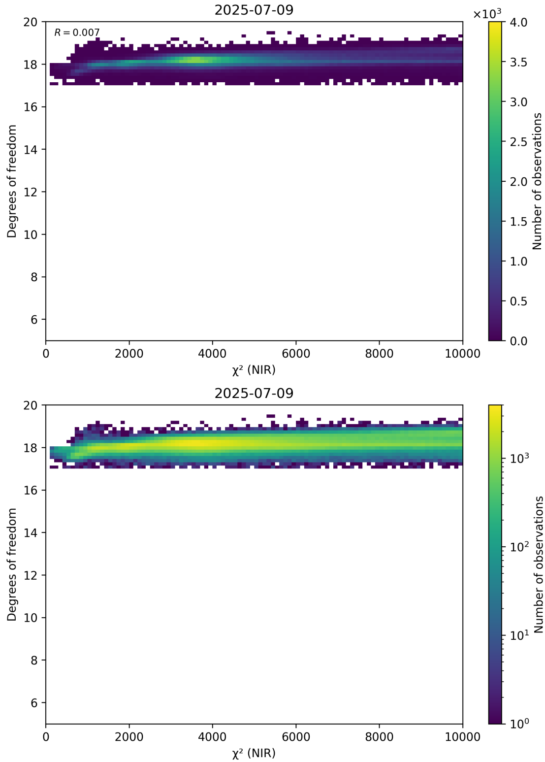
Figure 44: Scatter density plot of “ \chi^2 (NIR)” against “Degrees of freedom” for 2025-07-08 to 2025-07-10.
