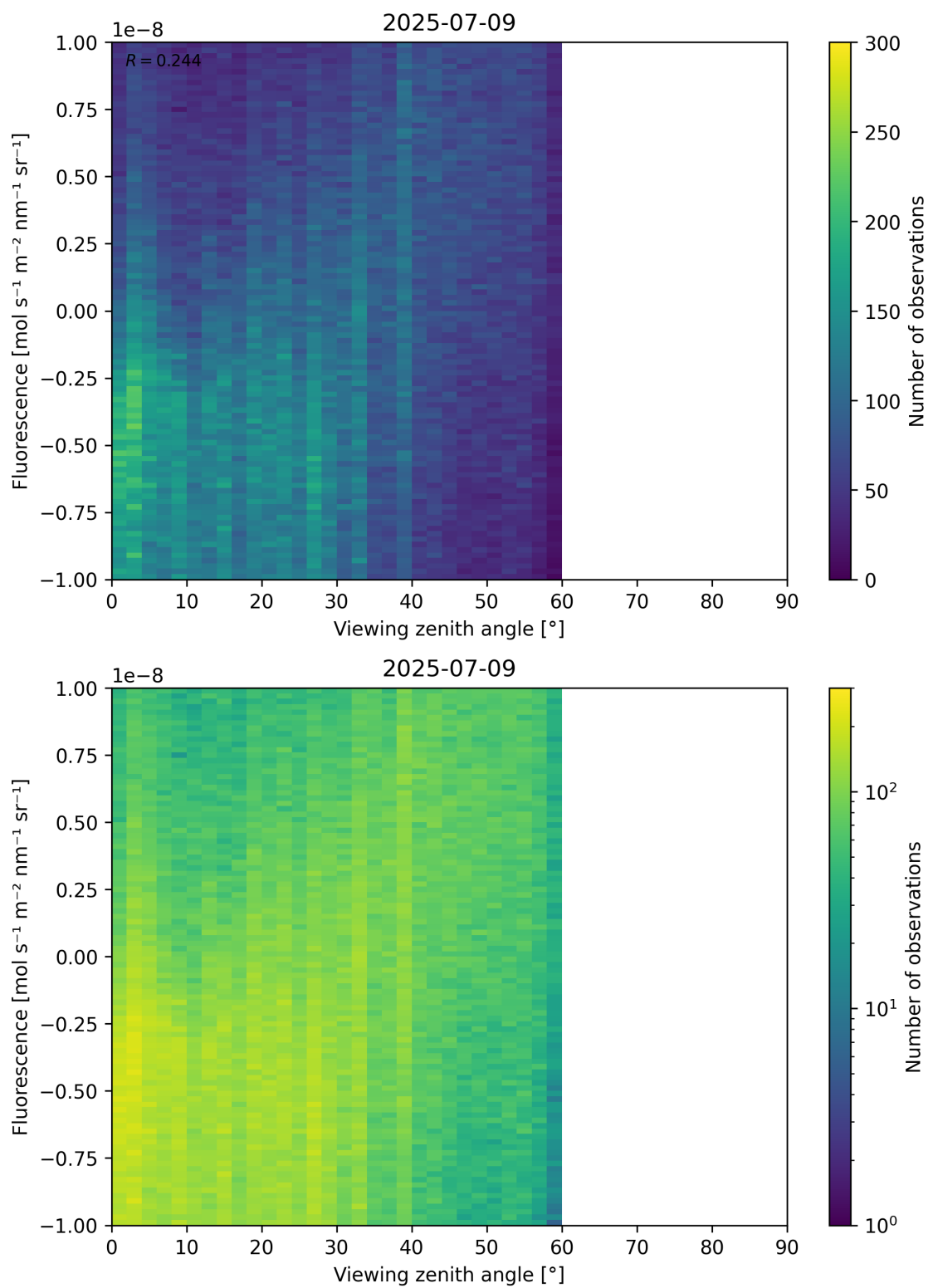
Figure 108: Scatter density plot of “Viewing zenith angle” against “Fluorescence” for 2025-07-08 to 2025-07-10.
