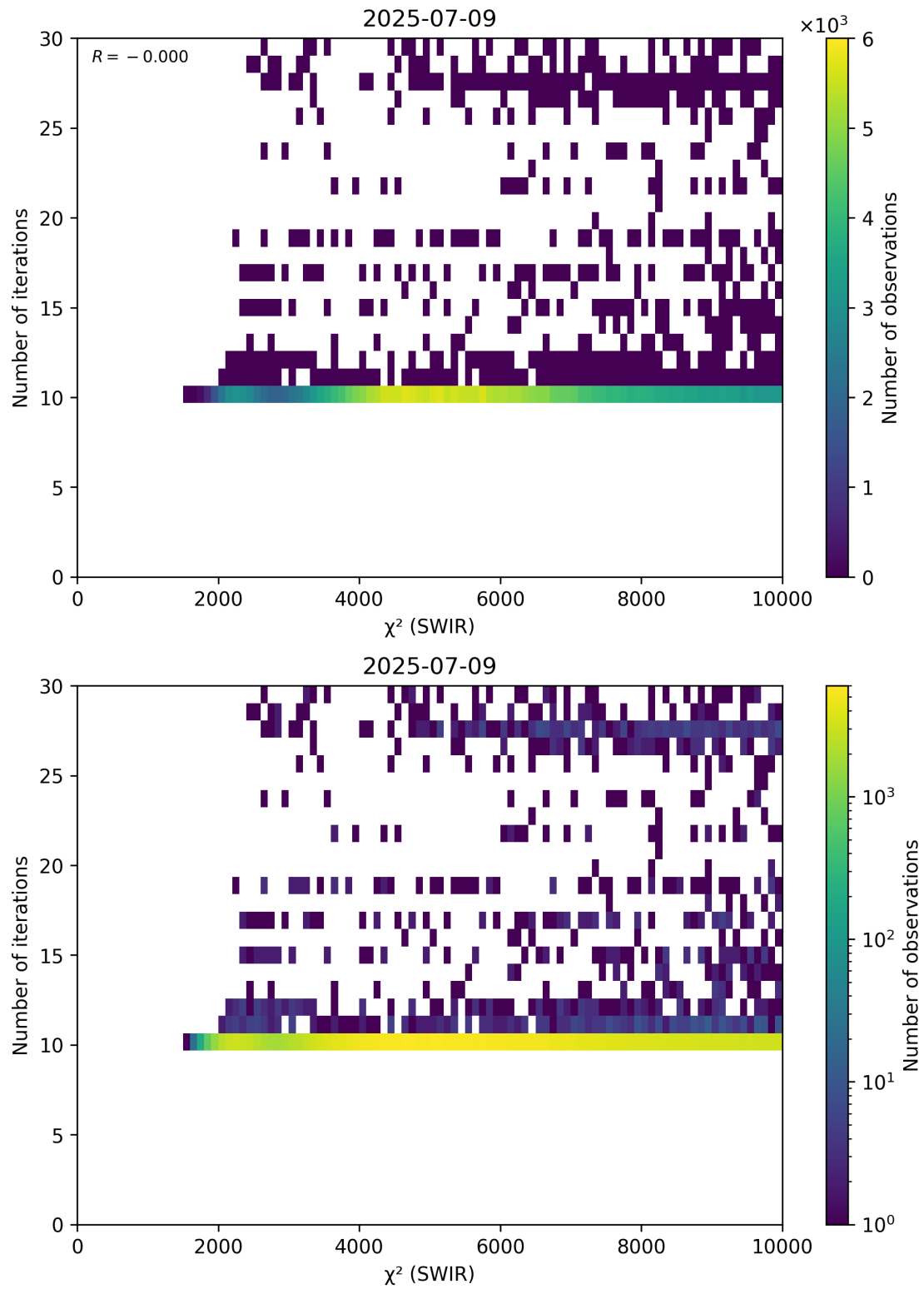
Figure 50: Scatter density plot of “ \chi^2 (SWIR)” against “Number of iterations” for 2025-07-08 to 2025-07-10.
