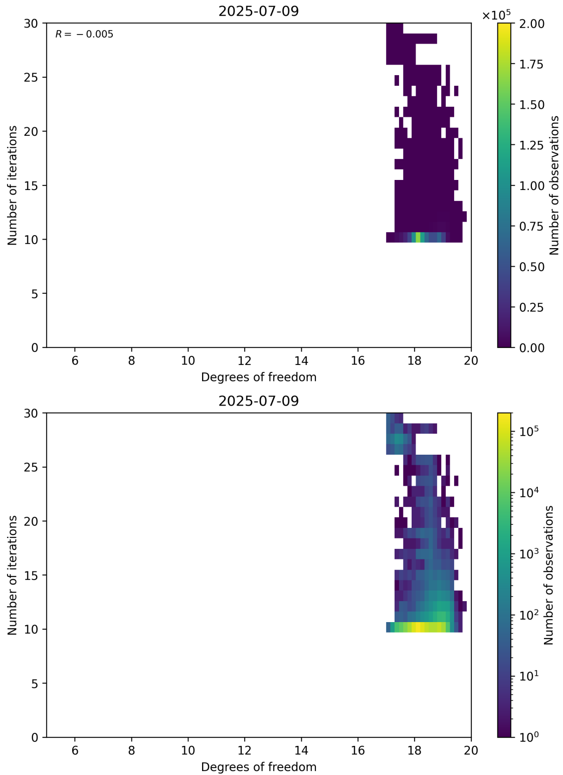
Figure 52: Scatter density plot of “Degrees of freedom” against “Number of iterations” for 2025-07-08 to 2025-07-10.
