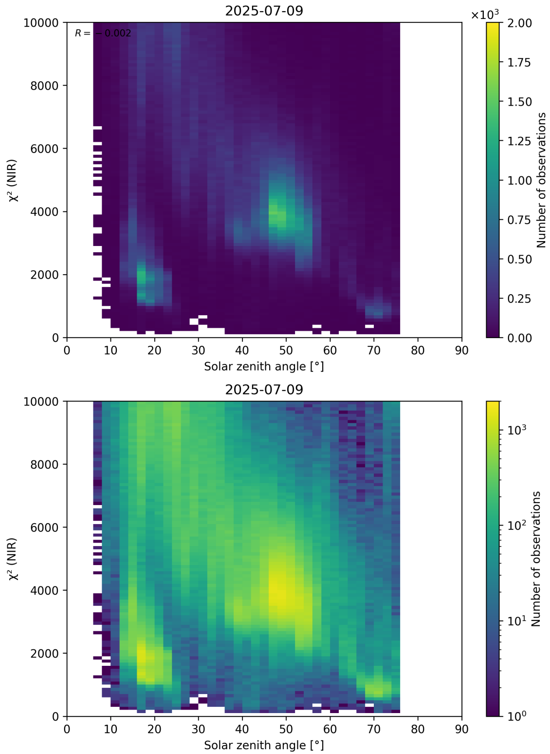
Figure 94: Scatter density plot of “Solar zenith angle” against “ \chi^2 (NIR)” for 2025-07-08 to 2025-07-10.
