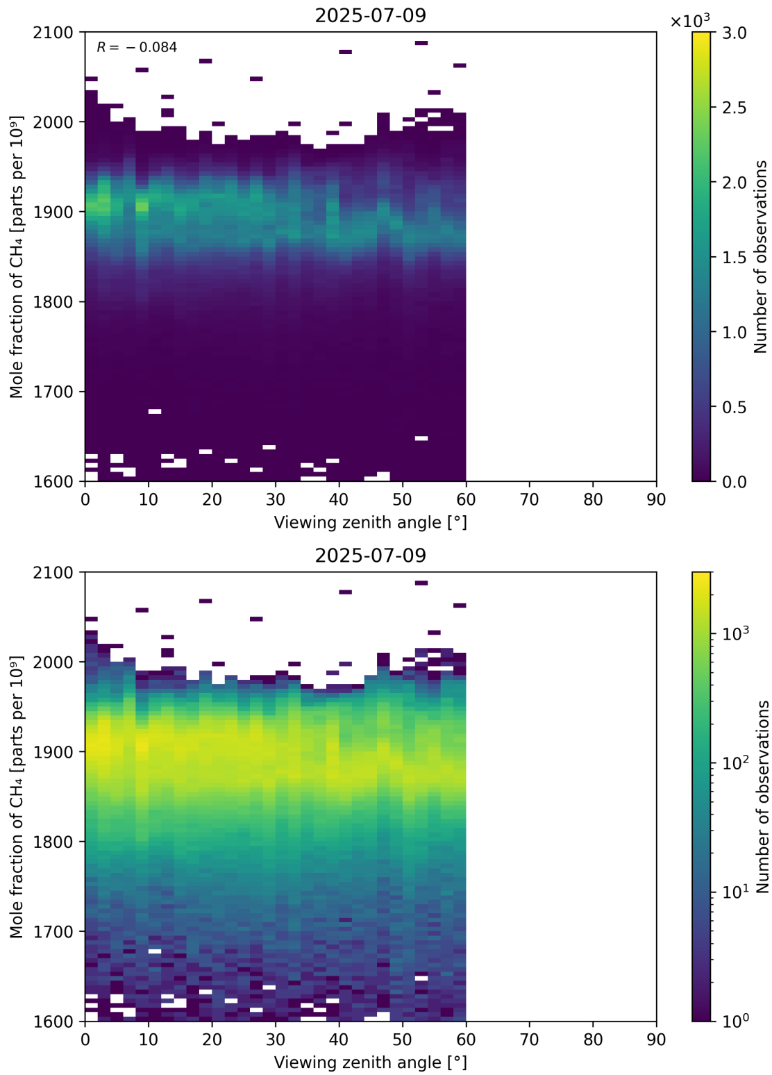
Figure 110: Scatter density plot of “Viewing zenith angle” against “Mole fraction of CH 4 ” for 2025-07-08 to 2025-07-10.
