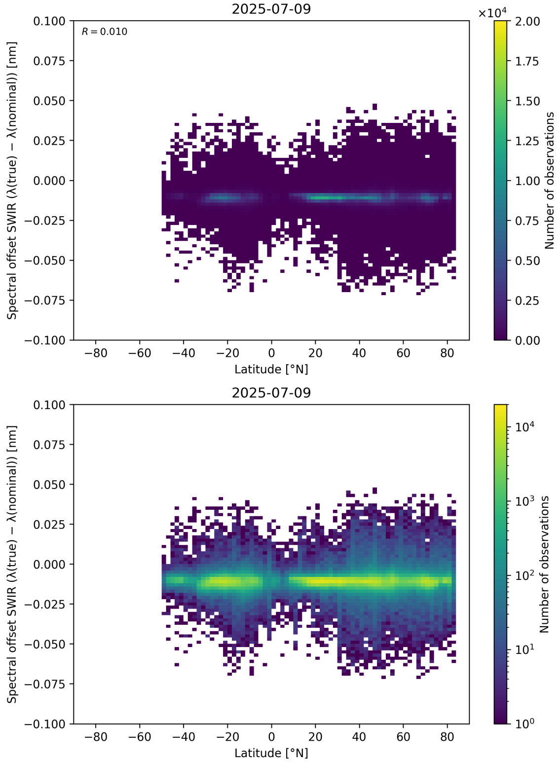
Figure 62: Scatter density plot of “Latitude” against “Spectral offset SWIR ( \lambda_{\text{true}} - \lambda_{\text{nominal}} )” for 2025-07-08 to 2025-07-10.
