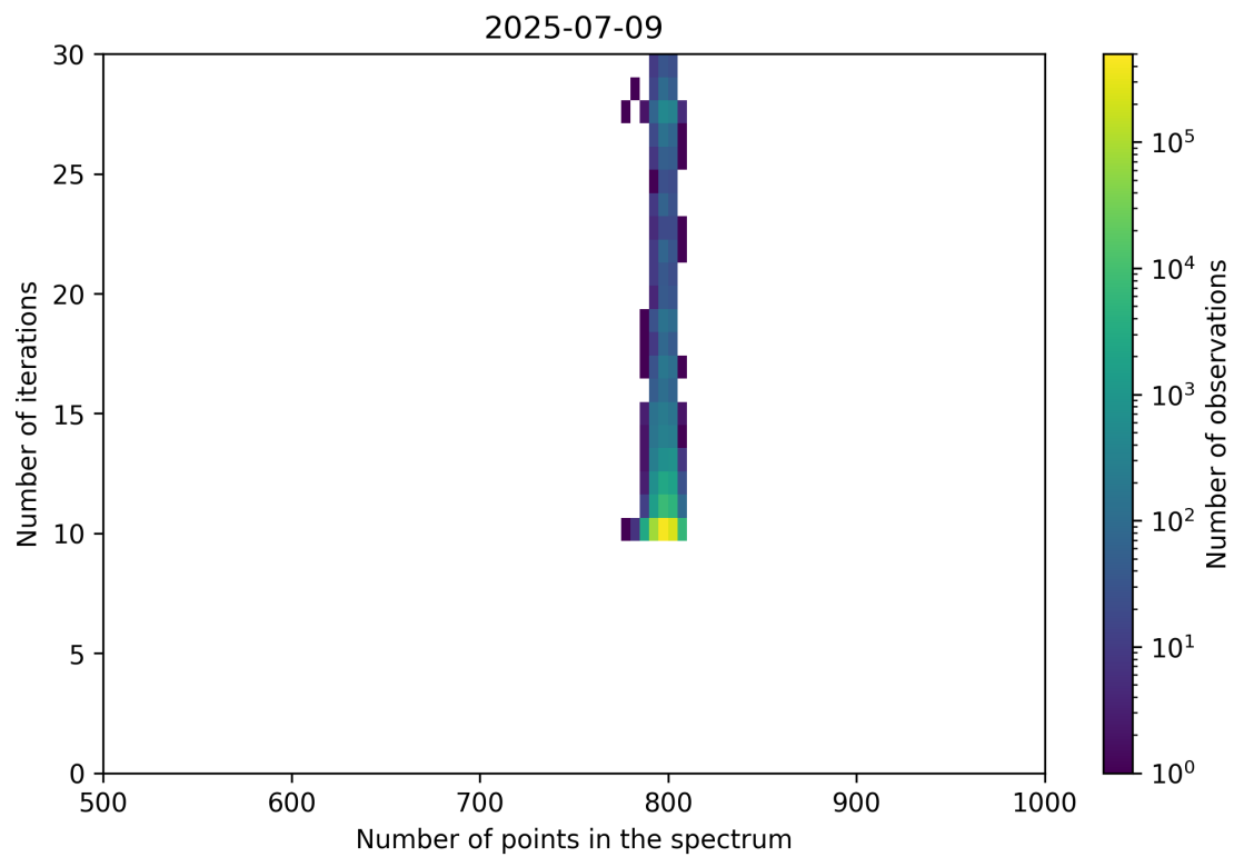
Figure 92: Scatter density plot of “Number of points in the spectrum” against “Number of iterations” for 2025-07-08 to 2025-07-10.
