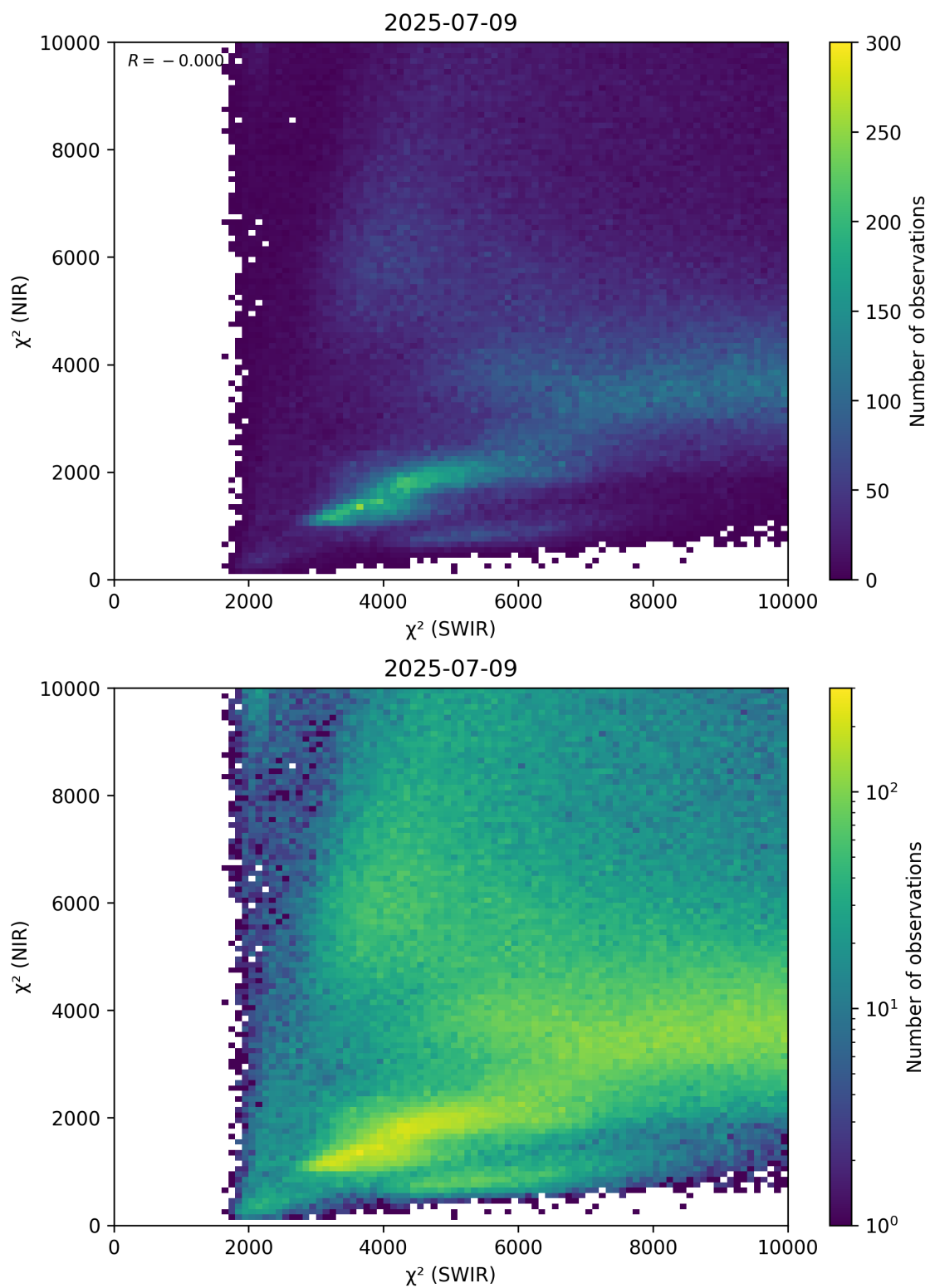
Figure 47: Scatter density plot of “ \chi^2 (SWIR)” against “ \chi^2 (NIR)” for 2025-07-08 to 2025-07-10.
