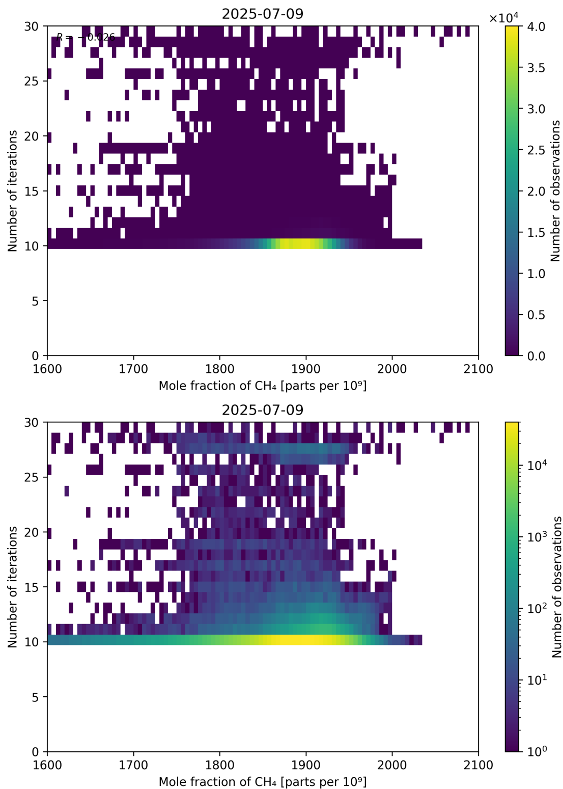
Figure 76: Scatter density plot of “Mole fraction of CH 4 ” against “Number of iterations” for 2025-07-08 to 2025-07-10.
