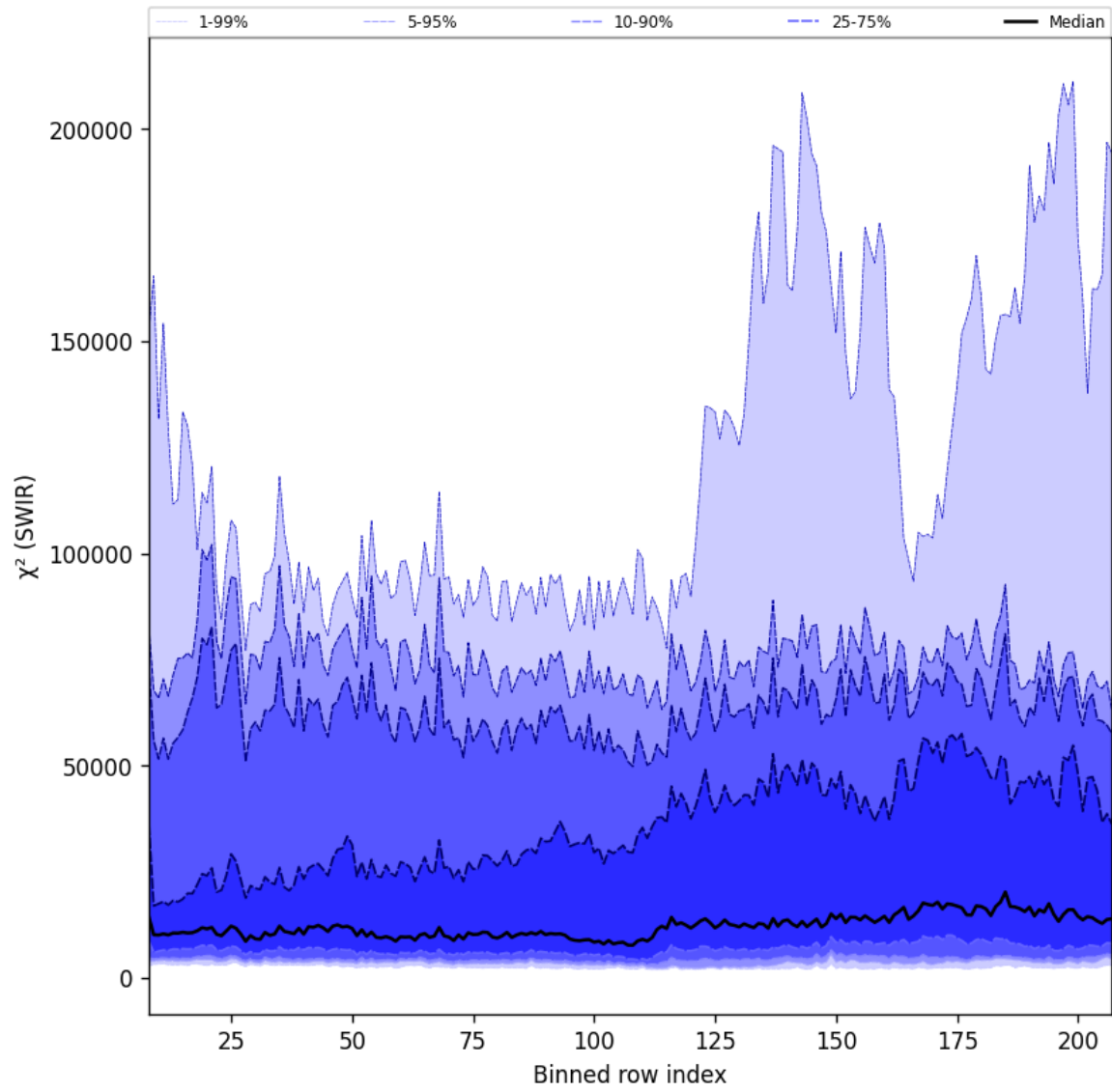
Figure 39: Along track statistics of " \chi^2 (SWIR)" for 2025-07-08 to 2025-07-10
