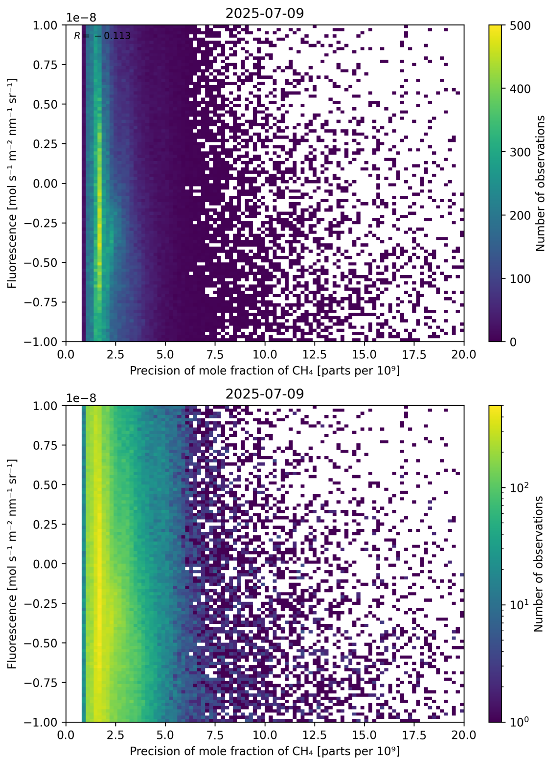
Figure 81: Scatter density plot of “Precision of mole fraction of CH 4 ” against “Fluorescence” for 2025-07-08 to 2025-07-10.
