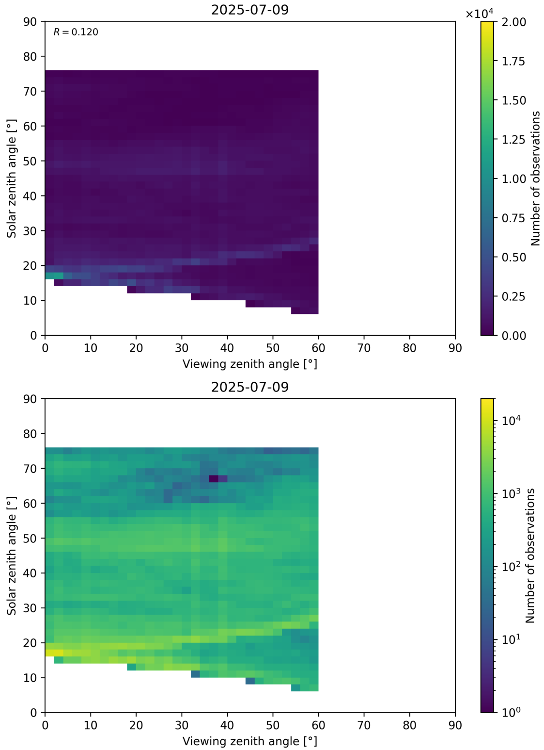
Figure 115: Scatter density plot of “Viewing zenith angle” against “Solar zenith angle” for 2025-07-08 to 2025-07-10.
