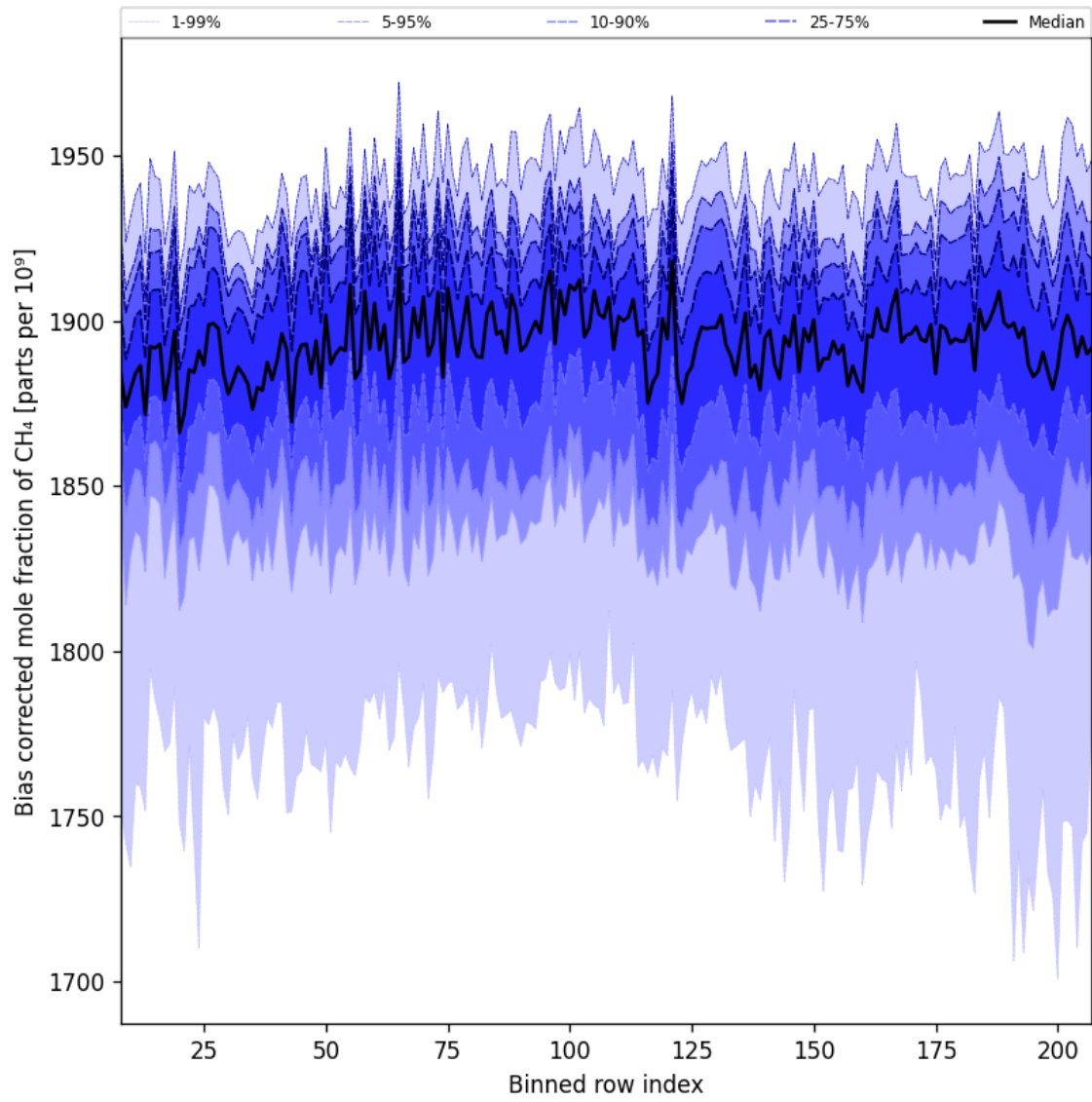
Figure 36: Along track statistics of “Bias corrected mole fraction of CH 4 ” for 2025-07-08 to 2025-07-10
