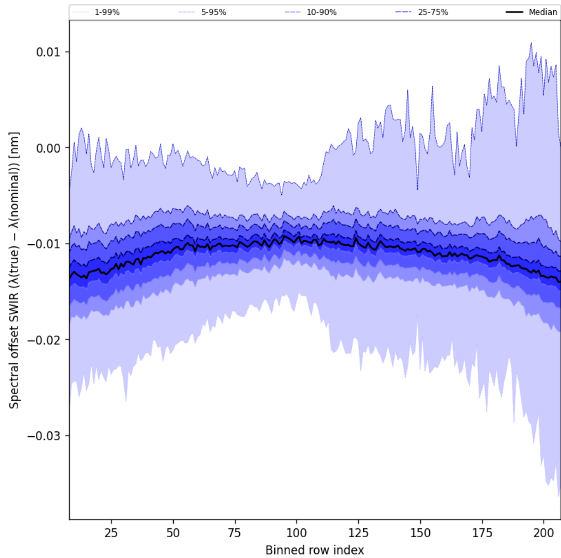
Figure 38: Along track statistics of “Spectral offset SWIR ( \lambda_{\text{true}} - \lambda_{\text{nominal}} )” for 2025-07-08 to 2025-07-10
