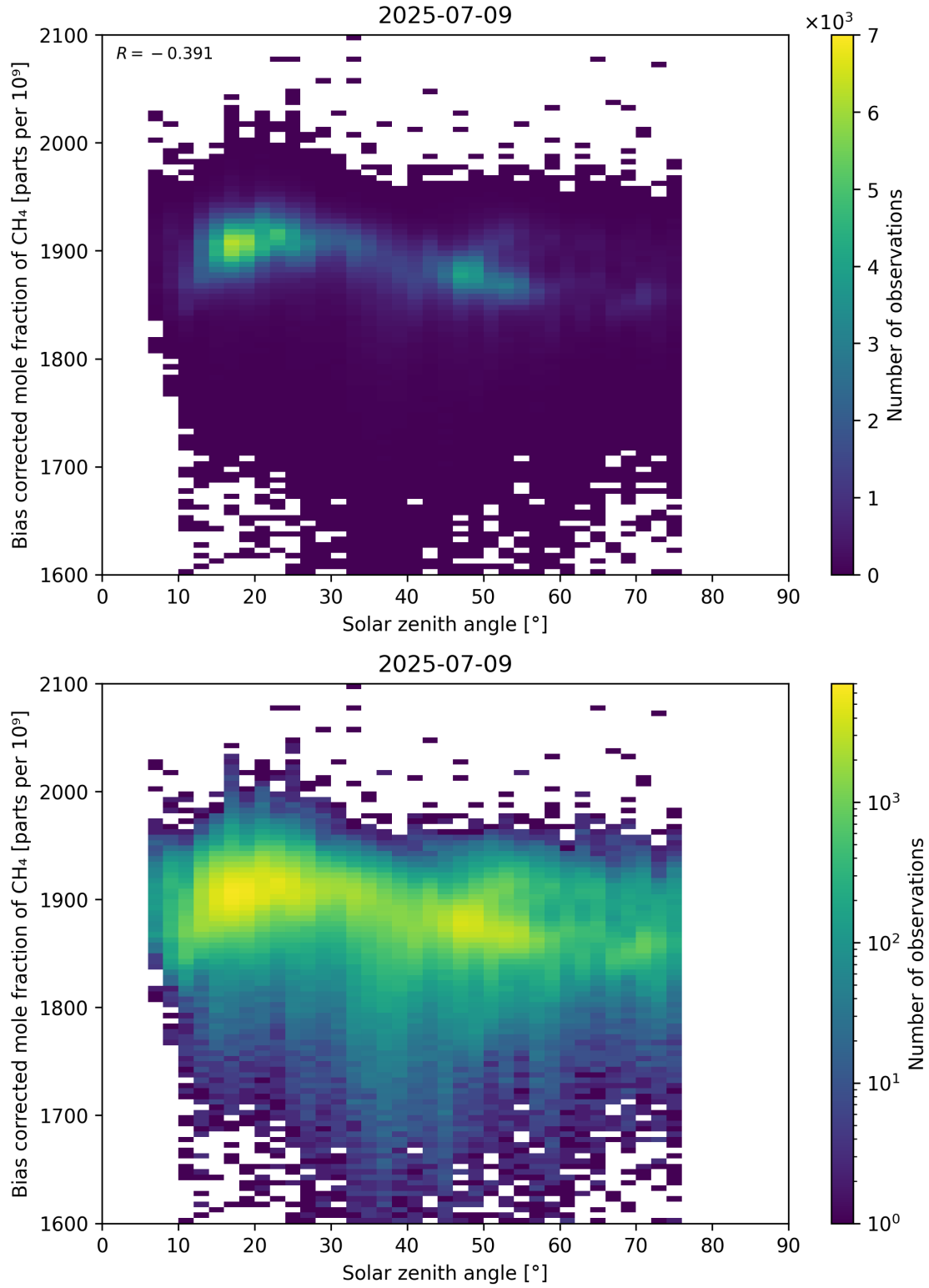
Figure 100: Scatter density plot of “Solar zenith angle” against “Bias corrected mole fraction of CH 4 ” for 2025-07-08 to 2025-07-10.
