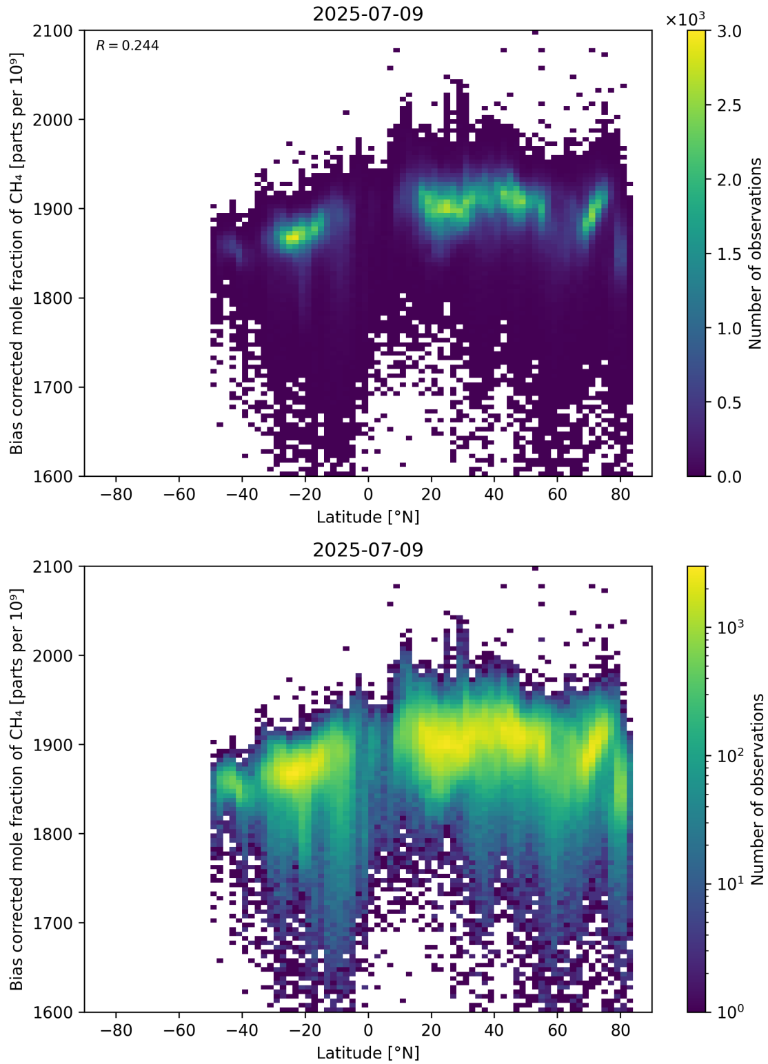
Figure 58: Scatter density plot of “Latitude” against “Bias corrected mole fraction of \text{CH}_4 ” for 2025-07-08 to 2025-07-10.
