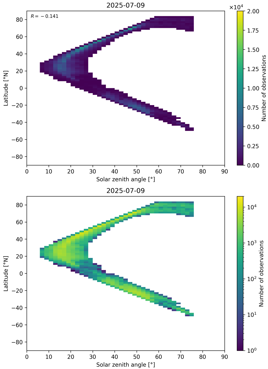
Figure 98: Scatter density plot of “Solar zenith angle” against “Latitude” for 2025-07-08 to 2025-07-10.
