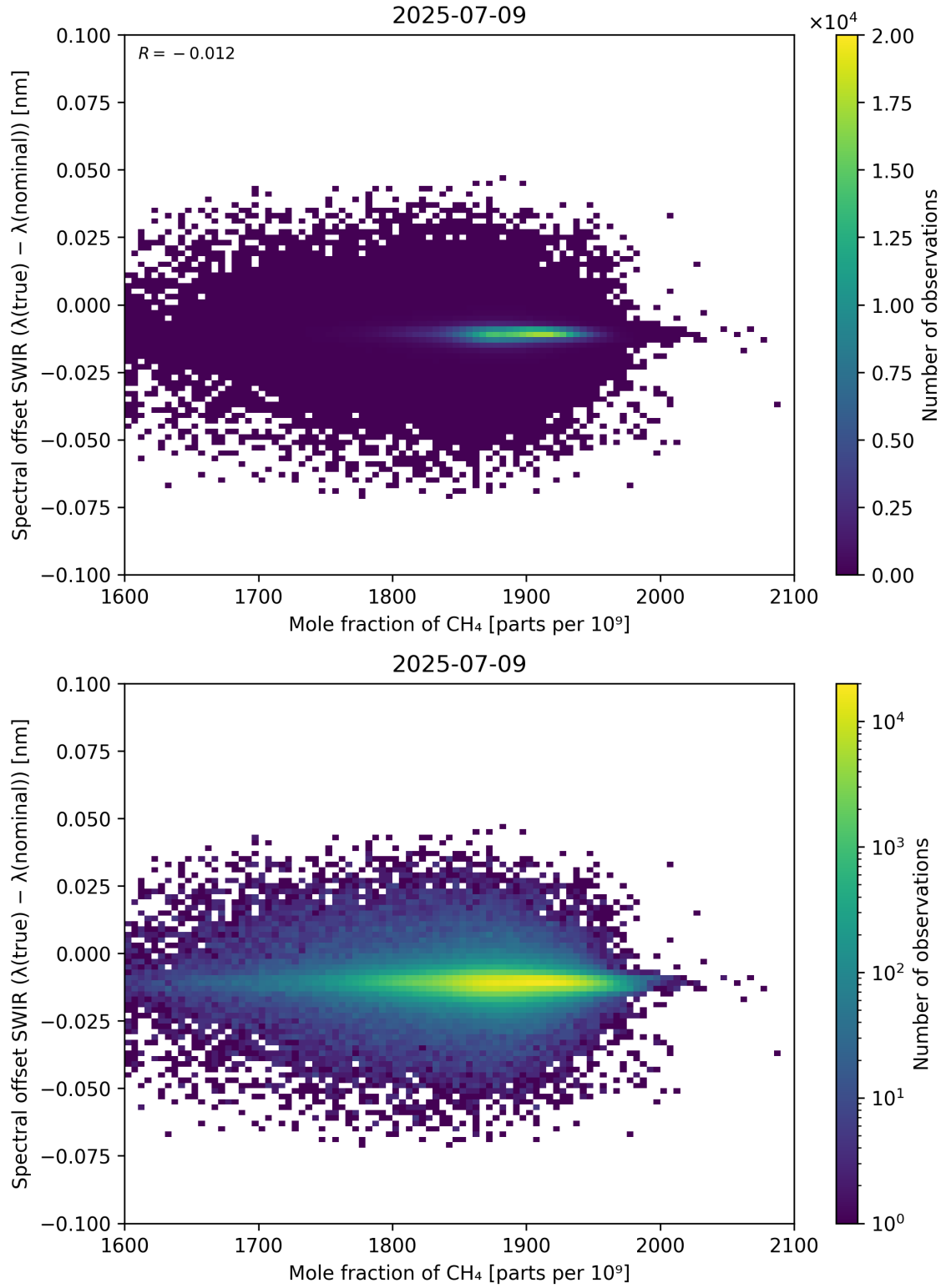
Figure 86: Scatter density plot of “Mole fraction of CH 4 ” against “Spectral offset SWIR ( \lambda_{\text{true}} - \lambda_{\text{nominal}} )” for 2025-07-08 to 2025-07-10.
