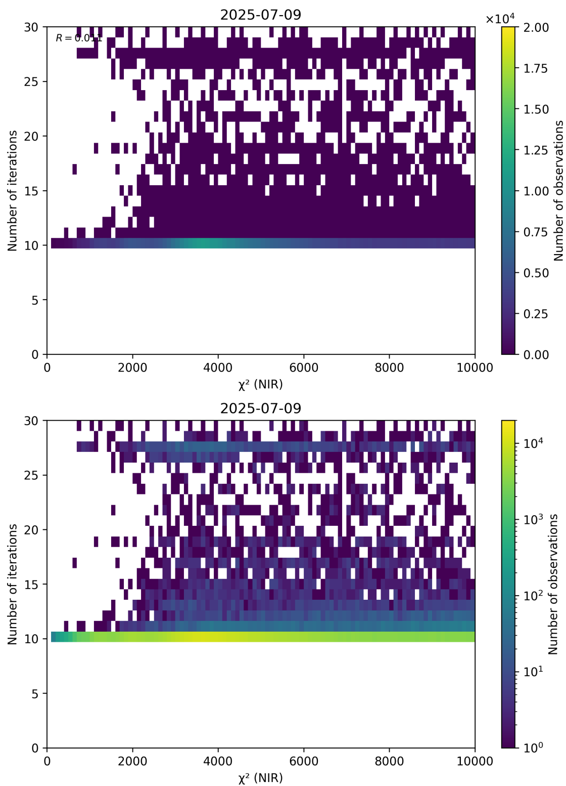
Figure 46: Scatter density plot of “ \chi^2 (NIR)” against “Number of iterations” for 2025-07-08 to 2025-07-10.
