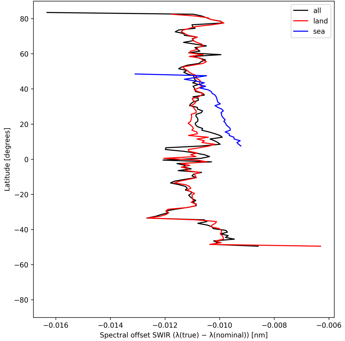
Figure 16: Zonal average of “Spectral offset SWIR ( \lambda_{\text{true}} - \lambda_{\text{nominal}} )” for 2025-07-08 to 2025-07-10.
