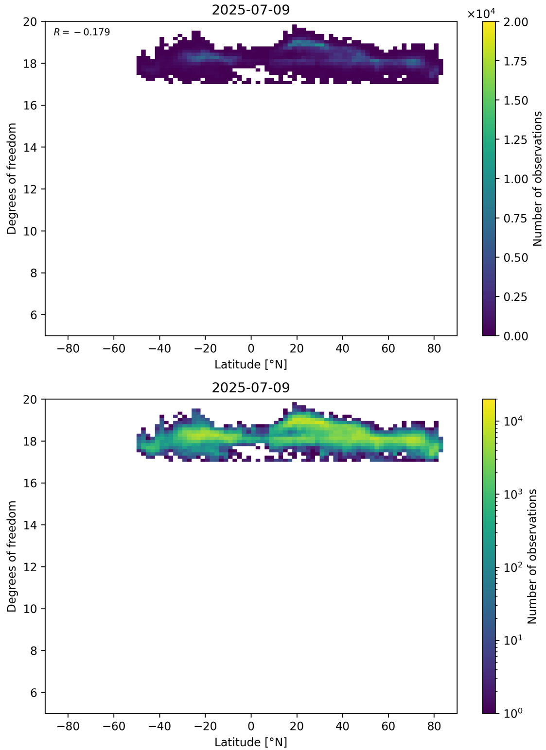
Figure 55: Scatter density plot of “Latitude” against “Degrees of freedom” for 2025-07-08 to 2025-07-10.
