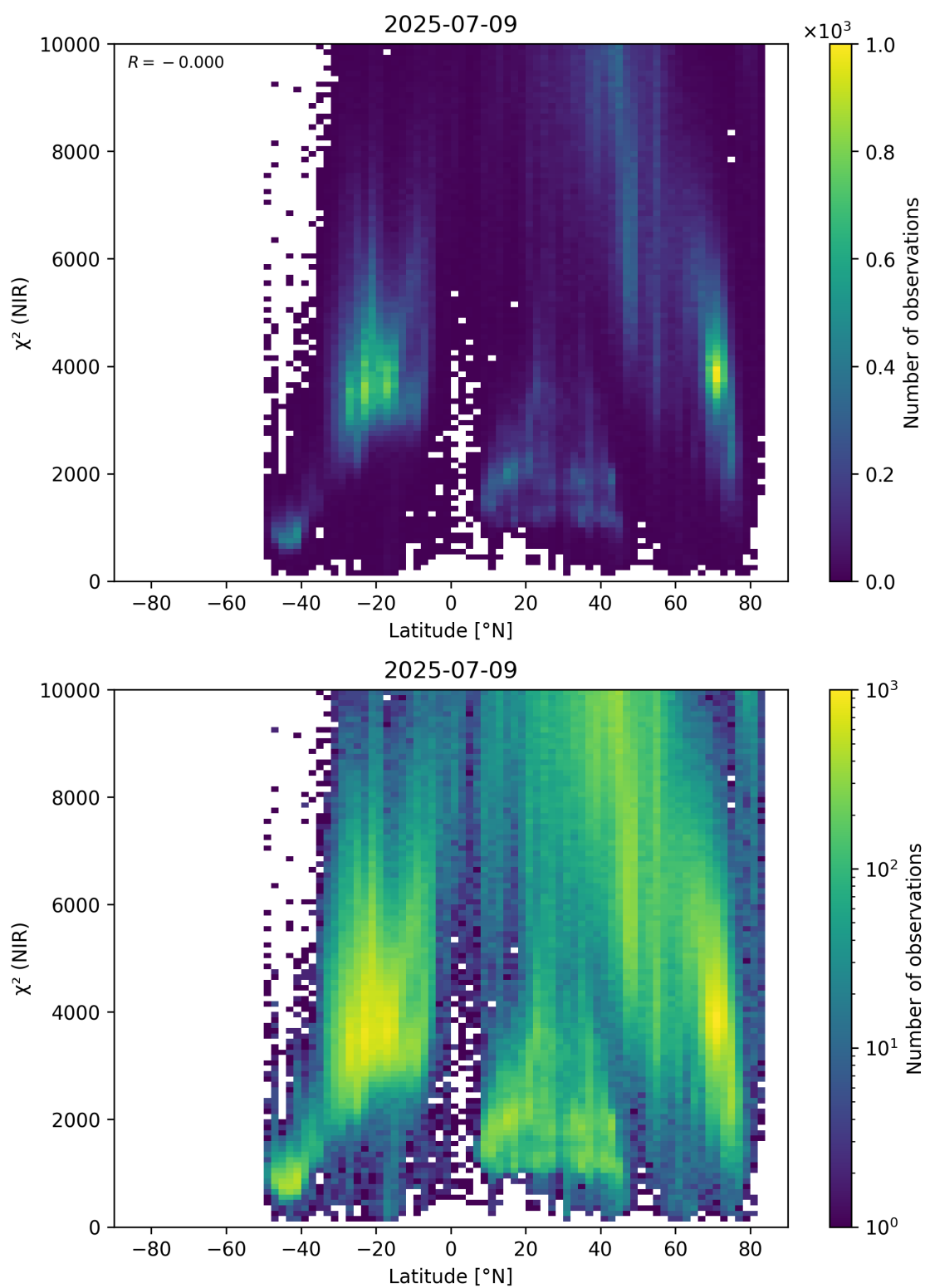
Figure 53: Scatter density plot of “Latitude” against “ \chi^2 (NIR)” for 2025-07-08 to 2025-07-10.
