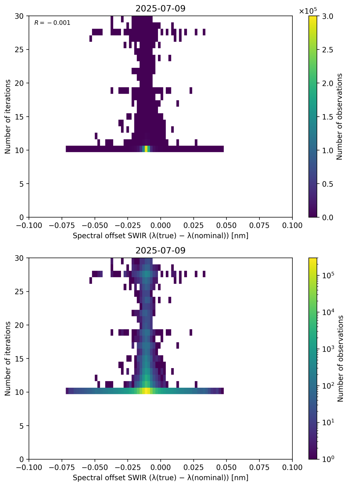
Figure 121: Scatter density plot of “Spectral offset SWIR ( \lambda_{\text{true}} - \lambda_{\text{nominal}} )” against “Number of iterations” for 2025-07-08 to 2025-07-10.
