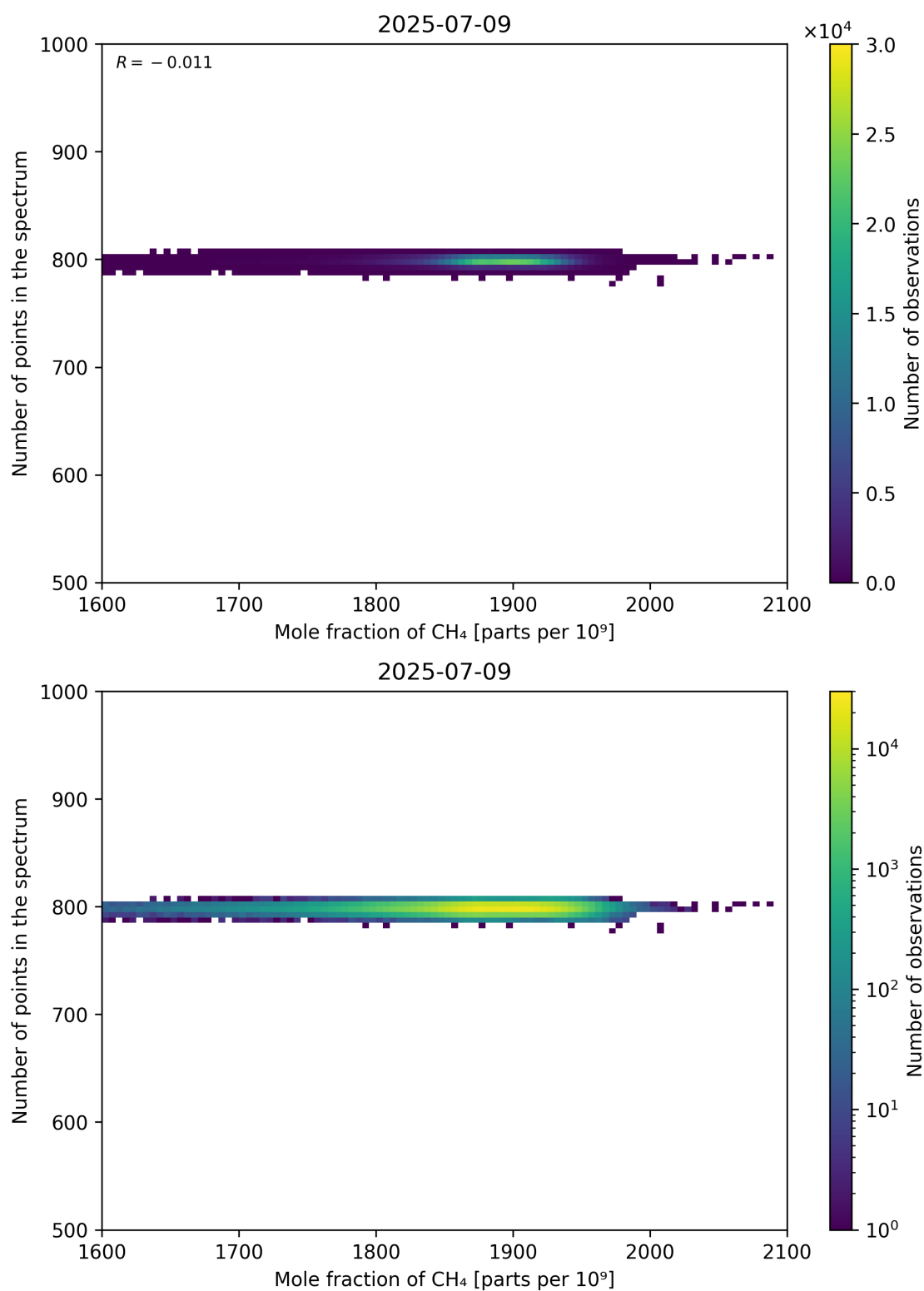
Figure 77: Scatter density plot of “Mole fraction of CH 4 ” against “Number of points in the spectrum” for 2025-07-08 to 2025-07-10.
