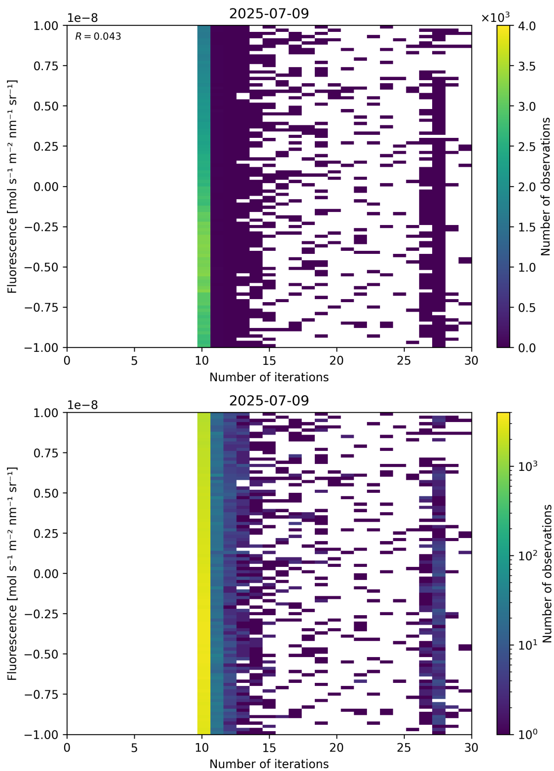
Figure 87: Scatter density plot of “Number of iterations” against “Fluorescence” for 2025-07-08 to 2025-07-10.
