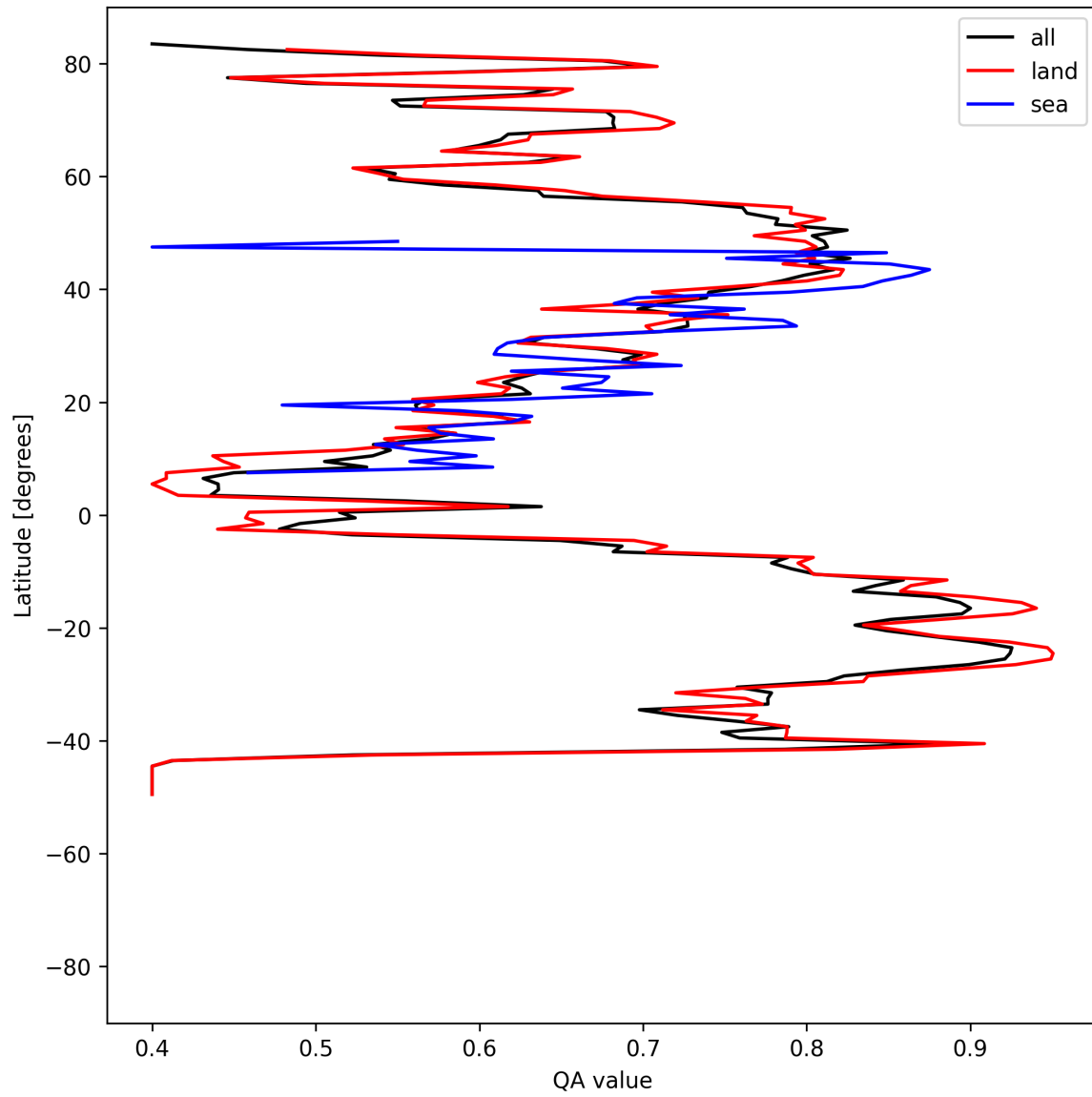
Figure 11: Zonal average of “QA value” for 2025-07-08 to 2025-07-10.
