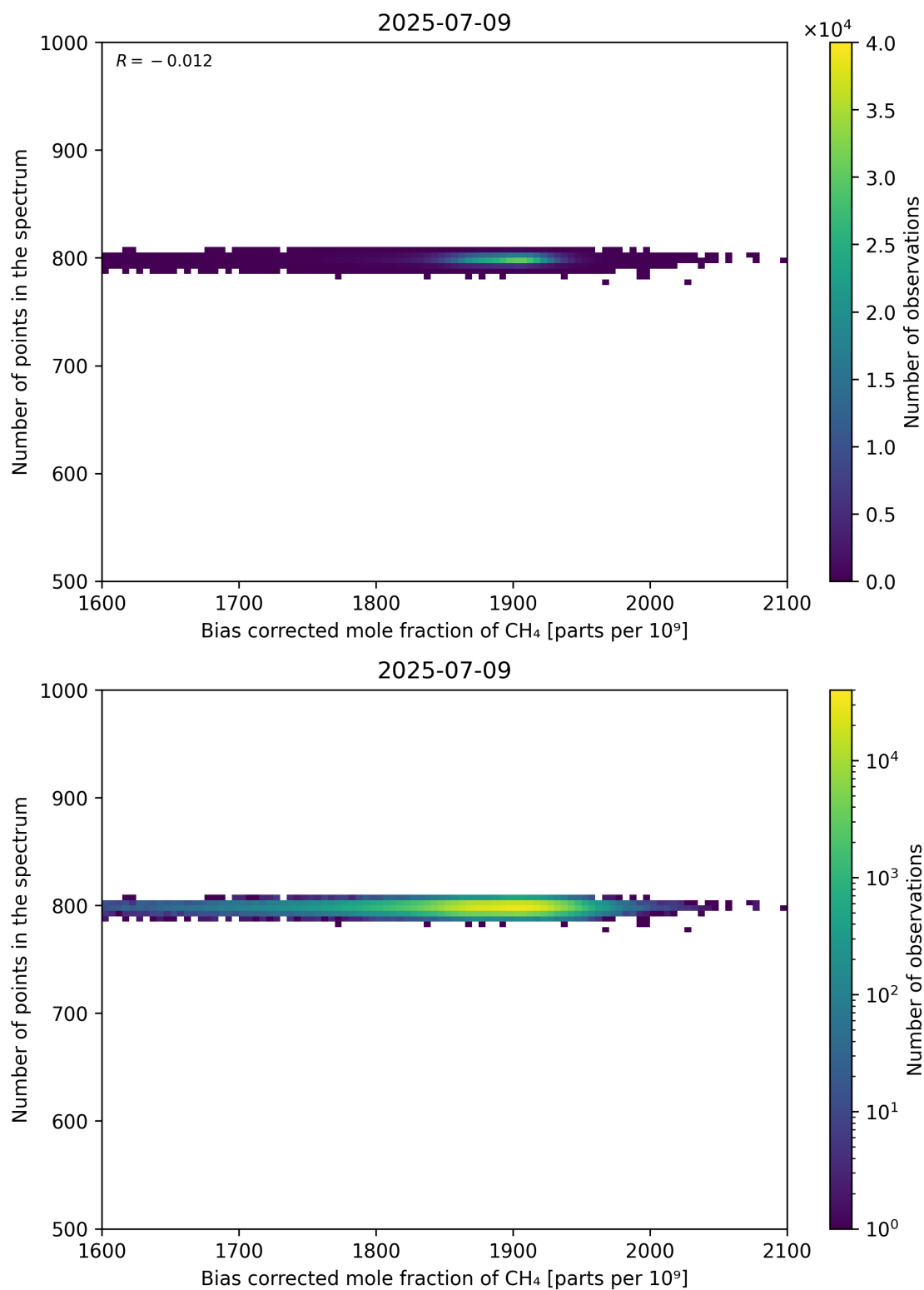
Figure 68: Scatter density plot of “Bias corrected mole fraction of CH 4 ” against “Number of points in the spectrum” for 2025-07-08 to 2025-07-10.
