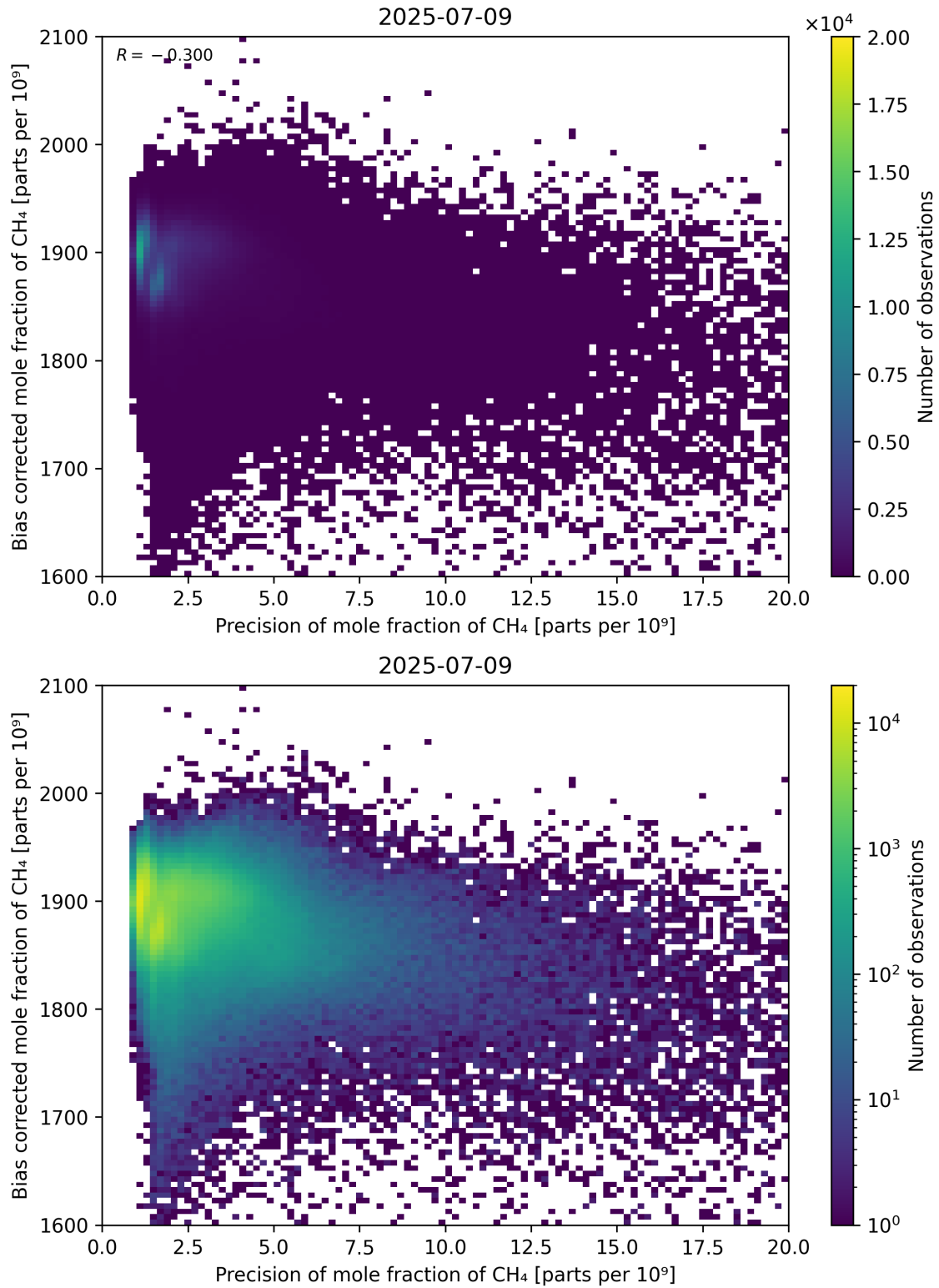
Figure 82: Scatter density plot of “Precision of mole fraction of CH 4 ” against “Bias corrected mole fraction of CH 4 ” for 2025-07-08 to 2025-07-10.
