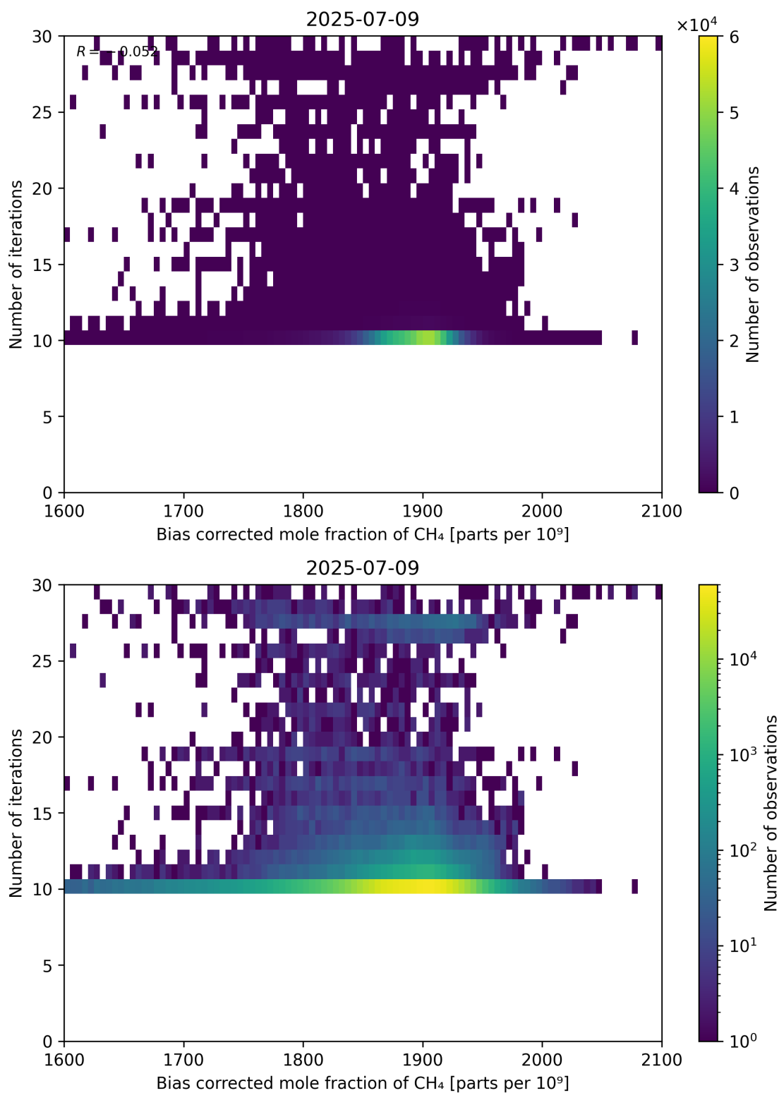
Figure 67: Scatter density plot of “Bias corrected mole fraction of CH 4 ” against “Number of iterations” for 2025-07-08 to 2025-07-10.
