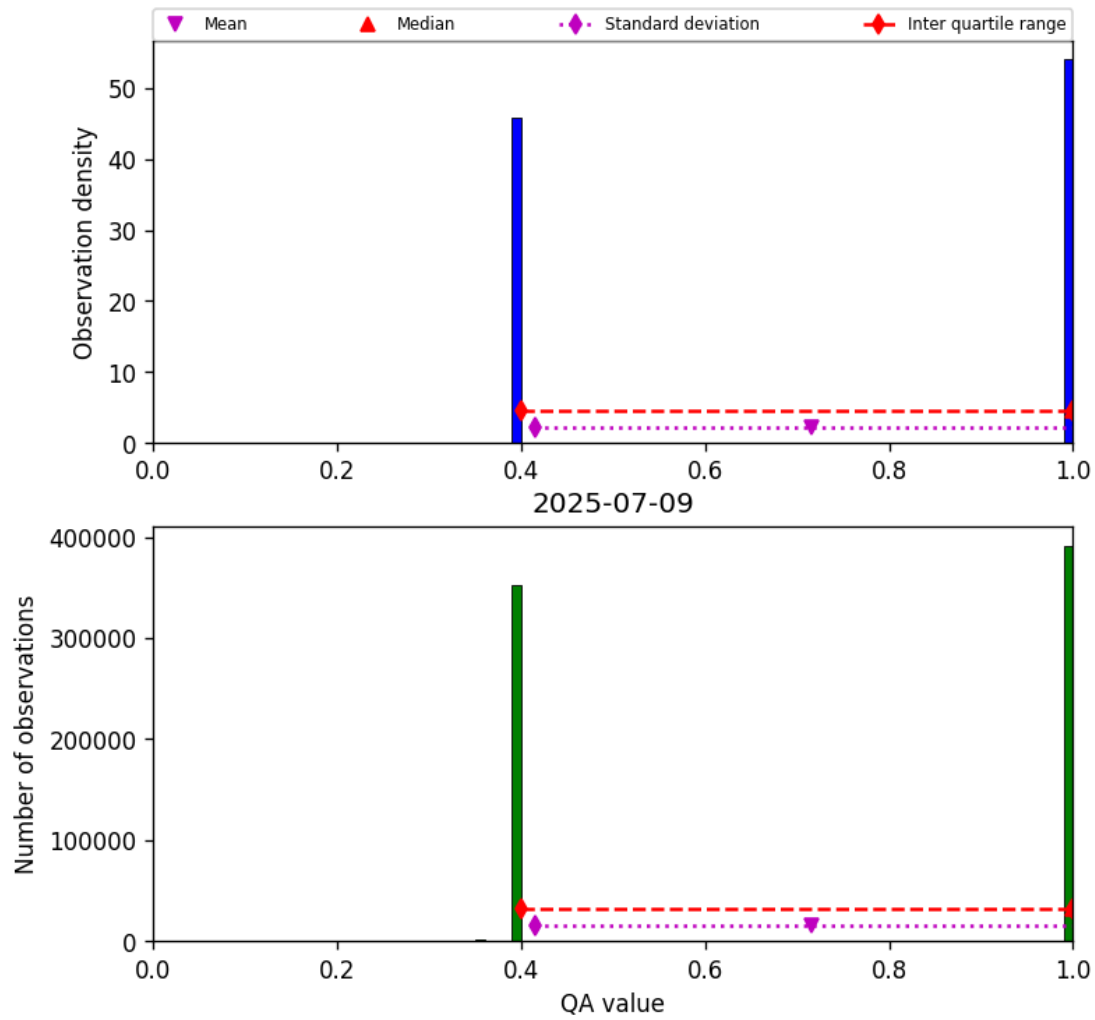
Figure 22: Histogram of “QA value” for 2025-07-08 to 2025-07-10
