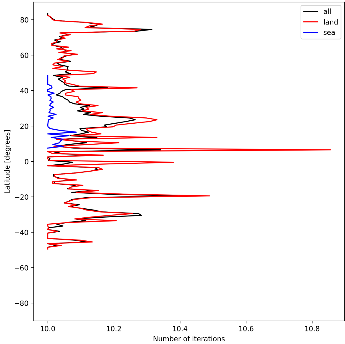
Figure 20: Zonal average of “Number of iterations” for 2025-07-08 to 2025-07-10.
