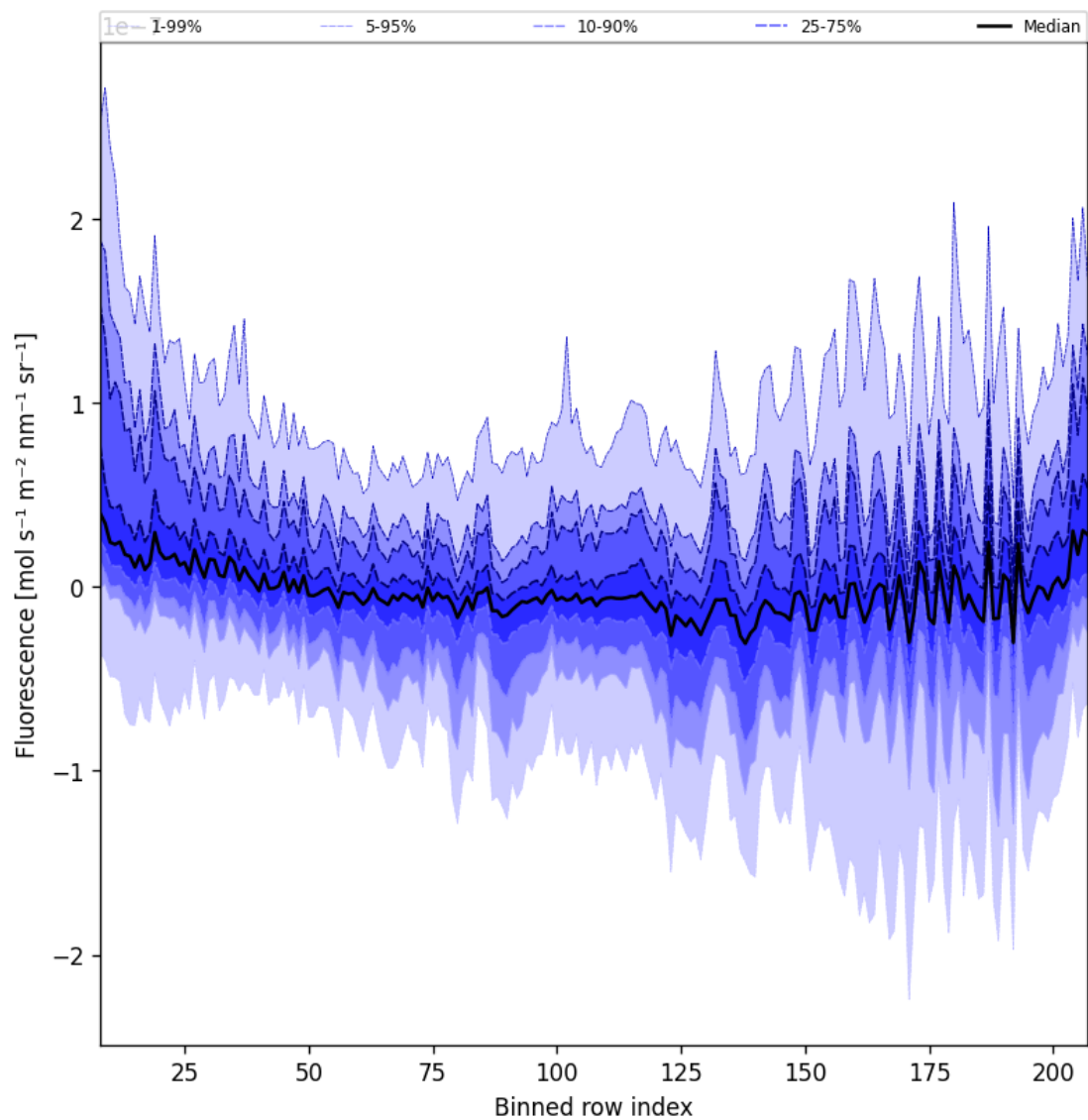
Figure 43: Along track statistics of “Fluorescence” for 2025-07-08 to 2025-07-10
