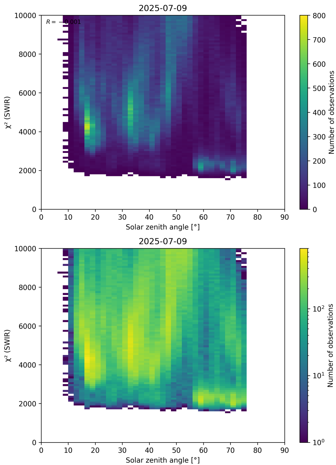
Figure 95: Scatter density plot of “Solar zenith angle” against “ \chi^2 (SWIR)” for 2025-07-08 to 2025-07-10.
