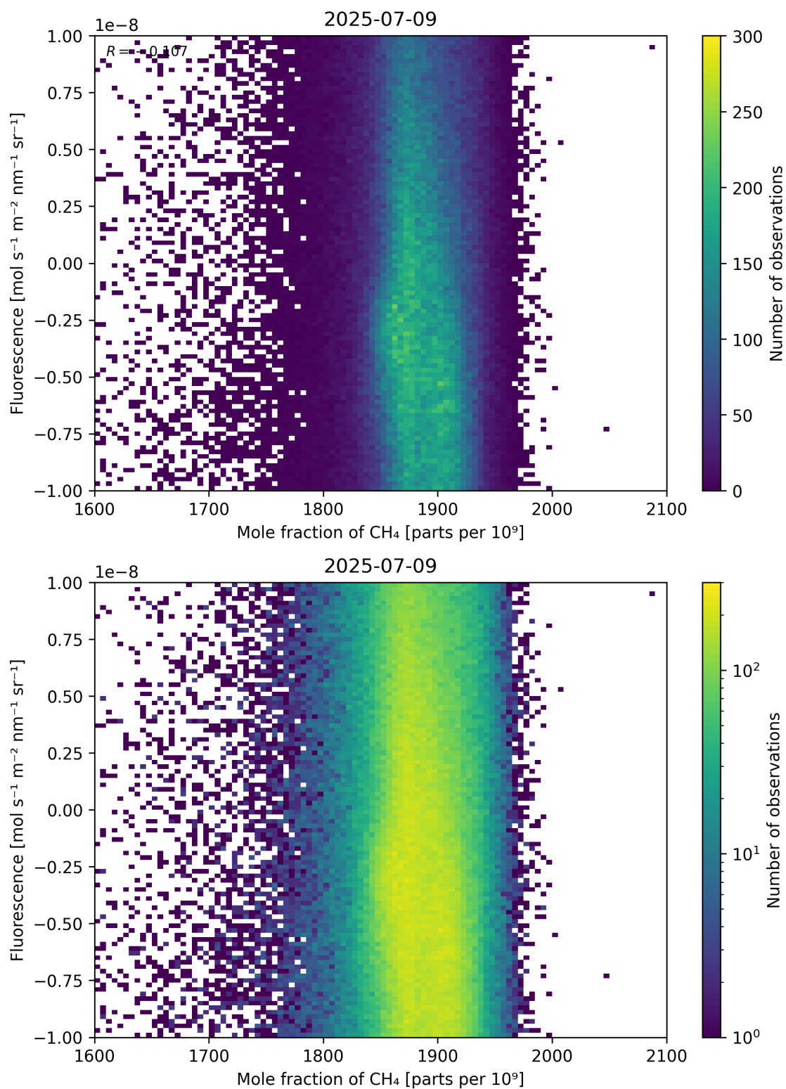
Figure 73: Scatter density plot of “Mole fraction of \text{CH}_4 ” against “Fluorescence” for 2025-07-08 to 2025-07-10.
