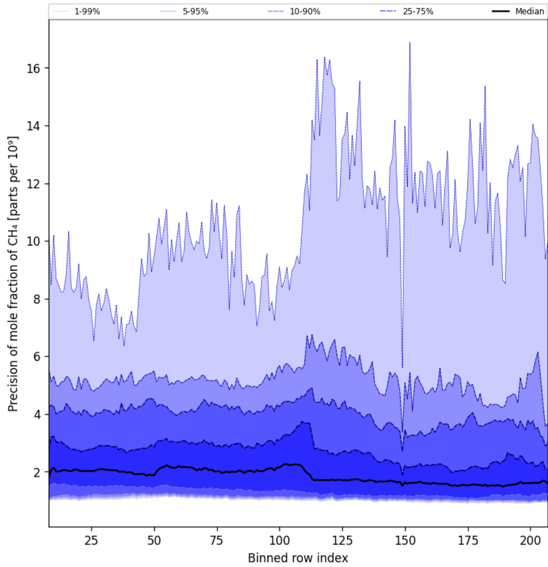
Figure 35: Along track statistics of “Precision of mole fraction of CH 4 ” for 2025-07-08 to 2025-07-10
