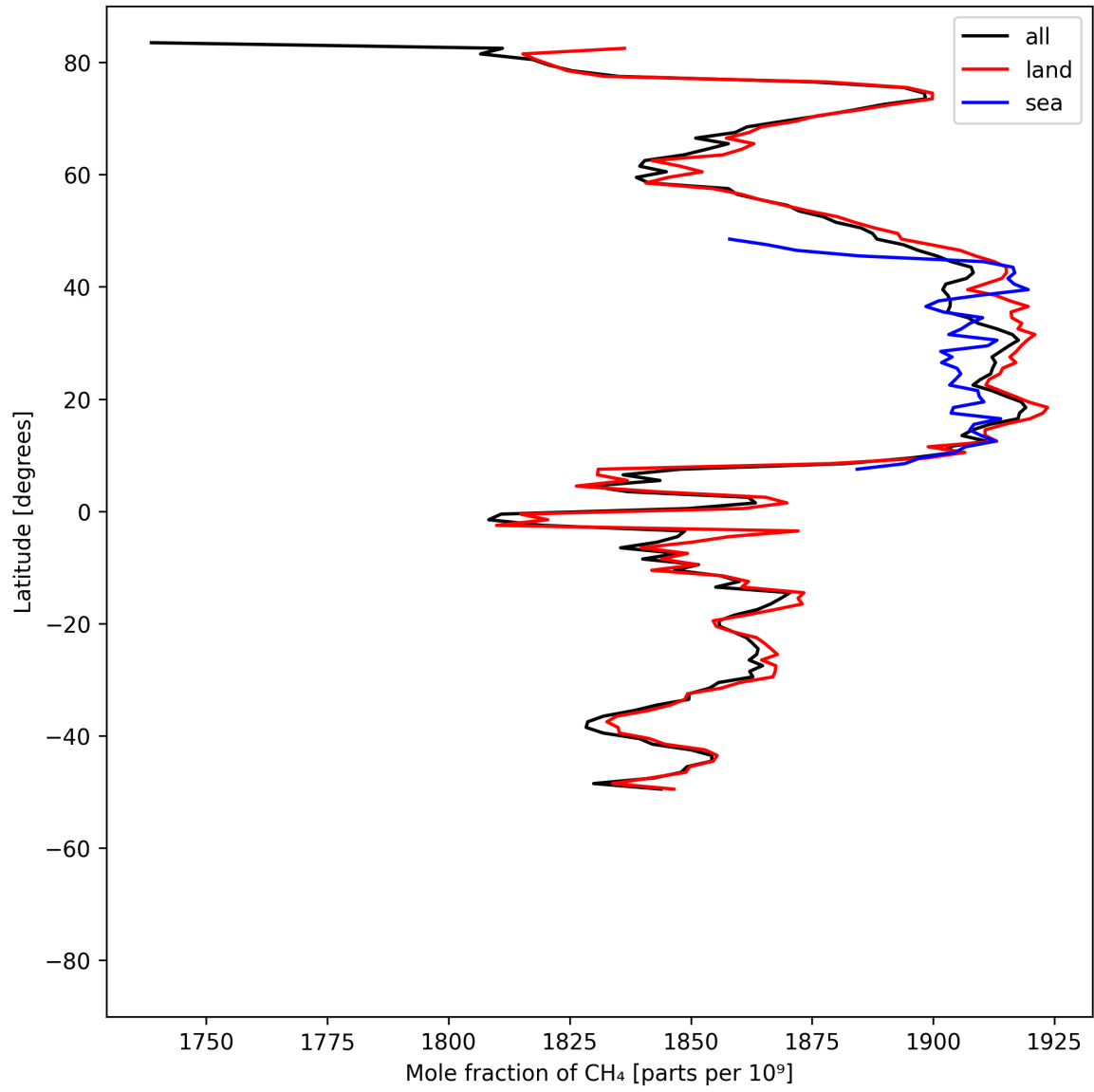
Figure 12: Zonal average of “Mole fraction of \text{CH}_4 ” for 2025-07-08 to 2025-07-10.
