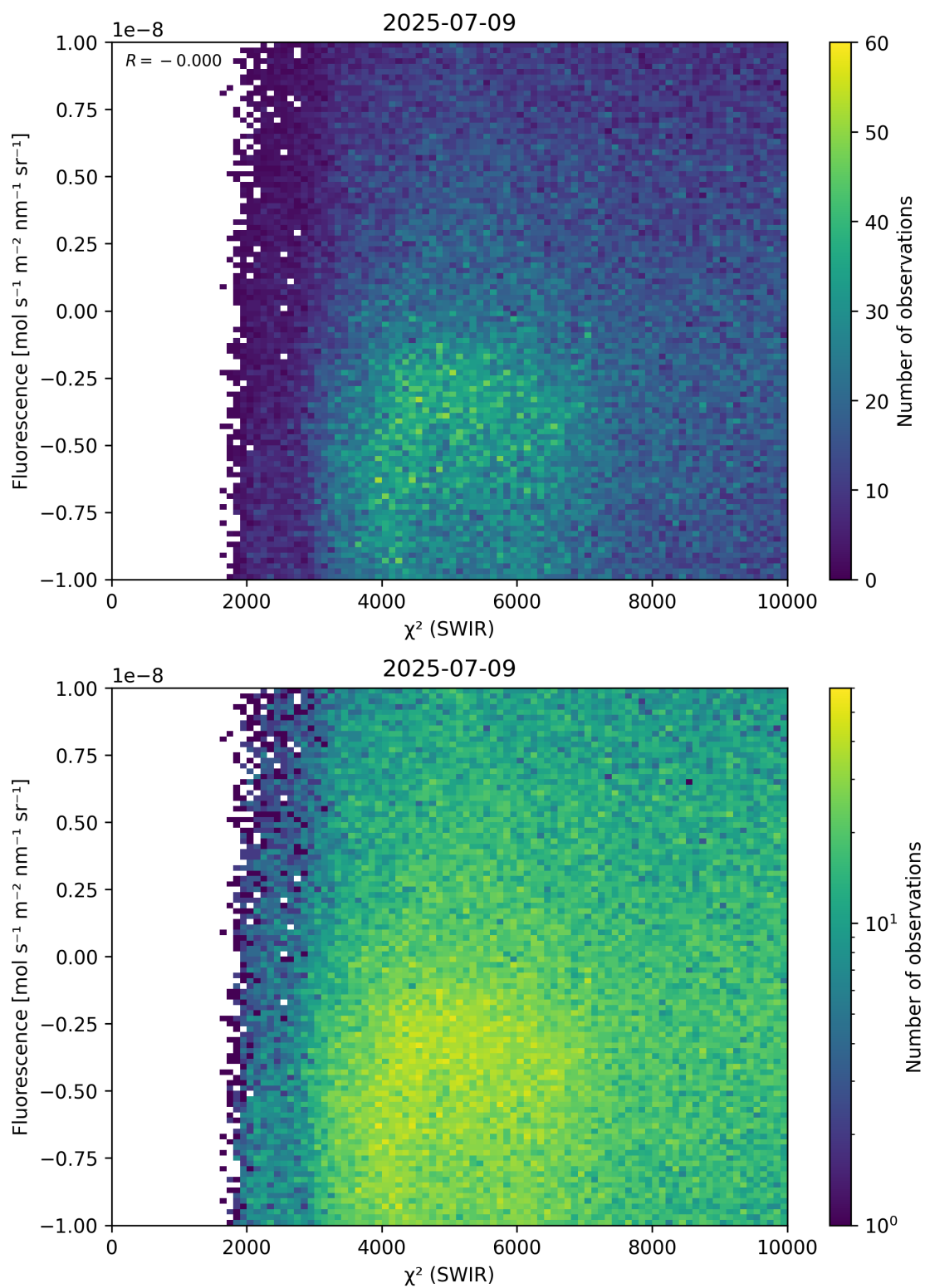
Figure 49: Scatter density plot of “ \chi^2 (SWIR)” against “Fluorescence” for 2025-07-08 to 2025-07-10.
