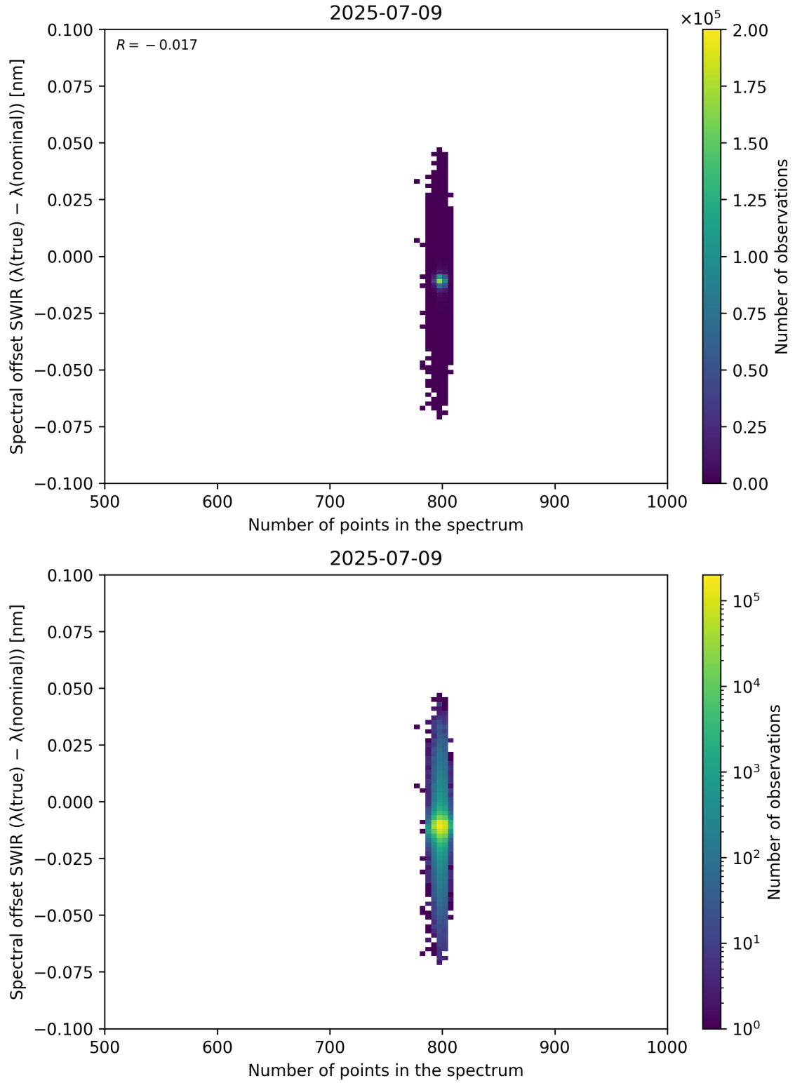
Figure 93: Scatter density plot of “Number of points in the spectrum” against “Spectral offset SWIR ( \lambda_{\text{true}} - \lambda_{\text{nominal}} )” for 2025-07-08 to 2025-07-10.
