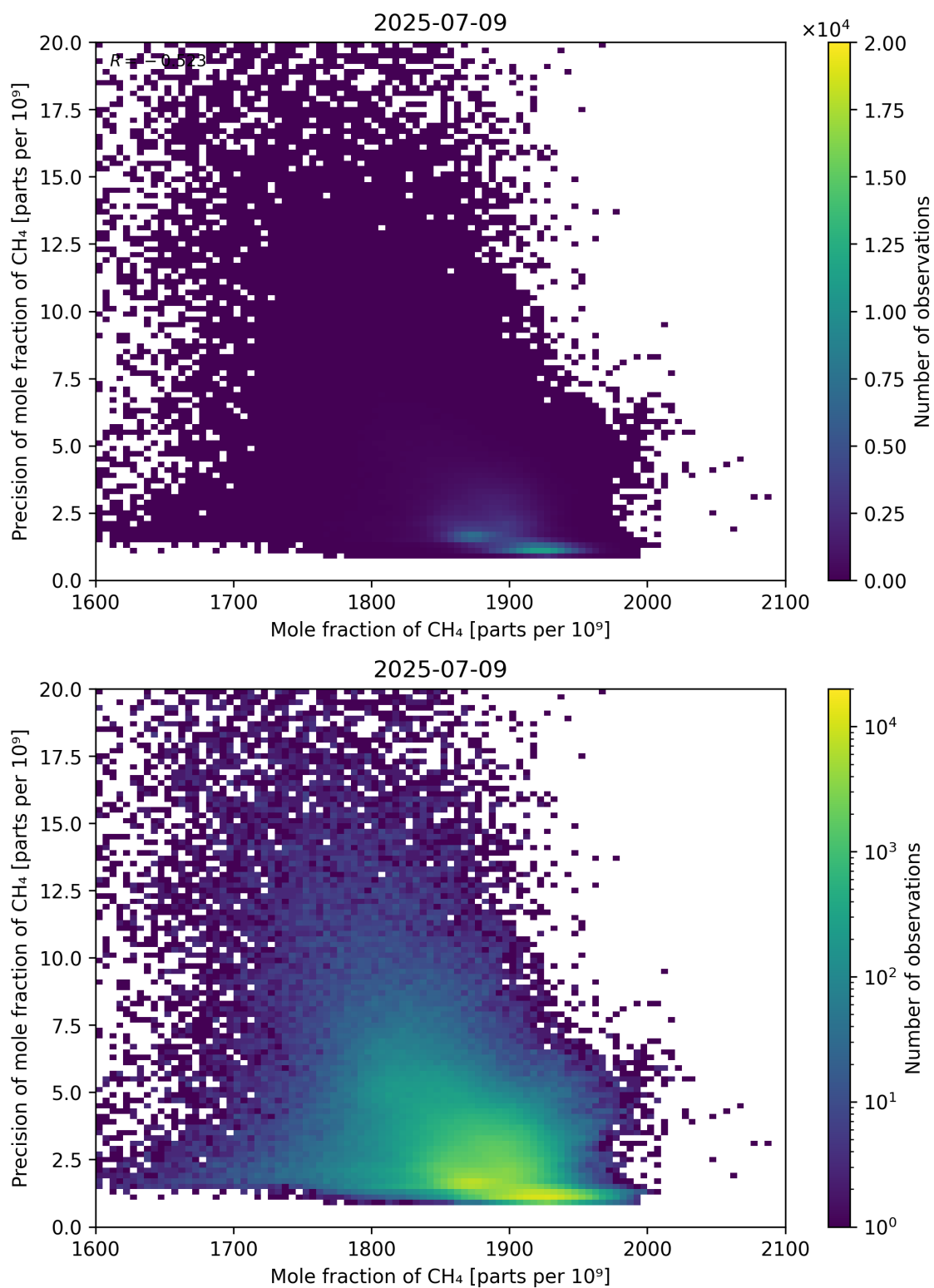
Figure 75: Scatter density plot of “Mole fraction of CH 4 ” against “Precision of mole fraction of CH 4 ” for 2025-07-08 to 2025-07-10.
