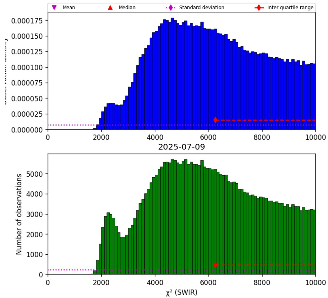
Figure 28: Histogram of “ \chi^2 (SWIR)” for 2025-07-08 to 2025-07-10
