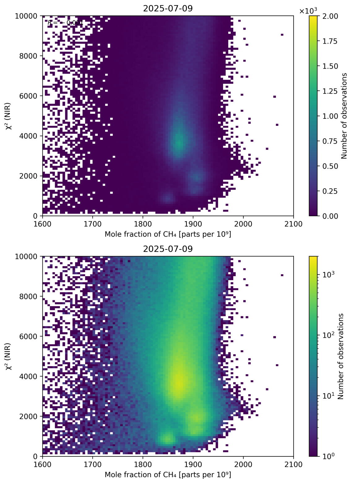
Figure 70: Scatter density plot of “Mole fraction of \text{CH}_4 ” against “ \chi^2 (NIR)” for 2025-07-08 to 2025-07-10.
