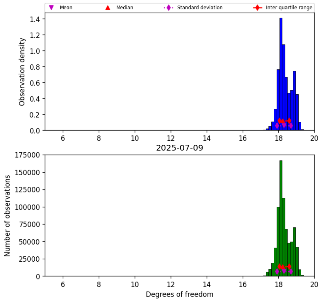
Figure 30: Histogram of “Degrees of freedom” for 2025-07-08 to 2025-07-10
