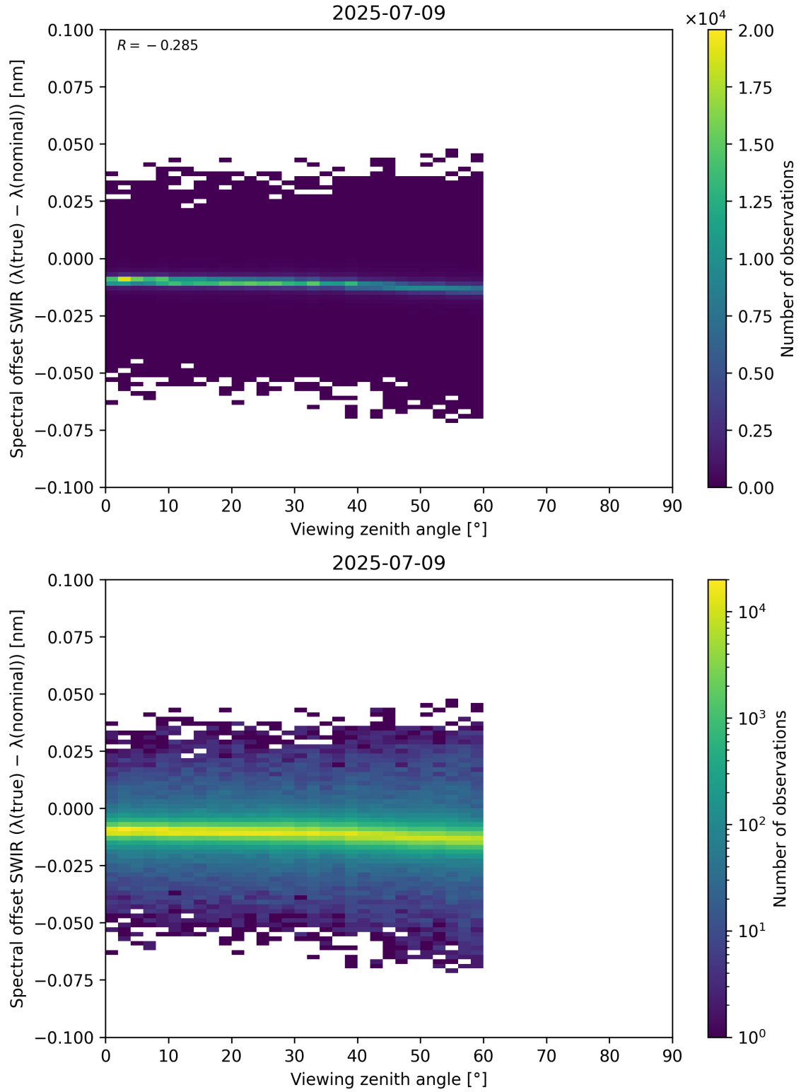
Figure 116: Scatter density plot of “Viewing zenith angle” against “Spectral offset SWIR ( \lambda_{\text{true}} - \lambda_{\text{nominal}} )” for 2025-07-08 to 2025-07-10.
