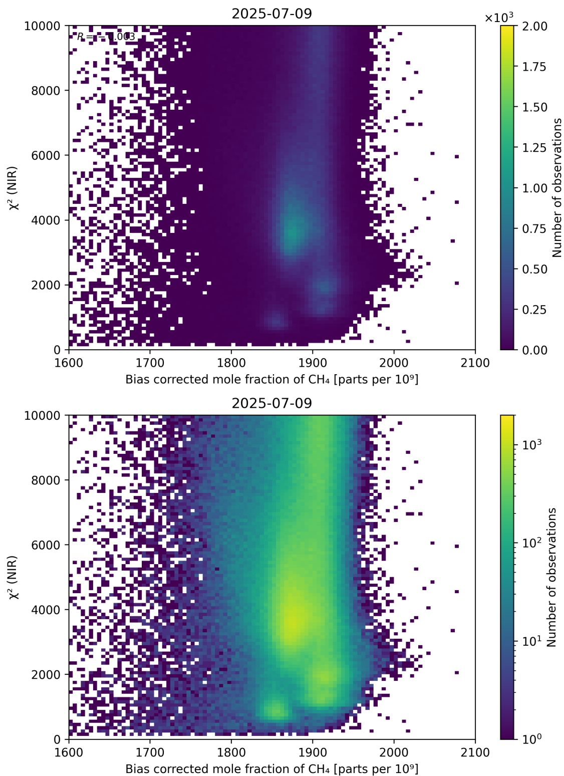
Figure 63: Scatter density plot of “Bias corrected mole fraction of \text{CH}_4 ” against “ \chi^2 (NIR)” for 2025-07-08 to 2025-07-10.
