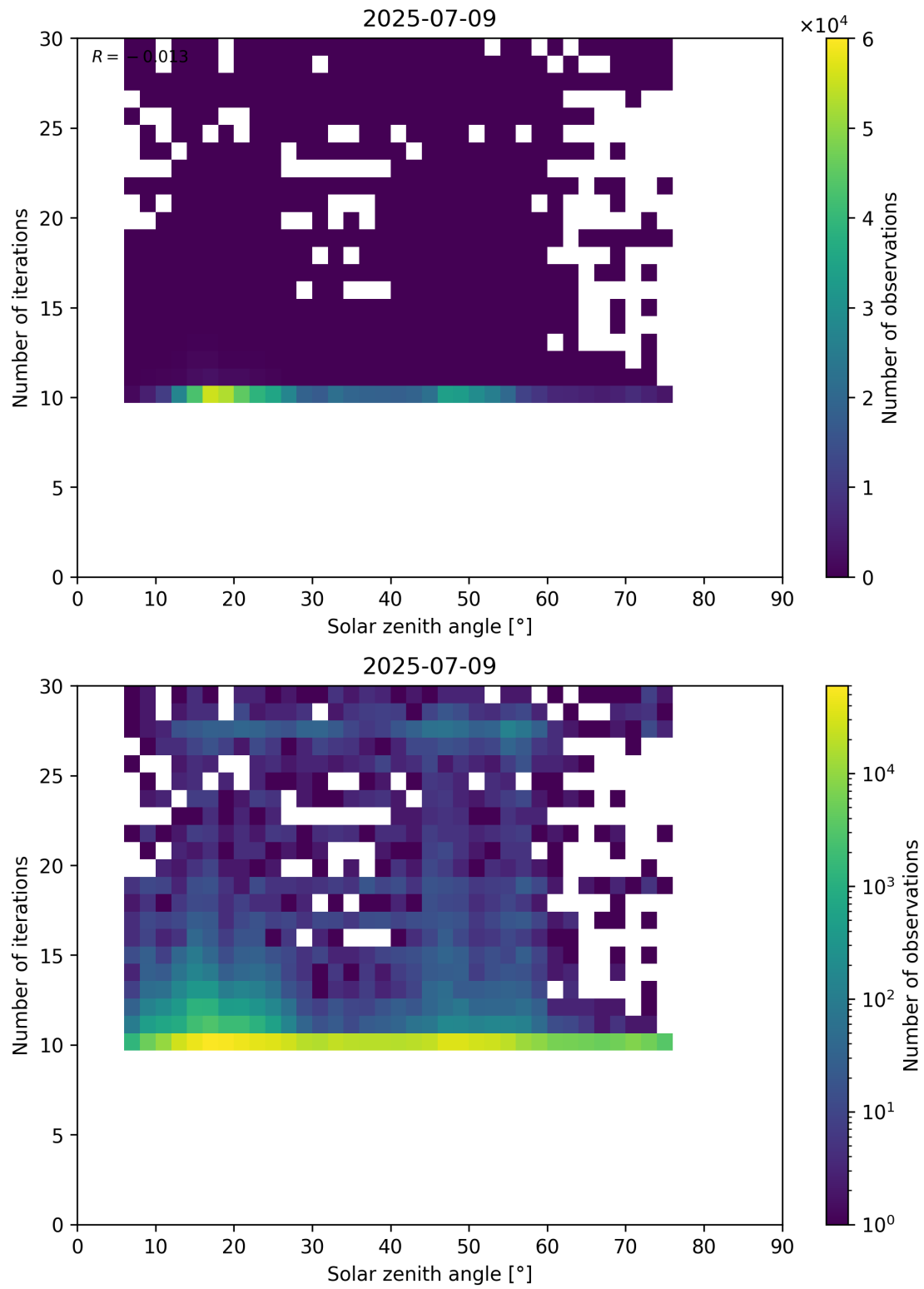
Figure 102: Scatter density plot of “Solar zenith angle” against “Number of iterations” for 2025-07-08 to 2025-07-10.
