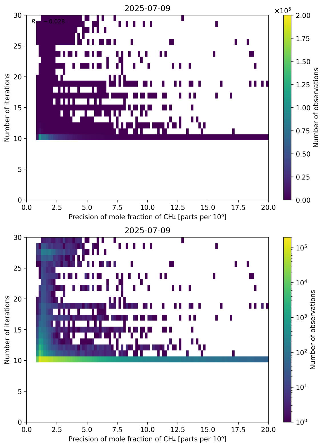
Figure 83: Scatter density plot of “Precision of mole fraction of CH 4 ” against “Number of iterations” for 2025-07-08 to 2025-07-10.
