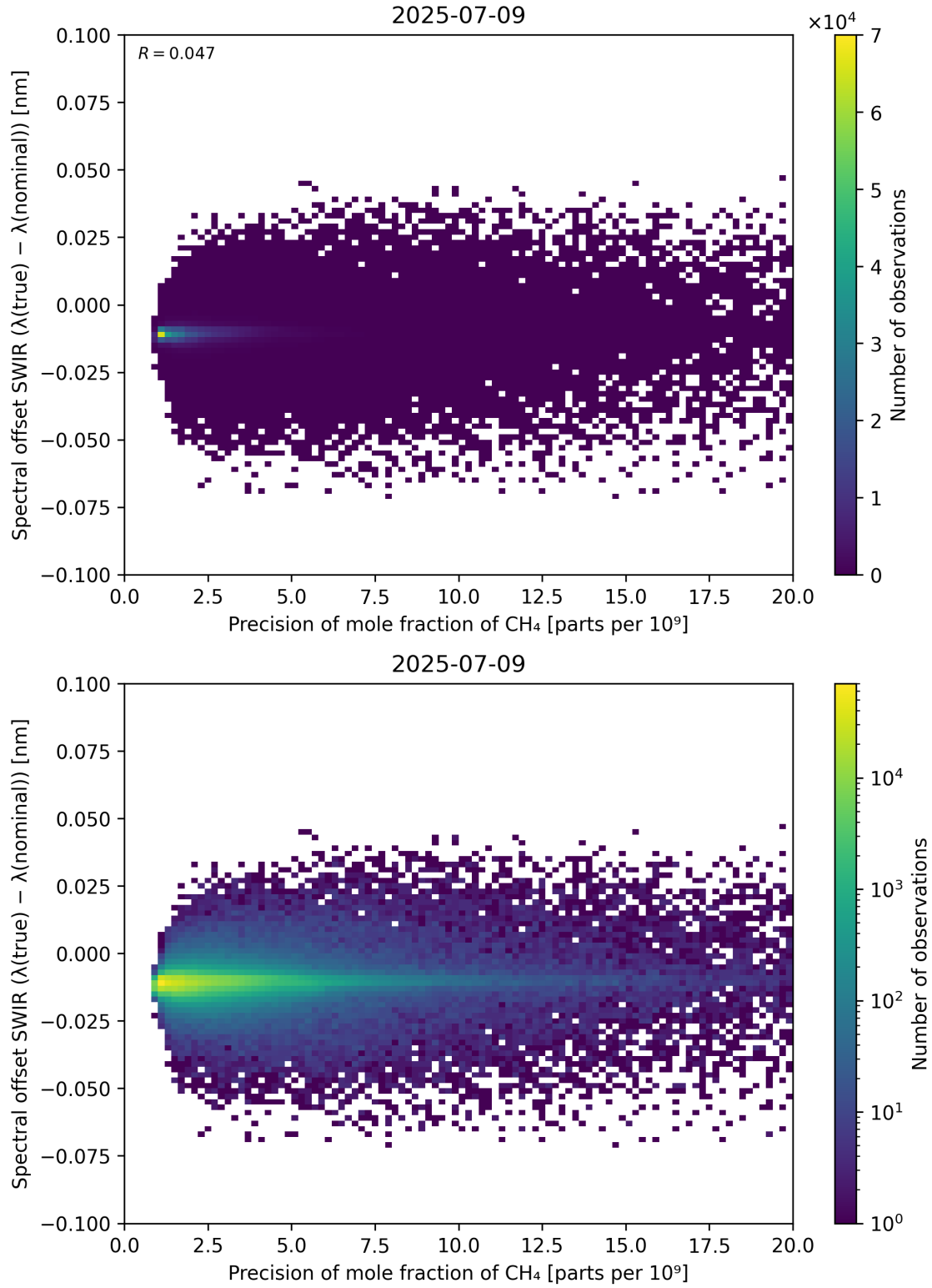
Figure 85: Scatter density plot of “Precision of mole fraction of CH 4 ” against “Spectral offset SWIR ( \lambda_{\text{true}} - \lambda_{\text{nominal}} )” for 2025-07-08 to 2025-07-10.
