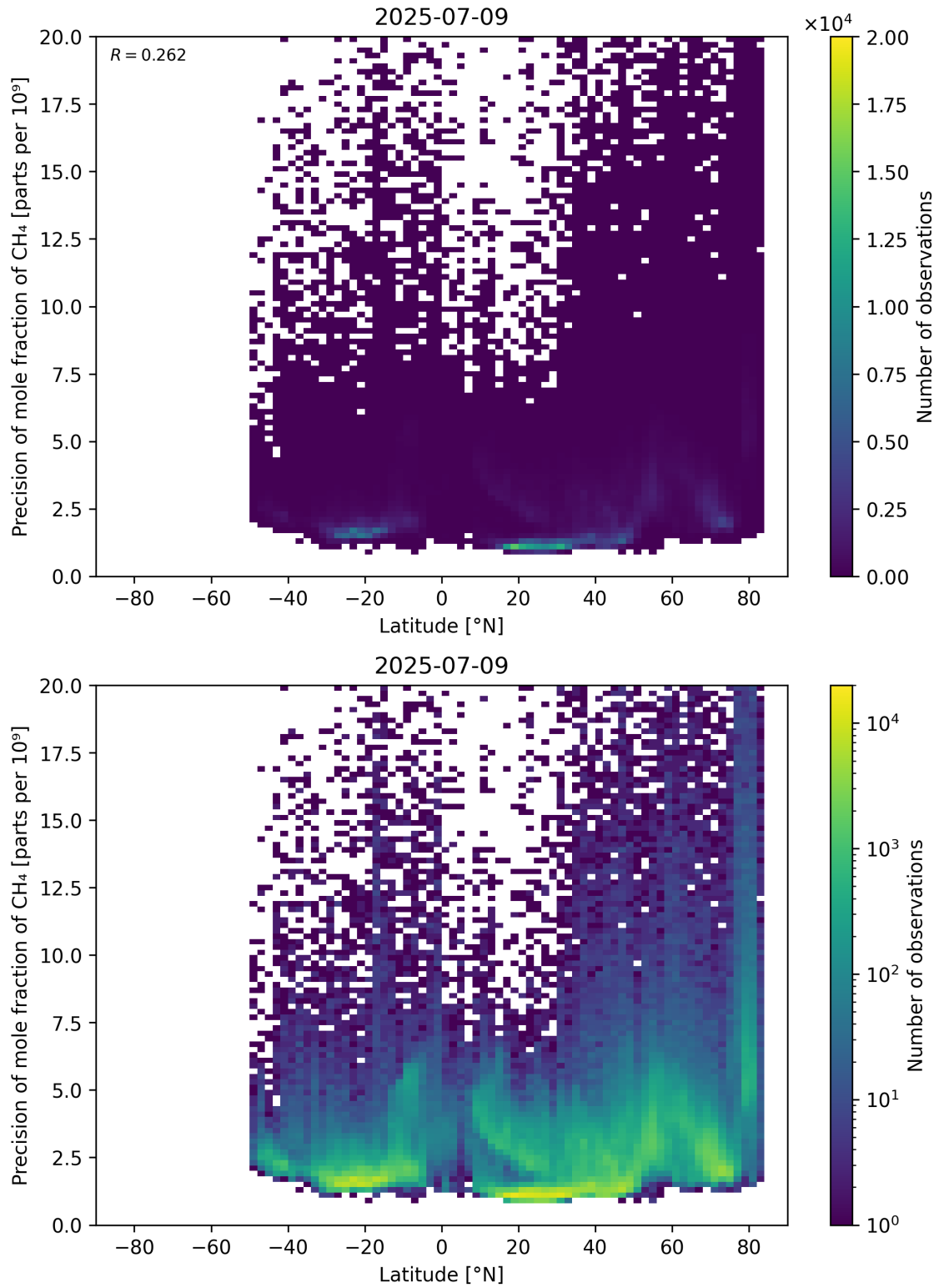
Figure 59: Scatter density plot of “Latitude” against “Precision of mole fraction of \text{CH}_4 ” for 2025-07-08 to 2025-07-10.
