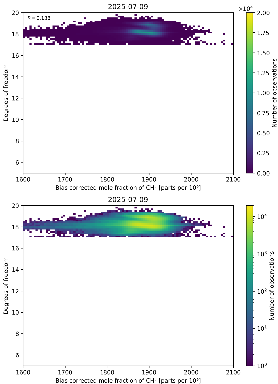
Figure 65: Scatter density plot of “Bias corrected mole fraction of CH 4 ” against “Degrees of freedom” for 2025-07-08 to 2025-07-10.
