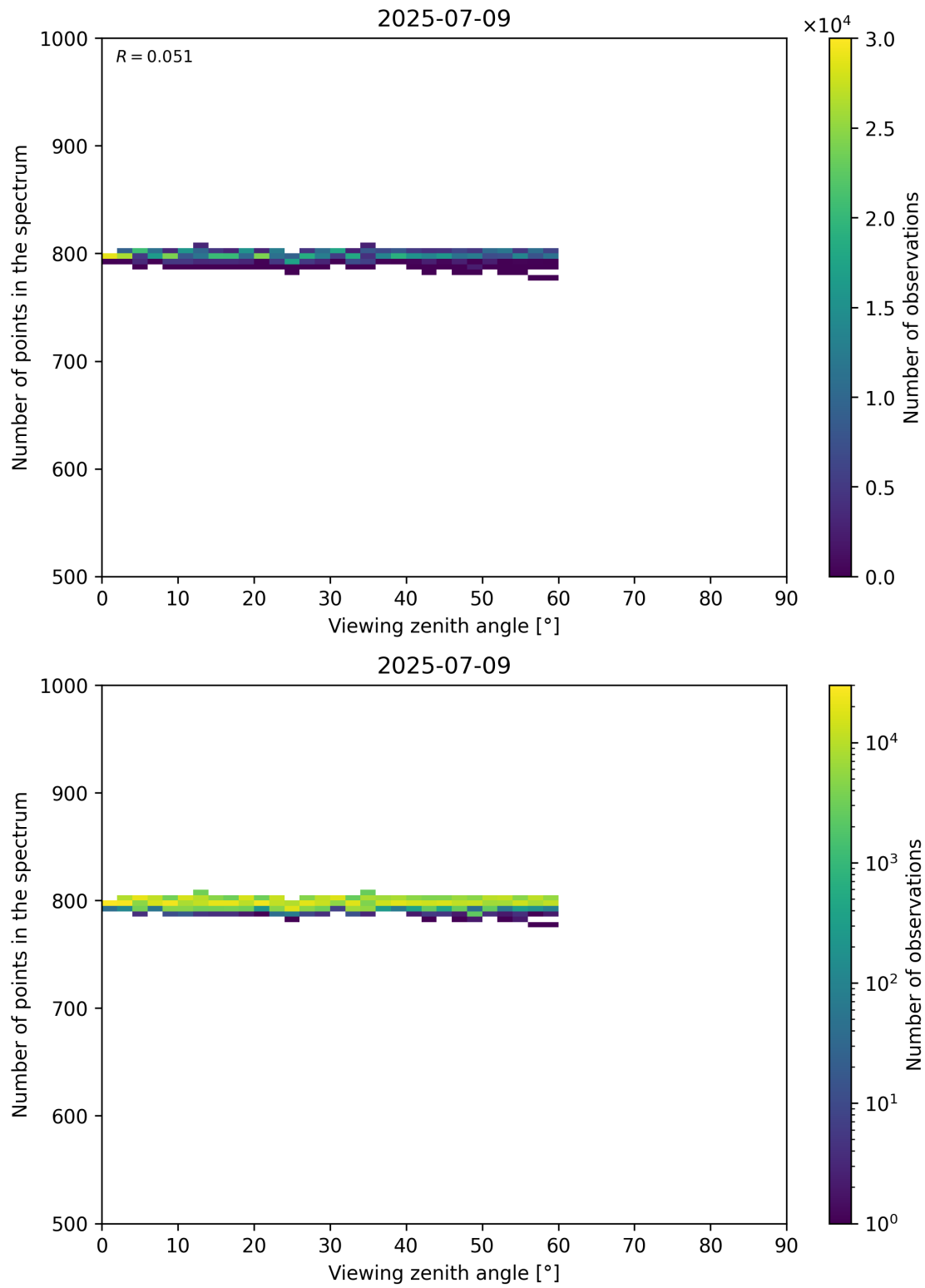
Figure 114: Scatter density plot of “Viewing zenith angle” against “Number of points in the spectrum” for 2025-07-08 to 2025-07-10.
