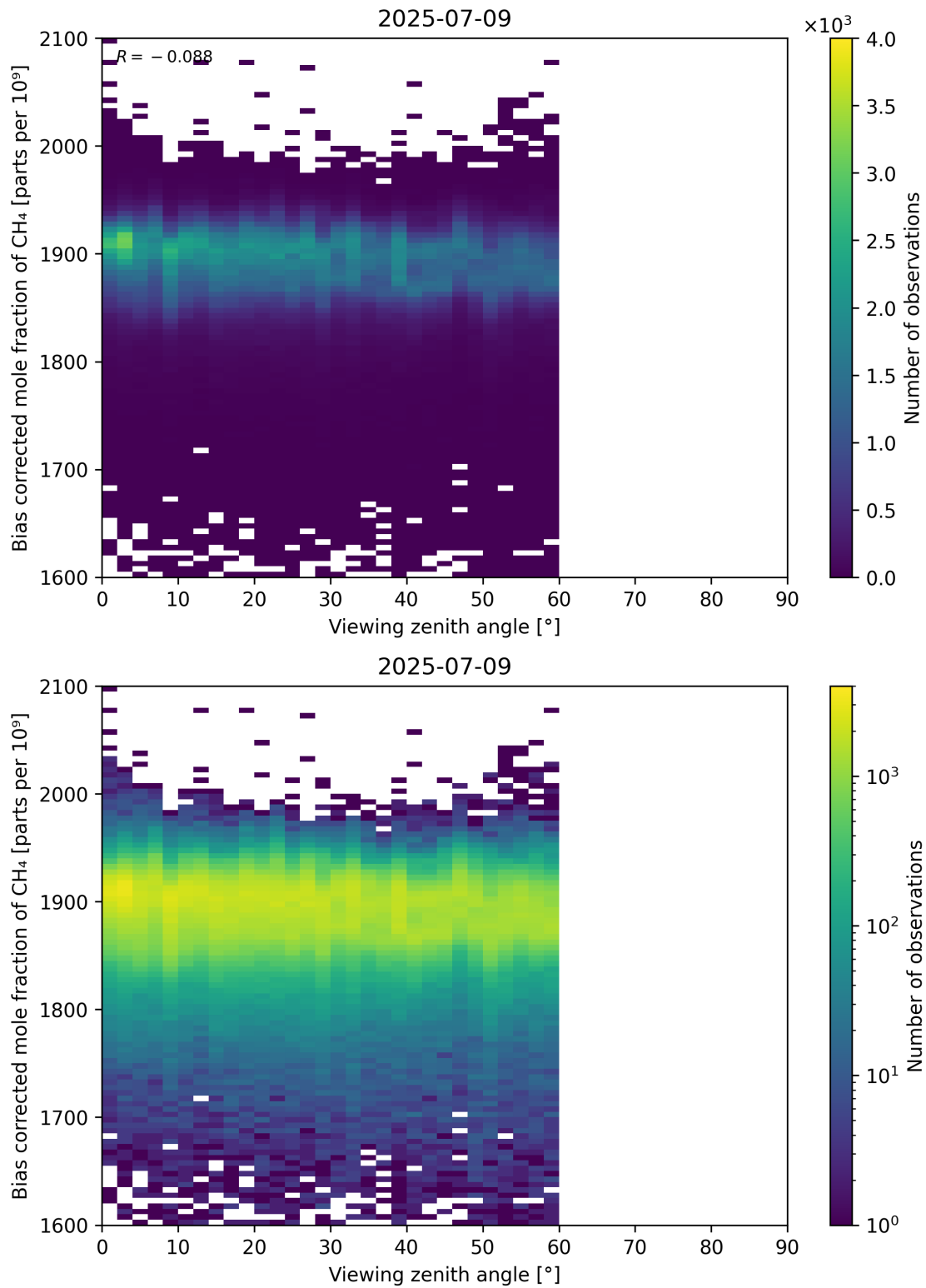
Figure 111: Scatter density plot of “Viewing zenith angle” against “Bias corrected mole fraction of CH 4 ” for 2025-07-08 to 2025-07-10.
