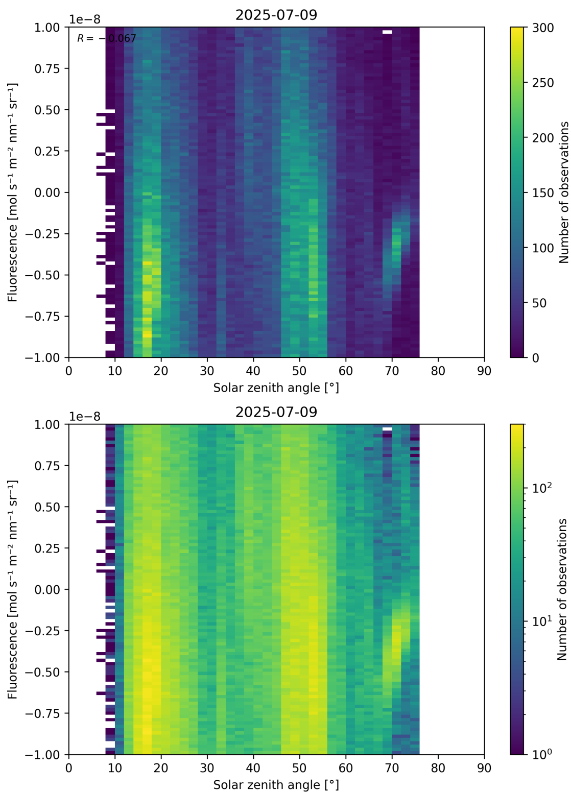
Figure 97: Scatter density plot of “Solar zenith angle” against “Fluorescence” for 2025-07-08 to 2025-07-10.
