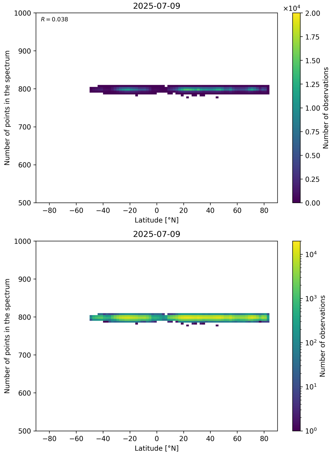
Figure 61: Scatter density plot of “Latitude” against “Number of points in the spectrum” for 2025-07-08 to 2025-07-10.
