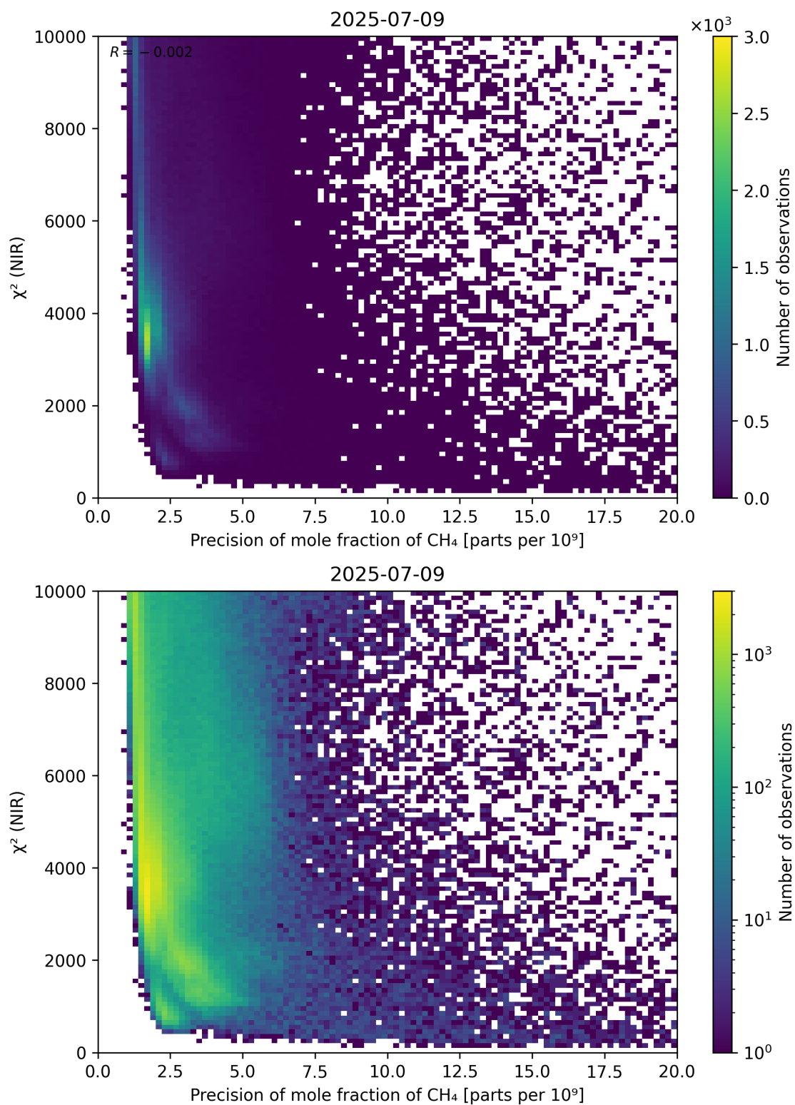
Figure 78: Scatter density plot of “Precision of mole fraction of CH 4 ” against “ \chi^2 (NIR)” for 2025-07-08 to 2025-07-10.
