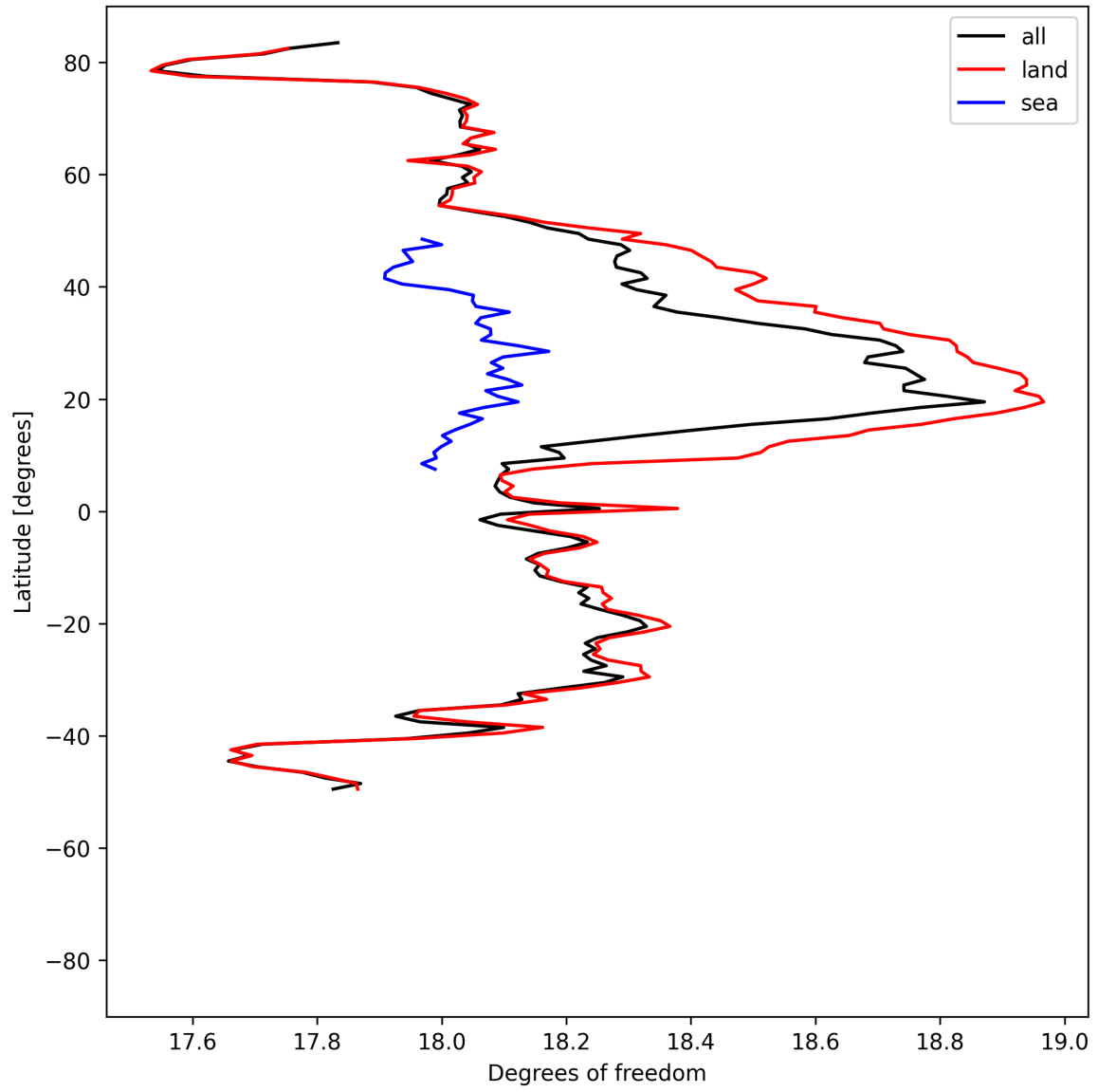
Figure 19: Zonal average of “Degrees of freedom” for 2025-07-08 to 2025-07-10.
