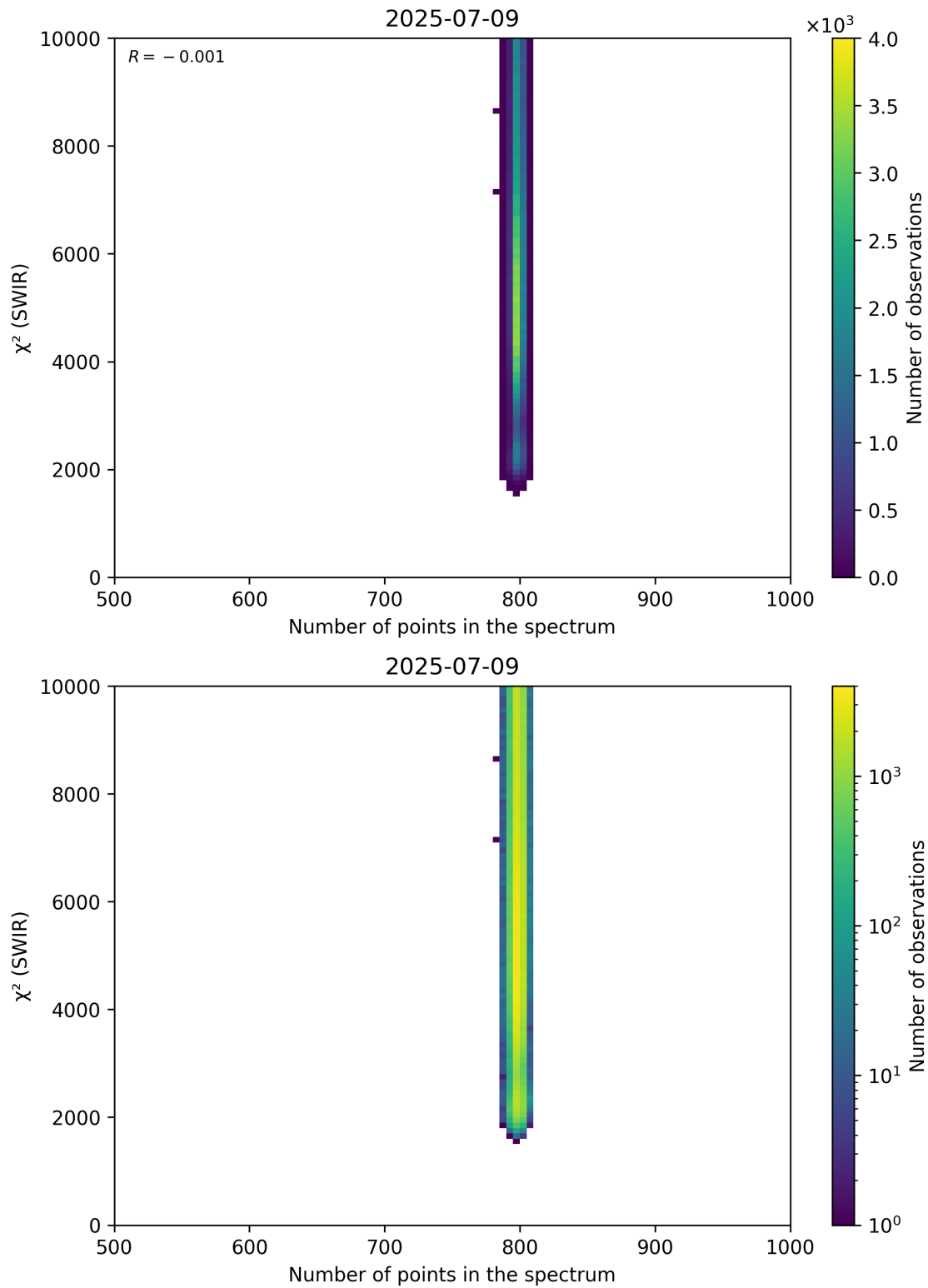
Figure 89: Scatter density plot of “Number of points in the spectrum” against “ \chi^2 (SWIR)” for 2025-07-08 to 2025-07-10.
