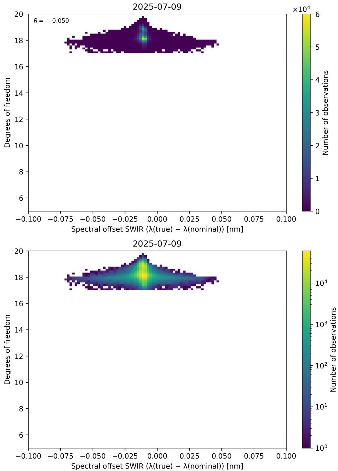
Figure 119: Scatter density plot of “Spectral offset SWIR ( \lambda_{\text{true}} - \lambda_{\text{nominal}} )” against “Degrees of freedom” for 2025-07-08 to 2025-07-10.
