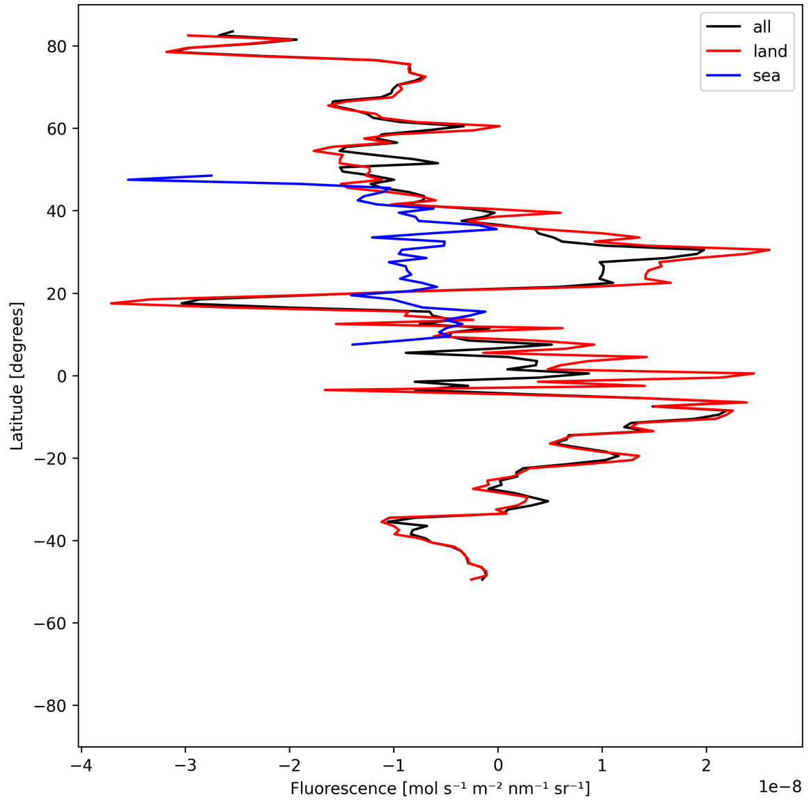
Figure 21: Zonal average of “Fluorescence” for 2025-07-08 to 2025-07-10.
