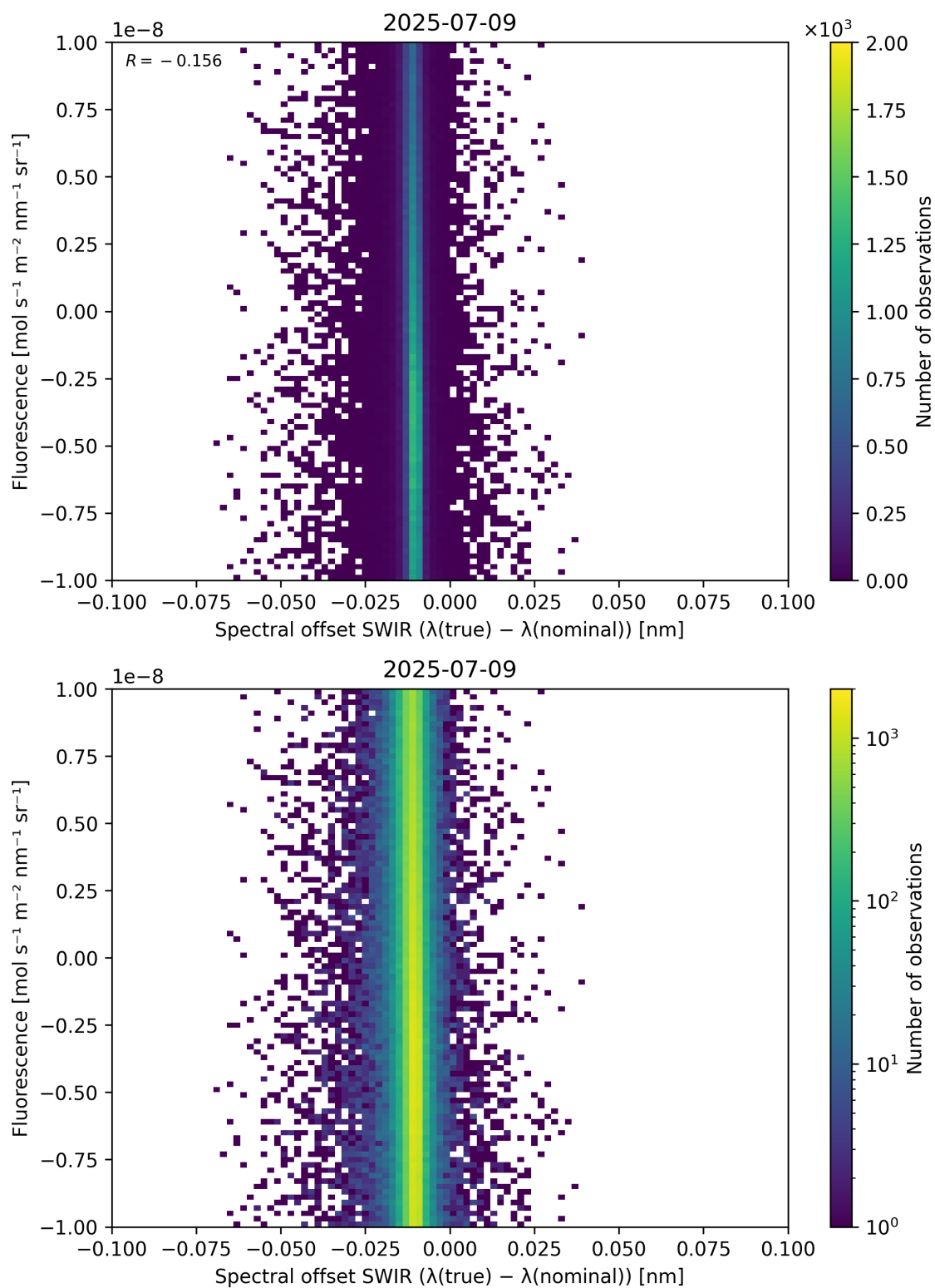
Figure 120: Scatter density plot of “Spectral offset SWIR ( \lambda_{\text{true}} - \lambda_{\text{nominal}} )” against “Fluorescence” for 2025-07-08 to 2025-07-10.
