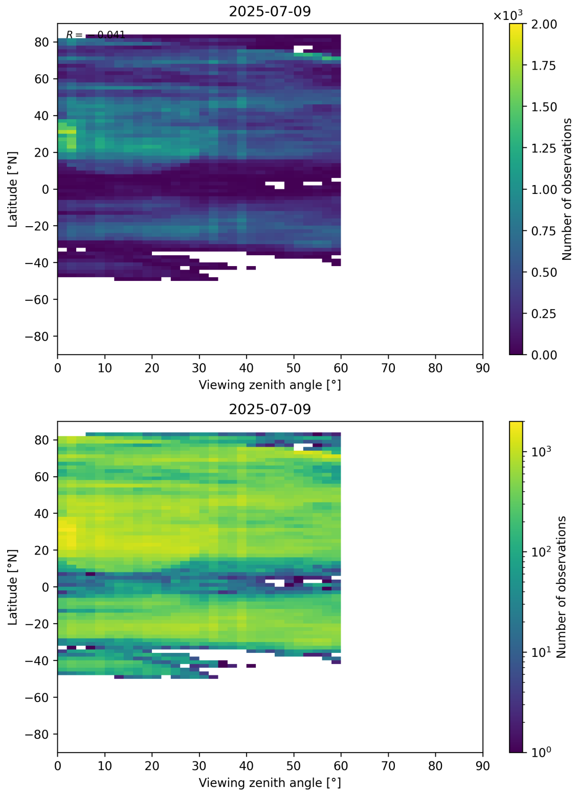
Figure 109: Scatter density plot of “Viewing zenith angle” against “Latitude” for 2025-07-08 to 2025-07-10.
