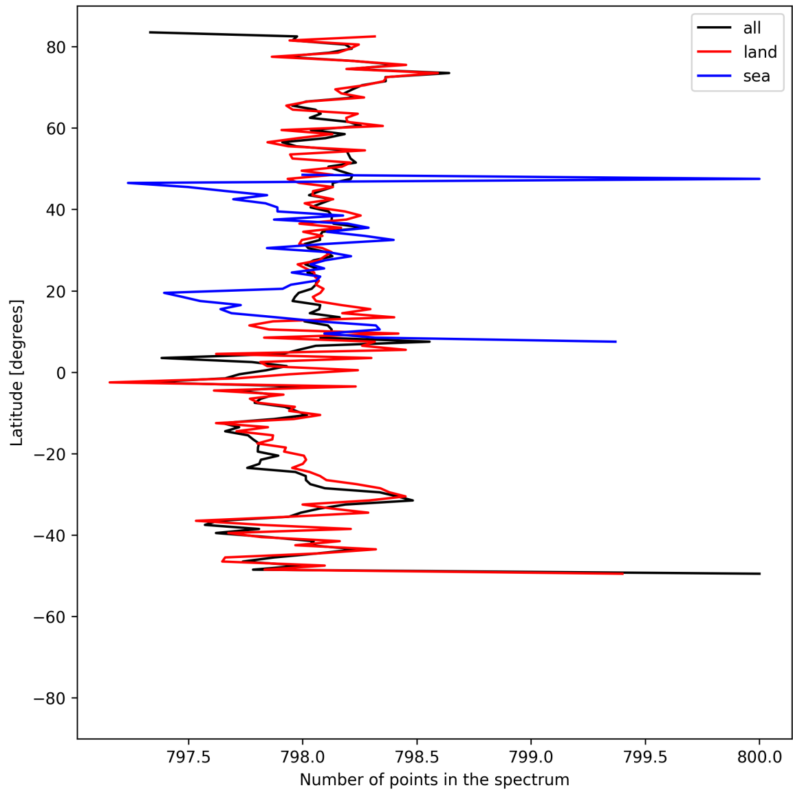
Figure 15: Zonal average of “Number of points in the spectrum” for 2025-07-08 to 2025-07-10.
