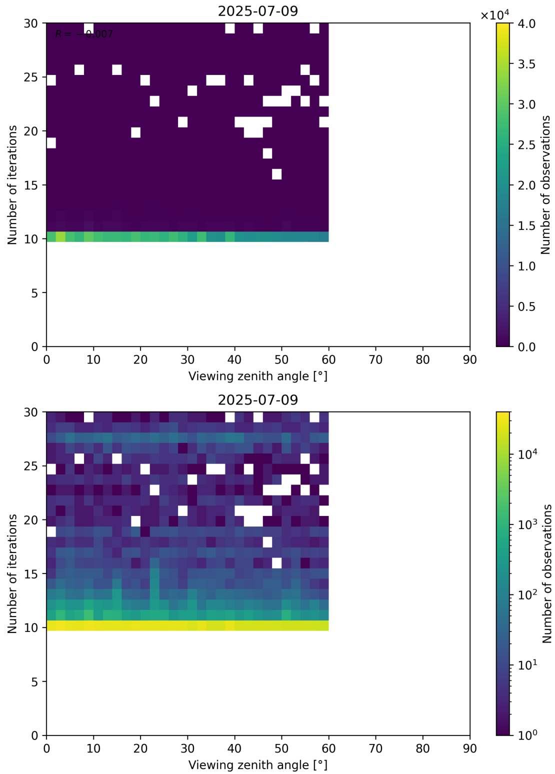
Figure 113: Scatter density plot of “Viewing zenith angle” against “Number of iterations” for 2025-07-08 to 2025-07-10.
