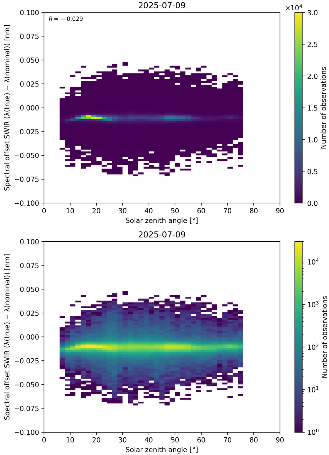
Figure 104: Scatter density plot of “Solar zenith angle” against “Spectral offset SWIR ( \lambda_{\text{true}} - \lambda_{\text{nominal}} )” for 2025-07-08 to 2025-07-10.
