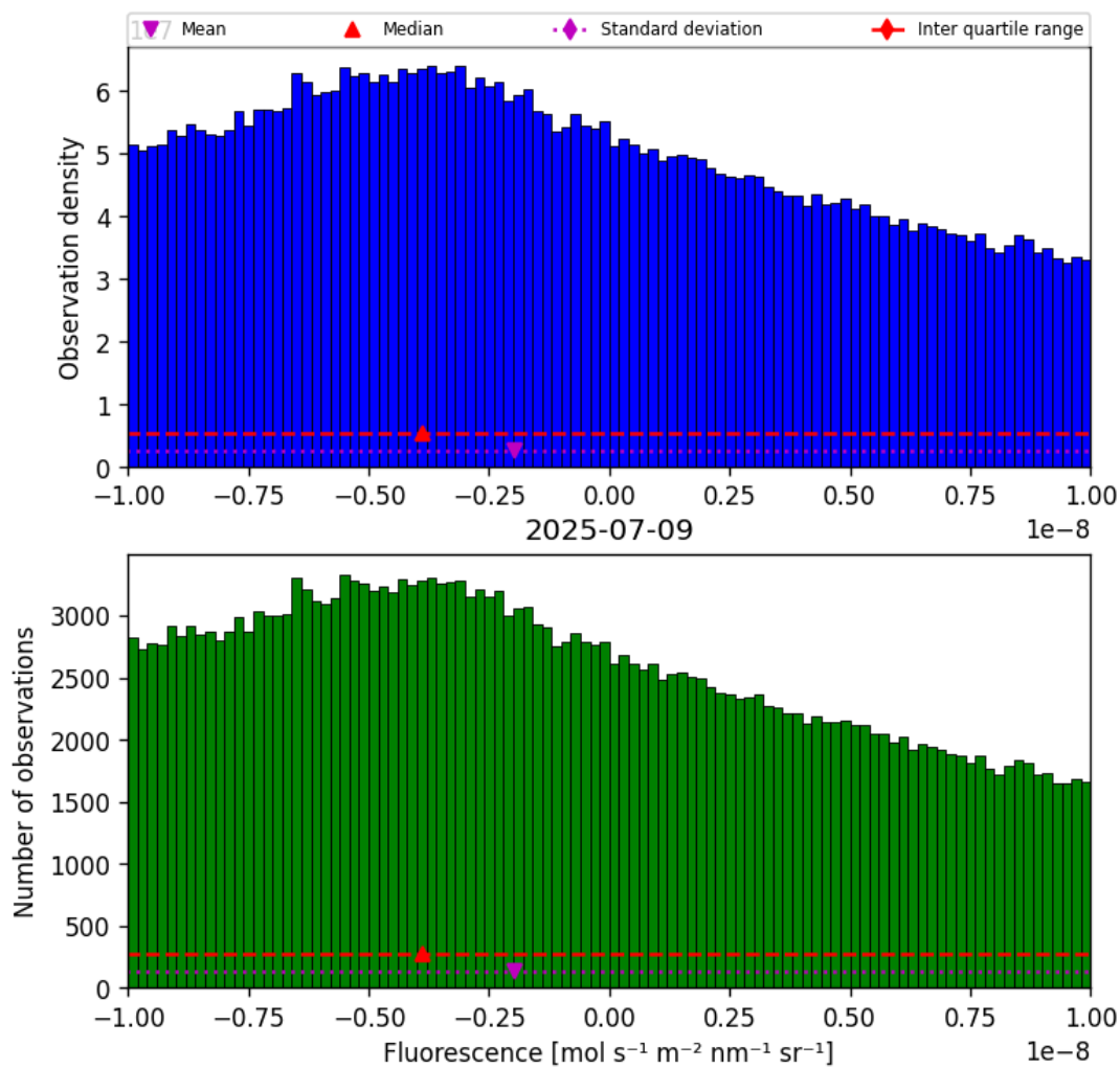
Figure 32: Histogram of “Fluorescence” for 2025-07-08 to 2025-07-10
