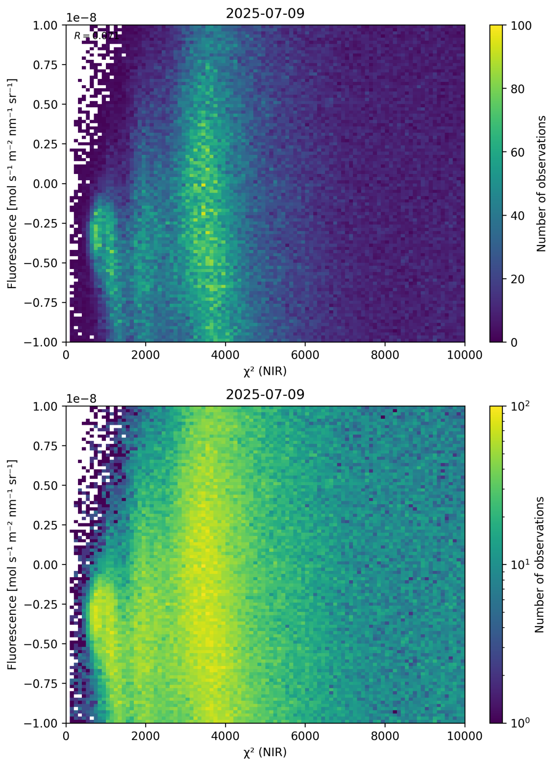
Figure 45: Scatter density plot of “ \chi^2 (NIR)” against “Fluorescence” for 2025-07-08 to 2025-07-10.
