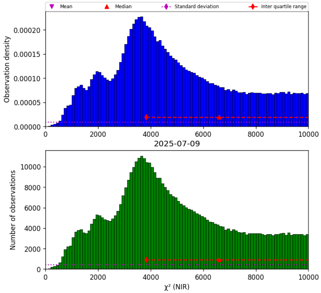
Figure 29: Histogram of “ \chi^2 (NIR)” for 2025-07-08 to 2025-07-10
