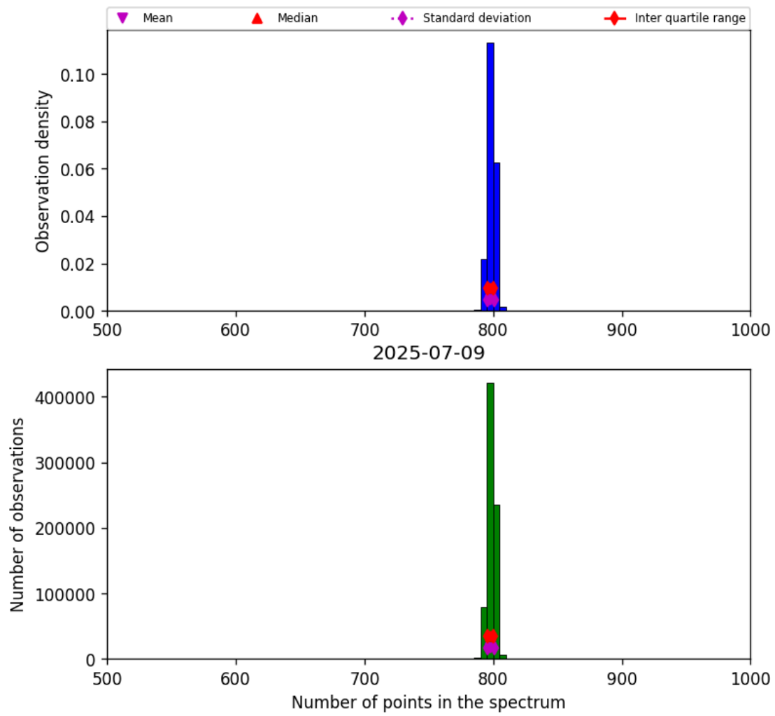
Figure 26: Histogram of “Number of points in the spectrum” for 2025-07-08 to 2025-07-10
