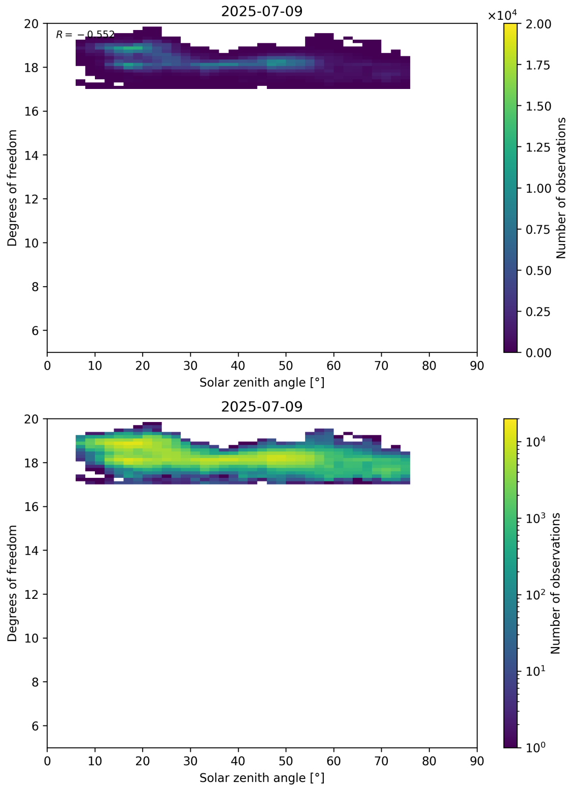
Figure 96: Scatter density plot of “Solar zenith angle” against “Degrees of freedom” for 2025-07-08 to 2025-07-10.
