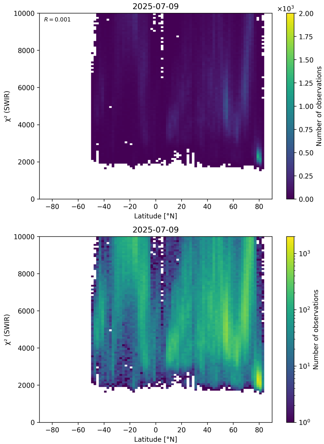
Figure 54: Scatter density plot of “Latitude” against “ \chi^2 (SWIR)” for 2025-07-08 to 2025-07-10.
