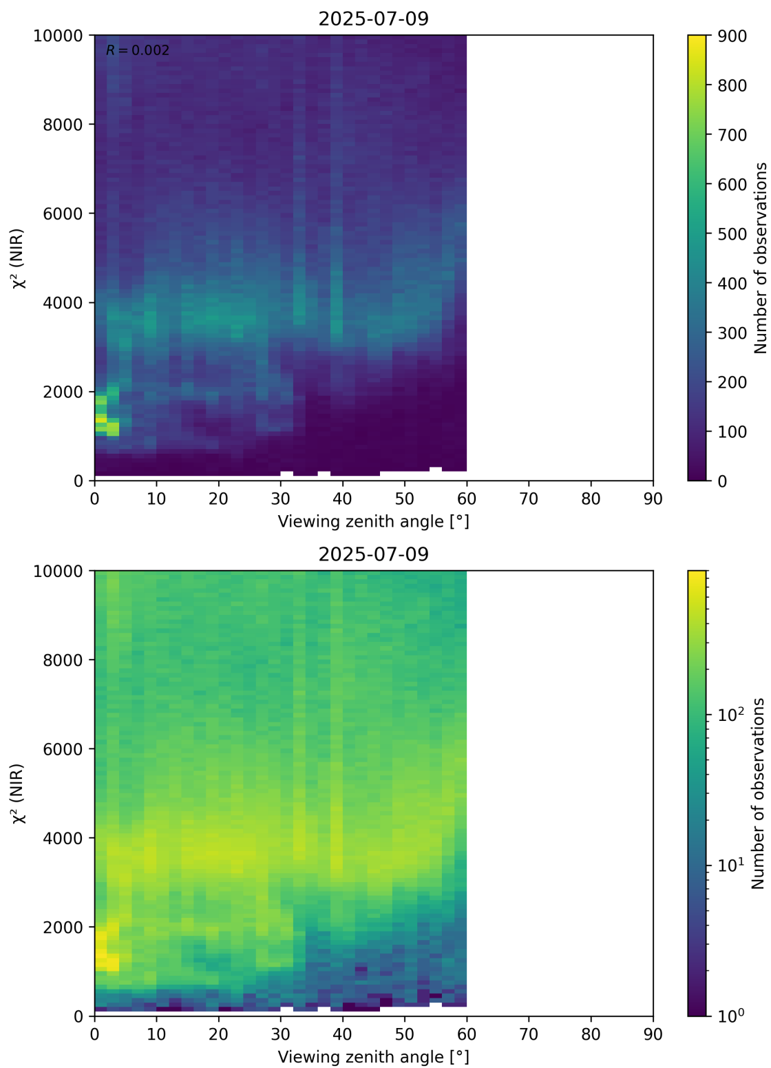
Figure 105: Scatter density plot of “Viewing zenith angle” against “ \chi^2 (NIR)” for 2025-07-08 to 2025-07-10.
