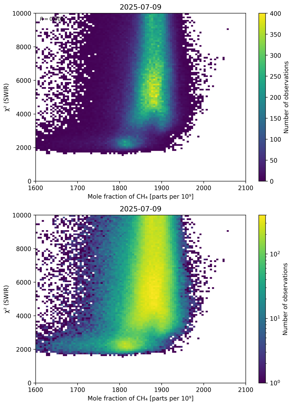
Figure 71: Scatter density plot of “Mole fraction of \text{CH}_4 ” against “ \chi^2 (SWIR)” for 2025-07-08 to 2025-07-10.
