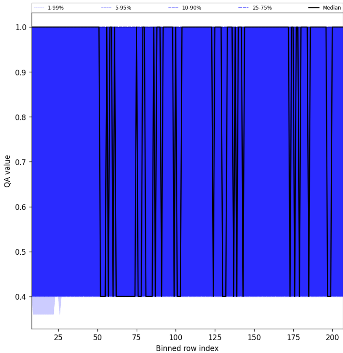
Figure 33: Along track statistics of "QA value" for 2025-07-08 to 2025-07-10
