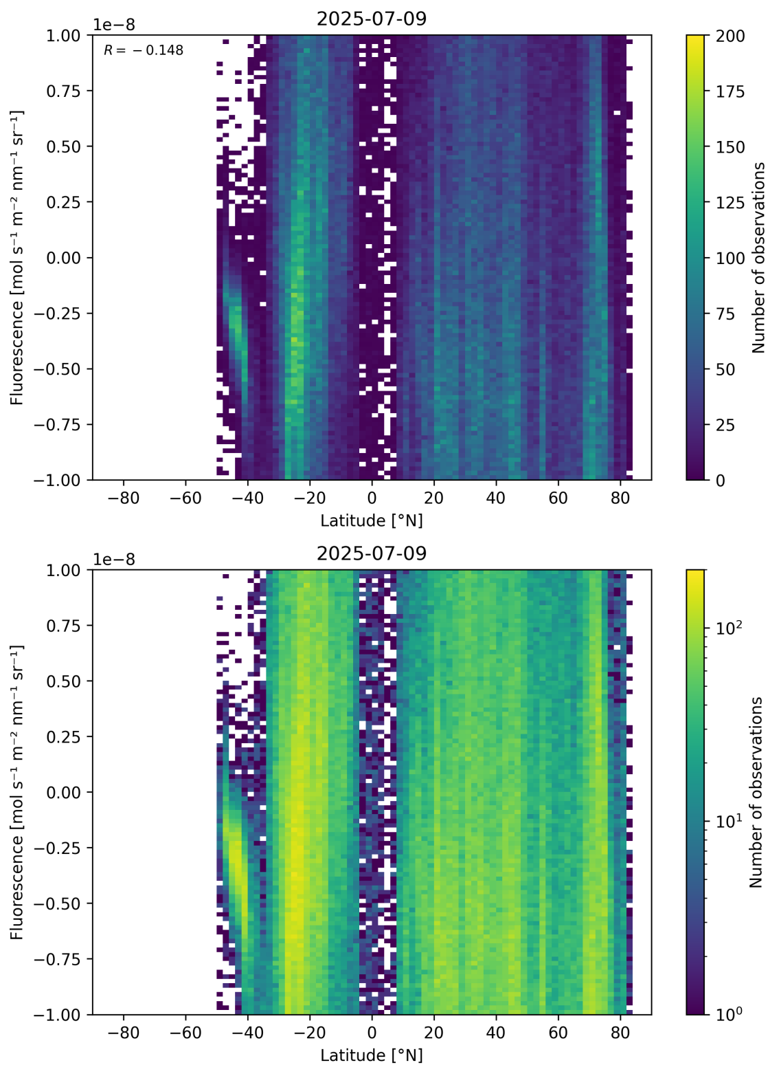
Figure 56: Scatter density plot of “Latitude” against “Fluorescence” for 2025-07-08 to 2025-07-10.
