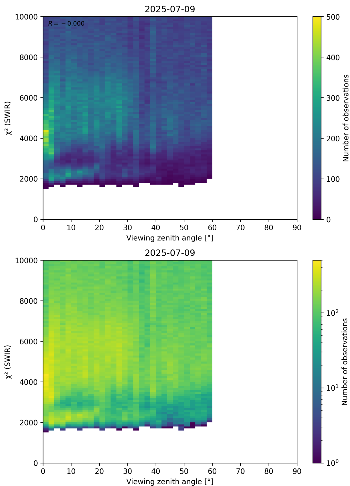
Figure 106: Scatter density plot of “Viewing zenith angle” against “ \chi^2 (SWIR)” for 2025-07-08 to 2025-07-10.
