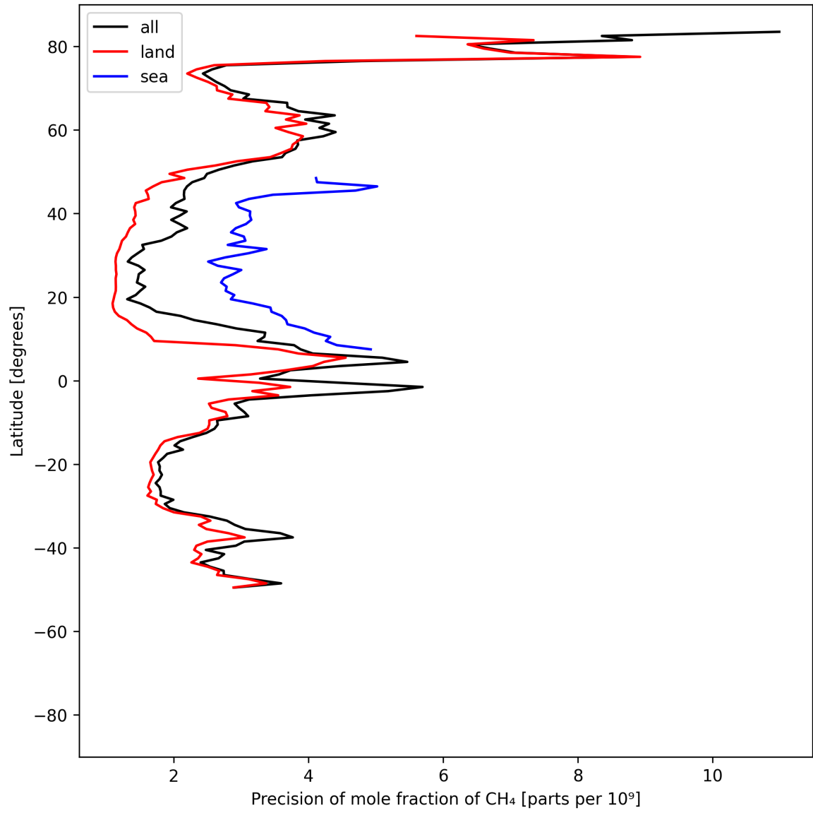
Figure 13: Zonal average of “Precision of mole fraction of CH 4 ” for 2025-07-08 to 2025-07-10.
