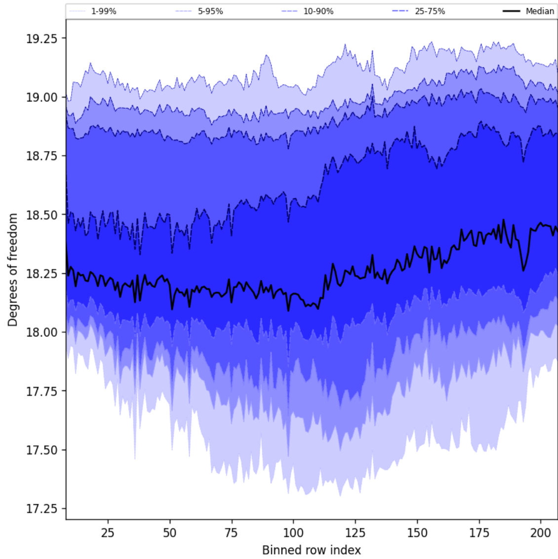
Figure 41: Along track statistics of “Degrees of freedom” for 2025-07-08 to 2025-07-10
