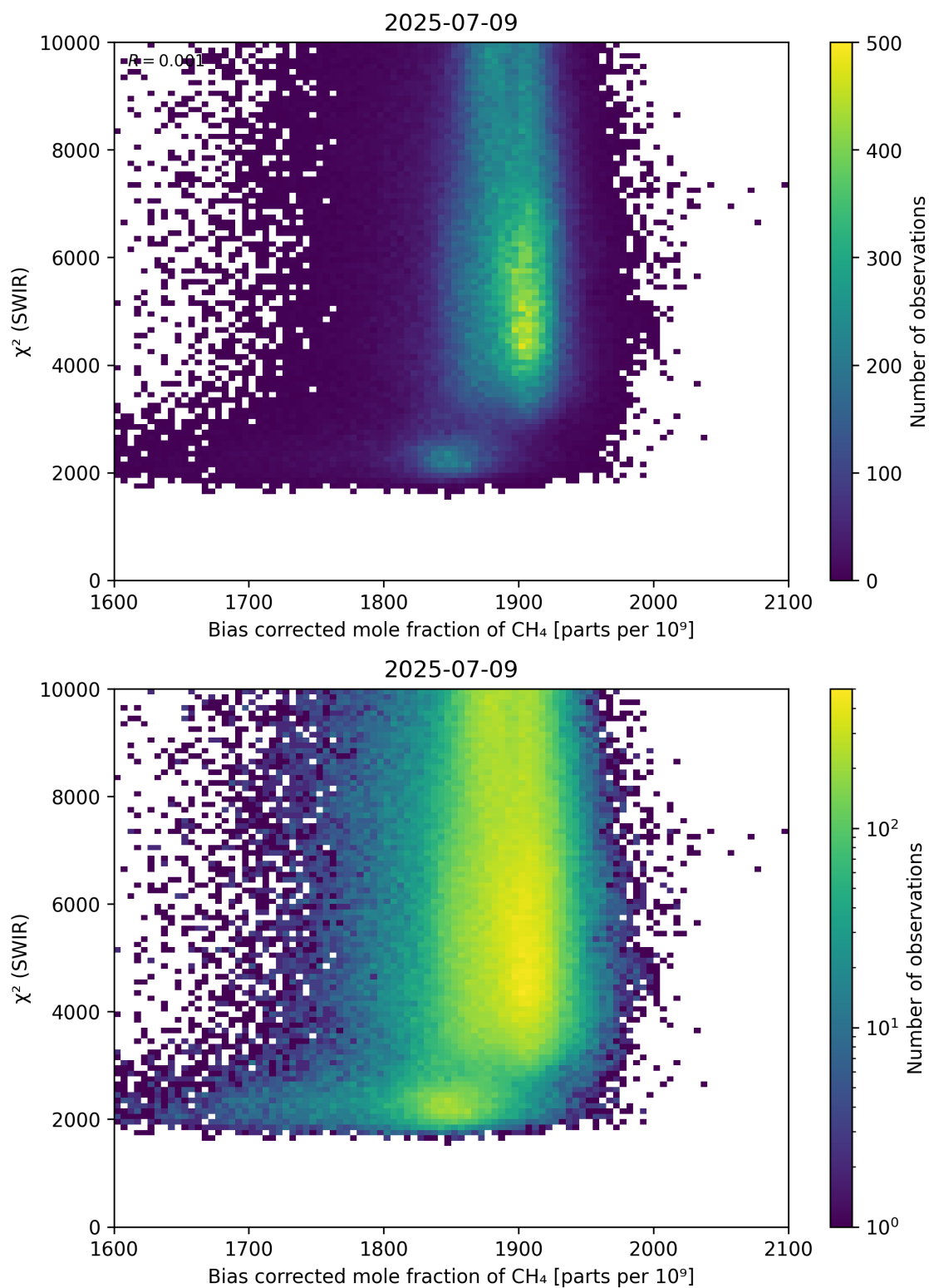
Figure 64: Scatter density plot of “Bias corrected mole fraction of \text{CH}_4 ” against “ \chi^2 (SWIR)” for 2025-07-08 to 2025-07-10.
