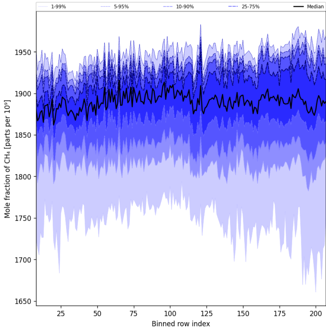
Figure 34: Along track statistics of “Mole fraction of CH 4 ” for 2025-07-08 to 2025-07-10
