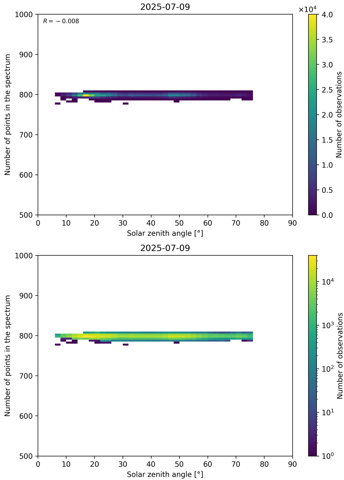
Figure 103: Scatter density plot of “Solar zenith angle” against “Number of points in the spectrum” for 2025-07-08 to 2025-07-10.
