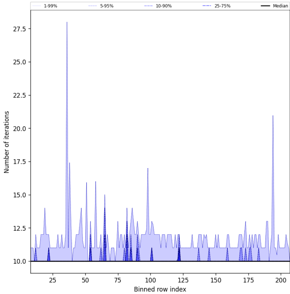
Figure 42: Along track statistics of “Number of iterations” for 2025-07-08 to 2025-07-10
