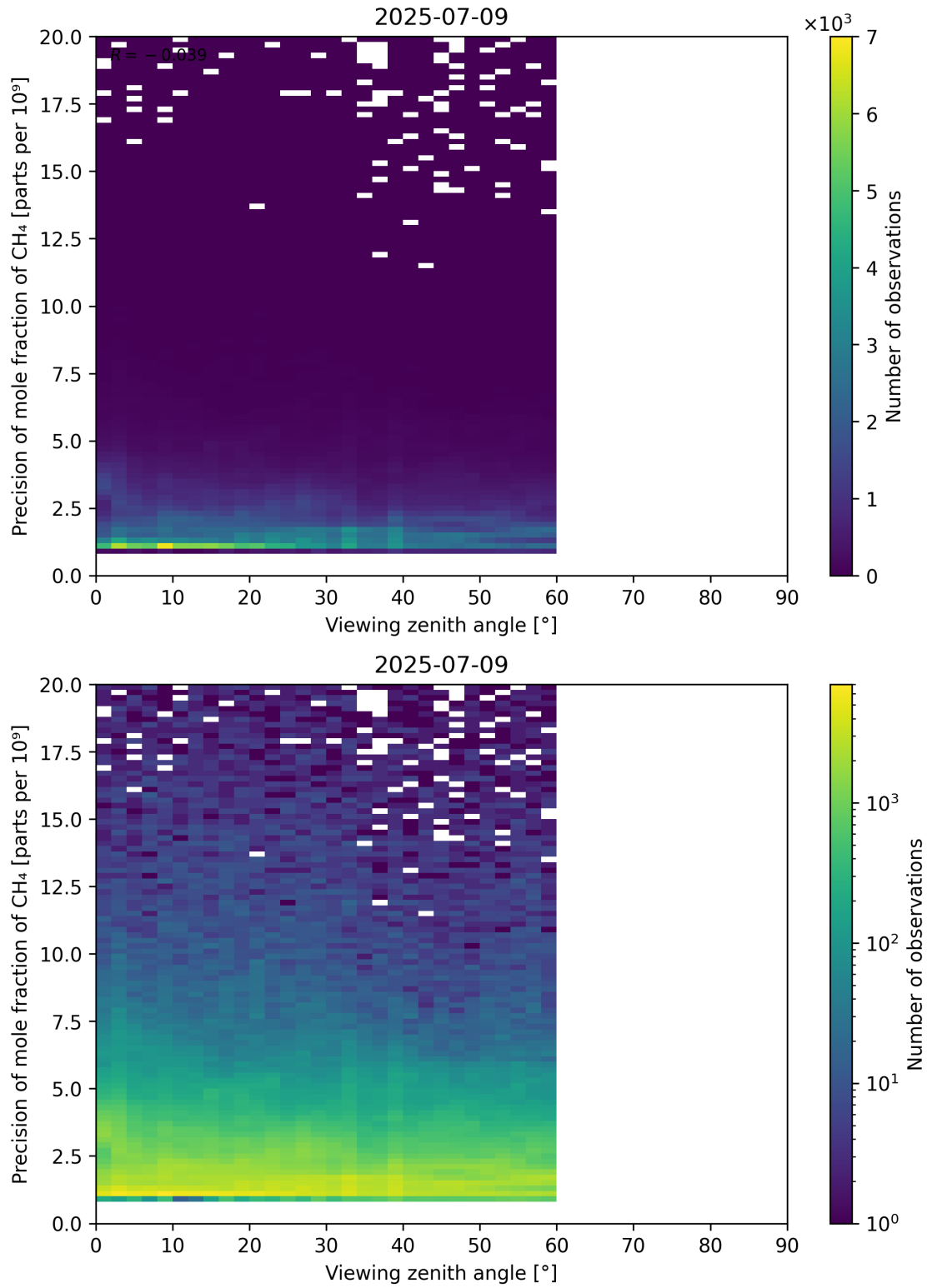
Figure 112: Scatter density plot of “Viewing zenith angle” against “Precision of mole fraction of CH 4 ” for 2025-07-08 to 2025-07-10.
