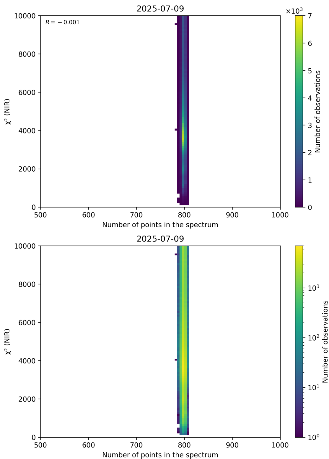
Figure 88: Scatter density plot of “Number of points in the spectrum” against “ \chi^2 (NIR)” for 2025-07-08 to 2025-07-10.
