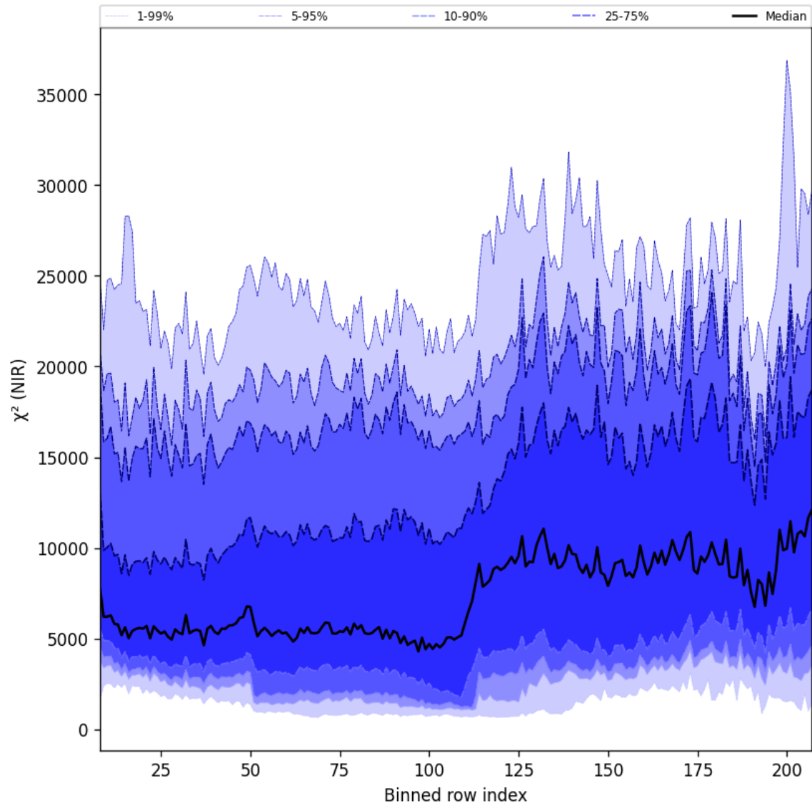
Figure 40: Along track statistics of “ \chi^2 (NIR)” for 2025-07-08 to 2025-07-10
