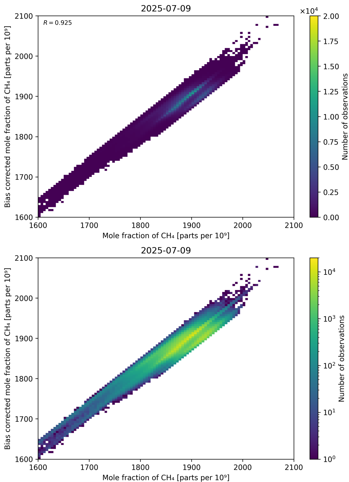
Figure 74: Scatter density plot of “Mole fraction of CH 4 ” against “Bias corrected mole fraction of CH 4 ” for 2025-07-08 to 2025-07-10.
