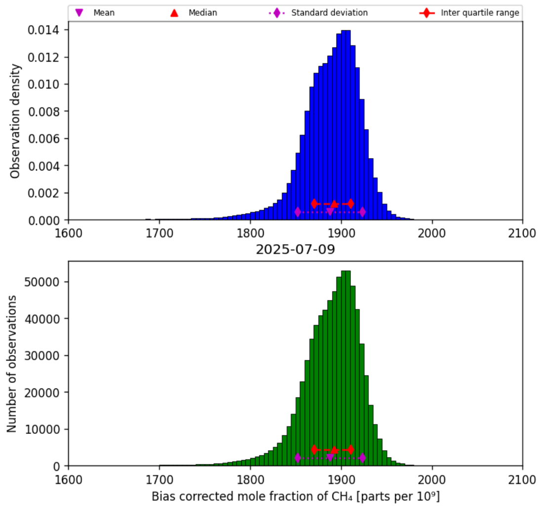
Figure 25: Histogram of “Bias corrected mole fraction of CH 4 ” for 2025-07-08 to 2025-07-10
