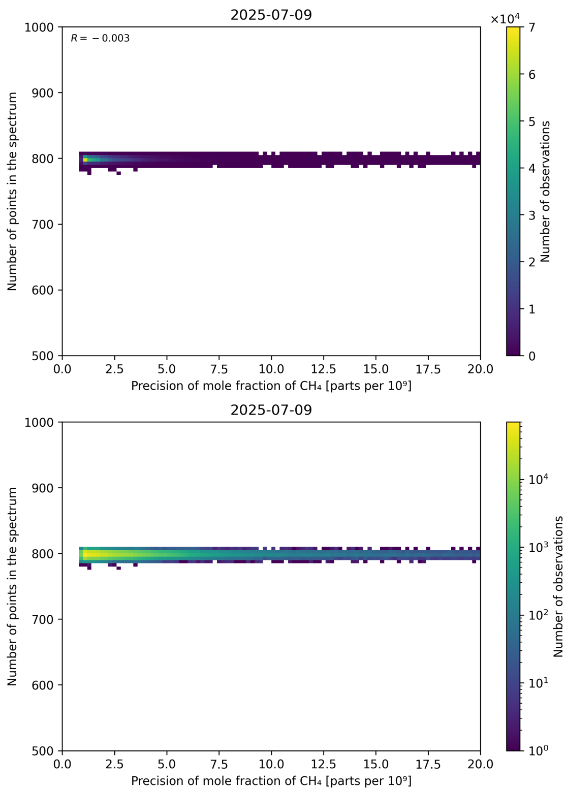
Figure 84: Scatter density plot of “Precision of mole fraction of CH 4 ” against “Number of points in the spectrum” for 2025-07-08 to 2025-07-10.
