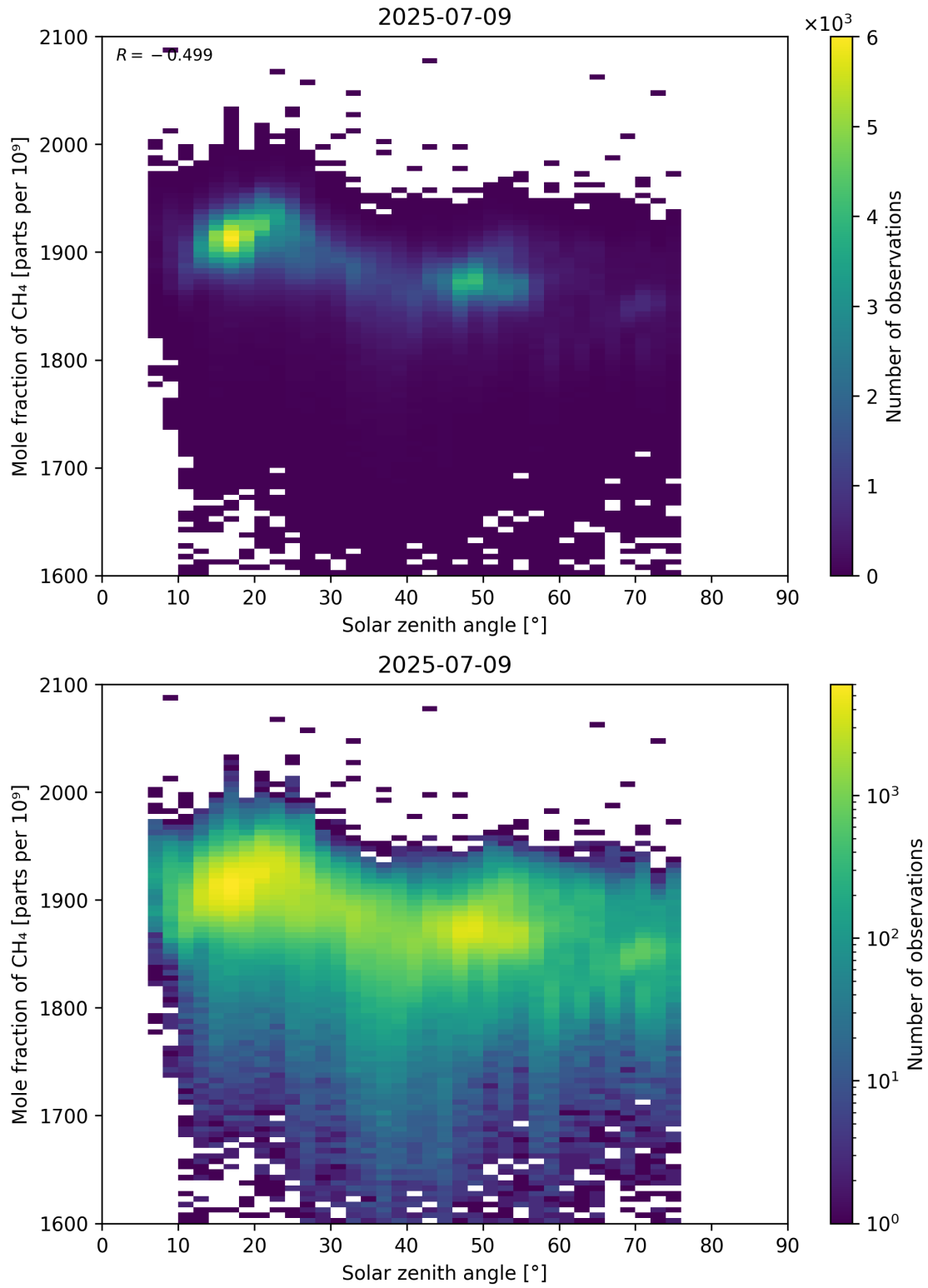
Figure 99: Scatter density plot of “Solar zenith angle” against “Mole fraction of CH 4 ” for 2025-07-08 to 2025-07-10.
