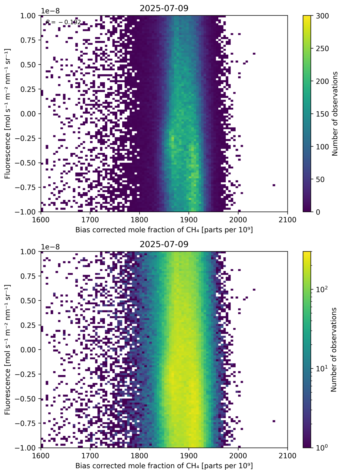
Figure 66: Scatter density plot of “Bias corrected mole fraction of \text{CH}_4 ” against “Fluorescence” for 2025-07-08 to 2025-07-10.
