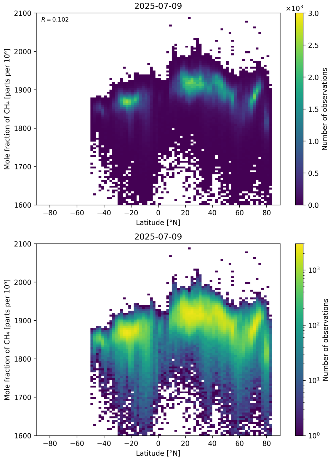
Figure 57: Scatter density plot of “Latitude” against “Mole fraction of CH 4 ” for 2025-07-08 to 2025-07-10.
