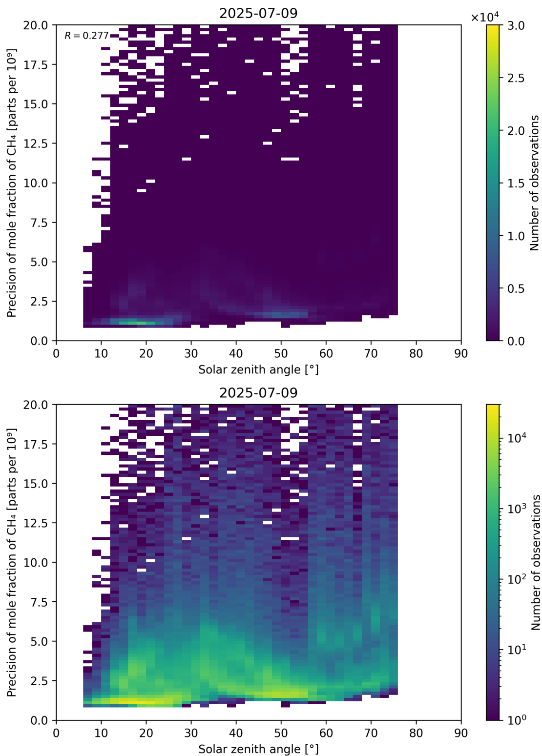
Figure 101: Scatter density plot of “Solar zenith angle” against “Precision of mole fraction of CH 4 ” for 2025-07-08 to 2025-07-10.
