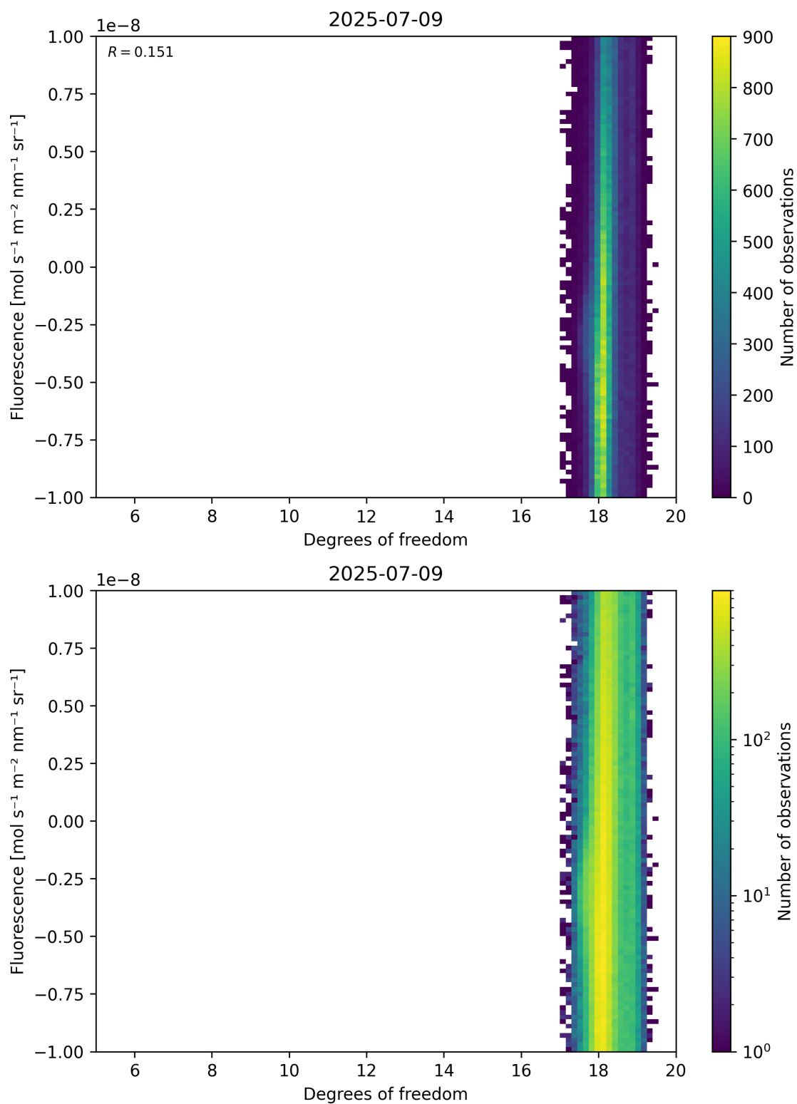
Figure 51: Scatter density plot of “Degrees of freedom” against “Fluorescence” for 2025-07-08 to 2025-07-10.
