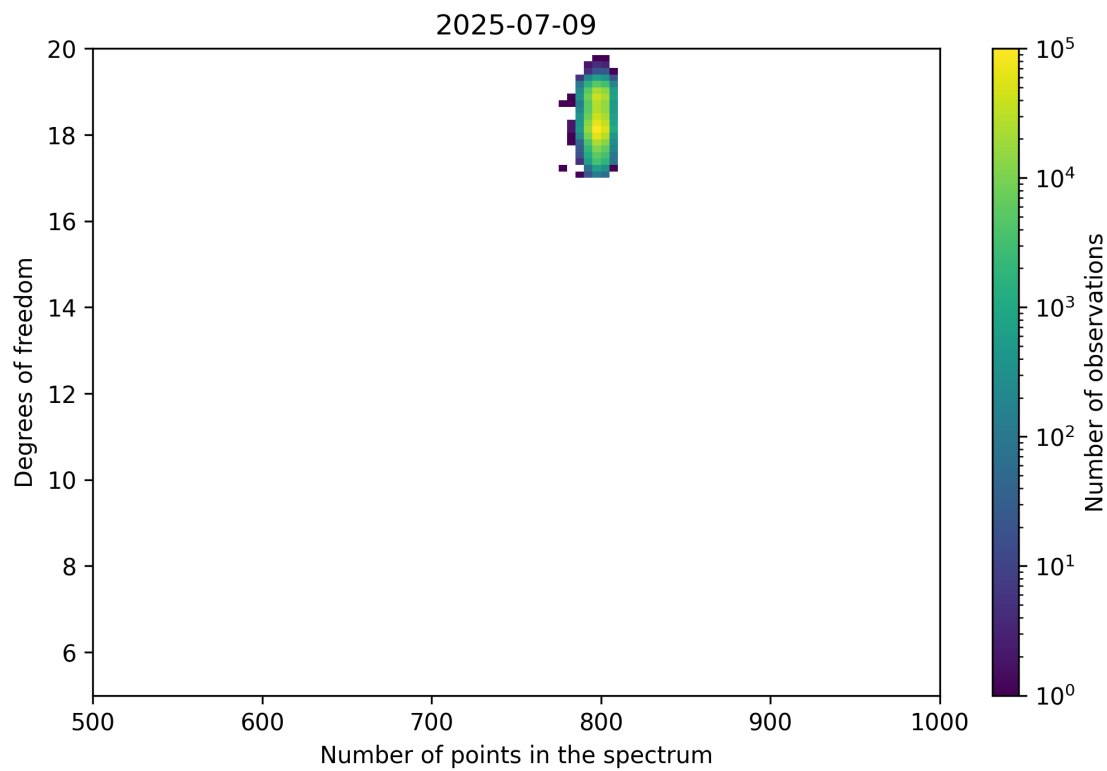
Figure 90: Scatter density plot of “Number of points in the spectrum” against “Degrees of freedom” for 2025-07-08 to 2025-07-10.
