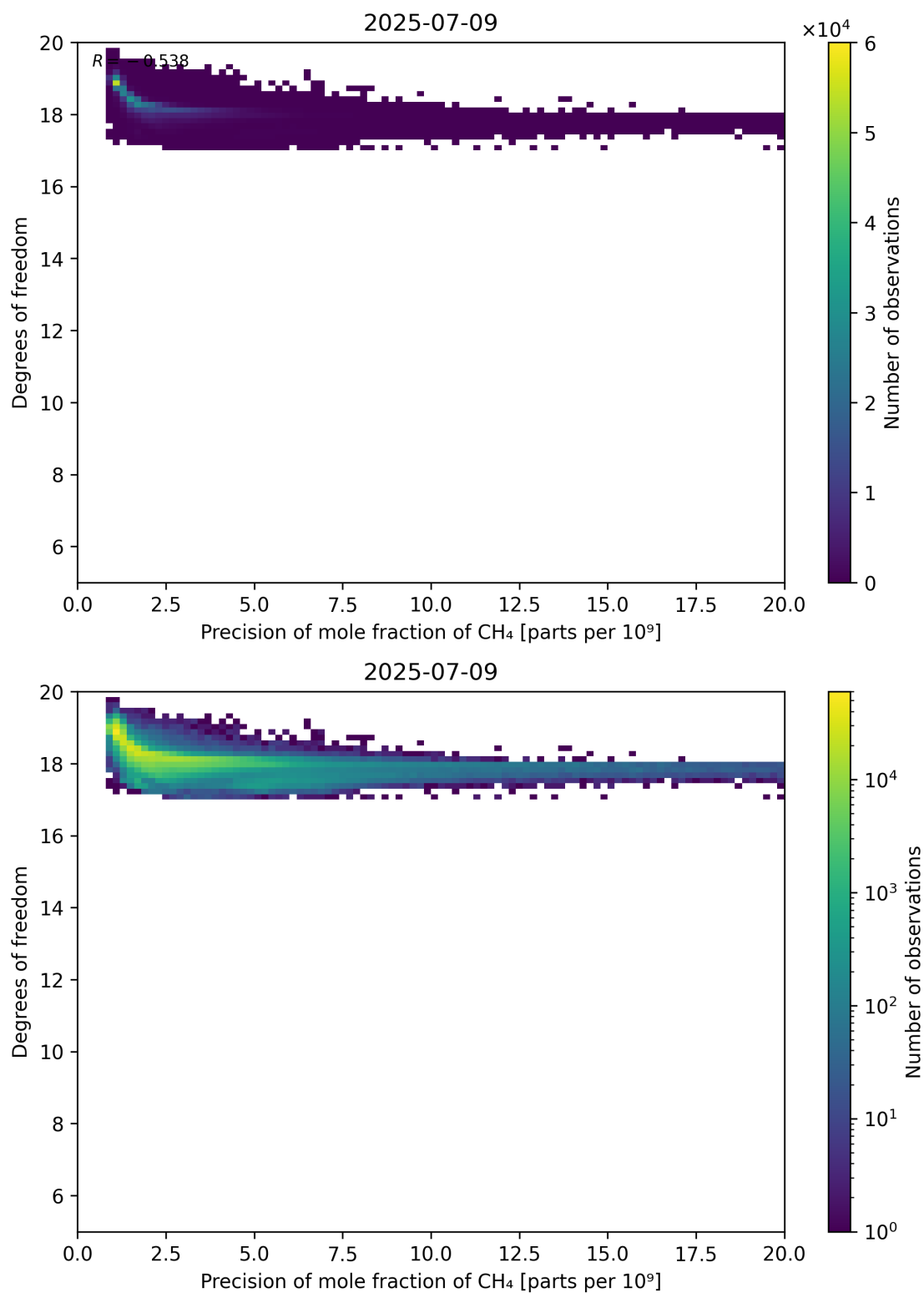
Figure 80: Scatter density plot of “Precision of mole fraction of CH 4 ” against “Degrees of freedom” for 2025-07-08 to 2025-07-10.
