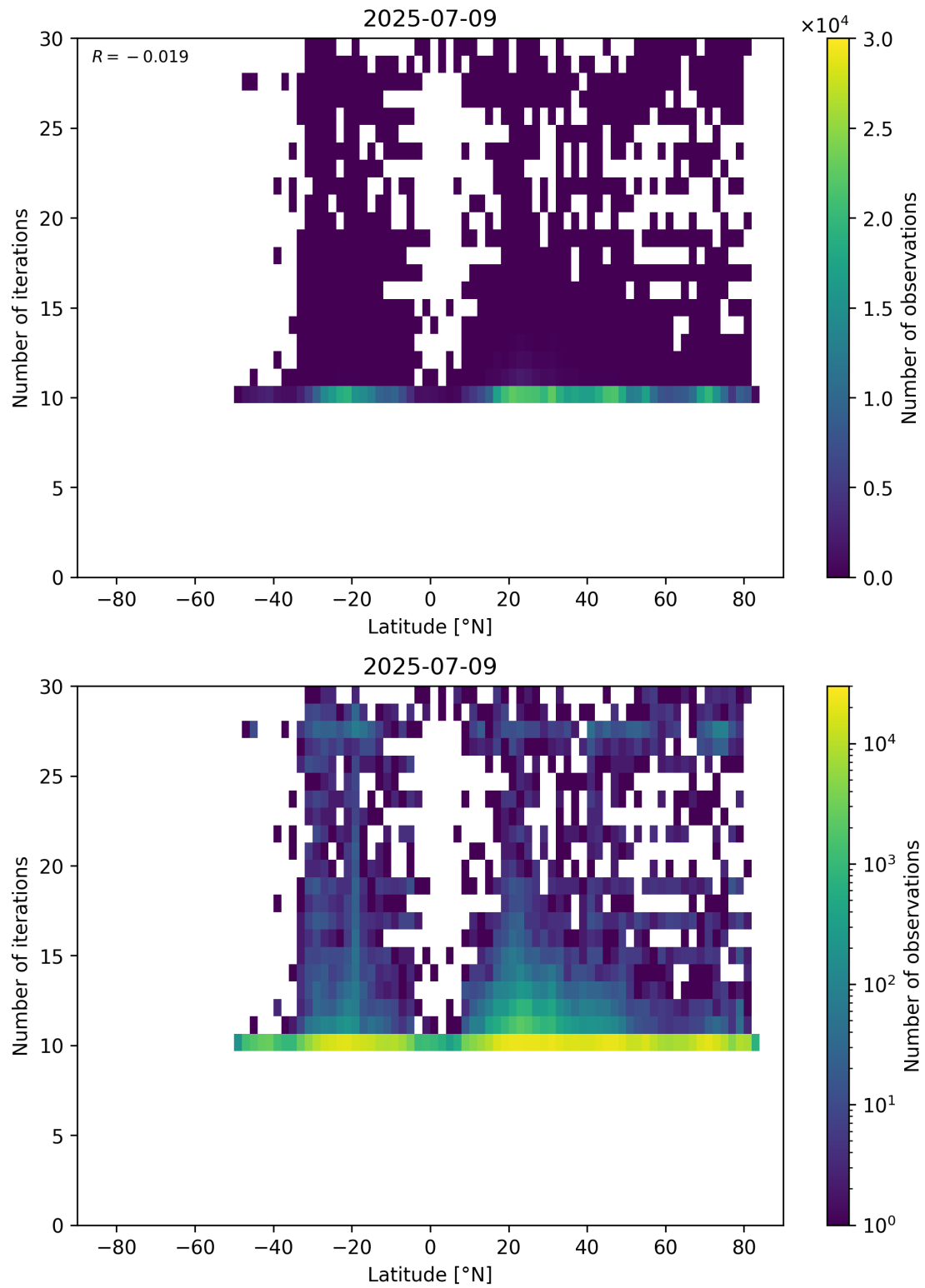
Figure 60: Scatter density plot of “Latitude” against “Number of iterations” for 2025-07-08 to 2025-07-10.
