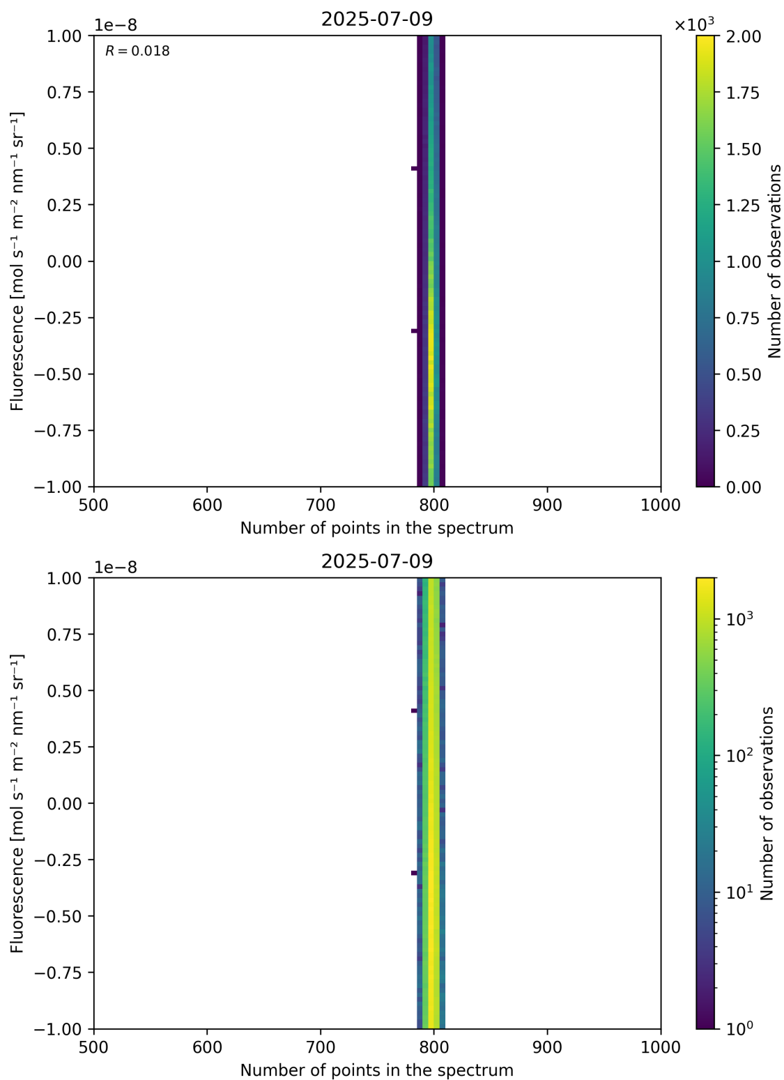
Figure 91: Scatter density plot of “Number of points in the spectrum” against “Fluorescence” for 2025-07-08 to 2025-07-10.
