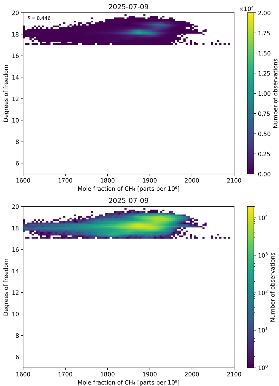
Figure 72: Scatter density plot of “Mole fraction of CH 4 ” against “Degrees of freedom” for 2025-07-08 to 2025-07-10.
