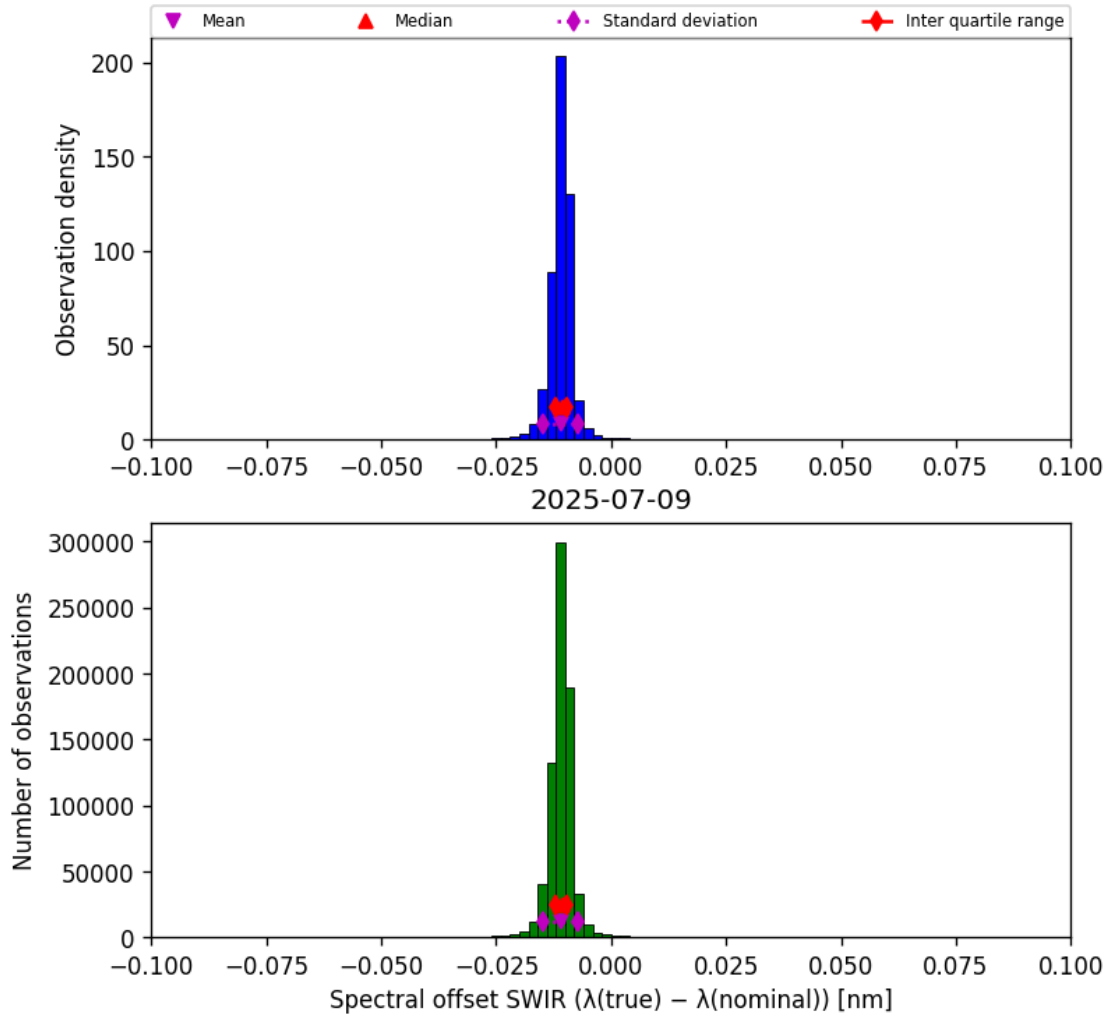
Figure 27: Histogram of “Spectral offset SWIR ( \lambda_{\text{true}} - \lambda_{\text{nominal}} )” for 2025-07-08 to 2025-07-10
