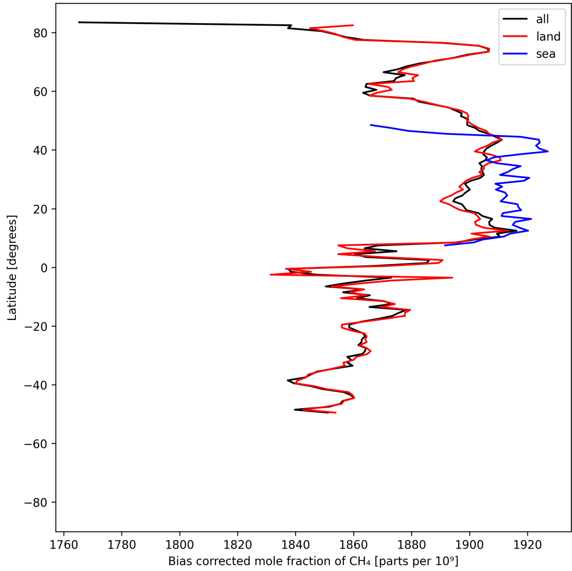
Figure 14: Zonal average of “Bias corrected mole fraction of \text{CH}_4 ” for 2025-07-08 to 2025-07-10.
