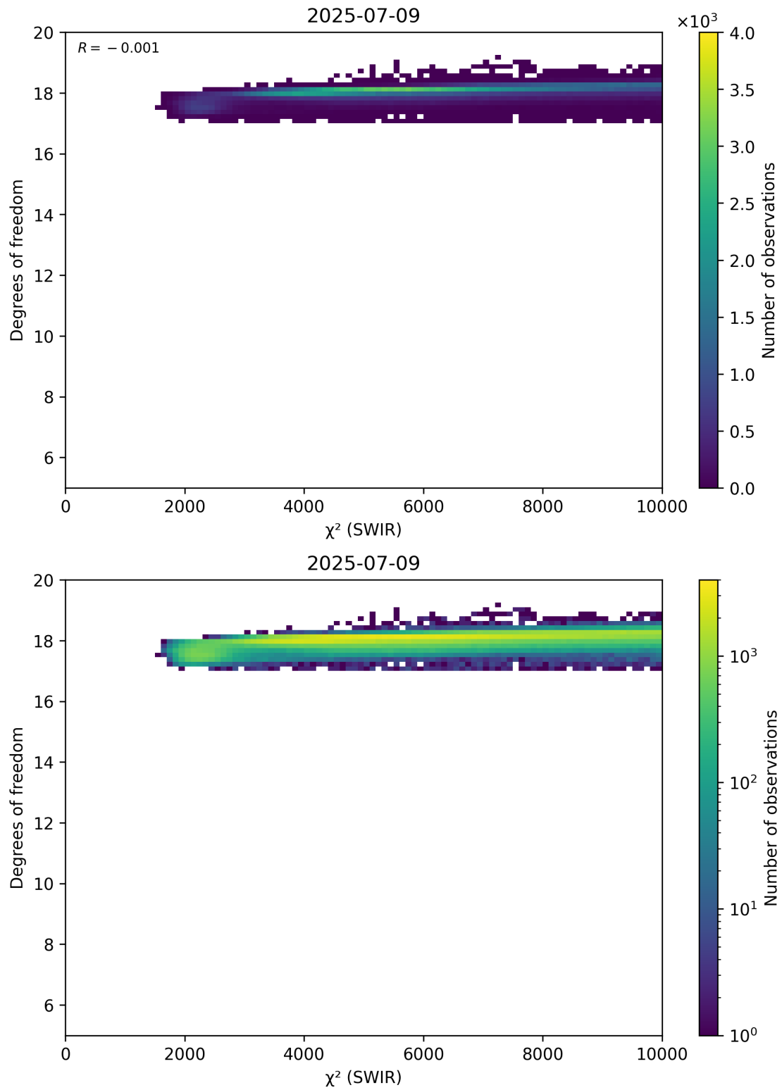
Figure 48: Scatter density plot of “ \chi^2 (SWIR)” against “Degrees of freedom” for 2025-07-08 to 2025-07-10.
