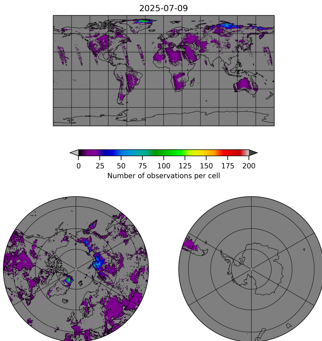
Figure 10: Map of the number of observations for 2025-07-08 to 2025-07-10
