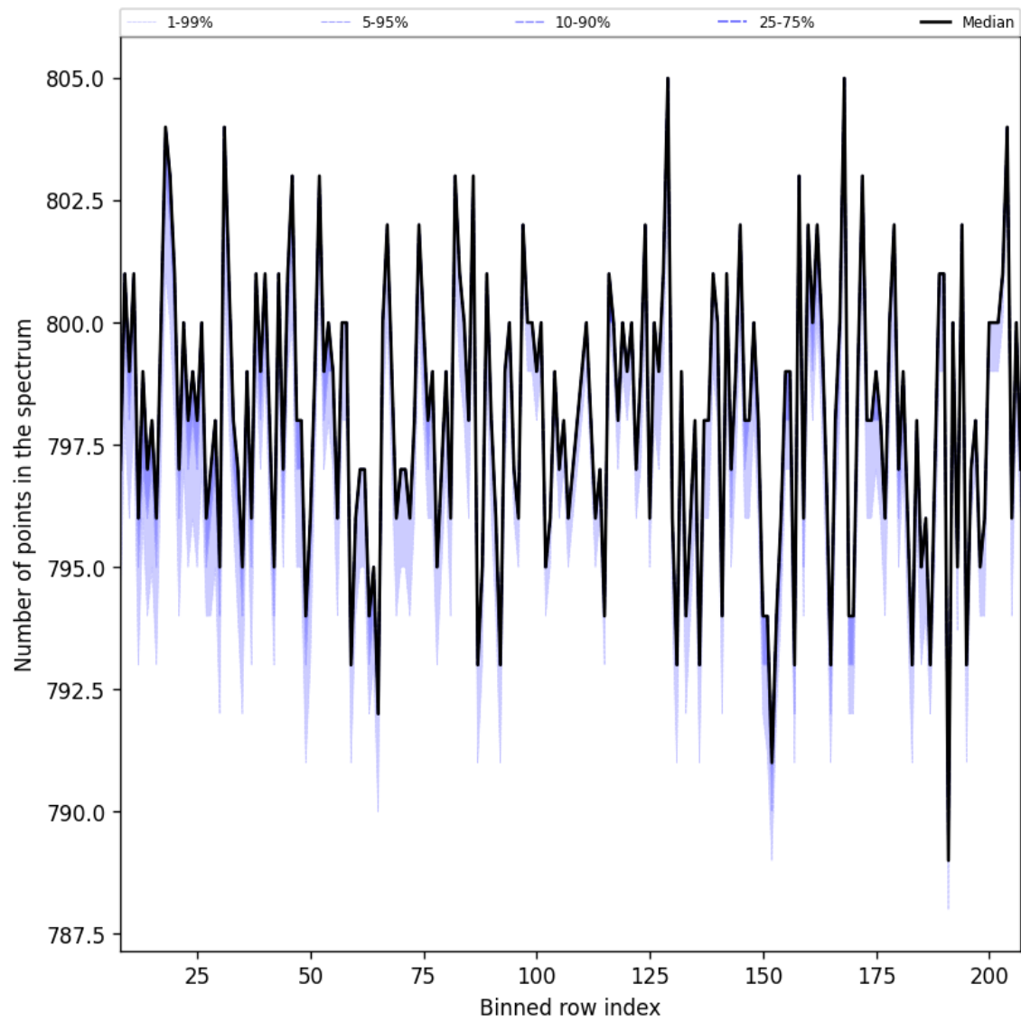
Figure 37: Along track statistics of “Number of points in the spectrum” for 2025-07-08 to 2025-07-10
