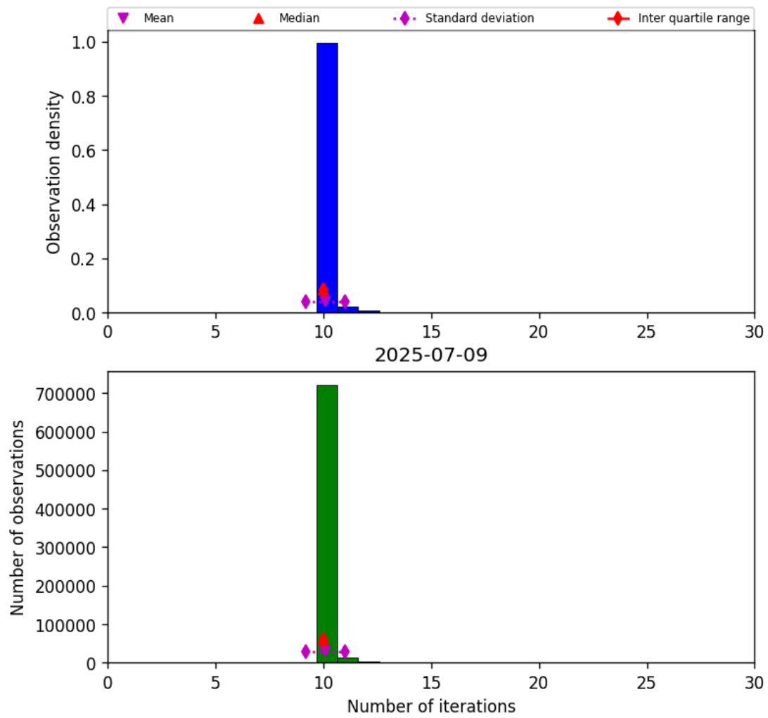
Figure 31: Histogram of “Number of iterations” for 2025-07-08 to 2025-07-10
