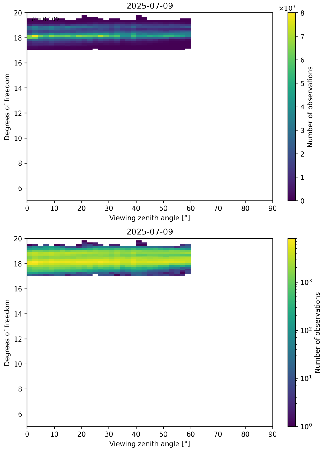
Figure 107: Scatter density plot of “Viewing zenith angle” against “Degrees of freedom” for 2025-07-08 to 2025-07-10.
