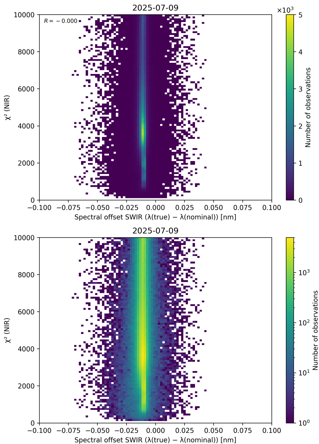
Figure 117: Scatter density plot of “Spectral offset SWIR ( \lambda_{\text{true}} - \lambda_{\text{nominal}} )” against “ \chi^2 (NIR)” for 2025-07-08 to 2025-07-10.
