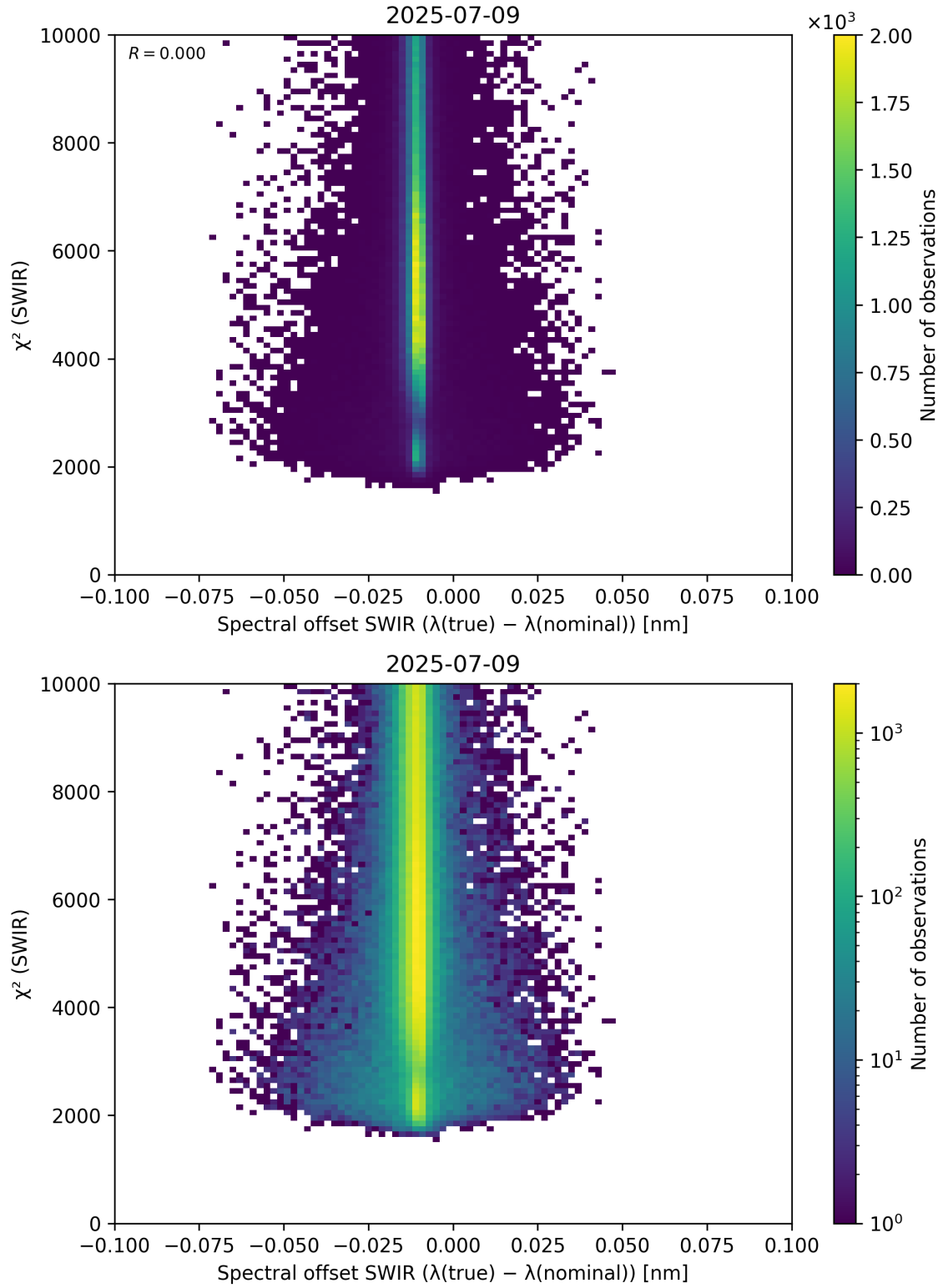
Figure 118: Scatter density plot of “Spectral offset SWIR ( \lambda_{\text{true}} - \lambda_{\text{nominal}} )” against “ \chi^2 (SWIR)” for 2025-07-08 to 2025-07-10.
