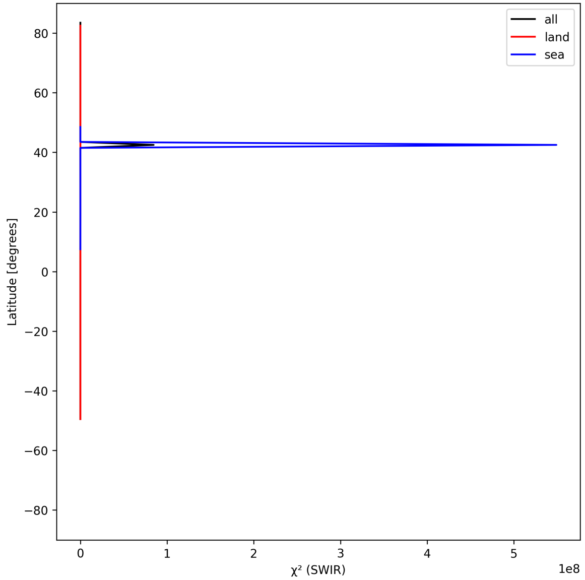
Figure 17: Zonal average of “ \chi^2 (SWIR)” for 2025-07-08 to 2025-07-10.
