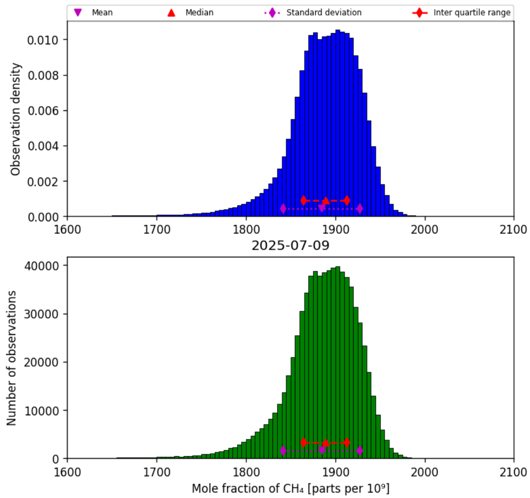
Figure 23: Histogram of “Mole fraction of CH 4 ” for 2025-07-08 to 2025-07-10
