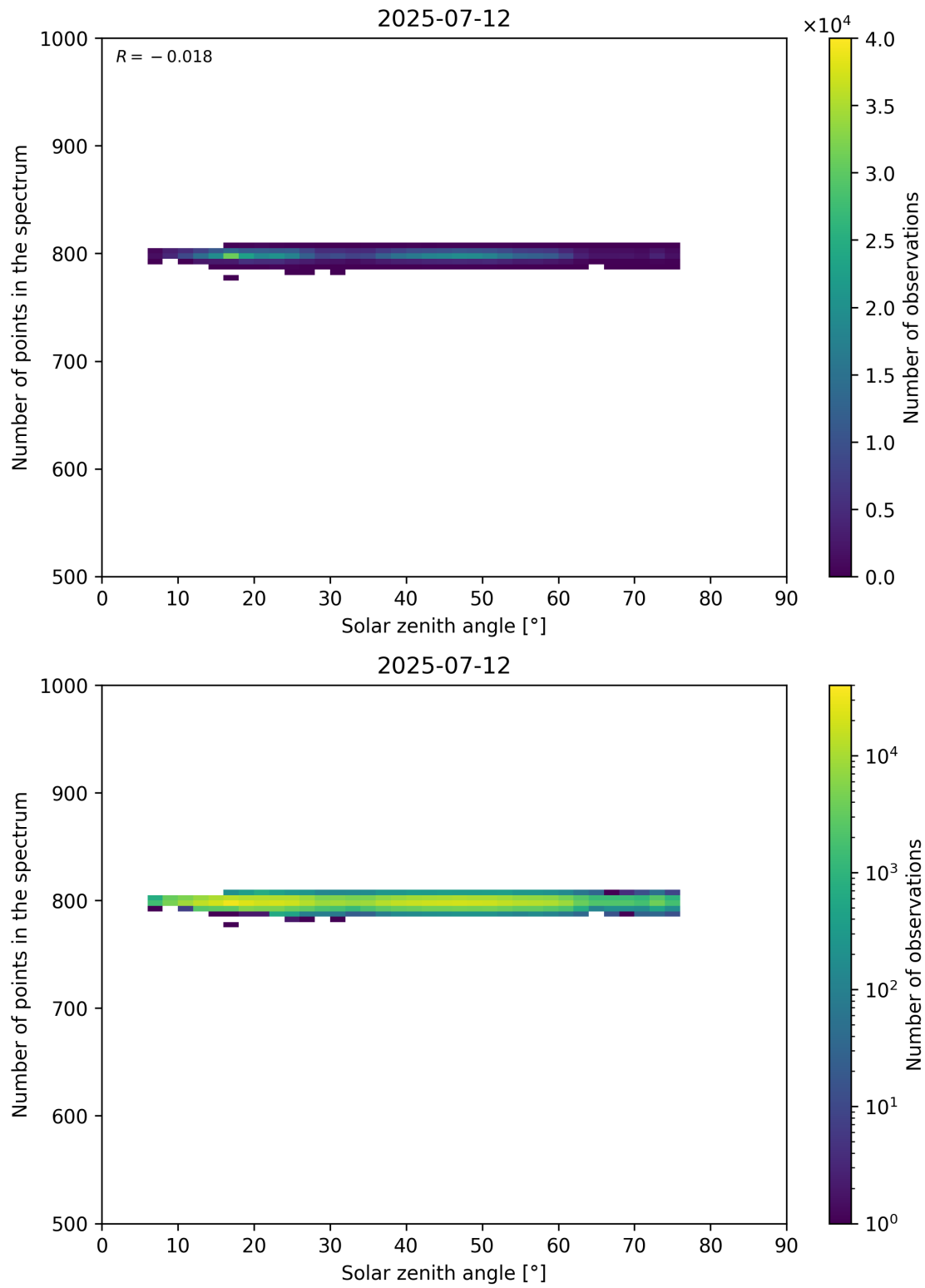
Figure 103: Scatter density plot of “Solar zenith angle” against “Number of points in the spectrum” for 2025-07-11 to 2025-07-13.
