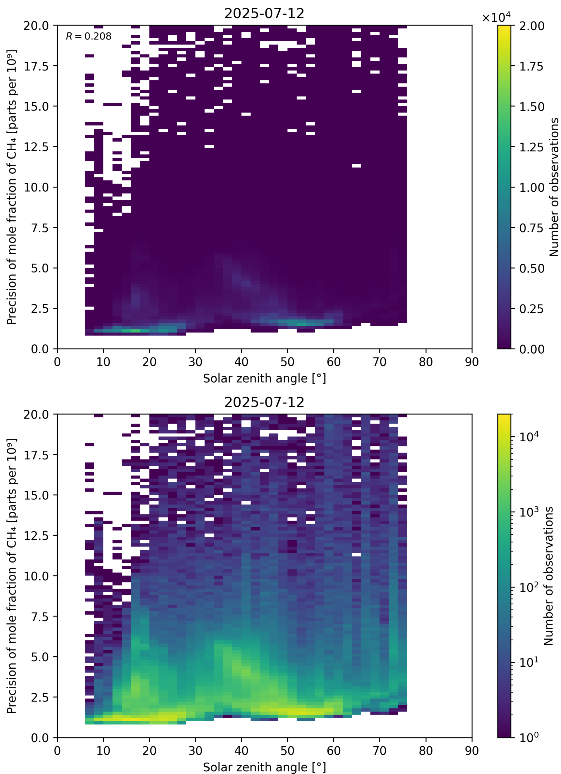
Figure 101: Scatter density plot of “Solar zenith angle” against “Precision of mole fraction of \text{CH}_4 ” for 2025-07-11 to 2025-07-13.
