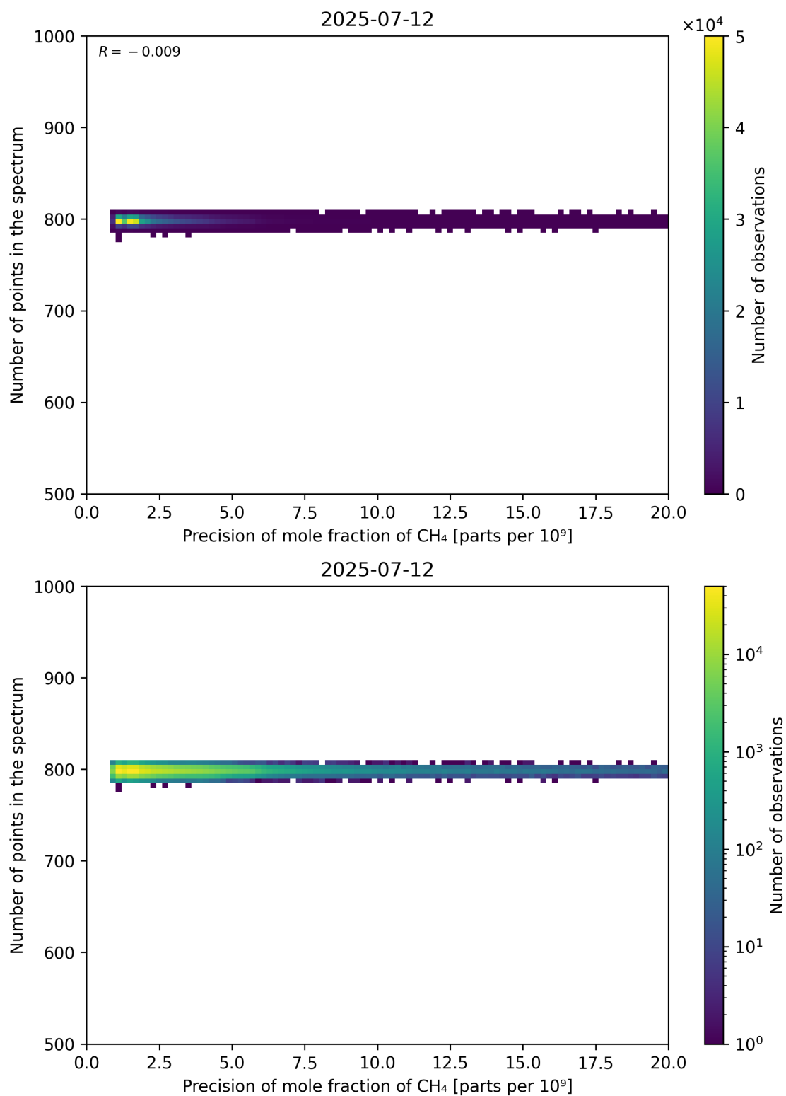
Figure 84: Scatter density plot of “Precision of mole fraction of CH 4 ” against “Number of points in the spectrum” for 2025-07-11 to 2025-07-13.
