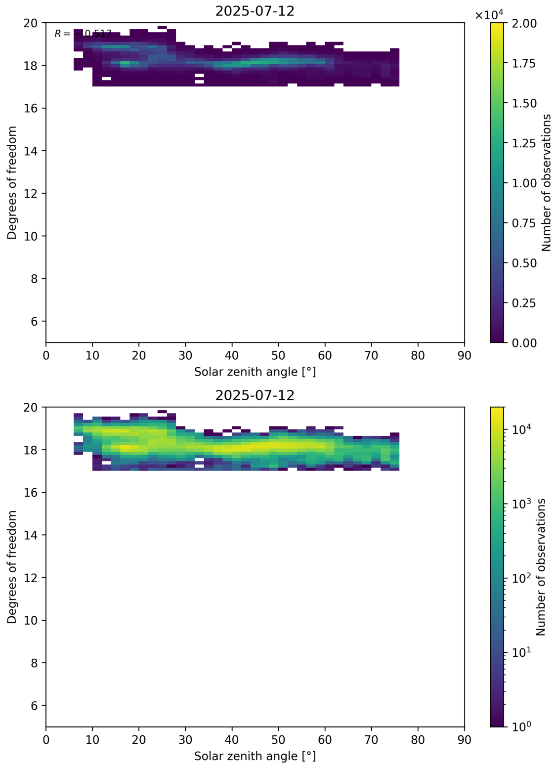
Figure 96: Scatter density plot of “Solar zenith angle” against “Degrees of freedom” for 2025-07-11 to 2025-07-13.
