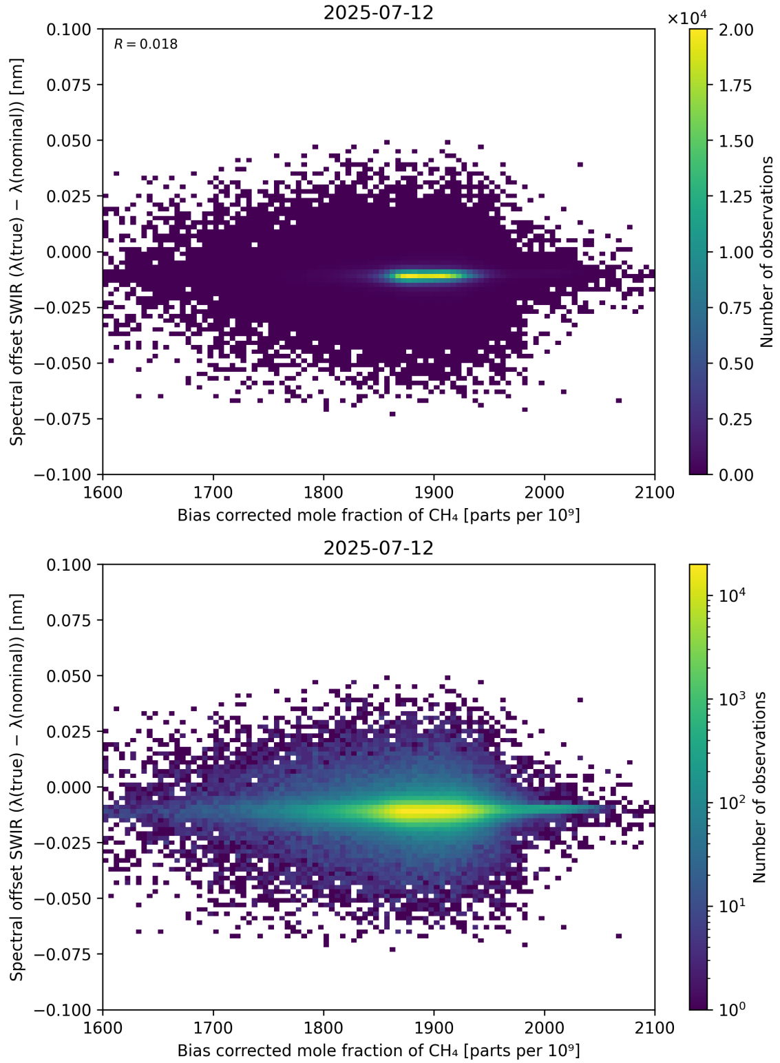
Figure 69: Scatter density plot of “Bias corrected mole fraction of CH 4 ” against “Spectral offset SWIR ( \lambda_{\text{true}} - \lambda_{\text{nominal}} )” for 2025-07-11 to 2025-07-13.
