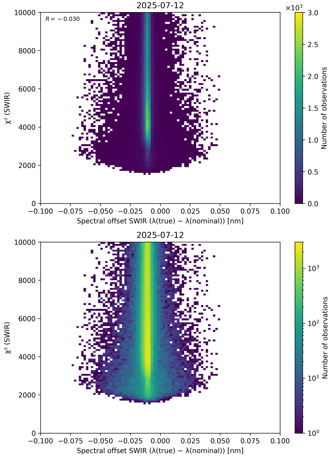
Figure 118: Scatter density plot of “Spectral offset SWIR ( \lambda_{\text{true}} - \lambda_{\text{nominal}} )” against “ \chi^2 (SWIR)” for 2025-07-11 to 2025-07-13.
