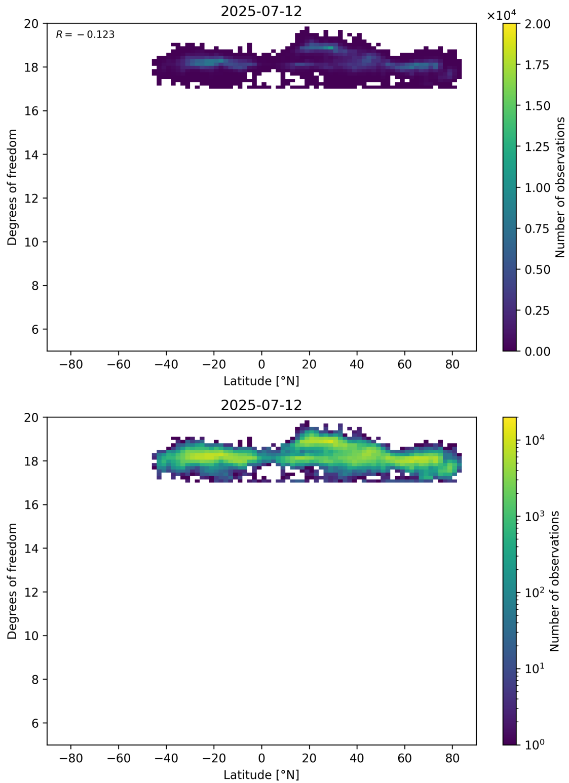
Figure 55: Scatter density plot of “Latitude” against “Degrees of freedom” for 2025-07-11 to 2025-07-13.
