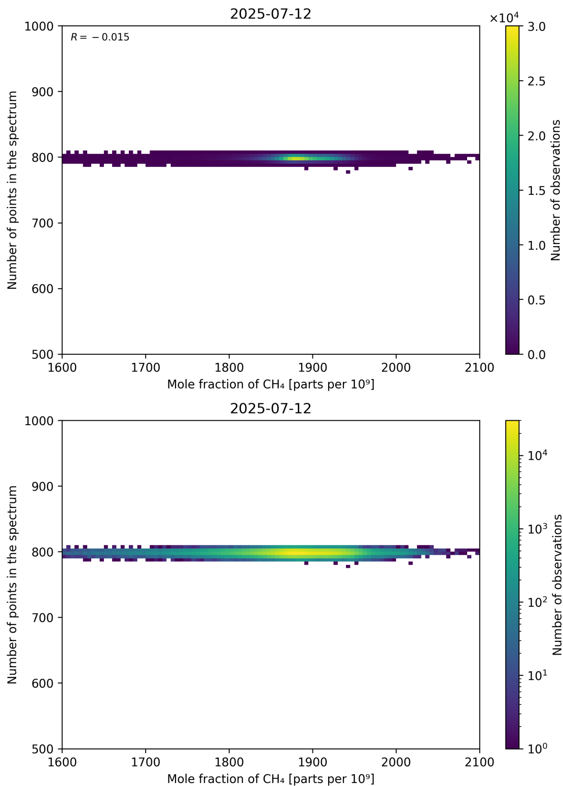
Figure 77: Scatter density plot of “Mole fraction of CH 4 ” against “Number of points in the spectrum” for 2025-07-11 to 2025-07-13.
