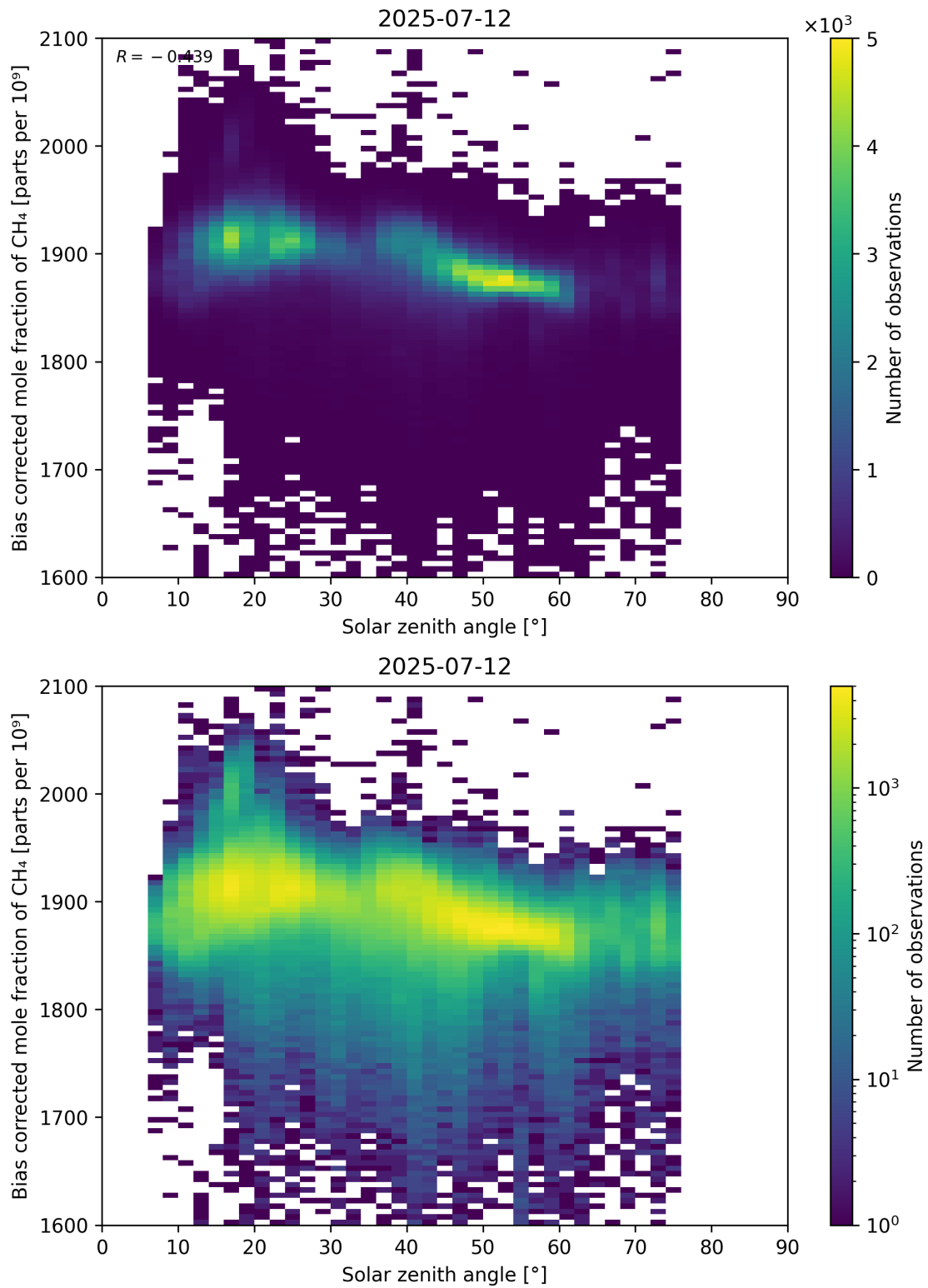
Figure 100: Scatter density plot of “Solar zenith angle” against “Bias corrected mole fraction of \text{CH}_4 ” for 2025-07-11 to 2025-07-13.
