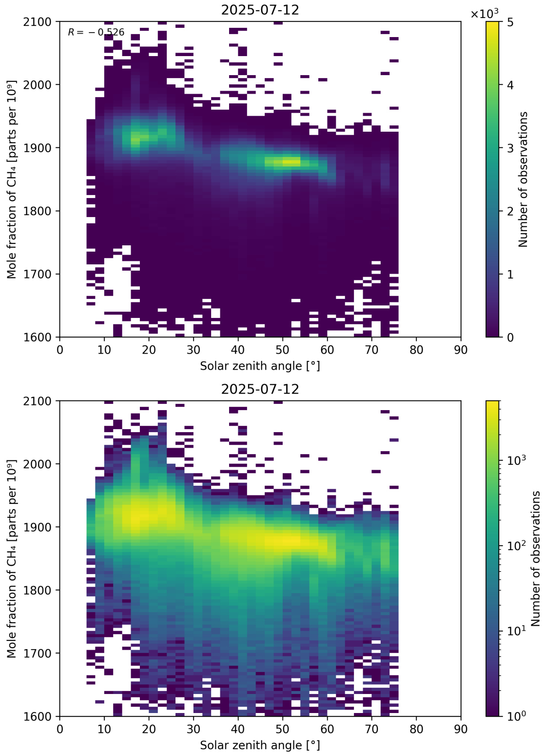
Figure 99: Scatter density plot of “Solar zenith angle” against “Mole fraction of CH 4 ” for 2025-07-11 to 2025-07-13.
