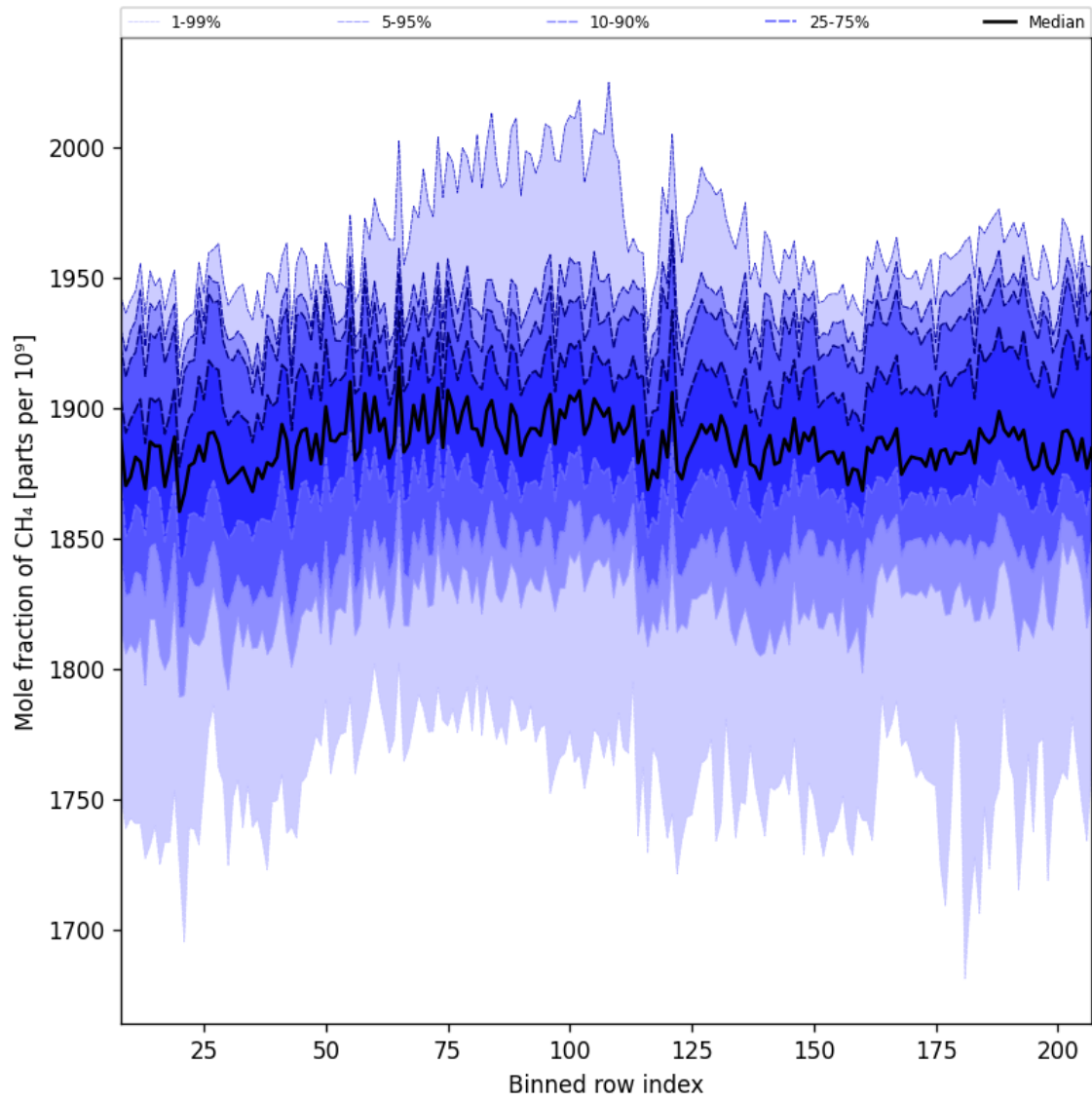
Figure 34: Along track statistics of “Mole fraction of CH 4 ” for 2025-07-11 to 2025-07-13
