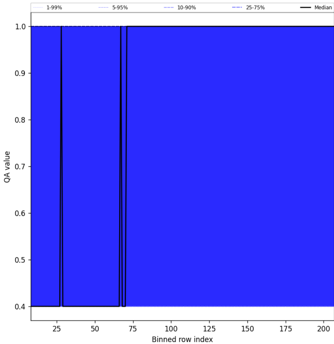
Figure 33: Along track statistics of “QA value” for 2025-07-11 to 2025-07-13
