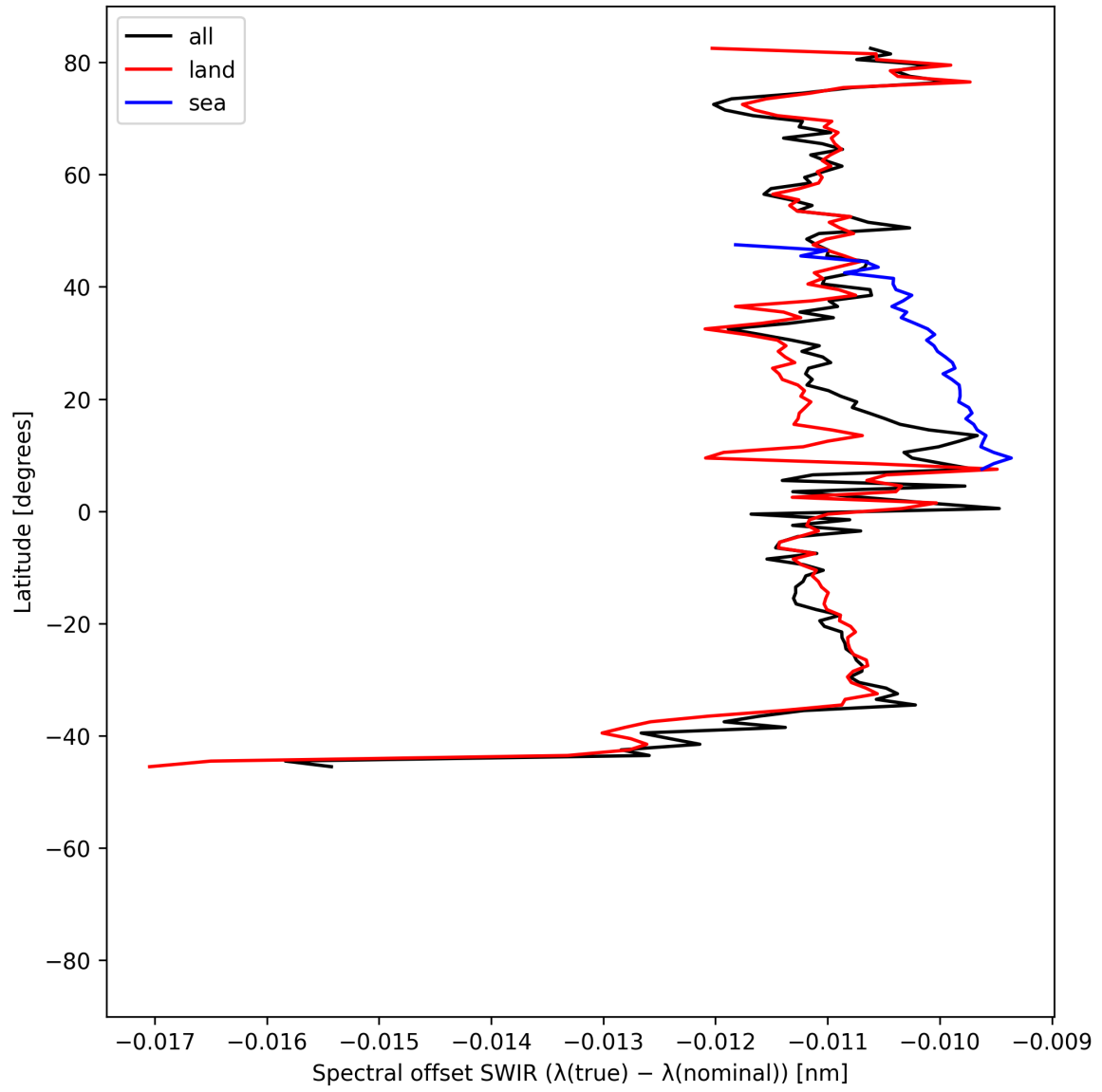
Figure 16: Zonal average of “Spectral offset SWIR ( \lambda_{\text{true}} - \lambda_{\text{nominal}} )” for 2025-07-11 to 2025-07-13.
