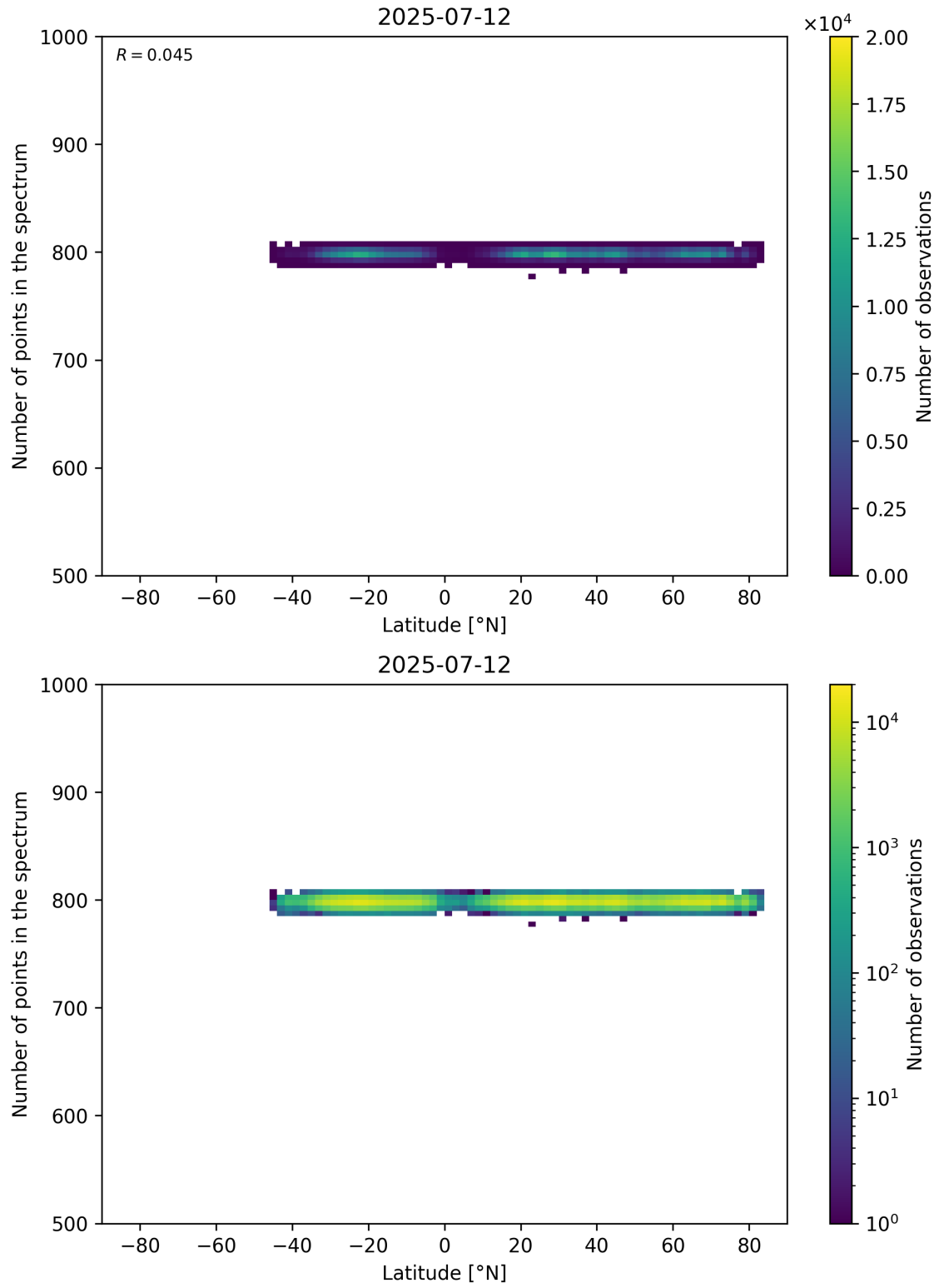
Figure 61: Scatter density plot of “Latitude” against “Number of points in the spectrum” for 2025-07-11 to 2025-07-13.
