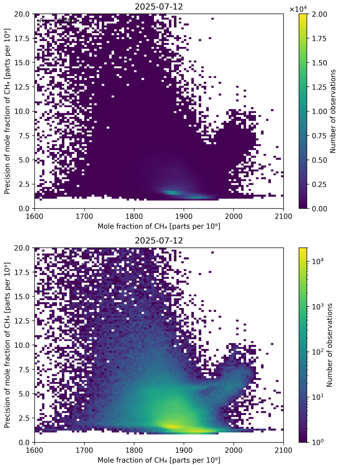
Figure 75: Scatter density plot of “Mole fraction of CH 4 ” against “Precision of mole fraction of CH 4 ” for 2025-07-11 to 2025-07-13.
