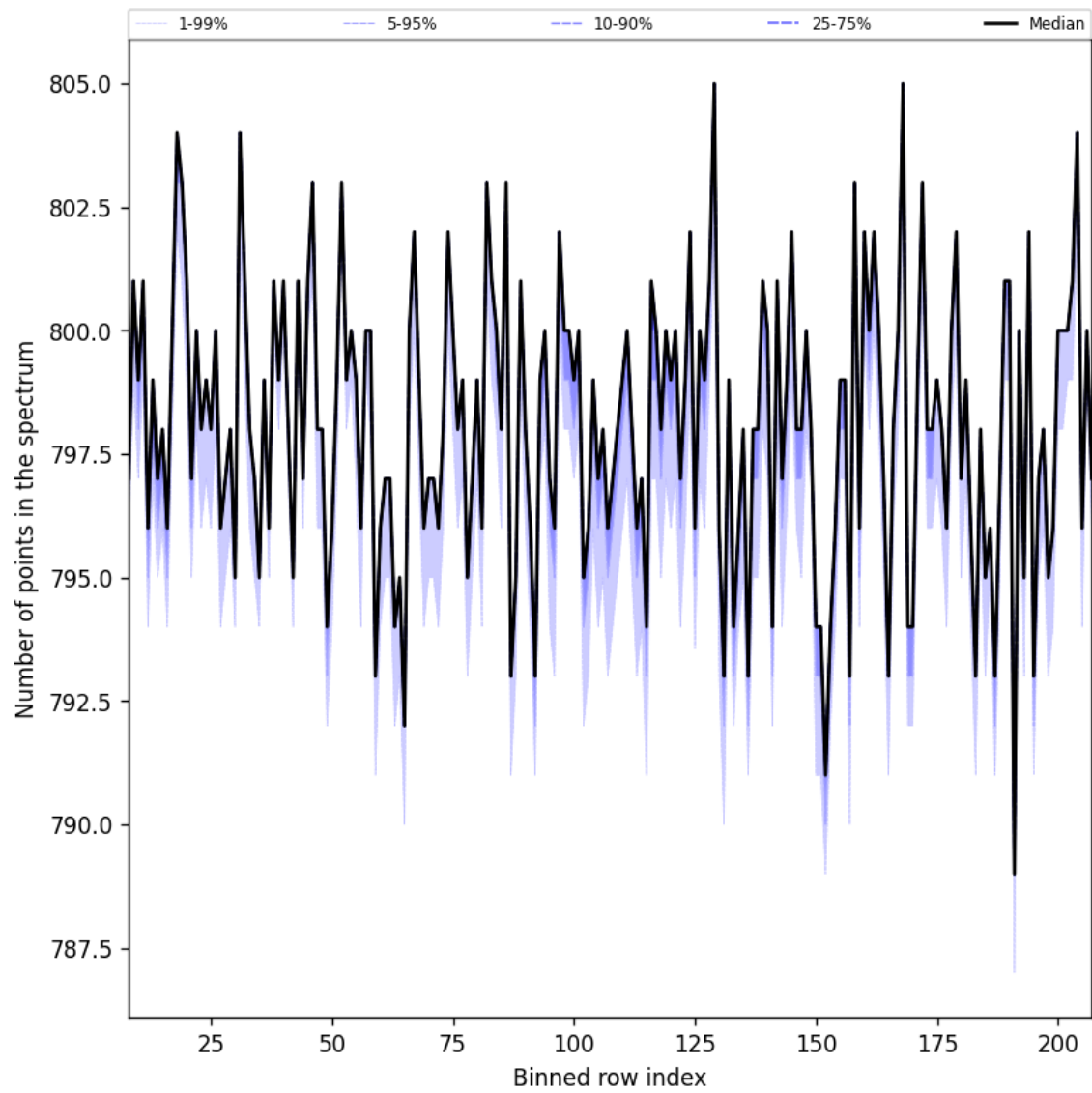
Figure 37: Along track statistics of “Number of points in the spectrum” for 2025-07-11 to 2025-07-13
