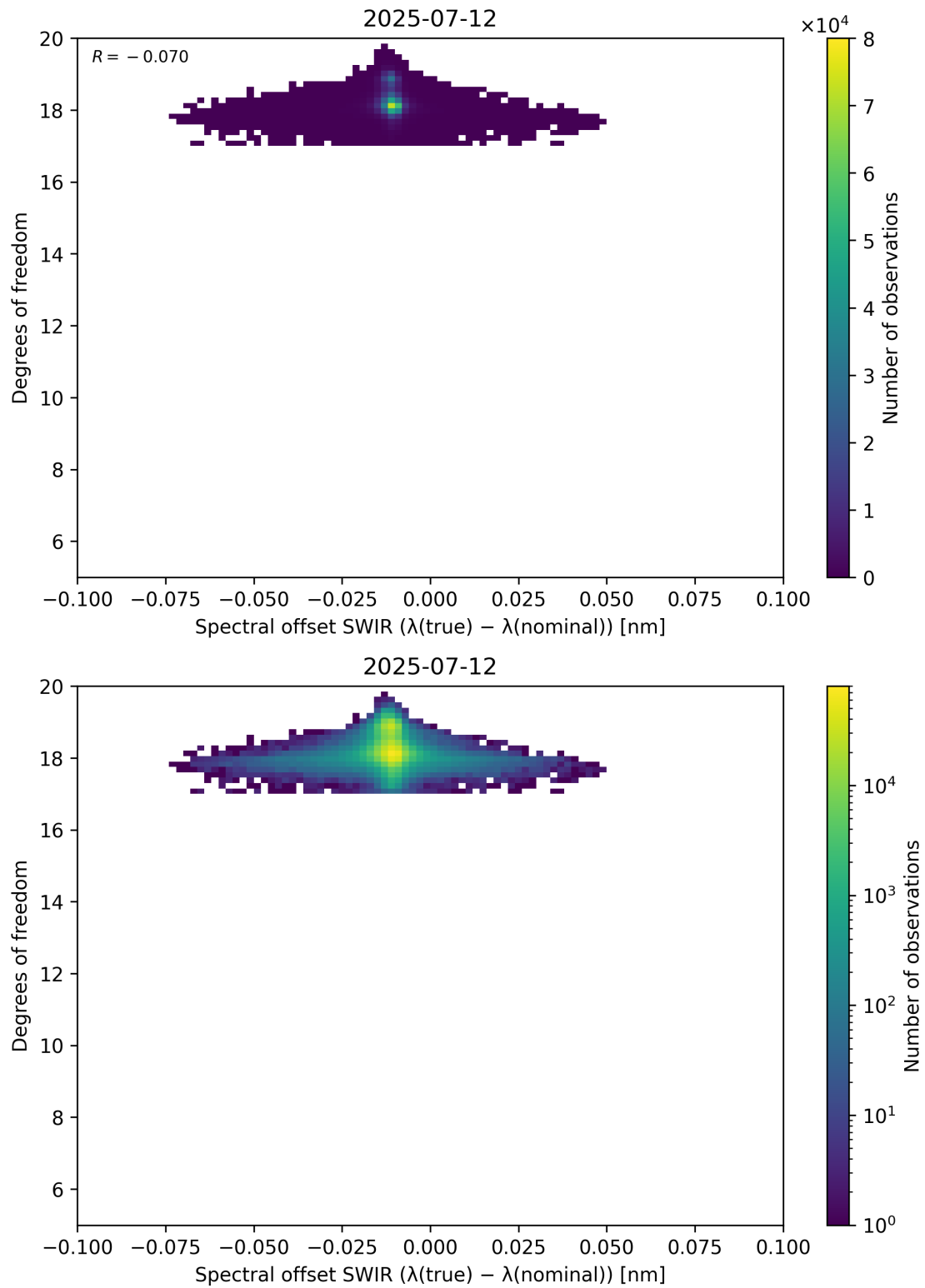
Figure 119: Scatter density plot of “Spectral offset SWIR ( \lambda_{\text{true}} - \lambda_{\text{nominal}} )” against “Degrees of freedom” for 2025-07-11 to 2025-07-13.
