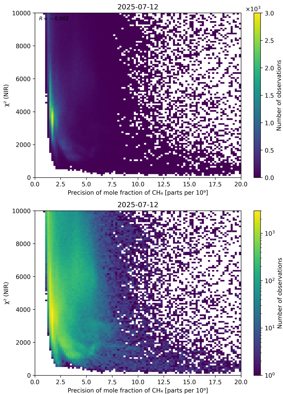
Figure 78: Scatter density plot of “Precision of mole fraction of CH 4 ” against “ \chi^2 (NIR)” for 2025-07-11 to 2025-07-13.
