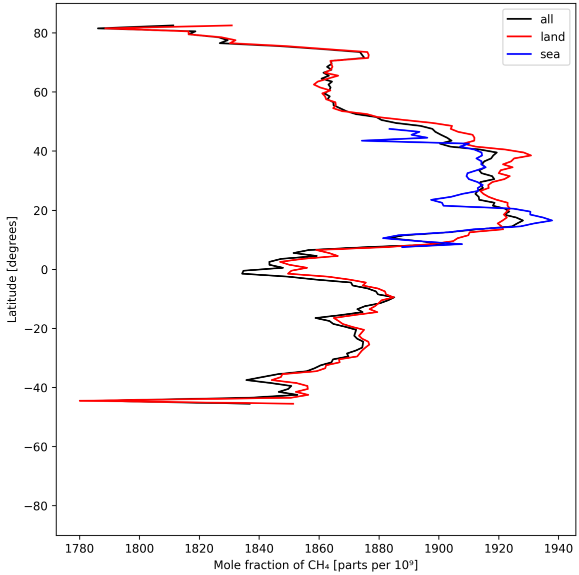
Figure 12: Zonal average of “Mole fraction of CH 4 ” for 2025-07-11 to 2025-07-13.
