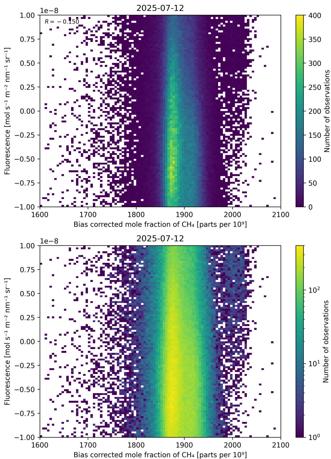
Figure 66: Scatter density plot of “Bias corrected mole fraction of \text{CH}_4 ” against “Fluorescence” for 2025-07-11 to 2025-07-13.
