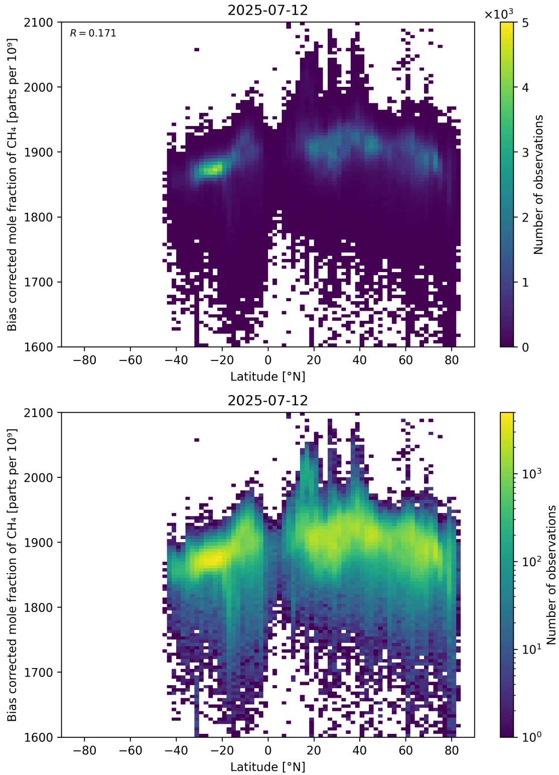
Figure 58: Scatter density plot of “Latitude” against “Bias corrected mole fraction of \text{CH}_4 ” for 2025-07-11 to 2025-07-13.
