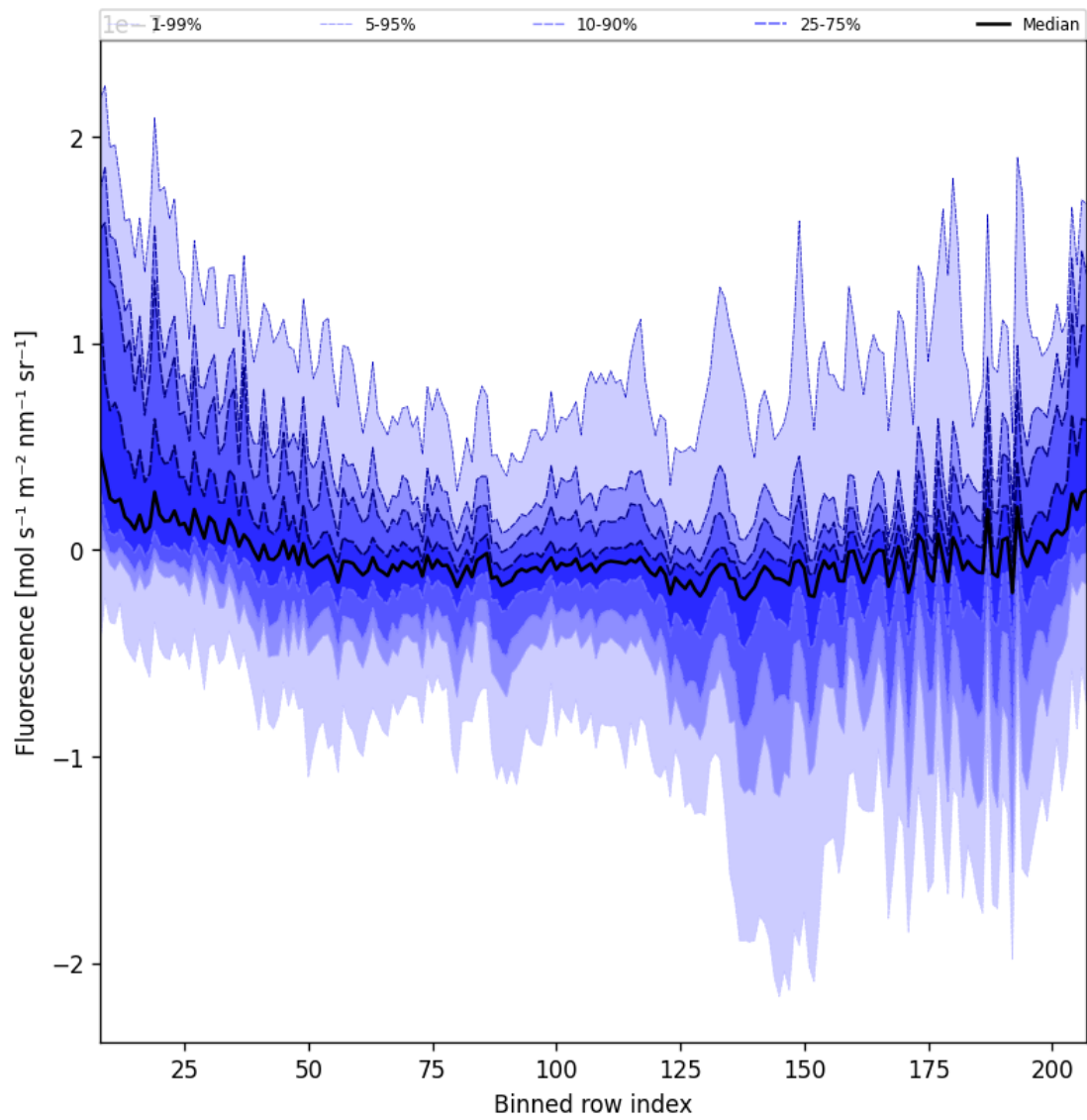
Figure 43: Along track statistics of “Fluorescence” for 2025-07-11 to 2025-07-13
