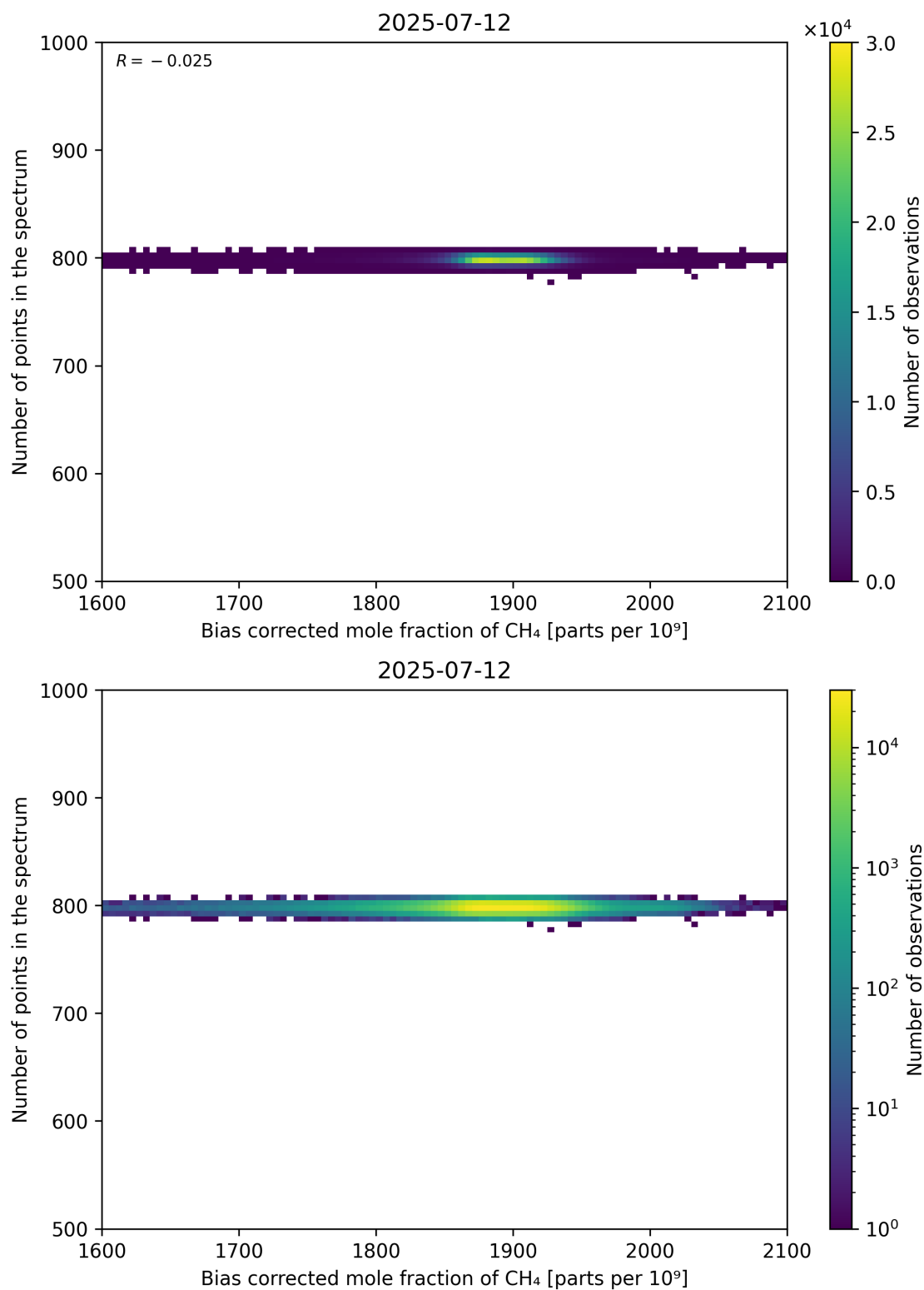
Figure 68: Scatter density plot of “Bias corrected mole fraction of CH 4 ” against “Number of points in the spectrum” for 2025-07-11 to 2025-07-13.
