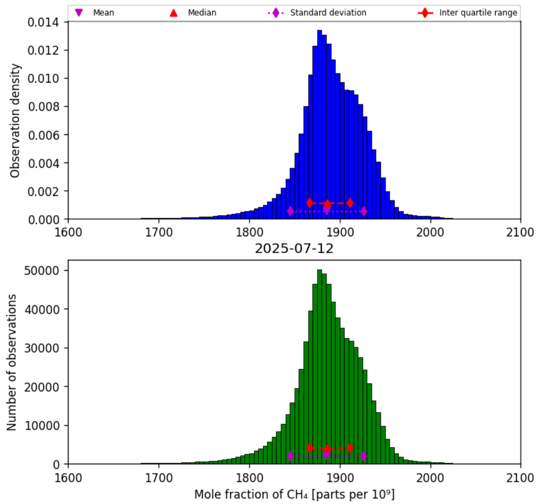
Figure 23: Histogram of “Mole fraction of CH 4 ” for 2025-07-11 to 2025-07-13
