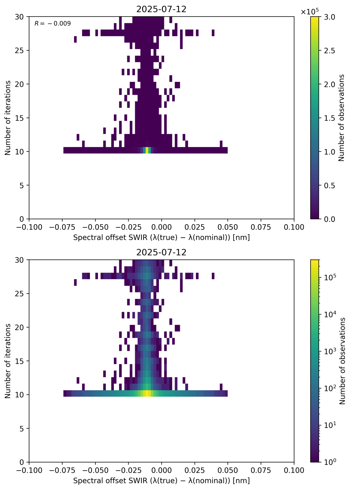
Figure 121: Scatter density plot of “Spectral offset SWIR ( \lambda_{\text{true}} - \lambda_{\text{nominal}} )” against “Number of iterations” for 2025-07-11 to 2025-07-13.
