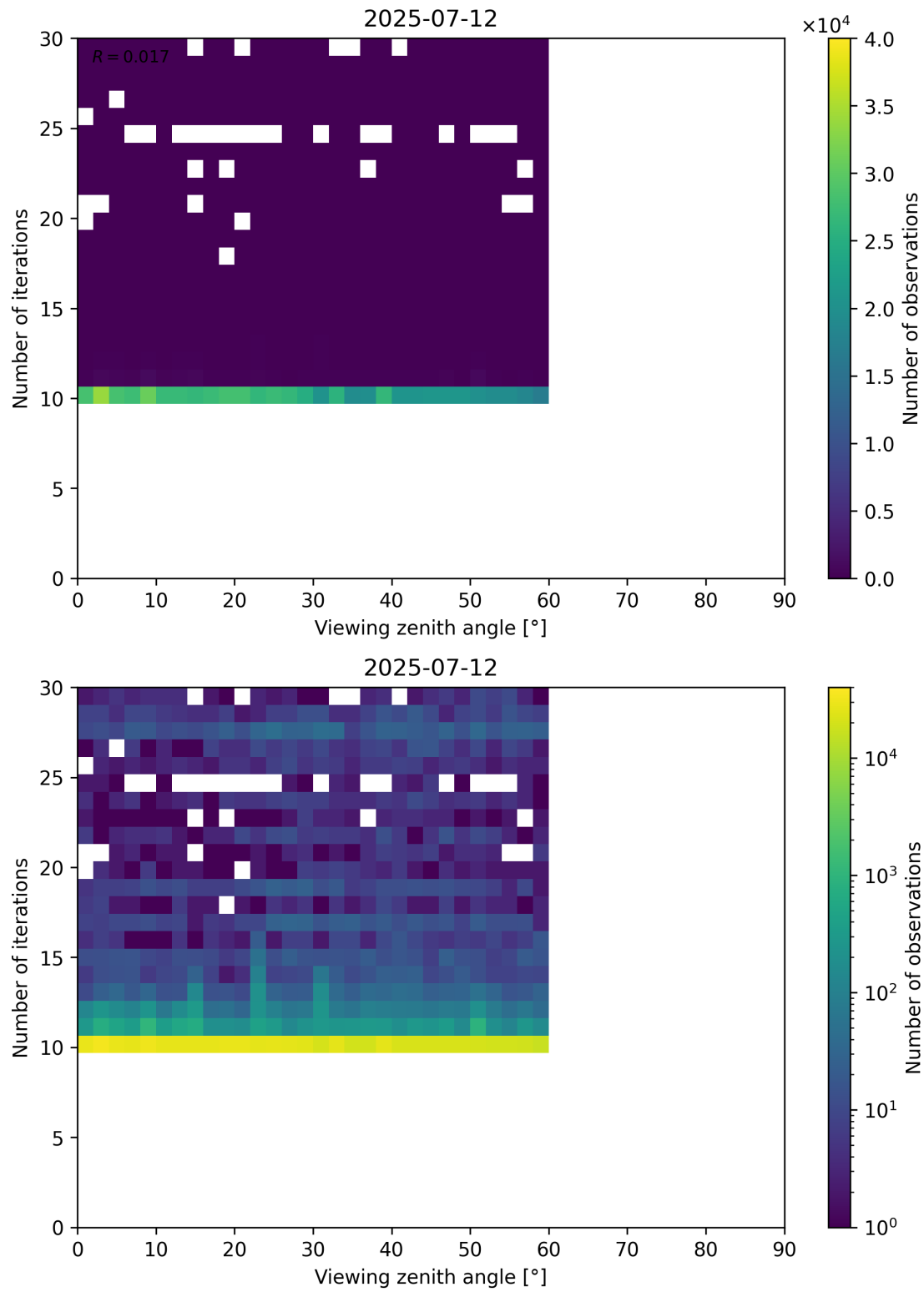
Figure 113: Scatter density plot of “Viewing zenith angle” against “Number of iterations” for 2025-07-11 to 2025-07-13.
