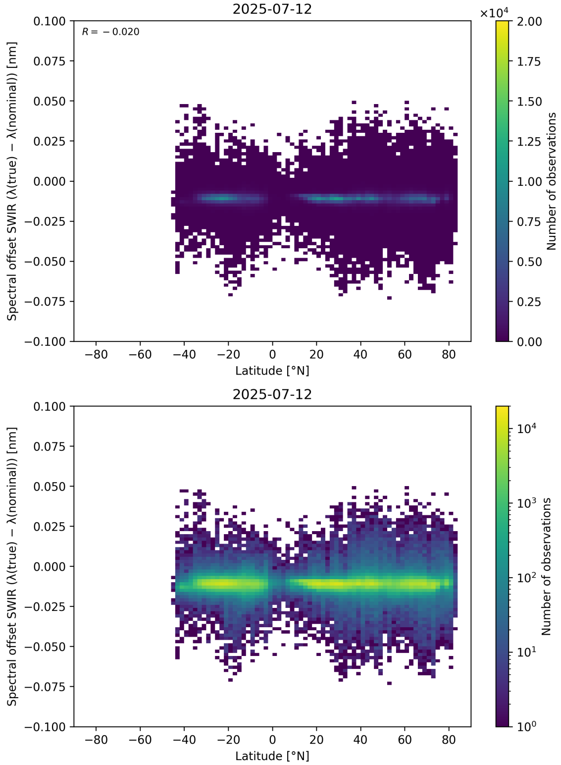
Figure 62: Scatter density plot of “Latitude” against “Spectral offset SWIR ( \lambda_{\text{true}} - \lambda_{\text{nominal}} )” for 2025-07-11 to 2025-07-13.
