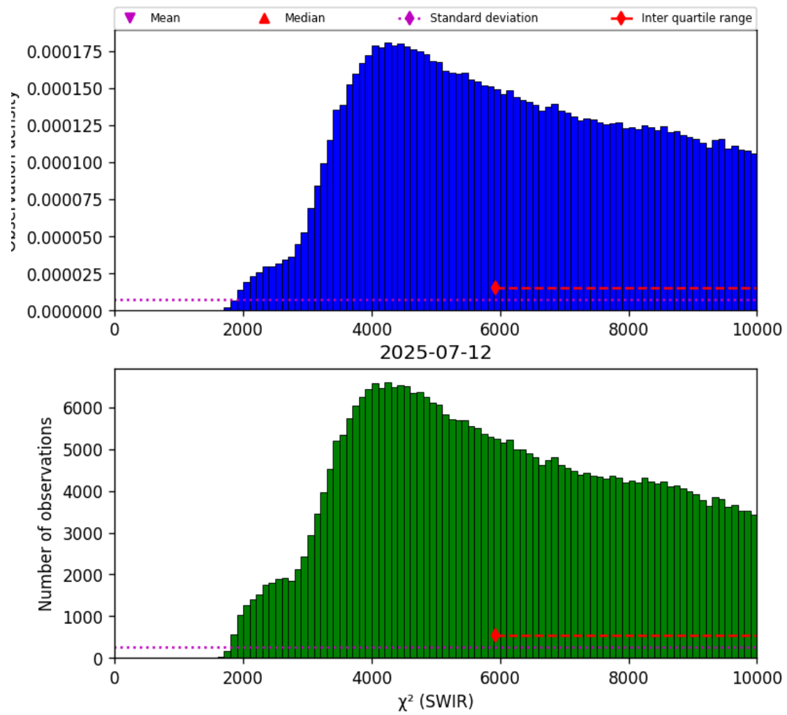
Figure 28: Histogram of “ \chi^2 (SWIR)” for 2025-07-11 to 2025-07-13
