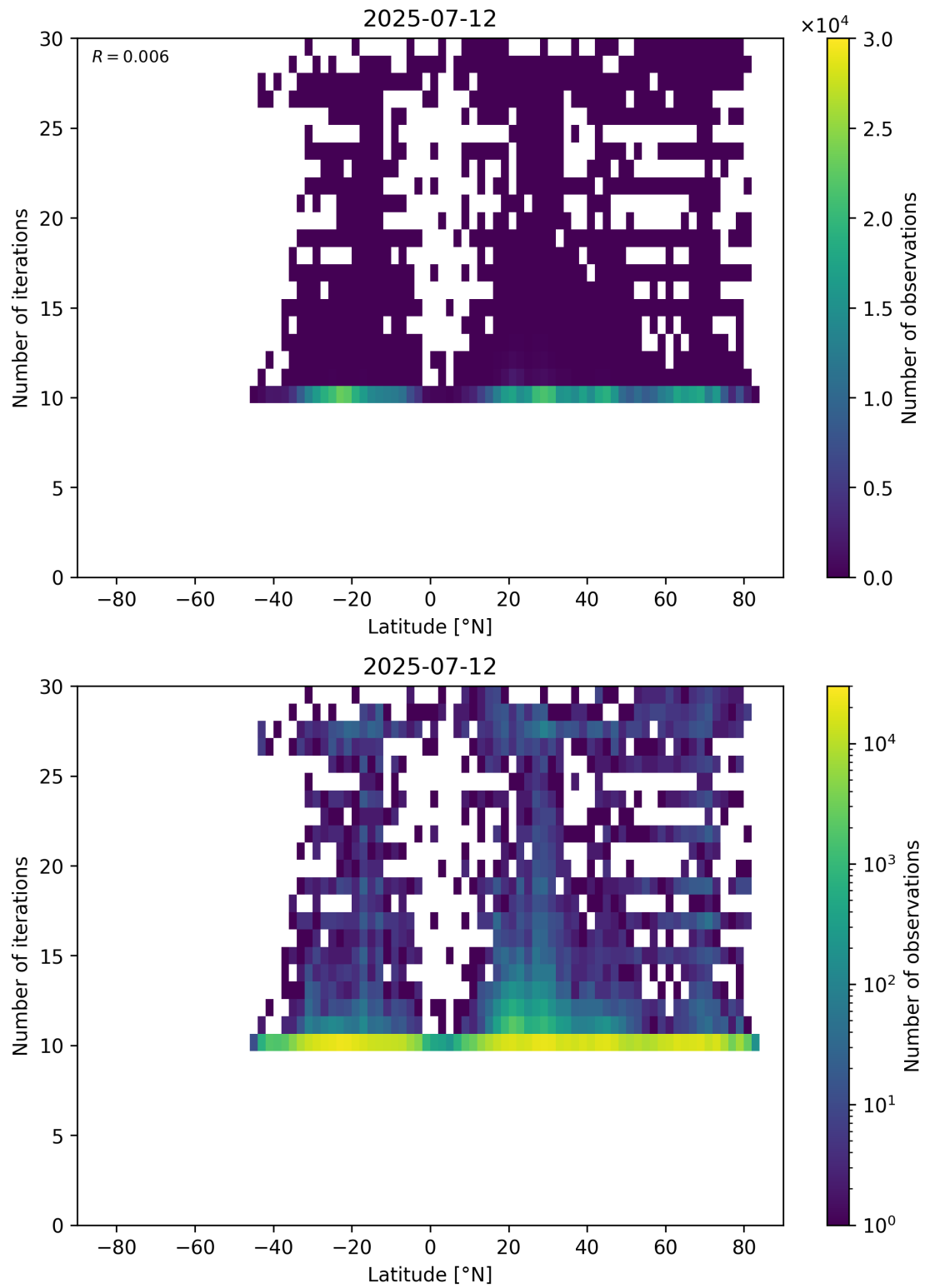
Figure 60: Scatter density plot of “Latitude” against “Number of iterations” for 2025-07-11 to 2025-07-13.
