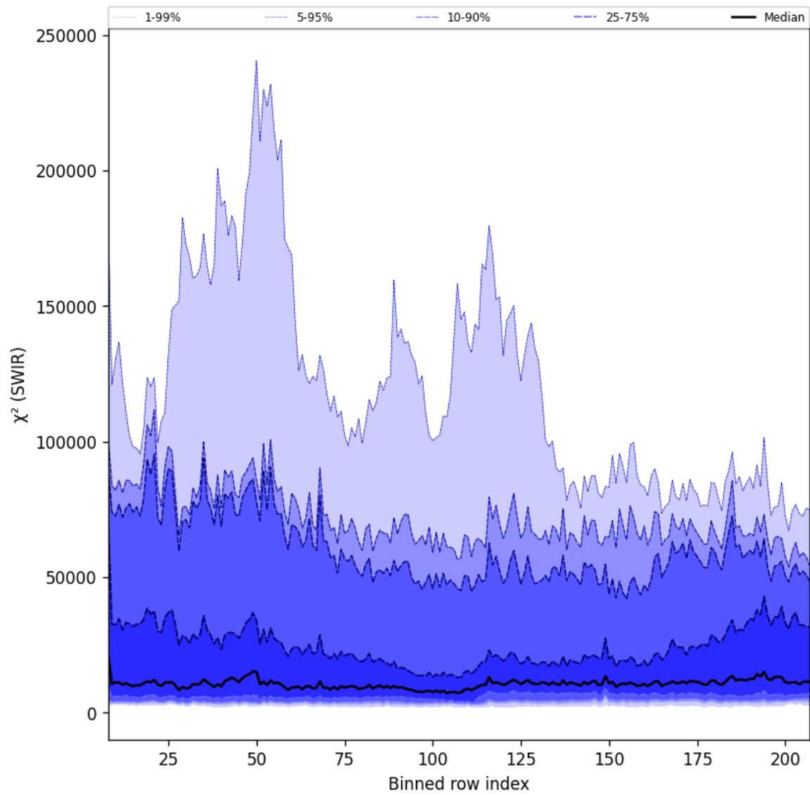
Figure 39: Along track statistics of “ \chi^2 (SWIR)” for 2025-07-11 to 2025-07-13
