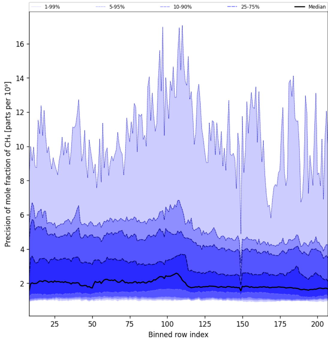
Figure 35: Along track statistics of “Precision of mole fraction of CH 4 ” for 2025-07-11 to 2025-07-13
