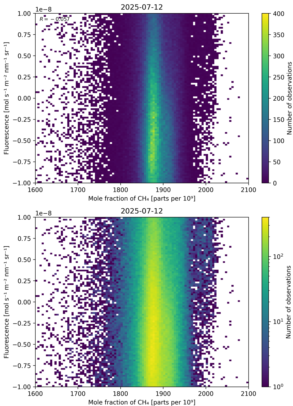
Figure 73: Scatter density plot of “Mole fraction of \text{CH}_4 ” against “Fluorescence” for 2025-07-11 to 2025-07-13.
