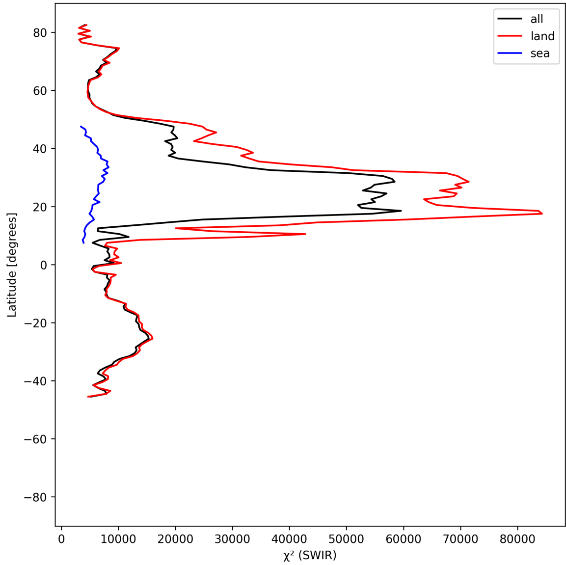
Figure 17: Zonal average of “ \chi^2 (SWIR)” for 2025-07-11 to 2025-07-13.
