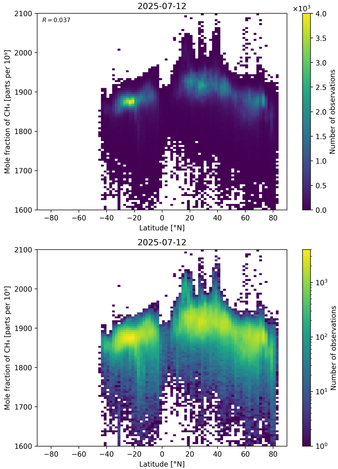
Figure 57: Scatter density plot of “Latitude” against “Mole fraction of CH 4 ” for 2025-07-11 to 2025-07-13.
