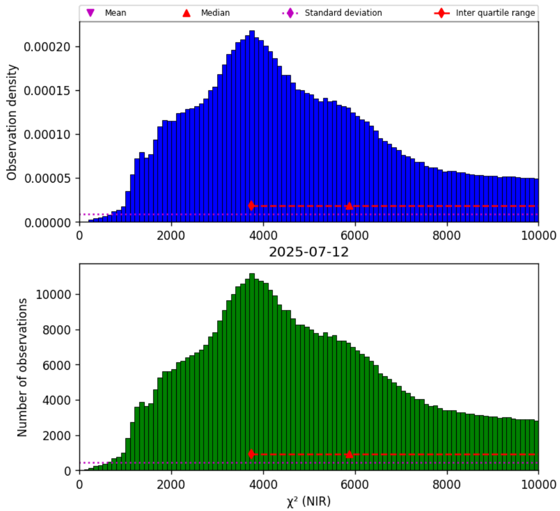
Figure 29: Histogram of “ \chi^2 (NIR)” for 2025-07-11 to 2025-07-13
