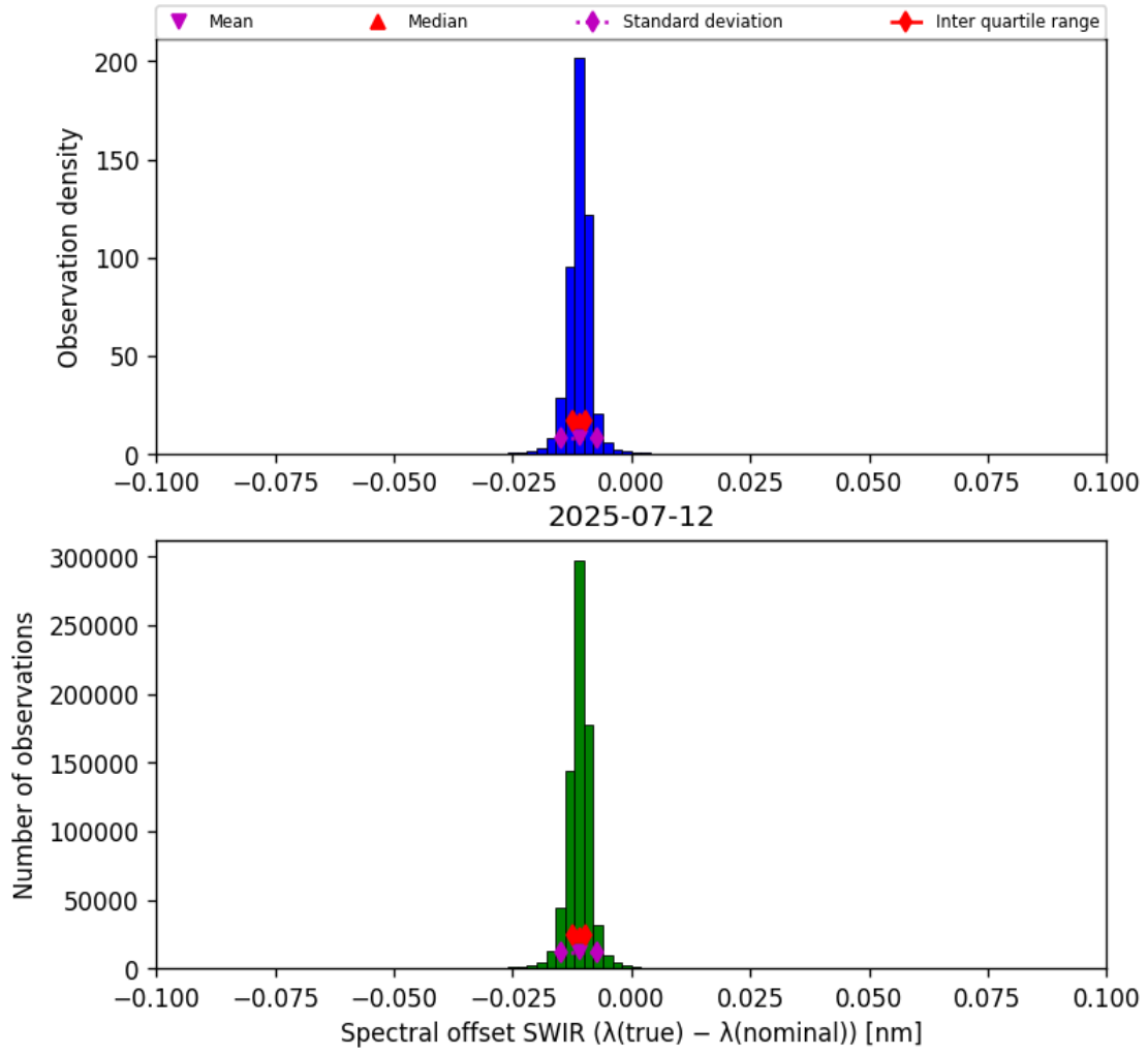
Figure 27: Histogram of “Spectral offset SWIR ( \lambda_{\text{true}} - \lambda_{\text{nominal}} )” for 2025-07-11 to 2025-07-13
