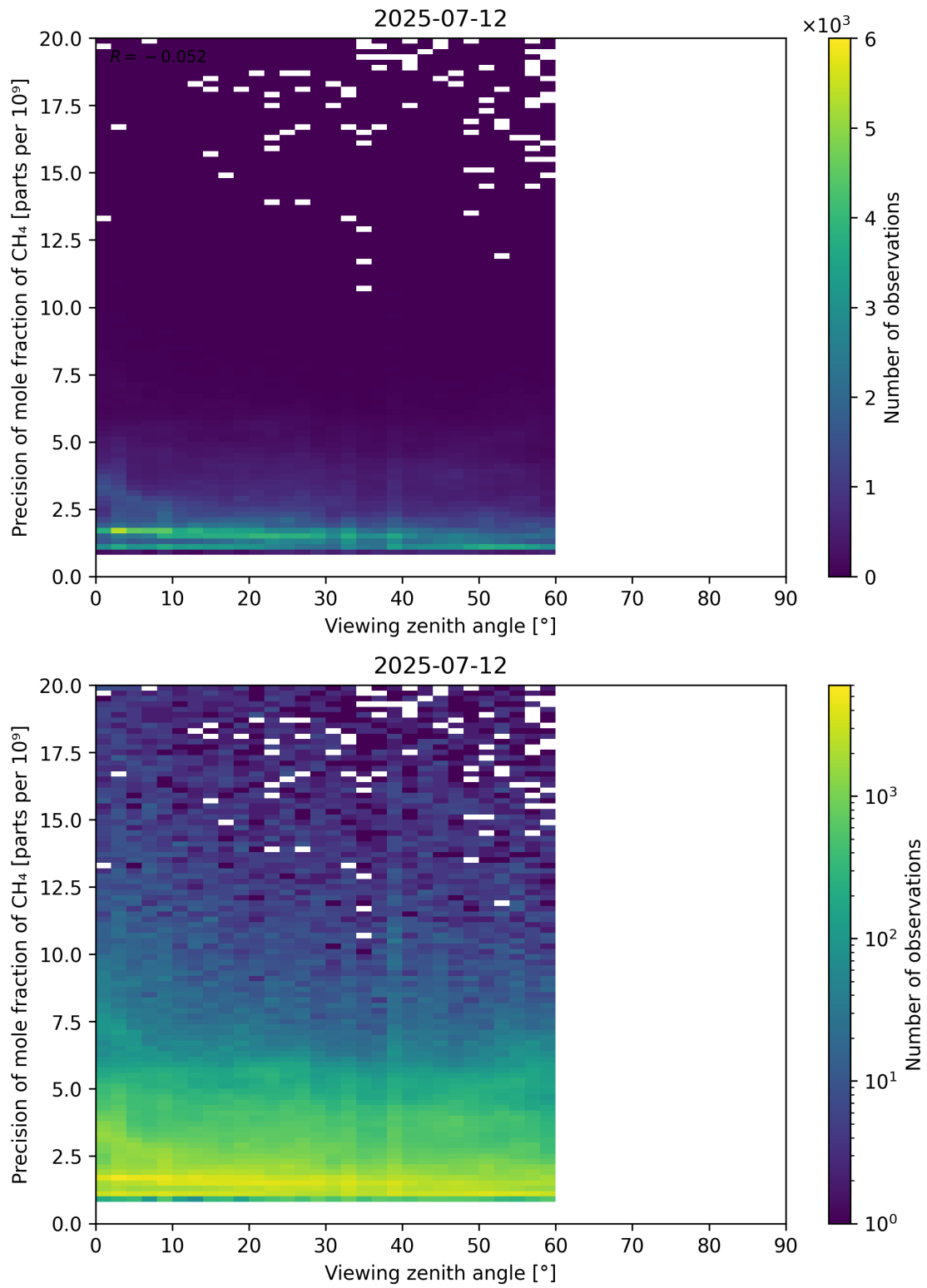
Figure 112: Scatter density plot of “Viewing zenith angle” against “Precision of mole fraction of CH 4 ” for 2025-07-11 to 2025-07-13.
