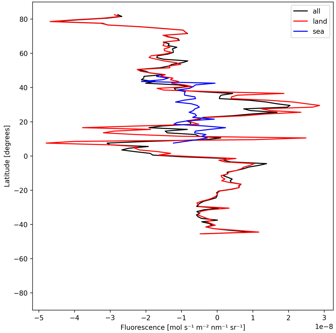
Figure 21: Zonal average of “Fluorescence” for 2025-07-11 to 2025-07-13.
