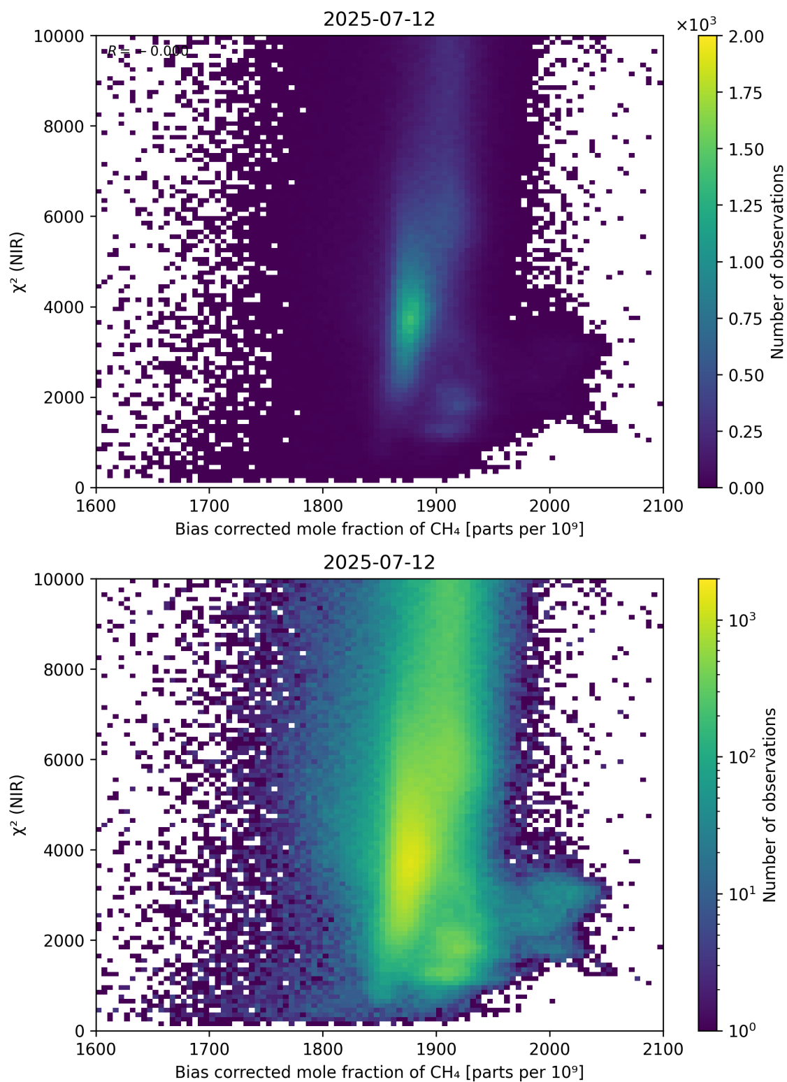
Figure 63: Scatter density plot of “Bias corrected mole fraction of \text{CH}_4 ” against “ \chi^2 (NIR)” for 2025-07-11 to 2025-07-13.
