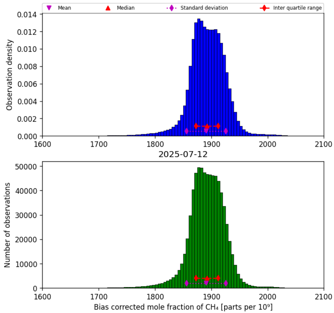
Figure 25: Histogram of “Bias corrected mole fraction of CH 4 ” for 2025-07-11 to 2025-07-13
