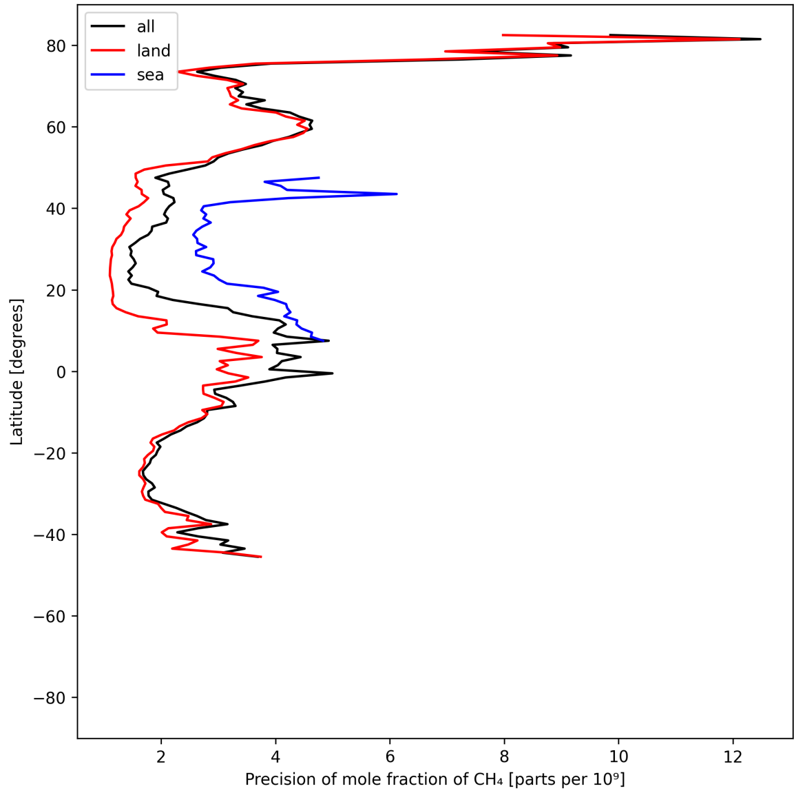
Figure 13: Zonal average of “Precision of mole fraction of CH 4 ” for 2025-07-11 to 2025-07-13.
