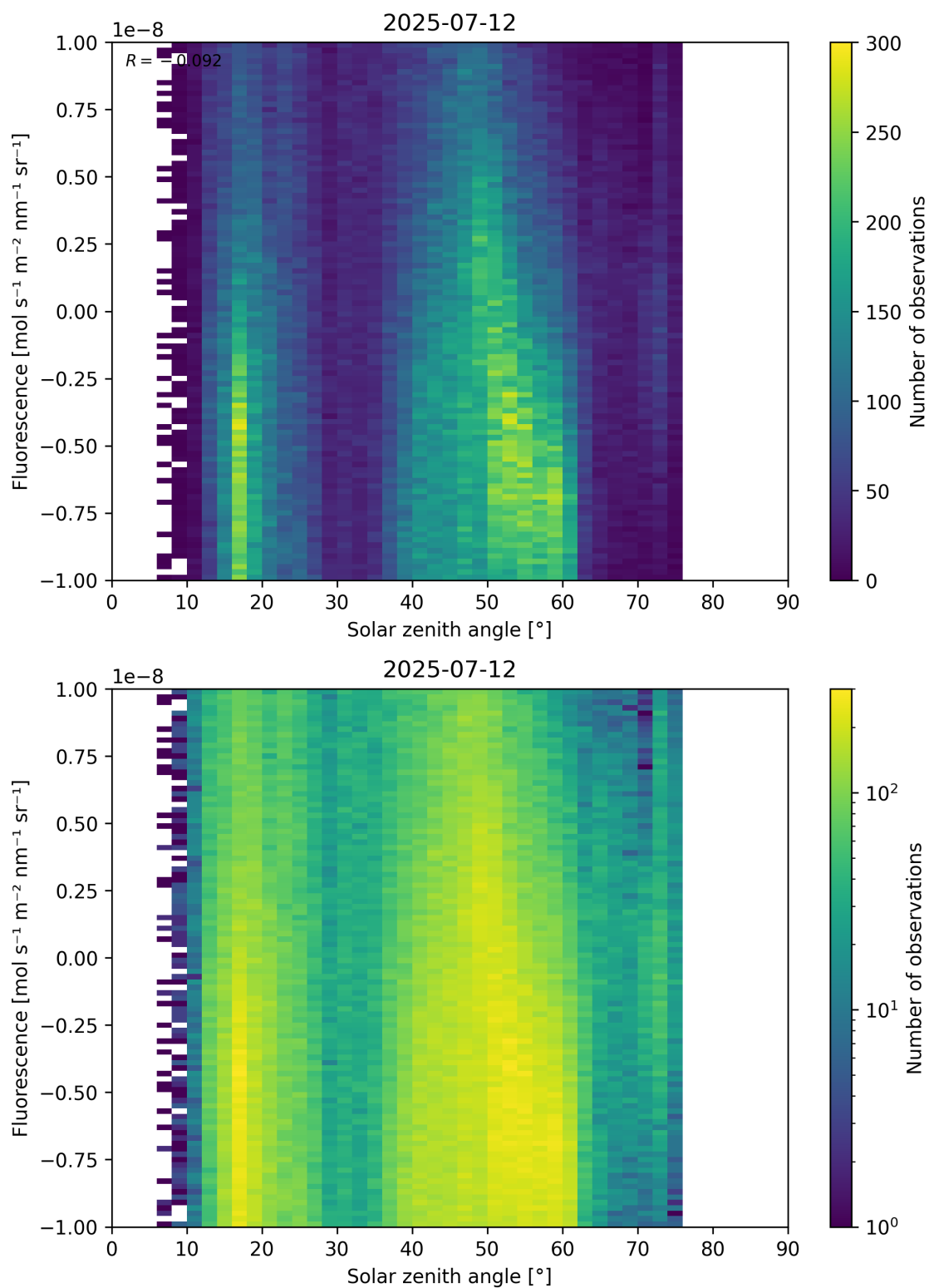
Figure 97: Scatter density plot of “Solar zenith angle” against “Fluorescence” for 2025-07-11 to 2025-07-13.
