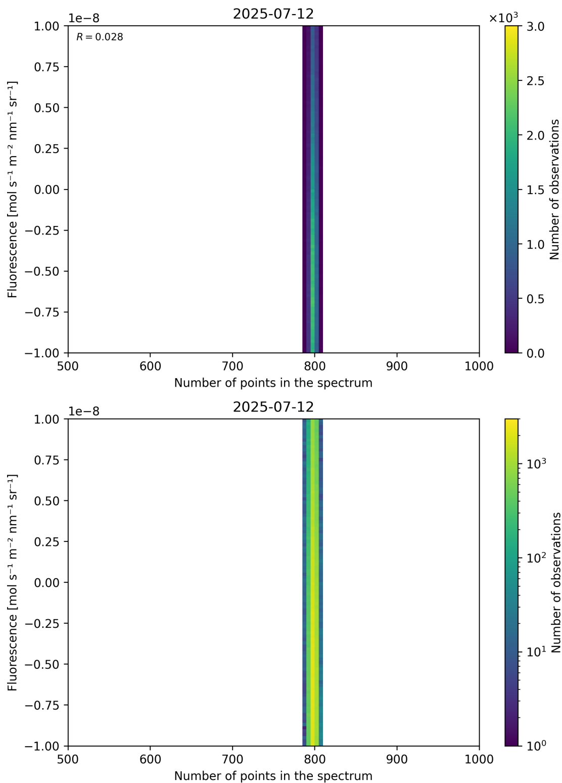
Figure 91: Scatter density plot of “Number of points in the spectrum” against “Fluorescence” for 2025-07-11 to 2025-07-13.
