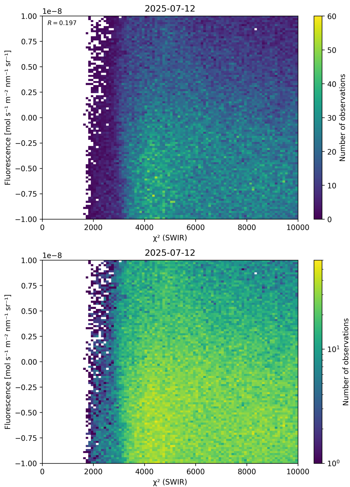
Figure 49: Scatter density plot of “ \chi^2 (SWIR)” against “Fluorescence” for 2025-07-11 to 2025-07-13.
