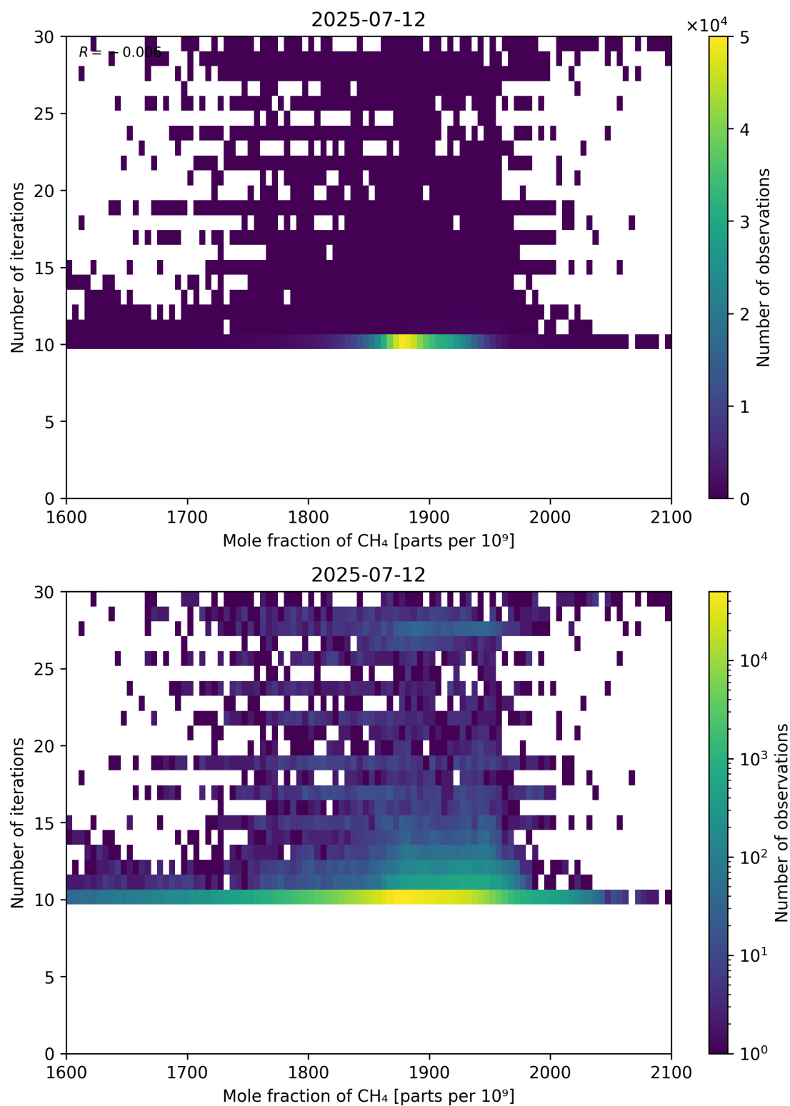
Figure 76: Scatter density plot of “Mole fraction of CH 4 ” against “Number of iterations” for 2025-07-11 to 2025-07-13.
