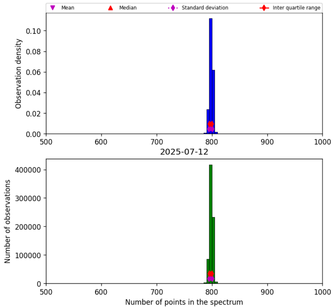
Figure 26: Histogram of “Number of points in the spectrum” for 2025-07-11 to 2025-07-13
