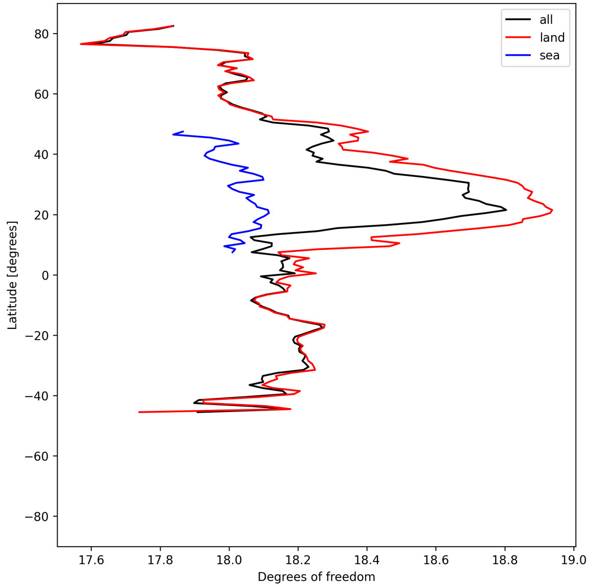
Figure 19: Zonal average of “Degrees of freedom” for 2025-07-11 to 2025-07-13.
