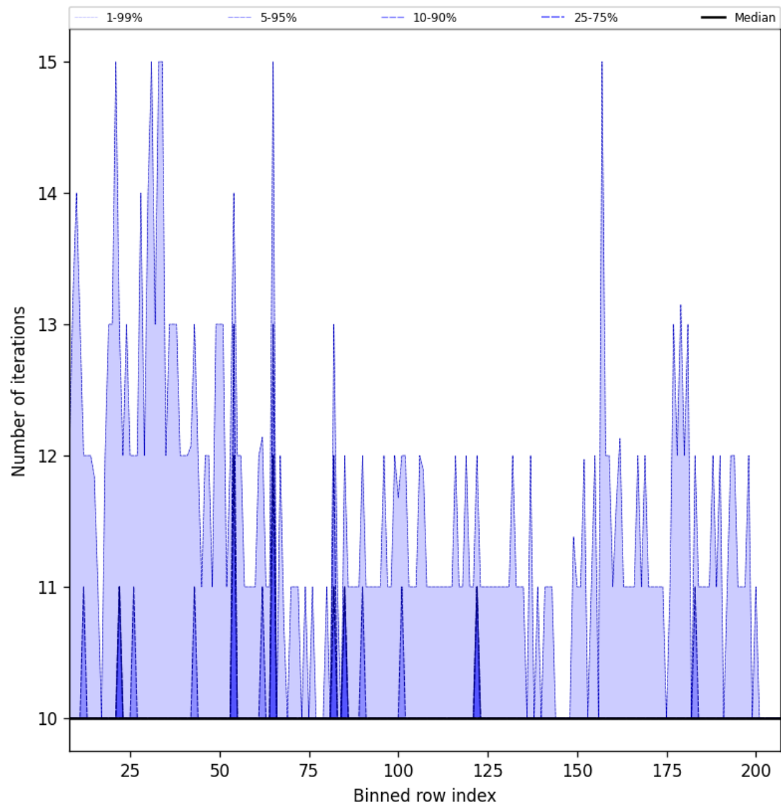
Figure 42: Along track statistics of “Number of iterations” for 2025-07-11 to 2025-07-13
