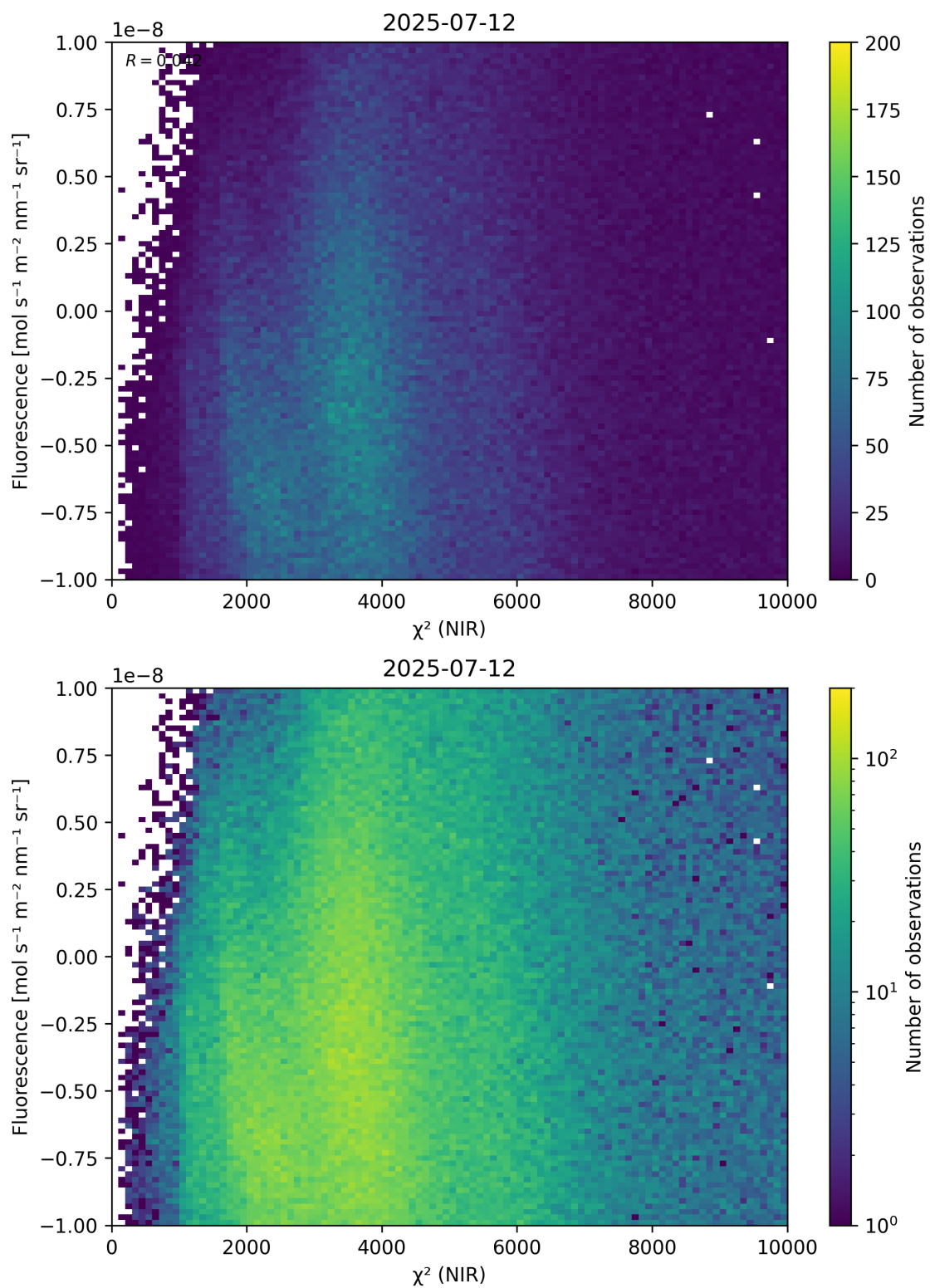
Figure 45: Scatter density plot of “ \chi^2 (NIR)” against “Fluorescence” for 2025-07-11 to 2025-07-13.
