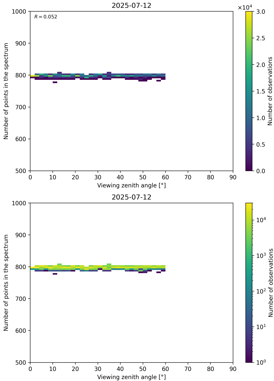
Figure 114: Scatter density plot of “Viewing zenith angle” against “Number of points in the spectrum” for 2025-07-11 to 2025-07-13.
