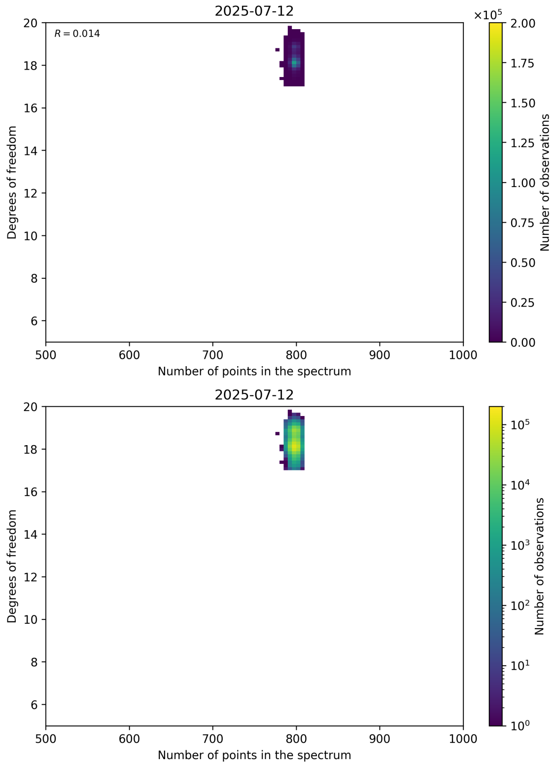
Figure 90: Scatter density plot of “Number of points in the spectrum” against “Degrees of freedom” for 2025-07-11 to 2025-07-13.
