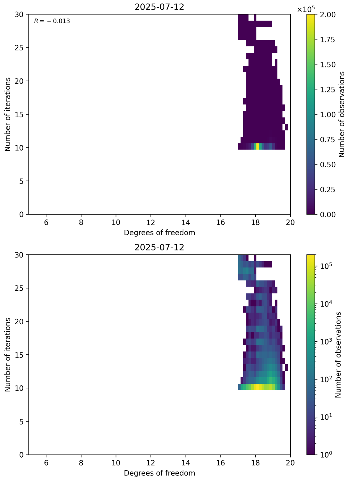
Figure 52: Scatter density plot of “Degrees of freedom” against “Number of iterations” for 2025-07-11 to 2025-07-13.
