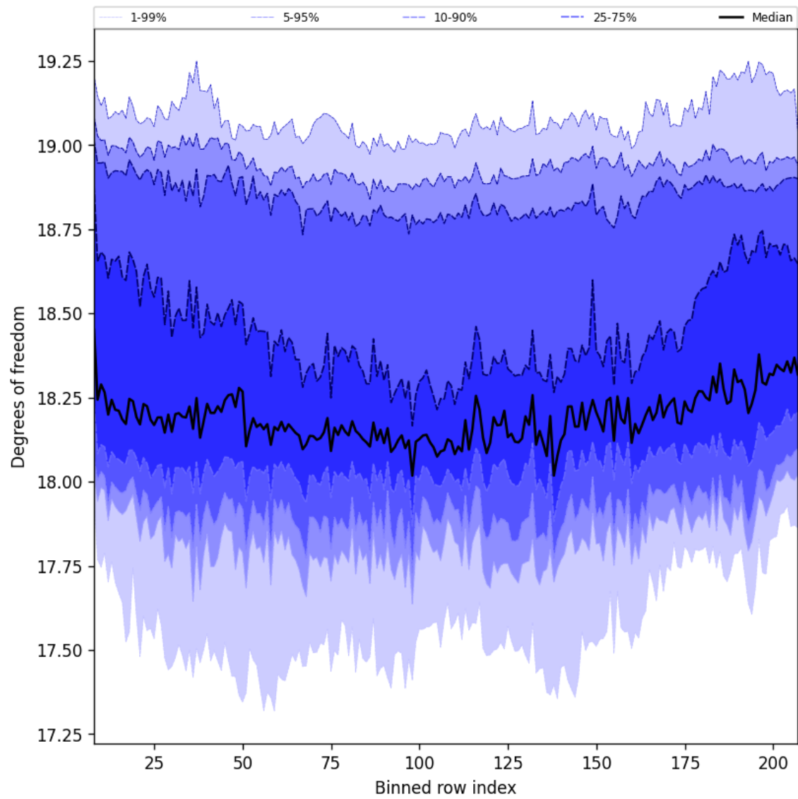
Figure 41: Along track statistics of “Degrees of freedom” for 2025-07-11 to 2025-07-13
