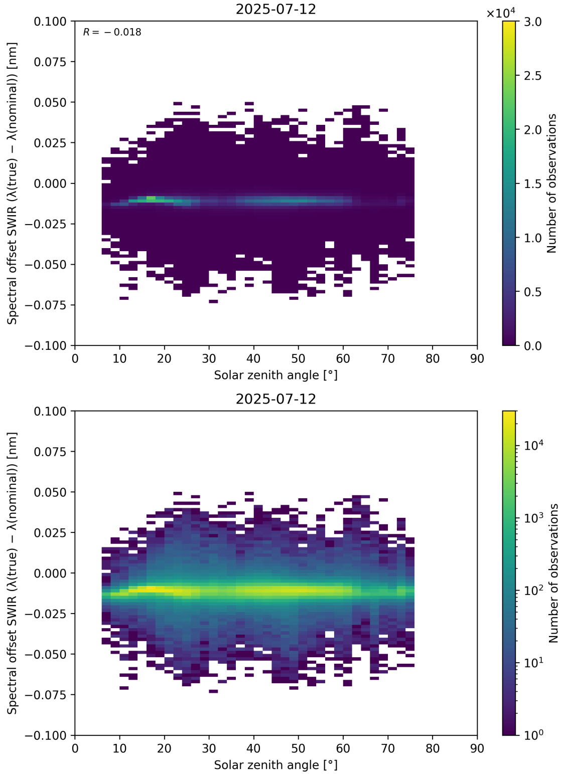
Figure 104: Scatter density plot of “Solar zenith angle” against “Spectral offset SWIR ( \lambda_{\text{true}} - \lambda_{\text{nominal}} )” for 2025-07-11 to 2025-07-13.
