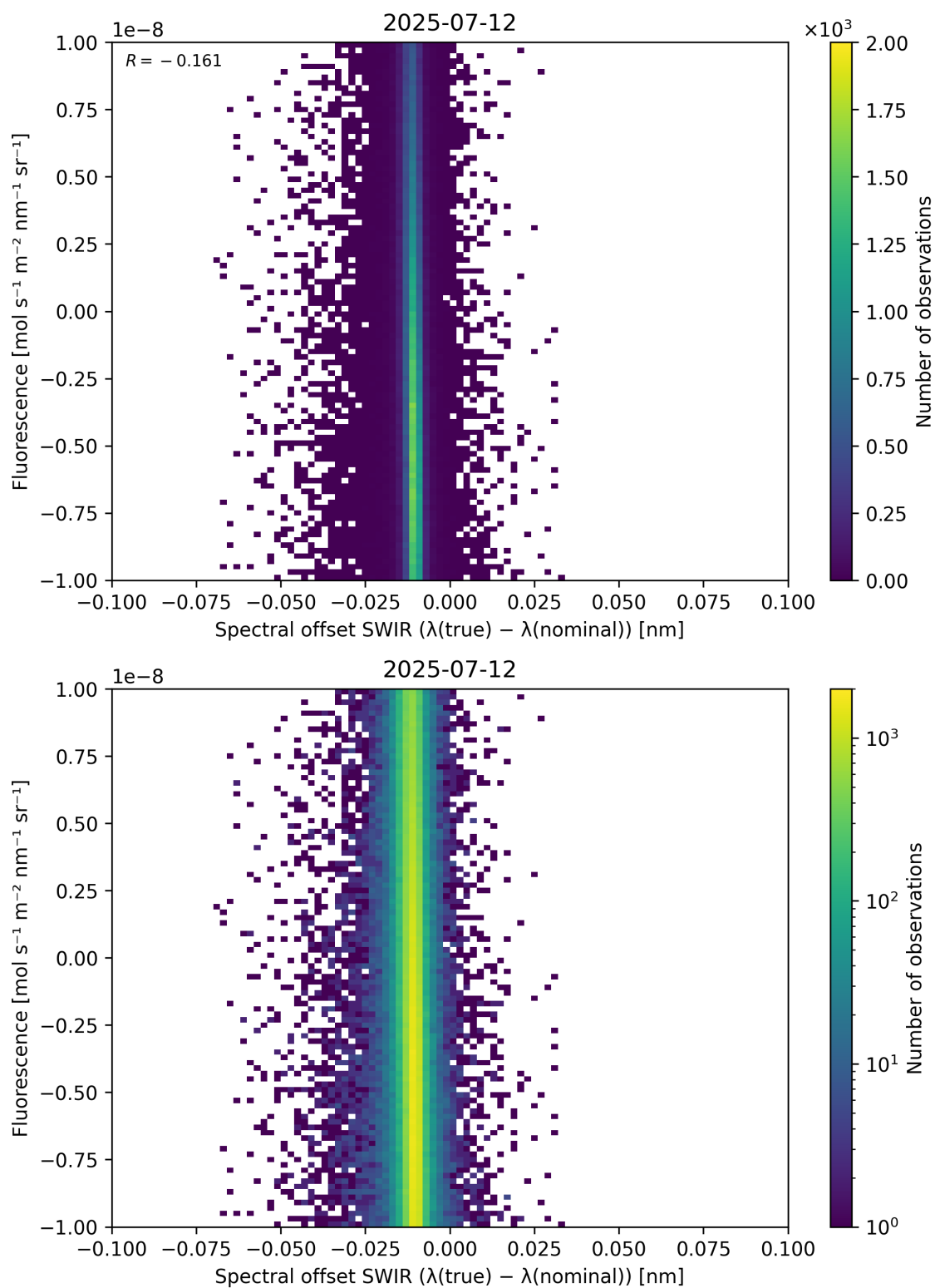
Figure 120: Scatter density plot of “Spectral offset SWIR ( \lambda_{\text{true}} - \lambda_{\text{nominal}} )” against “Fluorescence” for 2025-07-11 to 2025-07-13.
