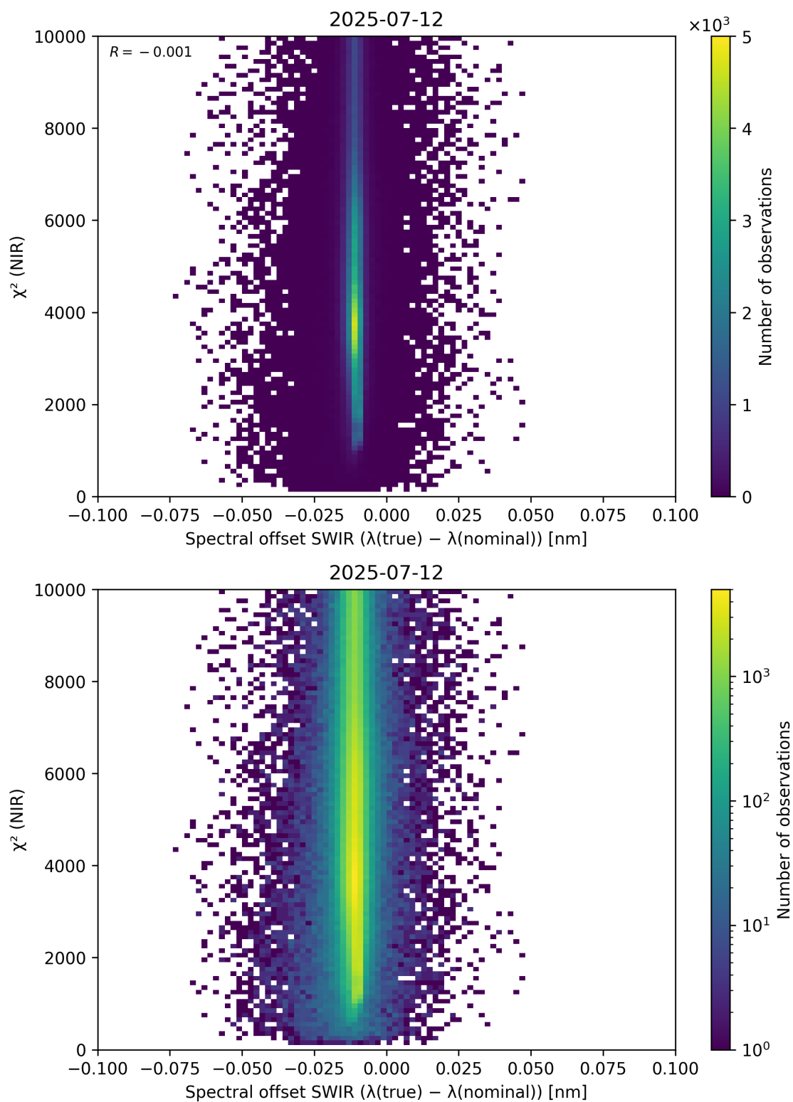
Figure 117: Scatter density plot of “Spectral offset SWIR ( \lambda_{\text{true}} - \lambda_{\text{nominal}} )” against “ \chi^2 (NIR)” for 2025-07-11 to 2025-07-13.
