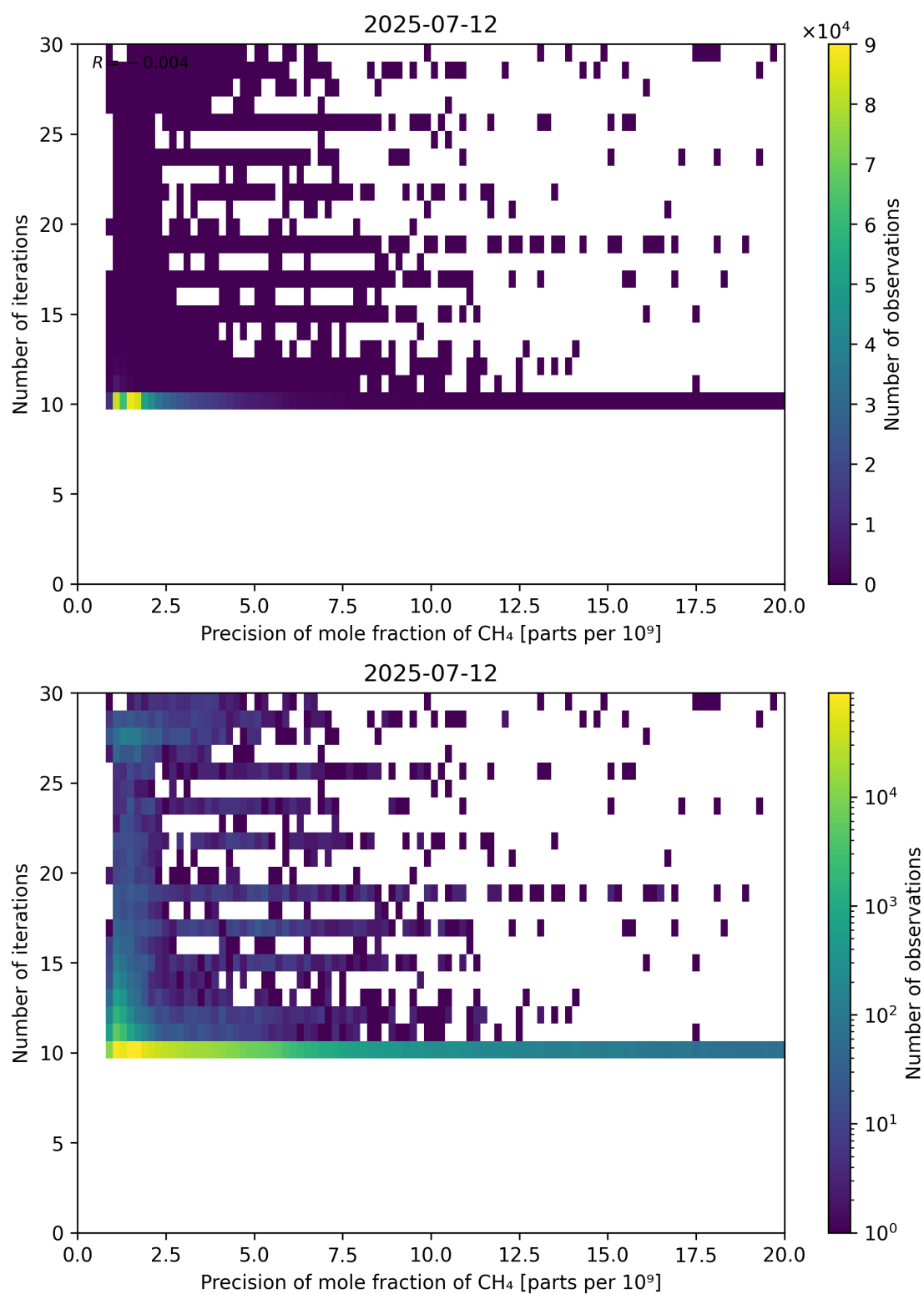
Figure 83: Scatter density plot of “Precision of mole fraction of CH 4 ” against “Number of iterations” for 2025-07-11 to 2025-07-13.
