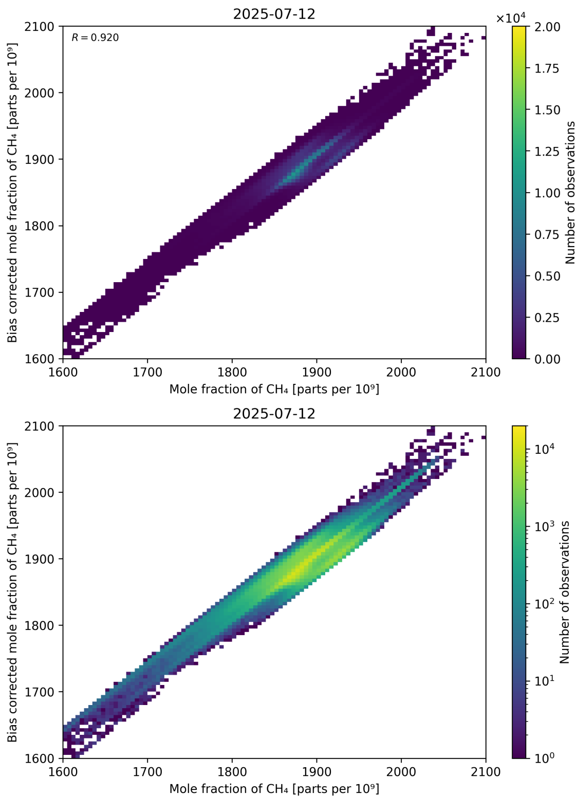
Figure 74: Scatter density plot of “Mole fraction of CH 4 ” against “Bias corrected mole fraction of CH 4 ” for 2025-07-11 to 2025-07-13.
