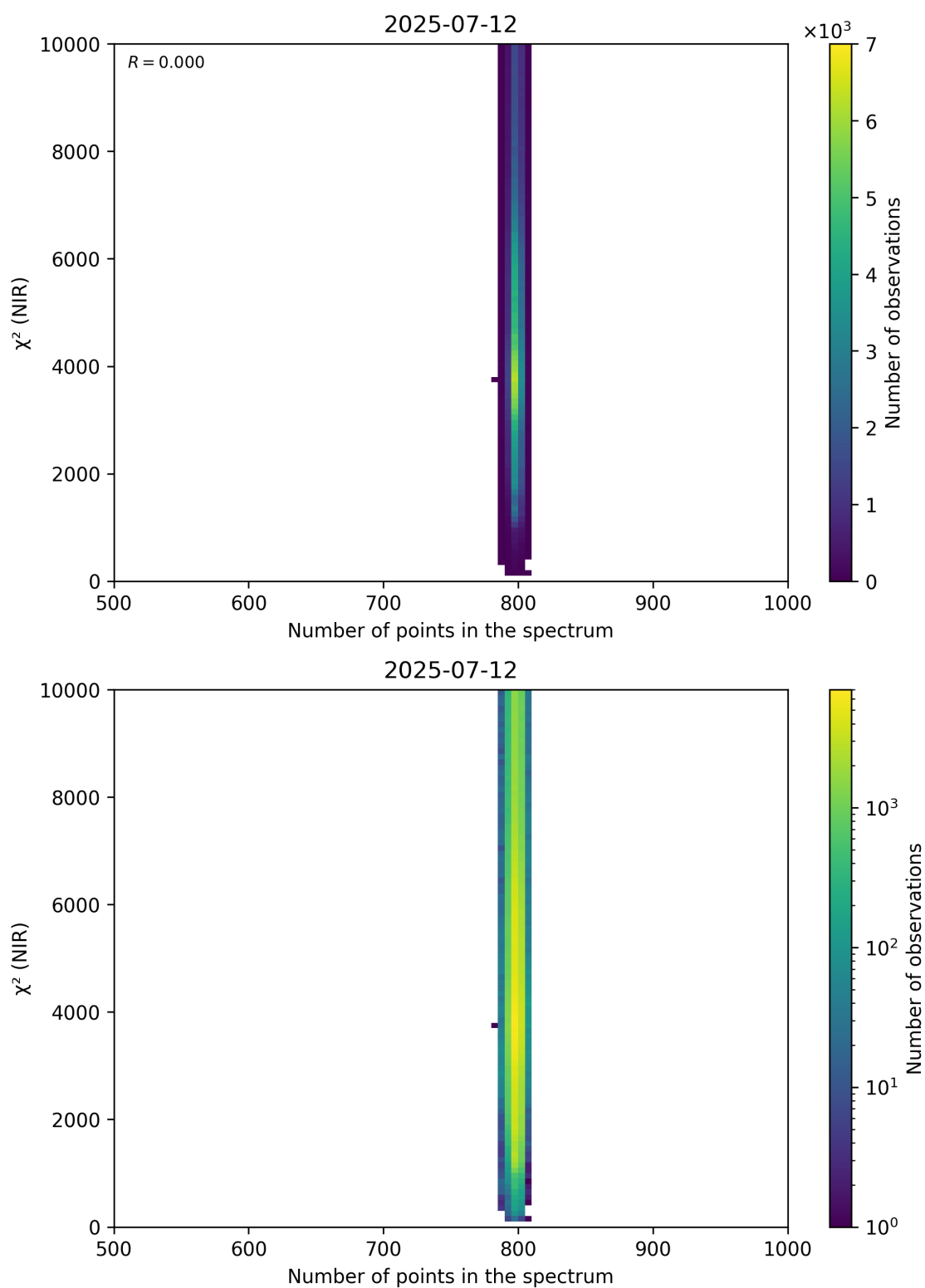
Figure 88: Scatter density plot of “Number of points in the spectrum” against “ \chi^2 (NIR)” for 2025-07-11 to 2025-07-13.
