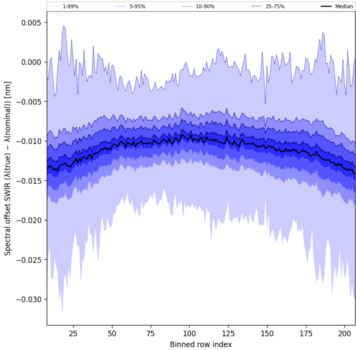
Figure 38: Along track statistics of “Spectral offset SWIR ( \lambda_{\text{true}} - \lambda_{\text{nominal}} )” for 2025-07-11 to 2025-07-13
