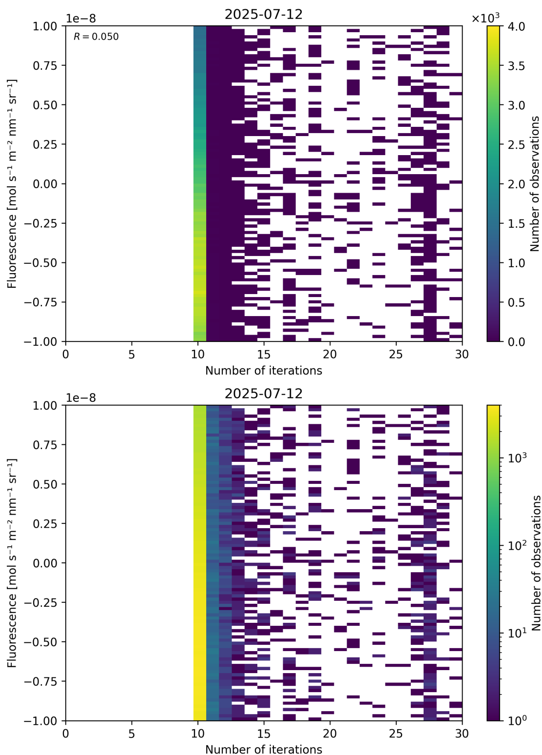
Figure 87: Scatter density plot of “Number of iterations” against “Fluorescence” for 2025-07-11 to 2025-07-13.
