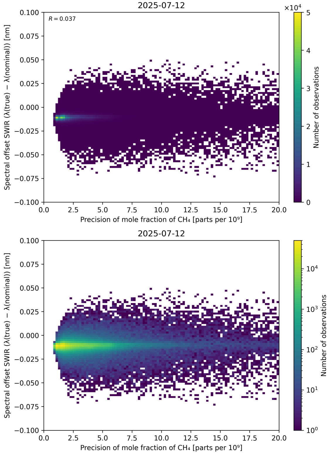
Figure 85: Scatter density plot of “Precision of mole fraction of CH 4 ” against “Spectral offset SWIR ( \lambda_{\text{true}} - \lambda_{\text{nominal}} )” for 2025-07-11 to 2025-07-13.
