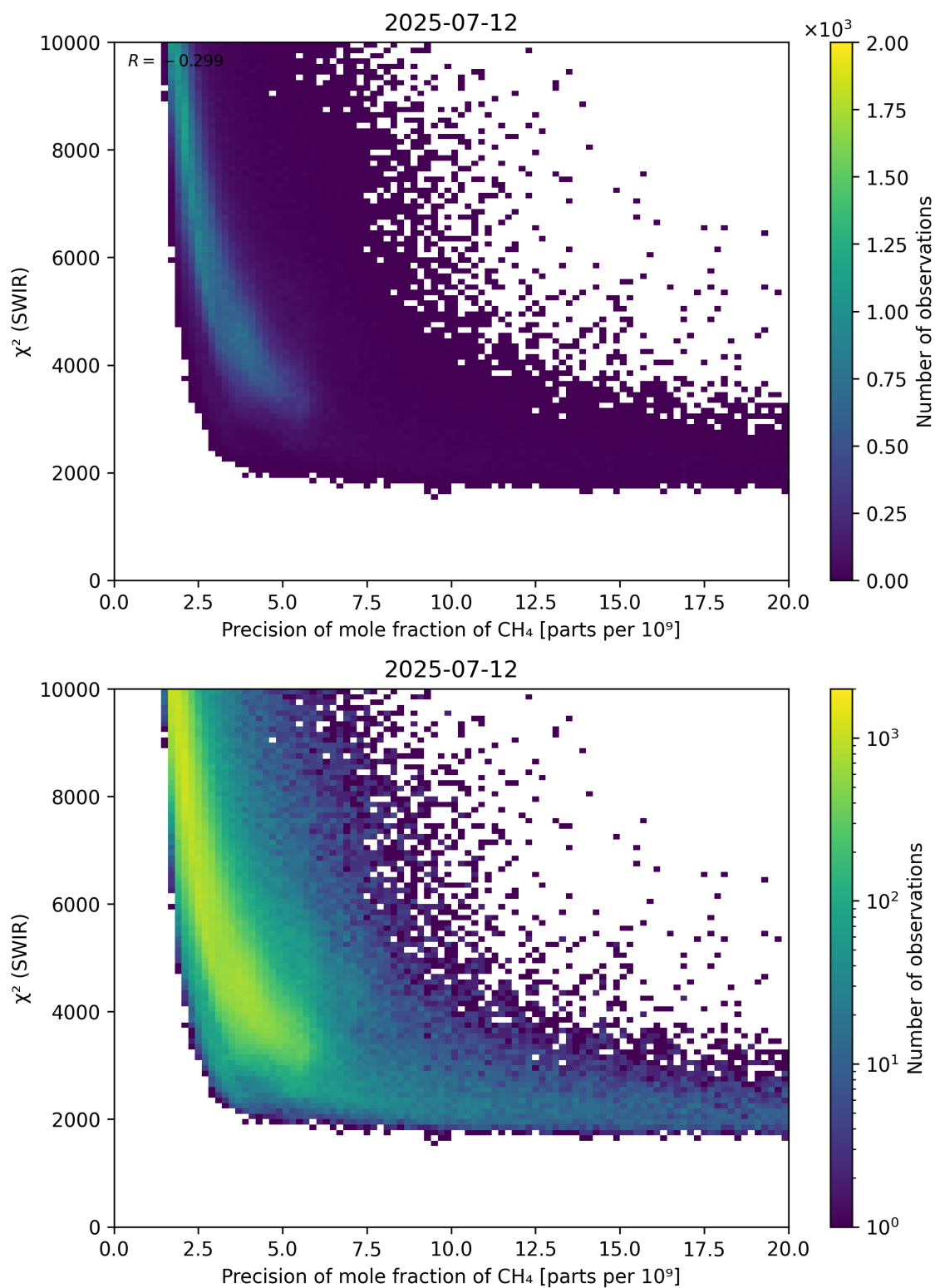
Figure 79: Scatter density plot of “Precision of mole fraction of \text{CH}_4 ” against “ \chi^2 (SWIR)” for 2025-07-11 to 2025-07-13.
