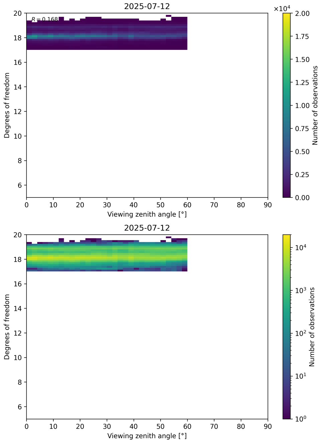
Figure 107: Scatter density plot of “Viewing zenith angle” against “Degrees of freedom” for 2025-07-11 to 2025-07-13.
