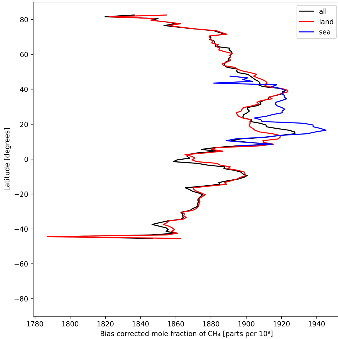
Figure 14: Zonal average of “Bias corrected mole fraction of CH 4 ” for 2025-07-11 to 2025-07-13.
