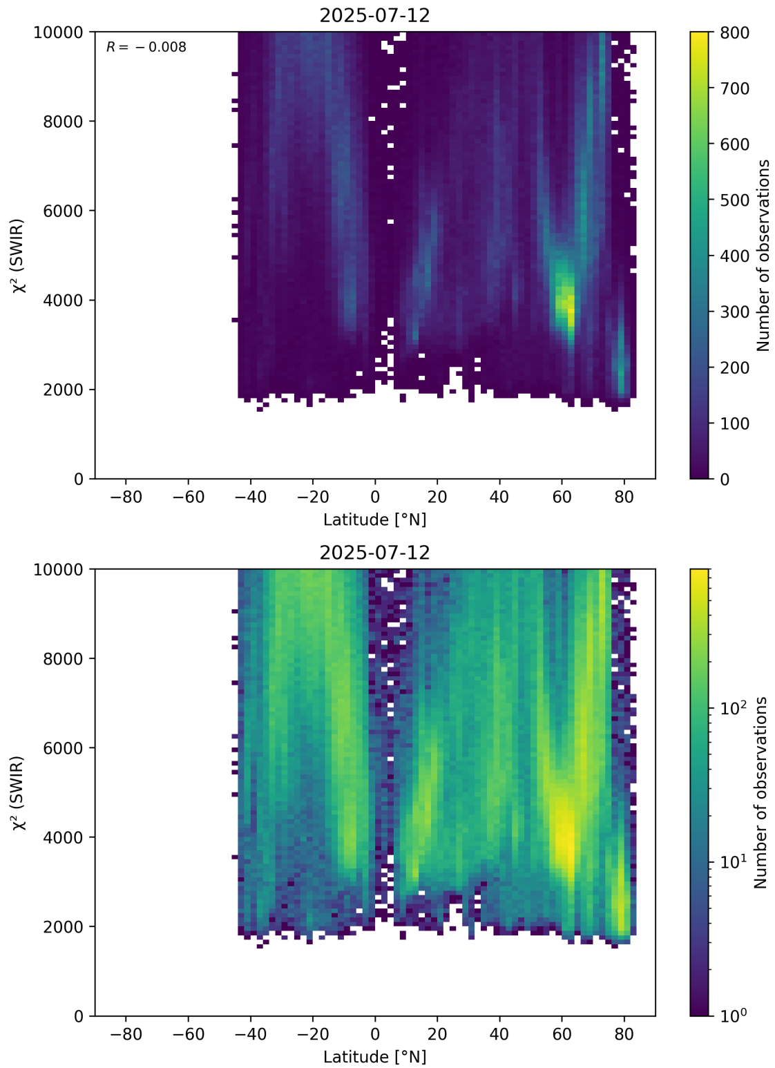
Figure 54: Scatter density plot of “Latitude” against “ \chi^2 (SWIR)” for 2025-07-11 to 2025-07-13.
