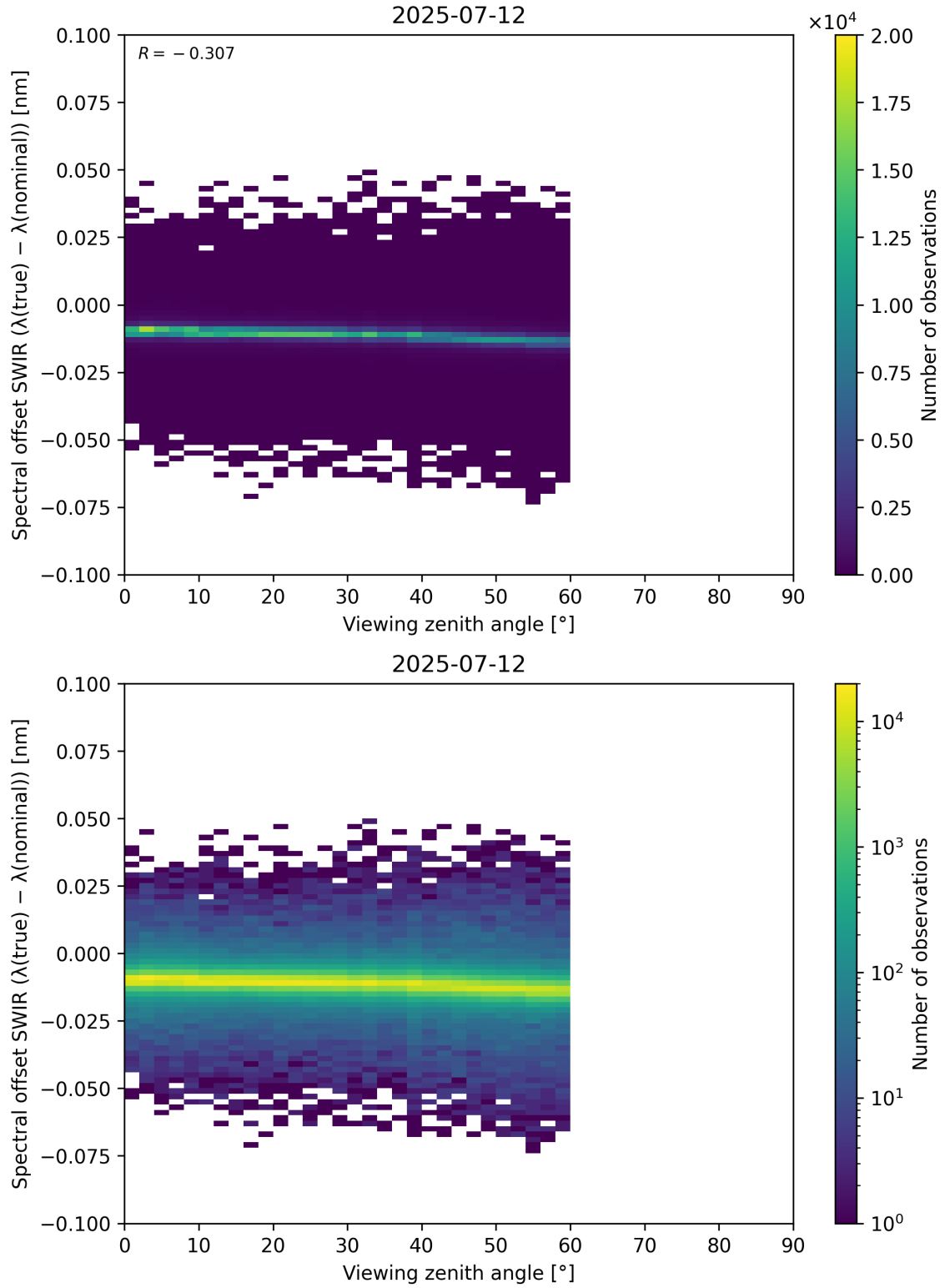
Figure 116: Scatter density plot of “Viewing zenith angle” against “Spectral offset SWIR ( \lambda_{\text{true}} - \lambda_{\text{nominal}} )” for 2025-07-11 to 2025-07-13.
