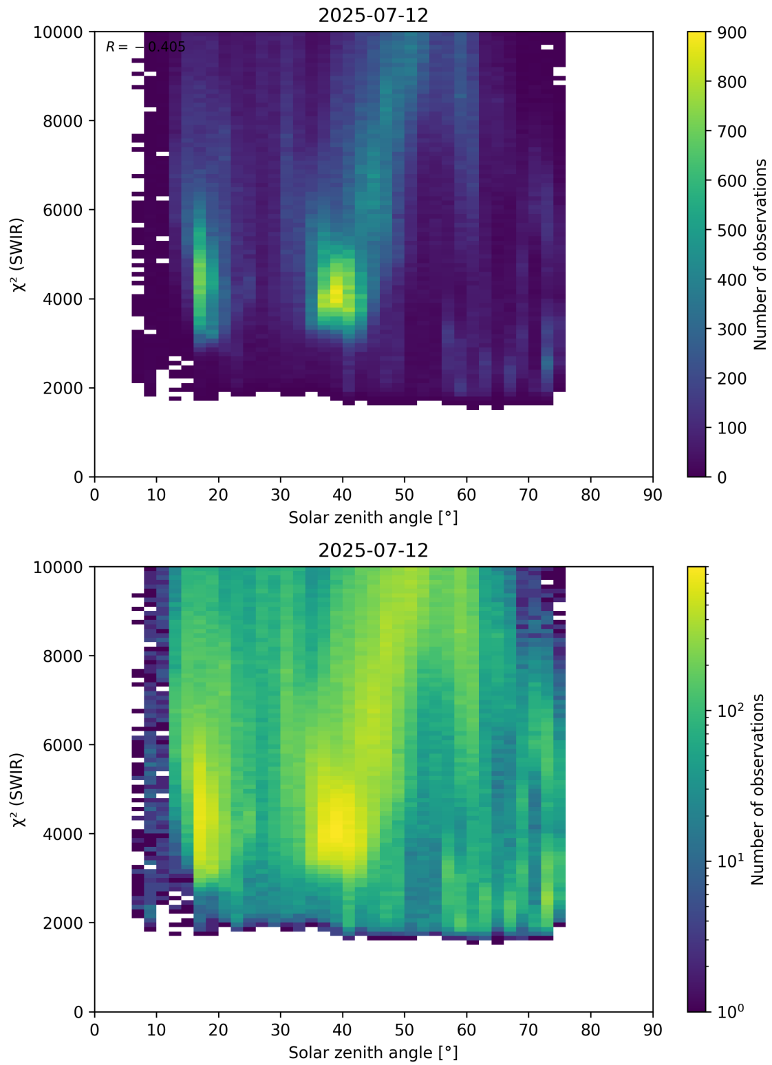
Figure 95: Scatter density plot of “Solar zenith angle” against “ \chi^2 (SWIR)” for 2025-07-11 to 2025-07-13.
