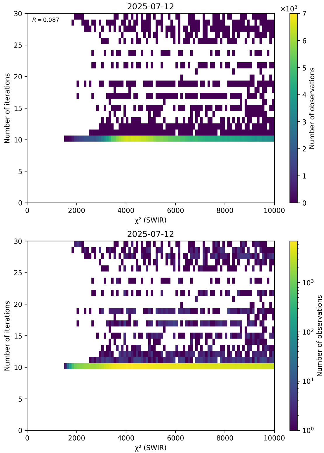
Figure 50: Scatter density plot of “ \chi^2 (SWIR)” against “Number of iterations” for 2025-07-11 to 2025-07-13.
