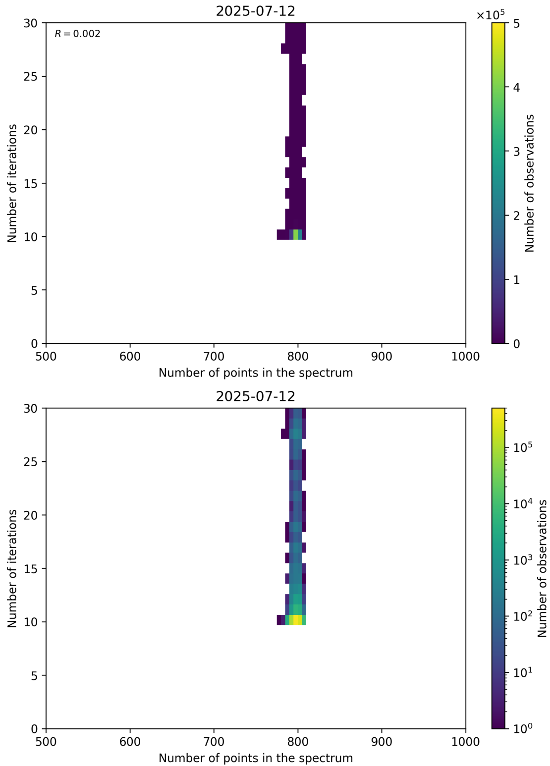
Figure 92: Scatter density plot of “Number of points in the spectrum” against “Number of iterations” for 2025-07-11 to 2025-07-13.
