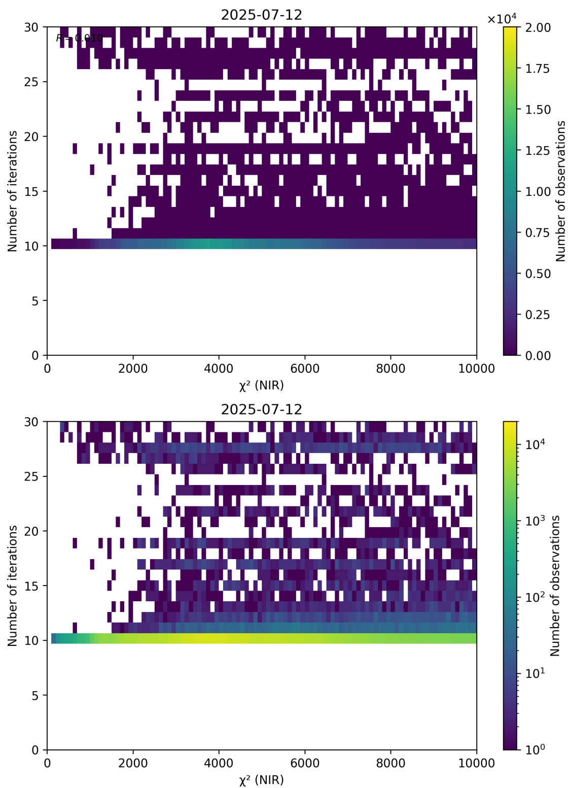
Figure 46: Scatter density plot of “ \chi^2 (NIR)” against “Number of iterations” for 2025-07-11 to 2025-07-13.
