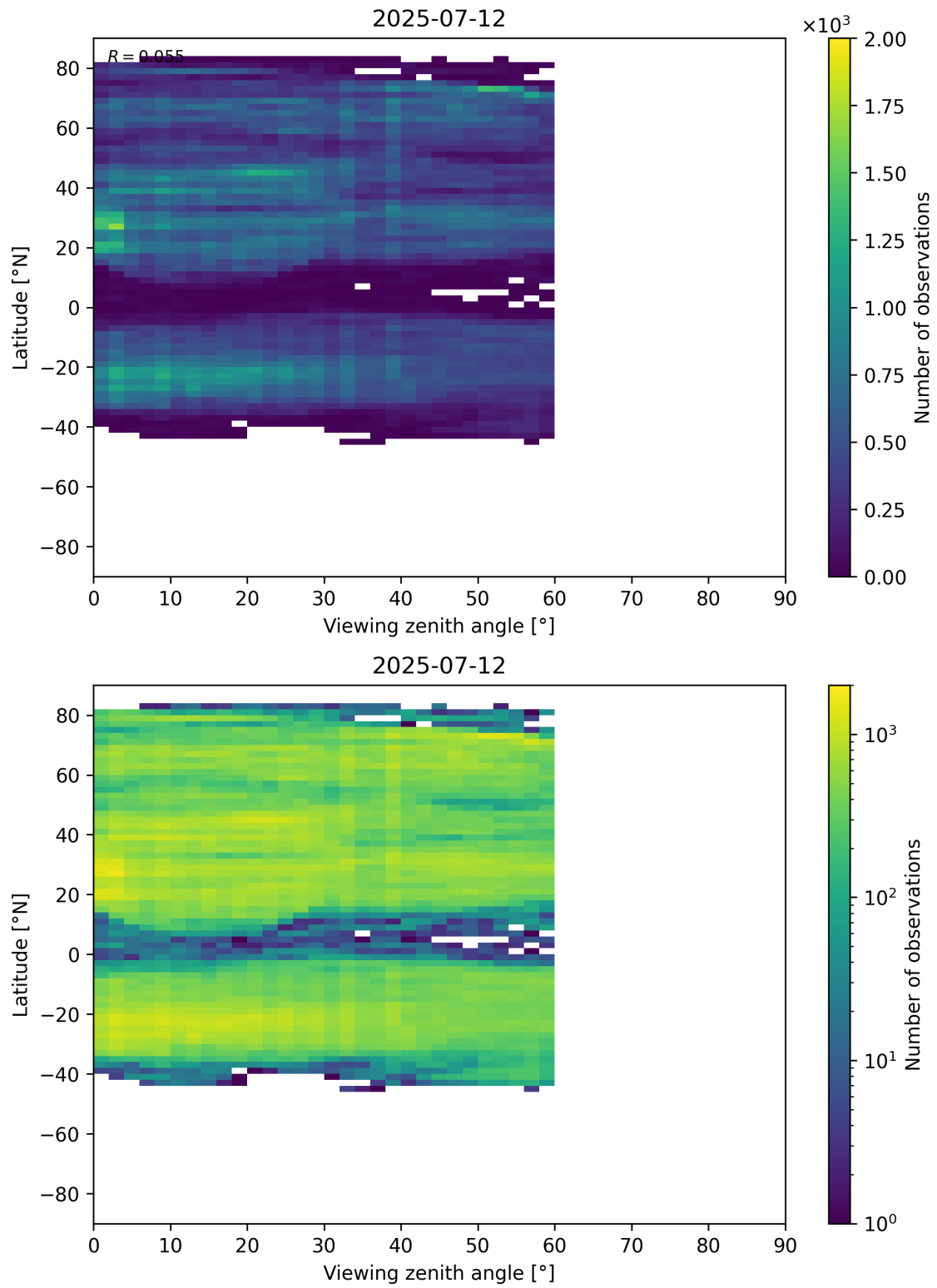
Figure 109: Scatter density plot of “Viewing zenith angle” against “Latitude” for 2025-07-11 to 2025-07-13.
