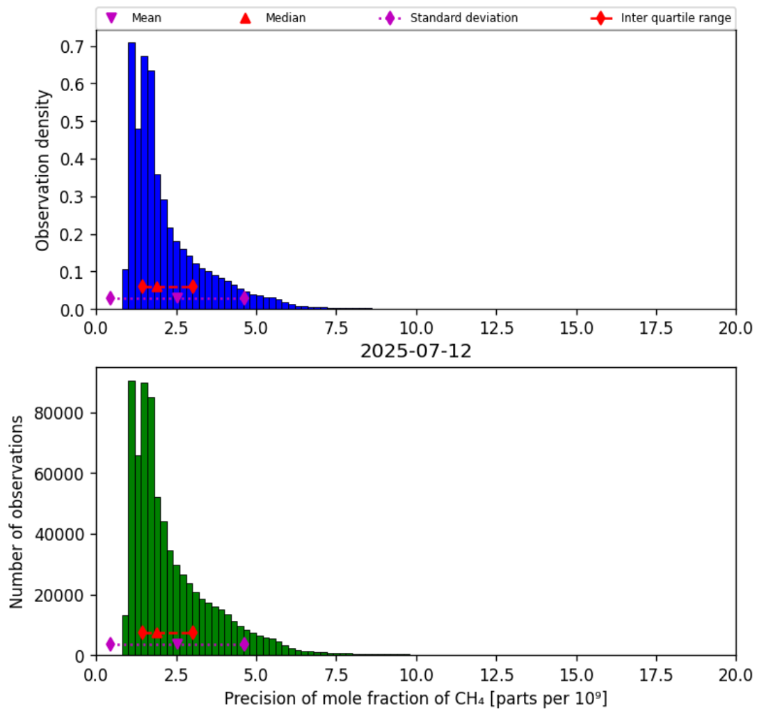
Figure 24: Histogram of “Precision of mole fraction of CH 4 ” for 2025-07-11 to 2025-07-13
