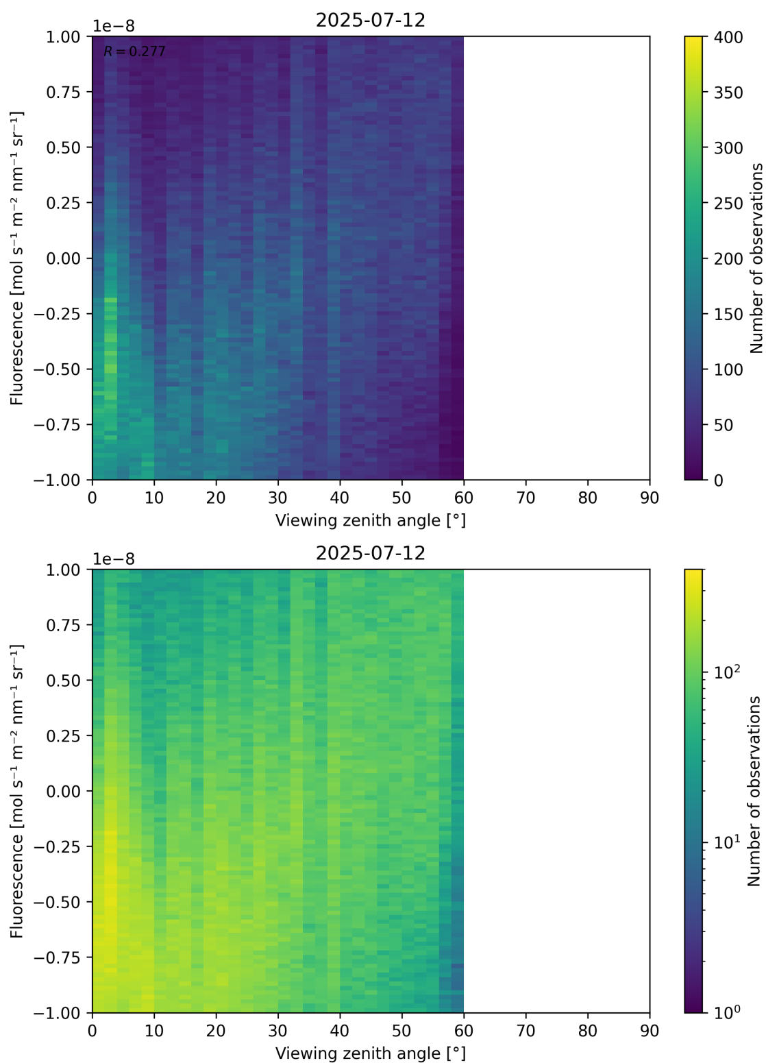
Figure 108: Scatter density plot of “Viewing zenith angle” against “Fluorescence” for 2025-07-11 to 2025-07-13.
