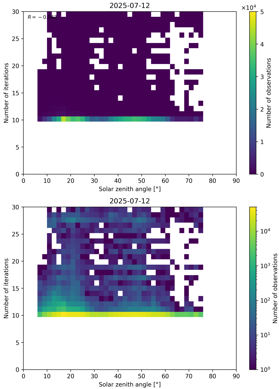
Figure 102: Scatter density plot of “Solar zenith angle” against “Number of iterations” for 2025-07-11 to 2025-07-13.
