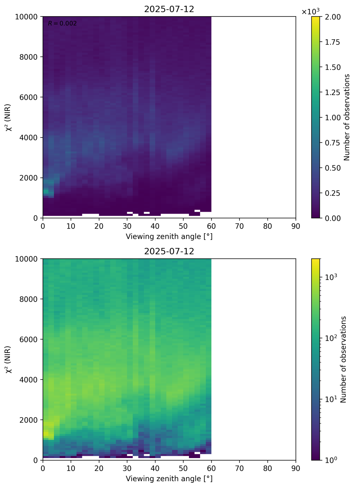
Figure 105: Scatter density plot of “Viewing zenith angle” against “ \chi^2 (NIR)” for 2025-07-11 to 2025-07-13.
