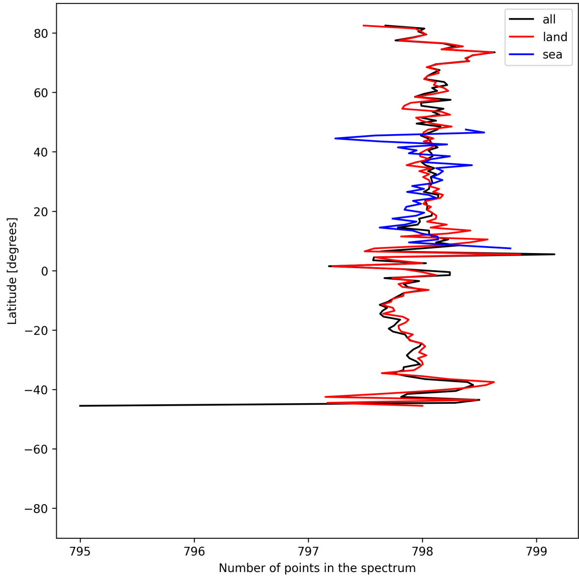
Figure 15: Zonal average of “Number of points in the spectrum” for 2025-07-11 to 2025-07-13.
