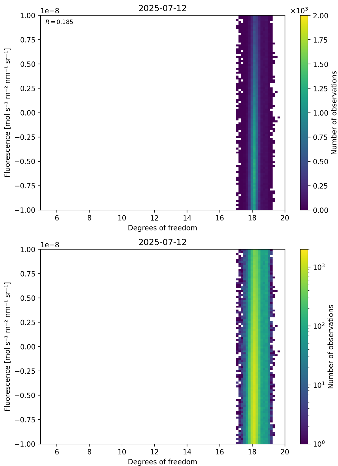
Figure 51: Scatter density plot of “Degrees of freedom” against “Fluorescence” for 2025-07-11 to 2025-07-13.
