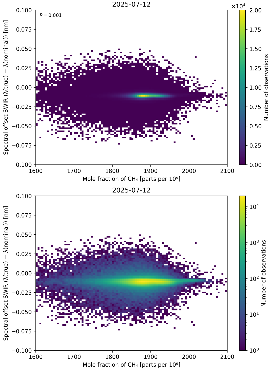
Figure 86: Scatter density plot of “Mole fraction of CH 4 ” against “Spectral offset SWIR ( \lambda_{\text{true}} - \lambda_{\text{nominal}} )” for 2025-07-11 to 2025-07-13.
