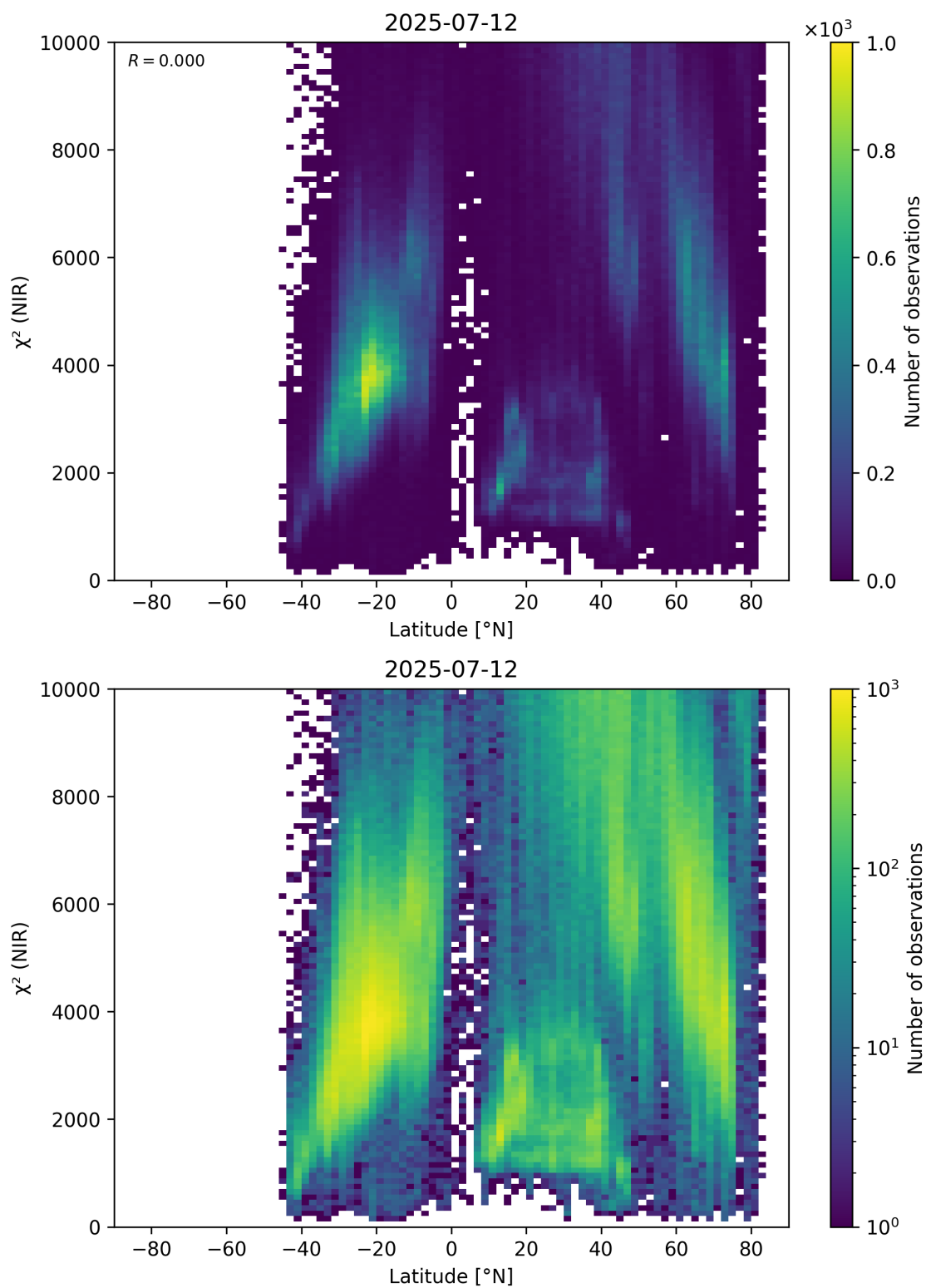
Figure 53: Scatter density plot of “Latitude” against “ \chi^2 (NIR)” for 2025-07-11 to 2025-07-13.
