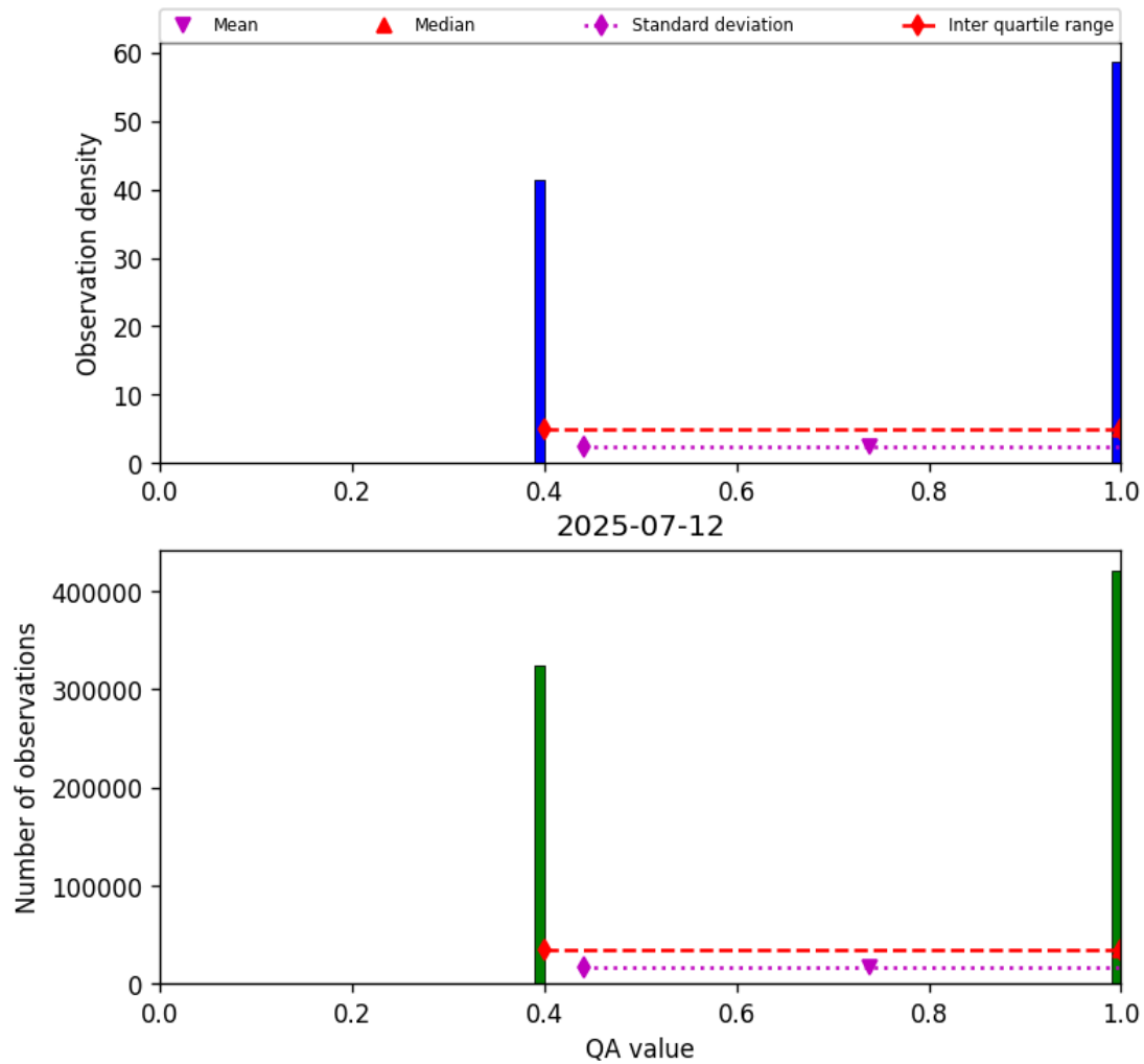
Figure 22: Histogram of “QA value” for 2025-07-11 to 2025-07-13
