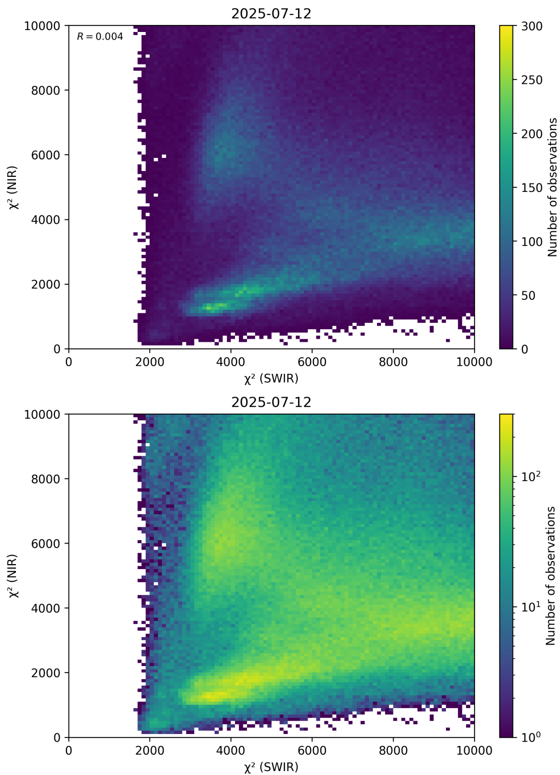
Figure 47: Scatter density plot of “ \chi^2 (SWIR)” against “ \chi^2 (NIR)” for 2025-07-11 to 2025-07-13.
