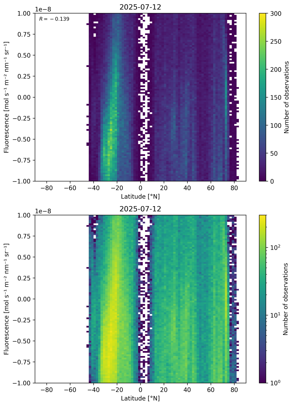
Figure 56: Scatter density plot of “Latitude” against “Fluorescence” for 2025-07-11 to 2025-07-13.
