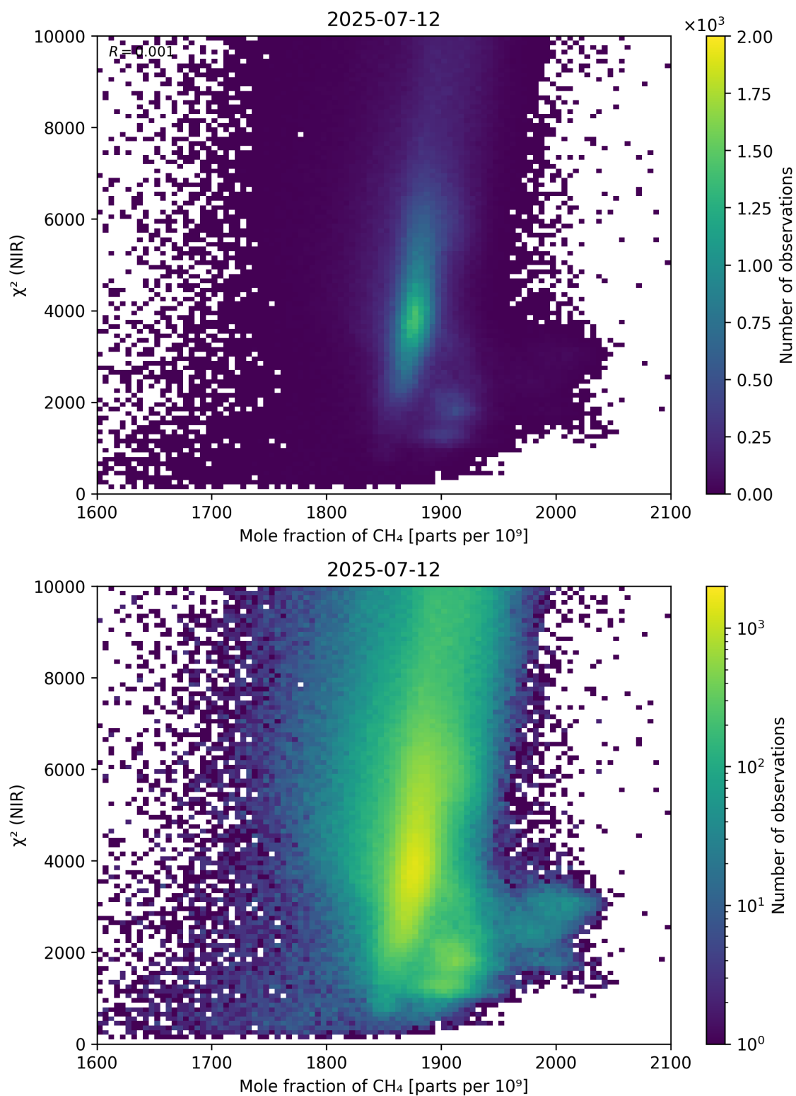
Figure 70: Scatter density plot of “Mole fraction of \text{CH}_4 ” against “ \chi^2 (NIR)” for 2025-07-11 to 2025-07-13.
