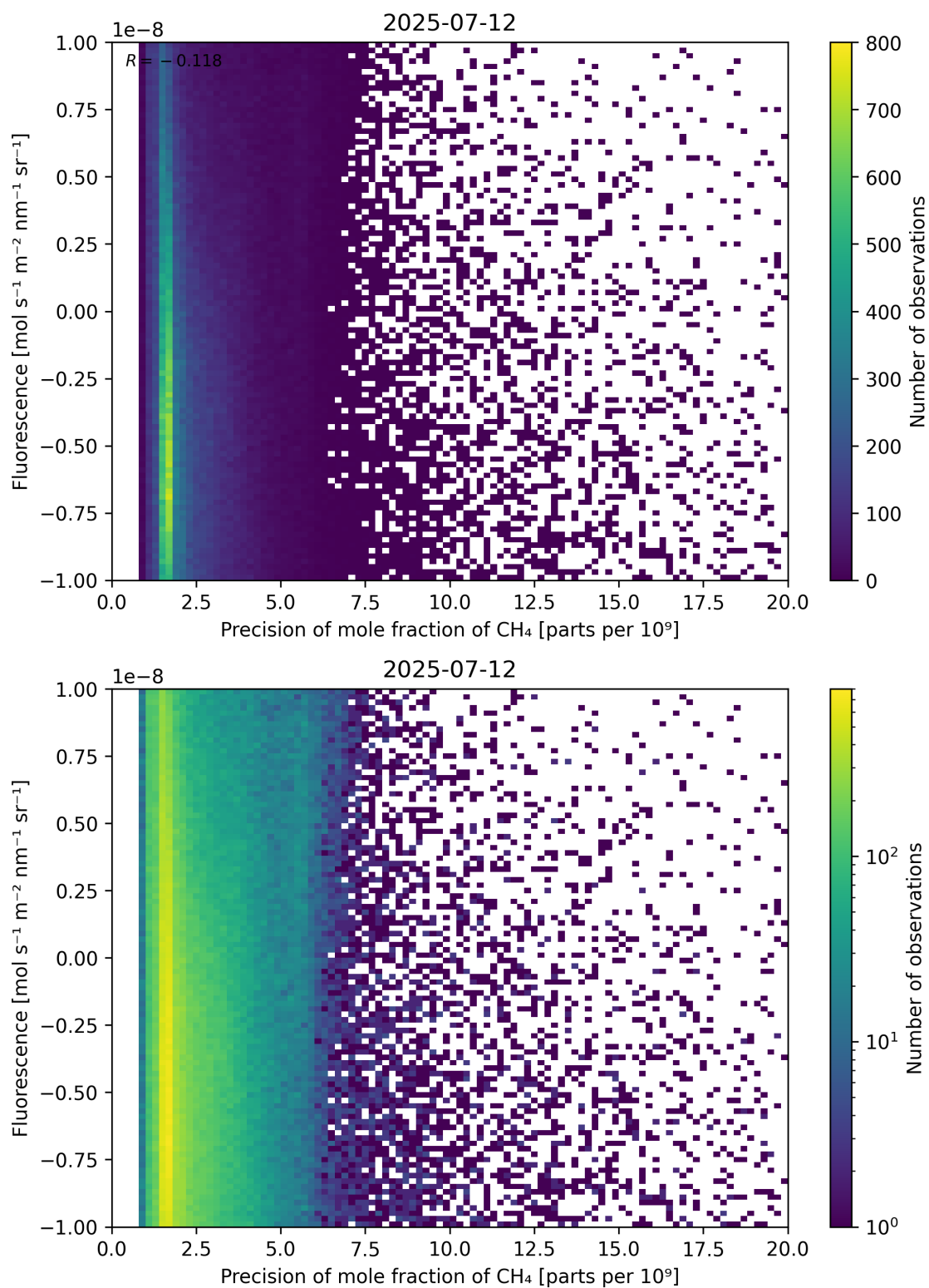
Figure 81: Scatter density plot of “Precision of mole fraction of \text{CH}_4 ” against “Fluorescence” for 2025-07-11 to 2025-07-13.
