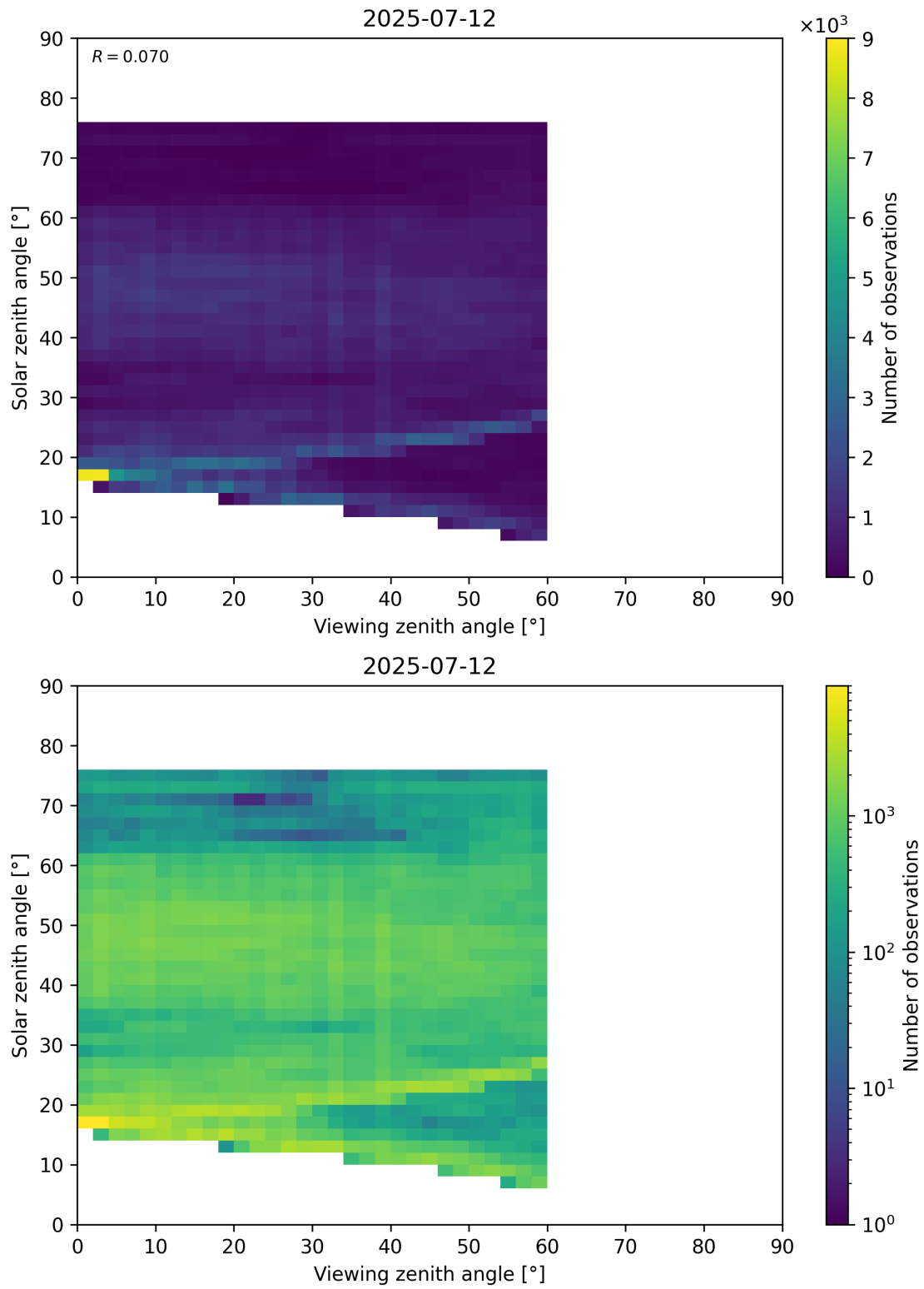
Figure 115: Scatter density plot of “Viewing zenith angle” against “Solar zenith angle” for 2025-07-11 to 2025-07-13.
