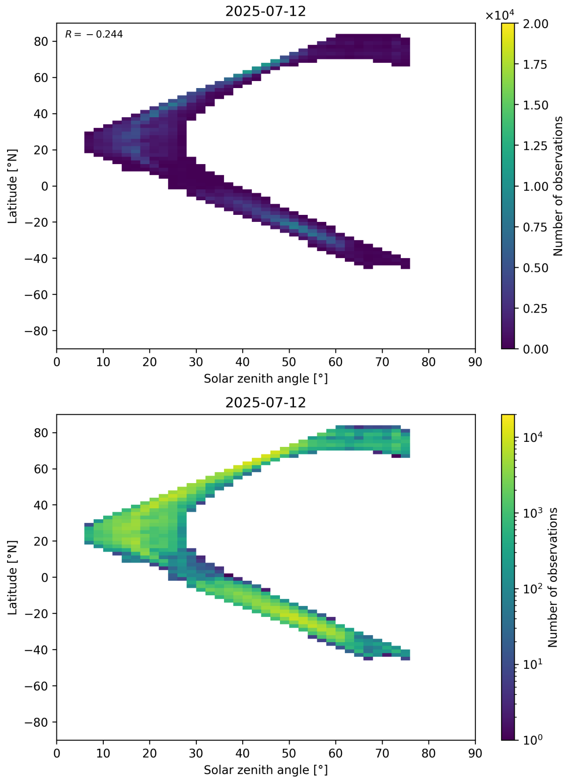
Figure 98: Scatter density plot of “Solar zenith angle” against “Latitude” for 2025-07-11 to 2025-07-13.
