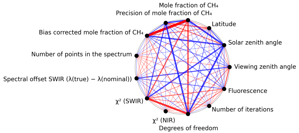
Figure 1: Map of correlation graph for 2025-07-11 to 2025-07-13.
