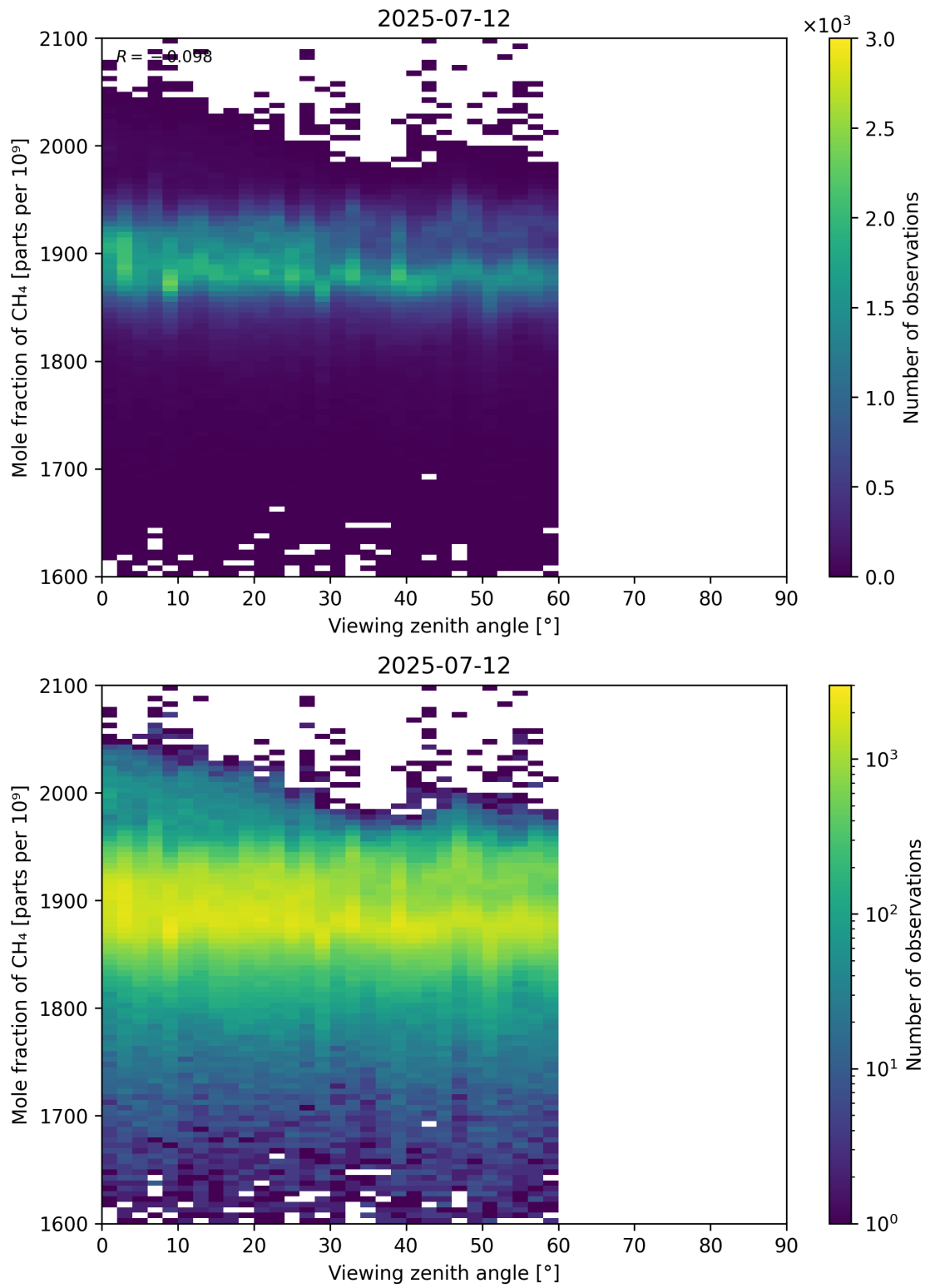
Figure 110: Scatter density plot of “Viewing zenith angle” against “Mole fraction of CH 4 ” for 2025-07-11 to 2025-07-13.
