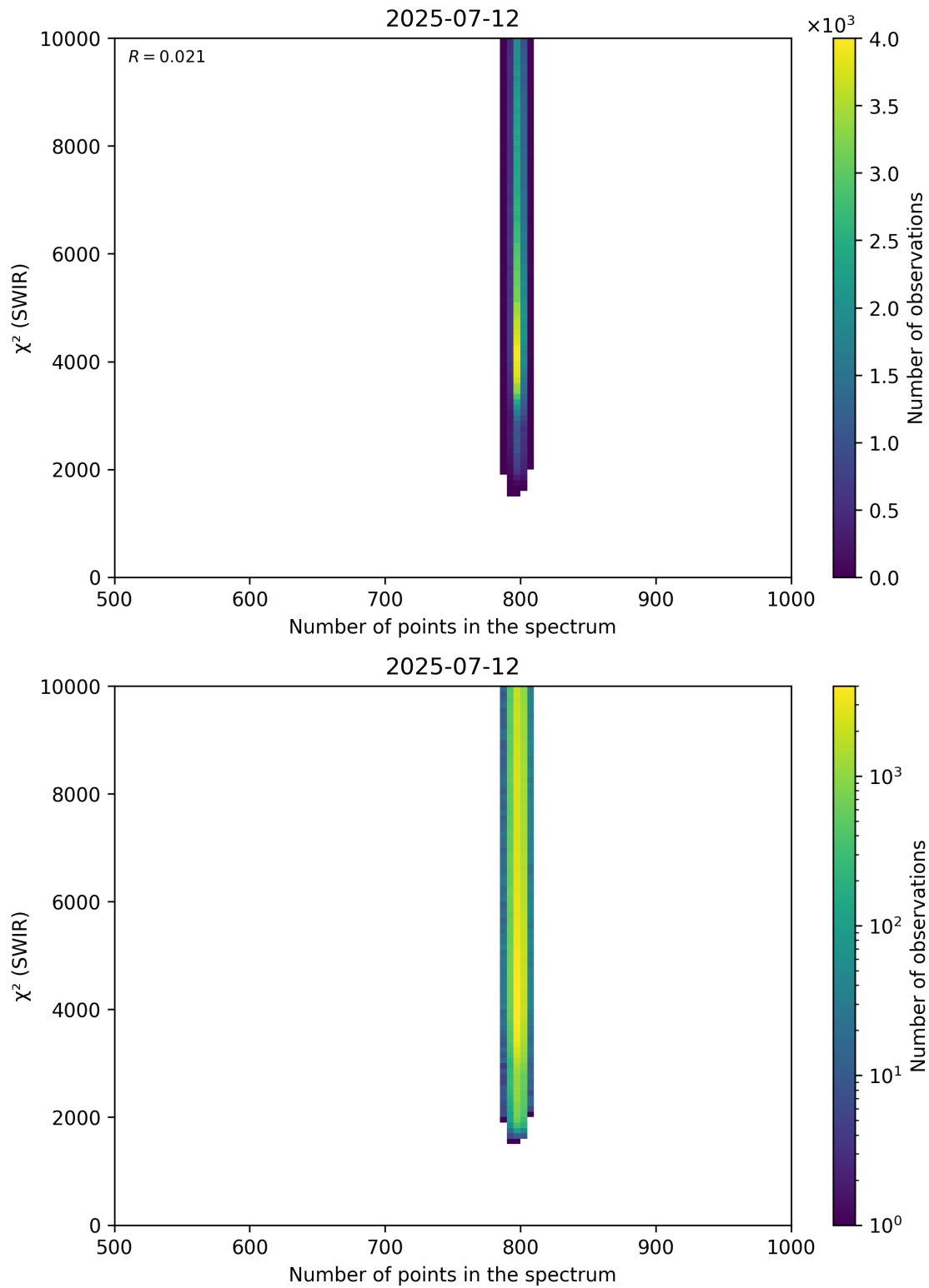
Figure 89: Scatter density plot of “Number of points in the spectrum” against “ \chi^2 (SWIR)” for 2025-07-11 to 2025-07-13.
