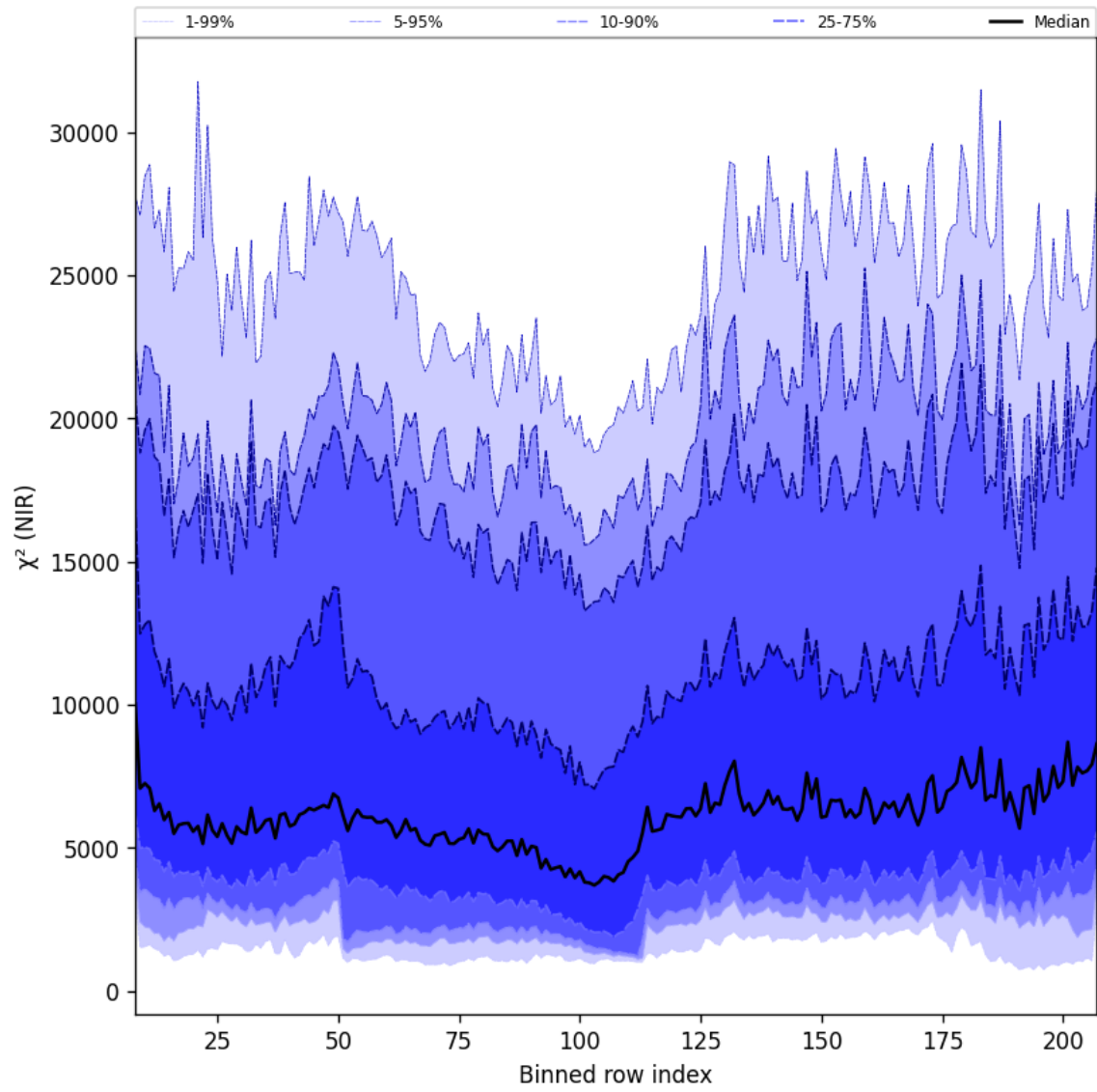
Figure 40: Along track statistics of “ \chi^2 (NIR)” for 2025-07-11 to 2025-07-13
