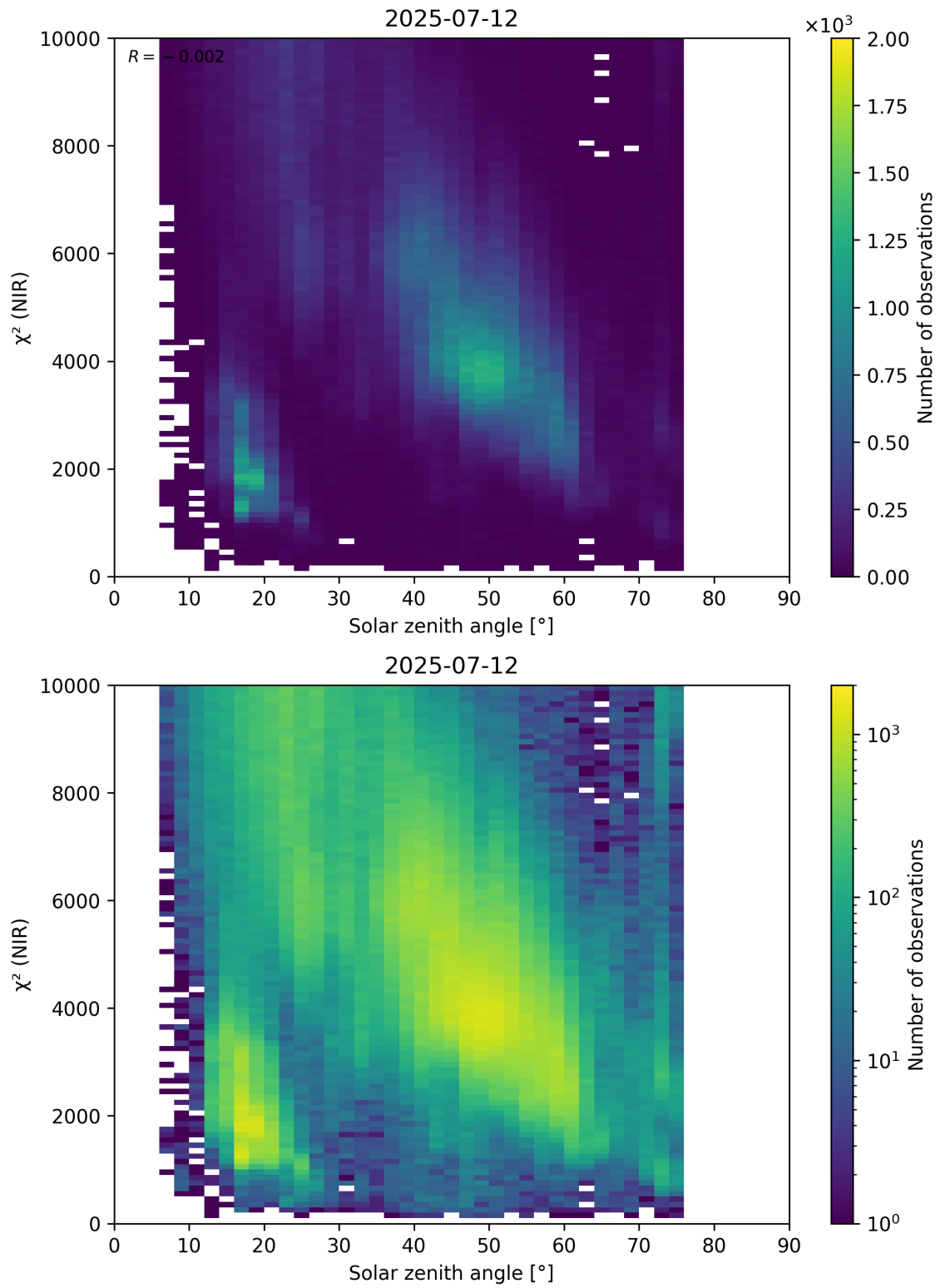
Figure 94: Scatter density plot of “Solar zenith angle” against “ \chi^2 (NIR)” for 2025-07-11 to 2025-07-13.
