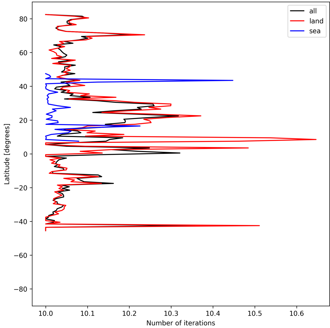
Figure 20: Zonal average of “Number of iterations” for 2025-07-11 to 2025-07-13.
