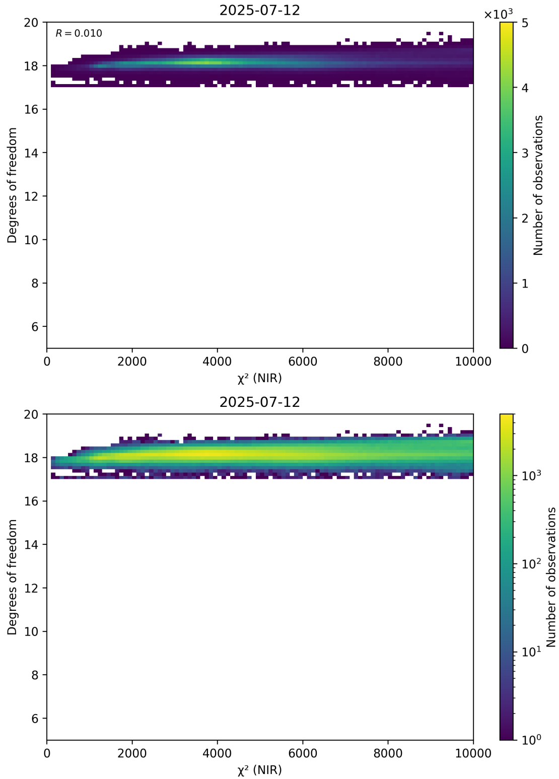
Figure 44: Scatter density plot of “ \chi^2 (NIR)” against “Degrees of freedom” for 2025-07-11 to 2025-07-13.
