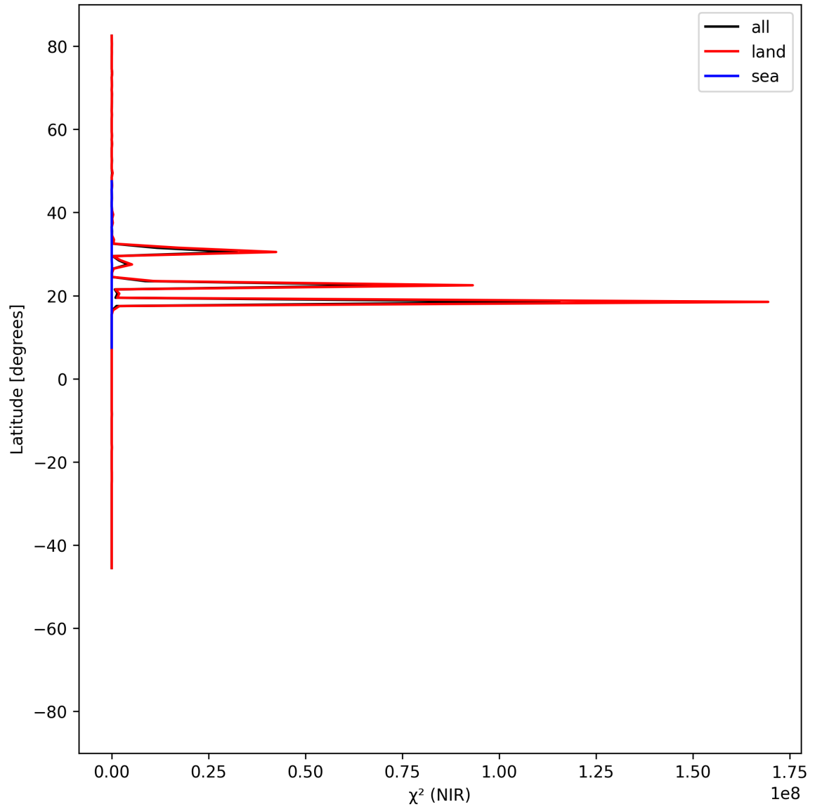
Figure 18: Zonal average of “ \chi^2 (NIR)” for 2025-07-11 to 2025-07-13.
