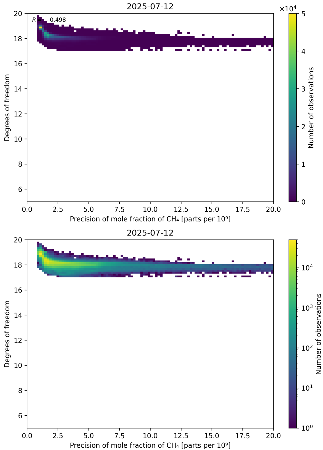
Figure 80: Scatter density plot of “Precision of mole fraction of CH 4 ” against “Degrees of freedom” for 2025-07-11 to 2025-07-13.
