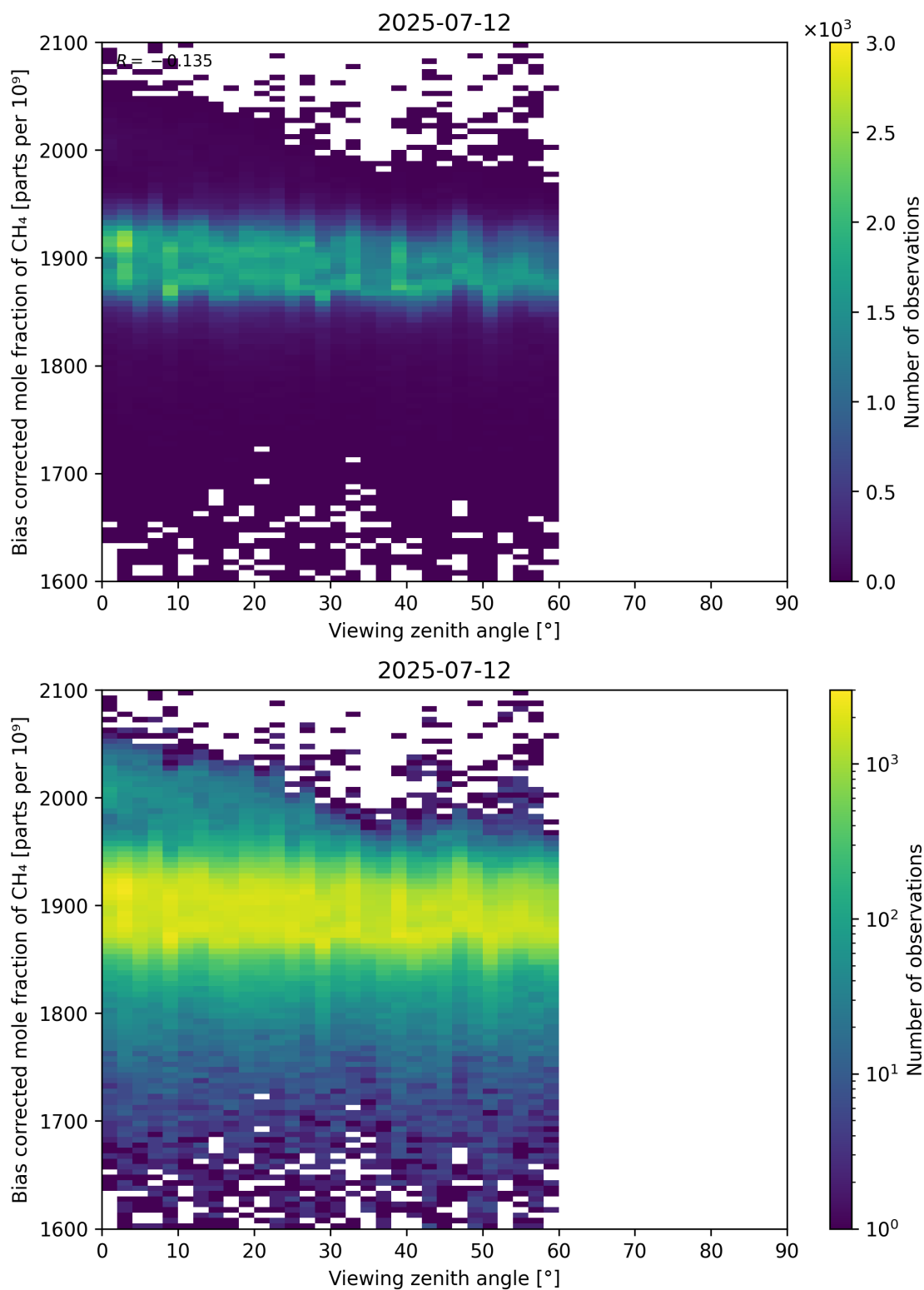
Figure 111: Scatter density plot of “Viewing zenith angle” against “Bias corrected mole fraction of CH 4 ” for 2025-07-11 to 2025-07-13.
