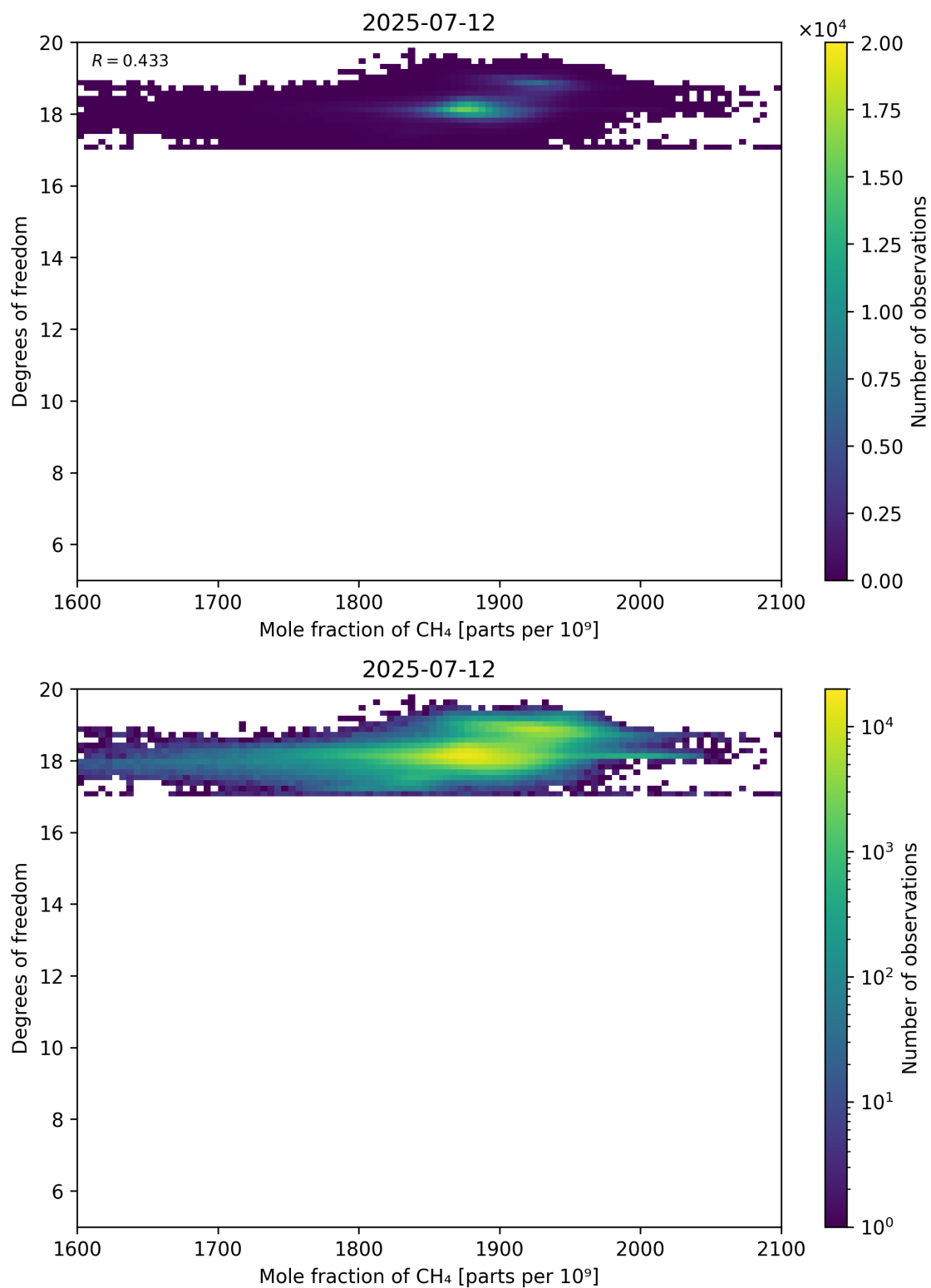
Figure 72: Scatter density plot of “Mole fraction of CH 4 ” against “Degrees of freedom” for 2025-07-11 to 2025-07-13.
