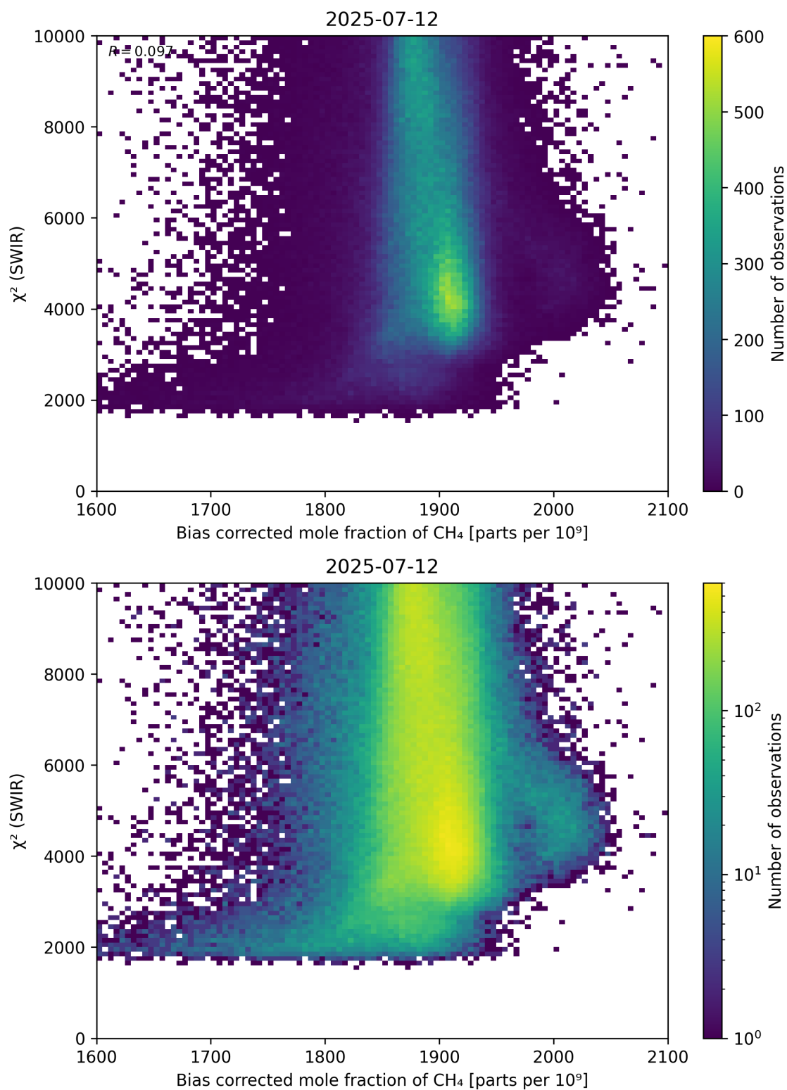
Figure 64: Scatter density plot of “Bias corrected mole fraction of \text{CH}_4 ” against “ \chi^2 (SWIR)” for 2025-07-11 to 2025-07-13.
