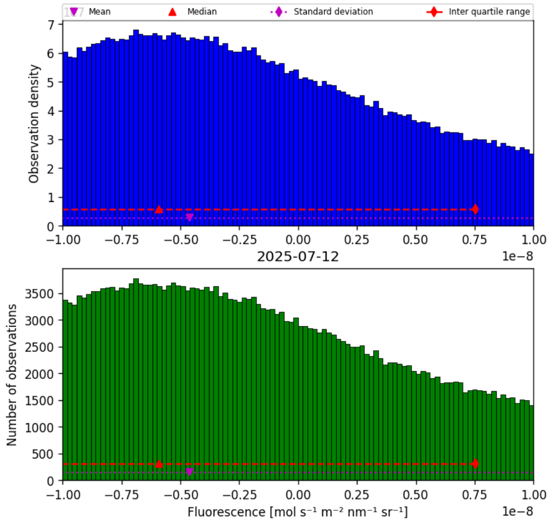
Figure 32: Histogram of “Fluorescence” for 2025-07-11 to 2025-07-13
