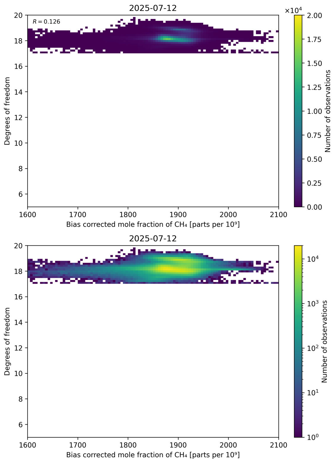
Figure 65: Scatter density plot of “Bias corrected mole fraction of CH 4 ” against “Degrees of freedom” for 2025-07-11 to 2025-07-13.
