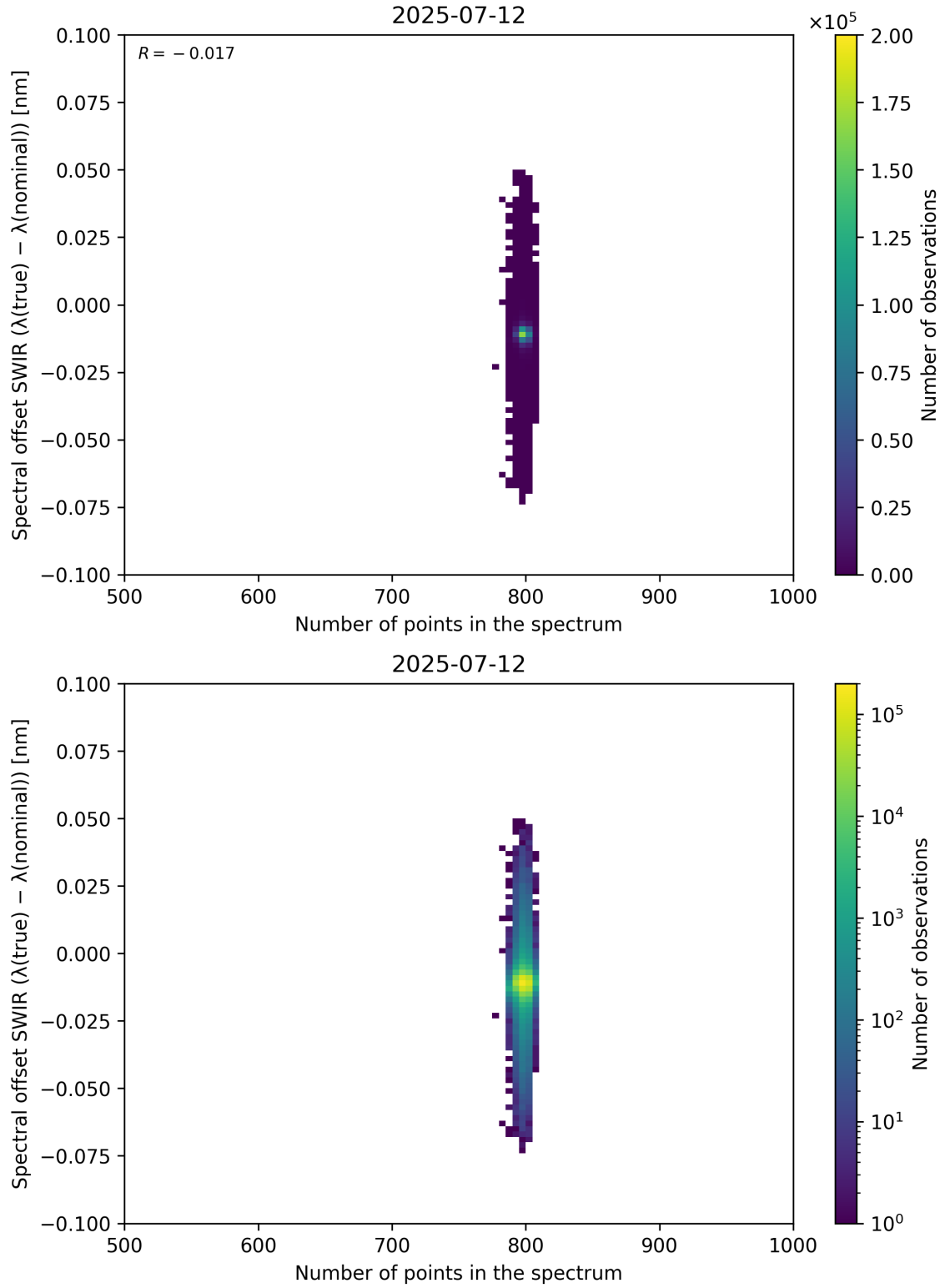
Figure 93: Scatter density plot of “Number of points in the spectrum” against “Spectral offset SWIR ( \lambda_{\text{true}} - \lambda_{\text{nominal}} )” for 2025-07-11 to 2025-07-13.
