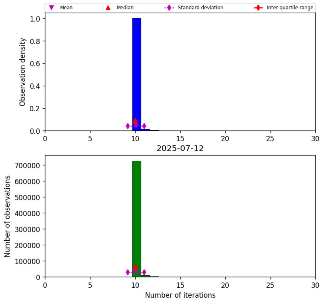
Figure 31: Histogram of “Number of iterations” for 2025-07-11 to 2025-07-13
