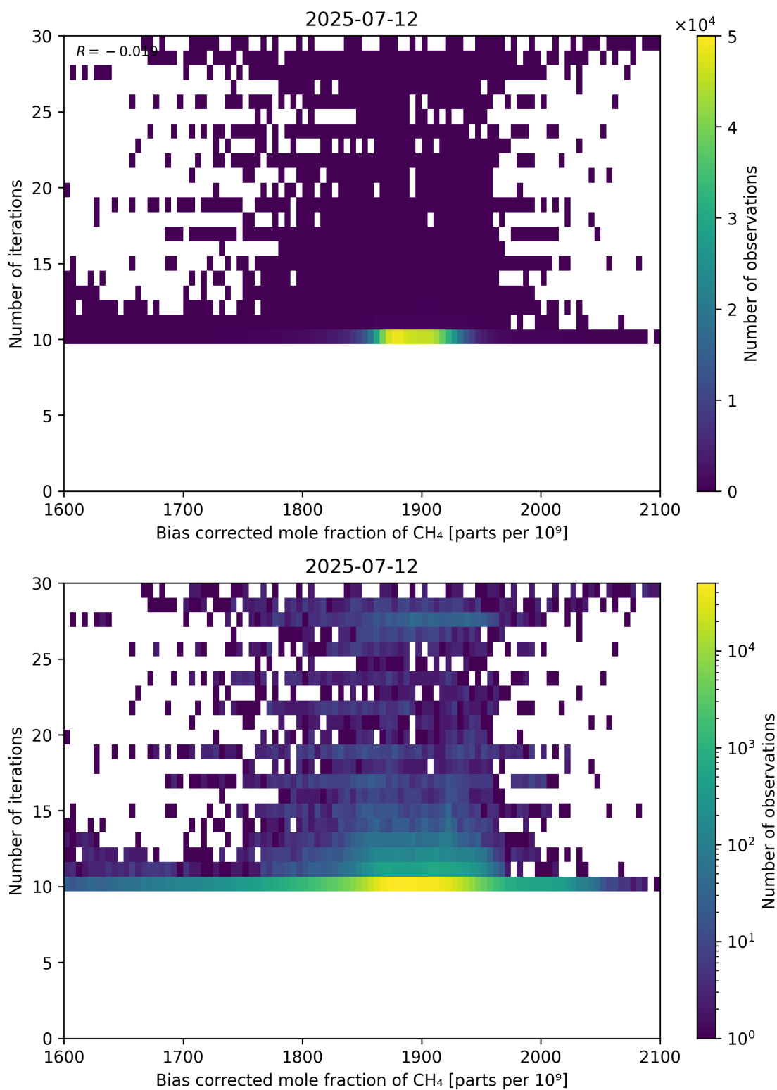
Figure 67: Scatter density plot of “Bias corrected mole fraction of CH 4 ” against “Number of iterations” for 2025-07-11 to 2025-07-13.
