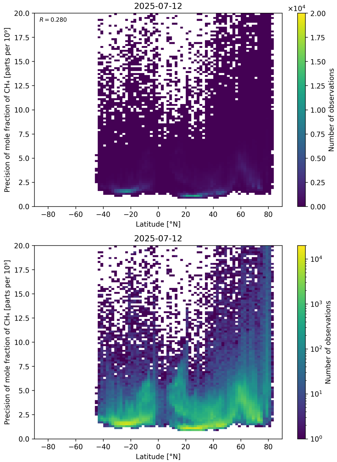
Figure 59: Scatter density plot of “Latitude” against “Precision of mole fraction of \text{CH}_4 ” for 2025-07-11 to 2025-07-13.
