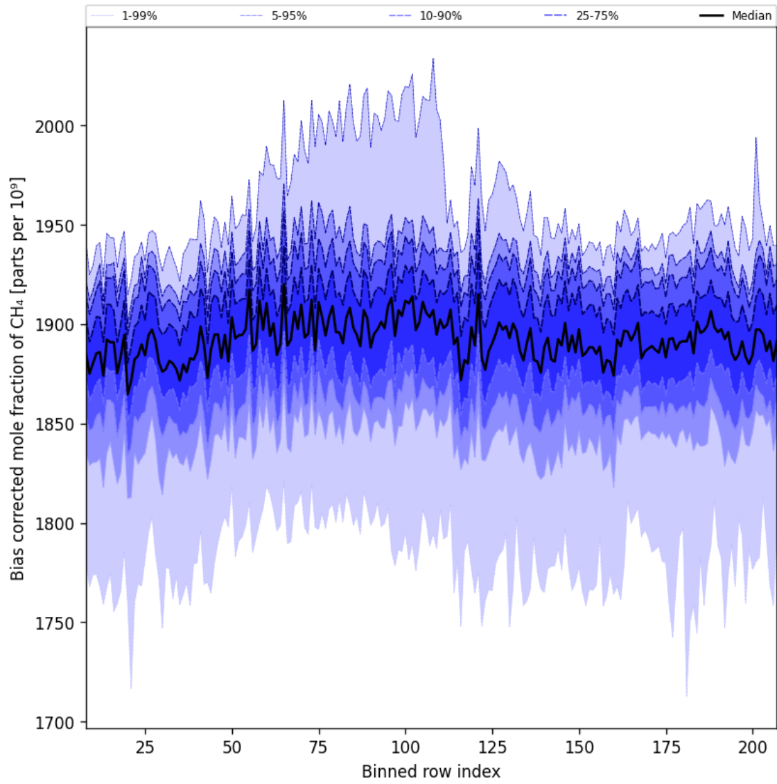
Figure 36: Along track statistics of “Bias corrected mole fraction of CH 4 ” for 2025-07-11 to 2025-07-13
