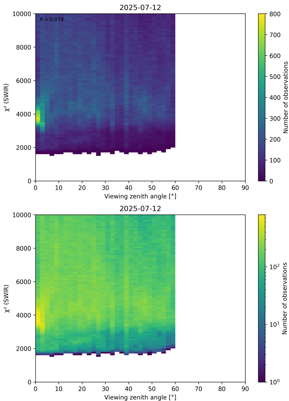
Figure 106: Scatter density plot of “Viewing zenith angle” against “ \chi^2 (SWIR)” for 2025-07-11 to 2025-07-13.
