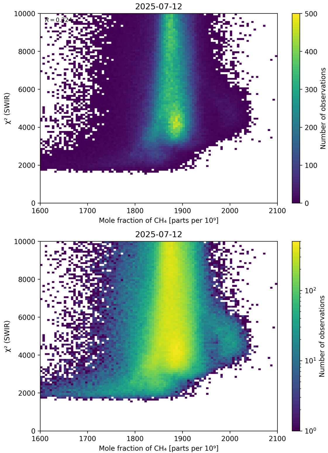
Figure 71: Scatter density plot of “Mole fraction of \text{CH}_4 ” against “ \chi^2 (SWIR)” for 2025-07-11 to 2025-07-13.
