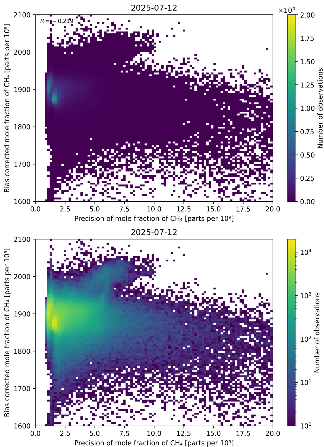
Figure 82: Scatter density plot of “Precision of mole fraction of CH 4 ” against “Bias corrected mole fraction of CH 4 ” for 2025-07-11 to 2025-07-13.
