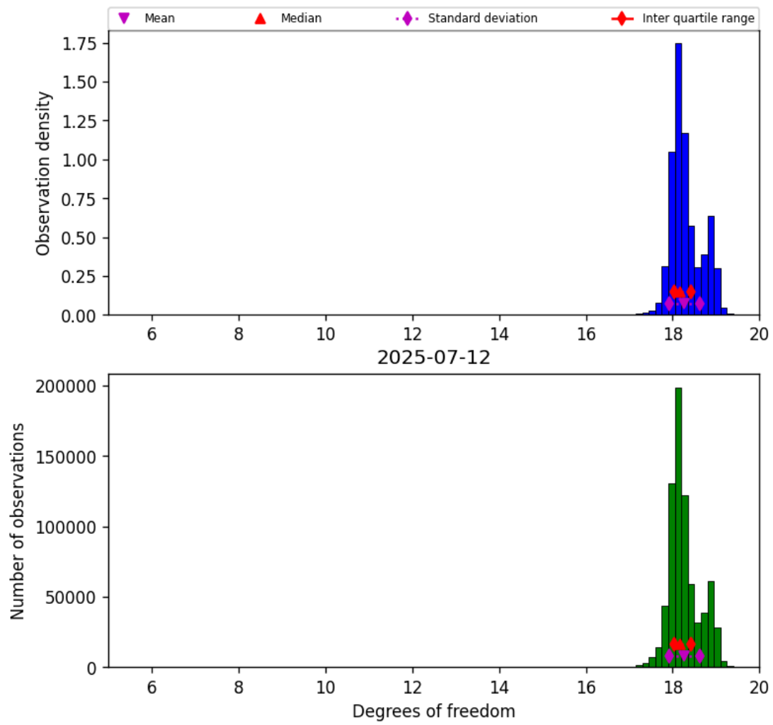
Figure 30: Histogram of “Degrees of freedom” for 2025-07-11 to 2025-07-13
