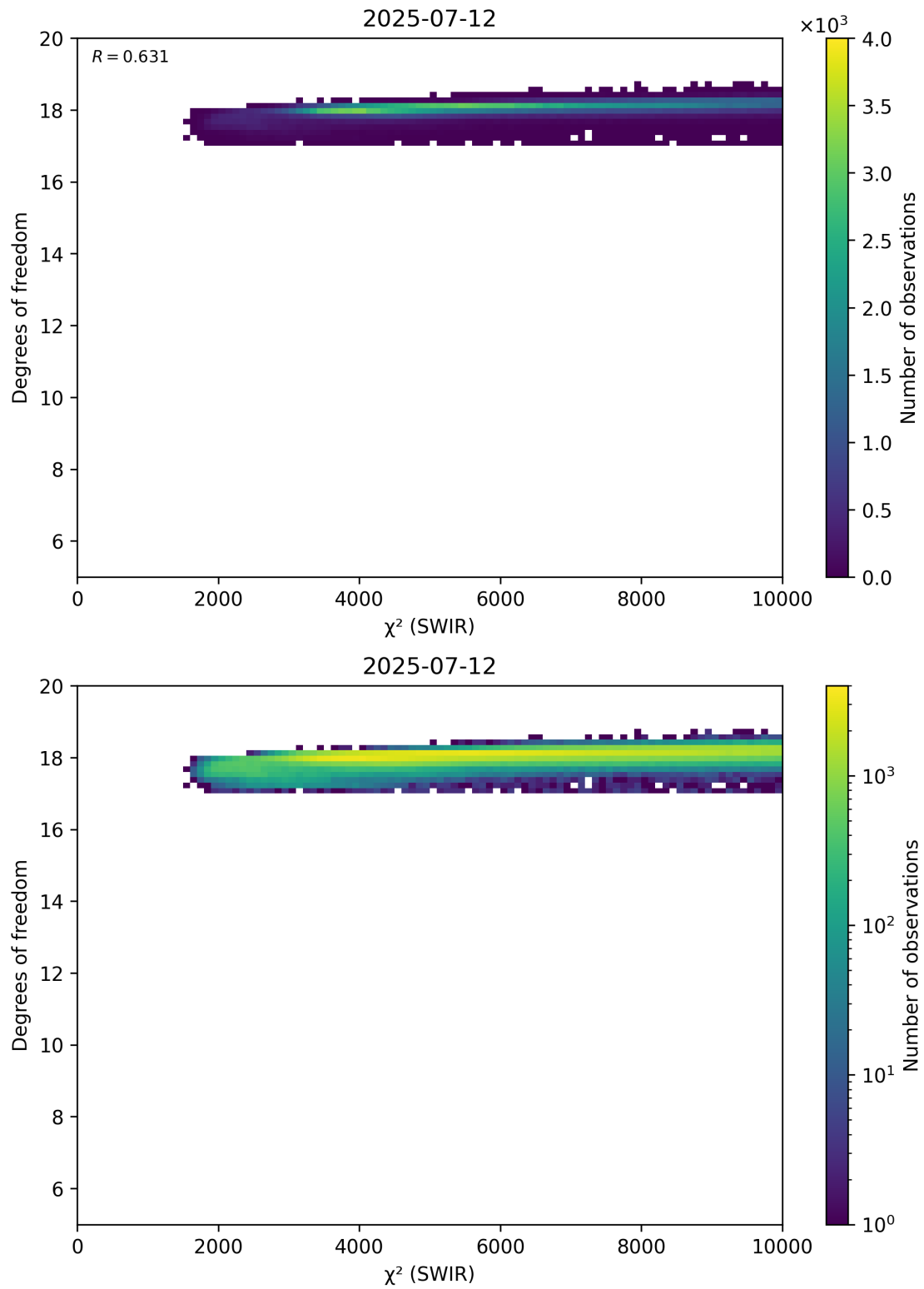
Figure 48: Scatter density plot of “ \chi^2 (SWIR)” against “Degrees of freedom” for 2025-07-11 to 2025-07-13.
