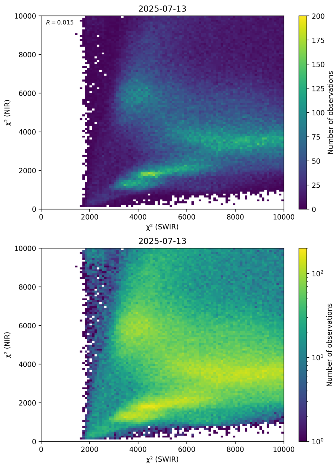
Figure 47: Scatter density plot of “ \chi^2 (SWIR)” against “ \chi^2 (NIR)” for 2025-07-13 to 2025-07-14.
