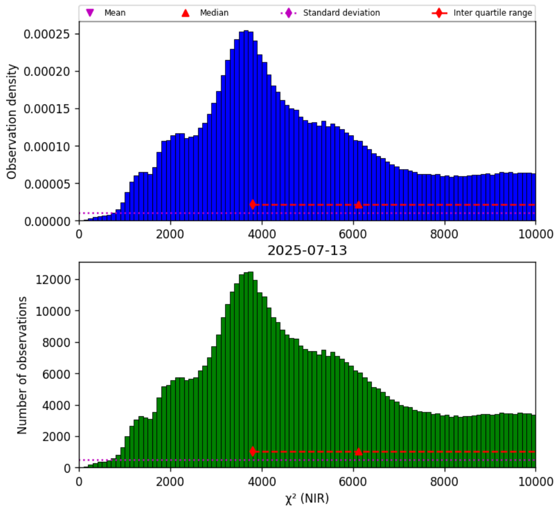
Figure 29: Histogram of “ \chi^2 (NIR)” for 2025-07-13 to 2025-07-14
