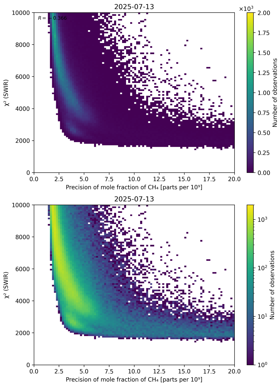
Figure 79: Scatter density plot of “Precision of mole fraction of \text{CH}_4 ” against “ \chi^2 (SWIR)” for 2025-07-13 to 2025-07-14.
