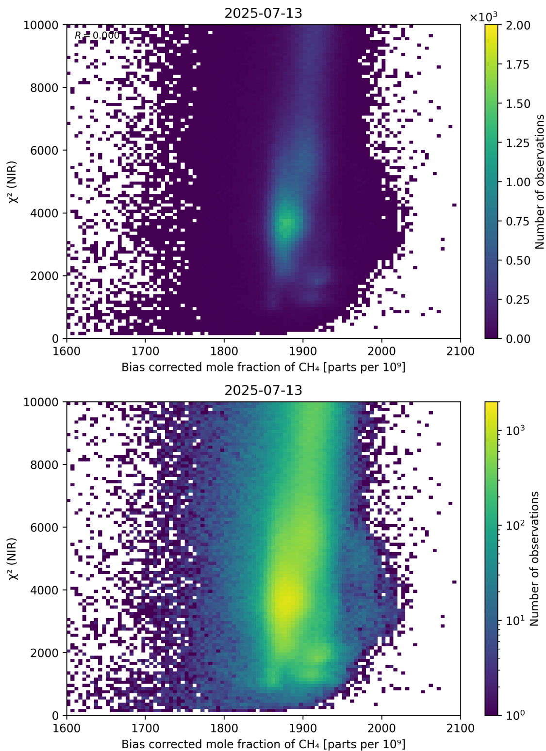
Figure 63: Scatter density plot of “Bias corrected mole fraction of \text{CH}_4 ” against “ \chi^2 (NIR)” for 2025-07-13 to 2025-07-14.
