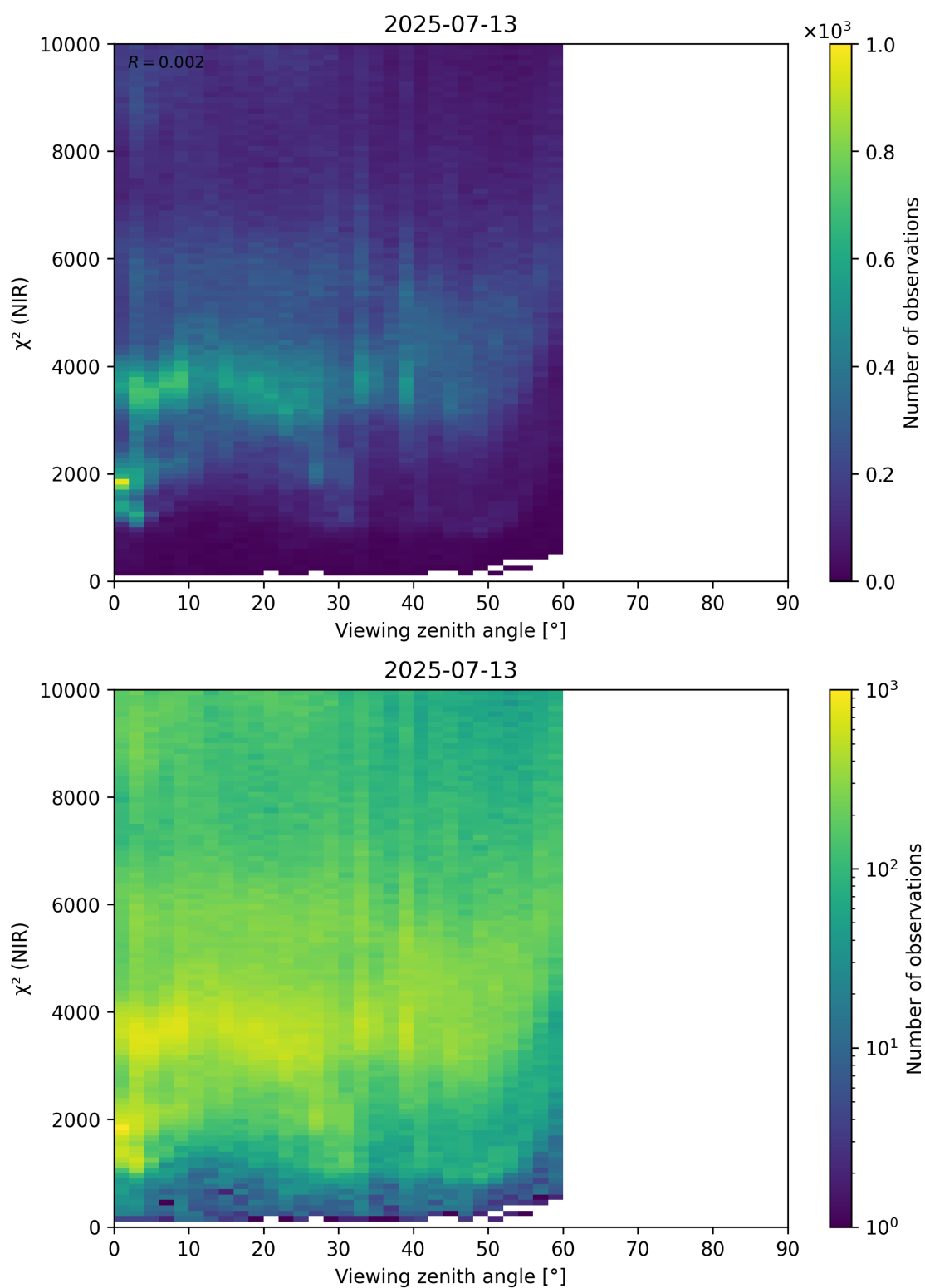
Figure 105: Scatter density plot of “Viewing zenith angle” against “ \chi^2 (NIR)” for 2025-07-13 to 2025-07-14.
