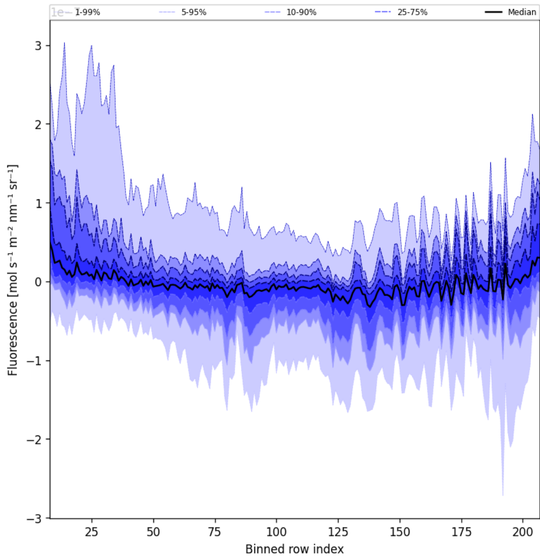
Figure 43: Along track statistics of “Fluorescence” for 2025-07-13 to 2025-07-14
