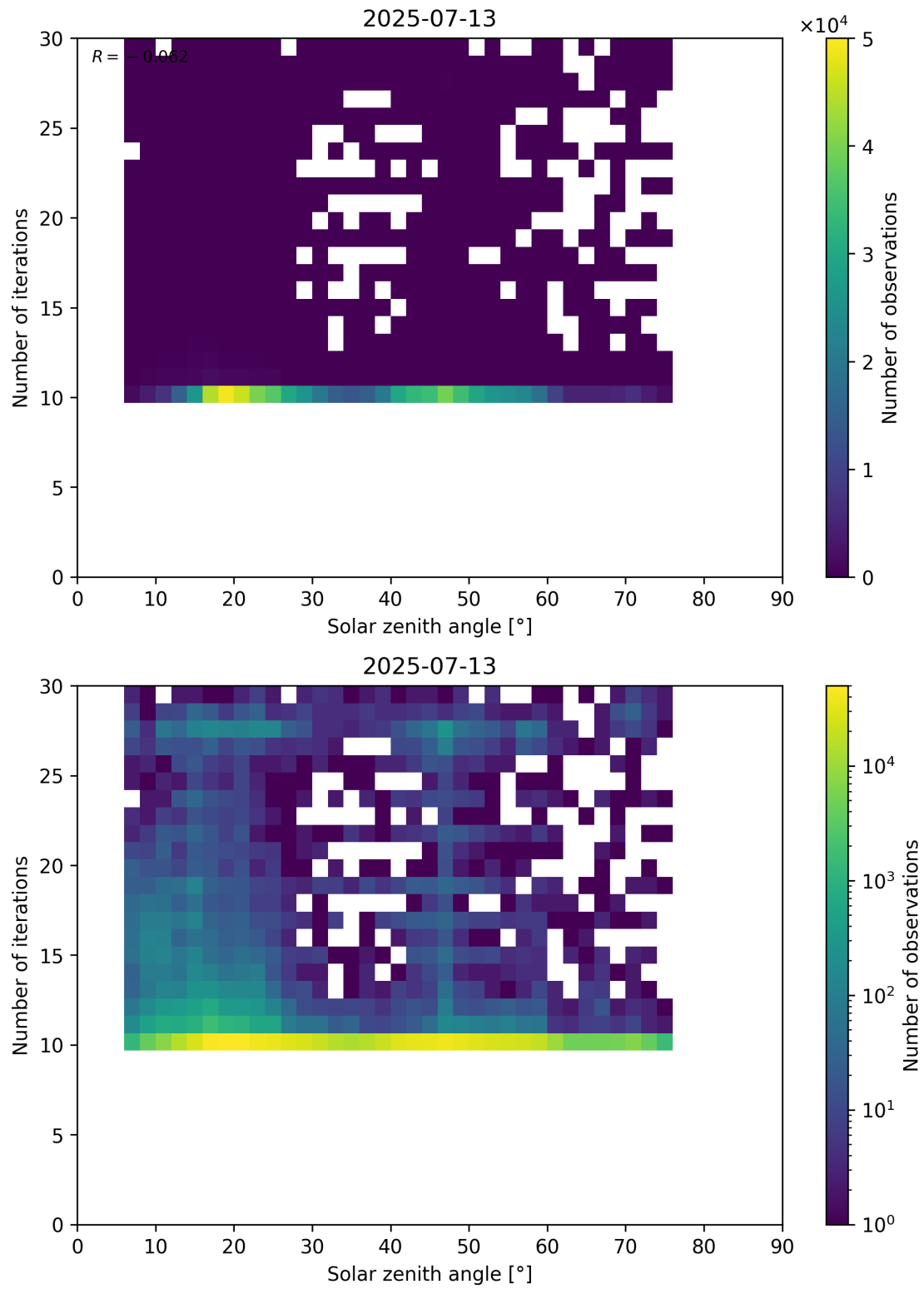
Figure 102: Scatter density plot of “Solar zenith angle” against “Number of iterations” for 2025-07-13 to 2025-07-14.
