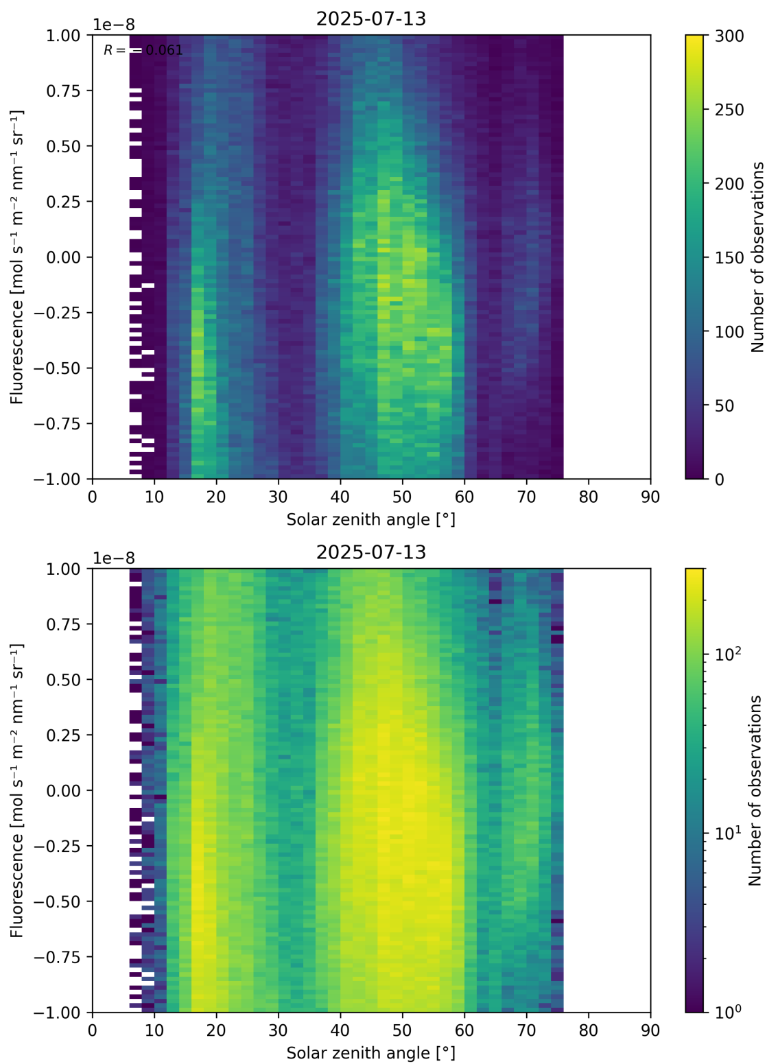
Figure 97: Scatter density plot of “Solar zenith angle” against “Fluorescence” for 2025-07-13 to 2025-07-14.
