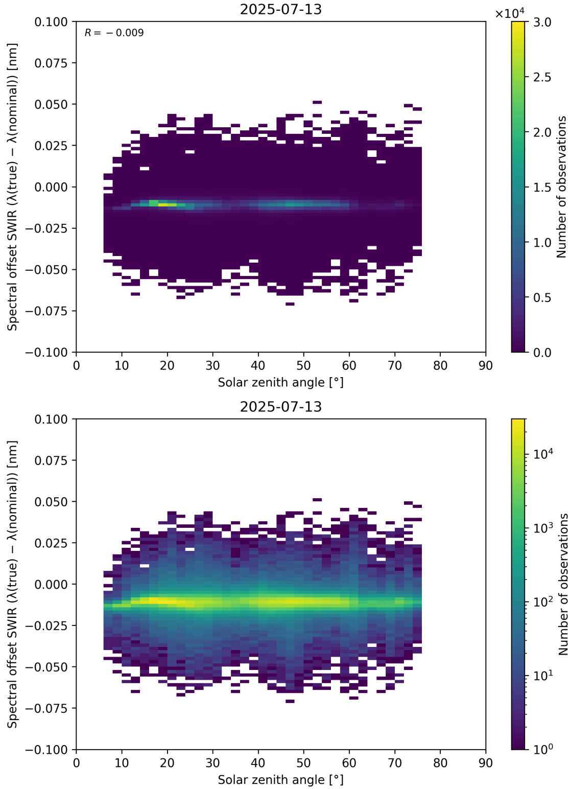
Figure 104: Scatter density plot of “Solar zenith angle” against “Spectral offset SWIR ( \lambda_{\text{true}} - \lambda_{\text{nominal}} )” for 2025-07-13 to 2025-07-14.
