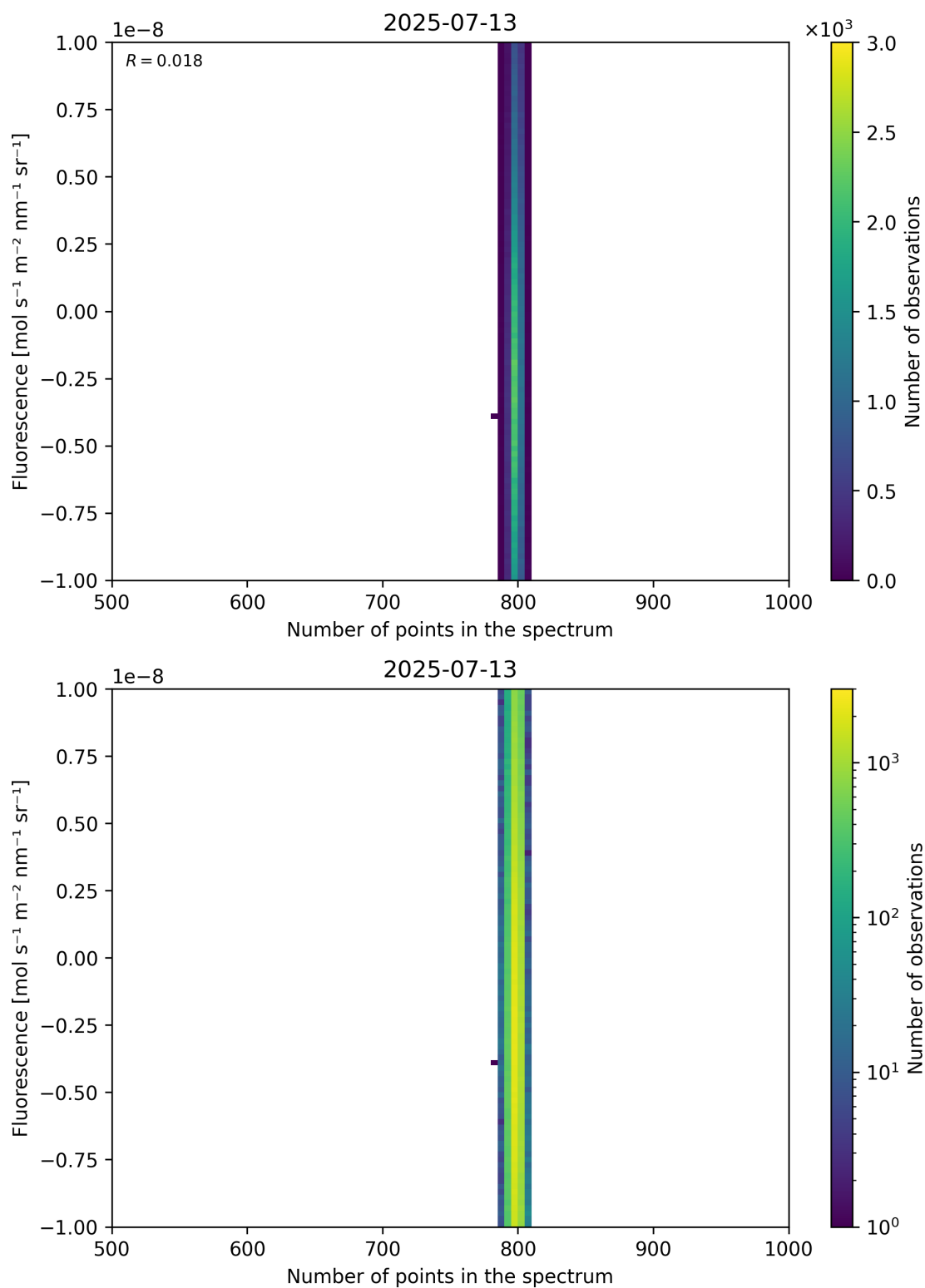
Figure 91: Scatter density plot of “Number of points in the spectrum” against “Fluorescence” for 2025-07-13 to 2025-07-14.
