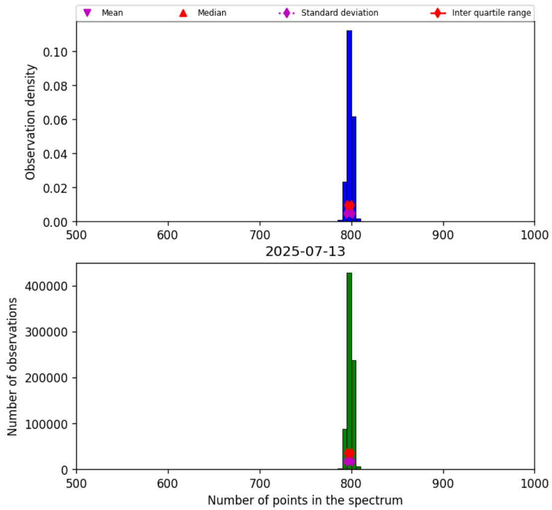
Figure 26: Histogram of “Number of points in the spectrum” for 2025-07-13 to 2025-07-14
