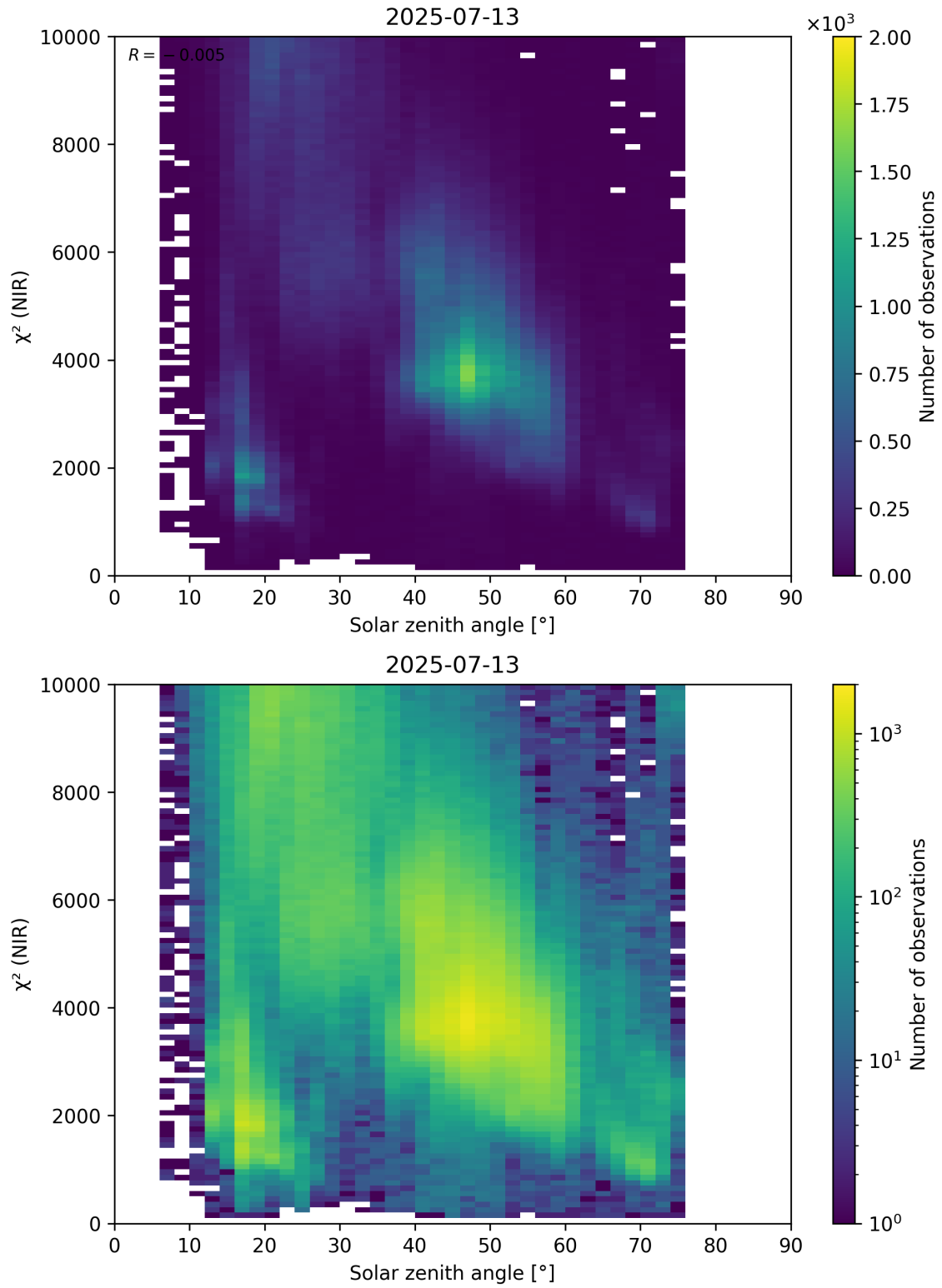
Figure 94: Scatter density plot of “Solar zenith angle” against “ \chi^2 (NIR)” for 2025-07-13 to 2025-07-14.
