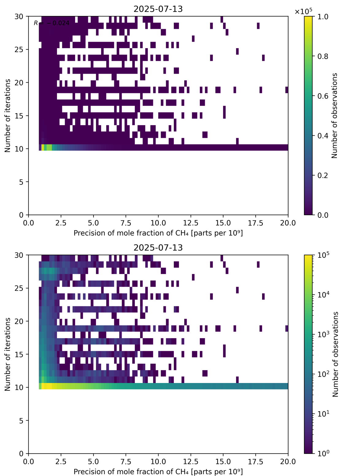
Figure 83: Scatter density plot of “Precision of mole fraction of CH 4 ” against “Number of iterations” for 2025-07-13 to 2025-07-14.
