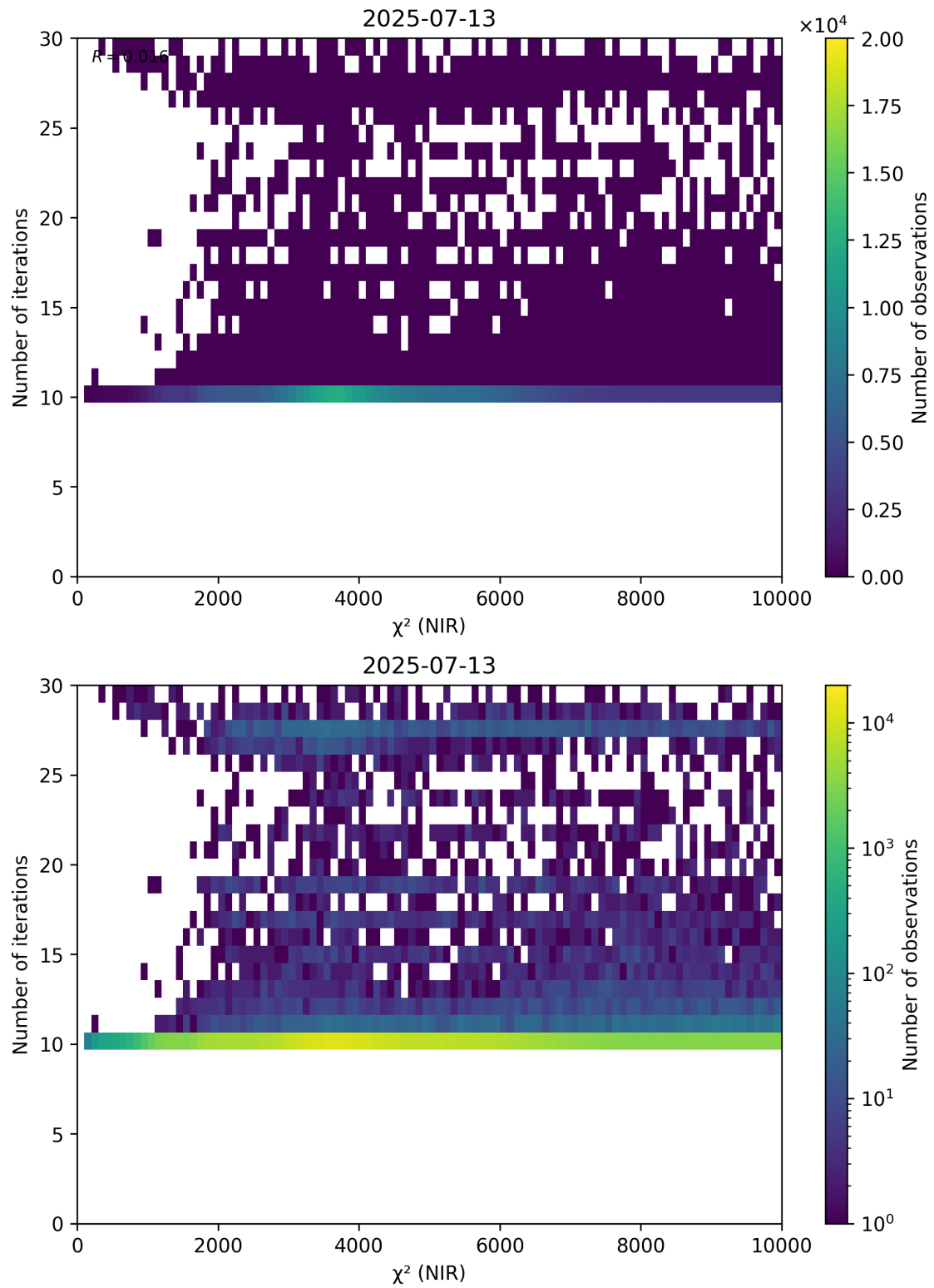
Figure 46: Scatter density plot of “ \chi^2 (NIR)” against “Number of iterations” for 2025-07-13 to 2025-07-14.
