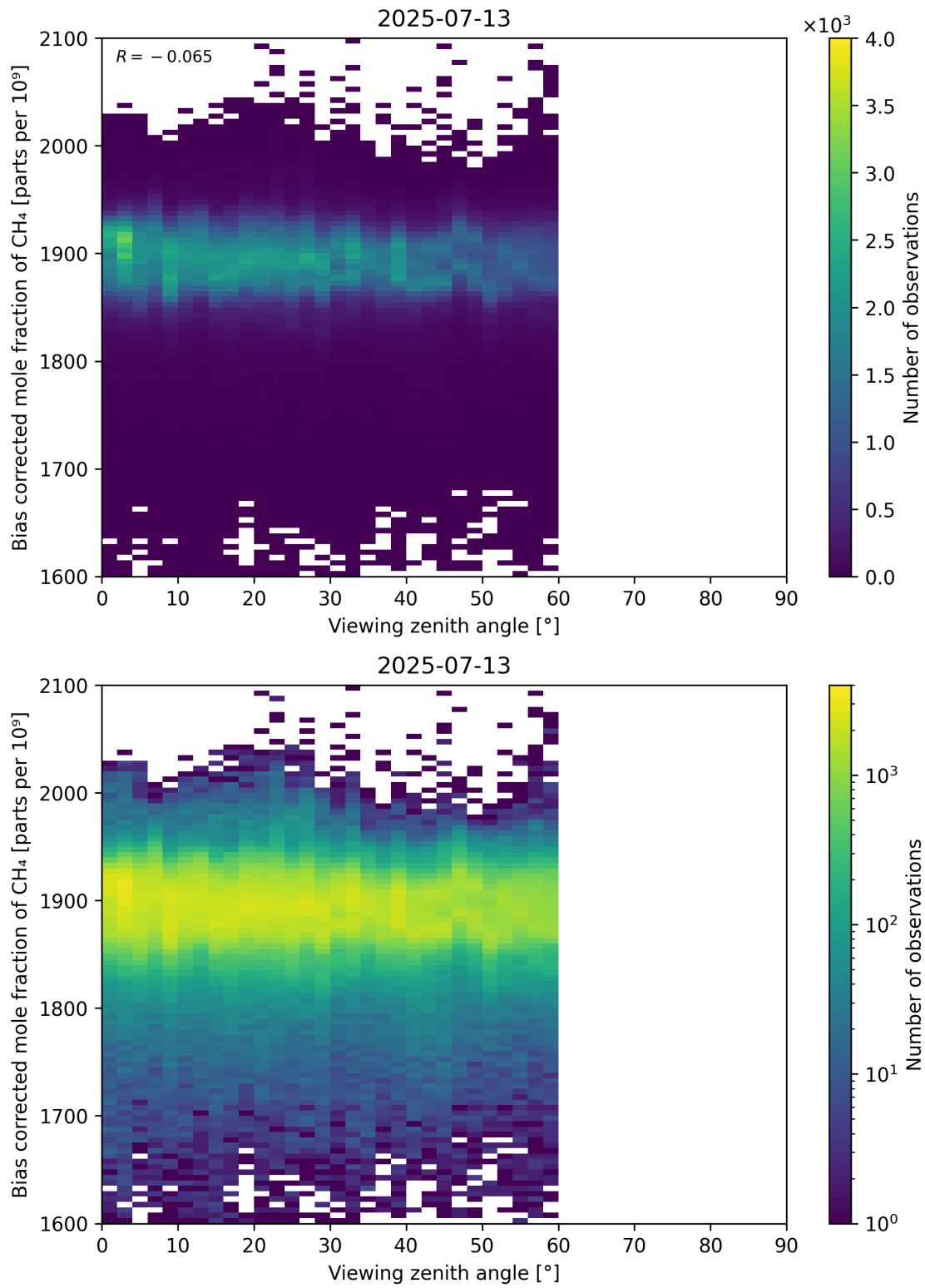
Figure 111: Scatter density plot of “Viewing zenith angle” against “Bias corrected mole fraction of CH 4 ” for 2025-07-13 to 2025-07-14.
