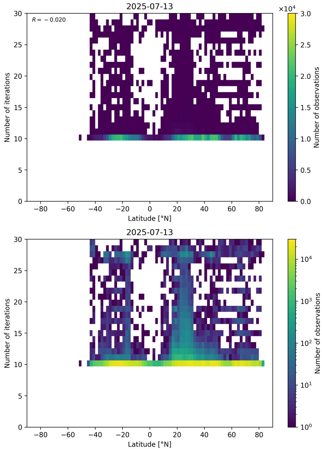
Figure 60: Scatter density plot of “Latitude” against “Number of iterations” for 2025-07-13 to 2025-07-14.
