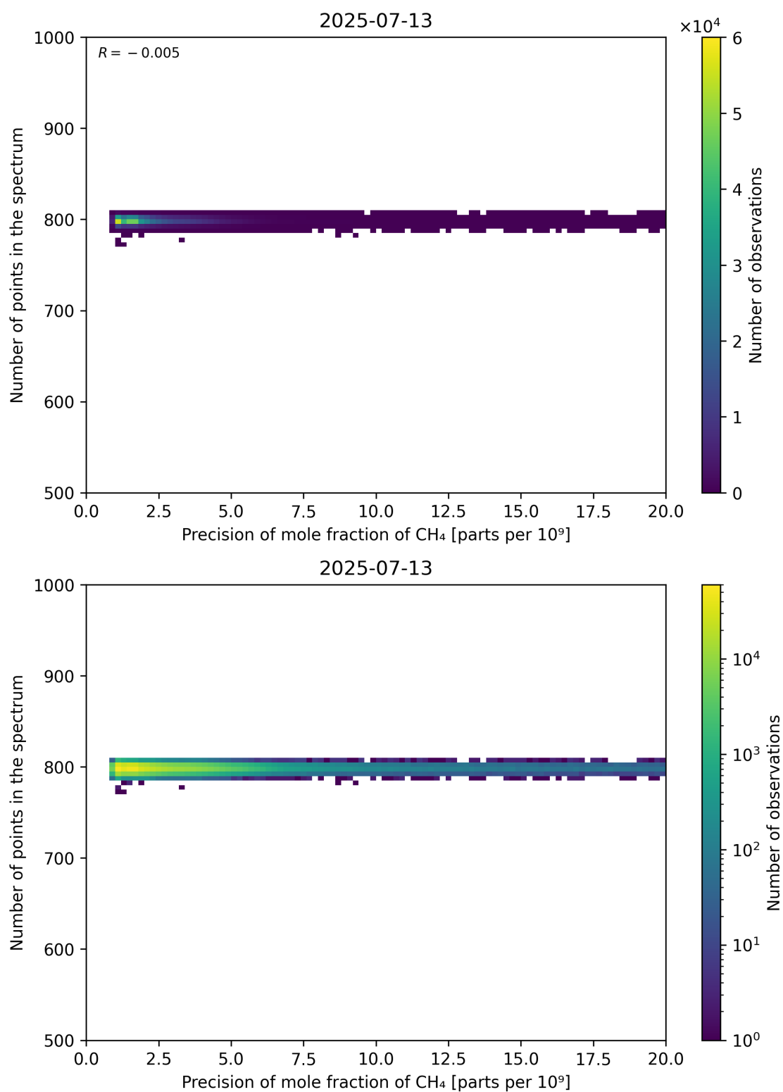
Figure 84: Scatter density plot of “Precision of mole fraction of CH 4 ” against “Number of points in the spectrum” for 2025-07-13 to 2025-07-14.
