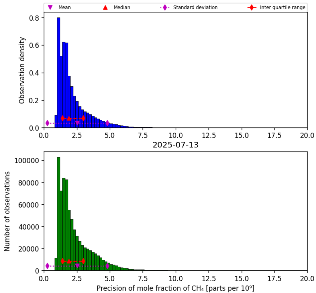
Figure 24: Histogram of “Precision of mole fraction of CH 4 ” for 2025-07-13 to 2025-07-14
