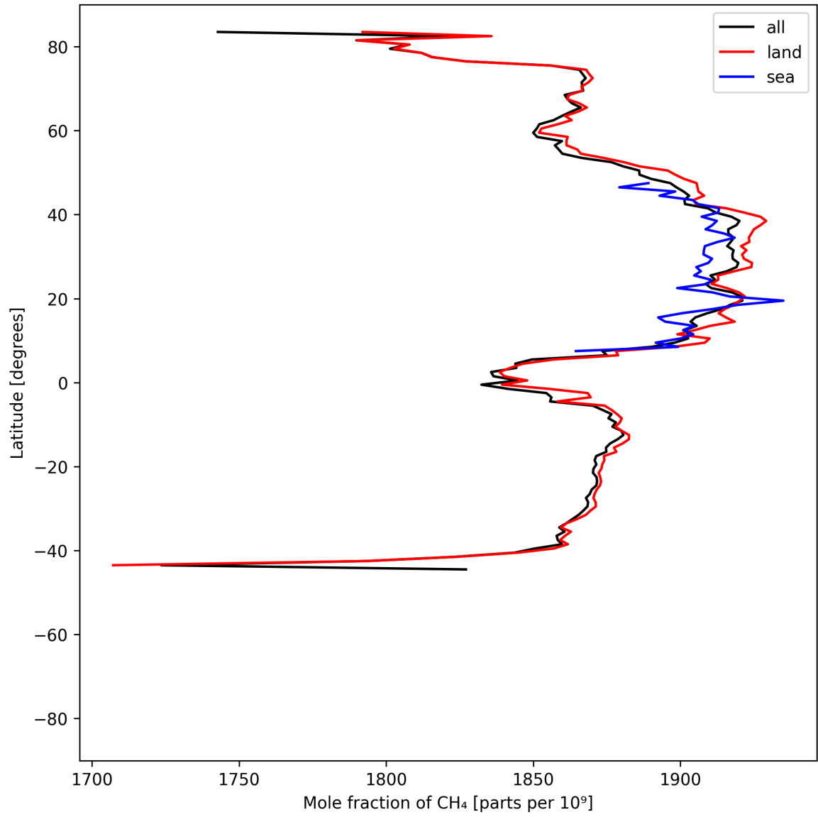
Figure 12: Zonal average of “Mole fraction of \text{CH}_4 ” for 2025-07-13 to 2025-07-14.
