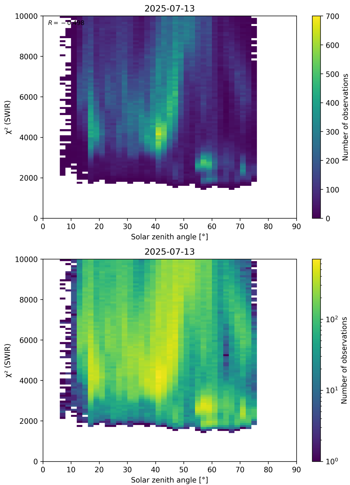
Figure 95: Scatter density plot of “Solar zenith angle” against “ \chi^2 (SWIR)” for 2025-07-13 to 2025-07-14.
