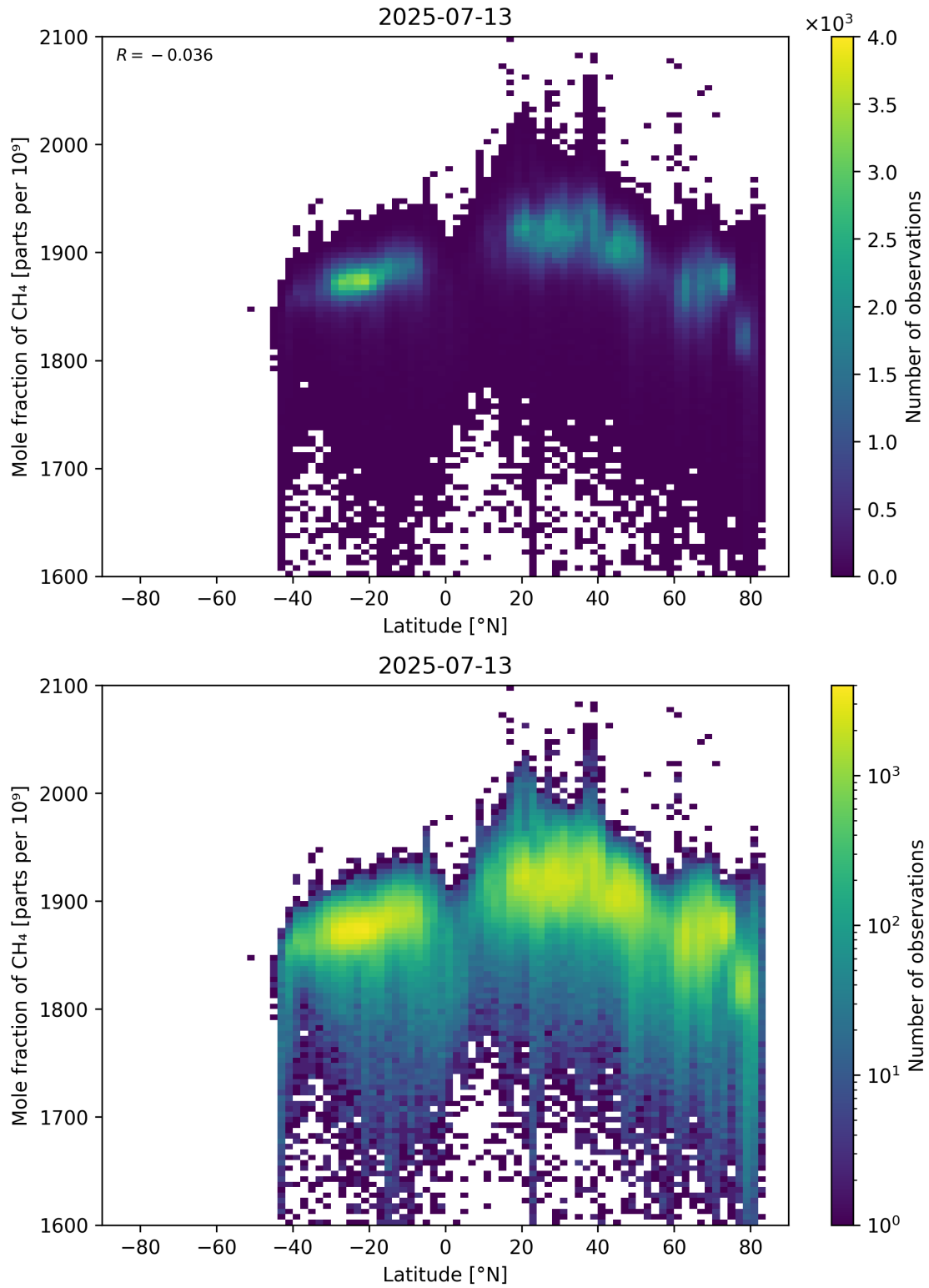
Figure 57: Scatter density plot of “Latitude” against “Mole fraction of CH 4 ” for 2025-07-13 to 2025-07-14.
