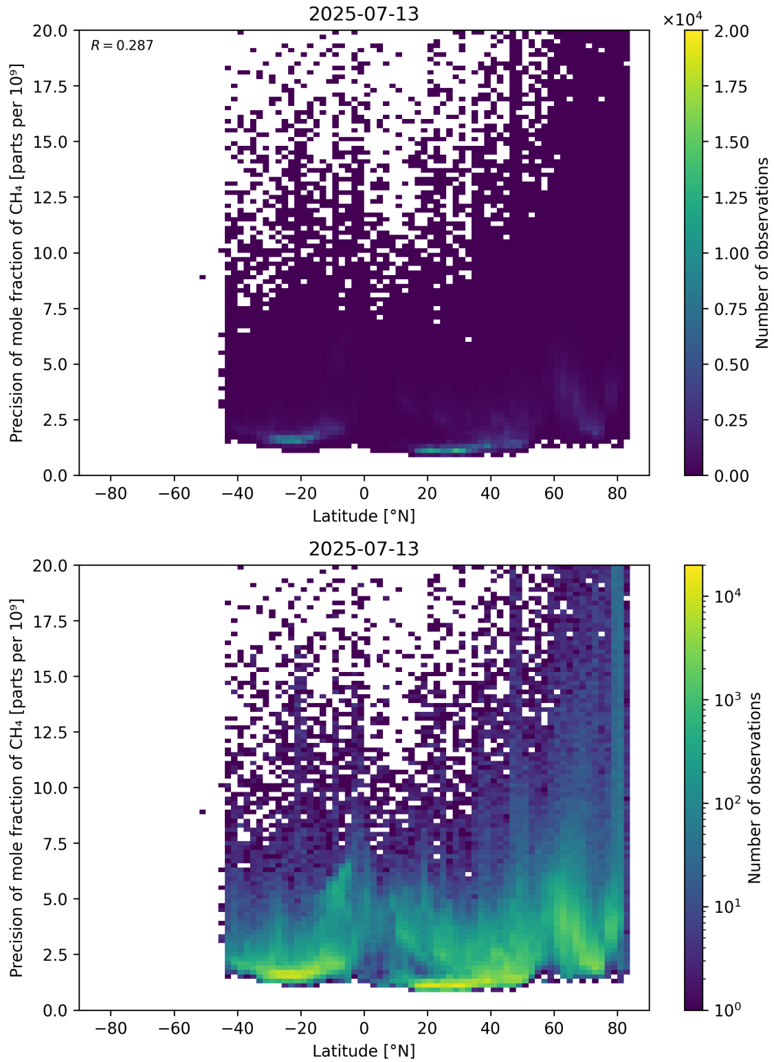
Figure 59: Scatter density plot of “Latitude” against “Precision of mole fraction of \text{CH}_4 ” for 2025-07-13 to 2025-07-14.
