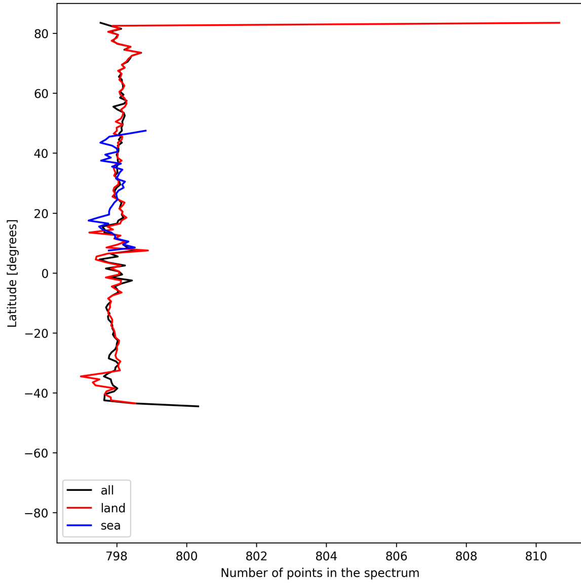
Figure 15: Zonal average of “Number of points in the spectrum” for 2025-07-13 to 2025-07-14.
