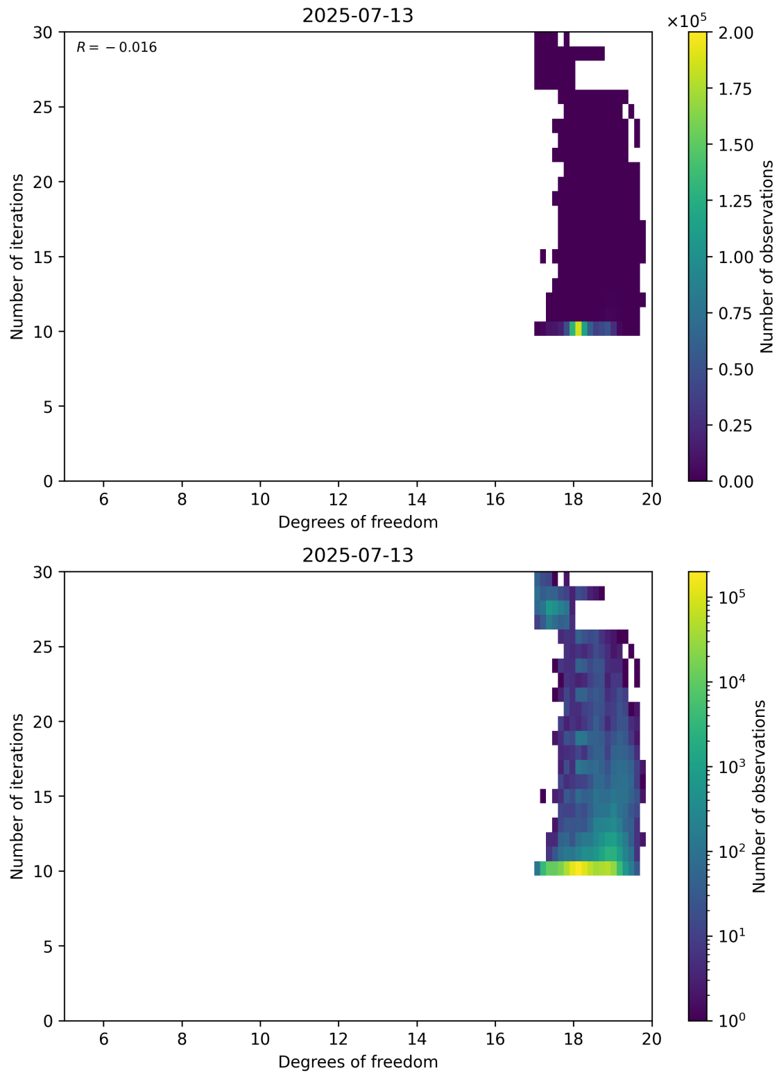
Figure 52: Scatter density plot of “Degrees of freedom” against “Number of iterations” for 2025-07-13 to 2025-07-14.
