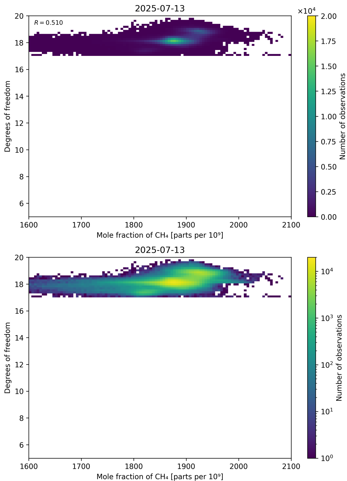
Figure 72: Scatter density plot of “Mole fraction of CH 4 ” against “Degrees of freedom” for 2025-07-13 to 2025-07-14.
