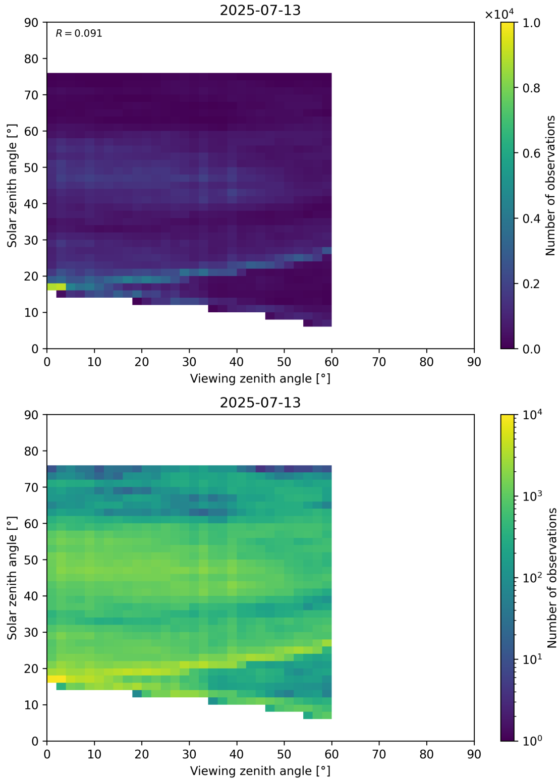
Figure 115: Scatter density plot of “Viewing zenith angle” against “Solar zenith angle” for 2025-07-13 to 2025-07-14.
