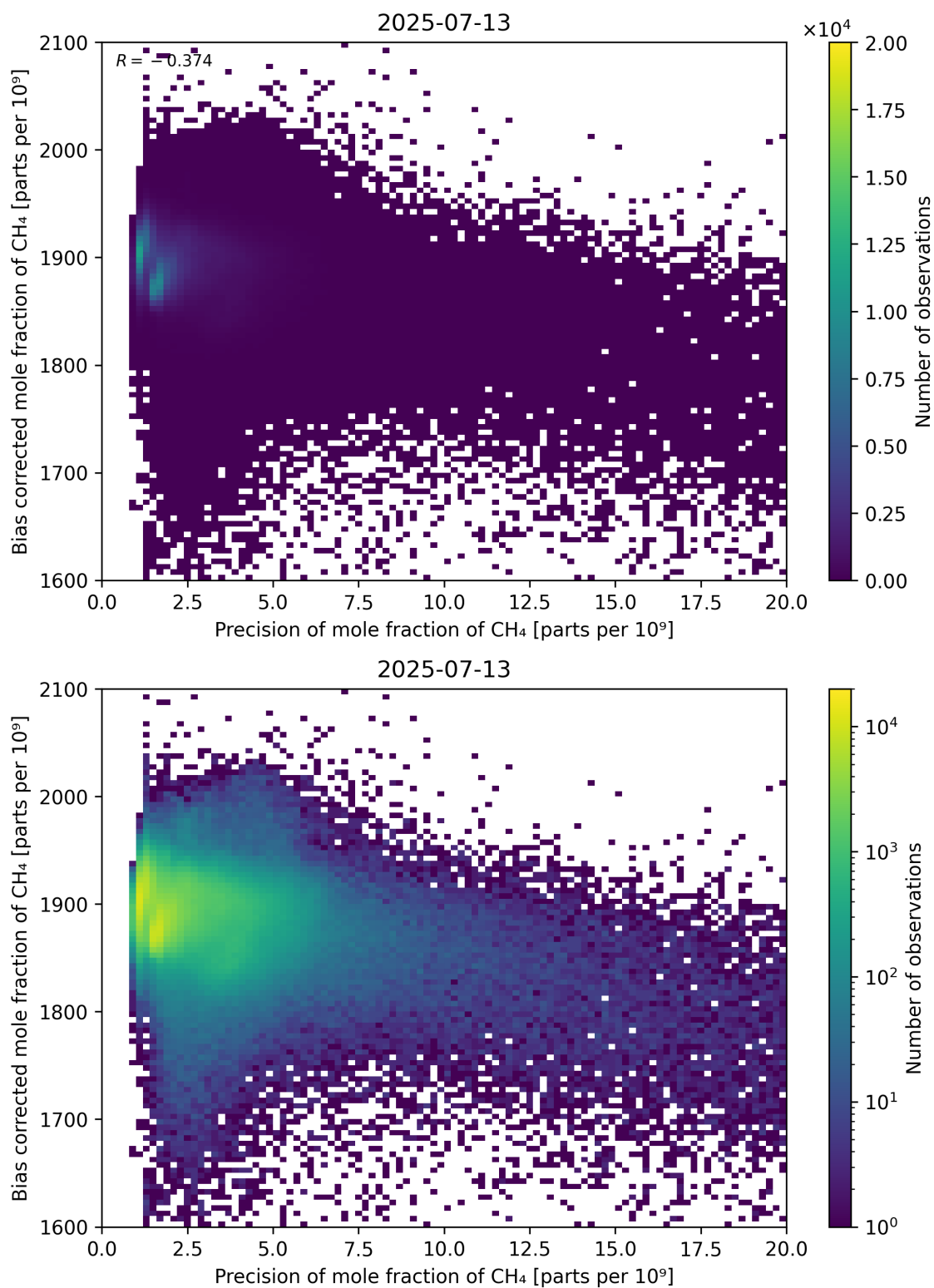
Figure 82: Scatter density plot of “Precision of mole fraction of CH 4 ” against “Bias corrected mole fraction of CH 4 ” for 2025-07-13 to 2025-07-14.
