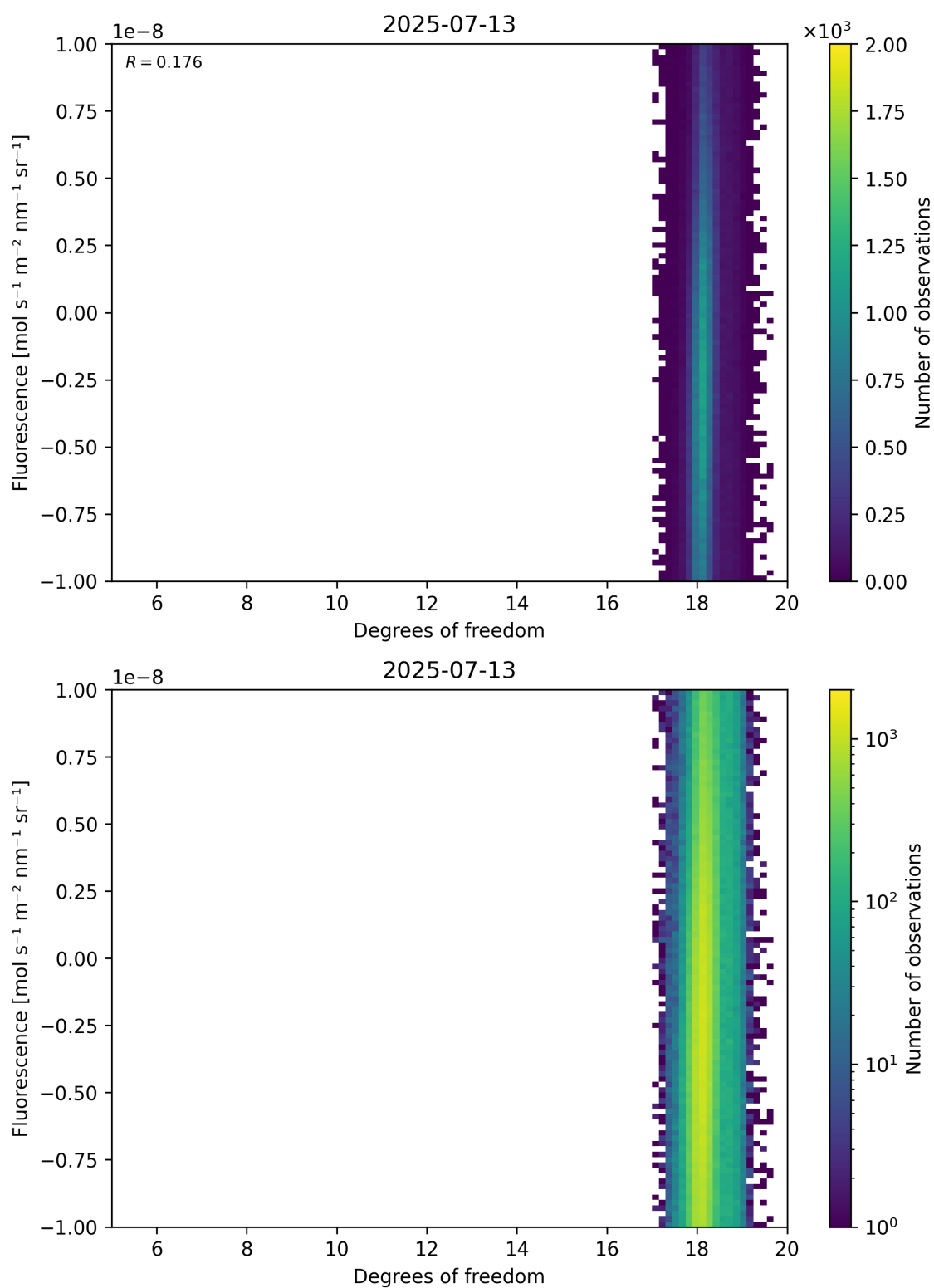
Figure 51: Scatter density plot of “Degrees of freedom” against “Fluorescence” for 2025-07-13 to 2025-07-14.
