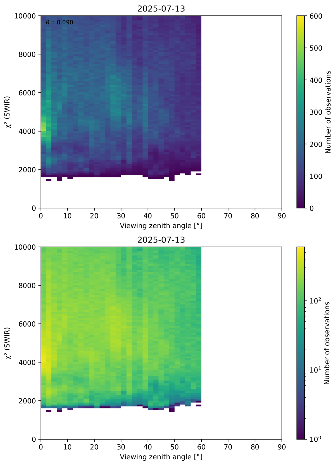
Figure 106: Scatter density plot of “Viewing zenith angle” against “ \chi^2 (SWIR)” for 2025-07-13 to 2025-07-14.
