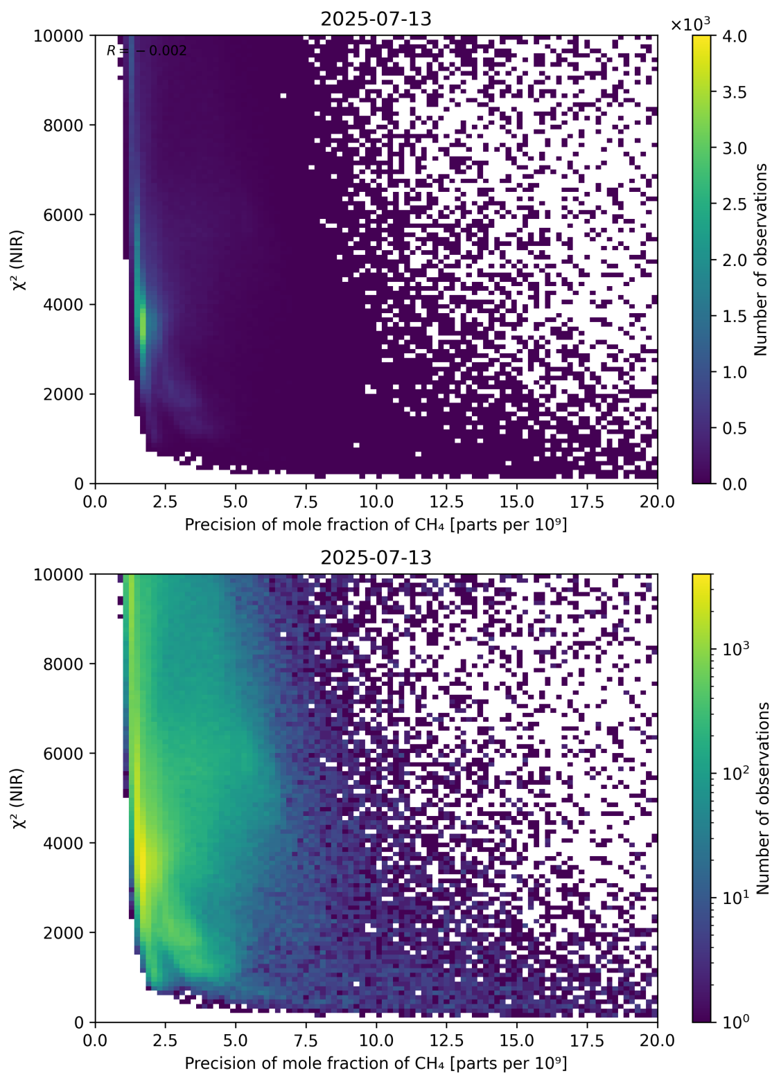
Figure 78: Scatter density plot of “Precision of mole fraction of \text{CH}_4 ” against “ \chi^2 (NIR)” for 2025-07-13 to 2025-07-14.
