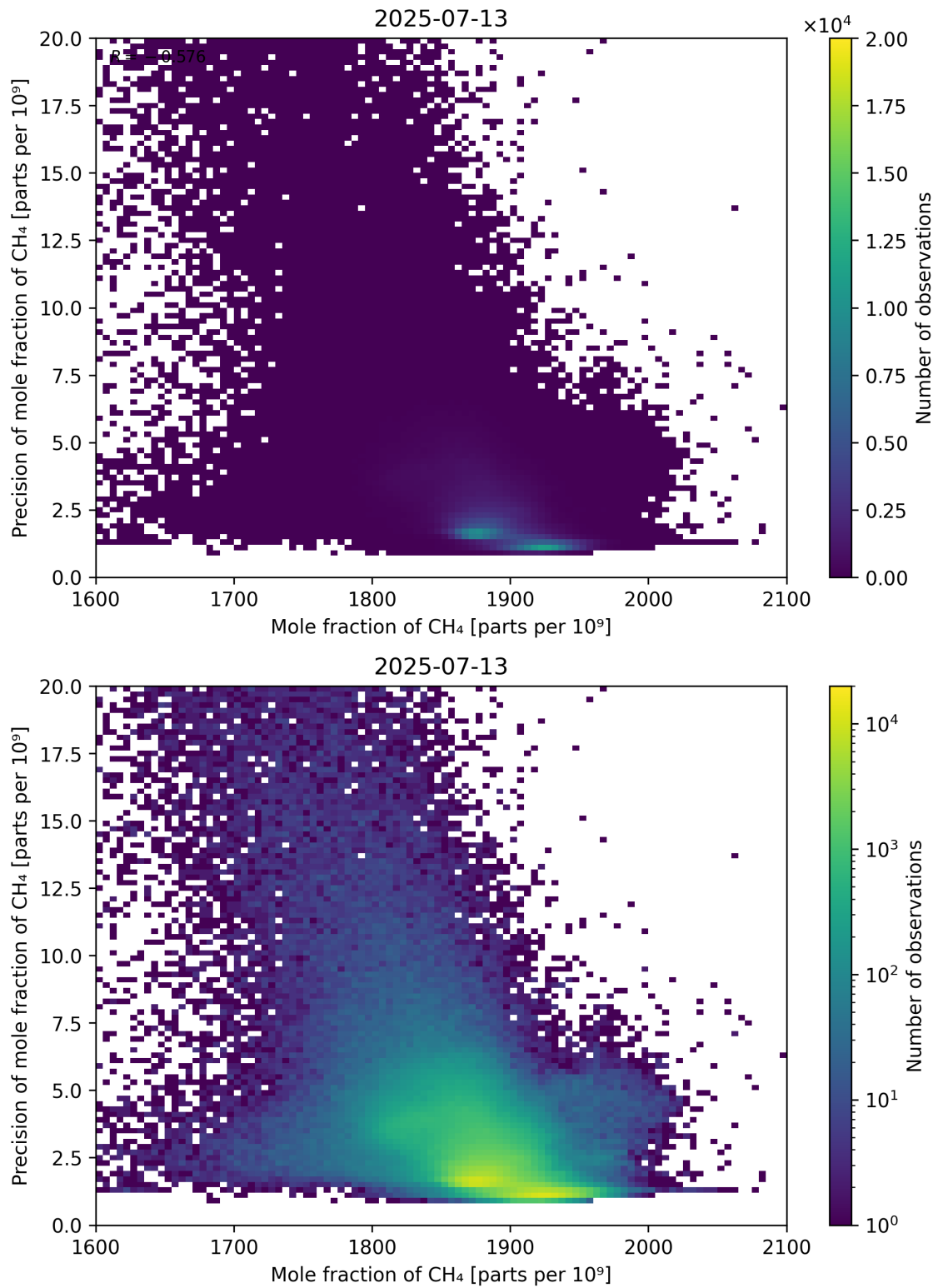
Figure 75: Scatter density plot of “Mole fraction of CH 4 ” against “Precision of mole fraction of CH 4 ” for 2025-07-13 to 2025-07-14.
