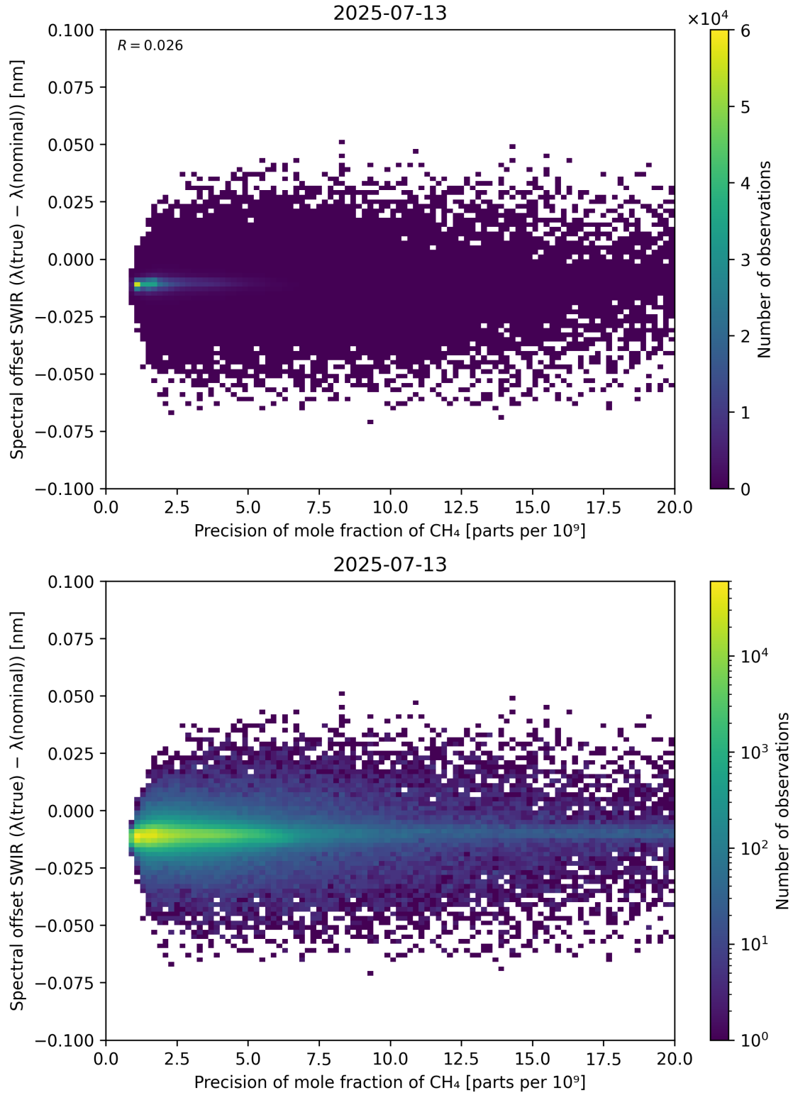
Figure 85: Scatter density plot of “Precision of mole fraction of CH 4 ” against “Spectral offset SWIR ( \lambda_{\text{true}} - \lambda_{\text{nominal}} )” for 2025-07-13 to 2025-07-14.
