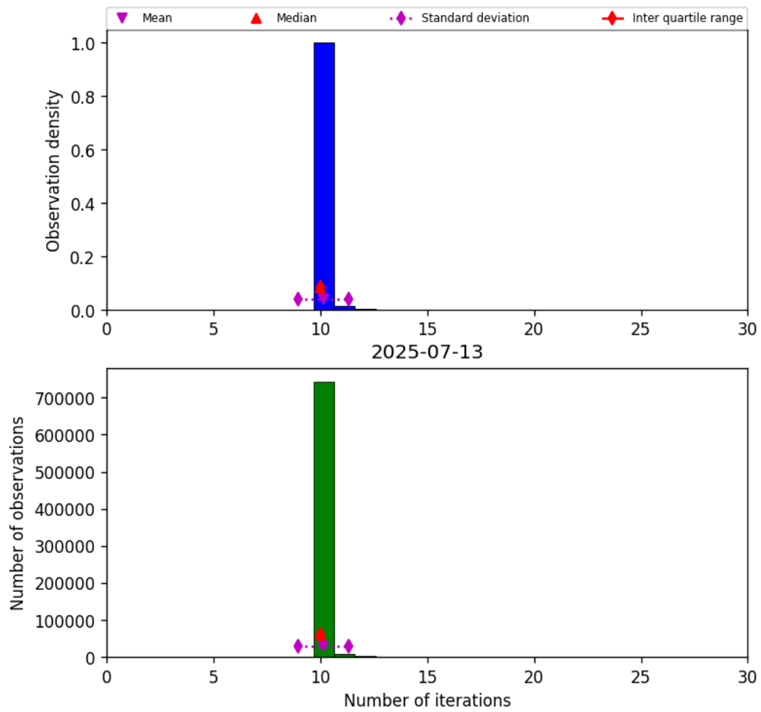
Figure 31: Histogram of “Number of iterations” for 2025-07-13 to 2025-07-14
