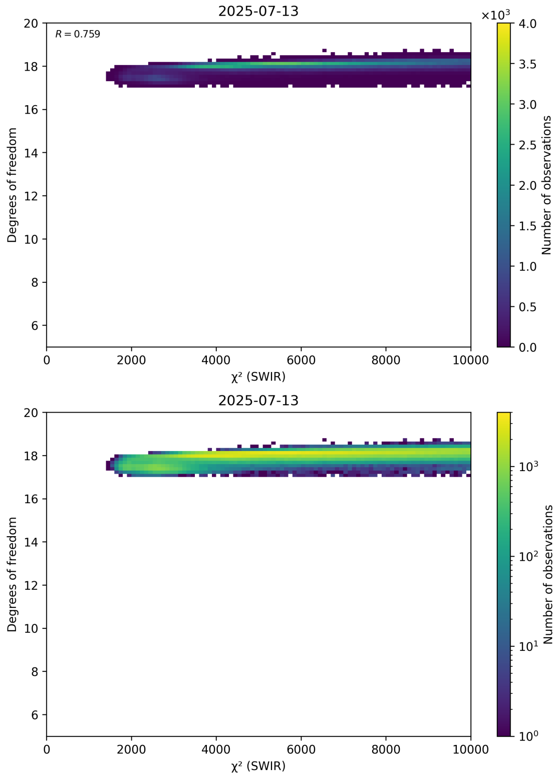
Figure 48: Scatter density plot of “ \chi^2 (SWIR)” against “Degrees of freedom” for 2025-07-13 to 2025-07-14.
