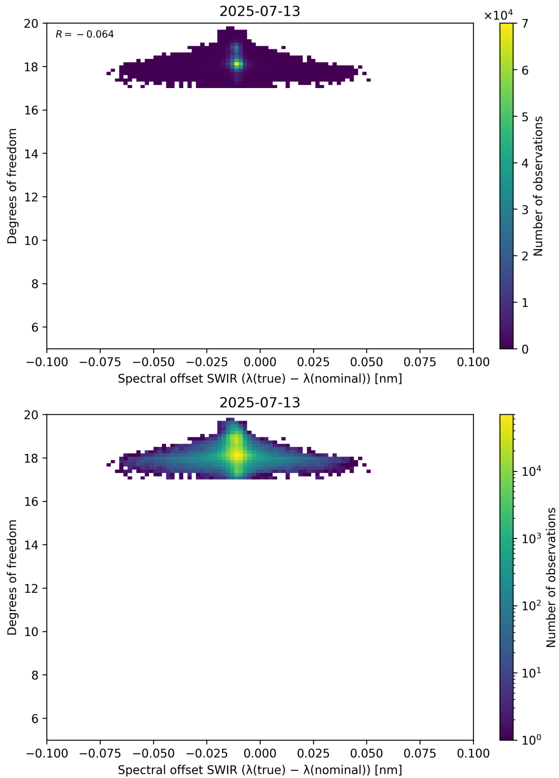
Figure 119: Scatter density plot of “Spectral offset SWIR ( \lambda_{\text{true}} - \lambda_{\text{nominal}} )” against “Degrees of freedom” for 2025-07-13 to 2025-07-14.
