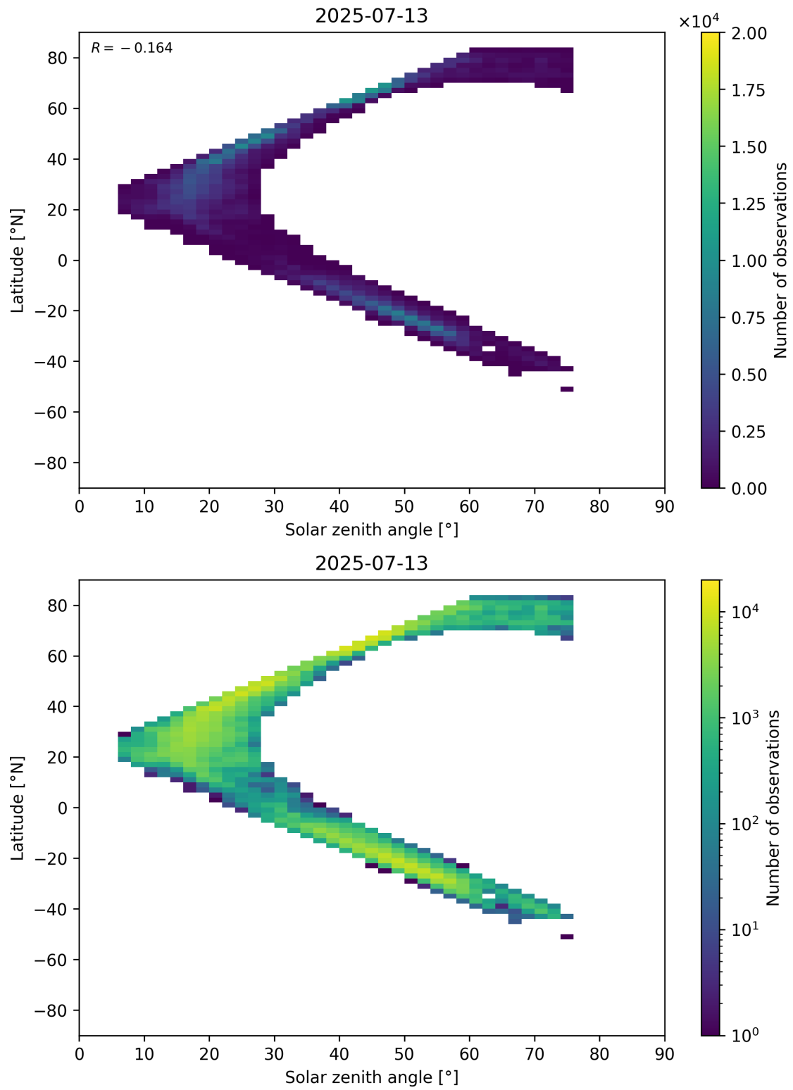
Figure 98: Scatter density plot of “Solar zenith angle” against “Latitude” for 2025-07-13 to 2025-07-14.
