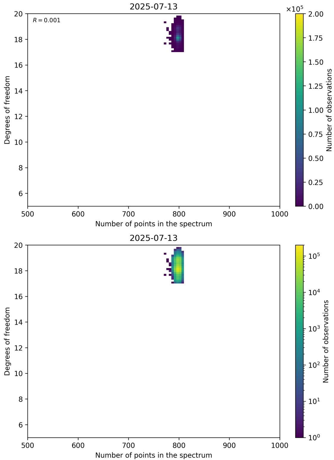
Figure 90: Scatter density plot of “Number of points in the spectrum” against “Degrees of freedom” for 2025-07-13 to 2025-07-14.
