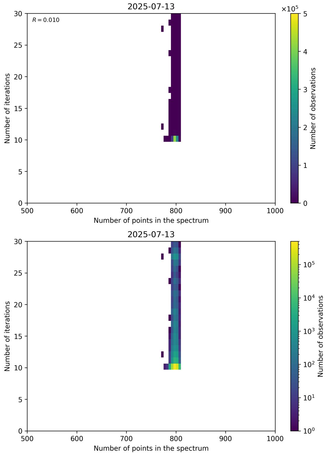
Figure 92: Scatter density plot of “Number of points in the spectrum” against “Number of iterations” for 2025-07-13 to 2025-07-14.
