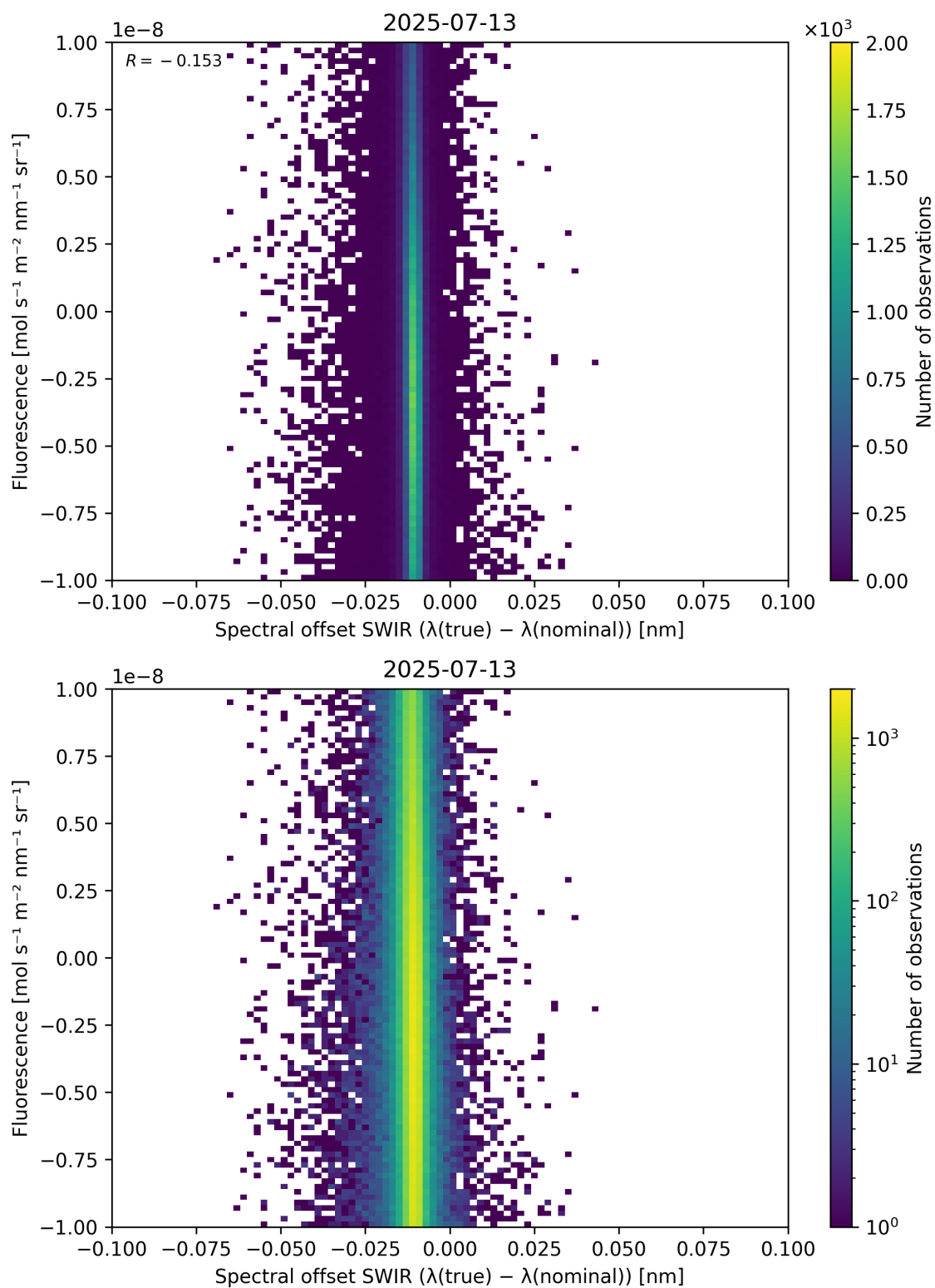
Figure 120: Scatter density plot of “Spectral offset SWIR ( \lambda_{\text{true}} - \lambda_{\text{nominal}} )” against “Fluorescence” for 2025-07-13 to 2025-07-14.
