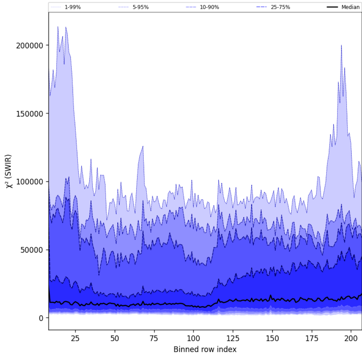
Figure 39: Along track statistics of " \chi^2 (SWIR)" for 2025-07-13 to 2025-07-14
