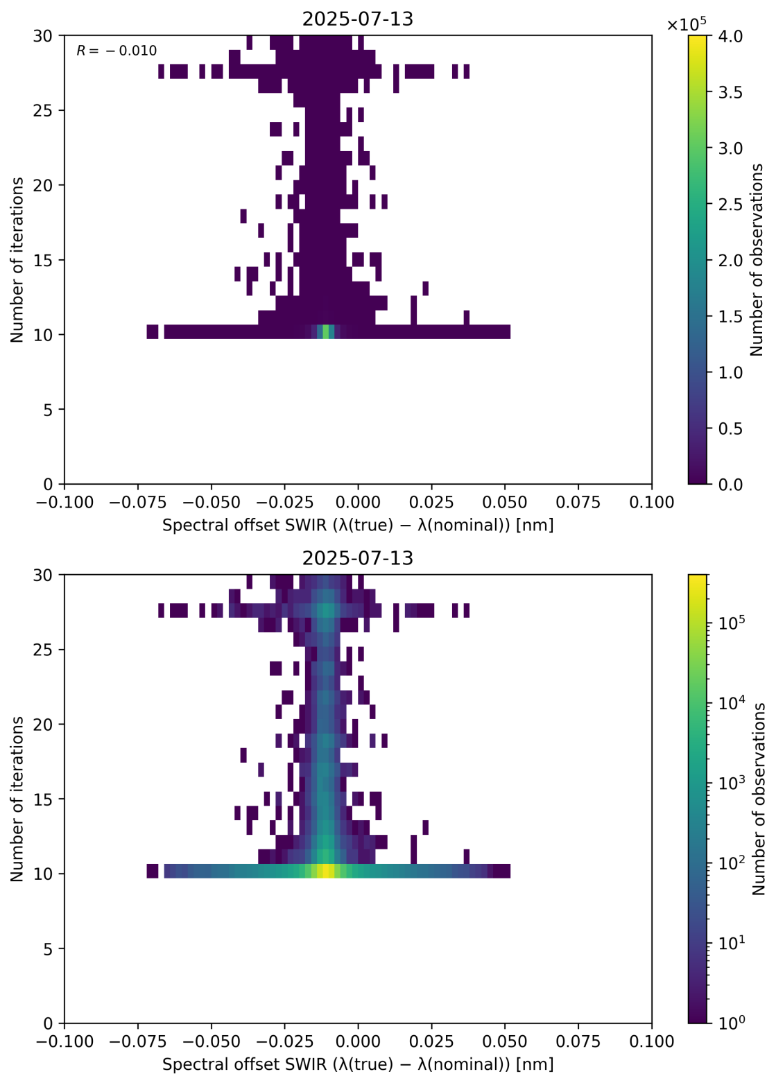
Figure 121: Scatter density plot of “Spectral offset SWIR ( \lambda_{\text{true}} - \lambda_{\text{nominal}} )” against “Number of iterations” for 2025-07-13 to 2025-07-14.
