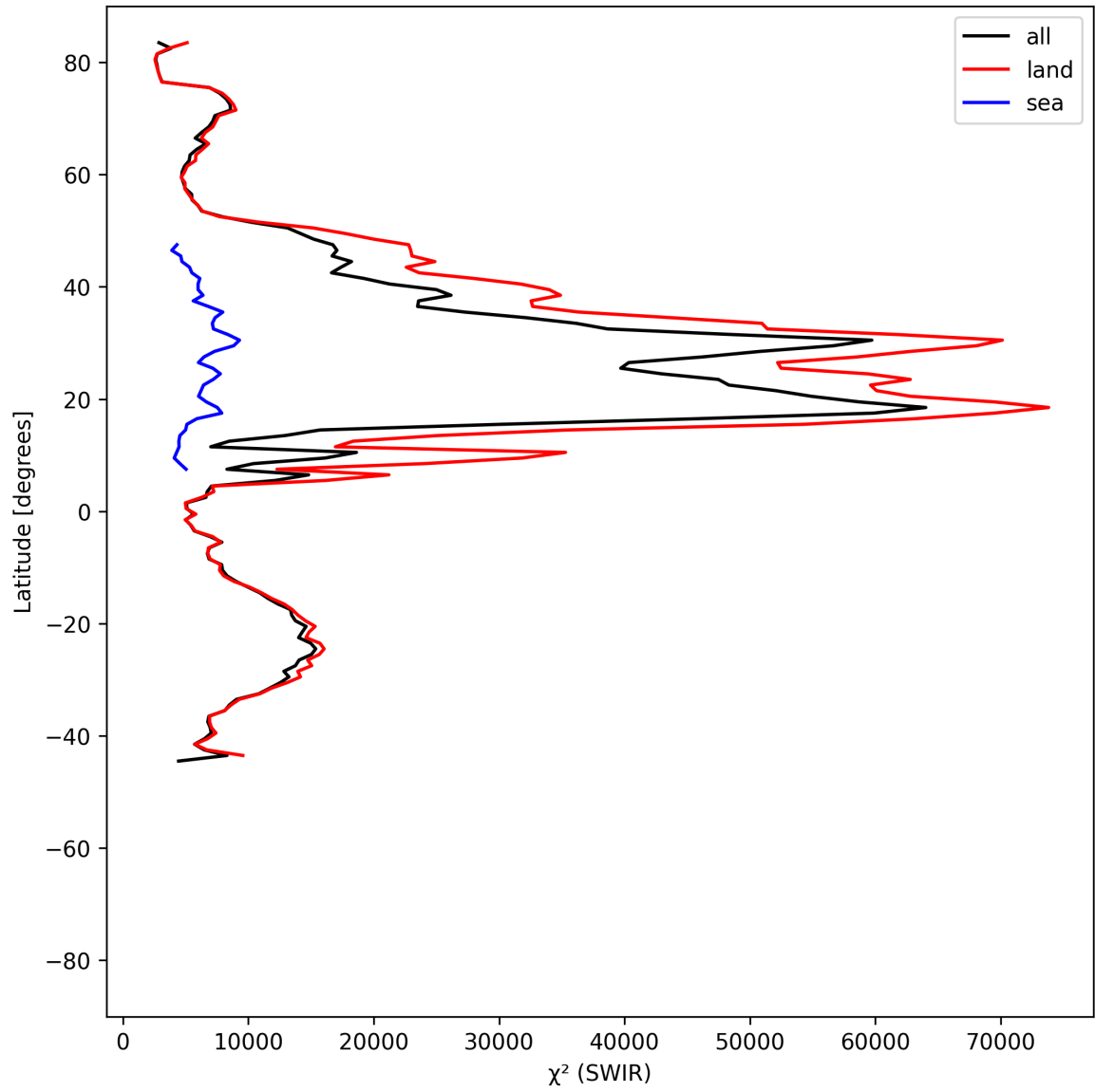
Figure 17: Zonal average of “ \chi^2 (SWIR)” for 2025-07-13 to 2025-07-14.
