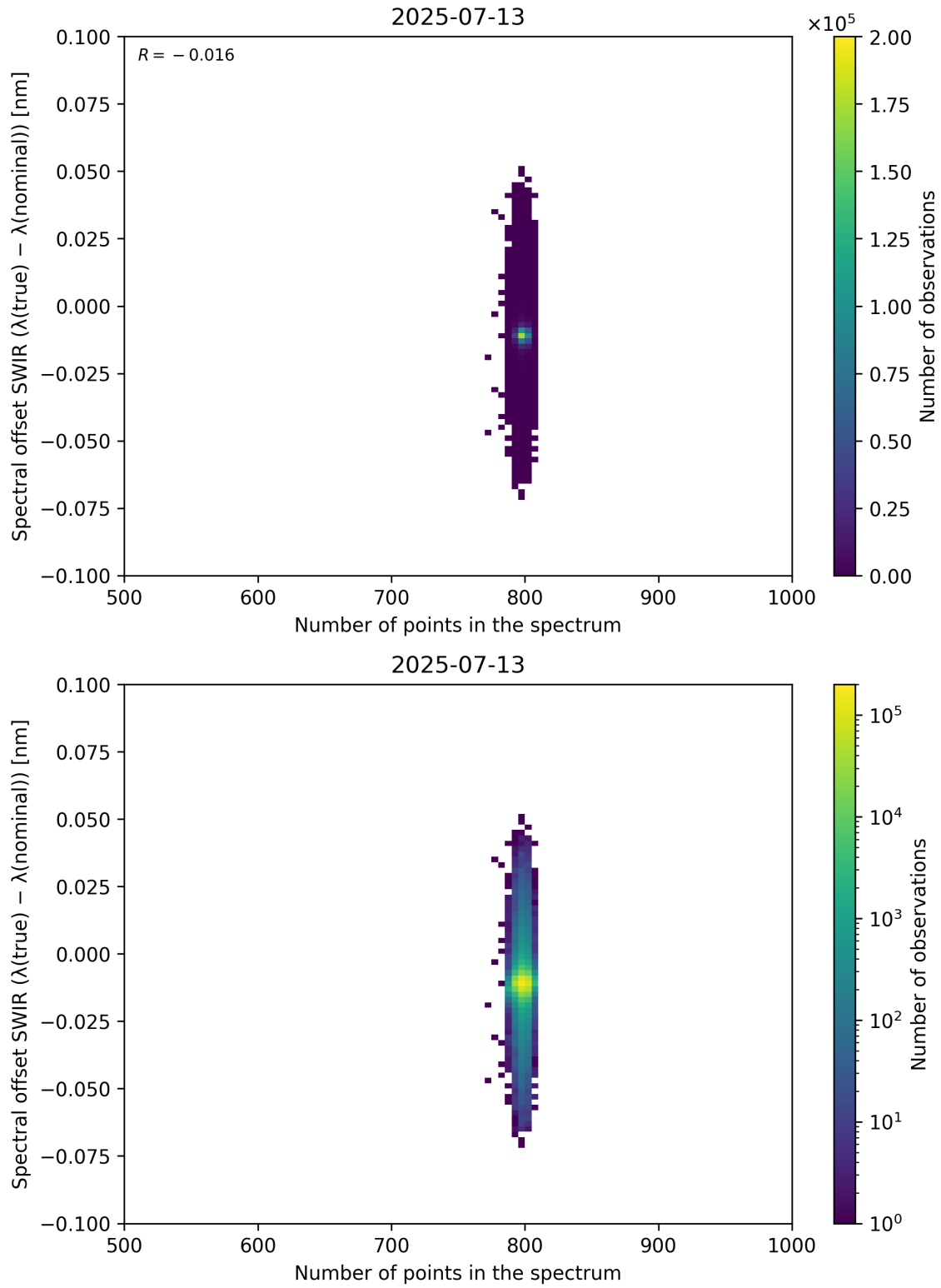
Figure 93: Scatter density plot of “Number of points in the spectrum” against “Spectral offset SWIR ( \lambda_{\text{true}} - \lambda_{\text{nominal}} )” for 2025-07-13 to 2025-07-14.
