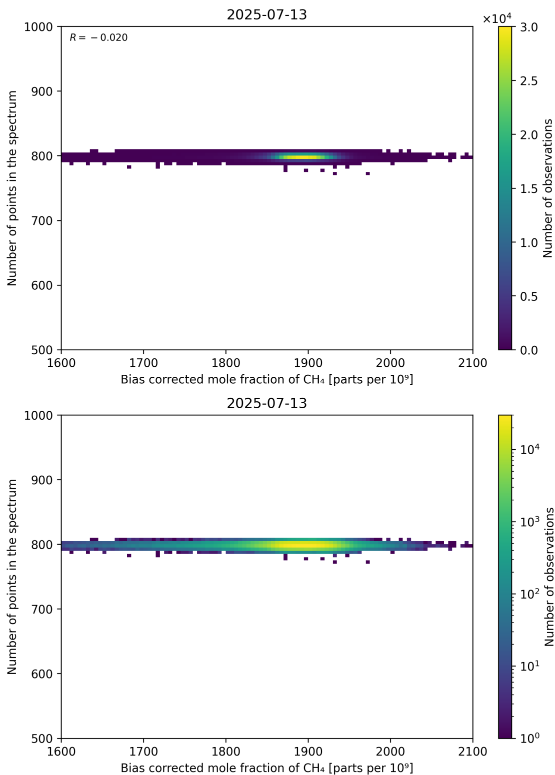
Figure 68: Scatter density plot of “Bias corrected mole fraction of CH 4 ” against “Number of points in the spectrum” for 2025-07-13 to 2025-07-14.
