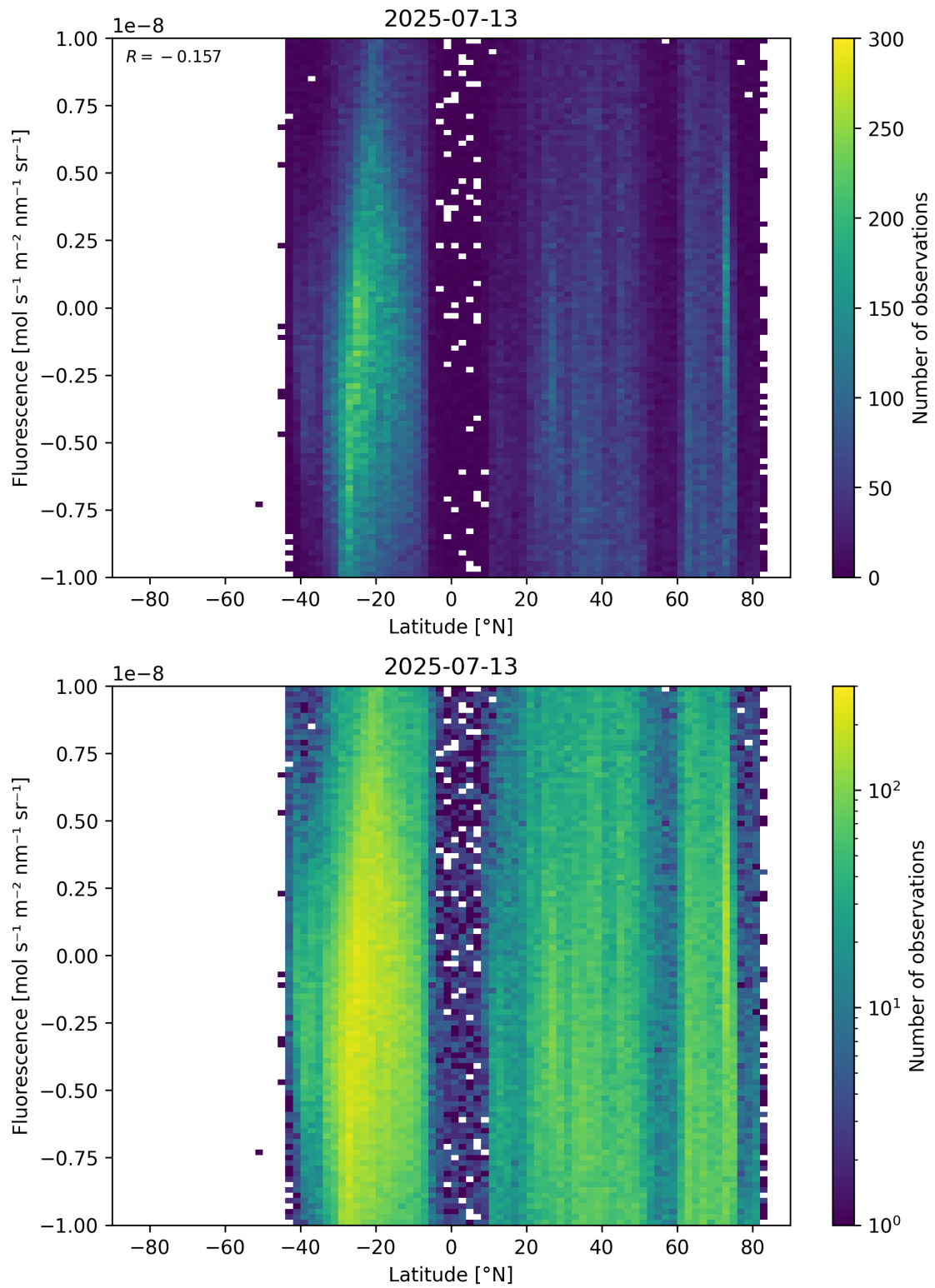
Figure 56: Scatter density plot of “Latitude” against “Fluorescence” for 2025-07-13 to 2025-07-14.
