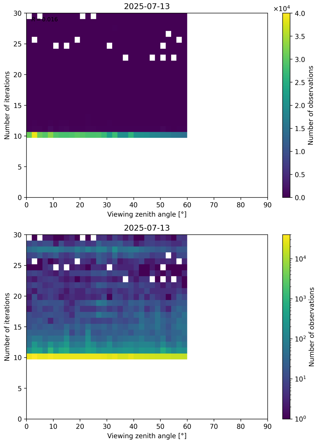
Figure 113: Scatter density plot of “Viewing zenith angle” against “Number of iterations” for 2025-07-13 to 2025-07-14.
