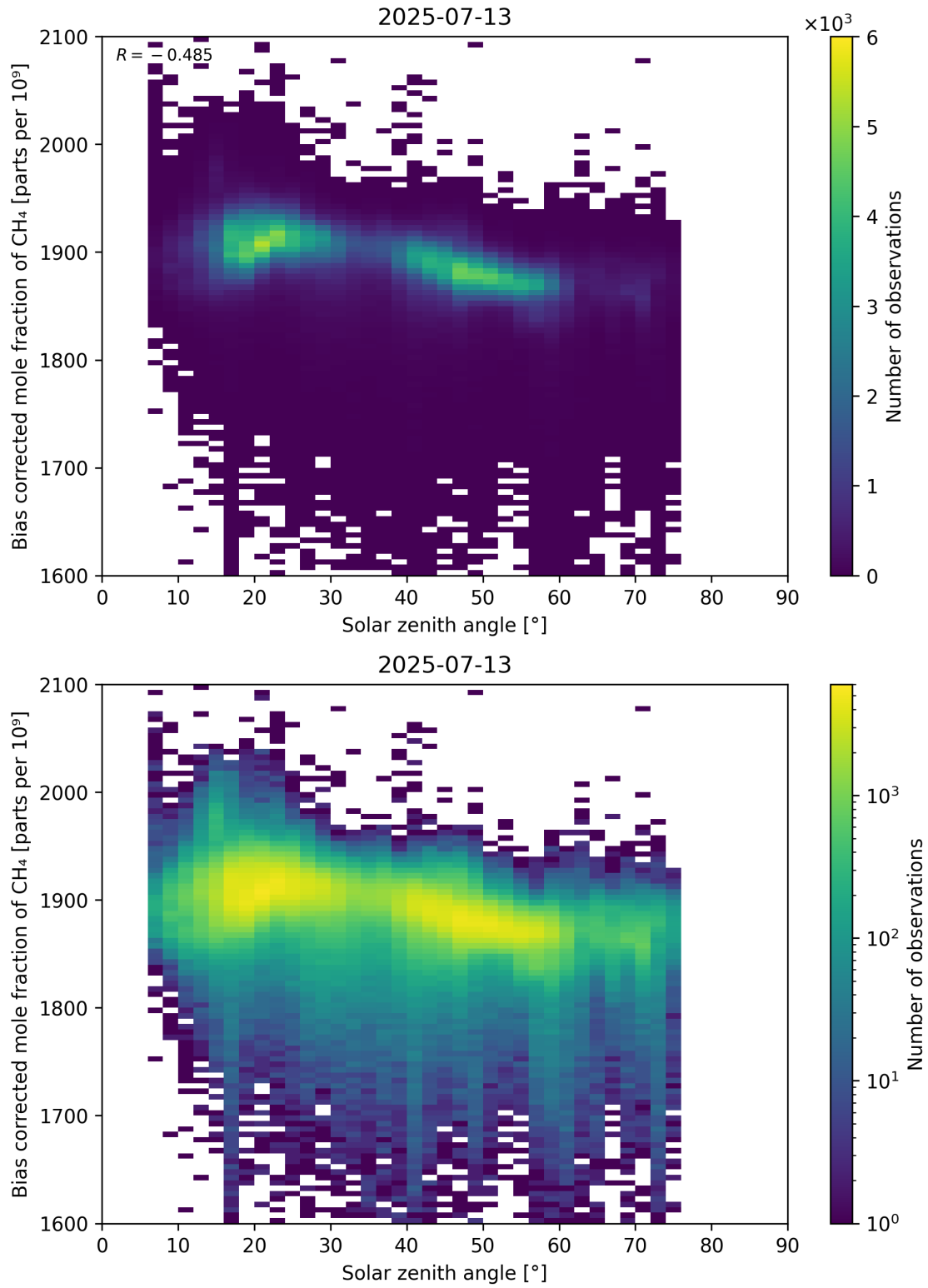
Figure 100: Scatter density plot of “Solar zenith angle” against “Bias corrected mole fraction of CH 4 ” for 2025-07-13 to 2025-07-14.
