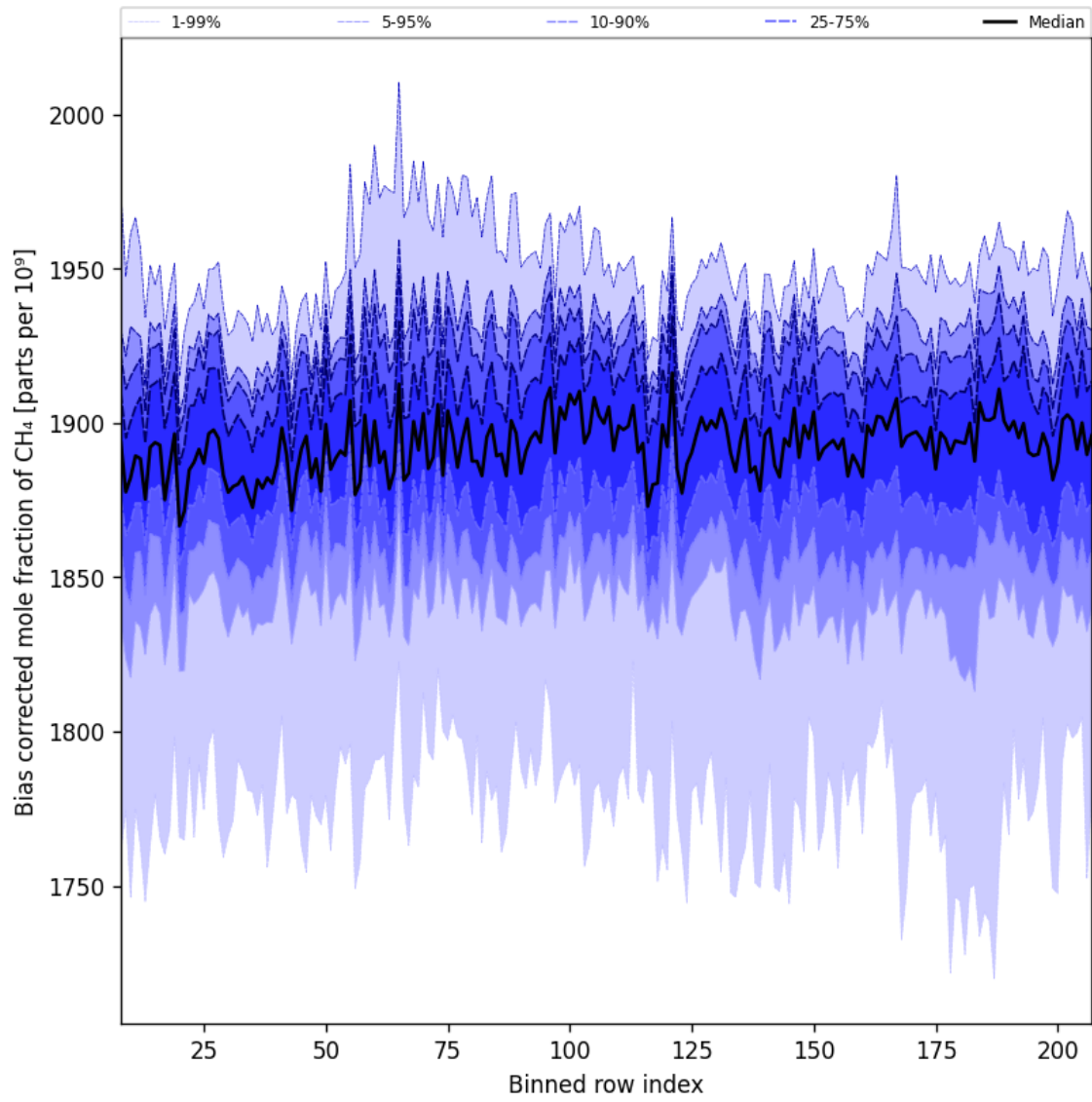
Figure 36: Along track statistics of “Bias corrected mole fraction of CH 4 ” for 2025-07-13 to 2025-07-14
