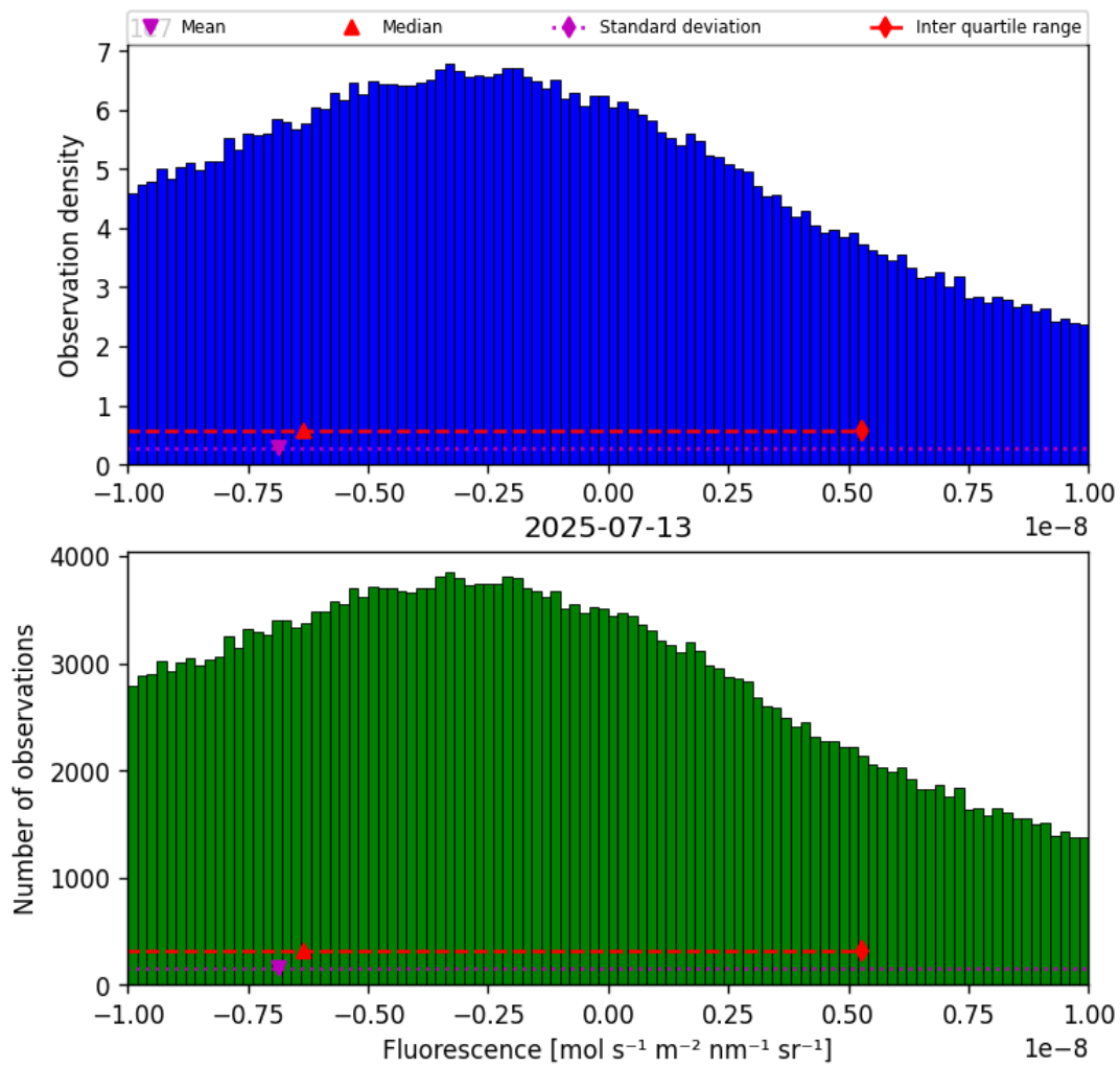
Figure 32: Histogram of “Fluorescence” for 2025-07-13 to 2025-07-14
