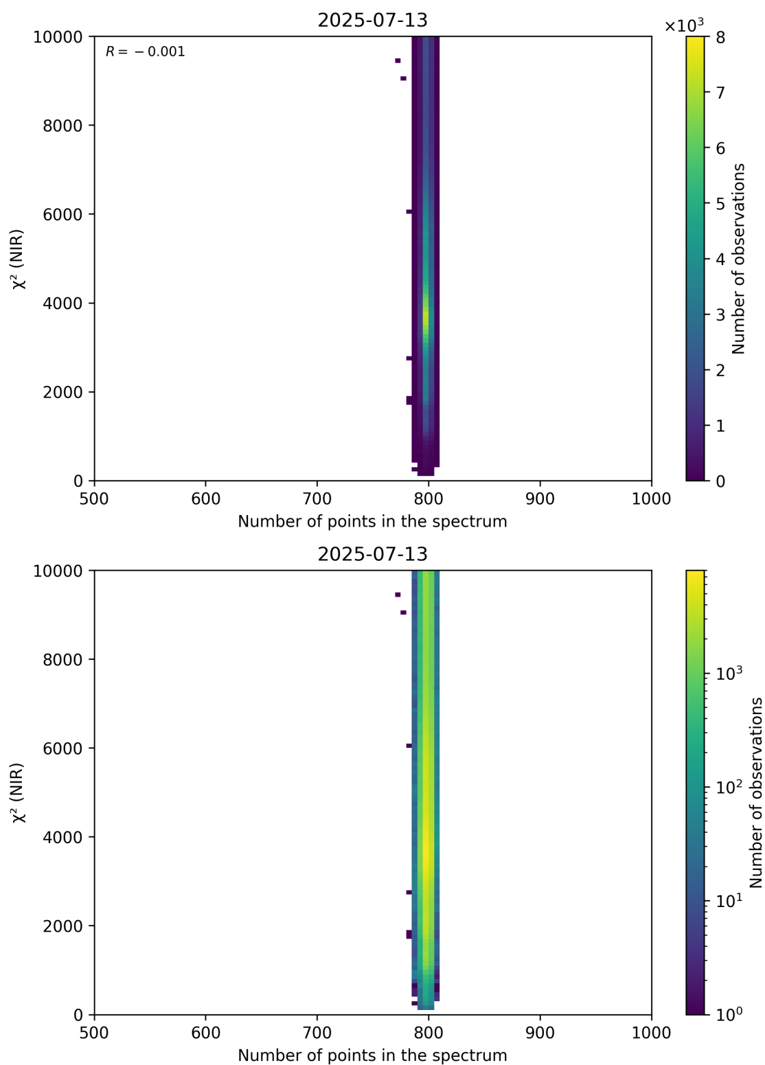
Figure 88: Scatter density plot of “Number of points in the spectrum” against “ \chi^2 (NIR)” for 2025-07-13 to 2025-07-14.
