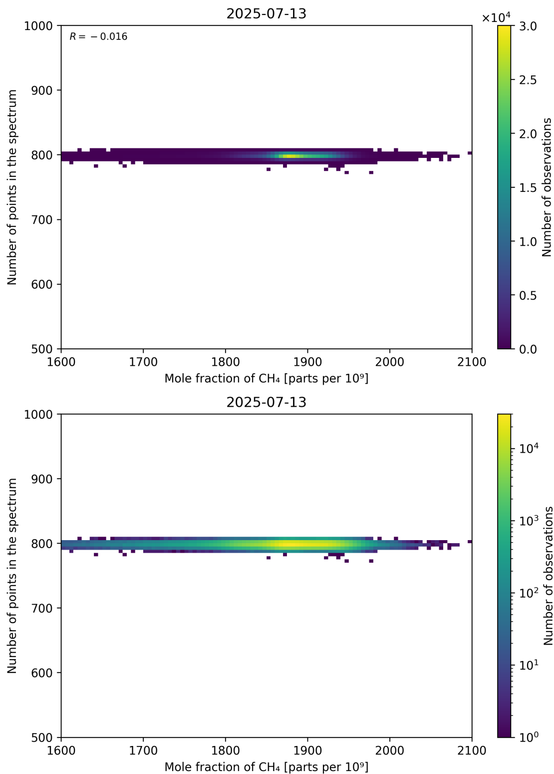
Figure 77: Scatter density plot of “Mole fraction of CH 4 ” against “Number of points in the spectrum” for 2025-07-13 to 2025-07-14.
