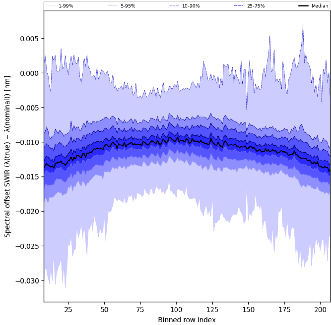
Figure 38: Along track statistics of “Spectral offset SWIR ( \lambda_{\text{true}} - \lambda_{\text{nominal}} )” for 2025-07-13 to 2025-07-14
