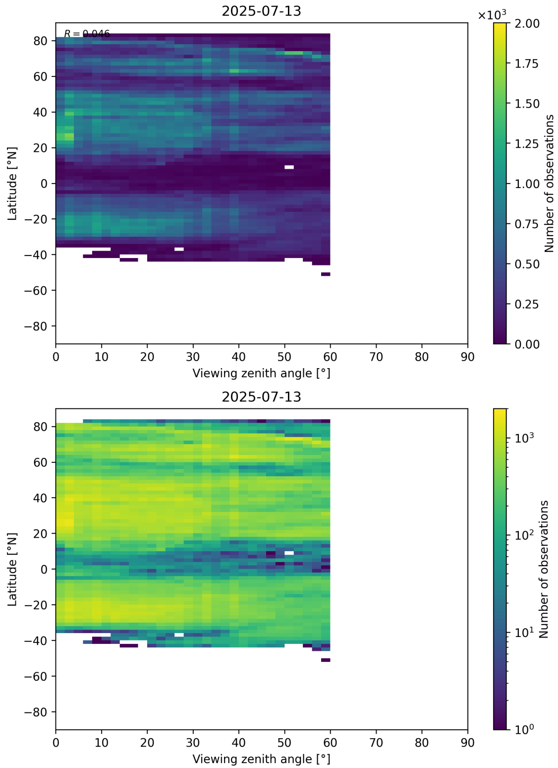
Figure 109: Scatter density plot of “Viewing zenith angle” against “Latitude” for 2025-07-13 to 2025-07-14.
