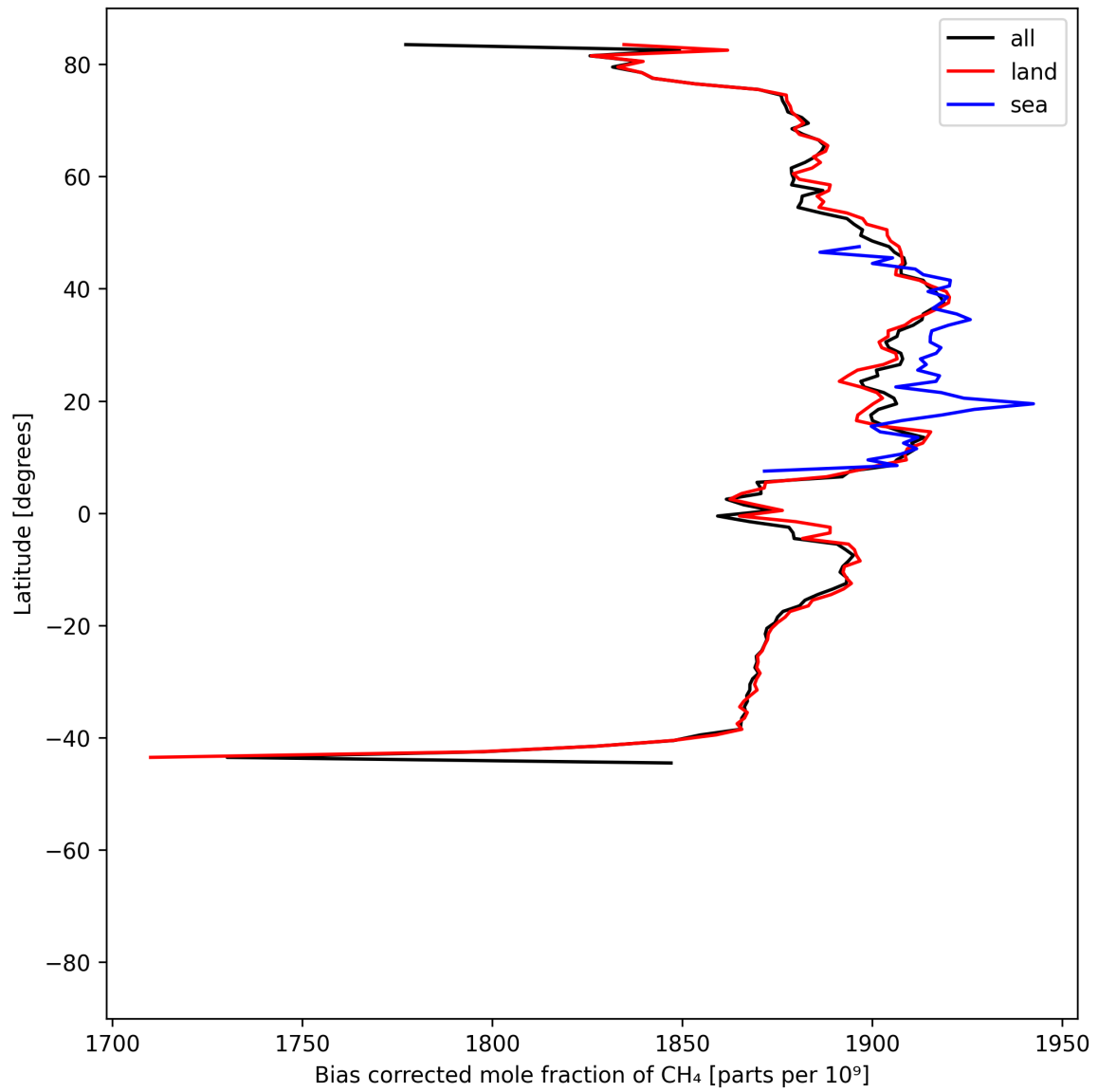
Figure 14: Zonal average of “Bias corrected mole fraction of CH 4 ” for 2025-07-13 to 2025-07-14.
