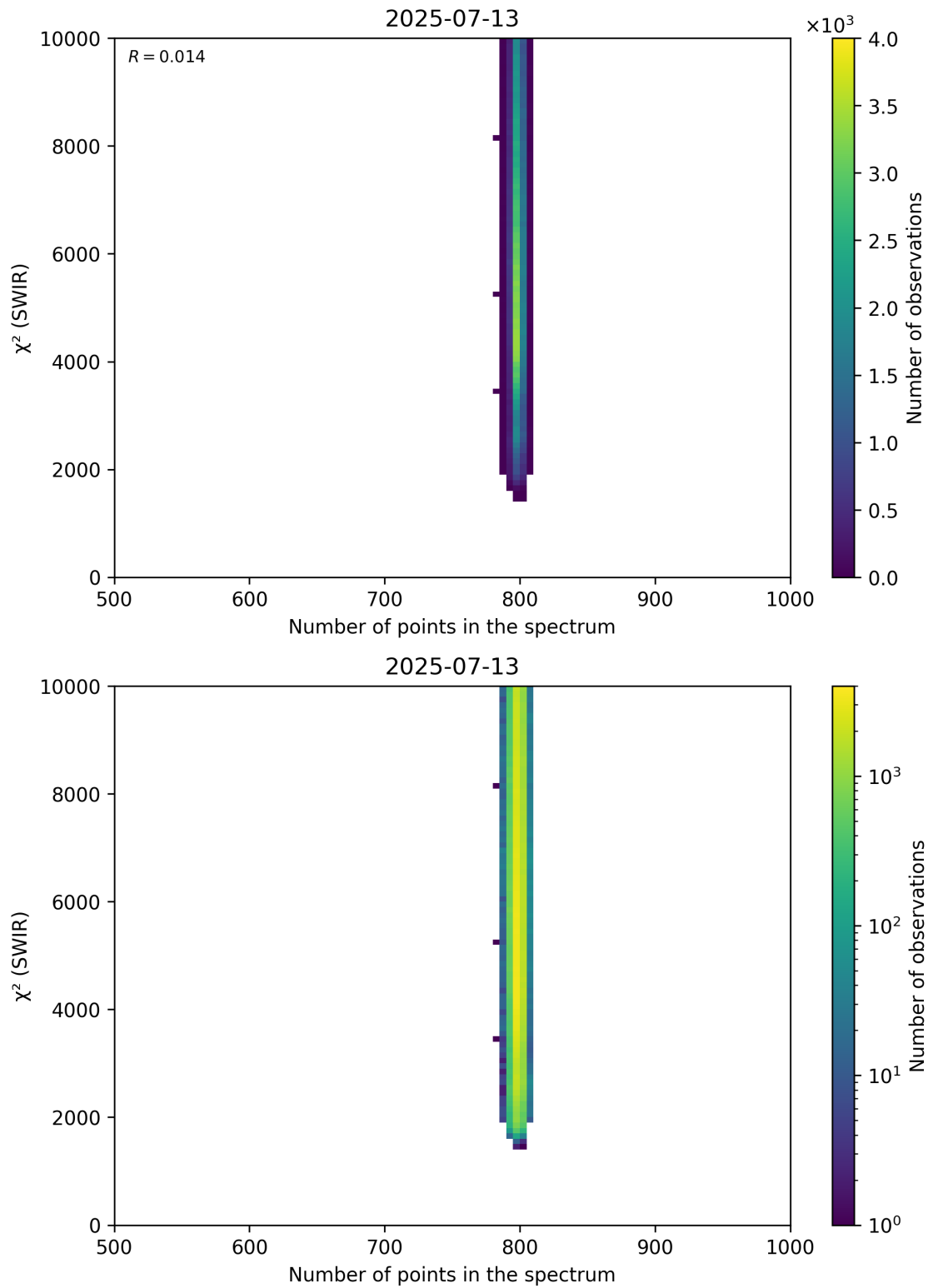
Figure 89: Scatter density plot of “Number of points in the spectrum” against “ \chi^2 (SWIR)” for 2025-07-13 to 2025-07-14.
