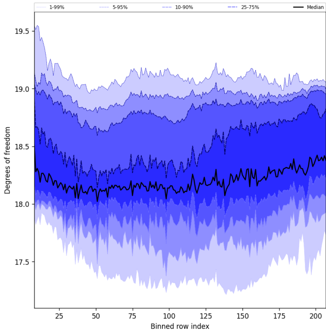
Figure 41: Along track statistics of “Degrees of freedom” for 2025-07-13 to 2025-07-14
