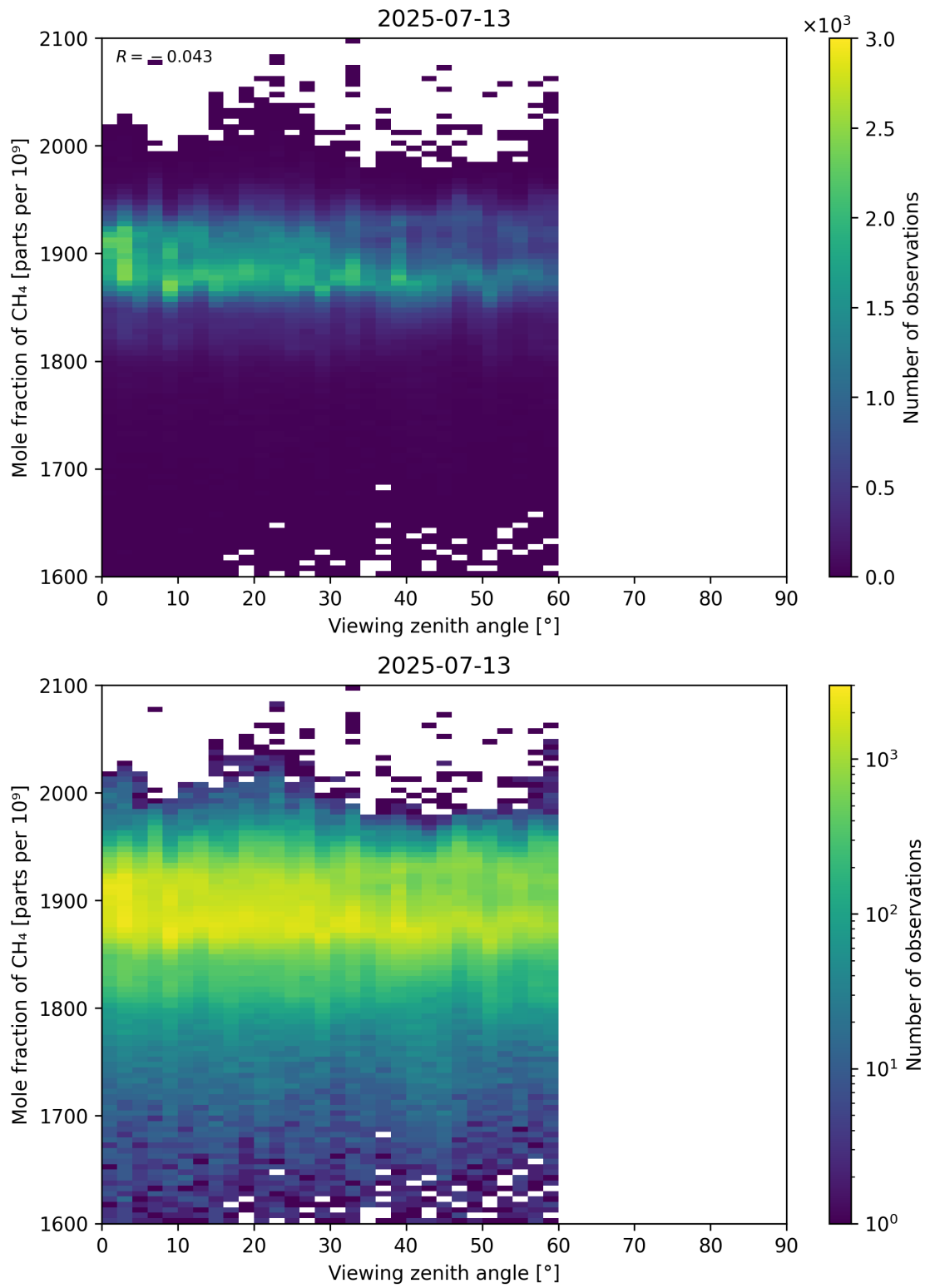
Figure 110: Scatter density plot of “Viewing zenith angle” against “Mole fraction of CH 4 ” for 2025-07-13 to 2025-07-14.
