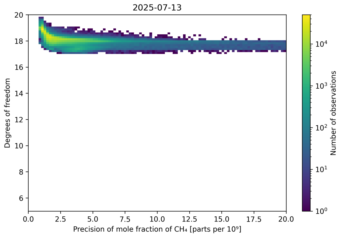
Figure 80: Scatter density plot of “Precision of mole fraction of CH 4 ” against “Degrees of freedom” for 2025-07-13 to 2025-07-14.
