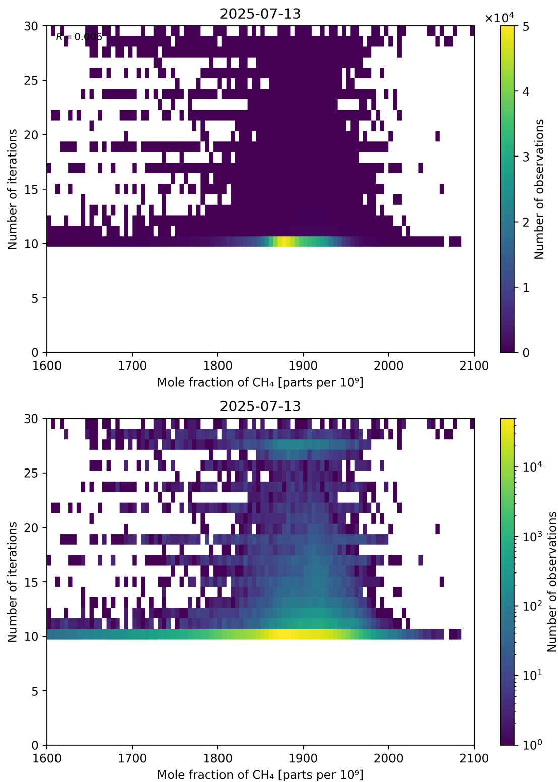
Figure 76: Scatter density plot of “Mole fraction of CH 4 ” against “Number of iterations” for 2025-07-13 to 2025-07-14.
