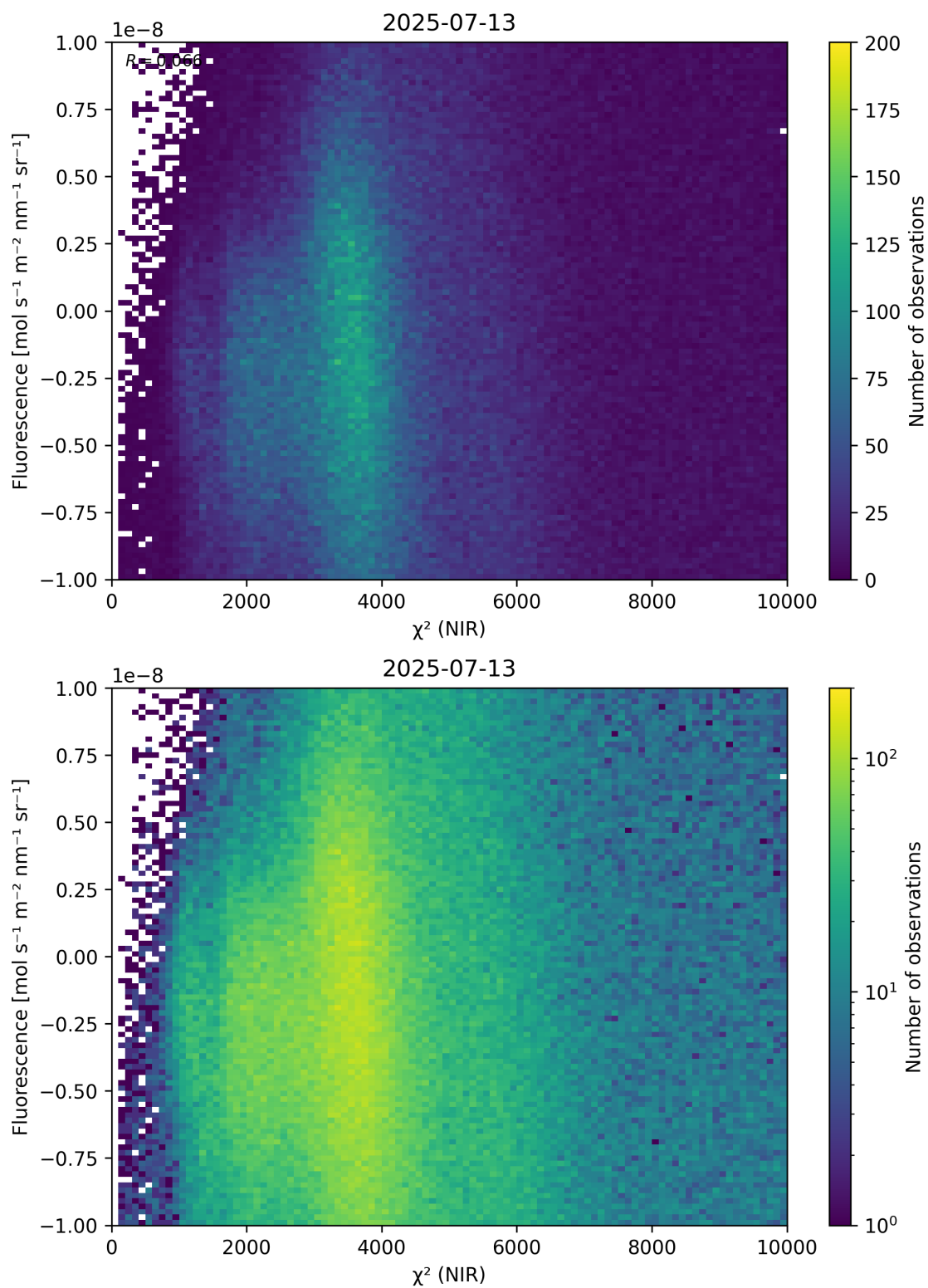
Figure 45: Scatter density plot of “ \chi^2 (NIR)” against “Fluorescence” for 2025-07-13 to 2025-07-14.
