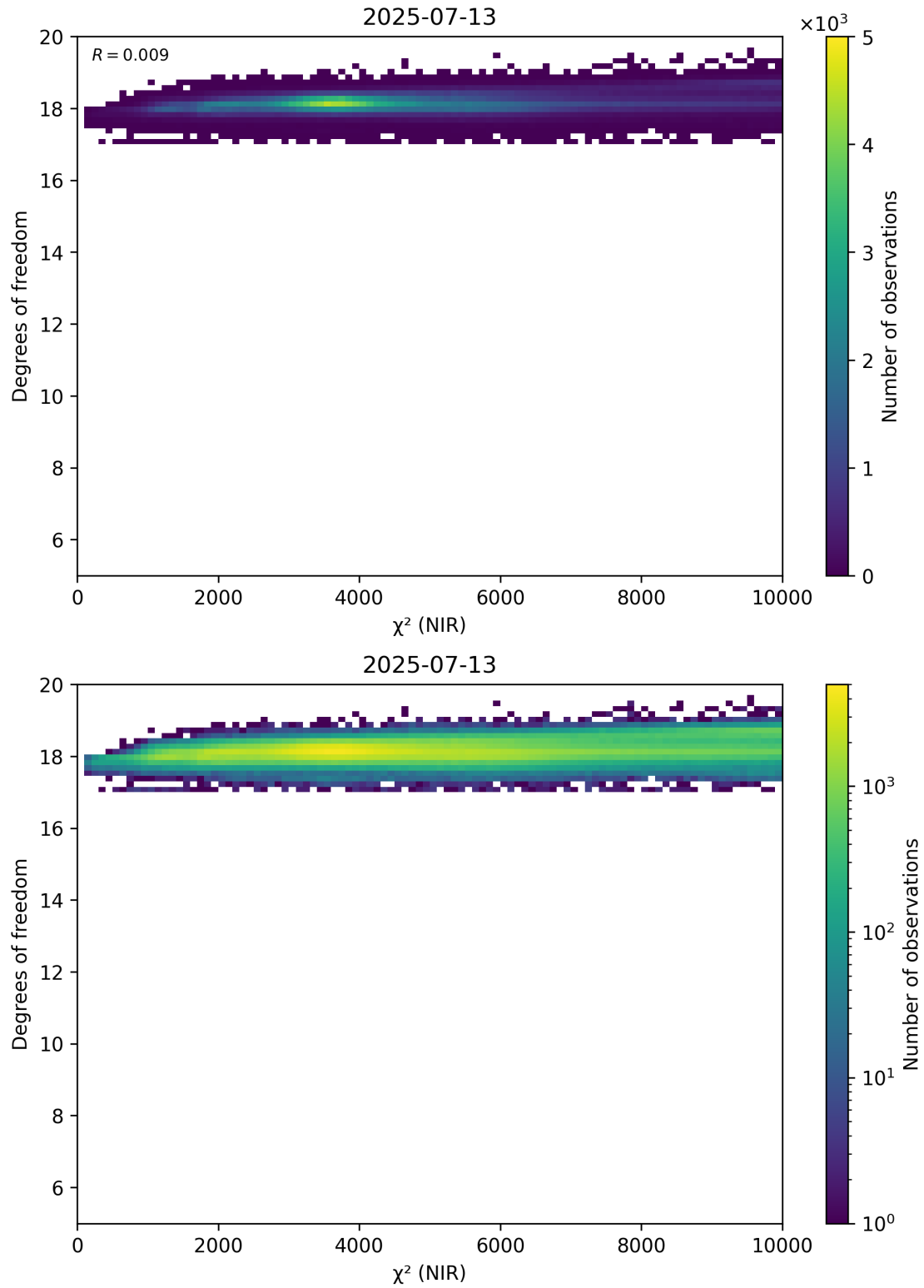
Figure 44: Scatter density plot of “ \chi^2 (NIR)” against “Degrees of freedom” for 2025-07-13 to 2025-07-14.
