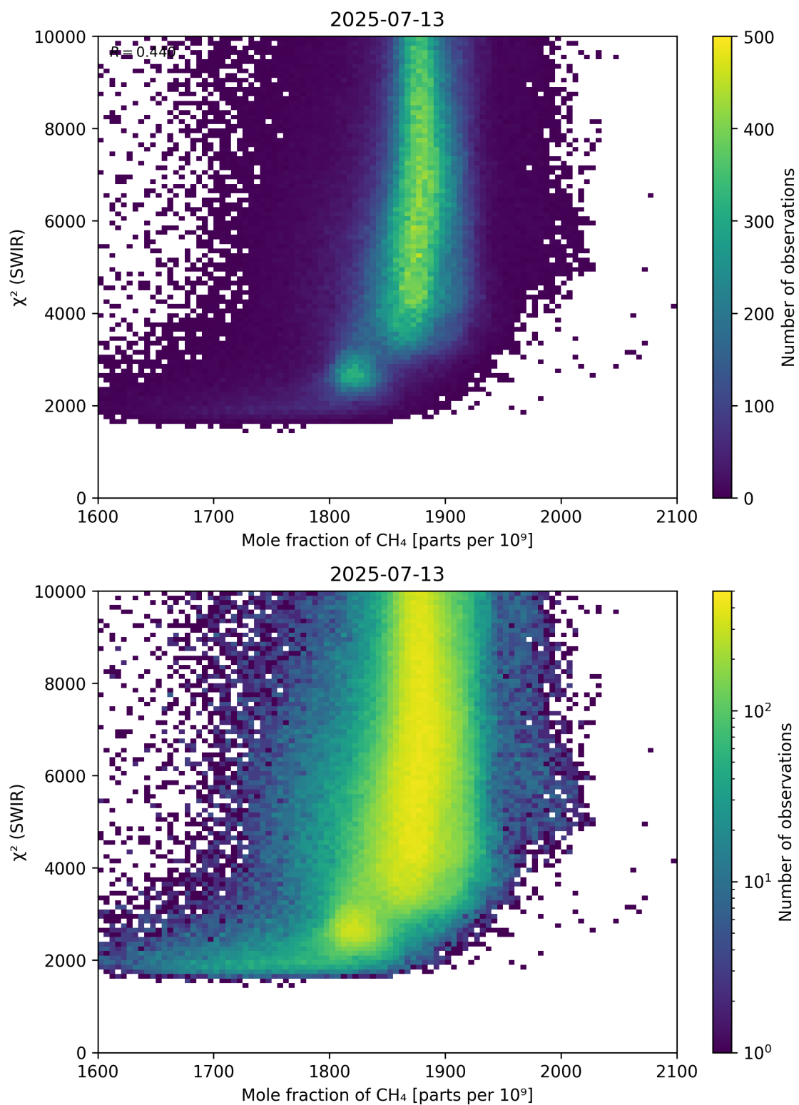
Figure 71: Scatter density plot of “Mole fraction of CH 4 ” against “ \chi^2 (SWIR)” for 2025-07-13 to 2025-07-14.
