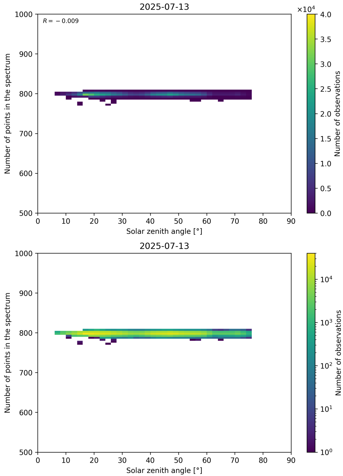
Figure 103: Scatter density plot of “Solar zenith angle” against “Number of points in the spectrum” for 2025-07-13 to 2025-07-14.
