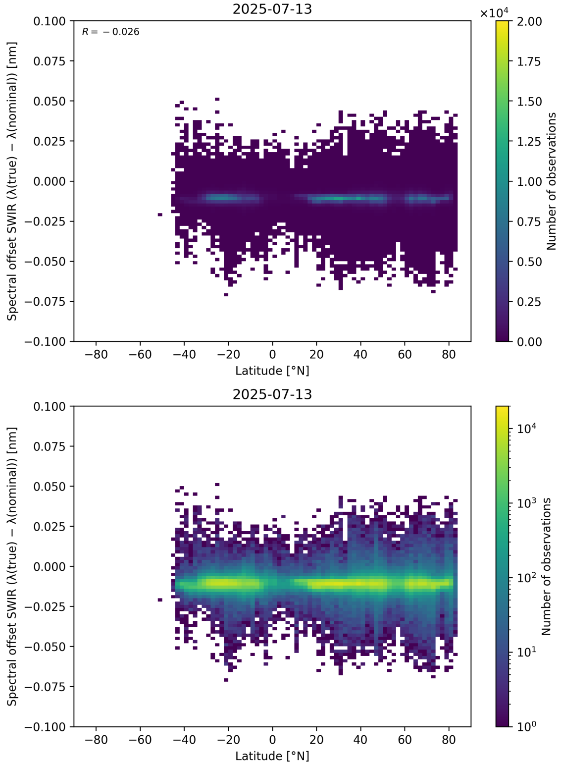
Figure 62: Scatter density plot of “Latitude” against “Spectral offset SWIR ( \lambda_{\text{true}} - \lambda_{\text{nominal}} )” for 2025-07-13 to 2025-07-14.
