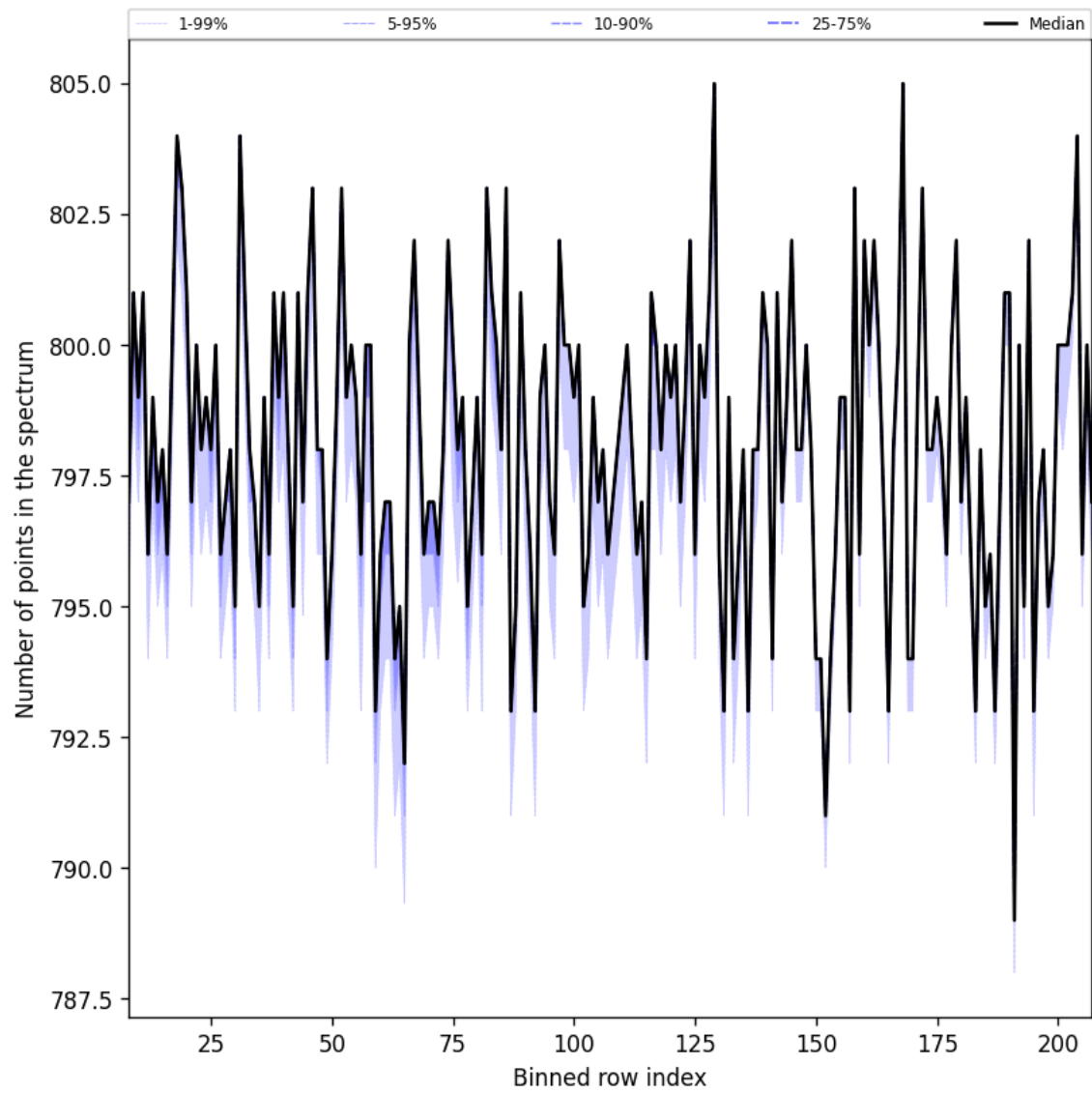
Figure 37: Along track statistics of “Number of points in the spectrum” for 2025-07-13 to 2025-07-14
