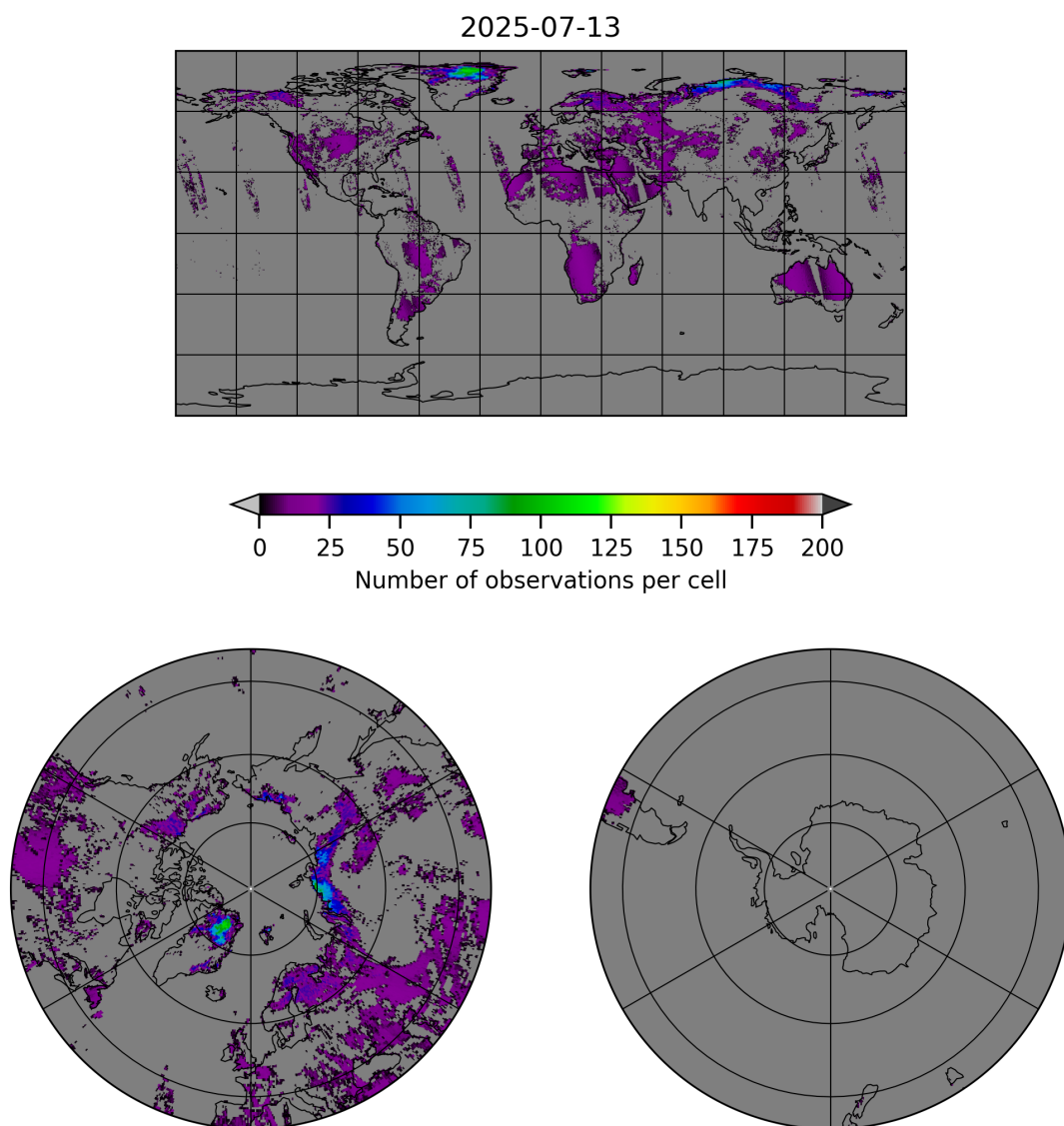
Figure 10: Map of the number of observations for 2025-07-13 to 2025-07-14
