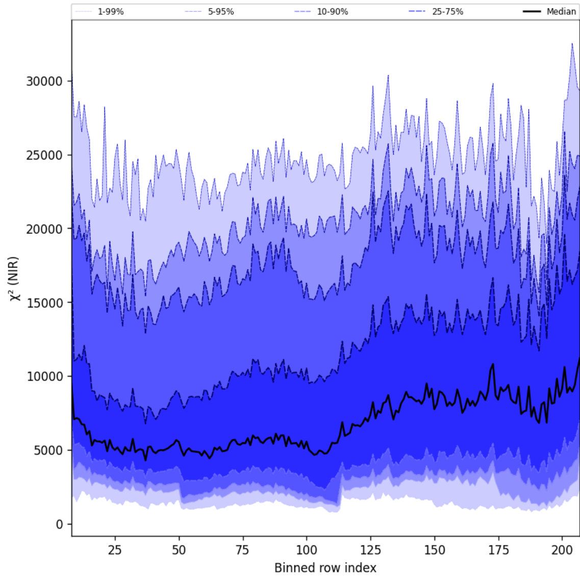
Figure 40: Along track statistics of “ \chi^2 (NIR)” for 2025-07-13 to 2025-07-14
