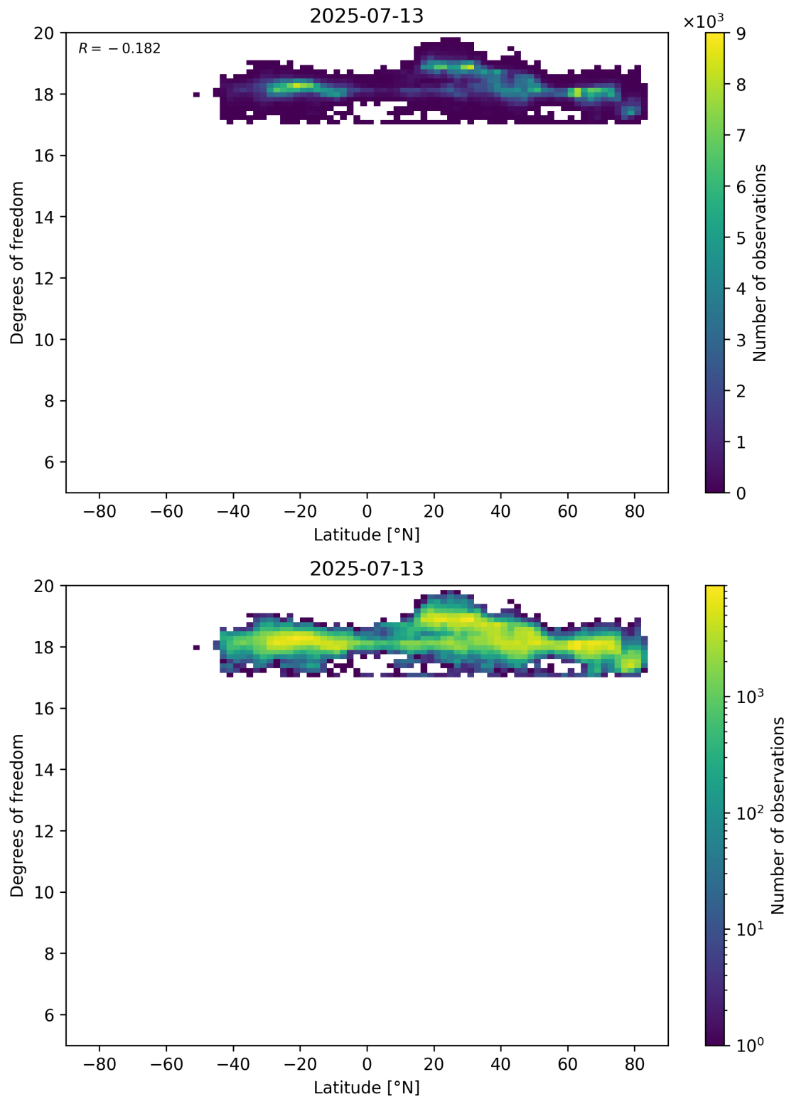
Figure 55: Scatter density plot of “Latitude” against “Degrees of freedom” for 2025-07-13 to 2025-07-14.
