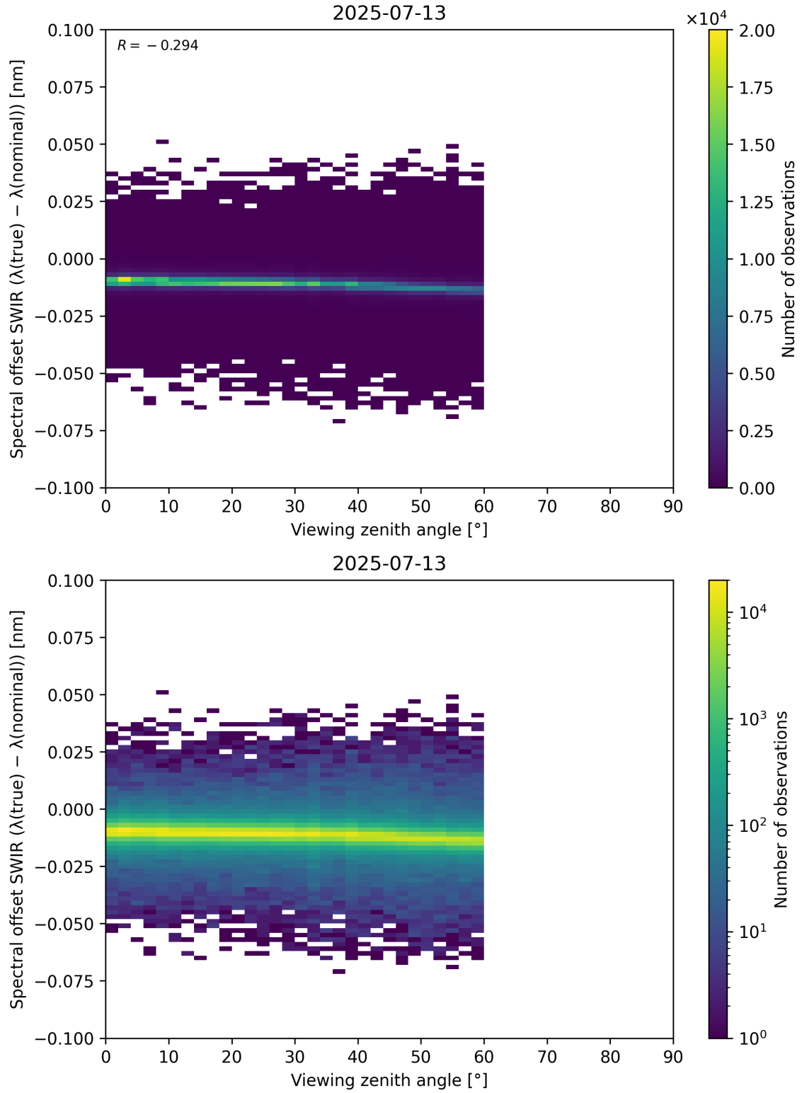
Figure 116: Scatter density plot of “Viewing zenith angle” against “Spectral offset SWIR ( \lambda_{\text{true}} - \lambda_{\text{nominal}} )” for 2025-07-13 to 2025-07-14.
