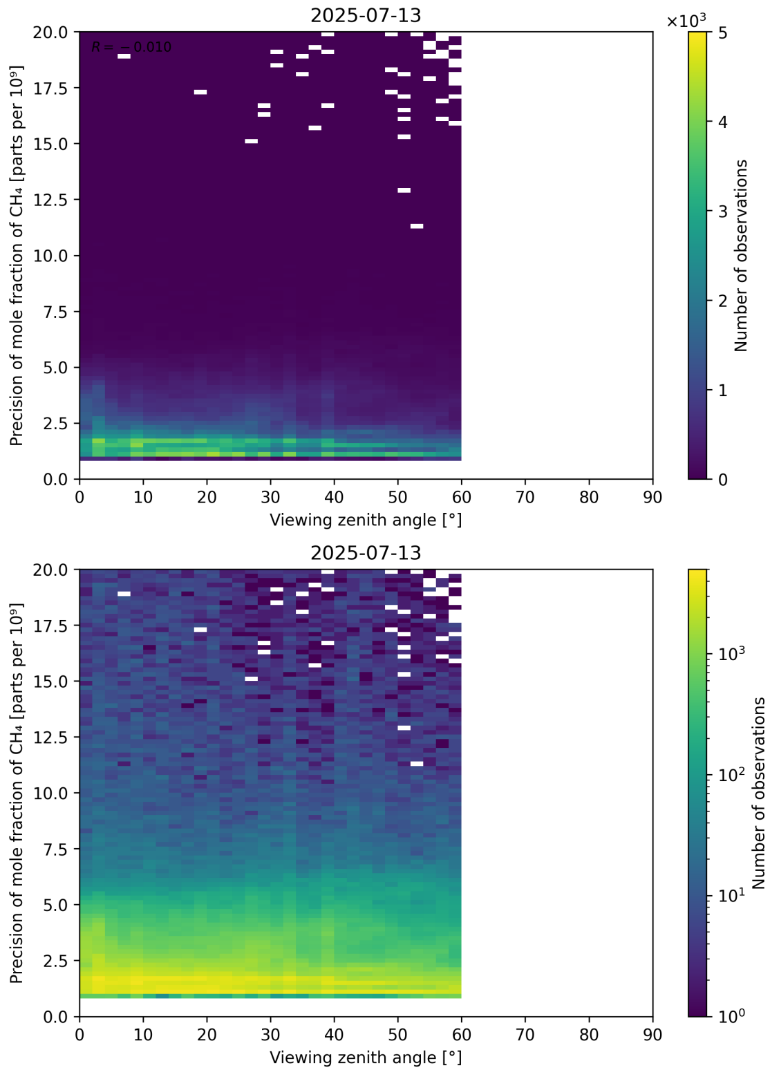
Figure 112: Scatter density plot of “Viewing zenith angle” against “Precision of mole fraction of CH 4 ” for 2025-07-13 to 2025-07-14.
