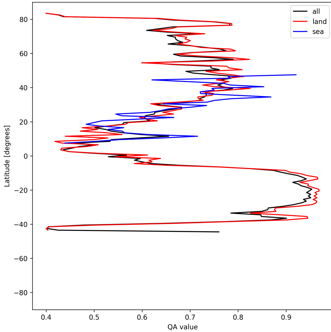
Figure 11: Zonal average of “QA value” for 2025-07-13 to 2025-07-14.
