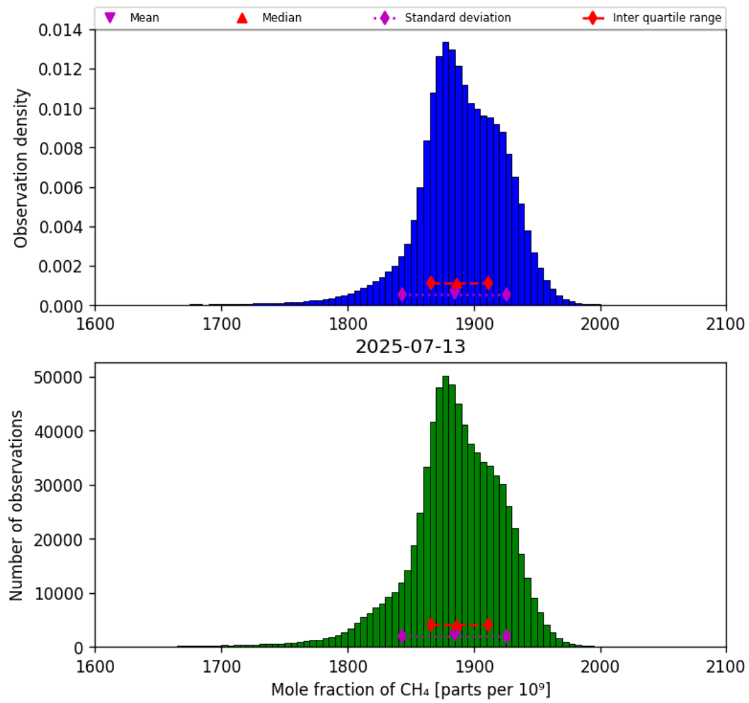
Figure 23: Histogram of “Mole fraction of CH 4 ” for 2025-07-13 to 2025-07-14
