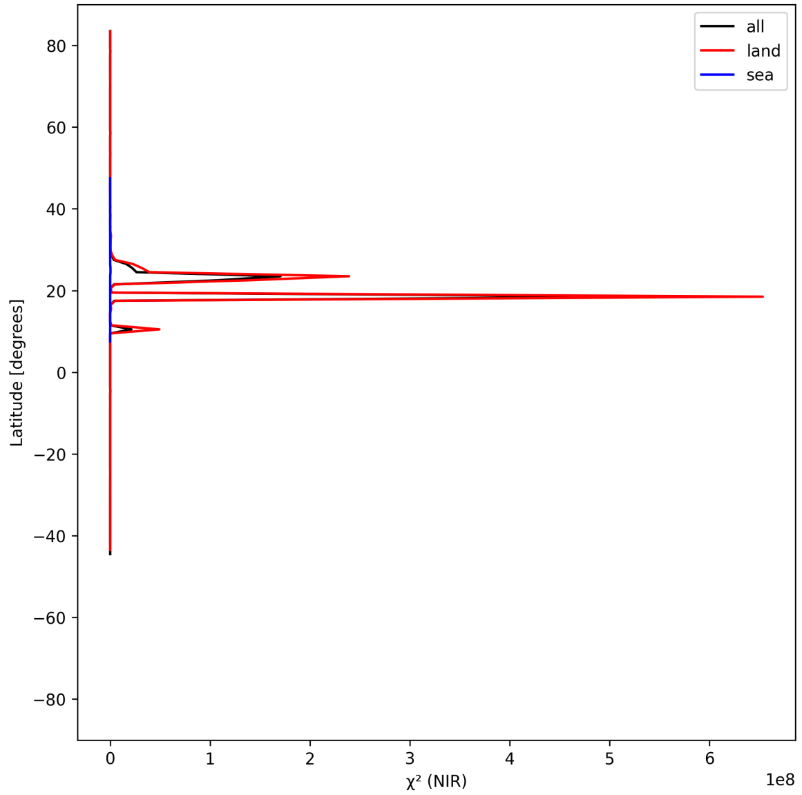
Figure 18: Zonal average of “ \chi^2 (NIR)” for 2025-07-13 to 2025-07-14.
