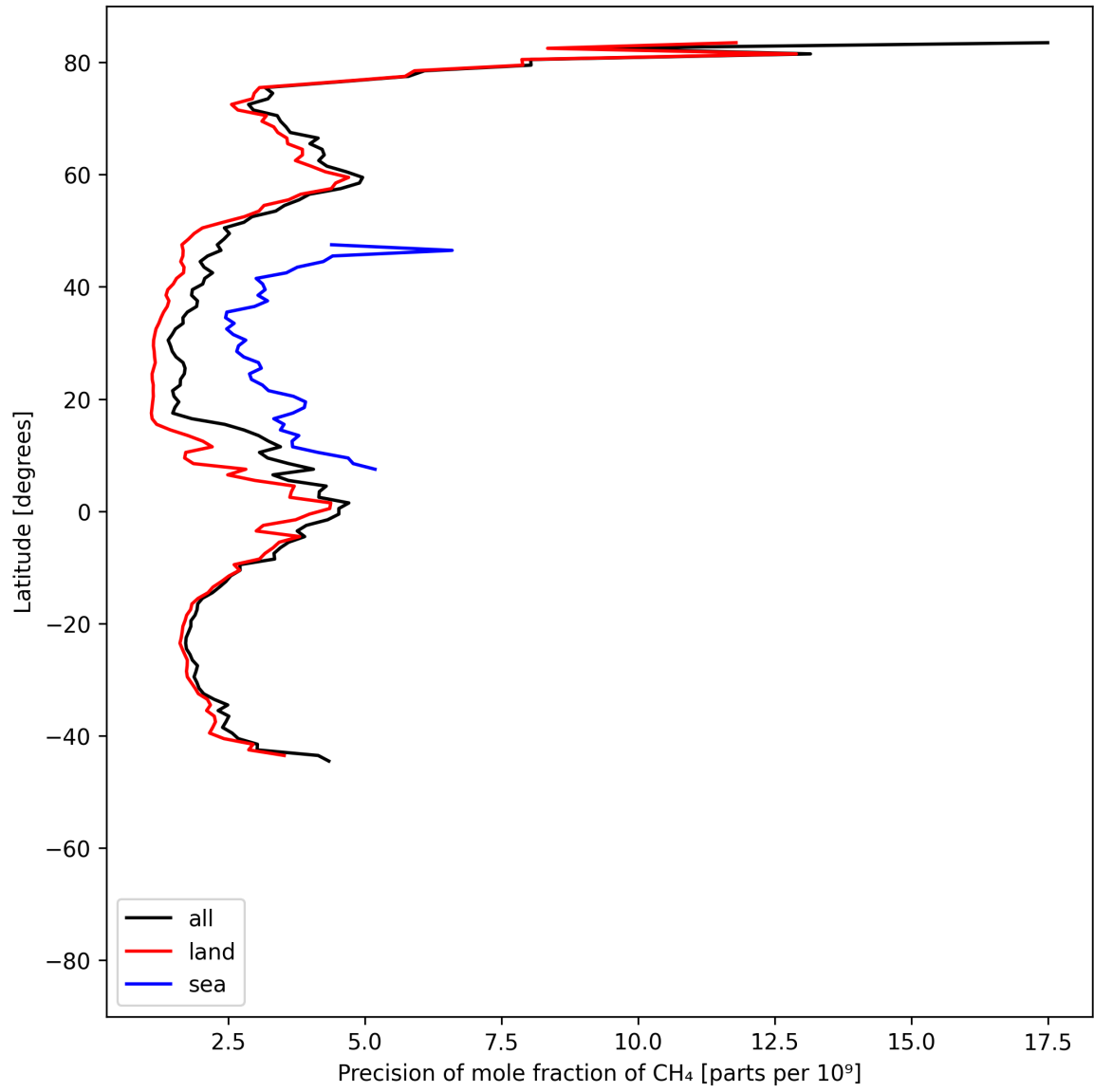
Figure 13: Zonal average of “Precision of mole fraction of CH 4 ” for 2025-07-13 to 2025-07-14.
