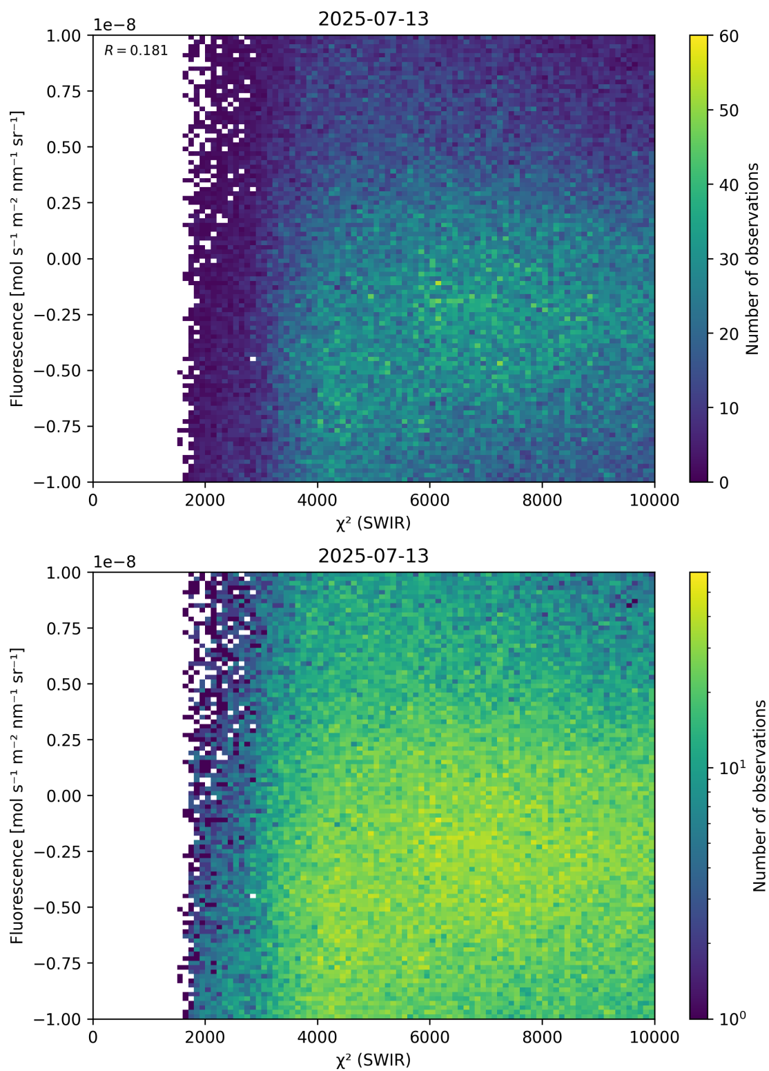
Figure 49: Scatter density plot of “ \chi^2 (SWIR)” against “Fluorescence” for 2025-07-13 to 2025-07-14.
