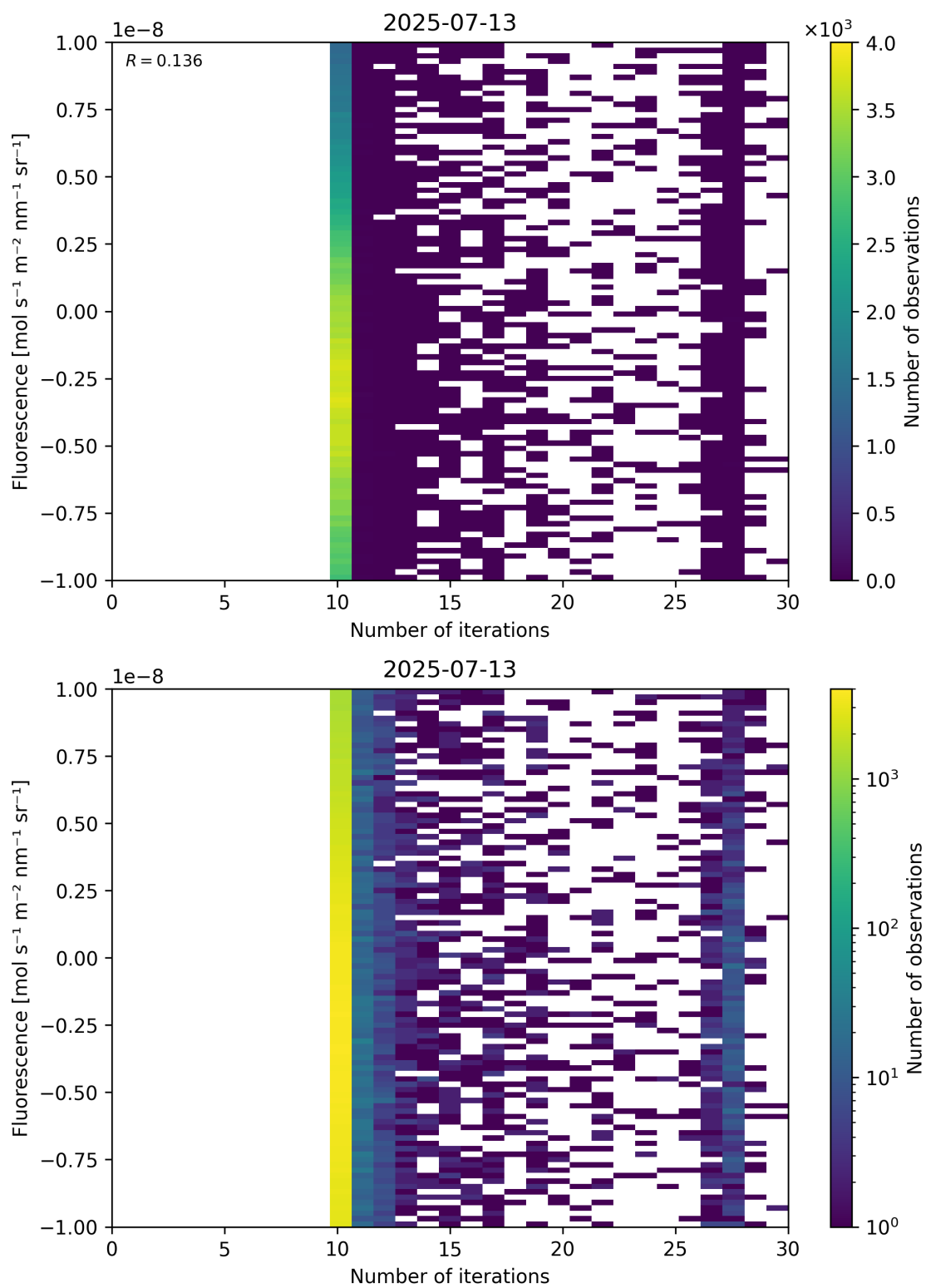
Figure 87: Scatter density plot of “Number of iterations” against “Fluorescence” for 2025-07-13 to 2025-07-14.
