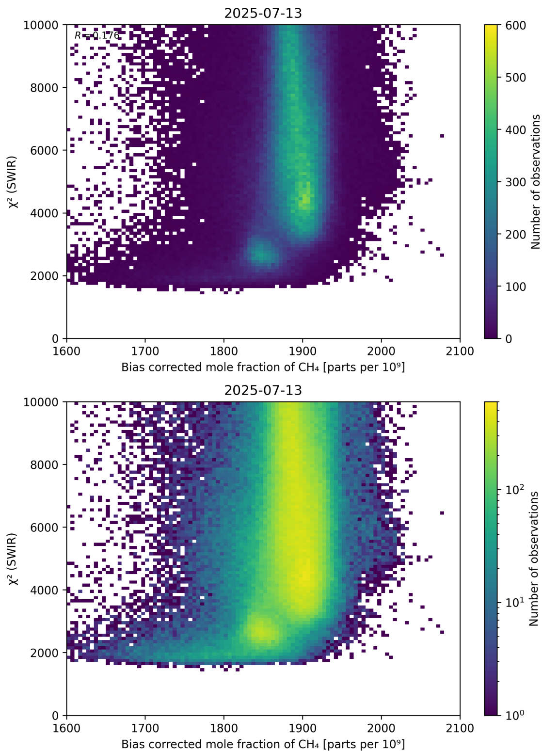
Figure 64: Scatter density plot of “Bias corrected mole fraction of \text{CH}_4 ” against “ \chi^2 (SWIR)” for 2025-07-13 to 2025-07-14.
