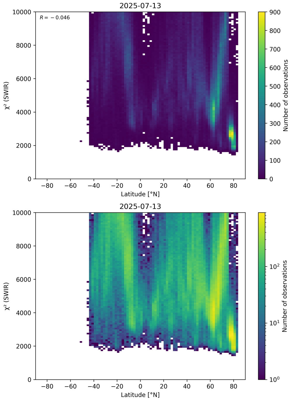
Figure 54: Scatter density plot of “Latitude” against “ \chi^2 (SWIR)” for 2025-07-13 to 2025-07-14.
