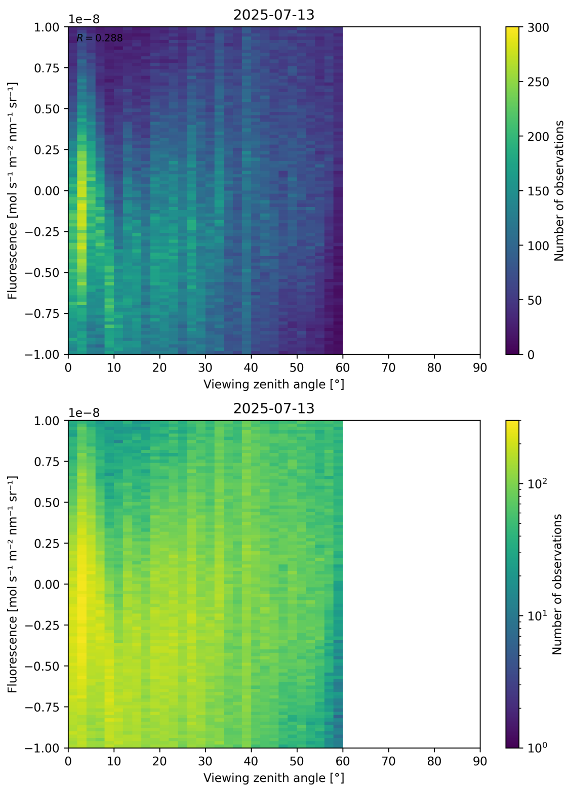
Figure 108: Scatter density plot of “Viewing zenith angle” against “Fluorescence” for 2025-07-13 to 2025-07-14.
