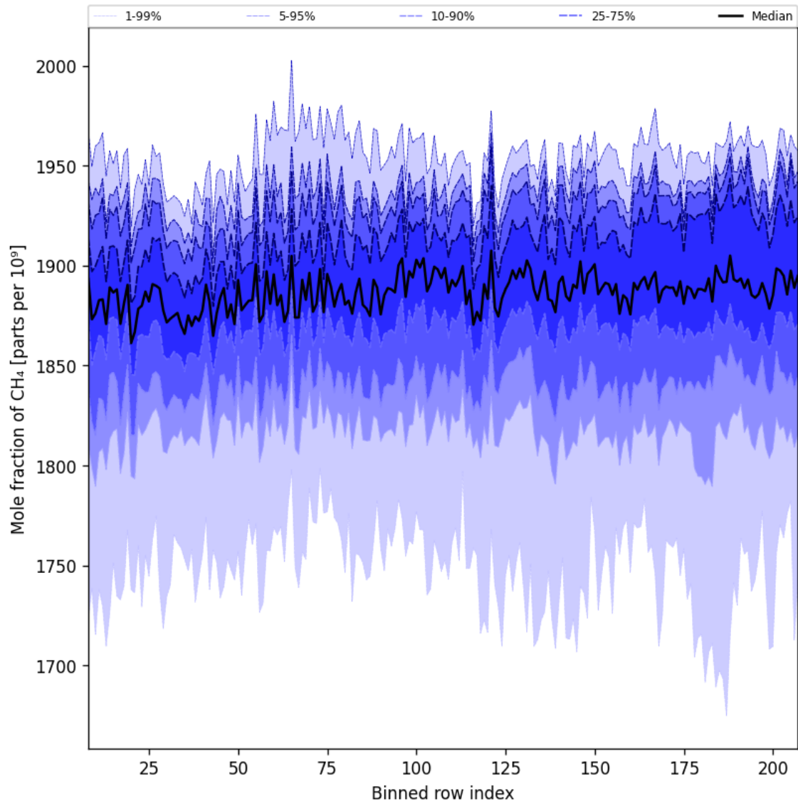
Figure 34: Along track statistics of “Mole fraction of CH 4 ” for 2025-07-13 to 2025-07-14
