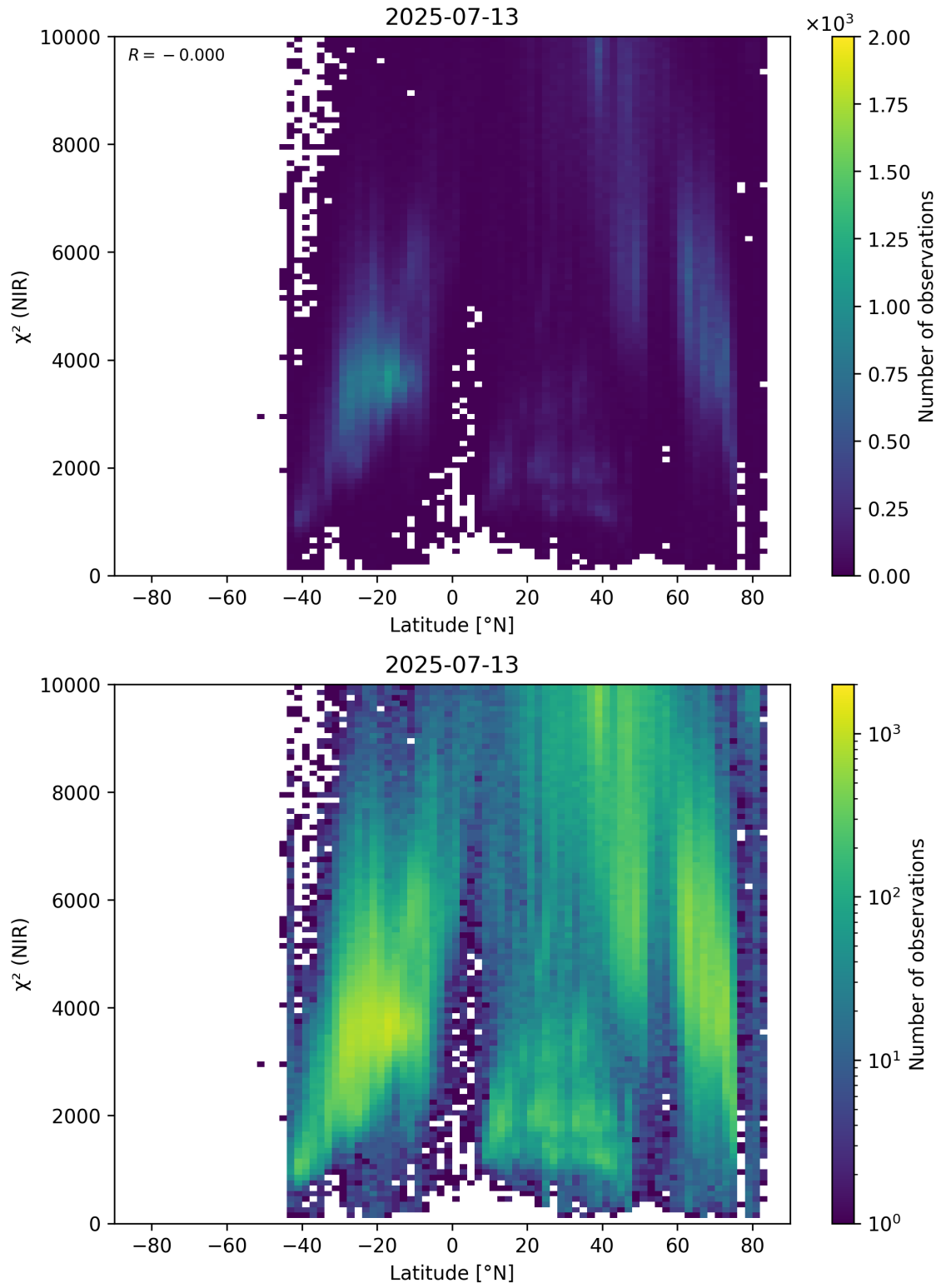
Figure 53: Scatter density plot of “Latitude” against “ \chi^2 (NIR)” for 2025-07-13 to 2025-07-14.
