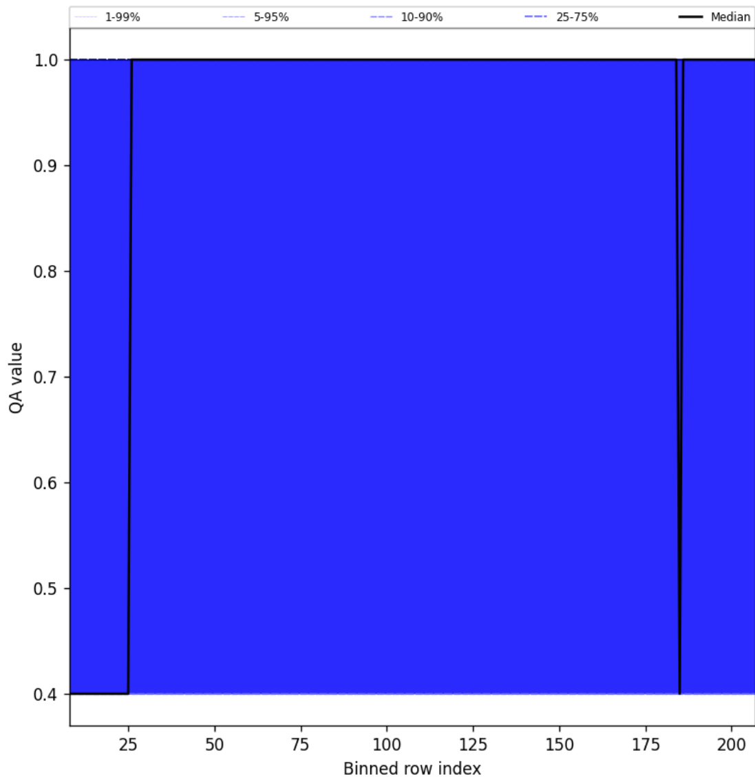
Figure 33: Along track statistics of “QA value” for 2025-07-13 to 2025-07-14
