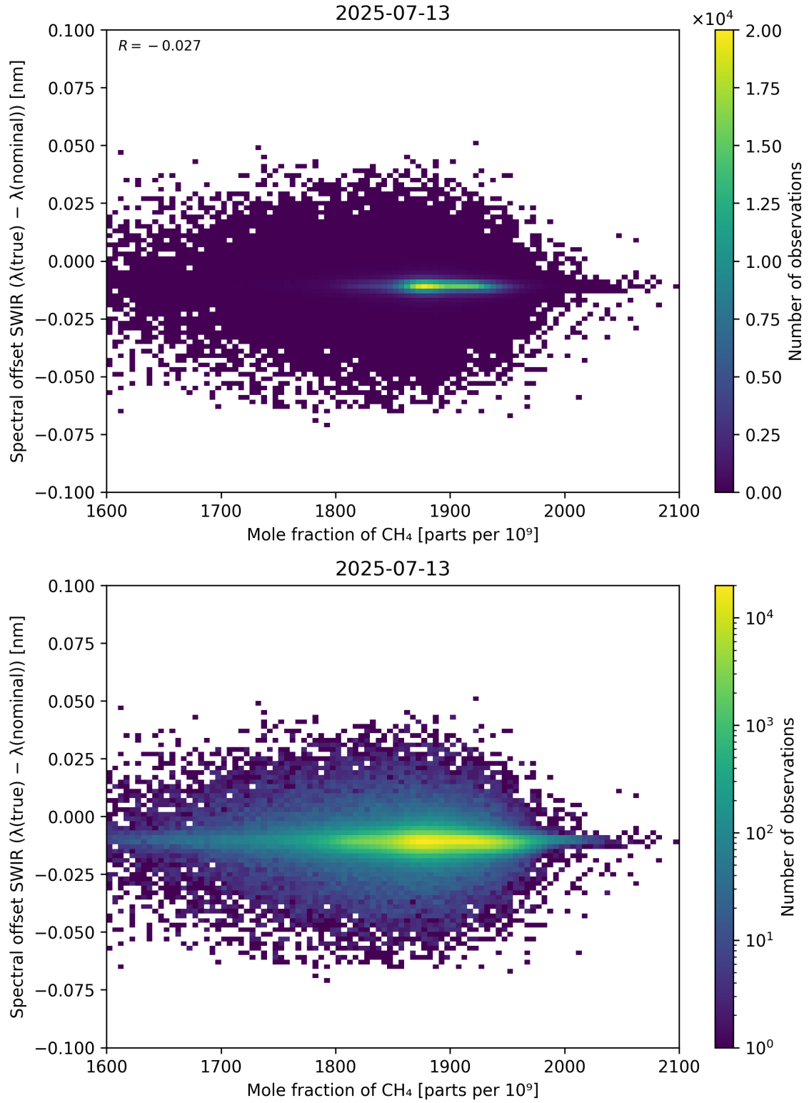
Figure 86: Scatter density plot of “Mole fraction of CH 4 ” against “Spectral offset SWIR ( \lambda_{\text{true}} - \lambda_{\text{nominal}} )” for 2025-07-13 to 2025-07-14.
