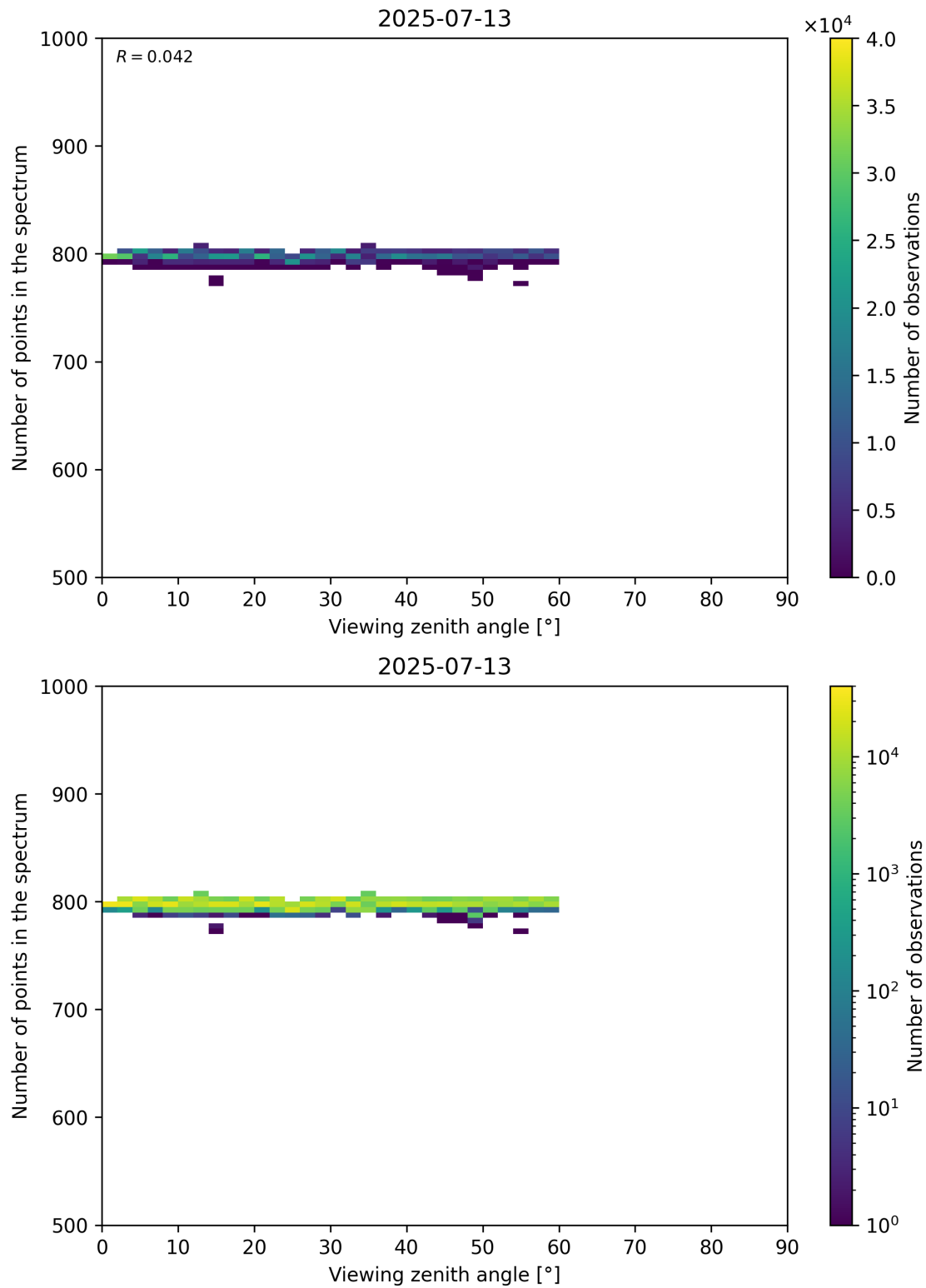
Figure 114: Scatter density plot of “Viewing zenith angle” against “Number of points in the spectrum” for 2025-07-13 to 2025-07-14.
