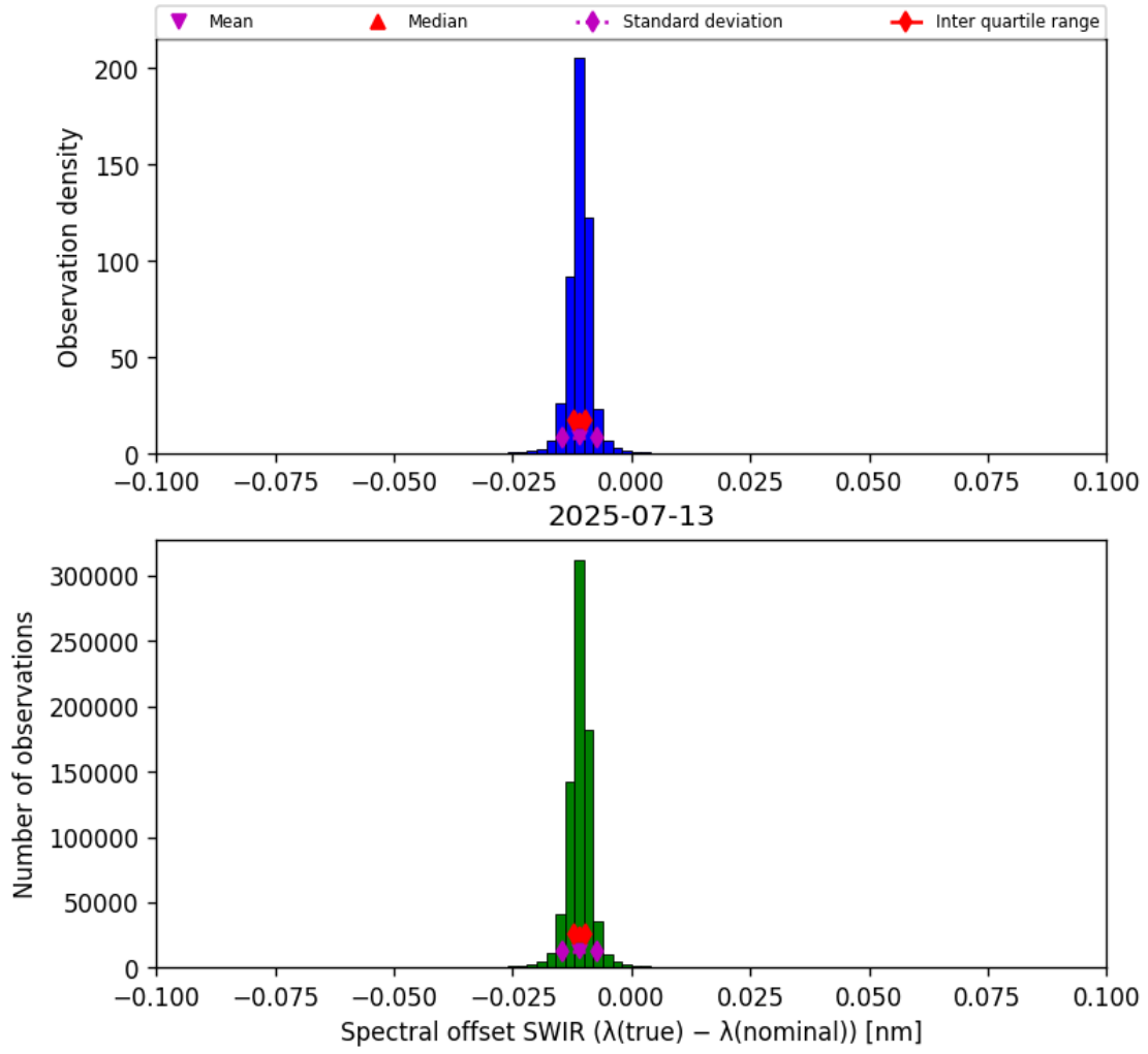
Figure 27: Histogram of “Spectral offset SWIR ( \lambda_{\text{true}} - \lambda_{\text{nominal}} )” for 2025-07-13 to 2025-07-14
