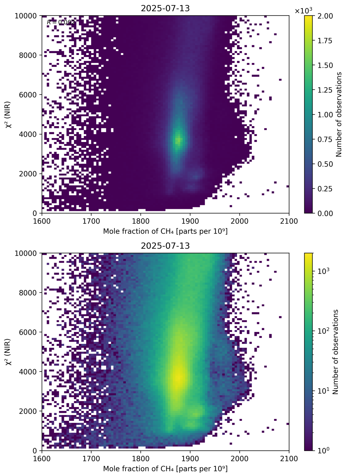
Figure 70: Scatter density plot of “Mole fraction of \text{CH}_4 ” against “ \chi^2 (NIR)” for 2025-07-13 to 2025-07-14.
