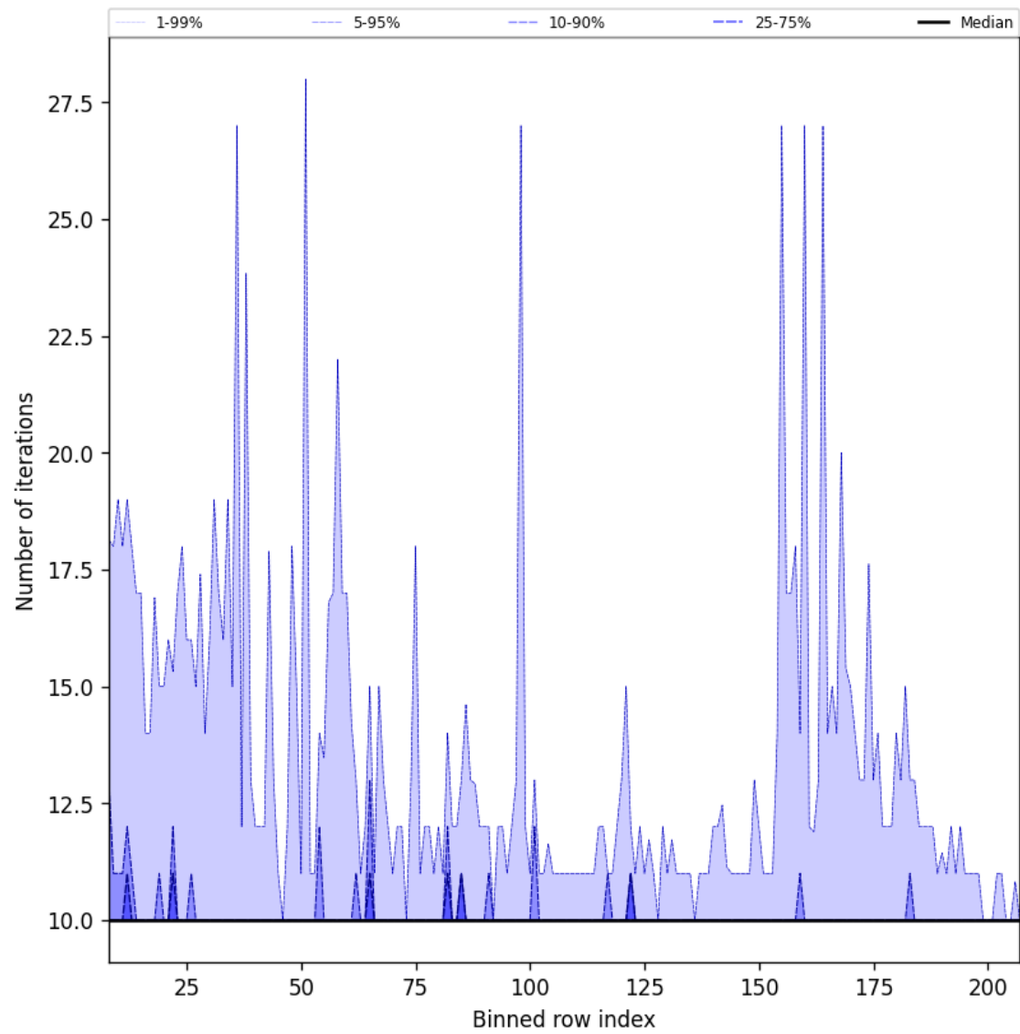
Figure 42: Along track statistics of “Number of iterations” for 2025-07-13 to 2025-07-14
