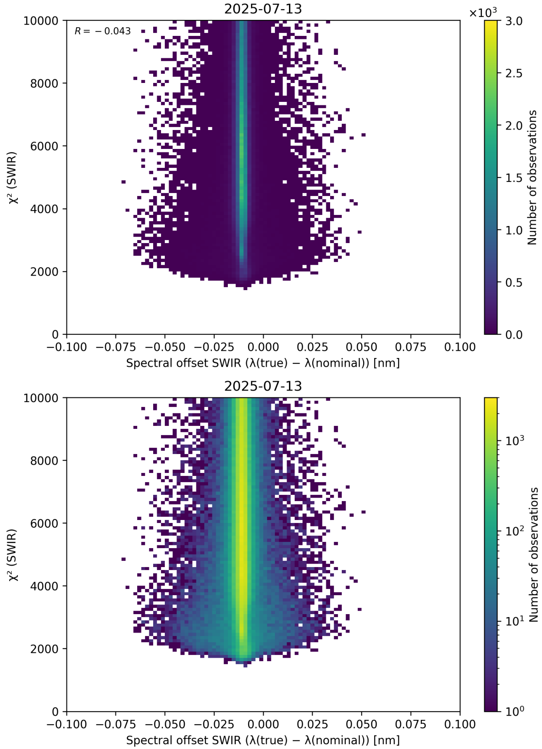
Figure 118: Scatter density plot of “Spectral offset SWIR ( \lambda_{\text{true}} - \lambda_{\text{nominal}} )” against “ \chi^2 (SWIR)” for 2025-07-13 to 2025-07-14.
