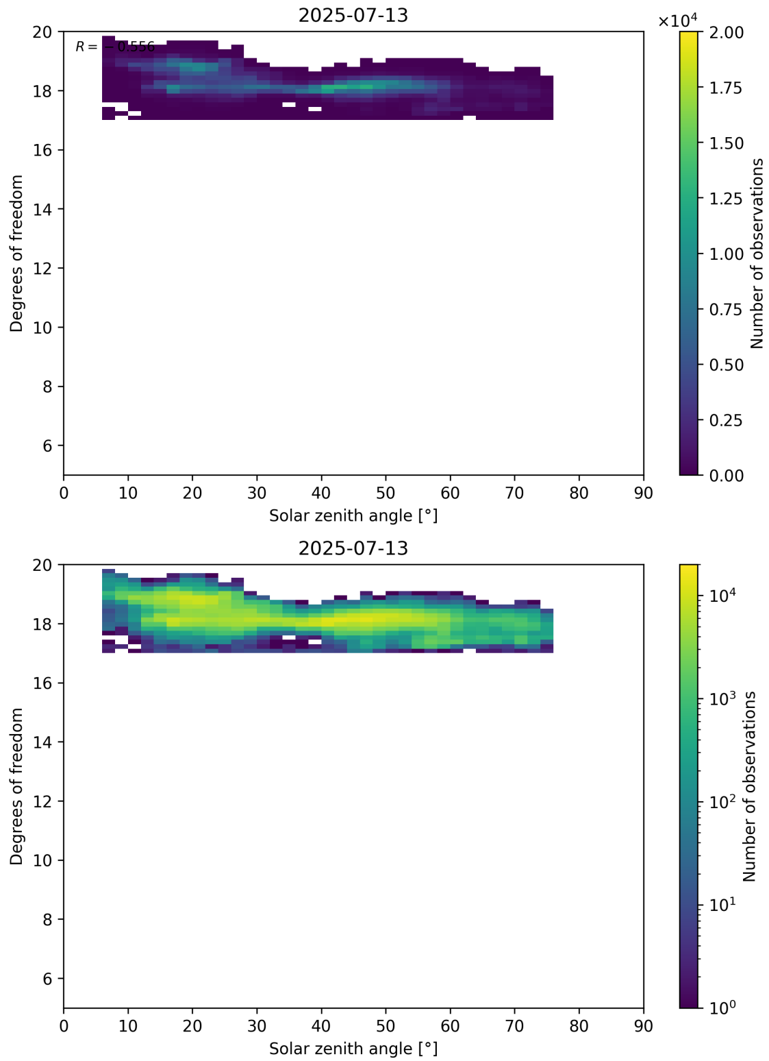
Figure 96: Scatter density plot of “Solar zenith angle” against “Degrees of freedom” for 2025-07-13 to 2025-07-14.
