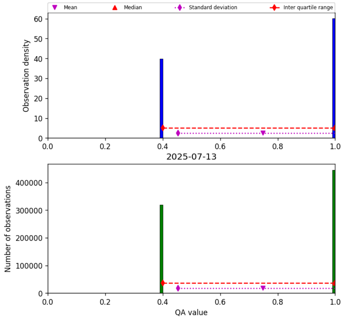
Figure 22: Histogram of “QA value” for 2025-07-13 to 2025-07-14
