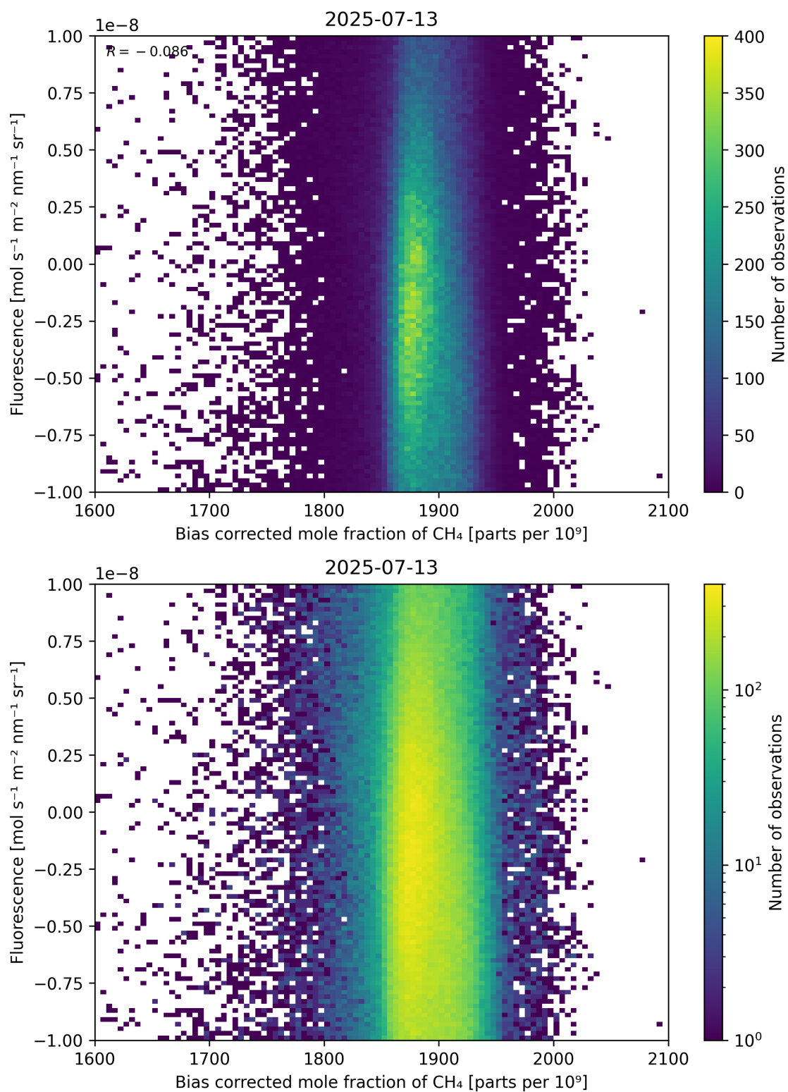
Figure 66: Scatter density plot of “Bias corrected mole fraction of \text{CH}_4 ” against “Fluorescence” for 2025-07-13 to 2025-07-14.
