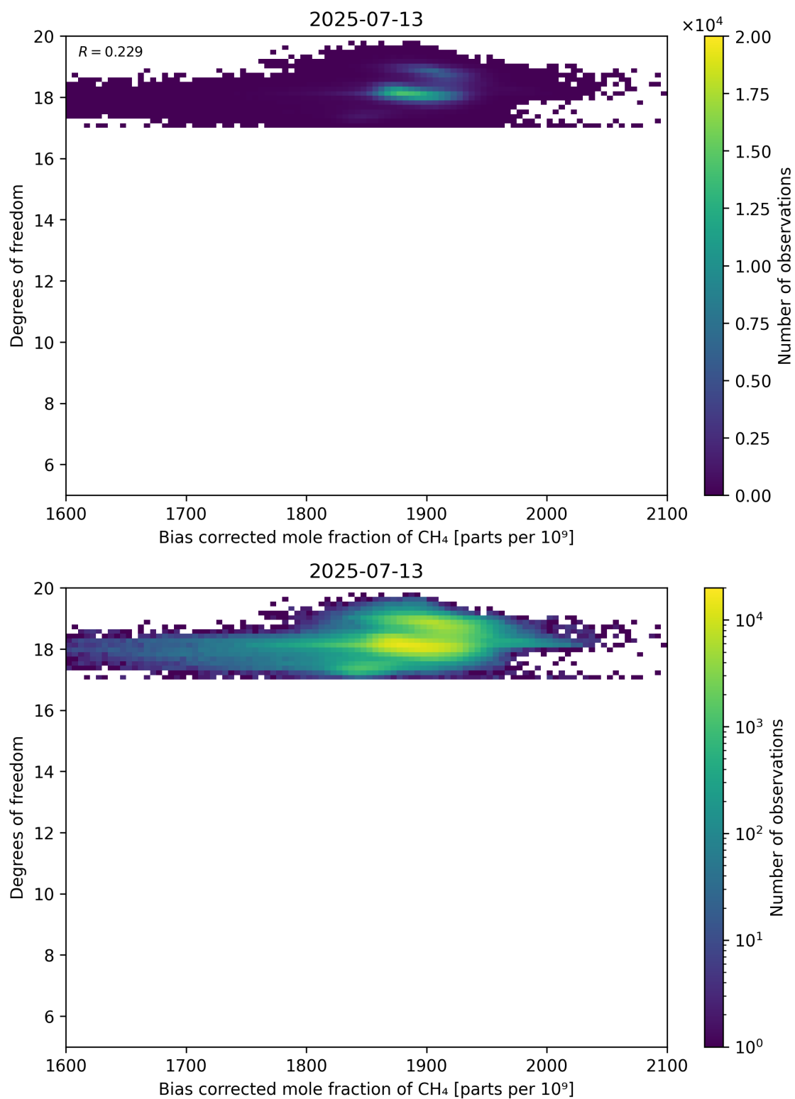
Figure 65: Scatter density plot of “Bias corrected mole fraction of \text{CH}_4 ” against “Degrees of freedom” for 2025-07-13 to 2025-07-14.
