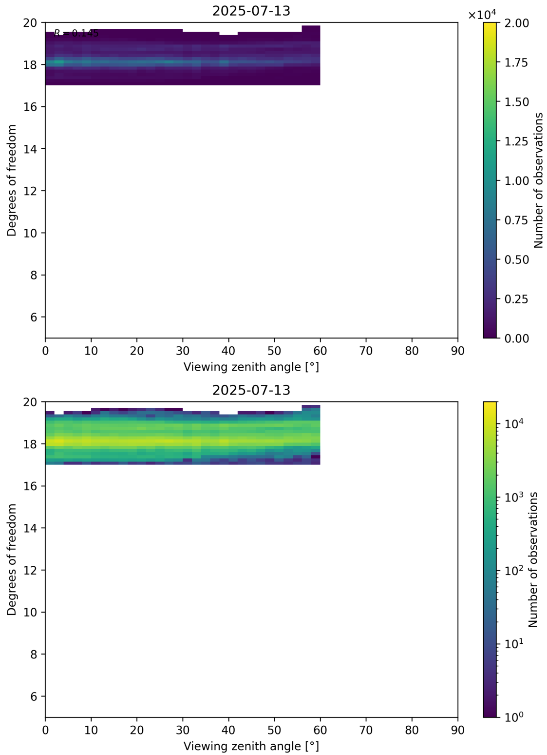
Figure 107: Scatter density plot of “Viewing zenith angle” against “Degrees of freedom” for 2025-07-13 to 2025-07-14.
