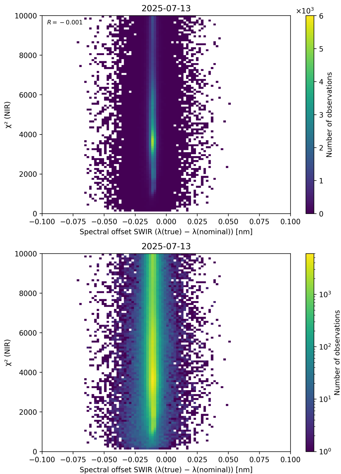
Figure 117: Scatter density plot of “Spectral offset SWIR ( \lambda_{\text{true}} - \lambda_{\text{nominal}} )” against “ \chi^2 (NIR)” for 2025-07-13 to 2025-07-14.
