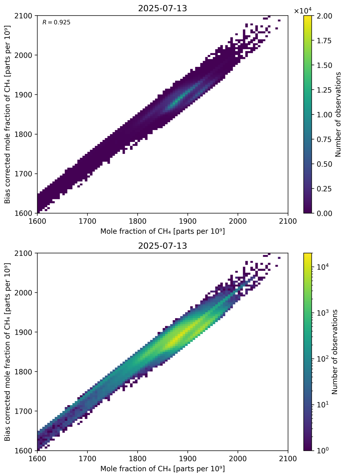
Figure 74: Scatter density plot of “Mole fraction of CH 4 ” against “Bias corrected mole fraction of CH 4 ” for 2025-07-13 to 2025-07-14.
