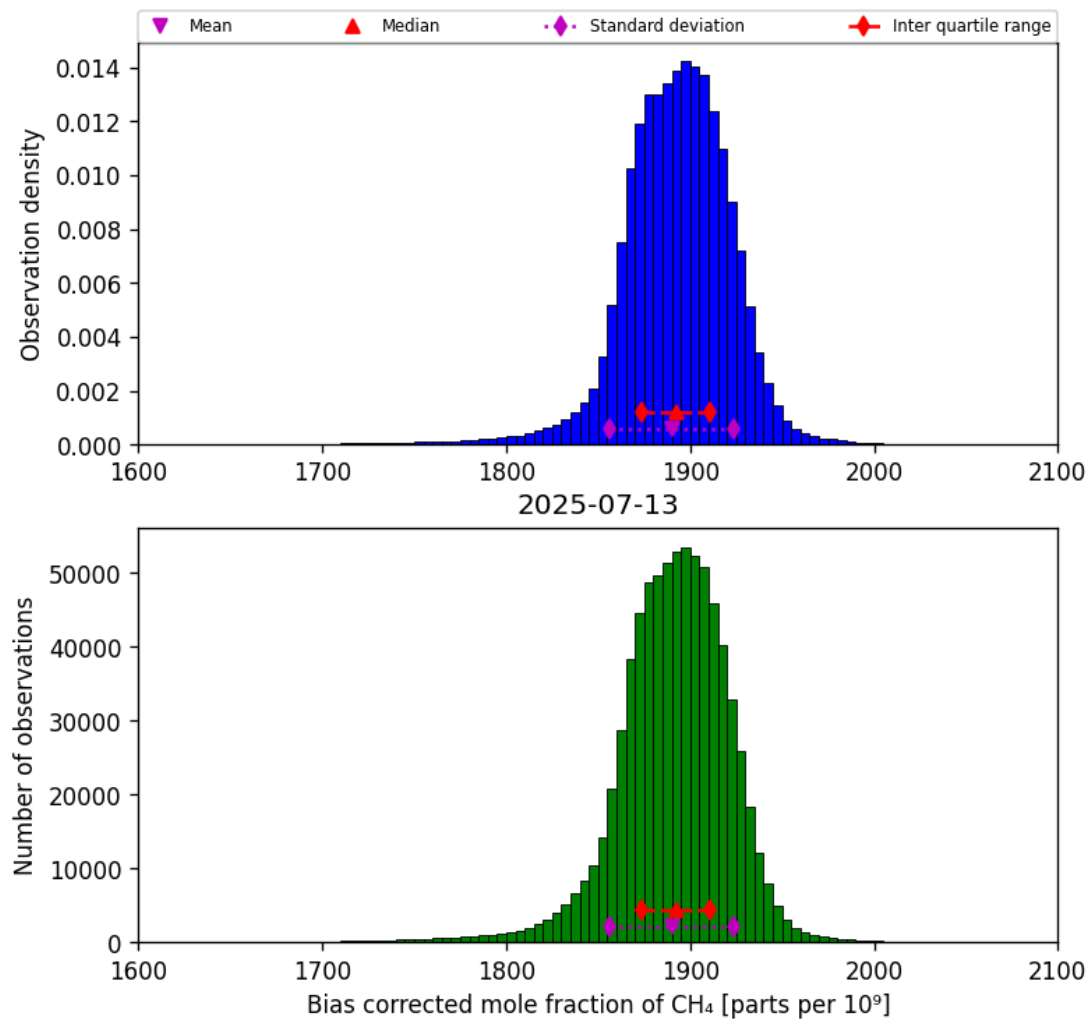
Figure 25: Histogram of “Bias corrected mole fraction of CH 4 ” for 2025-07-13 to 2025-07-14
