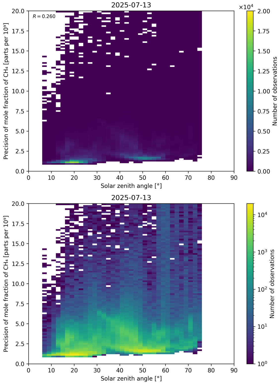
Figure 101: Scatter density plot of “Solar zenith angle” against “Precision of mole fraction of CH 4 ” for 2025-07-13 to 2025-07-14.
