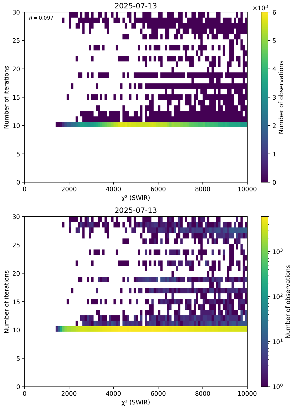
Figure 50: Scatter density plot of “ \chi^2 (SWIR)” against “Number of iterations” for 2025-07-13 to 2025-07-14.
