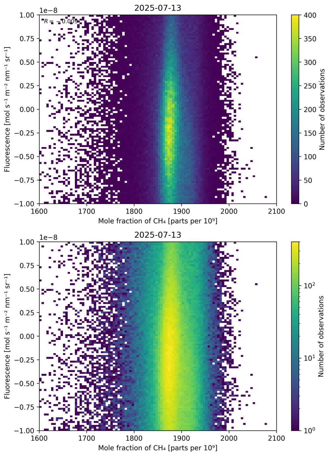
Figure 73: Scatter density plot of “Mole fraction of \text{CH}_4 ” against “Fluorescence” for 2025-07-13 to 2025-07-14.
