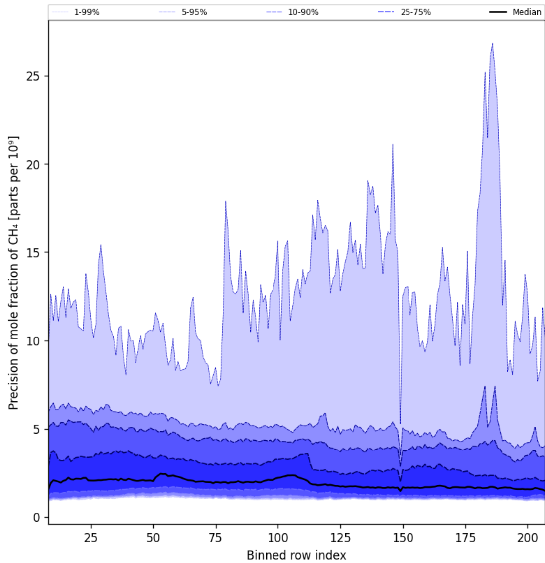
Figure 35: Along track statistics of “Precision of mole fraction of CH 4 ” for 2025-07-13 to 2025-07-14
