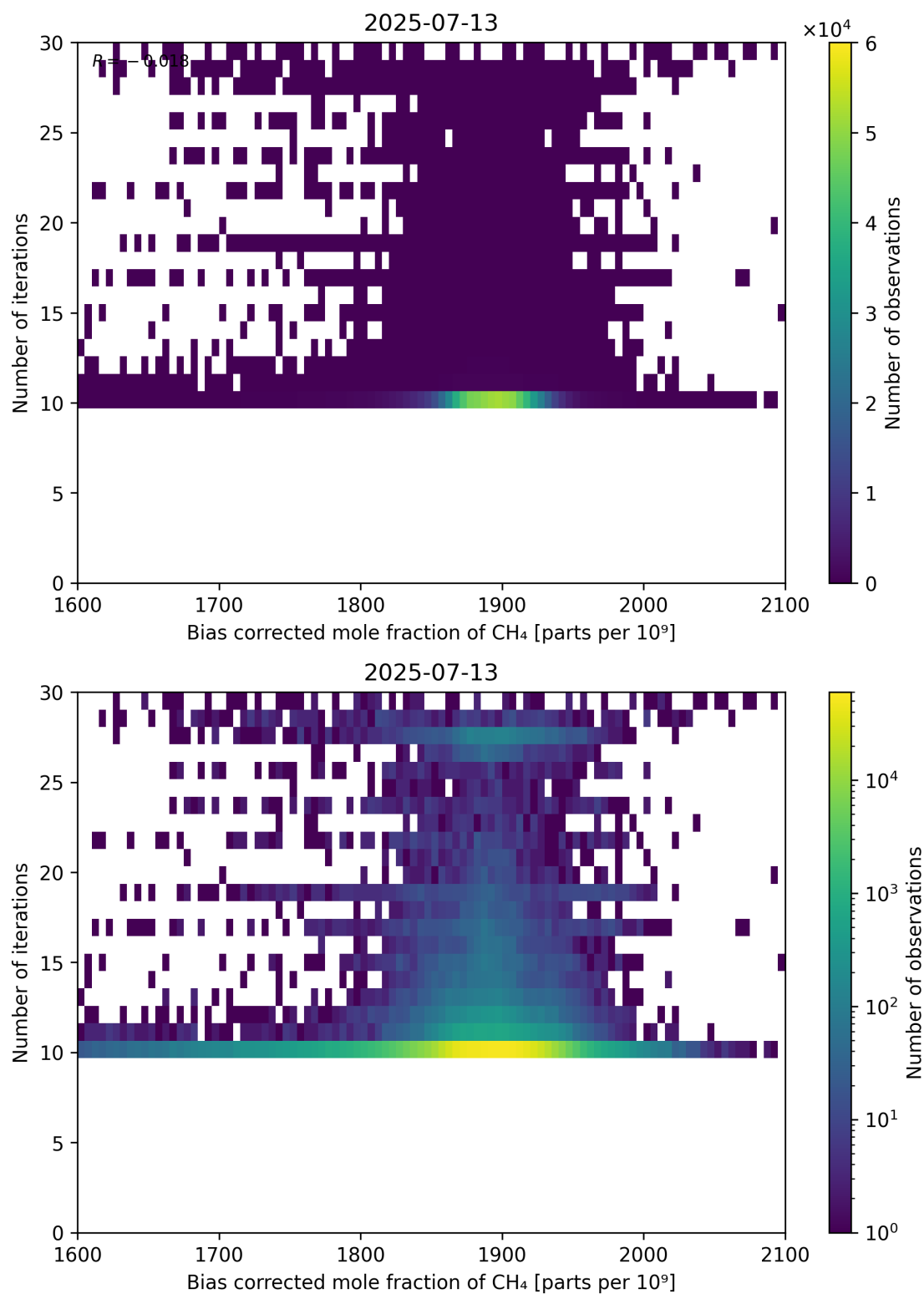
Figure 67: Scatter density plot of “Bias corrected mole fraction of CH 4 ” against “Number of iterations” for 2025-07-13 to 2025-07-14.
