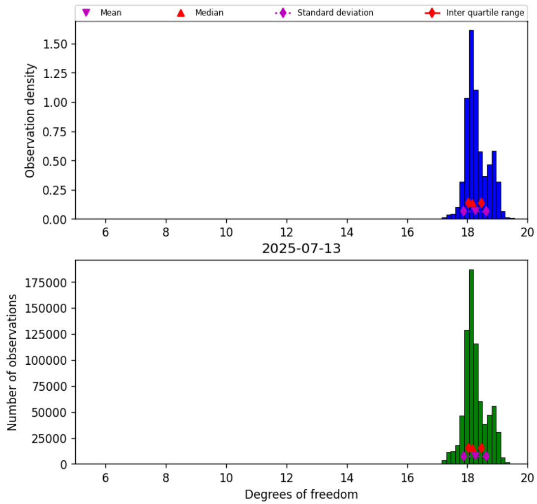
Figure 30: Histogram of “Degrees of freedom” for 2025-07-13 to 2025-07-14
