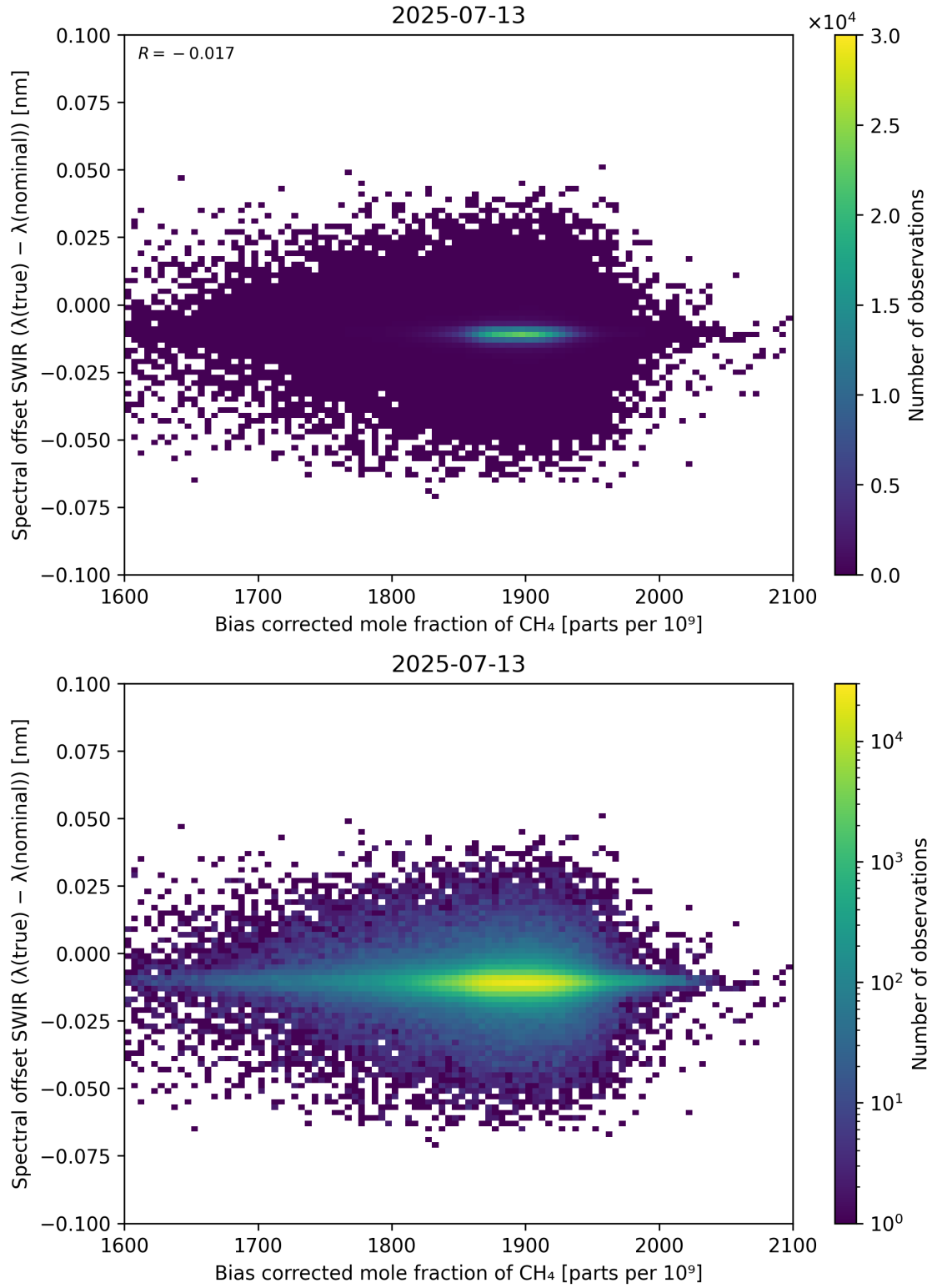
Figure 69: Scatter density plot of “Bias corrected mole fraction of \text{CH}_4 ” against “Spectral offset SWIR ( \lambda_{\text{true}} - \lambda_{\text{nominal}} )” for 2025-07-13 to 2025-07-14.
