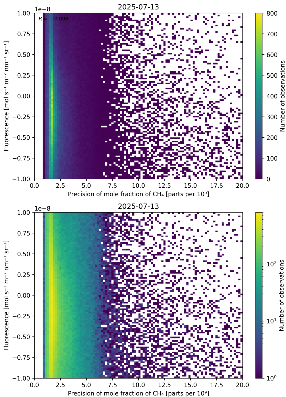
Figure 81: Scatter density plot of “Precision of mole fraction of CH 4 ” against “Fluorescence” for 2025-07-13 to 2025-07-14.
