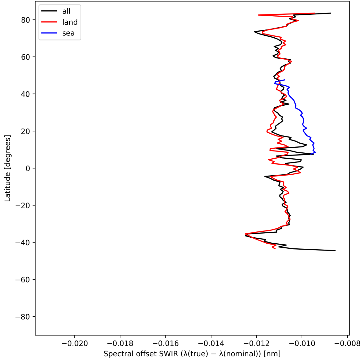
Figure 16: Zonal average of “Spectral offset SWIR ( \lambda_{\text{true}} - \lambda_{\text{nominal}} )” for 2025-07-13 to 2025-07-14.
