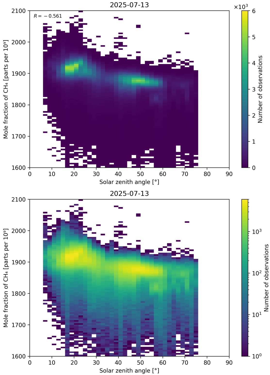
Figure 99: Scatter density plot of “Solar zenith angle” against “Mole fraction of CH 4 ” for 2025-07-13 to 2025-07-14.
