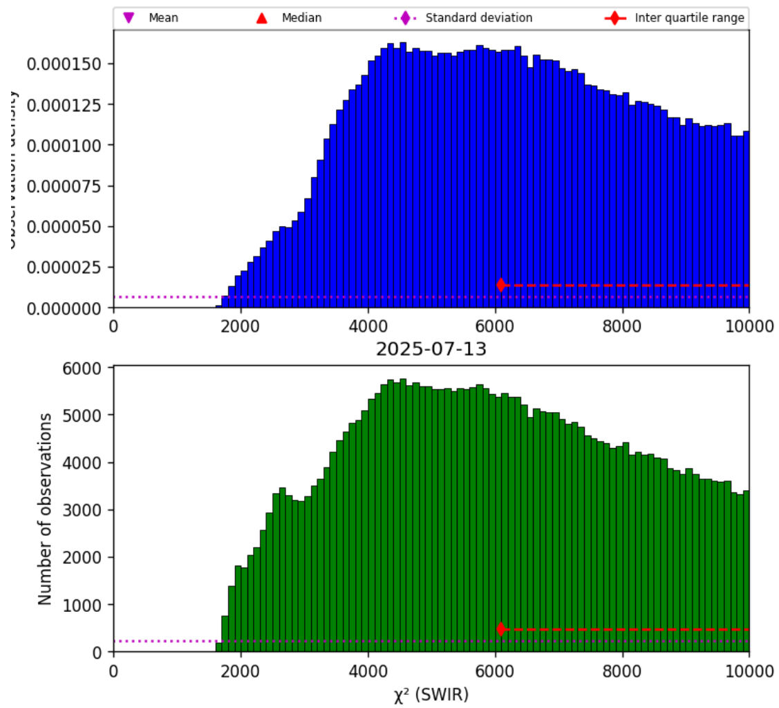
Figure 28: Histogram of “ \chi^2 (SWIR)” for 2025-07-13 to 2025-07-14
