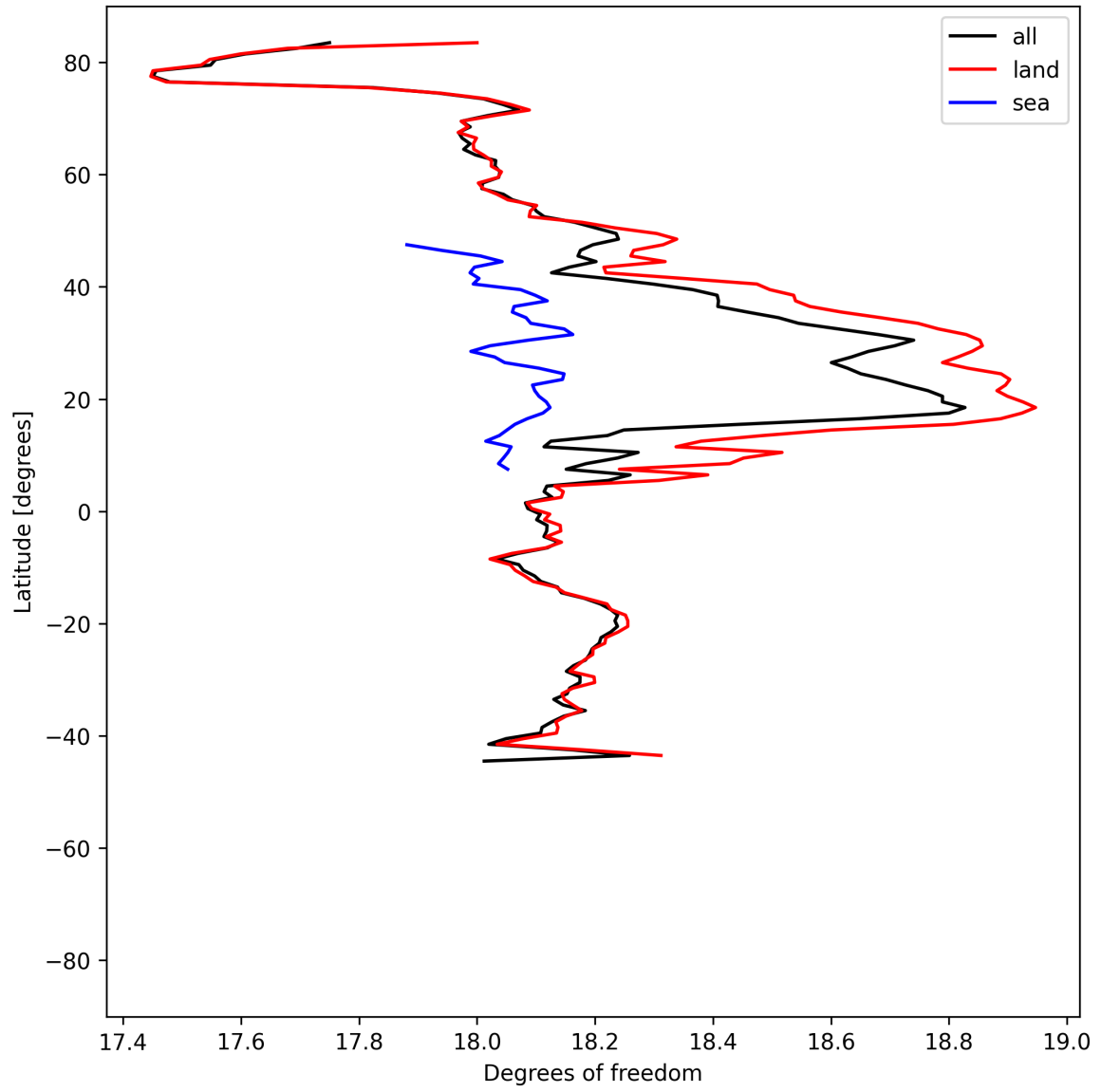
Figure 19: Zonal average of “Degrees of freedom” for 2025-07-13 to 2025-07-14.
