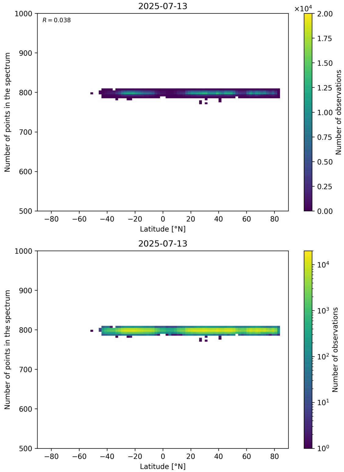
Figure 61: Scatter density plot of “Latitude” against “Number of points in the spectrum” for 2025-07-13 to 2025-07-14.
