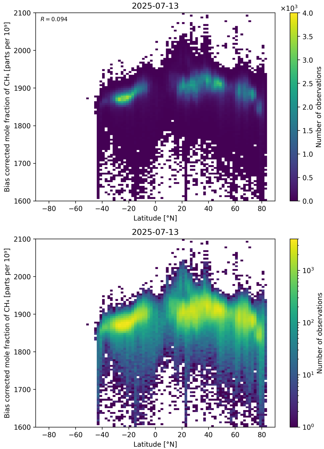
Figure 58: Scatter density plot of “Latitude” against “Bias corrected mole fraction of \text{CH}_4 ” for 2025-07-13 to 2025-07-14.
