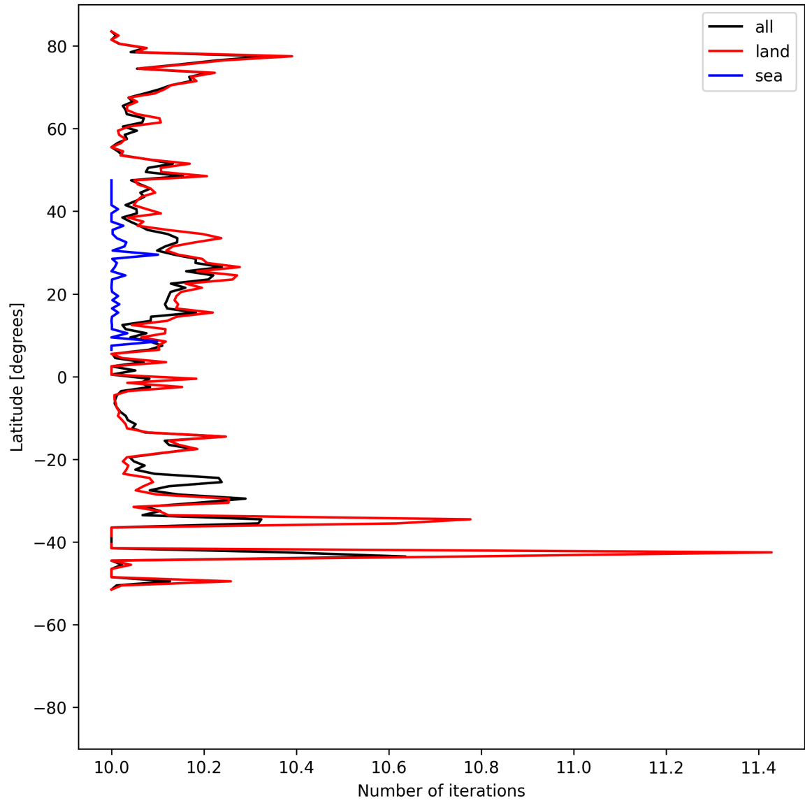
Figure 20: Zonal average of “Number of iterations” for 2025-07-14 to 2025-07-16.
