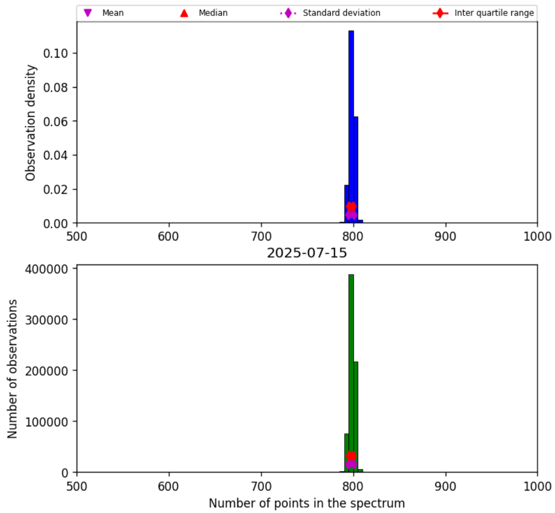
Figure 26: Histogram of “Number of points in the spectrum” for 2025-07-14 to 2025-07-16
