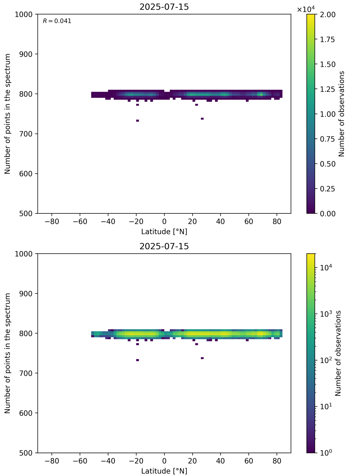
Figure 61: Scatter density plot of “Latitude” against “Number of points in the spectrum” for 2025-07-14 to 2025-07-16.
