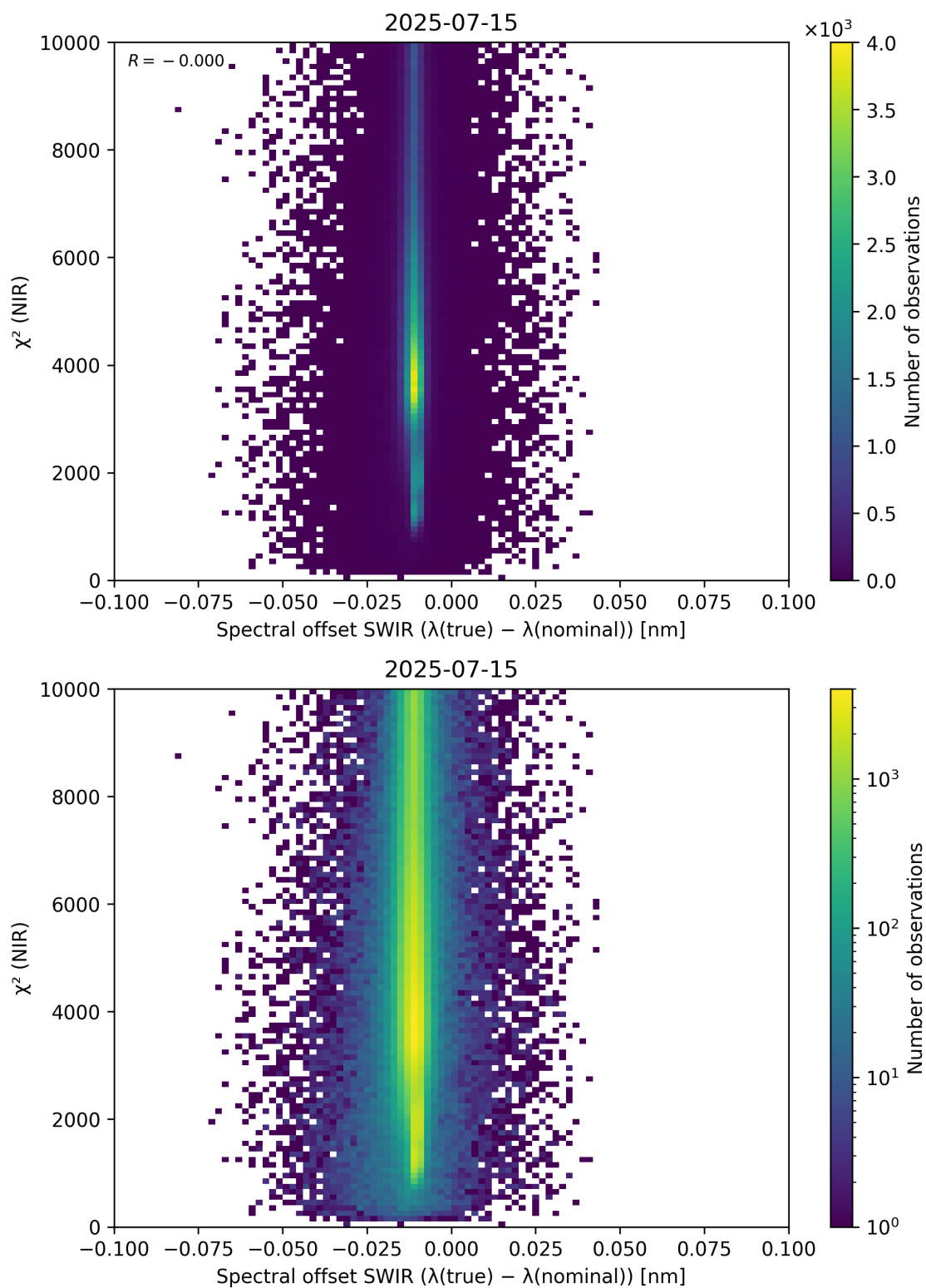
Figure 117: Scatter density plot of “Spectral offset SWIR ( \lambda_{\text{true}} - \lambda_{\text{nominal}} )” against “ \chi^2 (NIR)” for 2025-07-14 to 2025-07-16.
