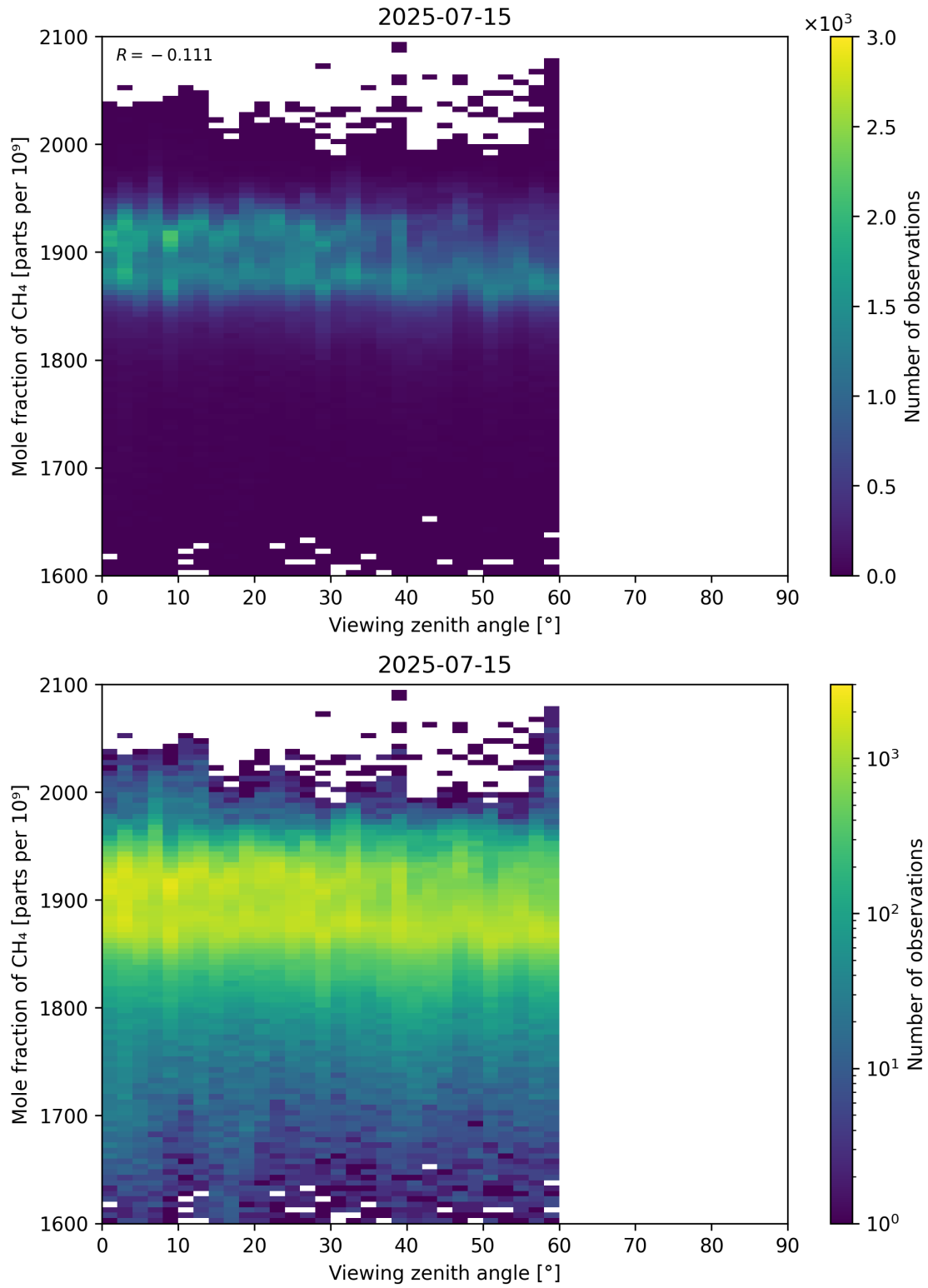
Figure 110: Scatter density plot of “Viewing zenith angle” against “Mole fraction of CH 4 ” for 2025-07-14 to 2025-07-16.
