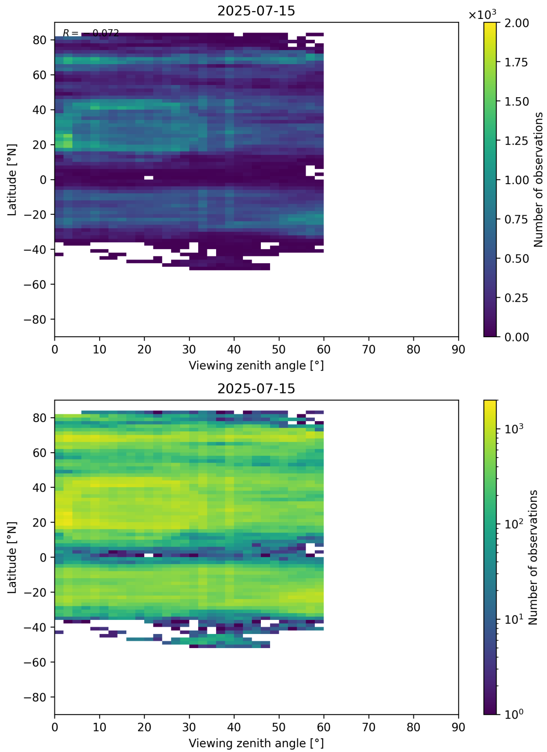
Figure 109: Scatter density plot of “Viewing zenith angle” against “Latitude” for 2025-07-14 to 2025-07-16.
