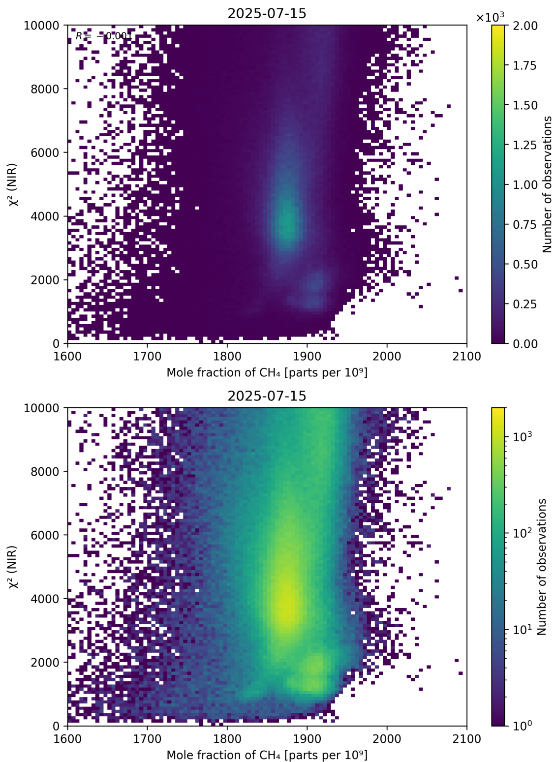
Figure 70: Scatter density plot of “Mole fraction of \text{CH}_4 ” against “ \chi^2 (NIR)” for 2025-07-14 to 2025-07-16.
