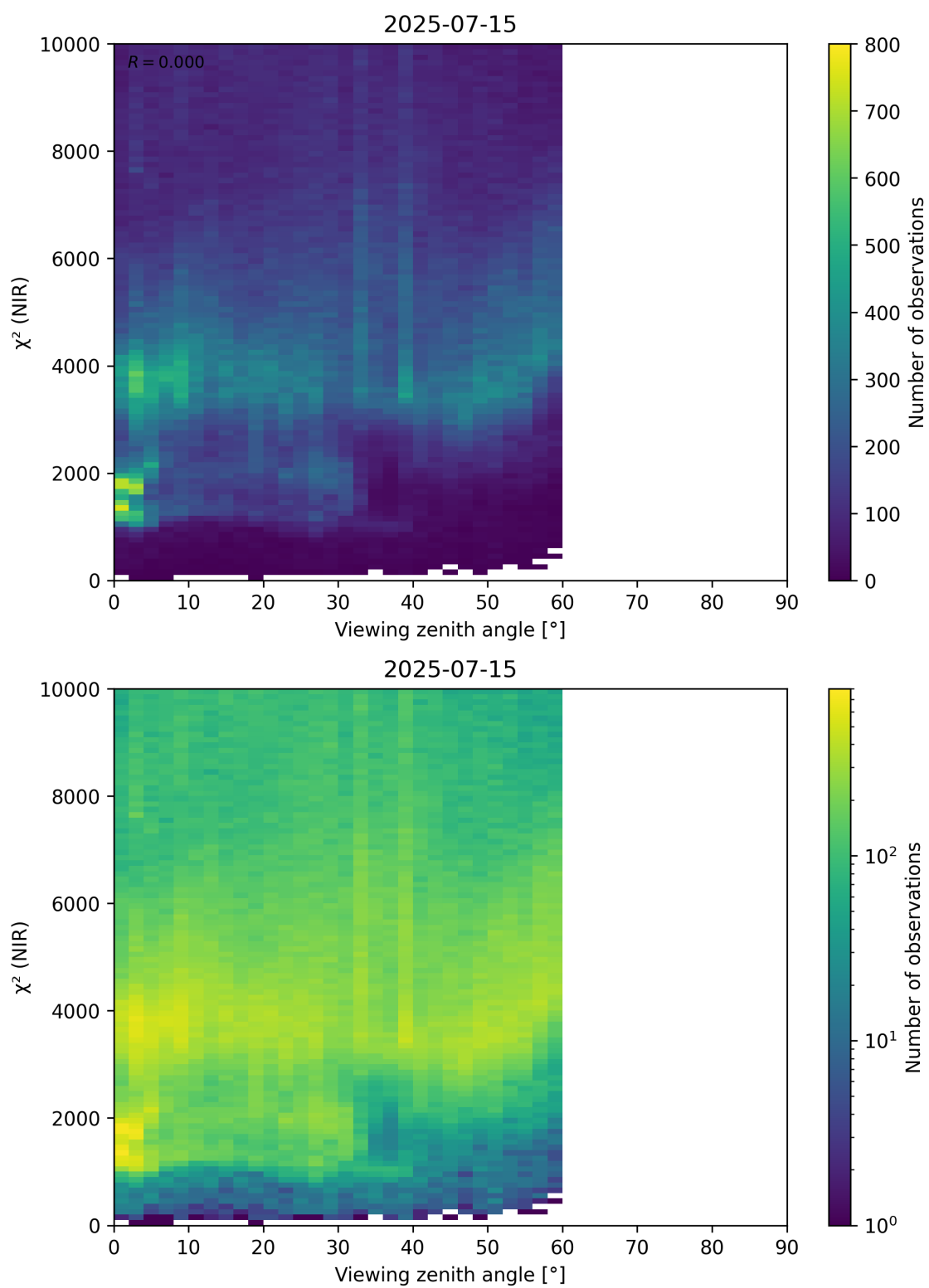
Figure 105: Scatter density plot of “Viewing zenith angle” against “ \chi^2 (NIR)” for 2025-07-14 to 2025-07-16.
