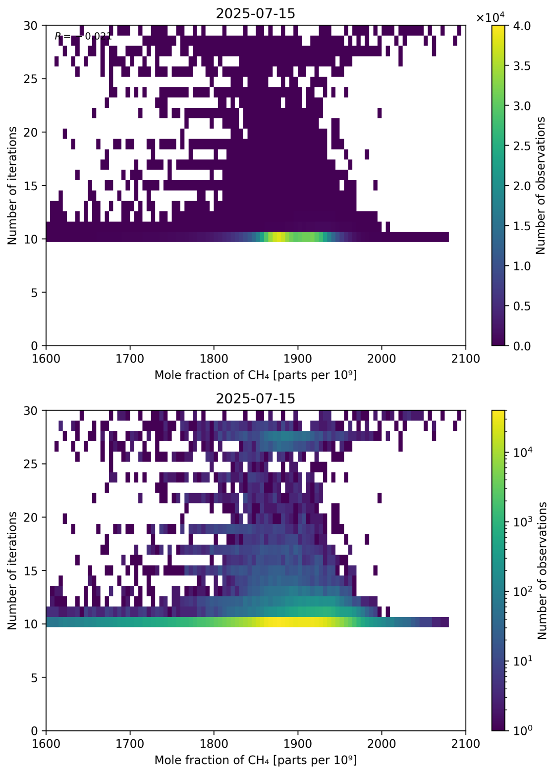
Figure 76: Scatter density plot of “Mole fraction of CH 4 ” against “Number of iterations” for 2025-07-14 to 2025-07-16.
