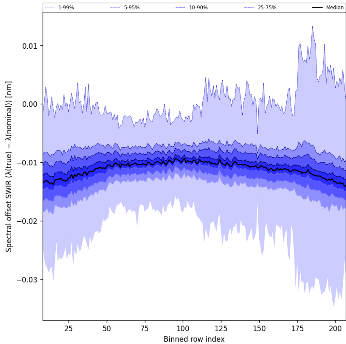
Figure 38: Along track statistics of “Spectral offset SWIR ( \lambda_{\text{true}} - \lambda_{\text{nominal}} )” for 2025-07-14 to 2025-07-16
