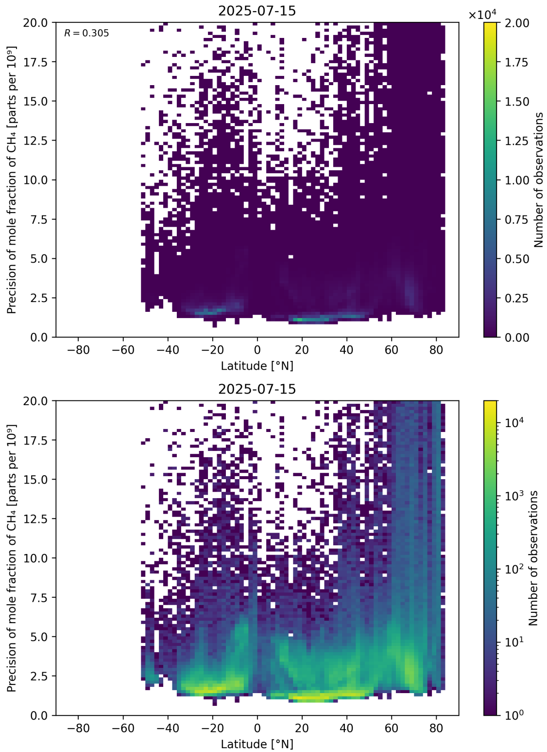
Figure 59: Scatter density plot of “Latitude” against “Precision of mole fraction of \text{CH}_4 ” for 2025-07-14 to 2025-07-16.
