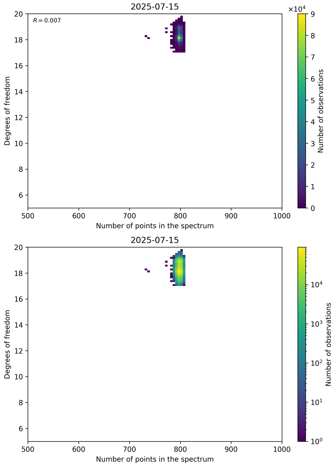
Figure 90: Scatter density plot of “Number of points in the spectrum” against “Degrees of freedom” for 2025-07-14 to 2025-07-16.
