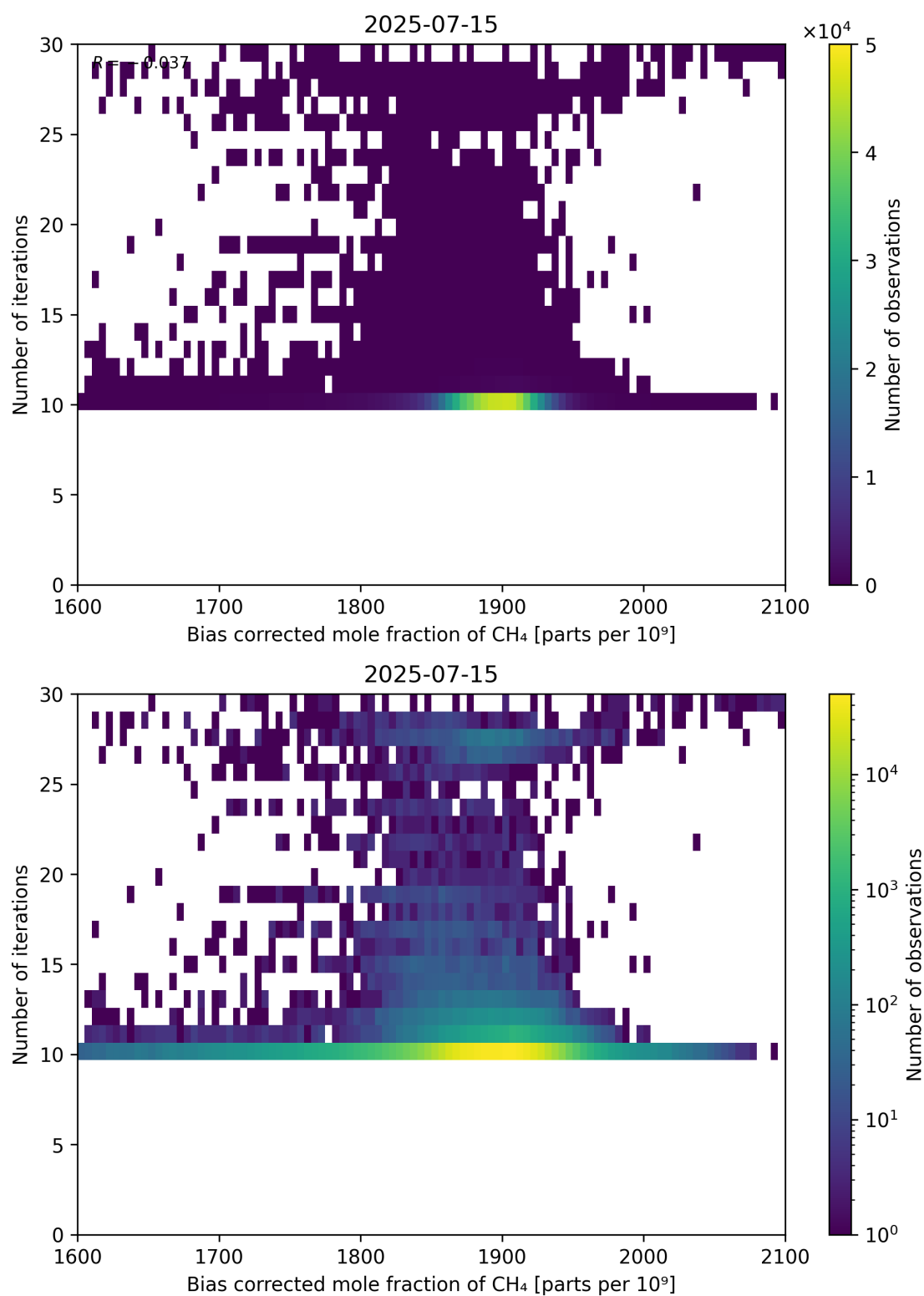
Figure 67: Scatter density plot of “Bias corrected mole fraction of CH 4 ” against “Number of iterations” for 2025-07-14 to 2025-07-16.
