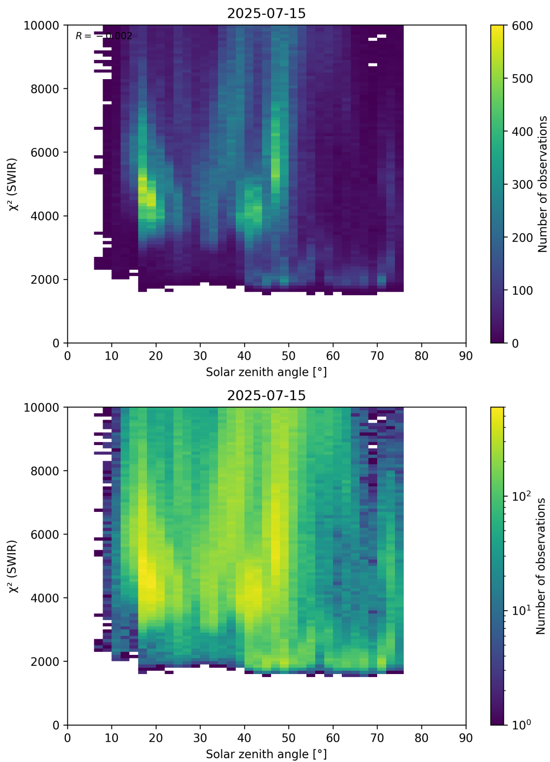
Figure 95: Scatter density plot of “Solar zenith angle” against “ \chi^2 (SWIR)” for 2025-07-14 to 2025-07-16.
