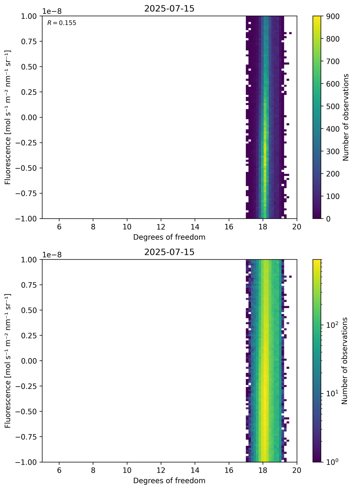
Figure 51: Scatter density plot of “Degrees of freedom” against “Fluorescence” for 2025-07-14 to 2025-07-16.
