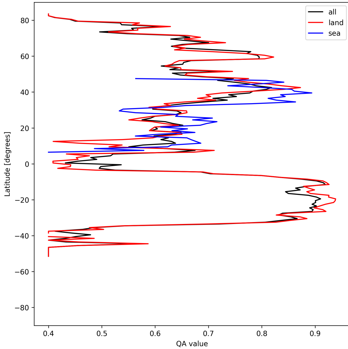
Figure 11: Zonal average of “QA value” for 2025-07-14 to 2025-07-16.
