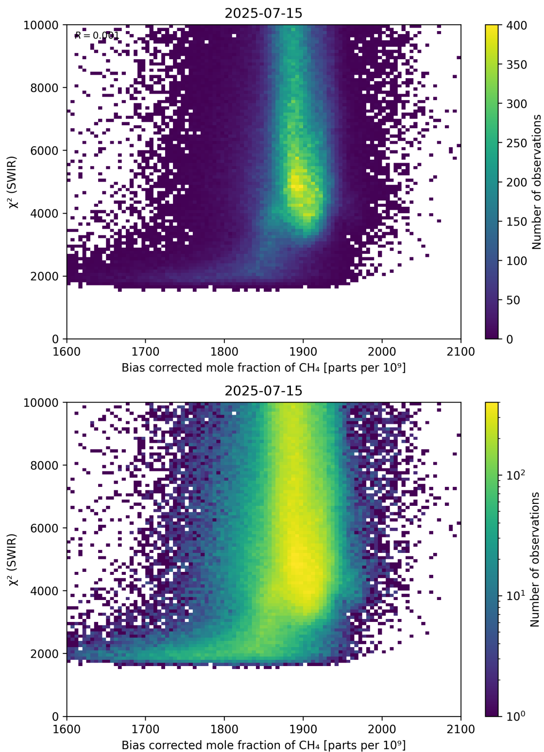
Figure 64: Scatter density plot of “Bias corrected mole fraction of \text{CH}_4 ” against “ \chi^2 (SWIR)” for 2025-07-14 to 2025-07-16.
