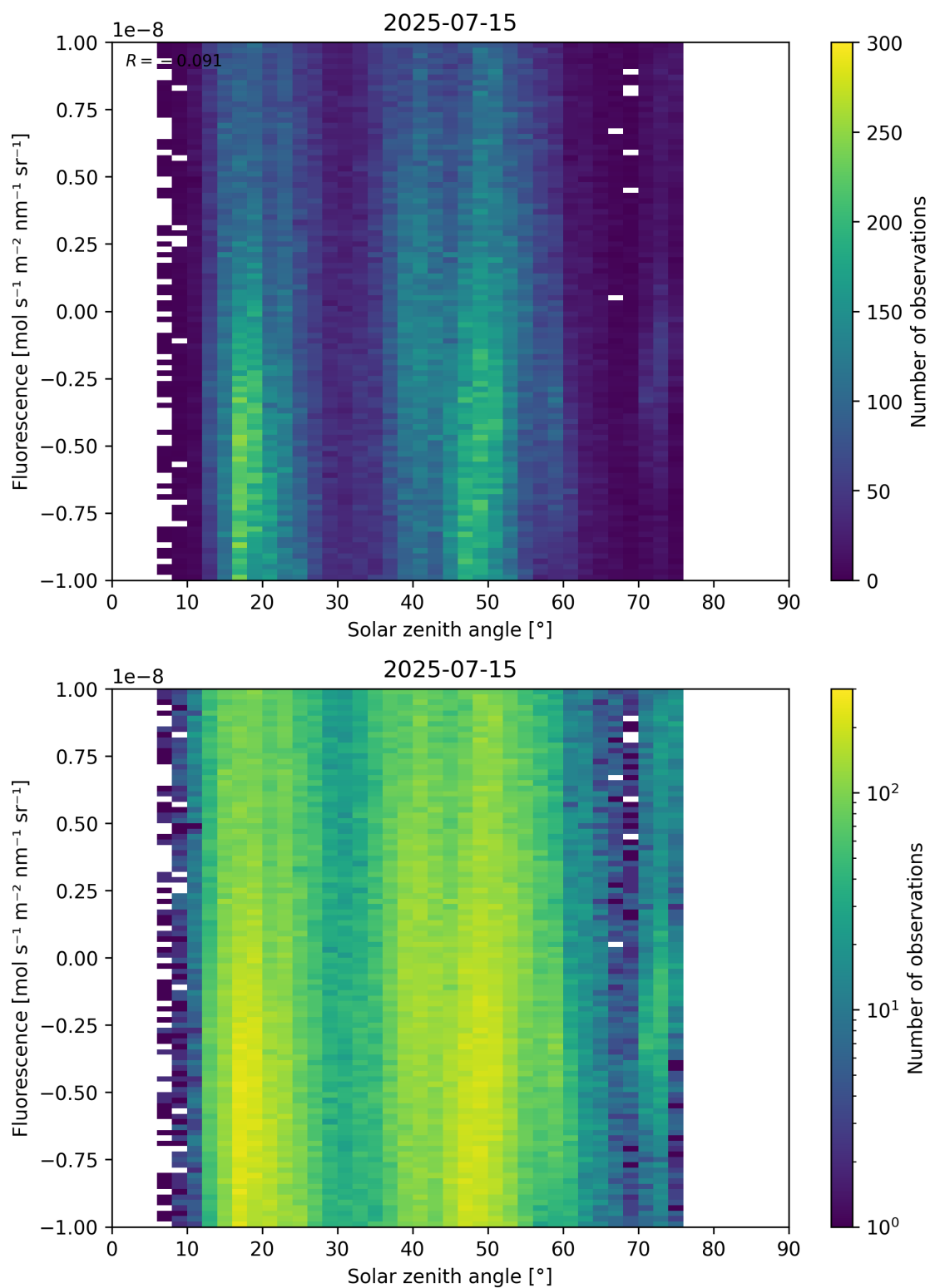
Figure 97: Scatter density plot of “Solar zenith angle” against “Fluorescence” for 2025-07-14 to 2025-07-16.
