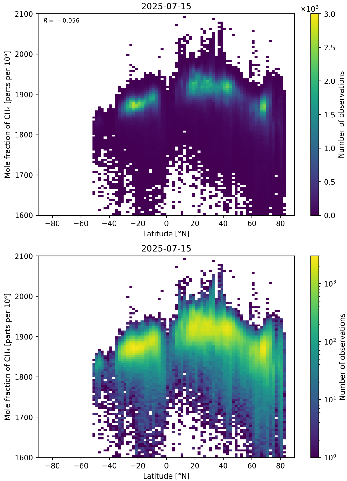
Figure 57: Scatter density plot of “Latitude” against “Mole fraction of CH 4 ” for 2025-07-14 to 2025-07-16.
