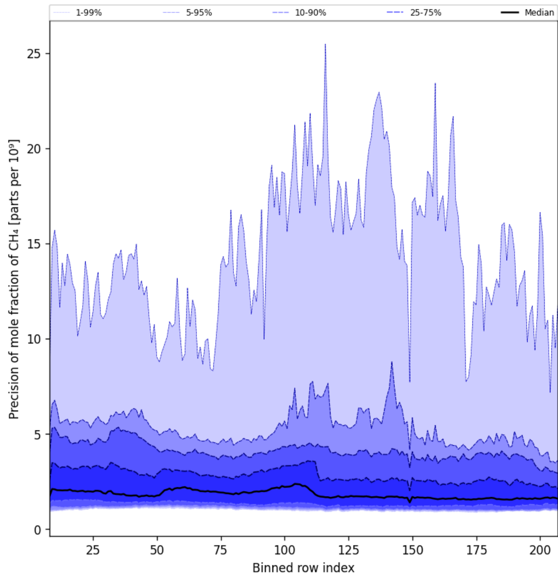
Figure 35: Along track statistics of “Precision of mole fraction of CH 4 ” for 2025-07-14 to 2025-07-16
