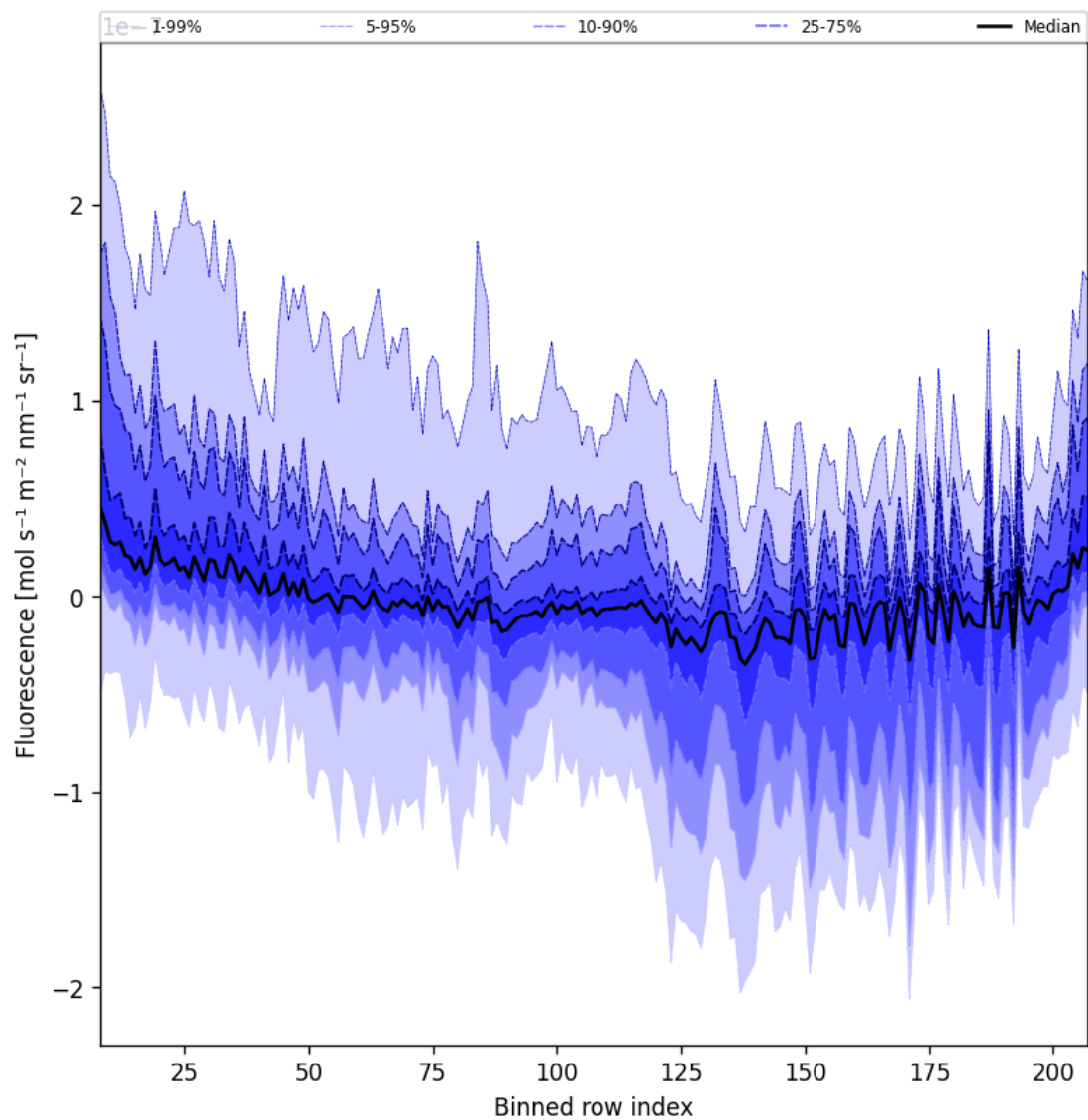
Figure 43: Along track statistics of “Fluorescence” for 2025-07-14 to 2025-07-16
