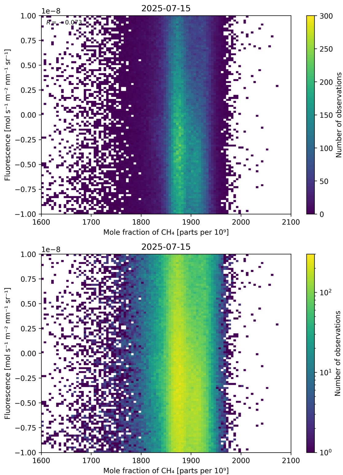
Figure 73: Scatter density plot of “Mole fraction of \text{CH}_4 ” against “Fluorescence” for 2025-07-14 to 2025-07-16.
