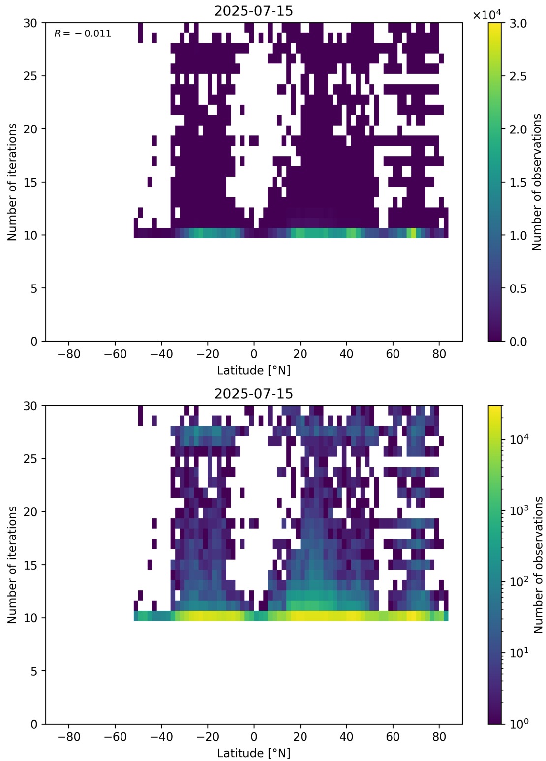
Figure 60: Scatter density plot of “Latitude” against “Number of iterations” for 2025-07-14 to 2025-07-16.
