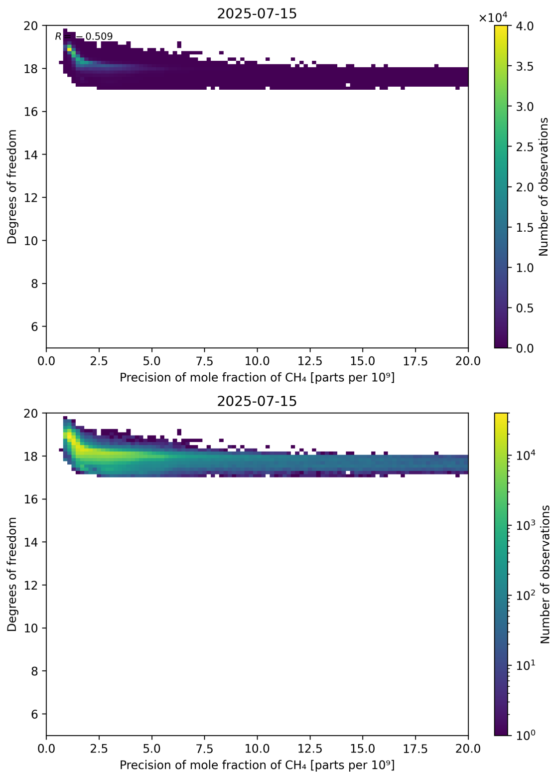
Figure 80: Scatter density plot of “Precision of mole fraction of CH 4 ” against “Degrees of freedom” for 2025-07-14 to 2025-07-16.
