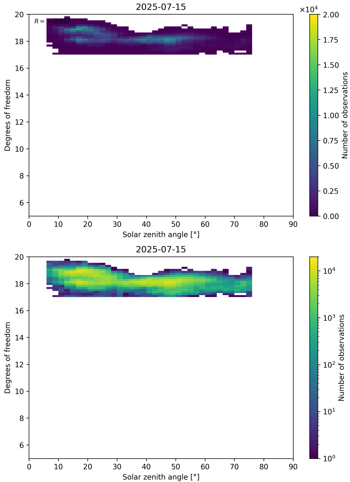
Figure 96: Scatter density plot of “Solar zenith angle” against “Degrees of freedom” for 2025-07-14 to 2025-07-16.
