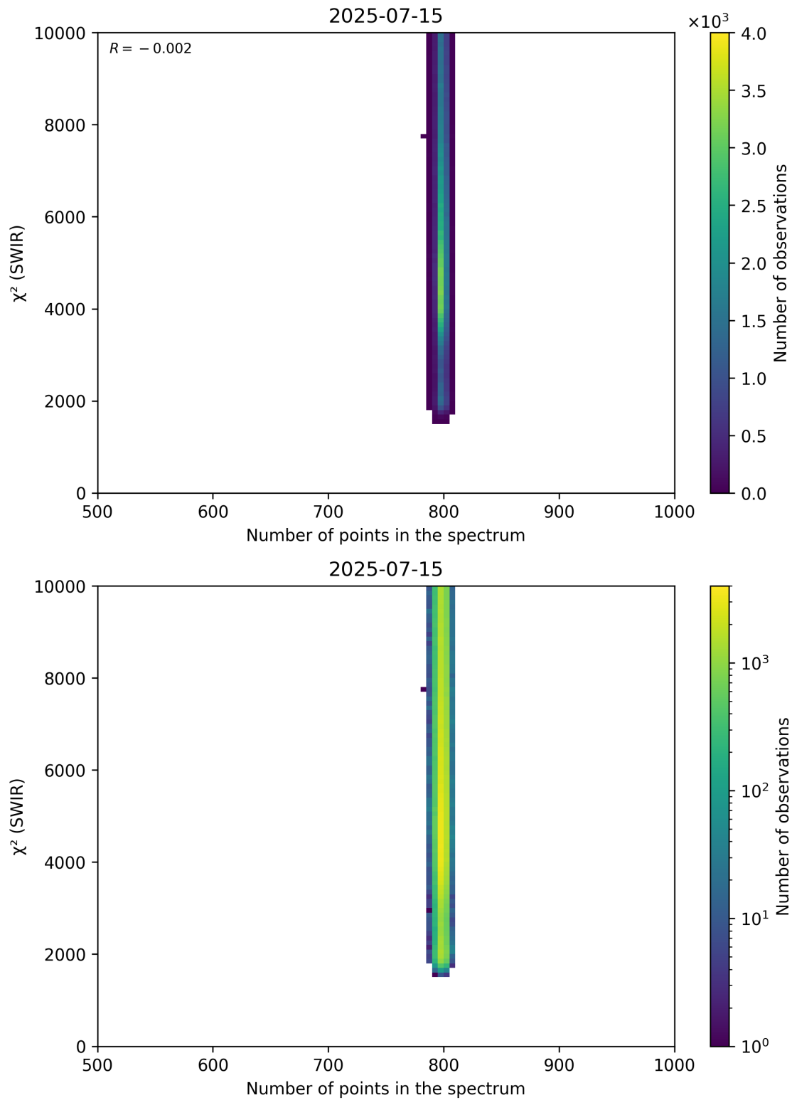
Figure 89: Scatter density plot of “Number of points in the spectrum” against “ \chi^2 (SWIR)” for 2025-07-14 to 2025-07-16.
