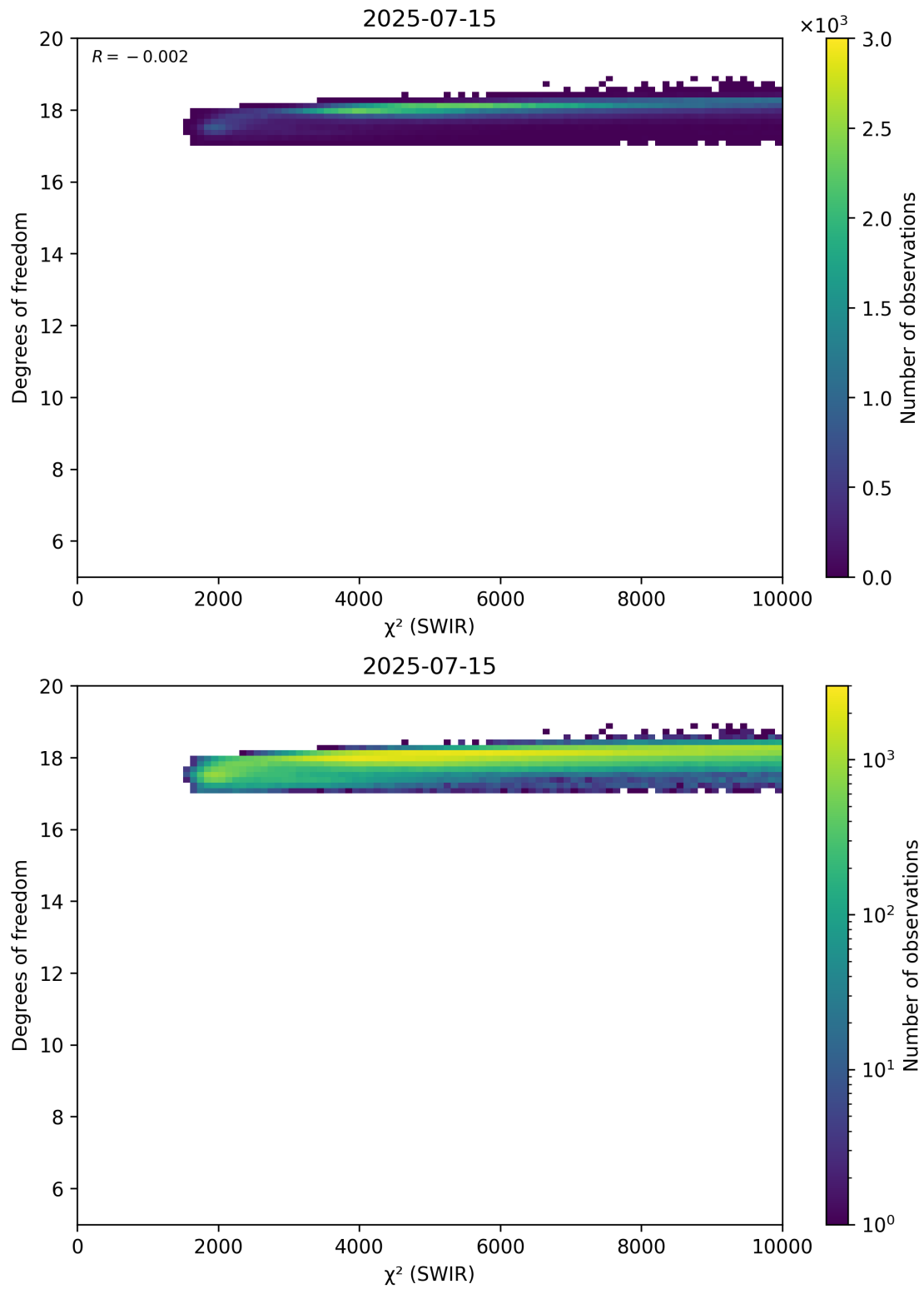
Figure 48: Scatter density plot of “ \chi^2 (SWIR)” against “Degrees of freedom” for 2025-07-14 to 2025-07-16.
