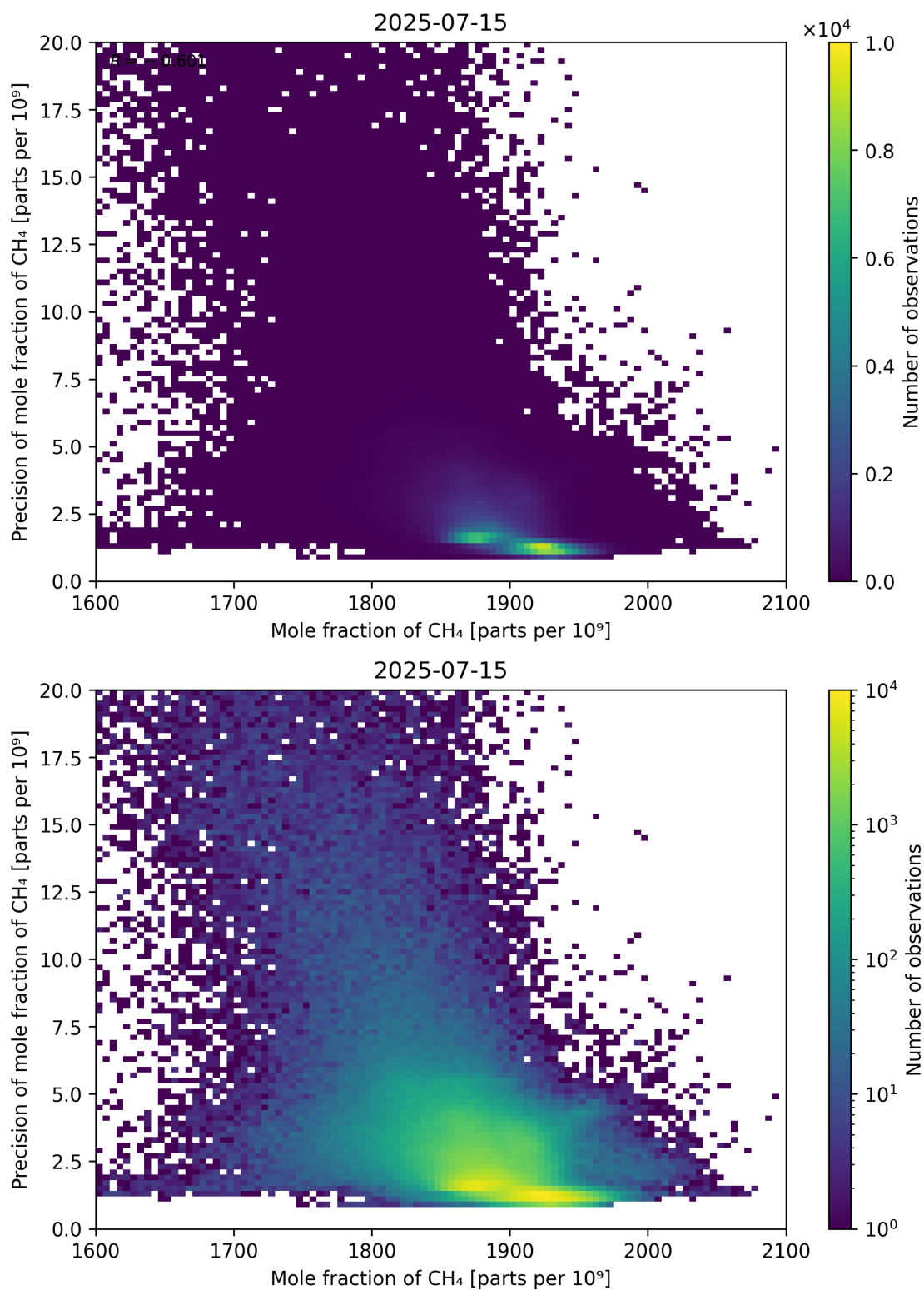
Figure 75: Scatter density plot of “Mole fraction of CH 4 ” against “Precision of mole fraction of CH 4 ” for 2025-07-14 to 2025-07-16.
