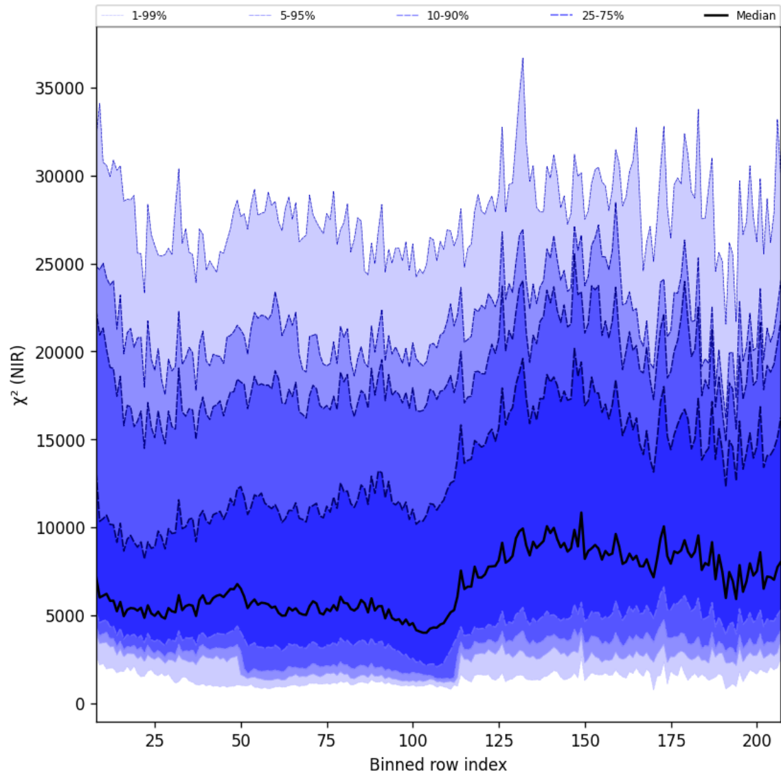
Figure 40: Along track statistics of “ \chi^2 (NIR)” for 2025-07-14 to 2025-07-16
