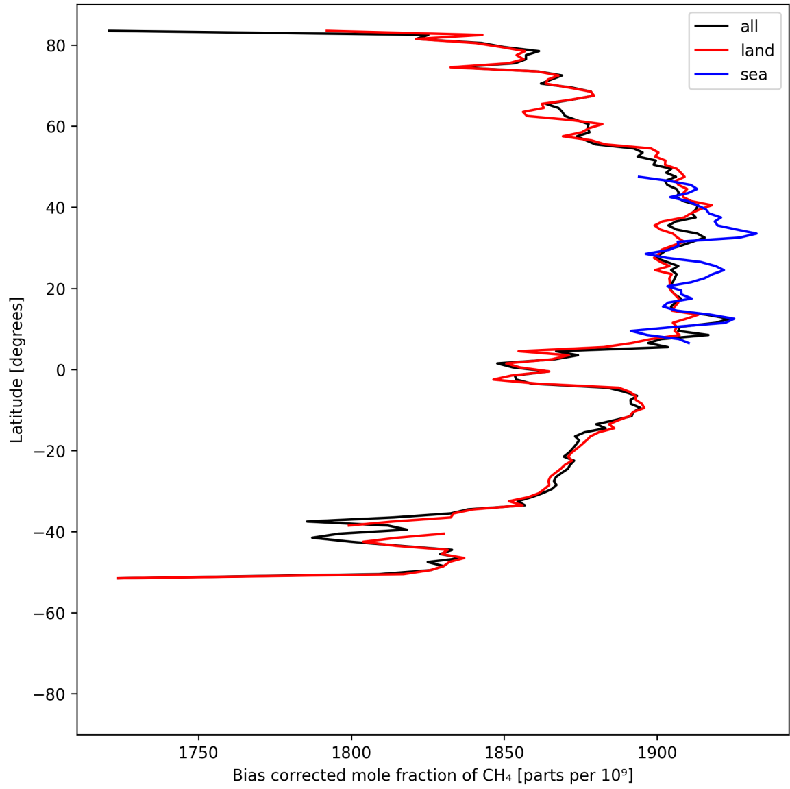
Figure 14: Zonal average of “Bias corrected mole fraction of \text{CH}_4 ” for 2025-07-14 to 2025-07-16.
