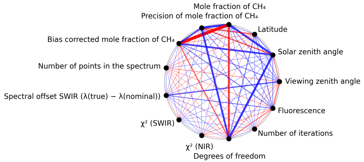
Figure 1: Map of correlation graph for 2025-07-14 to 2025-07-16.
