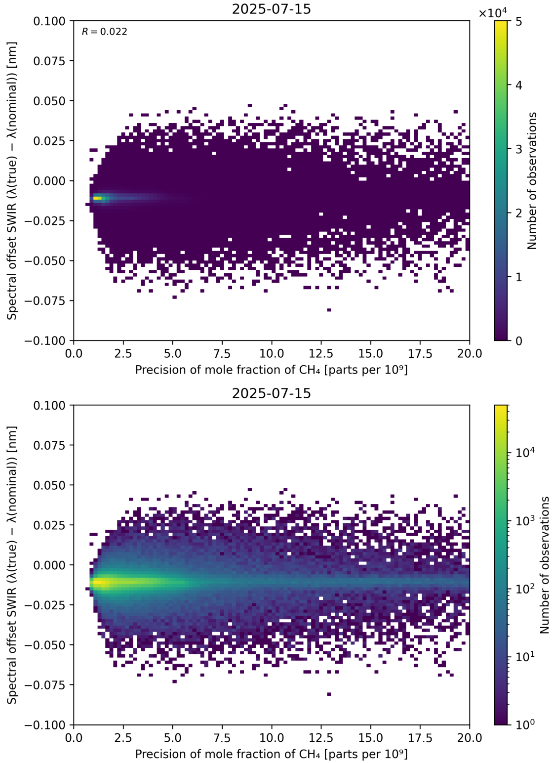
Figure 85: Scatter density plot of “Precision of mole fraction of CH 4 ” against “Spectral offset SWIR ( \lambda_{\text{true}} - \lambda_{\text{nominal}} )” for 2025-07-14 to 2025-07-16.
