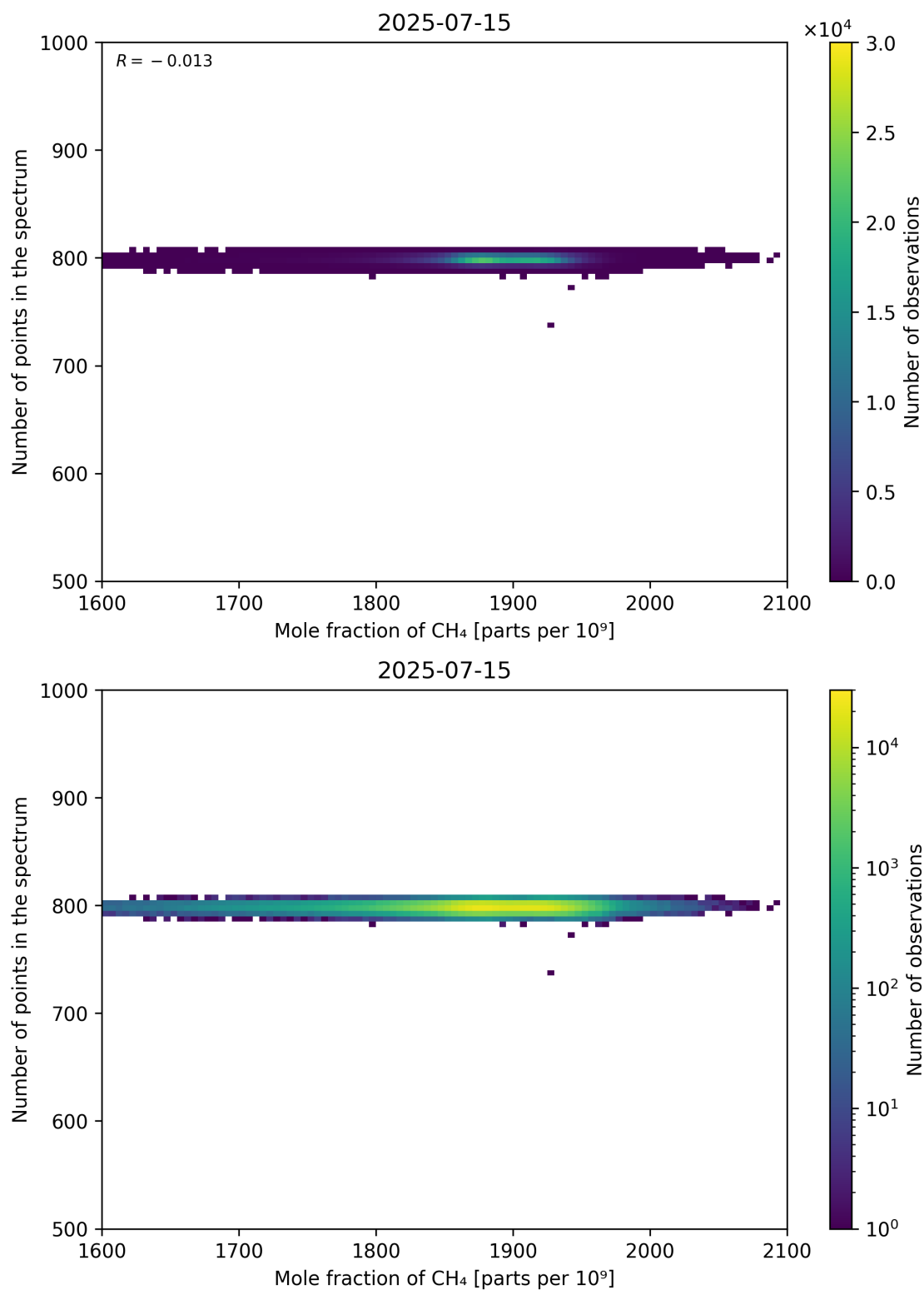
Figure 77: Scatter density plot of “Mole fraction of CH 4 ” against “Number of points in the spectrum” for 2025-07-14 to 2025-07-16.
