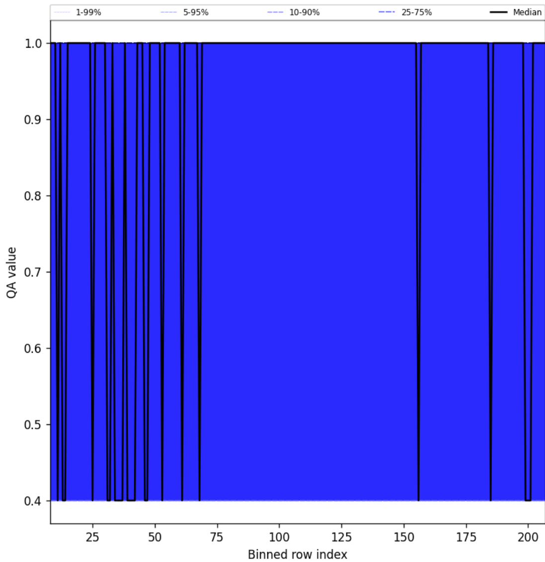
Figure 33: Along track statistics of “QA value” for 2025-07-14 to 2025-07-16
