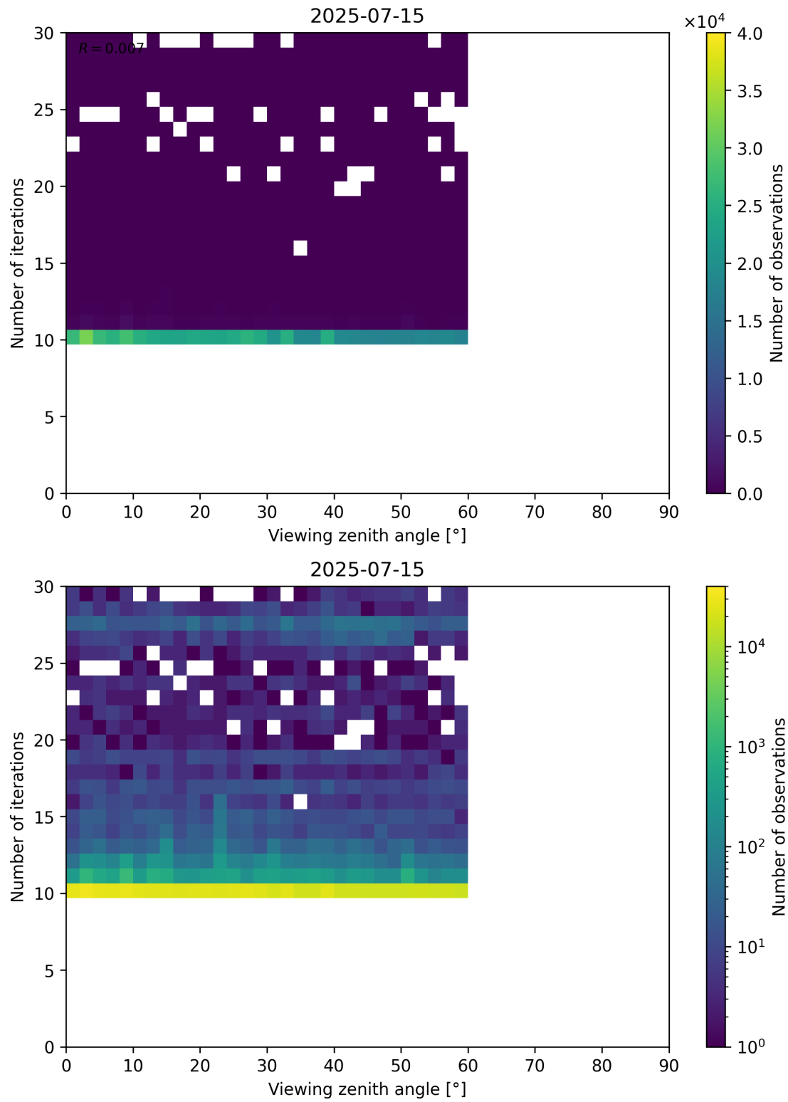
Figure 113: Scatter density plot of “Viewing zenith angle” against “Number of iterations” for 2025-07-14 to 2025-07-16.
