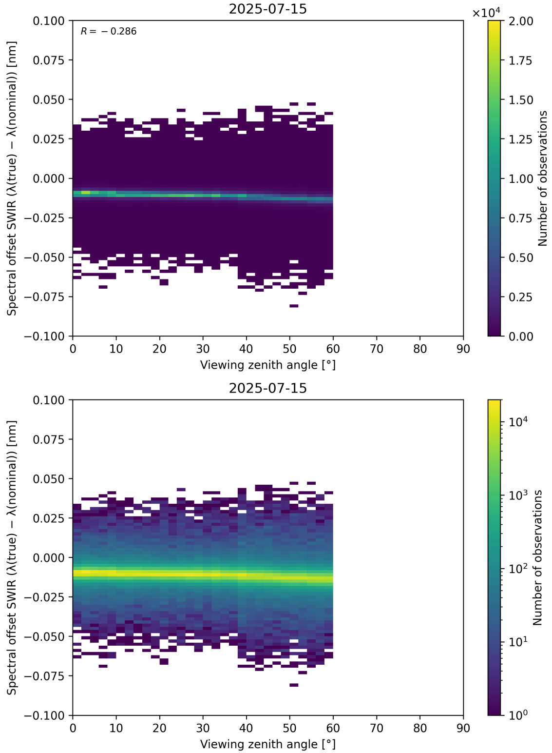
Figure 116: Scatter density plot of “Viewing zenith angle” against “Spectral offset SWIR ( \lambda_{\text{true}} - \lambda_{\text{nominal}} )” for 2025-07-14 to 2025-07-16.
