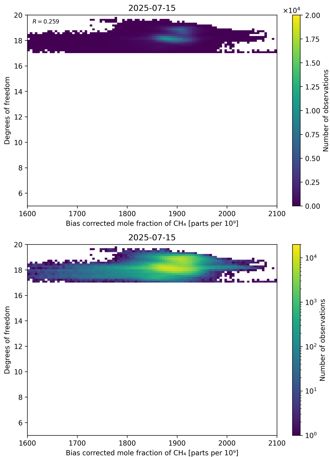
Figure 65: Scatter density plot of “Bias corrected mole fraction of CH 4 ” against “Degrees of freedom” for 2025-07-14 to 2025-07-16.
