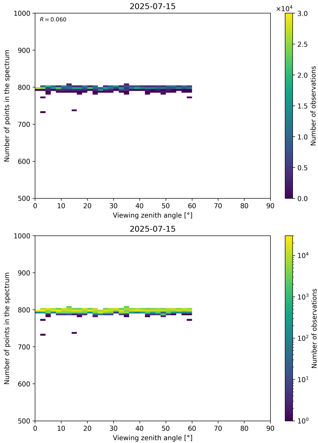
Figure 114: Scatter density plot of “Viewing zenith angle” against “Number of points in the spectrum” for 2025-07-14 to 2025-07-16.
