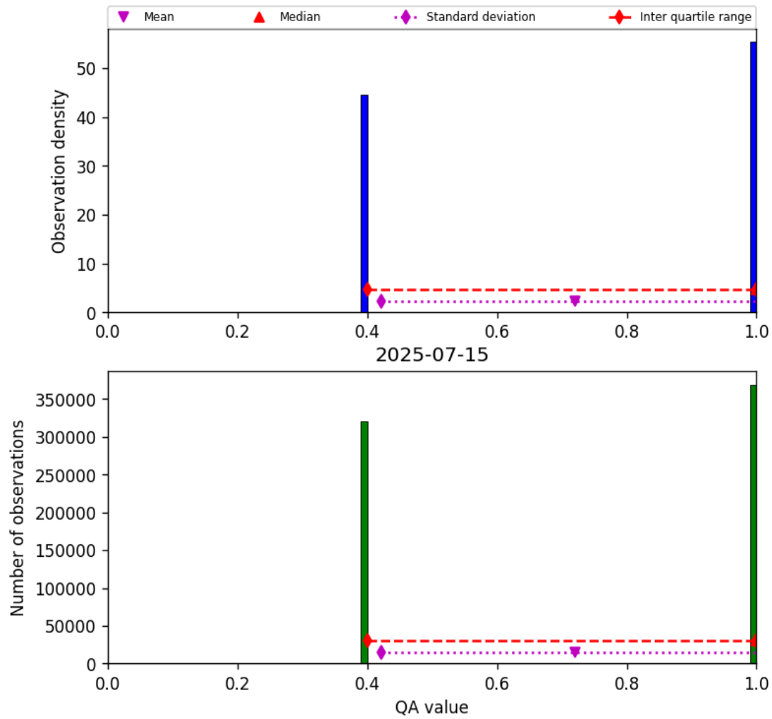
Figure 22: Histogram of “QA value” for 2025-07-14 to 2025-07-16
