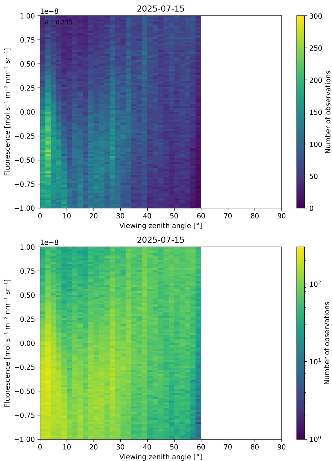
Figure 108: Scatter density plot of “Viewing zenith angle” against “Fluorescence” for 2025-07-14 to 2025-07-16.
