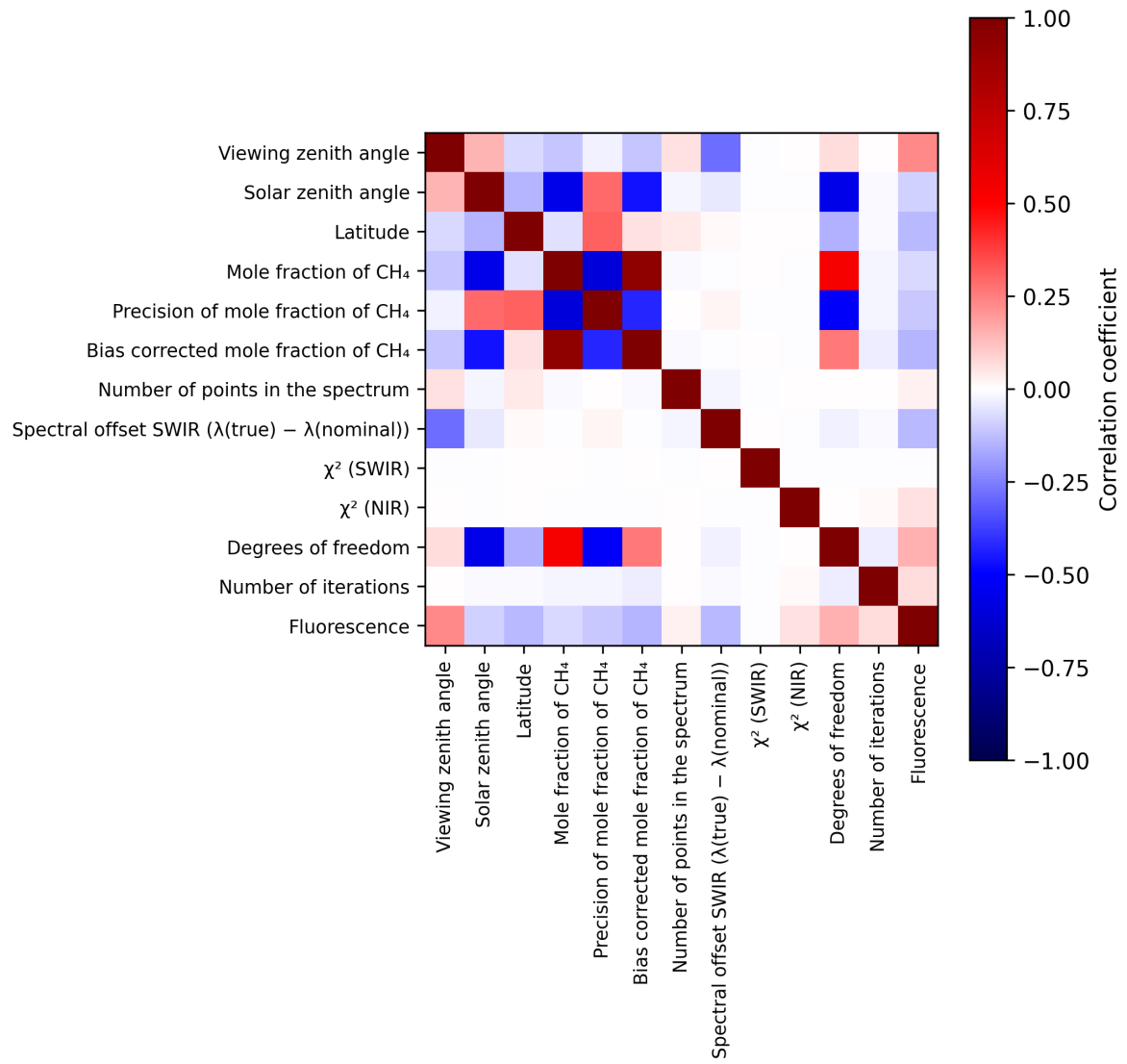
Figure 2: Map of correlation matrix for 2025-07-14 to 2025-07-16.
