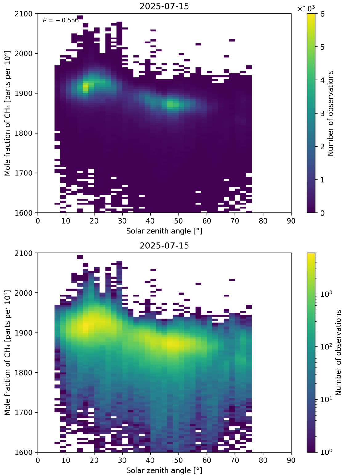
Figure 99: Scatter density plot of “Solar zenith angle” against “Mole fraction of CH 4 ” for 2025-07-14 to 2025-07-16.
