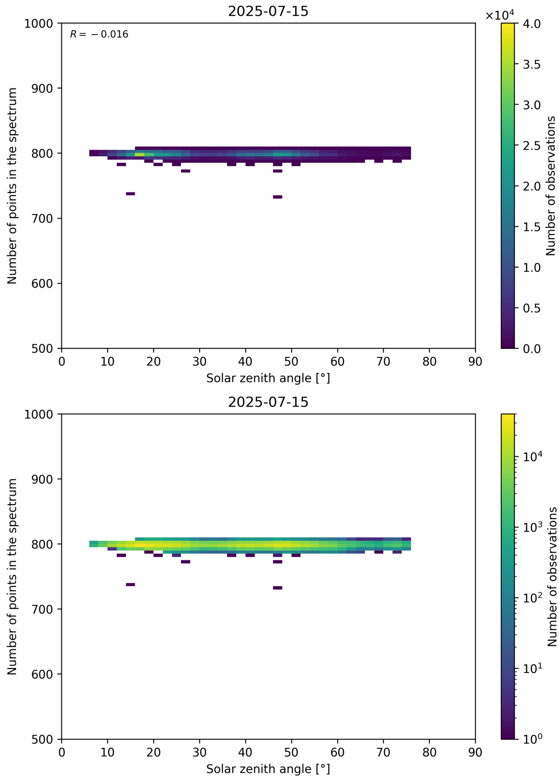
Figure 103: Scatter density plot of “Solar zenith angle” against “Number of points in the spectrum” for 2025-07-14 to 2025-07-16.
