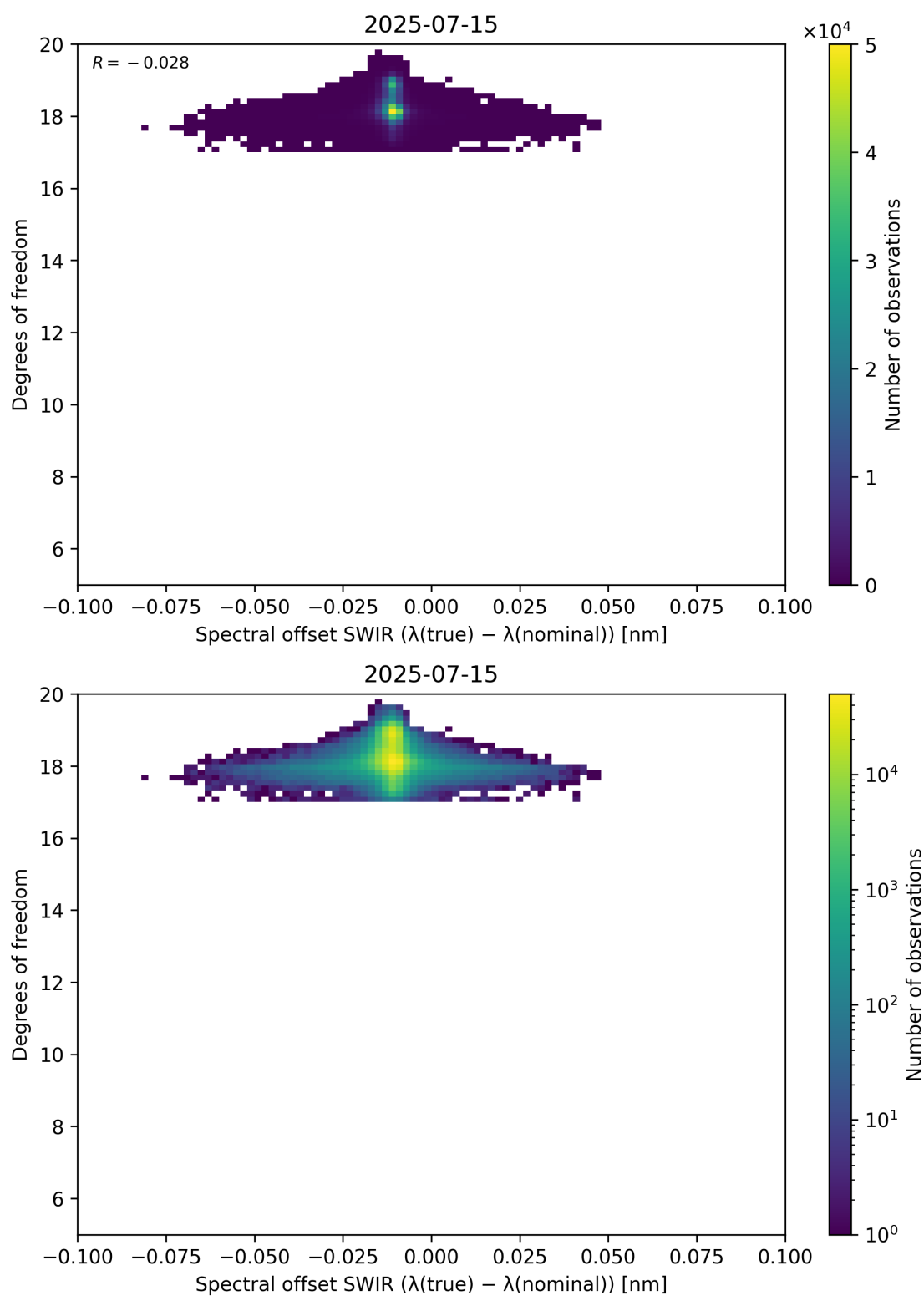
Figure 119: Scatter density plot of “Spectral offset SWIR ( \lambda_{\text{true}} - \lambda_{\text{nominal}} )” against “Degrees of freedom” for 2025-07-14 to 2025-07-16.
