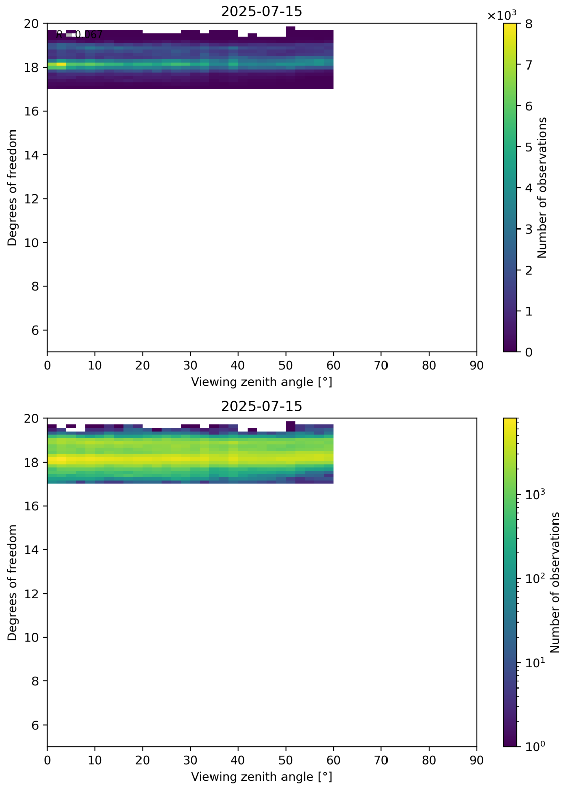
Figure 107: Scatter density plot of “Viewing zenith angle” against “Degrees of freedom” for 2025-07-14 to 2025-07-16.
