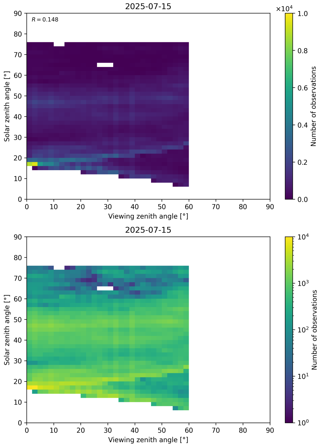
Figure 115: Scatter density plot of “Viewing zenith angle” against “Solar zenith angle” for 2025-07-14 to 2025-07-16.
