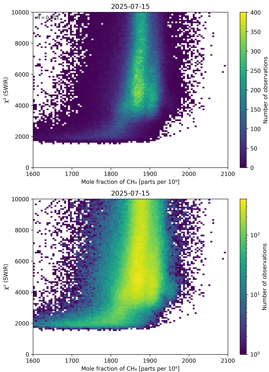
Figure 71: Scatter density plot of “Mole fraction of CH 4 ” against “ \chi^2 (SWIR)” for 2025-07-14 to 2025-07-16.
