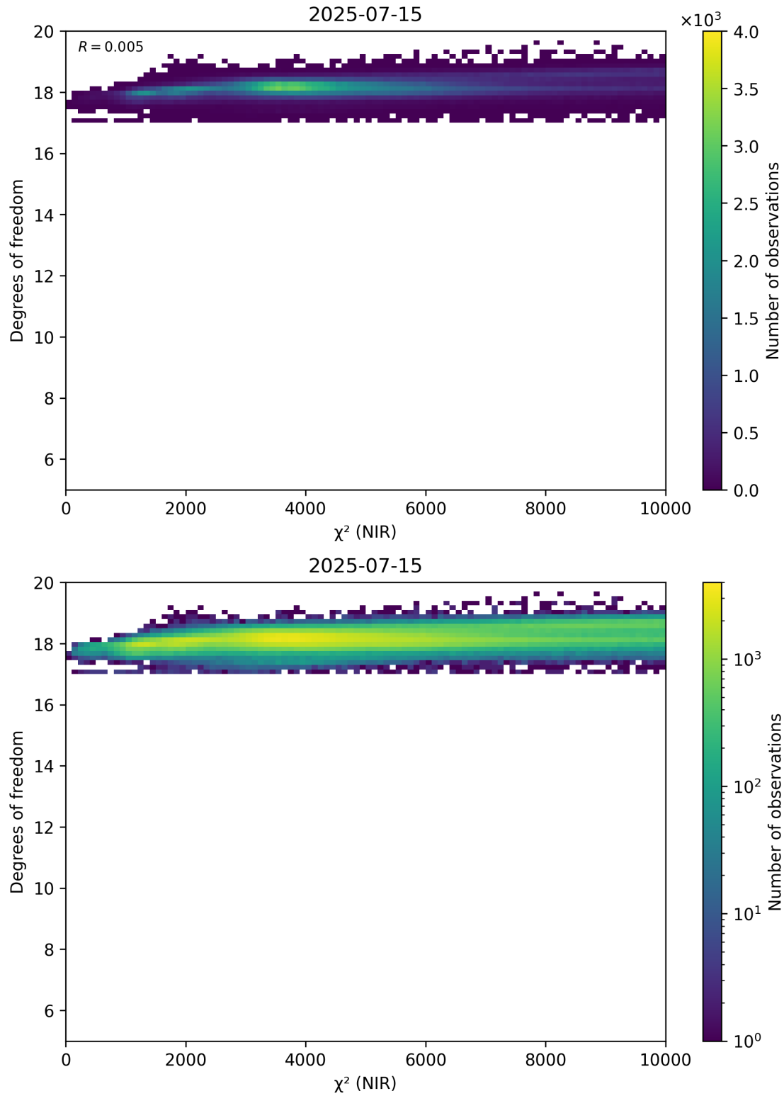
Figure 44: Scatter density plot of “ \chi^2 (NIR)” against “Degrees of freedom” for 2025-07-14 to 2025-07-16.
