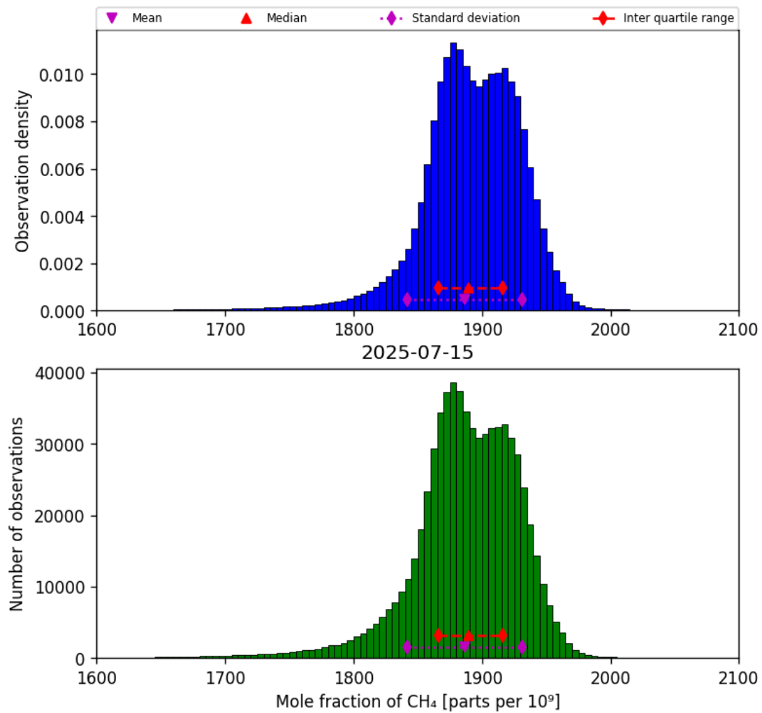
Figure 23: Histogram of “Mole fraction of CH 4 ” for 2025-07-14 to 2025-07-16
