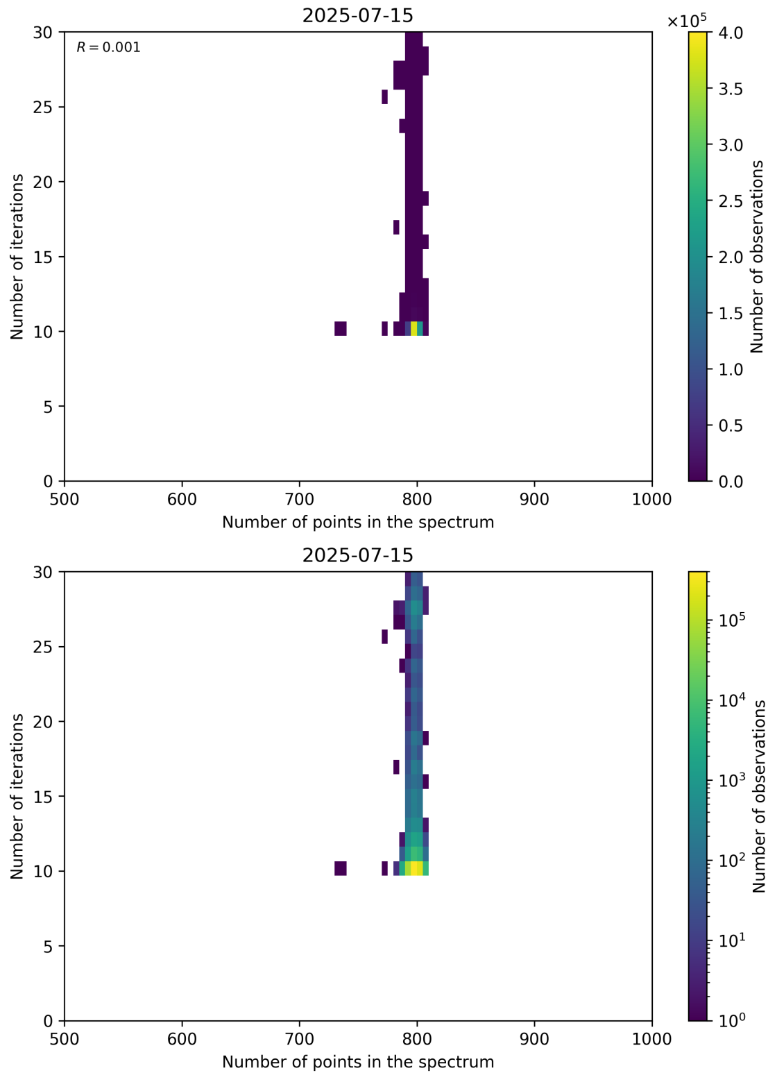
Figure 92: Scatter density plot of “Number of points in the spectrum” against “Number of iterations” for 2025-07-14 to 2025-07-16.
