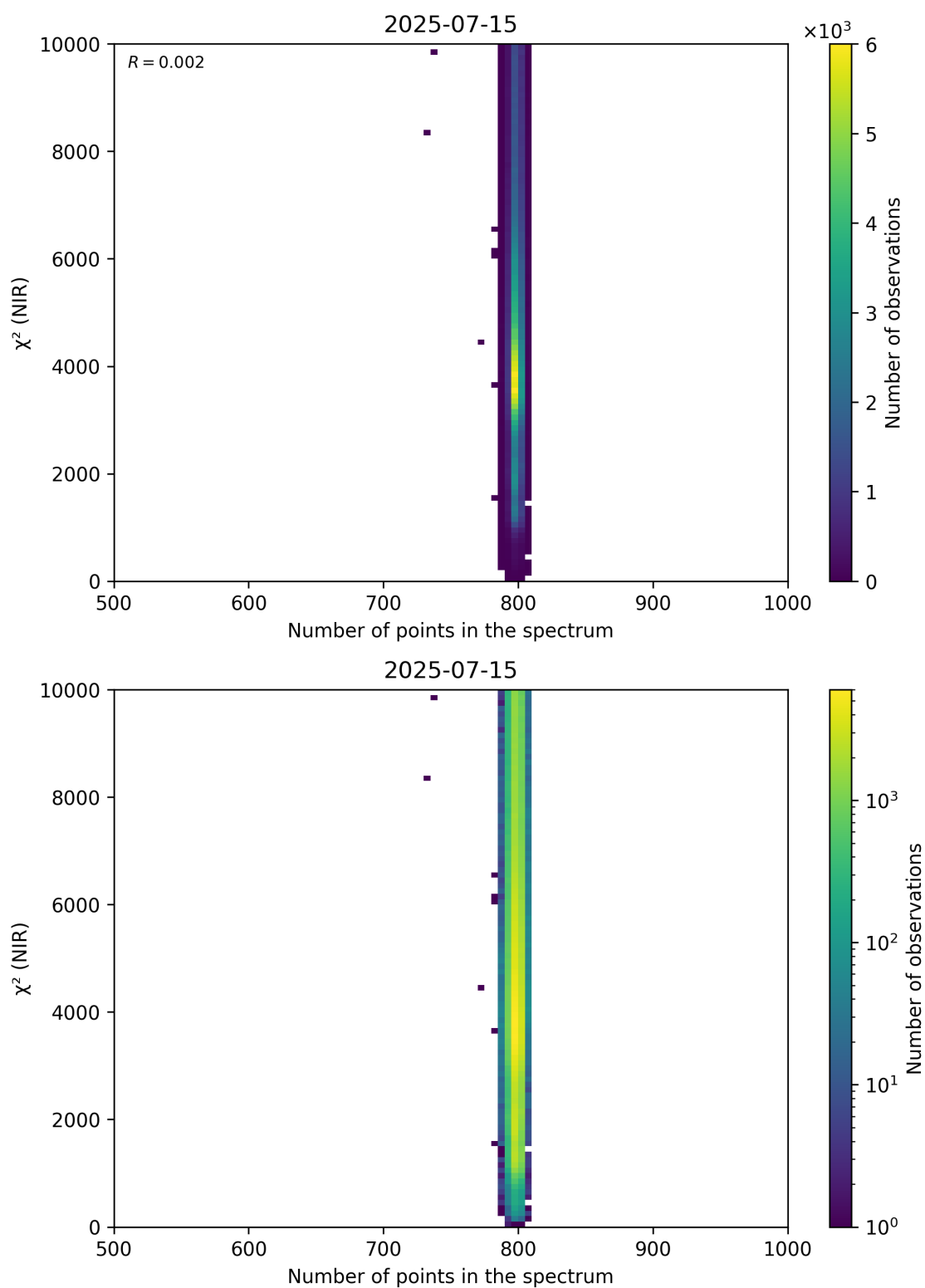
Figure 88: Scatter density plot of “Number of points in the spectrum” against “ \chi^2 (NIR)” for 2025-07-14 to 2025-07-16.
