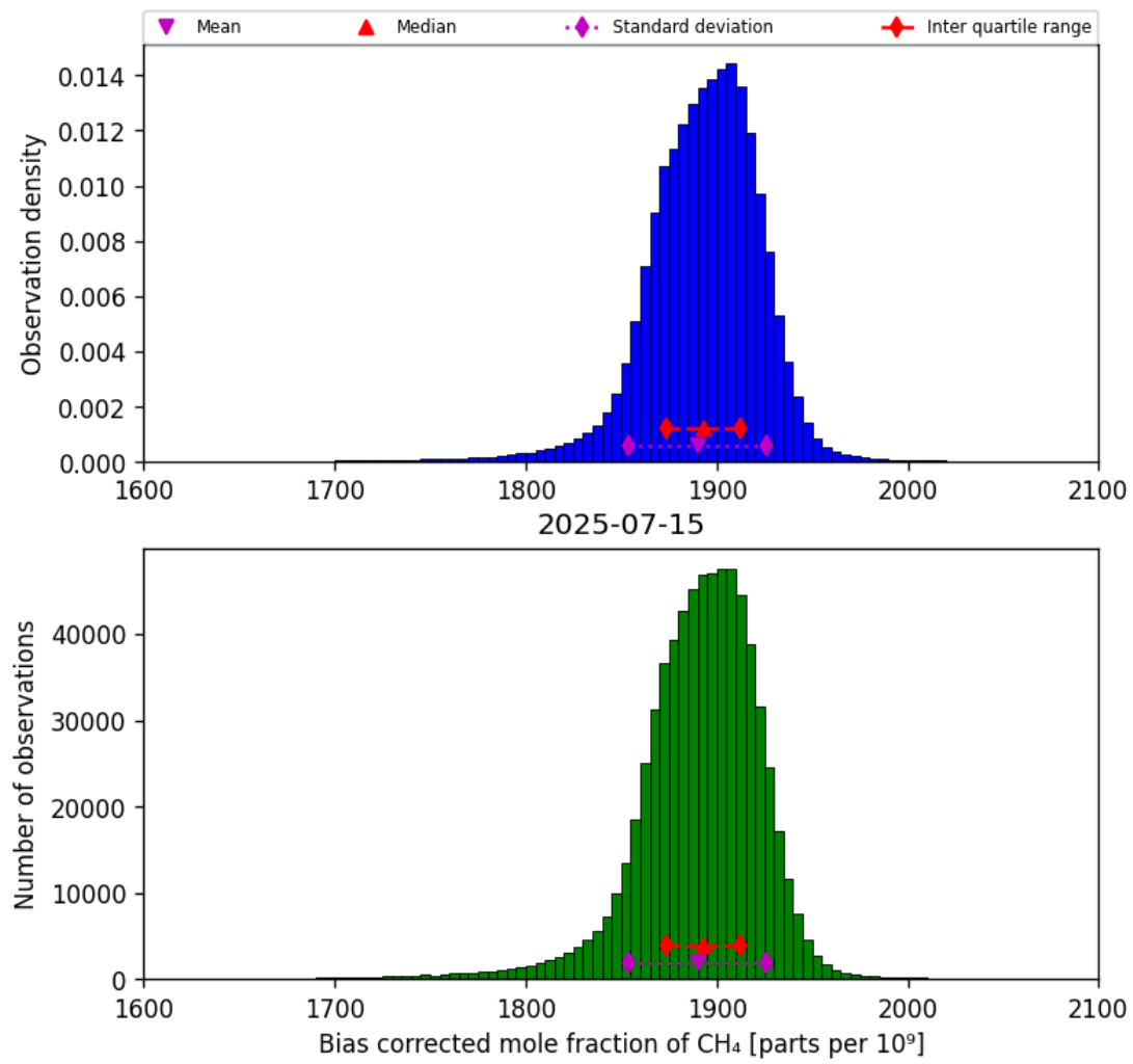
Figure 25: Histogram of “Bias corrected mole fraction of CH 4 ” for 2025-07-14 to 2025-07-16
