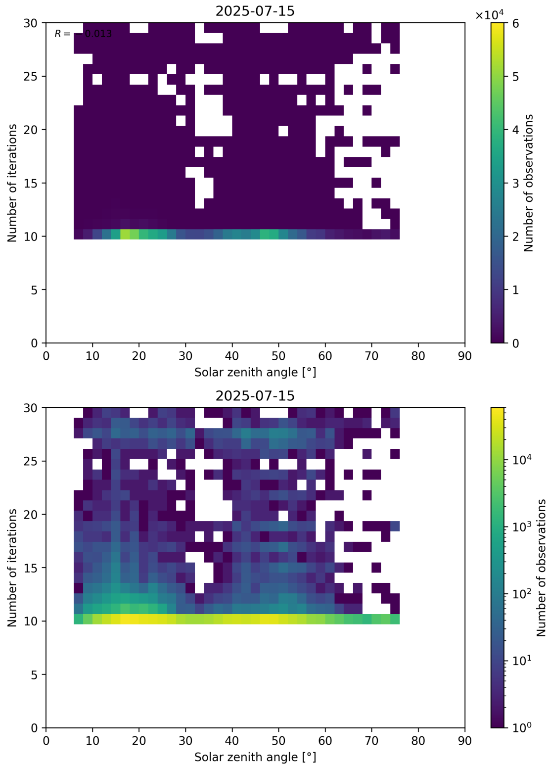
Figure 102: Scatter density plot of “Solar zenith angle” against “Number of iterations” for 2025-07-14 to 2025-07-16.
