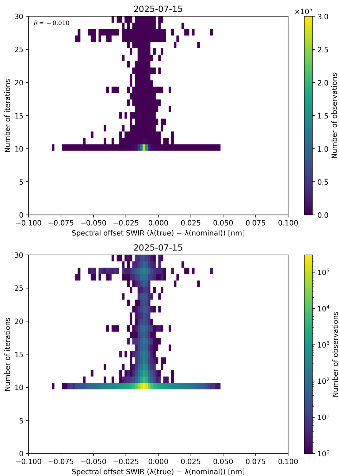
Figure 121: Scatter density plot of “Spectral offset SWIR ( \lambda_{\text{true}} - \lambda_{\text{nominal}} )” against “Number of iterations” for 2025-07-14 to 2025-07-16.
