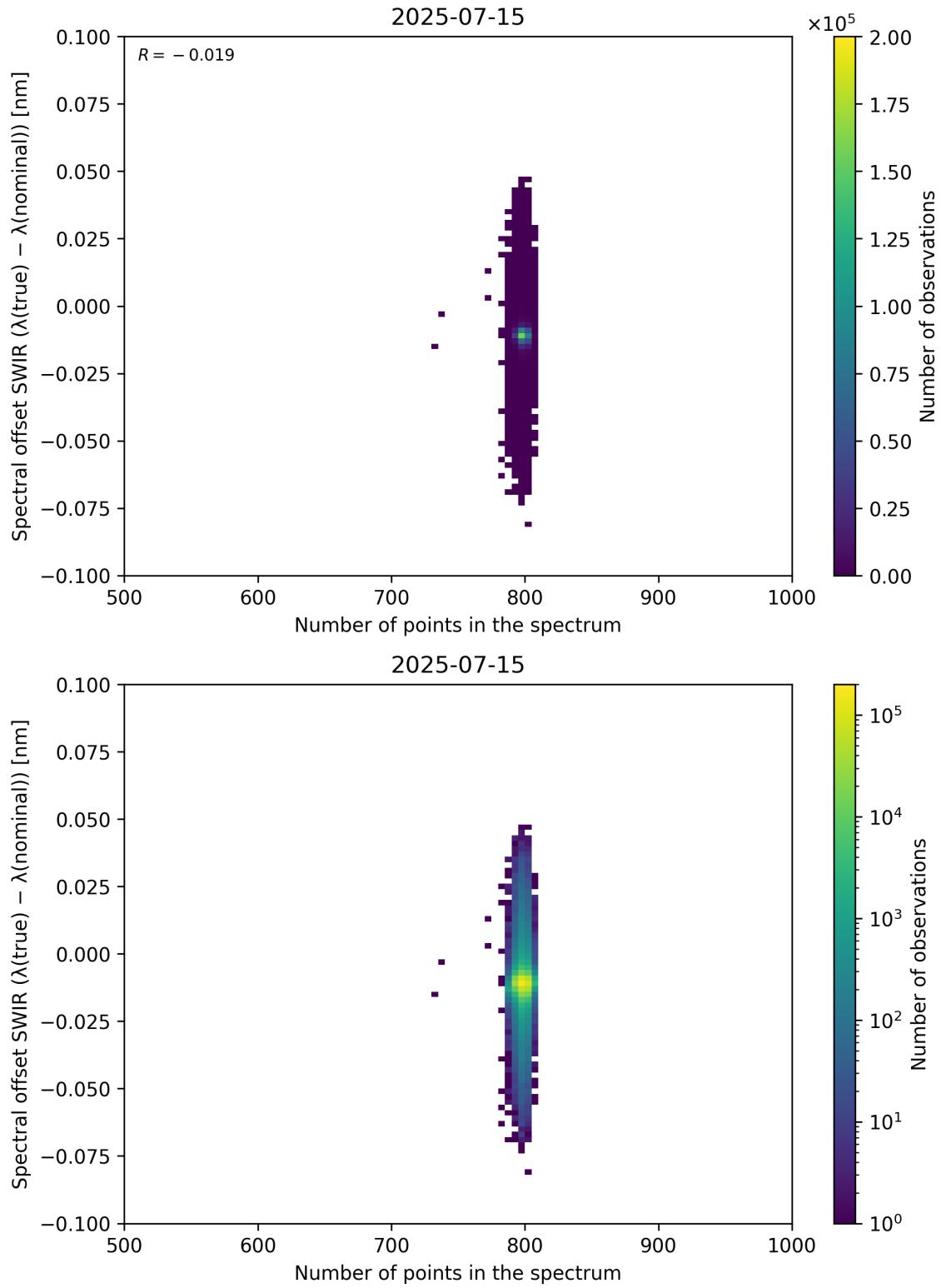
Figure 93: Scatter density plot of “Number of points in the spectrum” against “Spectral offset SWIR ( \lambda_{\text{true}} - \lambda_{\text{nominal}} )” for 2025-07-14 to 2025-07-16.
