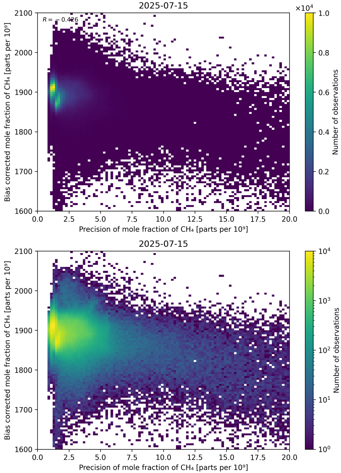
Figure 82: Scatter density plot of “Precision of mole fraction of CH 4 ” against “Bias corrected mole fraction of CH 4 ” for 2025-07-14 to 2025-07-16.
