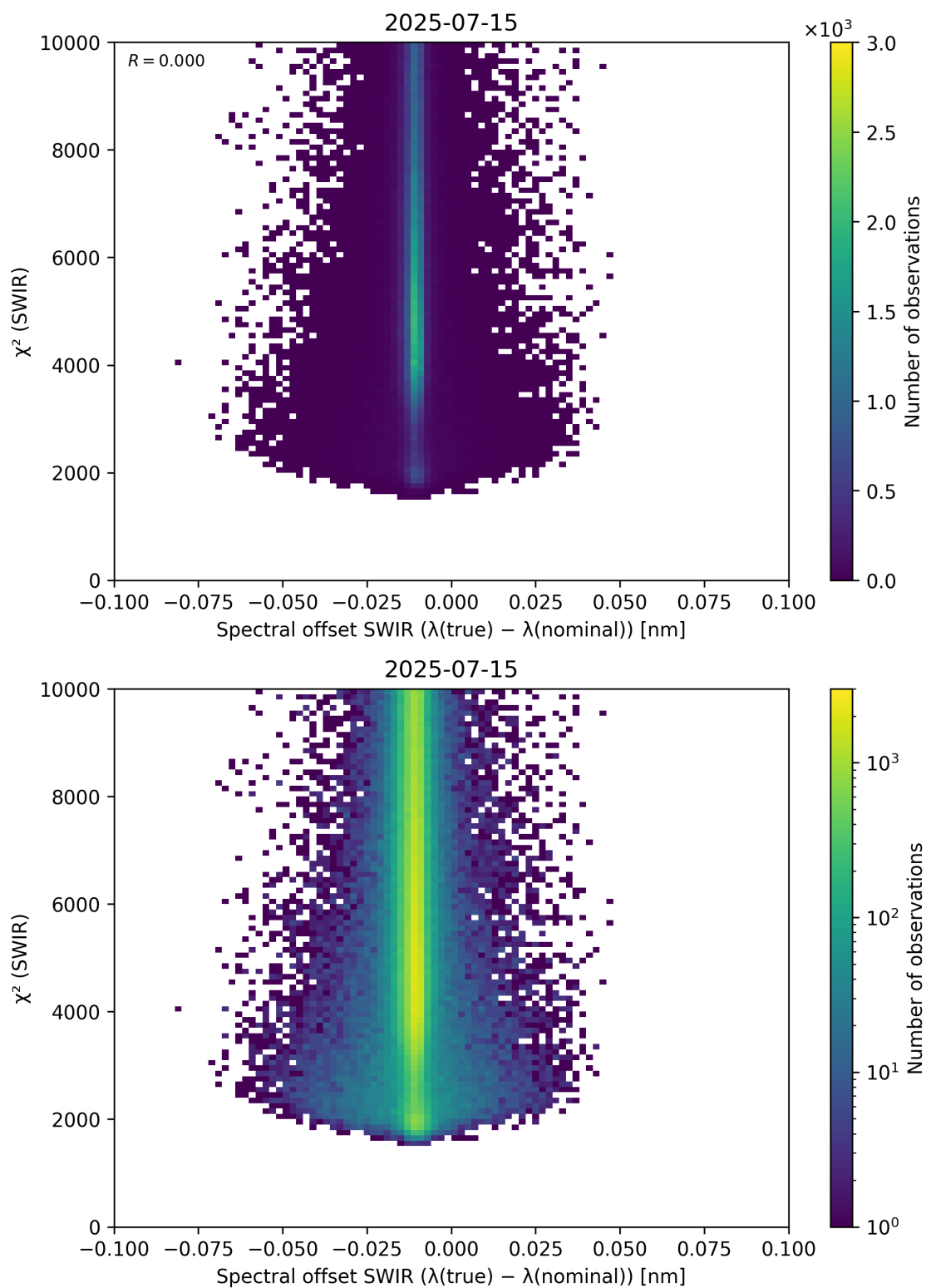
Figure 118: Scatter density plot of “Spectral offset SWIR ( \lambda_{\text{true}} - \lambda_{\text{nominal}} )” against “ \chi^2 (SWIR)” for 2025-07-14 to 2025-07-16.
