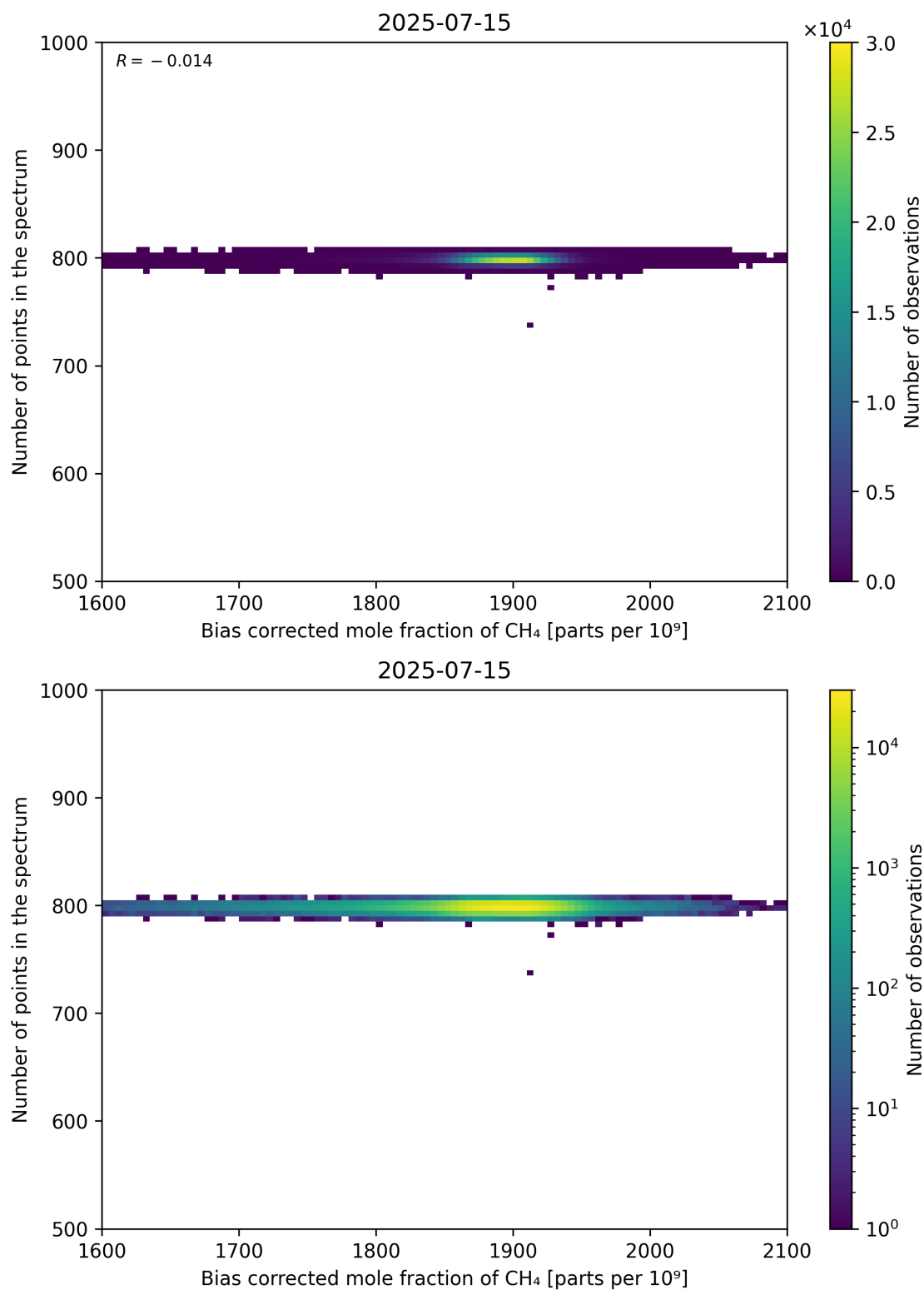
Figure 68: Scatter density plot of “Bias corrected mole fraction of CH 4 ” against “Number of points in the spectrum” for 2025-07-14 to 2025-07-16.
