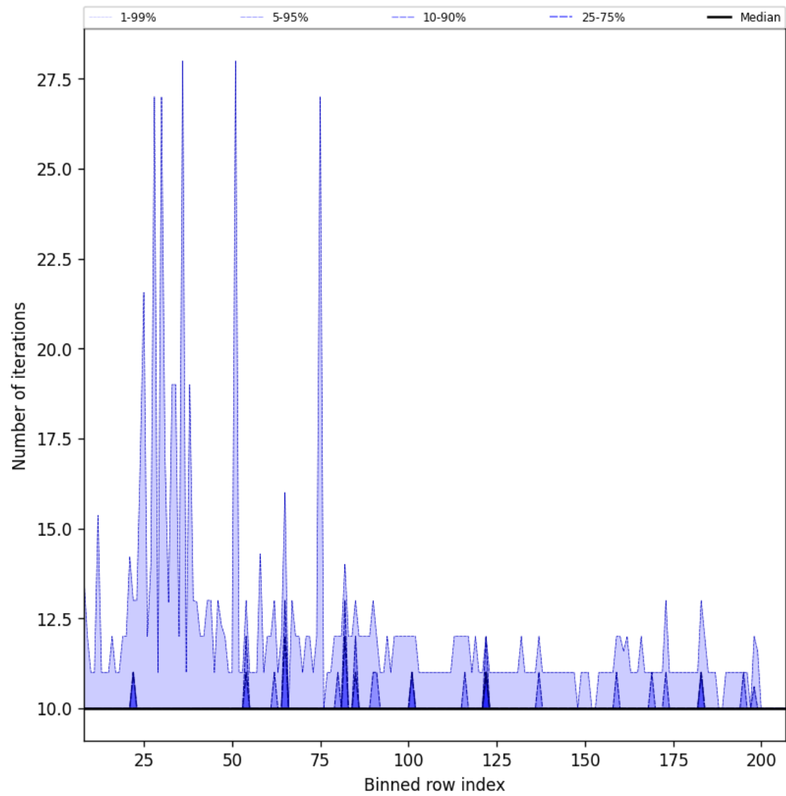
Figure 42: Along track statistics of “Number of iterations” for 2025-07-14 to 2025-07-16
