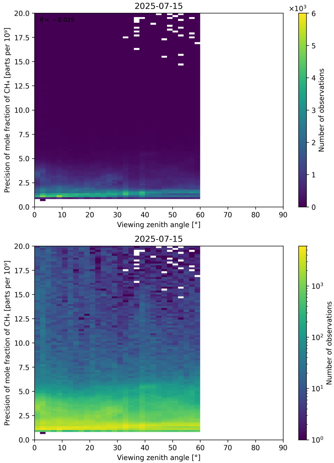
Figure 112: Scatter density plot of “Viewing zenith angle” against “Precision of mole fraction of CH 4 ” for 2025-07-14 to 2025-07-16.
