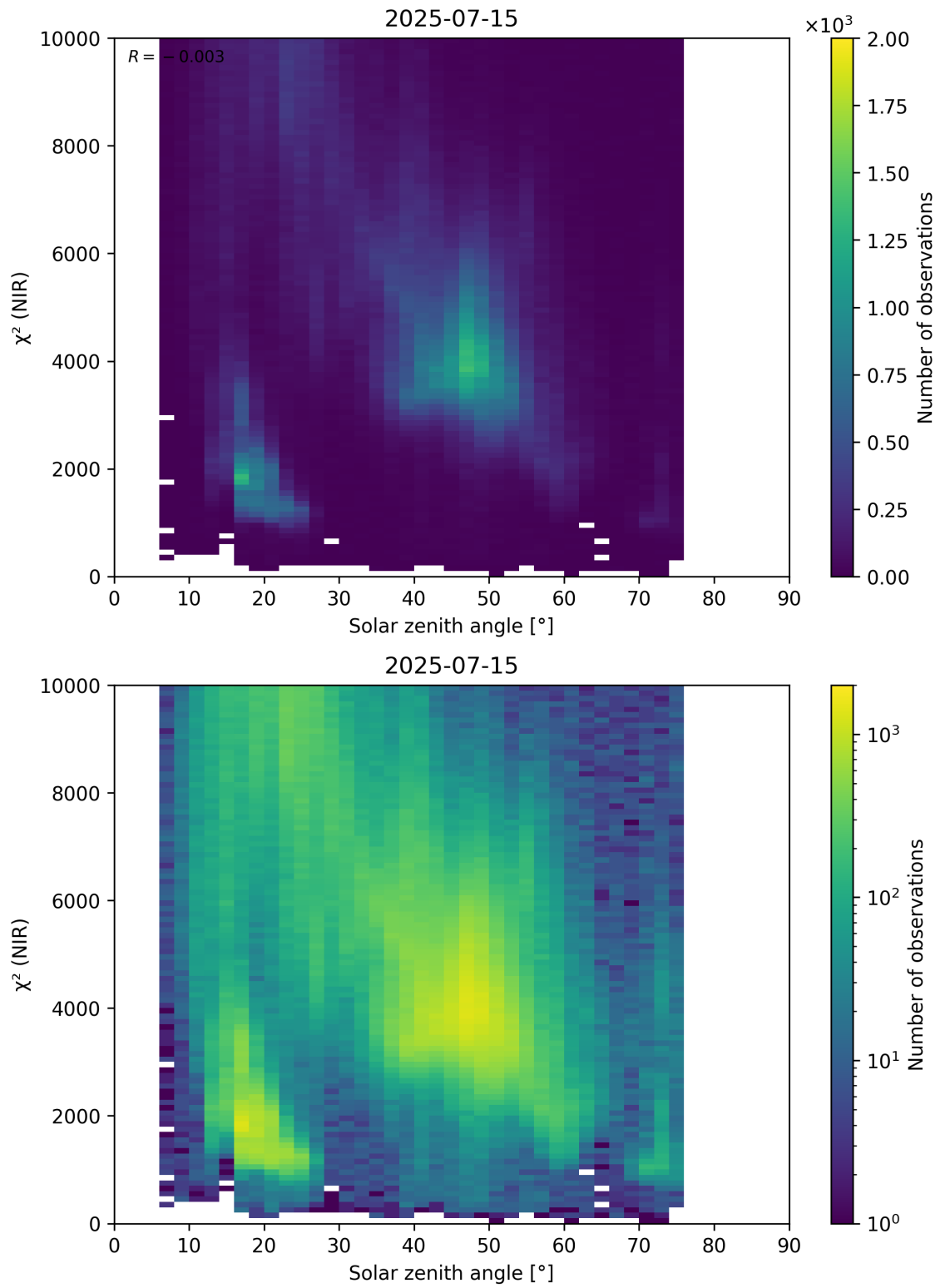
Figure 94: Scatter density plot of “Solar zenith angle” against “ \chi^2 (NIR)” for 2025-07-14 to 2025-07-16.
