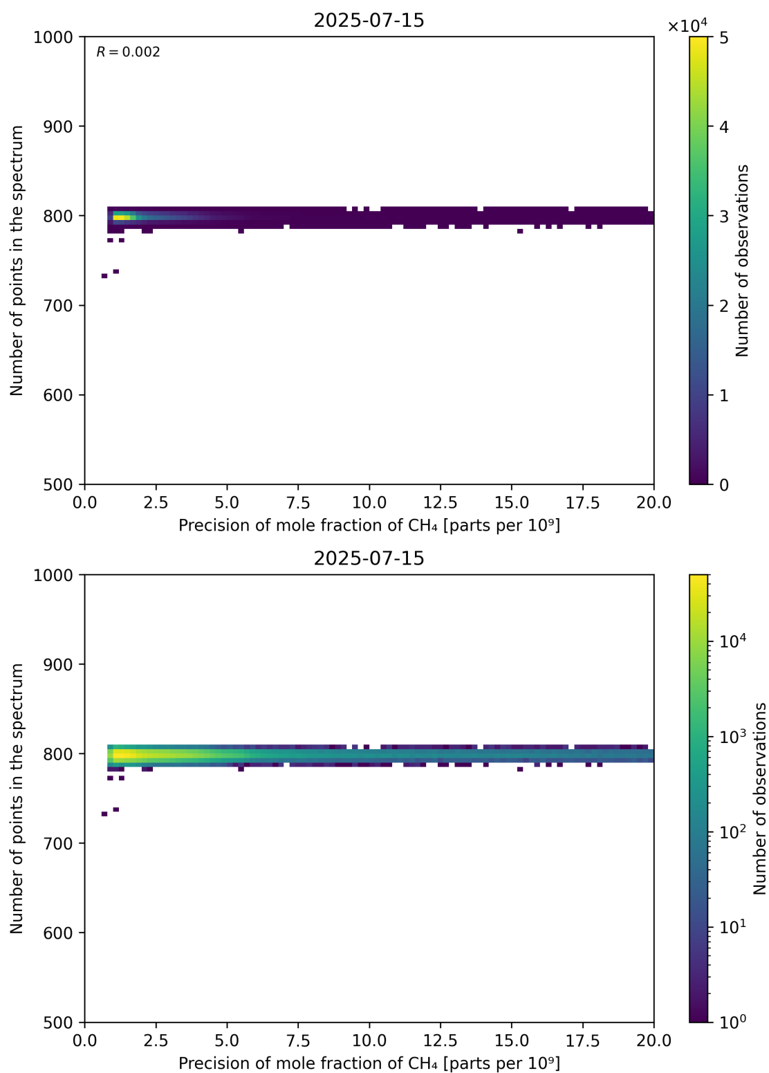
Figure 84: Scatter density plot of “Precision of mole fraction of CH 4 ” against “Number of points in the spectrum” for 2025-07-14 to 2025-07-16.
