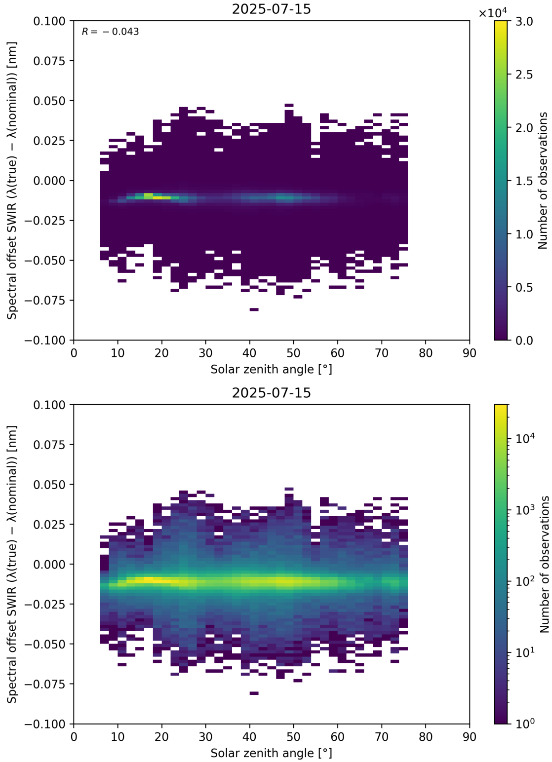
Figure 104: Scatter density plot of “Solar zenith angle” against “Spectral offset SWIR ( \lambda_{\text{true}} - \lambda_{\text{nominal}} )” for 2025-07-14 to 2025-07-16.
