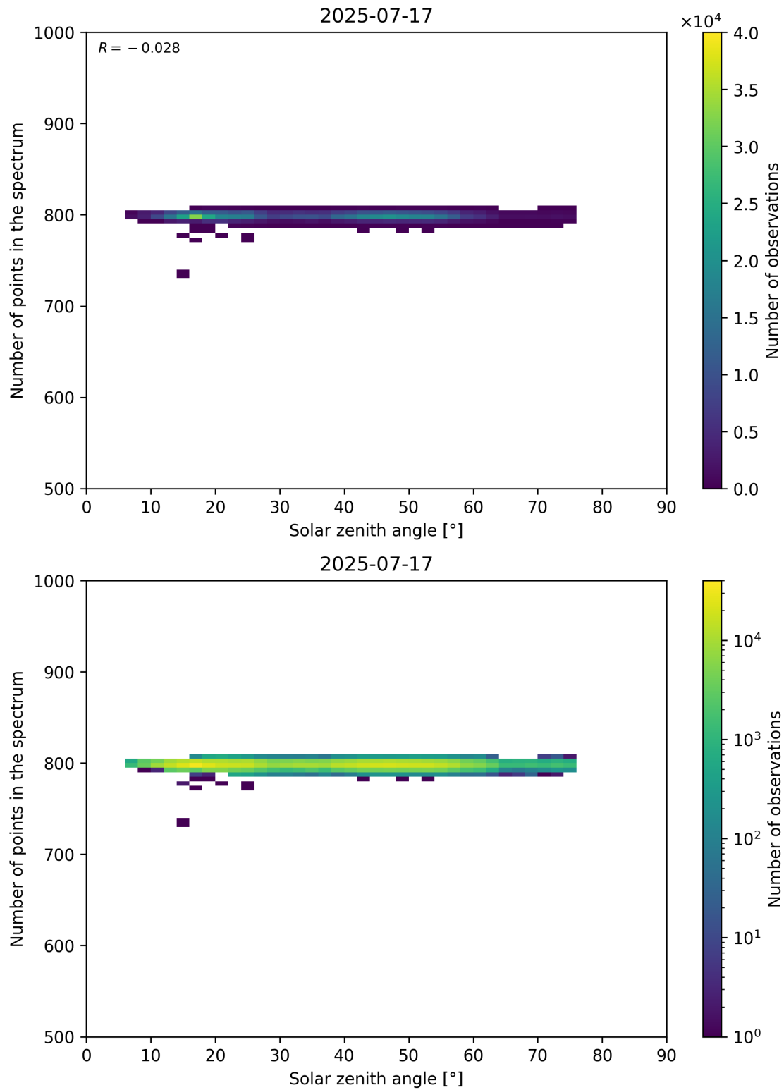
Figure 103: Scatter density plot of “Solar zenith angle” against “Number of points in the spectrum” for 2025-07-16 to 2025-07-18.
