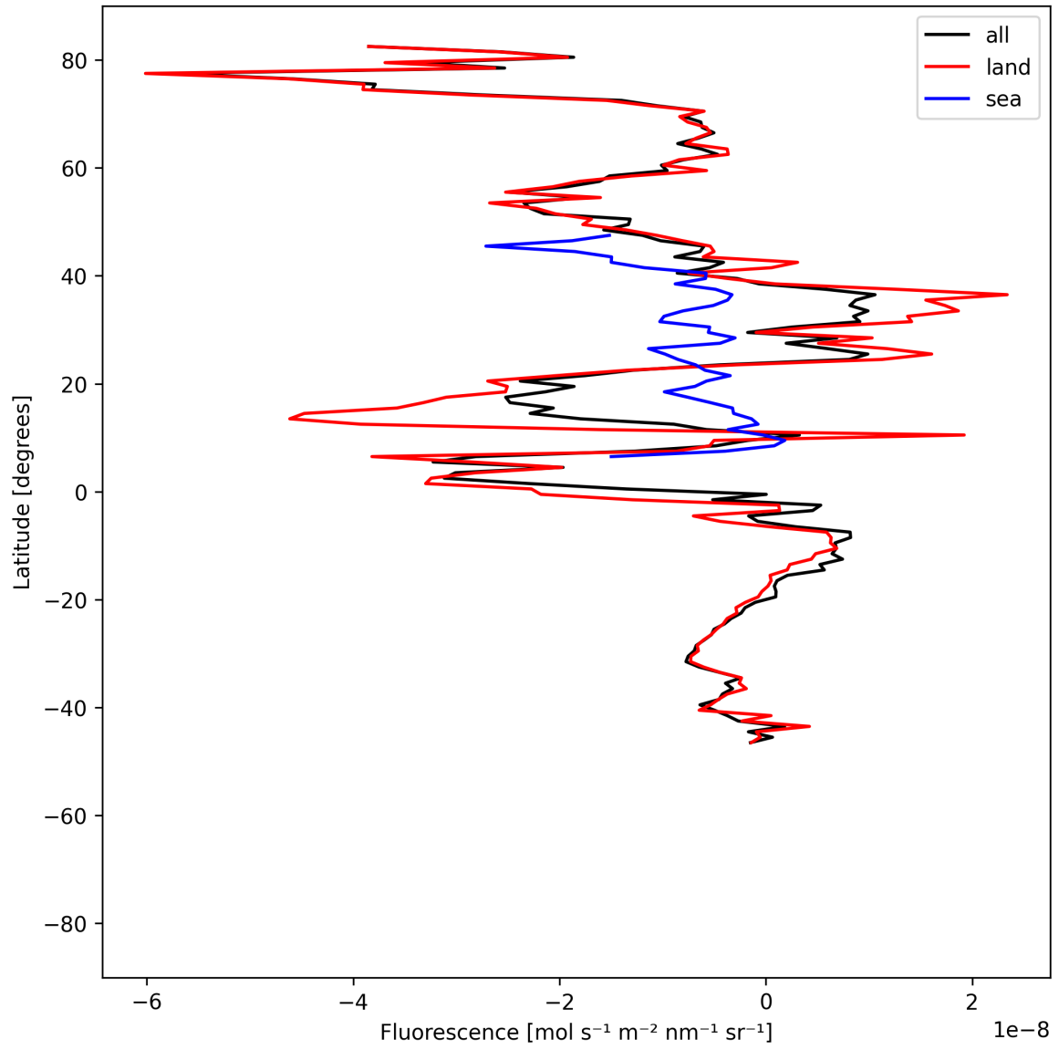
Figure 21: Zonal average of “Fluorescence” for 2025-07-16 to 2025-07-18.
