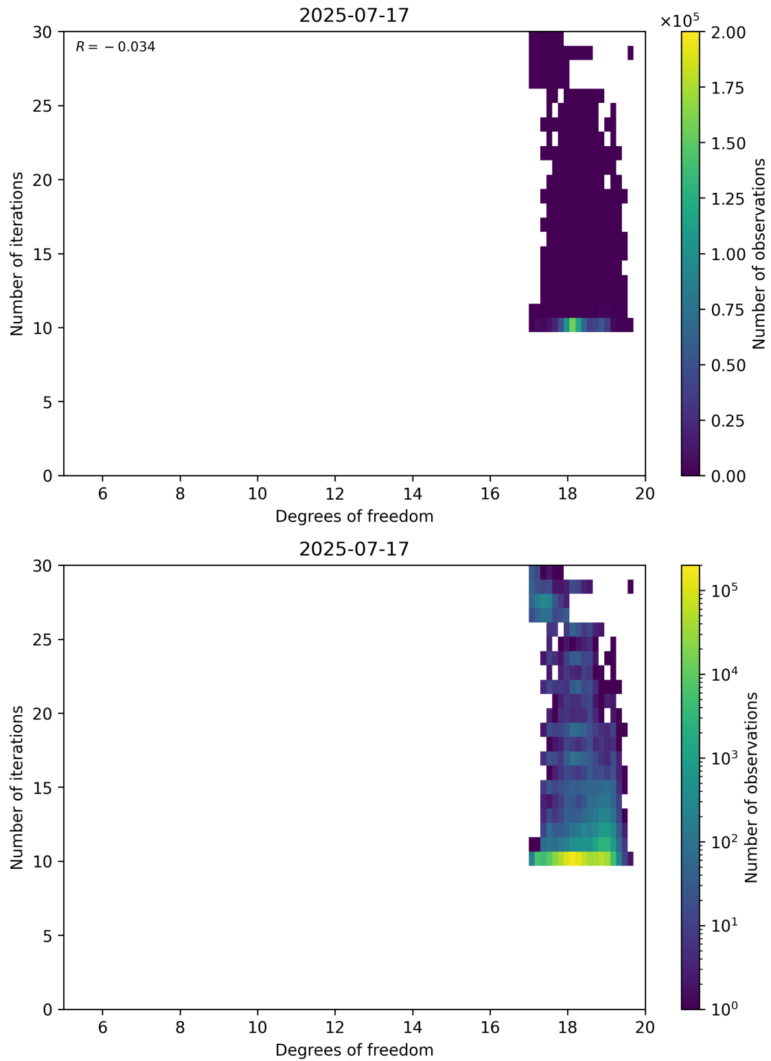
Figure 52: Scatter density plot of “Degrees of freedom” against “Number of iterations” for 2025-07-16 to 2025-07-18.
