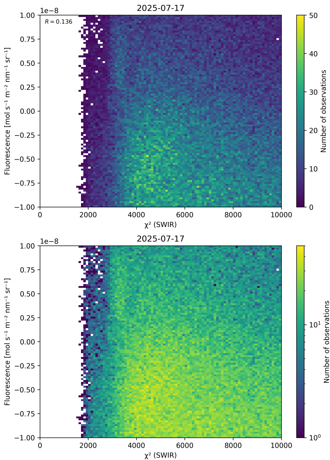
Figure 49: Scatter density plot of “ \chi^2 (SWIR)” against “Fluorescence” for 2025-07-16 to 2025-07-18.
