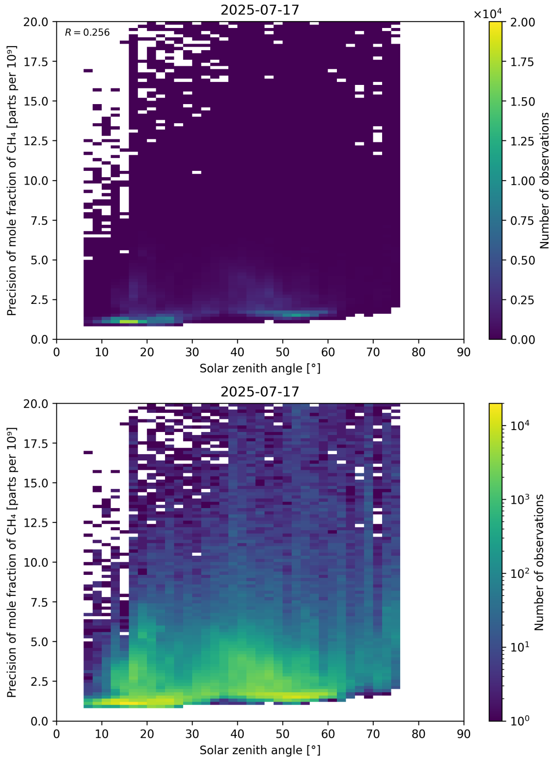
Figure 101: Scatter density plot of “Solar zenith angle” against “Precision of mole fraction of CH 4 ” for 2025-07-16 to 2025-07-18.
