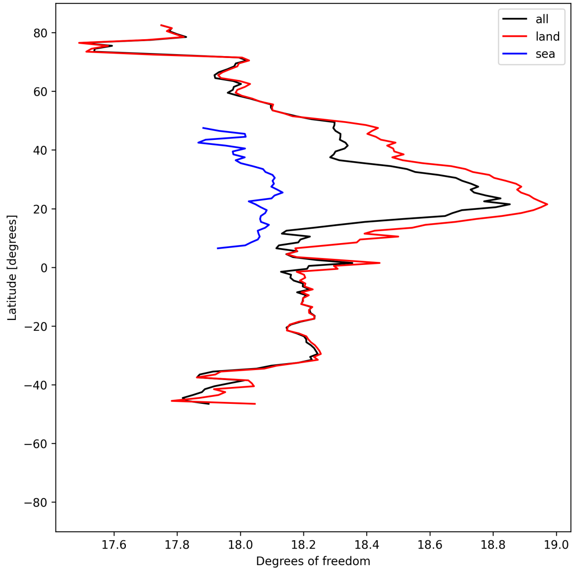
Figure 19: Zonal average of “Degrees of freedom” for 2025-07-16 to 2025-07-18.
