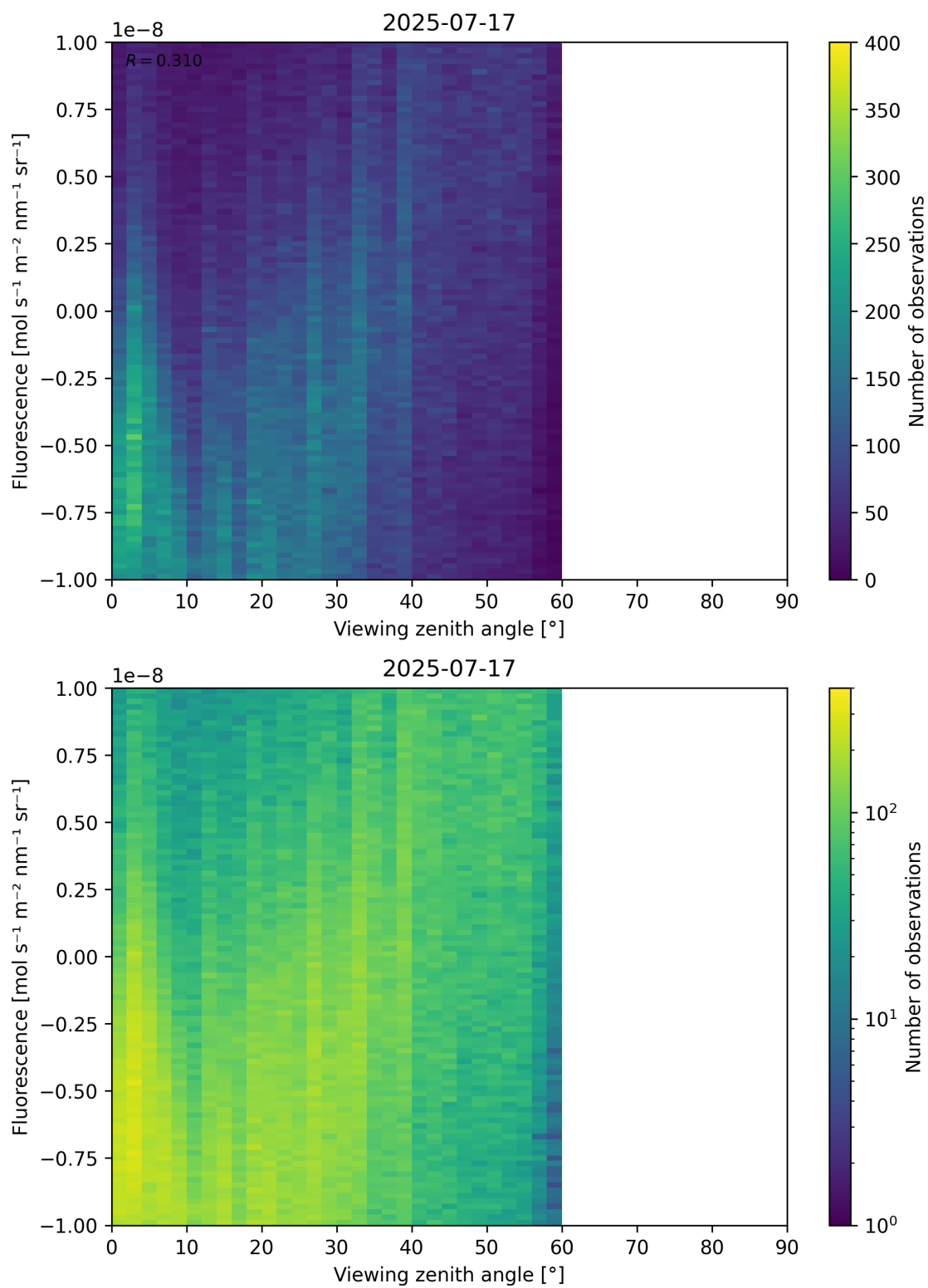
Figure 108: Scatter density plot of “Viewing zenith angle” against “Fluorescence” for 2025-07-16 to 2025-07-18.
