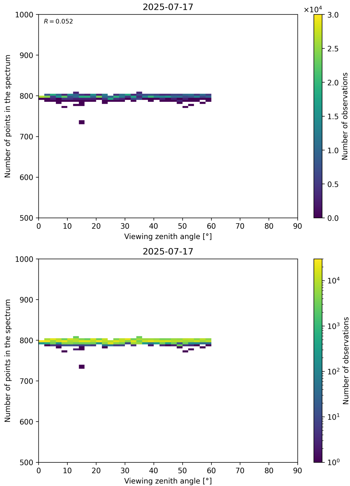
Figure 114: Scatter density plot of “Viewing zenith angle” against “Number of points in the spectrum” for 2025-07-16 to 2025-07-18.
