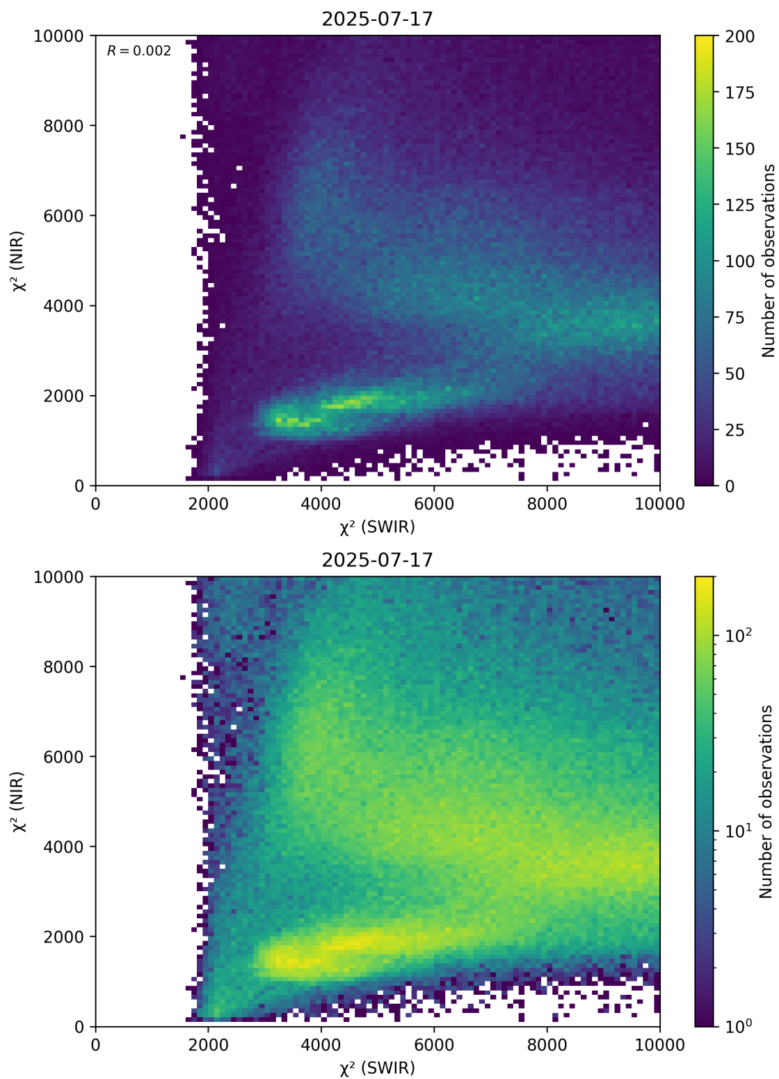
Figure 47: Scatter density plot of “ \chi^2 (SWIR)” against “ \chi^2 (NIR)” for 2025-07-16 to 2025-07-18.
