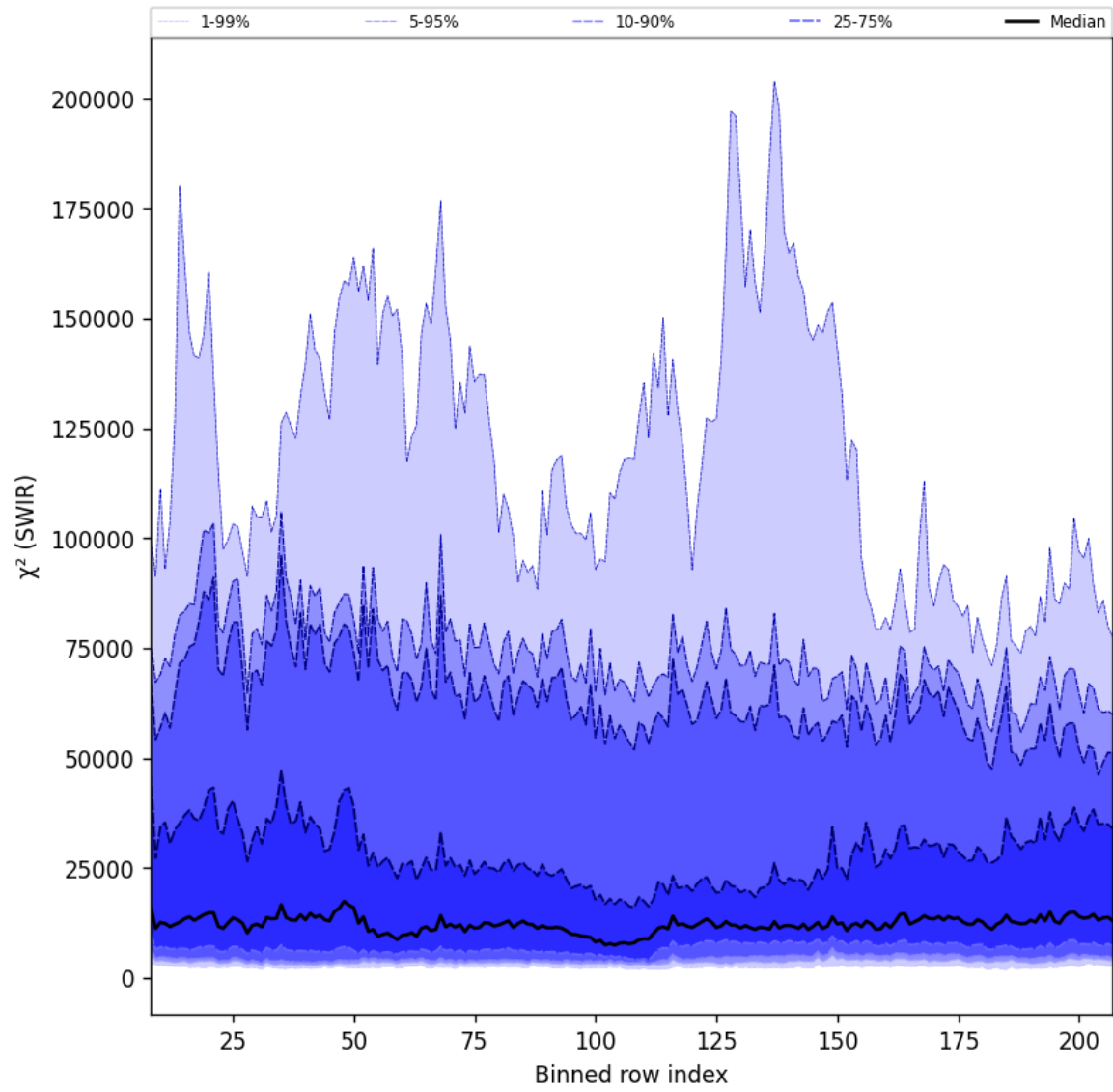
Figure 39: Along track statistics of “ \chi^2 (SWIR)” for 2025-07-16 to 2025-07-18
