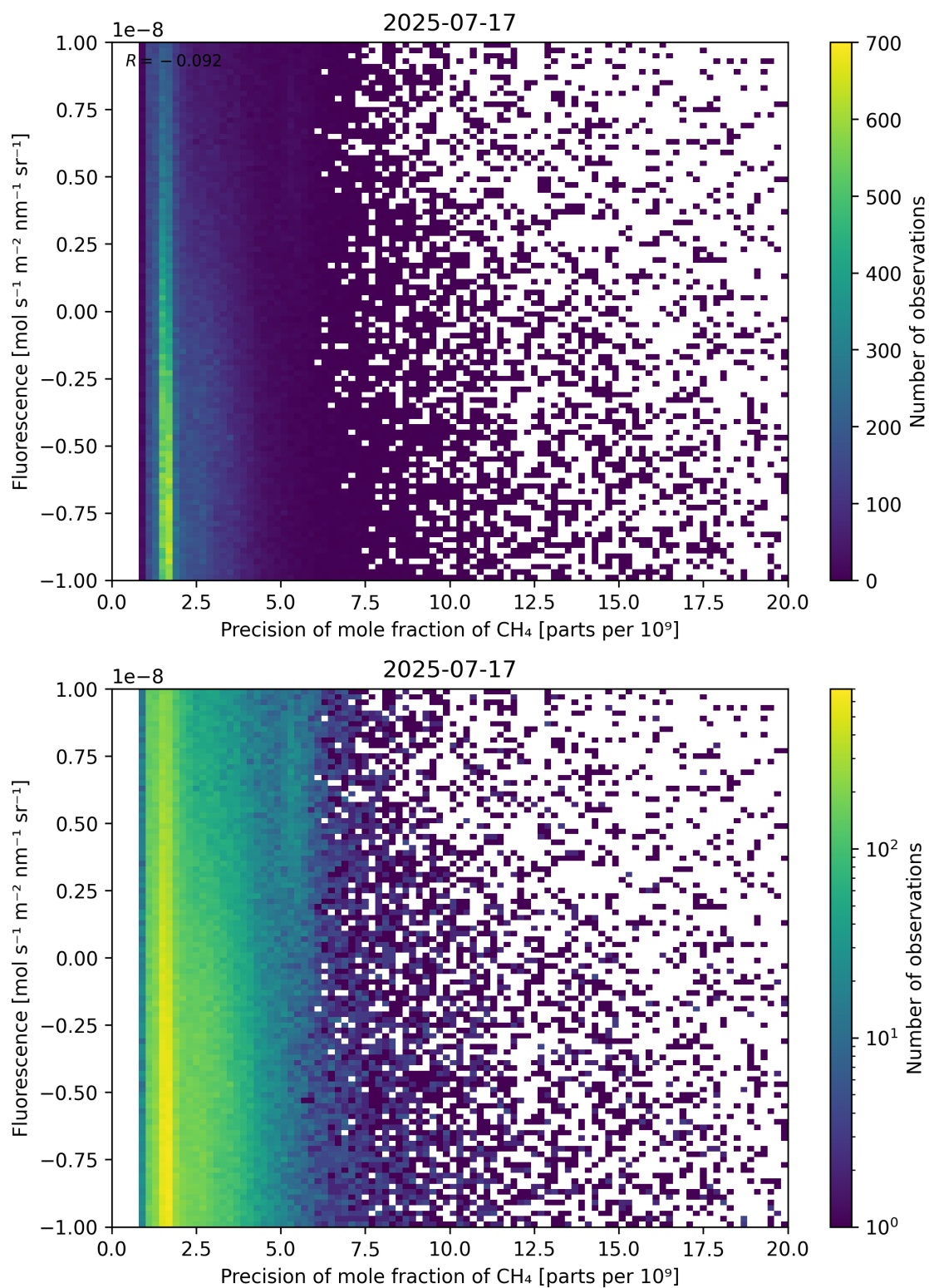
Figure 81: Scatter density plot of “Precision of mole fraction of CH 4 ” against “Fluorescence” for 2025-07-16 to 2025-07-18.
