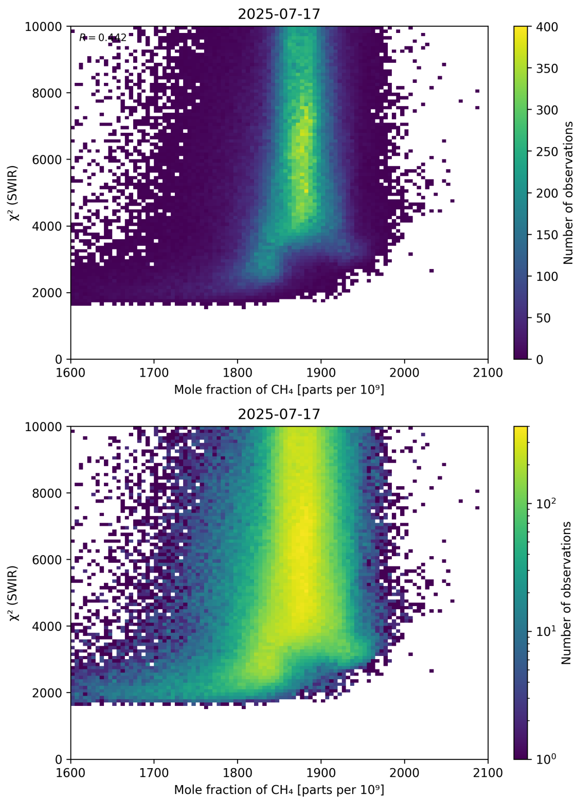
Figure 71: Scatter density plot of “Mole fraction of \text{CH}_4 ” against “ \chi^2 (SWIR)” for 2025-07-16 to 2025-07-18.
