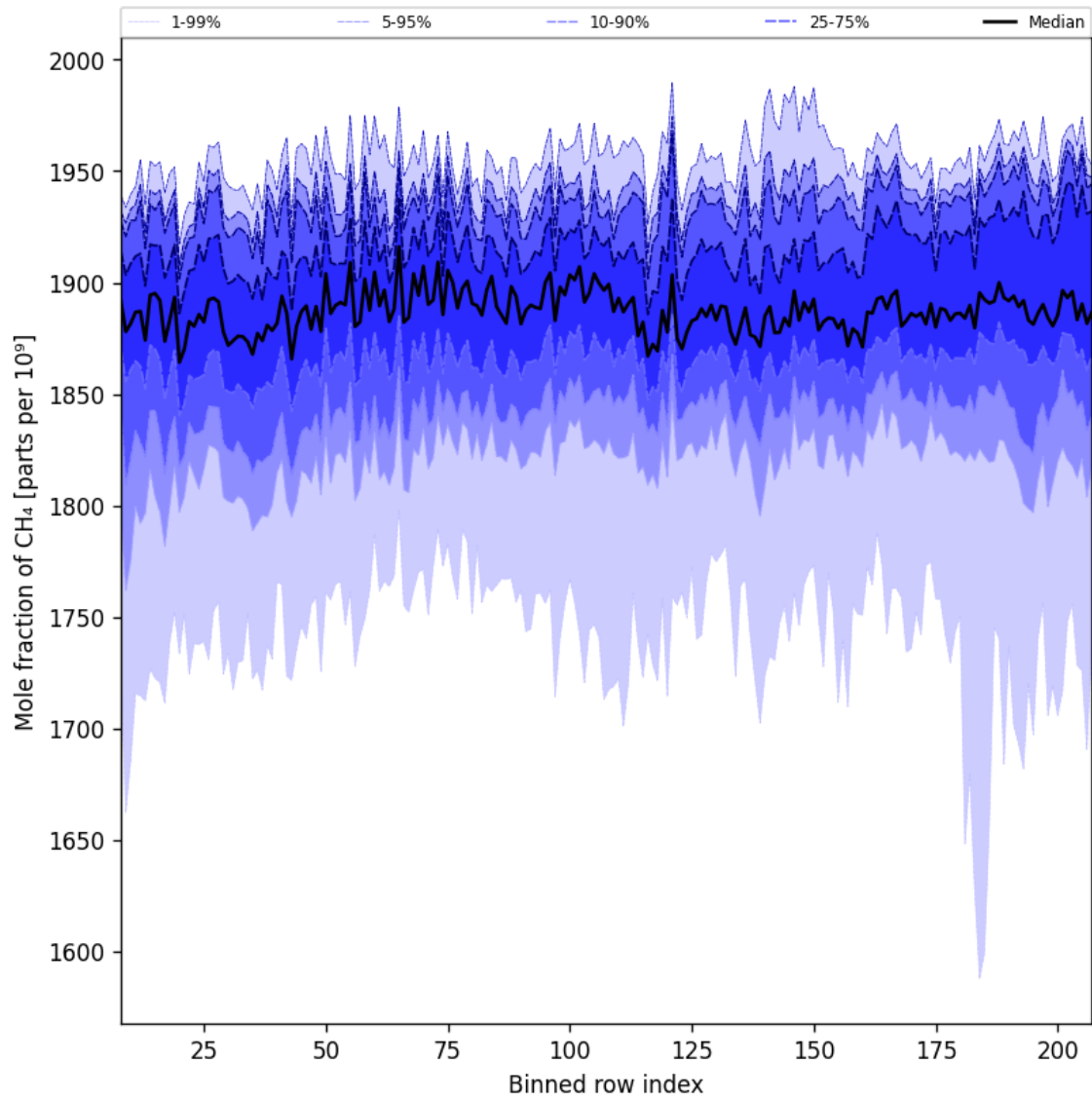
Figure 34: Along track statistics of “Mole fraction of CH 4 ” for 2025-07-16 to 2025-07-18
