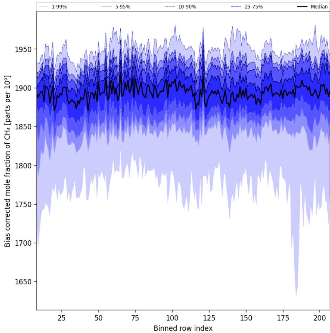
Figure 36: Along track statistics of “Bias corrected mole fraction of CH 4 ” for 2025-07-16 to 2025-07-18
