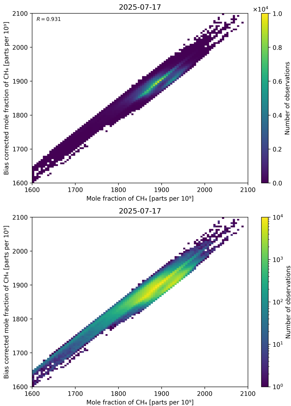
Figure 74: Scatter density plot of “Mole fraction of CH 4 ” against “Bias corrected mole fraction of CH 4 ” for 2025-07-16 to 2025-07-18.
