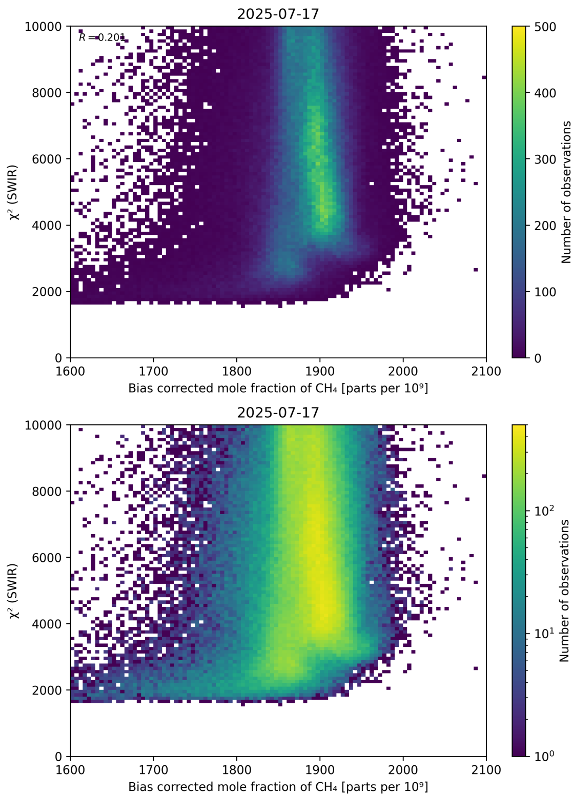
Figure 64: Scatter density plot of “Bias corrected mole fraction of \text{CH}_4 ” against “ \chi^2 (SWIR)” for 2025-07-16 to 2025-07-18.
