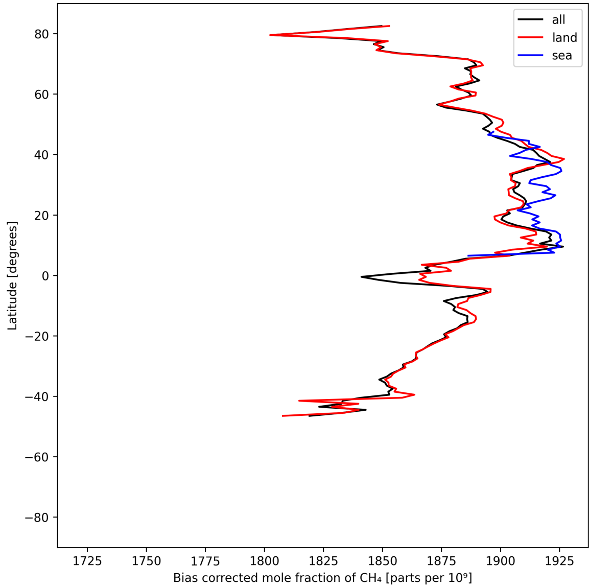
Figure 14: Zonal average of “Bias corrected mole fraction of \text{CH}_4 ” for 2025-07-16 to 2025-07-18.
