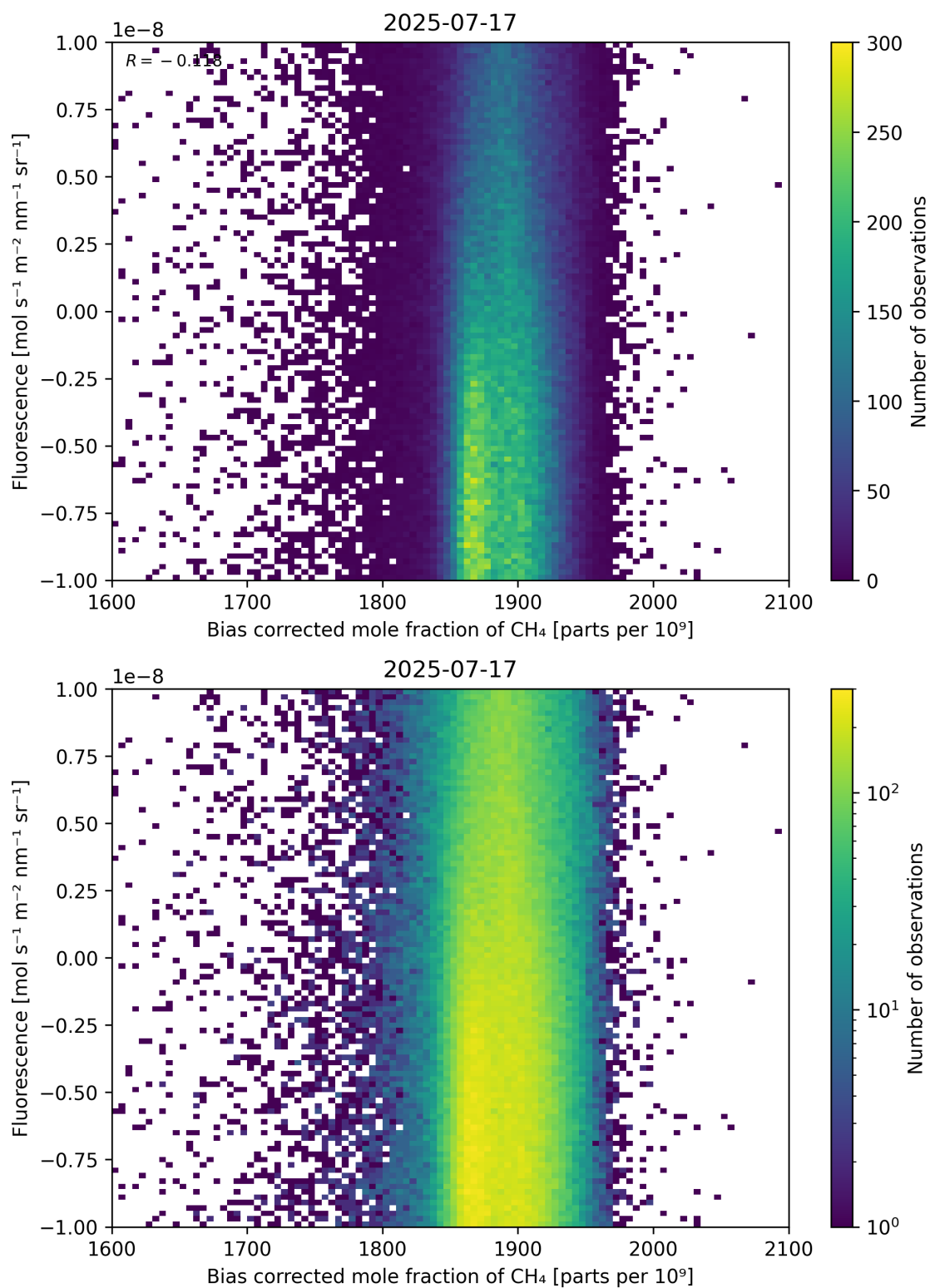
Figure 66: Scatter density plot of “Bias corrected mole fraction of \text{CH}_4 ” against “Fluorescence” for 2025-07-16 to 2025-07-18.
