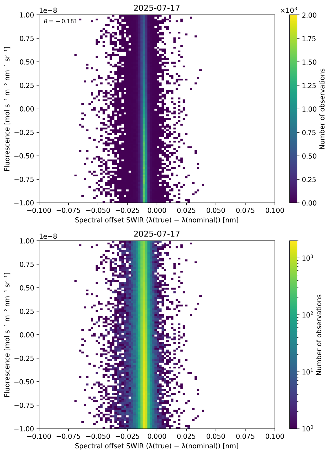
Figure 120: Scatter density plot of “Spectral offset SWIR ( \lambda_{\text{true}} - \lambda_{\text{nominal}} )” against “Fluorescence” for 2025-07-16 to 2025-07-18.
