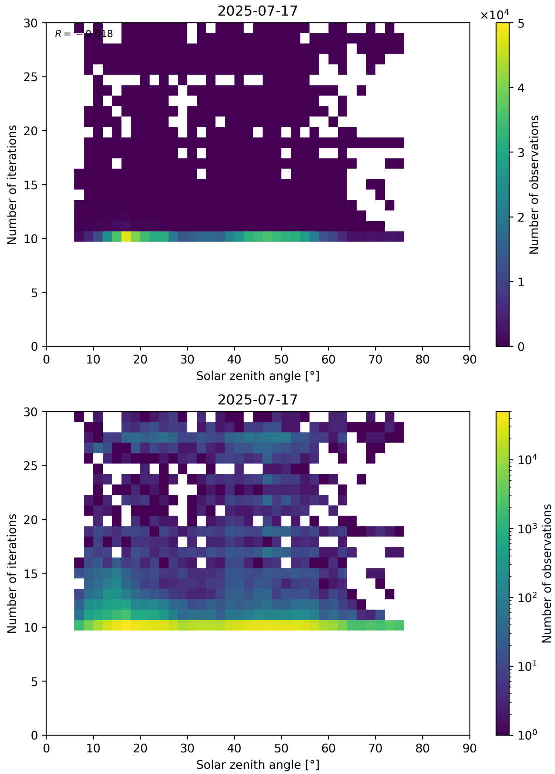
Figure 102: Scatter density plot of “Solar zenith angle” against “Number of iterations” for 2025-07-16 to 2025-07-18.
