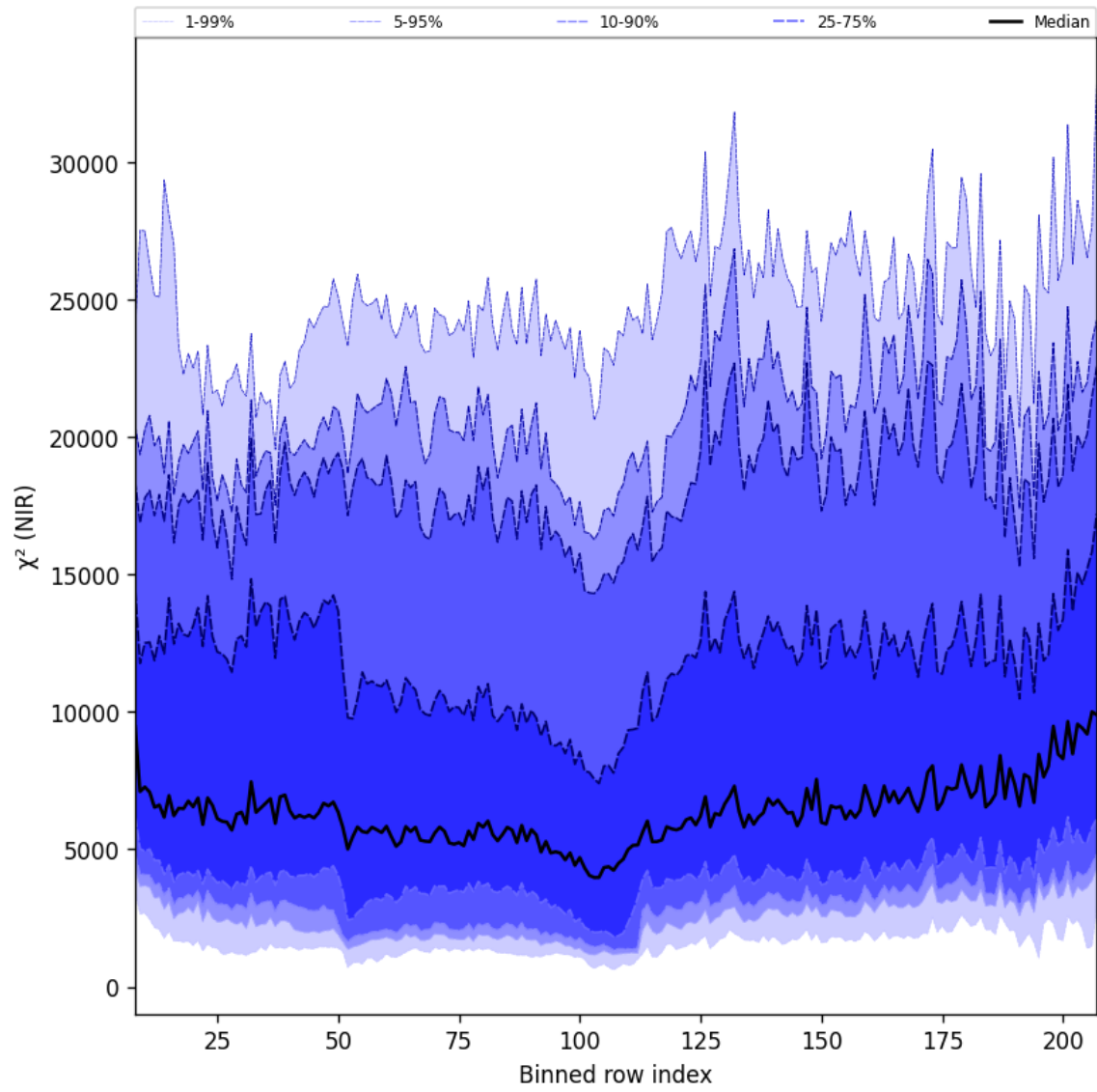
Figure 40: Along track statistics of “ \chi^2 (NIR)” for 2025-07-16 to 2025-07-18
