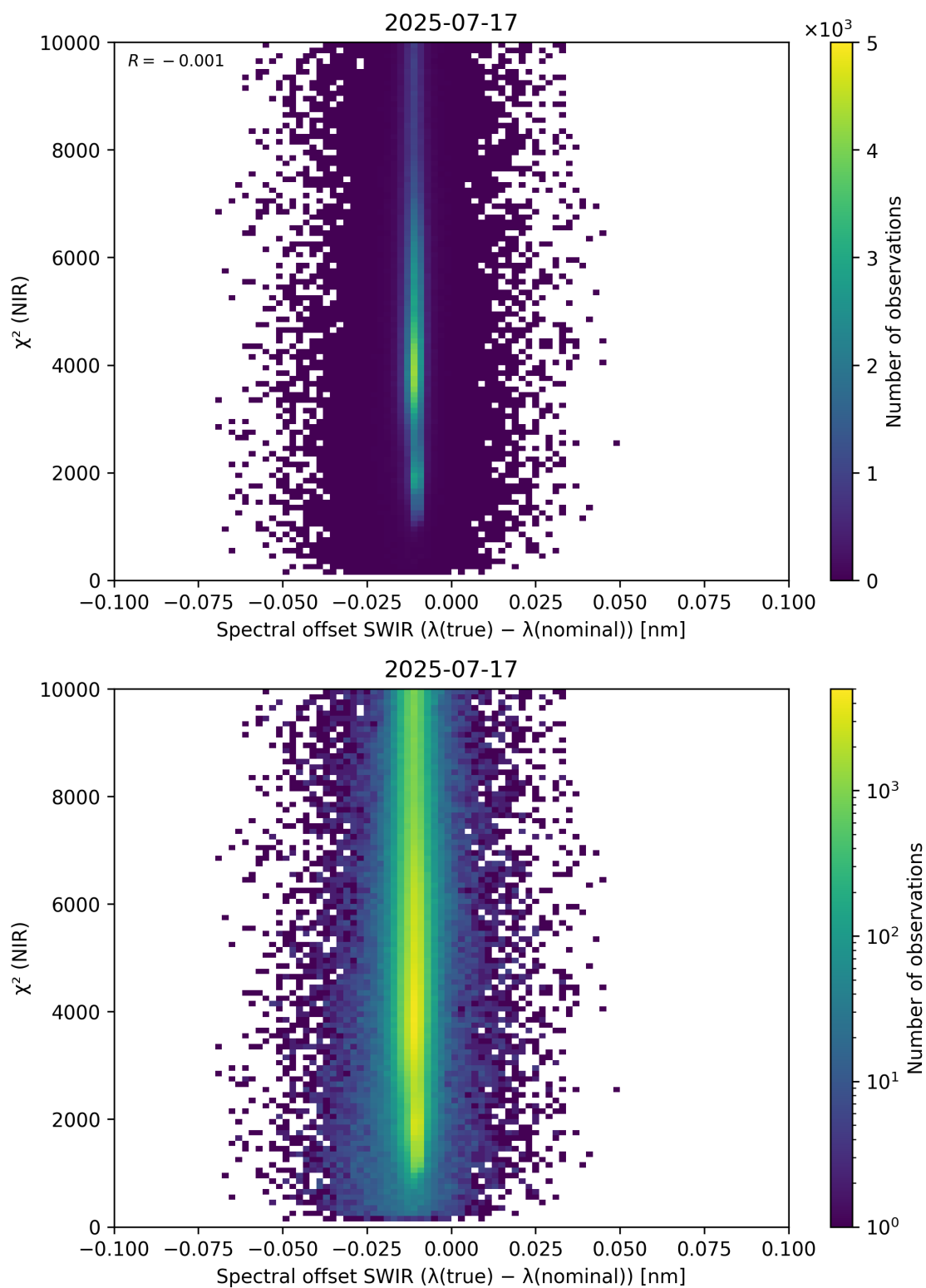
Figure 117: Scatter density plot of “Spectral offset SWIR ( \lambda_{\text{true}} - \lambda_{\text{nominal}} )” against “ \chi^2 (NIR)” for 2025-07-16 to 2025-07-18.
