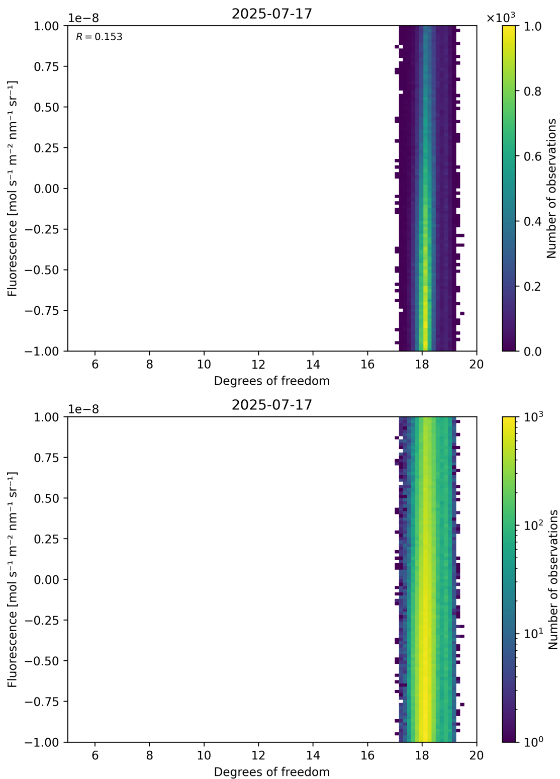
Figure 51: Scatter density plot of “Degrees of freedom” against “Fluorescence” for 2025-07-16 to 2025-07-18.
