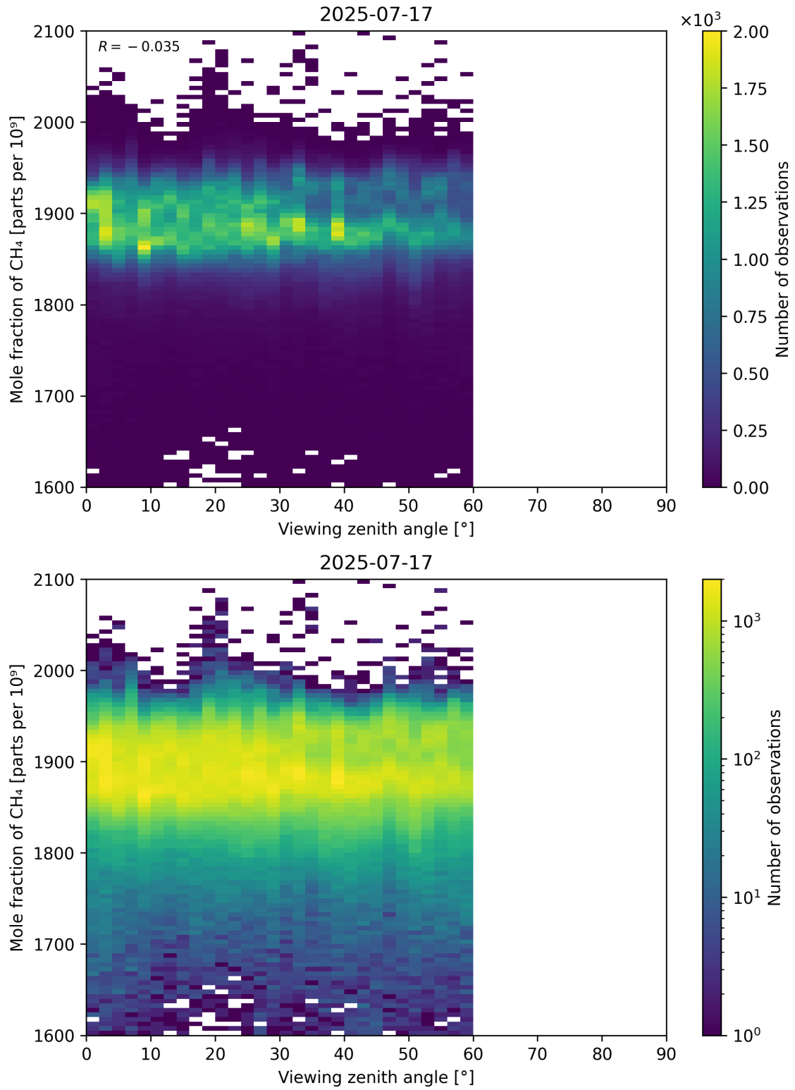
Figure 110: Scatter density plot of “Viewing zenith angle” against “Mole fraction of CH 4 ” for 2025-07-16 to 2025-07-18.
