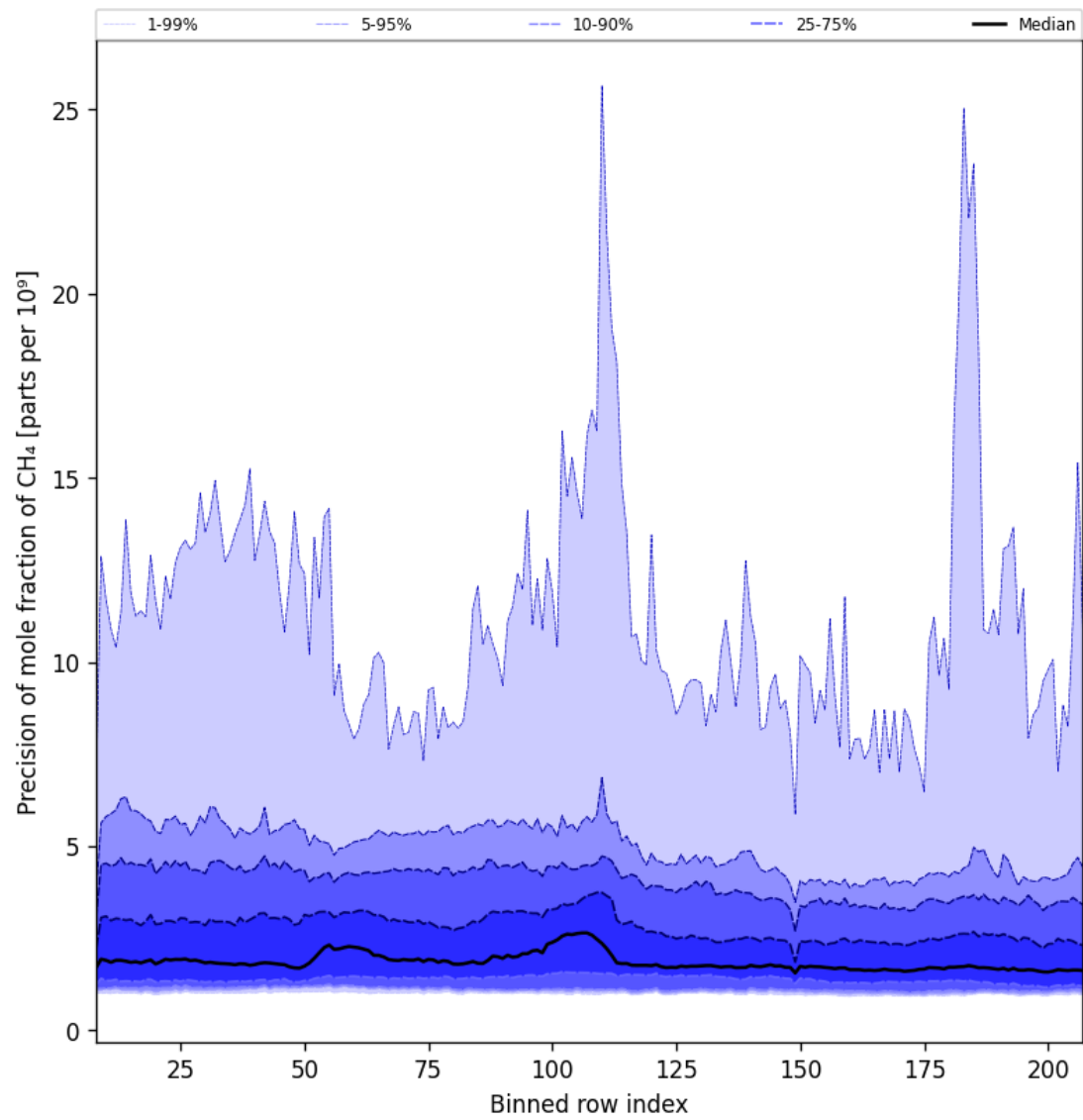
Figure 35: Along track statistics of “Precision of mole fraction of CH 4 ” for 2025-07-16 to 2025-07-18
