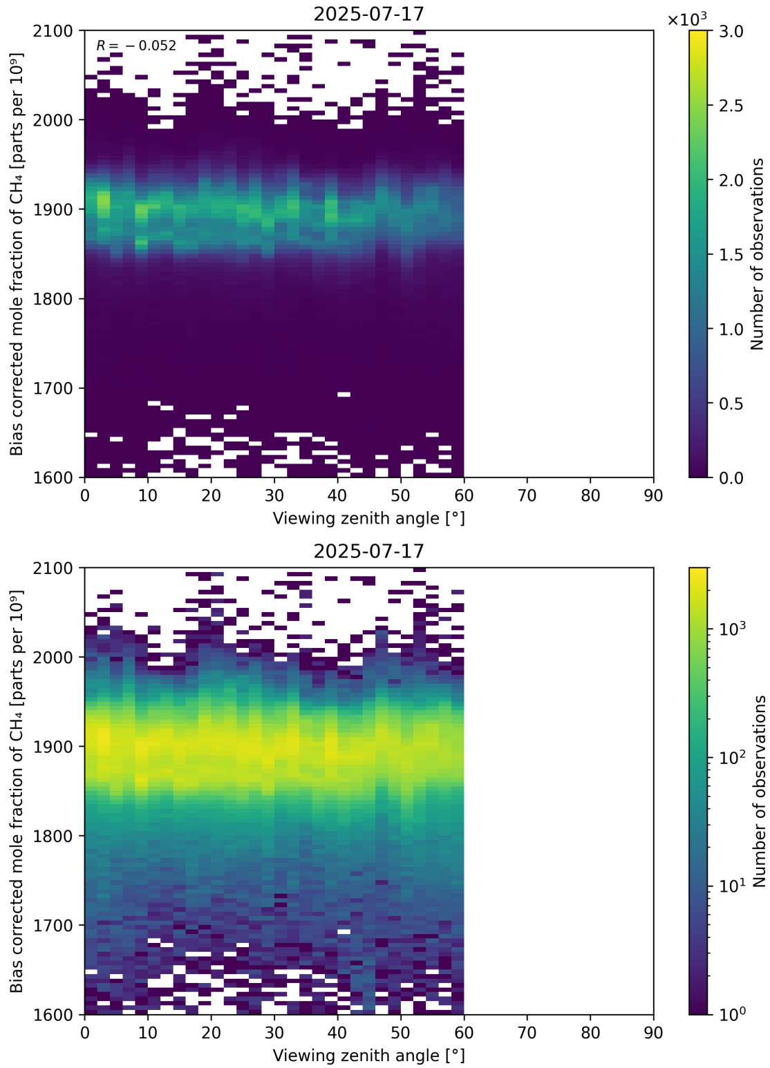
Figure 111: Scatter density plot of “Viewing zenith angle” against “Bias corrected mole fraction of CH 4 ” for 2025-07-16 to 2025-07-18.
