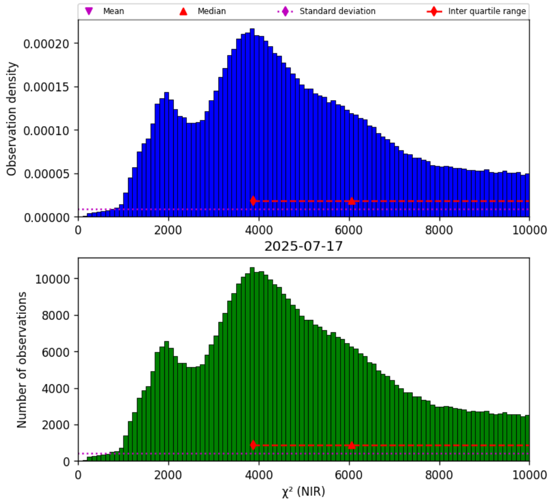
Figure 29: Histogram of “ \chi^2 (NIR)” for 2025-07-16 to 2025-07-18
