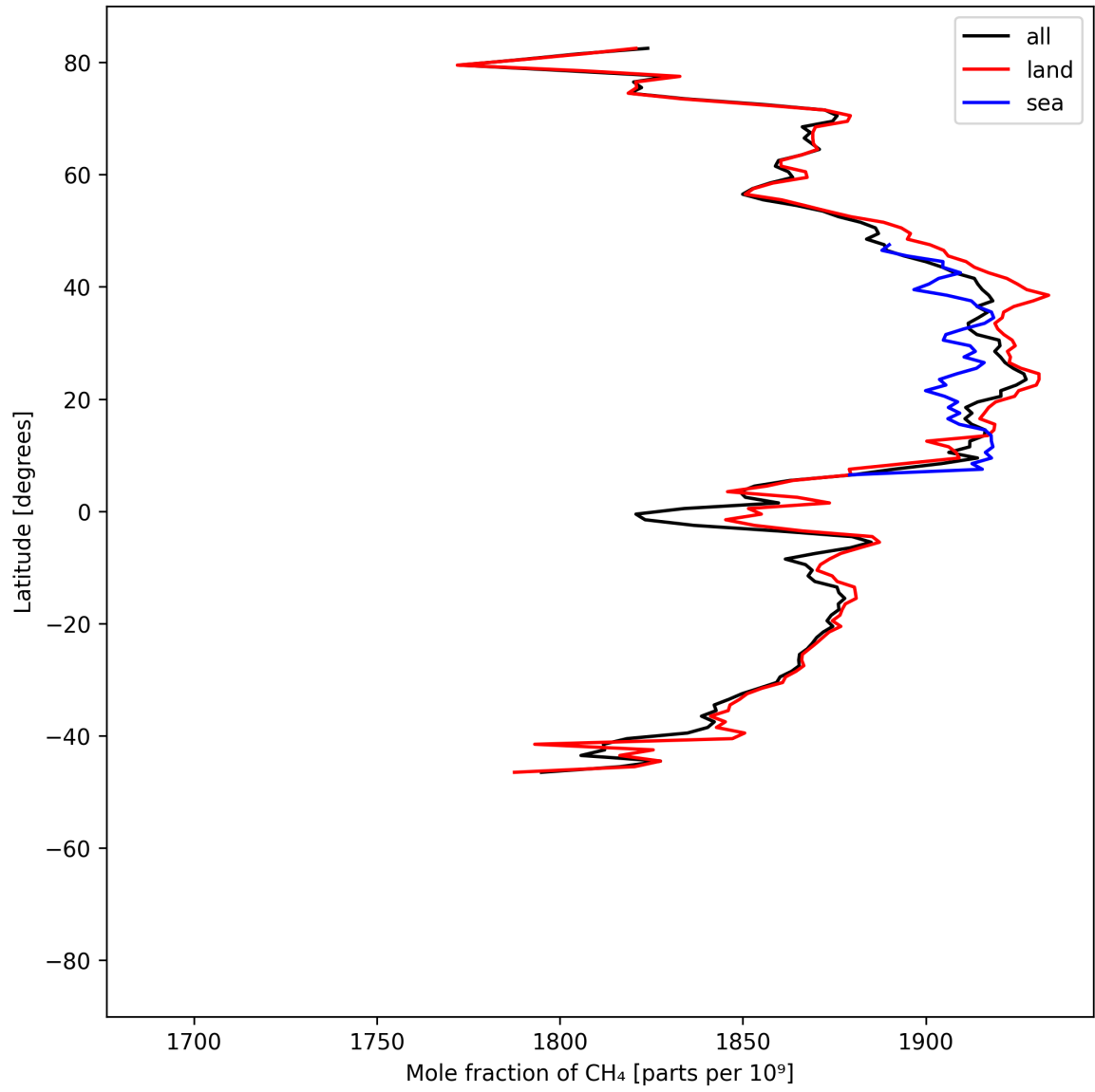
Figure 12: Zonal average of “Mole fraction of \text{CH}_4 ” for 2025-07-16 to 2025-07-18.
