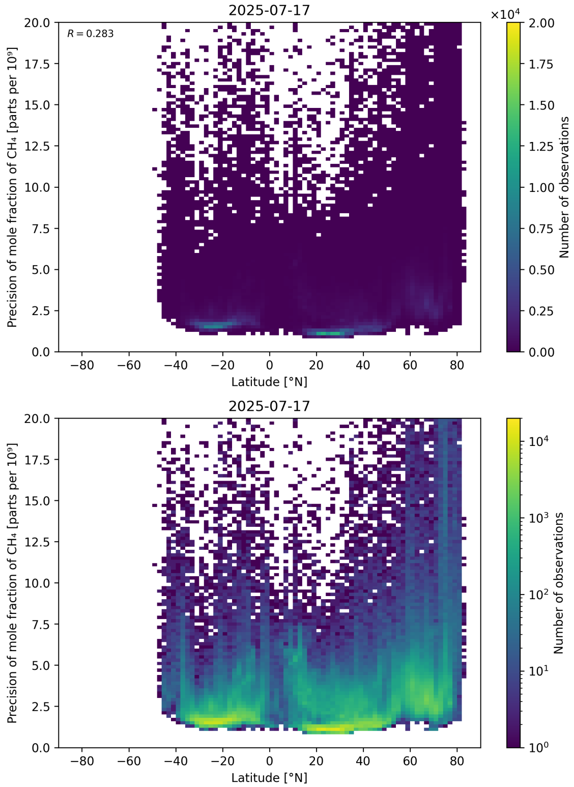
Figure 59: Scatter density plot of “Latitude” against “Precision of mole fraction of \text{CH}_4 ” for 2025-07-16 to 2025-07-18.
