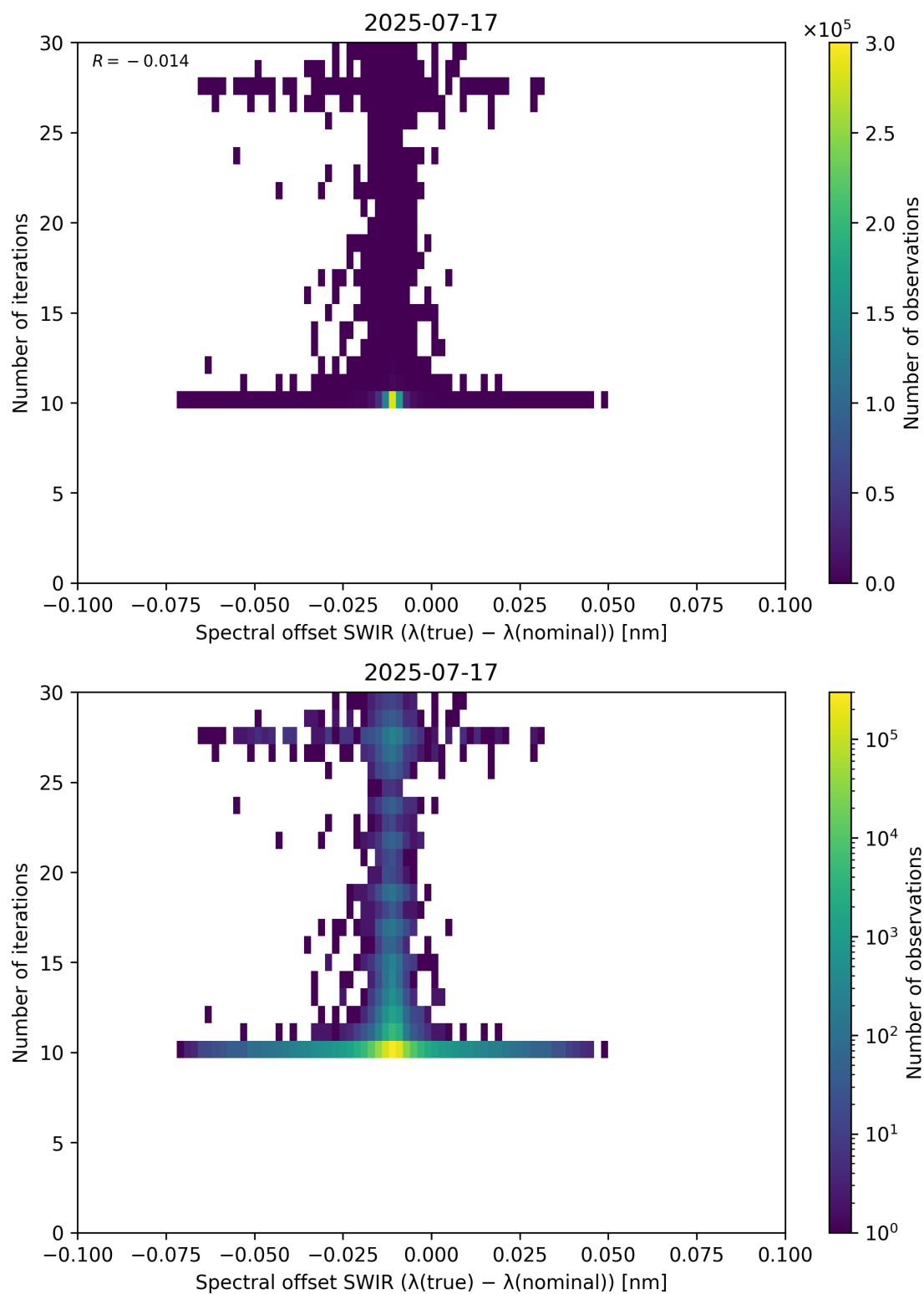
Figure 121: Scatter density plot of “Spectral offset SWIR ( \lambda_{\text{true}} - \lambda_{\text{nominal}} )” against “Number of iterations” for 2025-07-16 to 2025-07-18.
