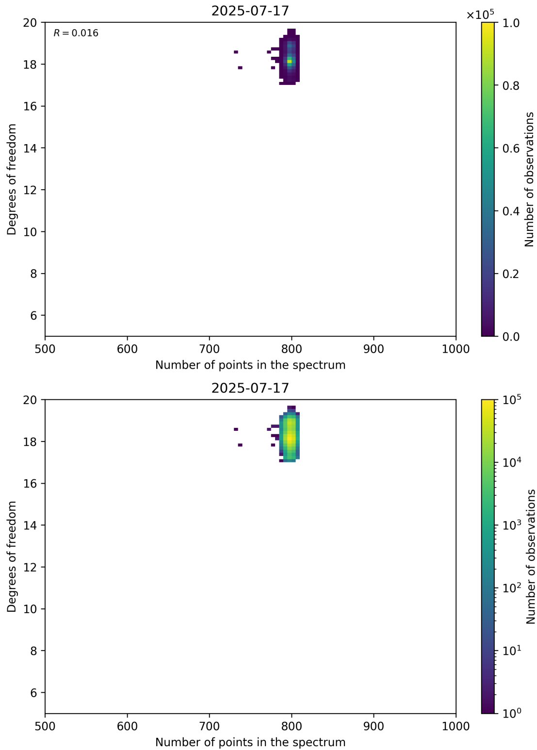
Figure 90: Scatter density plot of “Number of points in the spectrum” against “Degrees of freedom” for 2025-07-16 to 2025-07-18.
