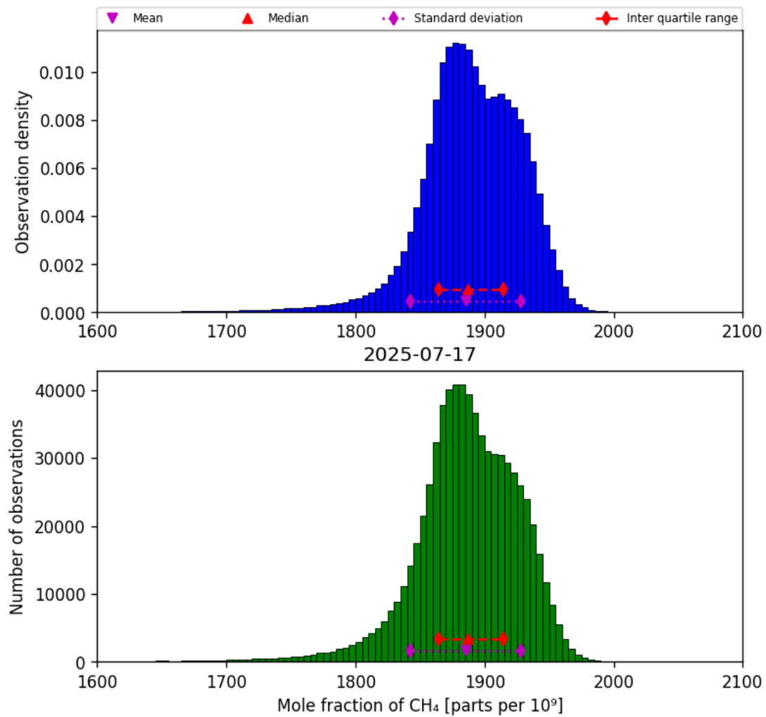
Figure 23: Histogram of “Mole fraction of CH 4 ” for 2025-07-16 to 2025-07-18
