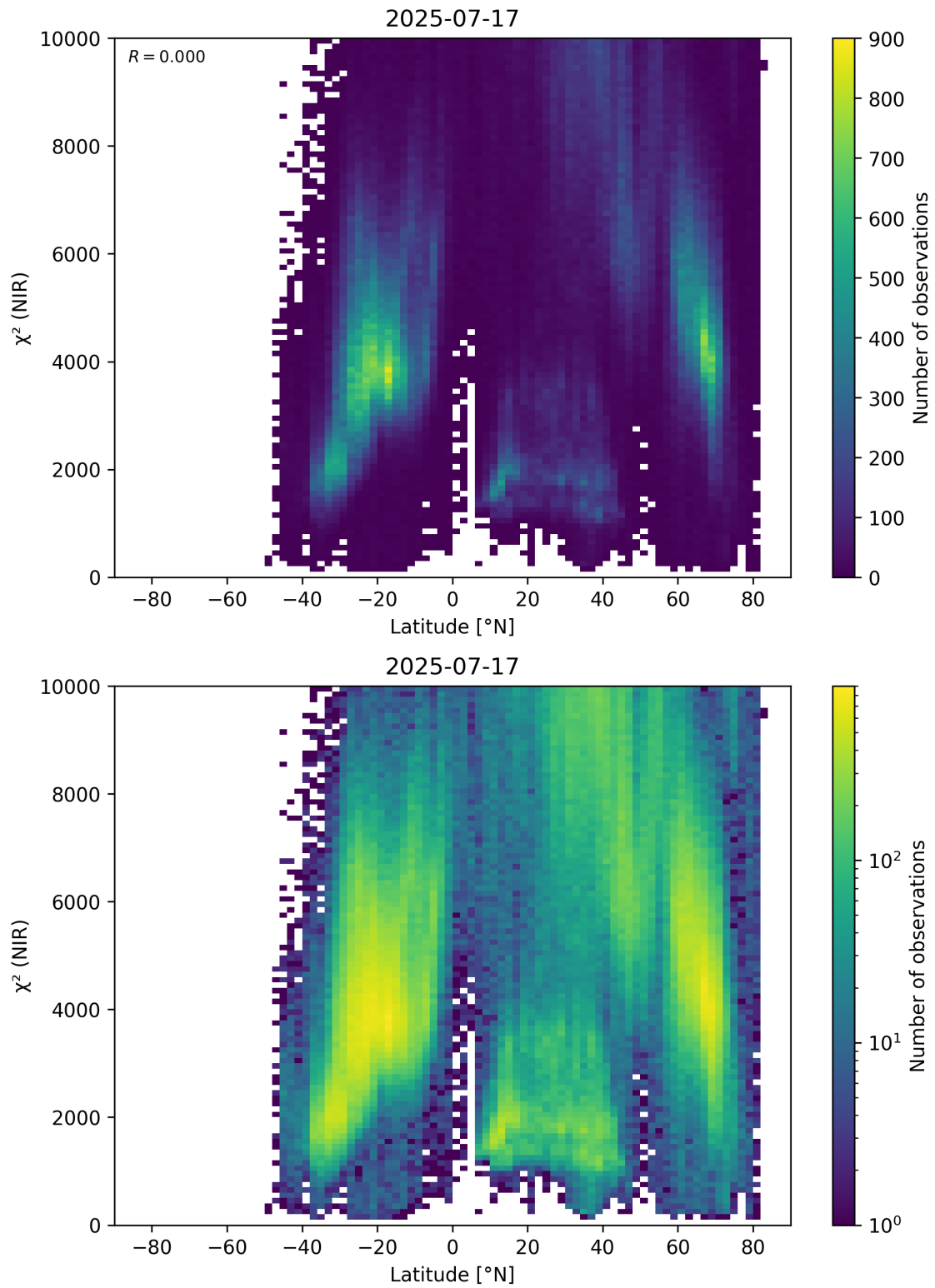
Figure 53: Scatter density plot of “Latitude” against “ \chi^2 (NIR)” for 2025-07-16 to 2025-07-18.
