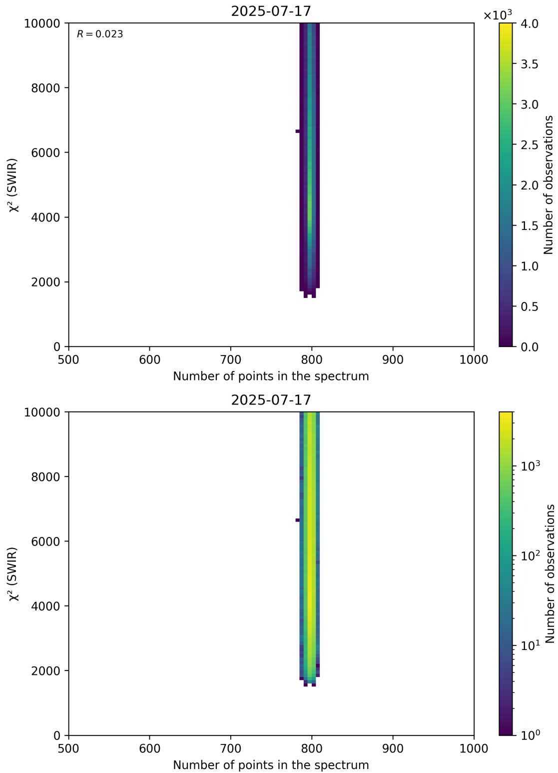
Figure 89: Scatter density plot of “Number of points in the spectrum” against “ \chi^2 (SWIR)” for 2025-07-16 to 2025-07-18.
