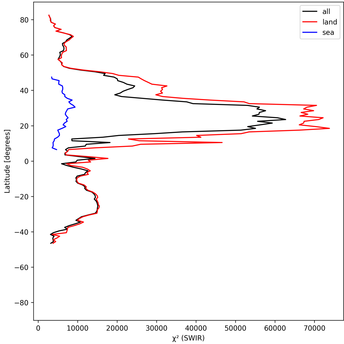
Figure 17: Zonal average of “ \chi^2 (SWIR)” for 2025-07-16 to 2025-07-18.
