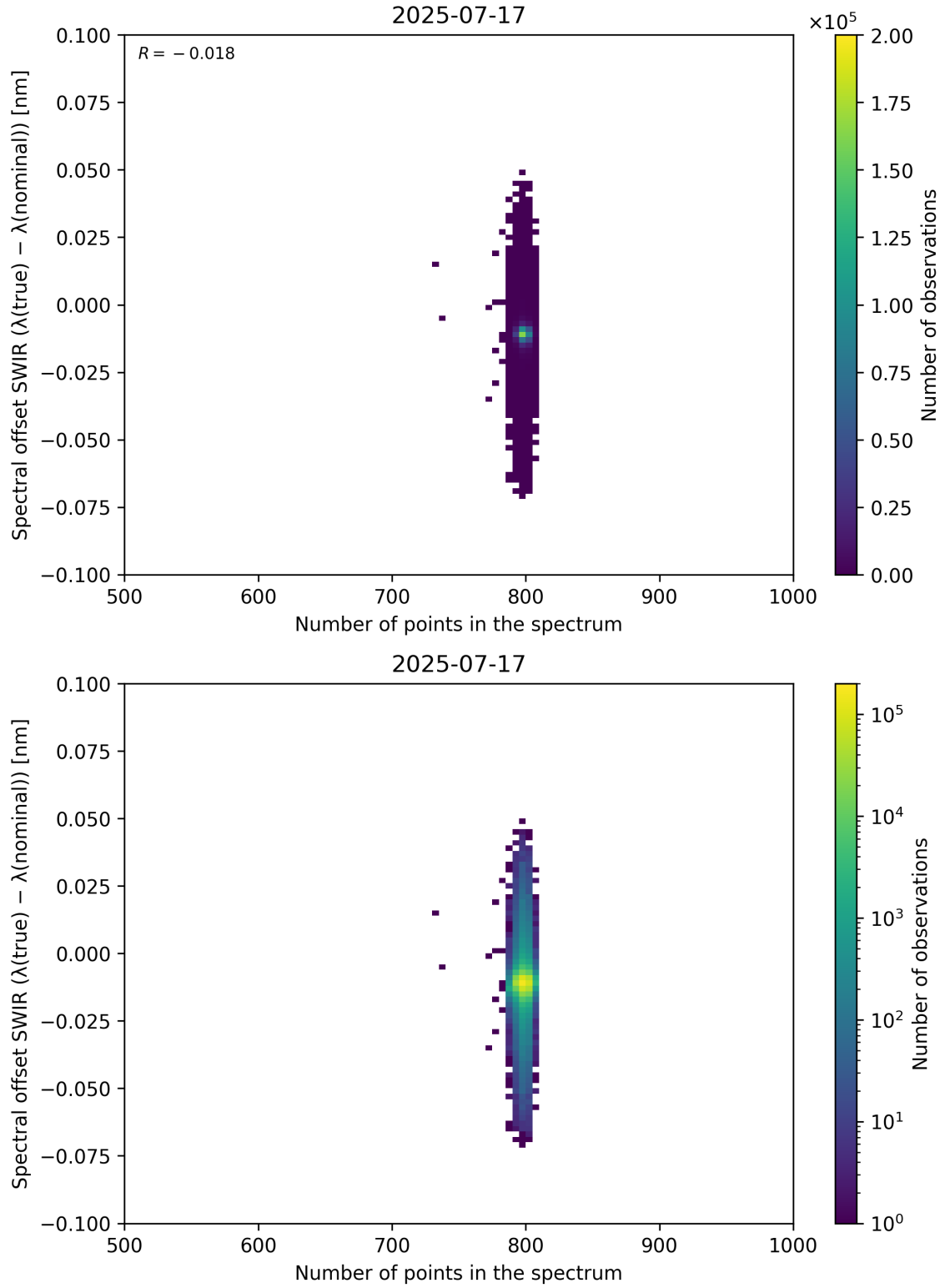
Figure 93: Scatter density plot of “Number of points in the spectrum” against “Spectral offset SWIR ( \lambda_{\text{true}} - \lambda_{\text{nominal}} )” for 2025-07-16 to 2025-07-18.
