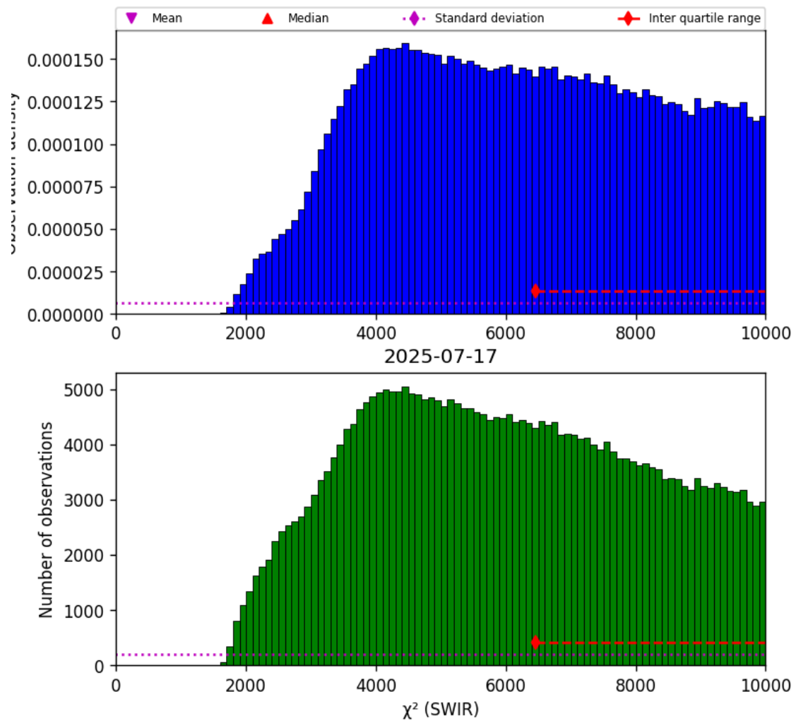
Figure 28: Histogram of “ \chi^2 (SWIR)” for 2025-07-16 to 2025-07-18
