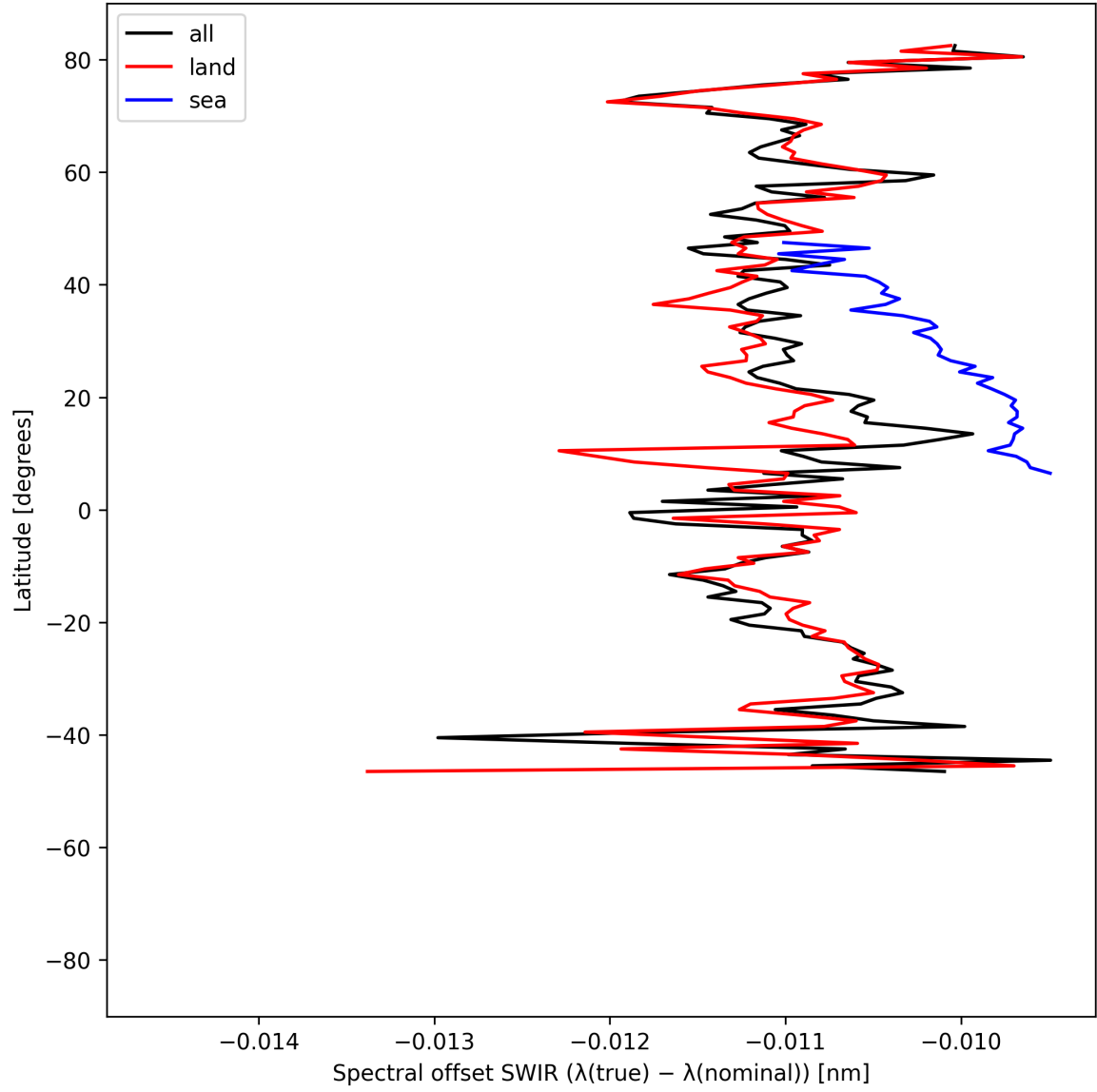
Figure 16: Zonal average of “Spectral offset SWIR ( \lambda_{\text{true}} - \lambda_{\text{nominal}} )” for 2025-07-16 to 2025-07-18.
