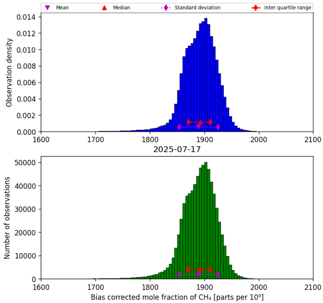
Figure 25: Histogram of “Bias corrected mole fraction of CH 4 ” for 2025-07-16 to 2025-07-18
