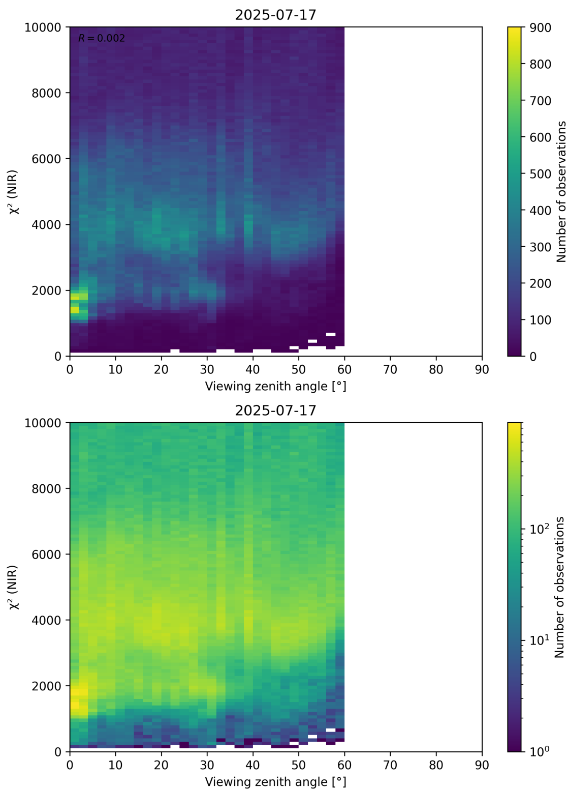
Figure 105: Scatter density plot of “Viewing zenith angle” against “ \chi^2 (NIR)” for 2025-07-16 to 2025-07-18.
