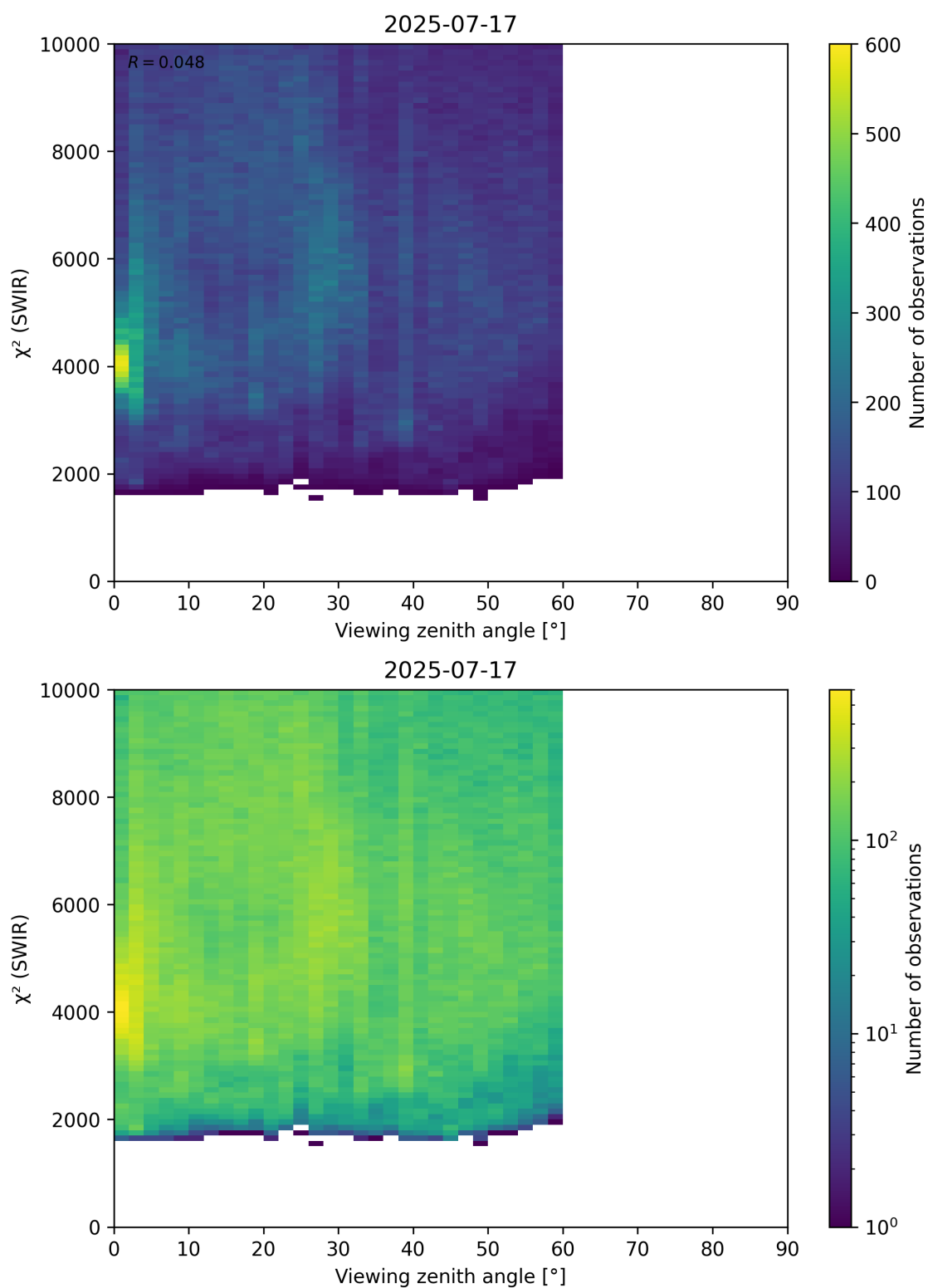
Figure 106: Scatter density plot of “Viewing zenith angle” against “ \chi^2 (SWIR)” for 2025-07-16 to 2025-07-18.
