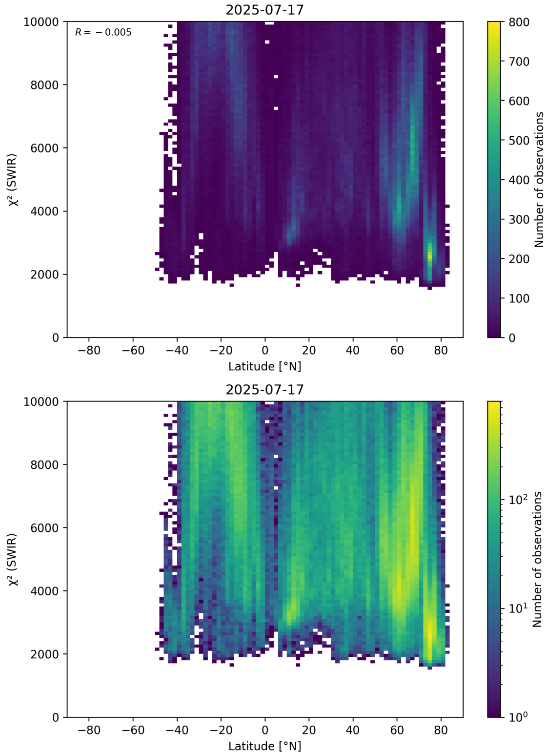
Figure 54: Scatter density plot of “Latitude” against “ \chi^2 (SWIR)” for 2025-07-16 to 2025-07-18.
