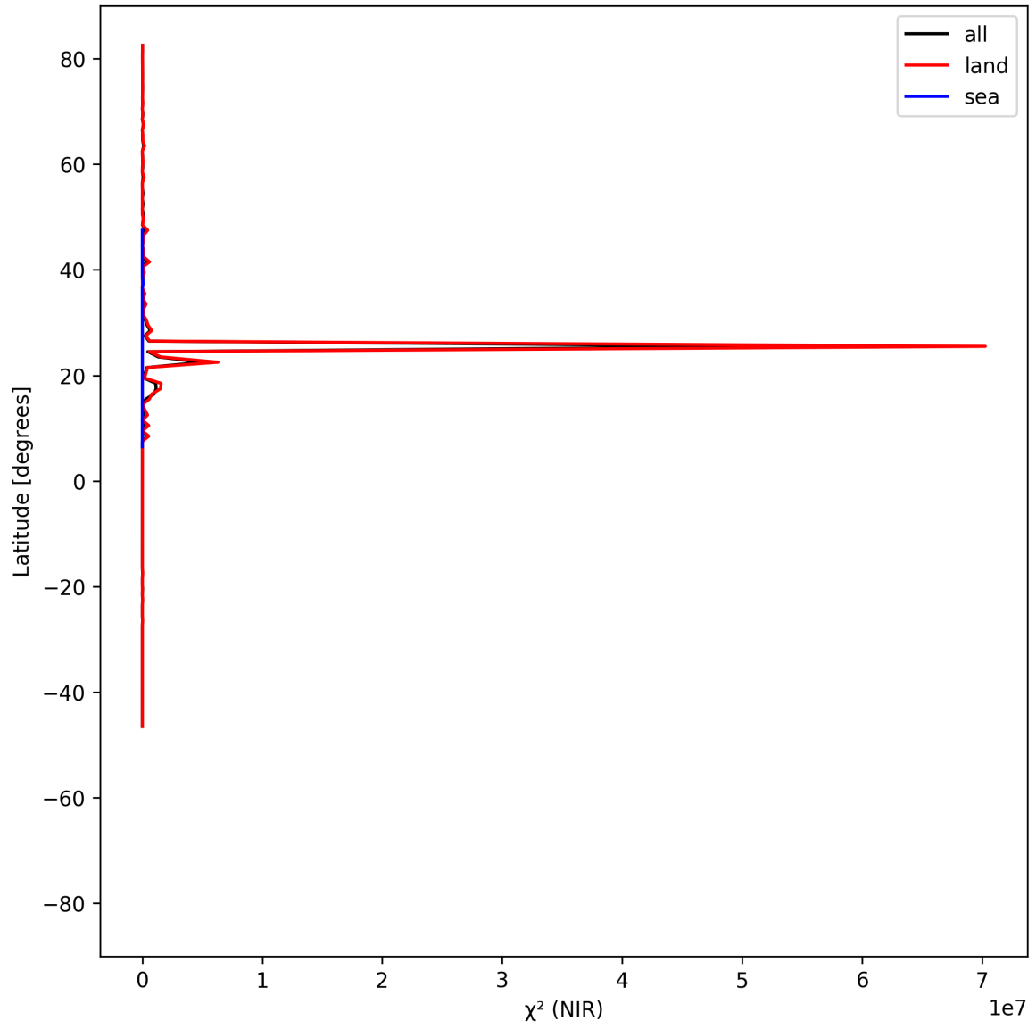
Figure 18: Zonal average of “ \chi^2 (NIR)” for 2025-07-16 to 2025-07-18.
