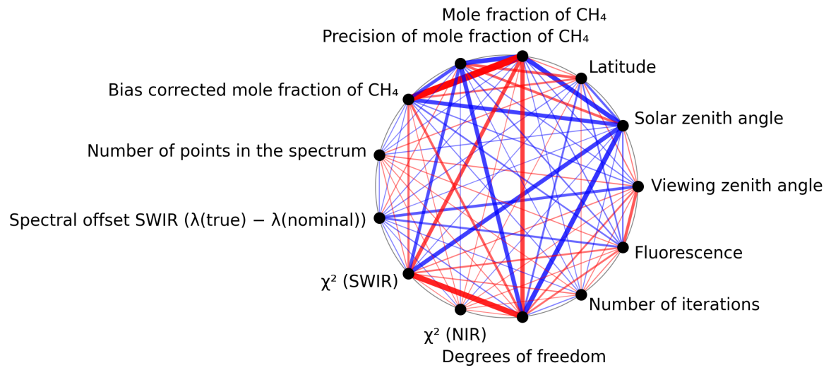
Figure 1: Map of correlation graph for 2025-07-16 to 2025-07-18.
