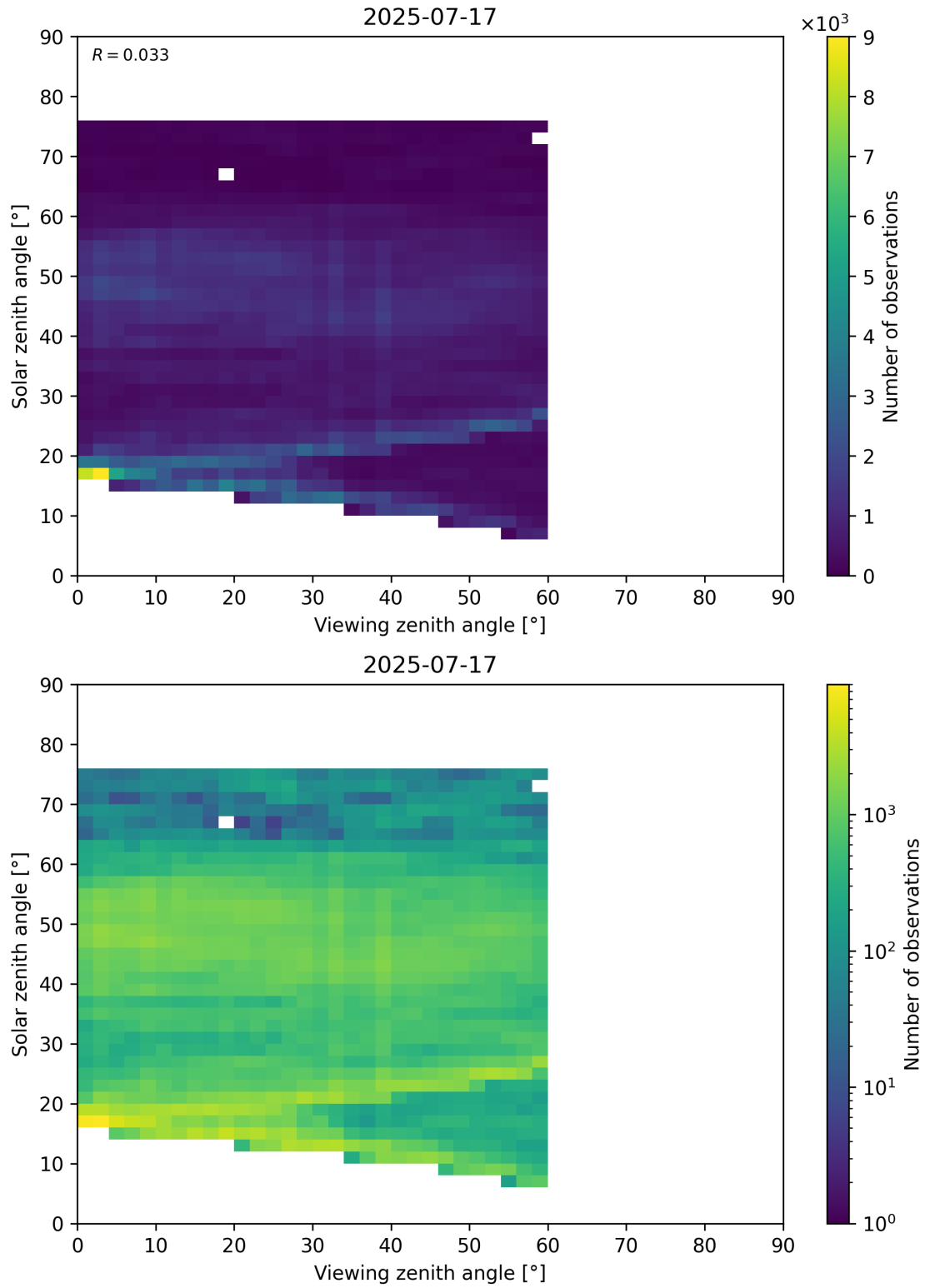
Figure 115: Scatter density plot of “Viewing zenith angle” against “Solar zenith angle” for 2025-07-16 to 2025-07-18.
