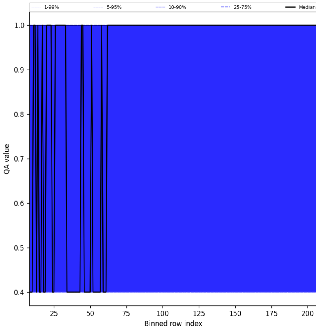
Figure 33: Along track statistics of “QA value” for 2025-07-16 to 2025-07-18
