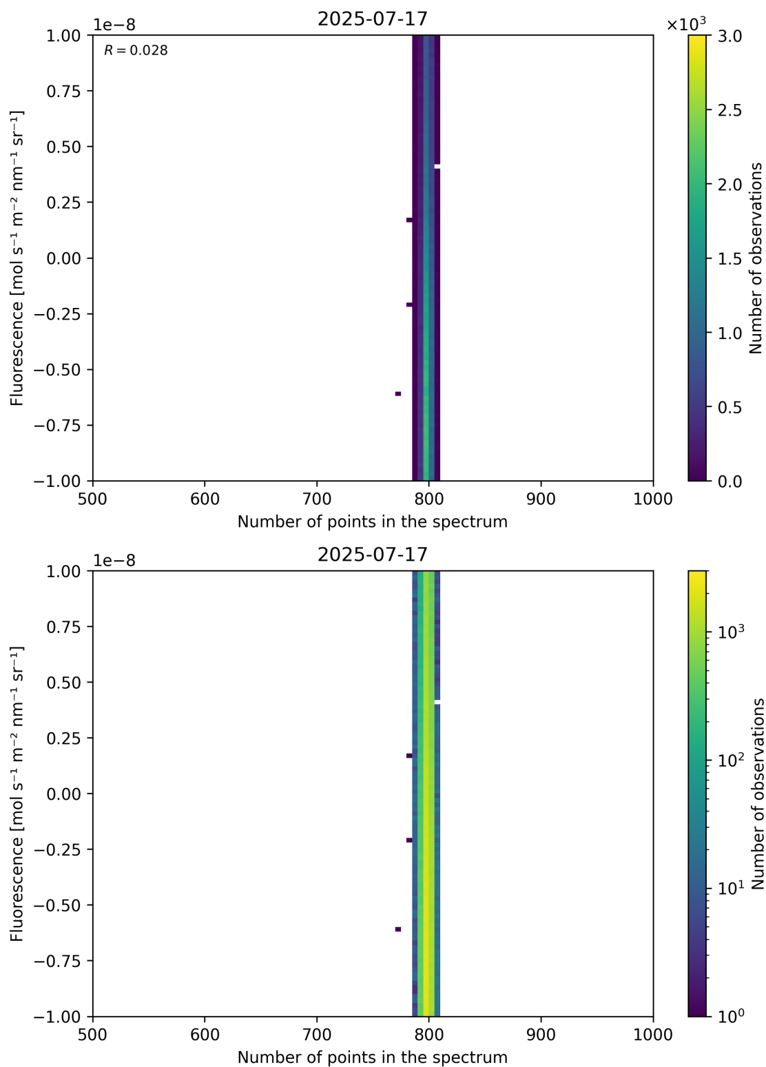
Figure 91: Scatter density plot of “Number of points in the spectrum” against “Fluorescence” for 2025-07-16 to 2025-07-18.
