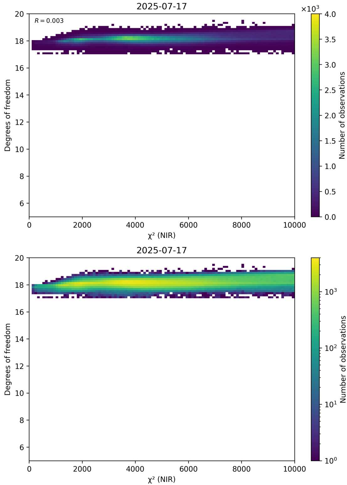
Figure 44: Scatter density plot of “ \chi^2 (NIR)” against “Degrees of freedom” for 2025-07-16 to 2025-07-18.
