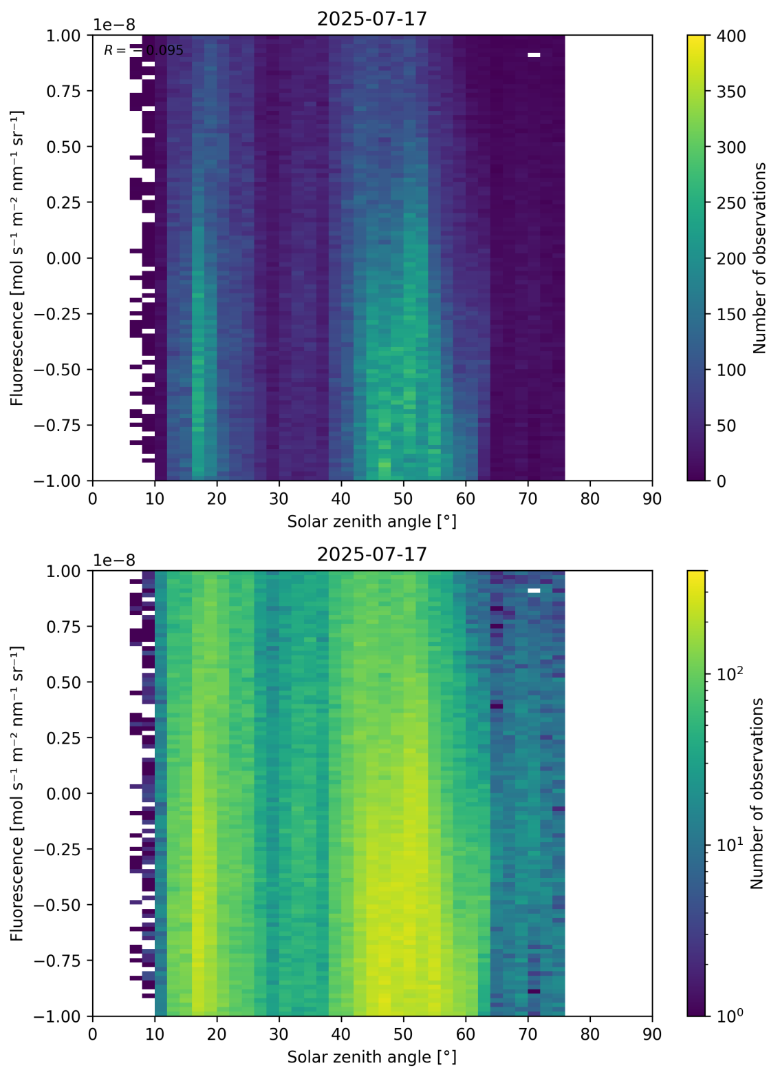
Figure 97: Scatter density plot of “Solar zenith angle” against “Fluorescence” for 2025-07-16 to 2025-07-18.
