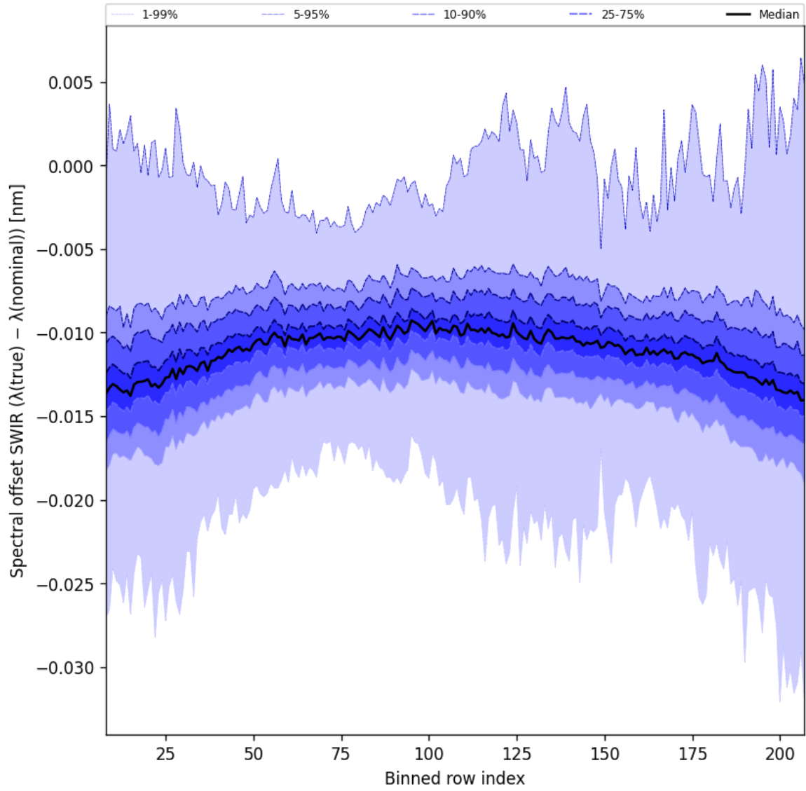
Figure 38: Along track statistics of “Spectral offset SWIR ( \lambda_{\text{true}} - \lambda_{\text{nominal}} )” for 2025-07-16 to 2025-07-18
