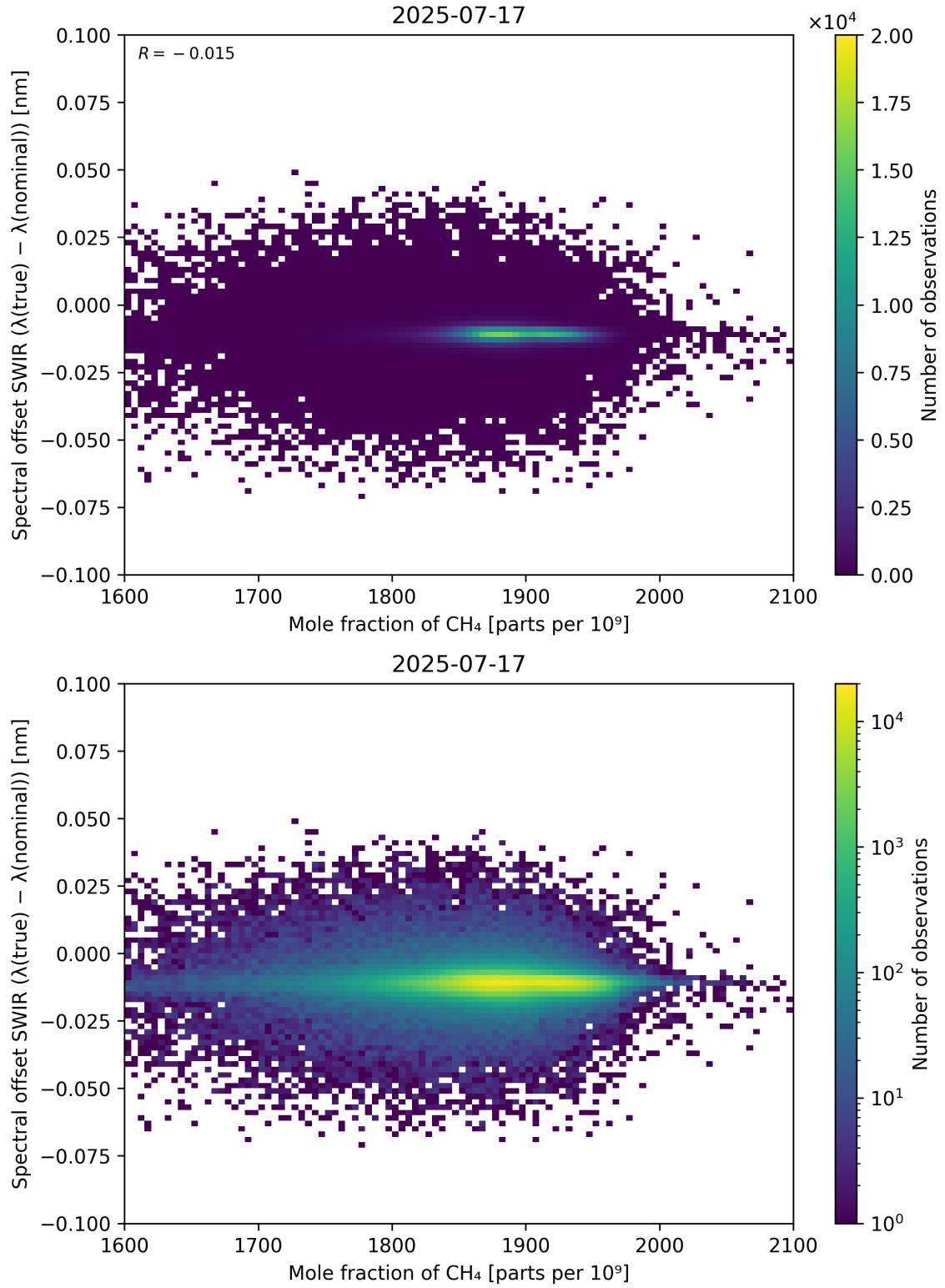
Figure 86: Scatter density plot of “Mole fraction of CH 4 ” against “Spectral offset SWIR ( \lambda_{\text{true}} - \lambda_{\text{nominal}} )” for 2025-07-16 to 2025-07-18.
