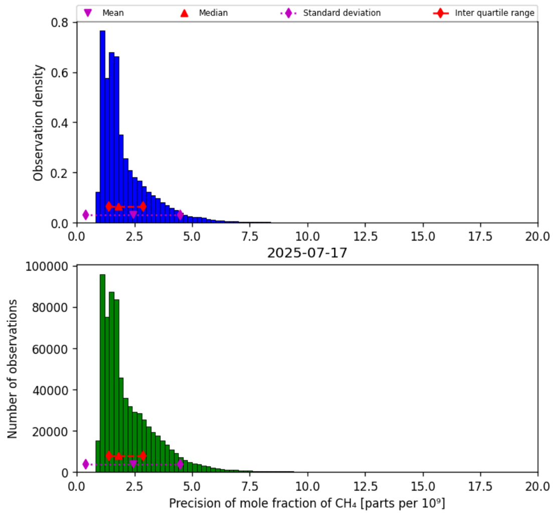
Figure 24: Histogram of “Precision of mole fraction of CH 4 ” for 2025-07-16 to 2025-07-18
