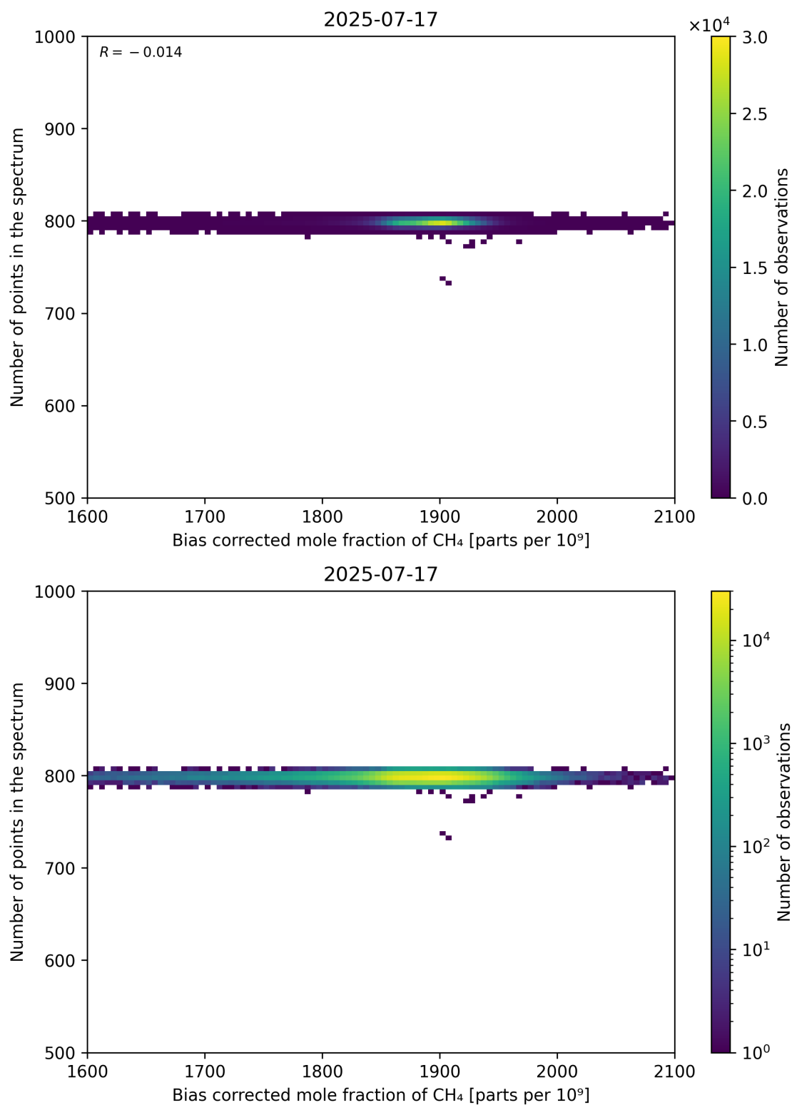
Figure 68: Scatter density plot of “Bias corrected mole fraction of CH 4 ” against “Number of points in the spectrum” for 2025-07-16 to 2025-07-18.
