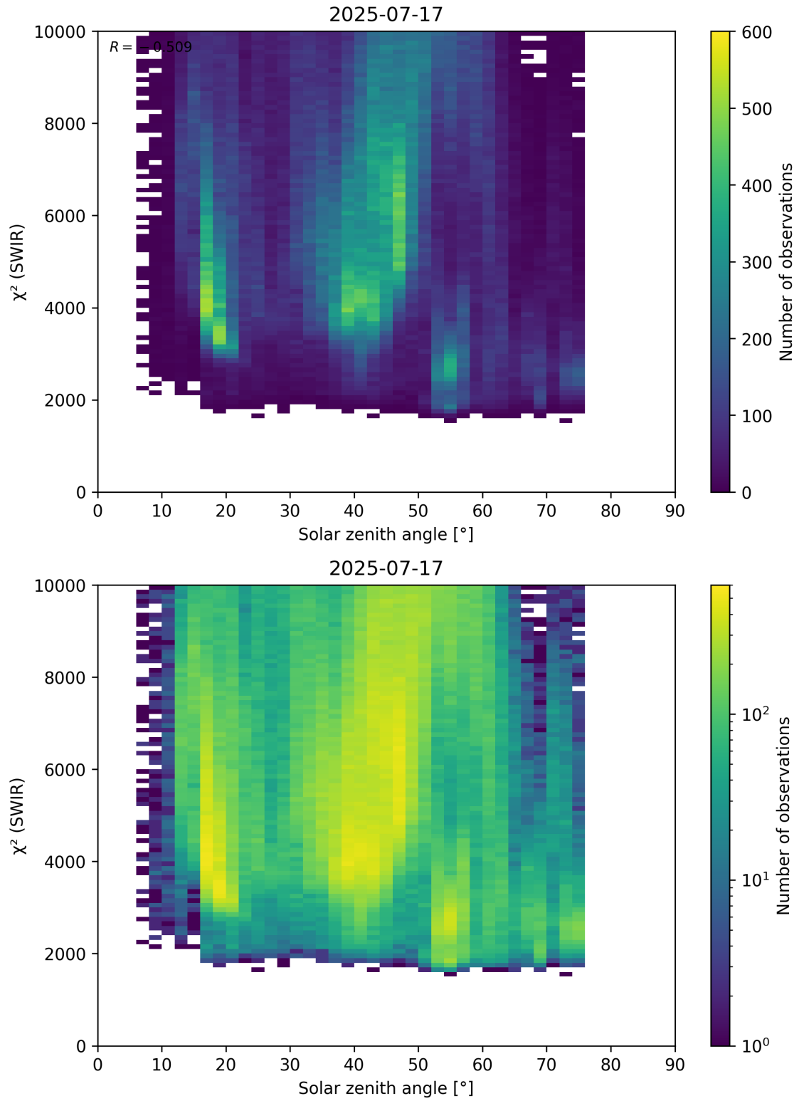
Figure 95: Scatter density plot of “Solar zenith angle” against “ \chi^2 (SWIR)” for 2025-07-16 to 2025-07-18.
