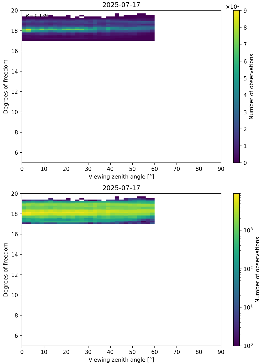
Figure 107: Scatter density plot of “Viewing zenith angle” against “Degrees of freedom” for 2025-07-16 to 2025-07-18.
