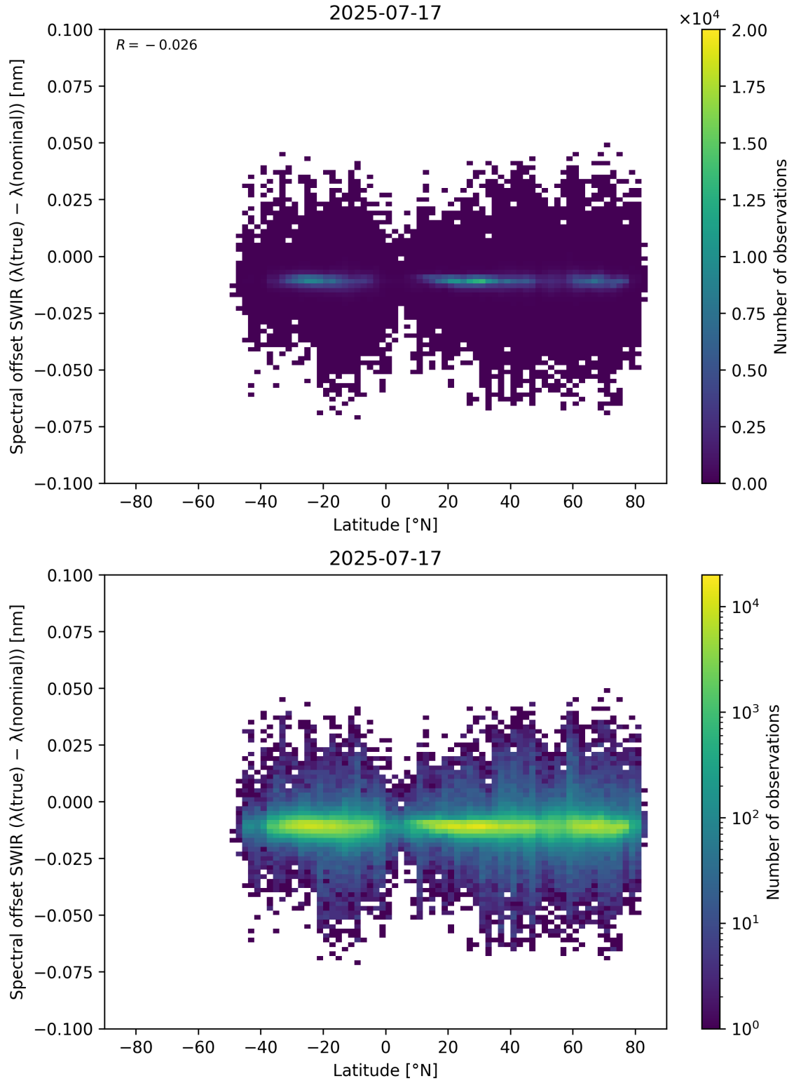
Figure 62: Scatter density plot of “Latitude” against “Spectral offset SWIR ( \lambda_{\text{true}} - \lambda_{\text{nominal}} )” for 2025-07-16 to 2025-07-18.
