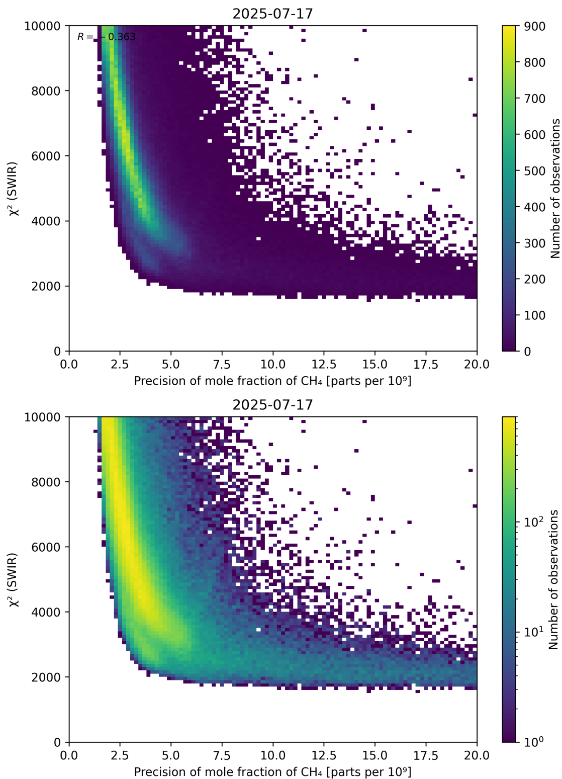
Figure 79: Scatter density plot of “Precision of mole fraction of \text{CH}_4 ” against “ \chi^2 (SWIR)” for 2025-07-16 to 2025-07-18.
