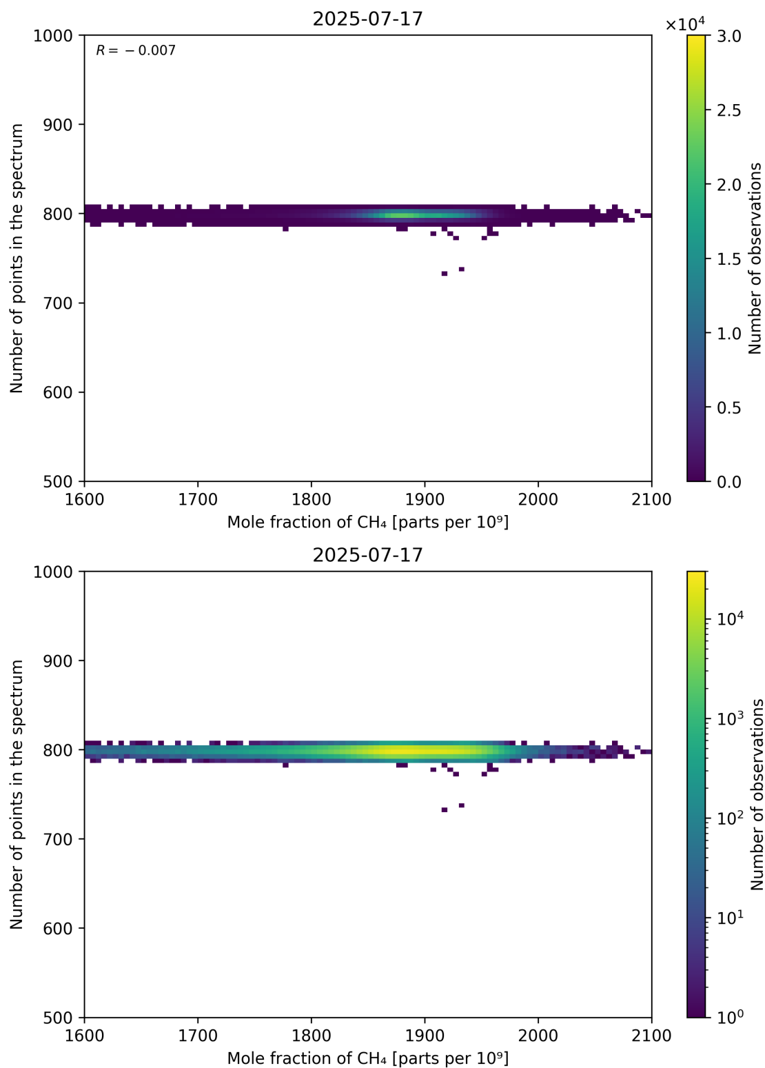
Figure 77: Scatter density plot of “Mole fraction of CH 4 ” against “Number of points in the spectrum” for 2025-07-16 to 2025-07-18.
