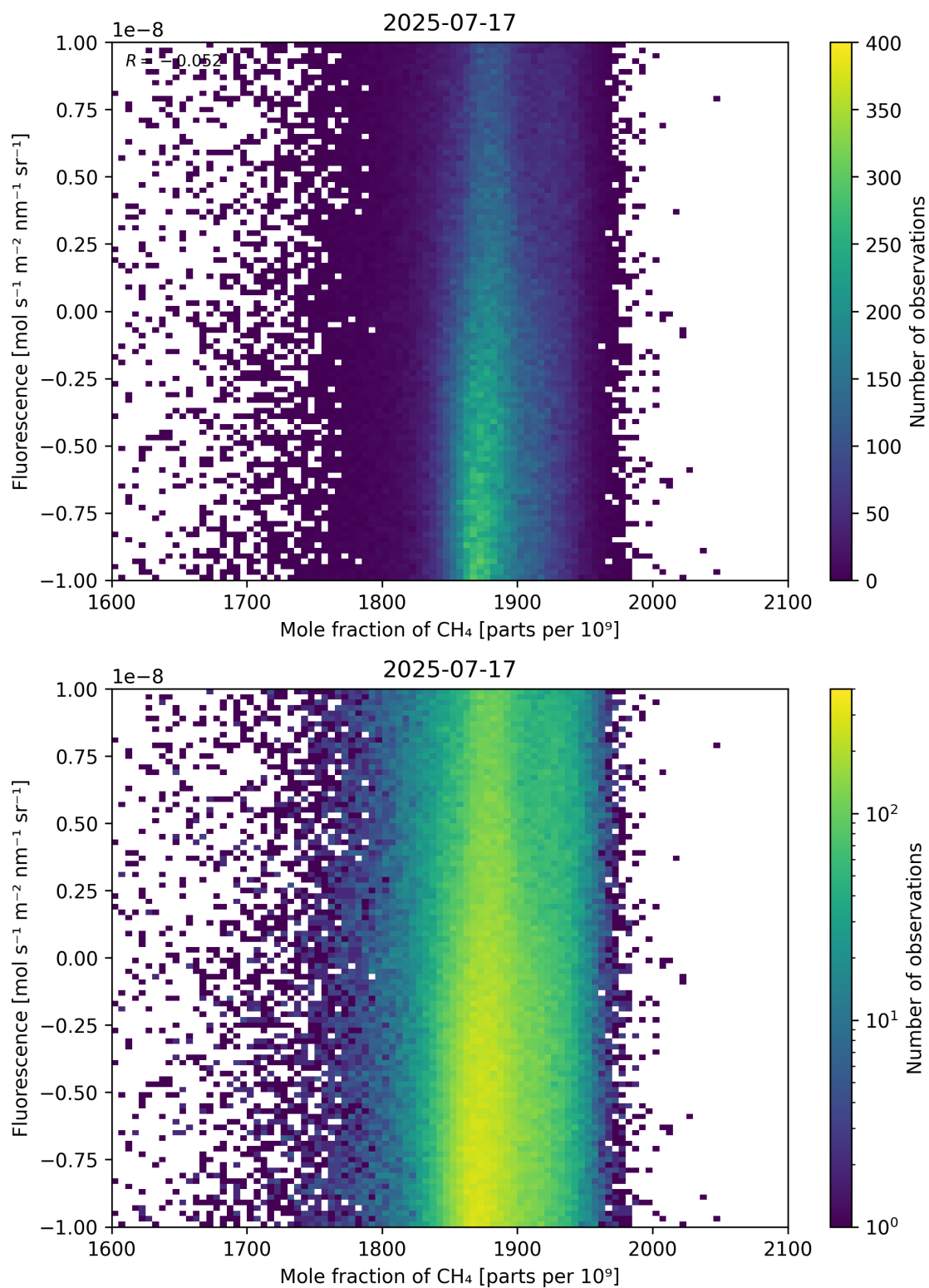
Figure 73: Scatter density plot of “Mole fraction of \text{CH}_4 ” against “Fluorescence” for 2025-07-16 to 2025-07-18.
