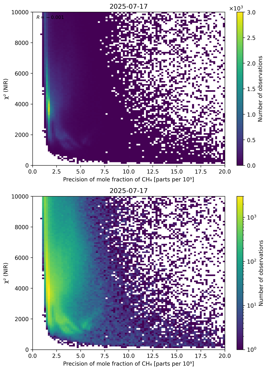
Figure 78: Scatter density plot of “Precision of mole fraction of CH 4 ” against “ \chi^2 (NIR)” for 2025-07-16 to 2025-07-18.
