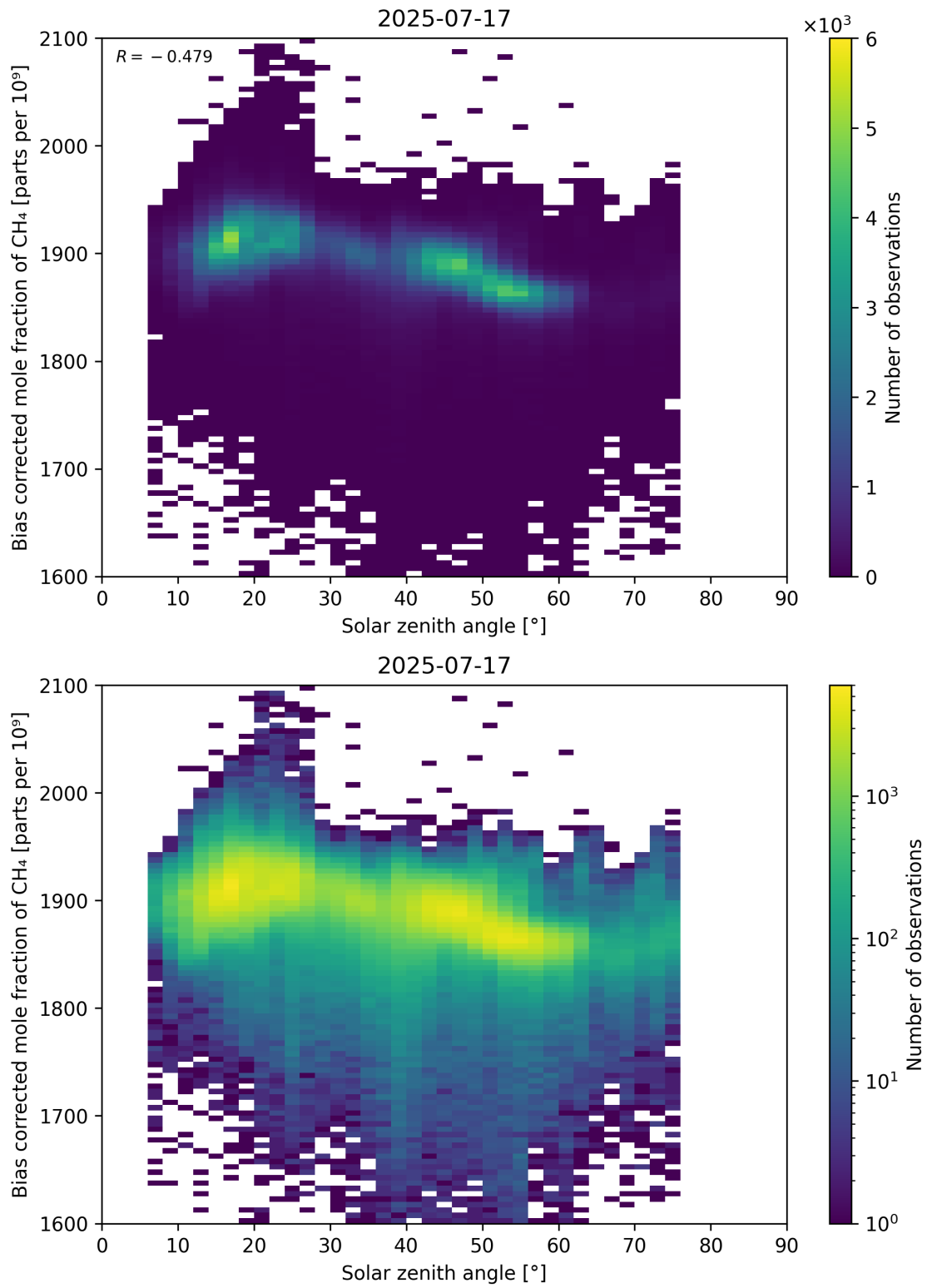
Figure 100: Scatter density plot of “Solar zenith angle” against “Bias corrected mole fraction of \text{CH}_4 ” for 2025-07-16 to 2025-07-18.
