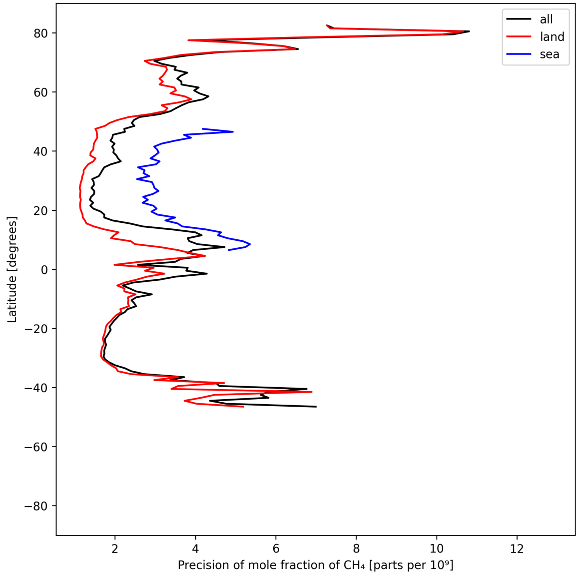
Figure 13: Zonal average of “Precision of mole fraction of CH 4 ” for 2025-07-16 to 2025-07-18.
