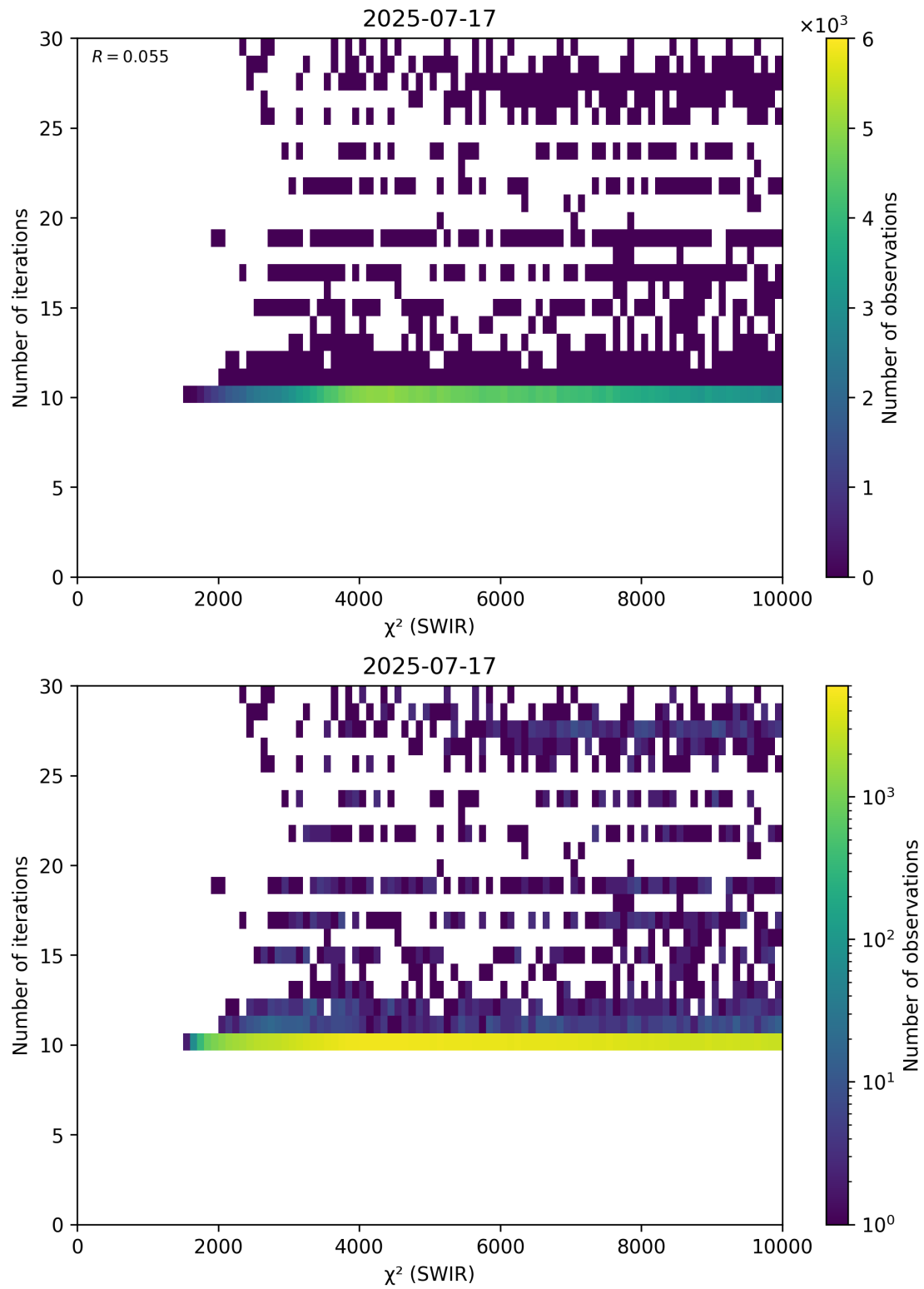
Figure 50: Scatter density plot of “ \chi^2 (SWIR)” against “Number of iterations” for 2025-07-16 to 2025-07-18.
