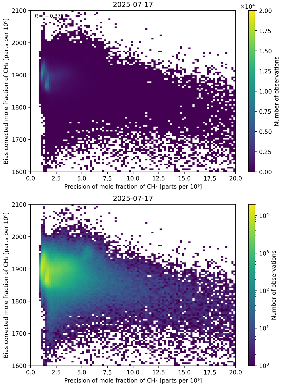
Figure 82: Scatter density plot of “Precision of mole fraction of CH 4 ” against “Bias corrected mole fraction of CH 4 ” for 2025-07-16 to 2025-07-18.
