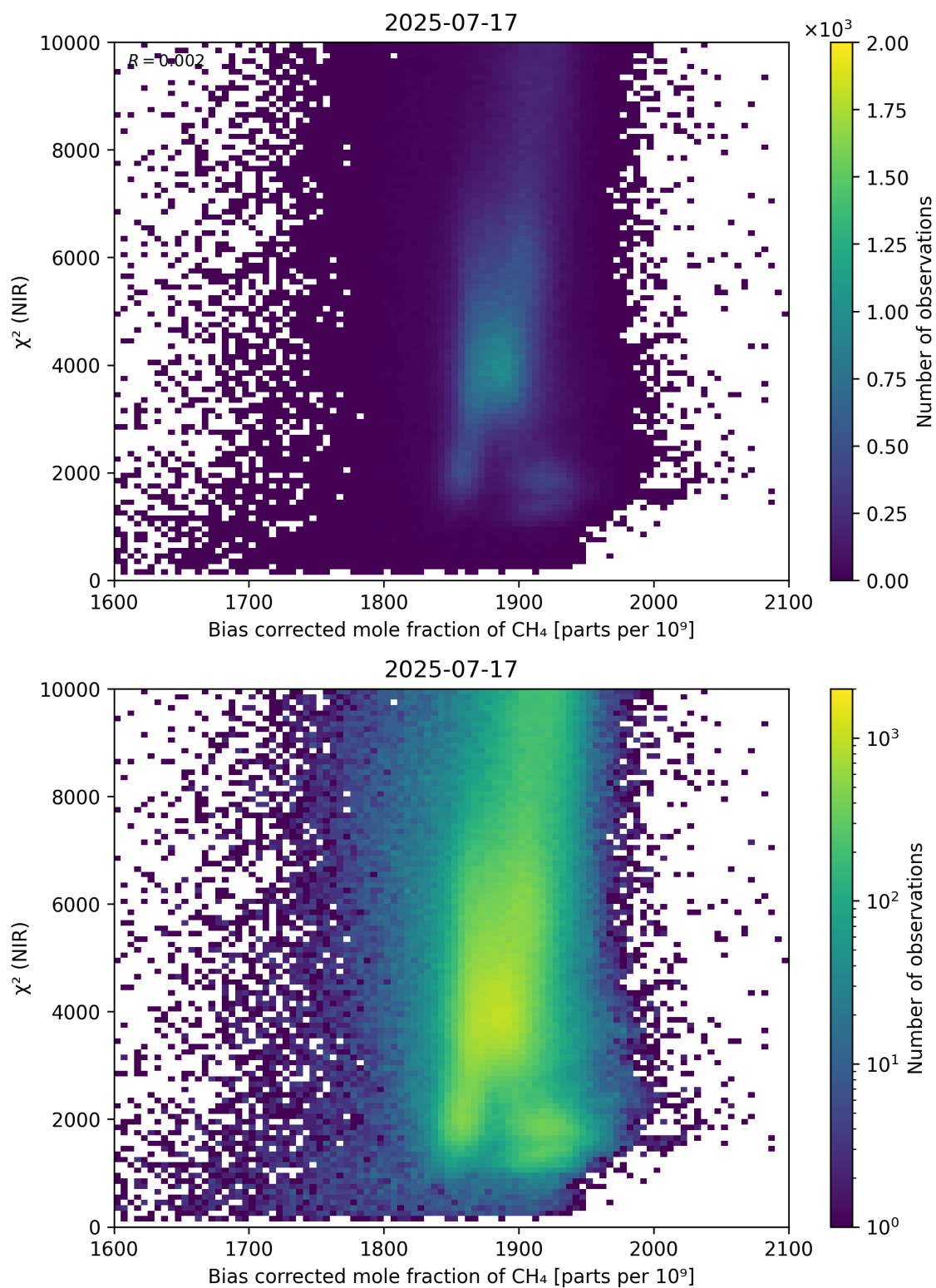
Figure 63: Scatter density plot of “Bias corrected mole fraction of CH 4 ” against “ \chi^2 (NIR)” for 2025-07-16 to 2025-07-18.
