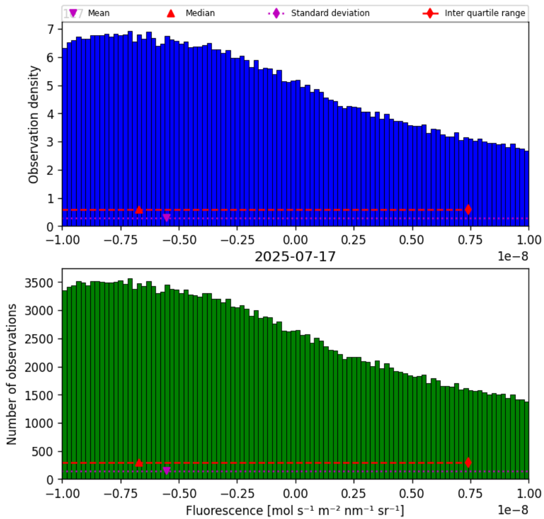
Figure 32: Histogram of “Fluorescence” for 2025-07-16 to 2025-07-18
