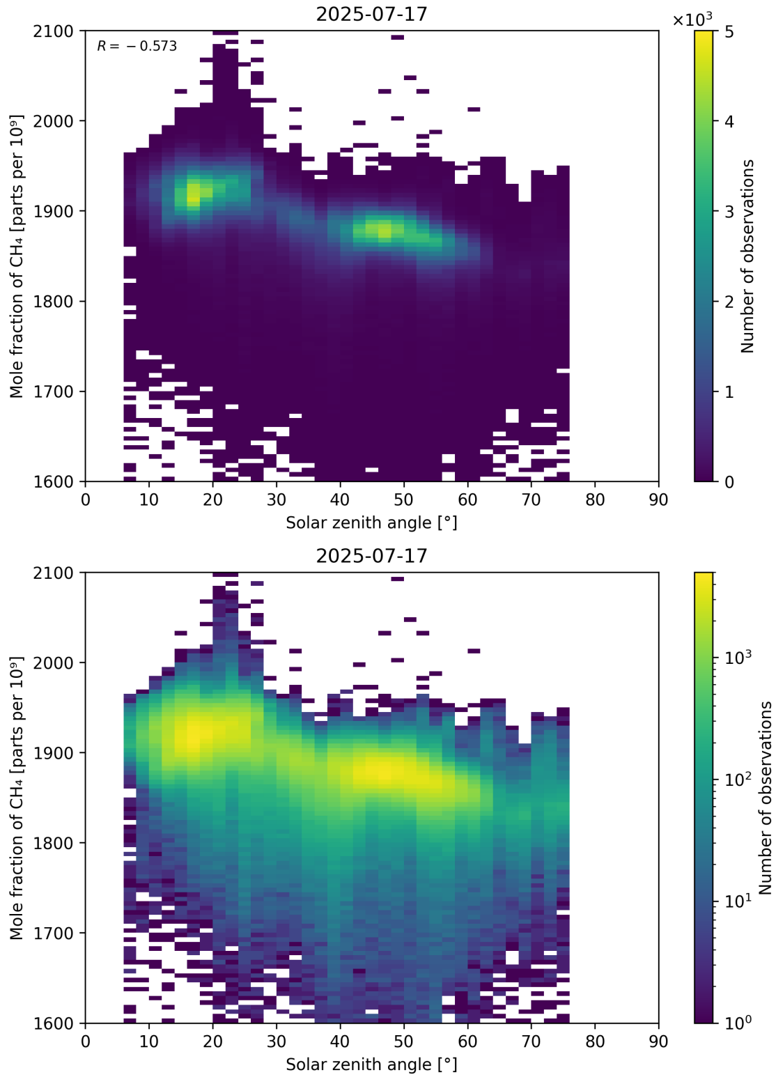
Figure 99: Scatter density plot of “Solar zenith angle” against “Mole fraction of CH 4 ” for 2025-07-16 to 2025-07-18.
