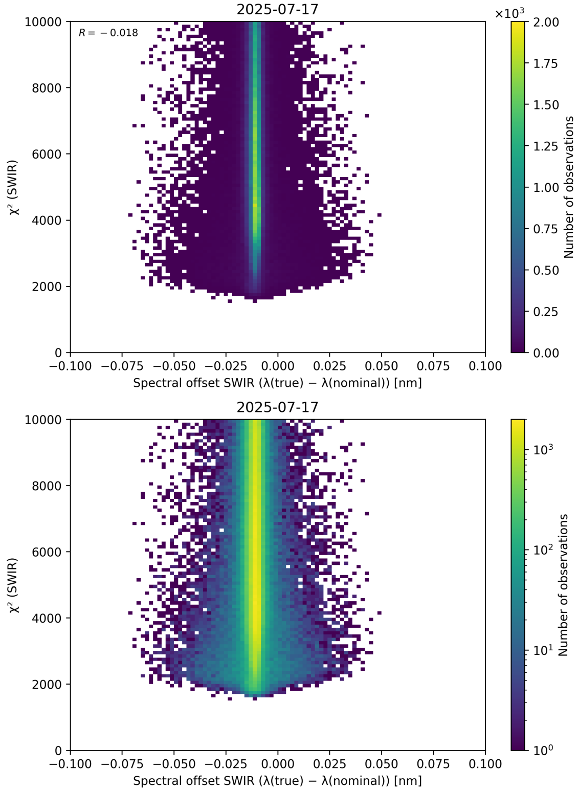
Figure 118: Scatter density plot of “Spectral offset SWIR ( \lambda_{\text{true}} - \lambda_{\text{nominal}} )” against “ \chi^2 (SWIR)” for 2025-07-16 to 2025-07-18.
