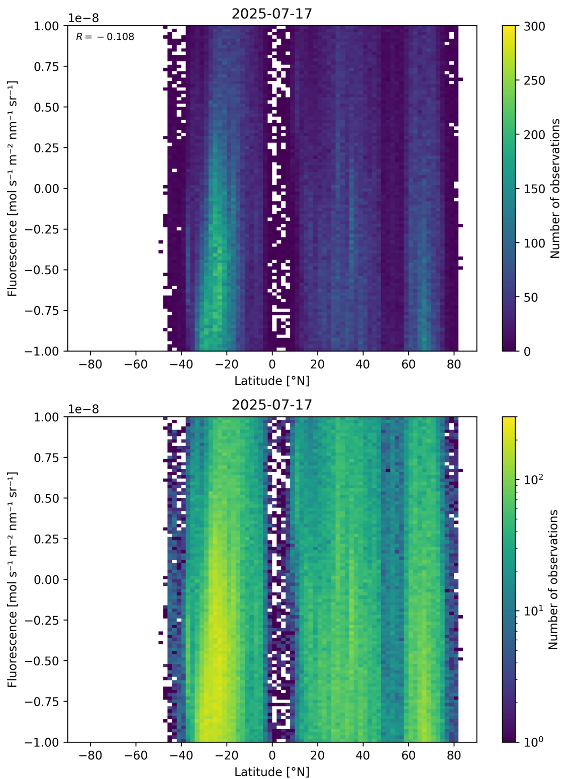
Figure 56: Scatter density plot of “Latitude” against “Fluorescence” for 2025-07-16 to 2025-07-18.
