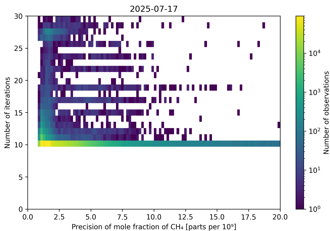
Figure 83: Scatter density plot of “Precision of mole fraction of \text{CH}_4 ” against “Number of iterations” for 2025-07-16 to 2025-07-18.
