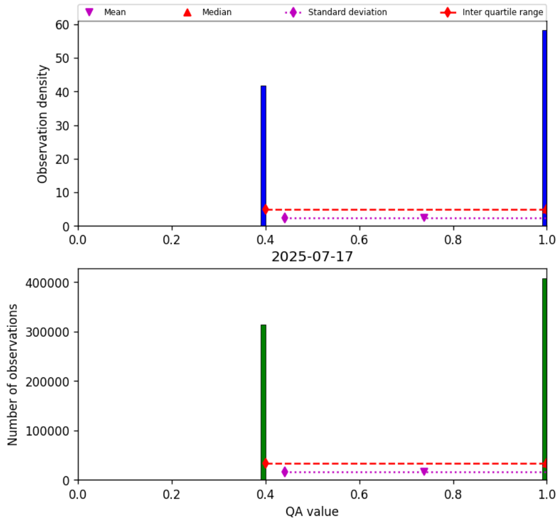
Figure 22: Histogram of “QA value” for 2025-07-16 to 2025-07-18
