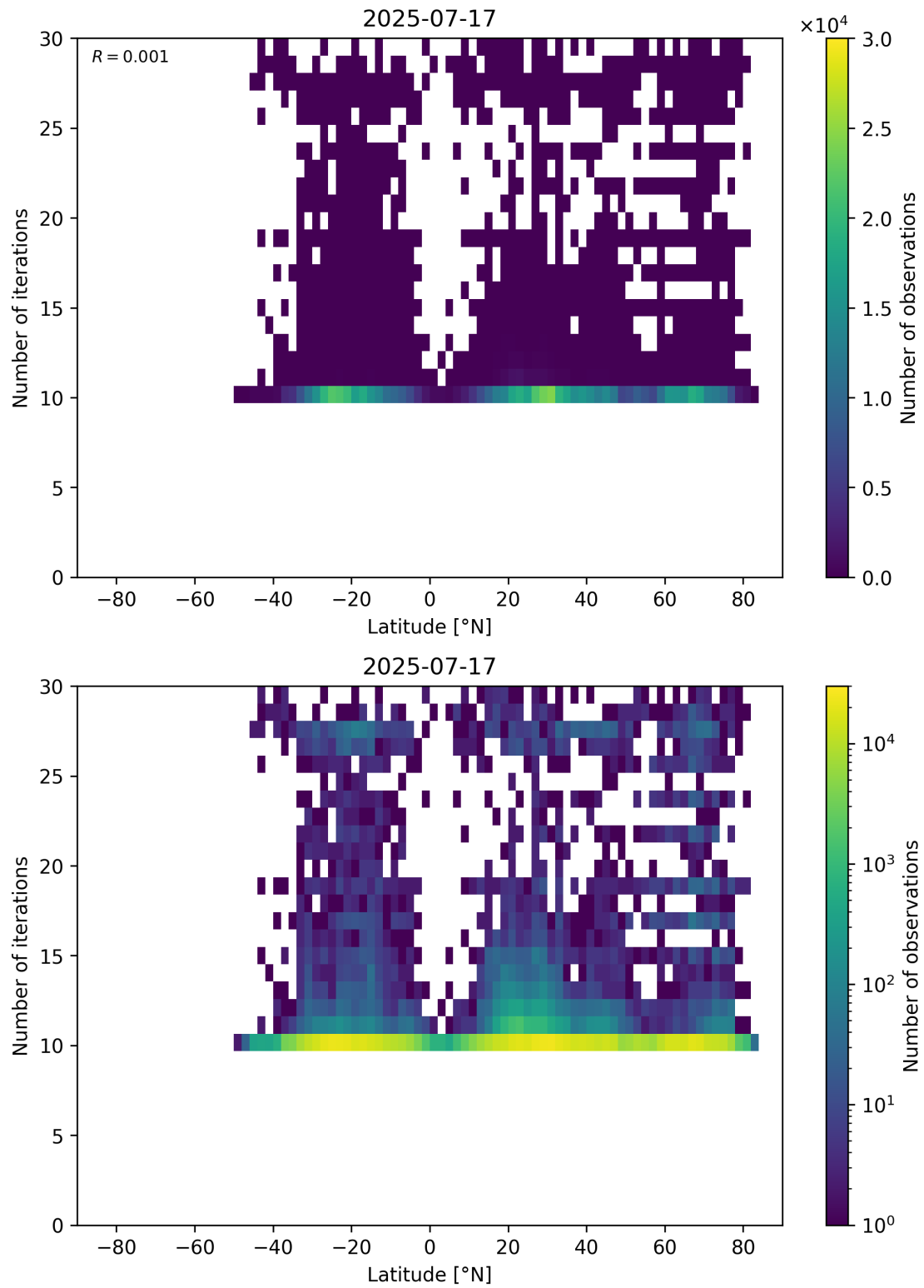
Figure 60: Scatter density plot of “Latitude” against “Number of iterations” for 2025-07-16 to 2025-07-18.
