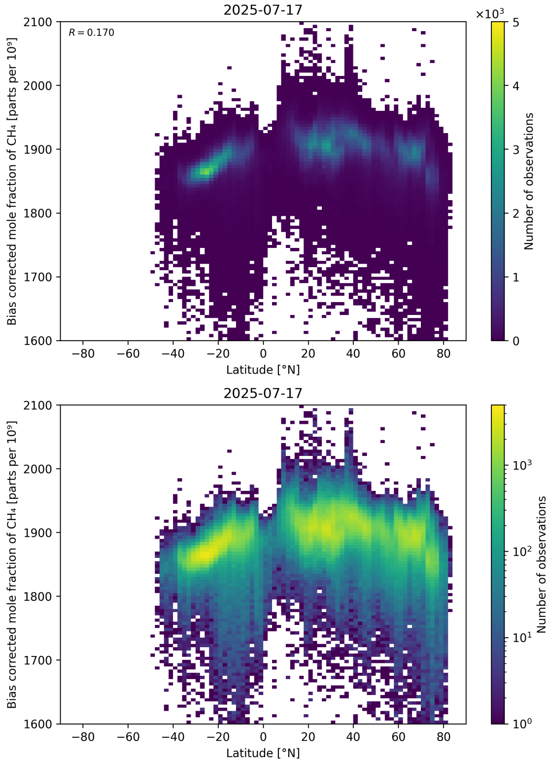
Figure 58: Scatter density plot of “Latitude” against “Bias corrected mole fraction of CH 4 ” for 2025-07-16 to 2025-07-18.
