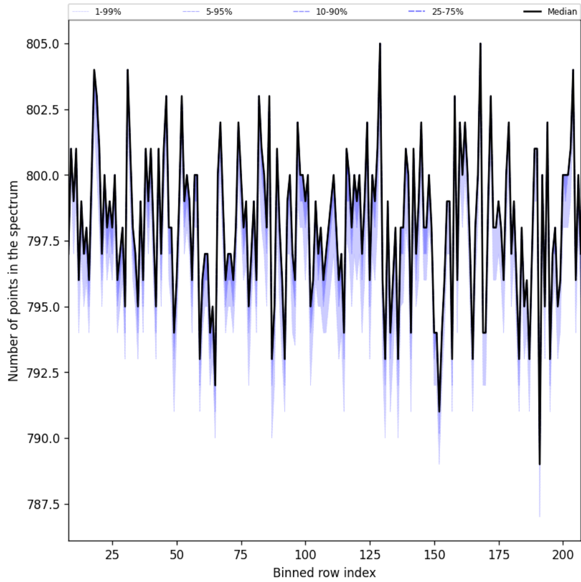
Figure 37: Along track statistics of “Number of points in the spectrum” for 2025-07-16 to 2025-07-18
