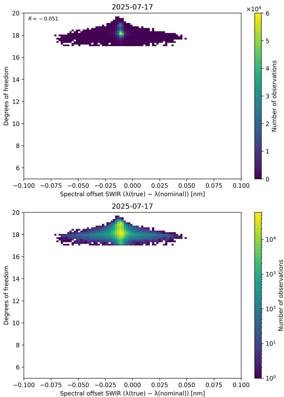
Figure 119: Scatter density plot of “Spectral offset SWIR ( \lambda_{\text{true}} - \lambda_{\text{nominal}} )” against “Degrees of freedom” for 2025-07-16 to 2025-07-18.
