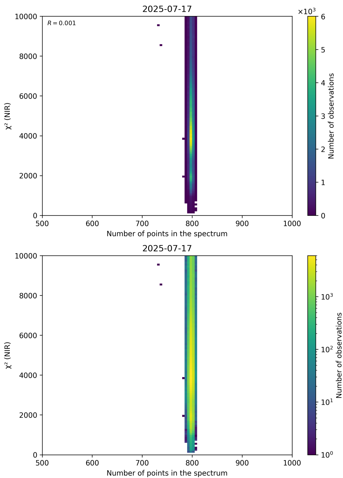
Figure 88: Scatter density plot of “Number of points in the spectrum” against “ \chi^2 (NIR)” for 2025-07-16 to 2025-07-18.
