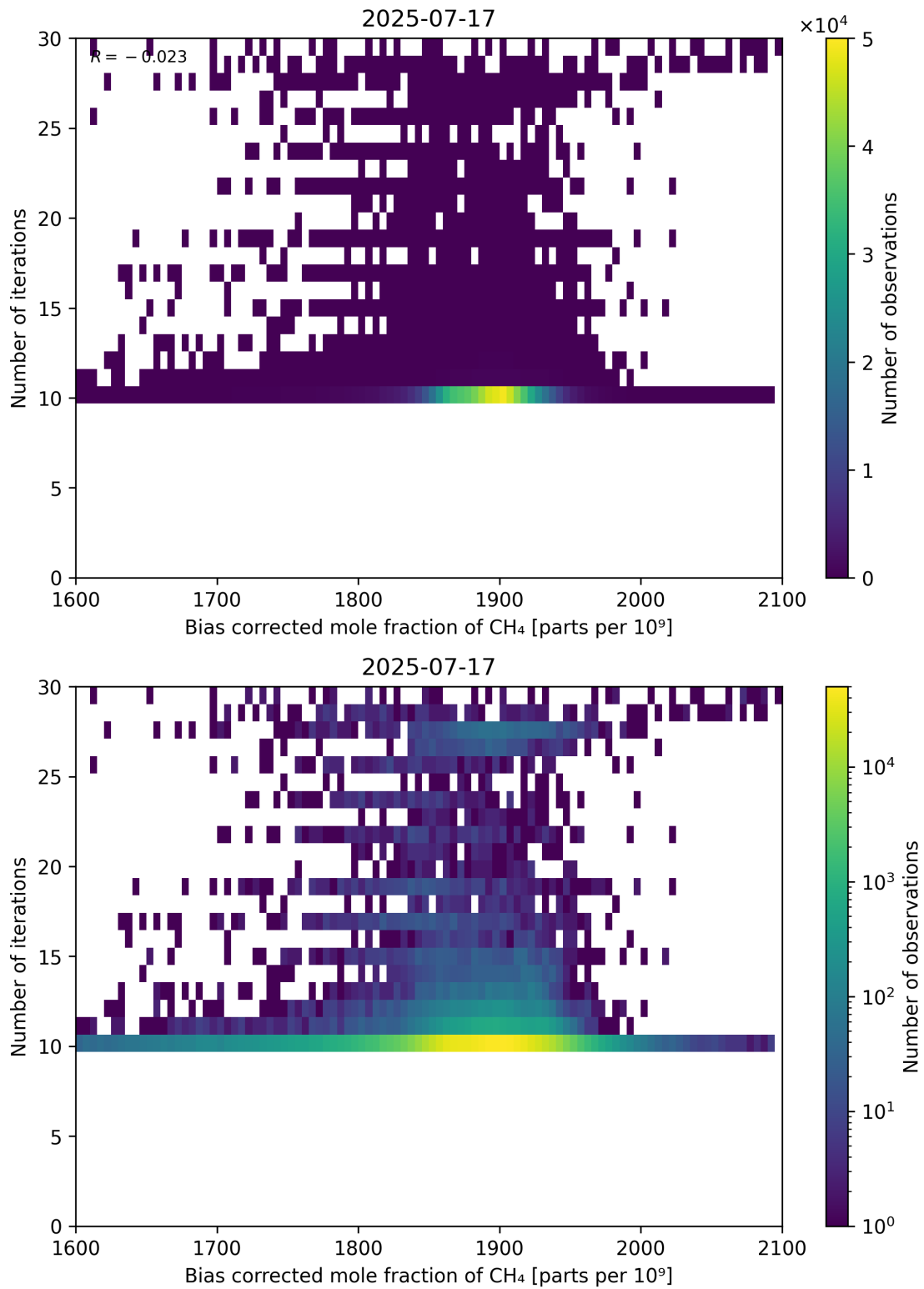
Figure 67: Scatter density plot of “Bias corrected mole fraction of CH 4 ” against “Number of iterations” for 2025-07-16 to 2025-07-18.
