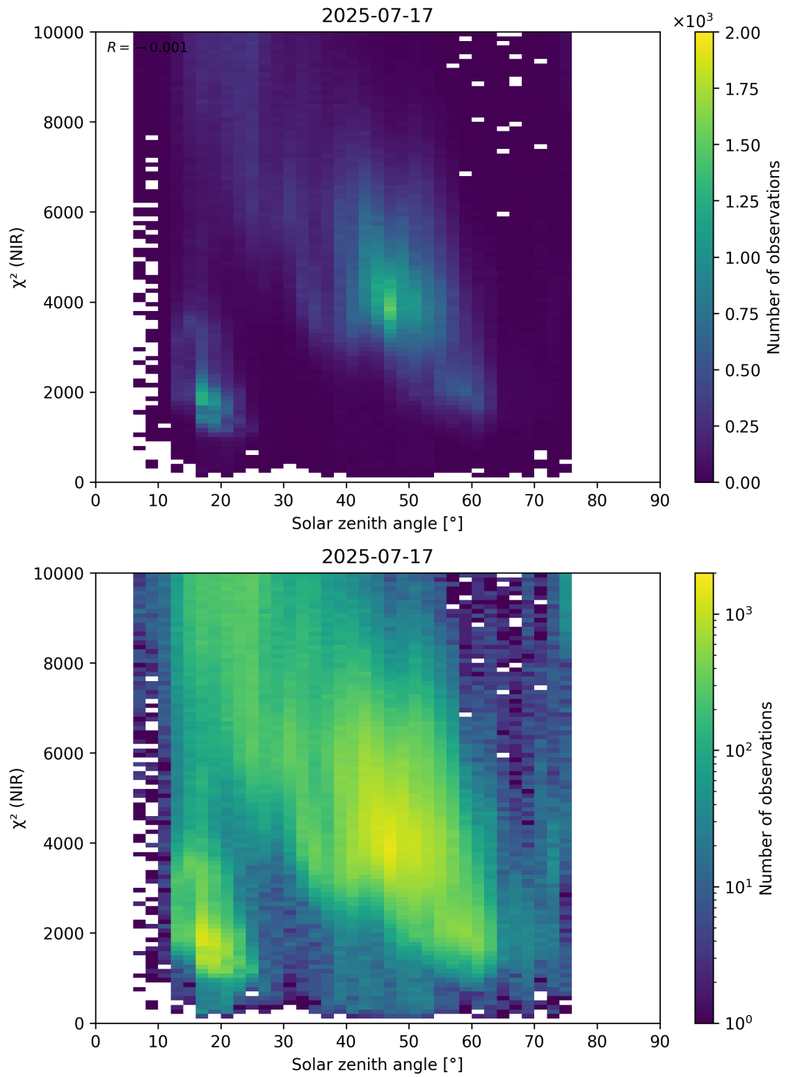
Figure 94: Scatter density plot of “Solar zenith angle” against “ \chi^2 (NIR)” for 2025-07-16 to 2025-07-18.
