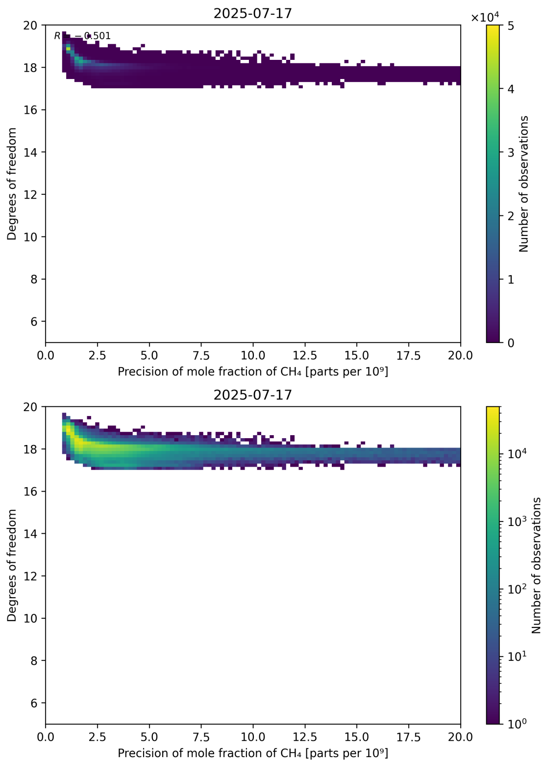
Figure 80: Scatter density plot of “Precision of mole fraction of CH 4 ” against “Degrees of freedom” for 2025-07-16 to 2025-07-18.
