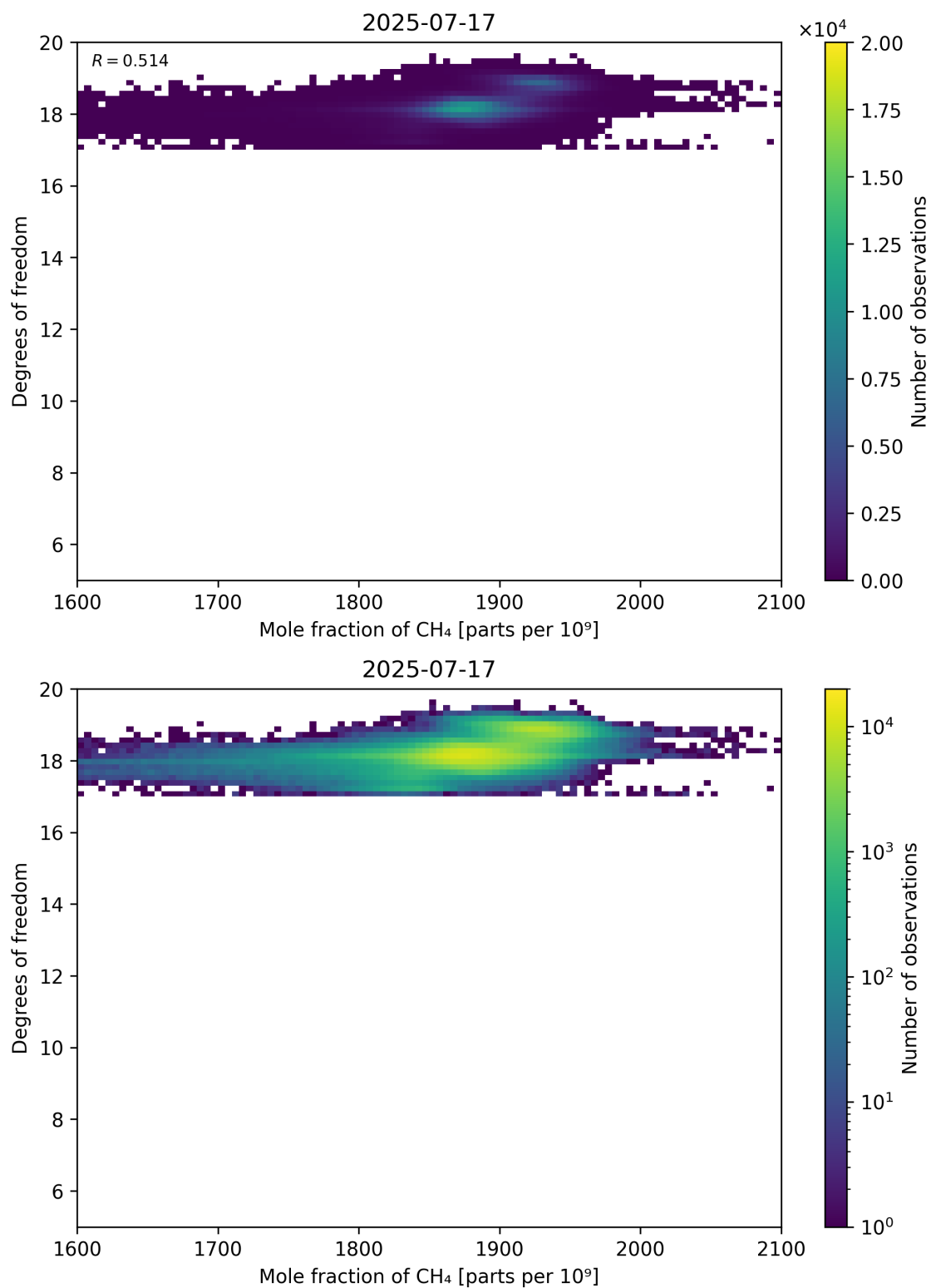
Figure 72: Scatter density plot of “Mole fraction of CH 4 ” against “Degrees of freedom” for 2025-07-16 to 2025-07-18.
