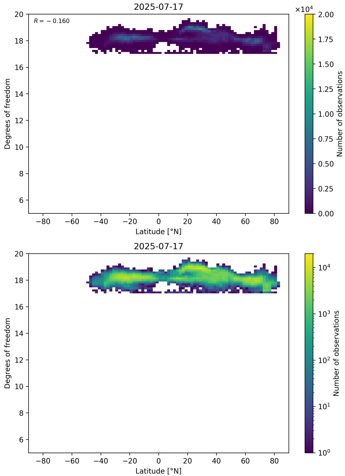
Figure 55: Scatter density plot of “Latitude” against “Degrees of freedom” for 2025-07-16 to 2025-07-18.
