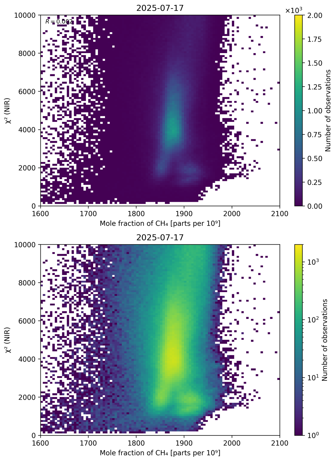
Figure 70: Scatter density plot of “Mole fraction of \text{CH}_4 ” against “ \chi^2 (NIR)” for 2025-07-16 to 2025-07-18.
