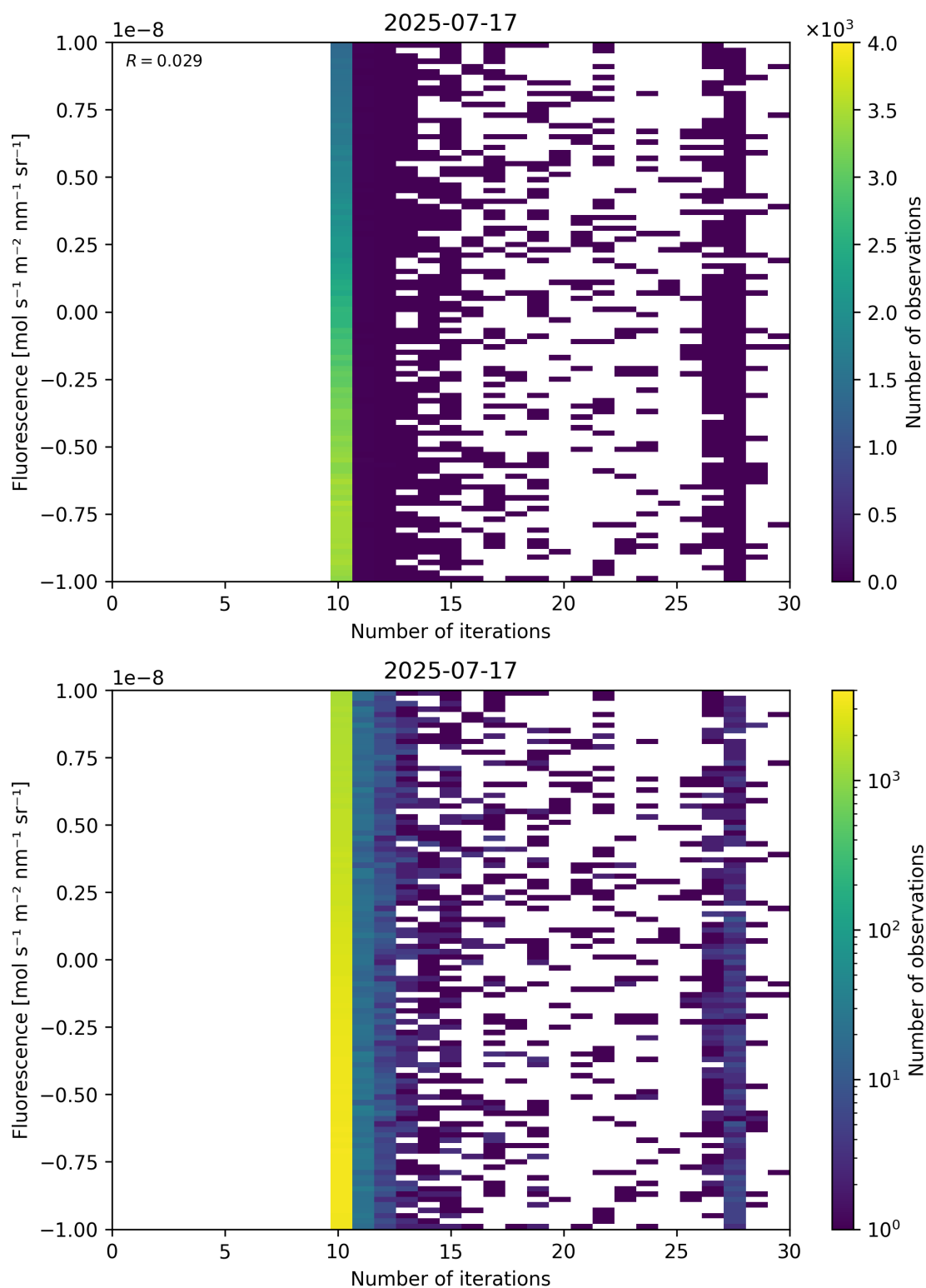
Figure 87: Scatter density plot of “Number of iterations” against “Fluorescence” for 2025-07-16 to 2025-07-18.
