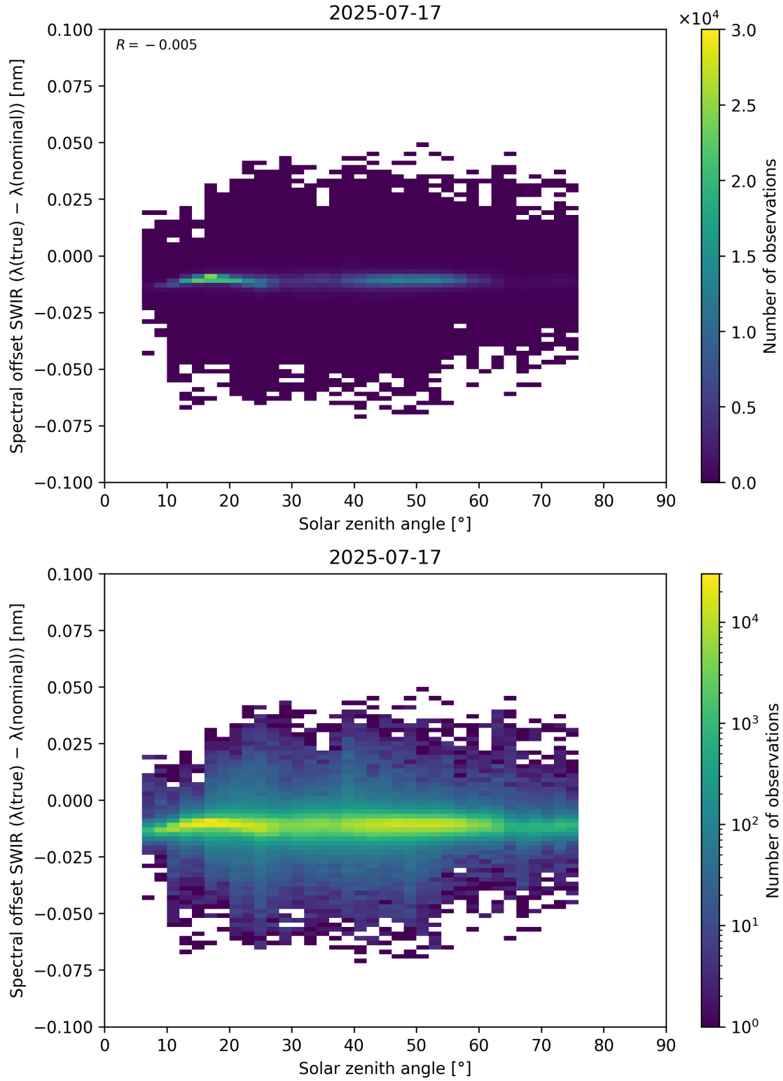
Figure 104: Scatter density plot of “Solar zenith angle” against “Spectral offset SWIR ( \lambda_{\text{true}} - \lambda_{\text{nominal}} )” for 2025-07-16 to 2025-07-18.
