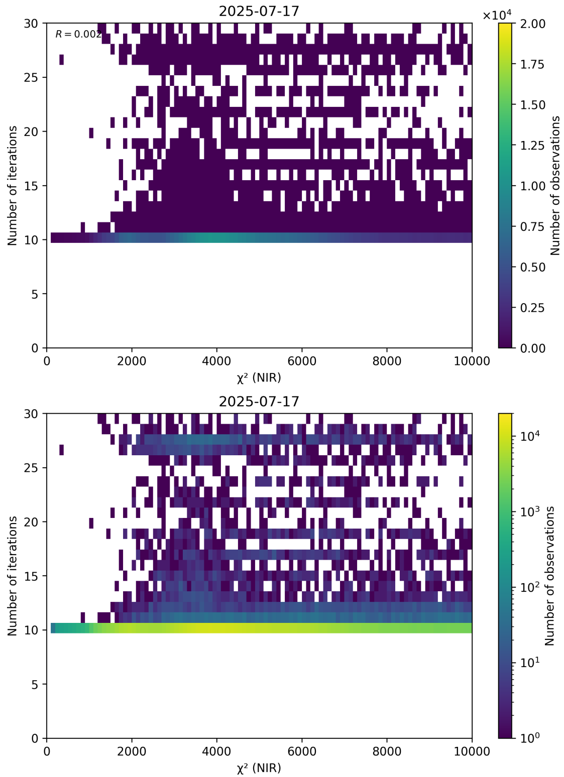
Figure 46: Scatter density plot of “ \chi^2 (NIR)” against “Number of iterations” for 2025-07-16 to 2025-07-18.
