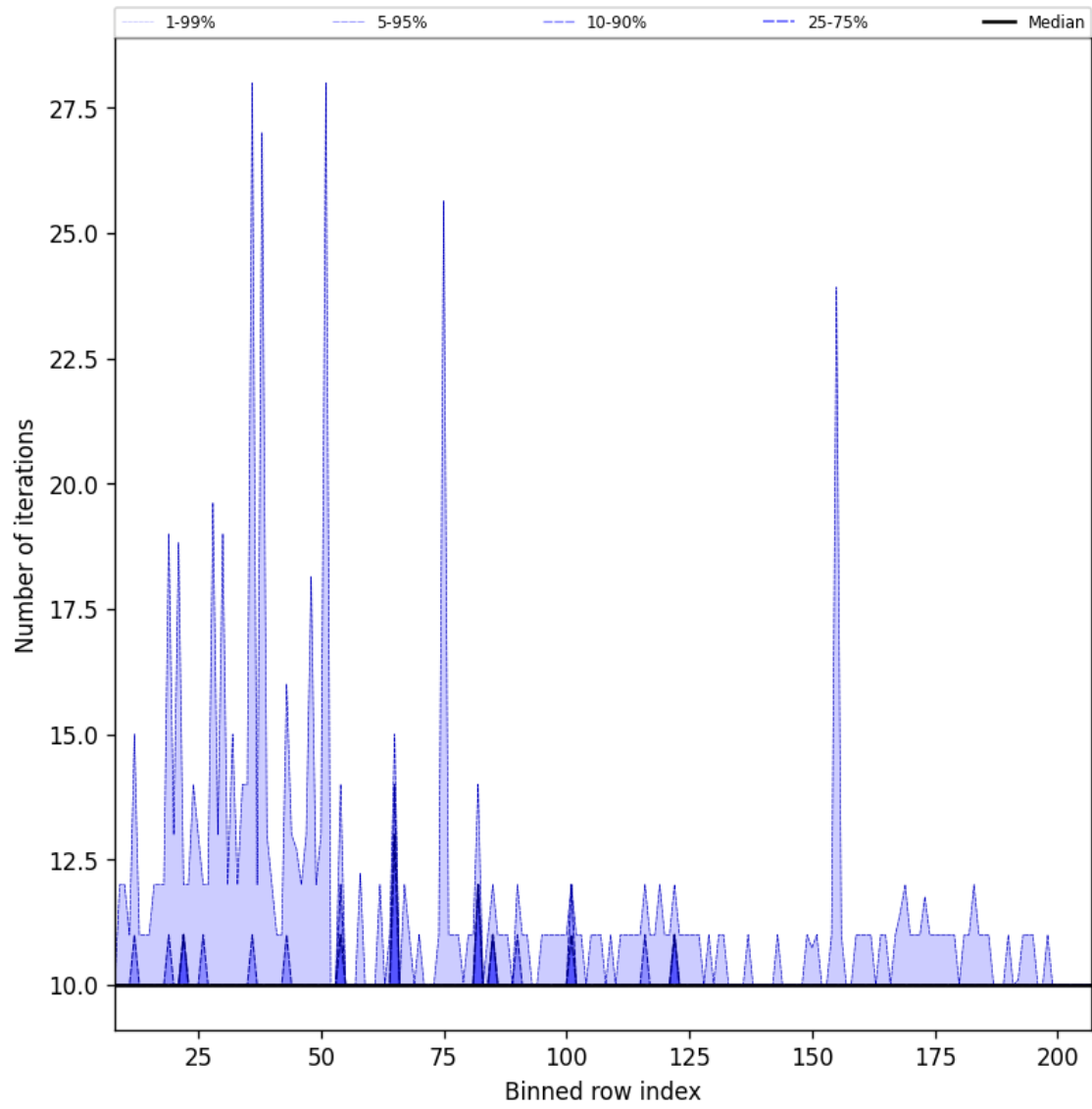
Figure 42: Along track statistics of “Number of iterations” for 2025-07-16 to 2025-07-18
