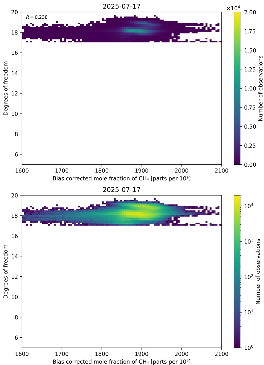
Figure 65: Scatter density plot of “Bias corrected mole fraction of CH 4 ” against “Degrees of freedom” for 2025-07-16 to 2025-07-18.
