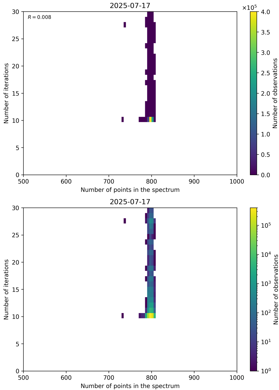
Figure 92: Scatter density plot of “Number of points in the spectrum” against “Number of iterations” for 2025-07-16 to 2025-07-18.
