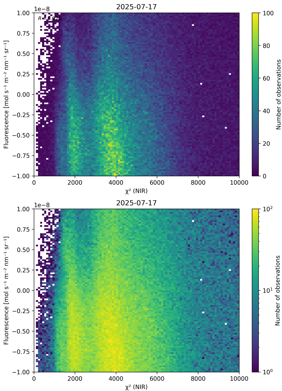
Figure 45: Scatter density plot of “ \chi^2 (NIR)” against “Fluorescence” for 2025-07-16 to 2025-07-18.
