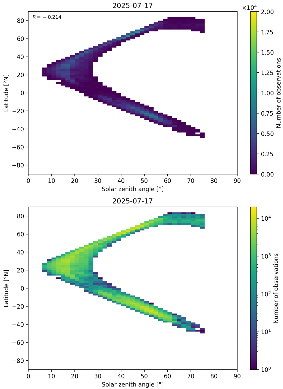
Figure 98: Scatter density plot of “Solar zenith angle” against “Latitude” for 2025-07-16 to 2025-07-18.
