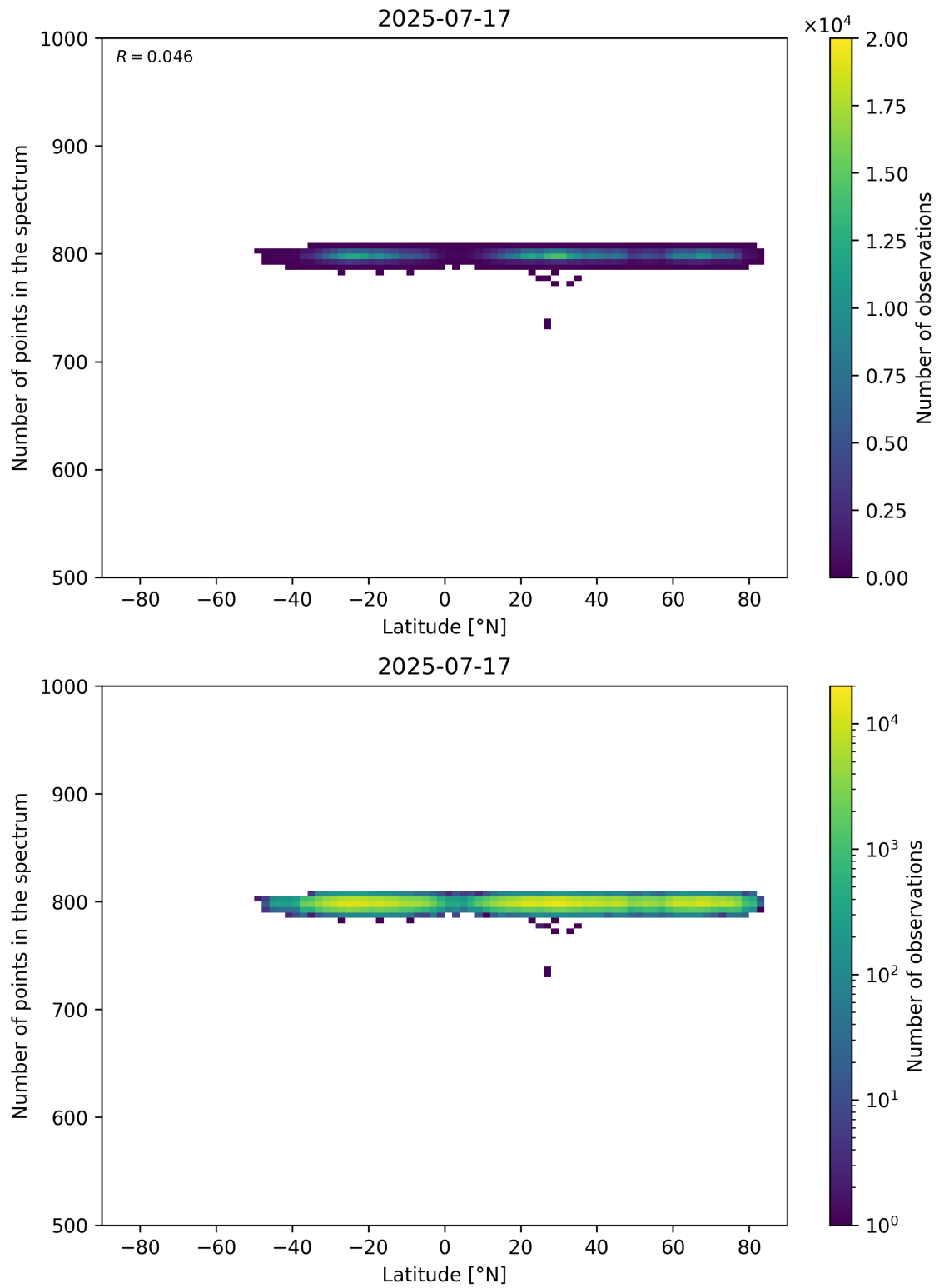
Figure 61: Scatter density plot of “Latitude” against “Number of points in the spectrum” for 2025-07-16 to 2025-07-18.
