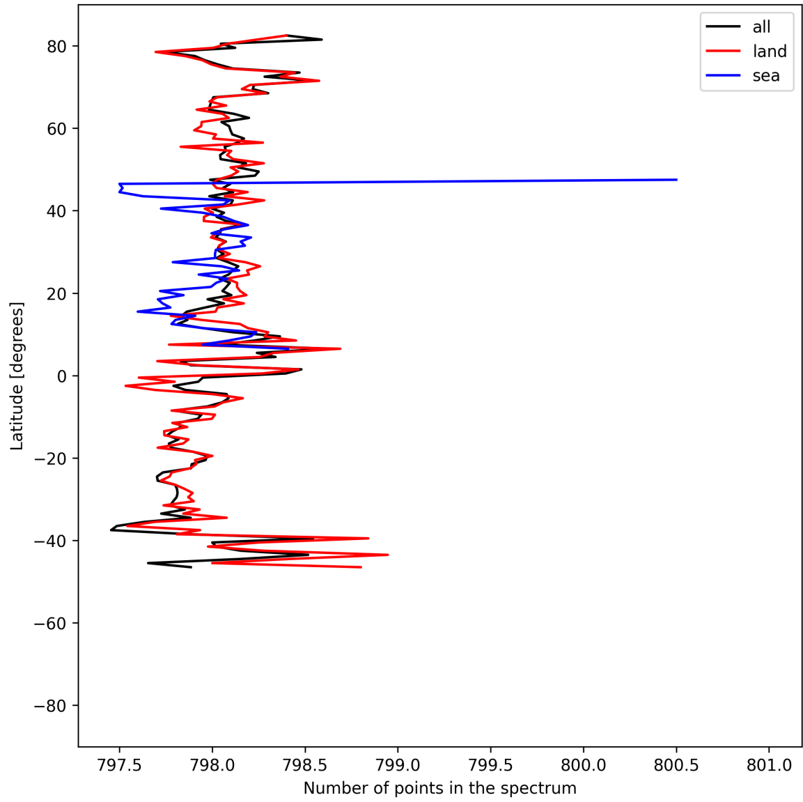
Figure 15: Zonal average of “Number of points in the spectrum” for 2025-07-16 to 2025-07-18.
