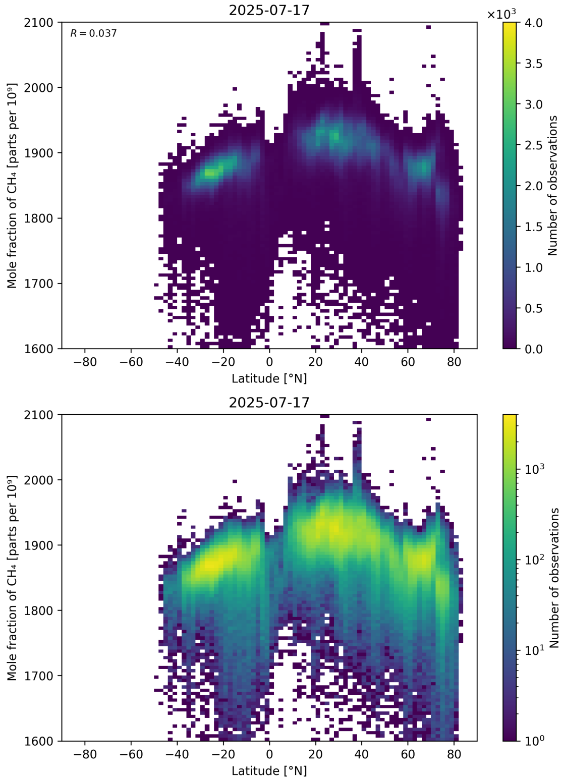
Figure 57: Scatter density plot of “Latitude” against “Mole fraction of \text{CH}_4 ” for 2025-07-16 to 2025-07-18.
