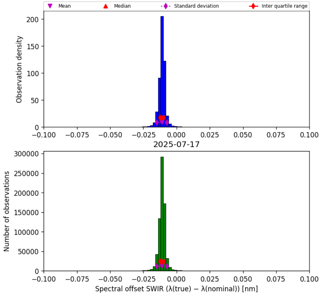
Figure 27: Histogram of “Spectral offset SWIR ( \lambda_{\text{true}} - \lambda_{\text{nominal}} )” for 2025-07-16 to 2025-07-18
