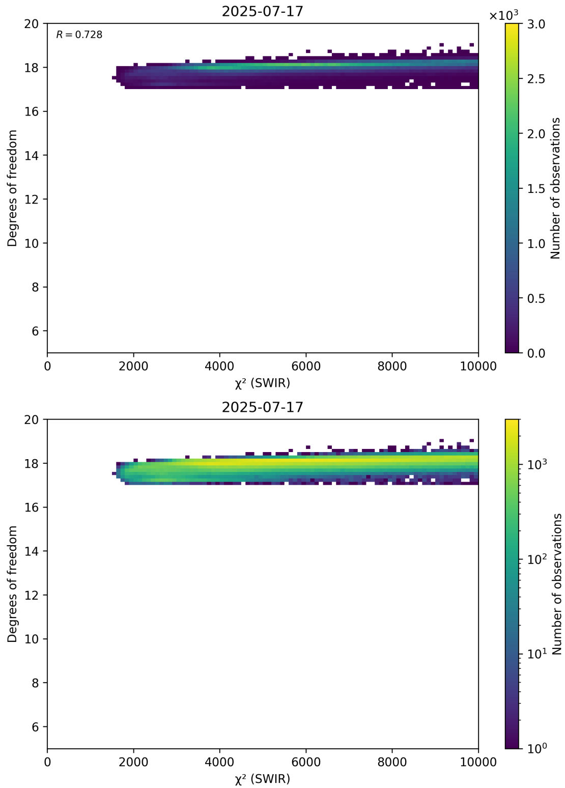
Figure 48: Scatter density plot of “ \chi^2 (SWIR)” against “Degrees of freedom” for 2025-07-16 to 2025-07-18.
