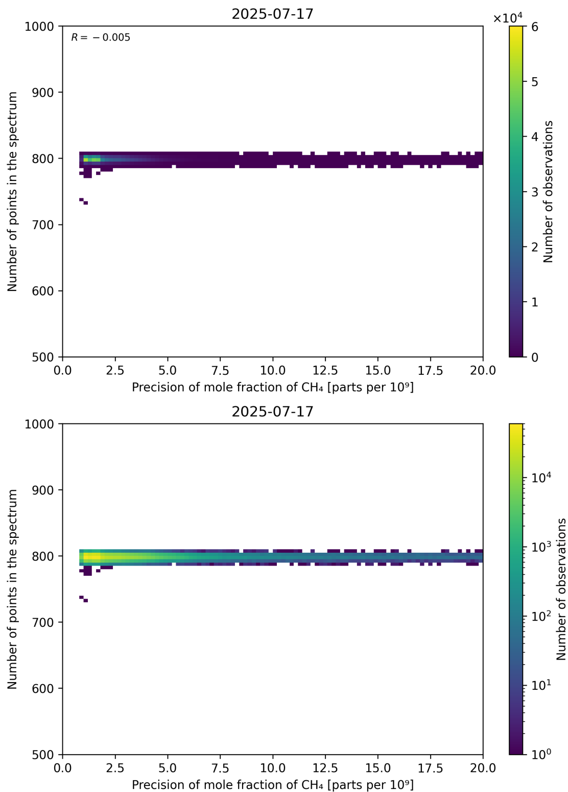
Figure 84: Scatter density plot of “Precision of mole fraction of CH 4 ” against “Number of points in the spectrum” for 2025-07-16 to 2025-07-18.
