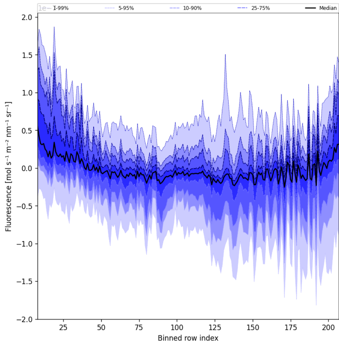
Figure 43: Along track statistics of “Fluorescence” for 2025-07-16 to 2025-07-18
