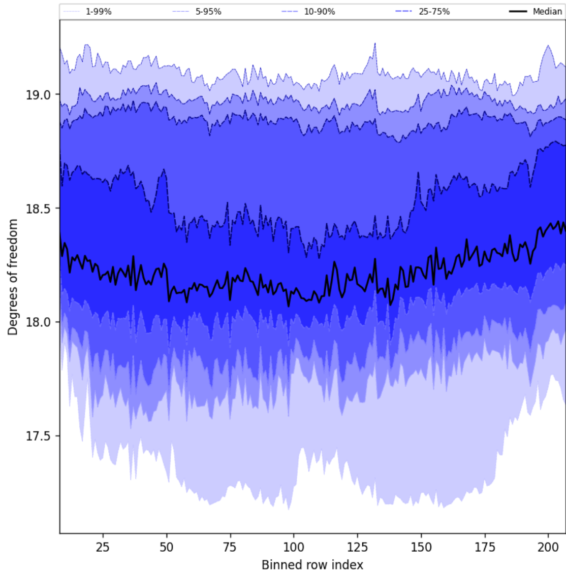
Figure 41: Along track statistics of “Degrees of freedom” for 2025-07-16 to 2025-07-18
