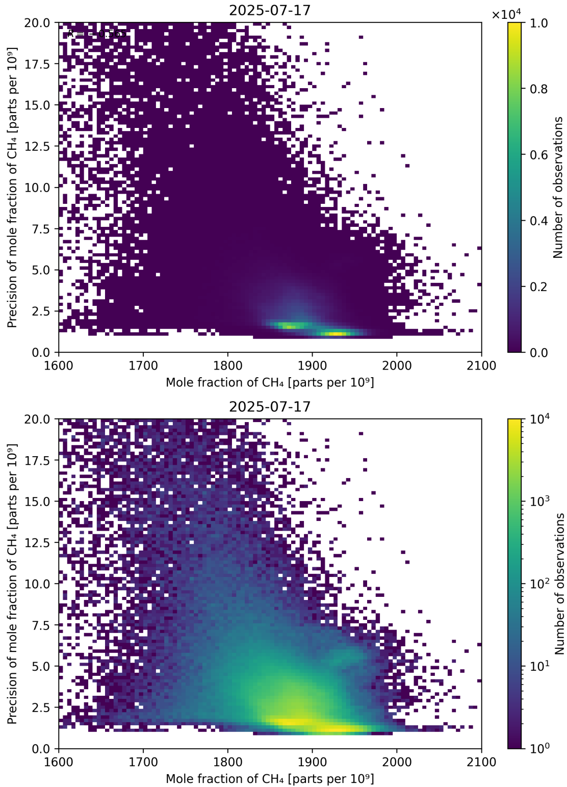
Figure 75: Scatter density plot of “Mole fraction of CH 4 ” against “Precision of mole fraction of CH 4 ” for 2025-07-16 to 2025-07-18.
