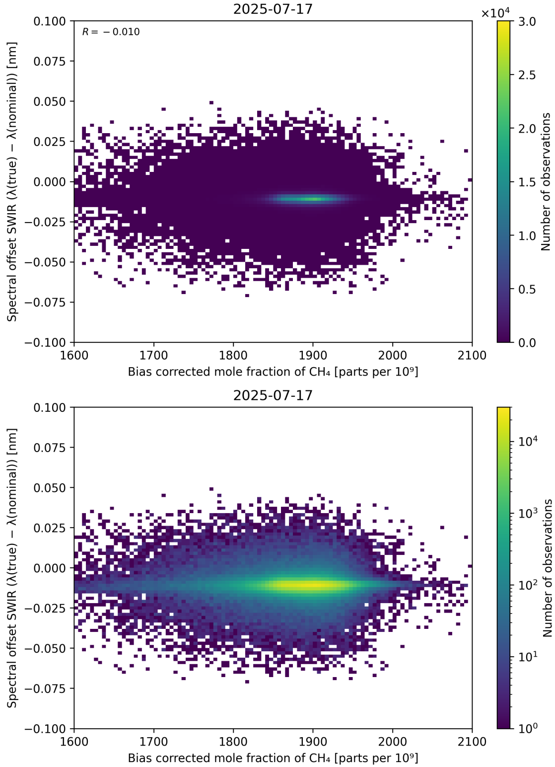
Figure 69: Scatter density plot of “Bias corrected mole fraction of \text{CH}_4 ” against “Spectral offset SWIR ( \lambda_{\text{true}} - \lambda_{\text{nominal}} )” for 2025-07-16 to 2025-07-18.
