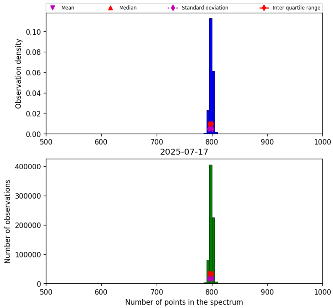
Figure 26: Histogram of “Number of points in the spectrum” for 2025-07-16 to 2025-07-18
