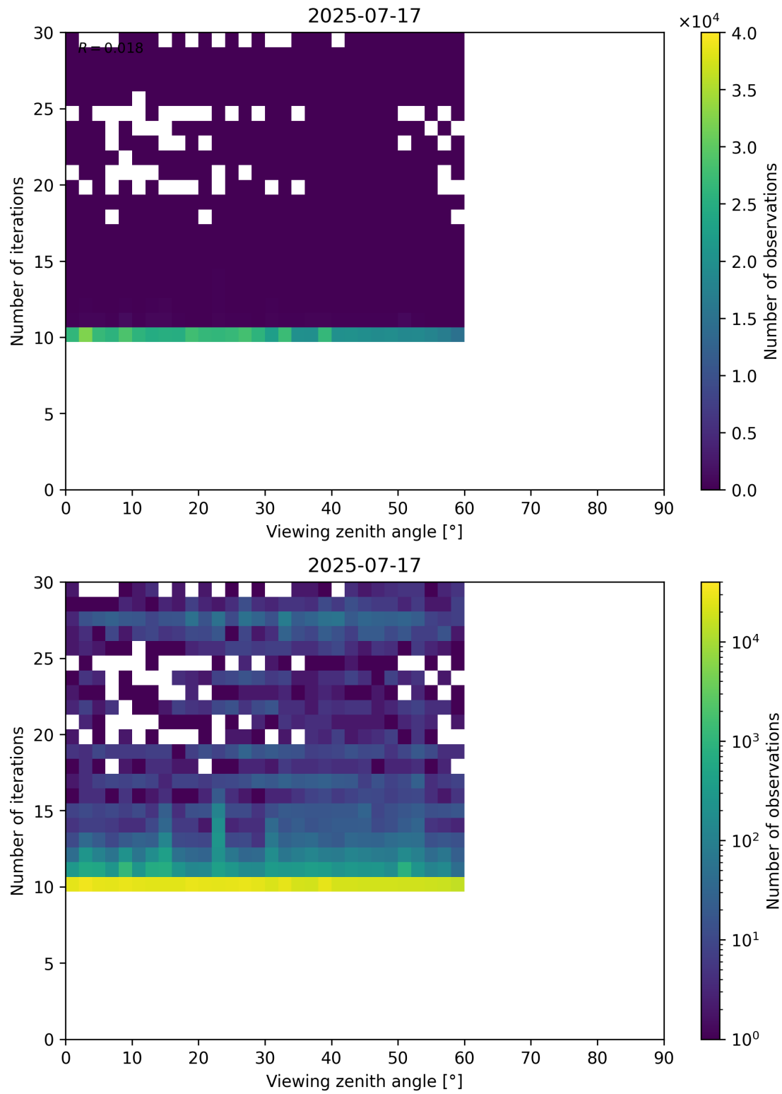
Figure 113: Scatter density plot of “Viewing zenith angle” against “Number of iterations” for 2025-07-16 to 2025-07-18.
