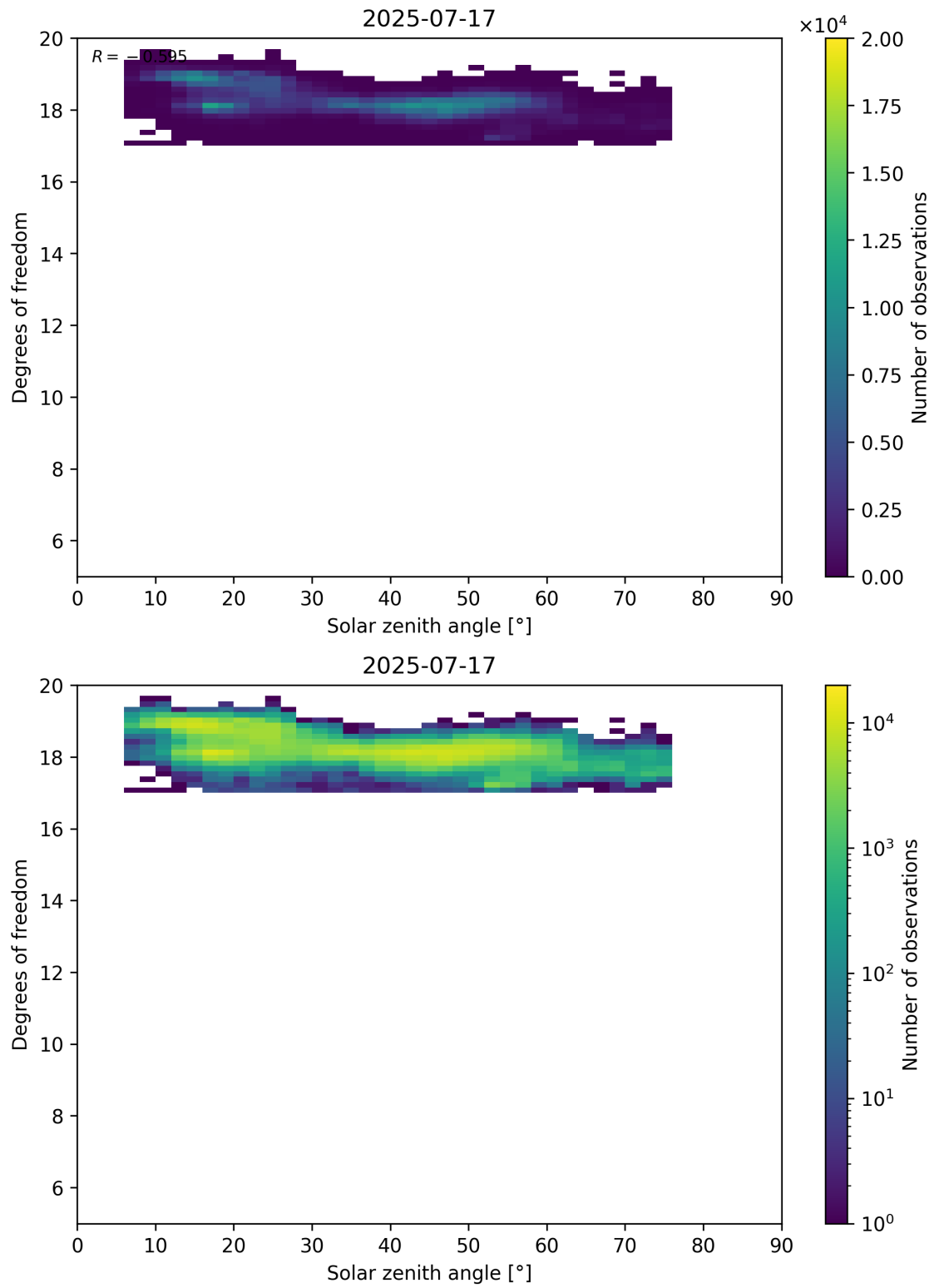
Figure 96: Scatter density plot of “Solar zenith angle” against “Degrees of freedom” for 2025-07-16 to 2025-07-18.
