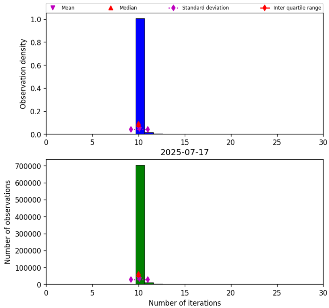
Figure 31: Histogram of “Number of iterations” for 2025-07-16 to 2025-07-18
