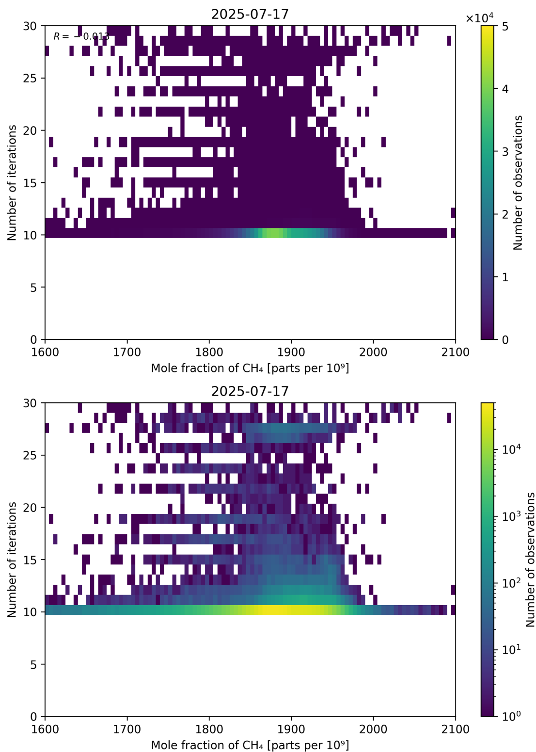
Figure 76: Scatter density plot of “Mole fraction of CH 4 ” against “Number of iterations” for 2025-07-16 to 2025-07-18.
