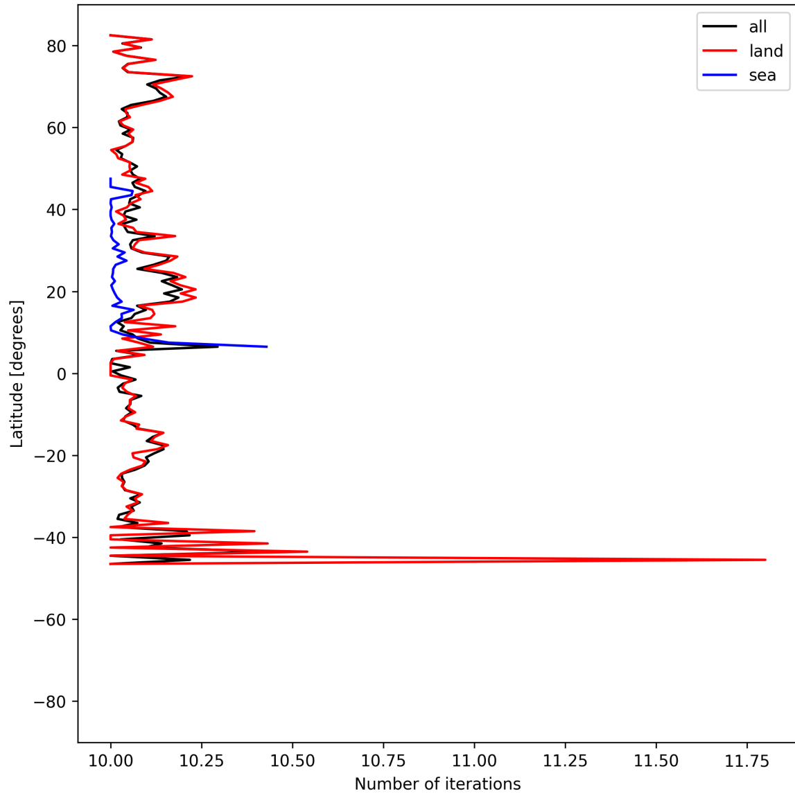
Figure 20: Zonal average of “Number of iterations” for 2025-07-16 to 2025-07-18.
