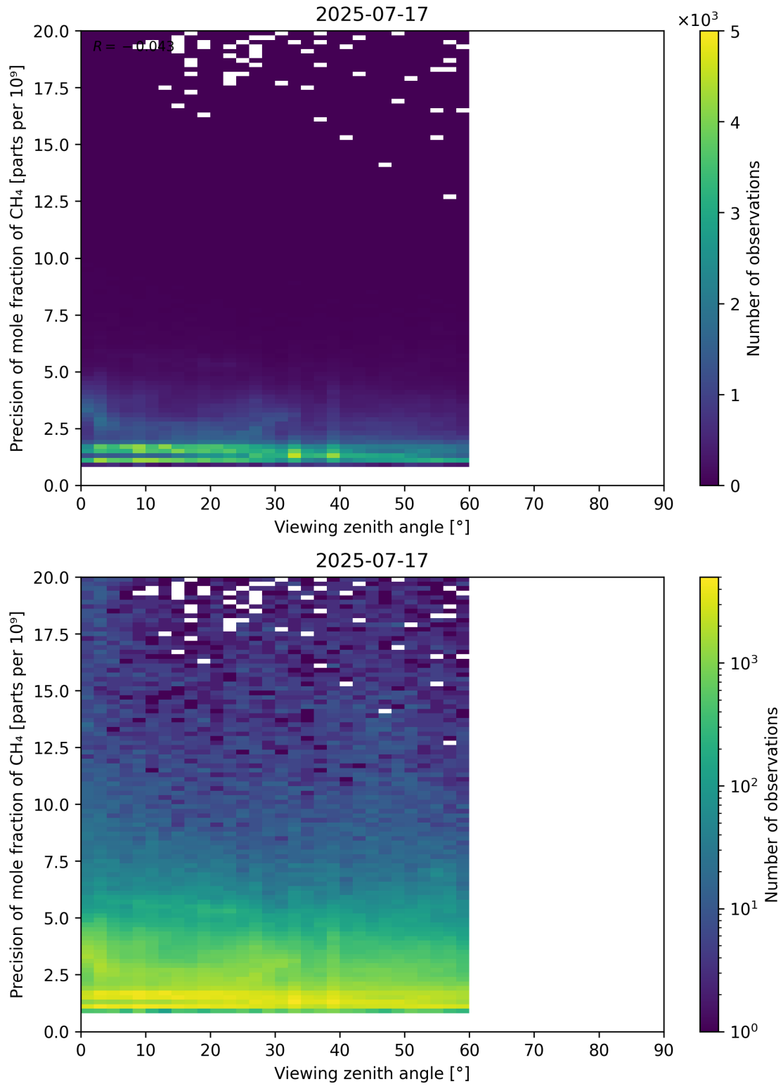
Figure 112: Scatter density plot of “Viewing zenith angle” against “Precision of mole fraction of CH 4 ” for 2025-07-16 to 2025-07-18.
