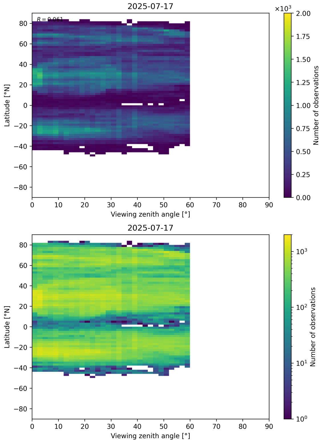
Figure 109: Scatter density plot of “Viewing zenith angle” against “Latitude” for 2025-07-16 to 2025-07-18.
