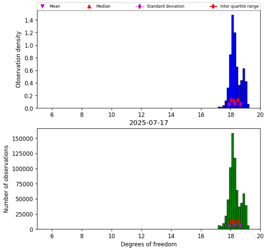
Figure 30: Histogram of “Degrees of freedom” for 2025-07-16 to 2025-07-18
