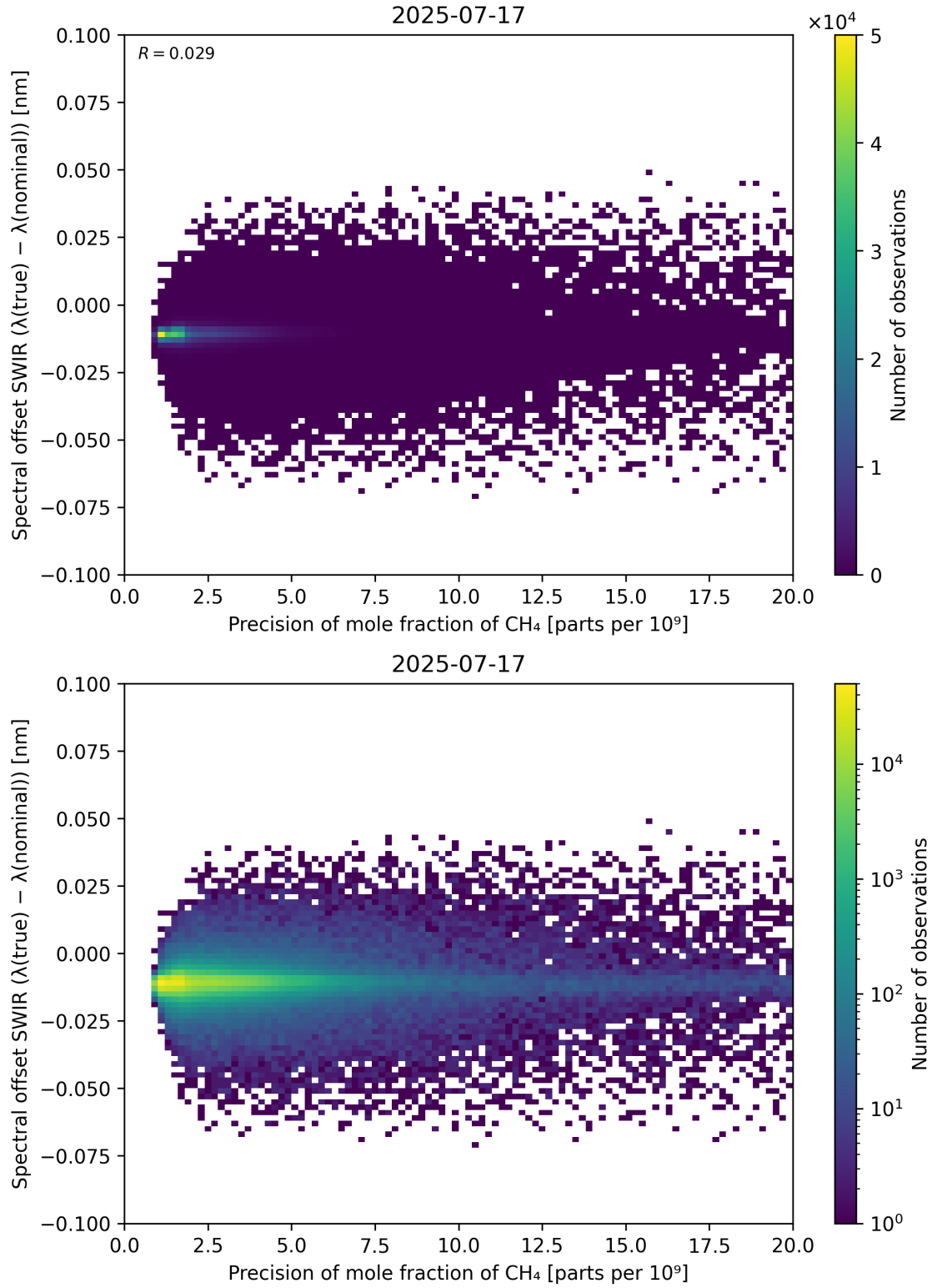
Figure 85: Scatter density plot of “Precision of mole fraction of CH 4 ” against “Spectral offset SWIR ( \lambda_{\text{true}} - \lambda_{\text{nominal}} )” for 2025-07-16 to 2025-07-18.
