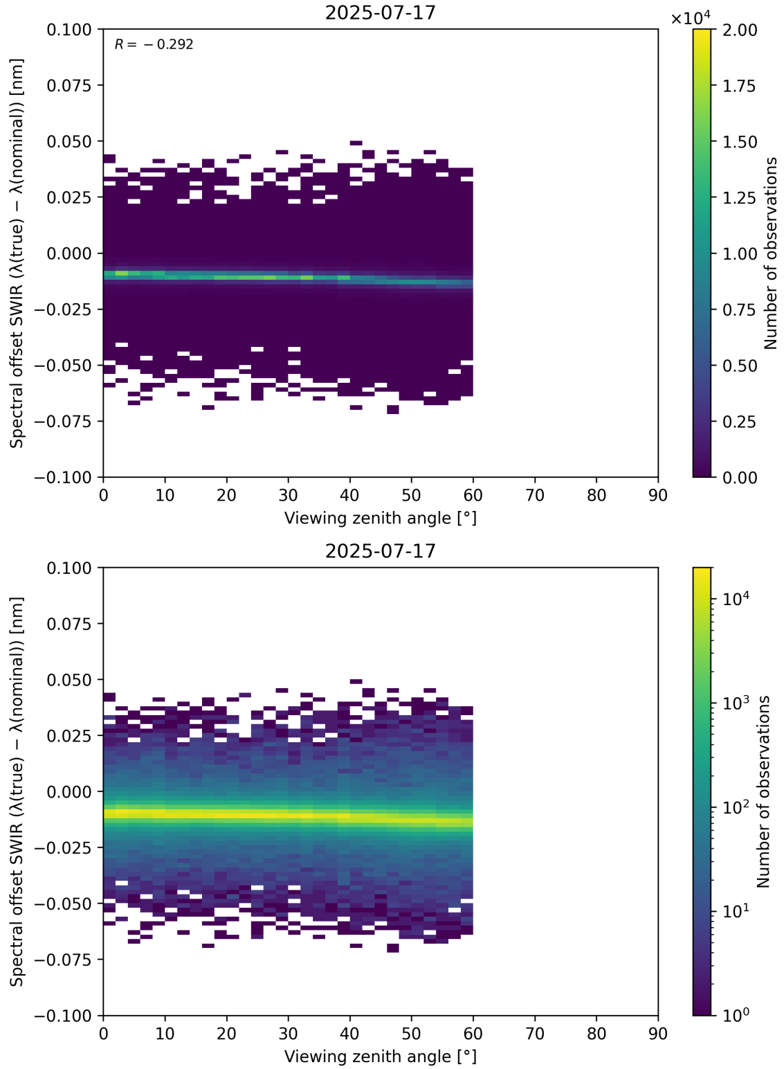
Figure 116: Scatter density plot of “Viewing zenith angle” against “Spectral offset SWIR ( \lambda_{\text{true}} - \lambda_{\text{nominal}} )” for 2025-07-16 to 2025-07-18.
