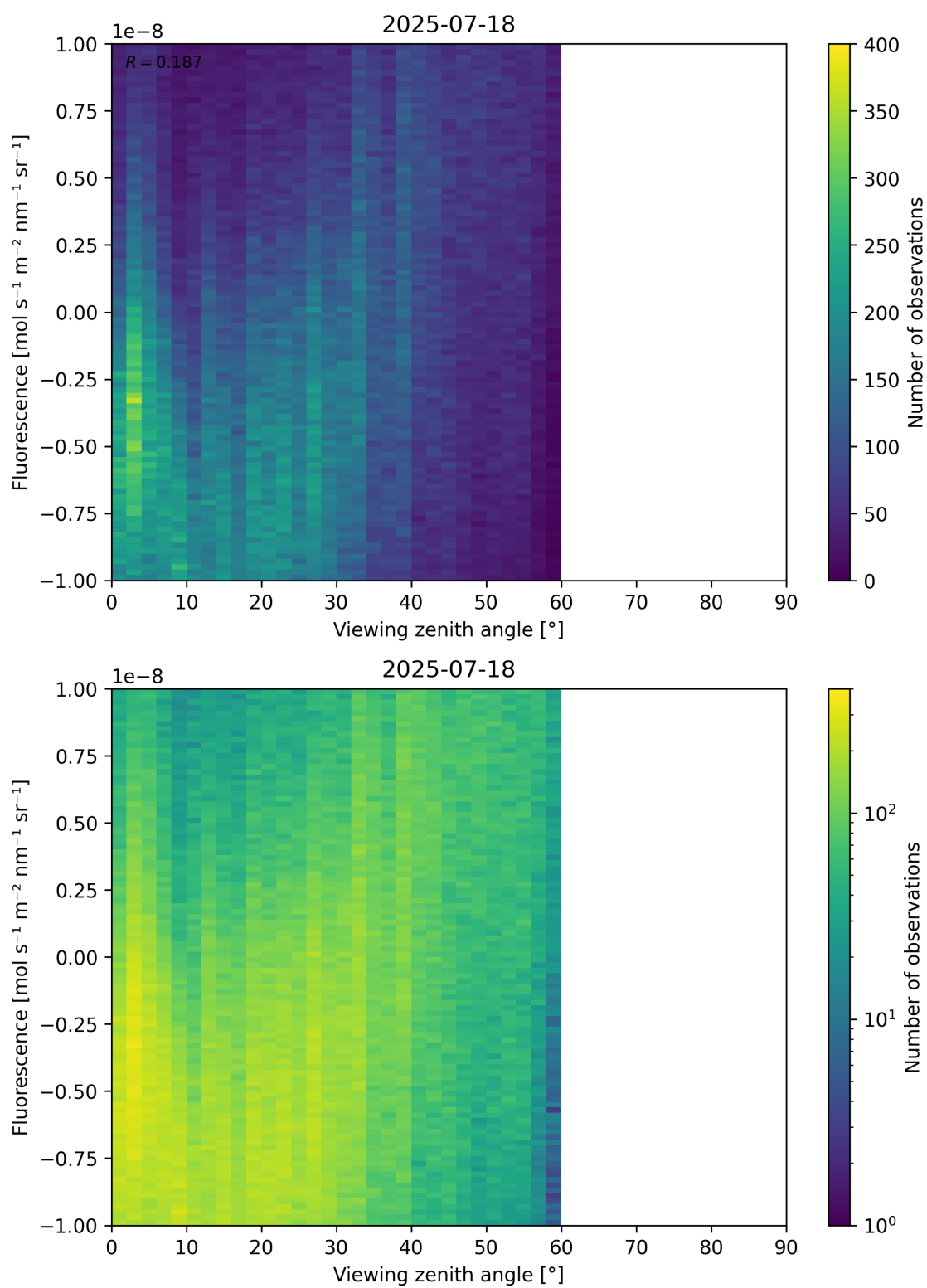
Figure 108: Scatter density plot of “Viewing zenith angle” against “Fluorescence” for 2025-07-18 to 2025-07-19.
