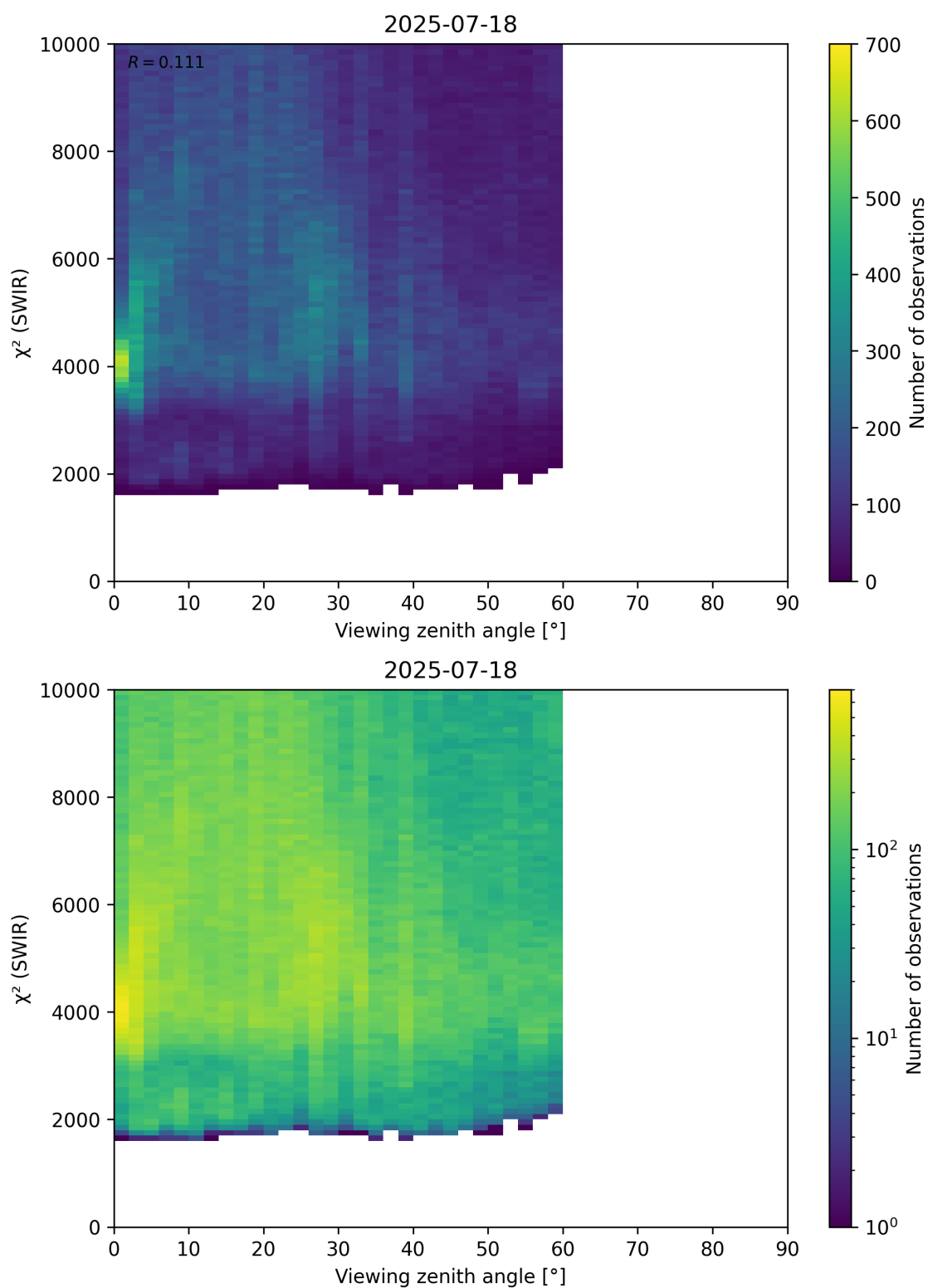
Figure 106: Scatter density plot of “Viewing zenith angle” against “ \chi^2 (SWIR)” for 2025-07-18 to 2025-07-19.
