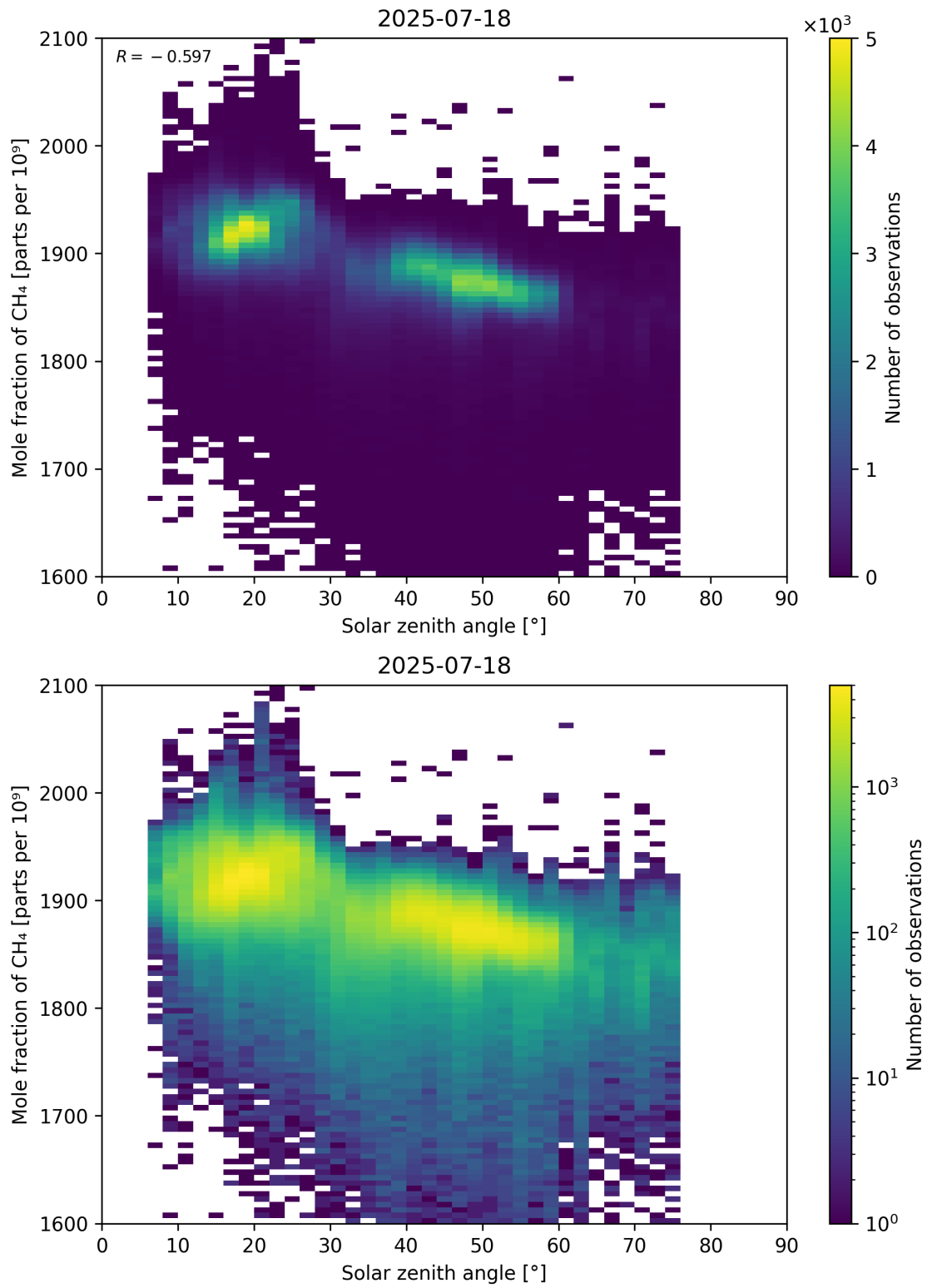
Figure 99: Scatter density plot of “Solar zenith angle” against “Mole fraction of CH 4 ” for 2025-07-18 to 2025-07-19.
