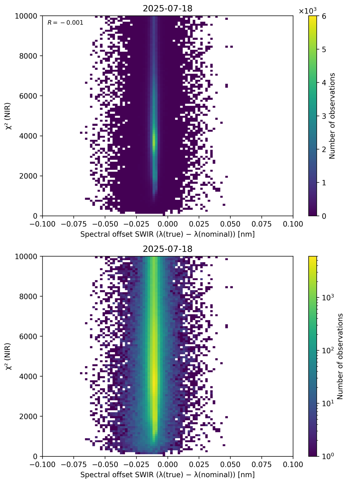
Figure 117: Scatter density plot of “Spectral offset SWIR ( \lambda_{\text{true}} - \lambda_{\text{nominal}} )” against “ \chi^2 (NIR)” for 2025-07-18 to 2025-07-19.
