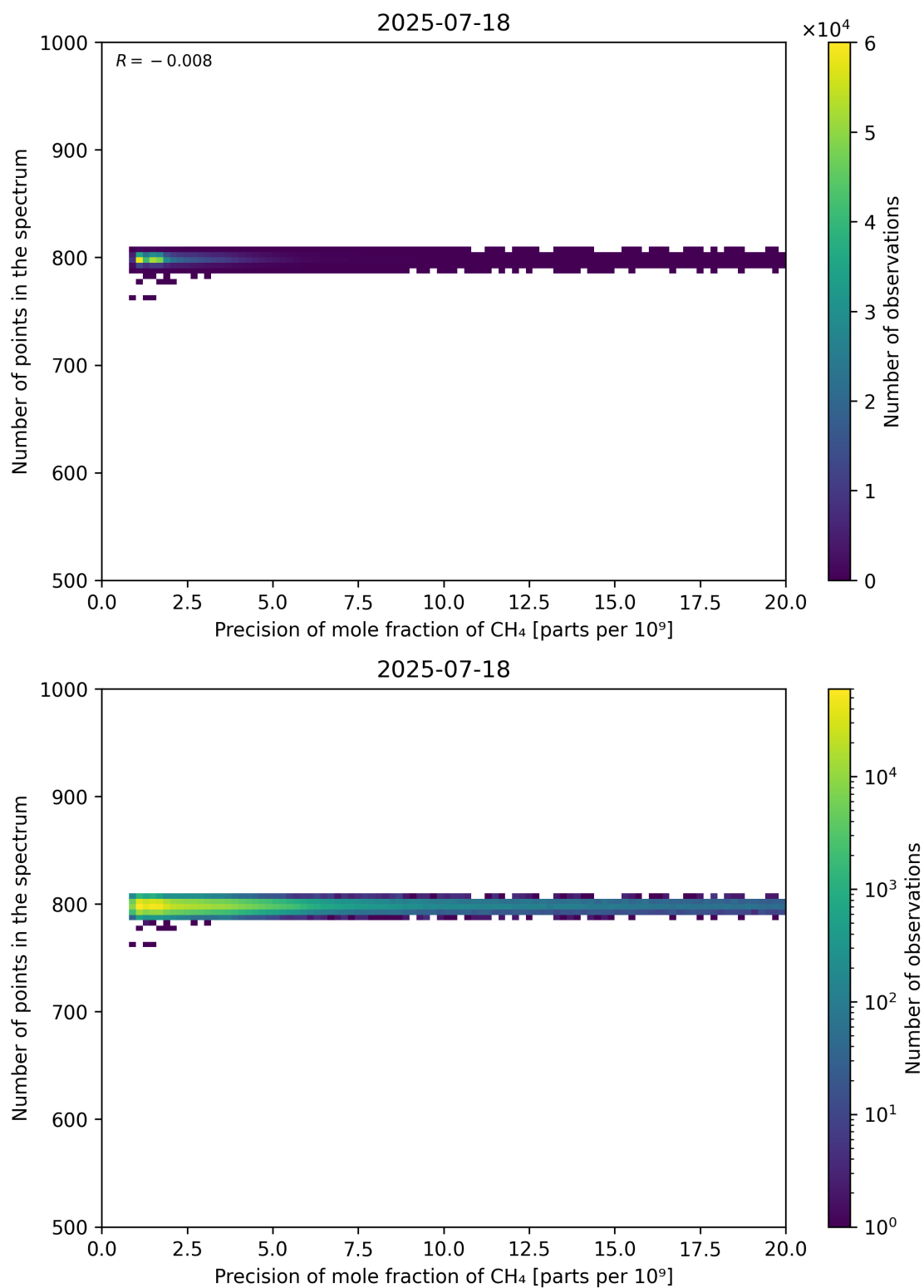
Figure 84: Scatter density plot of “Precision of mole fraction of CH 4 ” against “Number of points in the spectrum” for 2025-07-18 to 2025-07-19.
