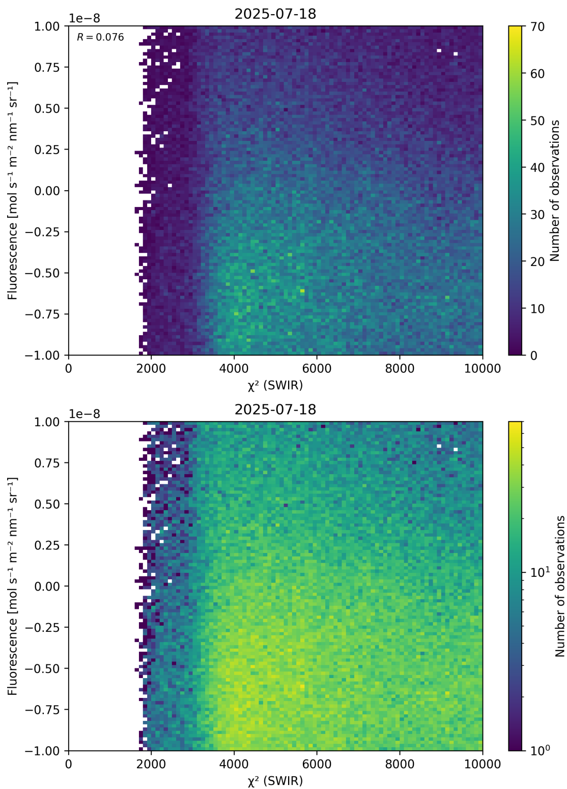
Figure 49: Scatter density plot of “ \chi^2 (SWIR)” against “Fluorescence” for 2025-07-18 to 2025-07-19.
