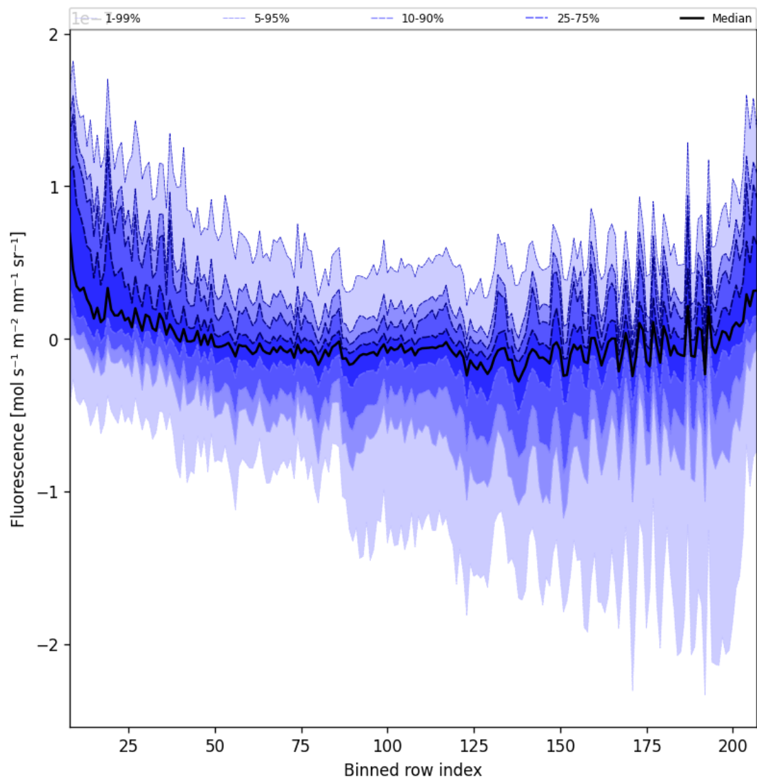
Figure 43: Along track statistics of “Fluorescence” for 2025-07-18 to 2025-07-19
