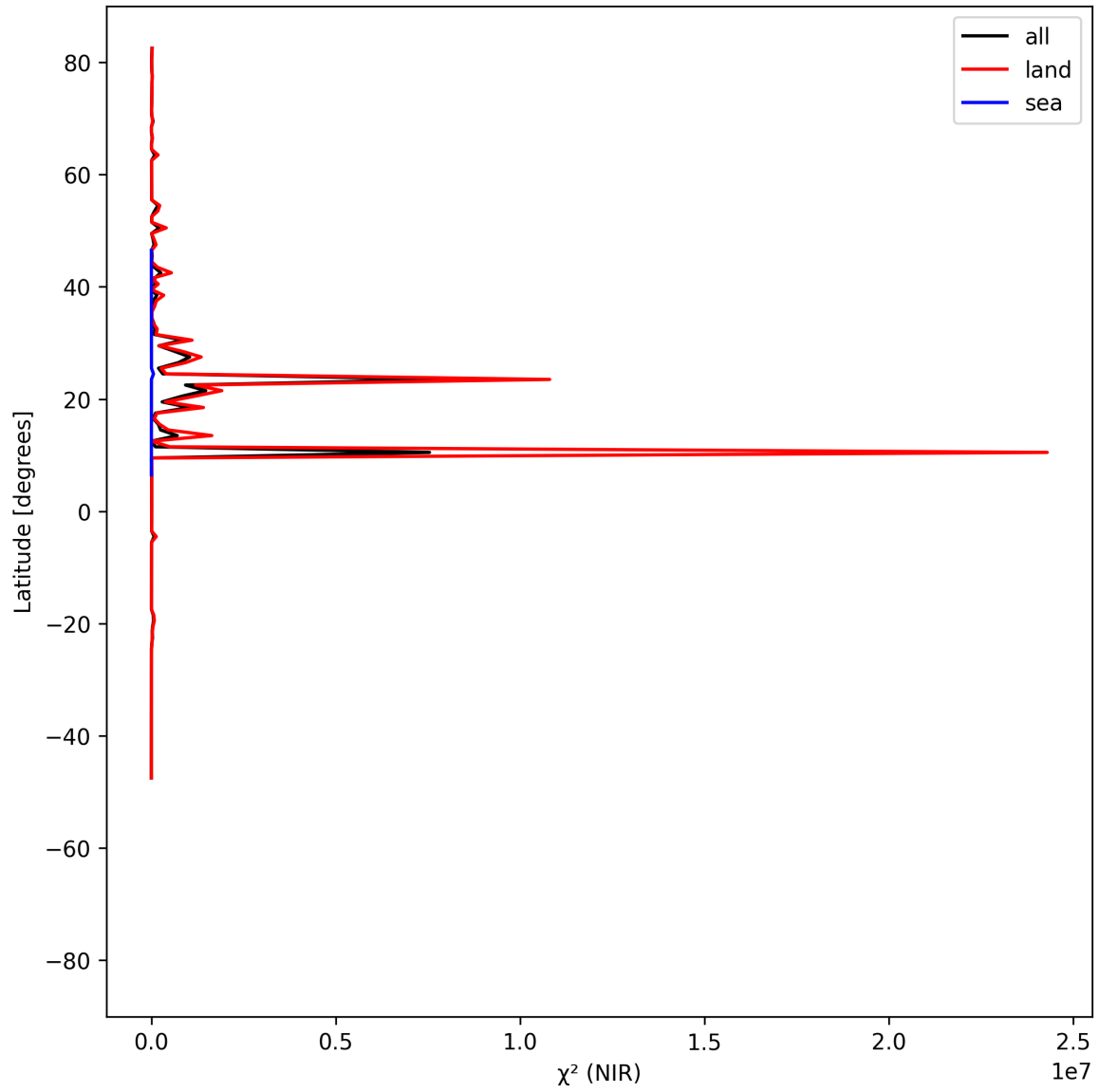
Figure 18: Zonal average of “ \chi^2 (NIR)” for 2025-07-18 to 2025-07-19.
