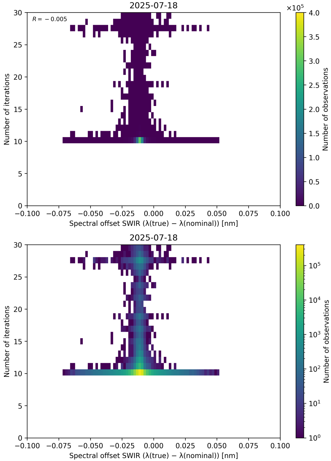
Figure 121: Scatter density plot of “Spectral offset SWIR ( \lambda_{\text{true}} - \lambda_{\text{nominal}} )” against “Number of iterations” for 2025-07-18 to 2025-07-19.
