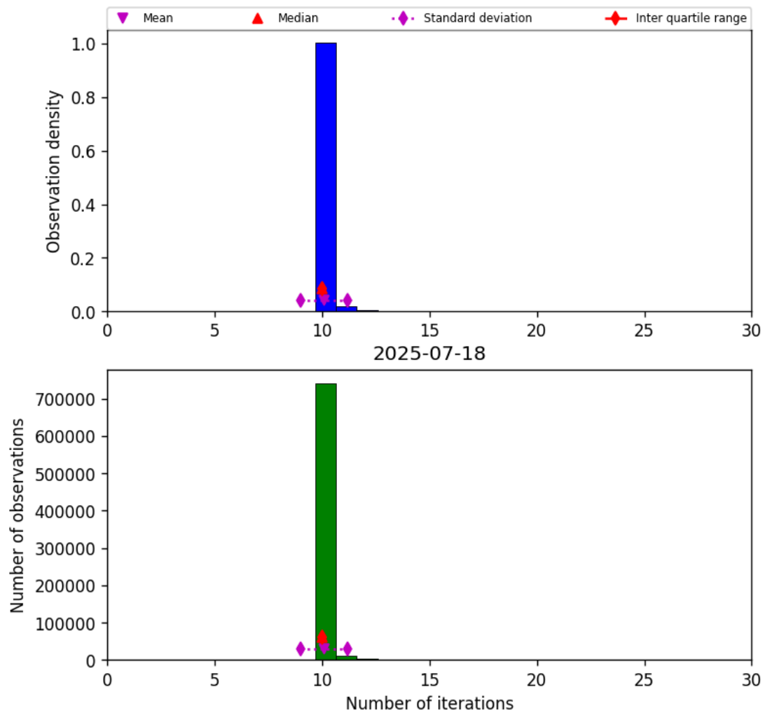
Figure 31: Histogram of “Number of iterations” for 2025-07-18 to 2025-07-19
