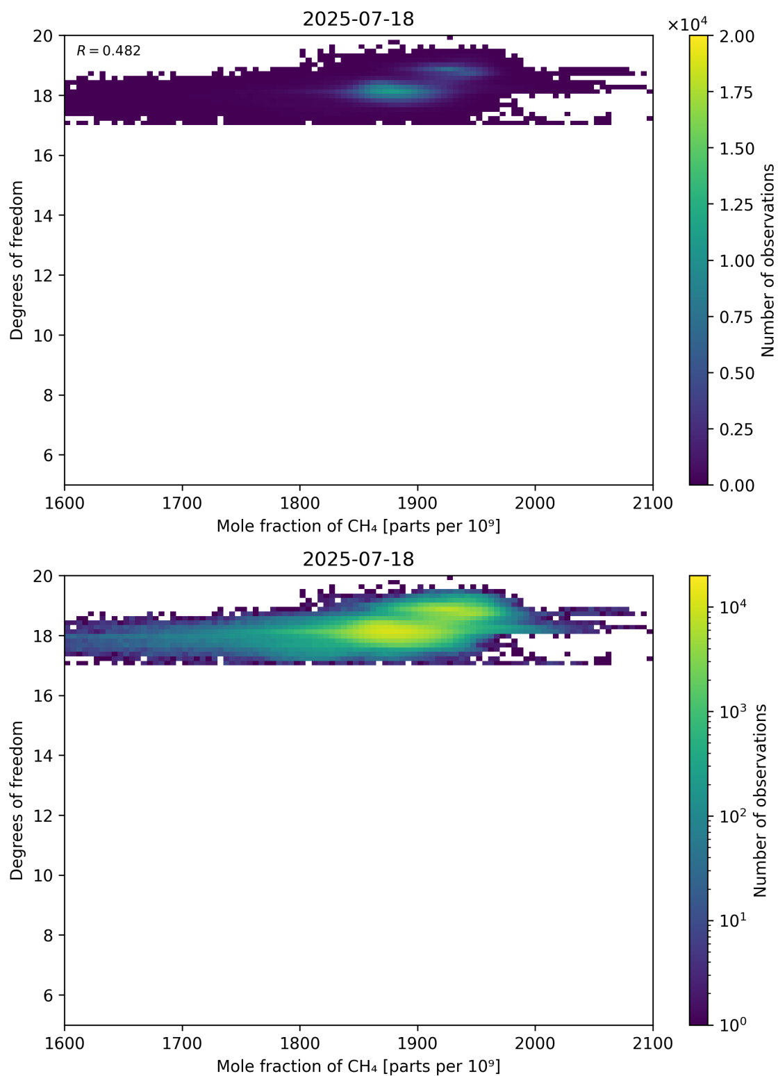
Figure 72: Scatter density plot of “Mole fraction of CH 4 ” against “Degrees of freedom” for 2025-07-18 to 2025-07-19.
