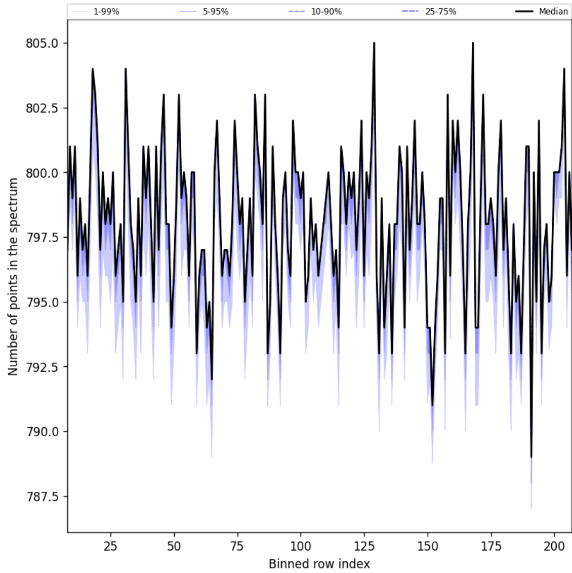
Figure 37: Along track statistics of “Number of points in the spectrum” for 2025-07-18 to 2025-07-19
