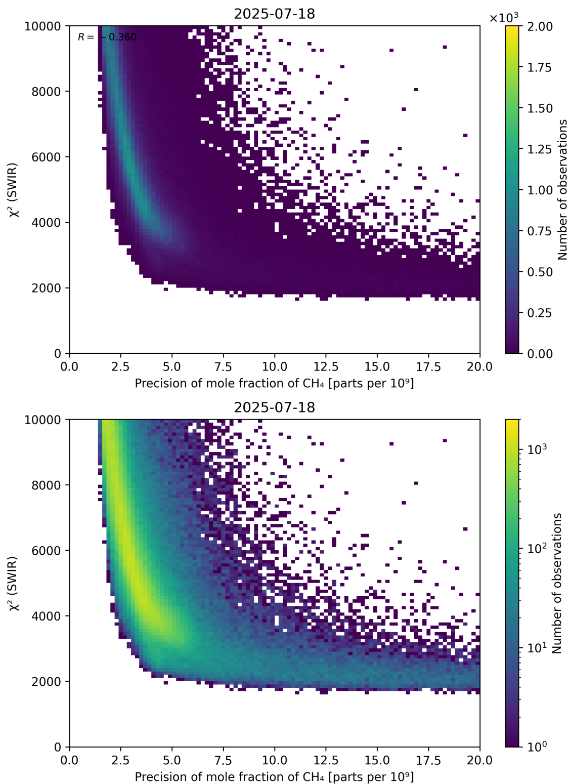
Figure 79: Scatter density plot of “Precision of mole fraction of CH 4 ” against “ \chi^2 (SWIR)” for 2025-07-18 to 2025-07-19.
