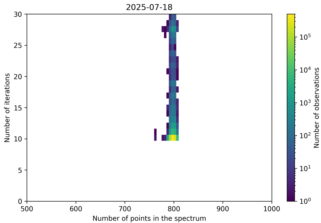
Figure 92: Scatter density plot of “Number of points in the spectrum” against “Number of iterations” for 2025-07-18 to 2025-07-19.
