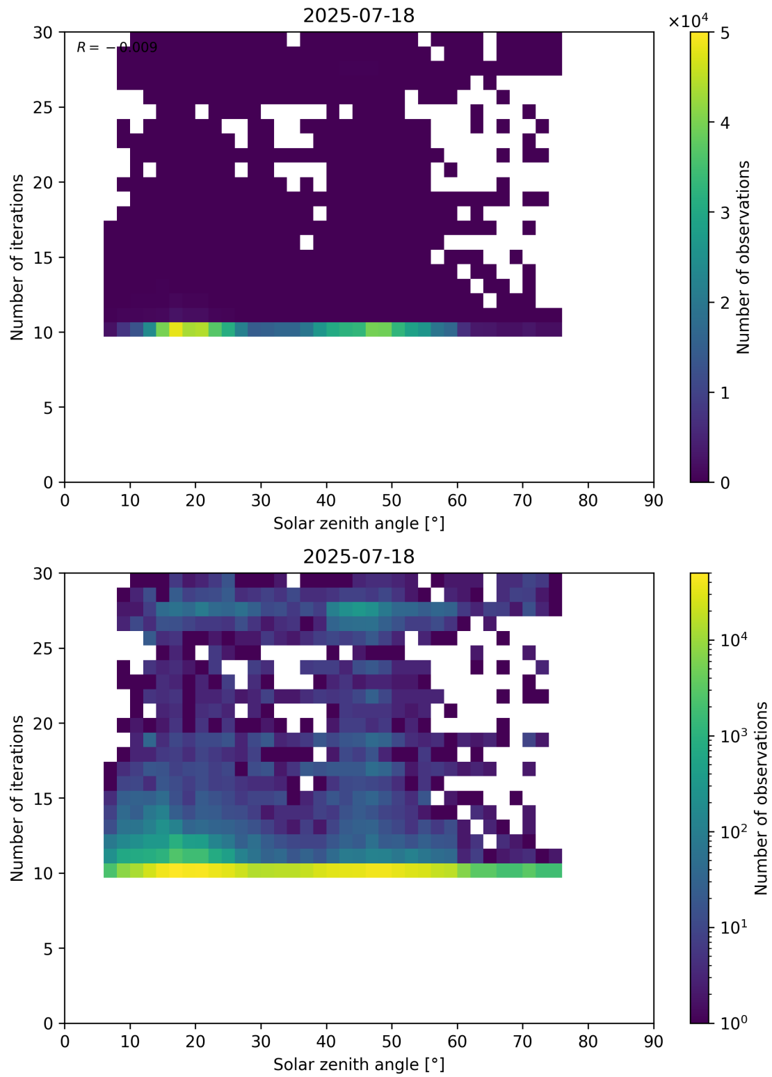
Figure 102: Scatter density plot of “Solar zenith angle” against “Number of iterations” for 2025-07-18 to 2025-07-19.
