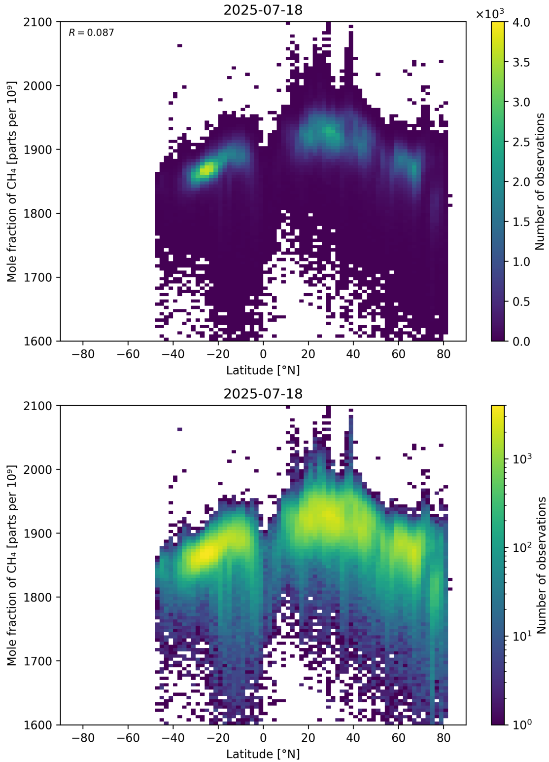
Figure 57: Scatter density plot of “Latitude” against “Mole fraction of CH 4 ” for 2025-07-18 to 2025-07-19.
