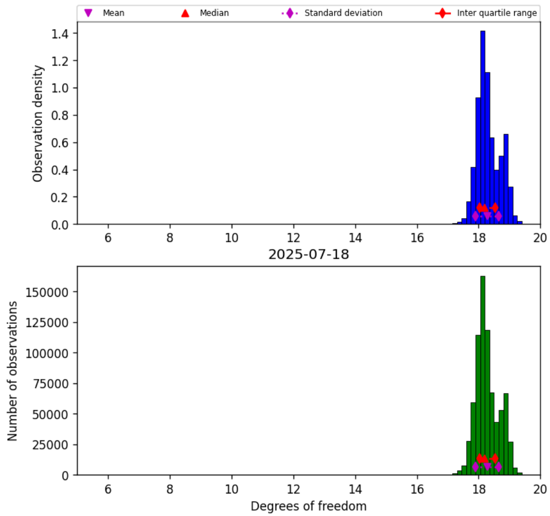
Figure 30: Histogram of “Degrees of freedom” for 2025-07-18 to 2025-07-19
