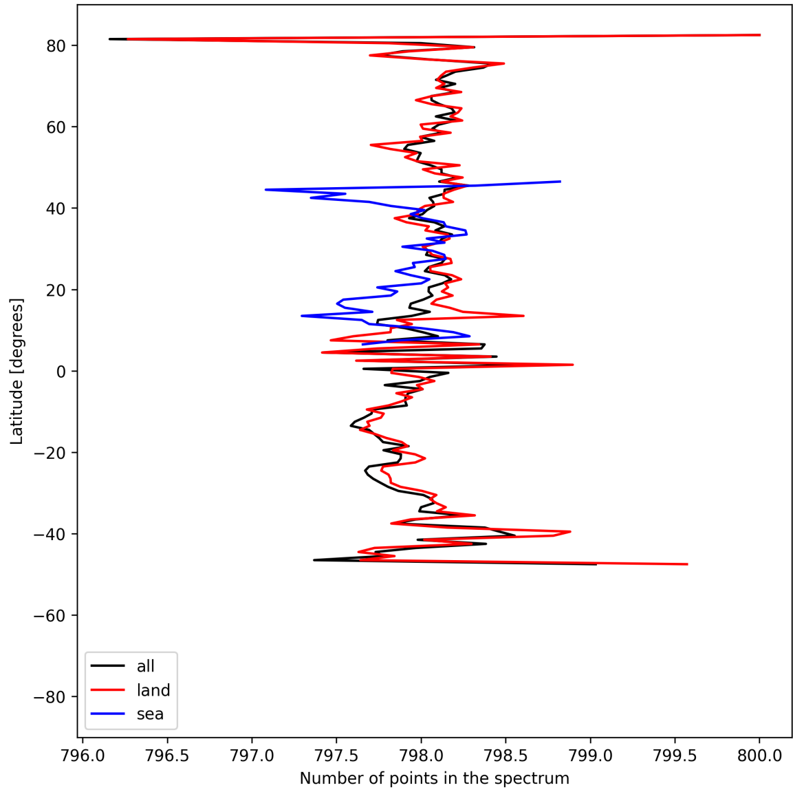
Figure 15: Zonal average of “Number of points in the spectrum” for 2025-07-18 to 2025-07-19.
