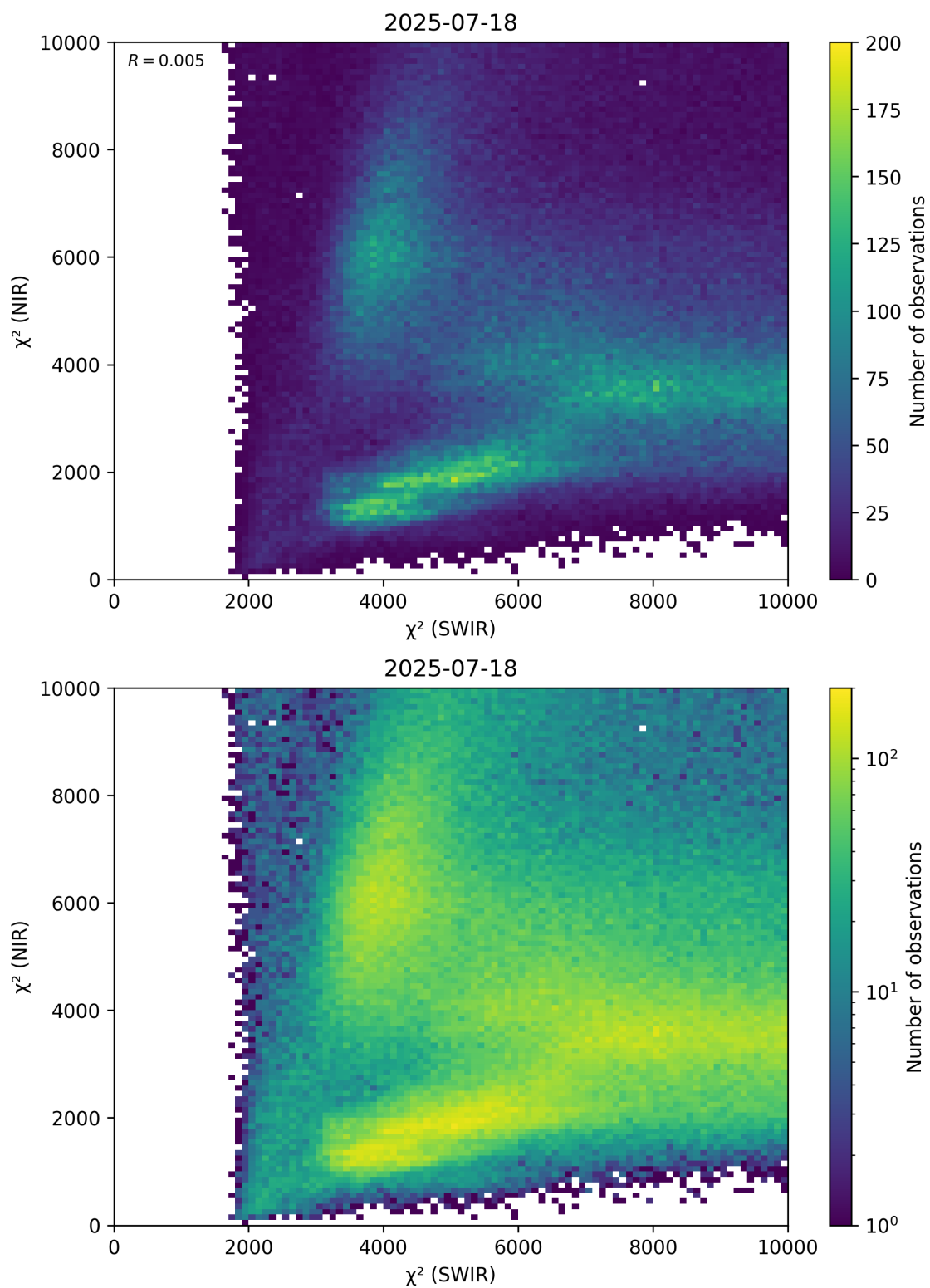
Figure 47: Scatter density plot of “ \chi^2 (SWIR)” against “ \chi^2 (NIR)” for 2025-07-18 to 2025-07-19.
