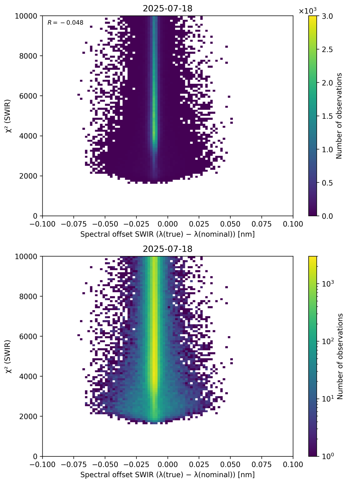
Figure 118: Scatter density plot of “Spectral offset SWIR ( \lambda_{\text{true}} - \lambda_{\text{nominal}} )” against “ \chi^2 (SWIR)” for 2025-07-18 to 2025-07-19.
