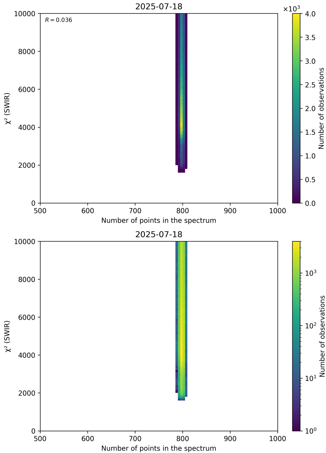
Figure 89: Scatter density plot of “Number of points in the spectrum” against “ \chi^2 (SWIR)” for 2025-07-18 to 2025-07-19.
