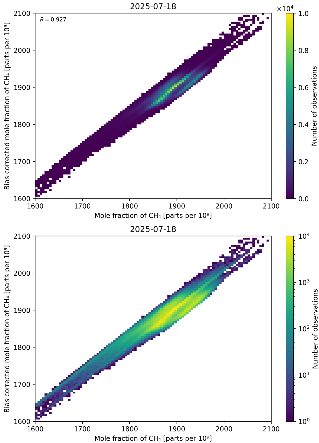
Figure 74: Scatter density plot of “Mole fraction of CH 4 ” against “Bias corrected mole fraction of CH 4 ” for 2025-07-18 to 2025-07-19.
