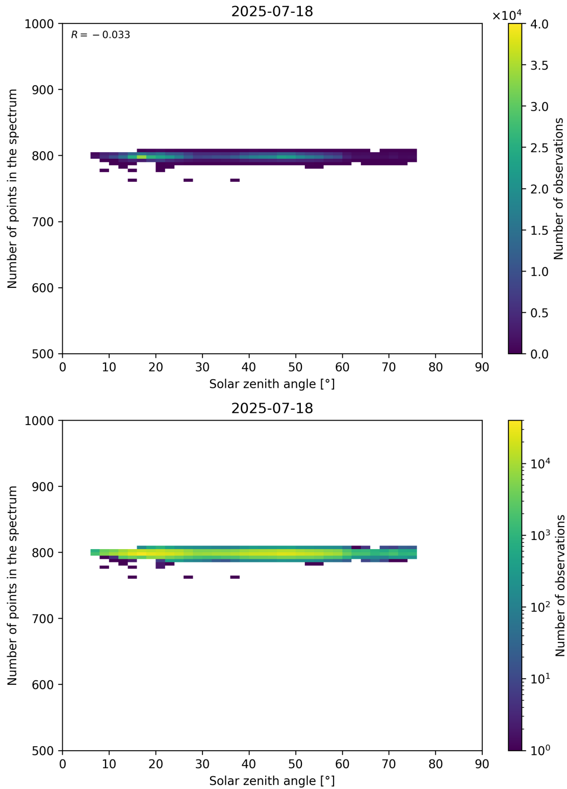
Figure 103: Scatter density plot of “Solar zenith angle” against “Number of points in the spectrum” for 2025-07-18 to 2025-07-19.
