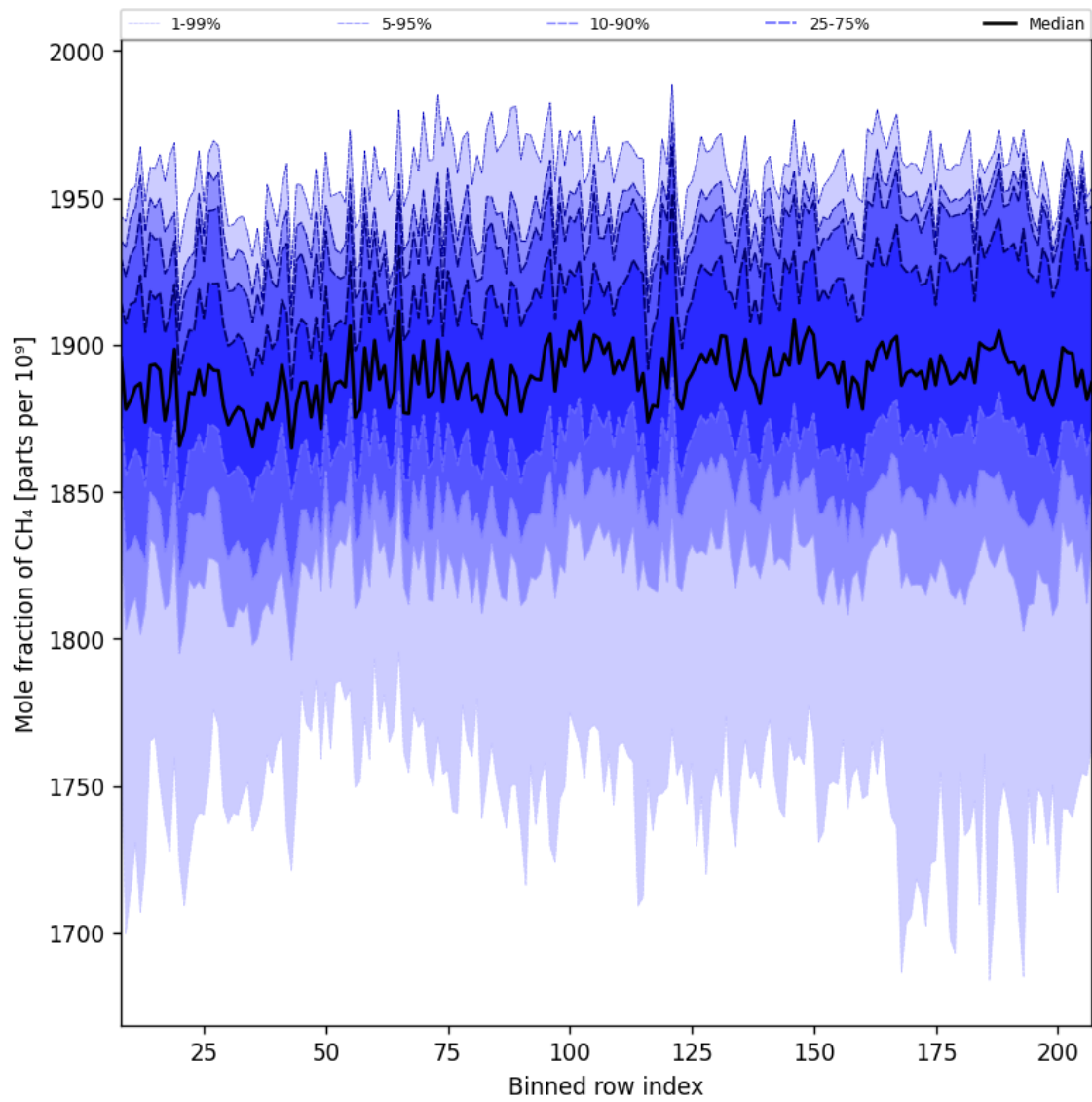
Figure 34: Along track statistics of “Mole fraction of CH 4 ” for 2025-07-18 to 2025-07-19
