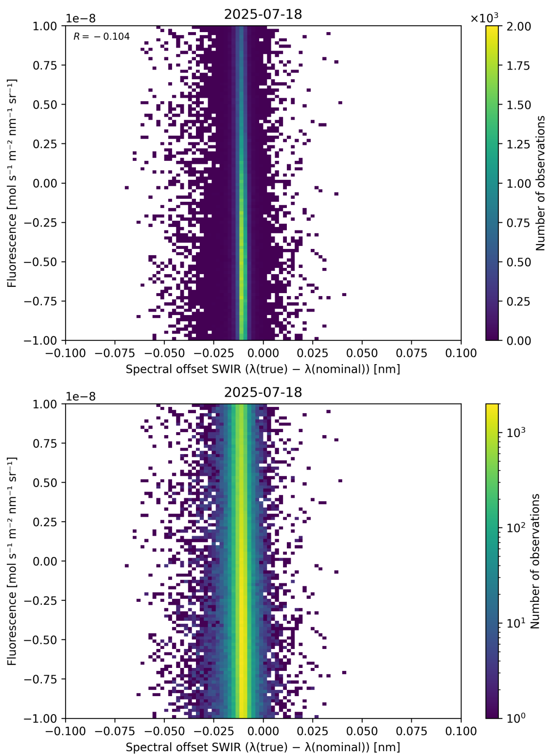
Figure 120: Scatter density plot of “Spectral offset SWIR ( \lambda_{\text{true}} - \lambda_{\text{nominal}} )” against “Fluorescence” for 2025-07-18 to 2025-07-19.
