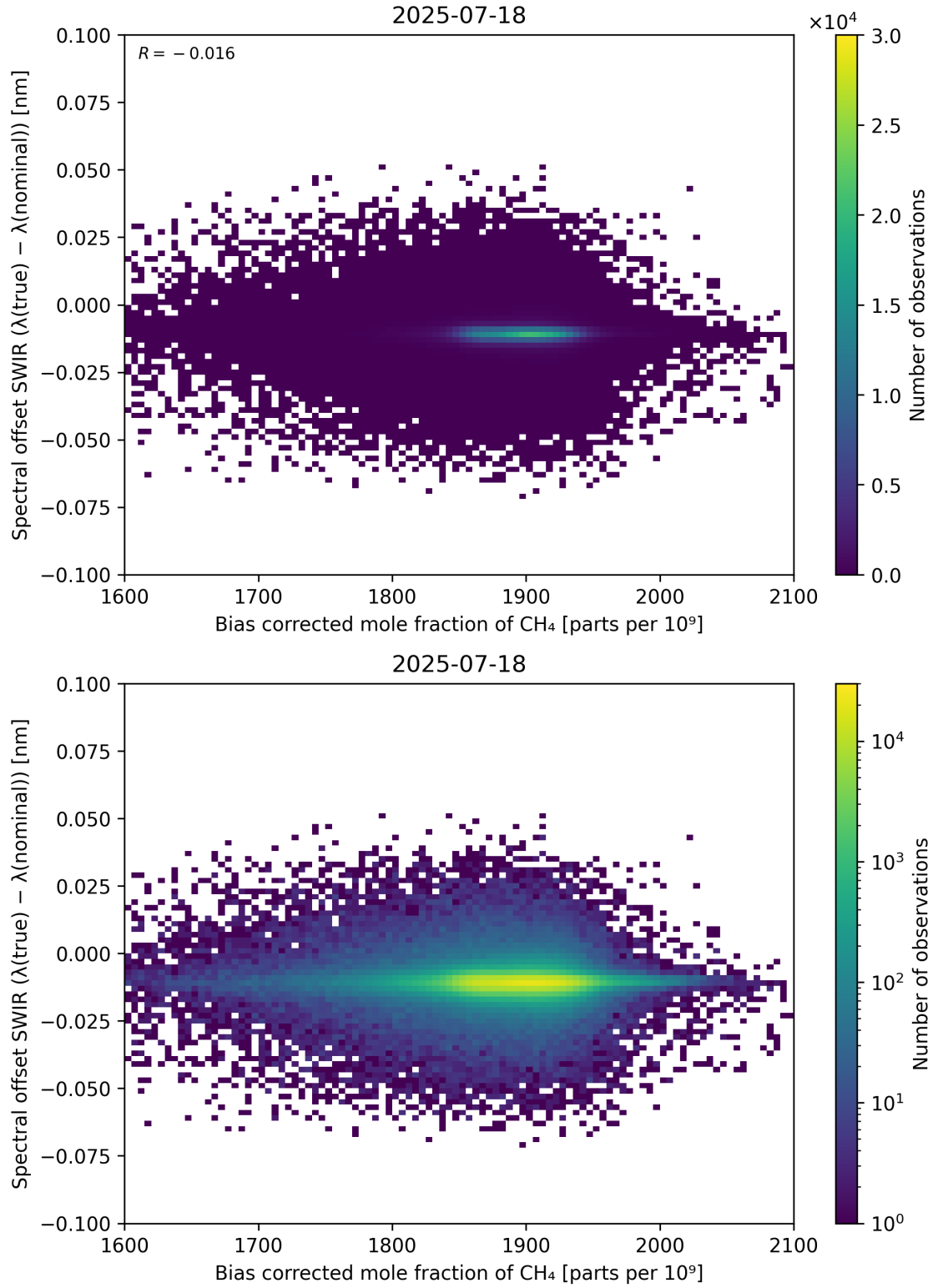
Figure 69: Scatter density plot of “Bias corrected mole fraction of CH 4 ” against “Spectral offset SWIR ( \lambda_{\text{true}} - \lambda_{\text{nominal}} )” for 2025-07-18 to 2025-07-19.
