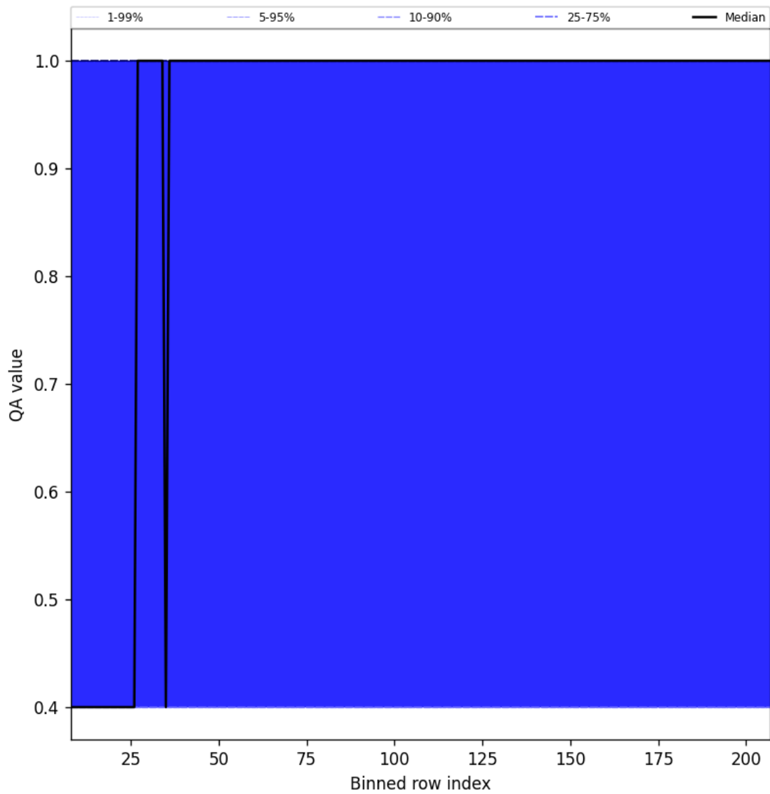
Figure 33: Along track statistics of “QA value” for 2025-07-18 to 2025-07-19
