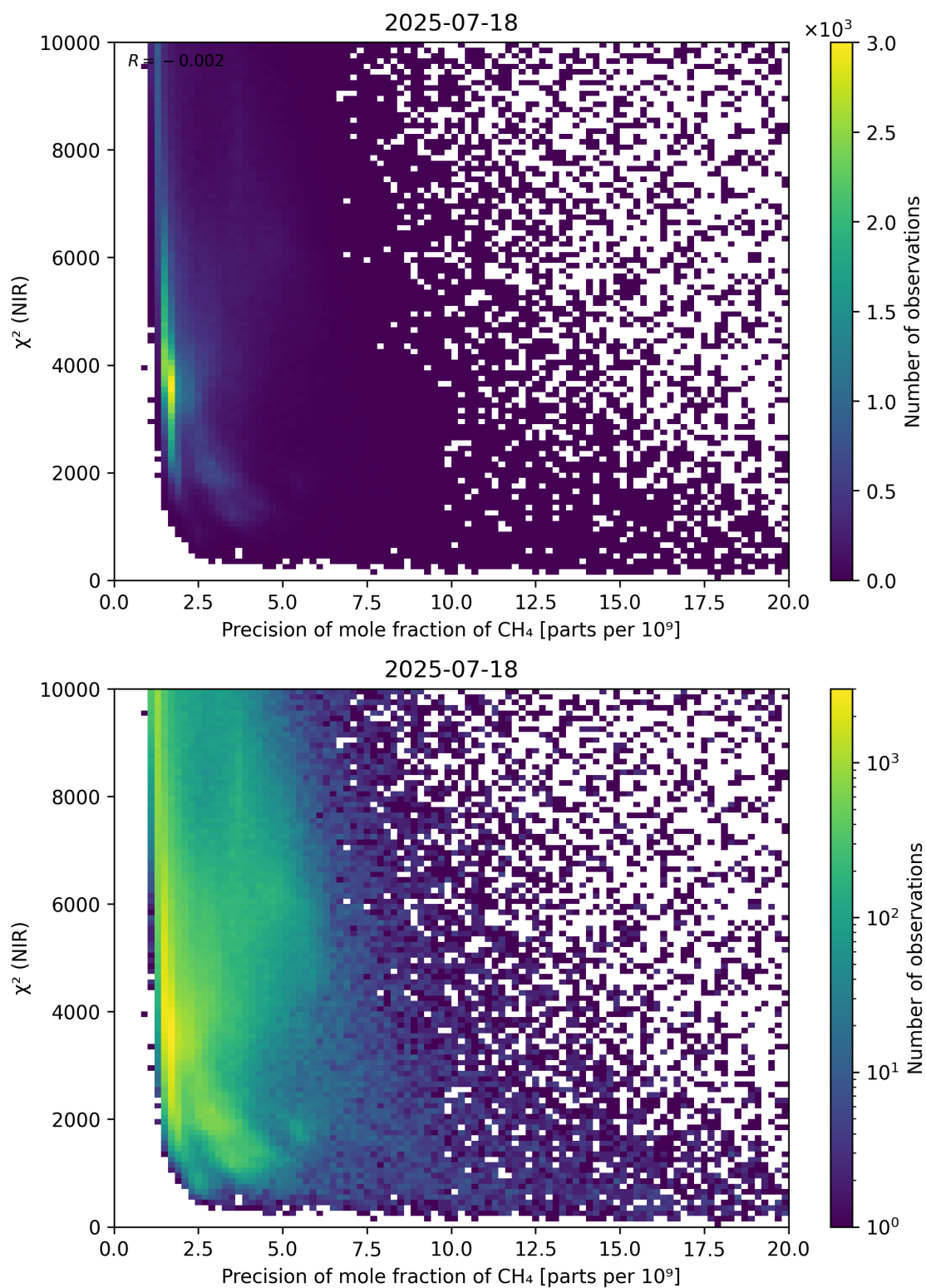
Figure 78: Scatter density plot of “Precision of mole fraction of CH 4 ” against “ \chi^2 (NIR)” for 2025-07-18 to 2025-07-19.
