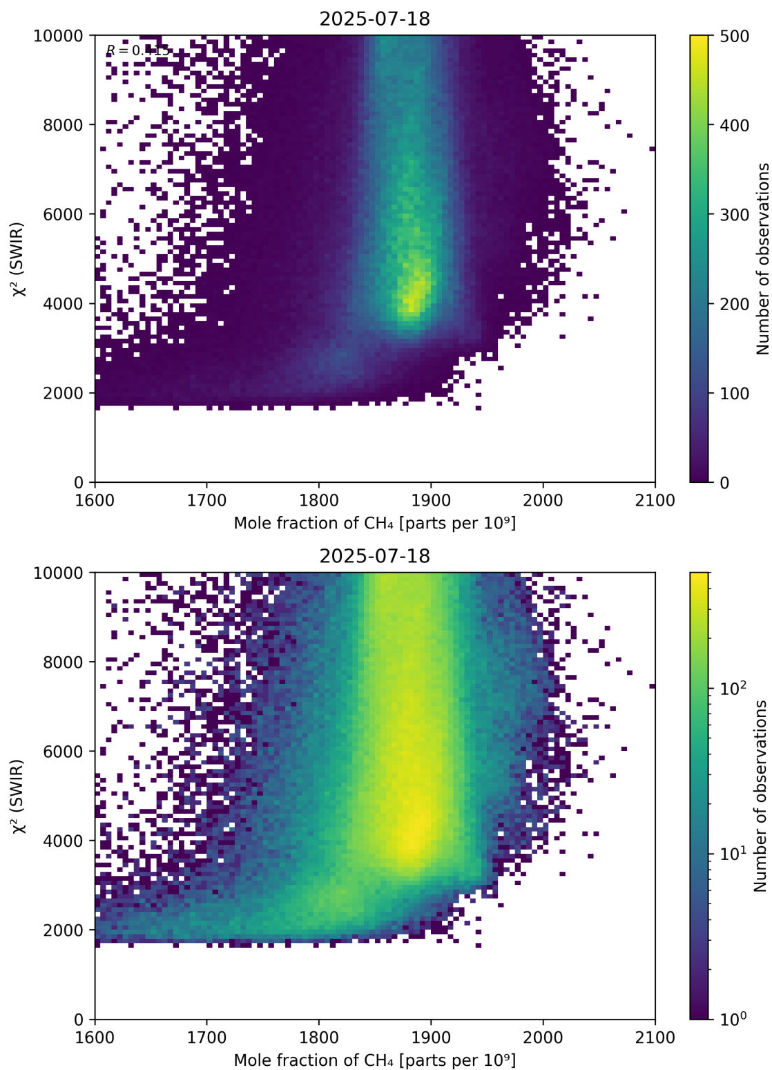
Figure 71: Scatter density plot of “Mole fraction of CH 4 ” against “ \chi^2 (SWIR)” for 2025-07-18 to 2025-07-19.
