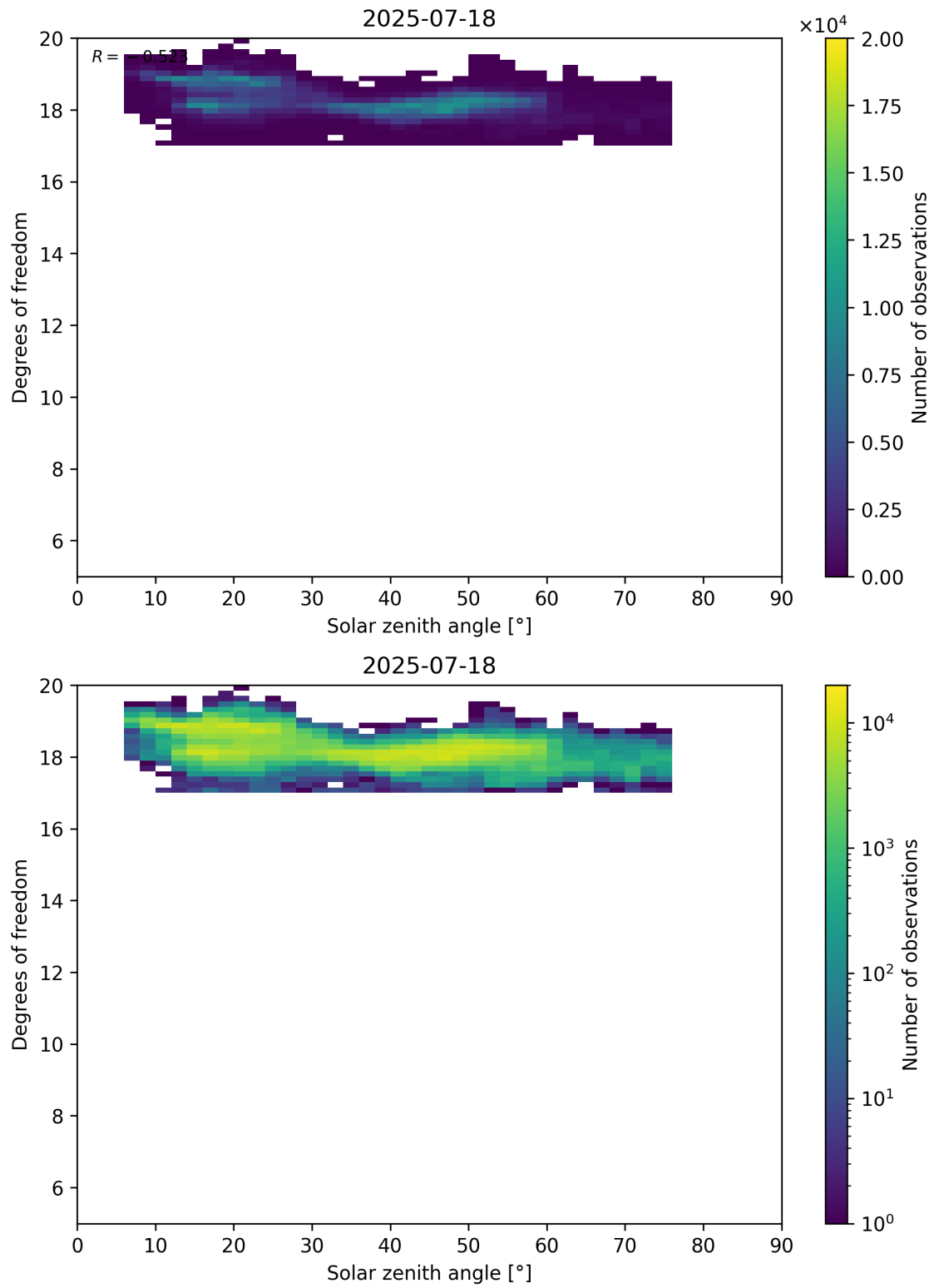
Figure 96: Scatter density plot of “Solar zenith angle” against “Degrees of freedom” for 2025-07-18 to 2025-07-19.
