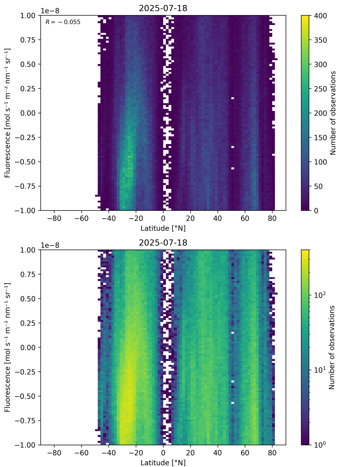
Figure 56: Scatter density plot of “Latitude” against “Fluorescence” for 2025-07-18 to 2025-07-19.
