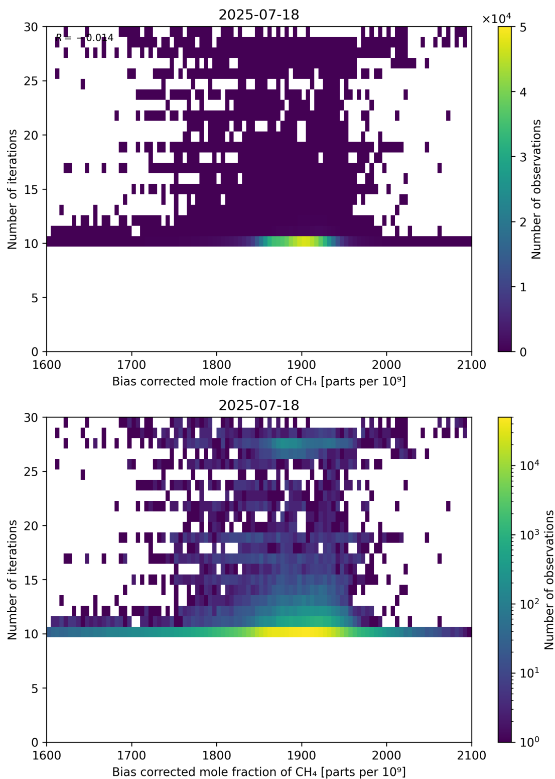
Figure 67: Scatter density plot of “Bias corrected mole fraction of CH 4 ” against “Number of iterations” for 2025-07-18 to 2025-07-19.
