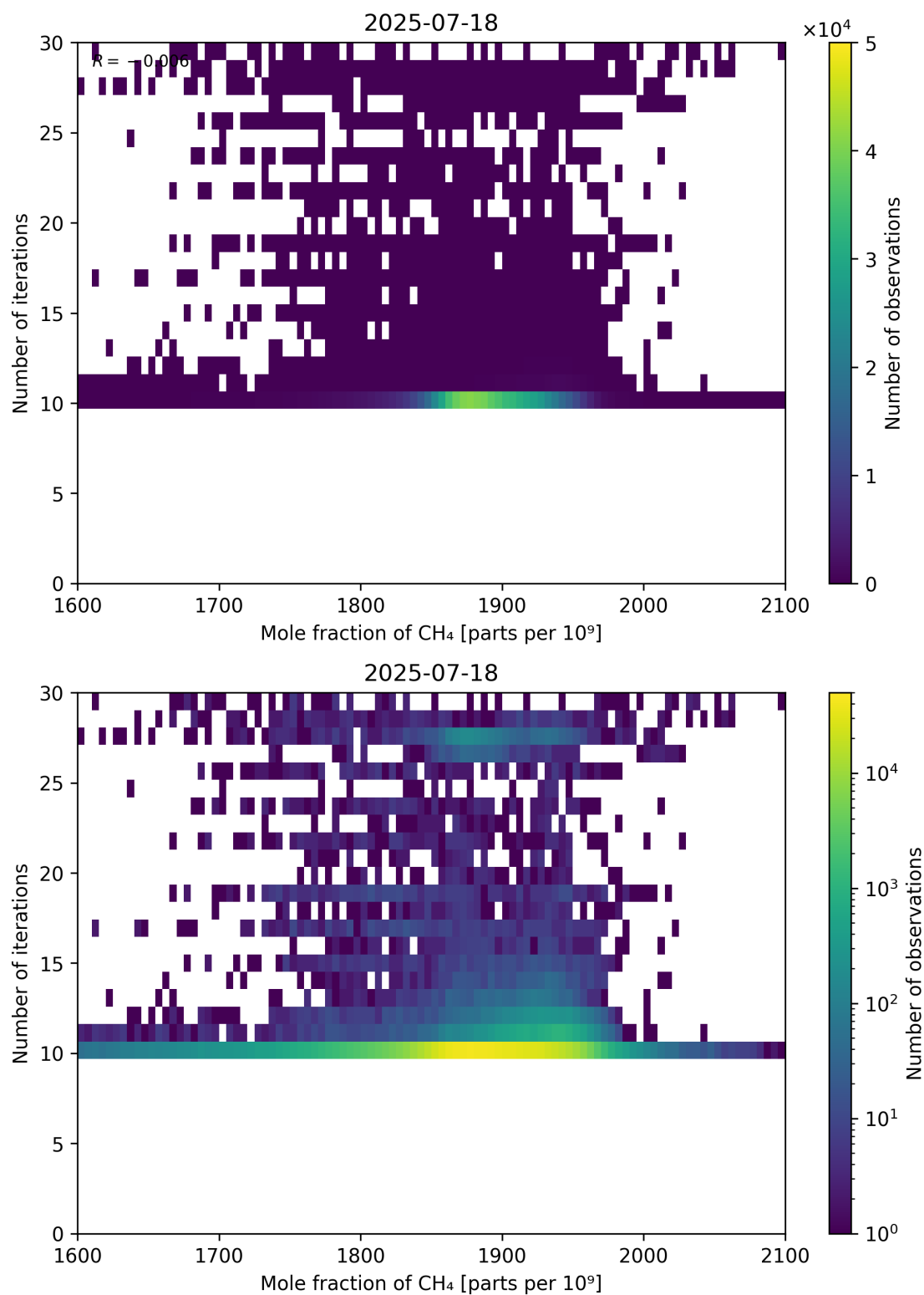
Figure 76: Scatter density plot of “Mole fraction of CH 4 ” against “Number of iterations” for 2025-07-18 to 2025-07-19.
