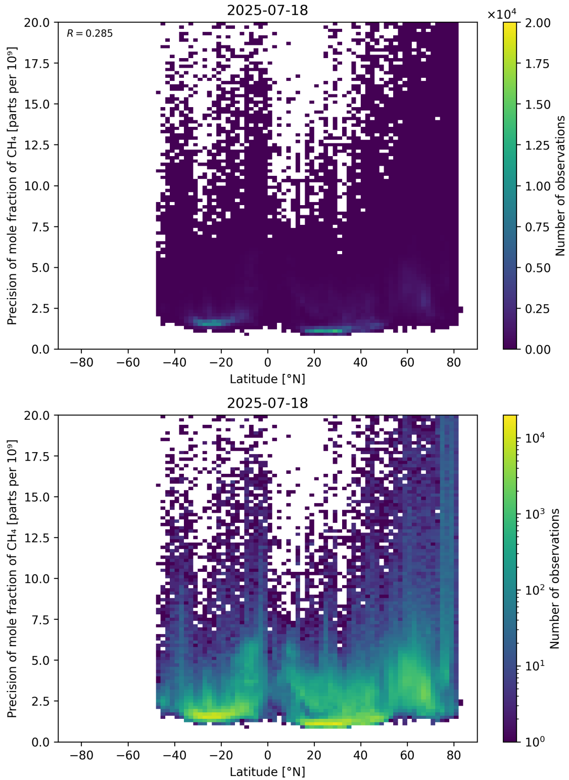
Figure 59: Scatter density plot of “Latitude” against “Precision of mole fraction of \text{CH}_4 ” for 2025-07-18 to 2025-07-19.
