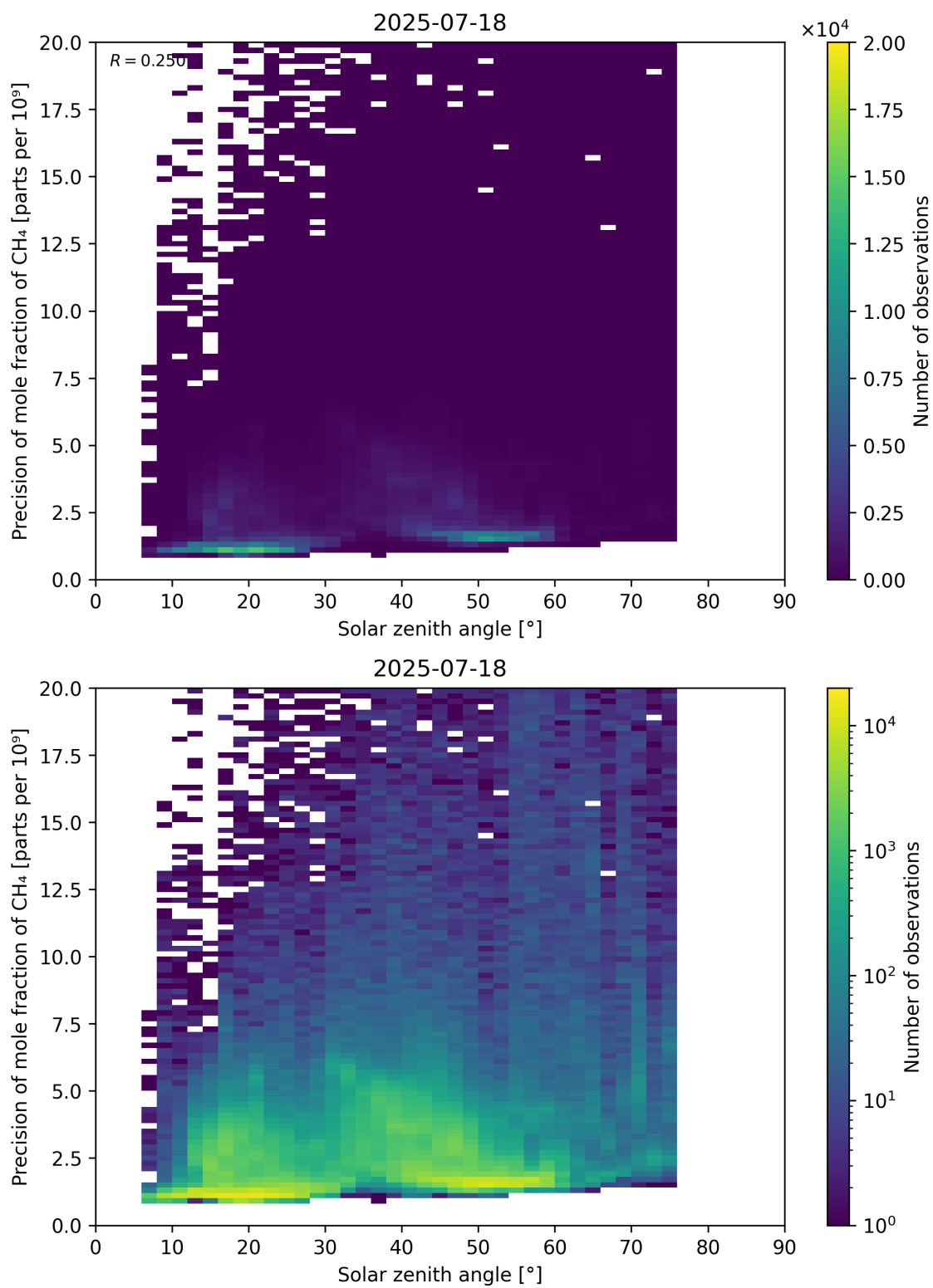
Figure 101: Scatter density plot of “Solar zenith angle” against “Precision of mole fraction of CH 4 ” for 2025-07-18 to 2025-07-19.
