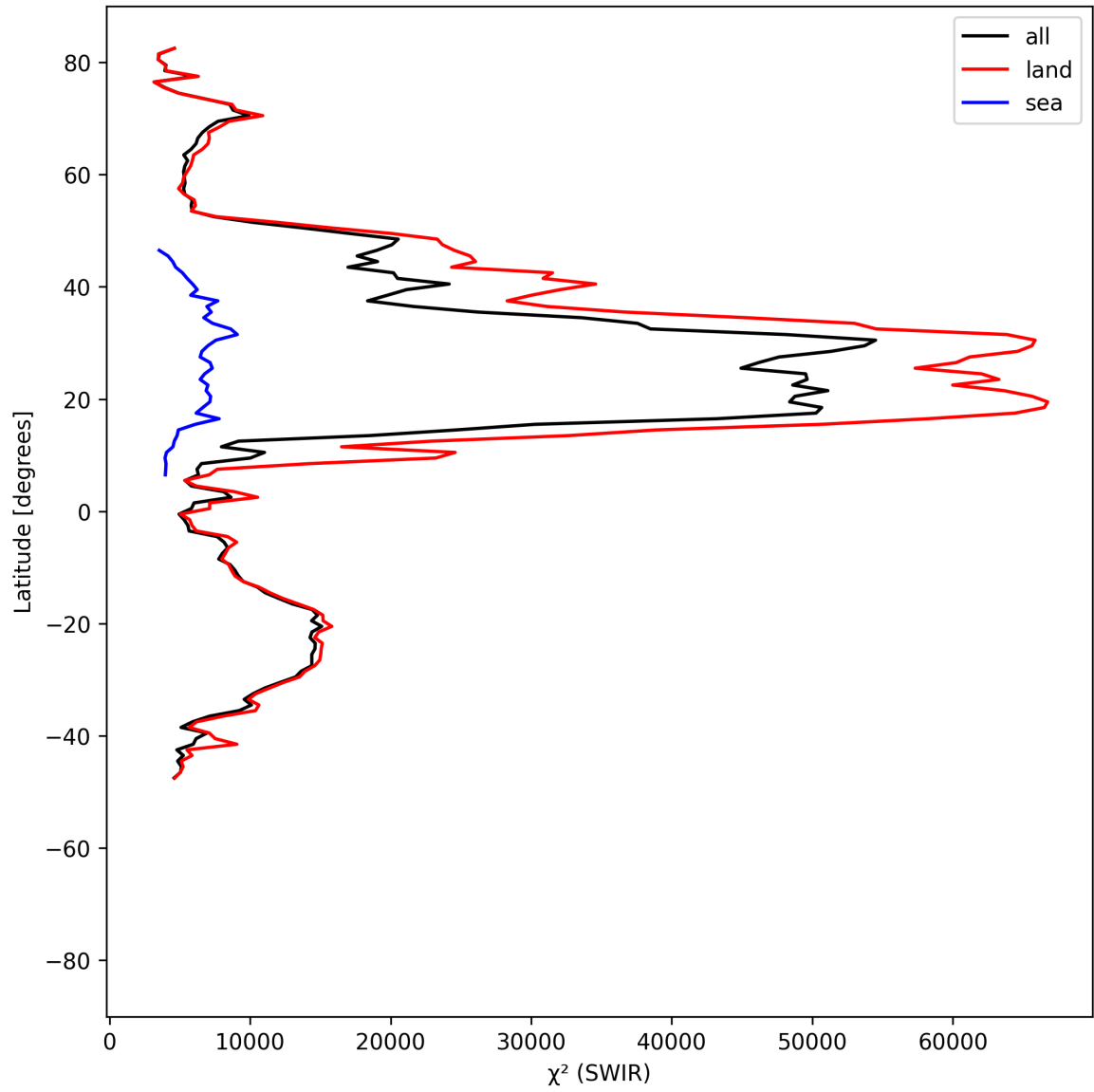
Figure 17: Zonal average of “ \chi^2 (SWIR)” for 2025-07-18 to 2025-07-19.
