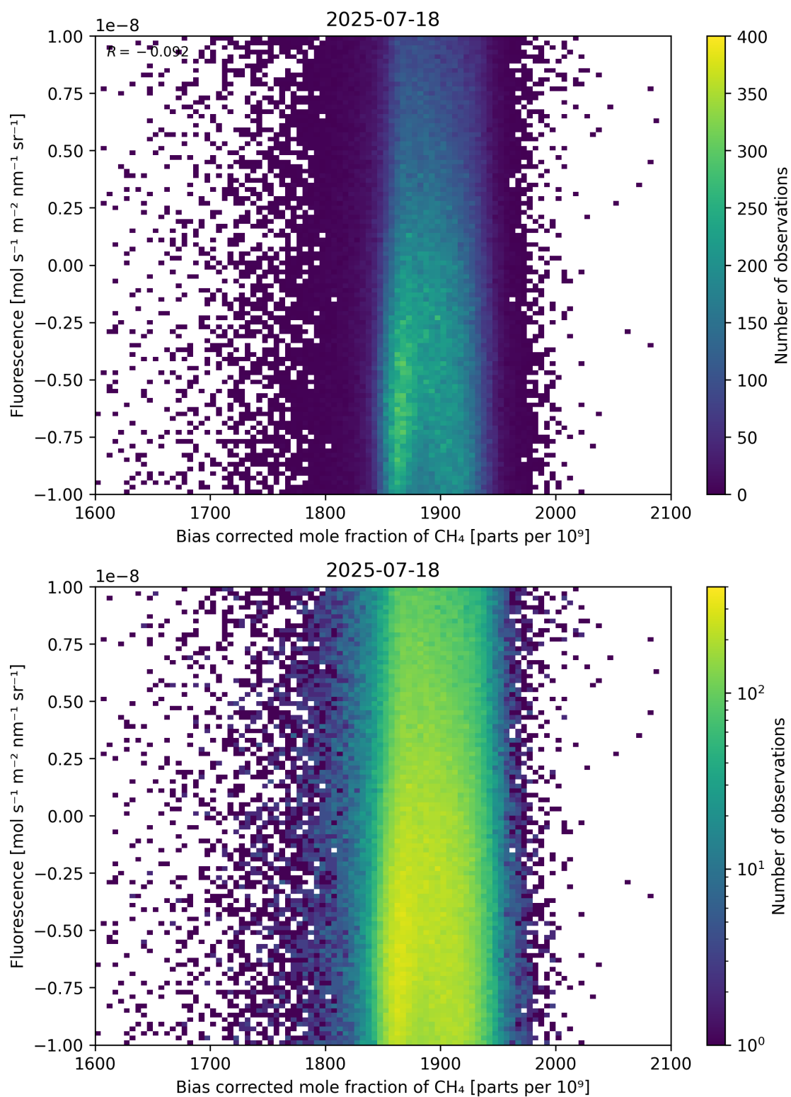
Figure 66: Scatter density plot of “Bias corrected mole fraction of \text{CH}_4 ” against “Fluorescence” for 2025-07-18 to 2025-07-19.
