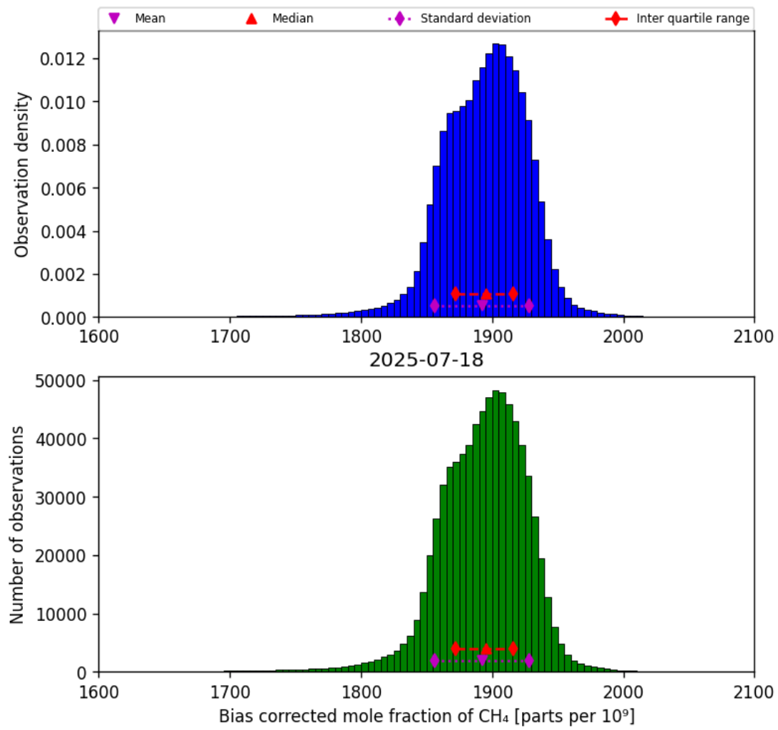
Figure 25: Histogram of “Bias corrected mole fraction of CH 4 ” for 2025-07-18 to 2025-07-19
