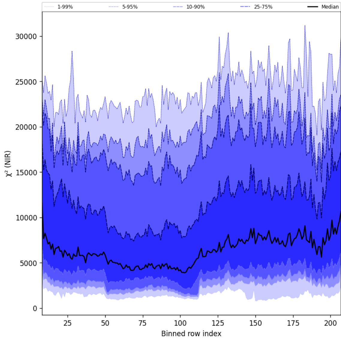
Figure 40: Along track statistics of “ \chi^2 (NIR)” for 2025-07-18 to 2025-07-19
