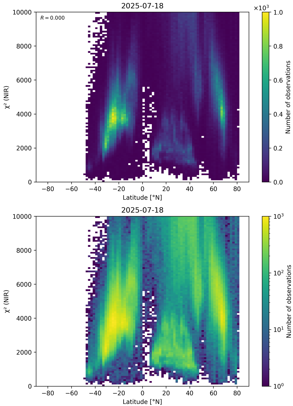
Figure 53: Scatter density plot of “Latitude” against “ \chi^2 (NIR)” for 2025-07-18 to 2025-07-19.
