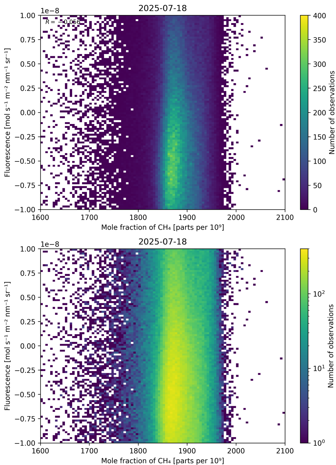
Figure 73: Scatter density plot of “Mole fraction of \text{CH}_4 ” against “Fluorescence” for 2025-07-18 to 2025-07-19.
