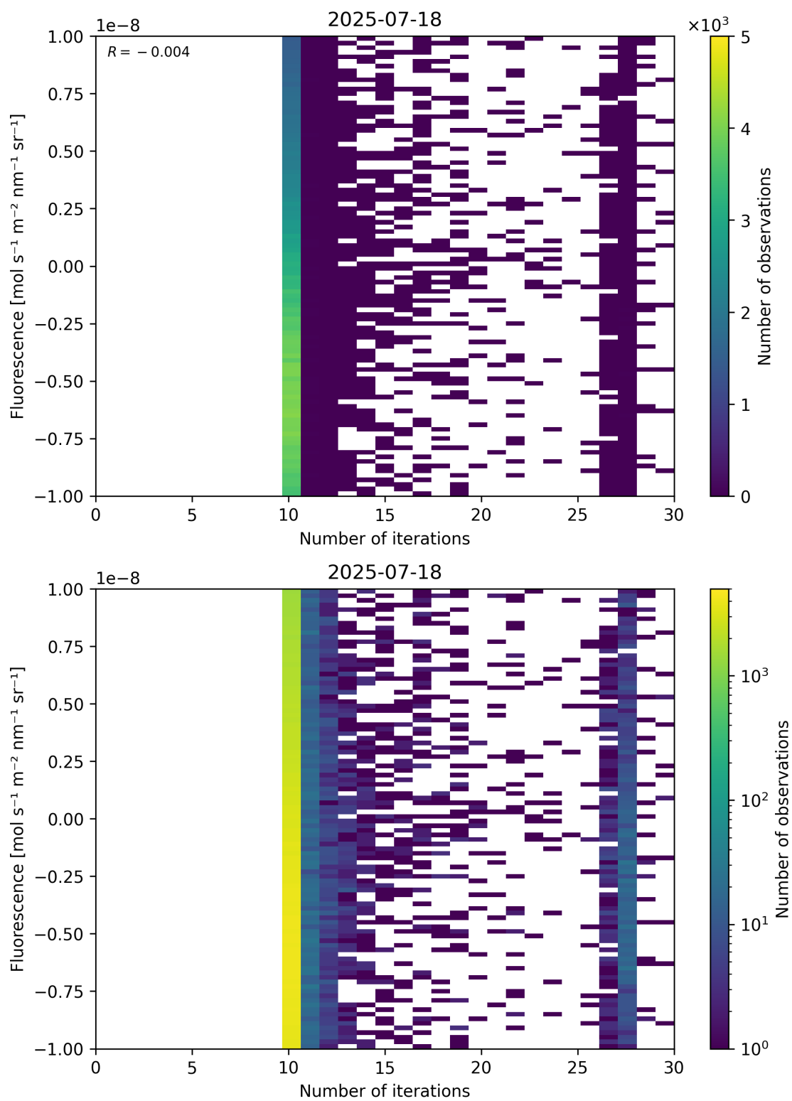
Figure 87: Scatter density plot of “Number of iterations” against “Fluorescence” for 2025-07-18 to 2025-07-19.
