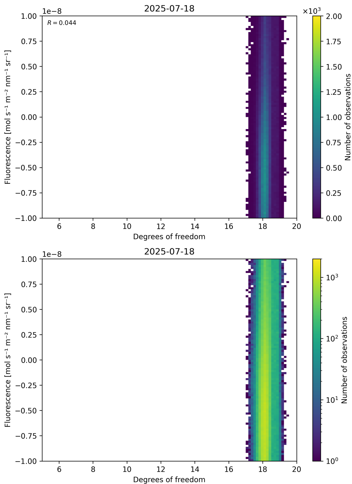
Figure 51: Scatter density plot of “Degrees of freedom” against “Fluorescence” for 2025-07-18 to 2025-07-19.
