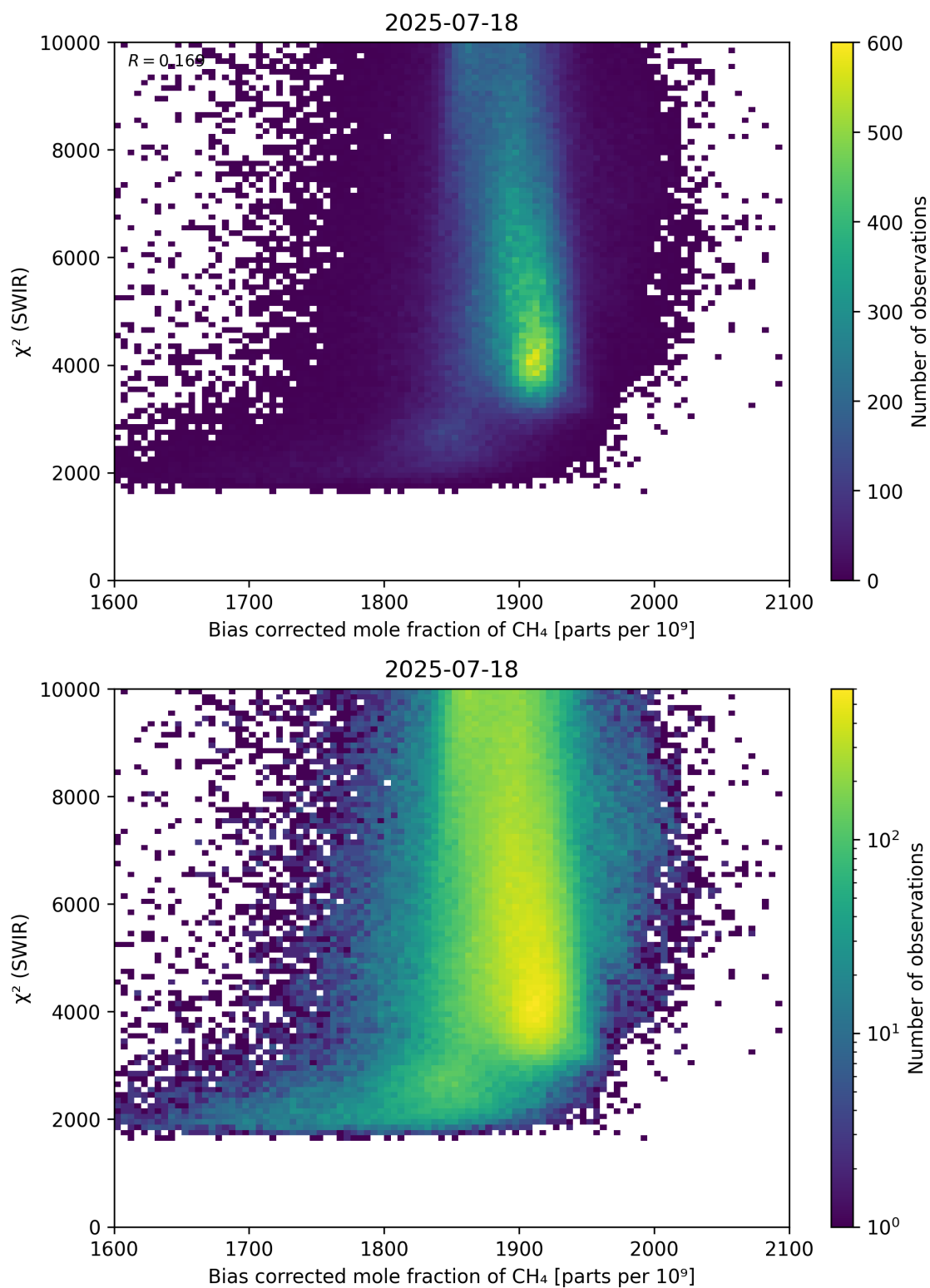
Figure 64: Scatter density plot of “Bias corrected mole fraction of \text{CH}_4 ” against “ \chi^2 (SWIR)” for 2025-07-18 to 2025-07-19.
