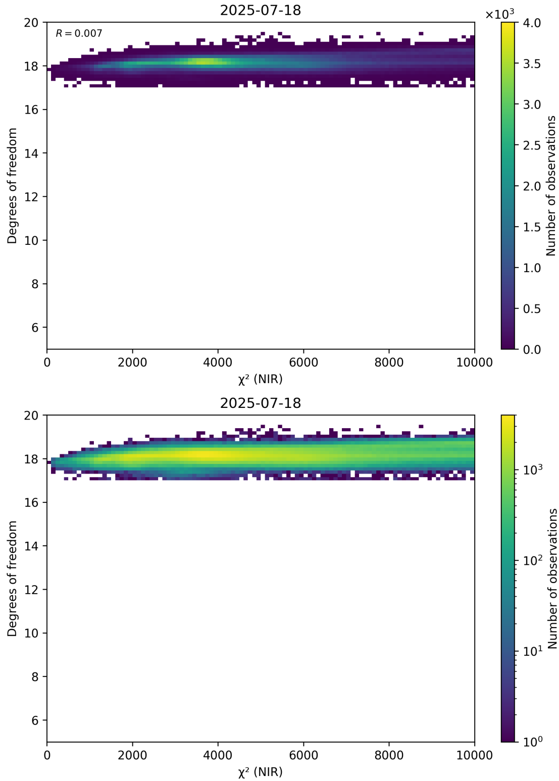
Figure 44: Scatter density plot of “ \chi^2 (NIR)” against “Degrees of freedom” for 2025-07-18 to 2025-07-19.
