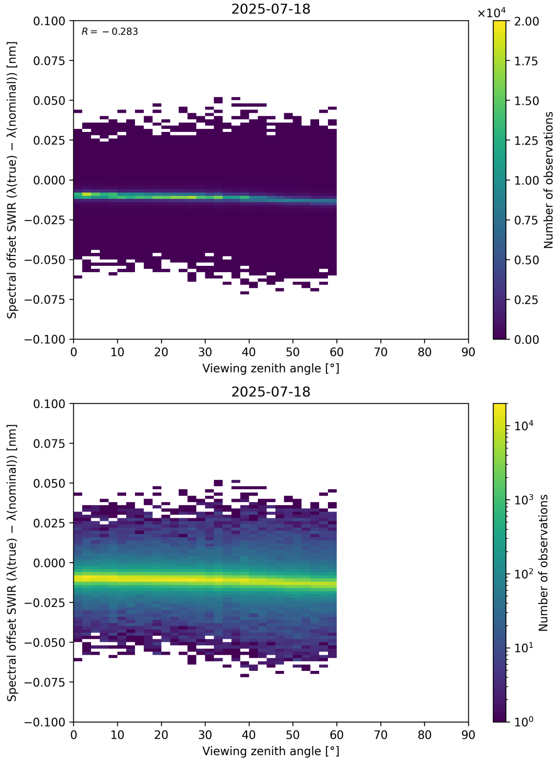
Figure 116: Scatter density plot of “Viewing zenith angle” against “Spectral offset SWIR ( \lambda_{\text{true}} - \lambda_{\text{nominal}} )” for 2025-07-18 to 2025-07-19.
