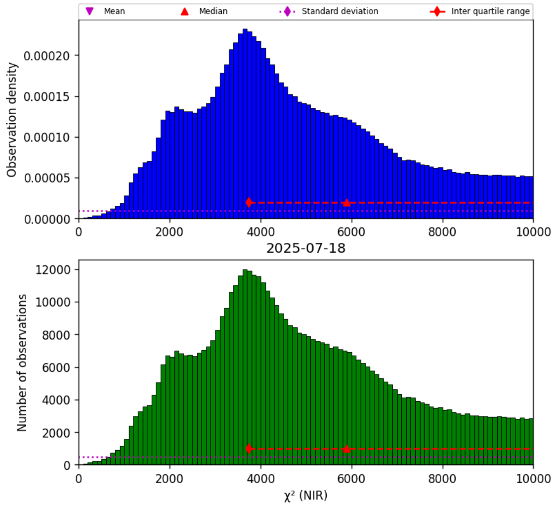
Figure 29: Histogram of “ \chi^2 (NIR)” for 2025-07-18 to 2025-07-19
