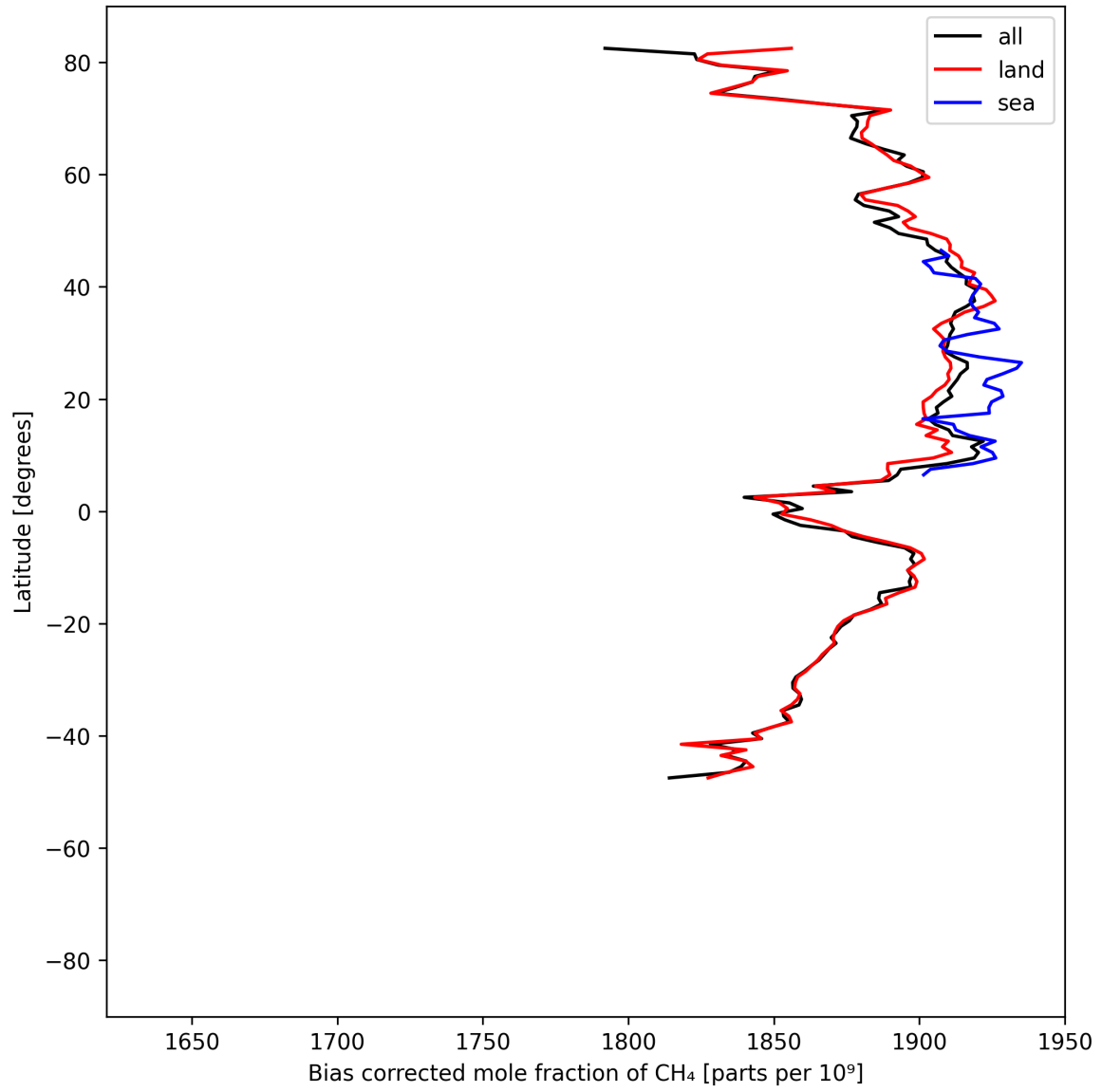
Figure 14: Zonal average of “Bias corrected mole fraction of \text{CH}_4 ” for 2025-07-18 to 2025-07-19.
