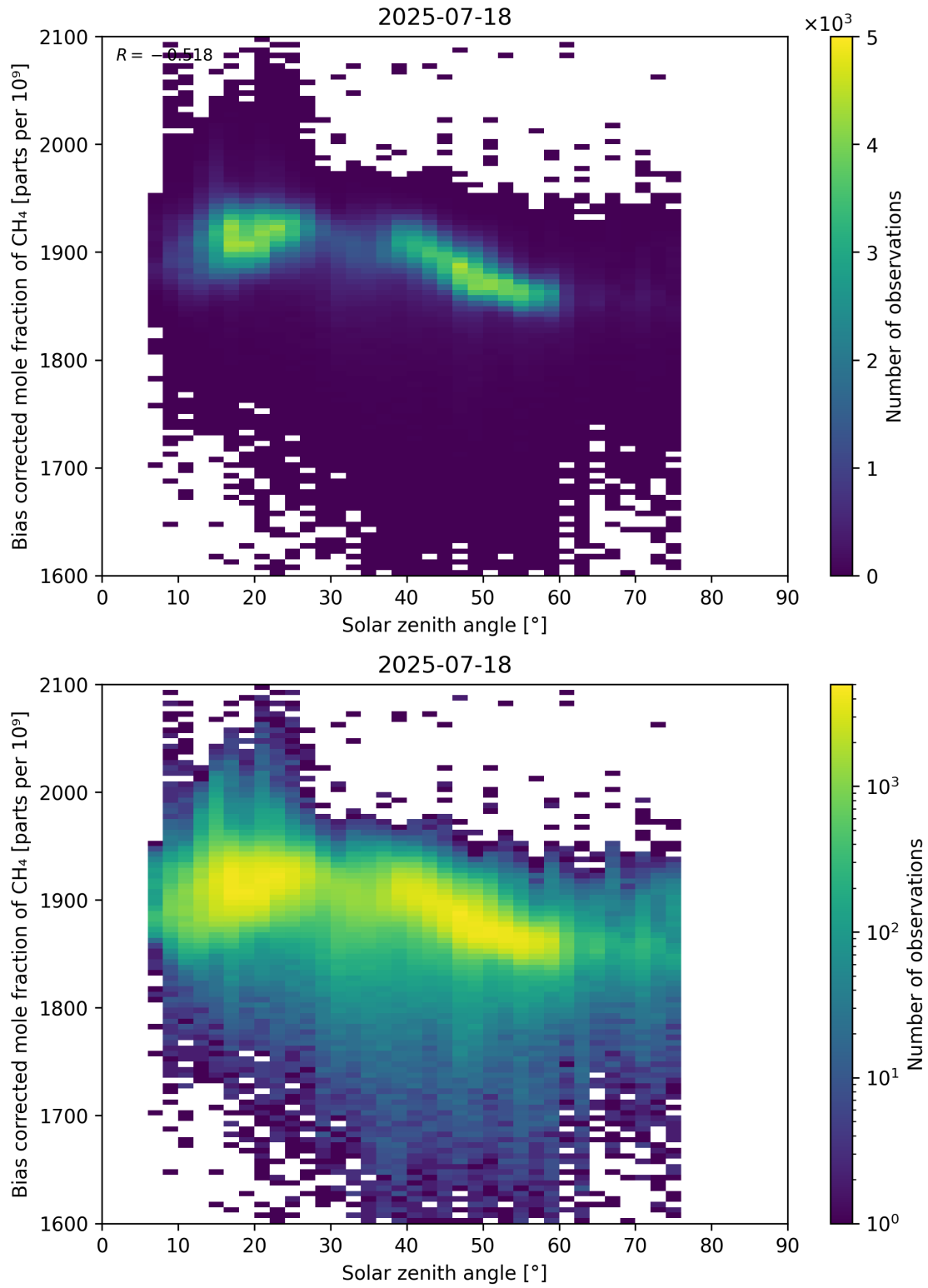
Figure 100: Scatter density plot of “Solar zenith angle” against “Bias corrected mole fraction of CH 4 ” for 2025-07-18 to 2025-07-19.
