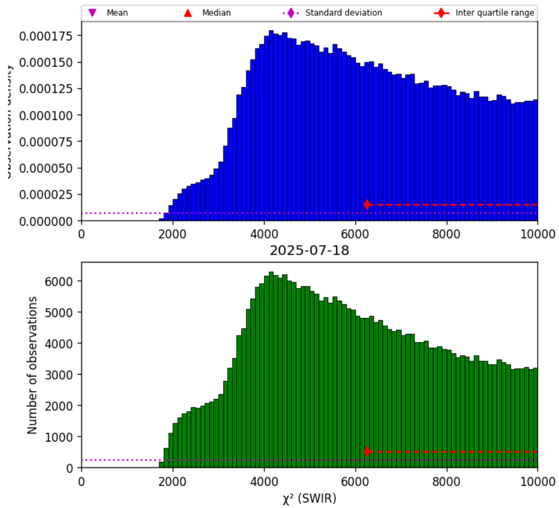
Figure 28: Histogram of “ \chi^2 (SWIR)” for 2025-07-18 to 2025-07-19
