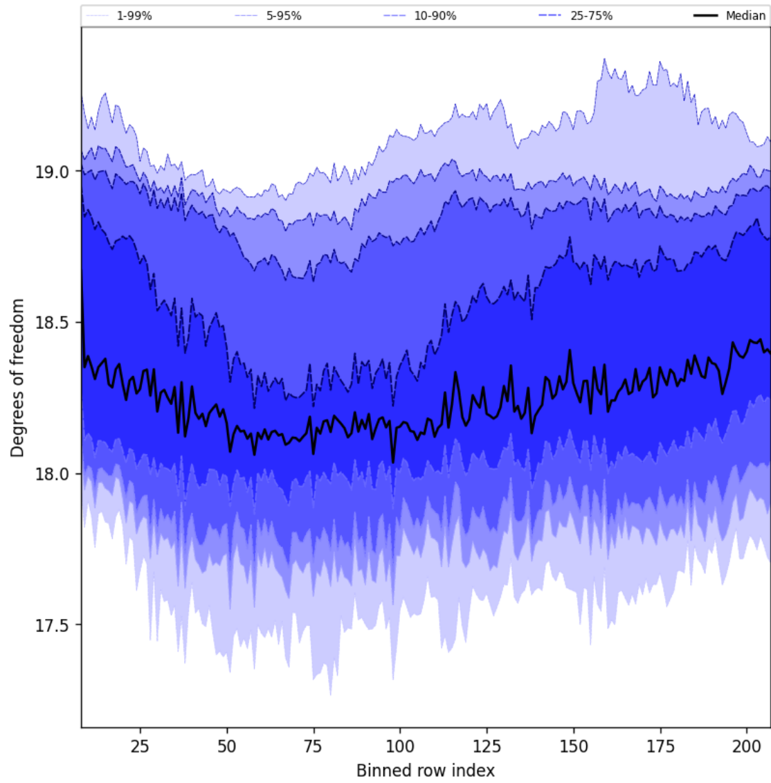
Figure 41: Along track statistics of “Degrees of freedom” for 2025-07-18 to 2025-07-19
