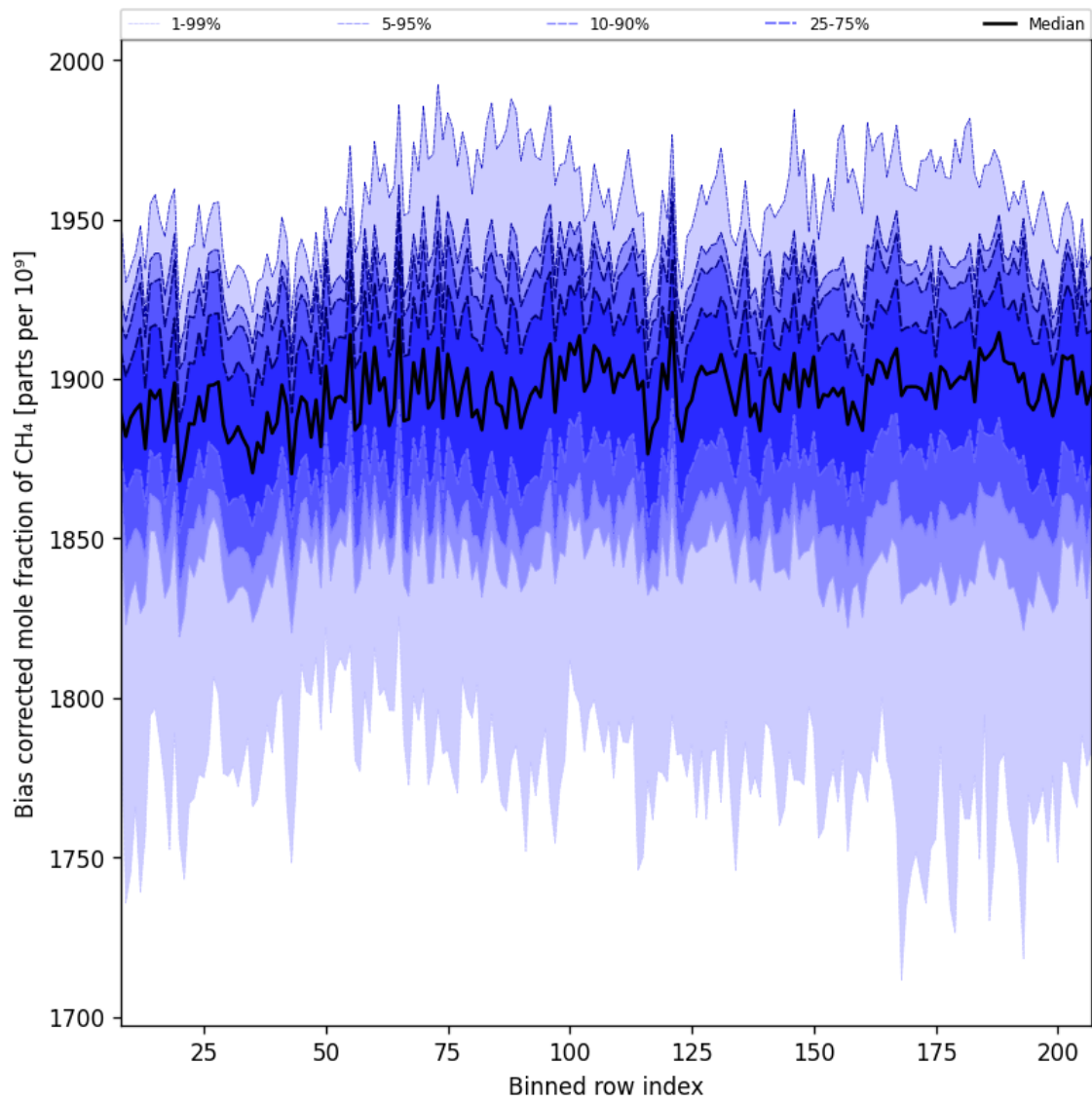
Figure 36: Along track statistics of “Bias corrected mole fraction of CH 4 ” for 2025-07-18 to 2025-07-19
