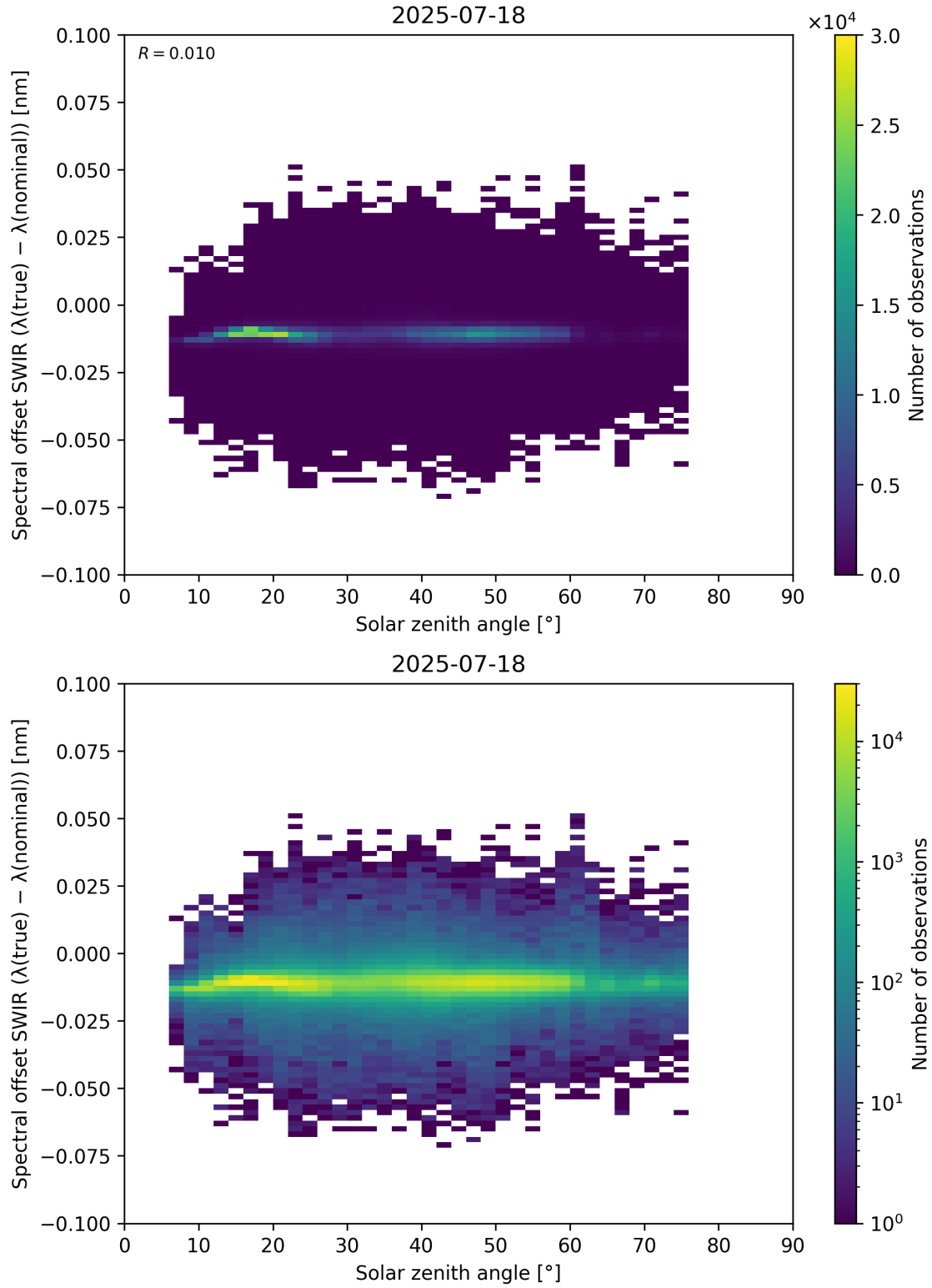
Figure 104: Scatter density plot of “Solar zenith angle” against “Spectral offset SWIR ( \lambda_{\text{true}} - \lambda_{\text{nominal}} )” for 2025-07-18 to 2025-07-19.
