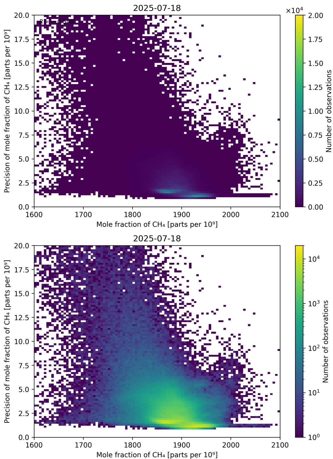
Figure 75: Scatter density plot of “Mole fraction of CH 4 ” against “Precision of mole fraction of CH 4 ” for 2025-07-18 to 2025-07-19.
