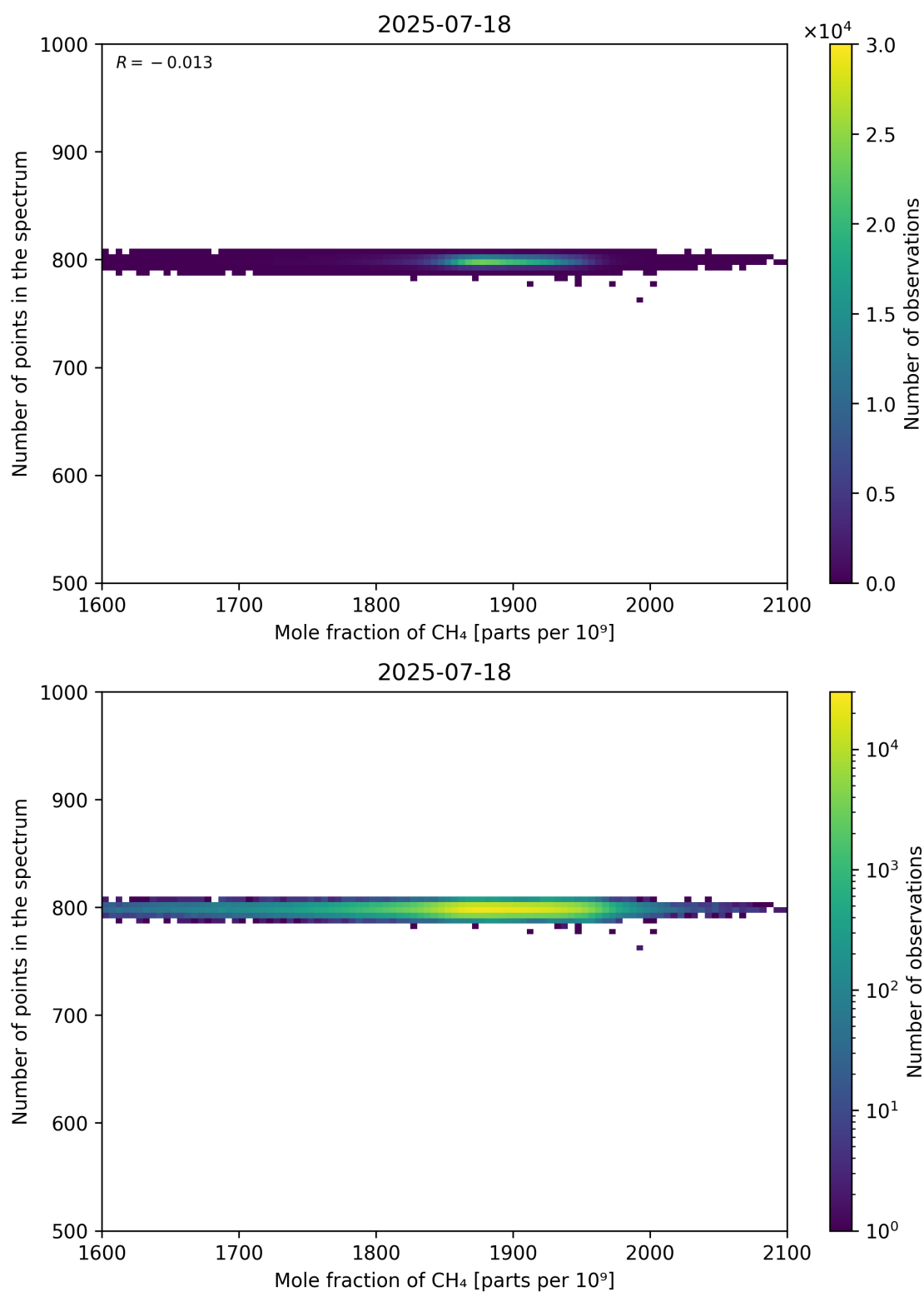
Figure 77: Scatter density plot of “Mole fraction of CH 4 ” against “Number of points in the spectrum” for 2025-07-18 to 2025-07-19.
