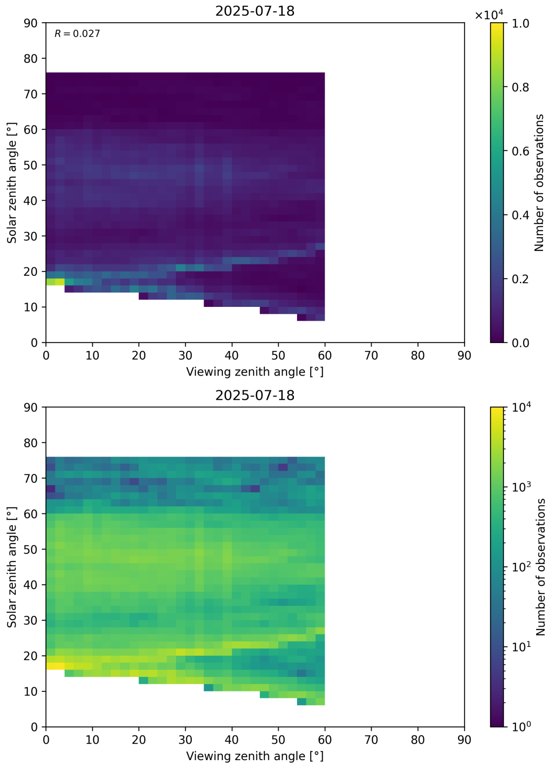
Figure 115: Scatter density plot of “Viewing zenith angle” against “Solar zenith angle” for 2025-07-18 to 2025-07-19.
