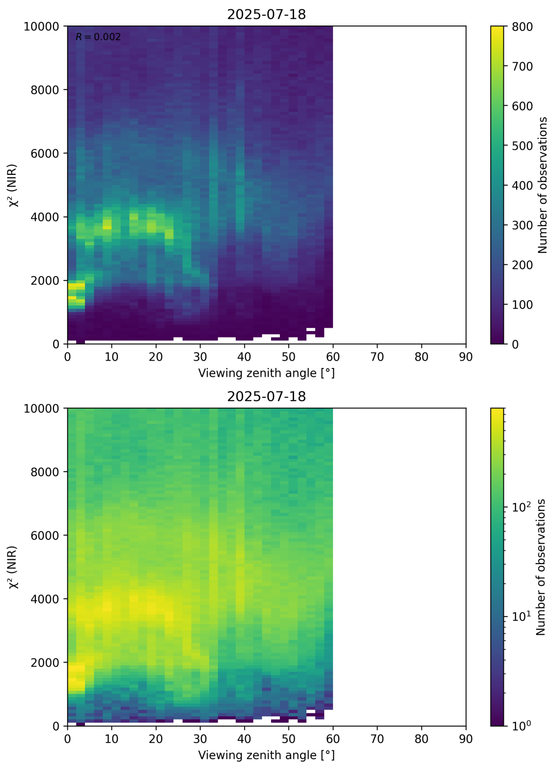
Figure 105: Scatter density plot of “Viewing zenith angle” against “ \chi^2 (NIR)” for 2025-07-18 to 2025-07-19.
