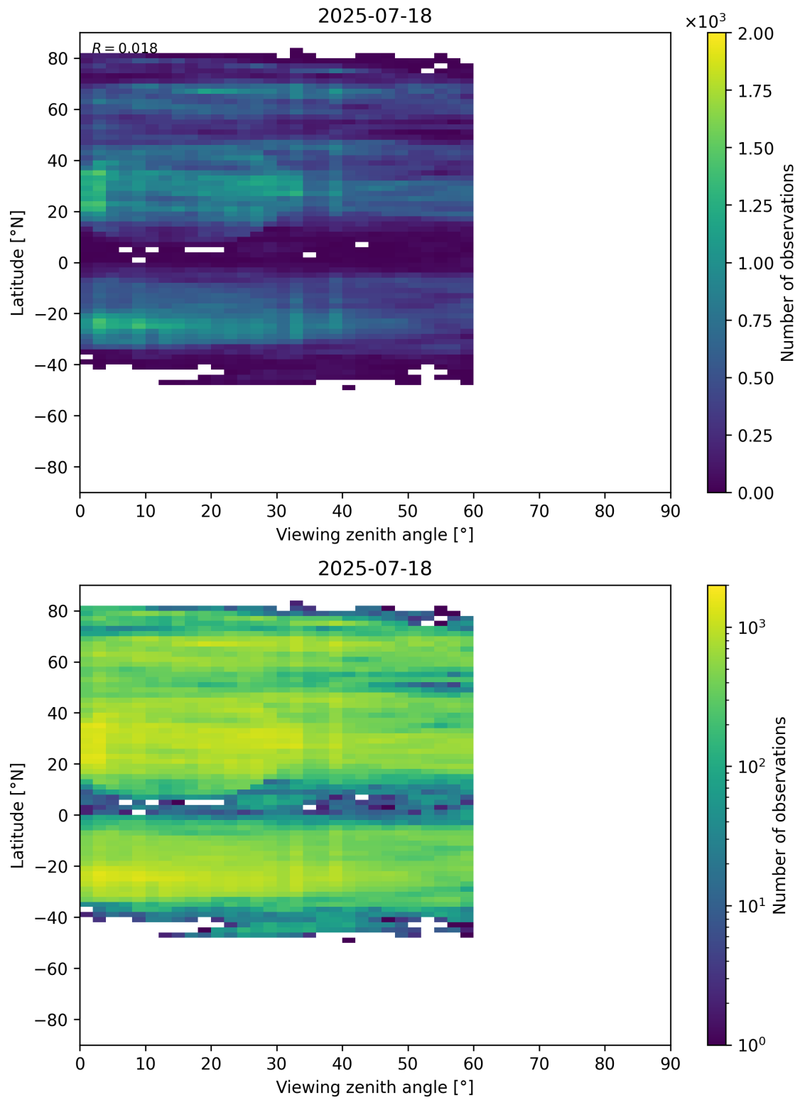
Figure 109: Scatter density plot of “Viewing zenith angle” against “Latitude” for 2025-07-18 to 2025-07-19.
