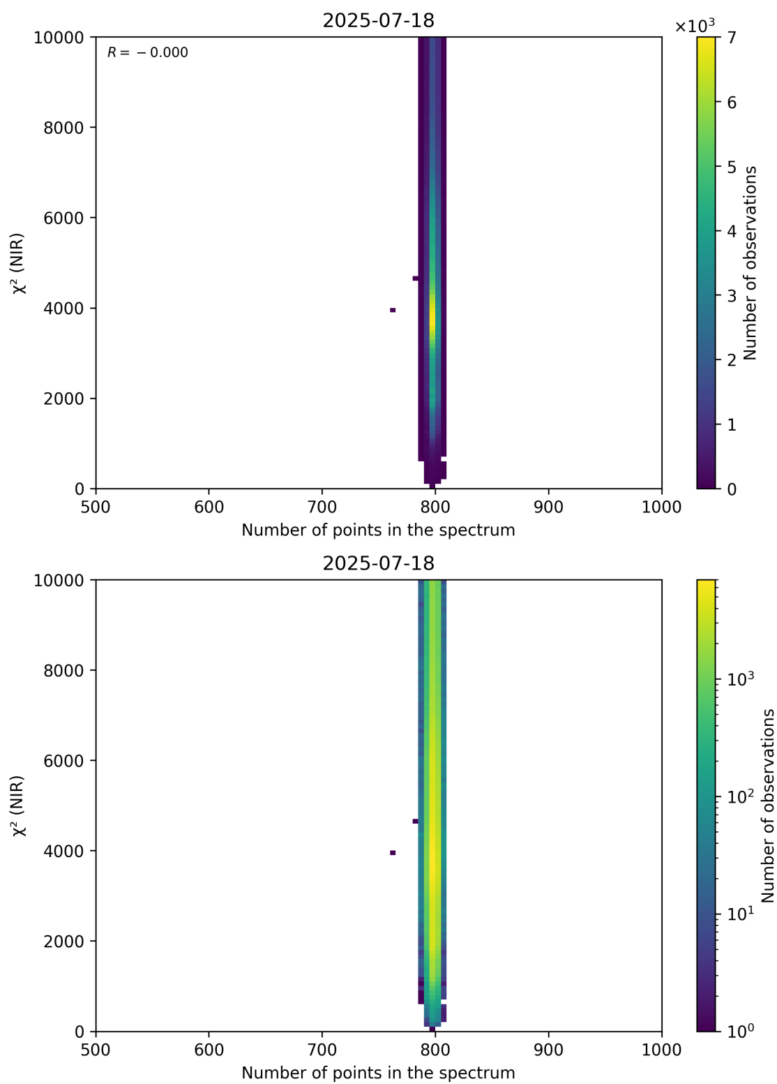
Figure 88: Scatter density plot of “Number of points in the spectrum” against “ \chi^2 (NIR)” for 2025-07-18 to 2025-07-19.
