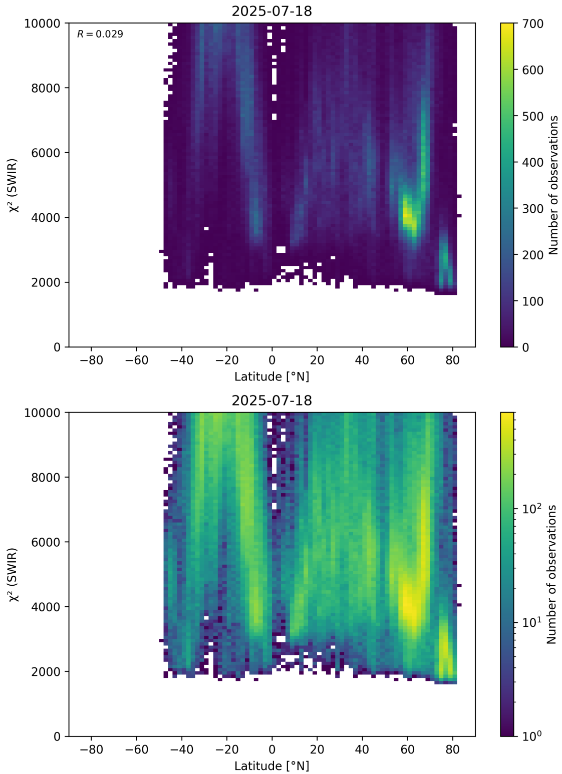
Figure 54: Scatter density plot of “Latitude” against “ \chi^2 (SWIR)” for 2025-07-18 to 2025-07-19.
