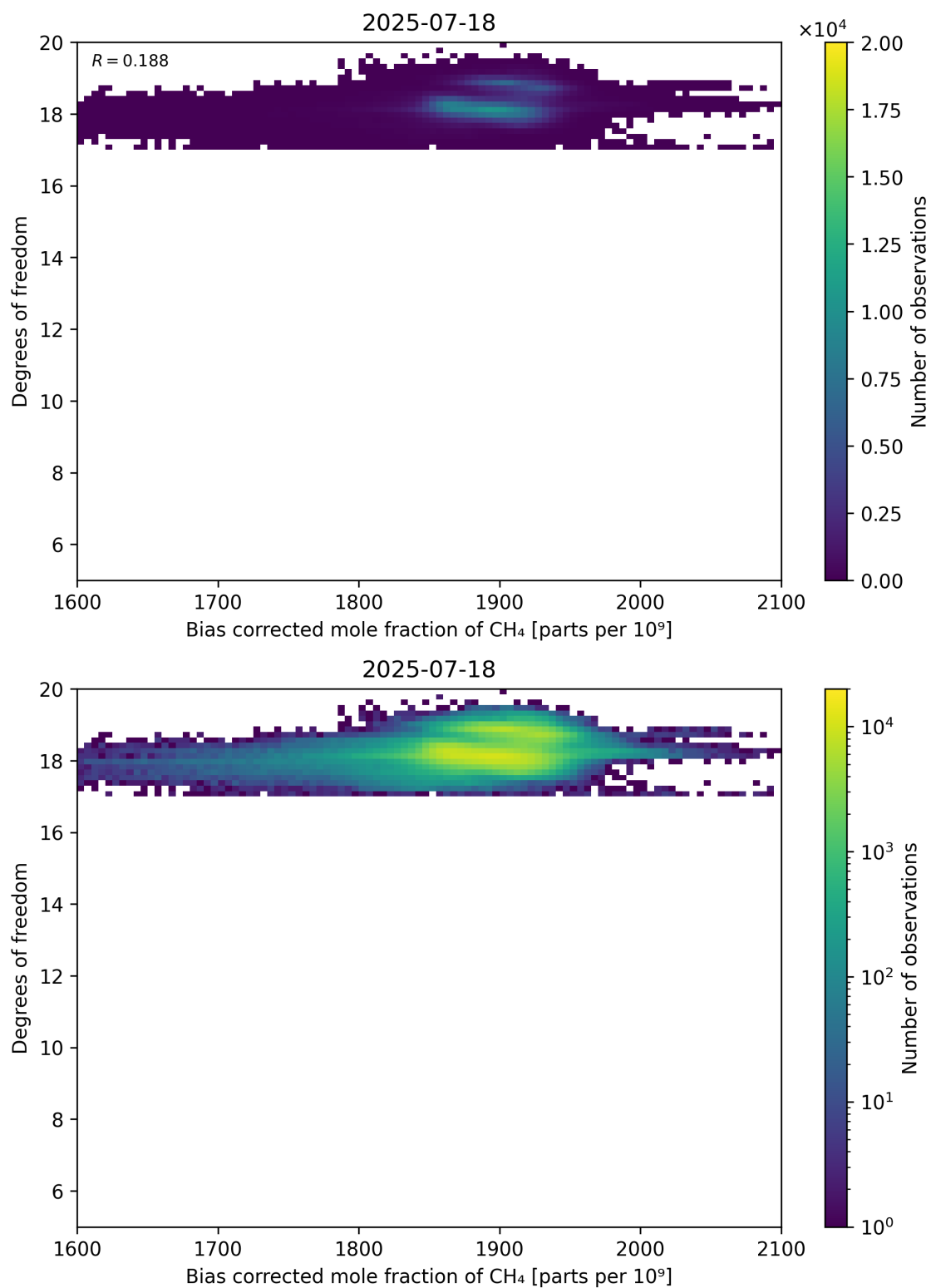
Figure 65: Scatter density plot of “Bias corrected mole fraction of CH 4 ” against “Degrees of freedom” for 2025-07-18 to 2025-07-19.
