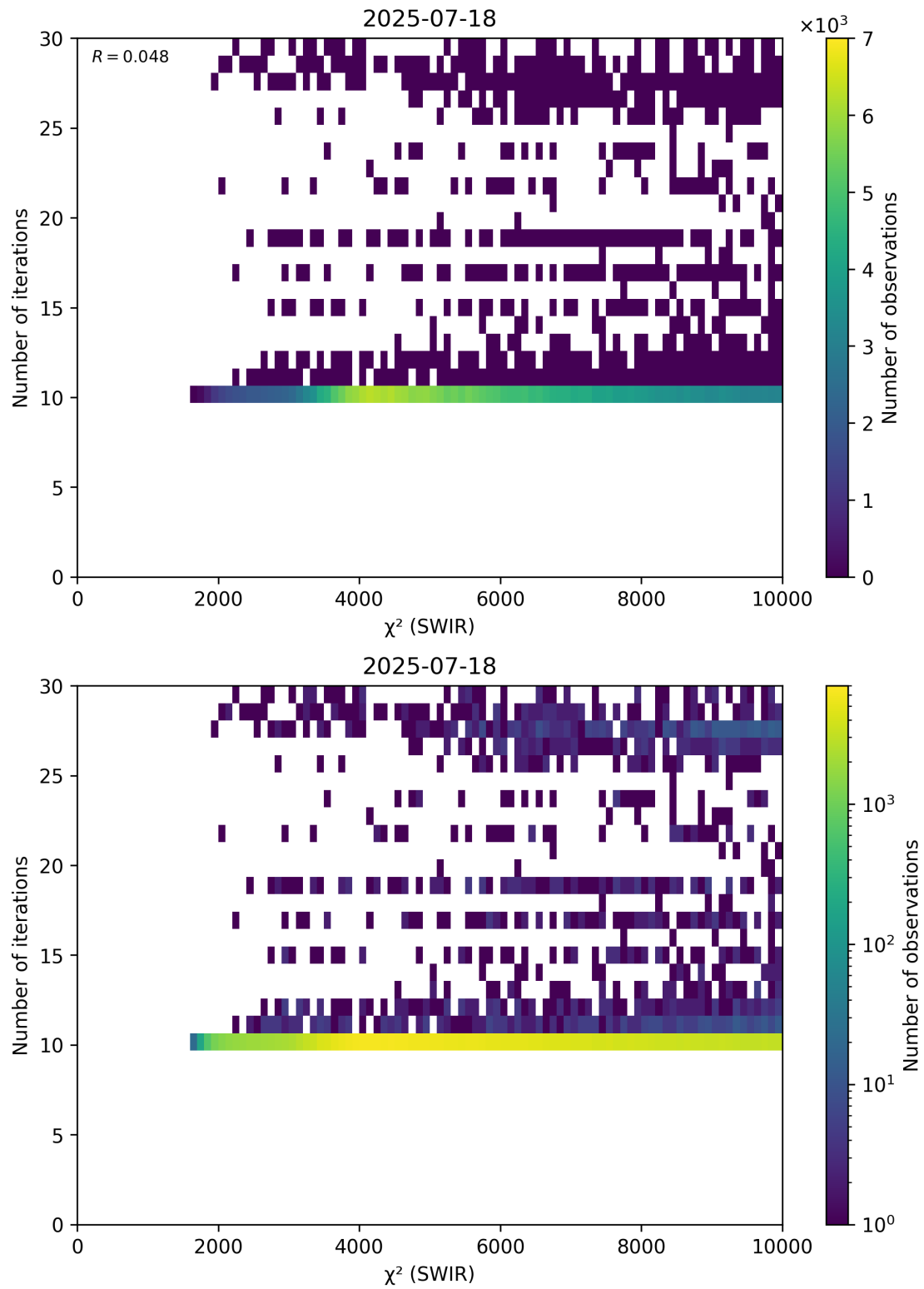
Figure 50: Scatter density plot of “ \chi^2 (SWIR)” against “Number of iterations” for 2025-07-18 to 2025-07-19.
