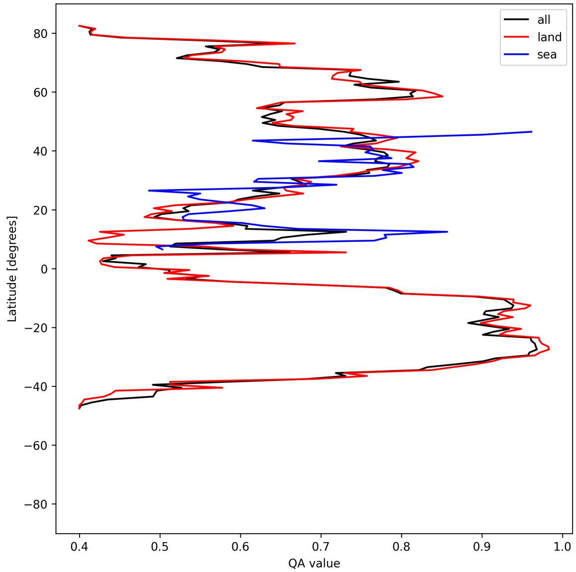
Figure 11: Zonal average of “QA value” for 2025-07-18 to 2025-07-19.
