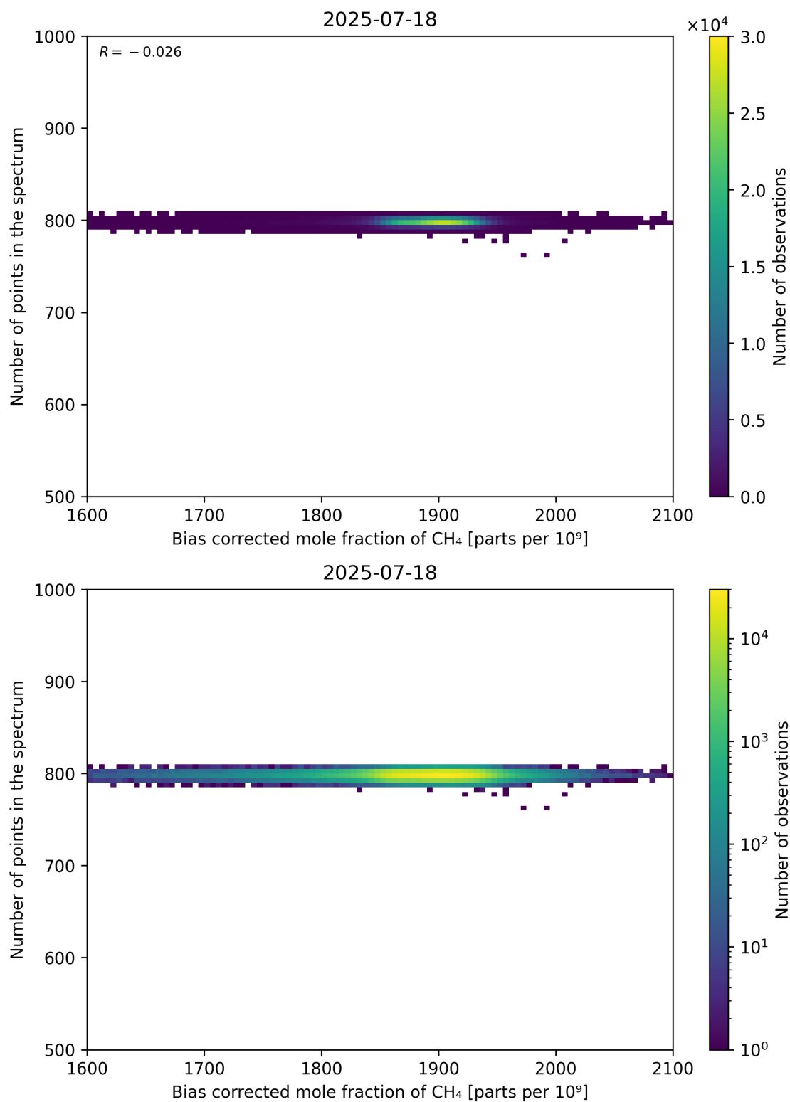
Figure 68: Scatter density plot of “Bias corrected mole fraction of CH 4 ” against “Number of points in the spectrum” for 2025-07-18 to 2025-07-19.
