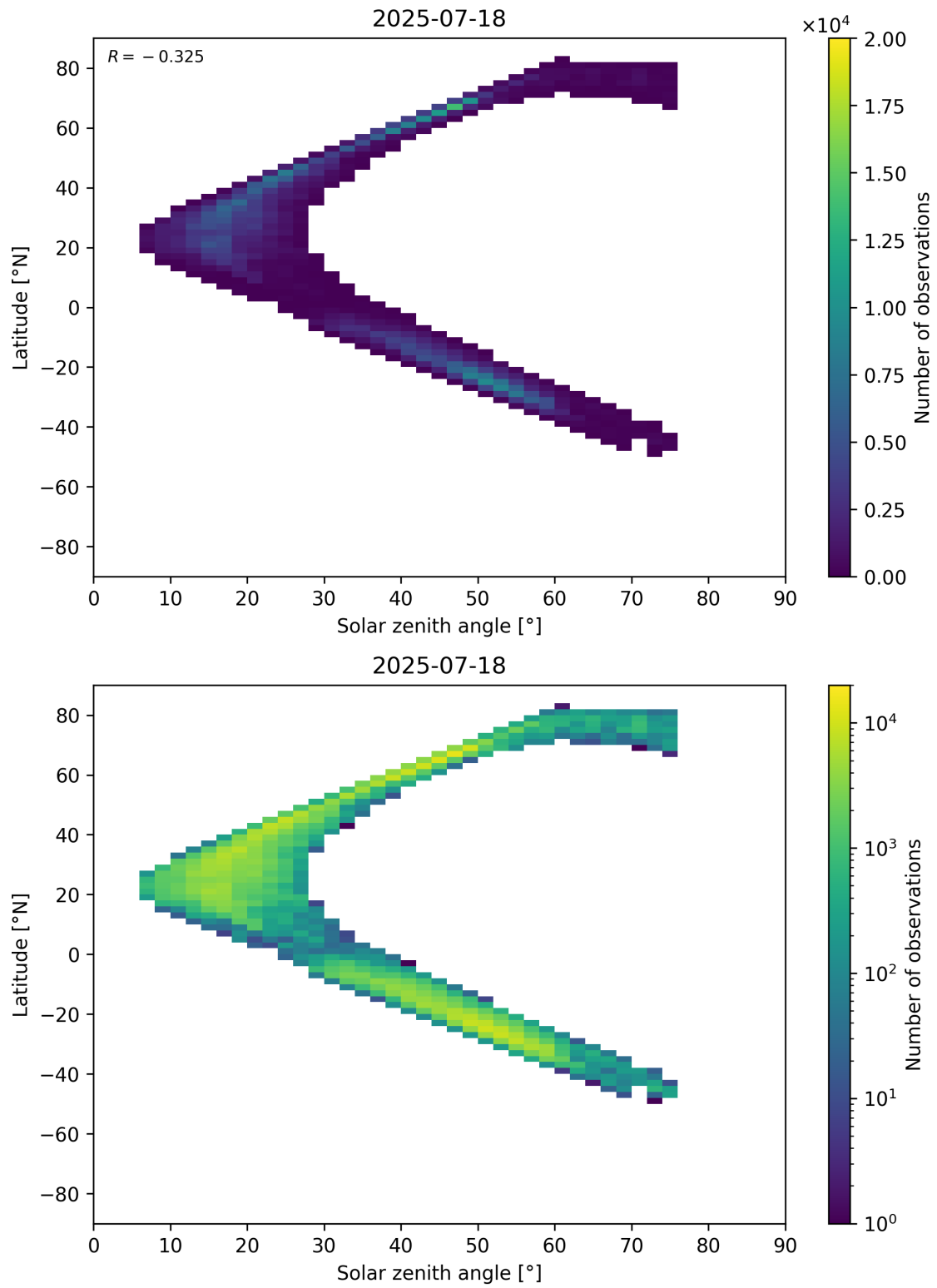
Figure 98: Scatter density plot of “Solar zenith angle” against “Latitude” for 2025-07-18 to 2025-07-19.
