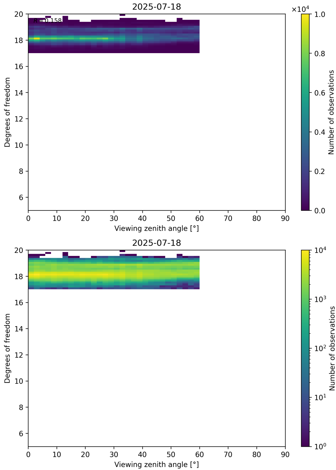
Figure 107: Scatter density plot of “Viewing zenith angle” against “Degrees of freedom” for 2025-07-18 to 2025-07-19.
