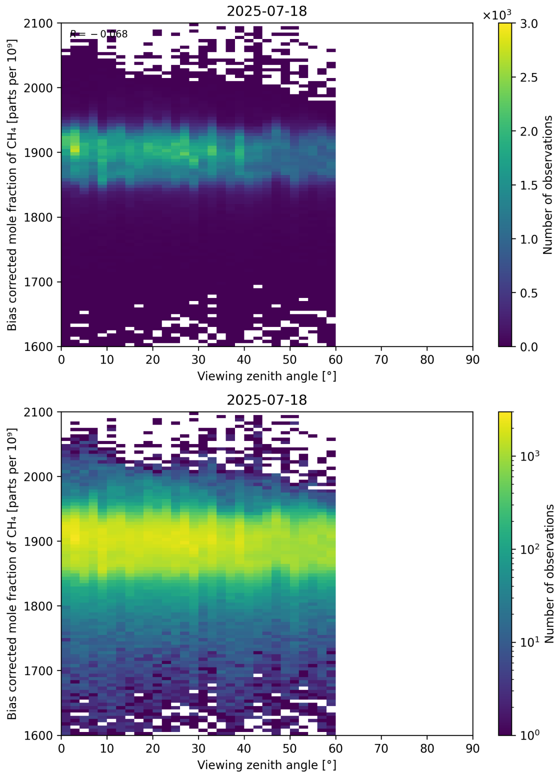
Figure 111: Scatter density plot of “Viewing zenith angle” against “Bias corrected mole fraction of CH 4 ” for 2025-07-18 to 2025-07-19.
