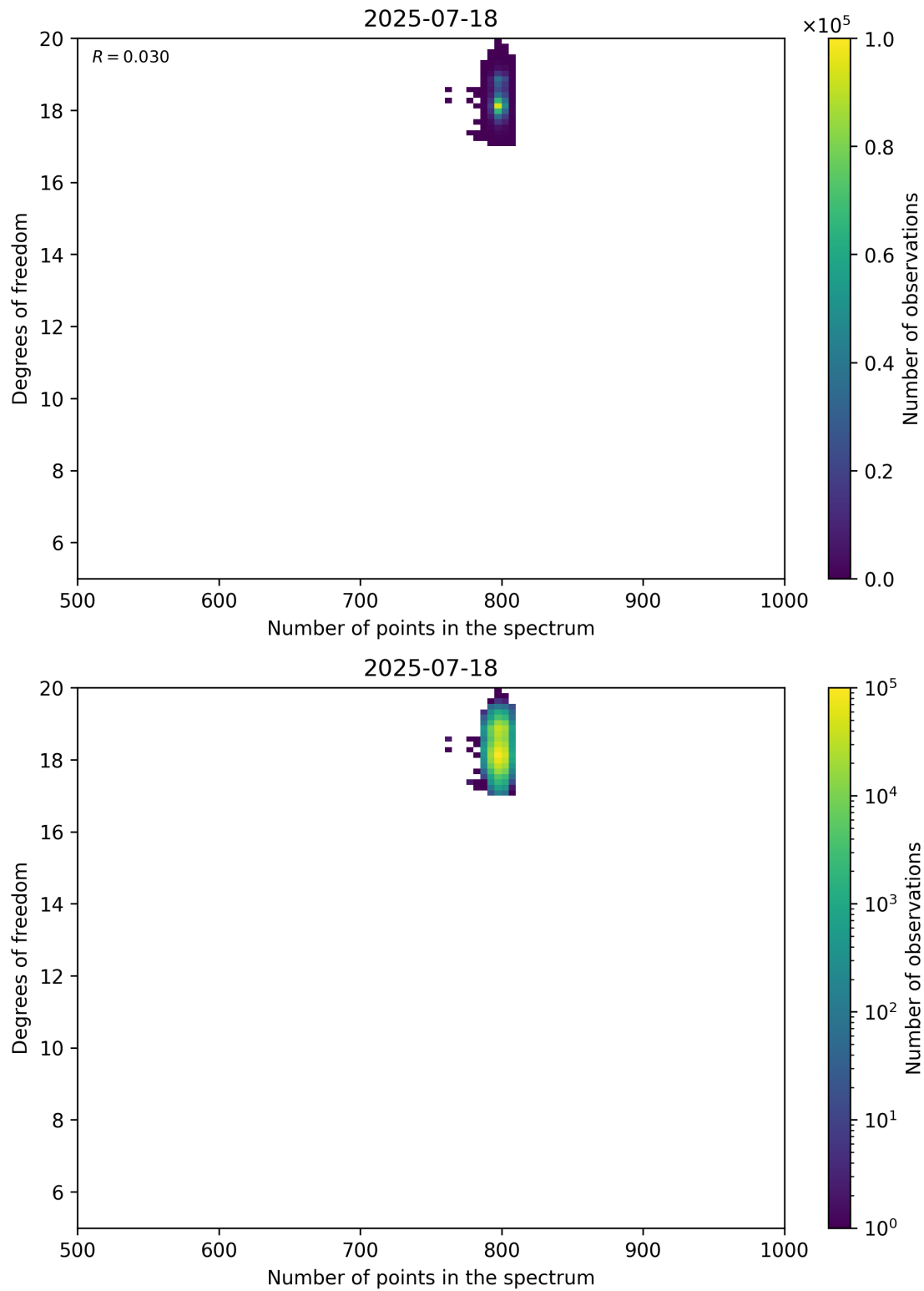
Figure 90: Scatter density plot of “Number of points in the spectrum” against “Degrees of freedom” for 2025-07-18 to 2025-07-19.
