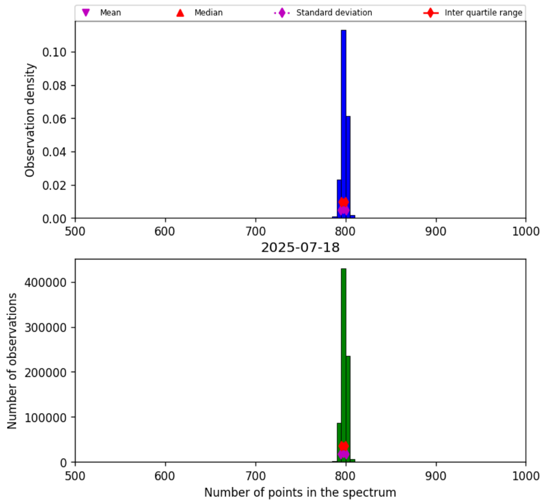
Figure 26: Histogram of “Number of points in the spectrum” for 2025-07-18 to 2025-07-19
