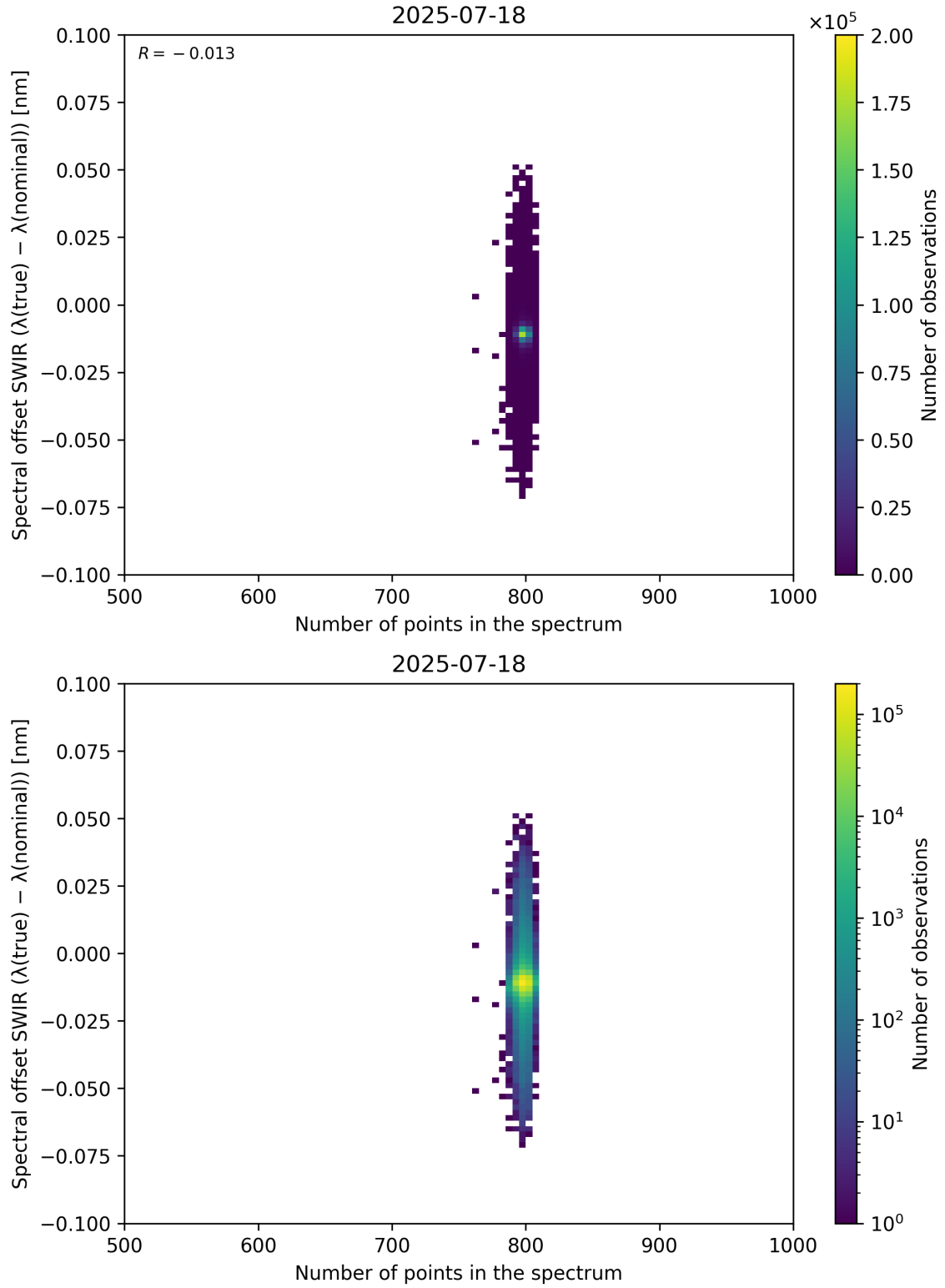
Figure 93: Scatter density plot of “Number of points in the spectrum” against “Spectral offset SWIR ( \lambda_{\text{true}} - \lambda_{\text{nominal}} )” for 2025-07-18 to 2025-07-19.
