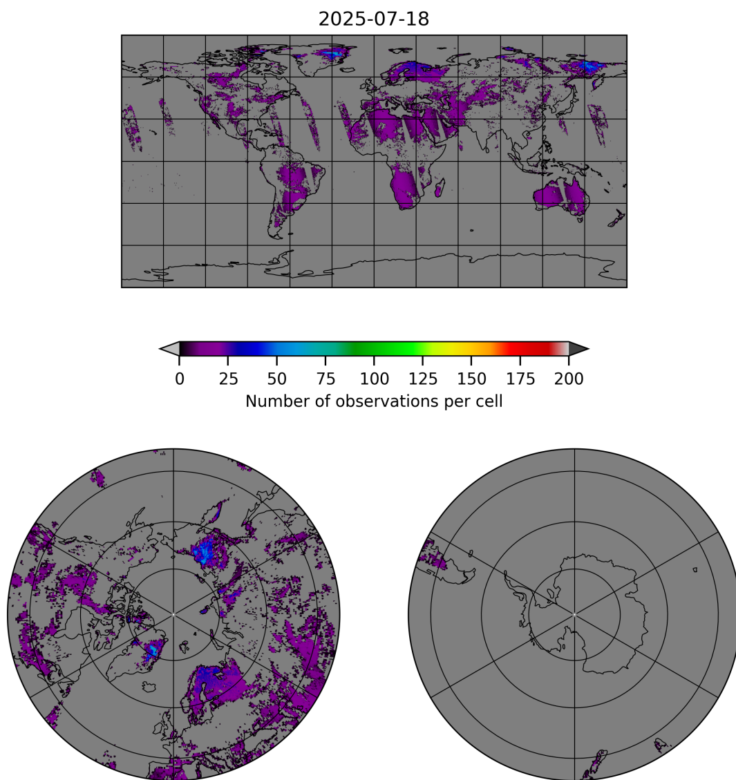
Figure 10: Map of the number of observations for 2025-07-18 to 2025-07-19
