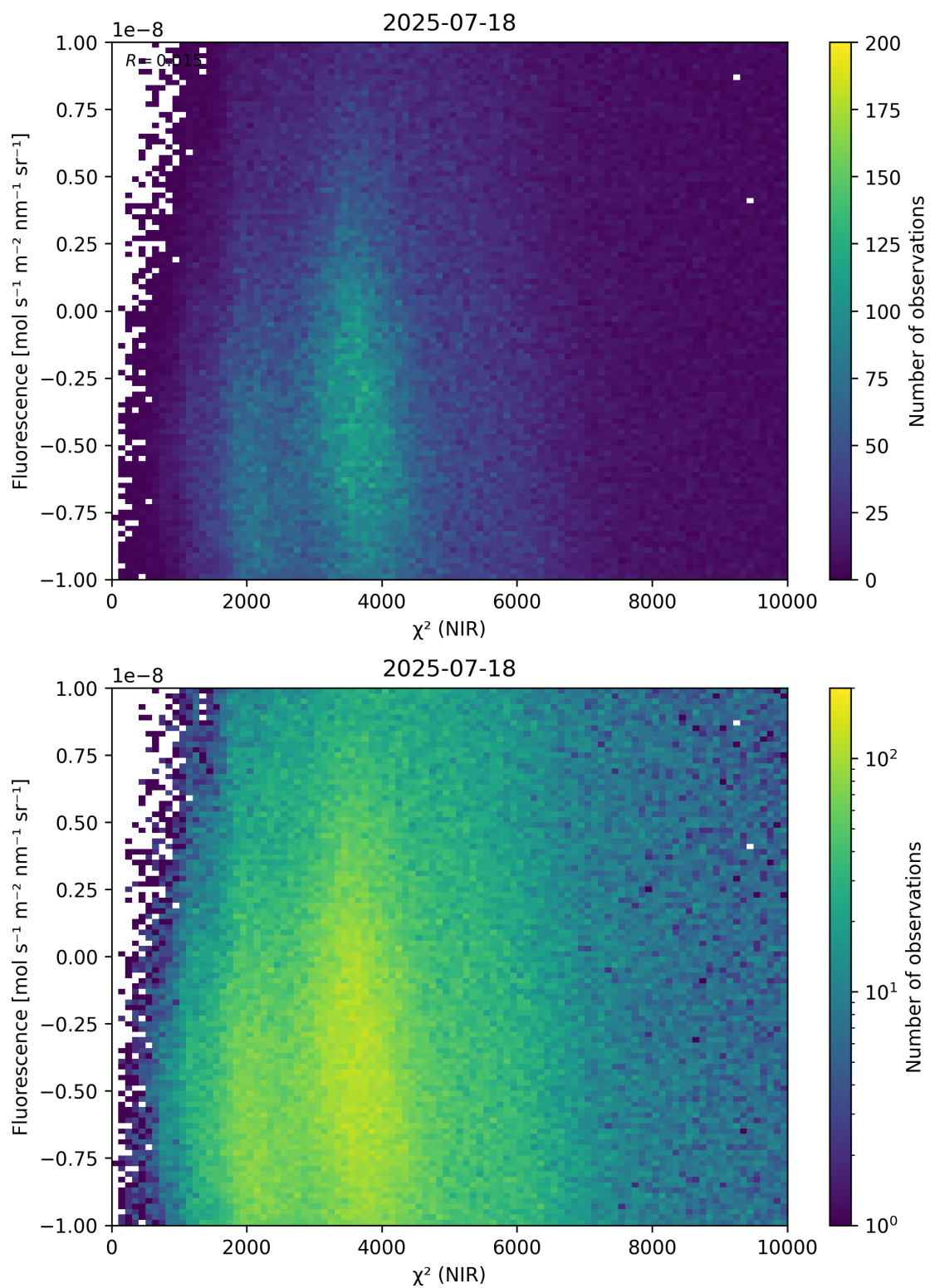
Figure 45: Scatter density plot of “ \chi^2 (NIR)” against “Fluorescence” for 2025-07-18 to 2025-07-19.
