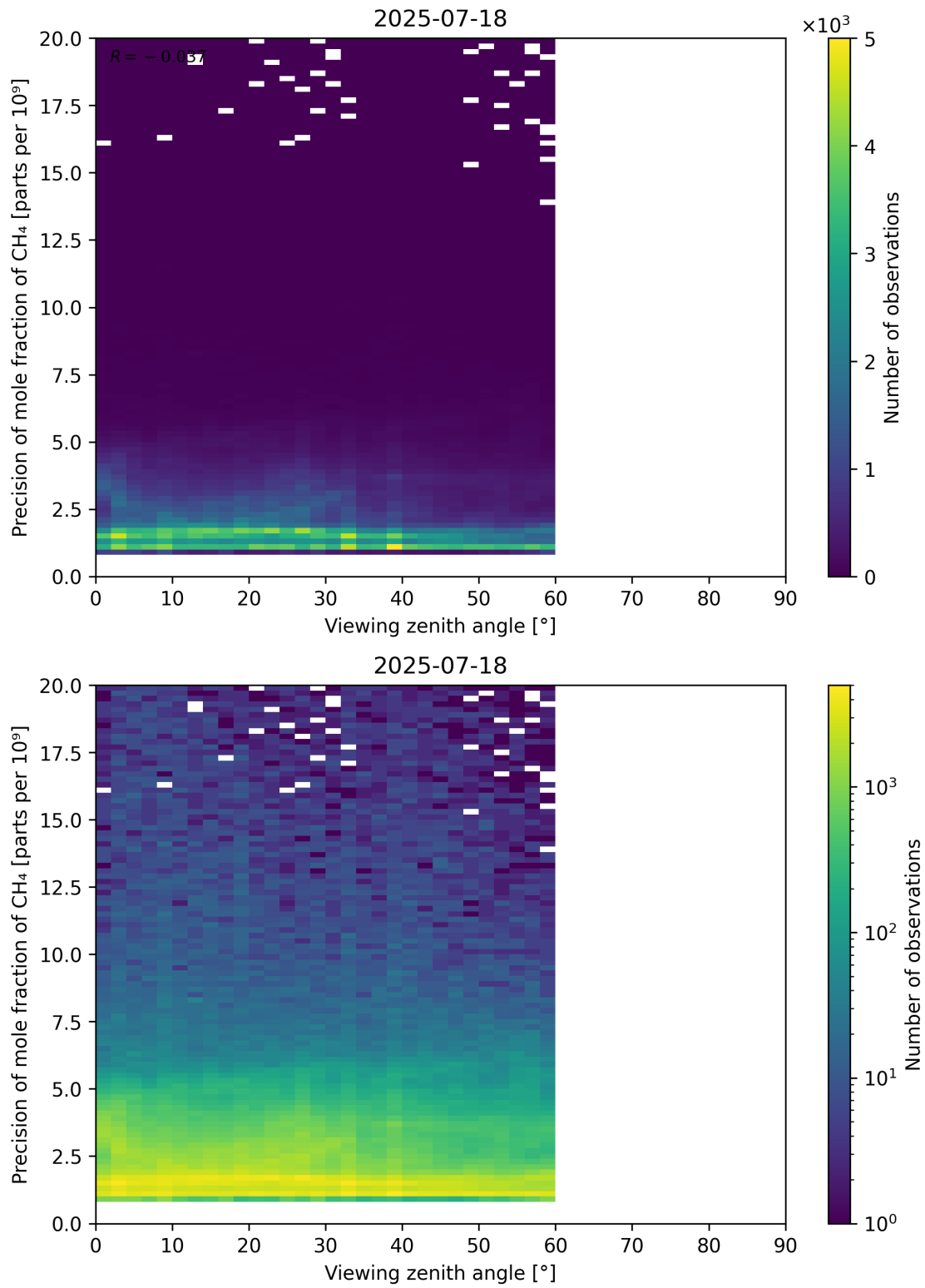
Figure 112: Scatter density plot of “Viewing zenith angle” against “Precision of mole fraction of CH 4 ” for 2025-07-18 to 2025-07-19.
