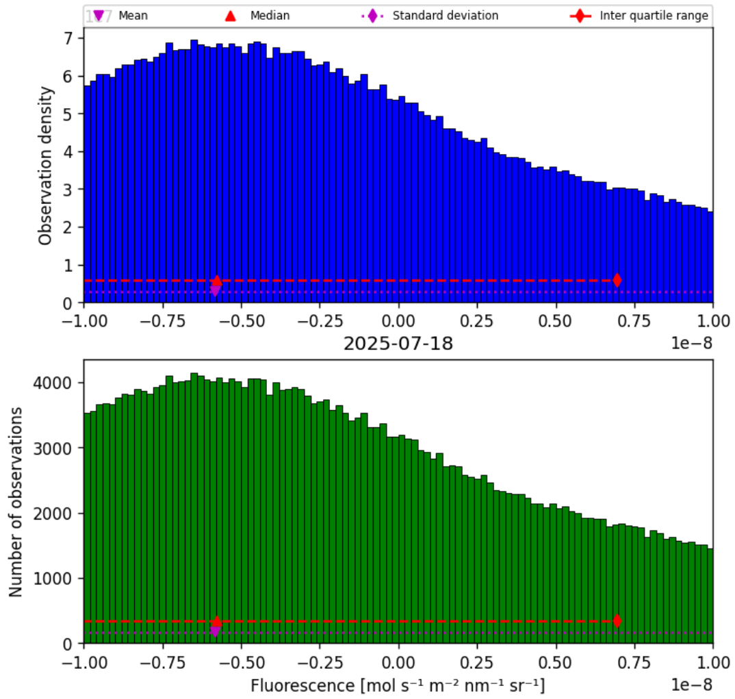
Figure 32: Histogram of “Fluorescence” for 2025-07-18 to 2025-07-19
