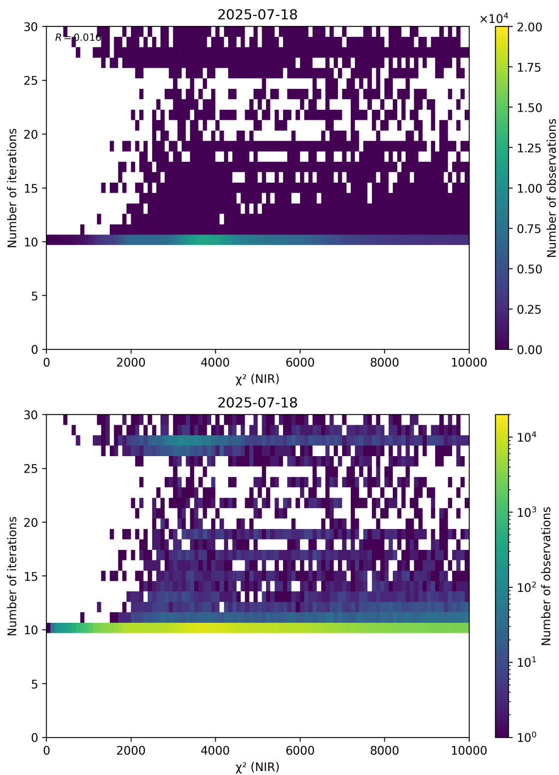
Figure 46: Scatter density plot of “ \chi^2 (NIR)” against “Number of iterations” for 2025-07-18 to 2025-07-19.
