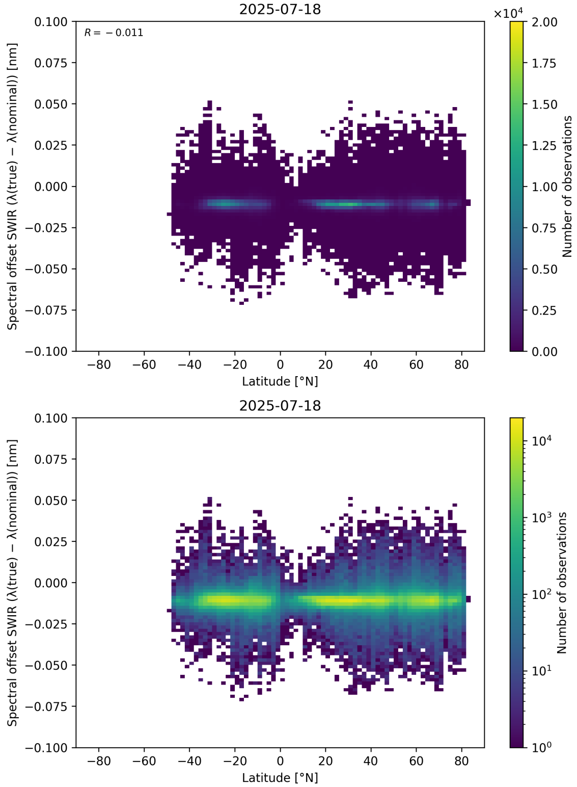
Figure 62: Scatter density plot of “Latitude” against “Spectral offset SWIR ( \lambda_{\text{true}} - \lambda_{\text{nominal}} )” for 2025-07-18 to 2025-07-19.
