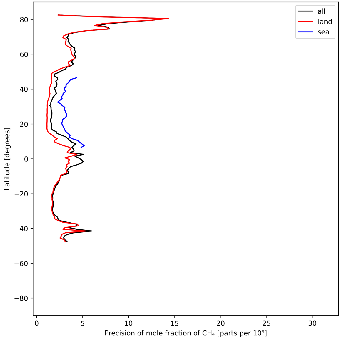
Figure 13: Zonal average of “Precision of mole fraction of CH 4 ” for 2025-07-18 to 2025-07-19.
