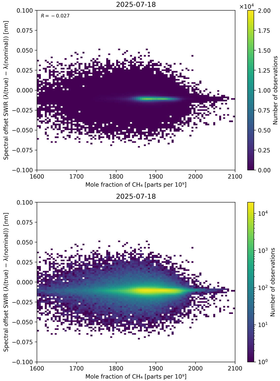
Figure 86: Scatter density plot of “Mole fraction of CH 4 ” against “Spectral offset SWIR ( \lambda_{\text{true}} - \lambda_{\text{nominal}} )” for 2025-07-18 to 2025-07-19.
