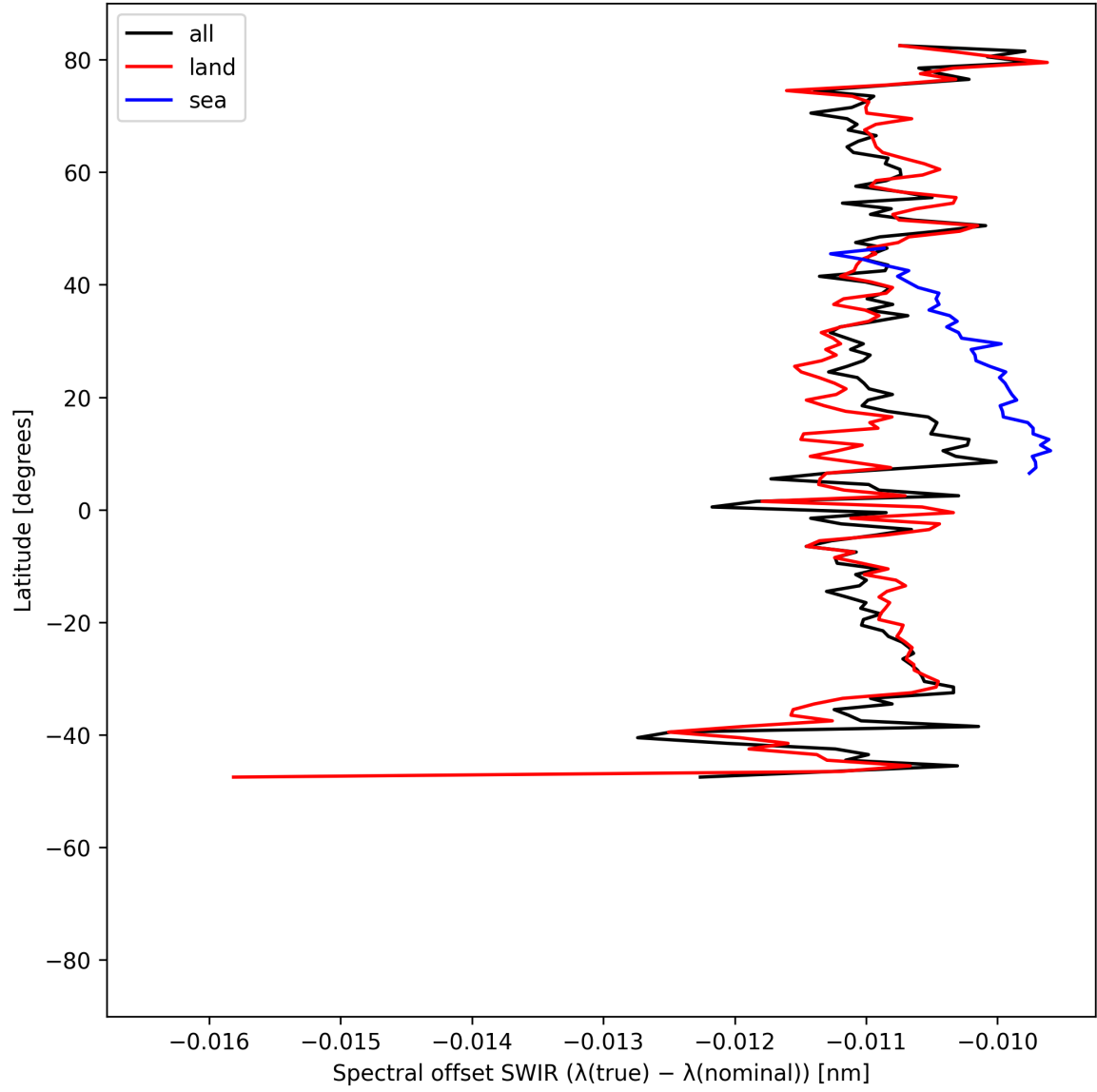
Figure 16: Zonal average of “Spectral offset SWIR ( \lambda_{\text{true}} - \lambda_{\text{nominal}} )” for 2025-07-18 to 2025-07-19.
