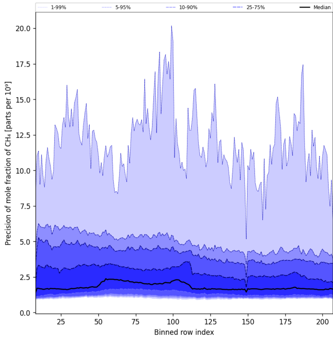
Figure 35: Along track statistics of “Precision of mole fraction of CH 4 ” for 2025-07-18 to 2025-07-19
