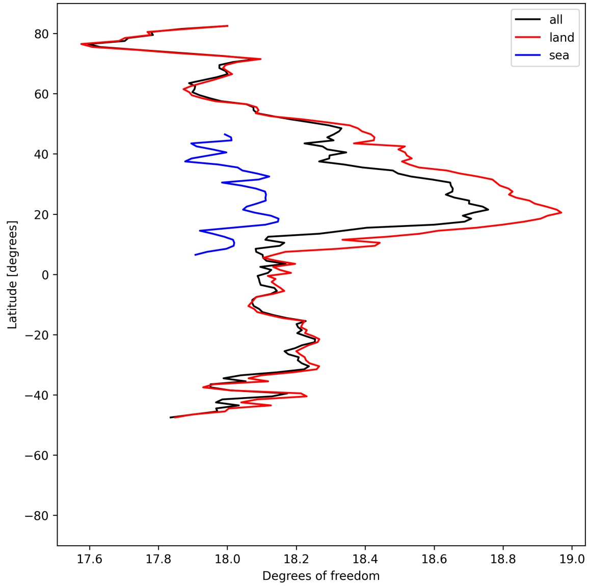
Figure 19: Zonal average of “Degrees of freedom” for 2025-07-18 to 2025-07-19.
