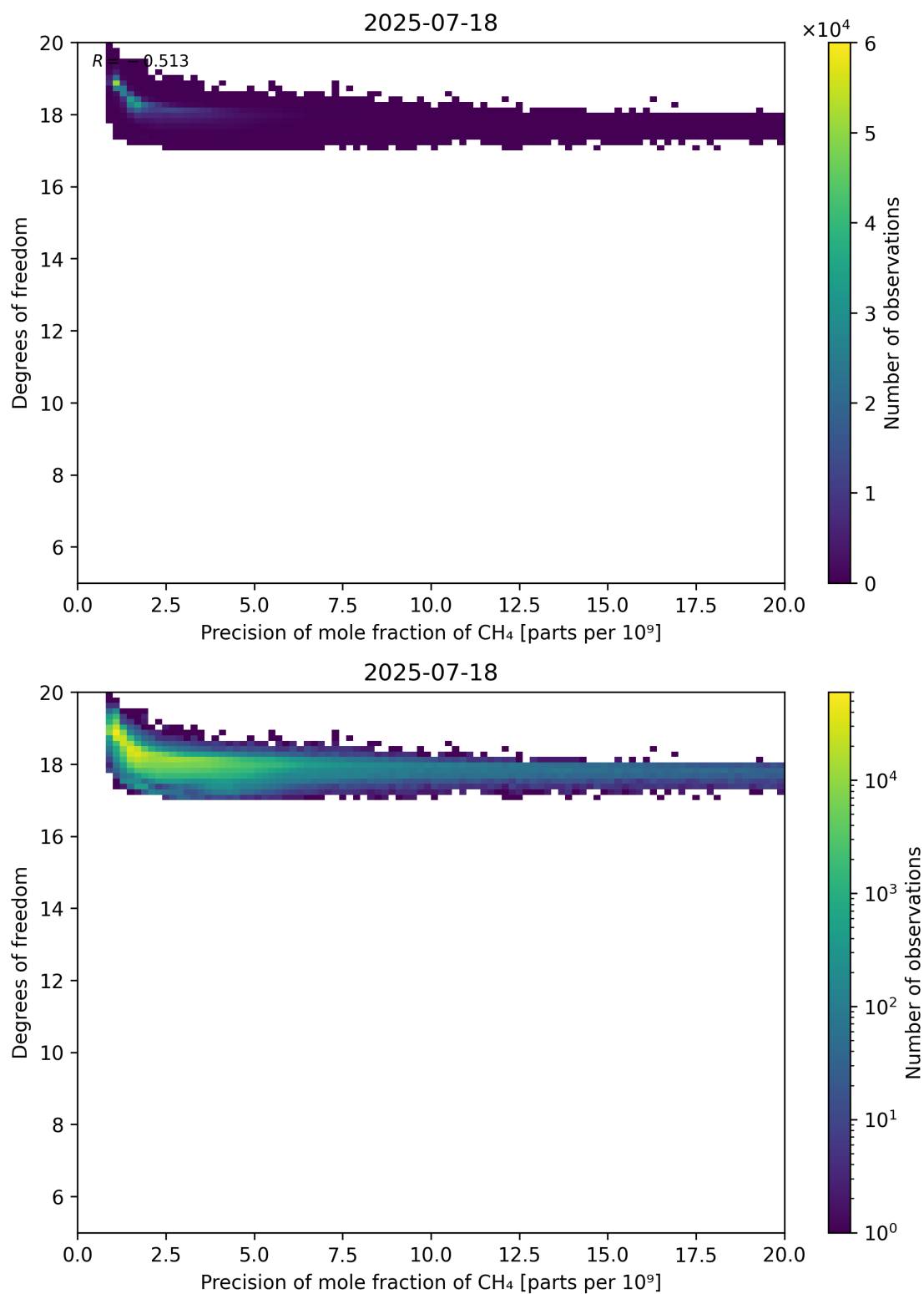
Figure 80: Scatter density plot of “Precision of mole fraction of CH 4 ” against “Degrees of freedom” for 2025-07-18 to 2025-07-19.
