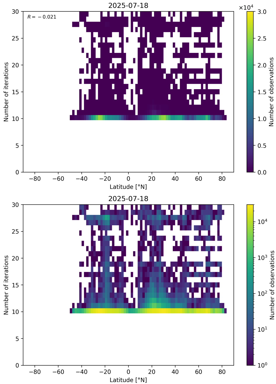
Figure 60: Scatter density plot of “Latitude” against “Number of iterations” for 2025-07-18 to 2025-07-19.
