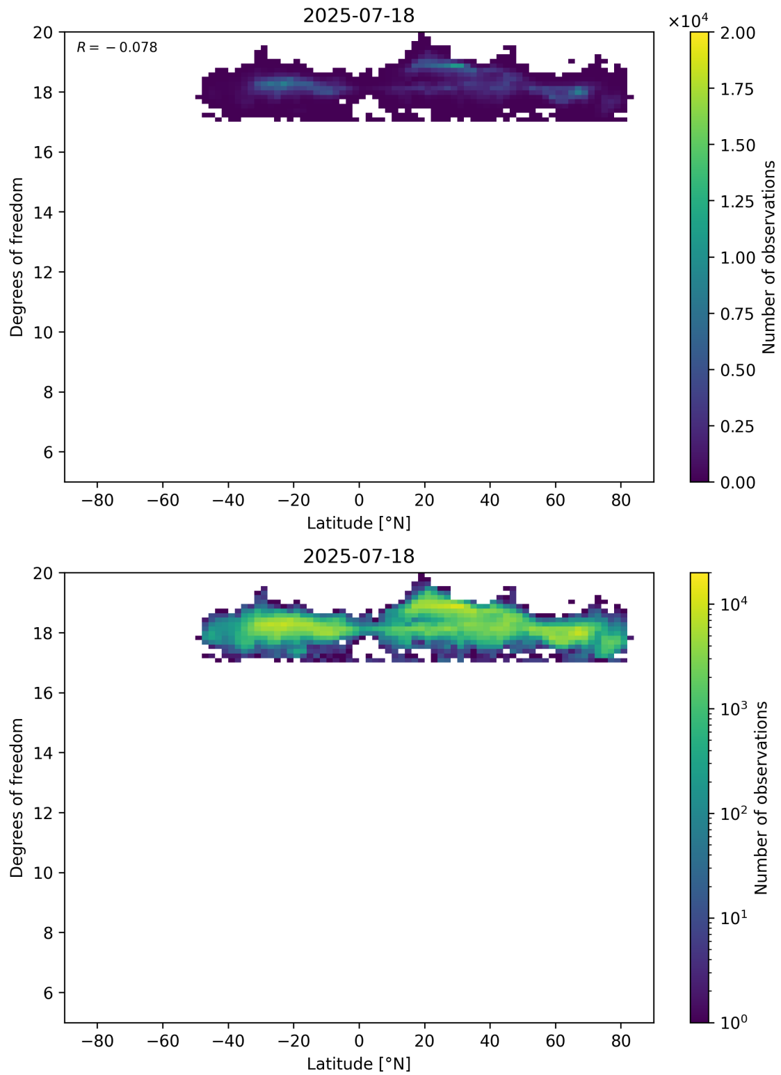
Figure 55: Scatter density plot of “Latitude” against “Degrees of freedom” for 2025-07-18 to 2025-07-19.
