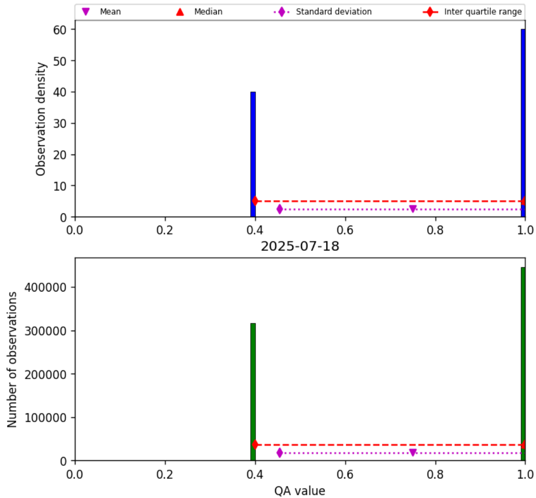
Figure 22: Histogram of “QA value” for 2025-07-18 to 2025-07-19
