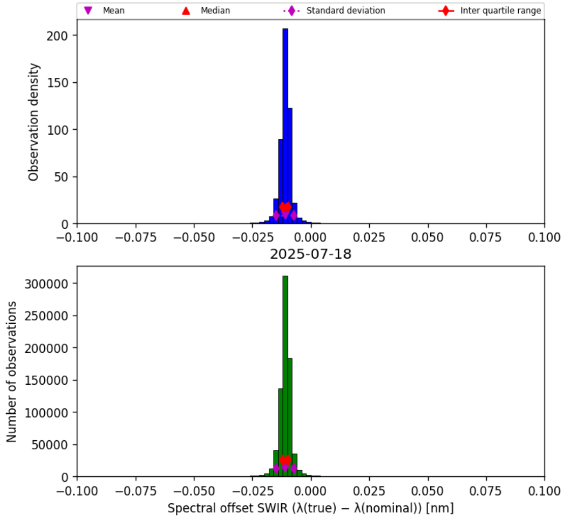
Figure 27: Histogram of “Spectral offset SWIR ( \lambda_{\text{true}} - \lambda_{\text{nominal}} )” for 2025-07-18 to 2025-07-19
