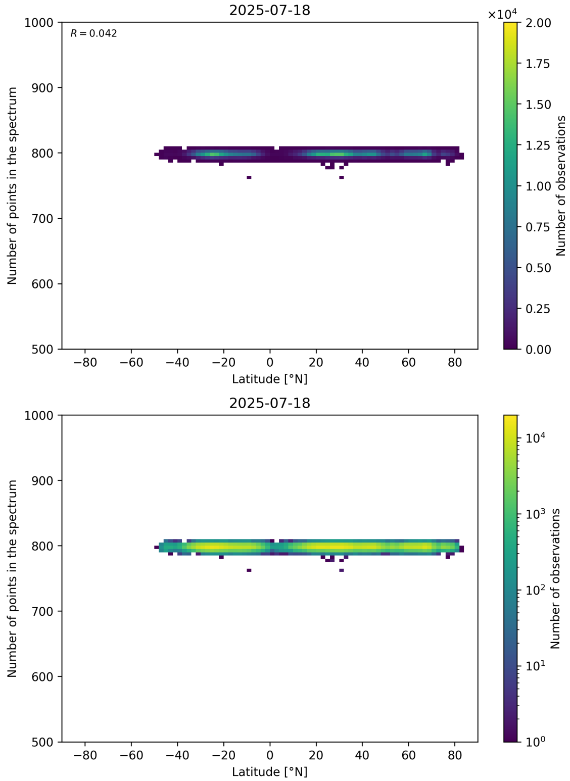
Figure 61: Scatter density plot of “Latitude” against “Number of points in the spectrum” for 2025-07-18 to 2025-07-19.
