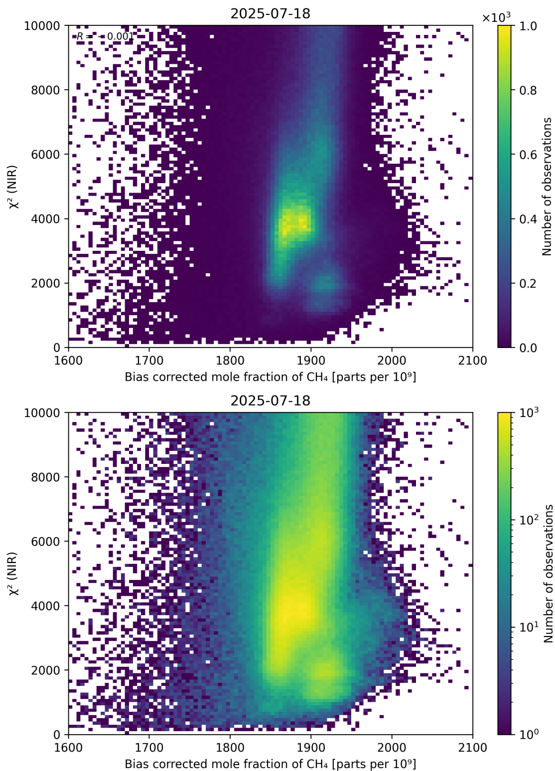
Figure 63: Scatter density plot of “Bias corrected mole fraction of CH 4 ” against “ \chi^2 (NIR)” for 2025-07-18 to 2025-07-19.
