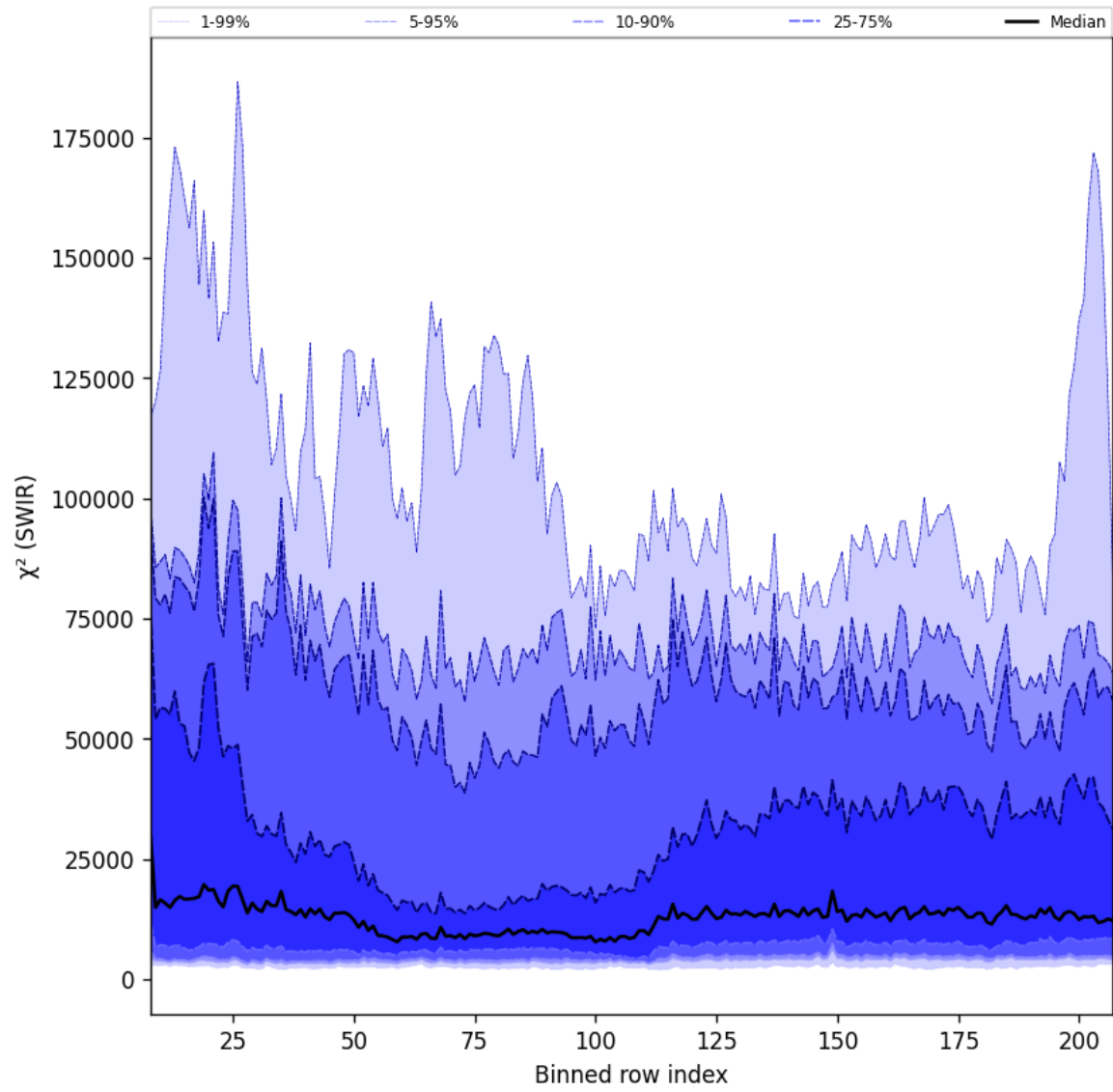
Figure 39: Along track statistics of " \chi^2 (SWIR)" for 2025-07-18 to 2025-07-19
