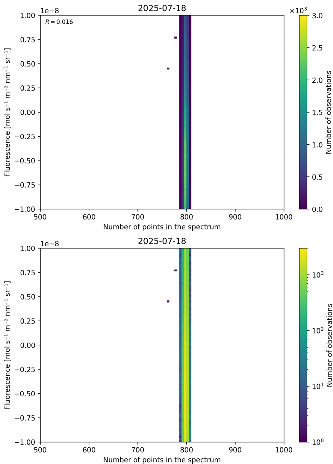
Figure 91: Scatter density plot of “Number of points in the spectrum” against “Fluorescence” for 2025-07-18 to 2025-07-19.
