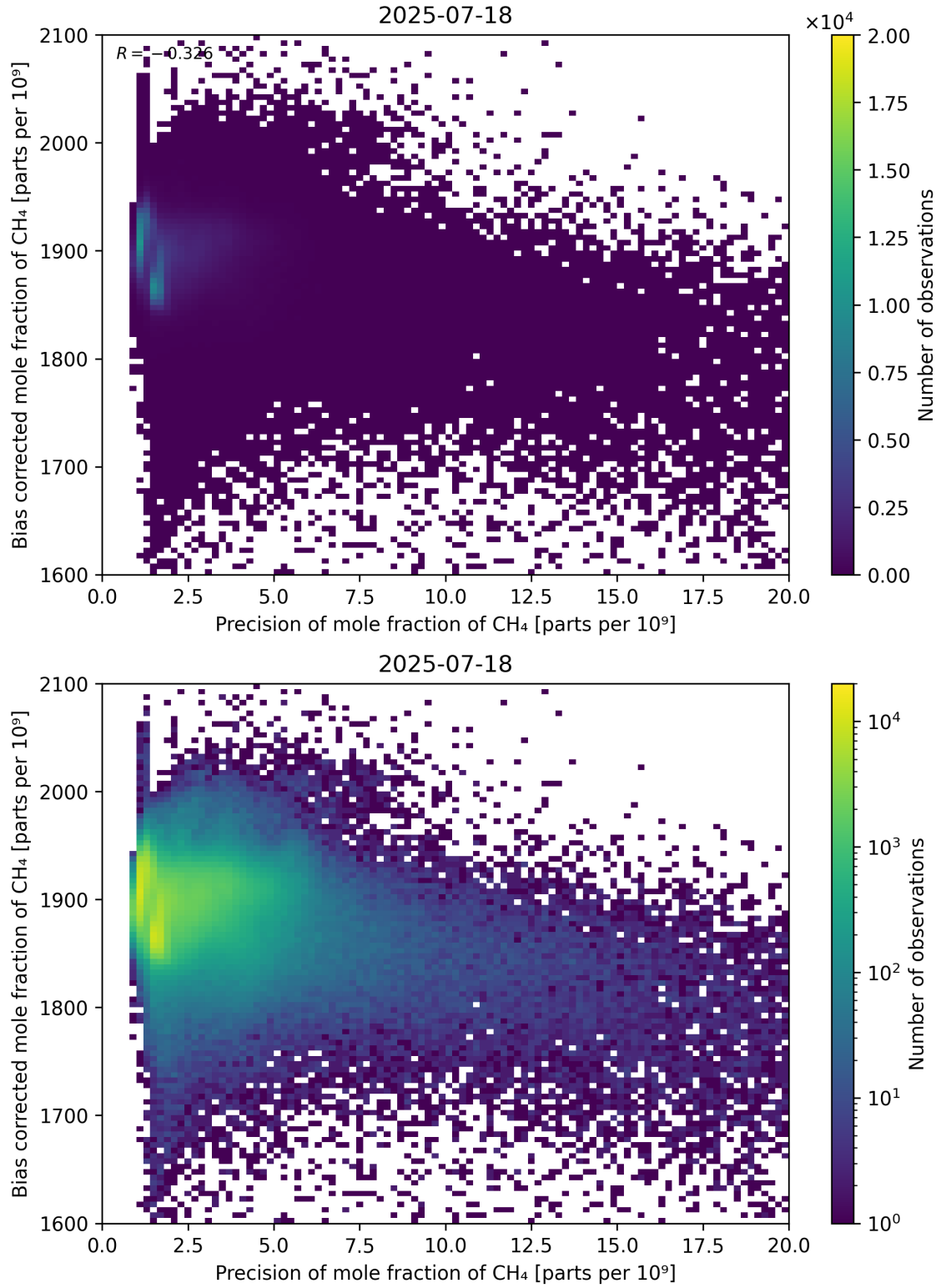
Figure 82: Scatter density plot of “Precision of mole fraction of CH 4 ” against “Bias corrected mole fraction of CH 4 ” for 2025-07-18 to 2025-07-19.
