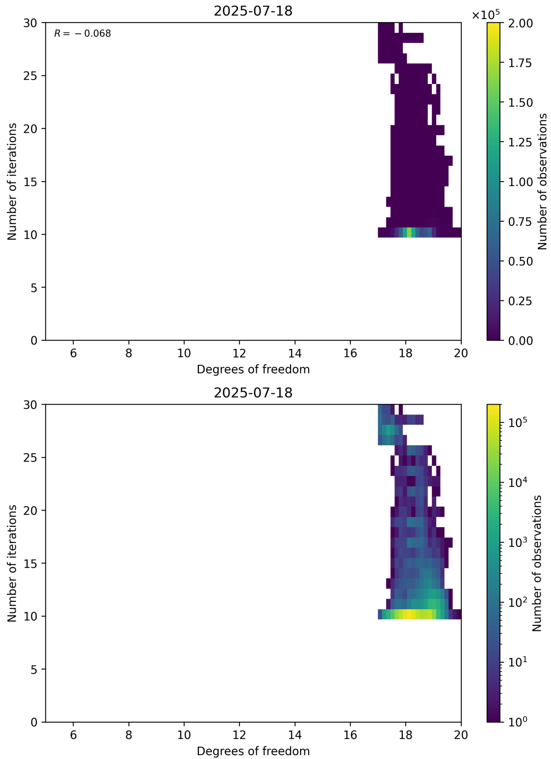
Figure 52: Scatter density plot of “Degrees of freedom” against “Number of iterations” for 2025-07-18 to 2025-07-19.
