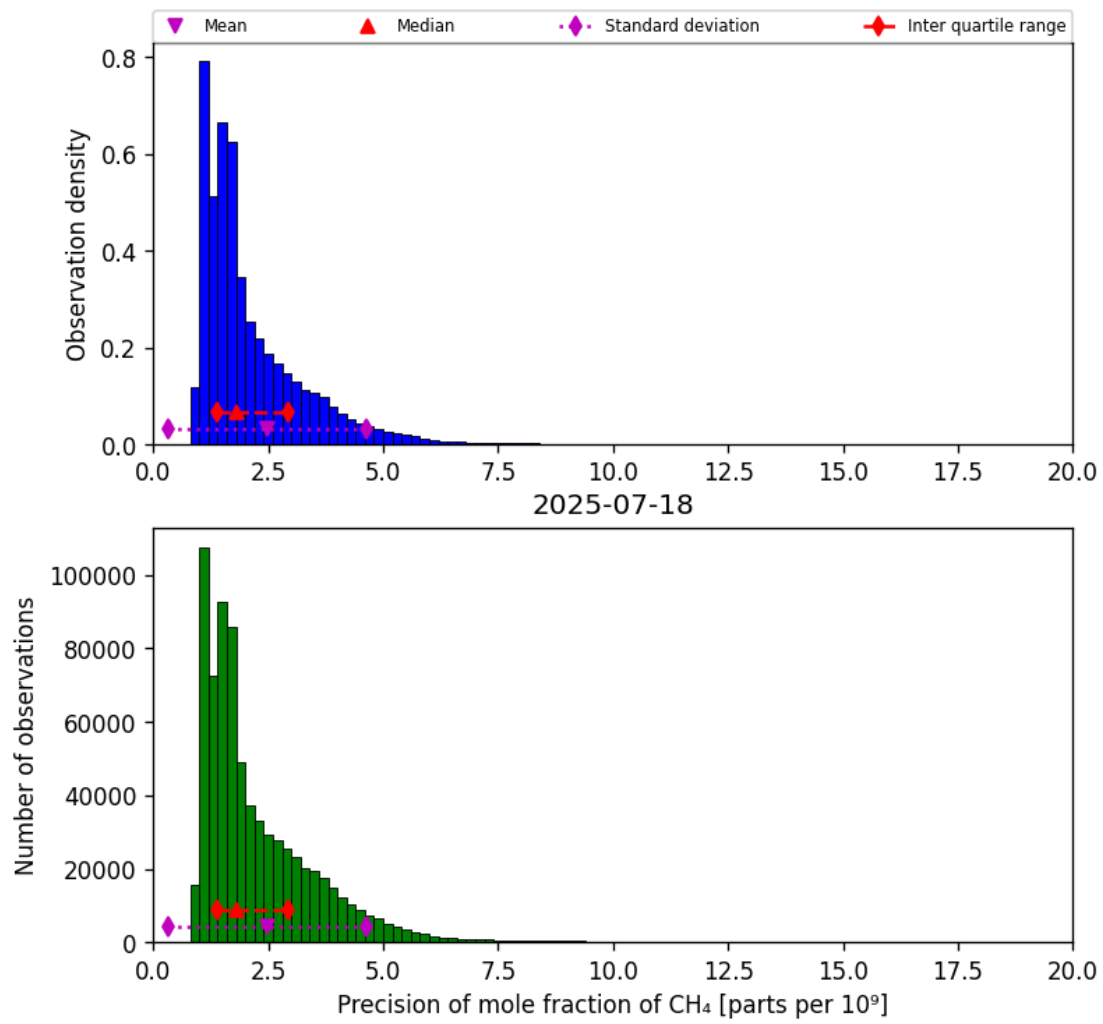
Figure 24: Histogram of “Precision of mole fraction of CH 4 ” for 2025-07-18 to 2025-07-19
