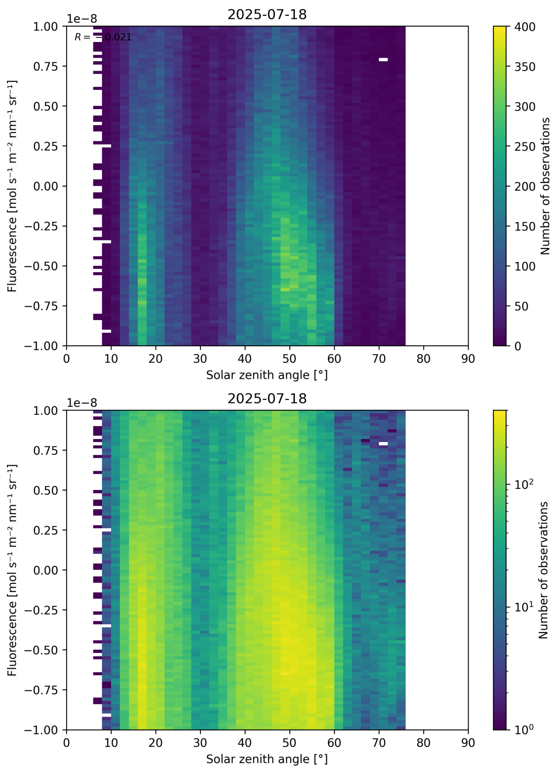
Figure 97: Scatter density plot of “Solar zenith angle” against “Fluorescence” for 2025-07-18 to 2025-07-19.
