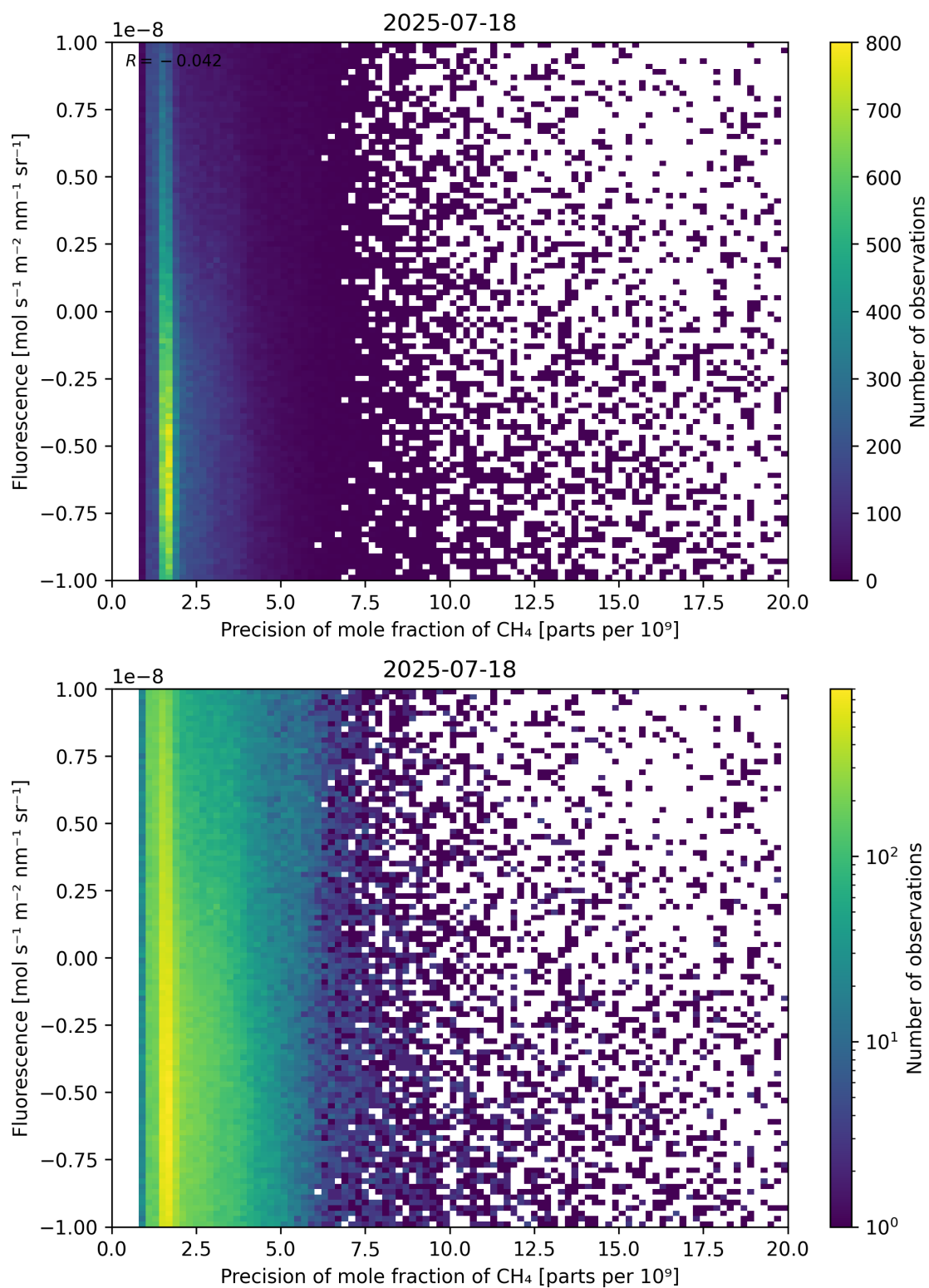
Figure 81: Scatter density plot of “Precision of mole fraction of CH 4 ” against “Fluorescence” for 2025-07-18 to 2025-07-19.
