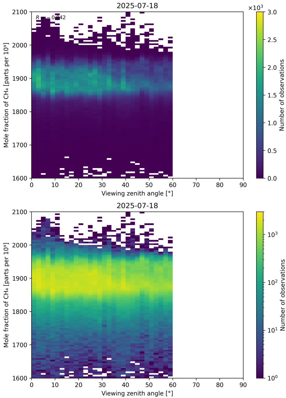
Figure 110: Scatter density plot of “Viewing zenith angle” against “Mole fraction of CH 4 ” for 2025-07-18 to 2025-07-19.
