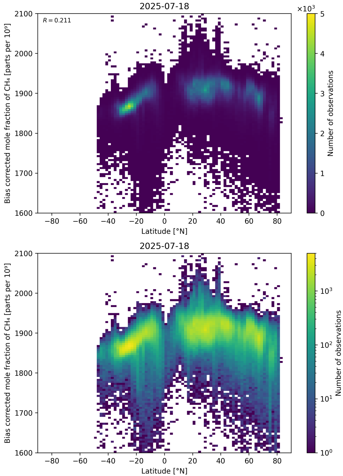
Figure 58: Scatter density plot of “Latitude” against “Bias corrected mole fraction of \text{CH}_4 ” for 2025-07-18 to 2025-07-19.
