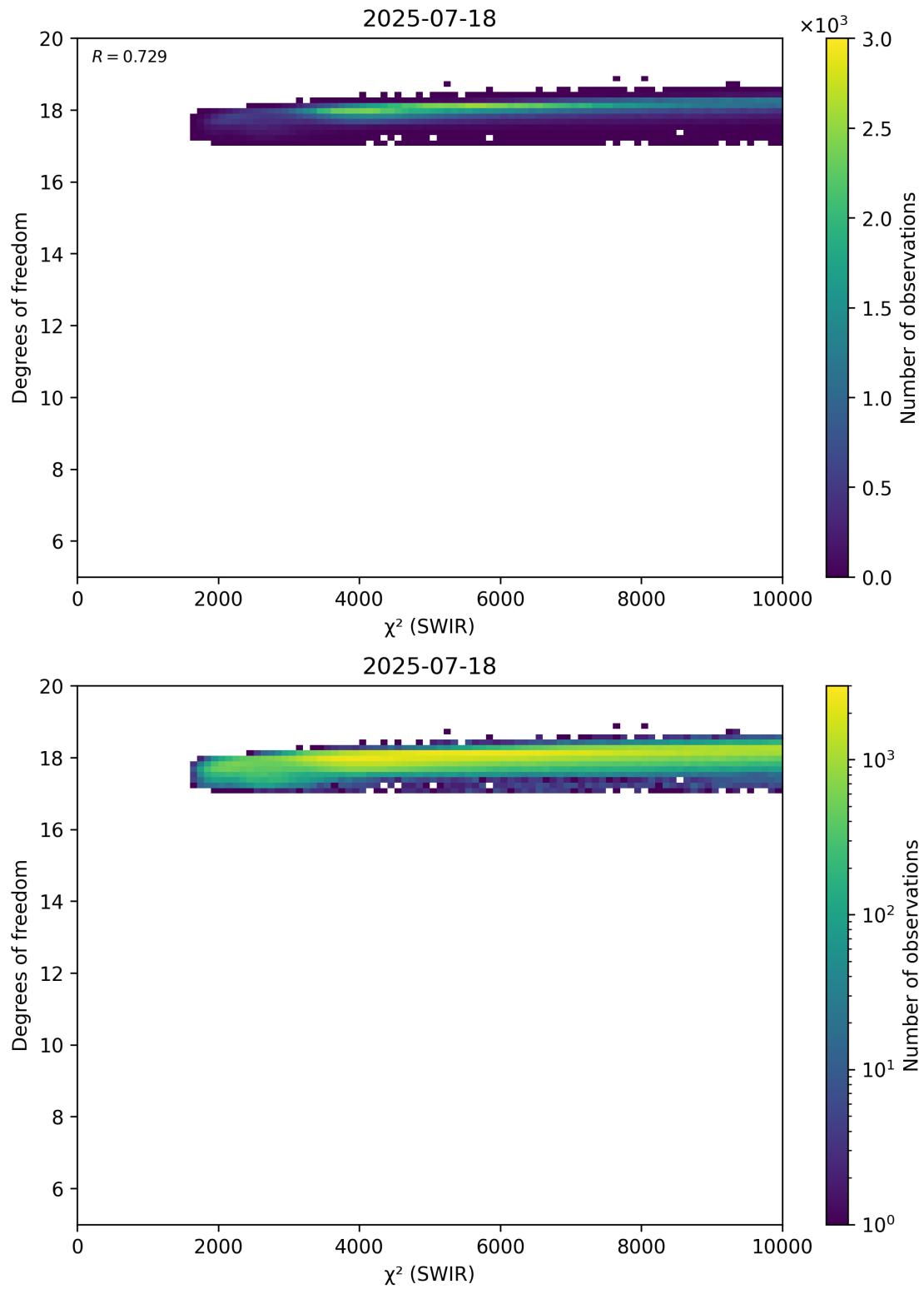
Figure 48: Scatter density plot of “ \chi^2 (SWIR)” against “Degrees of freedom” for 2025-07-18 to 2025-07-19.
