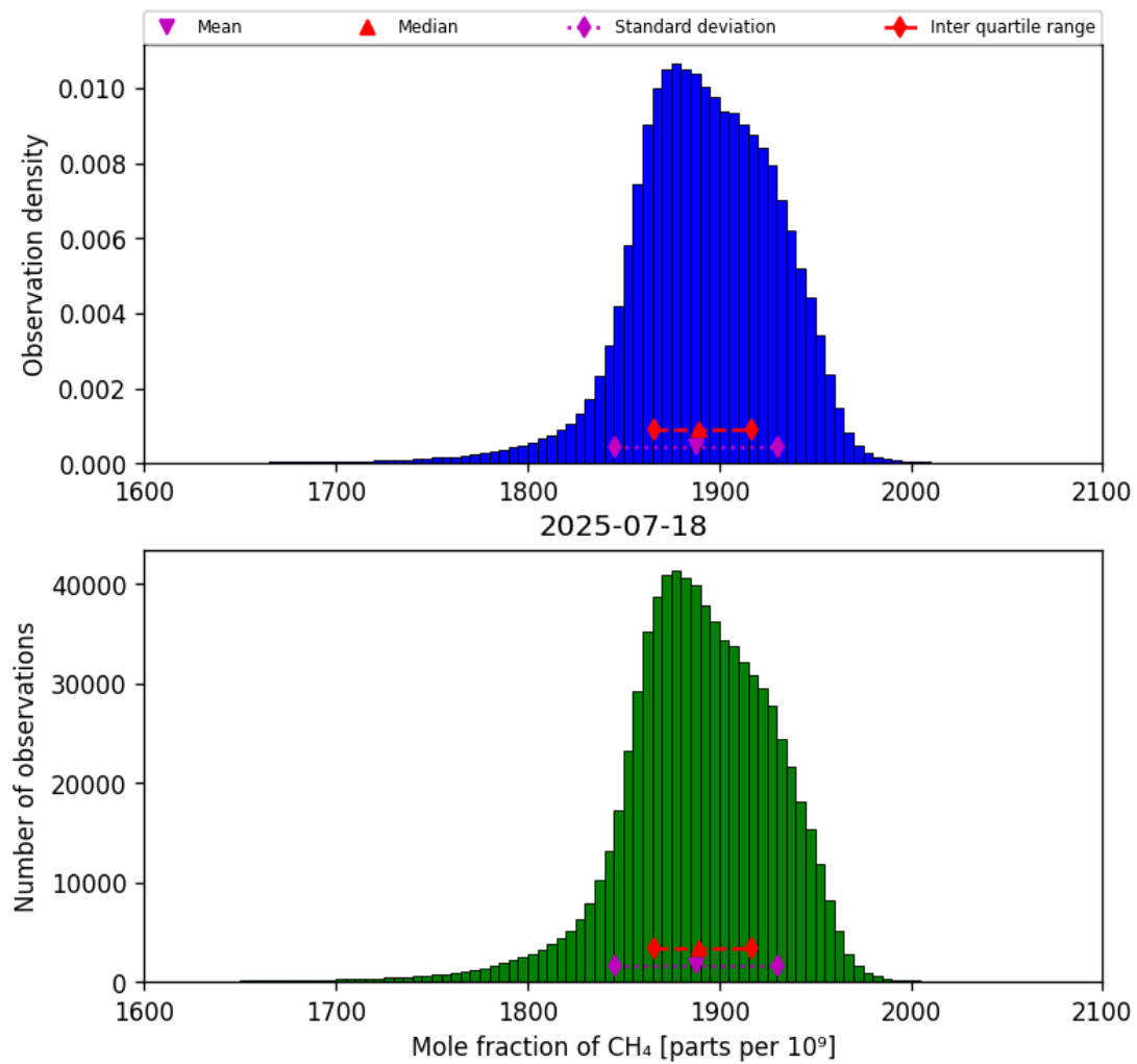
Figure 23: Histogram of “Mole fraction of CH 4 ” for 2025-07-18 to 2025-07-19
