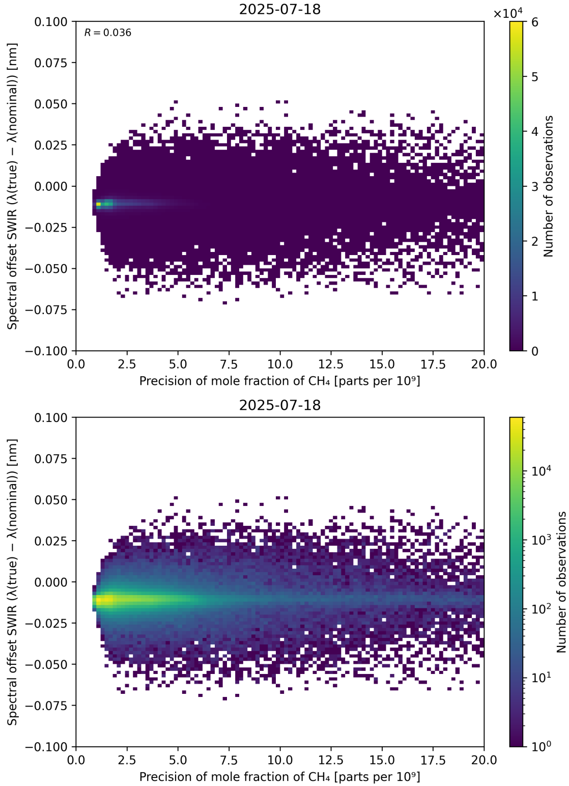
Figure 85: Scatter density plot of “Precision of mole fraction of CH 4 ” against “Spectral offset SWIR ( \lambda_{\text{true}} - \lambda_{\text{nominal}} )” for 2025-07-18 to 2025-07-19.
