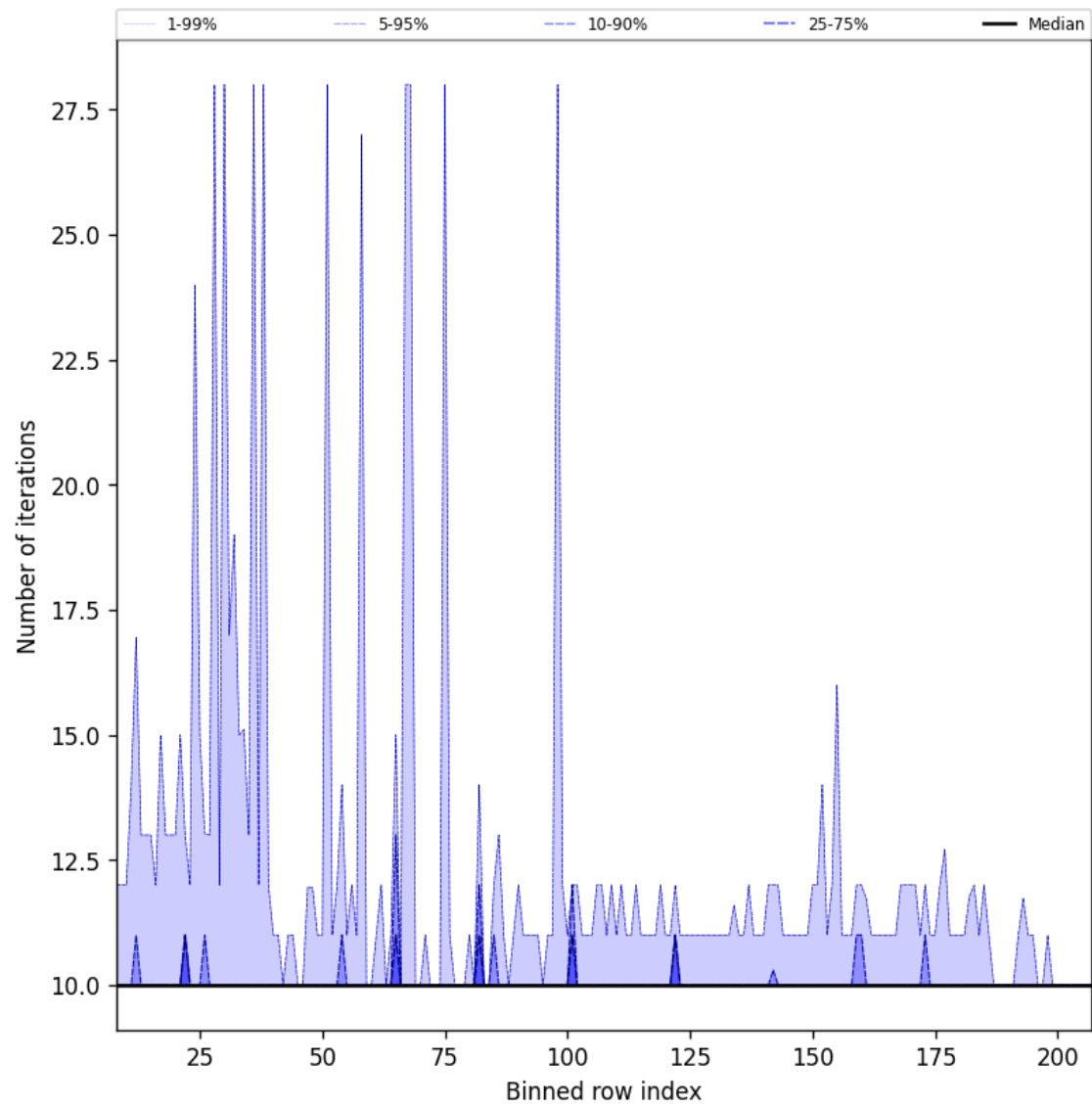
Figure 42: Along track statistics of “Number of iterations” for 2025-07-18 to 2025-07-19
