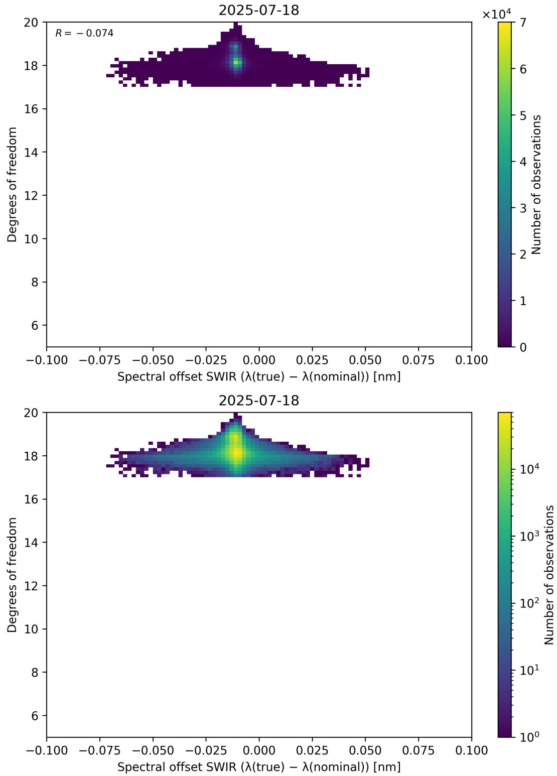
Figure 119: Scatter density plot of “Spectral offset SWIR ( \lambda_{\text{true}} - \lambda_{\text{nominal}} )” against “Degrees of freedom” for 2025-07-18 to 2025-07-19.
