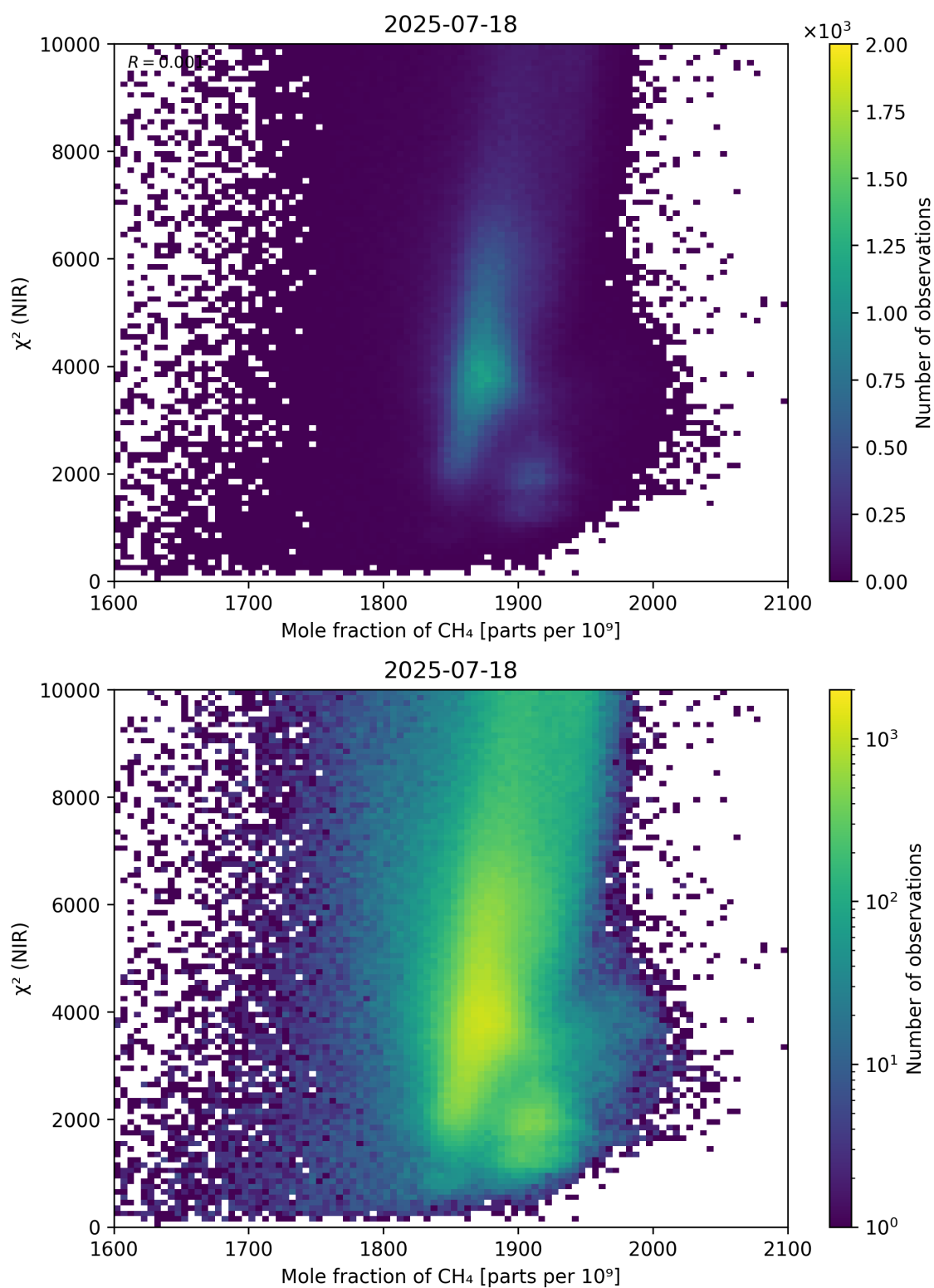
Figure 70: Scatter density plot of “Mole fraction of \text{CH}_4 ” against “ \chi^2 (NIR)” for 2025-07-18 to 2025-07-19.
