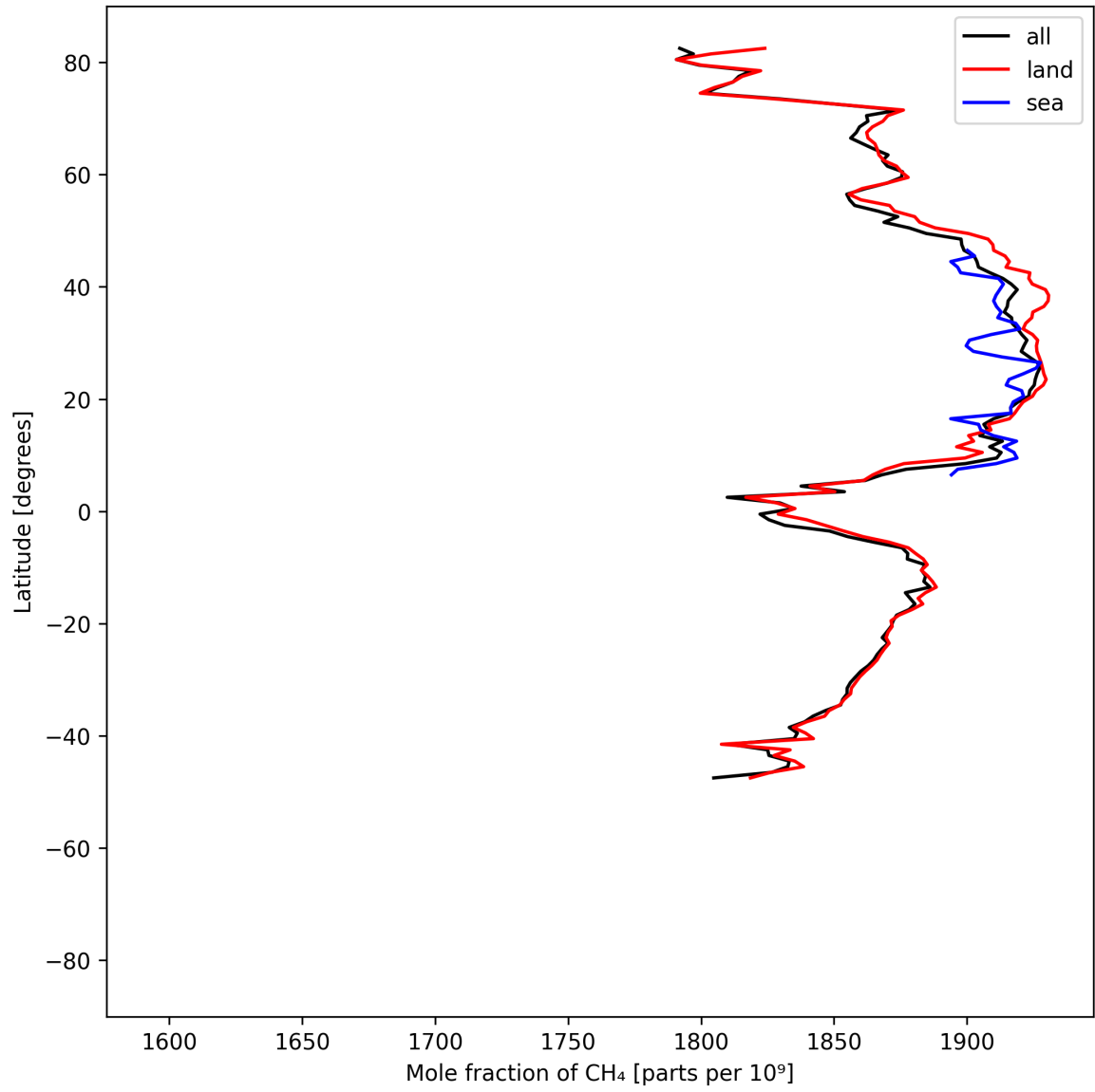
Figure 12: Zonal average of “Mole fraction of \text{CH}_4 ” for 2025-07-18 to 2025-07-19.
