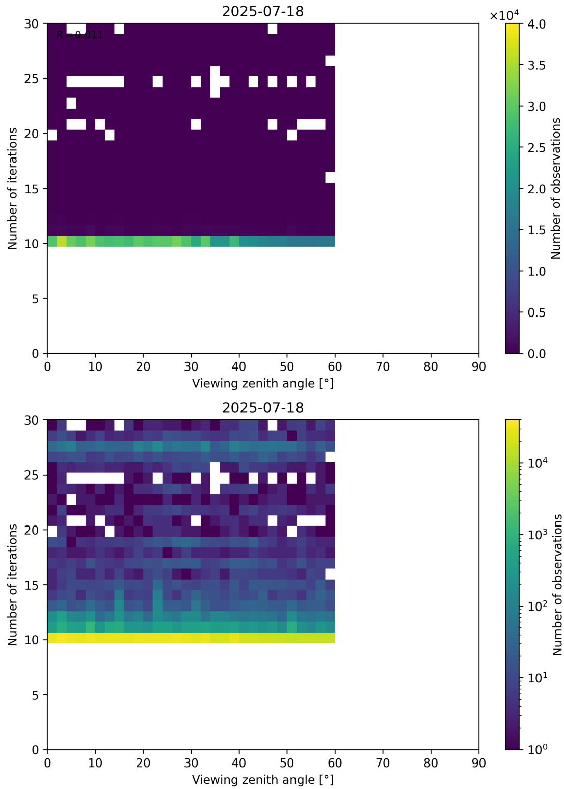
Figure 113: Scatter density plot of “Viewing zenith angle” against “Number of iterations” for 2025-07-18 to 2025-07-19.
