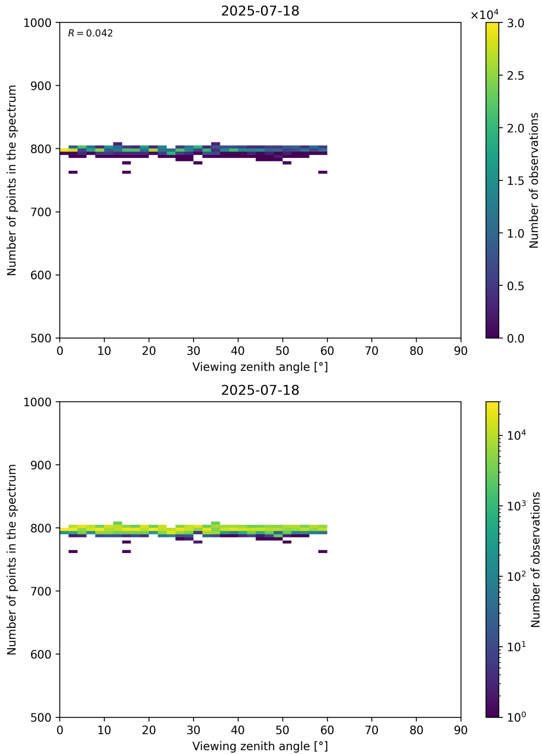
Figure 114: Scatter density plot of “Viewing zenith angle” against “Number of points in the spectrum” for 2025-07-18 to 2025-07-19.
