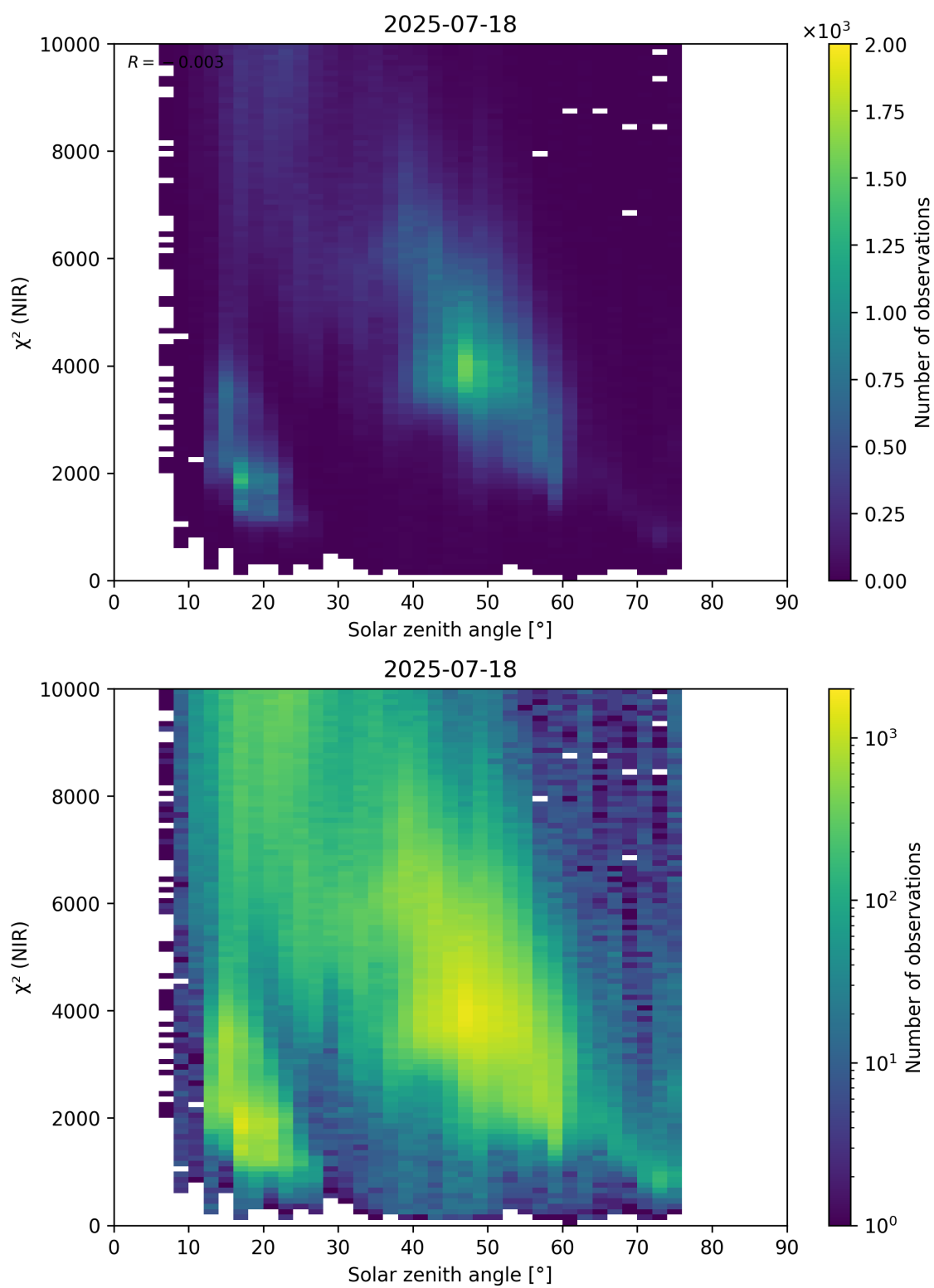
Figure 94: Scatter density plot of “Solar zenith angle” against “ \chi^2 (NIR)” for 2025-07-18 to 2025-07-19.
