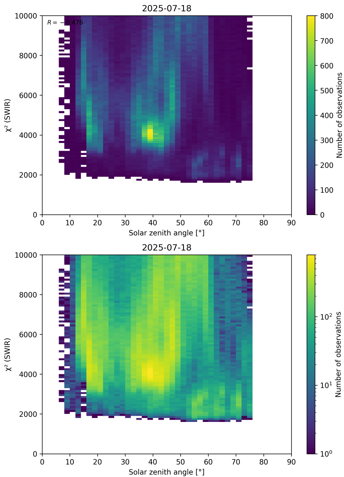
Figure 95: Scatter density plot of “Solar zenith angle” against “ \chi^2 (SWIR)” for 2025-07-18 to 2025-07-19.
