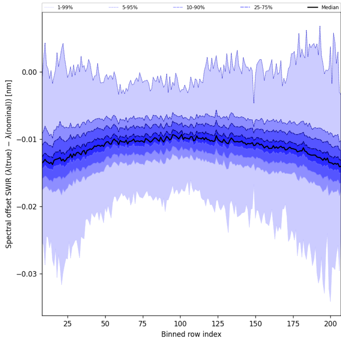
Figure 38: Along track statistics of “Spectral offset SWIR ( \lambda_{\text{true}} - \lambda_{\text{nominal}} )” for 2025-07-18 to 2025-07-19
