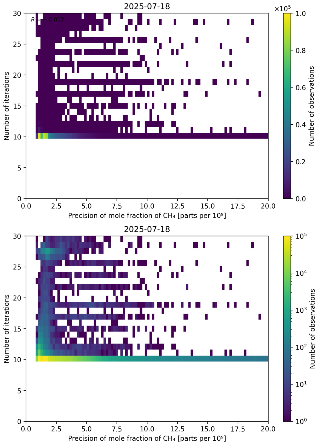
Figure 83: Scatter density plot of “Precision of mole fraction of CH 4 ” against “Number of iterations” for 2025-07-18 to 2025-07-19.
