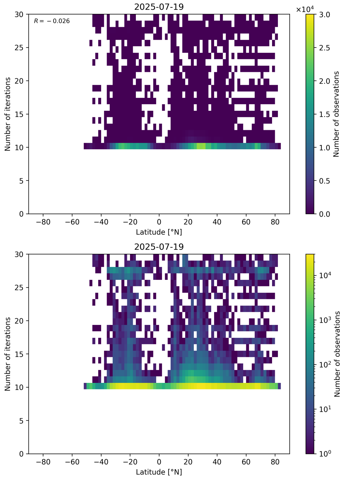
Figure 60: Scatter density plot of “Latitude” against “Number of iterations” for 2025-07-19 to 2025-07-20.
