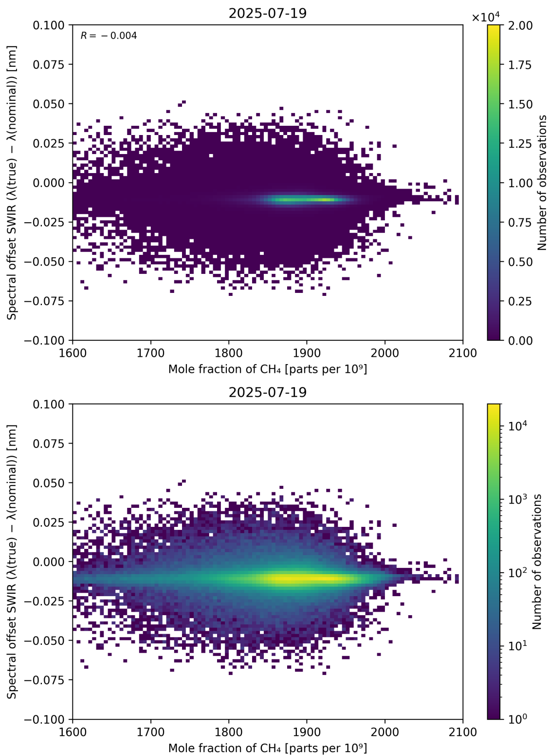
Figure 86: Scatter density plot of “Mole fraction of CH 4 ” against “Spectral offset SWIR ( \lambda_{\text{true}} - \lambda_{\text{nominal}} )” for 2025-07-19 to 2025-07-20.
