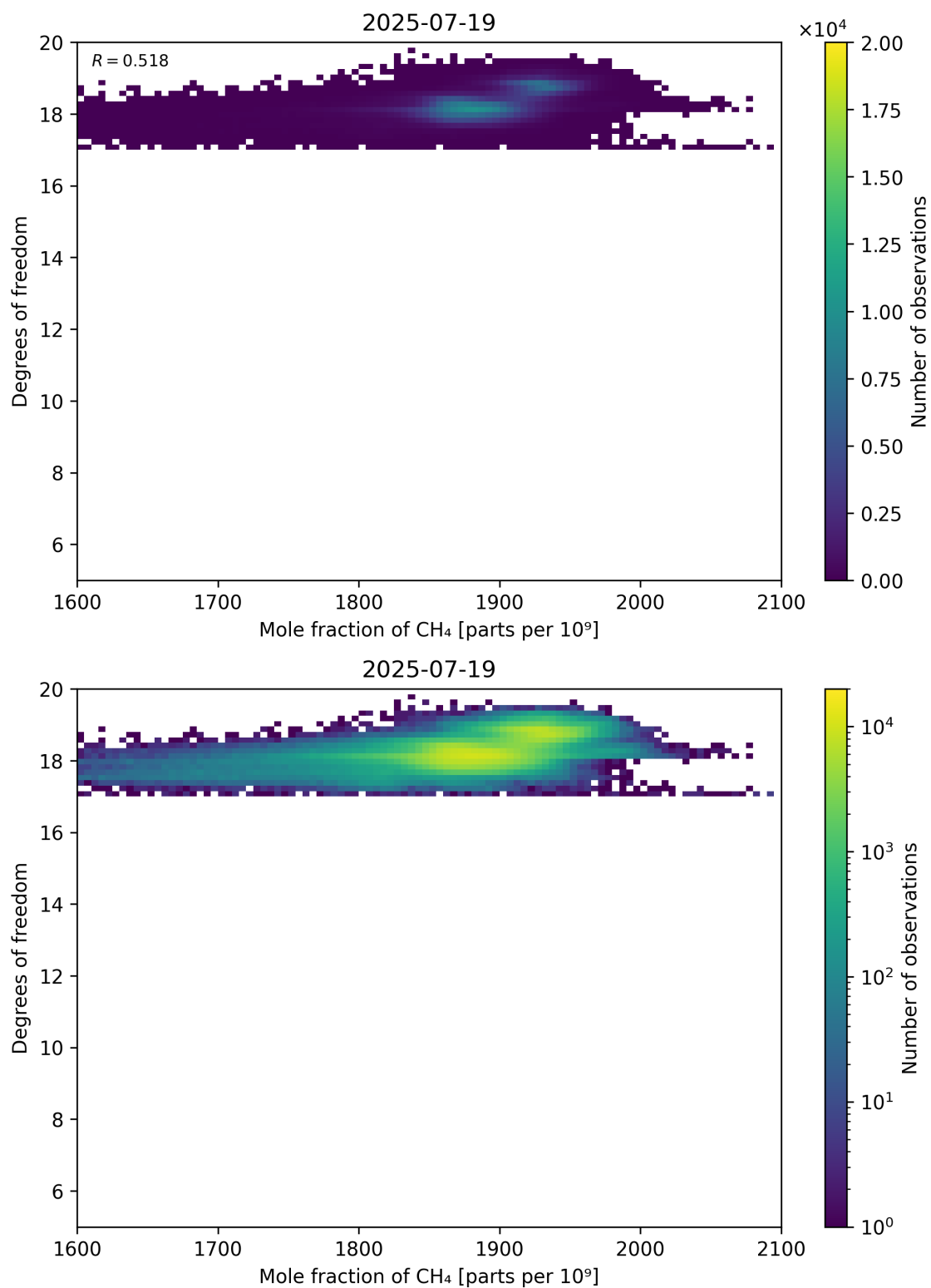
Figure 72: Scatter density plot of “Mole fraction of CH 4 ” against “Degrees of freedom” for 2025-07-19 to 2025-07-20.
