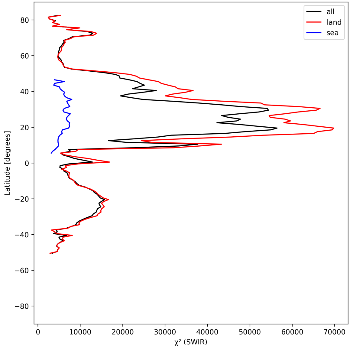
Figure 17: Zonal average of “ \chi^2 (SWIR)” for 2025-07-19 to 2025-07-20.
