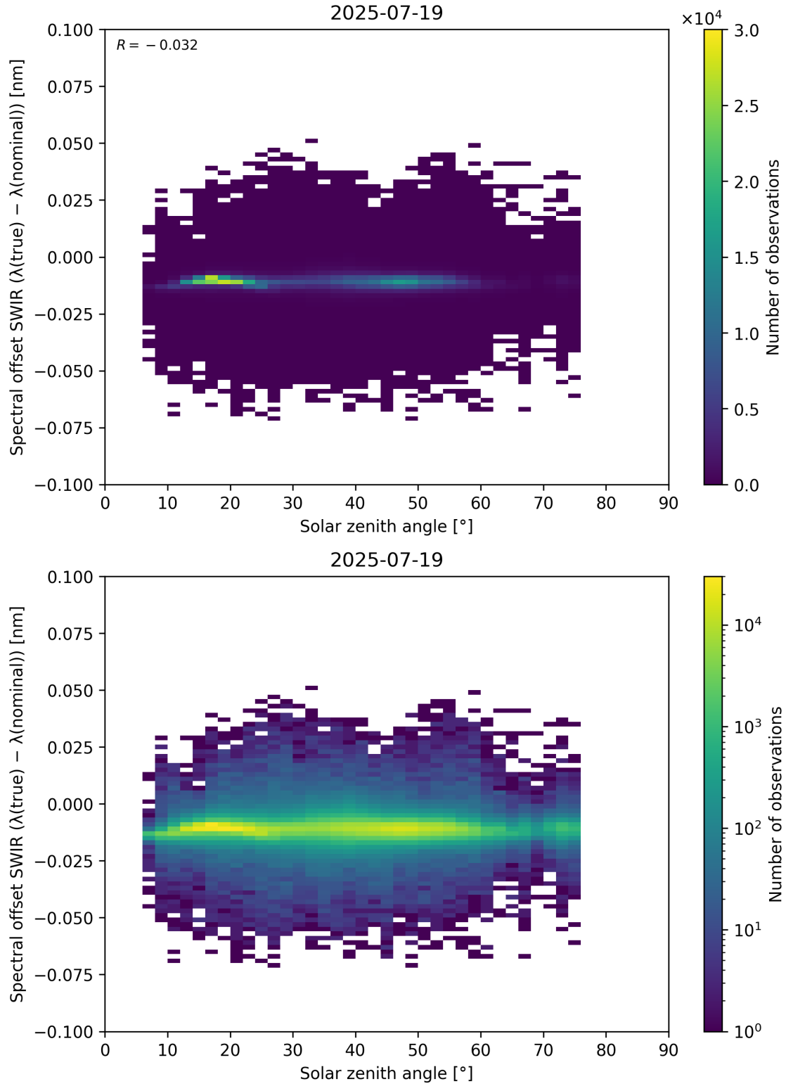
Figure 104: Scatter density plot of “Solar zenith angle” against “Spectral offset SWIR ( \lambda_{\text{true}} - \lambda_{\text{nominal}} )” for 2025-07-19 to 2025-07-20.
