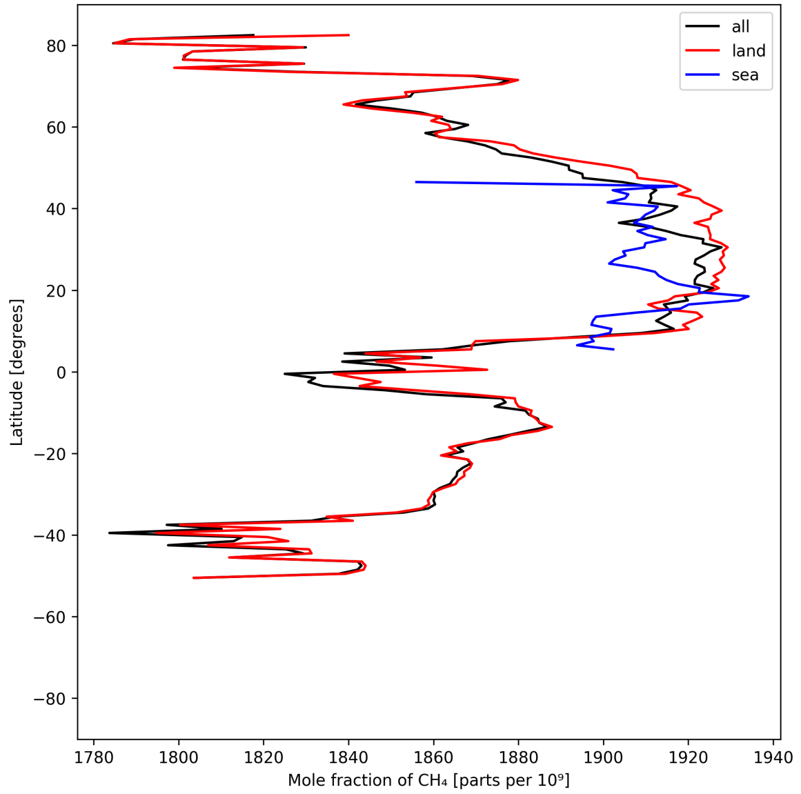
Figure 12: Zonal average of “Mole fraction of \text{CH}_4 ” for 2025-07-19 to 2025-07-20.
