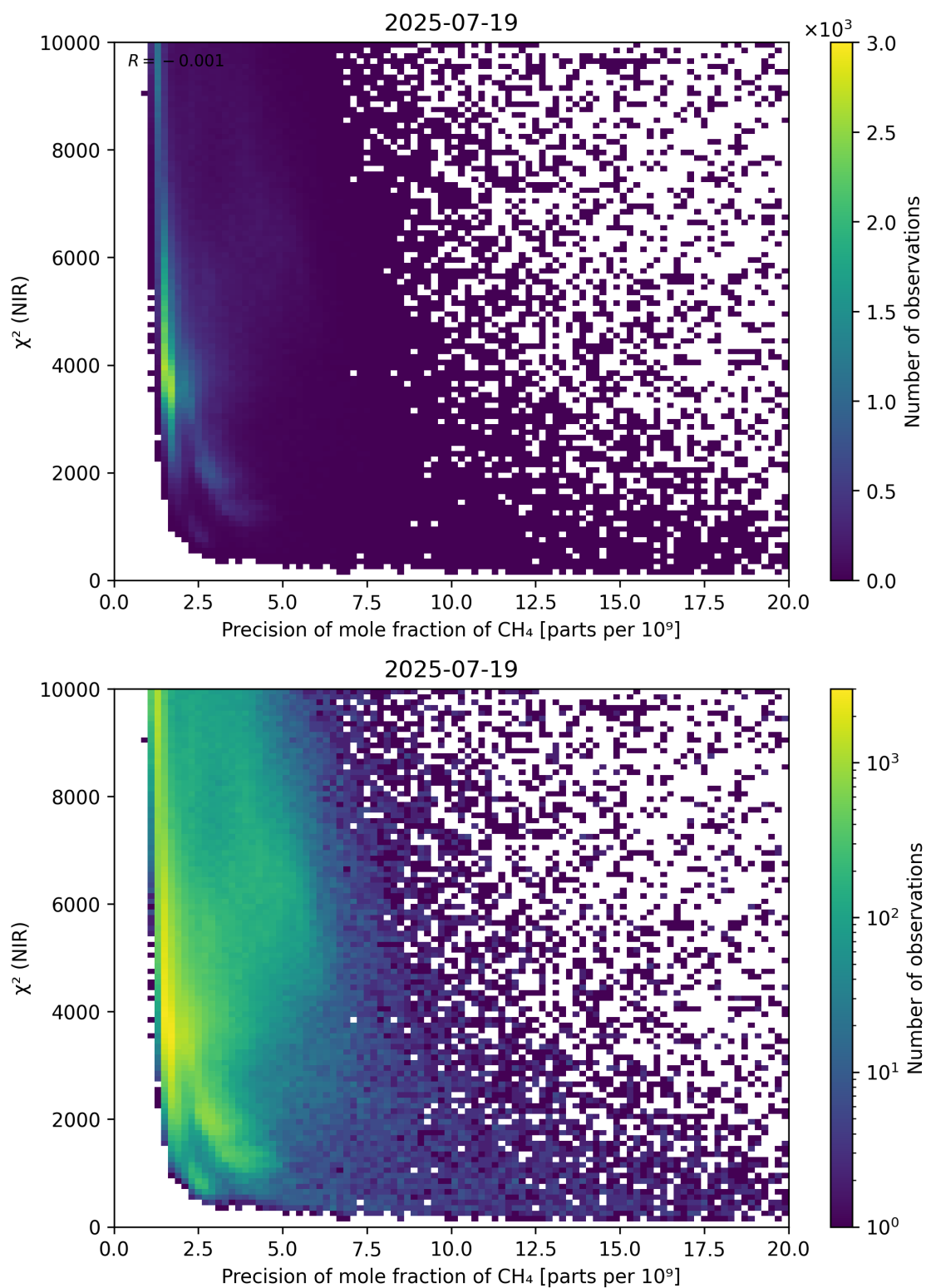
Figure 78: Scatter density plot of “Precision of mole fraction of CH 4 ” against “ \chi^2 (NIR)” for 2025-07-19 to 2025-07-20.
