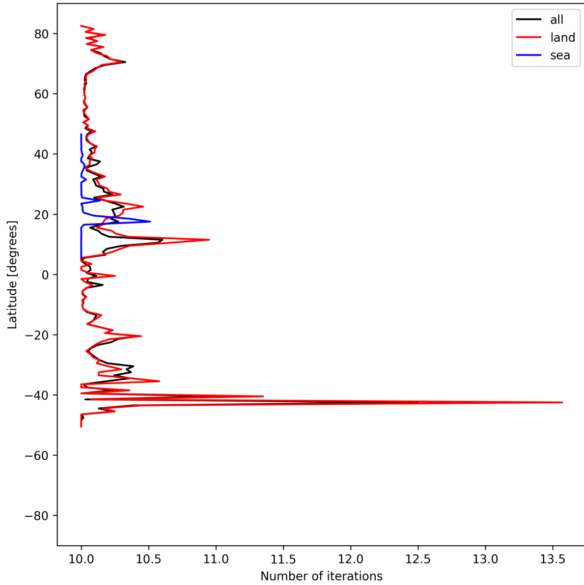
Figure 20: Zonal average of “Number of iterations” for 2025-07-19 to 2025-07-20.
