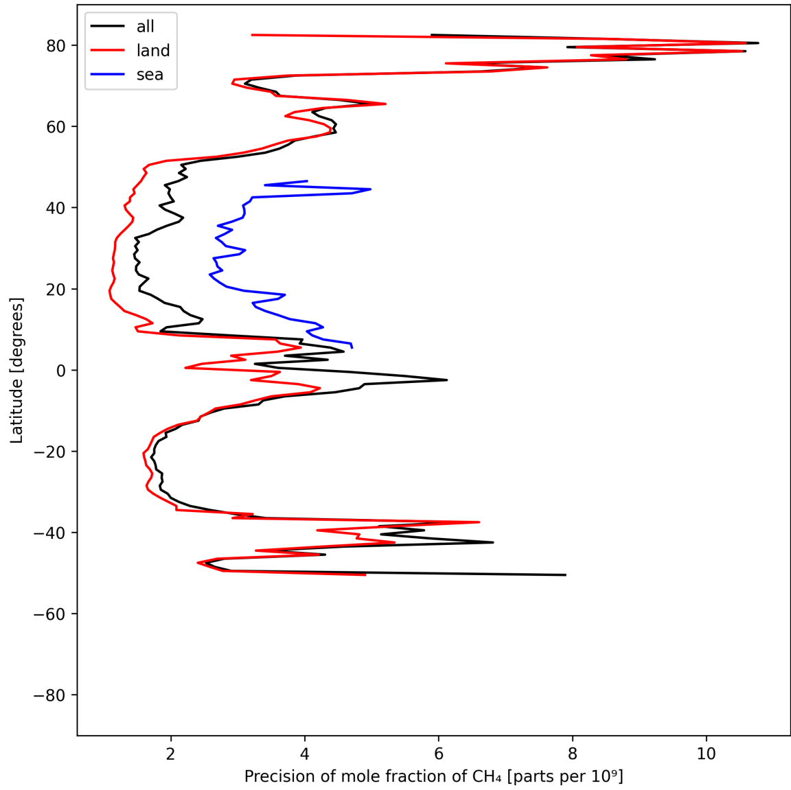
Figure 13: Zonal average of “Precision of mole fraction of CH 4 ” for 2025-07-19 to 2025-07-20.
