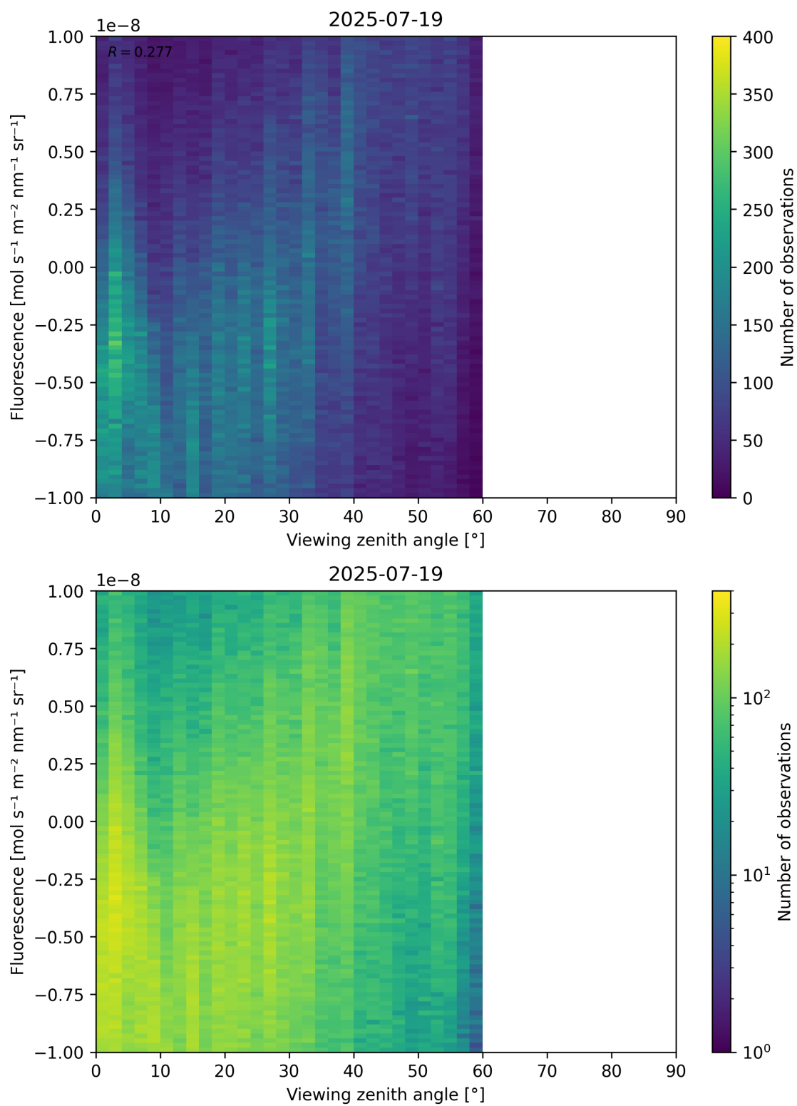
Figure 108: Scatter density plot of “Viewing zenith angle” against “Fluorescence” for 2025-07-19 to 2025-07-20.
