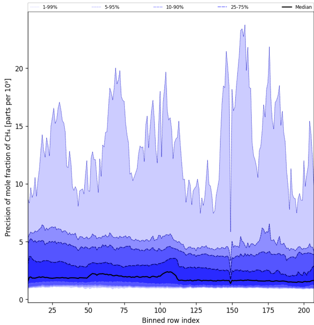
Figure 35: Along track statistics of “Precision of mole fraction of CH 4 ” for 2025-07-19 to 2025-07-20
