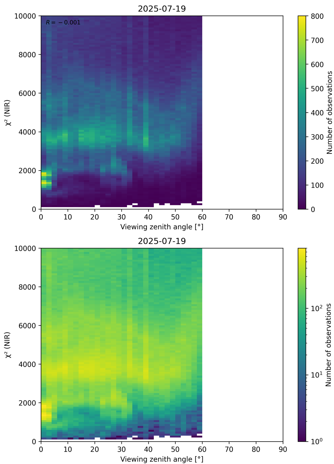
Figure 105: Scatter density plot of “Viewing zenith angle” against “ \chi^2 (NIR)” for 2025-07-19 to 2025-07-20.
