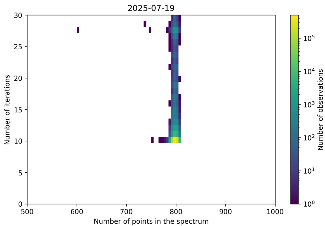
Figure 92: Scatter density plot of “Number of points in the spectrum” against “Number of iterations” for 2025-07-19 to 2025-07-20.
