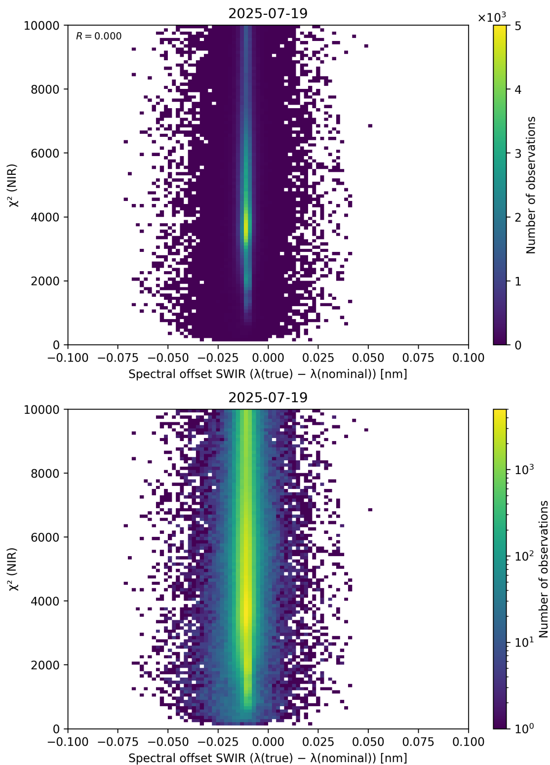
Figure 117: Scatter density plot of “Spectral offset SWIR ( \lambda_{\text{true}} - \lambda_{\text{nominal}} )” against “ \chi^2 (NIR)” for 2025-07-19 to 2025-07-20.
