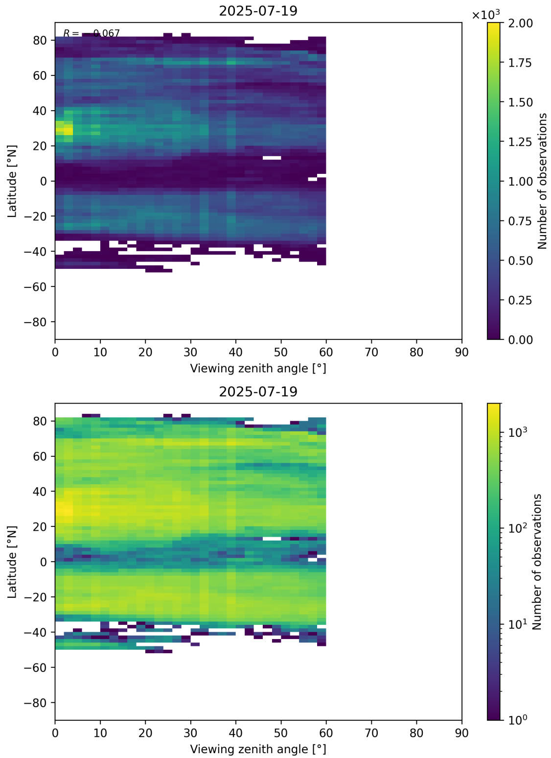
Figure 109: Scatter density plot of “Viewing zenith angle” against “Latitude” for 2025-07-19 to 2025-07-20.
