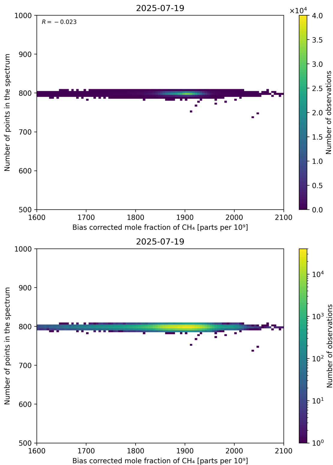
Figure 68: Scatter density plot of “Bias corrected mole fraction of CH 4 ” against “Number of points in the spectrum” for 2025-07-19 to 2025-07-20.
