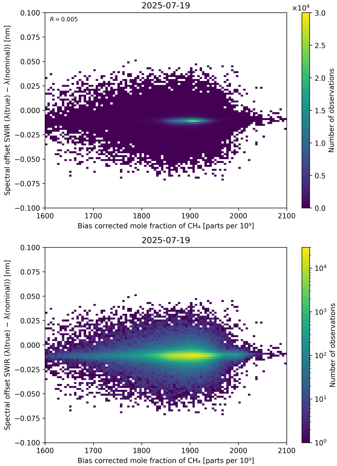
Figure 69: Scatter density plot of “Bias corrected mole fraction of \text{CH}_4 ” against “Spectral offset SWIR ( \lambda_{\text{true}} - \lambda_{\text{nominal}} )” for 2025-07-19 to 2025-07-20.
