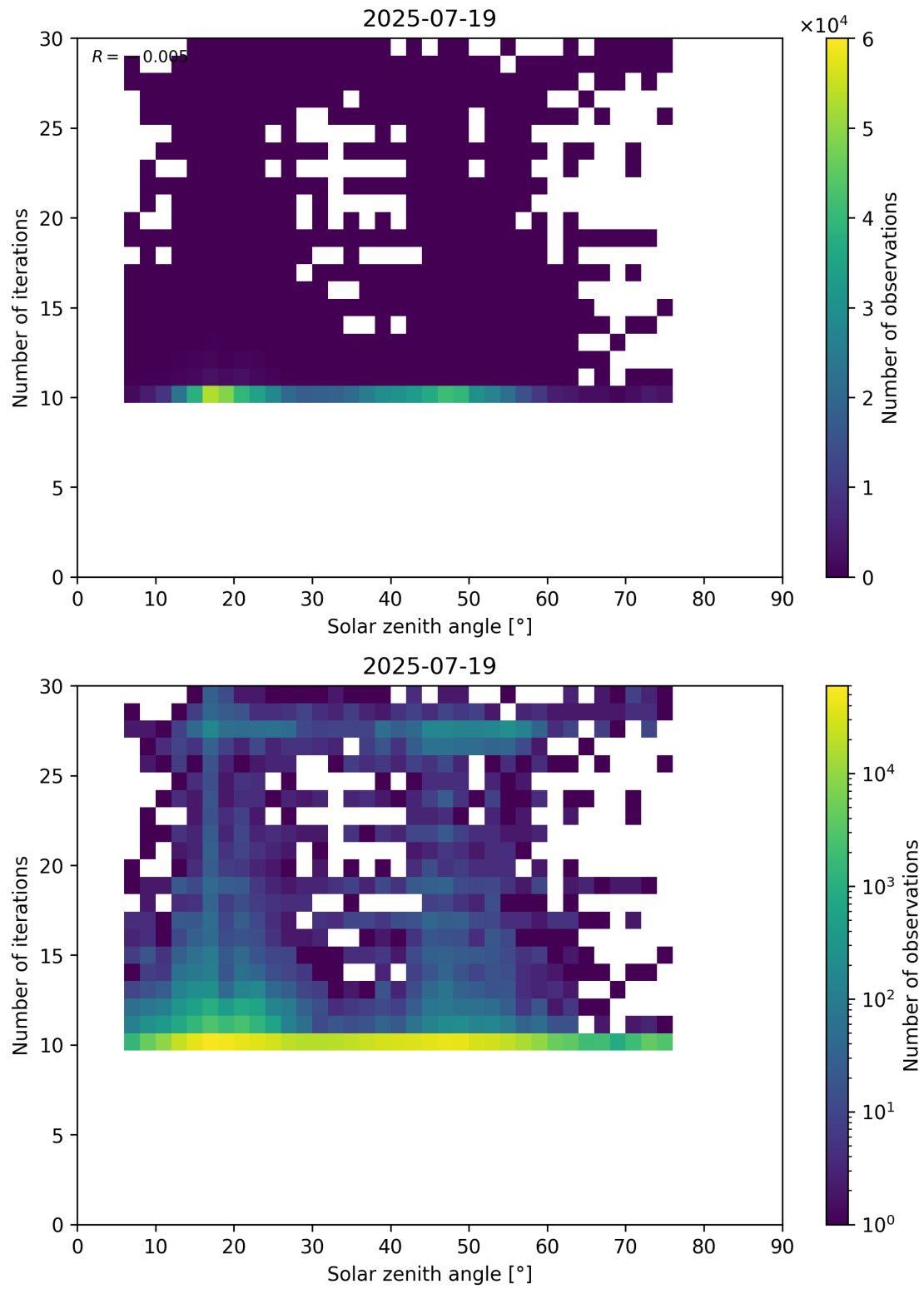
Figure 102: Scatter density plot of “Solar zenith angle” against “Number of iterations” for 2025-07-19 to 2025-07-20.
