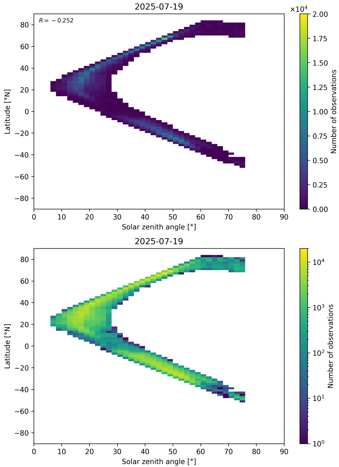
Figure 98: Scatter density plot of “Solar zenith angle” against “Latitude” for 2025-07-19 to 2025-07-20.
