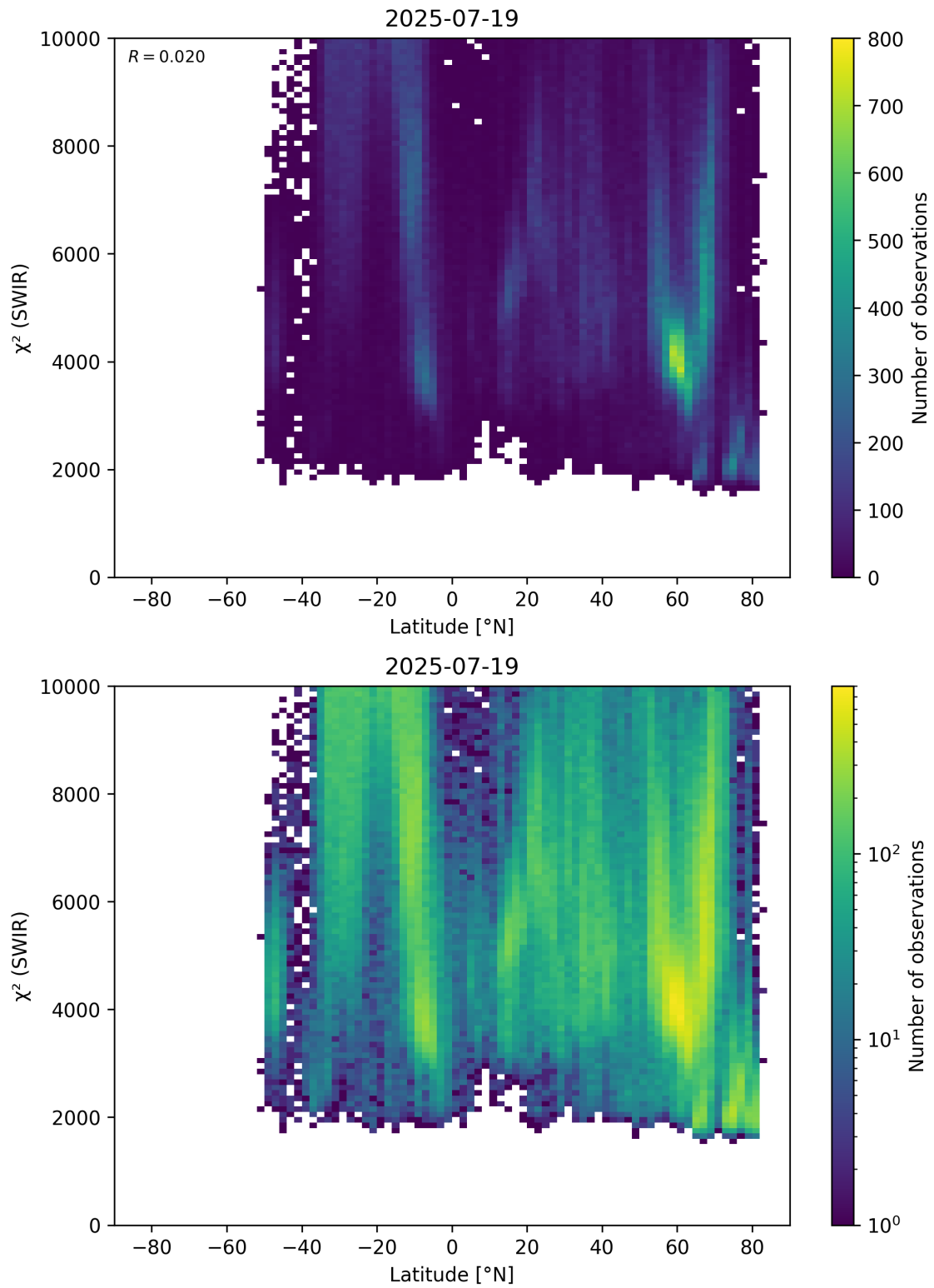
Figure 54: Scatter density plot of “Latitude” against “ \chi^2 (SWIR)” for 2025-07-19 to 2025-07-20.
