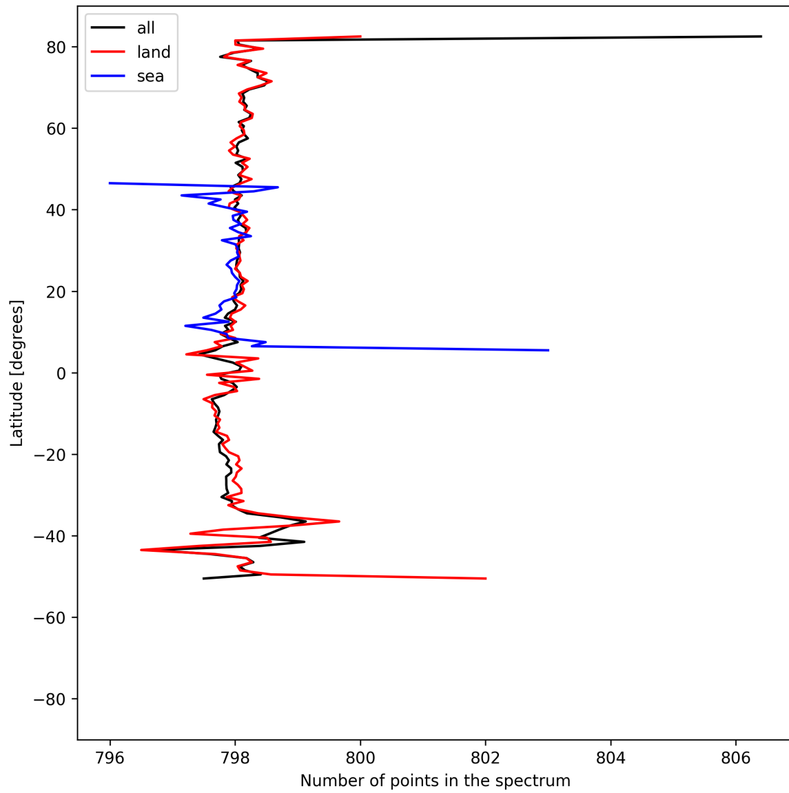
Figure 15: Zonal average of “Number of points in the spectrum” for 2025-07-19 to 2025-07-20.
