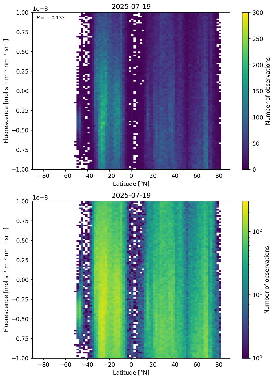
Figure 56: Scatter density plot of “Latitude” against “Fluorescence” for 2025-07-19 to 2025-07-20.
