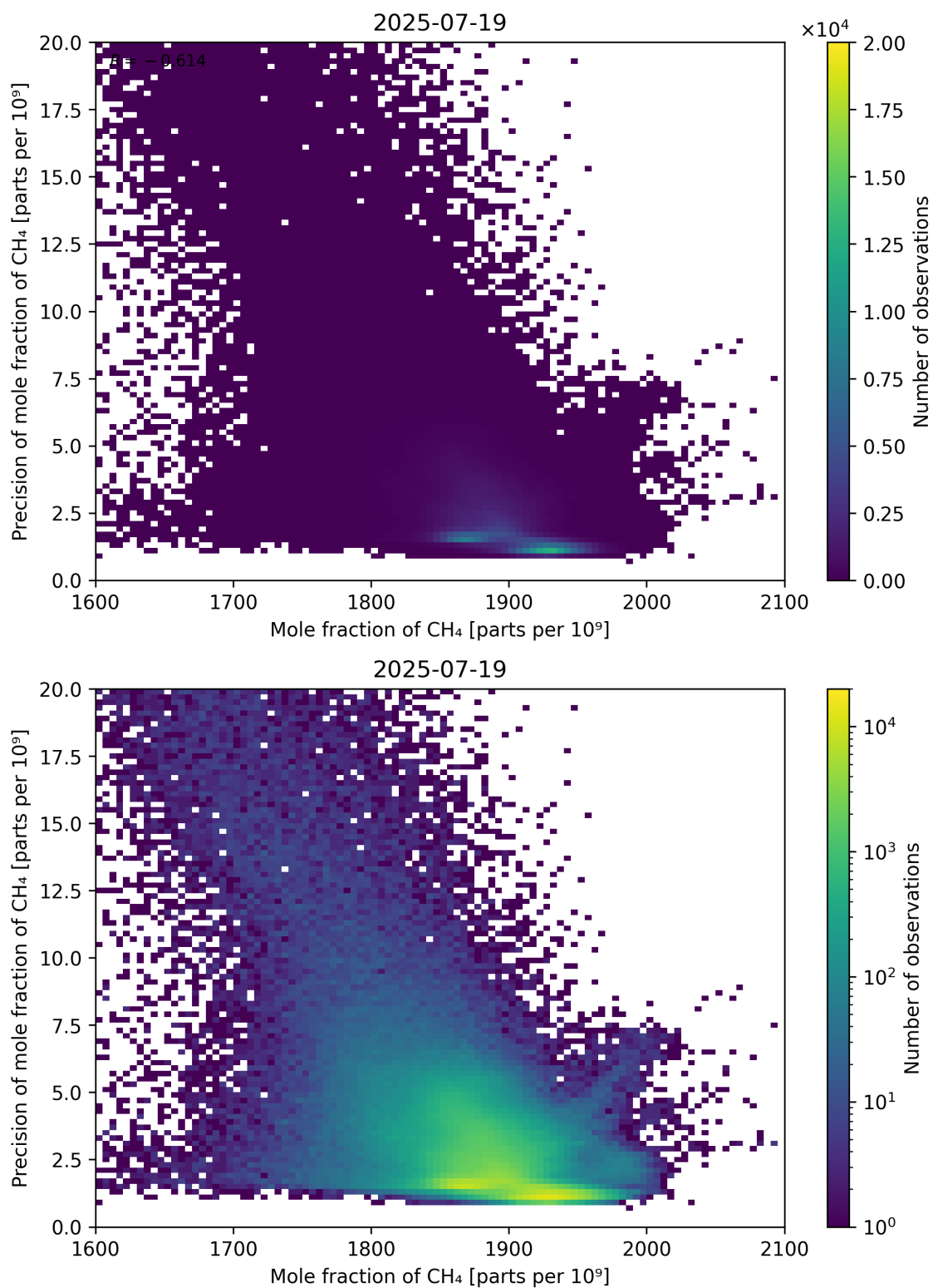
Figure 75: Scatter density plot of “Mole fraction of CH 4 ” against “Precision of mole fraction of CH 4 ” for 2025-07-19 to 2025-07-20.
