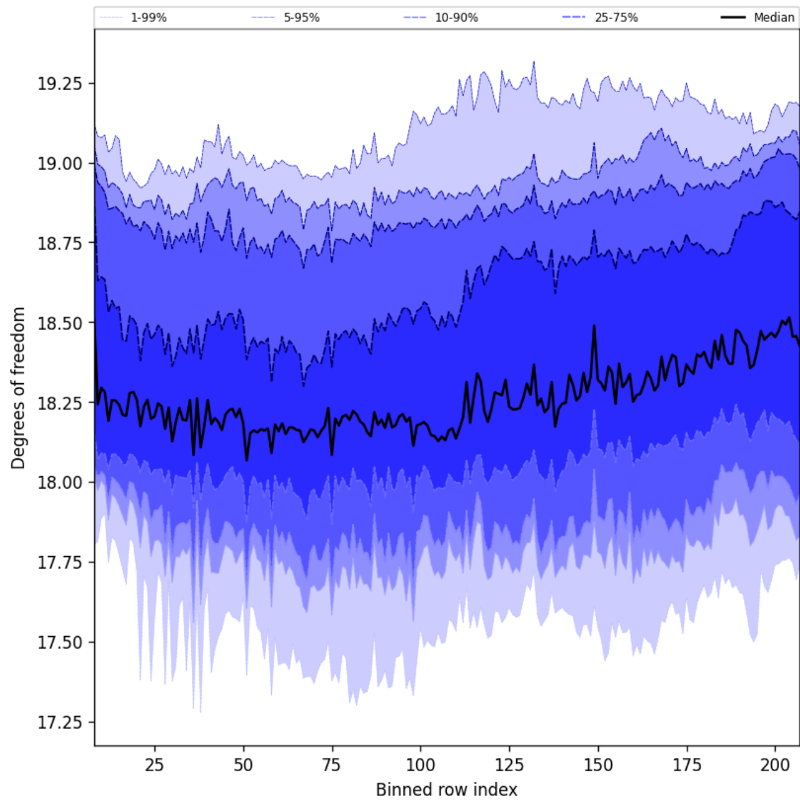
Figure 41: Along track statistics of “Degrees of freedom” for 2025-07-19 to 2025-07-20
