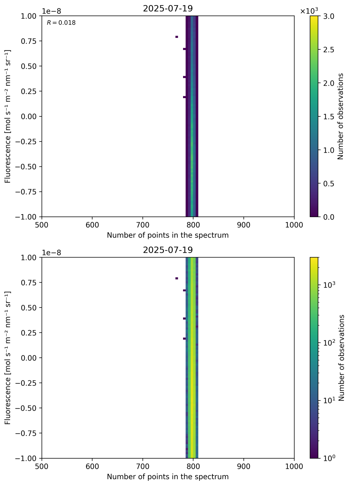
Figure 91: Scatter density plot of “Number of points in the spectrum” against “Fluorescence” for 2025-07-19 to 2025-07-20.
