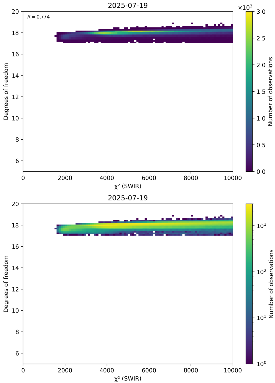
Figure 48: Scatter density plot of “ \chi^2 (SWIR)” against “Degrees of freedom” for 2025-07-19 to 2025-07-20.
