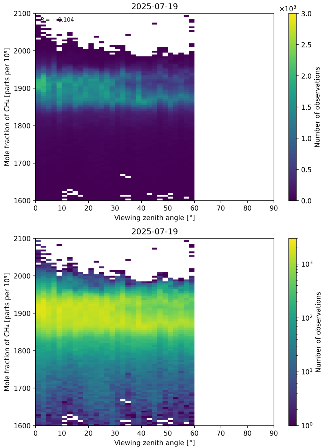
Figure 110: Scatter density plot of “Viewing zenith angle” against “Mole fraction of CH 4 ” for 2025-07-19 to 2025-07-20.
