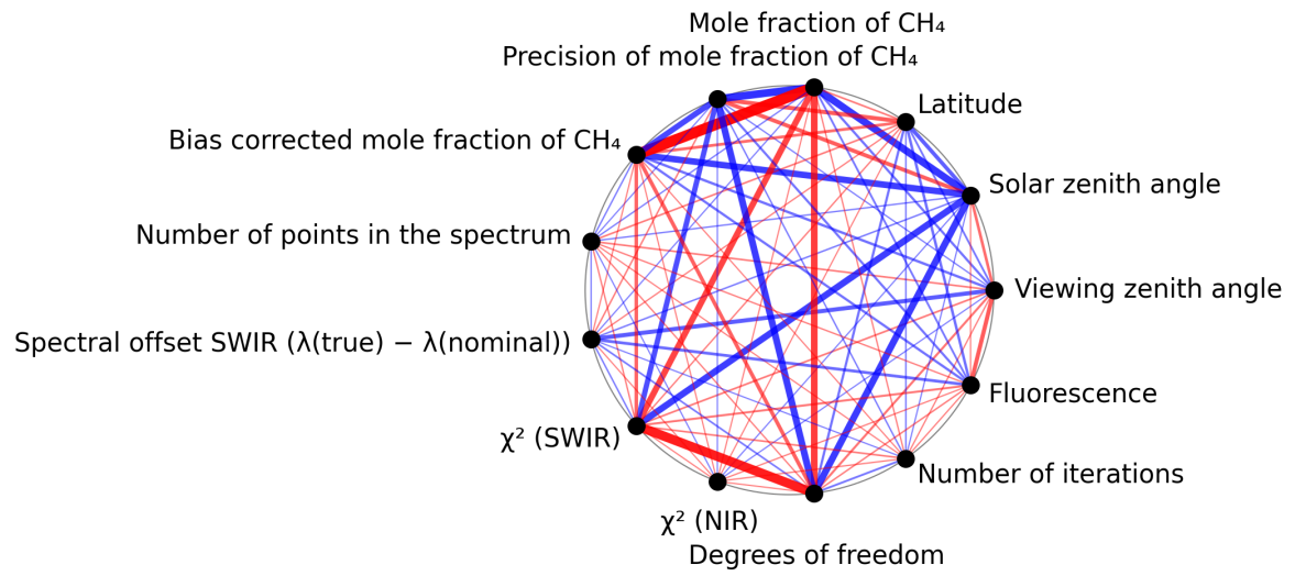
Figure 1: Map of correlation graph for 2025-07-19 to 2025-07-20.
