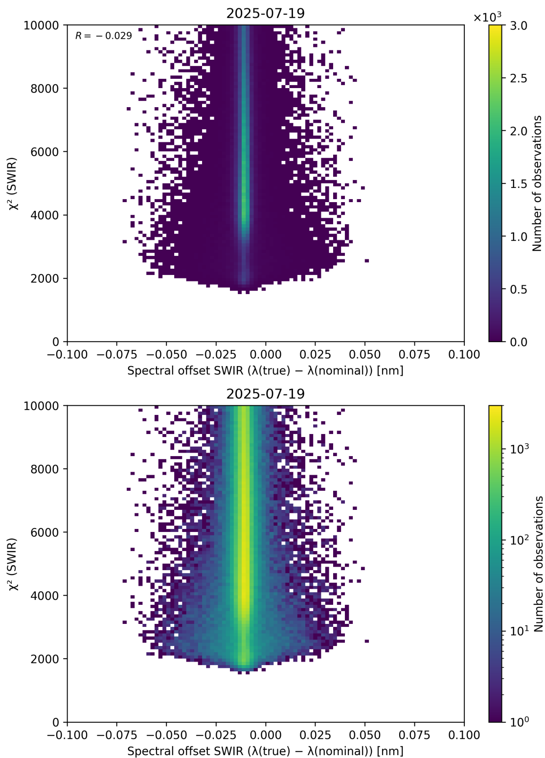
Figure 118: Scatter density plot of “Spectral offset SWIR ( \lambda_{\text{true}} - \lambda_{\text{nominal}} )” against “ \chi^2 (SWIR)” for 2025-07-19 to 2025-07-20.
