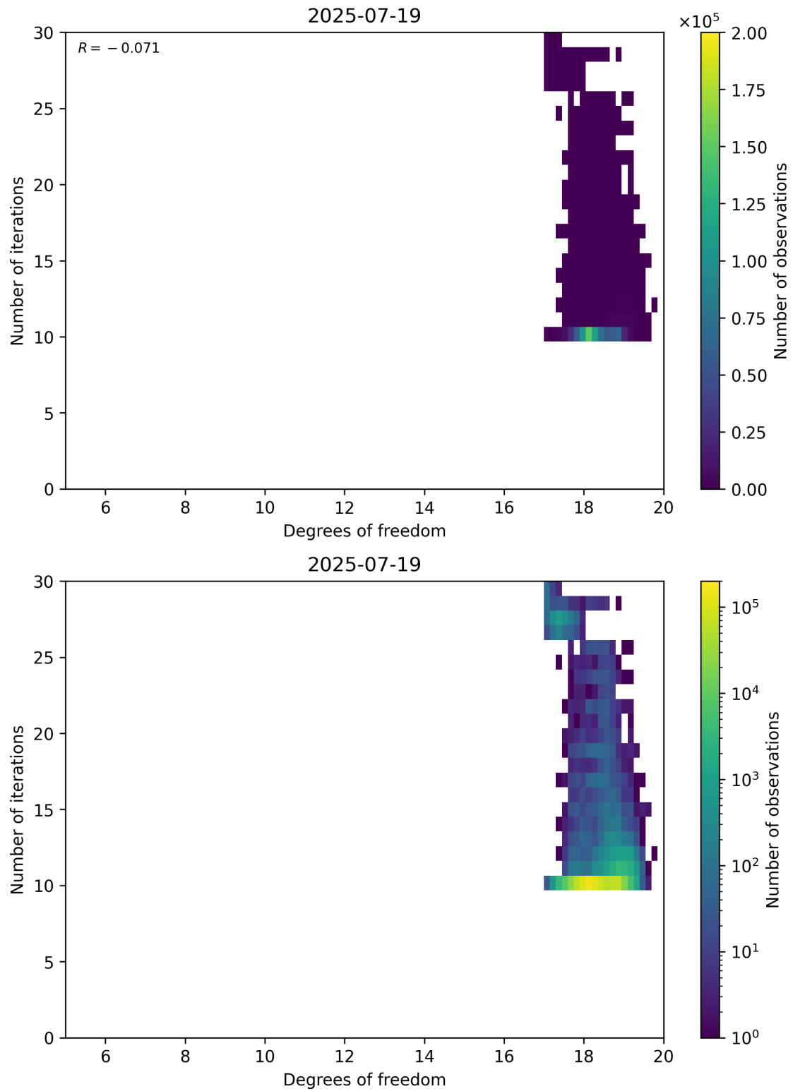
Figure 52: Scatter density plot of “Degrees of freedom” against “Number of iterations” for 2025-07-19 to 2025-07-20.
