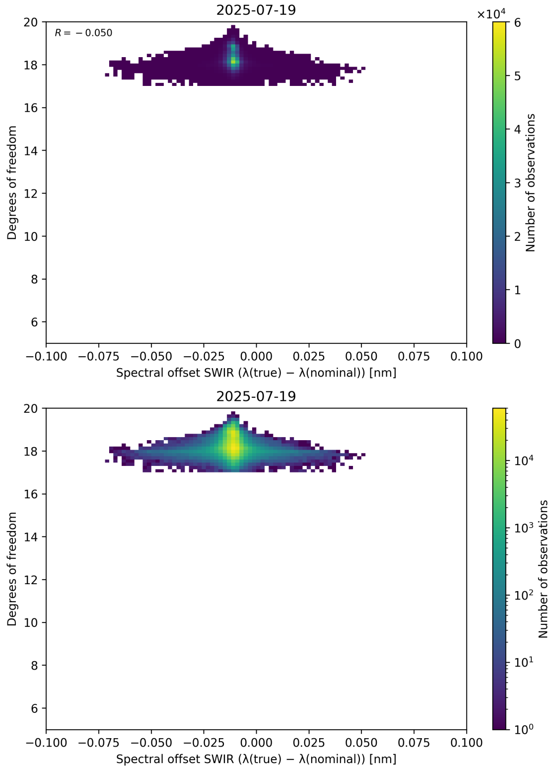
Figure 119: Scatter density plot of “Spectral offset SWIR ( \lambda_{\text{true}} - \lambda_{\text{nominal}} )” against “Degrees of freedom” for 2025-07-19 to 2025-07-20.
