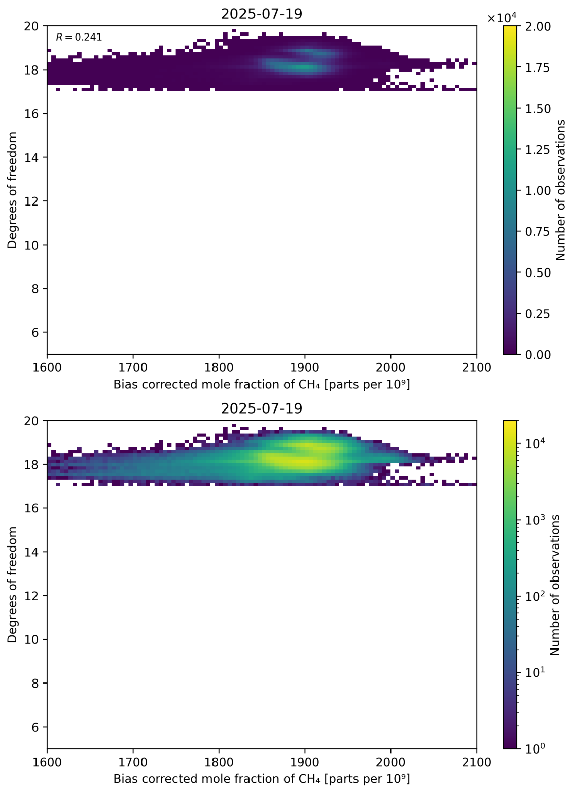
Figure 65: Scatter density plot of “Bias corrected mole fraction of CH 4 ” against “Degrees of freedom” for 2025-07-19 to 2025-07-20.
