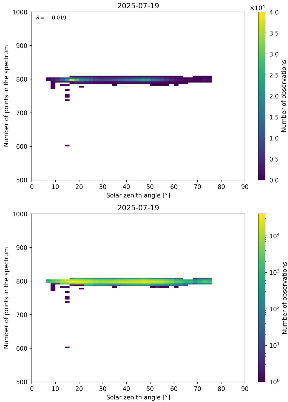
Figure 103: Scatter density plot of “Solar zenith angle” against “Number of points in the spectrum” for 2025-07-19 to 2025-07-20.
