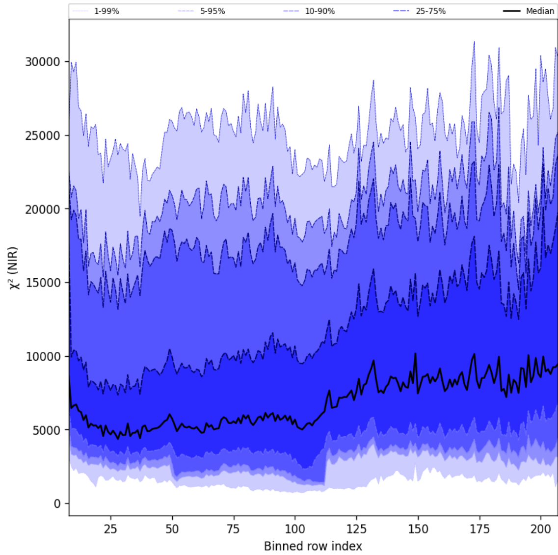
Figure 40: Along track statistics of “ \chi^2 (NIR)” for 2025-07-19 to 2025-07-20
