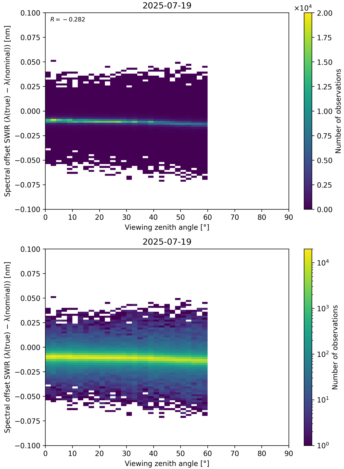
Figure 116: Scatter density plot of “Viewing zenith angle” against “Spectral offset SWIR ( \lambda_{\text{true}} - \lambda_{\text{nominal}} )” for 2025-07-19 to 2025-07-20.
