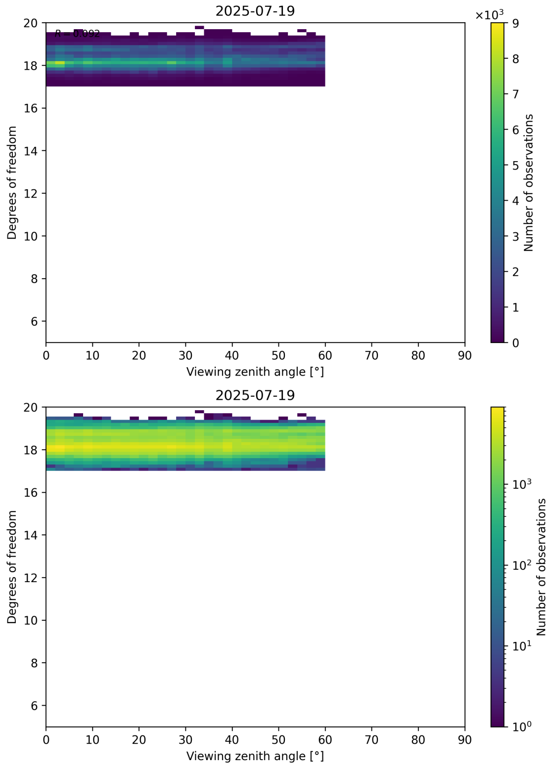
Figure 107: Scatter density plot of “Viewing zenith angle” against “Degrees of freedom” for 2025-07-19 to 2025-07-20.
