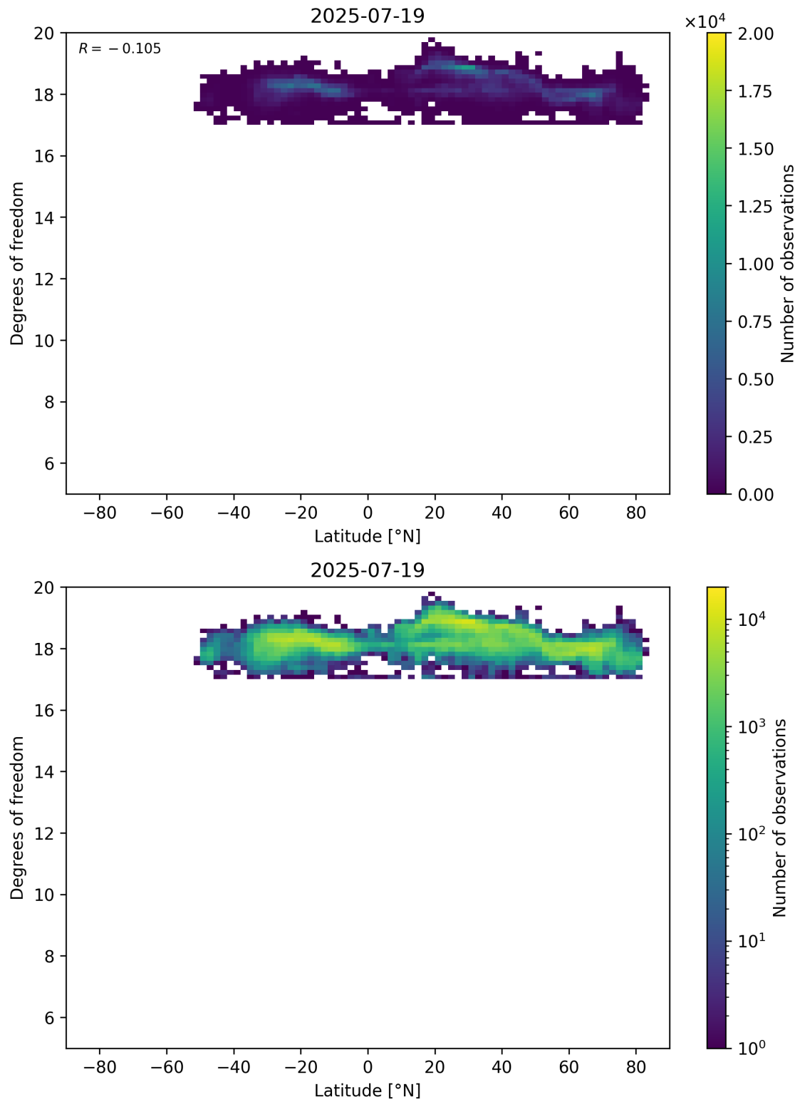
Figure 55: Scatter density plot of “Latitude” against “Degrees of freedom” for 2025-07-19 to 2025-07-20.
