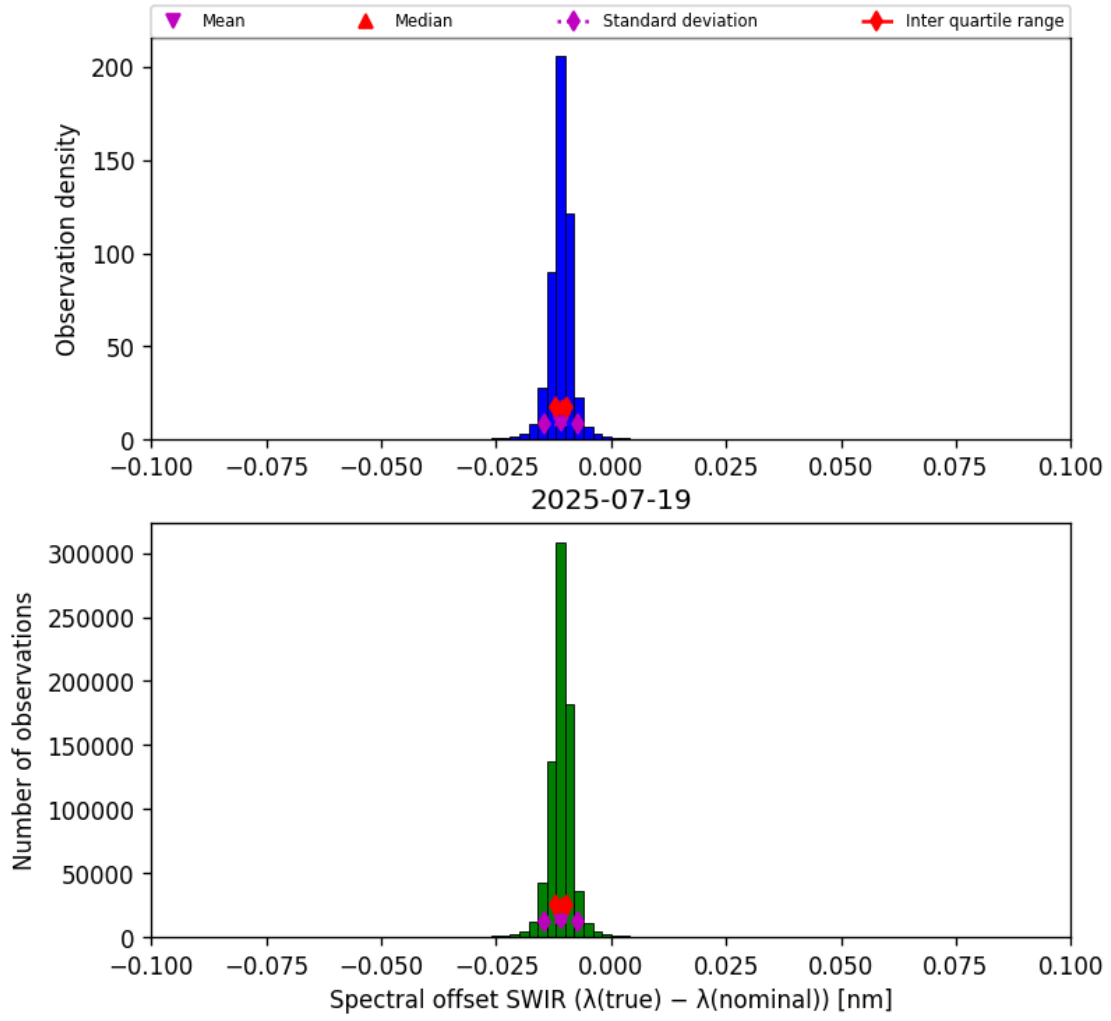
Figure 27: Histogram of “Spectral offset SWIR ( \lambda_{\text{true}} - \lambda_{\text{nominal}} )” for 2025-07-19 to 2025-07-20
