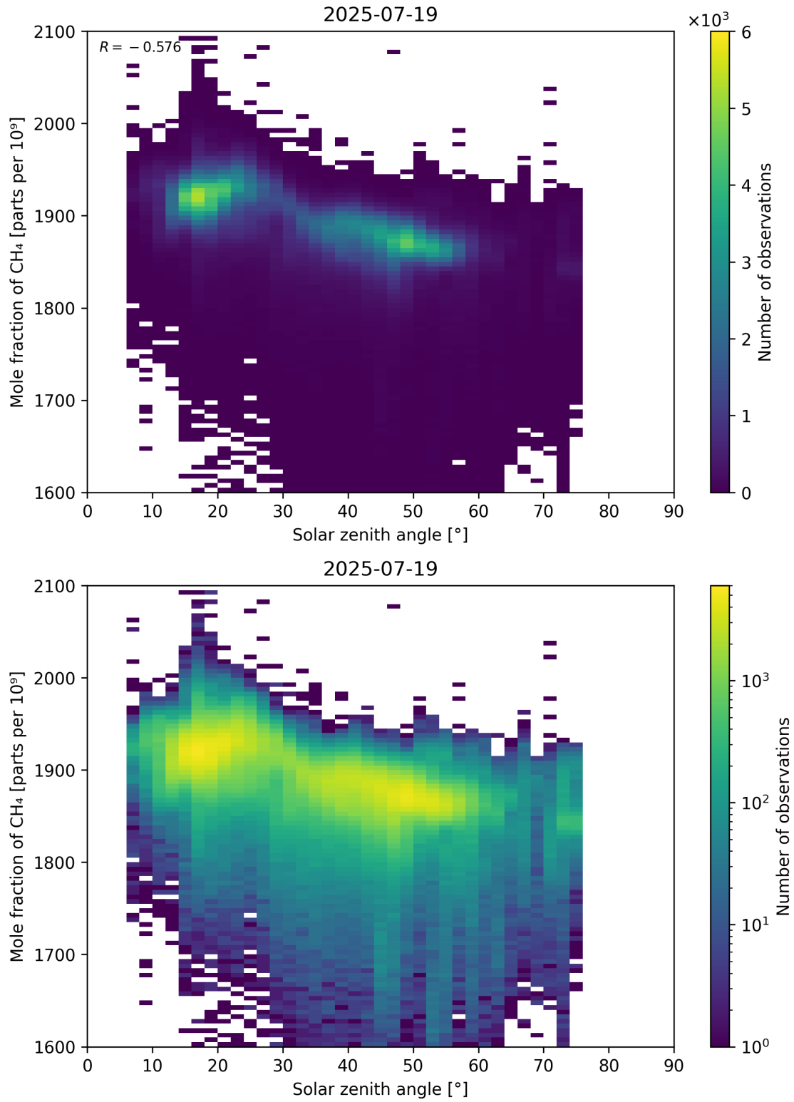
Figure 99: Scatter density plot of “Solar zenith angle” against “Mole fraction of CH 4 ” for 2025-07-19 to 2025-07-20.
