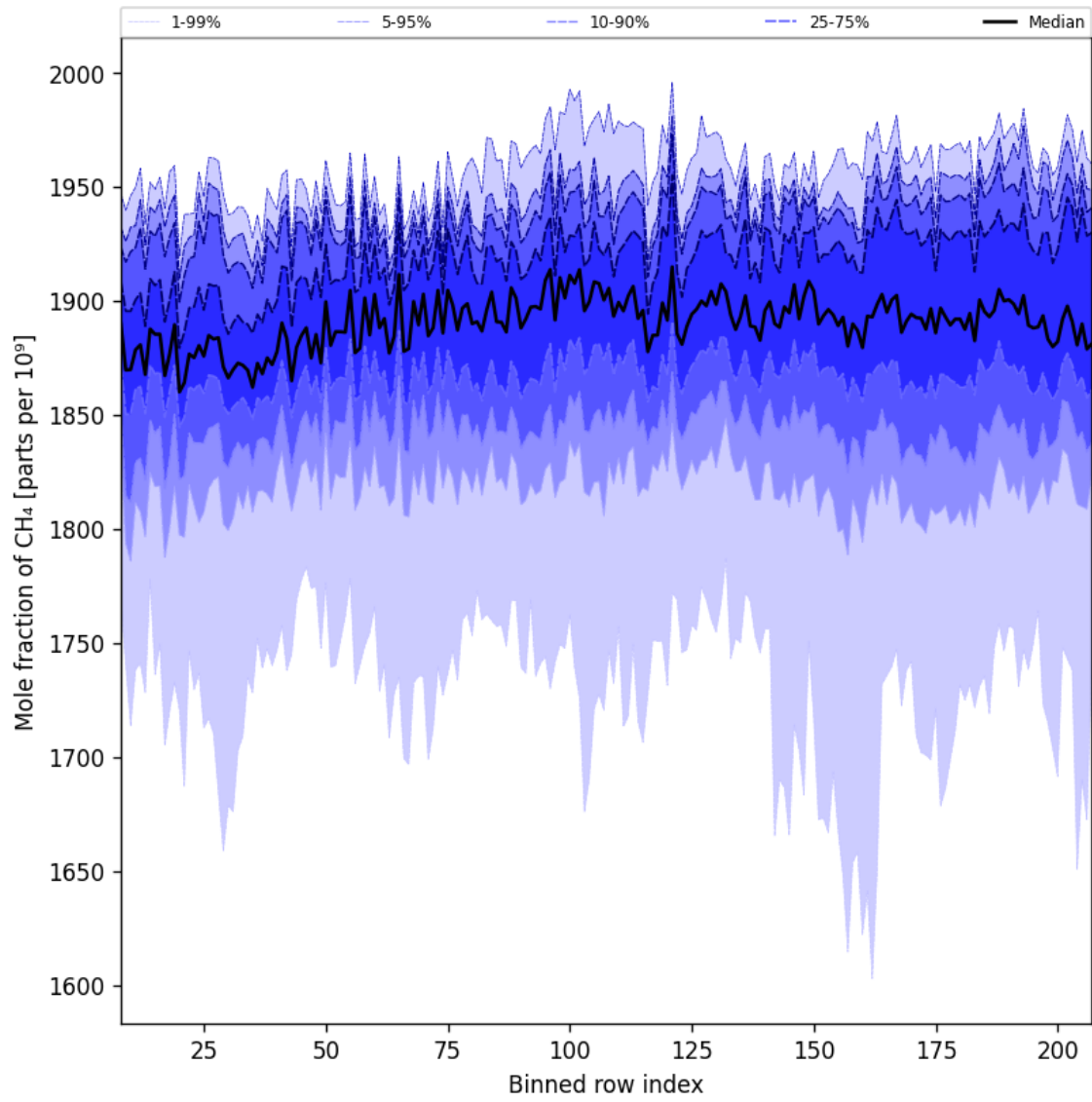
Figure 34: Along track statistics of “Mole fraction of CH 4 ” for 2025-07-19 to 2025-07-20
