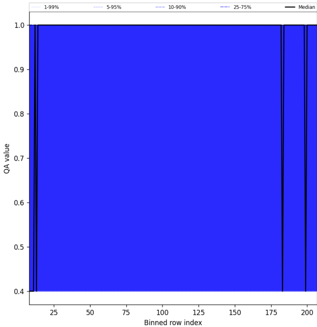
Figure 33: Along track statistics of “QA value” for 2025-07-19 to 2025-07-20
