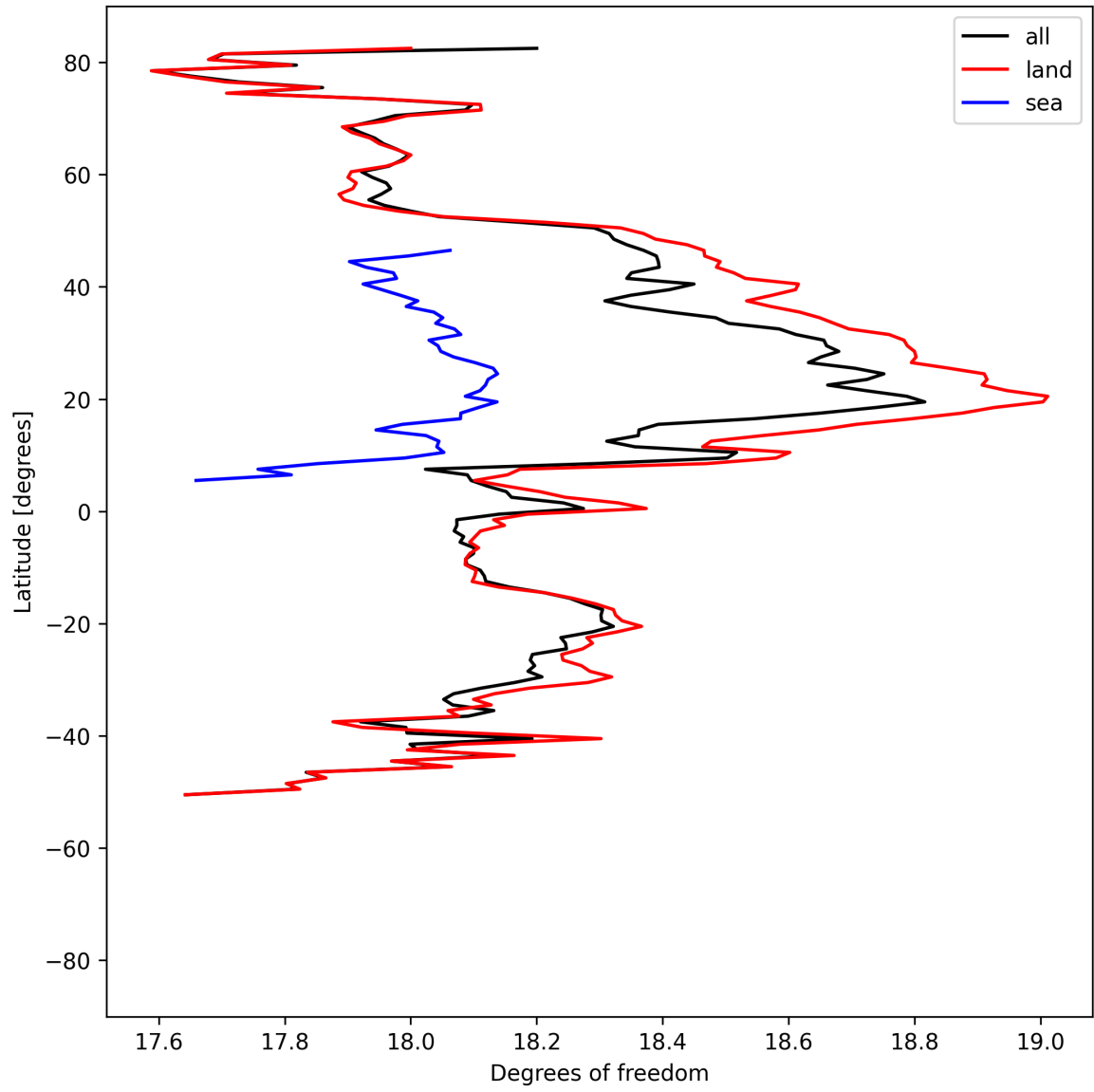
Figure 19: Zonal average of “Degrees of freedom” for 2025-07-19 to 2025-07-20.
