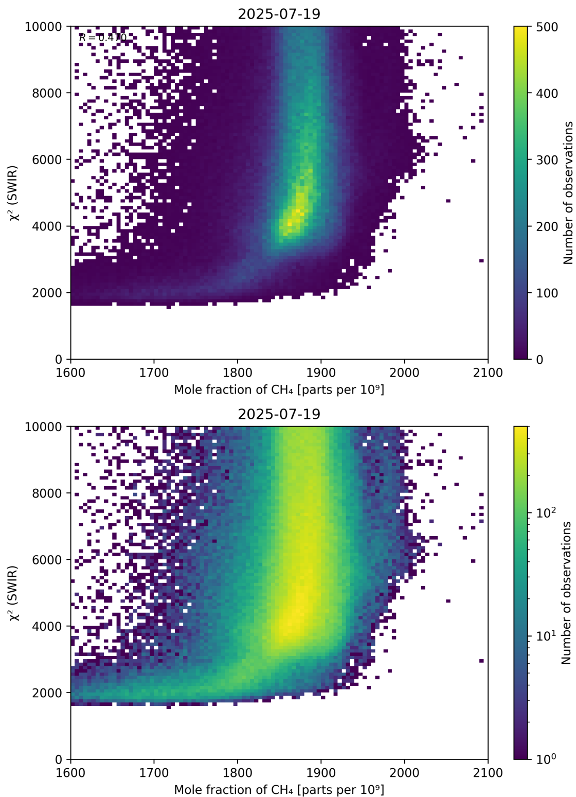
Figure 71: Scatter density plot of “Mole fraction of \text{CH}_4 ” against “ \chi^2 (SWIR)” for 2025-07-19 to 2025-07-20.
