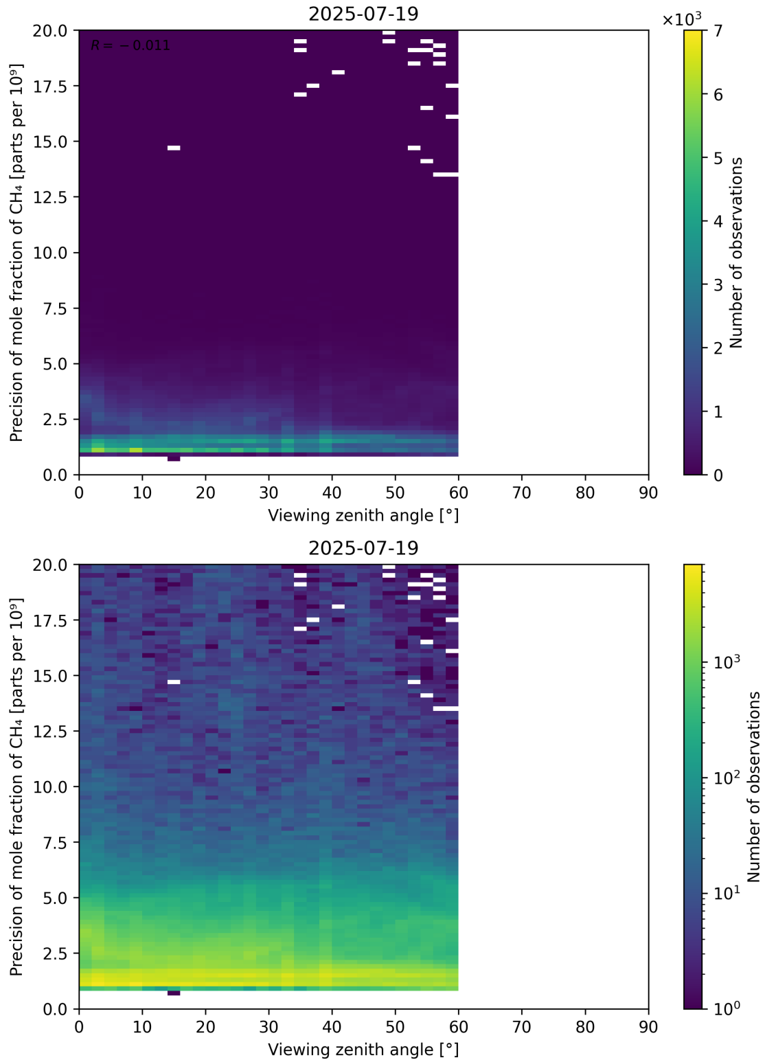
Figure 112: Scatter density plot of “Viewing zenith angle” against “Precision of mole fraction of CH 4 ” for 2025-07-19 to 2025-07-20.
