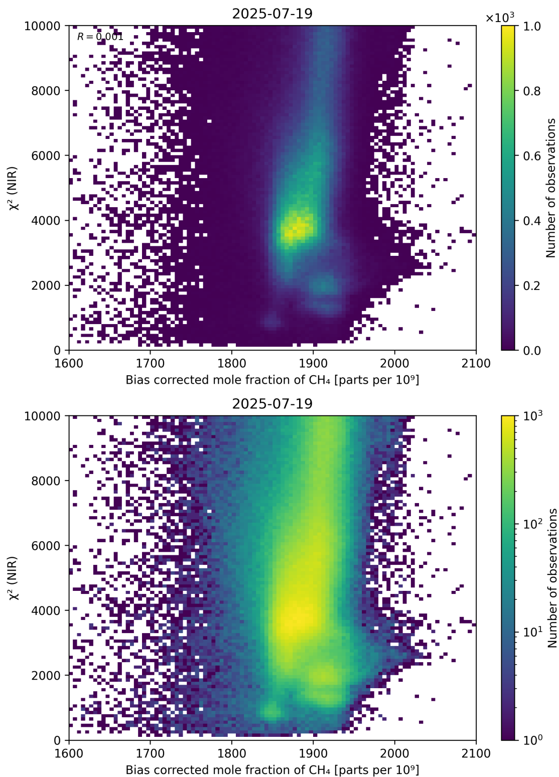
Figure 63: Scatter density plot of “Bias corrected mole fraction of CH 4 ” against “ \chi^2 (NIR)” for 2025-07-19 to 2025-07-20.
