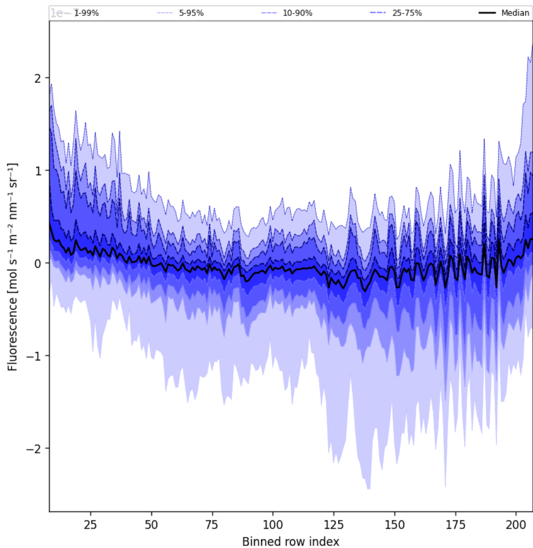
Figure 43: Along track statistics of “Fluorescence” for 2025-07-19 to 2025-07-20
