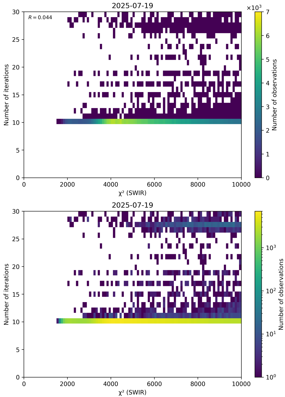
Figure 50: Scatter density plot of “ \chi^2 (SWIR)” against “Number of iterations” for 2025-07-19 to 2025-07-20.
