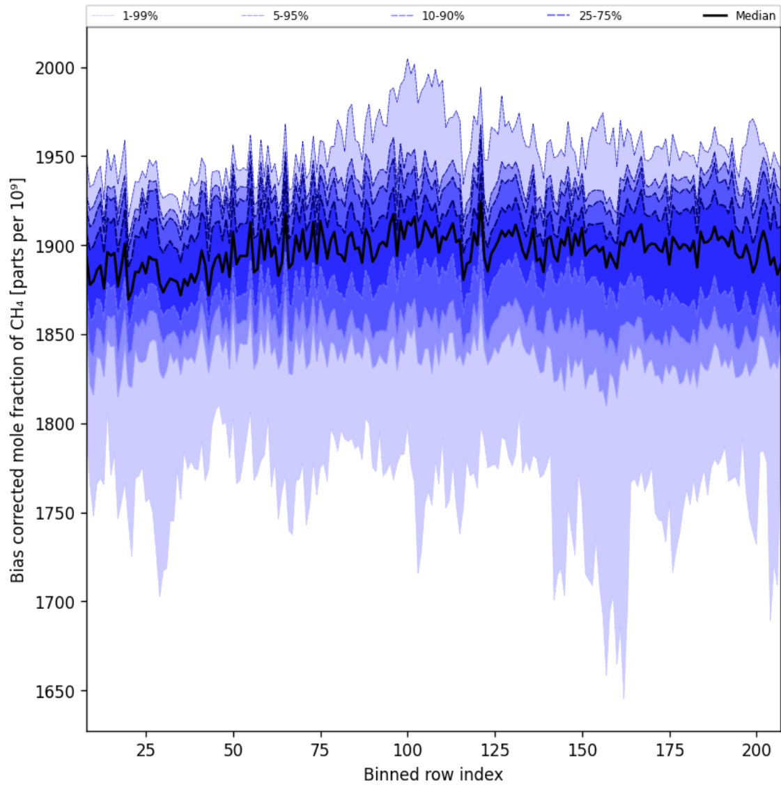
Figure 36: Along track statistics of “Bias corrected mole fraction of CH 4 ” for 2025-07-19 to 2025-07-20
