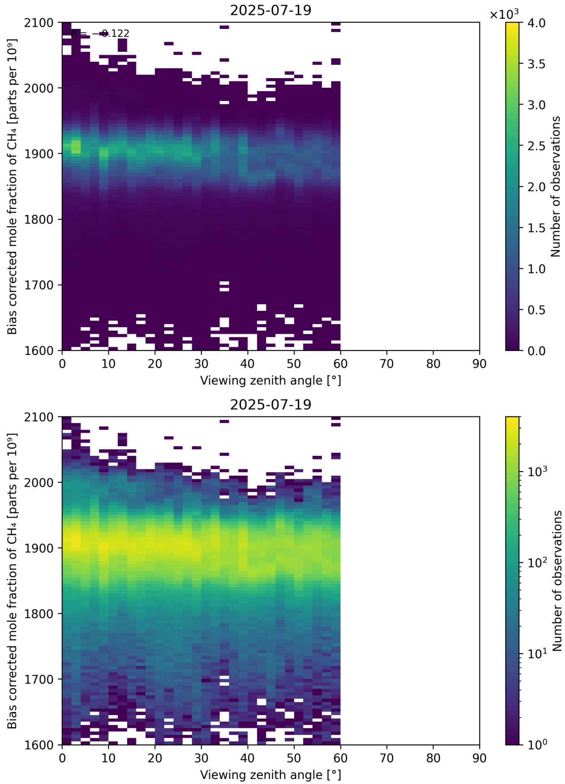
Figure 111: Scatter density plot of “Viewing zenith angle” against “Bias corrected mole fraction of CH 4 ” for 2025-07-19 to 2025-07-20.
