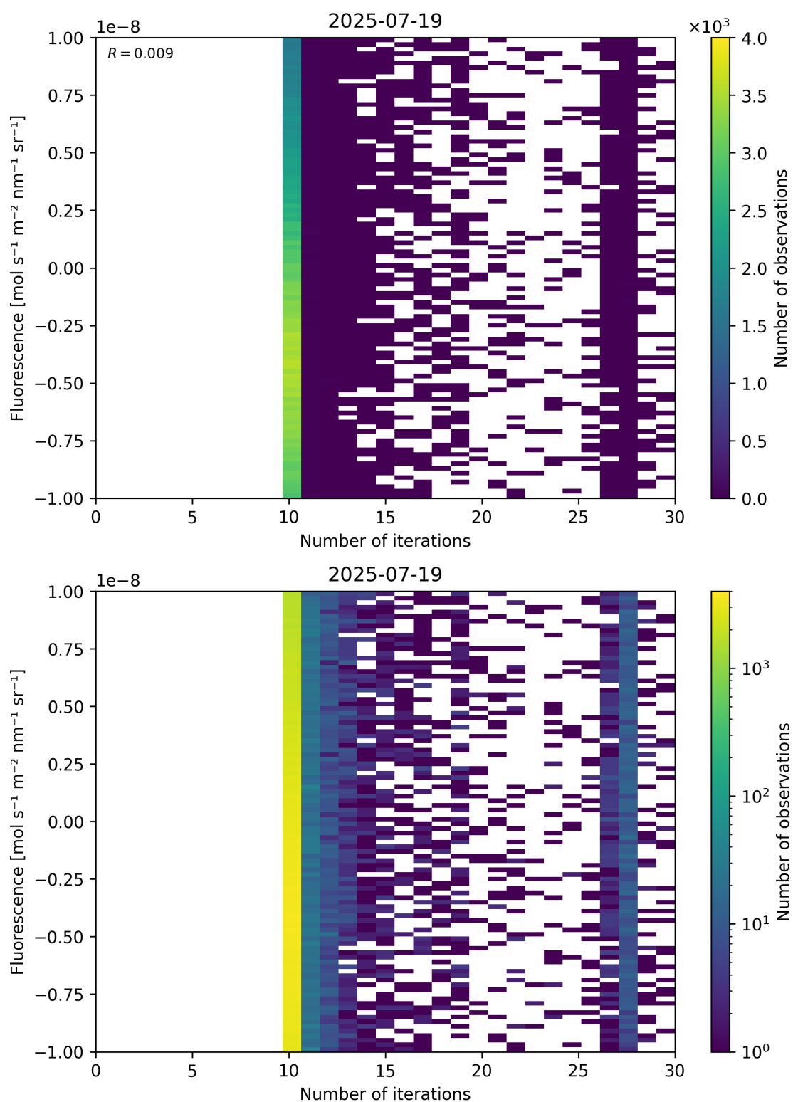
Figure 87: Scatter density plot of “Number of iterations” against “Fluorescence” for 2025-07-19 to 2025-07-20.
