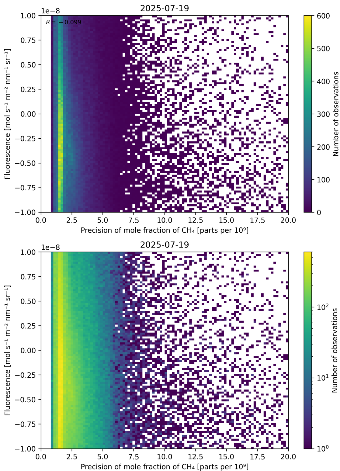
Figure 81: Scatter density plot of “Precision of mole fraction of CH 4 ” against “Fluorescence” for 2025-07-19 to 2025-07-20.
