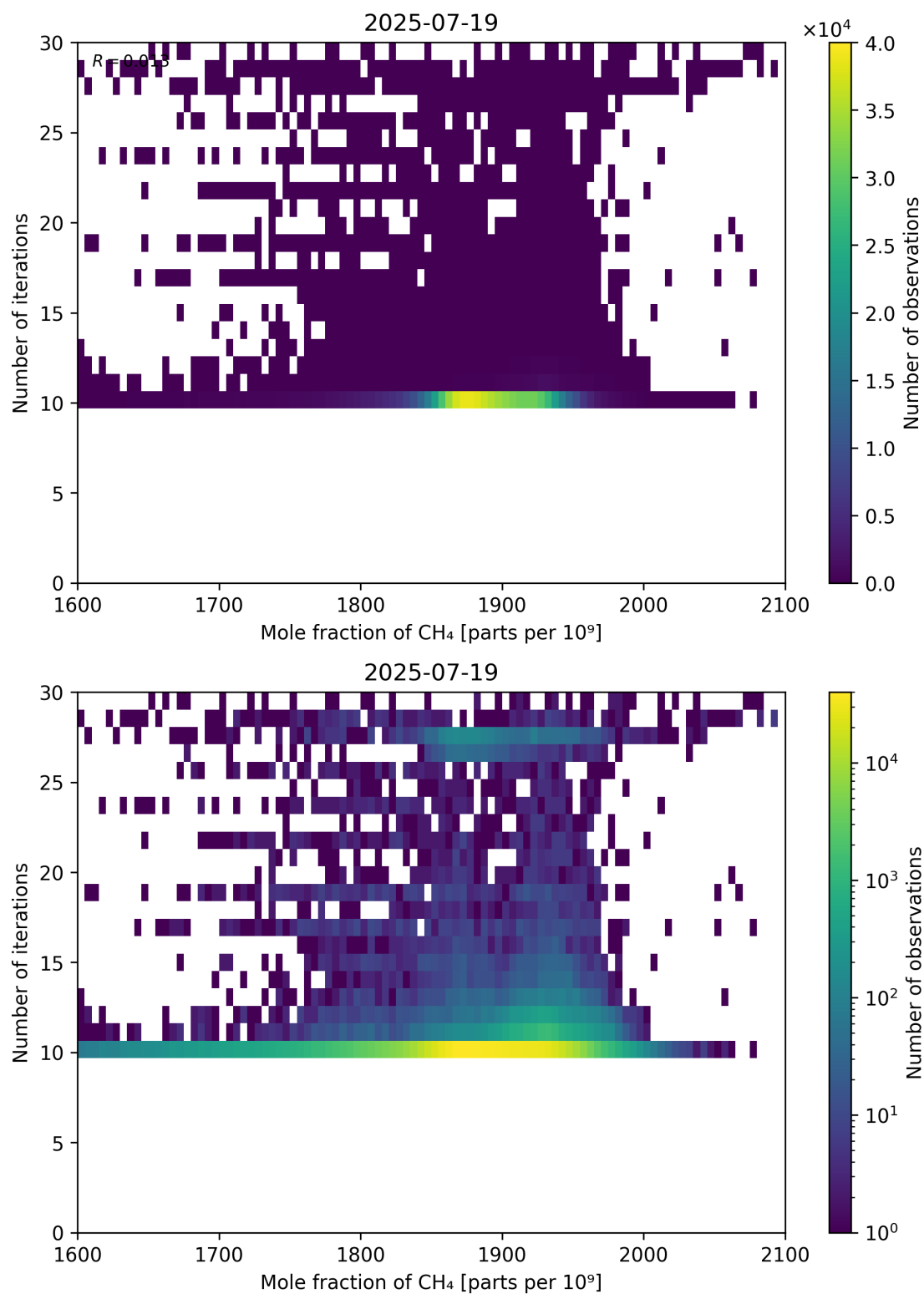
Figure 76: Scatter density plot of “Mole fraction of CH 4 ” against “Number of iterations” for 2025-07-19 to 2025-07-20.
