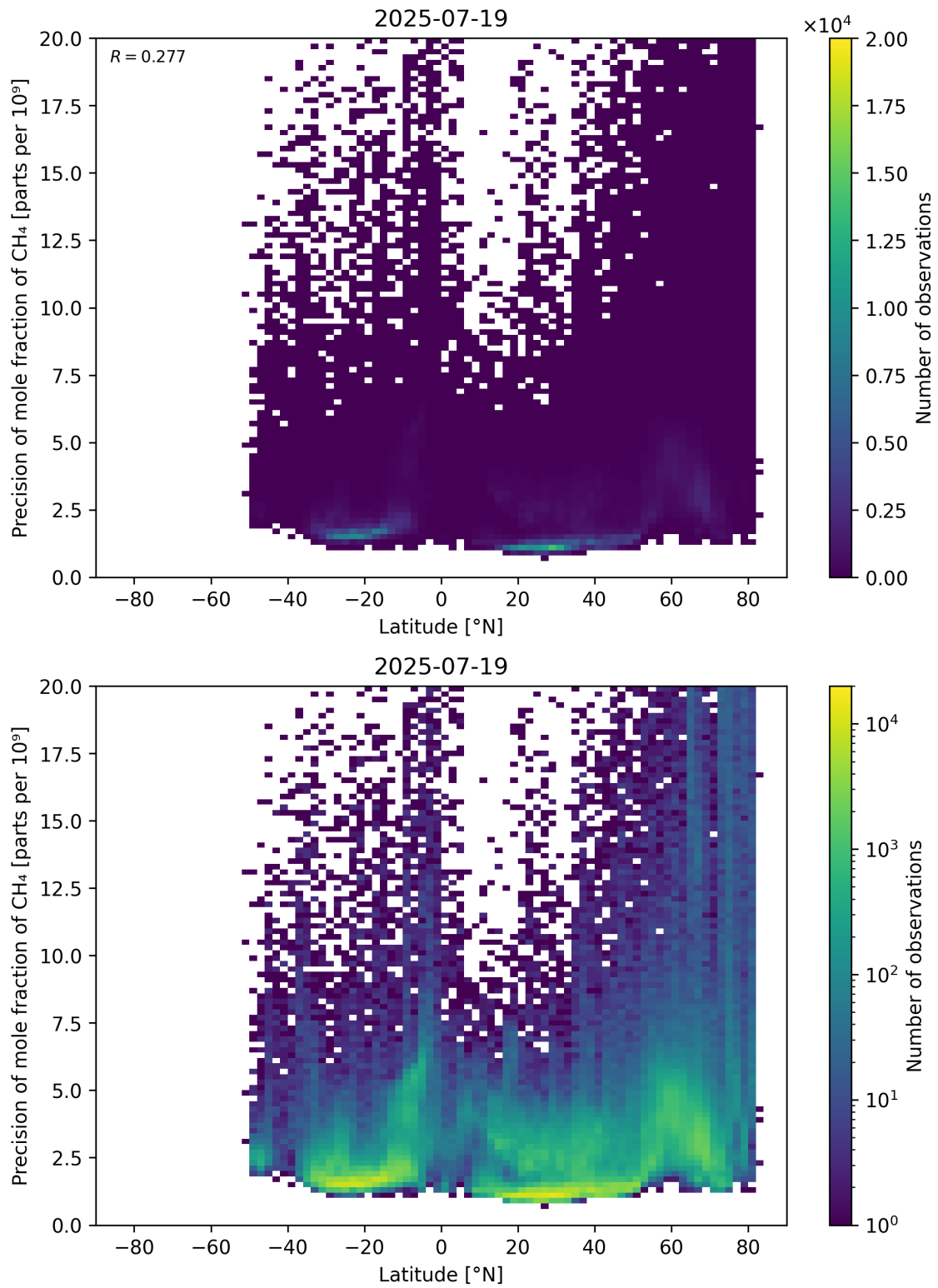
Figure 59: Scatter density plot of “Latitude” against “Precision of mole fraction of \text{CH}_4 ” for 2025-07-19 to 2025-07-20.
