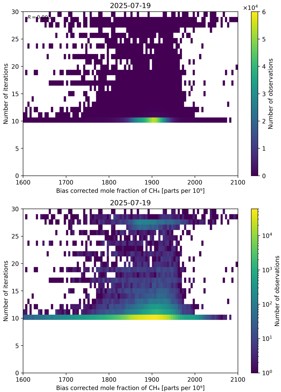
Figure 67: Scatter density plot of “Bias corrected mole fraction of \text{CH}_4 ” against “Number of iterations” for 2025-07-19 to 2025-07-20.
