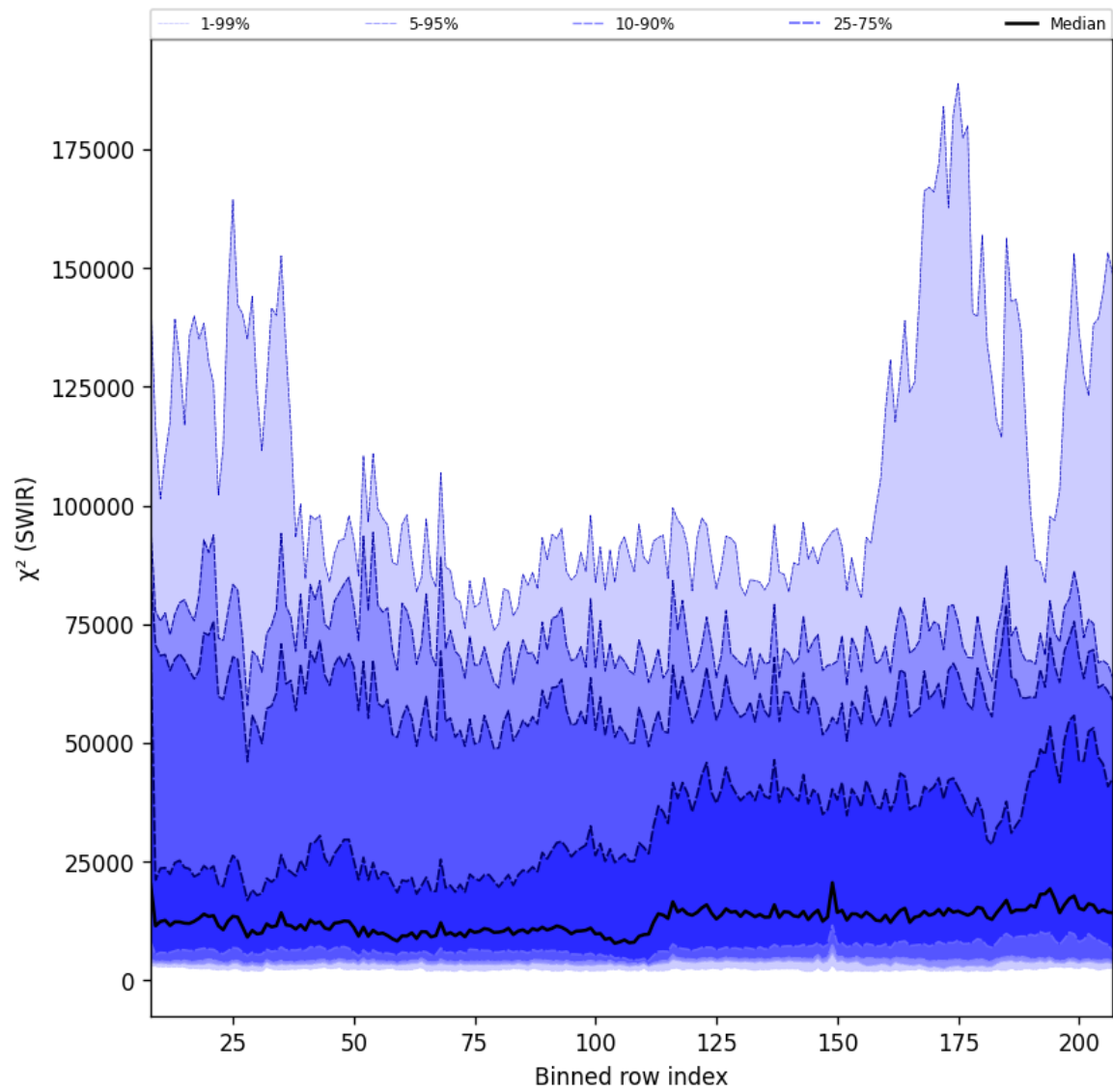
Figure 39: Along track statistics of “ \chi^2 (SWIR)” for 2025-07-19 to 2025-07-20
