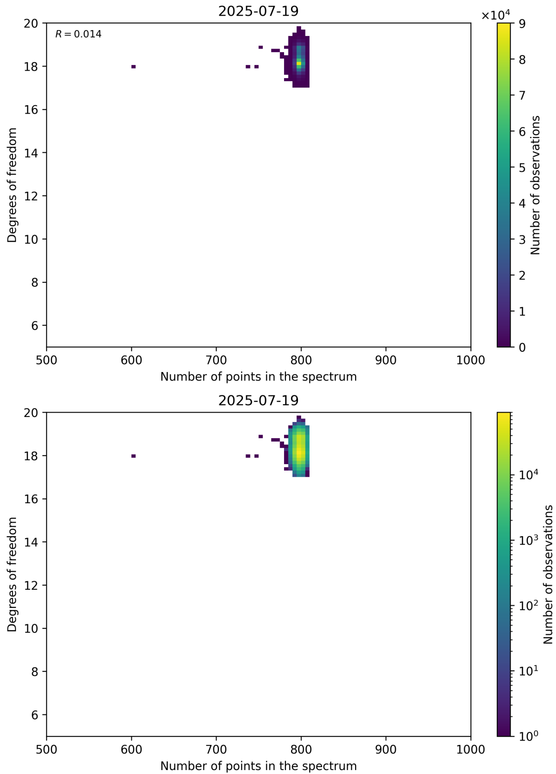
Figure 90: Scatter density plot of “Number of points in the spectrum” against “Degrees of freedom” for 2025-07-19 to 2025-07-20.
