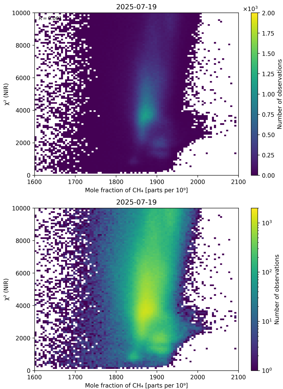
Figure 70: Scatter density plot of “Mole fraction of CH 4 ” against “ \chi^2 (NIR)” for 2025-07-19 to 2025-07-20.
