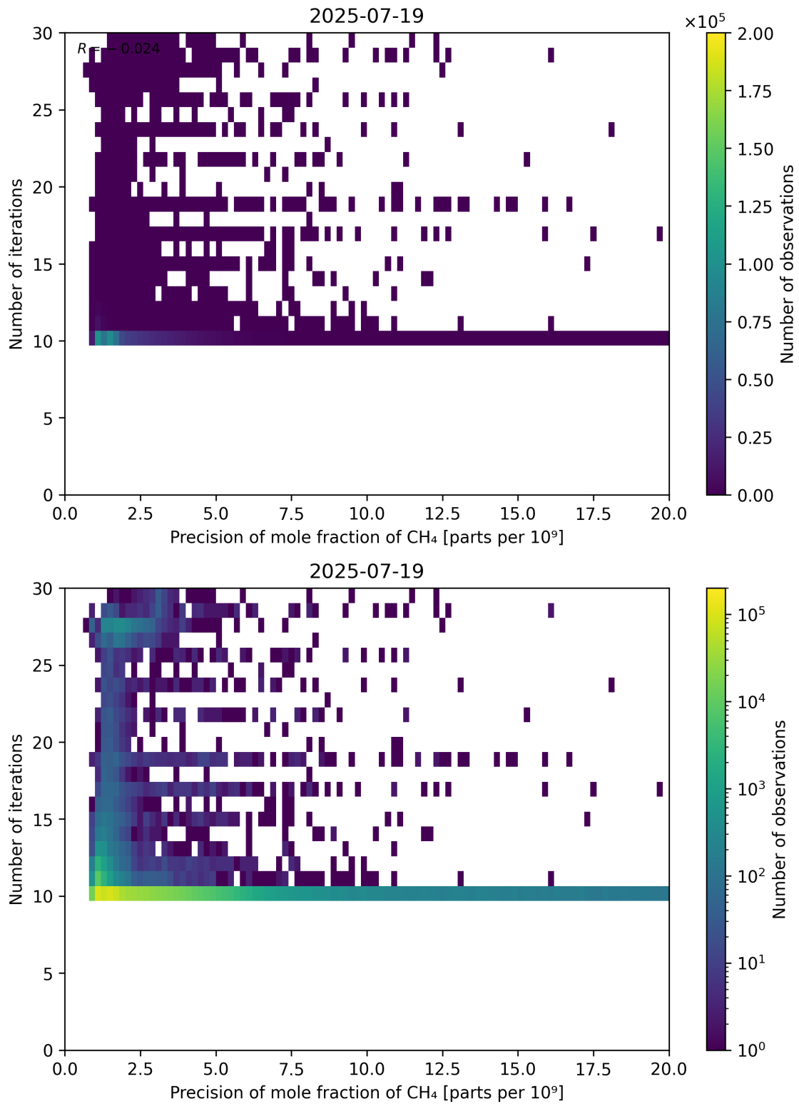
Figure 83: Scatter density plot of “Precision of mole fraction of CH 4 ” against “Number of iterations” for 2025-07-19 to 2025-07-20.
