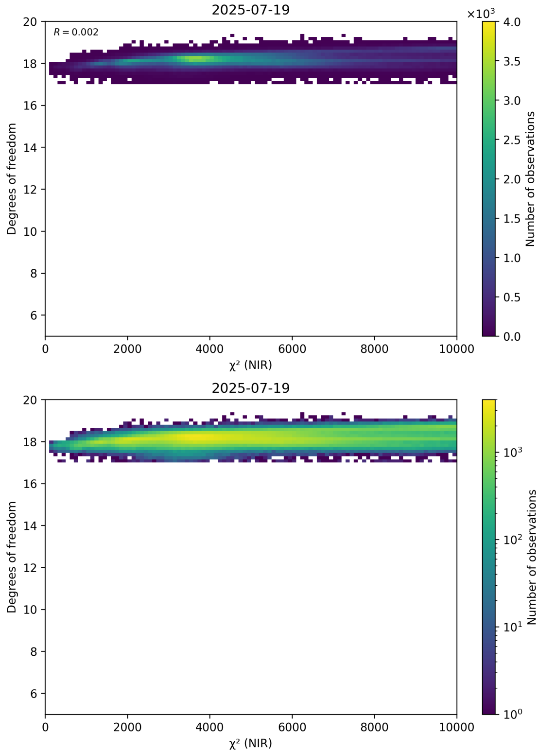
Figure 44: Scatter density plot of “ \chi^2 (NIR)” against “Degrees of freedom” for 2025-07-19 to 2025-07-20.
