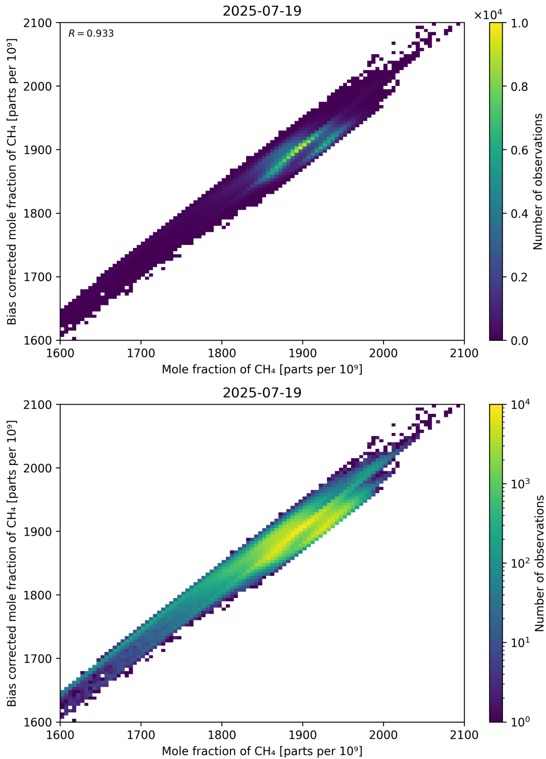
Figure 74: Scatter density plot of “Mole fraction of CH 4 ” against “Bias corrected mole fraction of CH 4 ” for 2025-07-19 to 2025-07-20.
