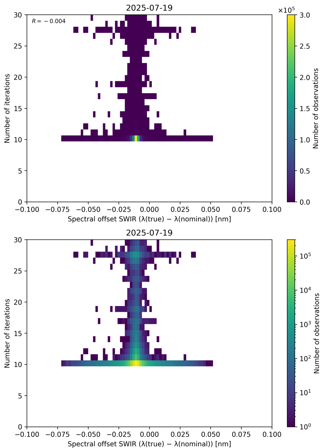
Figure 121: Scatter density plot of “Spectral offset SWIR ( \lambda_{\text{true}} - \lambda_{\text{nominal}} )” against “Number of iterations” for 2025-07-19 to 2025-07-20.
