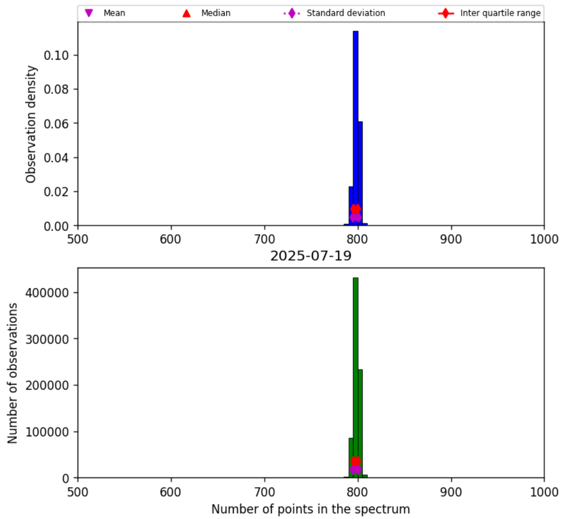
Figure 26: Histogram of “Number of points in the spectrum” for 2025-07-19 to 2025-07-20
