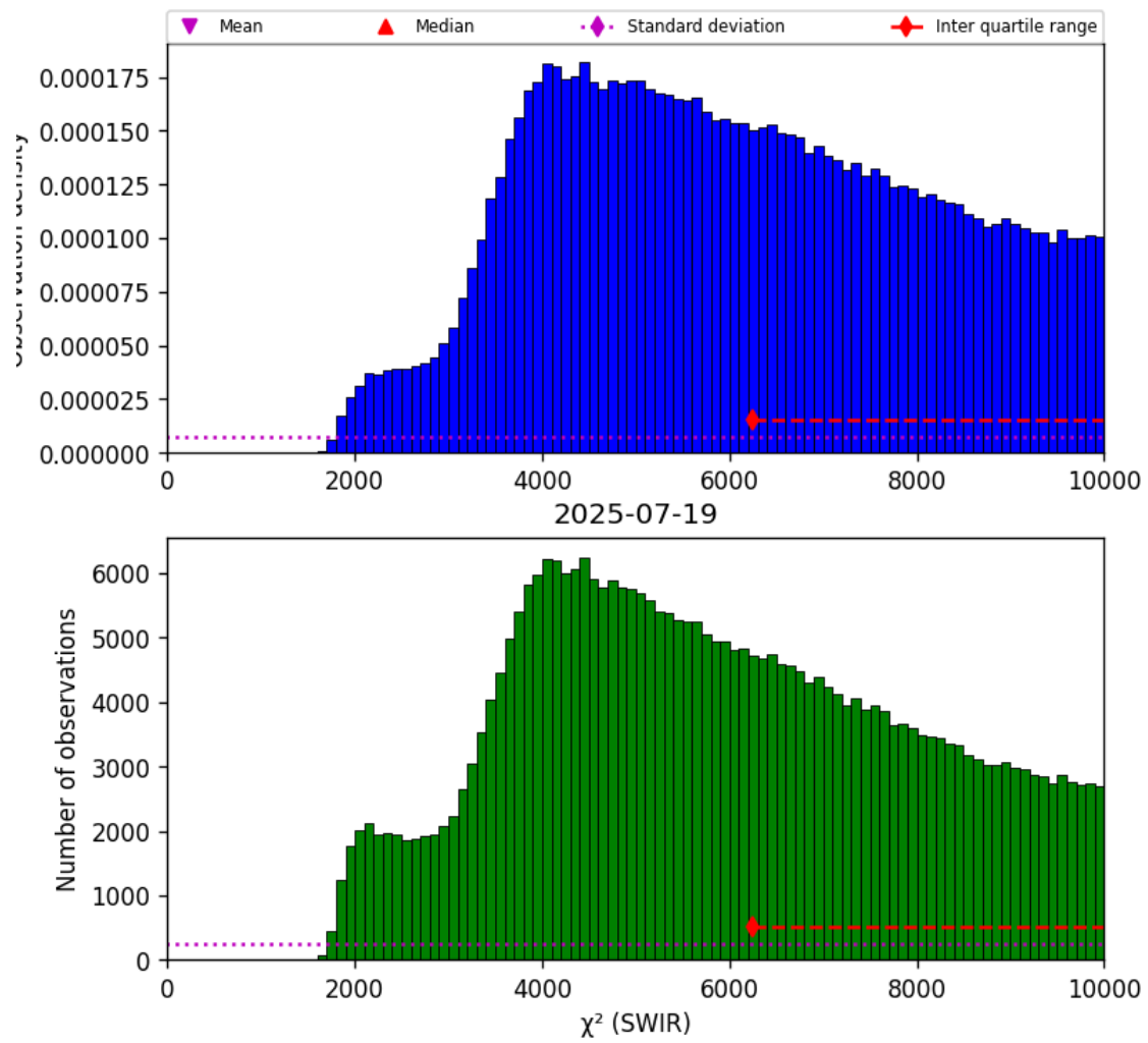
Figure 28: Histogram of “ \chi^2 (SWIR)” for 2025-07-19 to 2025-07-20
