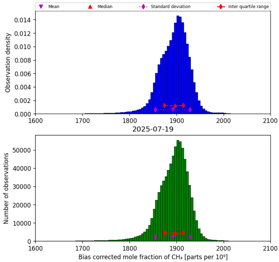
Figure 25: Histogram of “Bias corrected mole fraction of CH 4 ” for 2025-07-19 to 2025-07-20
