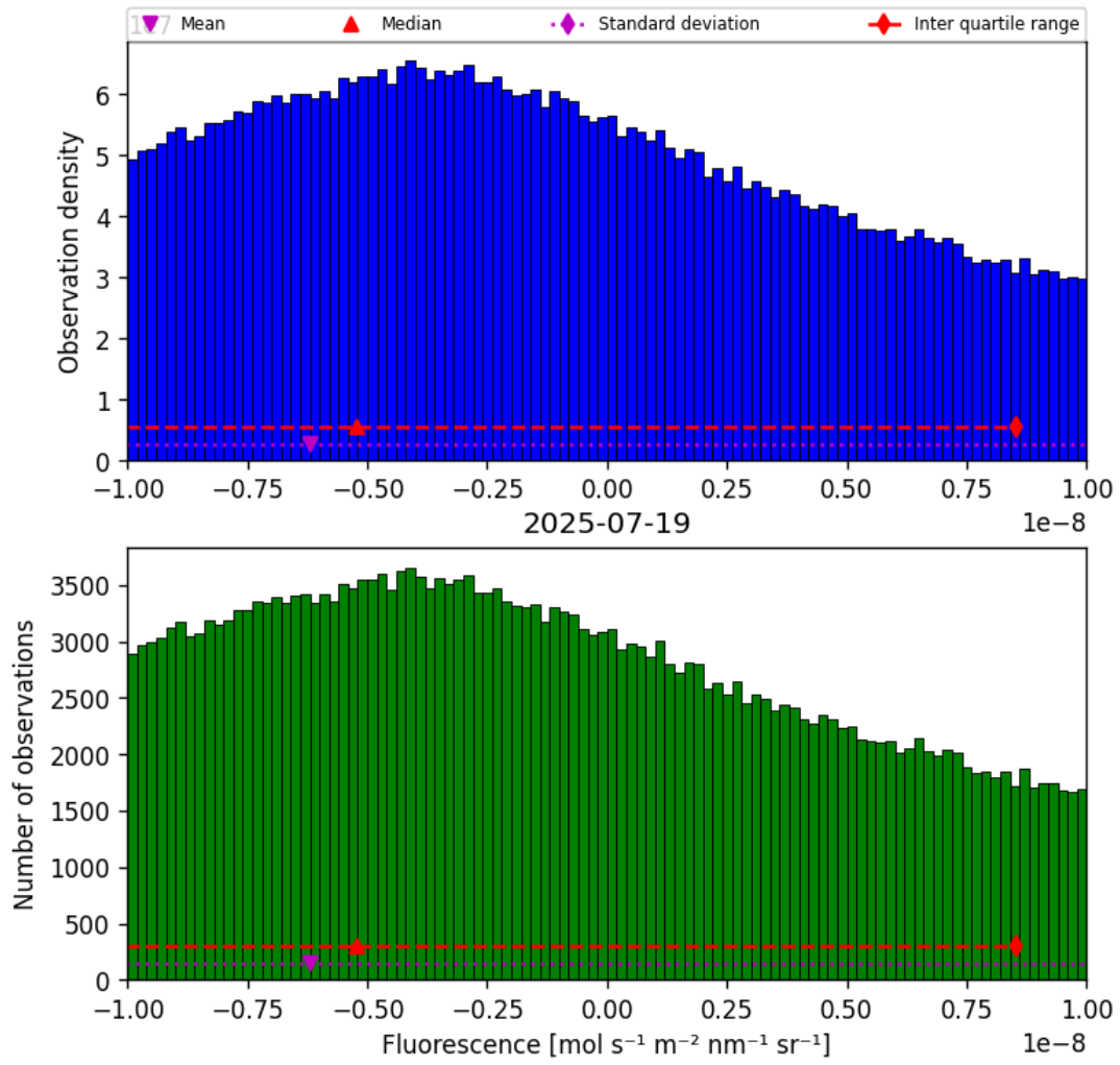
Figure 32: Histogram of “Fluorescence” for 2025-07-19 to 2025-07-20
