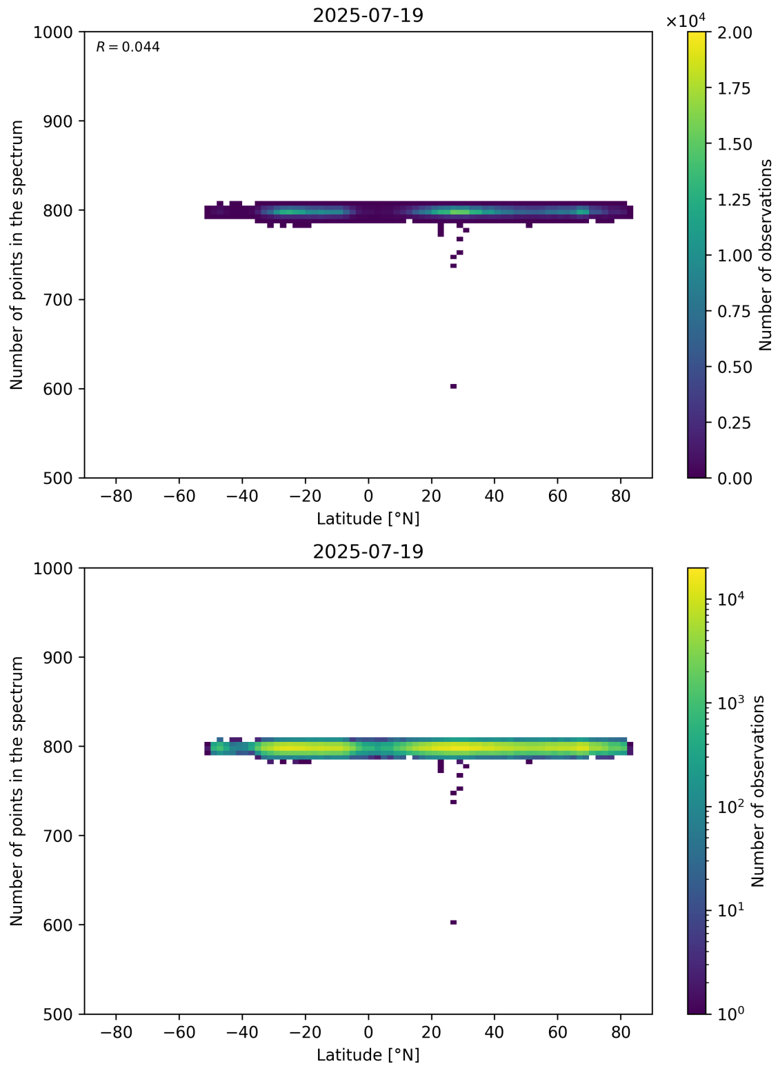
Figure 61: Scatter density plot of “Latitude” against “Number of points in the spectrum” for 2025-07-19 to 2025-07-20.
