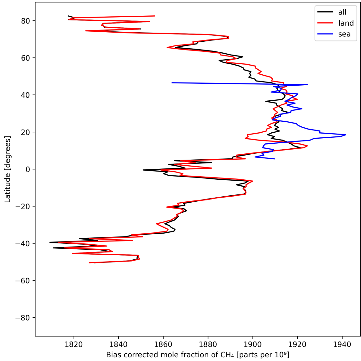
Figure 14: Zonal average of “Bias corrected mole fraction of CH 4 ” for 2025-07-19 to 2025-07-20.
