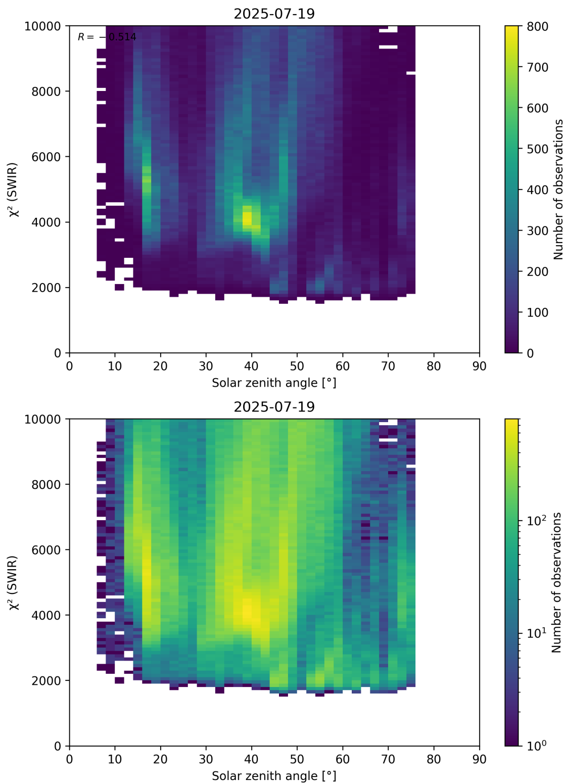
Figure 95: Scatter density plot of “Solar zenith angle” against “ \chi^2 (SWIR)” for 2025-07-19 to 2025-07-20.
