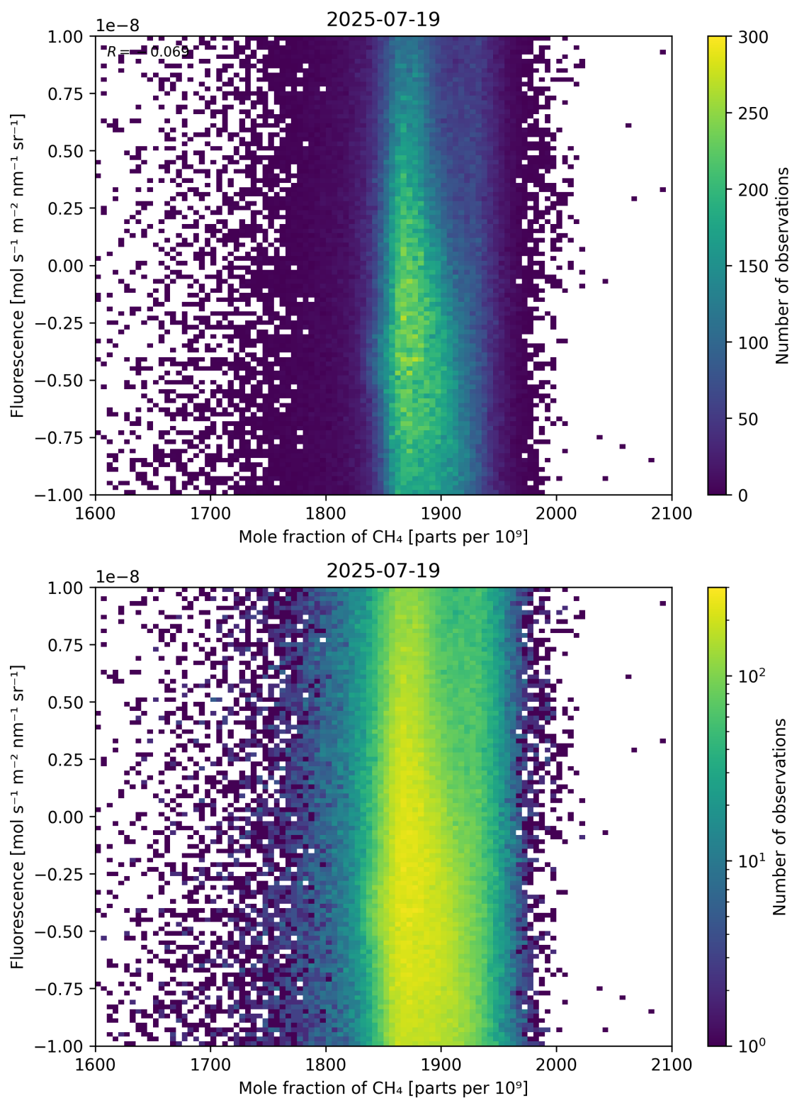
Figure 73: Scatter density plot of “Mole fraction of \text{CH}_4 ” against “Fluorescence” for 2025-07-19 to 2025-07-20.
