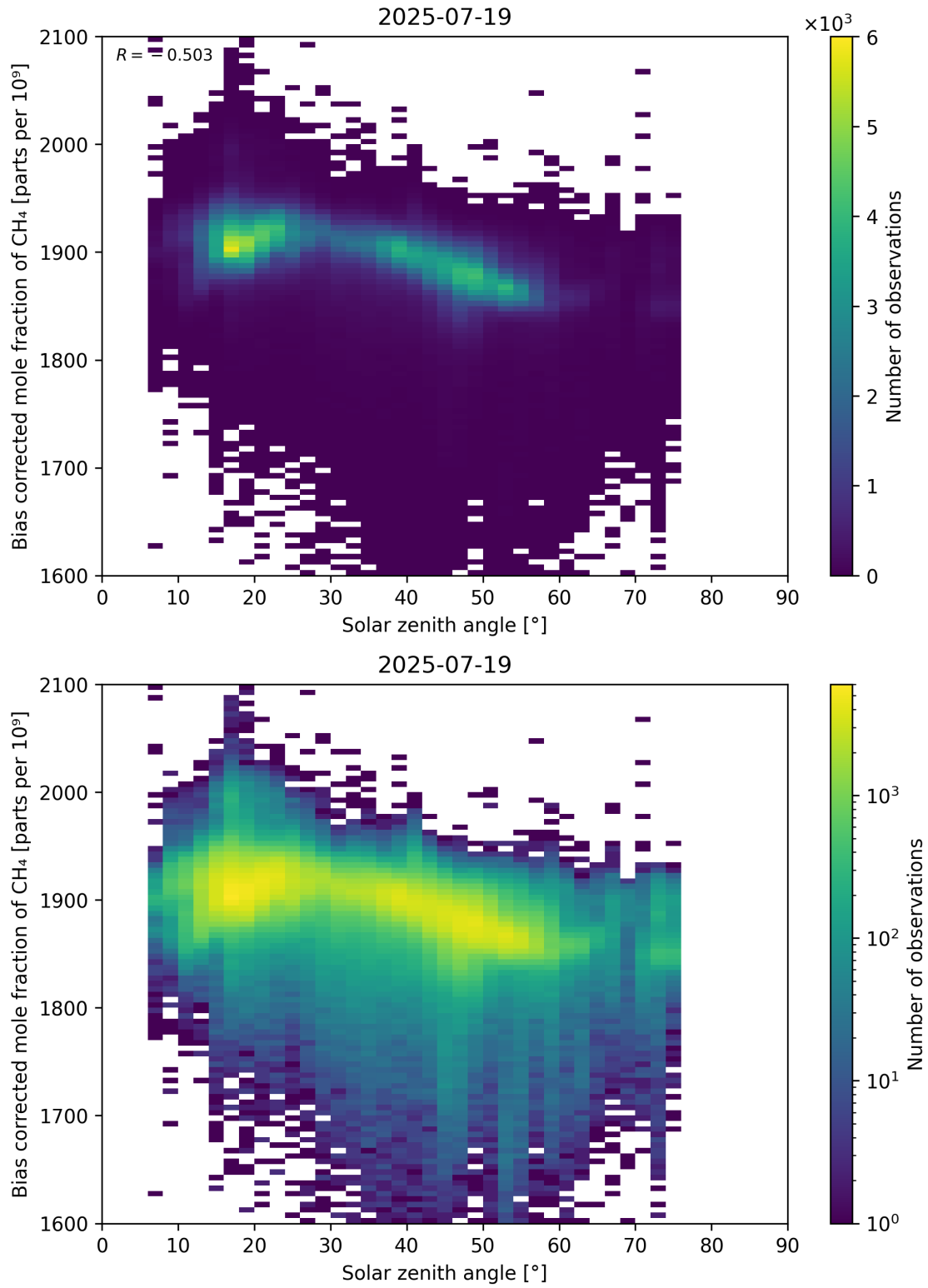
Figure 100: Scatter density plot of “Solar zenith angle” against “Bias corrected mole fraction of CH 4 ” for 2025-07-19 to 2025-07-20.
