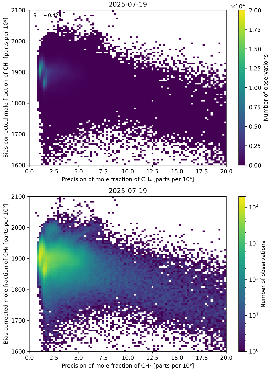
Figure 82: Scatter density plot of “Precision of mole fraction of CH 4 ” against “Bias corrected mole fraction of CH 4 ” for 2025-07-19 to 2025-07-20.
