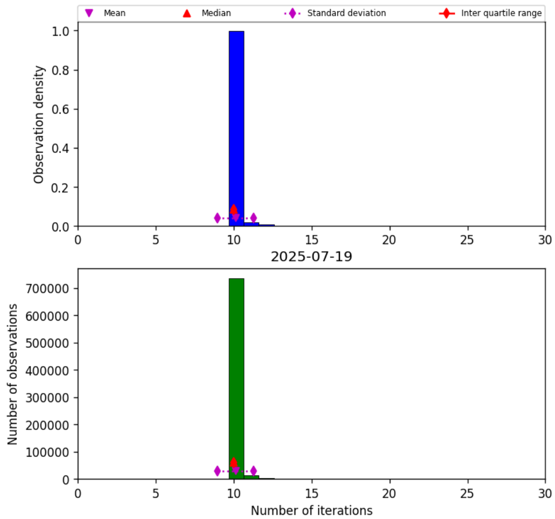
Figure 31: Histogram of “Number of iterations” for 2025-07-19 to 2025-07-20
