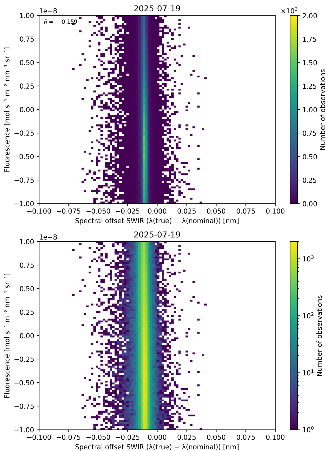
Figure 120: Scatter density plot of “Spectral offset SWIR ( \lambda_{\text{true}} - \lambda_{\text{nominal}} )” against “Fluorescence” for 2025-07-19 to 2025-07-20.
