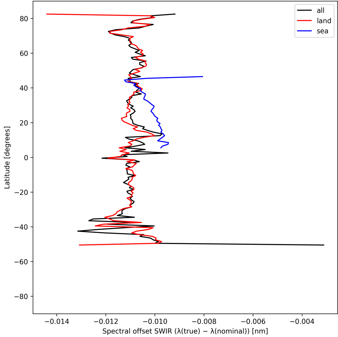
Figure 16: Zonal average of “Spectral offset SWIR ( \lambda_{\text{true}} - \lambda_{\text{nominal}} )” for 2025-07-19 to 2025-07-20.
