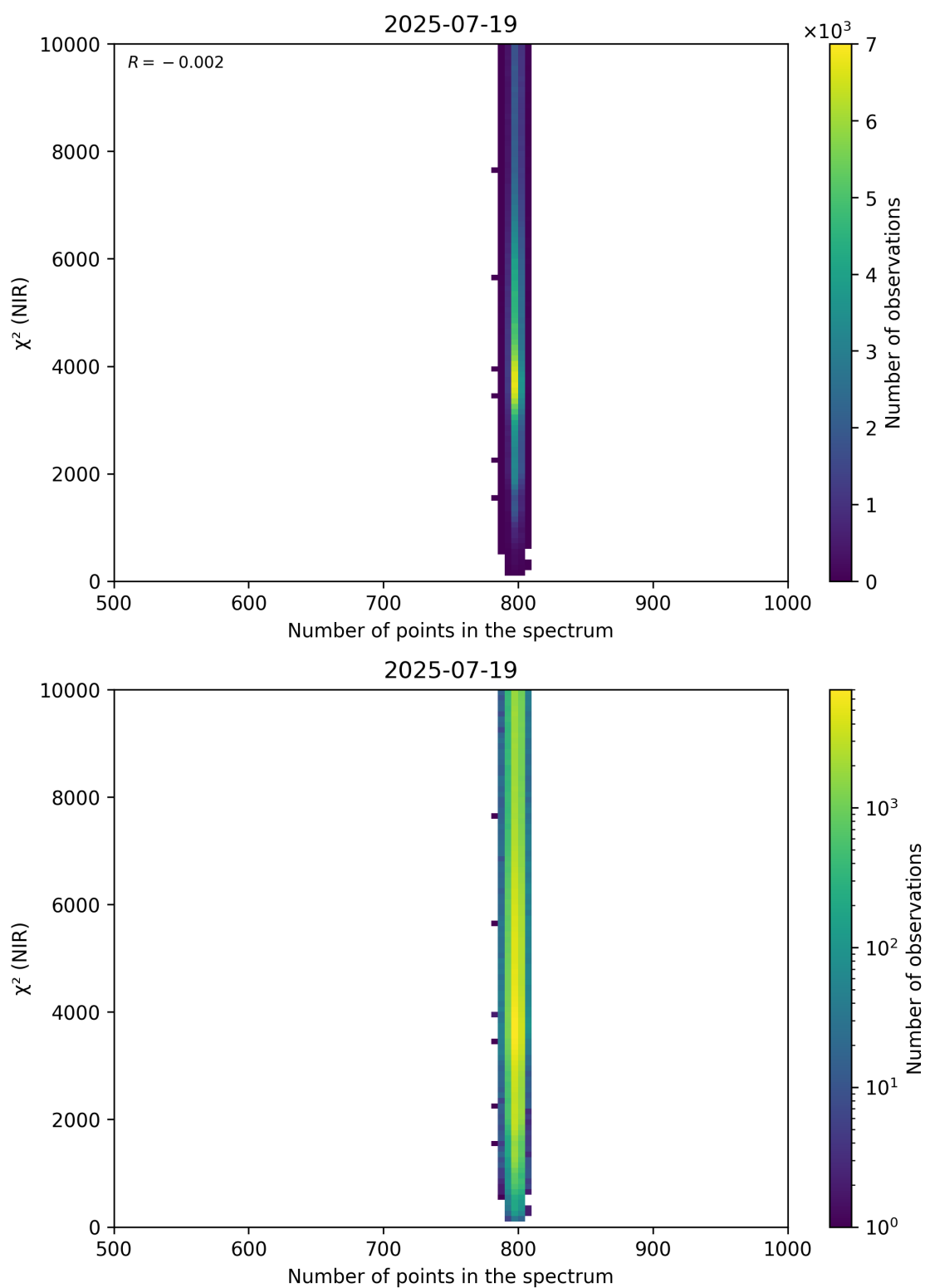
Figure 88: Scatter density plot of “Number of points in the spectrum” against “ \chi^2 (NIR)” for 2025-07-19 to 2025-07-20.
