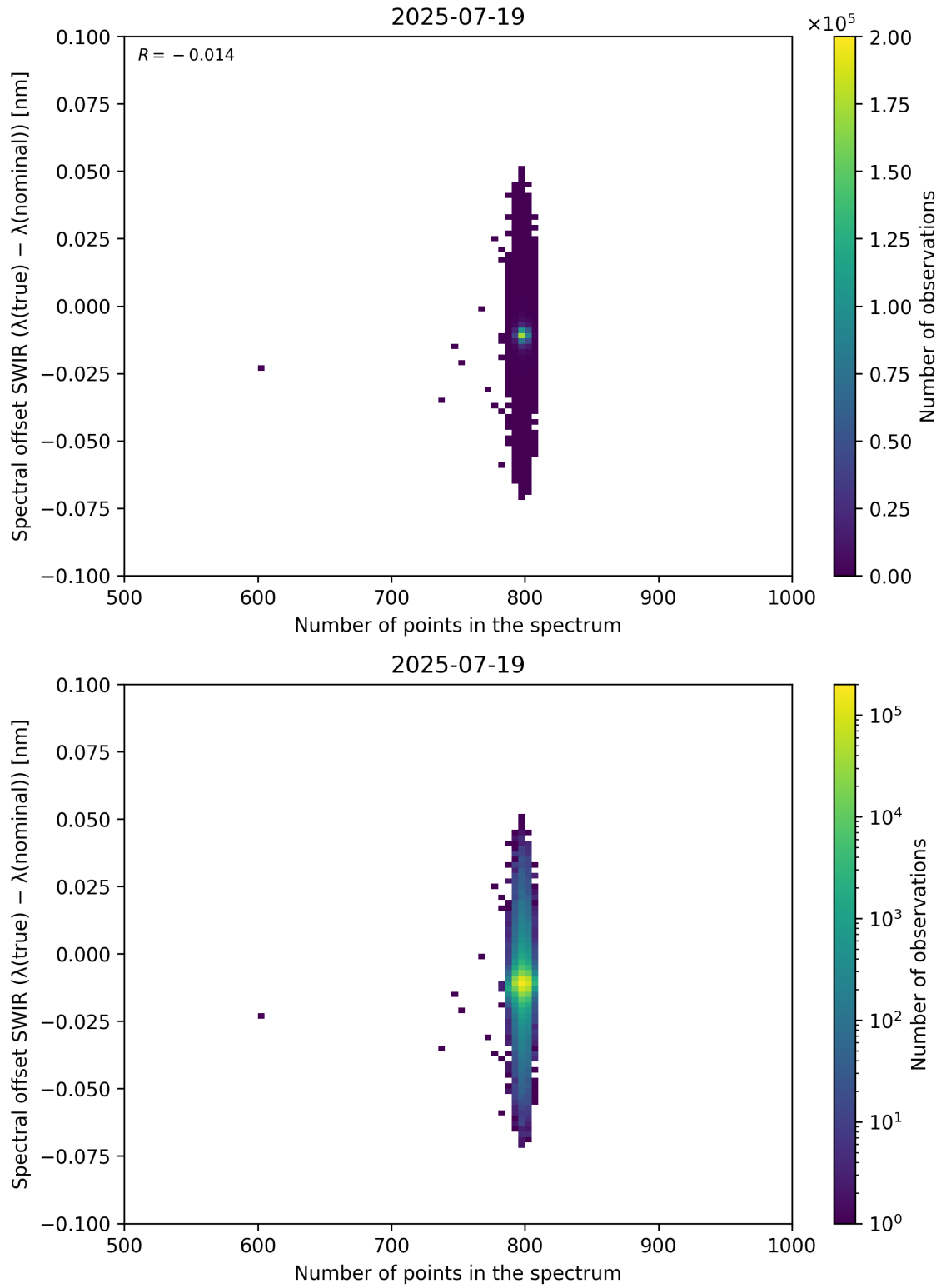
Figure 93: Scatter density plot of “Number of points in the spectrum” against “Spectral offset SWIR ( \lambda_{\text{true}} - \lambda_{\text{nominal}} )” for 2025-07-19 to 2025-07-20.
