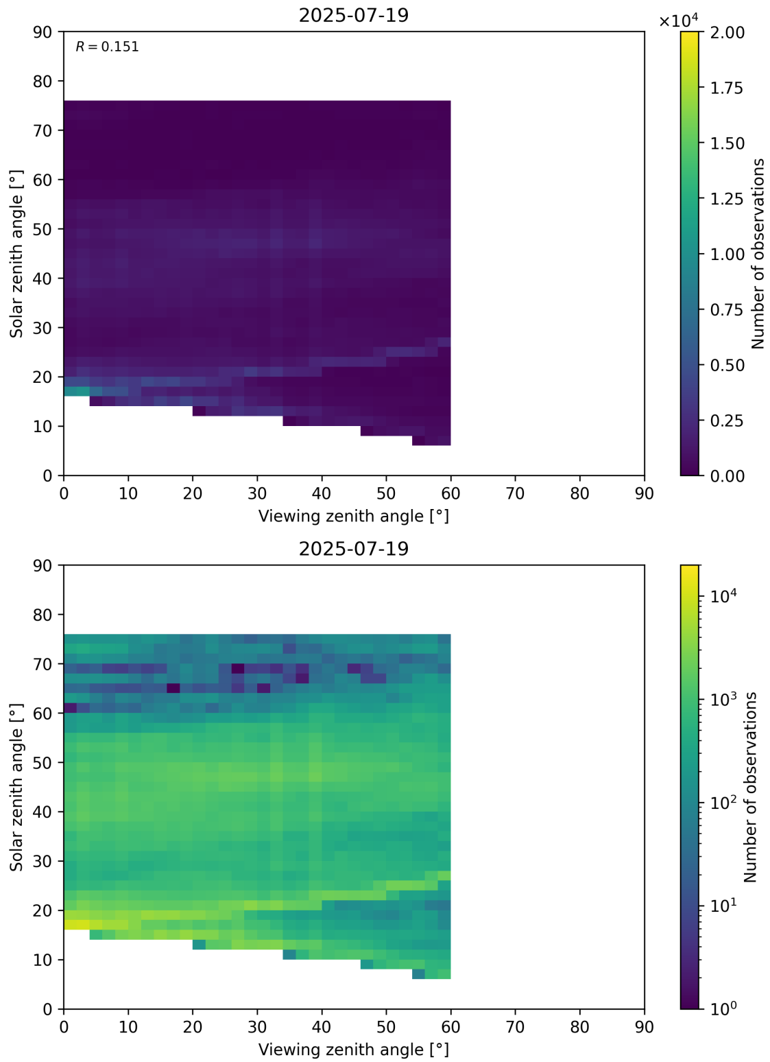
Figure 115: Scatter density plot of “Viewing zenith angle” against “Solar zenith angle” for 2025-07-19 to 2025-07-20.
