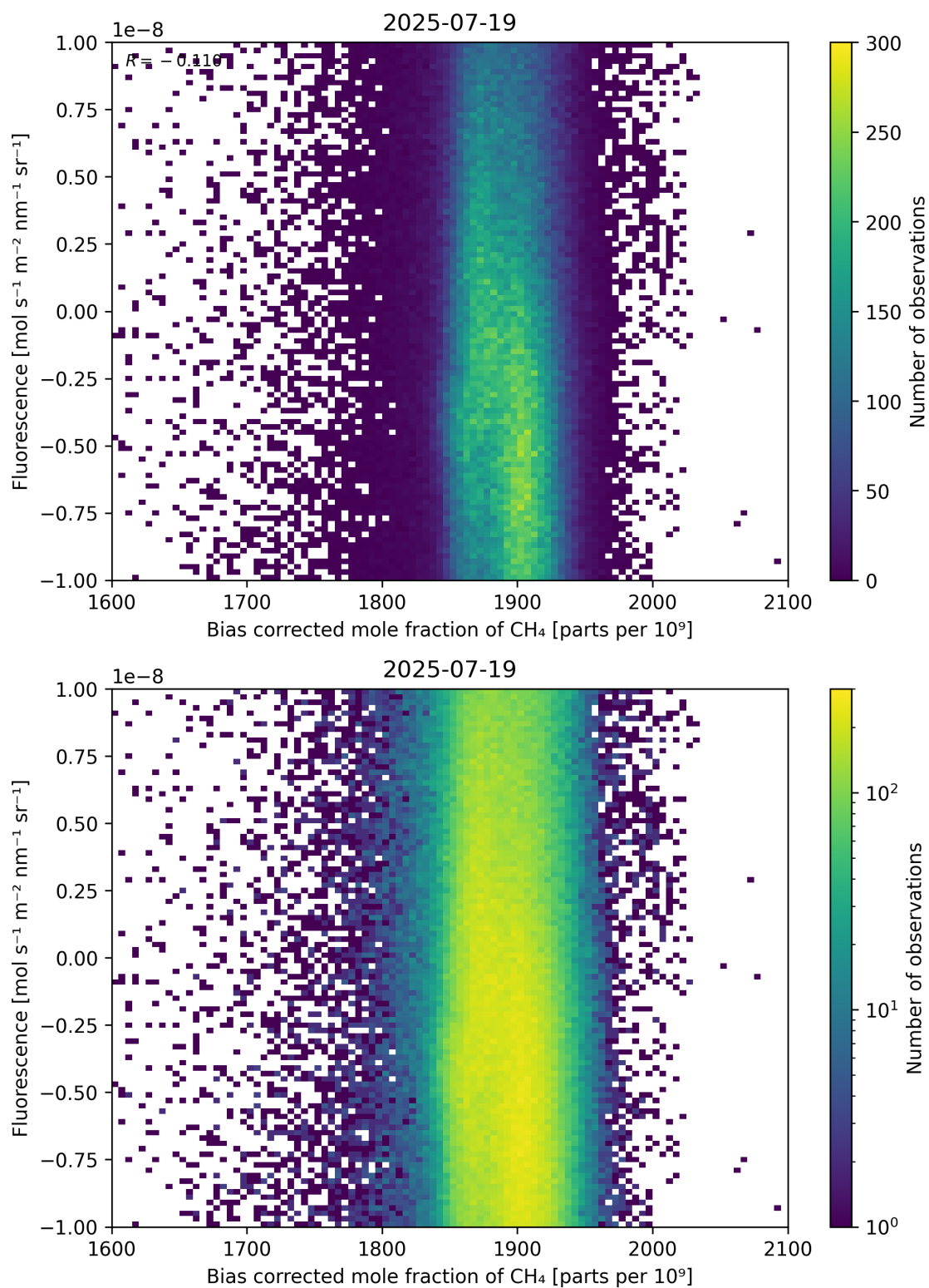
Figure 66: Scatter density plot of “Bias corrected mole fraction of \text{CH}_4 ” against “Fluorescence” for 2025-07-19 to 2025-07-20.
