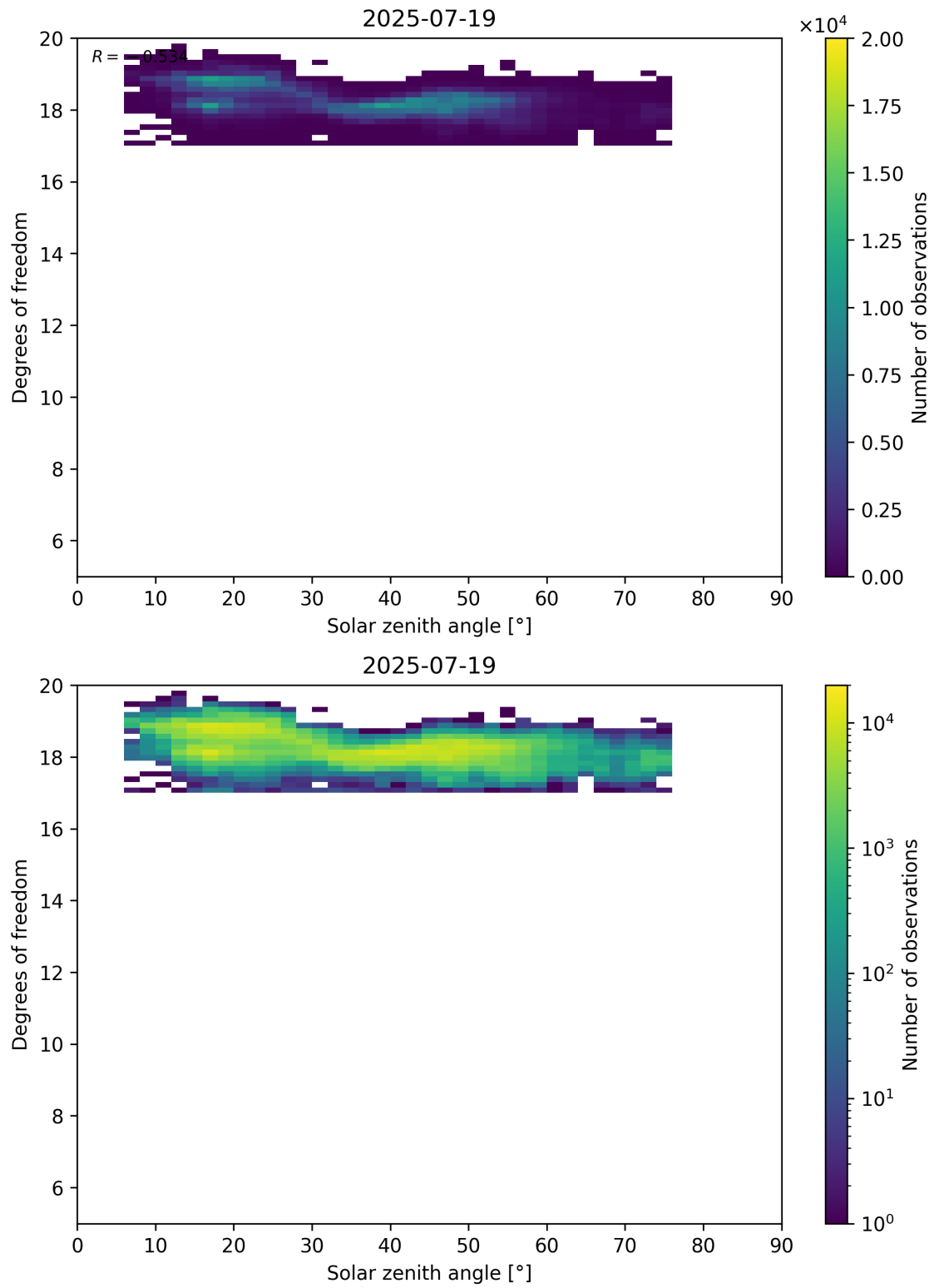
Figure 96: Scatter density plot of “Solar zenith angle” against “Degrees of freedom” for 2025-07-19 to 2025-07-20.
