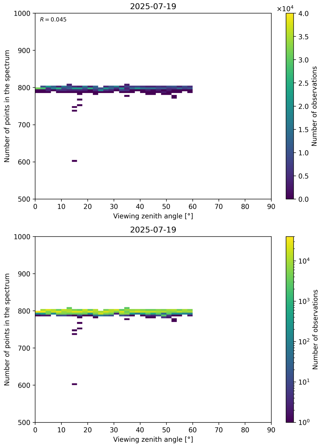
Figure 114: Scatter density plot of “Viewing zenith angle” against “Number of points in the spectrum” for 2025-07-19 to 2025-07-20.
