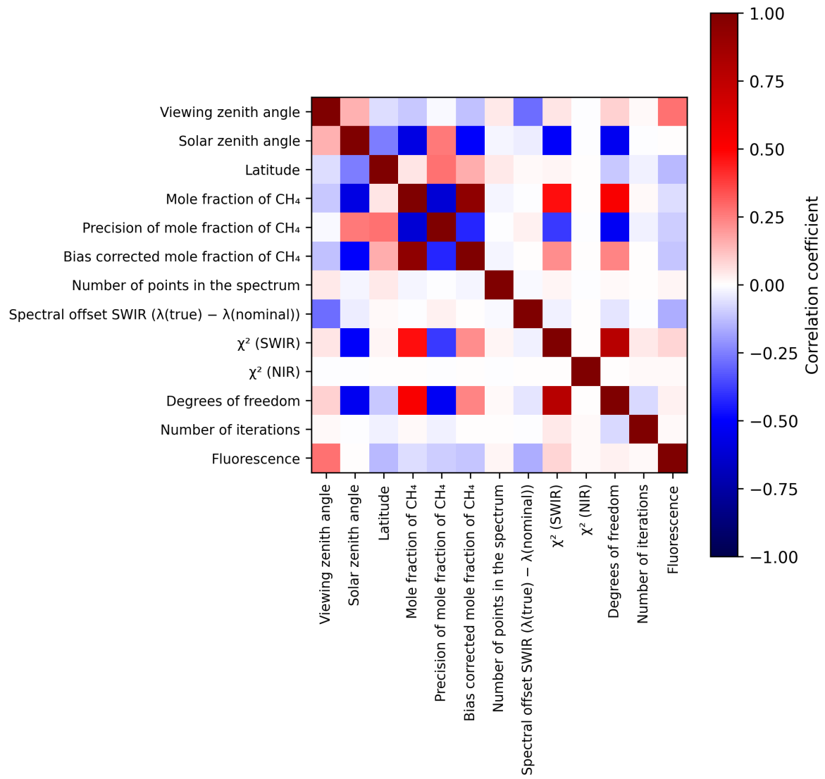
Figure 2: Map of correlation matrix for 2025-07-19 to 2025-07-20.
