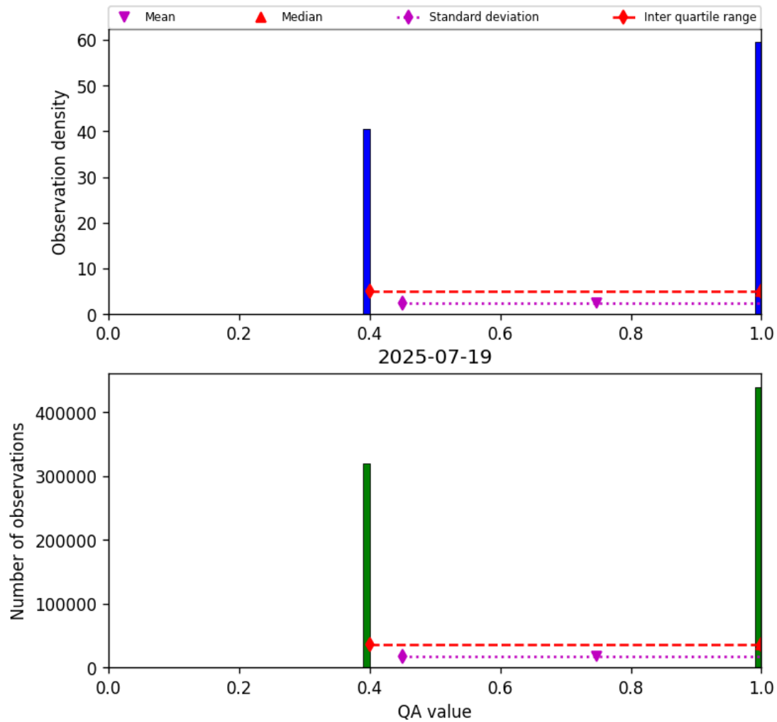
Figure 22: Histogram of “QA value” for 2025-07-19 to 2025-07-20
