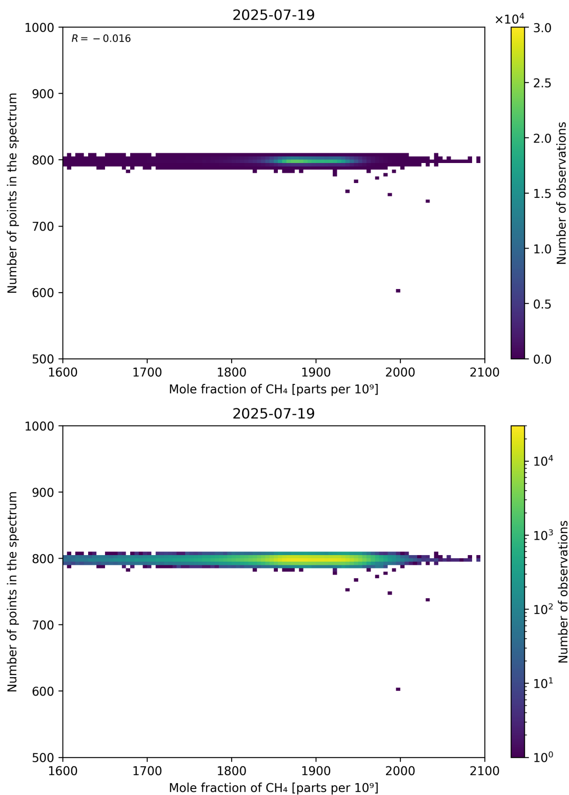
Figure 77: Scatter density plot of “Mole fraction of CH 4 ” against “Number of points in the spectrum” for 2025-07-19 to 2025-07-20.
