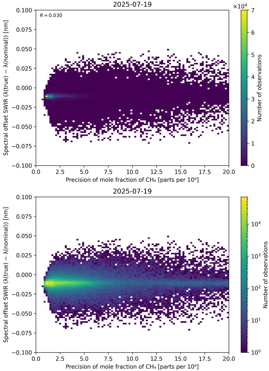
Figure 85: Scatter density plot of “Precision of mole fraction of \text{CH}_4 ” against “Spectral offset SWIR ( \lambda_{\text{true}} - \lambda_{\text{nominal}} )” for 2025-07-19 to 2025-07-20.
