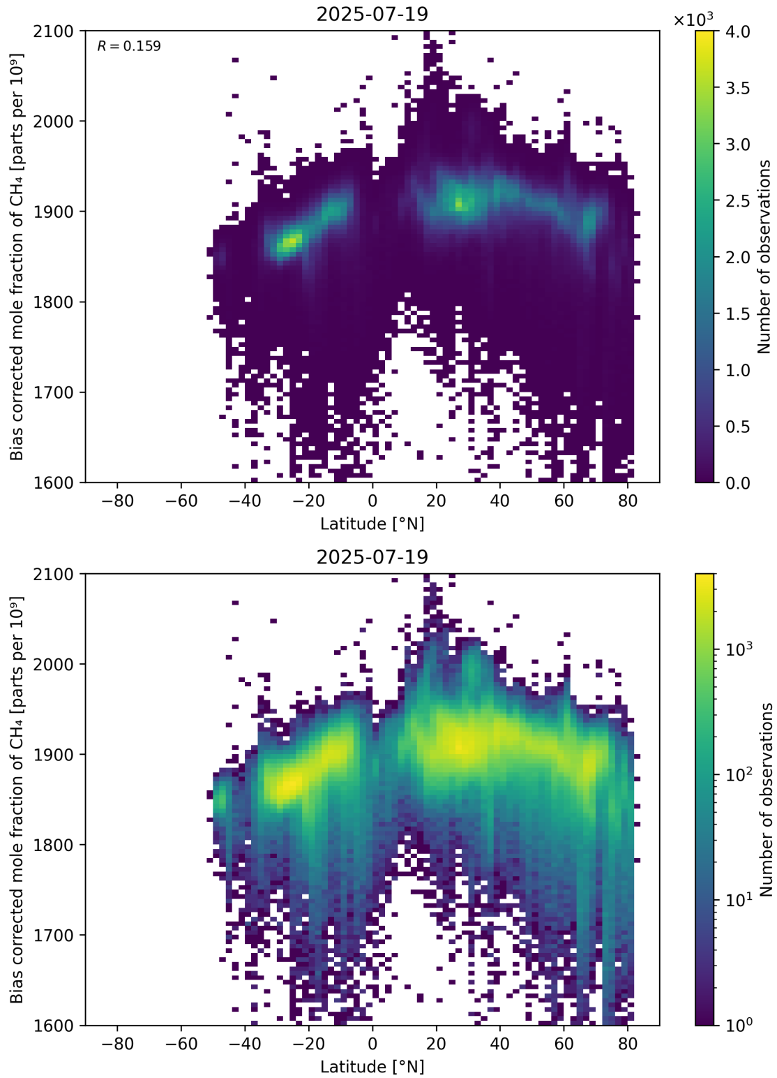
Figure 58: Scatter density plot of “Latitude” against “Bias corrected mole fraction of CH 4 ” for 2025-07-19 to 2025-07-20.
