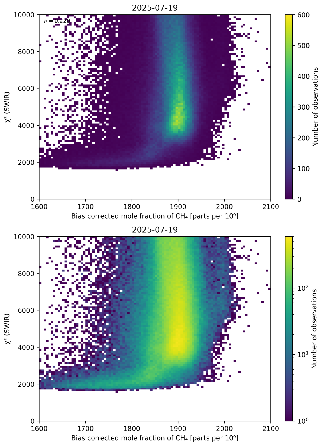
Figure 64: Scatter density plot of “Bias corrected mole fraction of \text{CH}_4 ” against “ \chi^2 (SWIR)” for 2025-07-19 to 2025-07-20.
