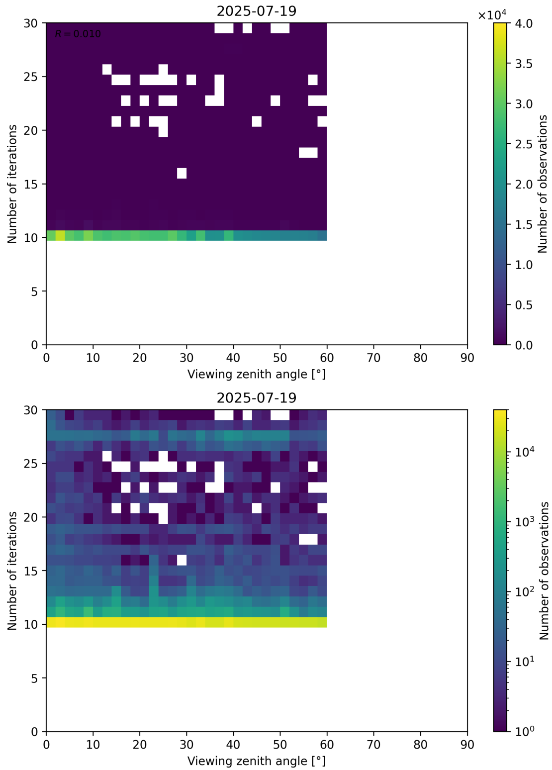
Figure 113: Scatter density plot of “Viewing zenith angle” against “Number of iterations” for 2025-07-19 to 2025-07-20.
