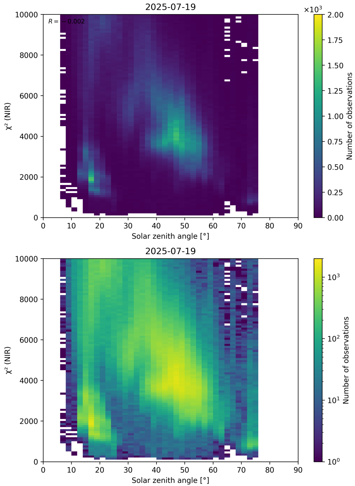
Figure 94: Scatter density plot of “Solar zenith angle” against “ \chi^2 (NIR)” for 2025-07-19 to 2025-07-20.
