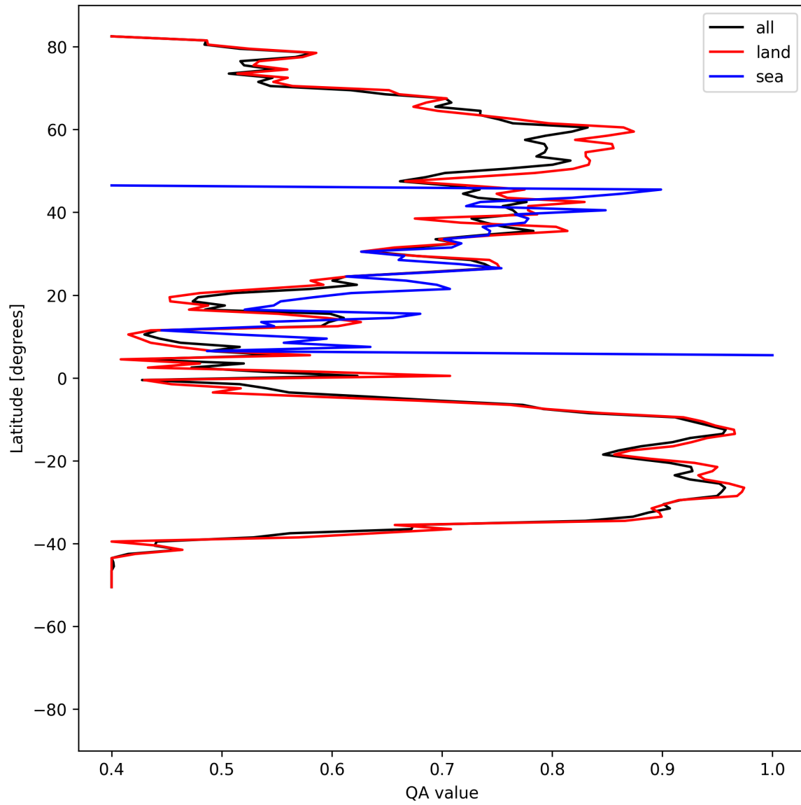
Figure 11: Zonal average of “QA value” for 2025-07-19 to 2025-07-20.
