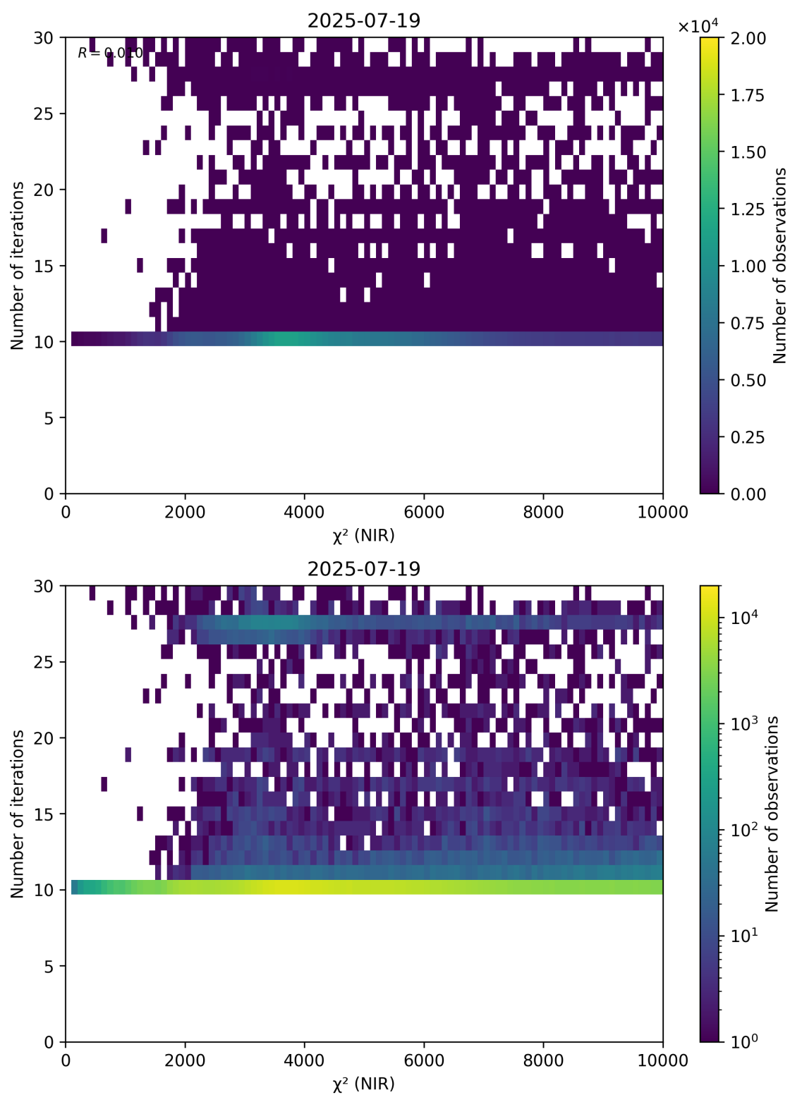
Figure 46: Scatter density plot of “ \chi^2 (NIR)” against “Number of iterations” for 2025-07-19 to 2025-07-20.
