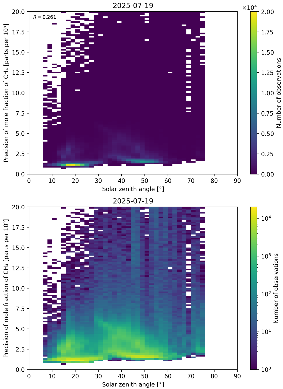
Figure 101: Scatter density plot of “Solar zenith angle” against “Precision of mole fraction of CH 4 ” for 2025-07-19 to 2025-07-20.
