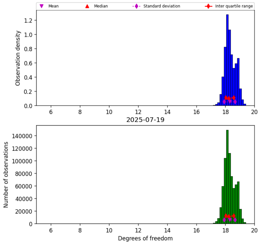
Figure 30: Histogram of “Degrees of freedom” for 2025-07-19 to 2025-07-20
