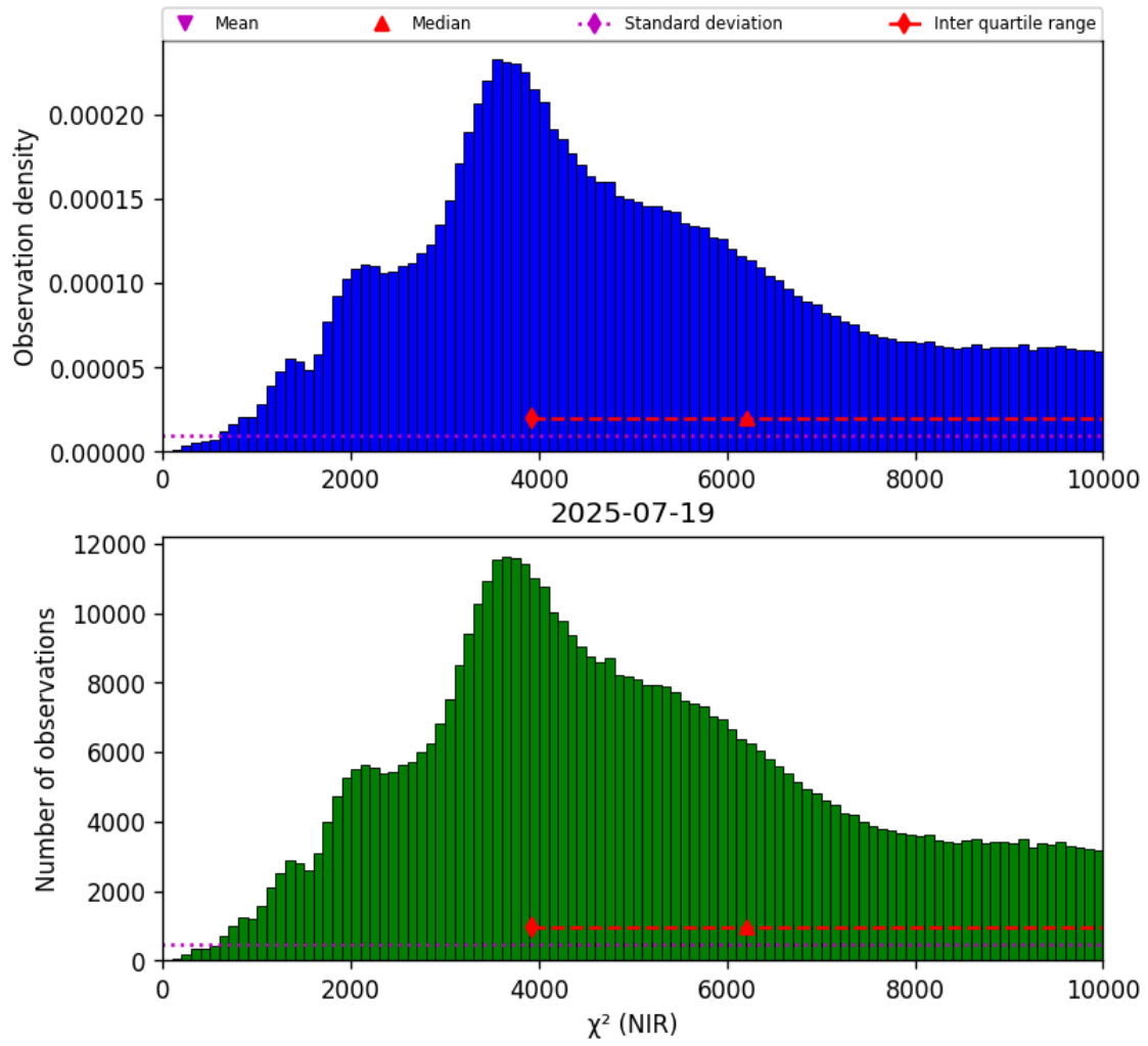
Figure 29: Histogram of “ \chi^2 (NIR)” for 2025-07-19 to 2025-07-20
