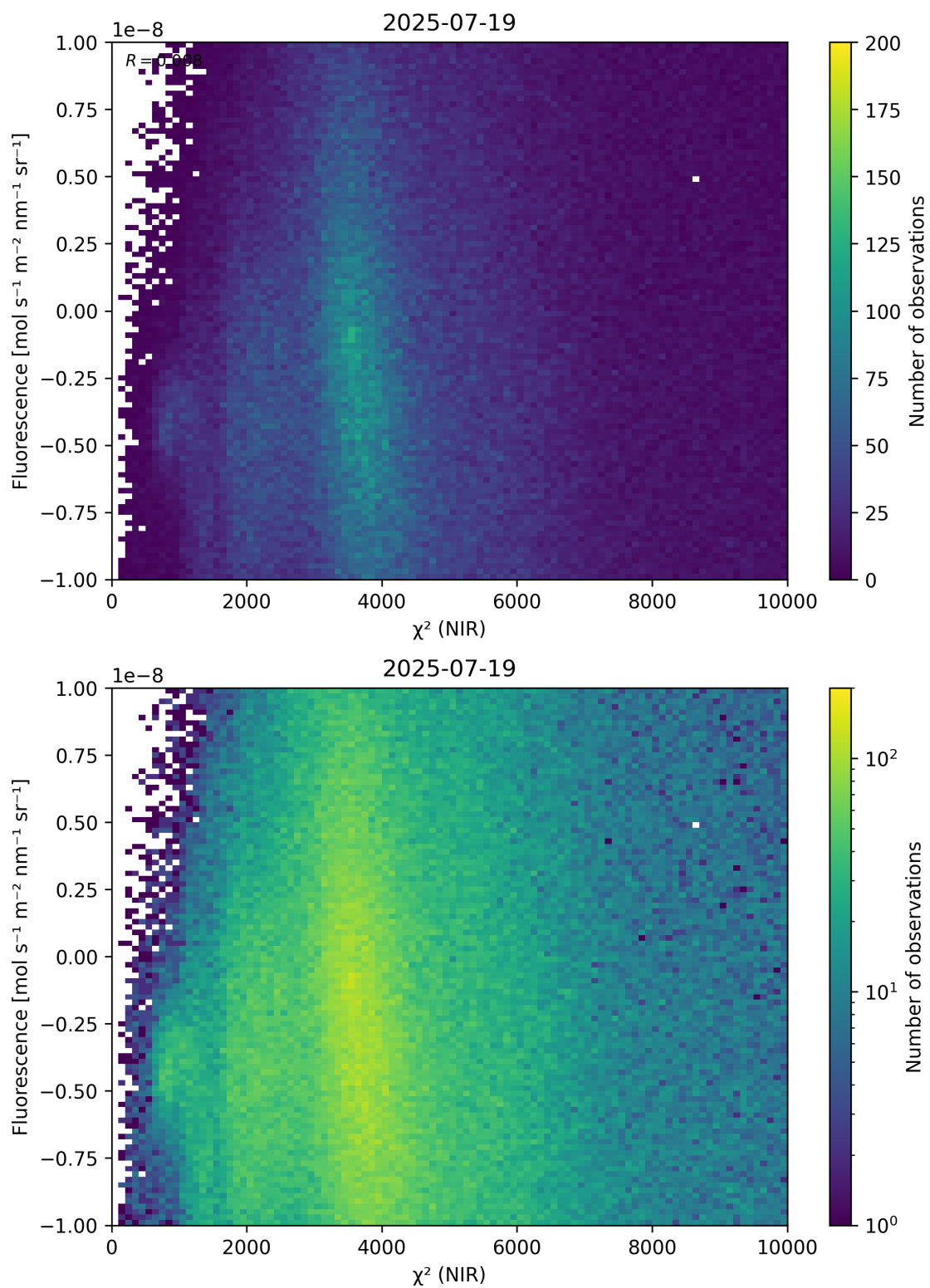
Figure 45: Scatter density plot of “ \chi^2 (NIR)” against “Fluorescence” for 2025-07-19 to 2025-07-20.
