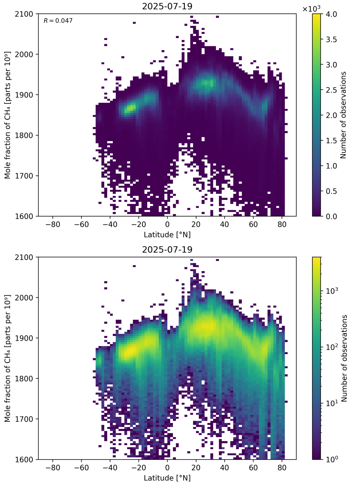
Figure 57: Scatter density plot of “Latitude” against “Mole fraction of \text{CH}_4 ” for 2025-07-19 to 2025-07-20.
