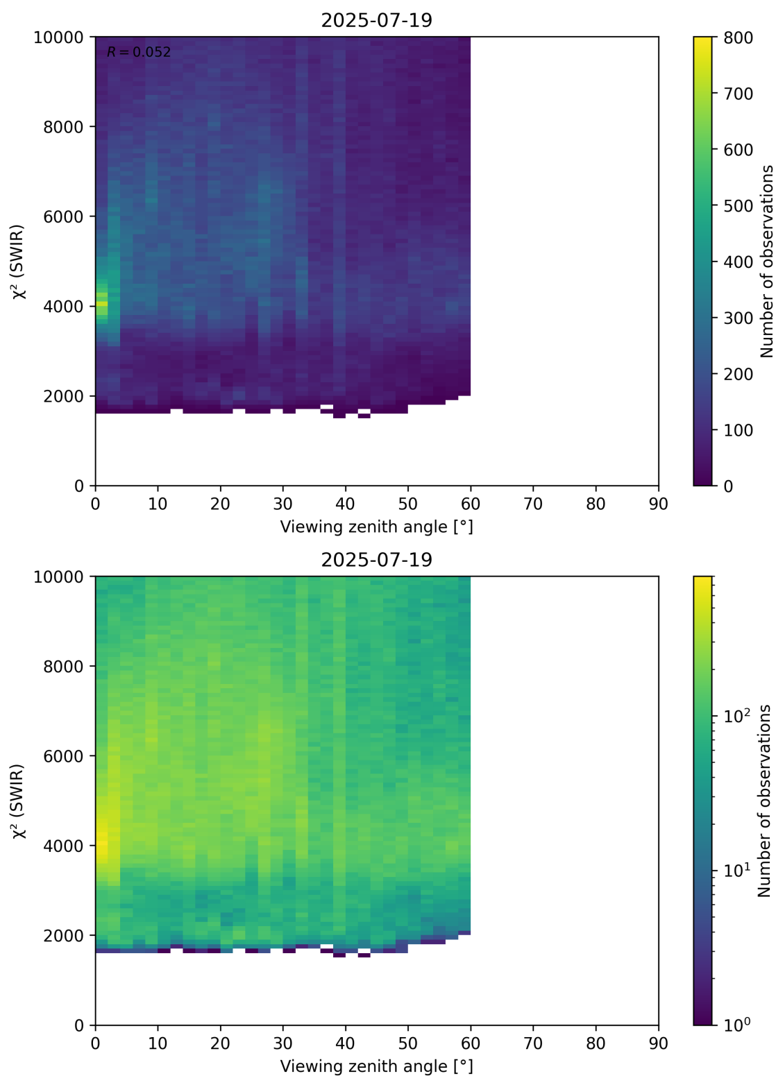
Figure 106: Scatter density plot of “Viewing zenith angle” against “ \chi^2 (SWIR)” for 2025-07-19 to 2025-07-20.
