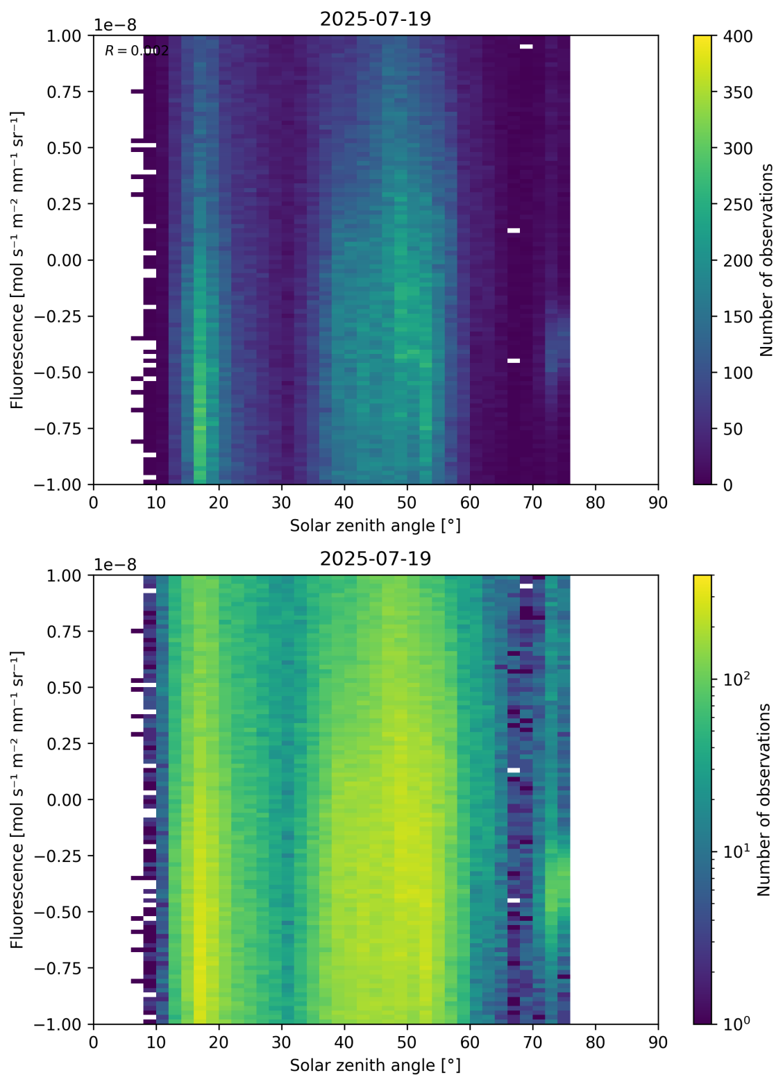
Figure 97: Scatter density plot of “Solar zenith angle” against “Fluorescence” for 2025-07-19 to 2025-07-20.
