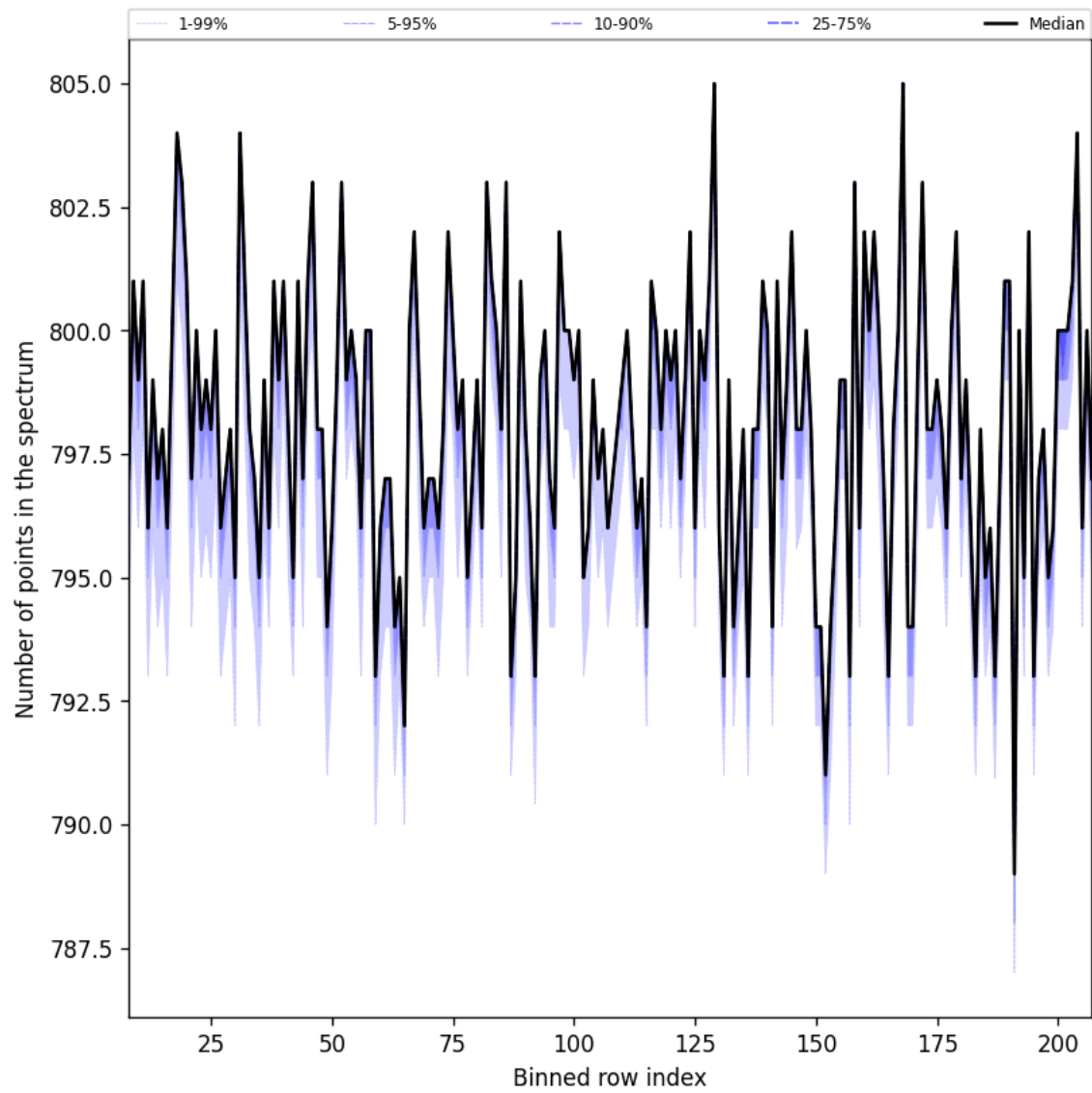
Figure 37: Along track statistics of “Number of points in the spectrum” for 2025-07-19 to 2025-07-20
