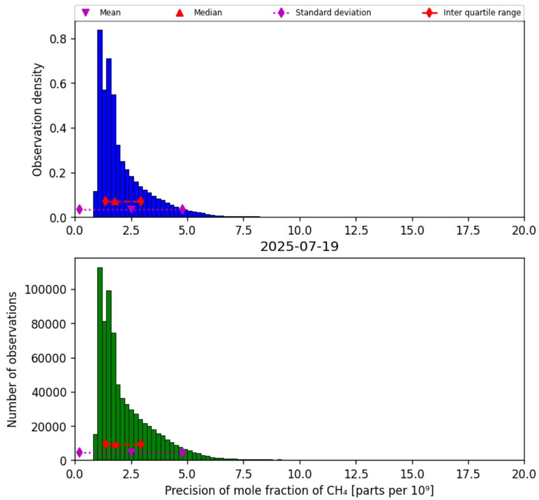
Figure 24: Histogram of “Precision of mole fraction of CH 4 ” for 2025-07-19 to 2025-07-20
