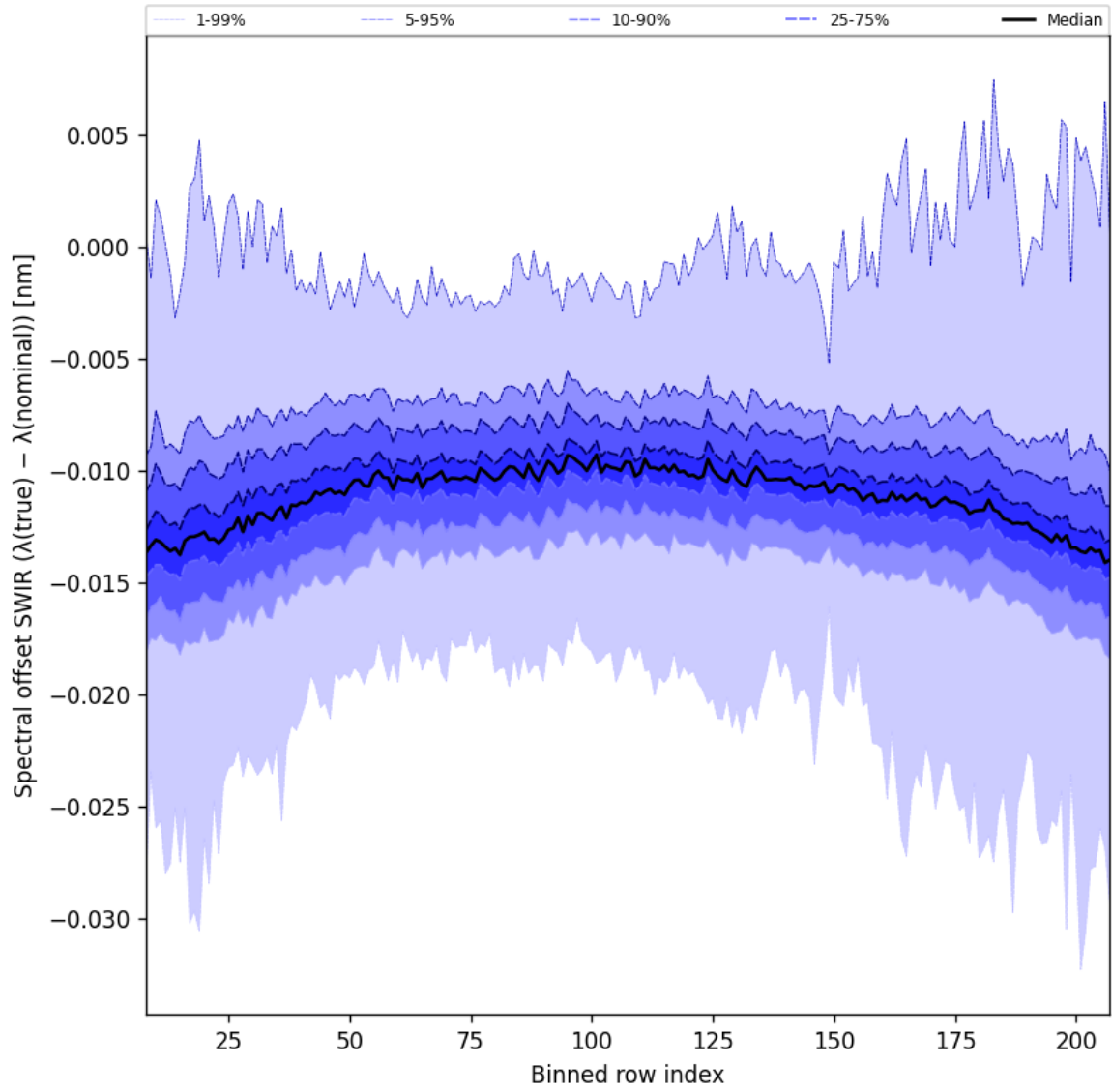
Figure 38: Along track statistics of “Spectral offset SWIR ( \lambda_{\text{true}} - \lambda_{\text{nominal}} )” for 2025-07-19 to 2025-07-20
