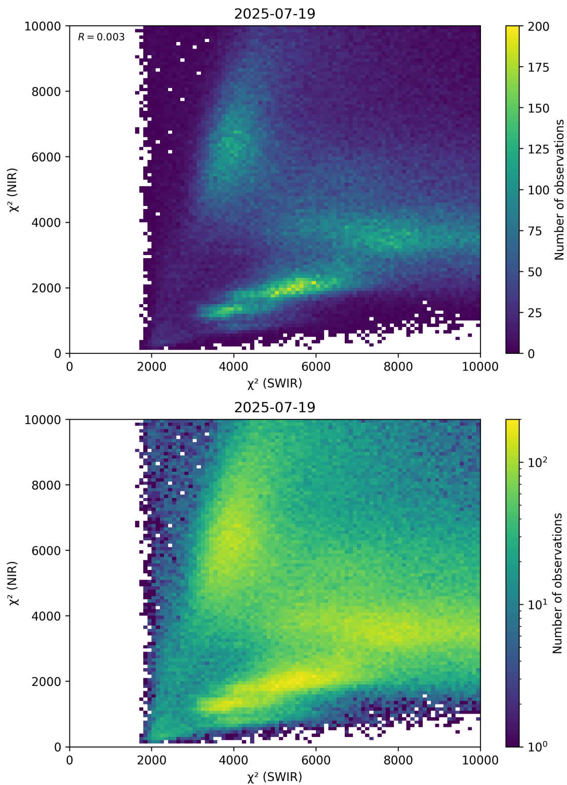
Figure 47: Scatter density plot of “ \chi^2 (SWIR)” against “ \chi^2 (NIR)” for 2025-07-19 to 2025-07-20.
