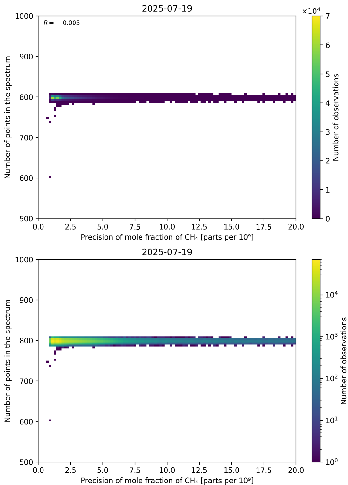
Figure 84: Scatter density plot of “Precision of mole fraction of CH 4 ” against “Number of points in the spectrum” for 2025-07-19 to 2025-07-20.
