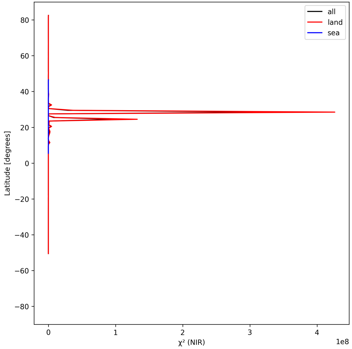
Figure 18: Zonal average of “ \chi^2 (NIR)” for 2025-07-19 to 2025-07-20.
