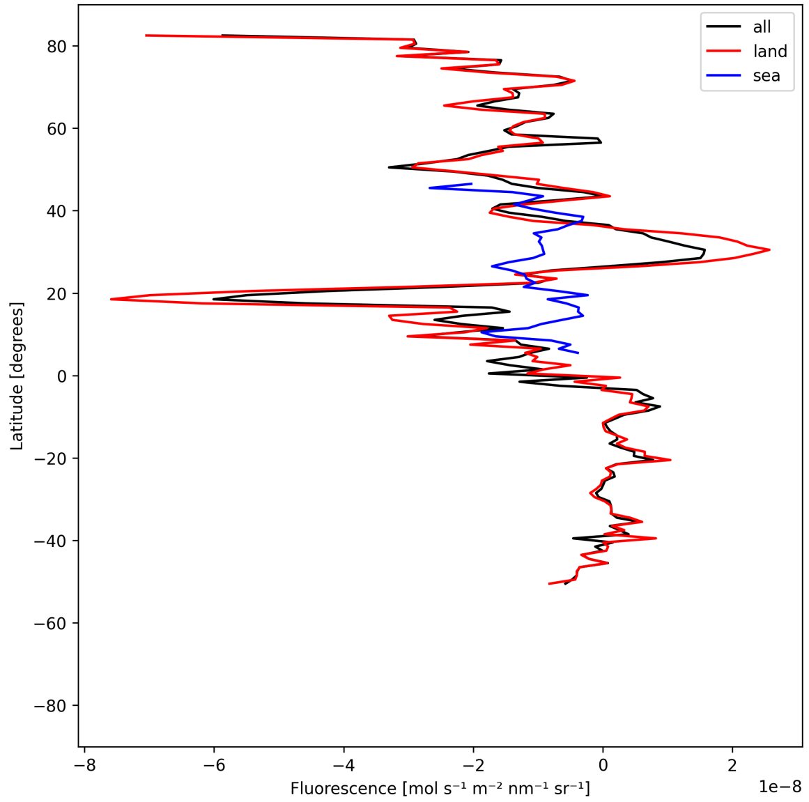
Figure 21: Zonal average of “Fluorescence” for 2025-07-19 to 2025-07-20.
