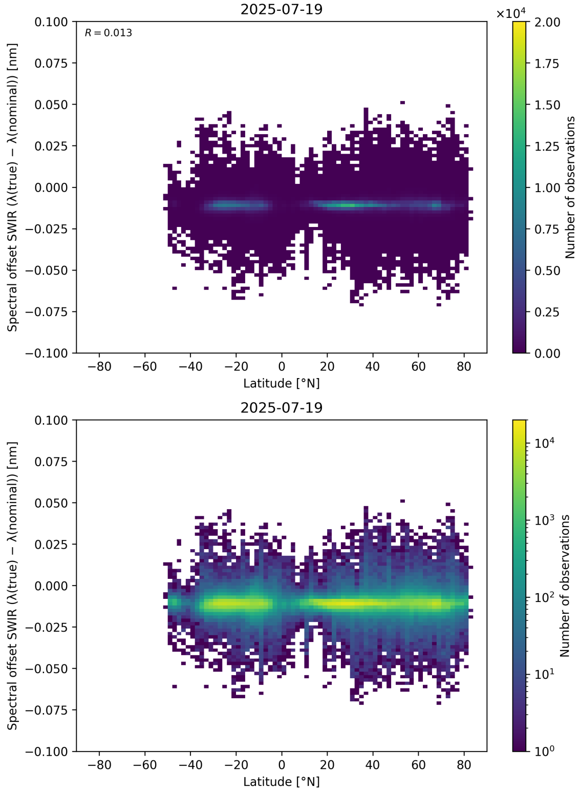
Figure 62: Scatter density plot of “Latitude” against “Spectral offset SWIR ( \lambda_{\text{true}} - \lambda_{\text{nominal}} )” for 2025-07-19 to 2025-07-20.
