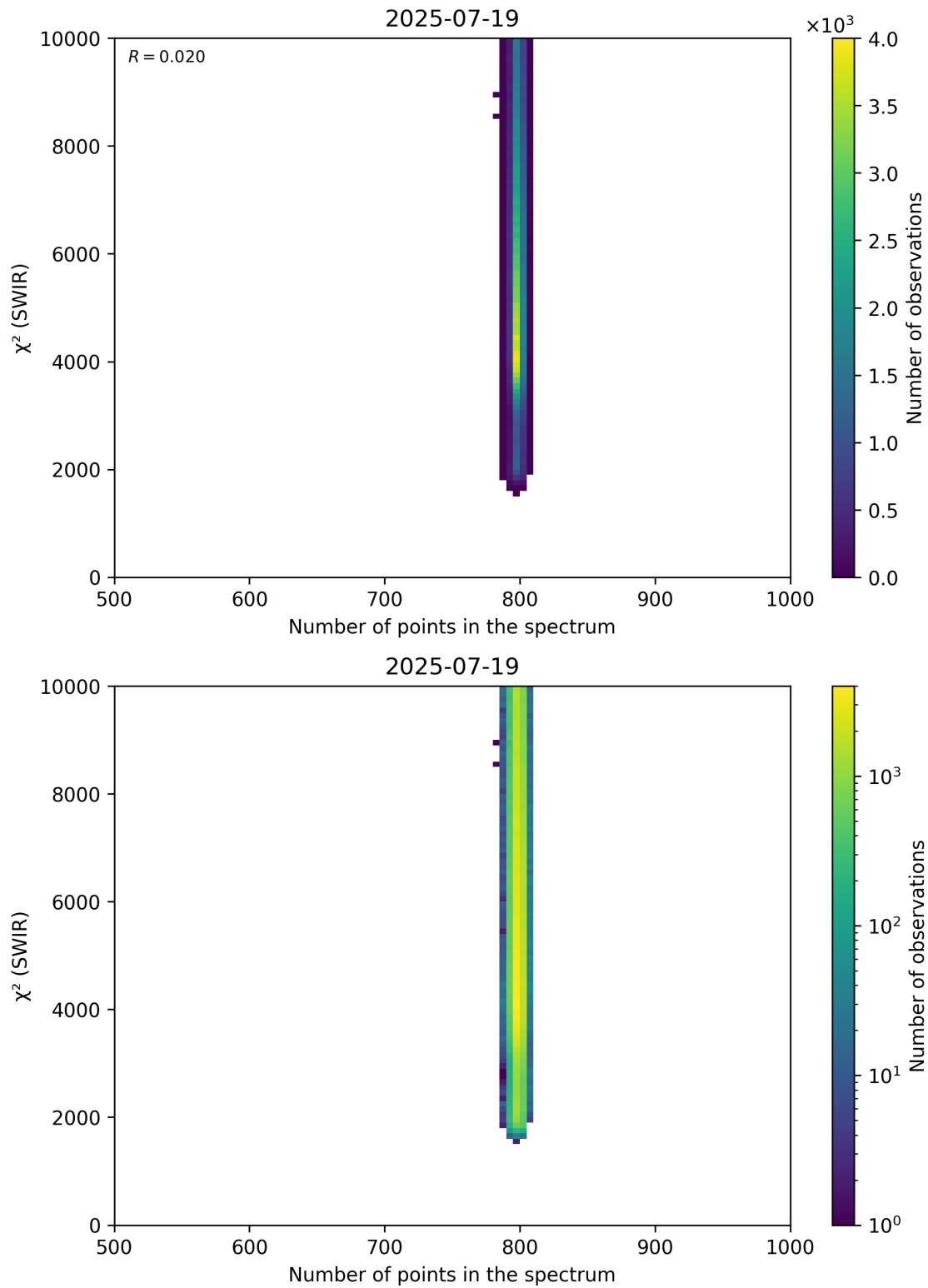
Figure 89: Scatter density plot of “Number of points in the spectrum” against “ \chi^2 (SWIR)” for 2025-07-19 to 2025-07-20.
