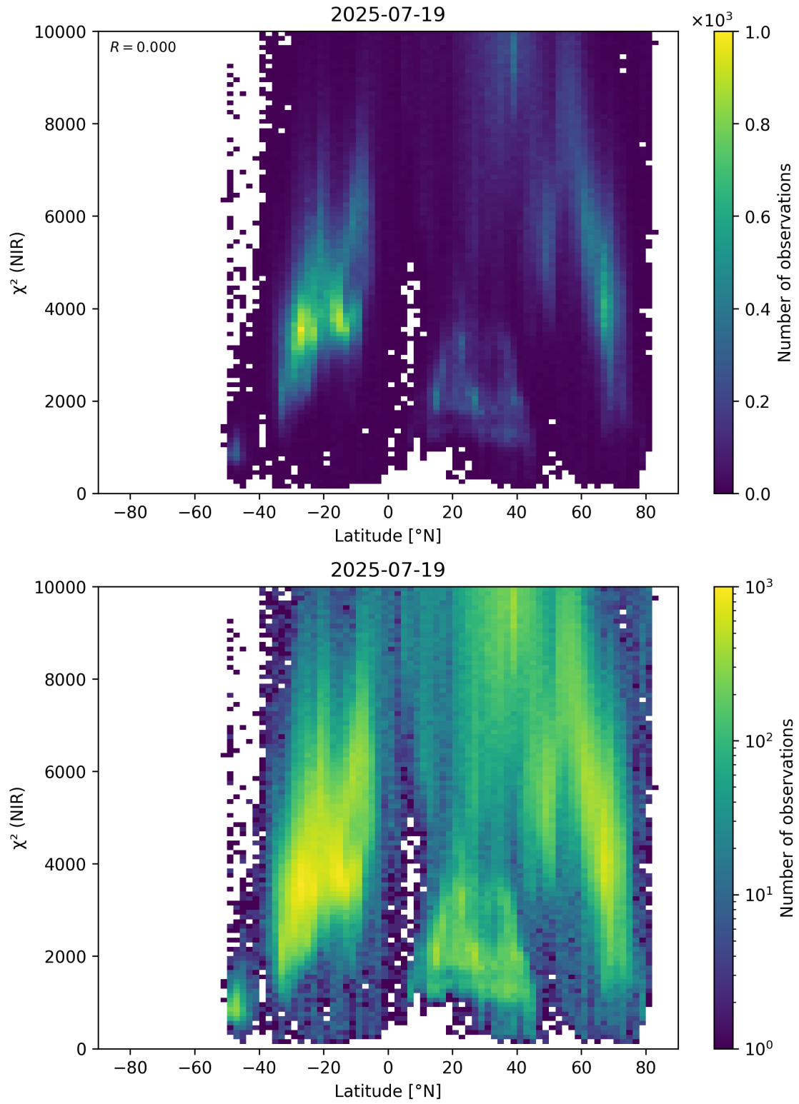
Figure 53: Scatter density plot of “Latitude” against “ \chi^2 (NIR)” for 2025-07-19 to 2025-07-20.
