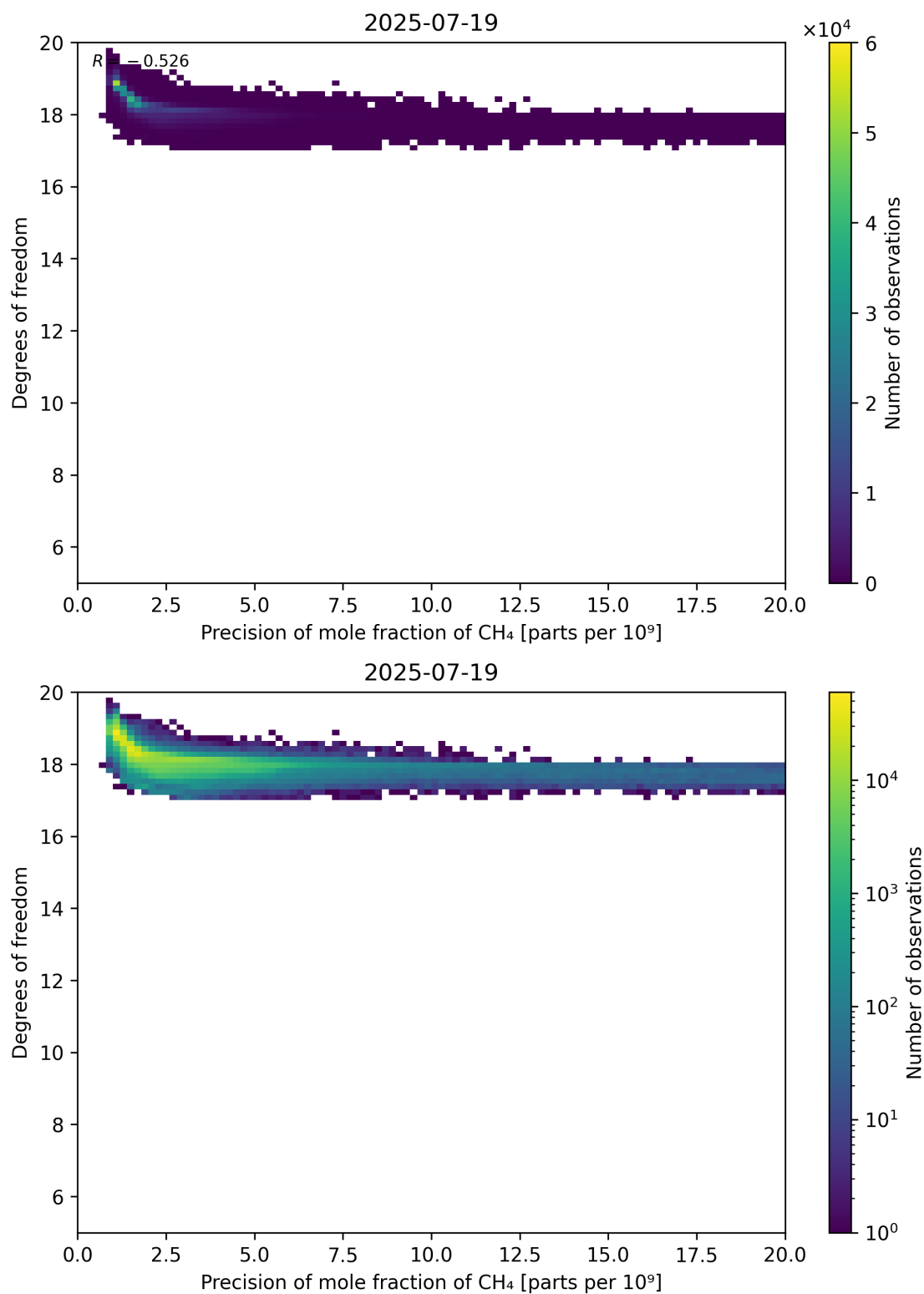
Figure 80: Scatter density plot of “Precision of mole fraction of CH 4 ” against “Degrees of freedom” for 2025-07-19 to 2025-07-20.
