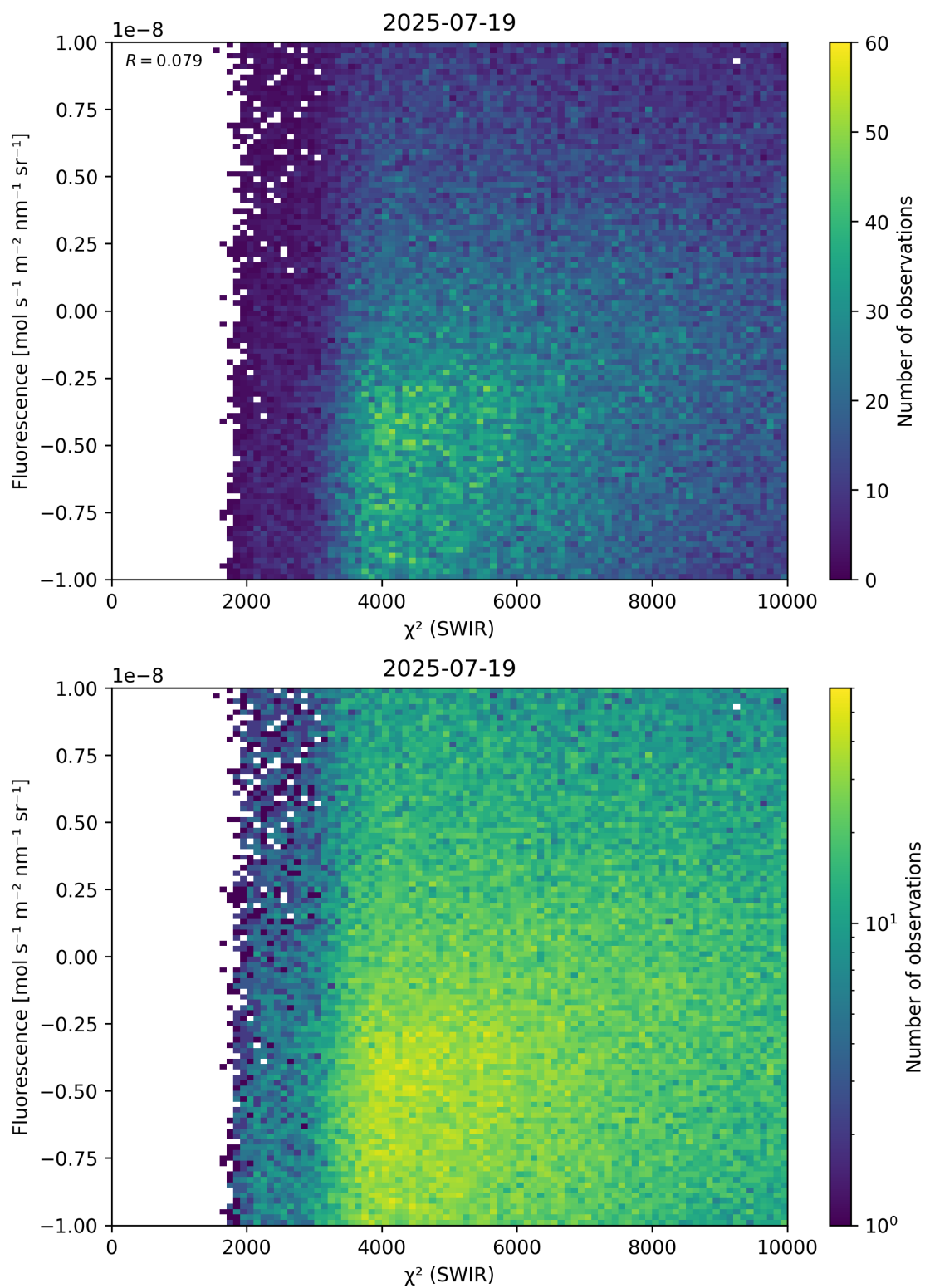
Figure 49: Scatter density plot of “ \chi^2 (SWIR)” against “Fluorescence” for 2025-07-19 to 2025-07-20.
