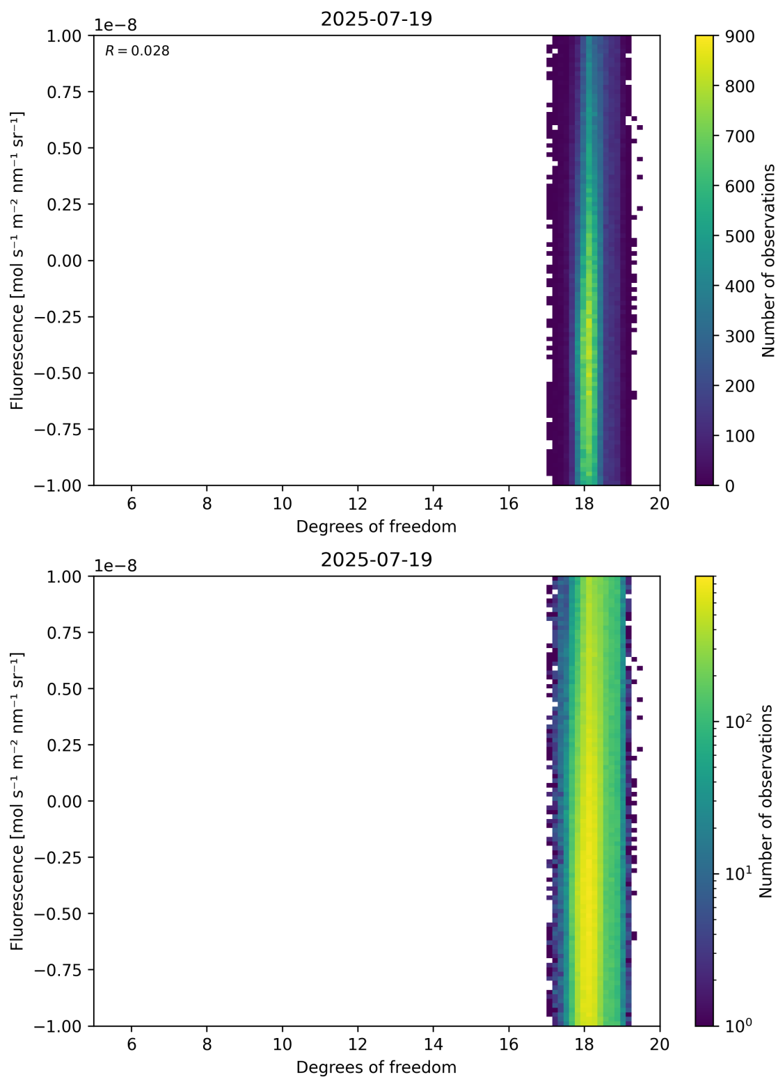
Figure 51: Scatter density plot of “Degrees of freedom” against “Fluorescence” for 2025-07-19 to 2025-07-20.
