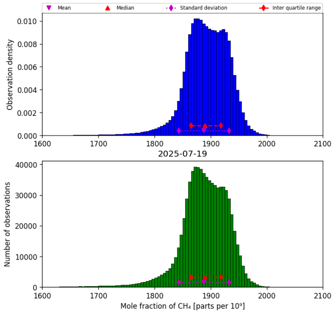
Figure 23: Histogram of “Mole fraction of CH 4 ” for 2025-07-19 to 2025-07-20
