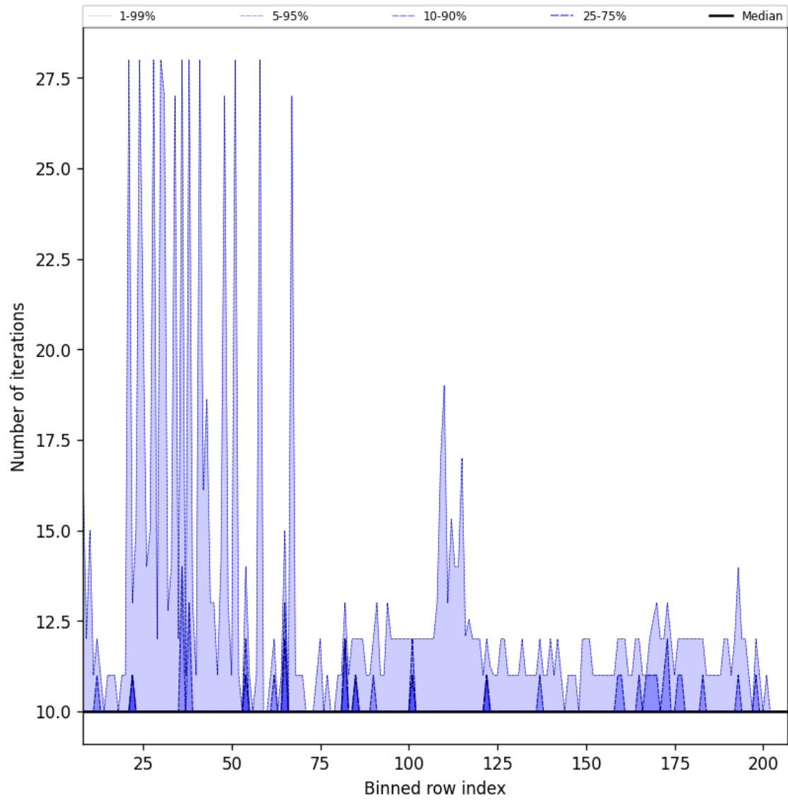
Figure 42: Along track statistics of “Number of iterations” for 2025-07-19 to 2025-07-20
