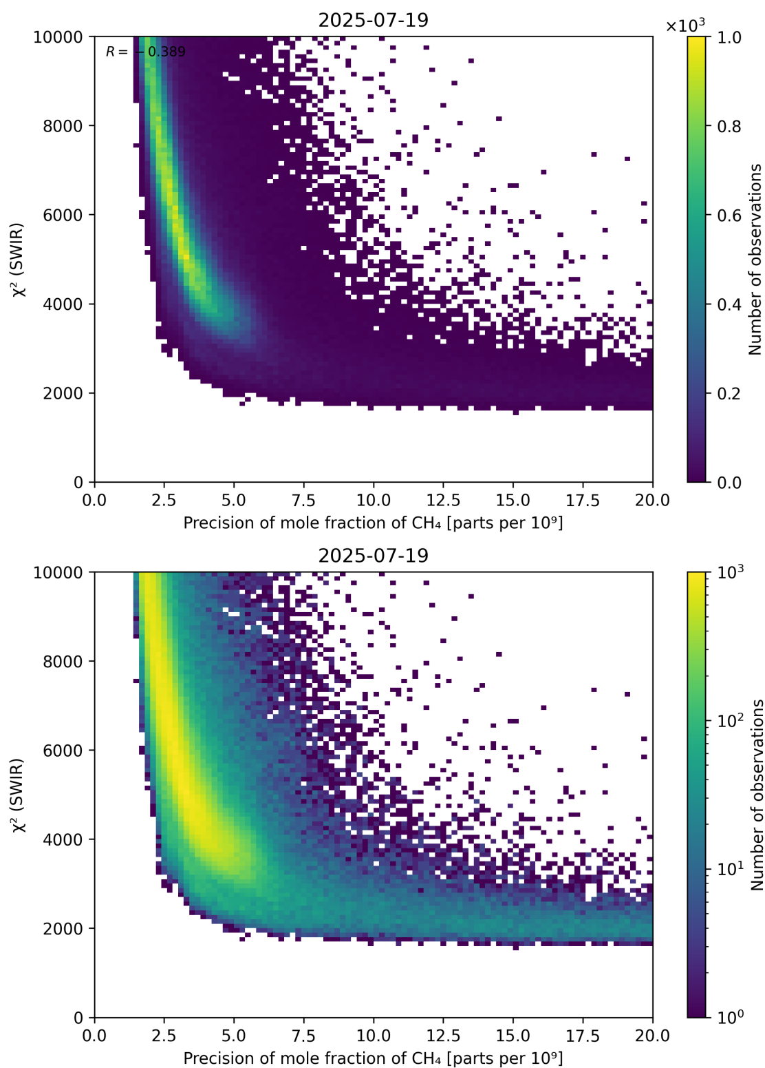
Figure 79: Scatter density plot of “Precision of mole fraction of \text{CH}_4 ” against “ \chi^2 (SWIR)” for 2025-07-19 to 2025-07-20.
